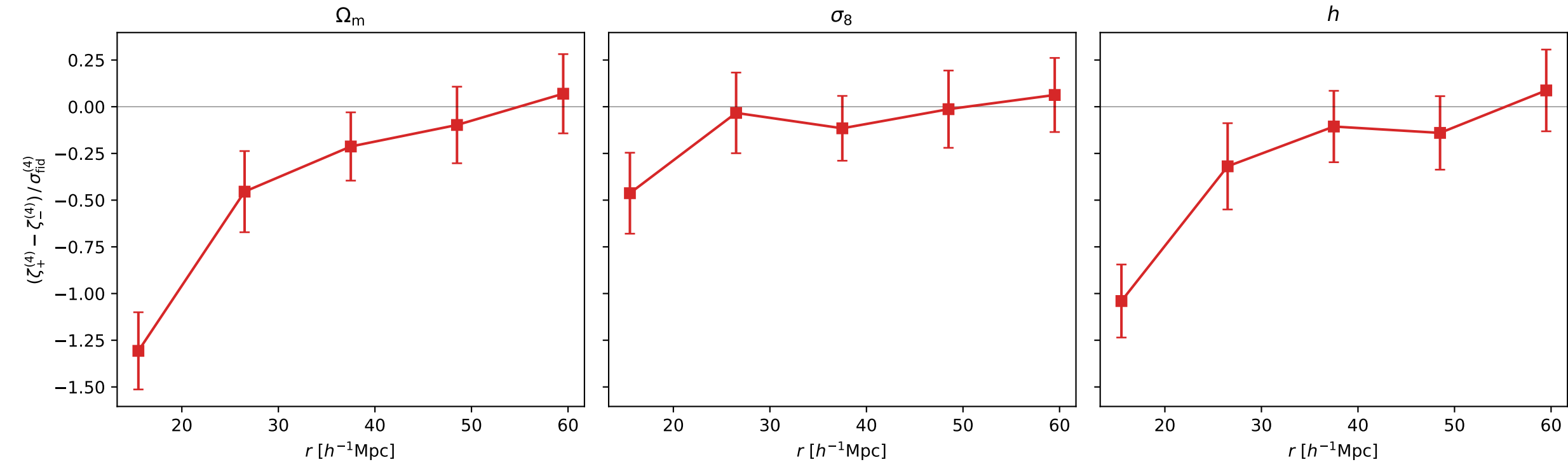
4PCF response to parameter variations (equilateral tetrahedra, 100 fiducial realizations)
