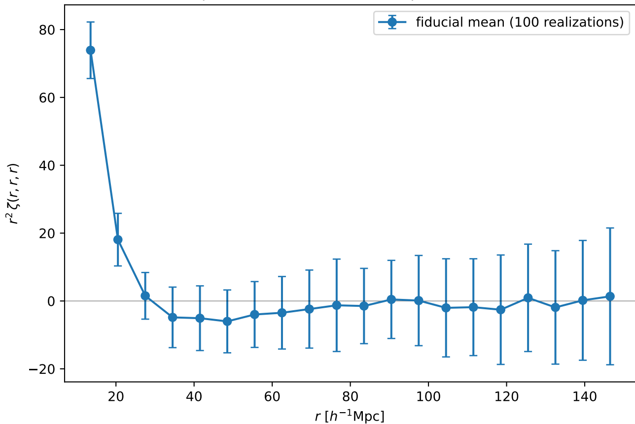
Quijote FoF halos, z=0.5 — equilateral 3PCF
