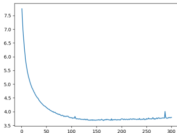
Total Loss vs. Epoch
