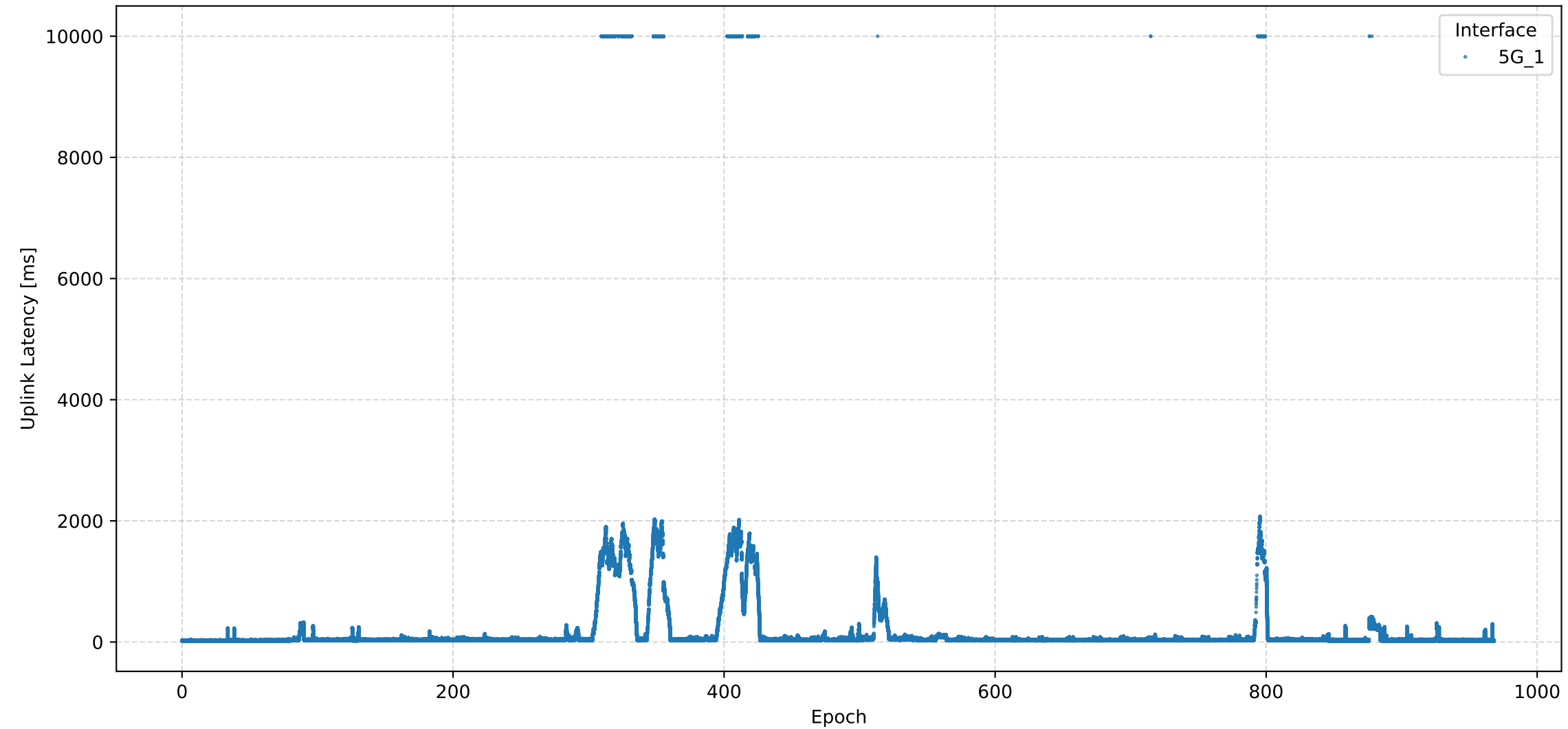
RURAL scenario for 4 mbps.
