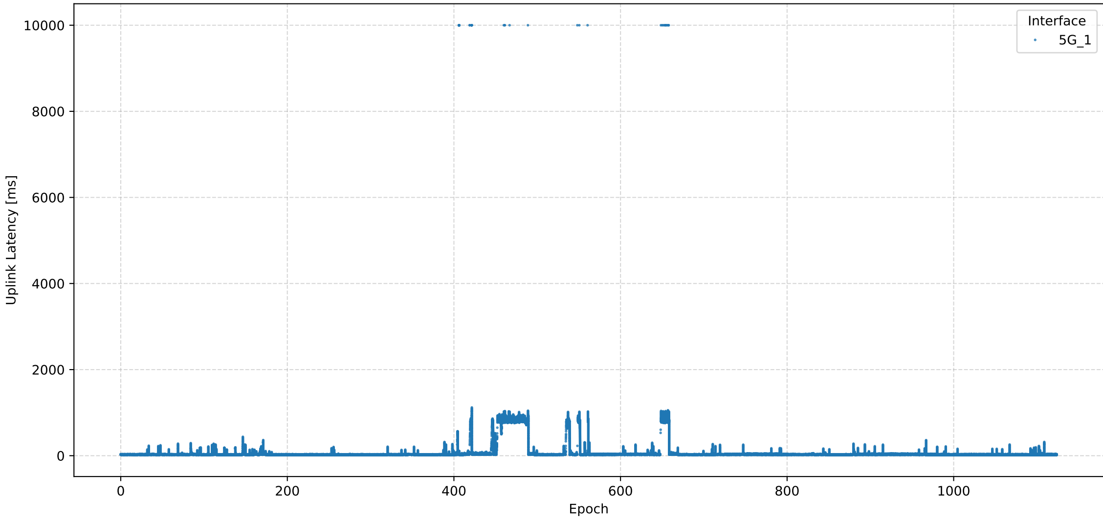
URBAN scenario for 1 mbps.
