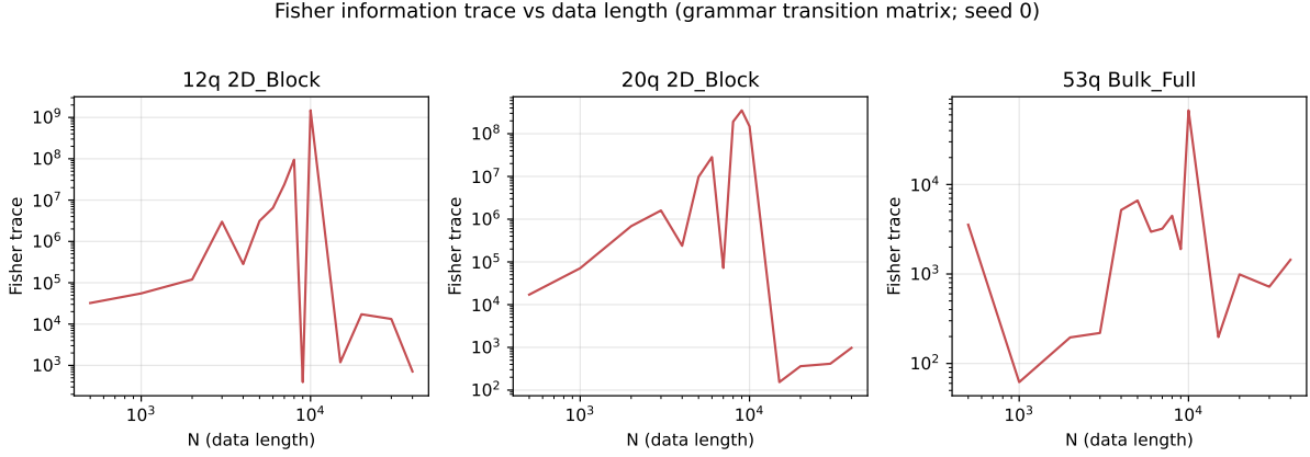
Figure 2: Fisher information trace vs. data length N for three representative readouts (seed 0). Log-log axes.
