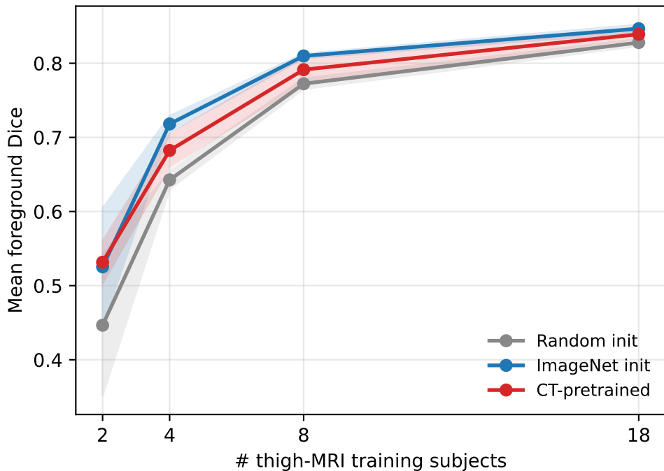
Encoder pretraining source
