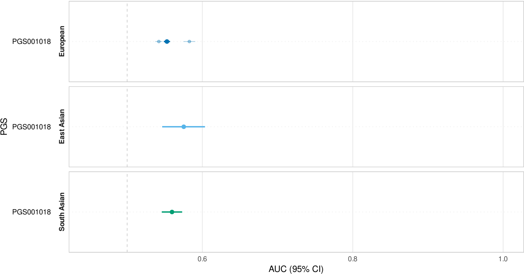
Raw and Stage-1 pooled AUC — Leisure/social activities (attend any of the followings in once a week or more often: Transparent: raw cohort evaluations; Solid: Stage-1 pooled (Matched)
