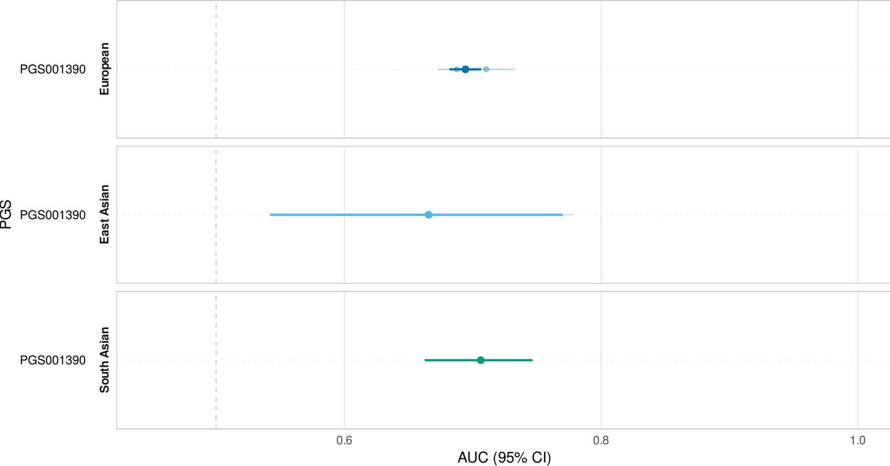
Raw and Stage-1 pooled AUC — TTE duodenal ulcer Transparent: raw cohort evaluations; Solid: Stage-1 pooled (Matched)
