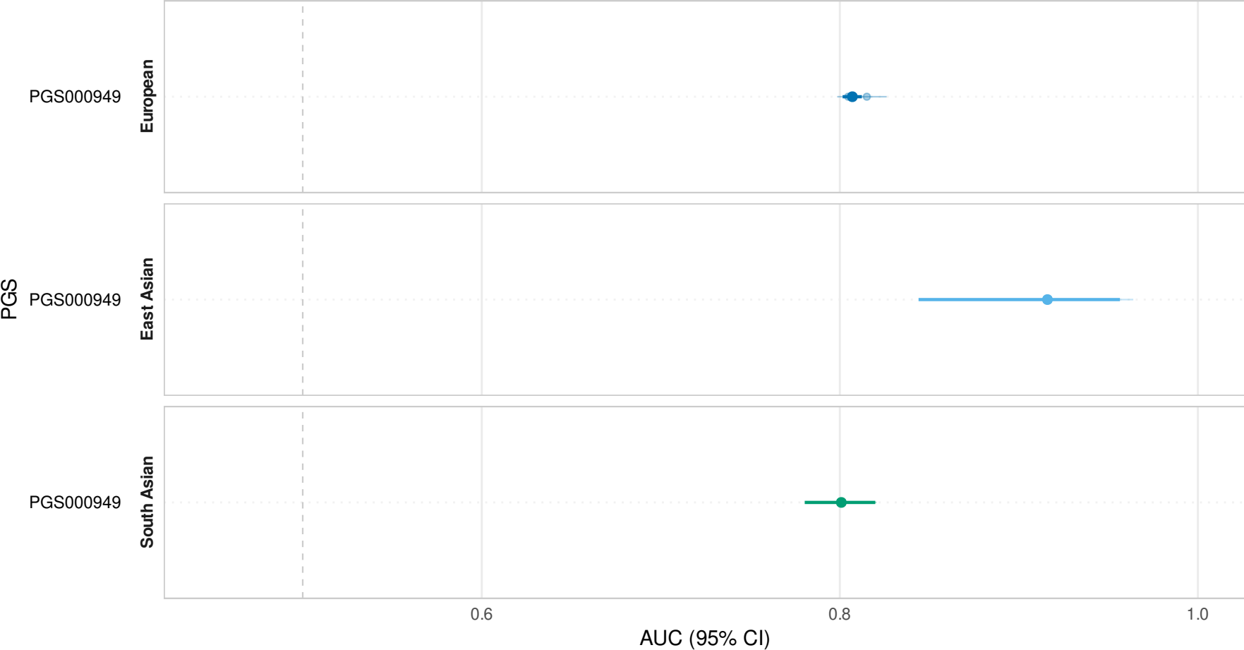
Raw and Stage-1 pooled AUC — TTE inguinal hernia Transparent: raw cohort evaluations; Solid: Stage-1 pooled (Matched)
