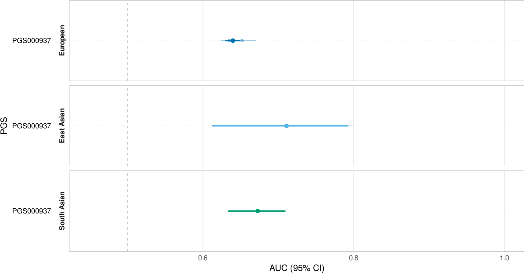
Raw and Stage-1 pooled AUC — Varicose veins Transparent: raw cohort evaluations; Solid: Stage-1 pooled (Matched)
