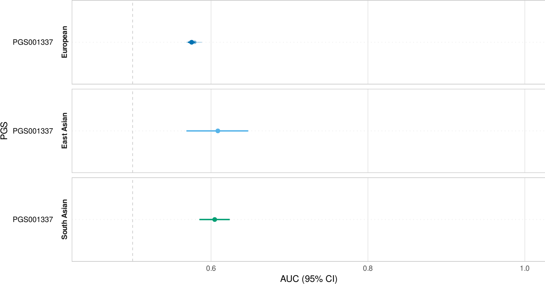
Raw and Stage-1 pooled AUC — Breast cancer (FH) Transparent: raw cohort evaluations; Solid: Stage-1 pooled (Matched)
