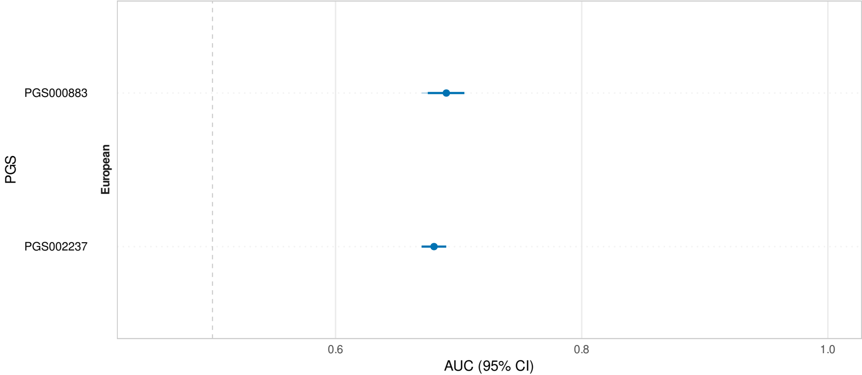
Raw and Stage-1 pooled AUC — Chronic kidney disease (eGFR <60 ml/min per 1.73 m2 or UACR >3.0 mg/mmol) Transparent: raw cohort evaluations; Solid: Stage-1 pooled (Matched)
