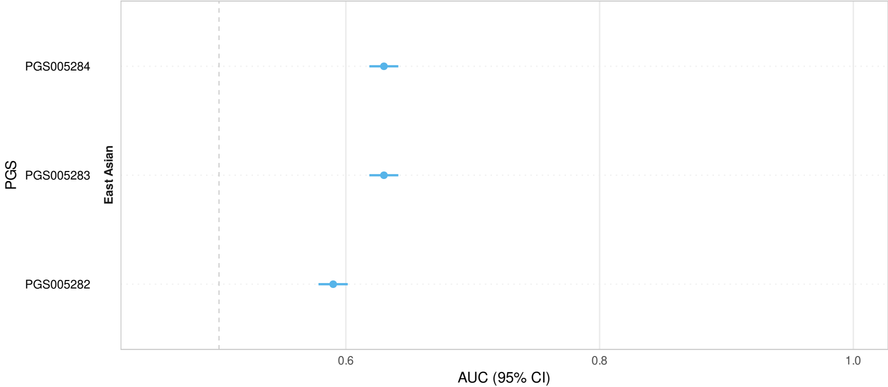
Raw and Stage-1 pooled AUC — IgA nephropathy Transparent: raw cohort evaluations; Solid: Stage-1 pooled (Matched)
