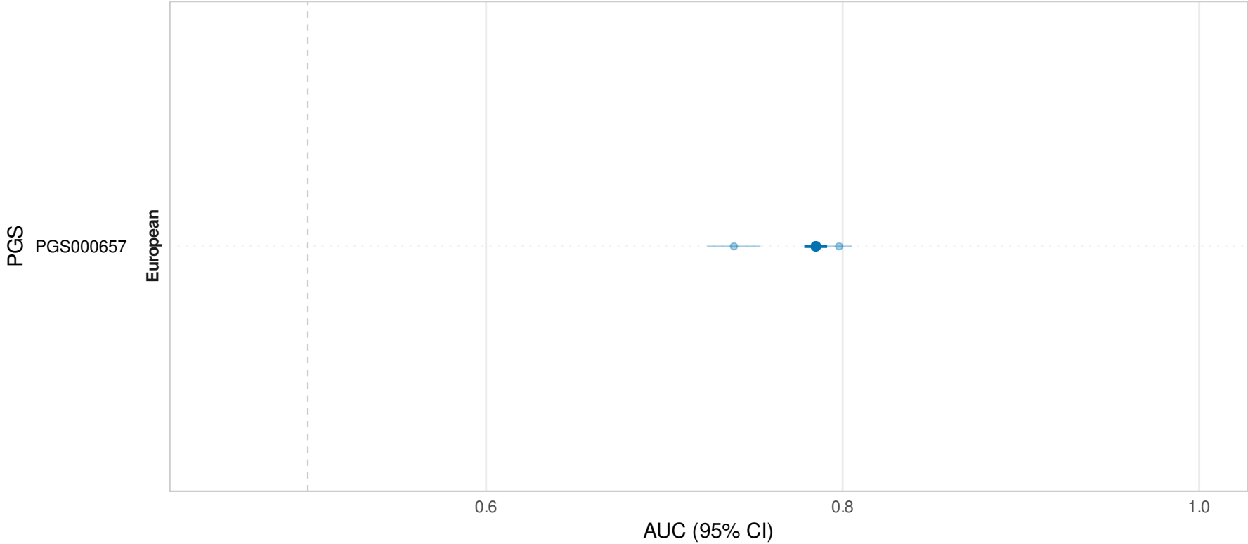
Raw and Stage-1 pooled AUC — Incident hip fracture Transparent: raw cohort evaluations; Solid: Stage-1 pooled (Matched)
