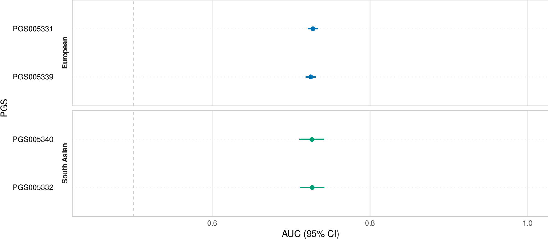
Raw and Stage-1 pooled AUC — Obesity (BMI≥30) Transparent: raw cohort evaluations; Solid: Stage-1 pooled (Matched)
