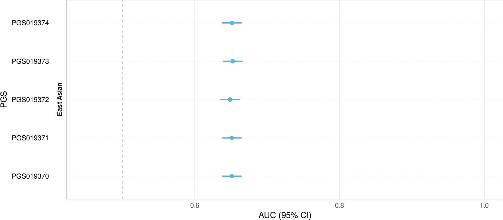
Raw and Stage-1 pooled AUC — Other disorders of liver Transparent: raw cohort evaluations; Solid: Stage-1 pooled (Matched)
