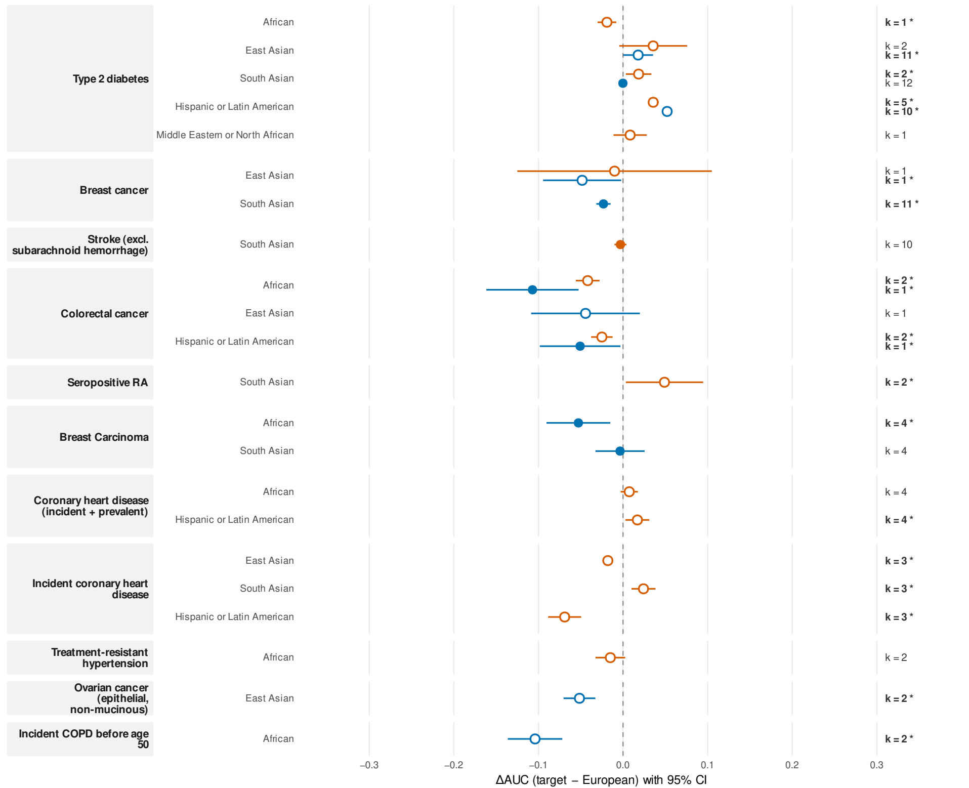
Figure 1C cells in the recovery-pack layout: within-PGS \Delta AUC (target – European)
