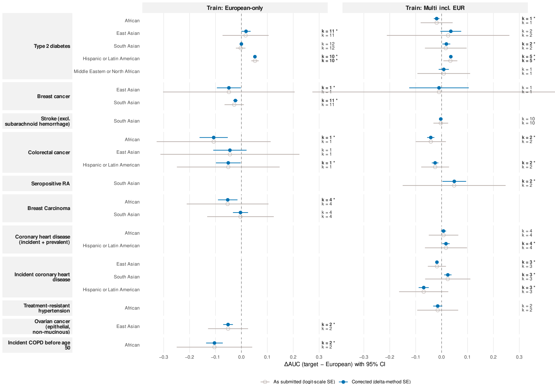
Figure 1C before and after putting Stage-2 standard errors on the AUC scale
