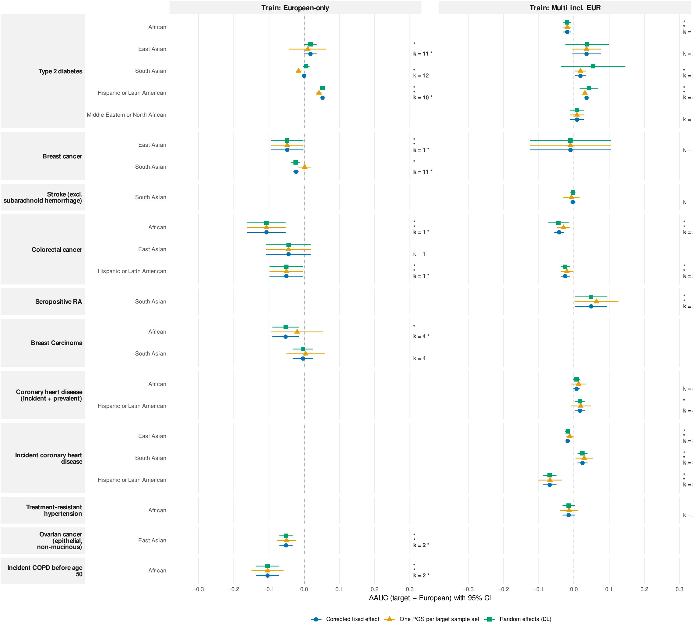
Dependence sensitivities on the delta-method \Delta AUC Significant cells: 19 fixed / 16 one-per-sample-set / 18 random effects; 14 significant in all three.
