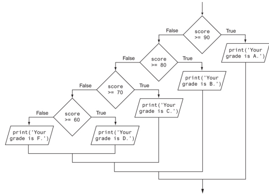
Figure 7: Multi-way decision structure to determine a grade (Gaddis, 2021, pg.16)
