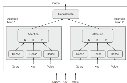
Figure 7: The Keras MultiHeadAttention layer. (Chollet, 2021 , pg.344)
