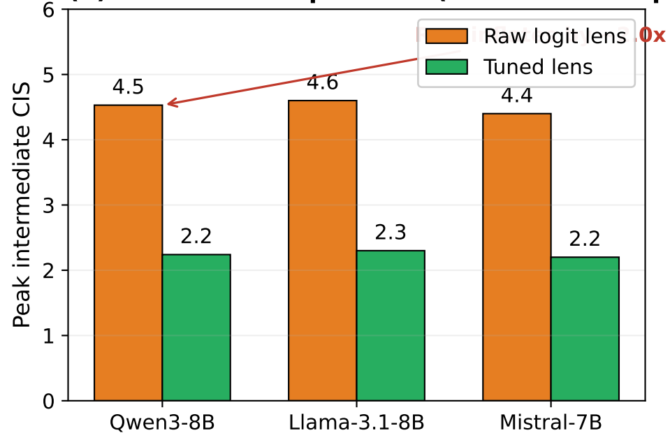
(b) Raw vs tuned peak CIS (incorrect examples)
