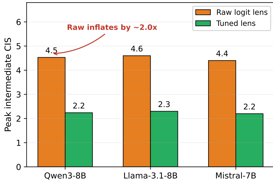
(b) Raw vs tuned peak CIS (incorrect examples)
