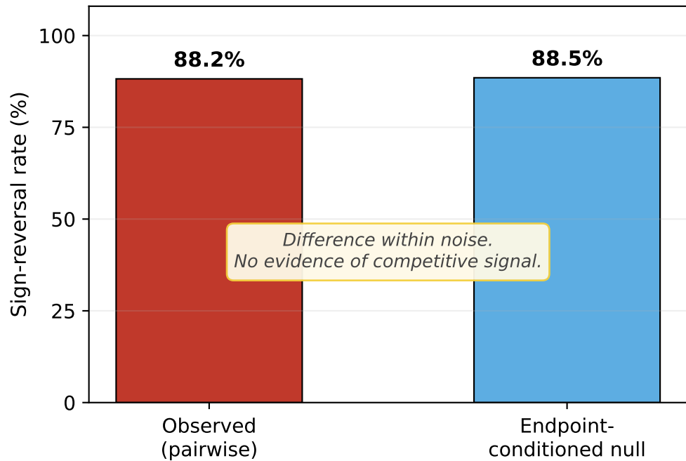
(a) Pairwise sign reversal
