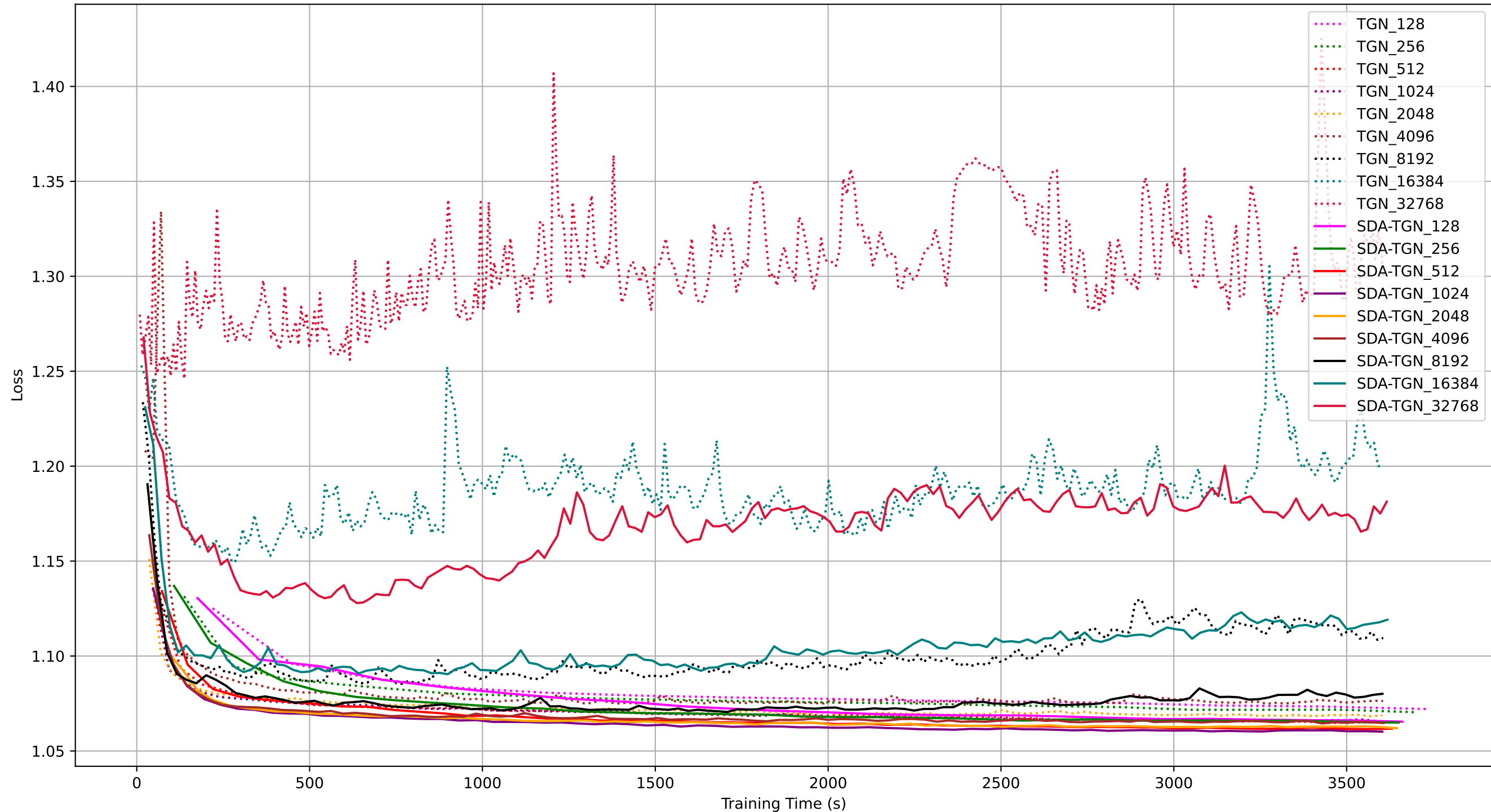
Training Loss vs. Training Time
