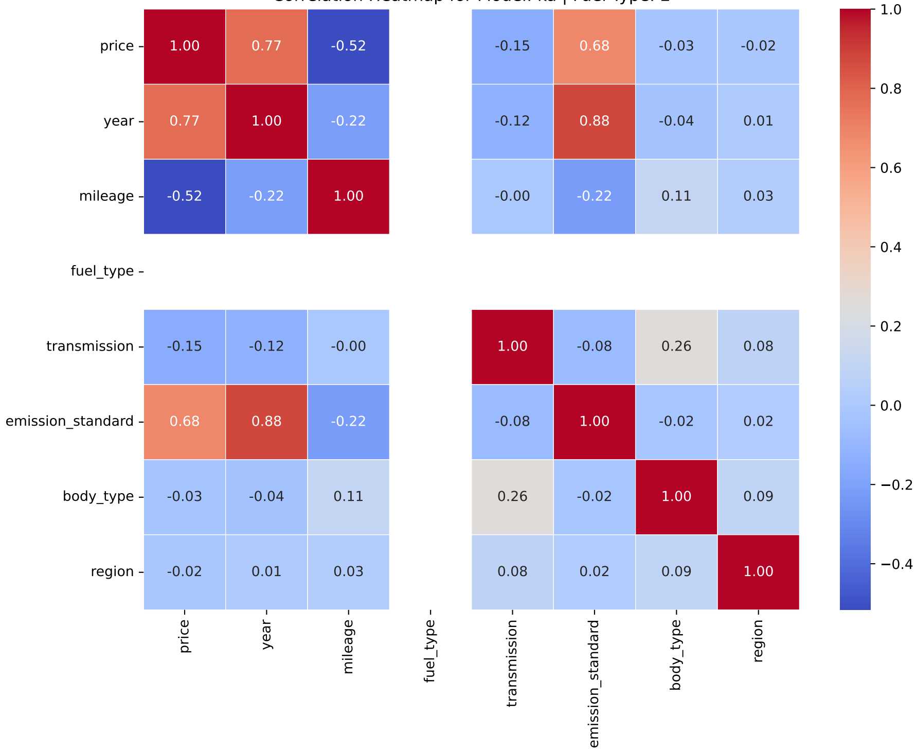
Correlation Heatmap for Model: ka | Fuel Type: 2
