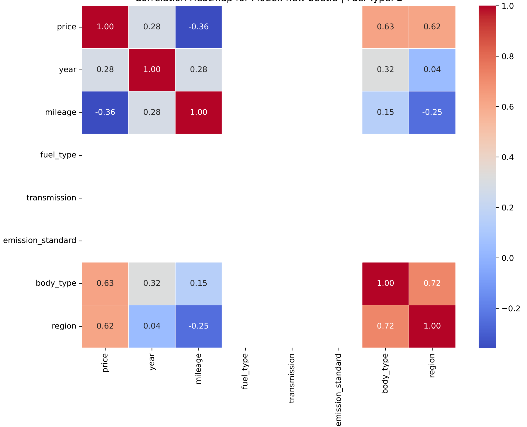
Correlation Heatmap for Model: new beetle | Fuel Type: 2
