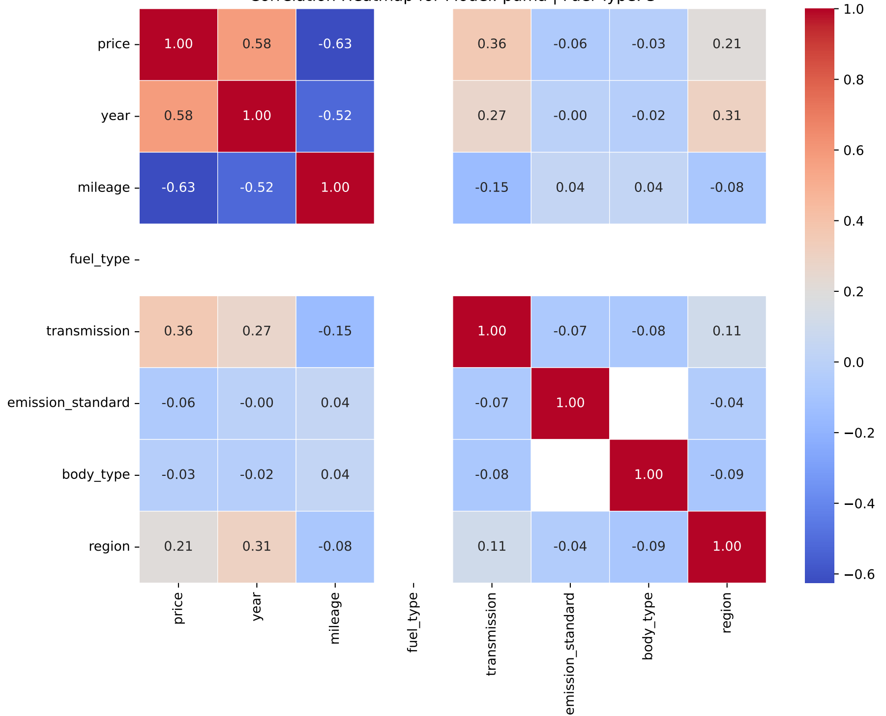
Correlation Heatmap for Model: puma | Fuel Type: 3
