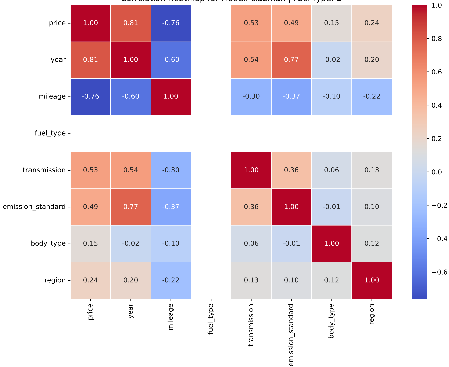
Correlation Heatmap for Model: clubman | Fuel Type: 1
