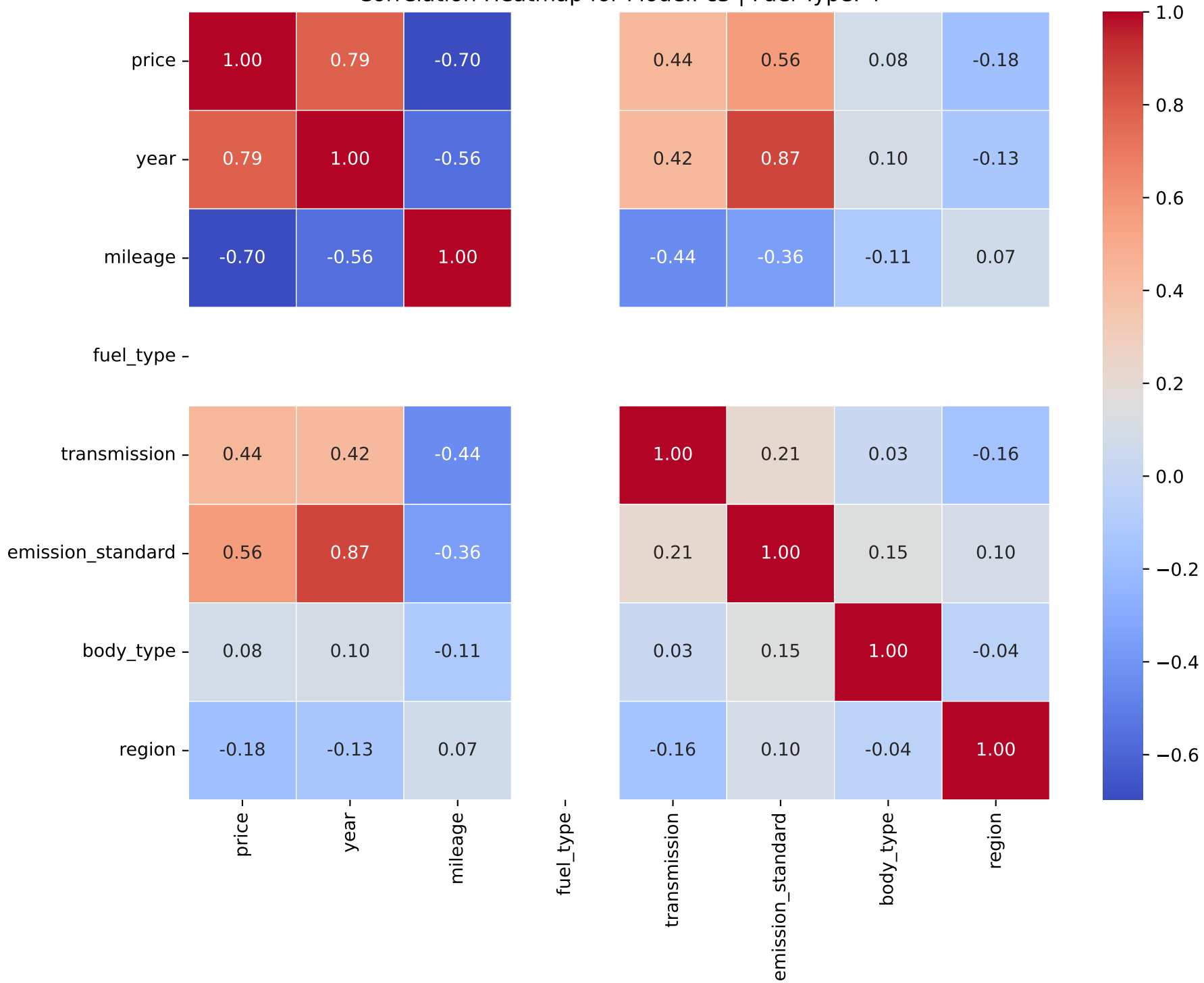
Correlation Heatmap for Model: c3 | Fuel Type: 4
