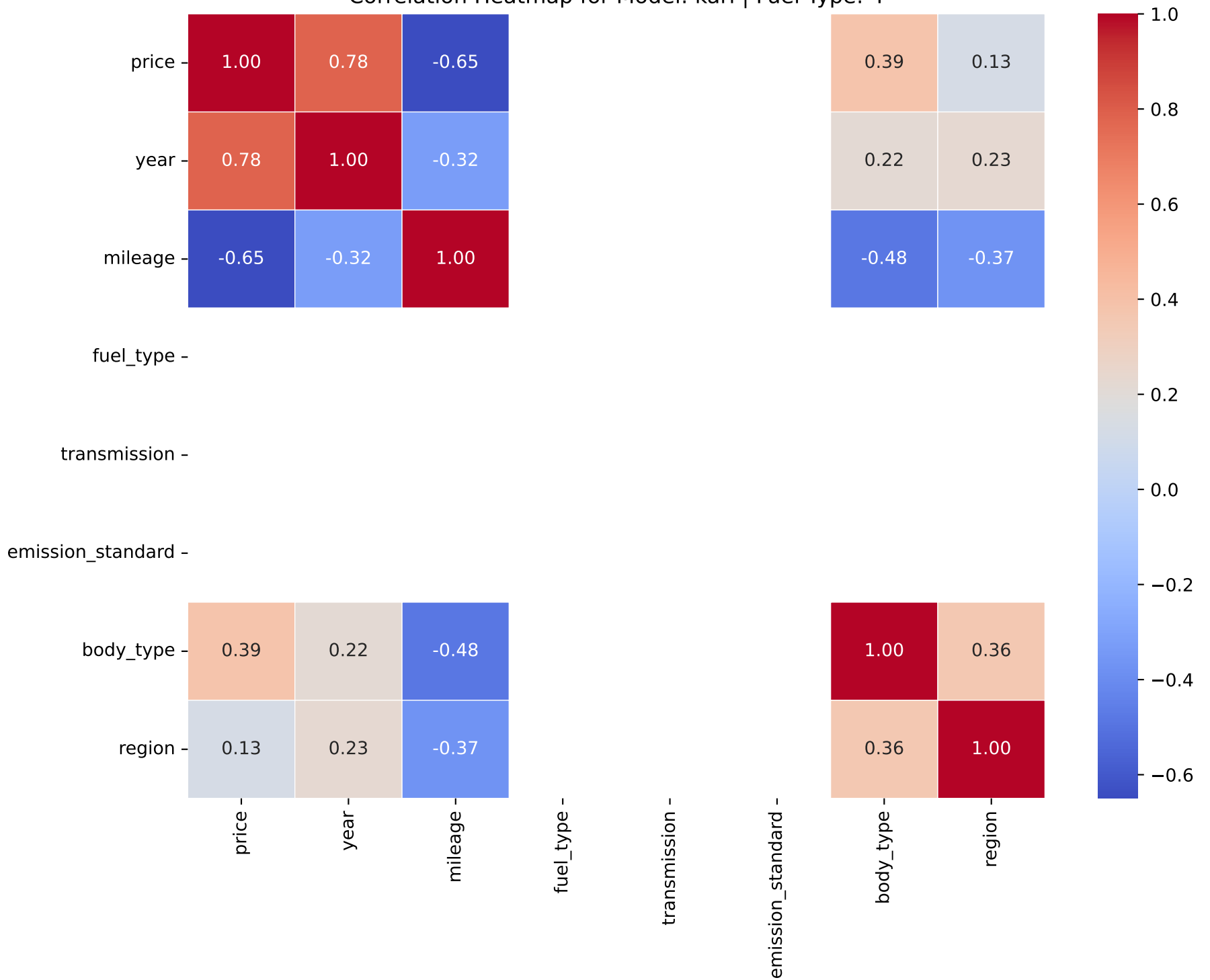
Correlation Heatmap for Model: karl | Fuel Type: 4
