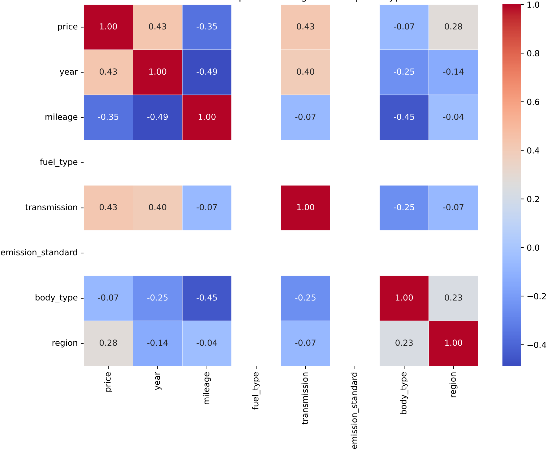
Correlation Heatmap for Model: grandland | Fuel Type: 2
