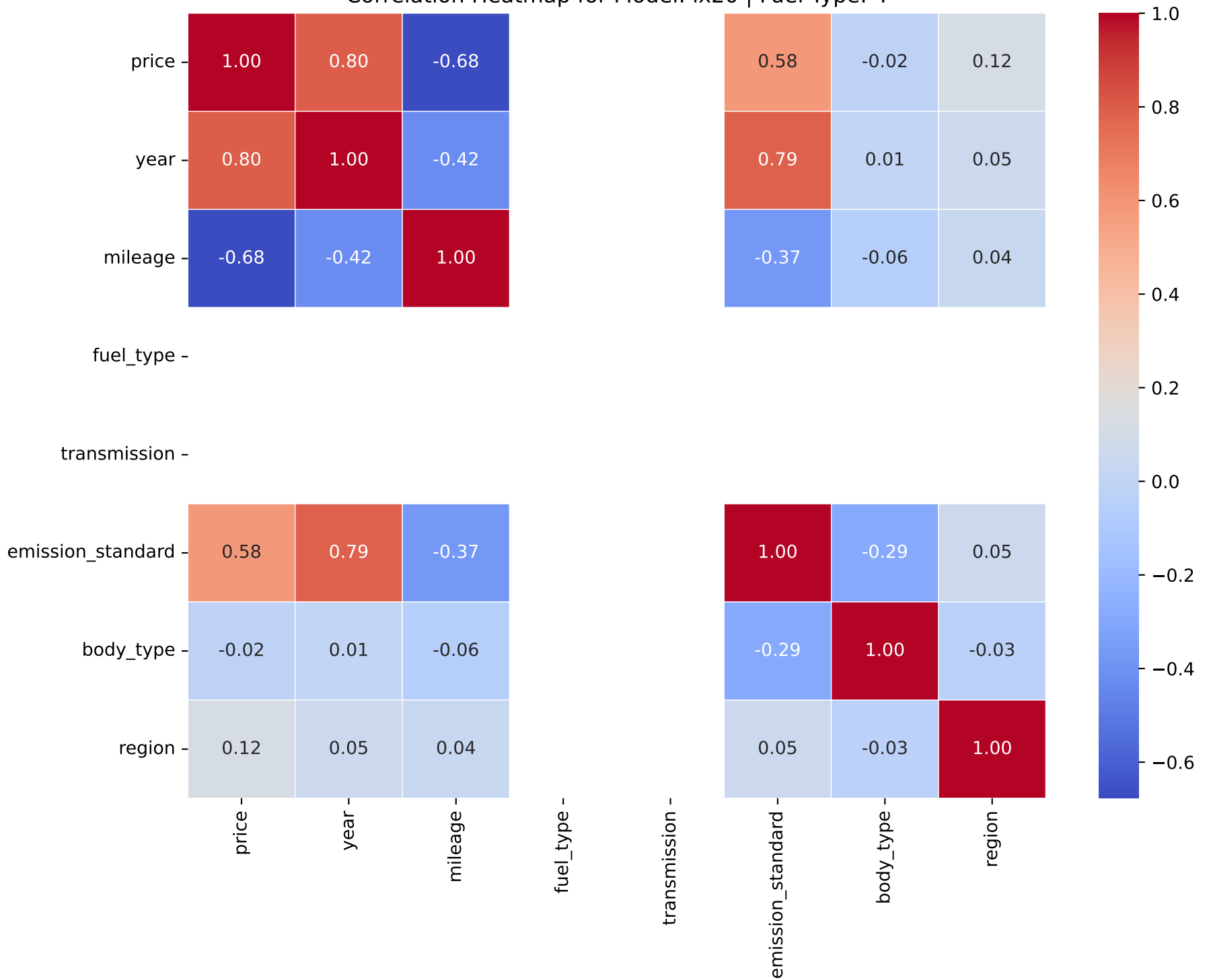
Correlation Heatmap for Model: ix20 | Fuel Type: 4
