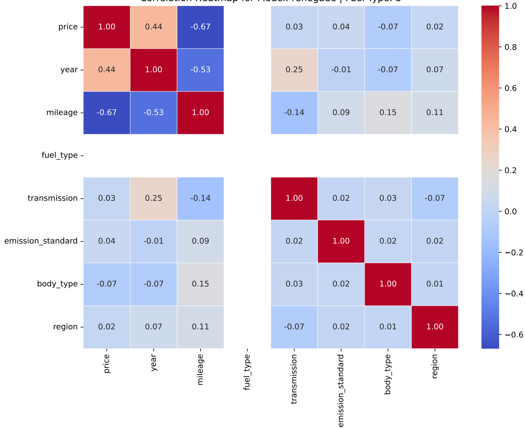
Correlation Heatmap for Model: renegade | Fuel Type: 3
