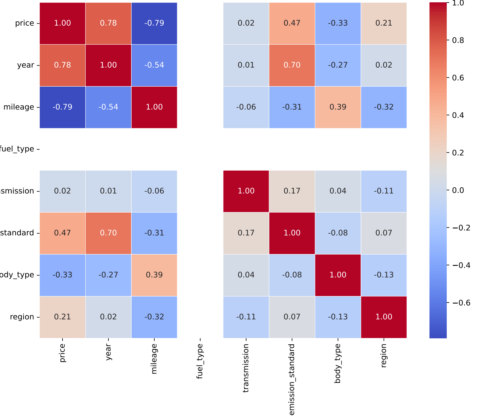
Correlation Heatmap for Model: adam | Fuel Type: 2
