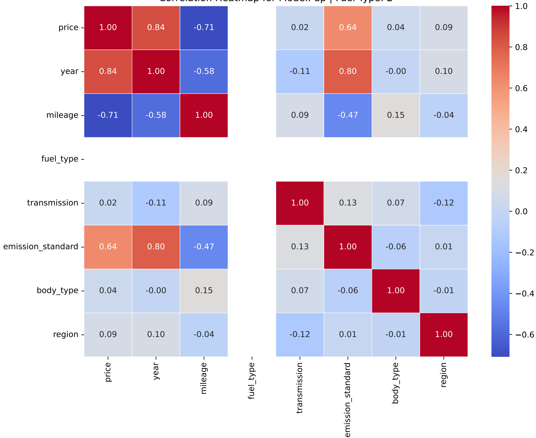
Correlation Heatmap for Model: up | Fuel Type: 2
