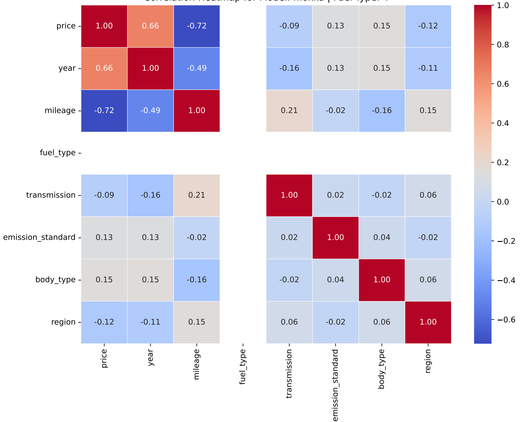
Correlation Heatmap for Model: mokka | Fuel Type: 4
