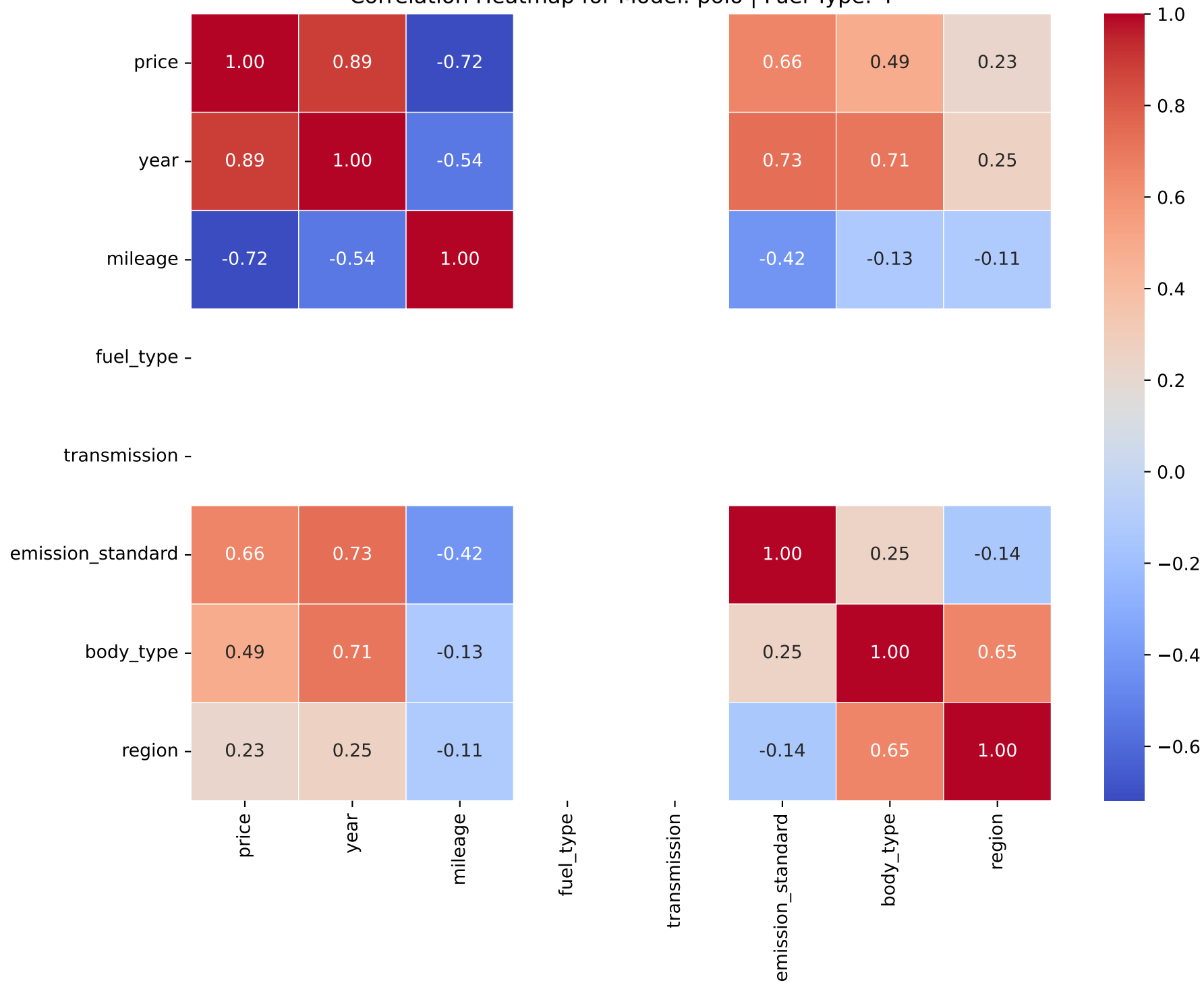
Correlation Heatmap for Model: polo | Fuel Type: 4
