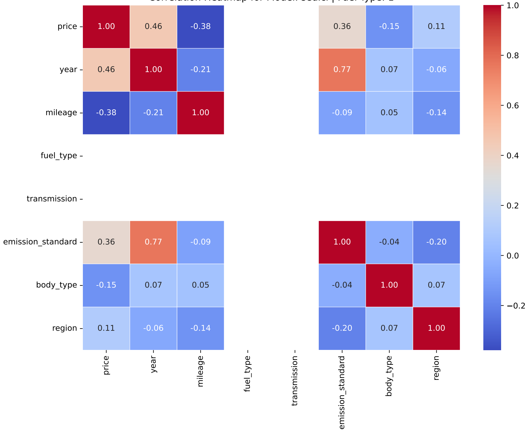
Correlation Heatmap for Model: sedici | Fuel Type: 1
