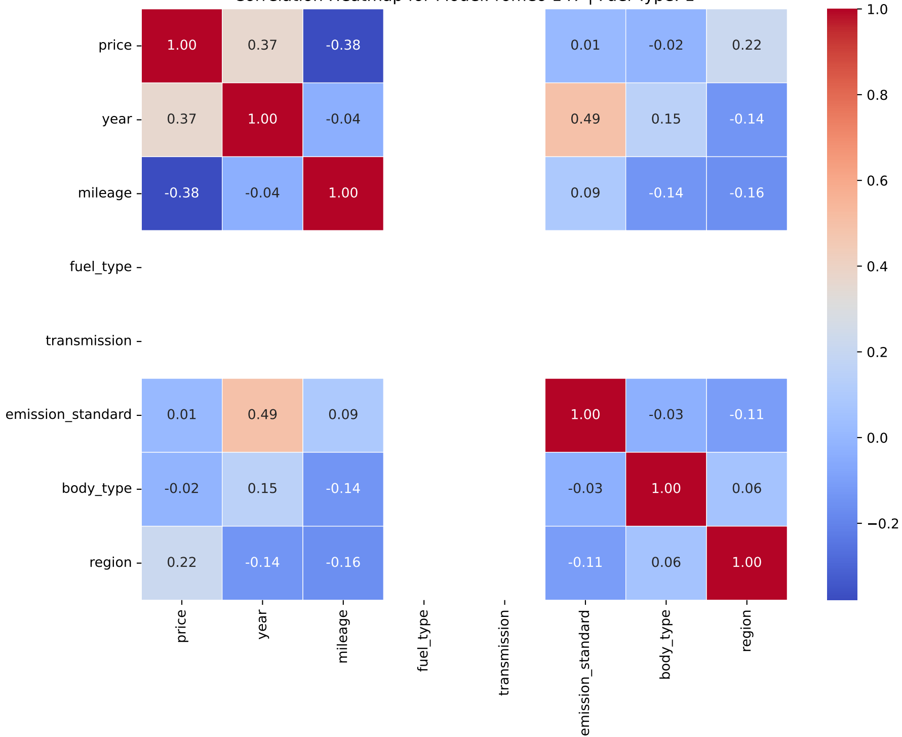
Correlation Heatmap for Model: romeo 147 | Fuel Type: 1
