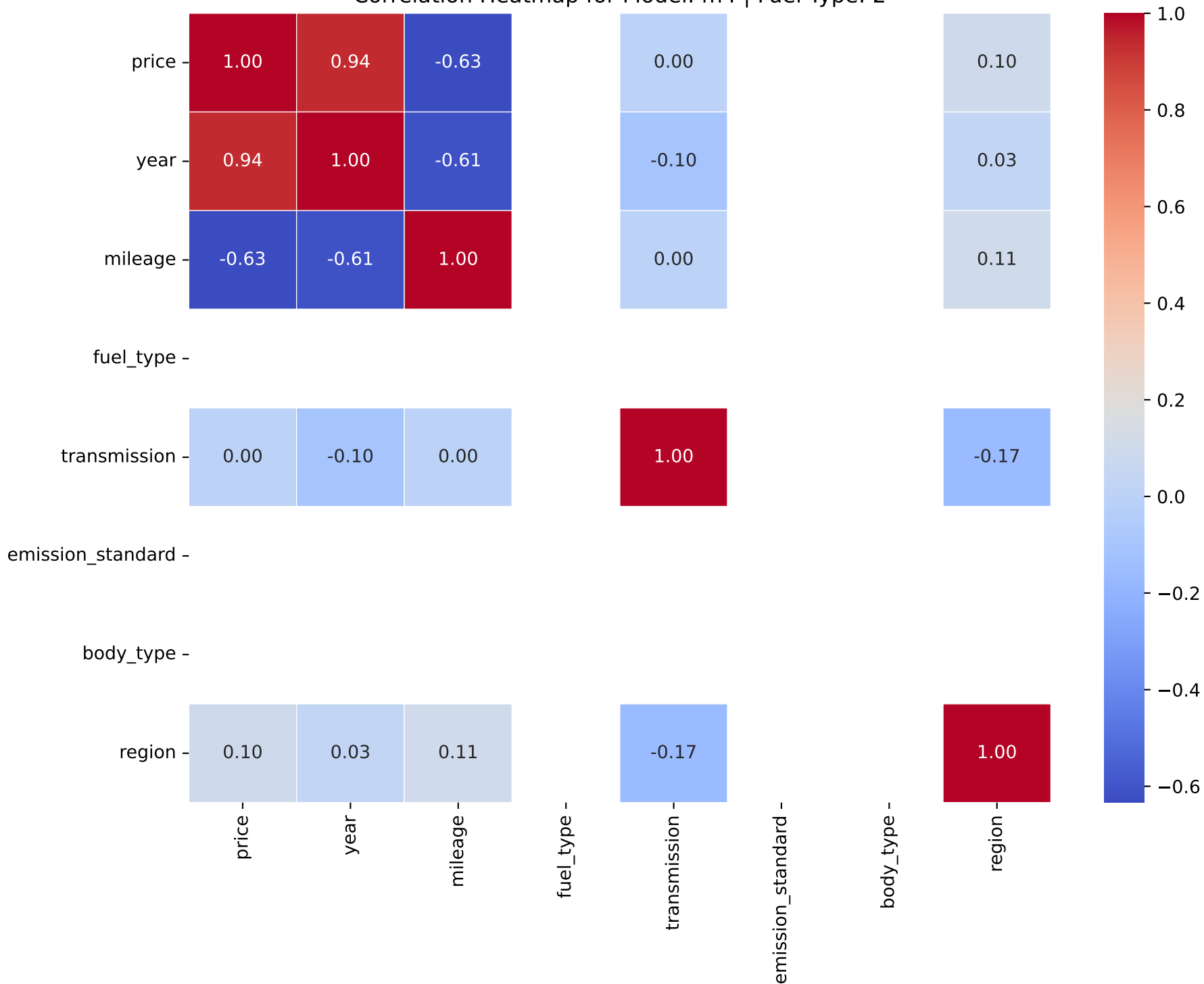
Correlation Heatmap for Model: m4 | Fuel Type: 2
