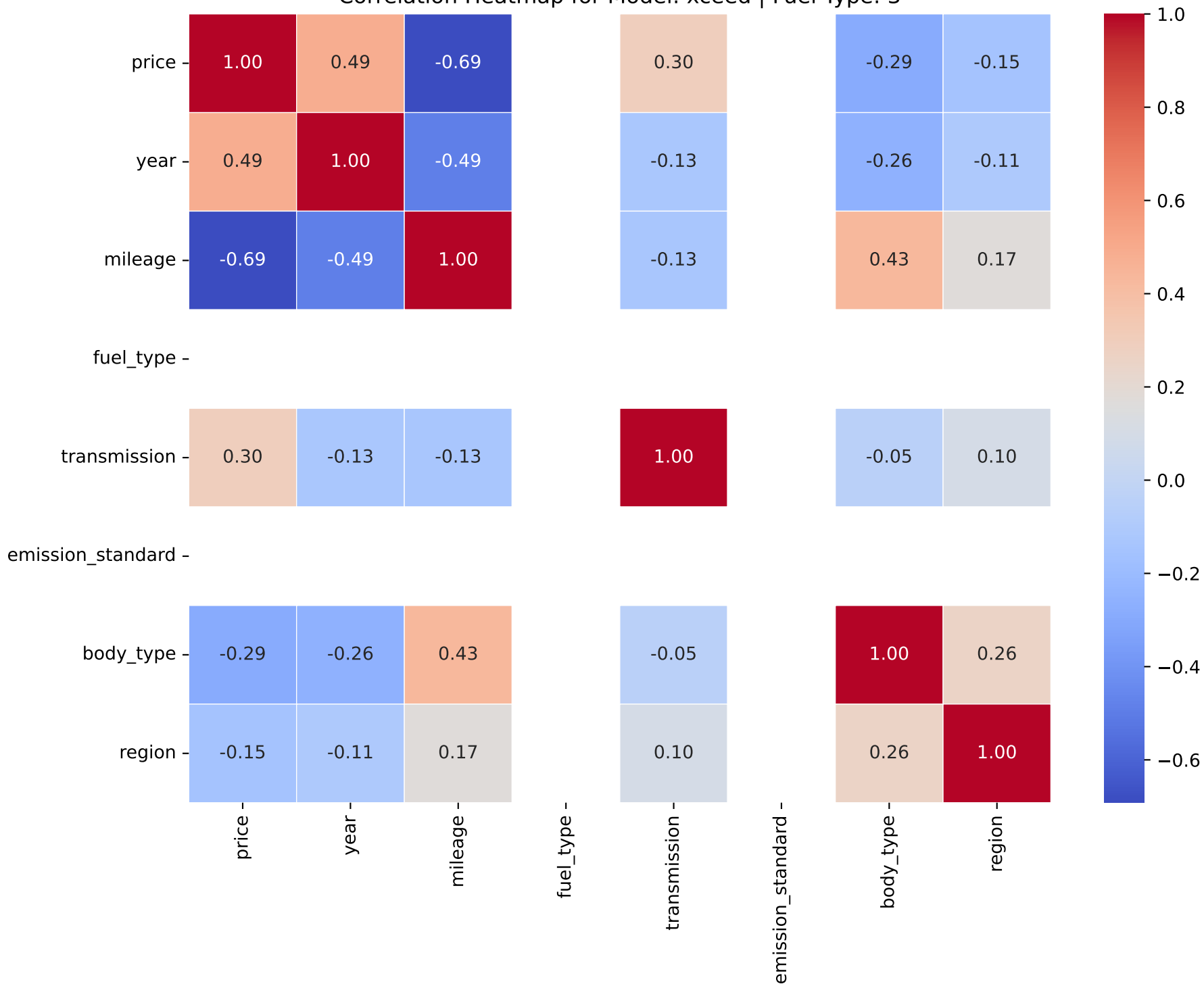
Correlation Heatmap for Model: xceed | Fuel Type: 3
