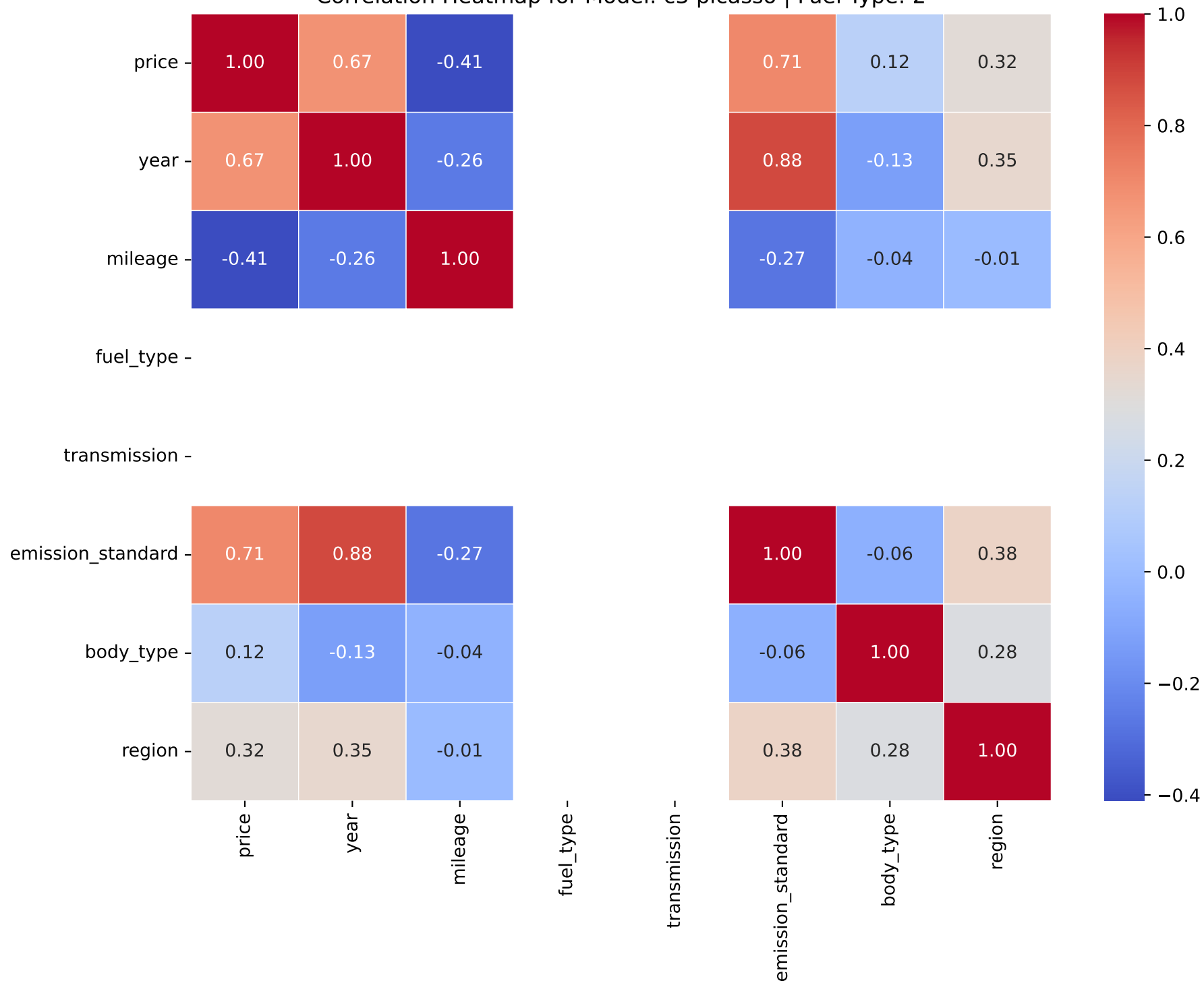
Correlation Heatmap for Model: c3 picasso | Fuel Type: 2
