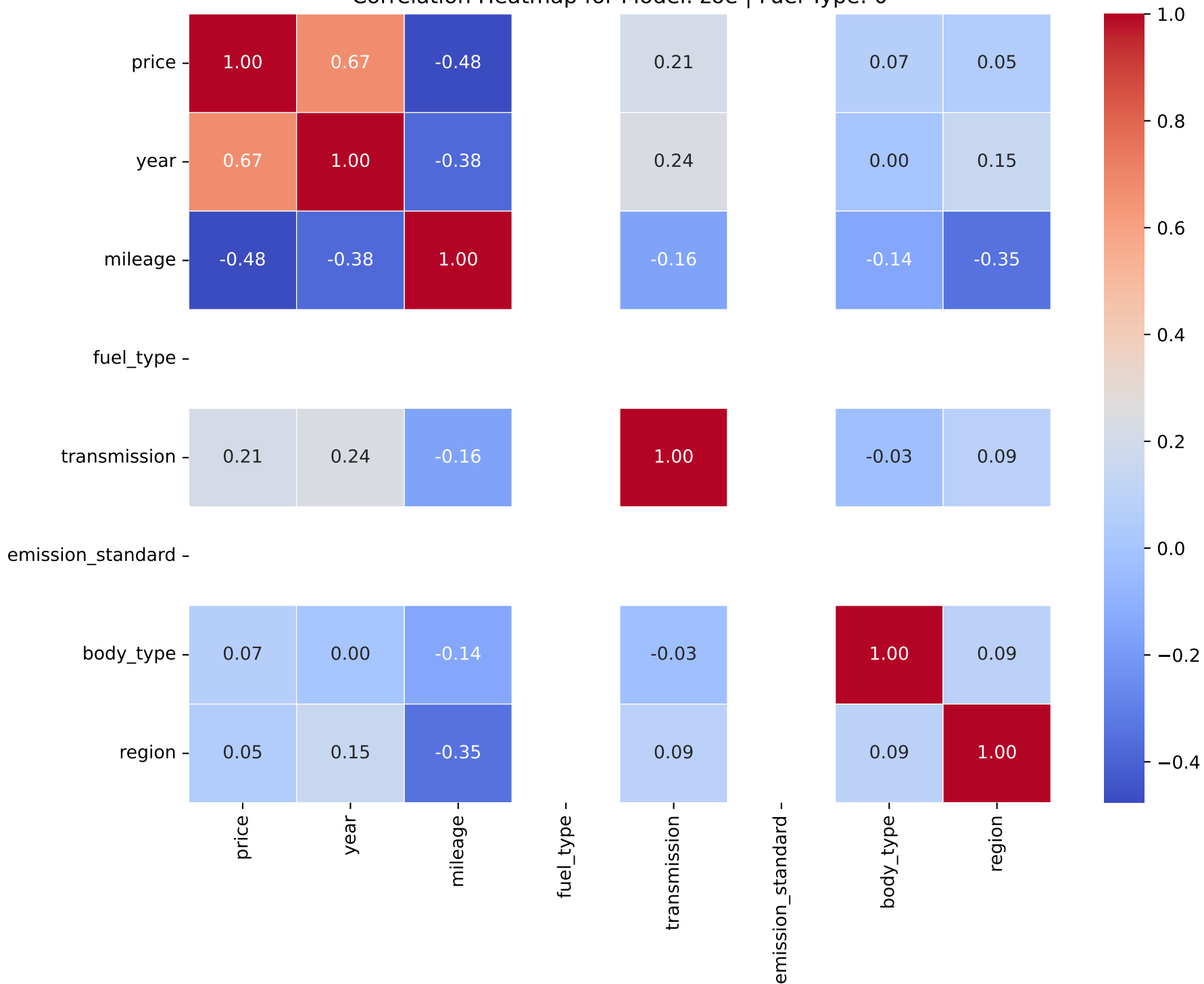
Correlation Heatmap for Model: zoe | Fuel Type: 0
