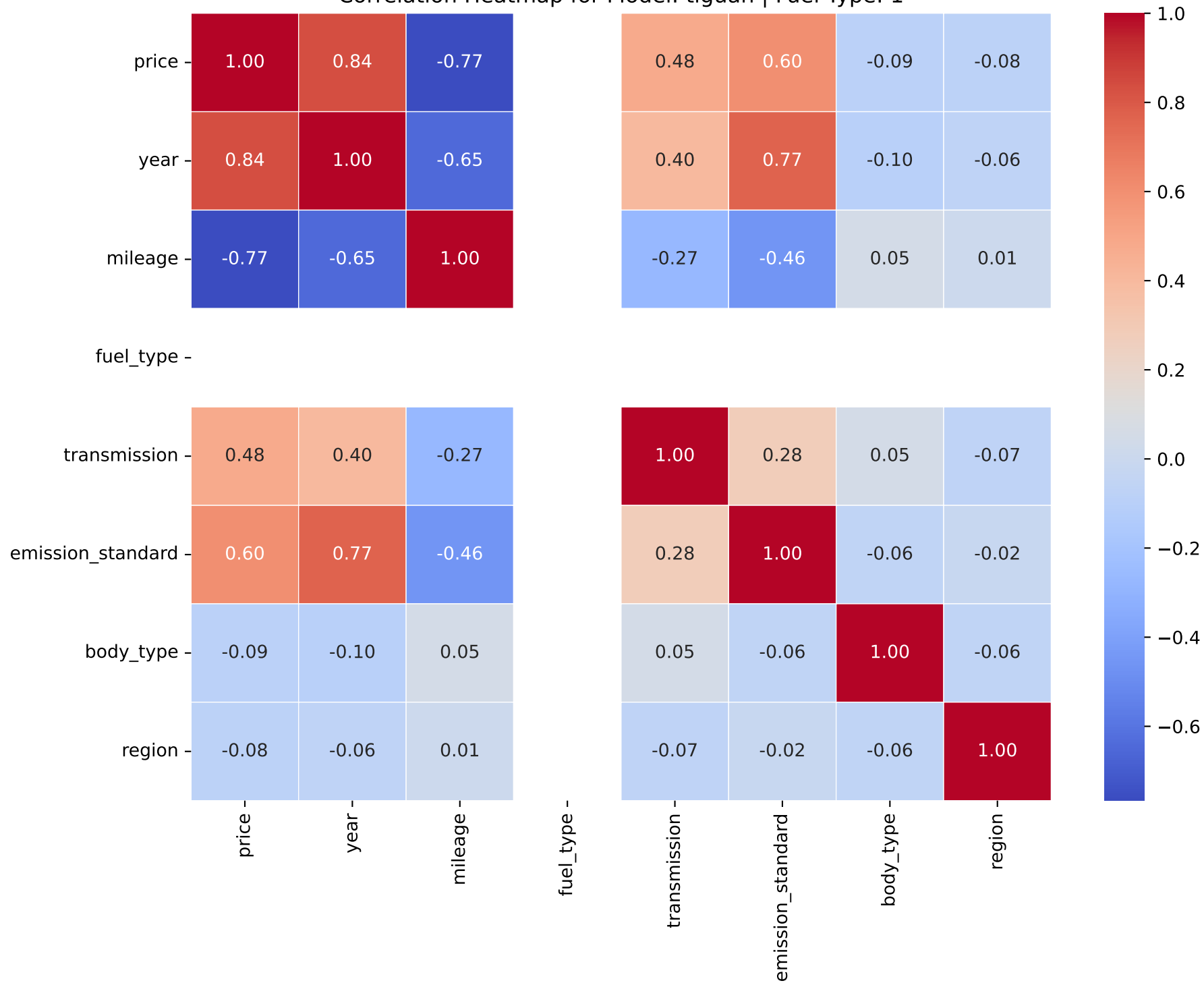
Correlation Heatmap for Model: tiguan | Fuel Type: 1
