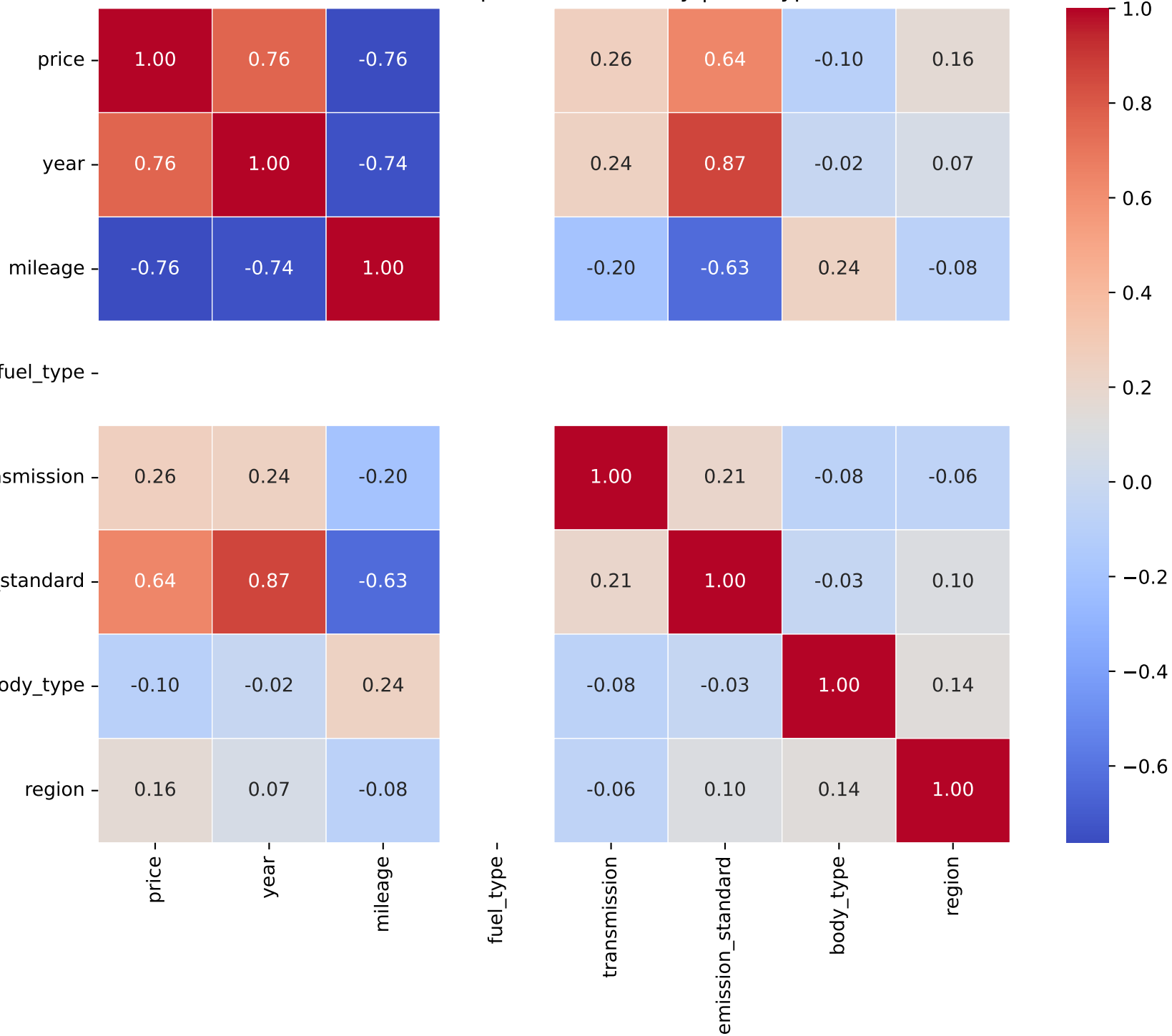
Correlation Heatmap for Model: caddy | Fuel Type: 1
