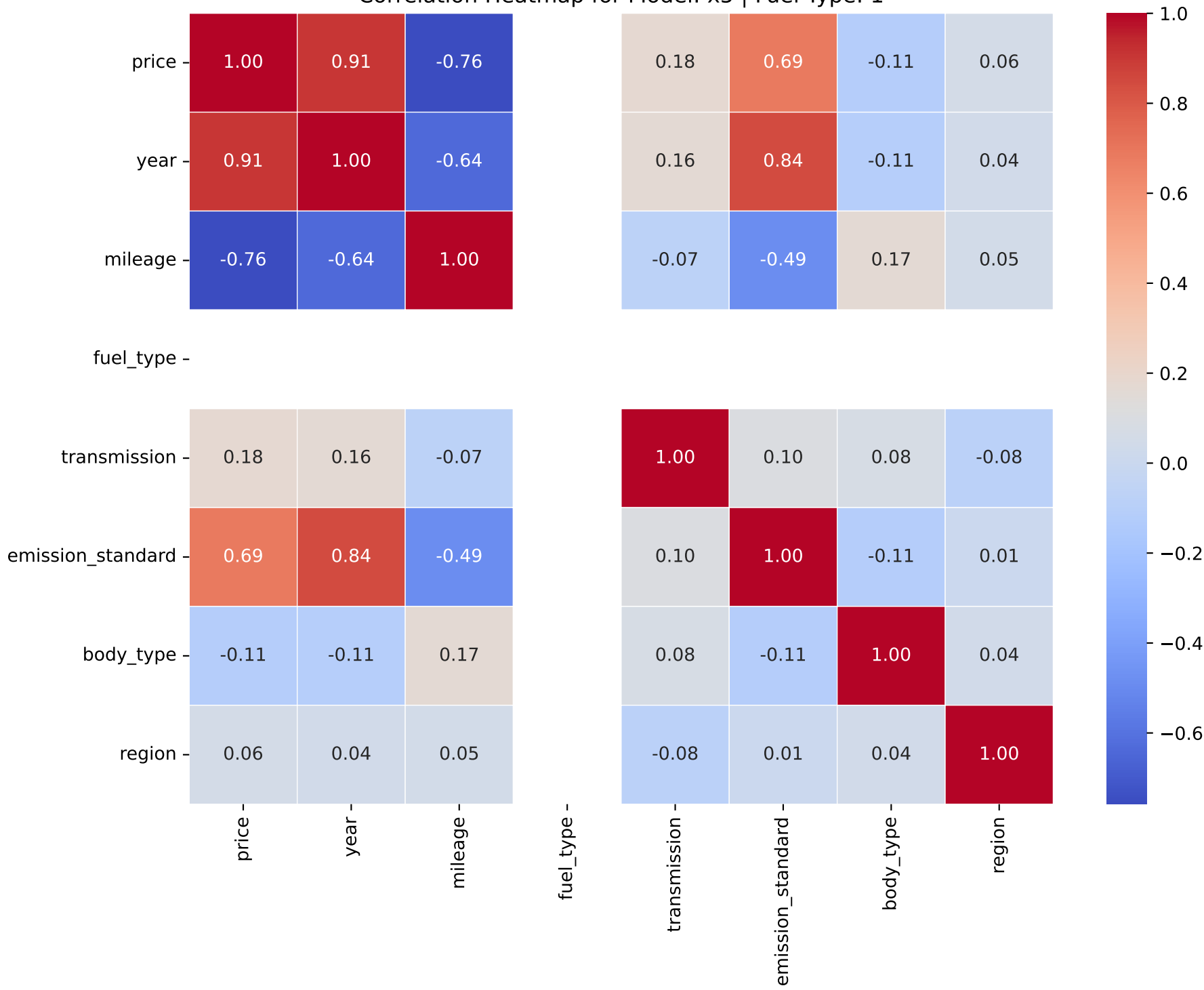
Correlation Heatmap for Model: x5 | Fuel Type: 1
