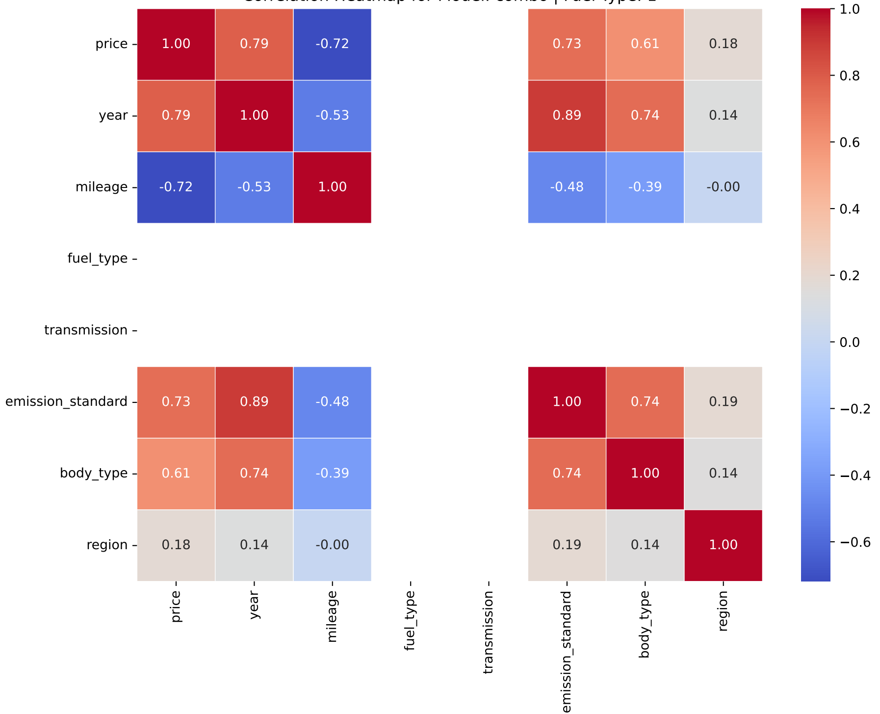
Correlation Heatmap for Model: combo | Fuel Type: 1
