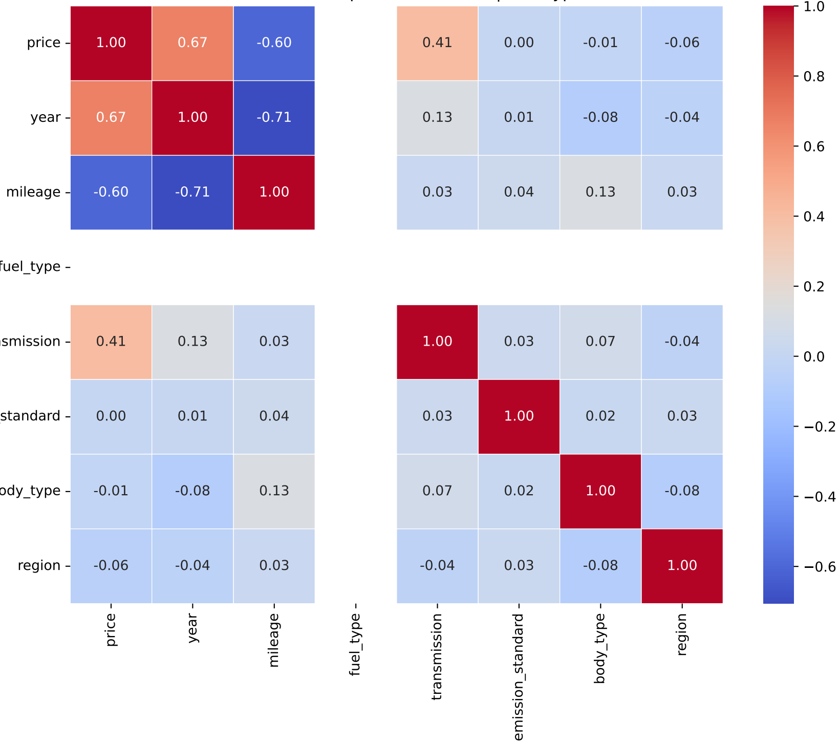
Correlation Heatmap for Model: t-roc | Fuel Type: 2
