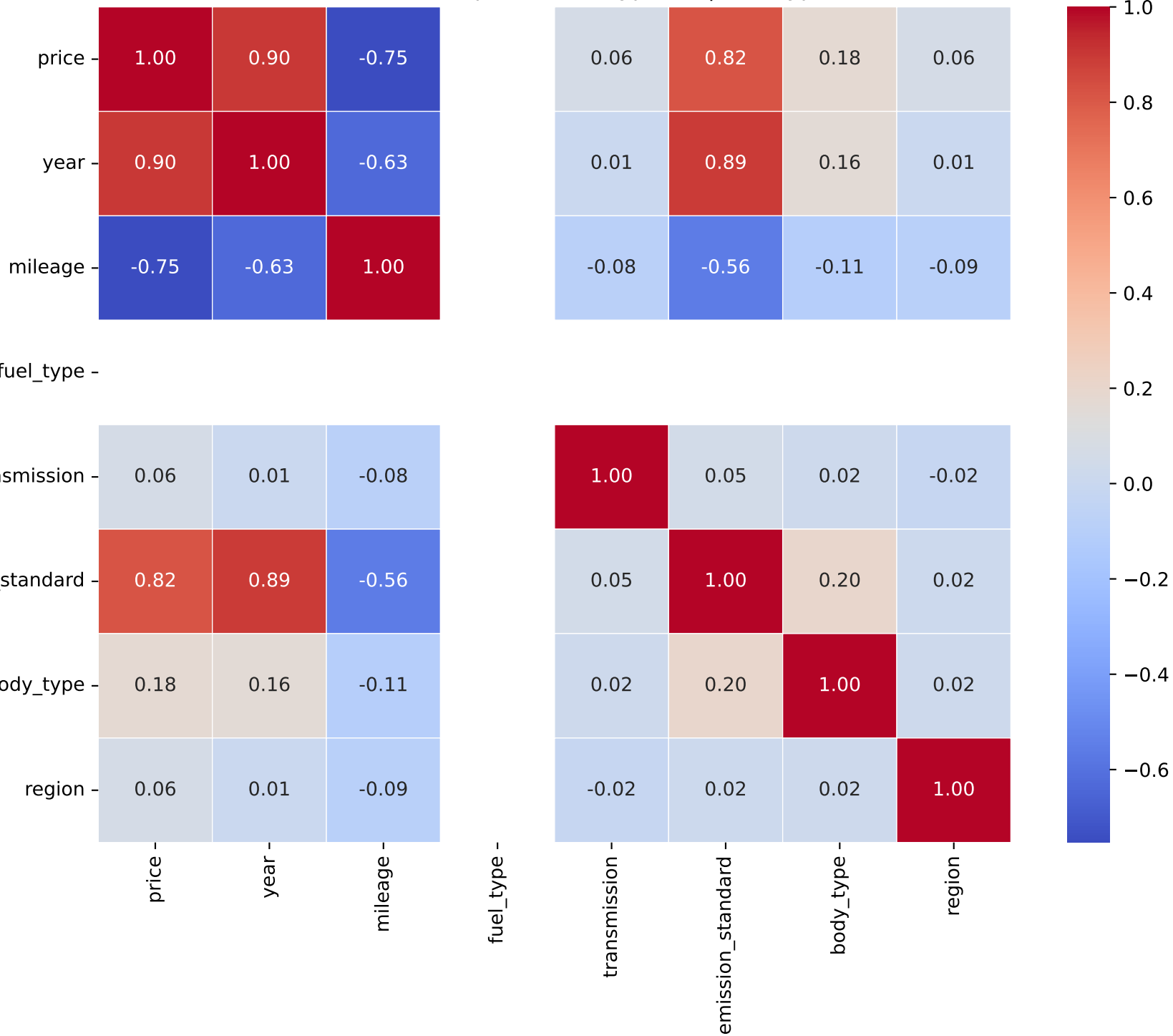
Correlation Heatmap for Model: ypsilon | Fuel Type: 2
