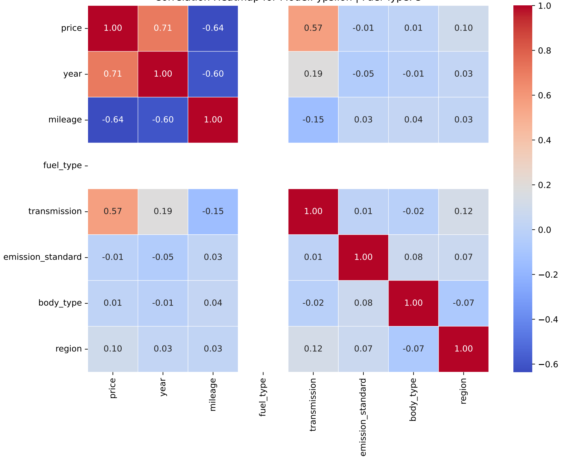
Correlation Heatmap for Model: ypsilon | Fuel Type: 3
