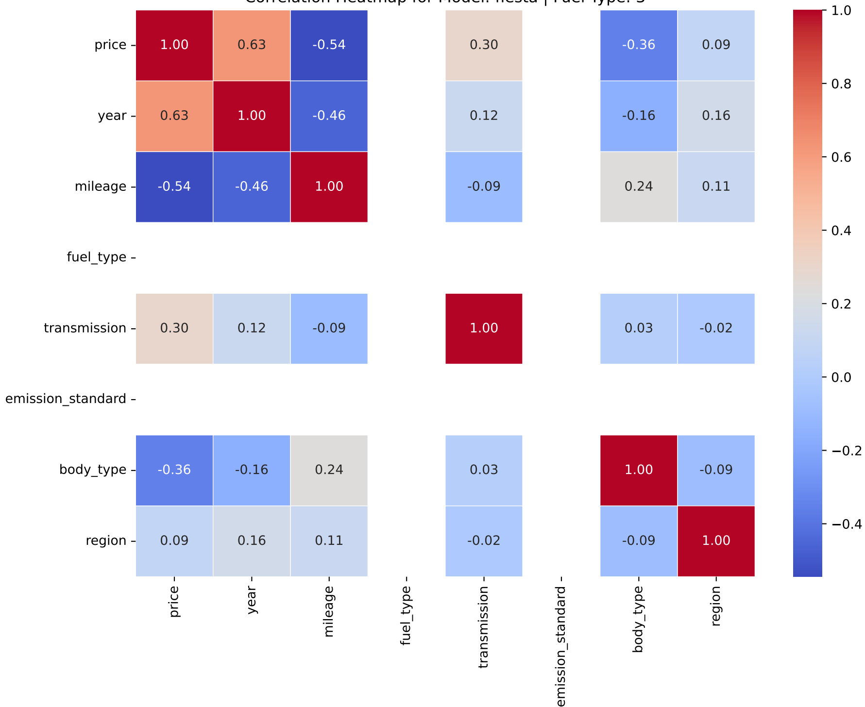
Correlation Heatmap for Model: fiesta | Fuel Type: 3
