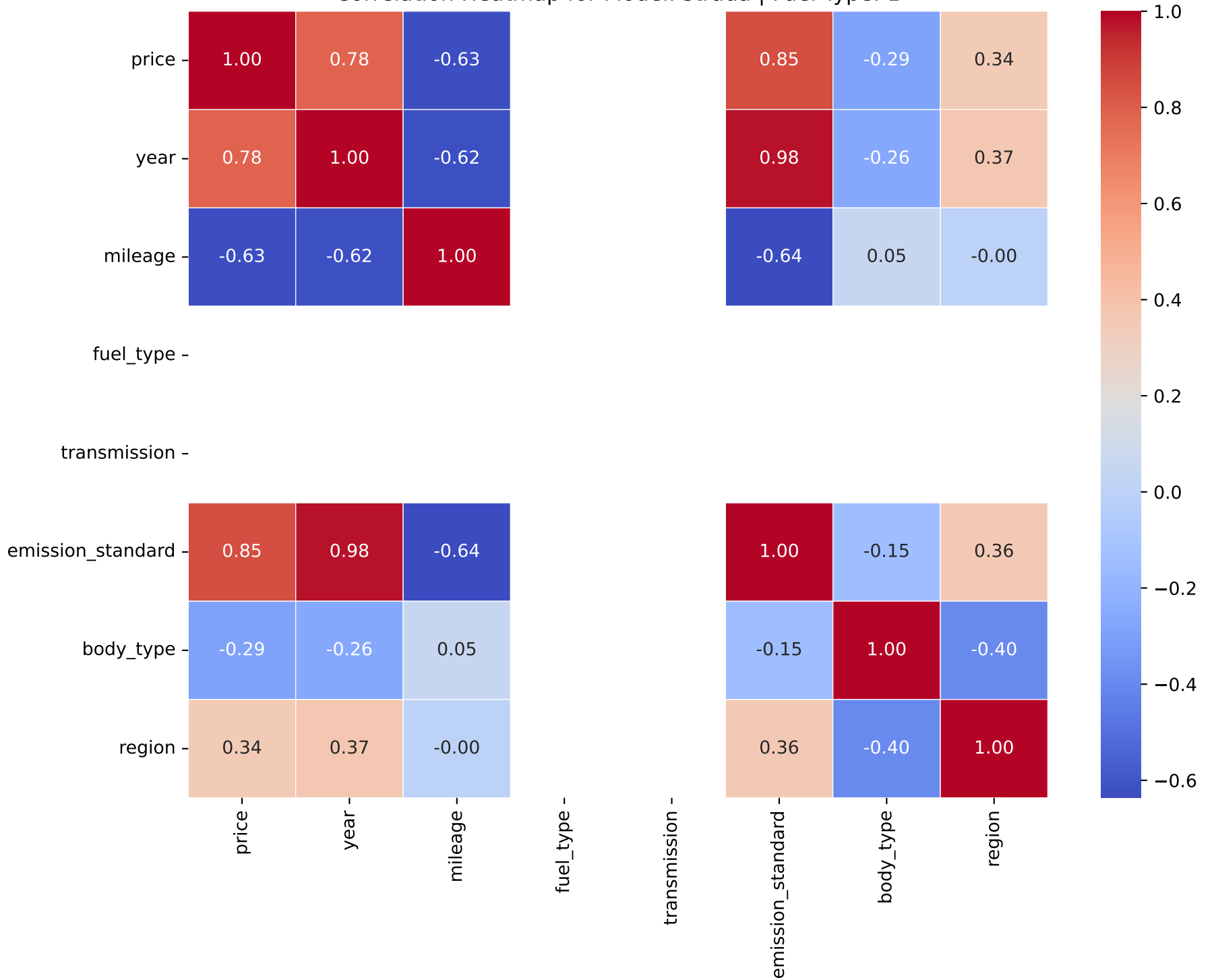
Correlation Heatmap for Model: strada | Fuel Type: 1
