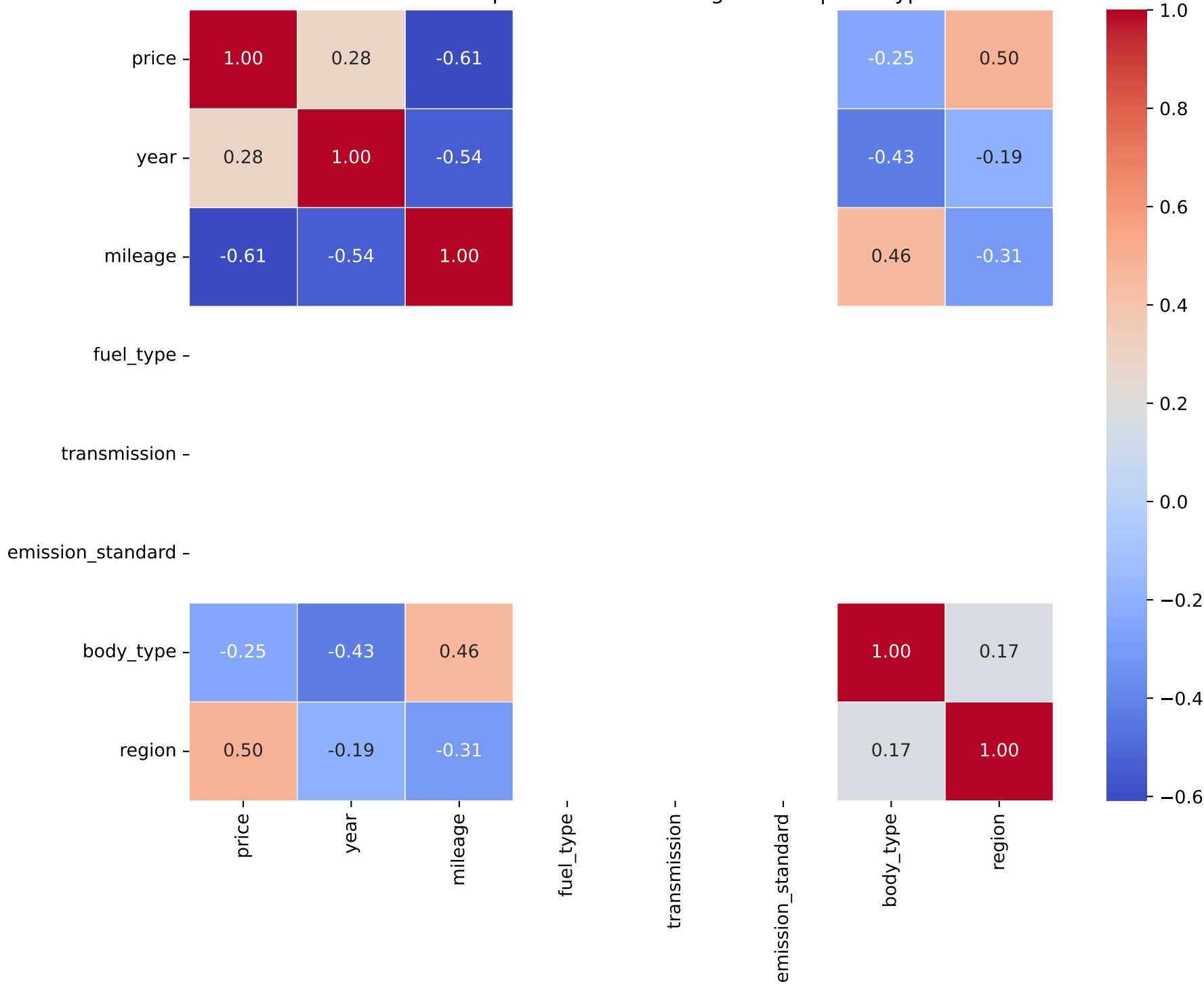
Correlation Heatmap for Model: mustang mach-e | Fuel Type: 0
