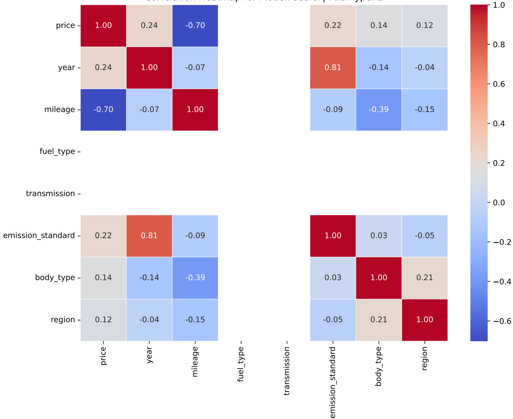
Correlation Heatmap for Model: sedici | Fuel Type: 2
