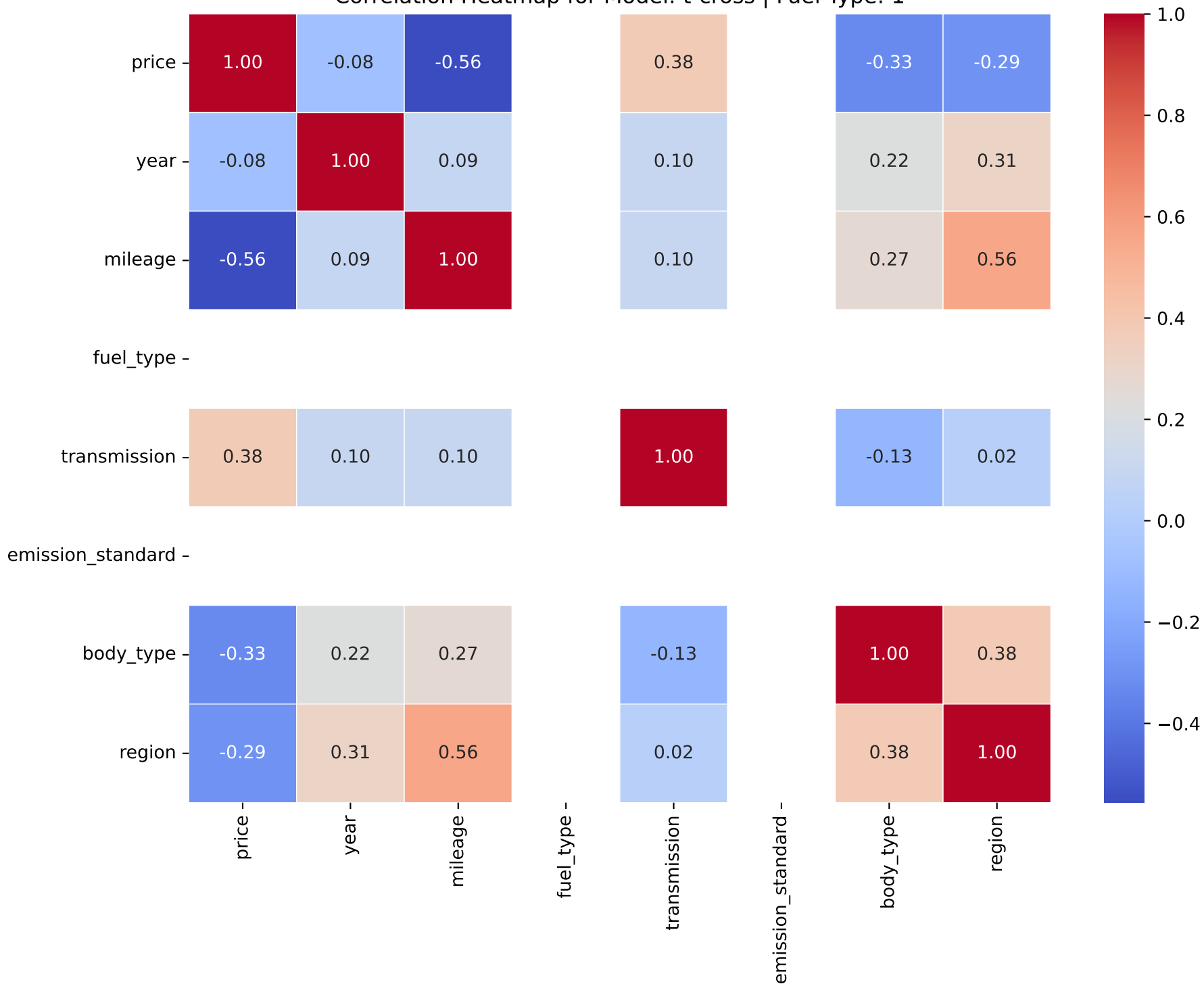
Correlation Heatmap for Model: t-cross | Fuel Type: 1
