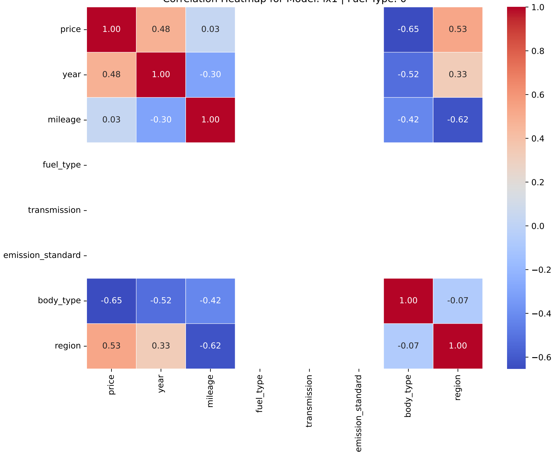
Correlation Heatmap for Model: ix1 | Fuel Type: 0
