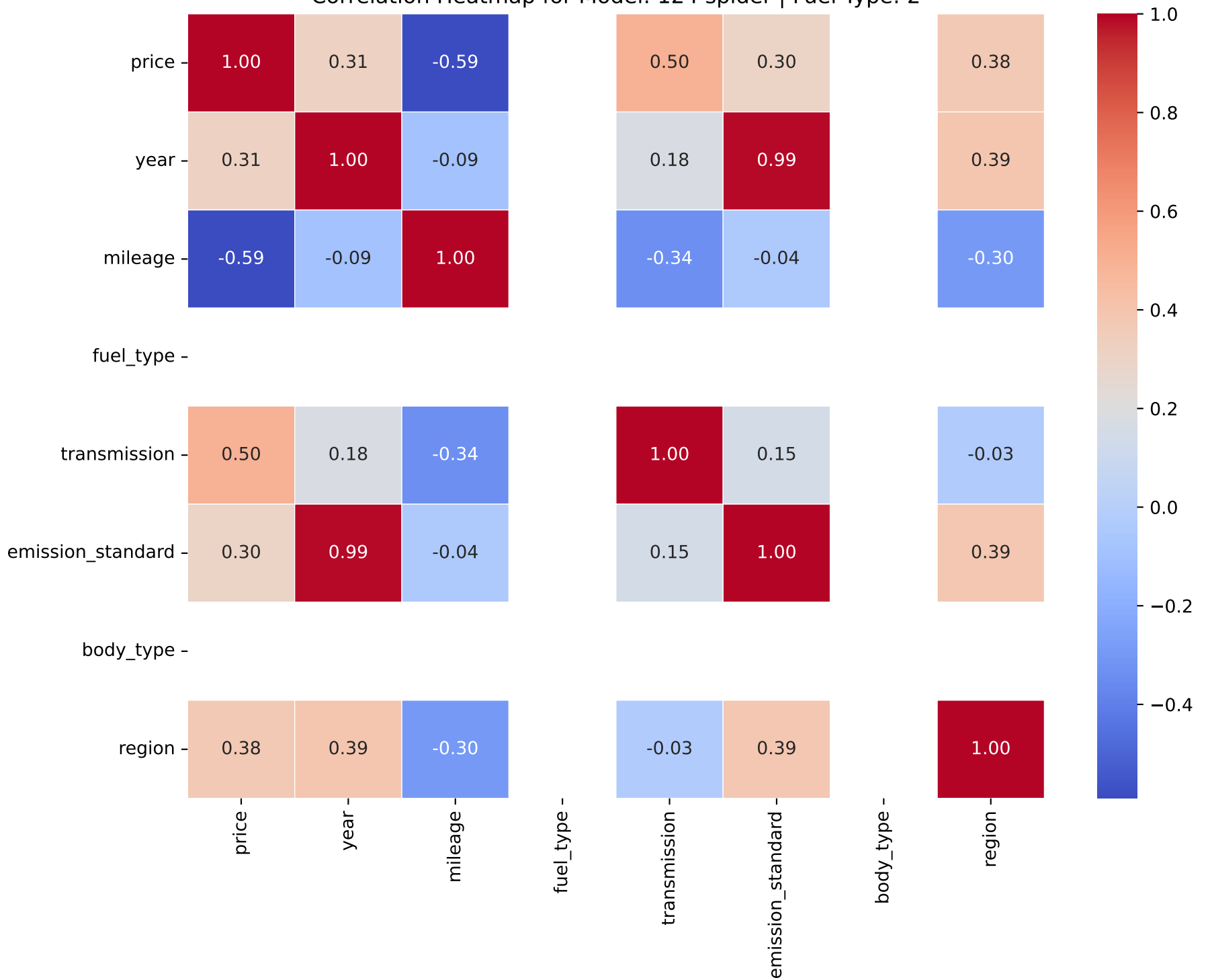
Correlation Heatmap for Model: 124 spider | Fuel Type: 2
