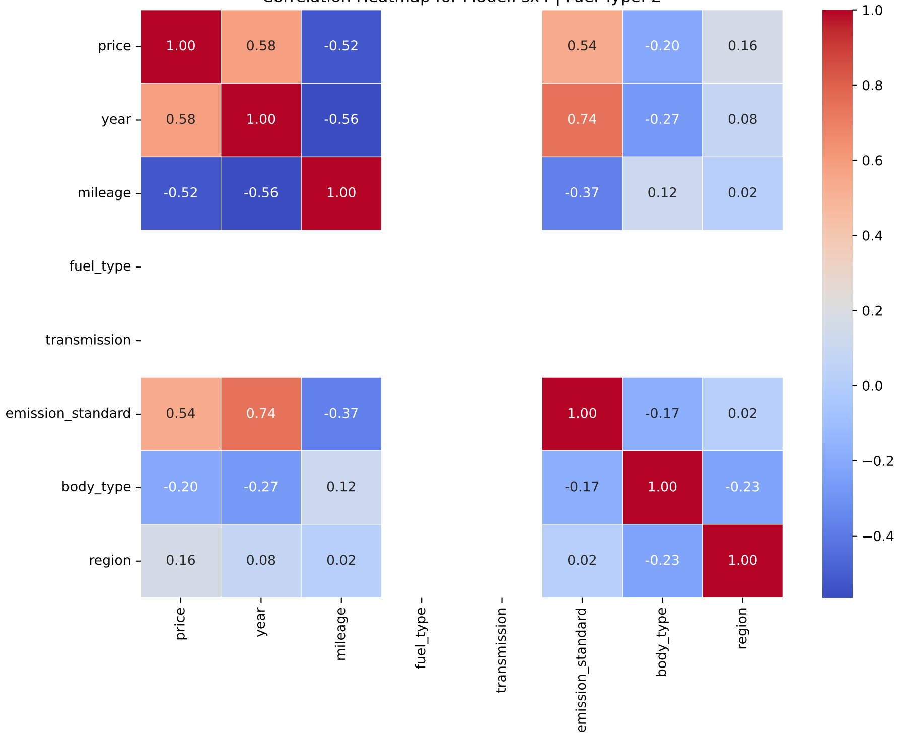
Correlation Heatmap for Model: sx4 | Fuel Type: 2
