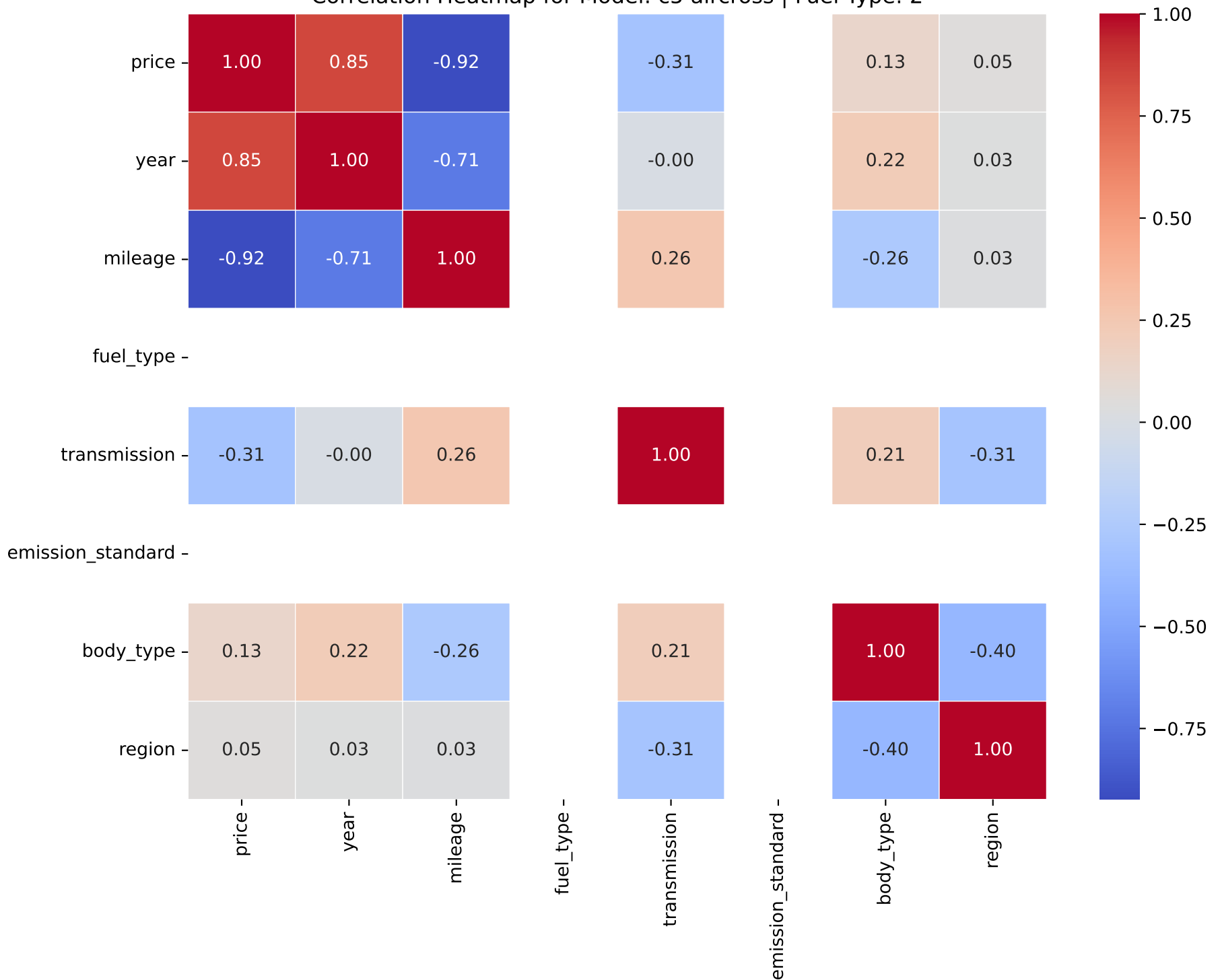
Correlation Heatmap for Model: c5 aircross | Fuel Type: 2
