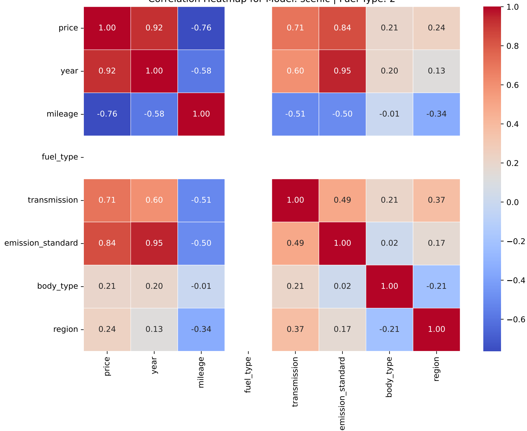
Correlation Heatmap for Model: scenic | Fuel Type: 2
