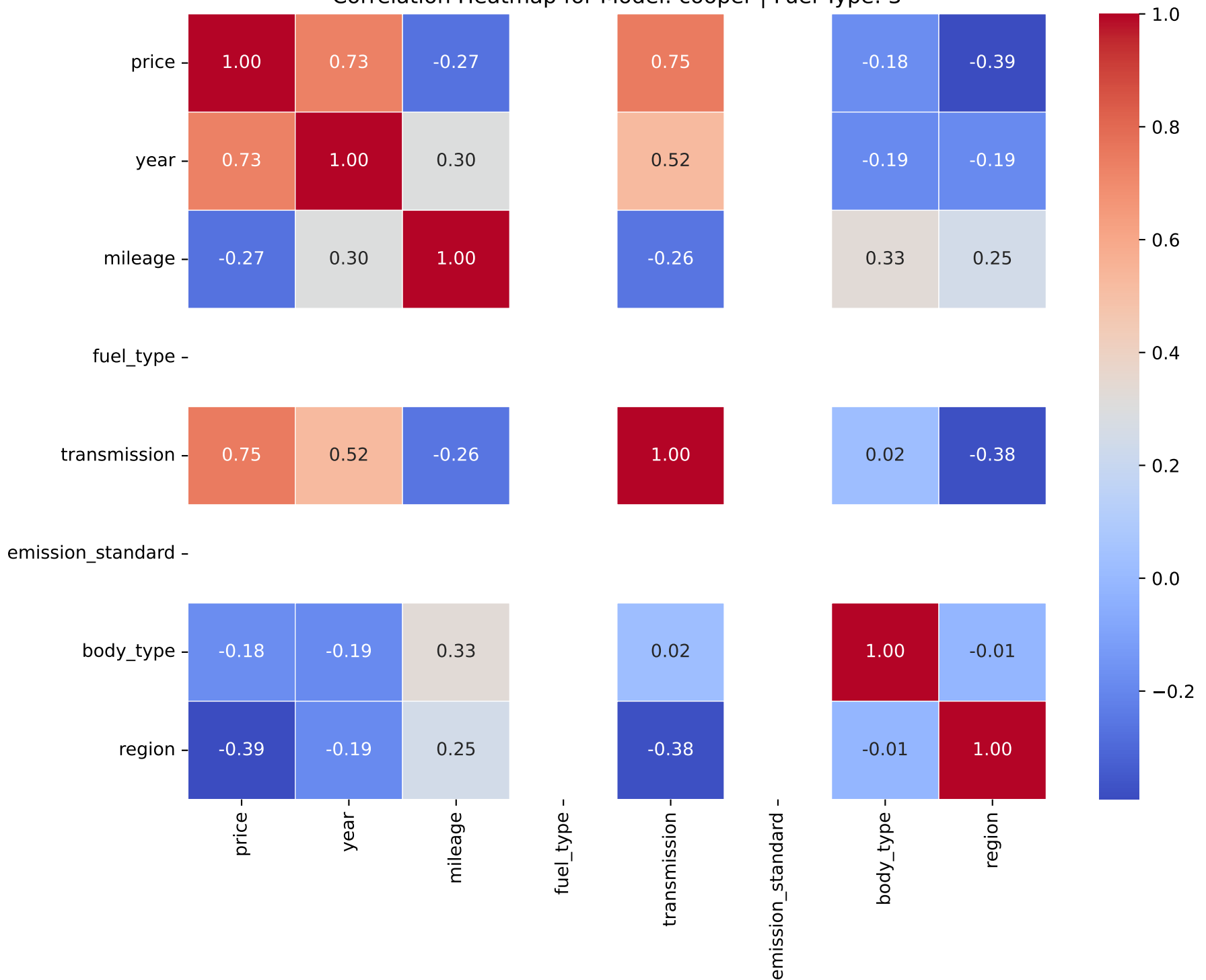
Correlation Heatmap for Model: cooper | Fuel Type: 3
