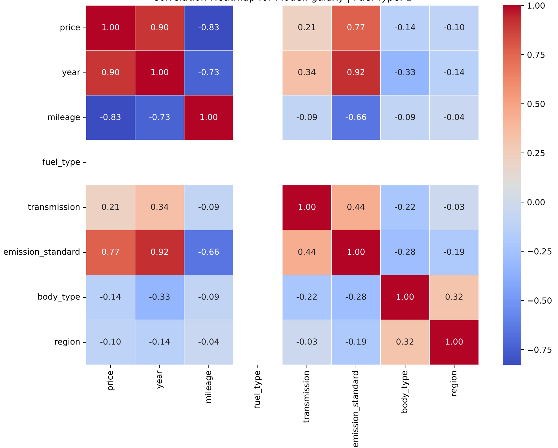
Correlation Heatmap for Model: galaxy | Fuel Type: 1
