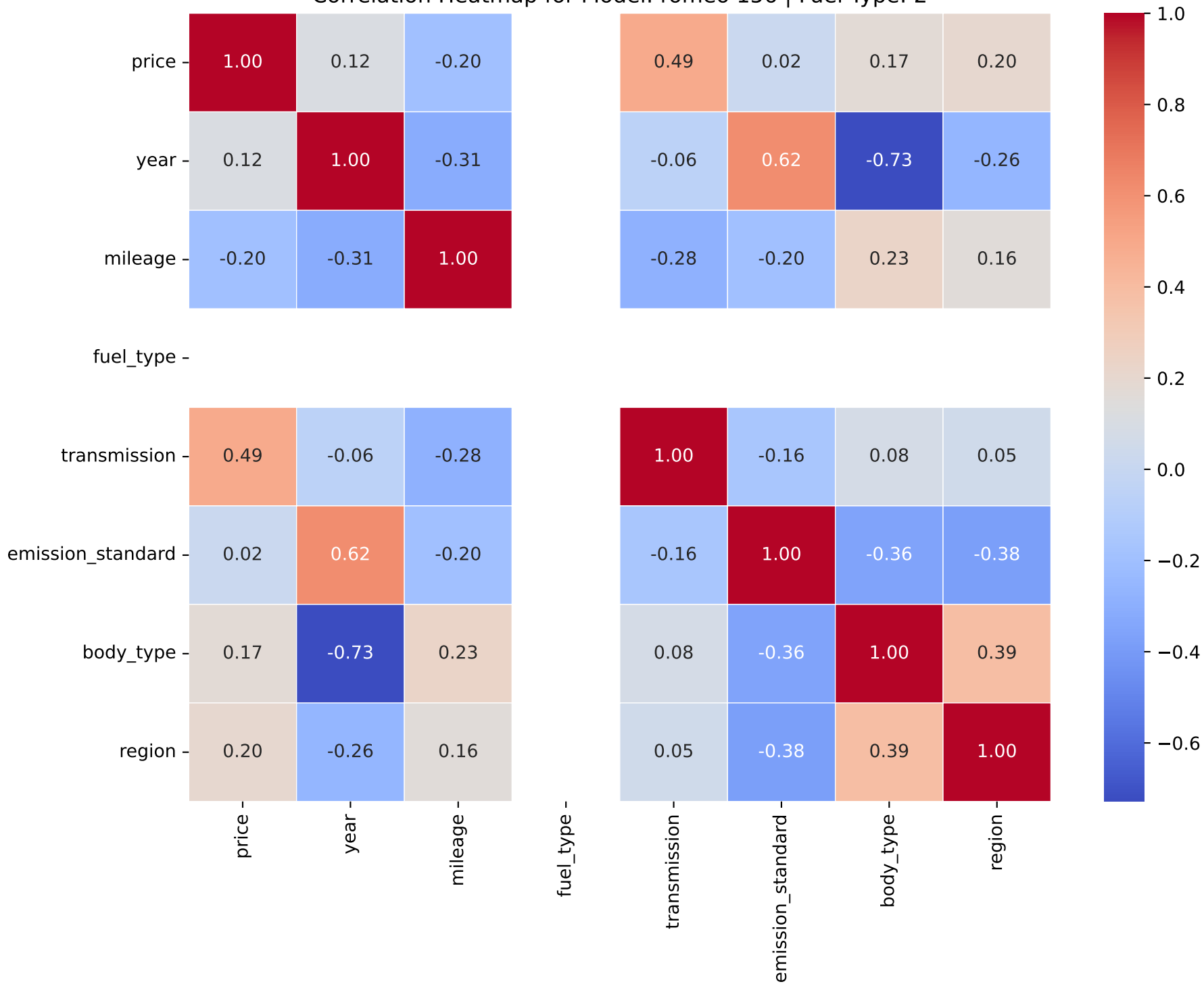
Correlation Heatmap for Model: romeo 156 | Fuel Type: 2
