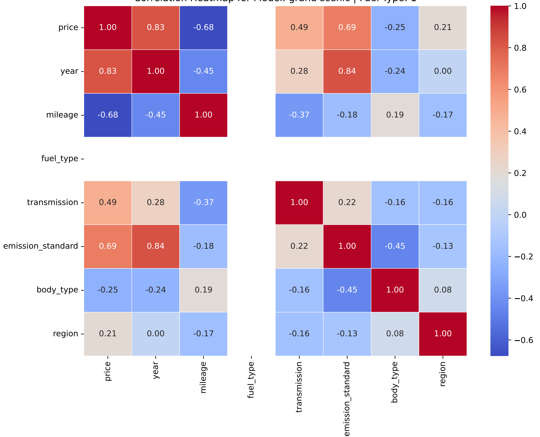
Correlation Heatmap for Model: grand scenic | Fuel Type: 1
