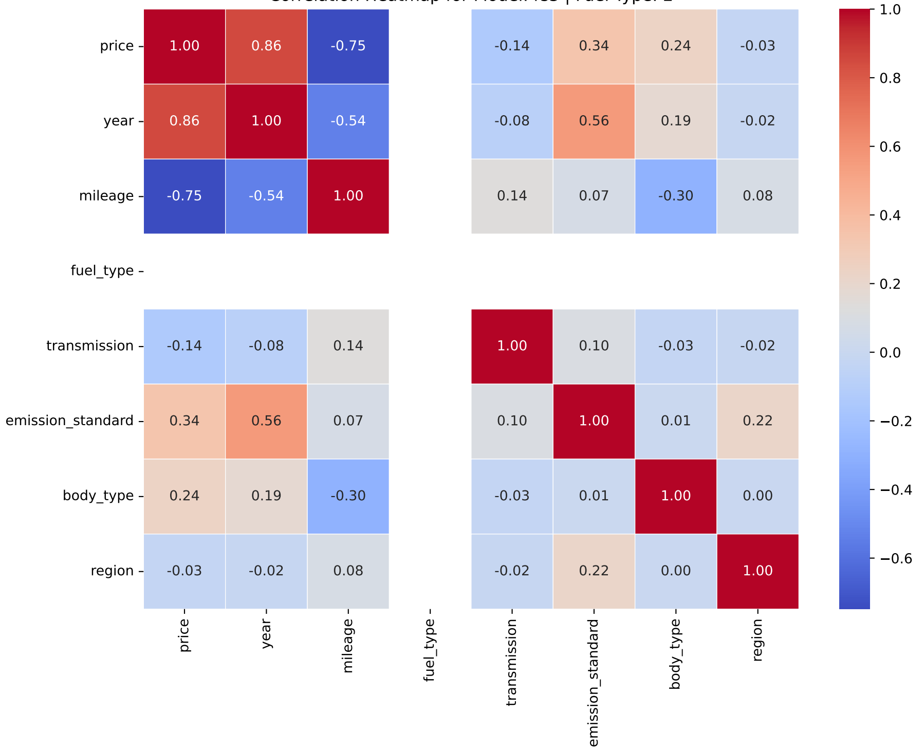
Correlation Heatmap for Model: rs3 | Fuel Type: 2
