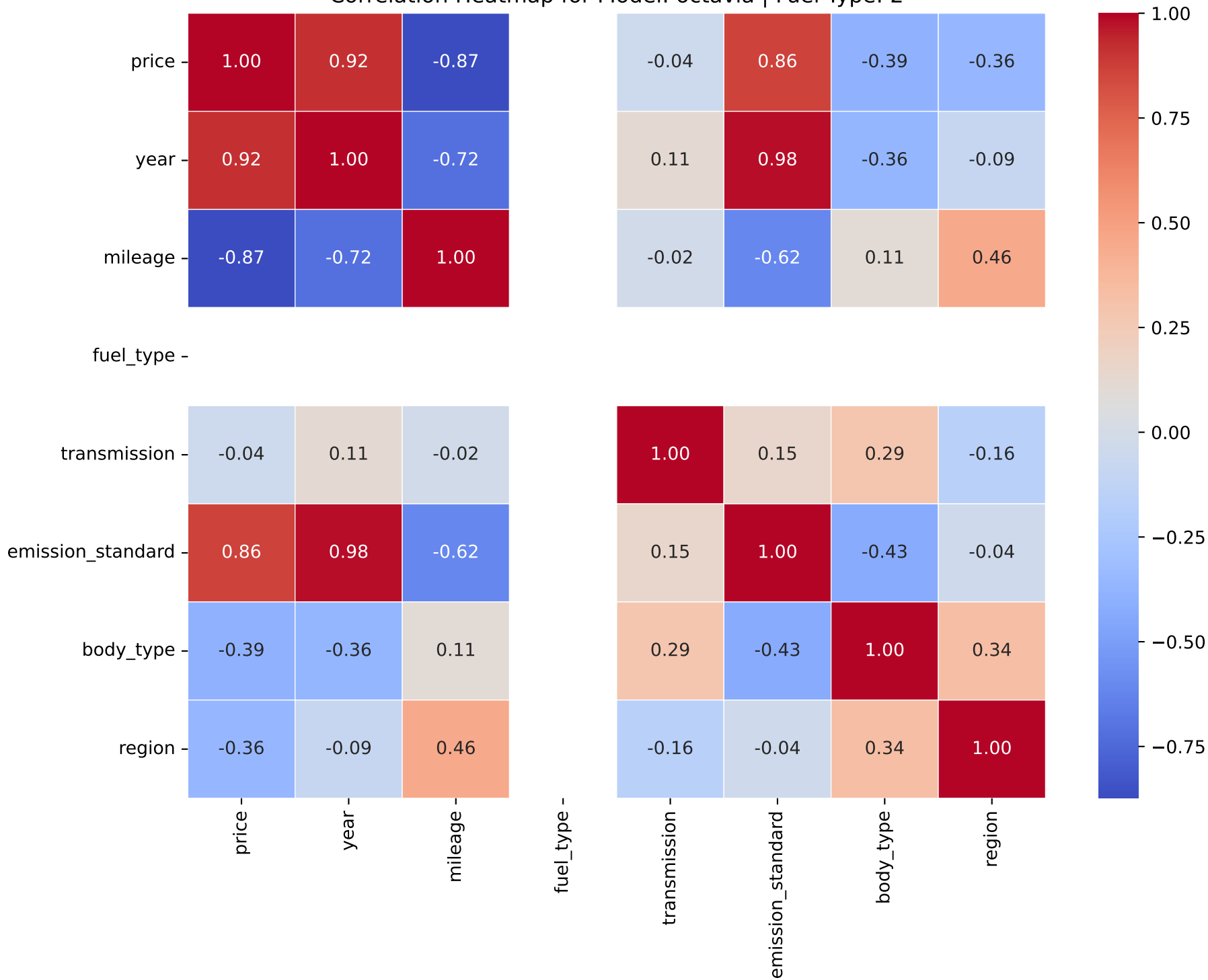
Correlation Heatmap for Model: octavia | Fuel Type: 2
