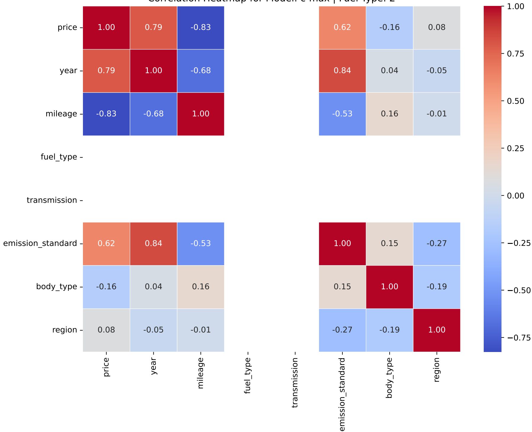
Correlation Heatmap for Model: c-max | Fuel Type: 2
