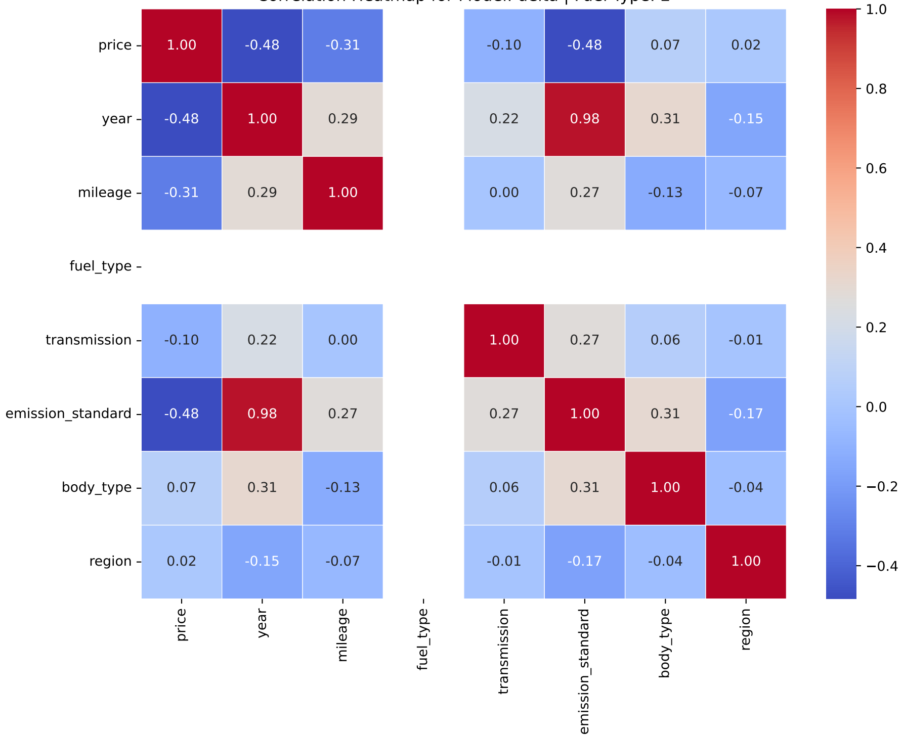
Correlation Heatmap for Model: delta | Fuel Type: 2
