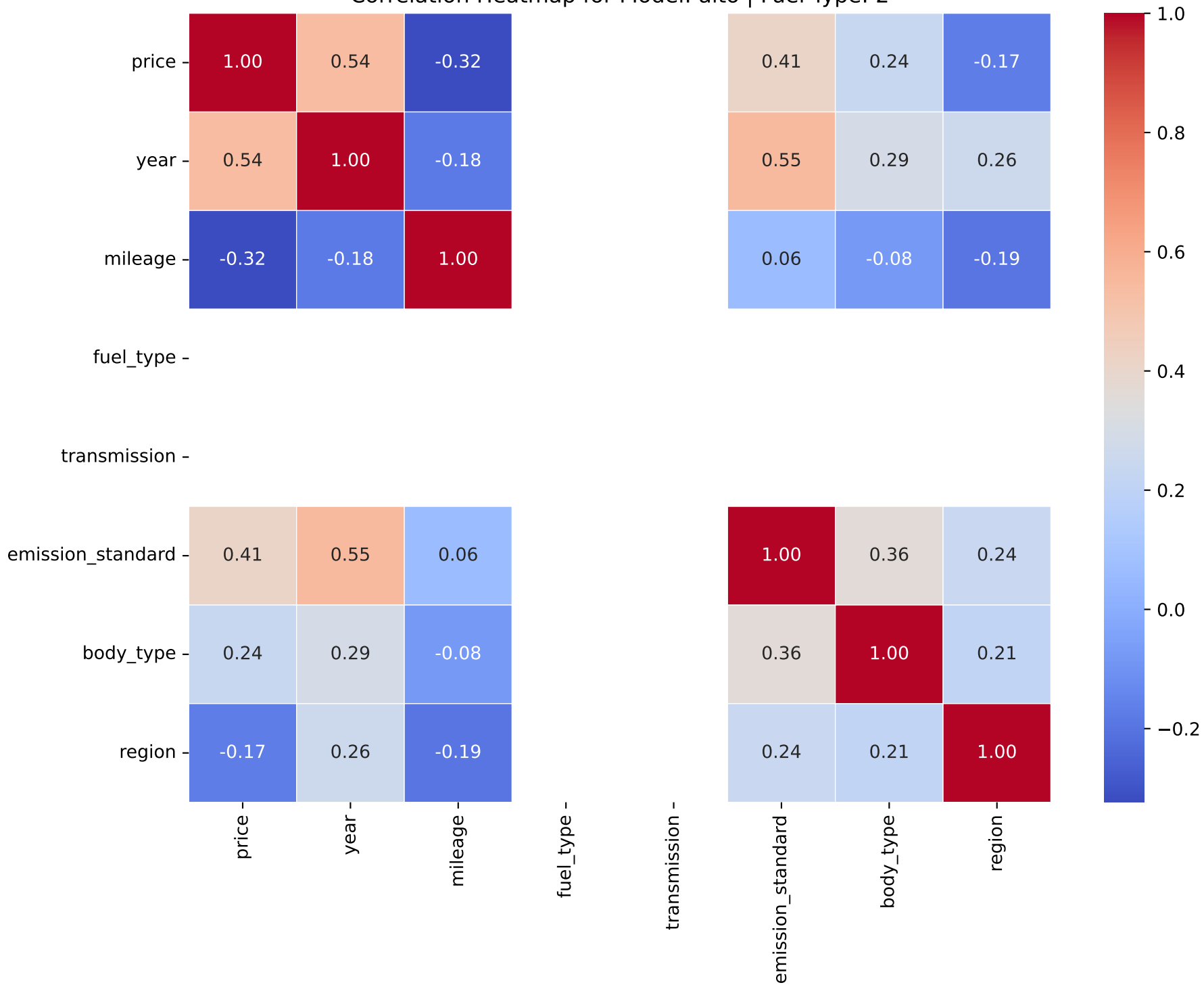
Correlation Heatmap for Model: alto | Fuel Type: 2
