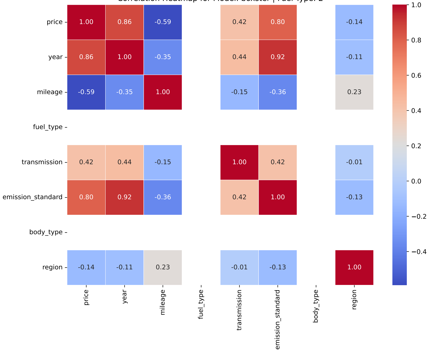
Correlation Heatmap for Model: boxster | Fuel Type: 2
