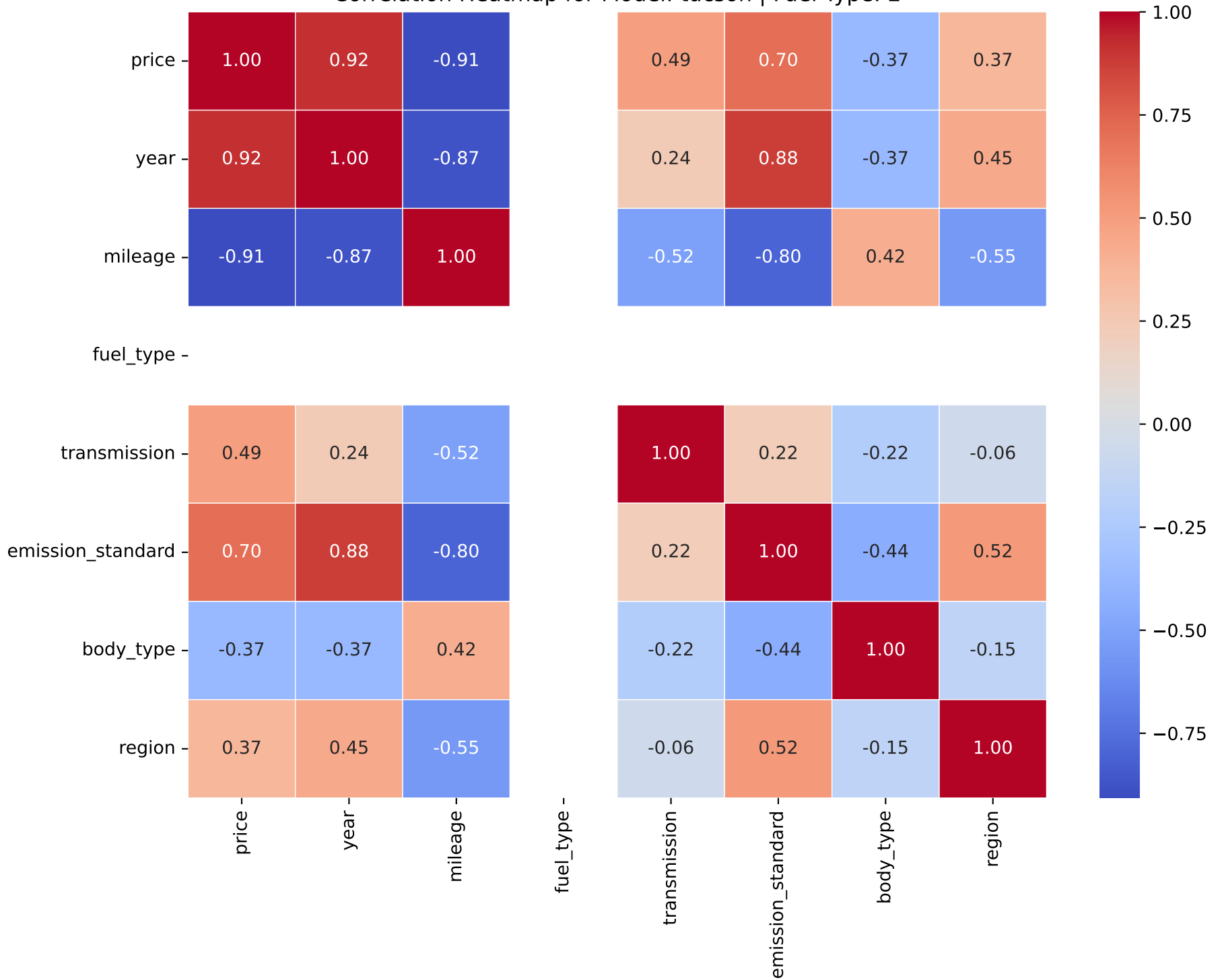
Correlation Heatmap for Model: tucson | Fuel Type: 2
