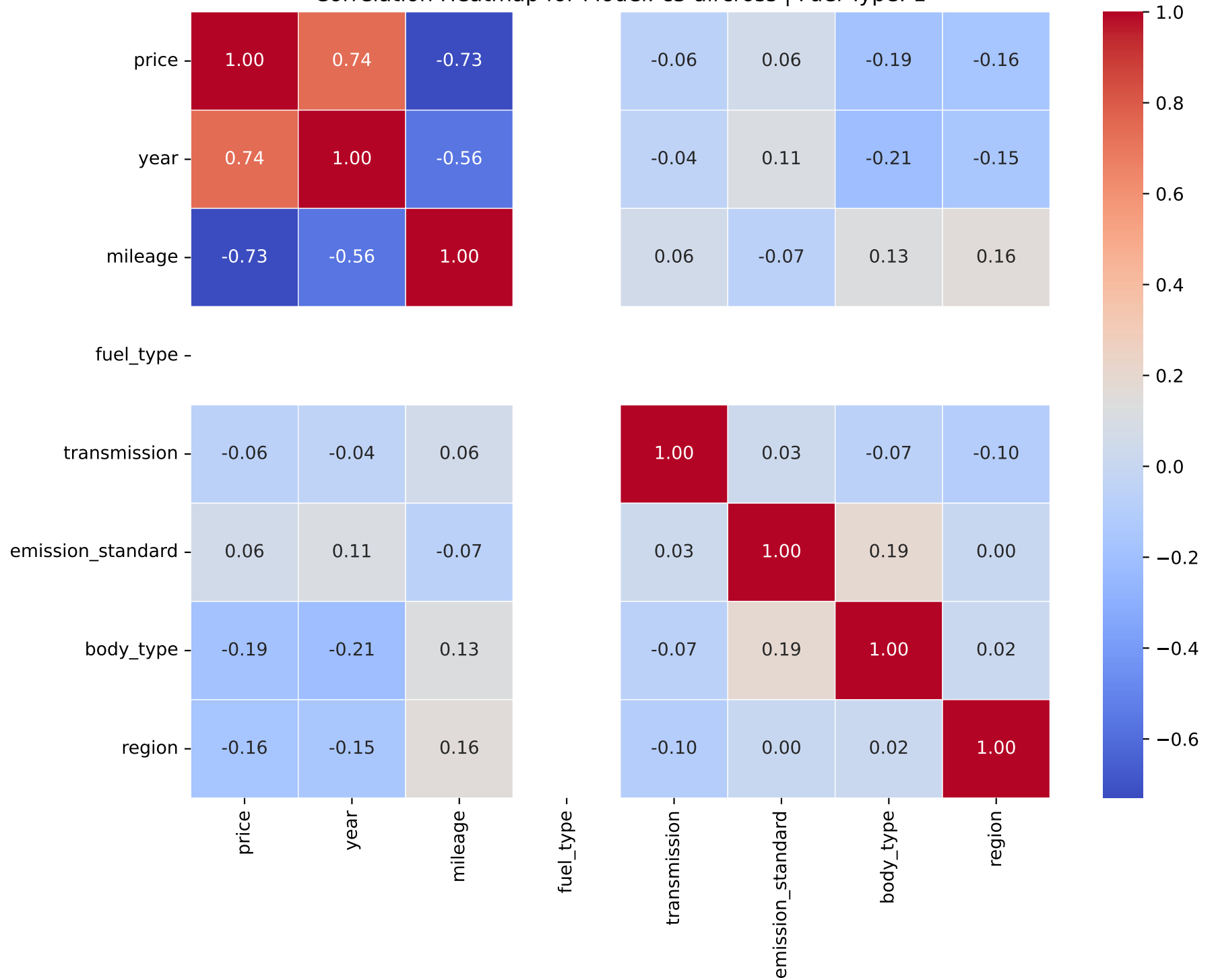
Correlation Heatmap for Model: c3 aircross | Fuel Type: 1
