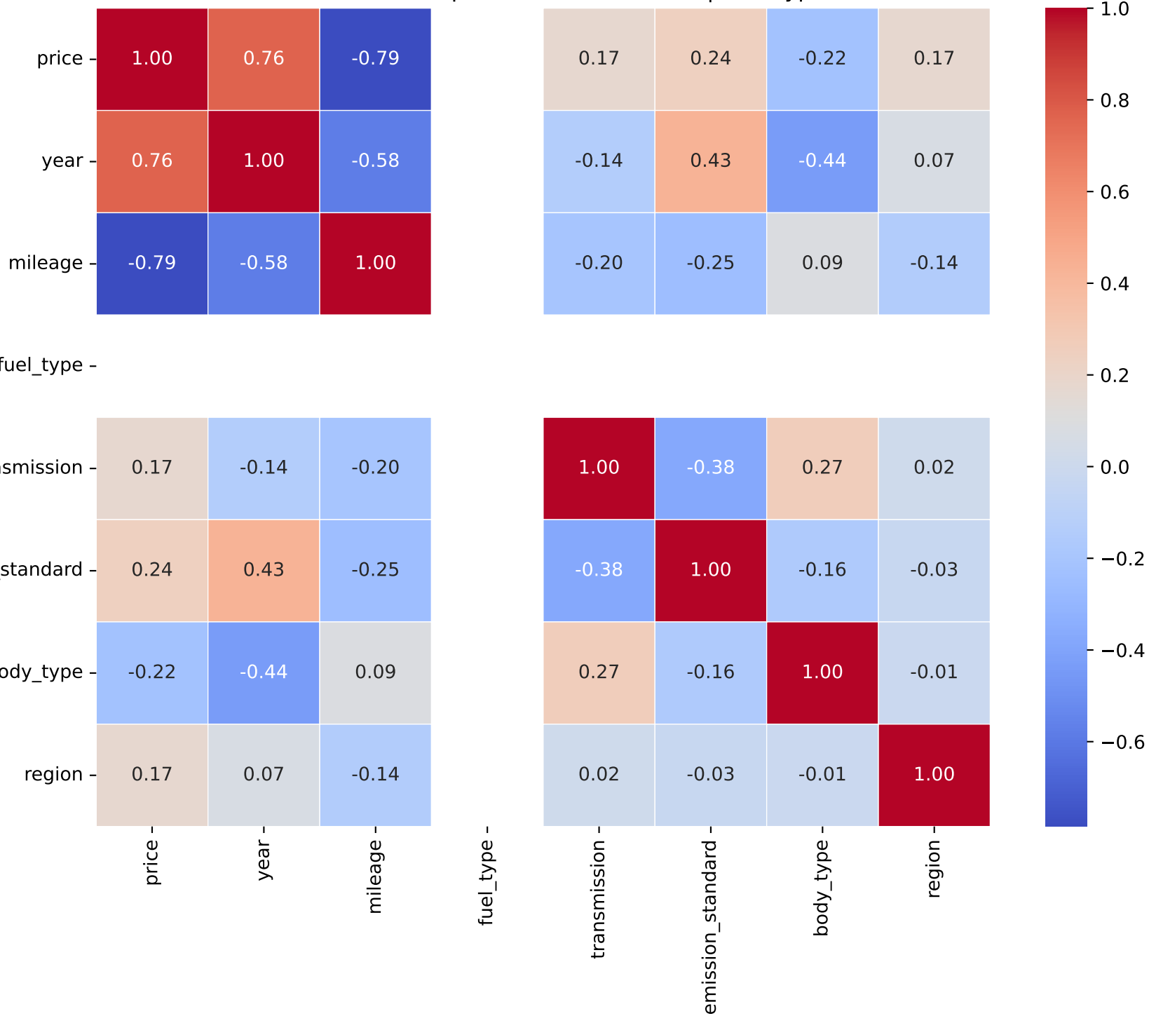
Correlation Heatmap for Model: c4 cactus | Fuel Type: 1
