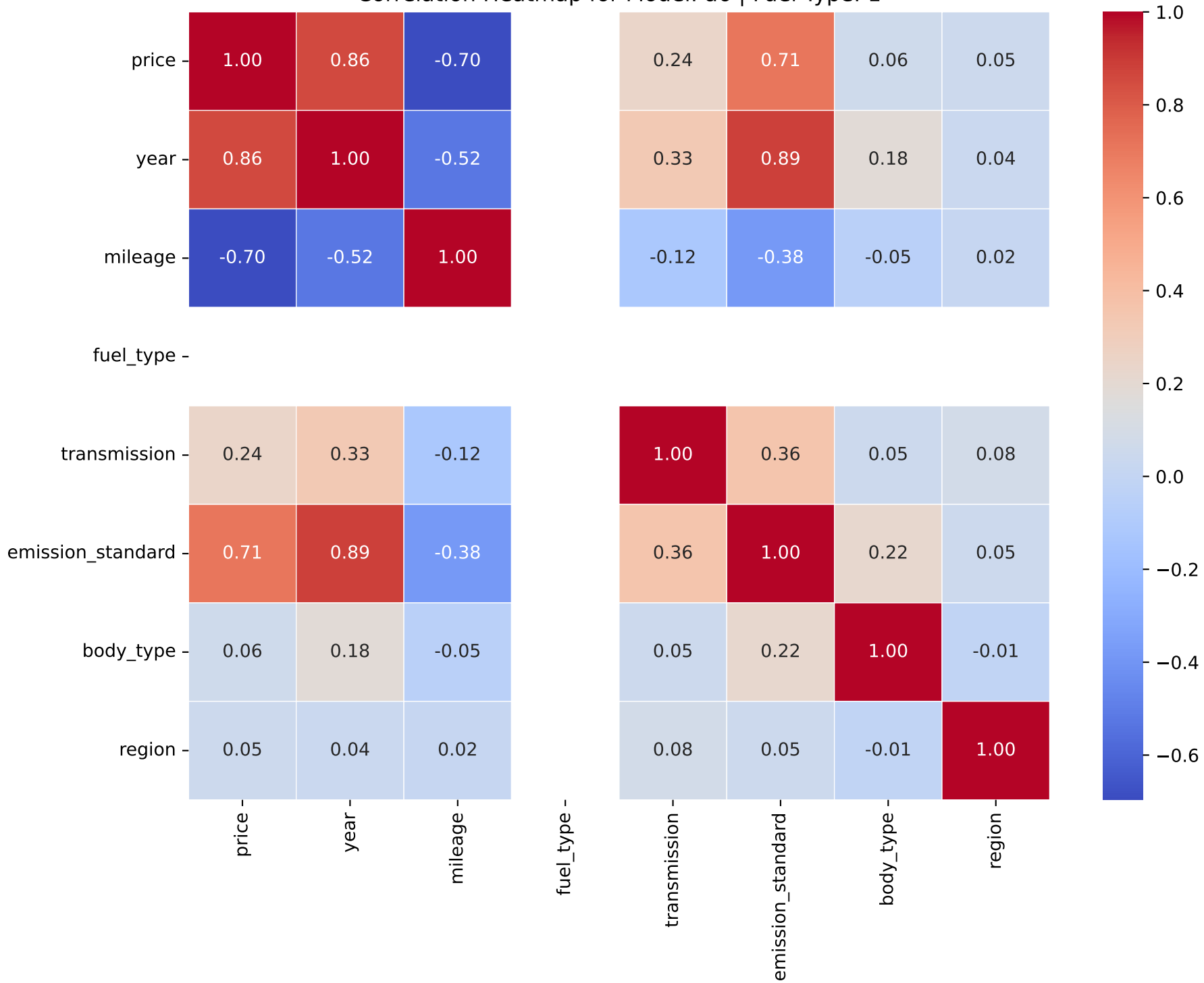
Correlation Heatmap for Model: a6 | Fuel Type: 1
