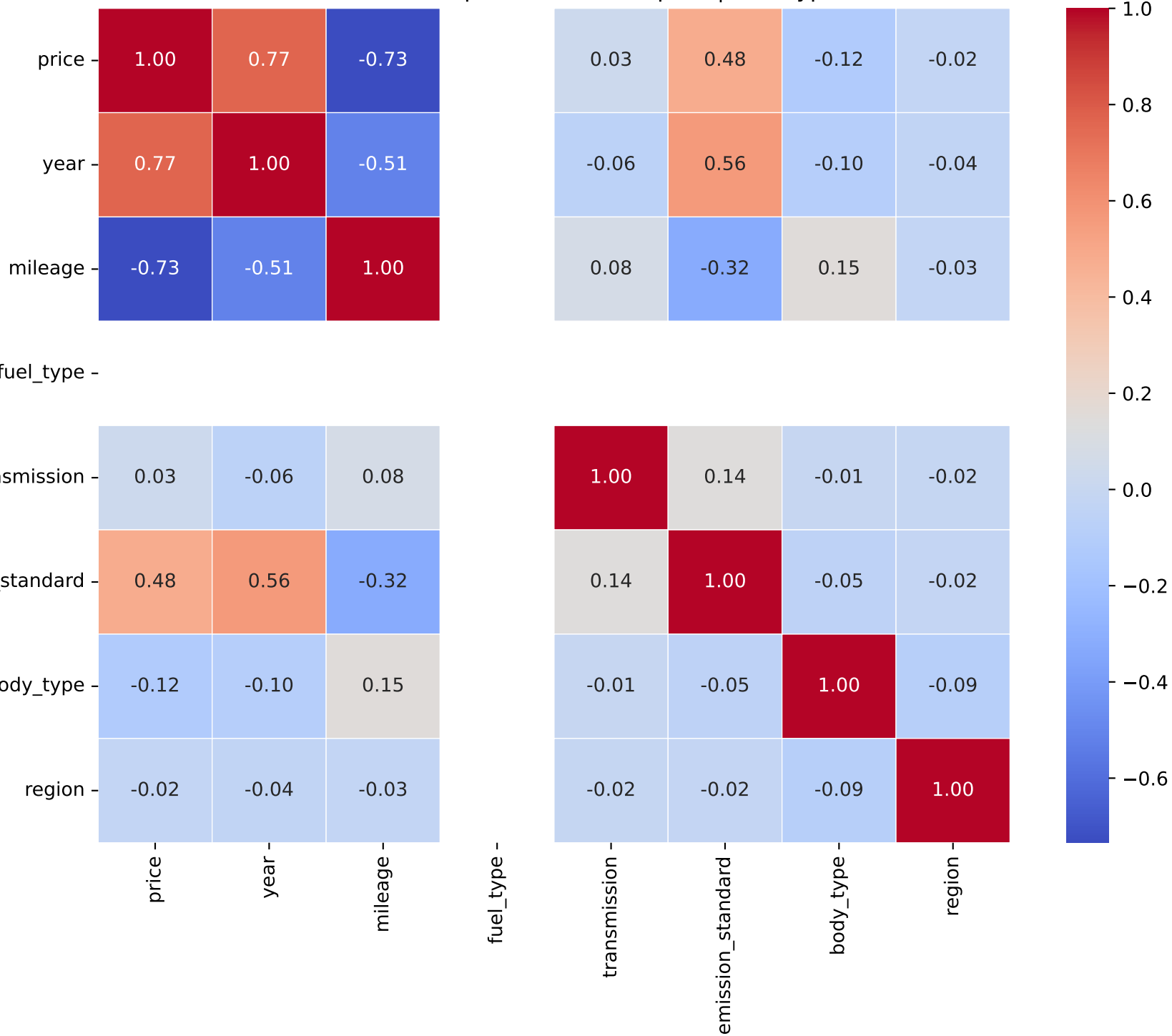
Correlation Heatmap for Model: compass | Fuel Type: 1
