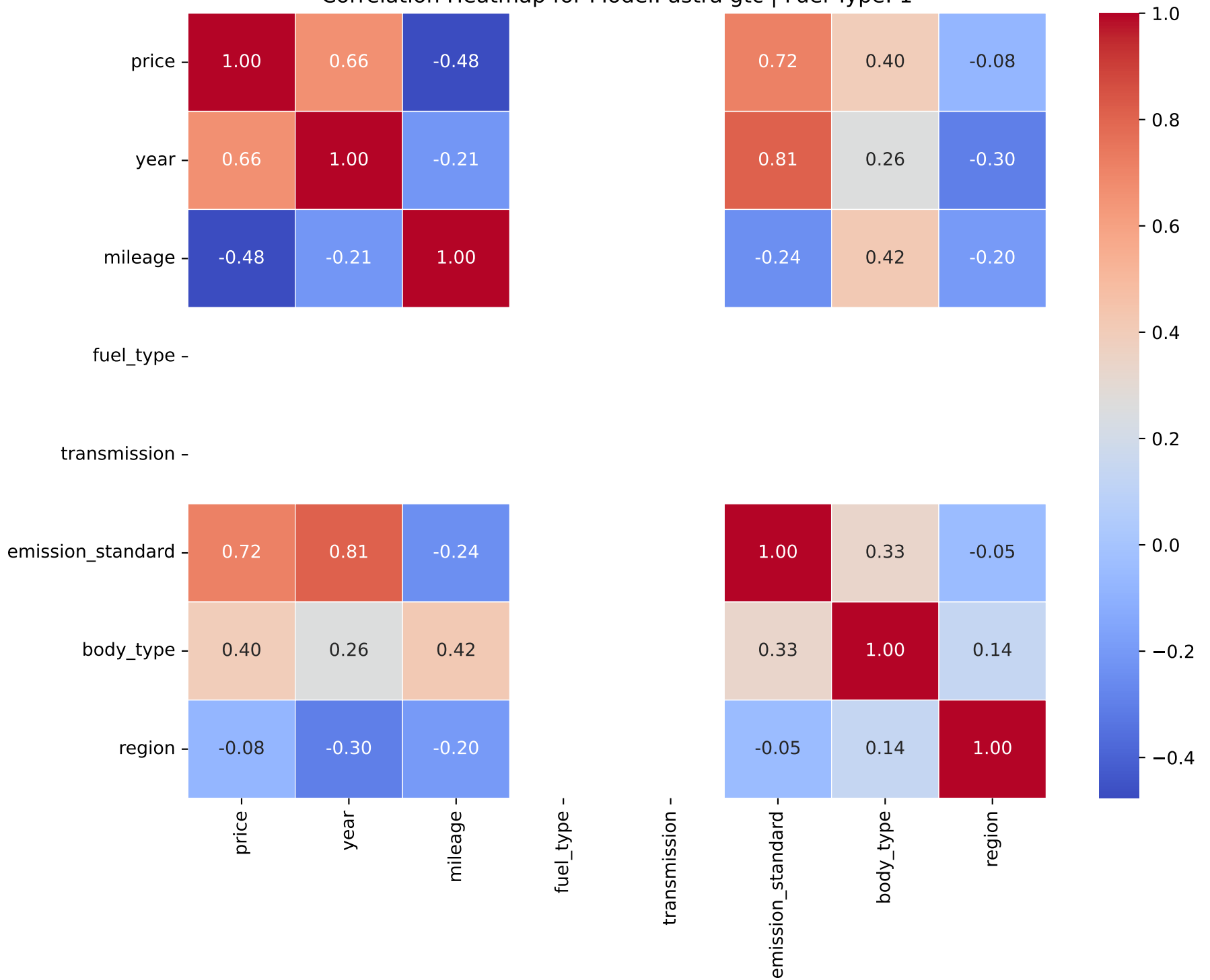
Correlation Heatmap for Model: astra gtc | Fuel Type: 1
