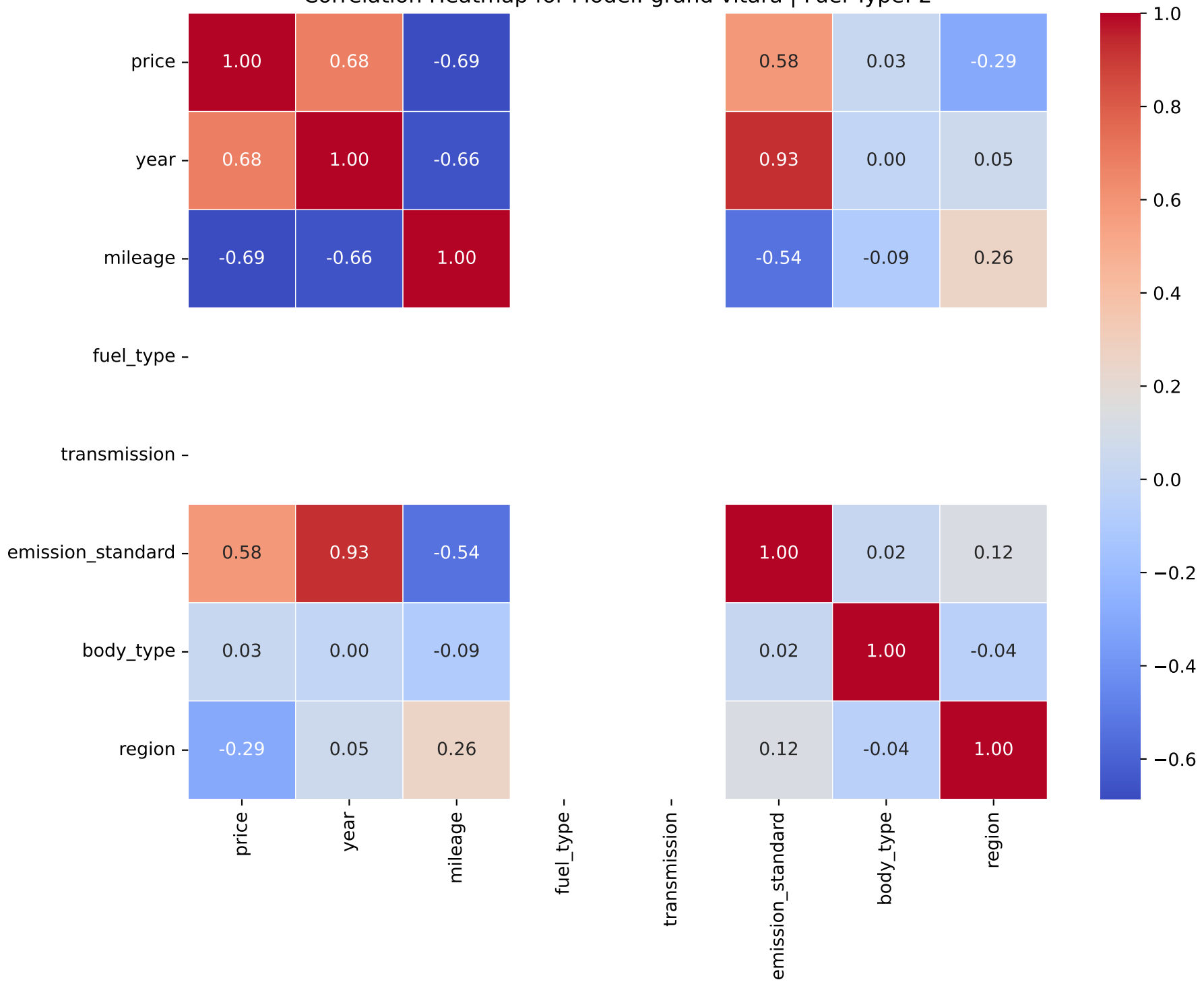
Correlation Heatmap for Model: grand vitara | Fuel Type: 2
