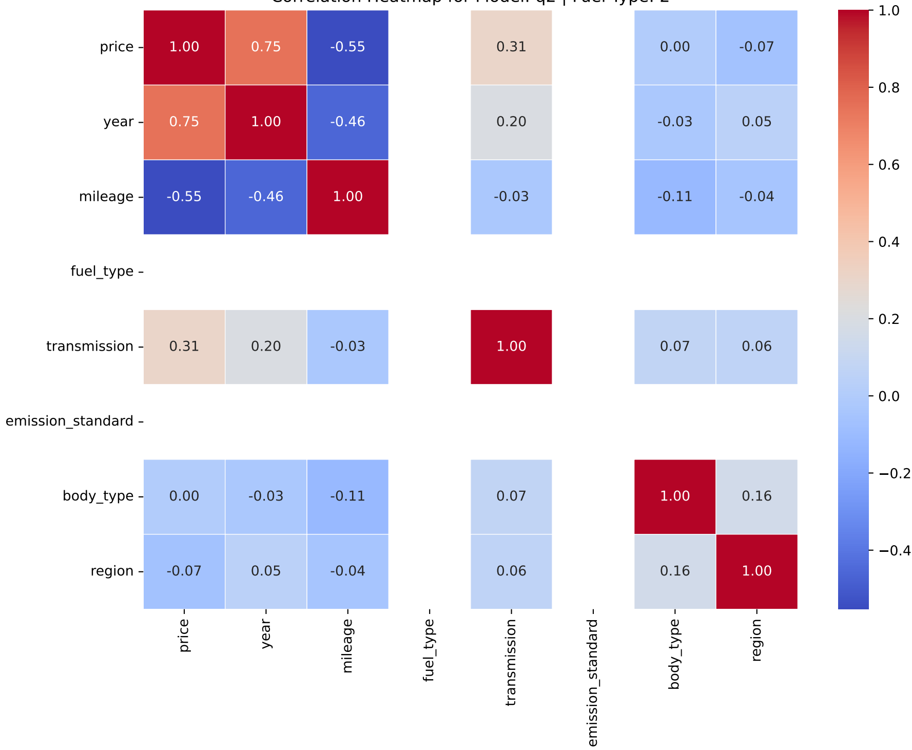
Correlation Heatmap for Model: q2 | Fuel Type: 2
