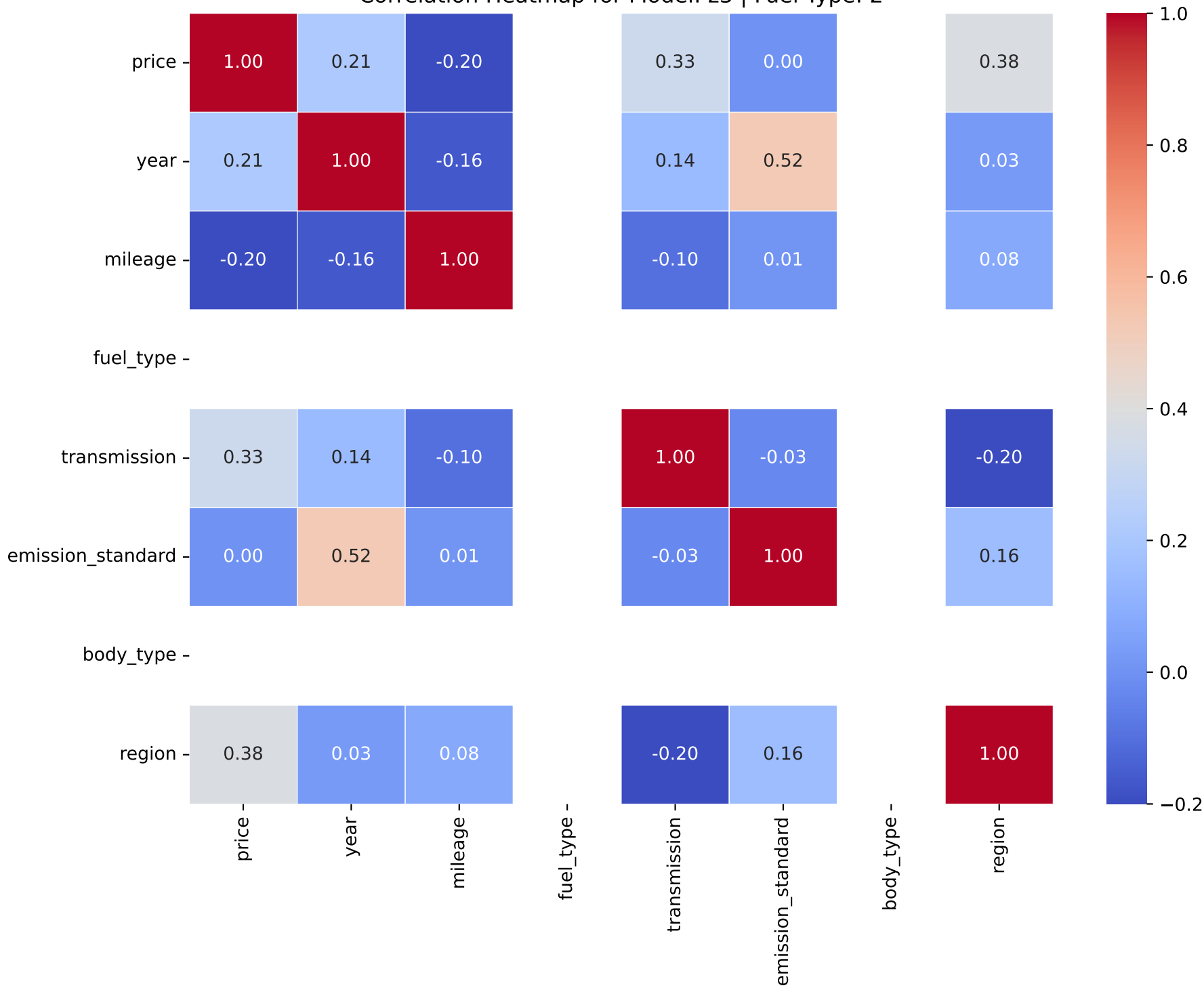
Correlation Heatmap for Model: z3 | Fuel Type: 2
