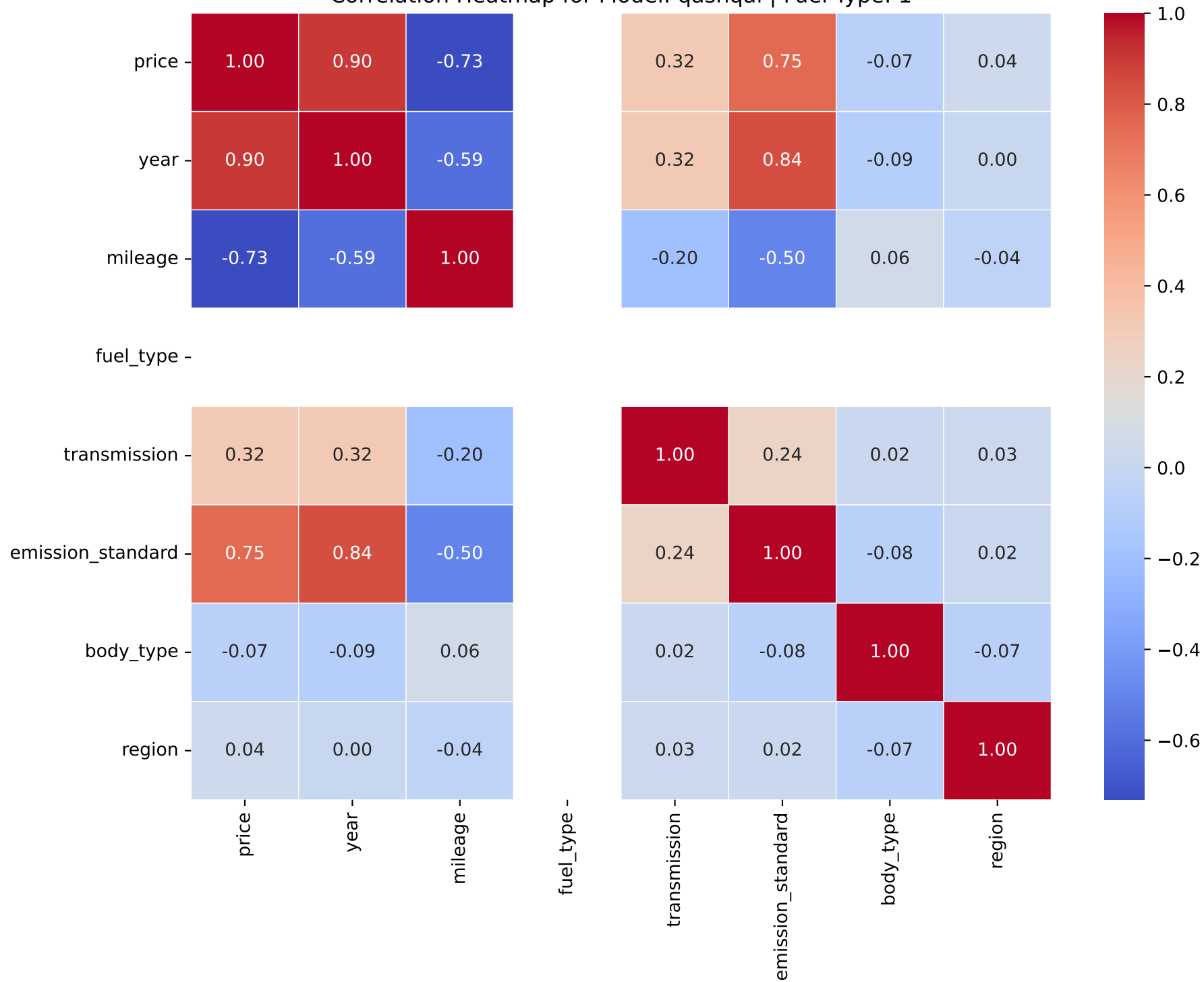
Correlation Heatmap for Model: qashqai | Fuel Type: 1
