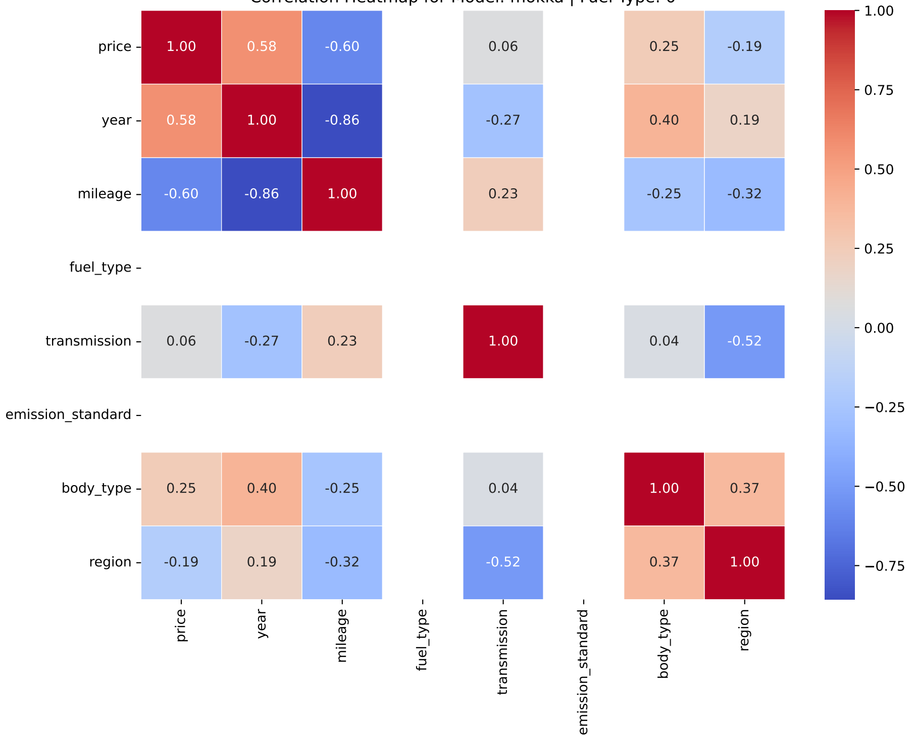
Correlation Heatmap for Model: mokka | Fuel Type: 0
