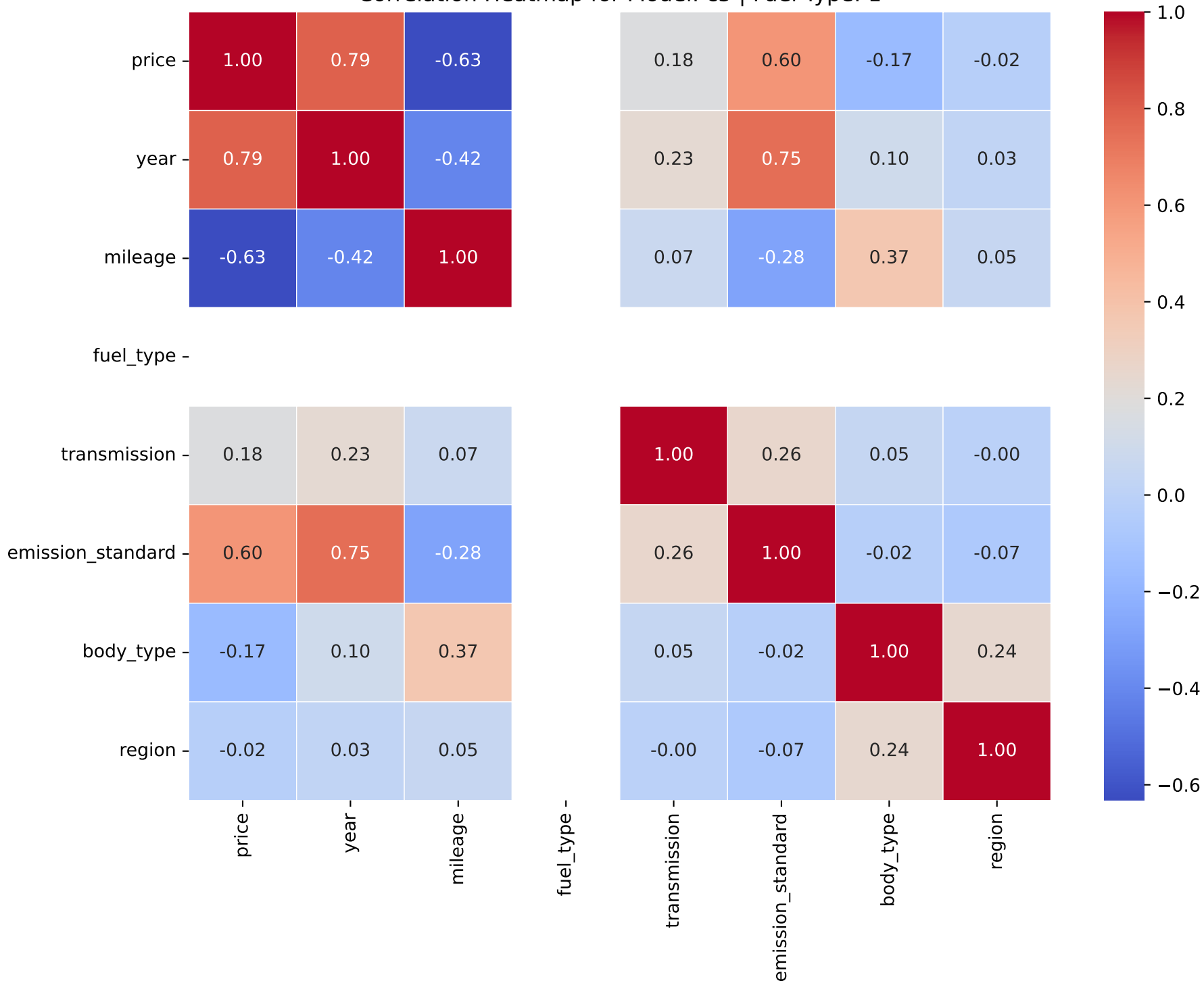
Correlation Heatmap for Model: c5 | Fuel Type: 1
