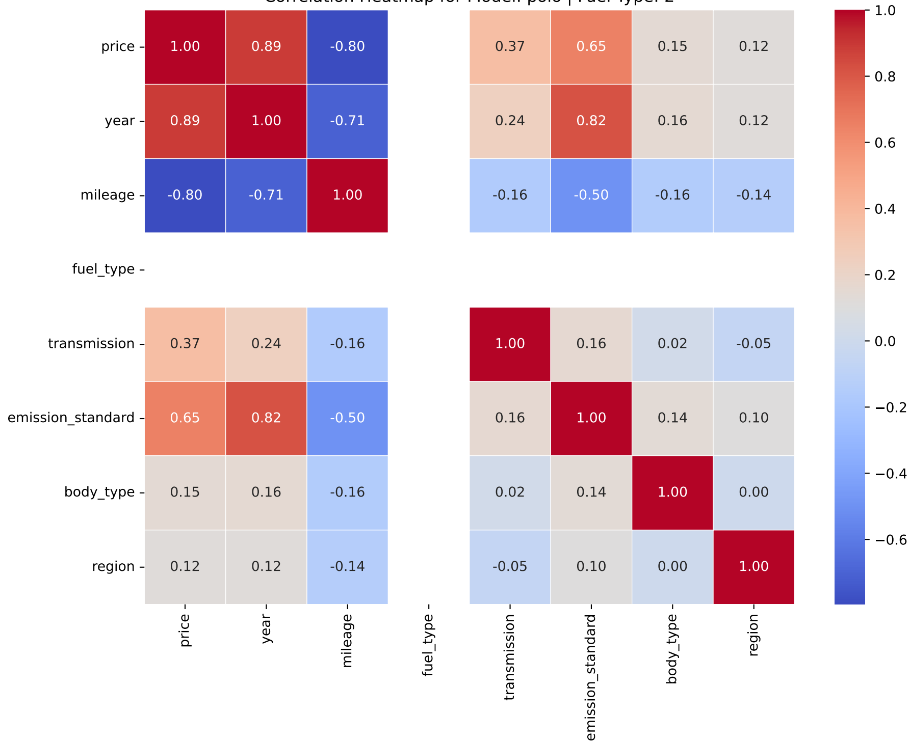
Correlation Heatmap for Model: polo | Fuel Type: 2
