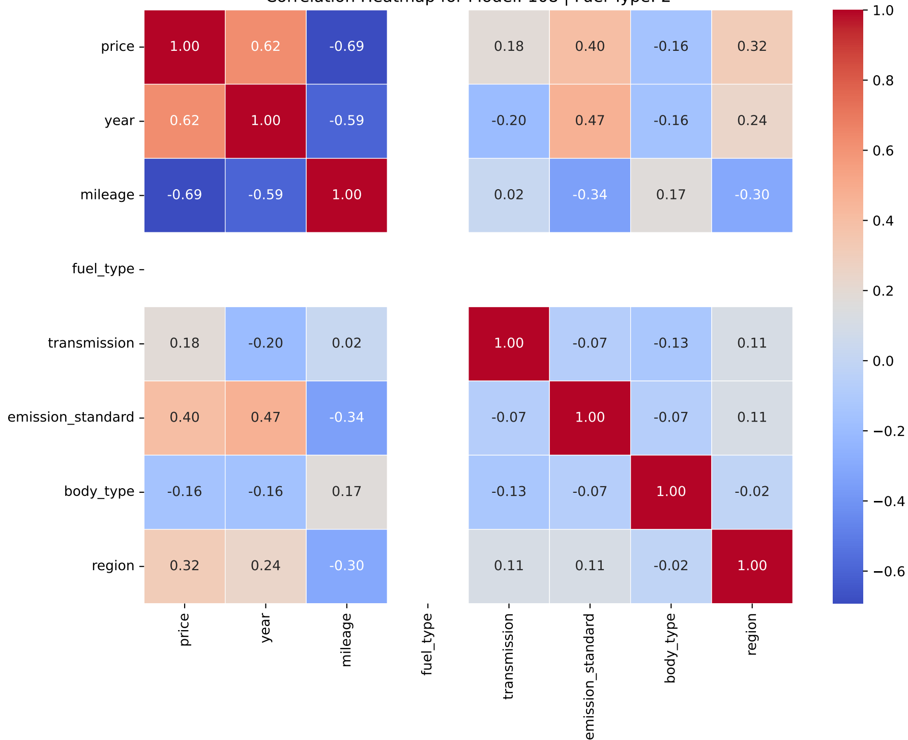
Correlation Heatmap for Model: 108 | Fuel Type: 2
