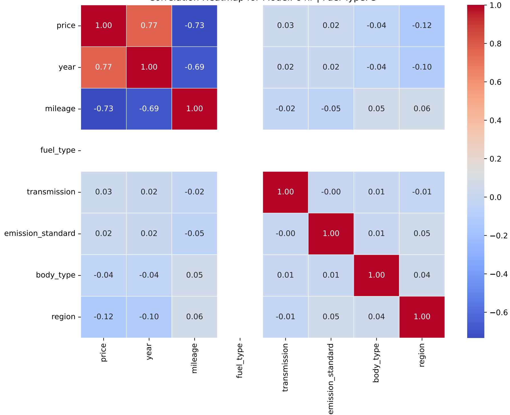
Correlation Heatmap for Model: c-hr | Fuel Type: 3
