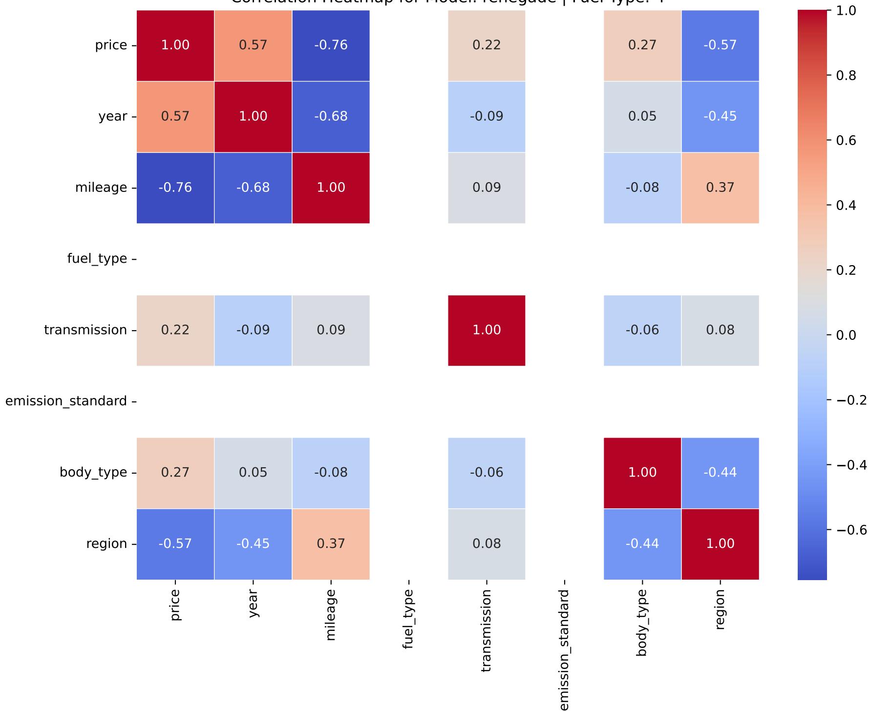
Correlation Heatmap for Model: renegade | Fuel Type: 4
