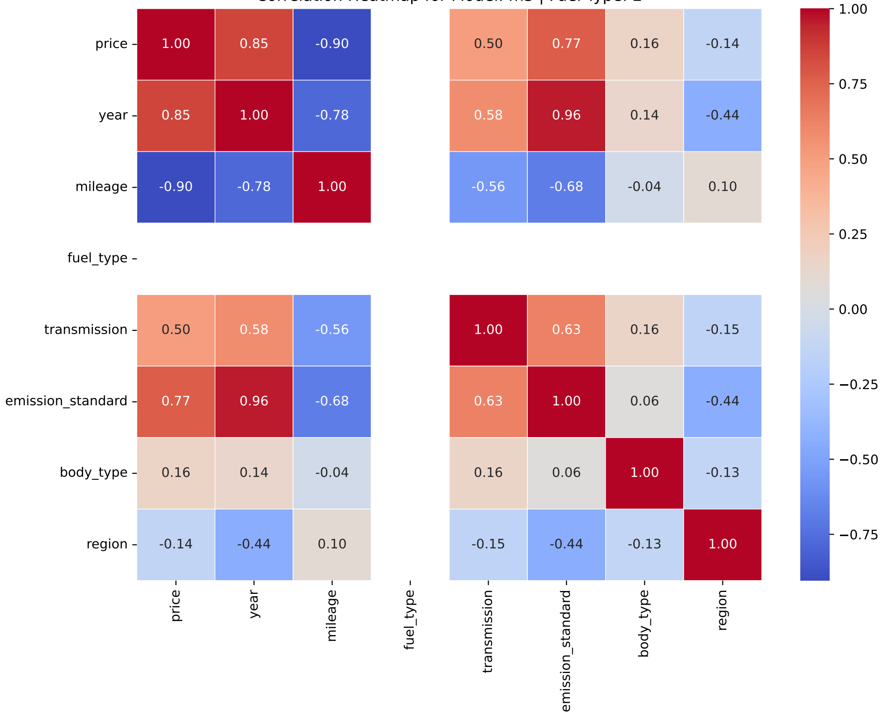
Correlation Heatmap for Model: m3 | Fuel Type: 2
