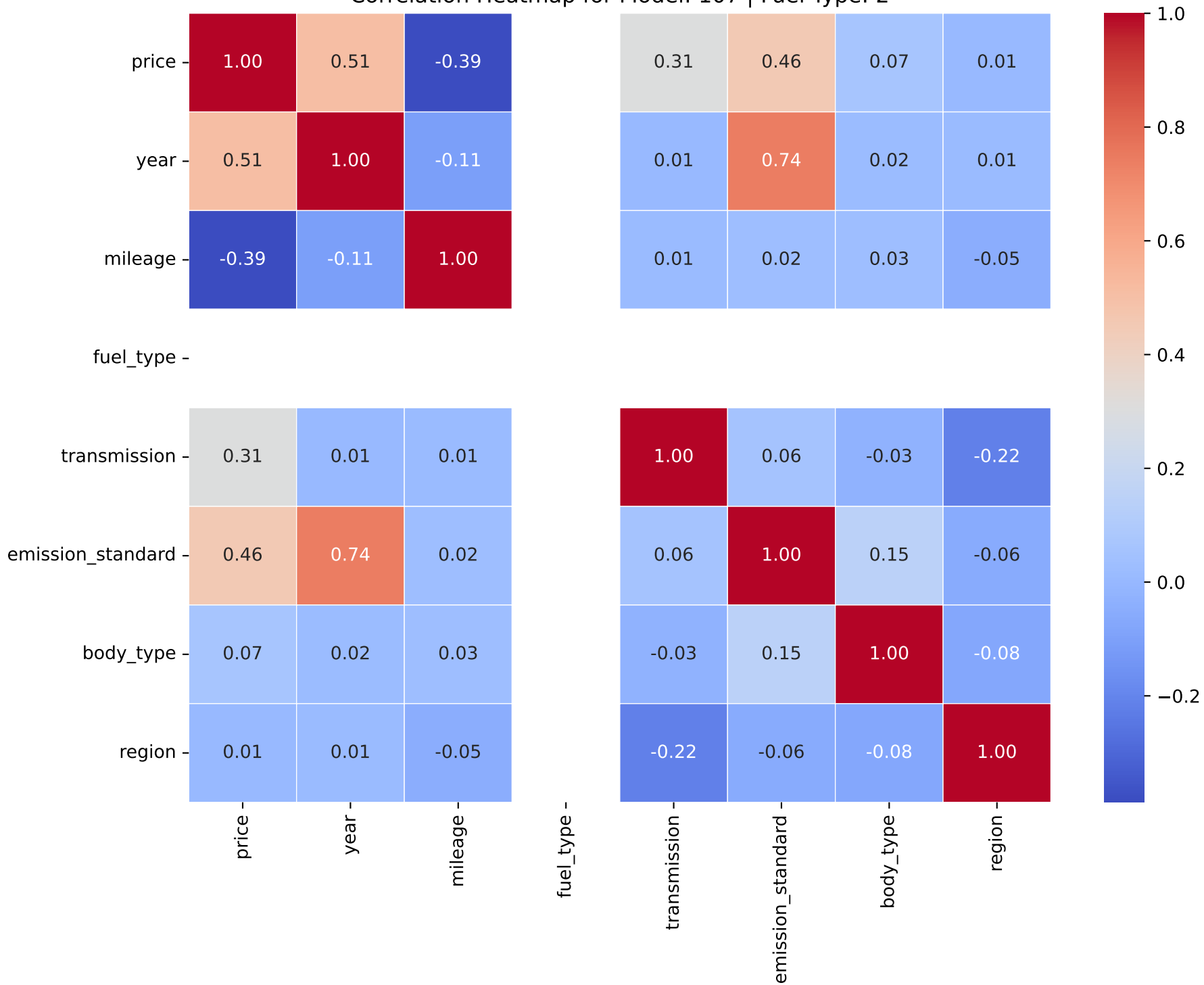
Correlation Heatmap for Model: 107 | Fuel Type: 2
