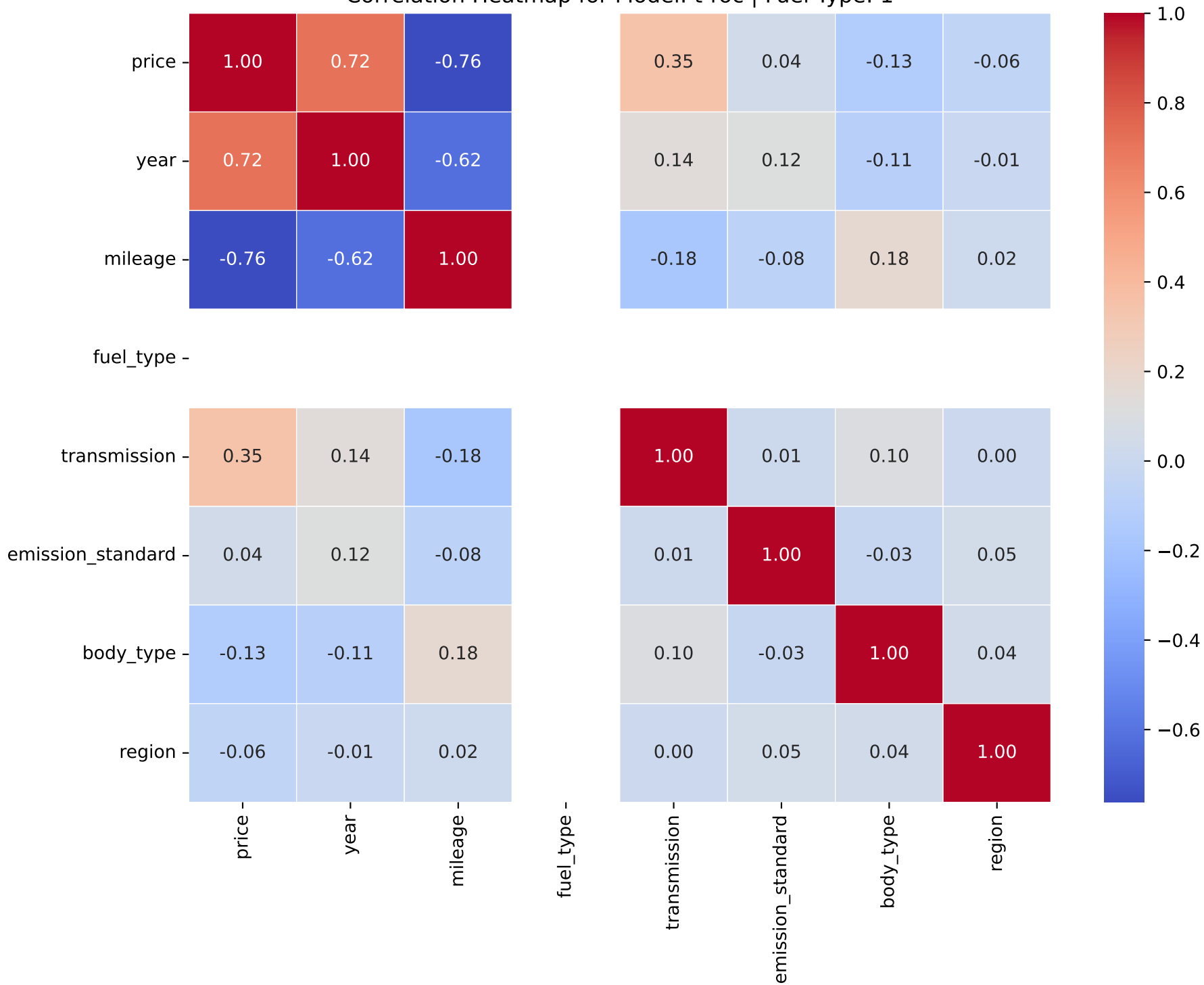
Correlation Heatmap for Model: t-roc | Fuel Type: 1
