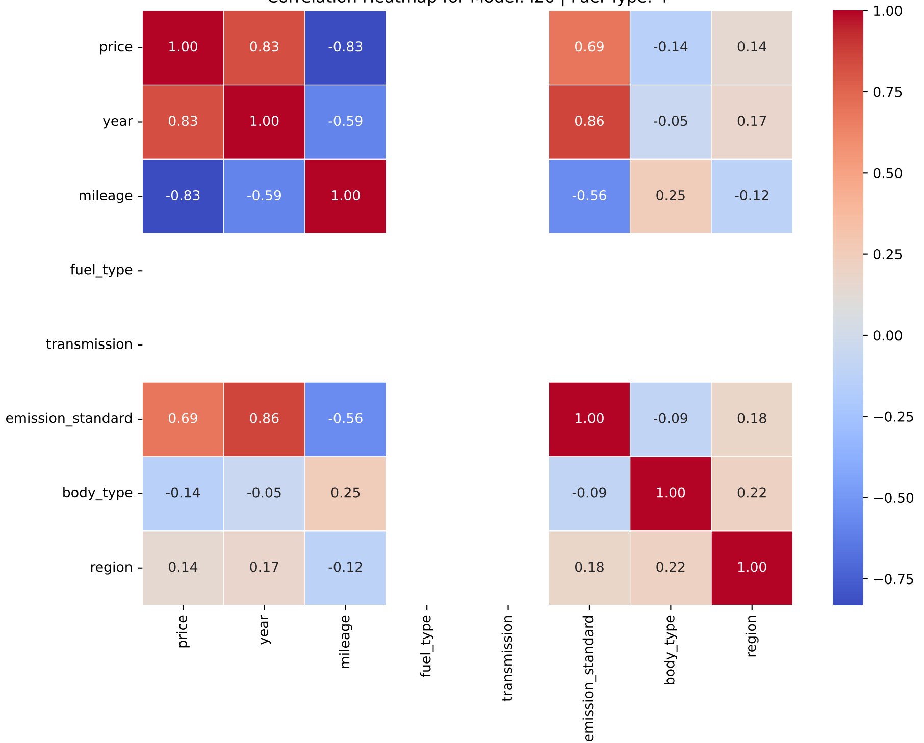
Correlation Heatmap for Model: i20 | Fuel Type: 4
