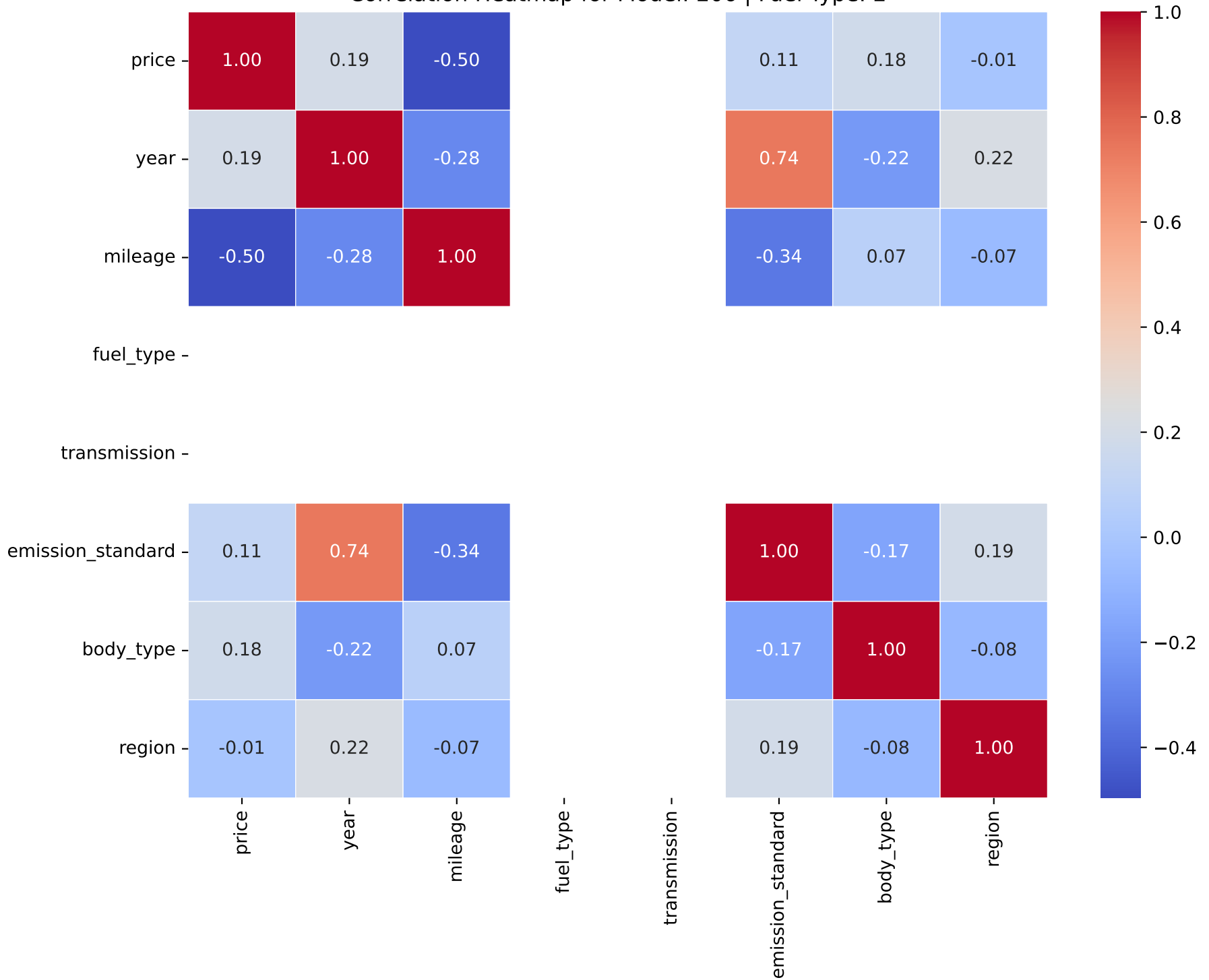
Correlation Heatmap for Model: 206 | Fuel Type: 2
