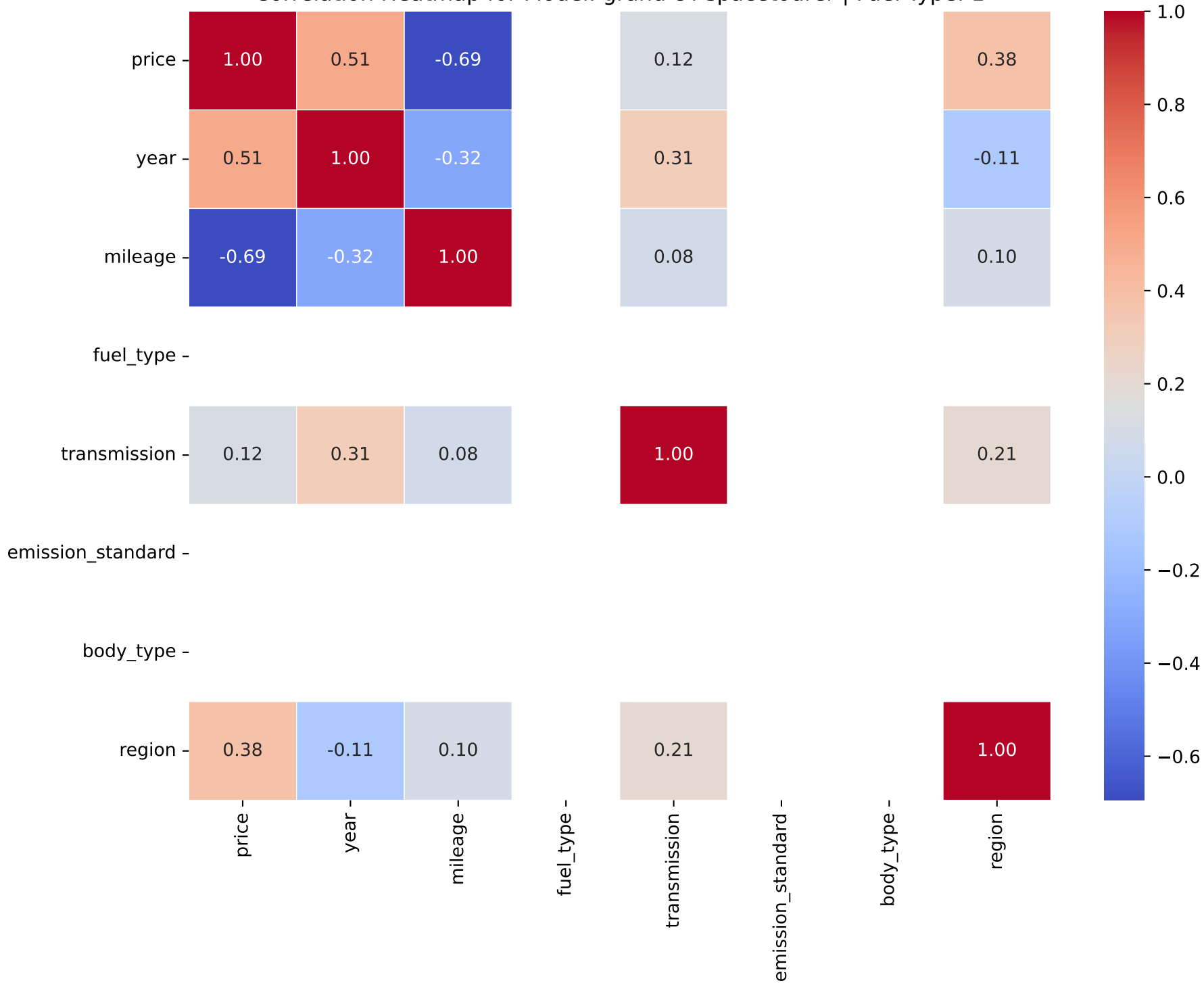
Correlation Heatmap for Model: grand c4 spacetourer | Fuel Type: 1
