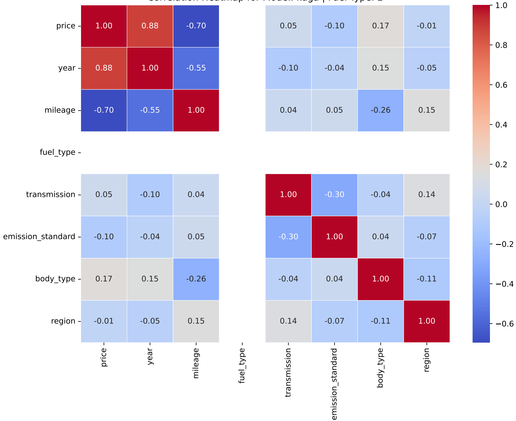
Correlation Heatmap for Model: kuga | Fuel Type: 2
