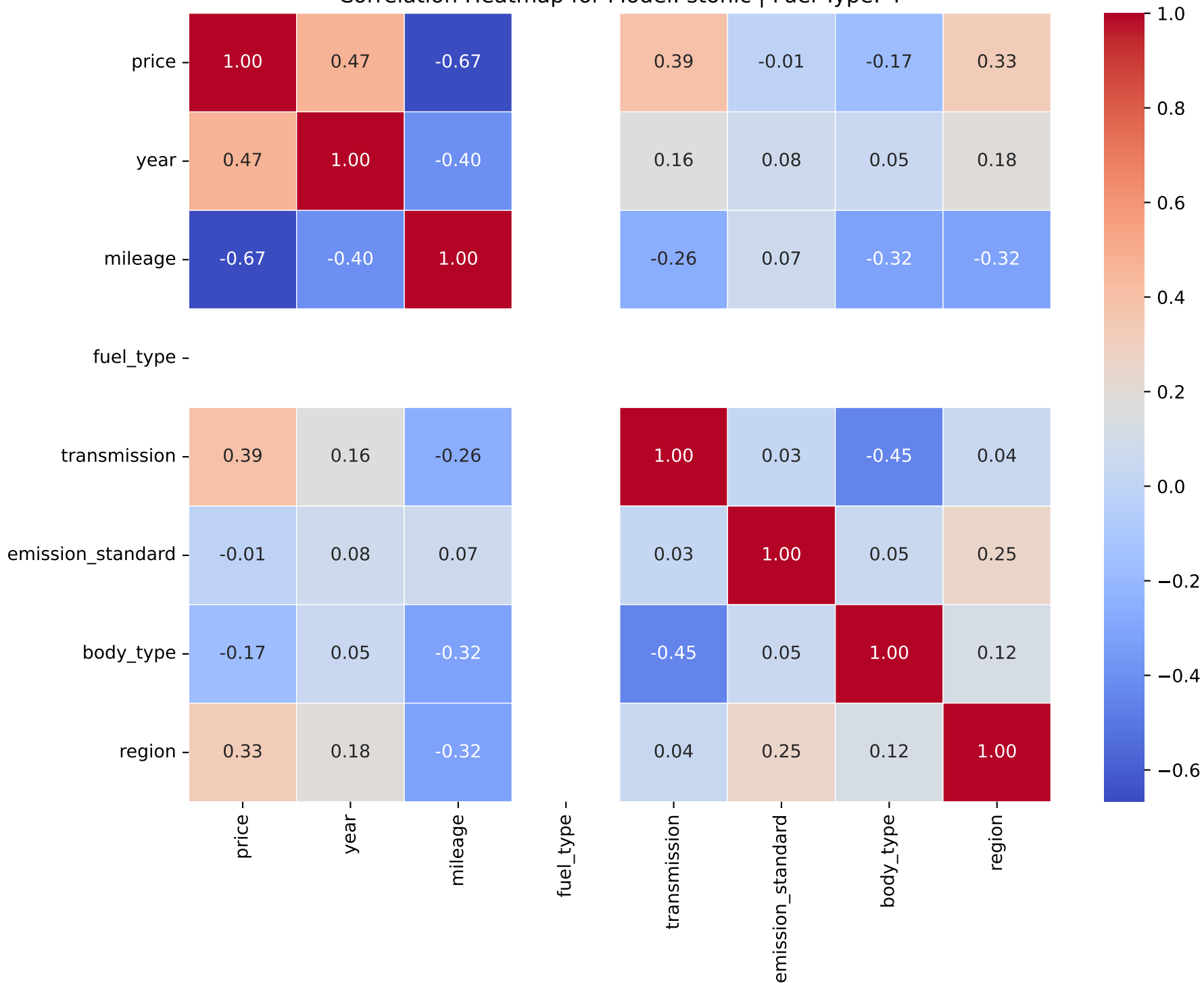
Correlation Heatmap for Model: stonic | Fuel Type: 4
