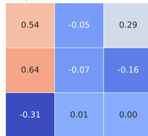
Correlation Heatmap for Model: multipla | Fuel Type: 1
