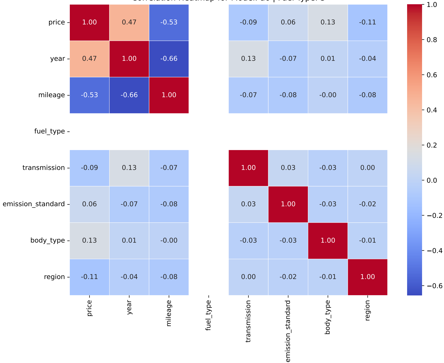
Correlation Heatmap for Model: a6 | Fuel Type: 3
