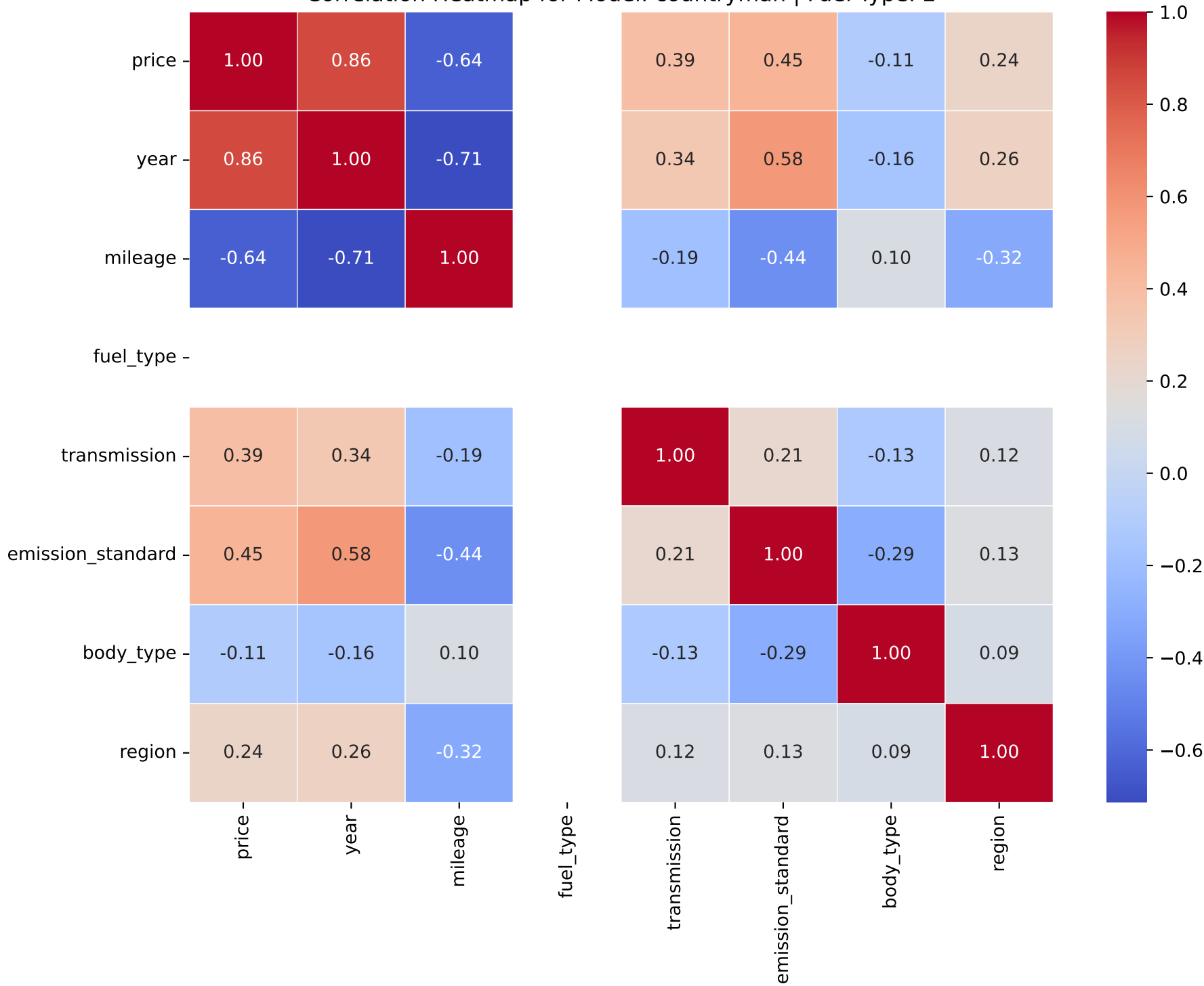
Correlation Heatmap for Model: countryman | Fuel Type: 2
