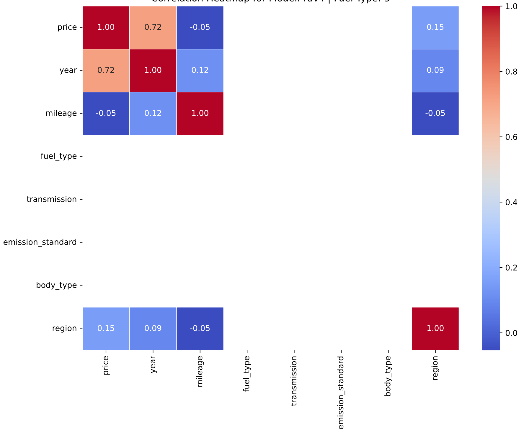
Correlation Heatmap for Model: rav4 | Fuel Type: 3
