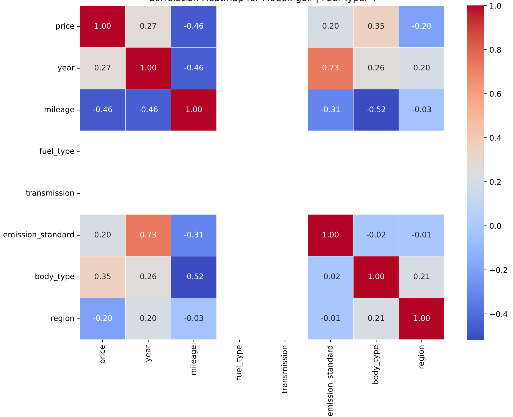
Correlation Heatmap for Model: golf | Fuel Type: 4
