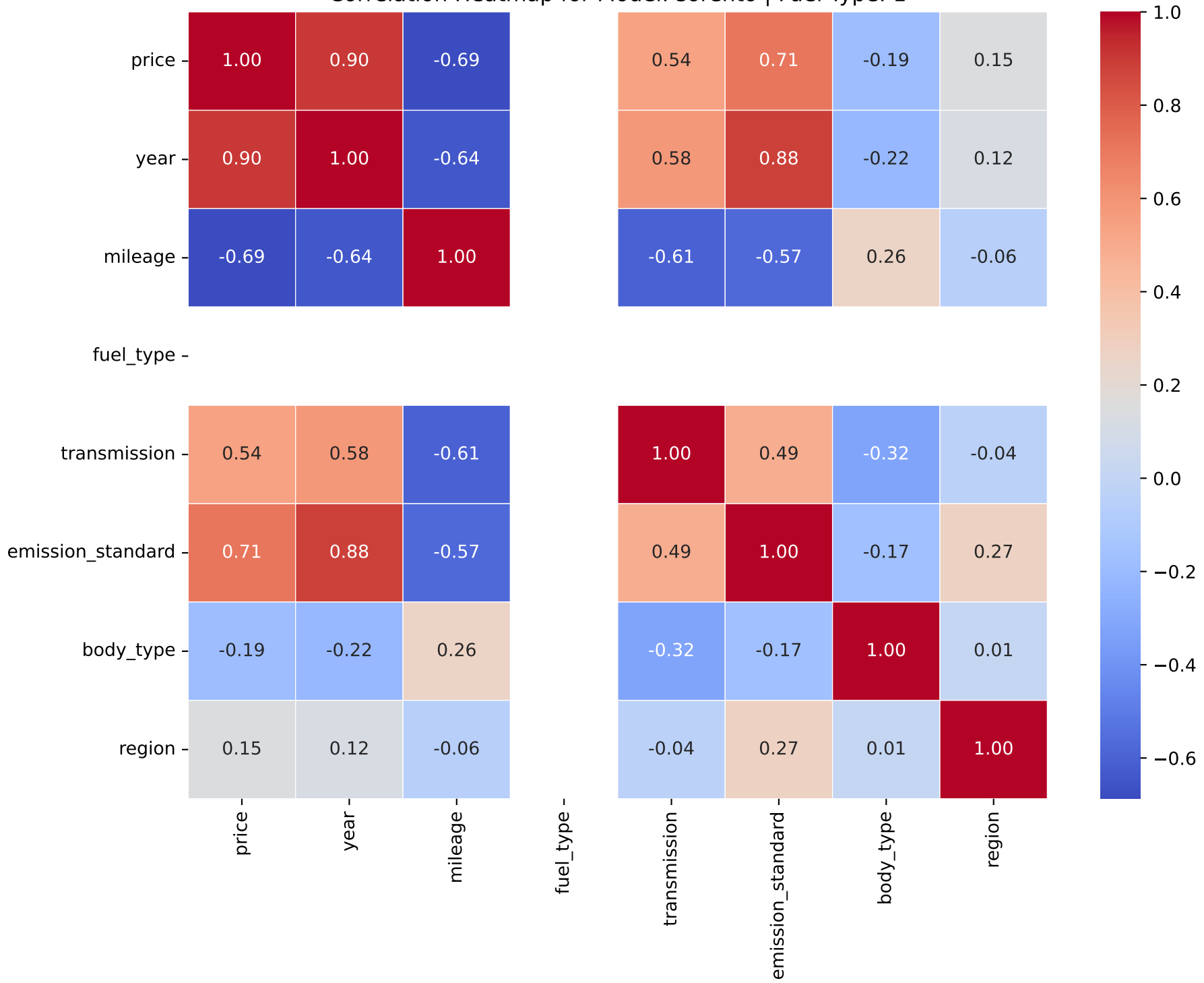
Correlation Heatmap for Model: sorento | Fuel Type: 1
