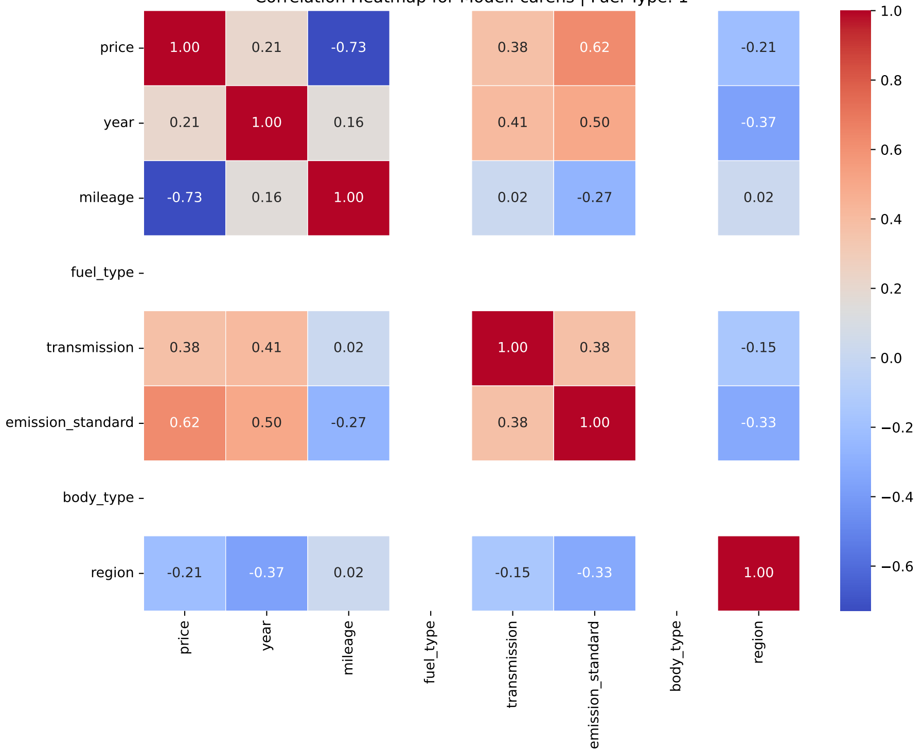
Correlation Heatmap for Model: carens | Fuel Type: 1
