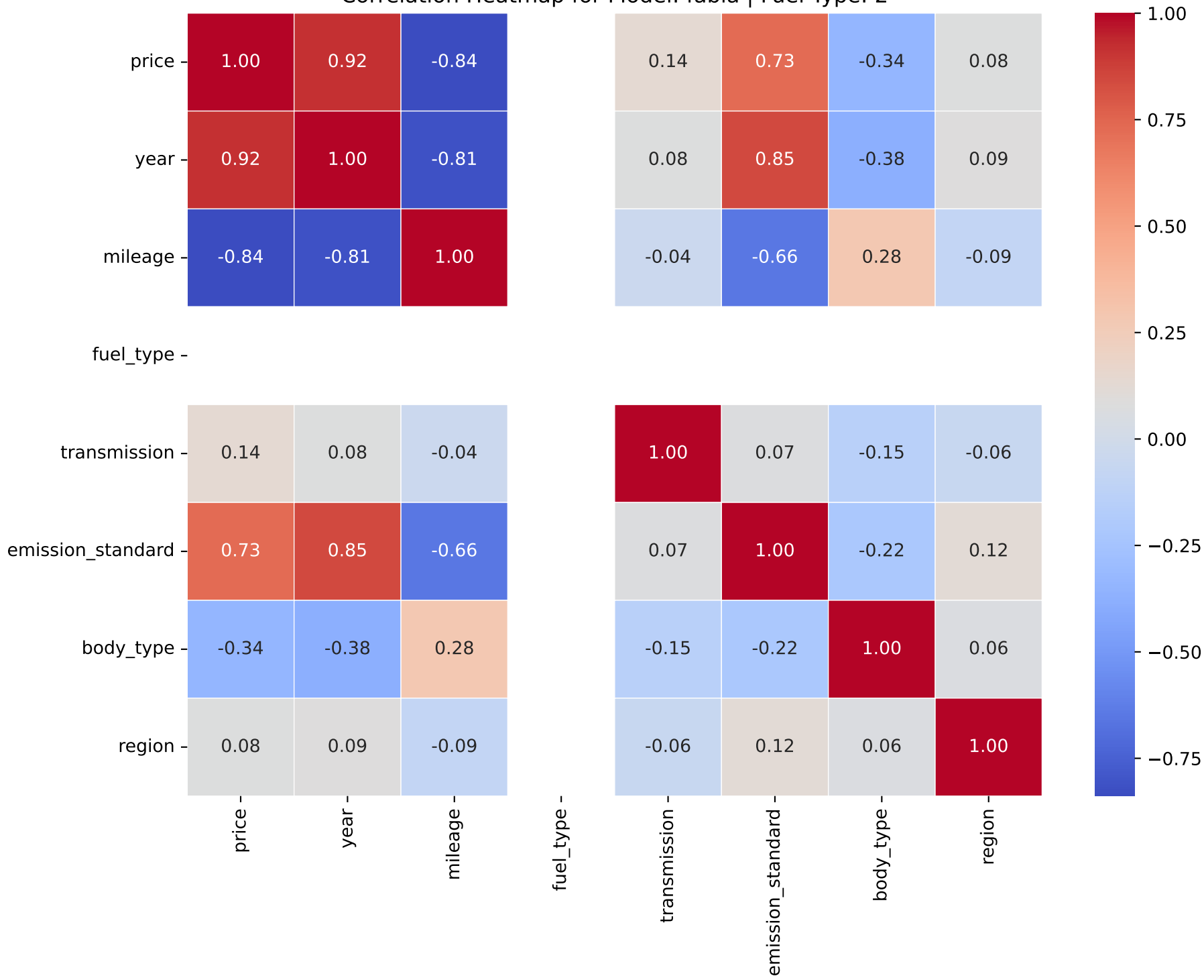
Correlation Heatmap for Model: fabia | Fuel Type: 2
