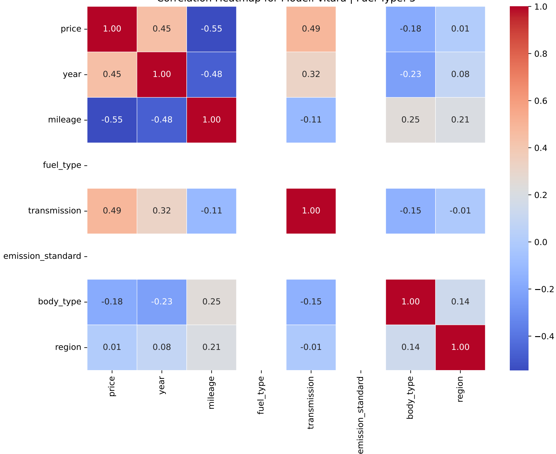
Correlation Heatmap for Model: vitara | Fuel Type: 3
