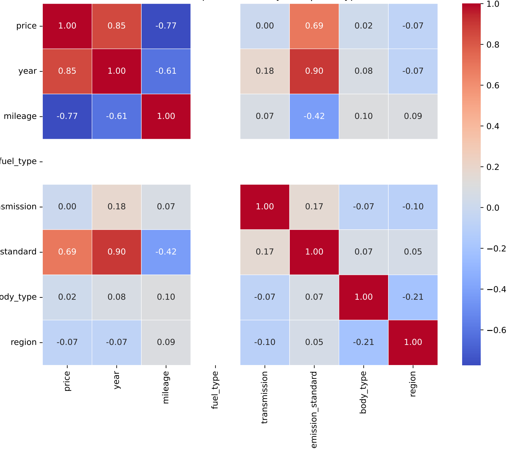
Correlation Heatmap for Model: cayenne | Fuel Type: 2
