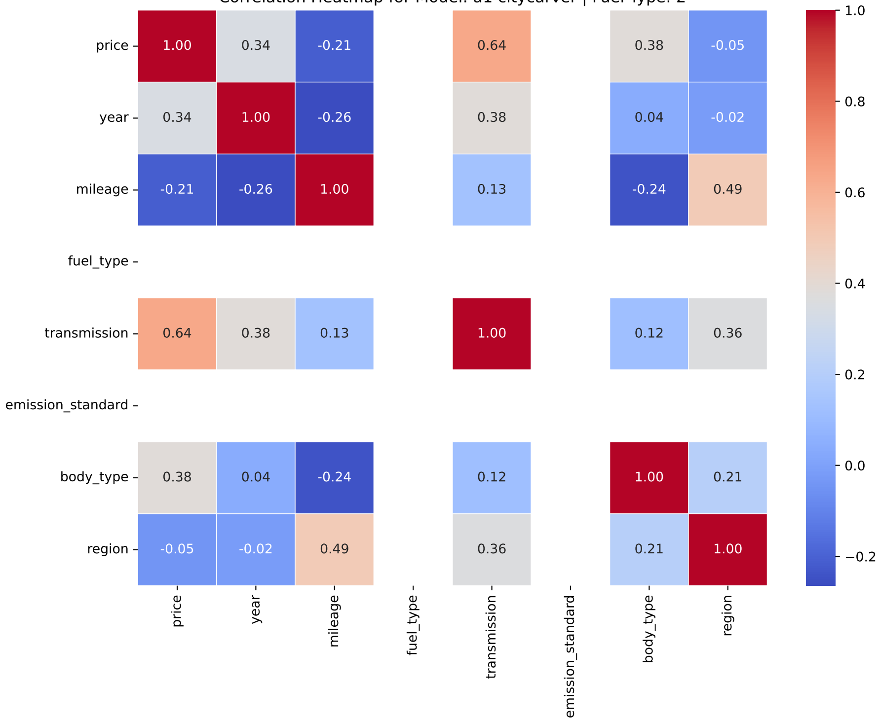
Correlation Heatmap for Model: a1 citycarver | Fuel Type: 2
