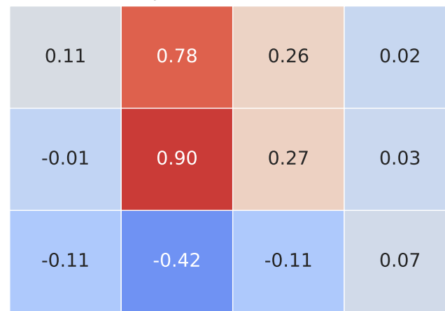
Correlation Heatmap for Model: micra | Fuel Type: 2
