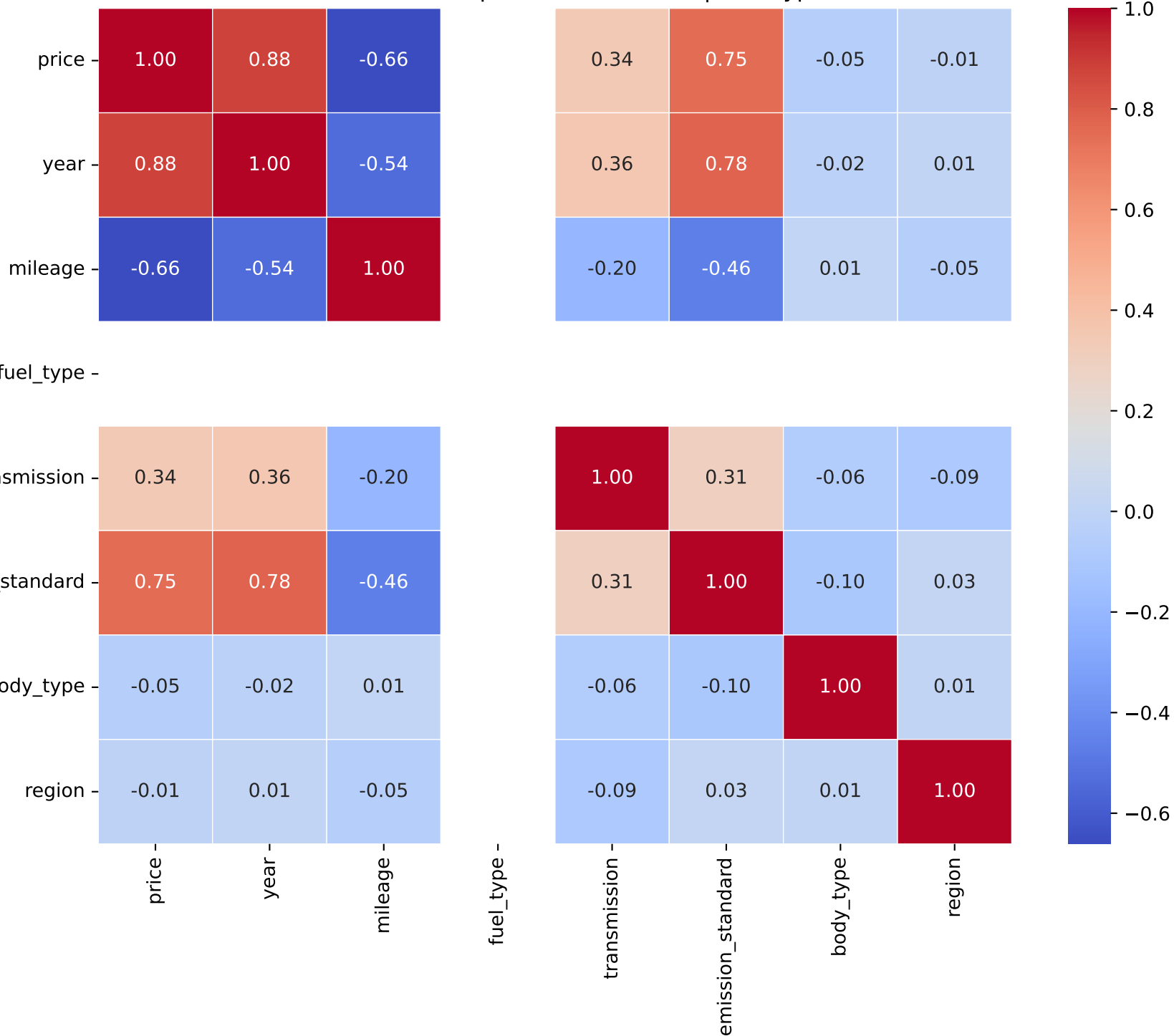
Correlation Heatmap for Model: scenic | Fuel Type: 1
