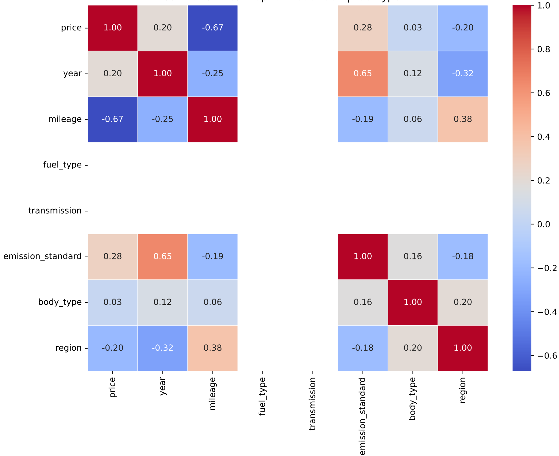
Correlation Heatmap for Model: 307 | Fuel Type: 1
