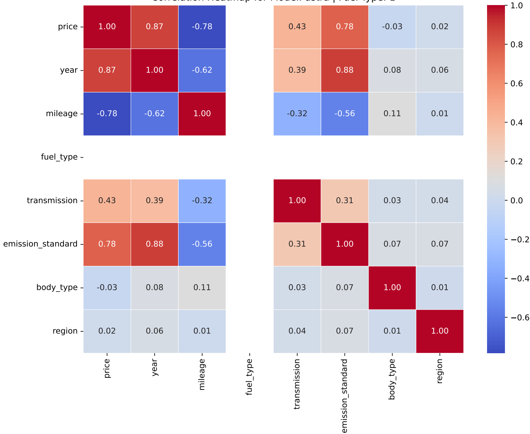
Correlation Heatmap for Model: astra | Fuel Type: 1
