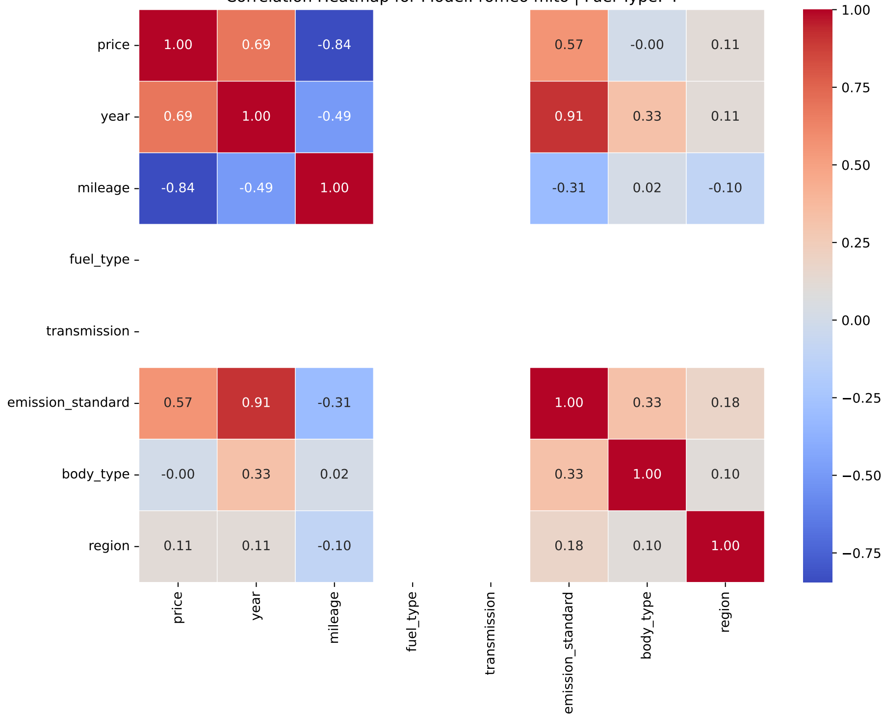
Correlation Heatmap for Model: romeo mito | Fuel Type: 4
