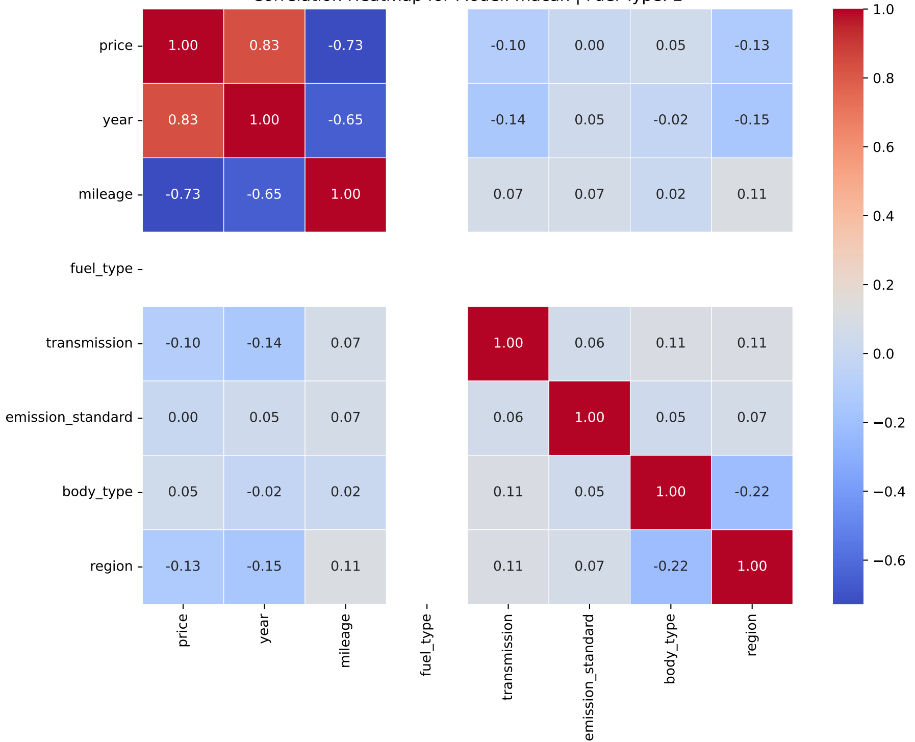
Correlation Heatmap for Model: macan | Fuel Type: 2
