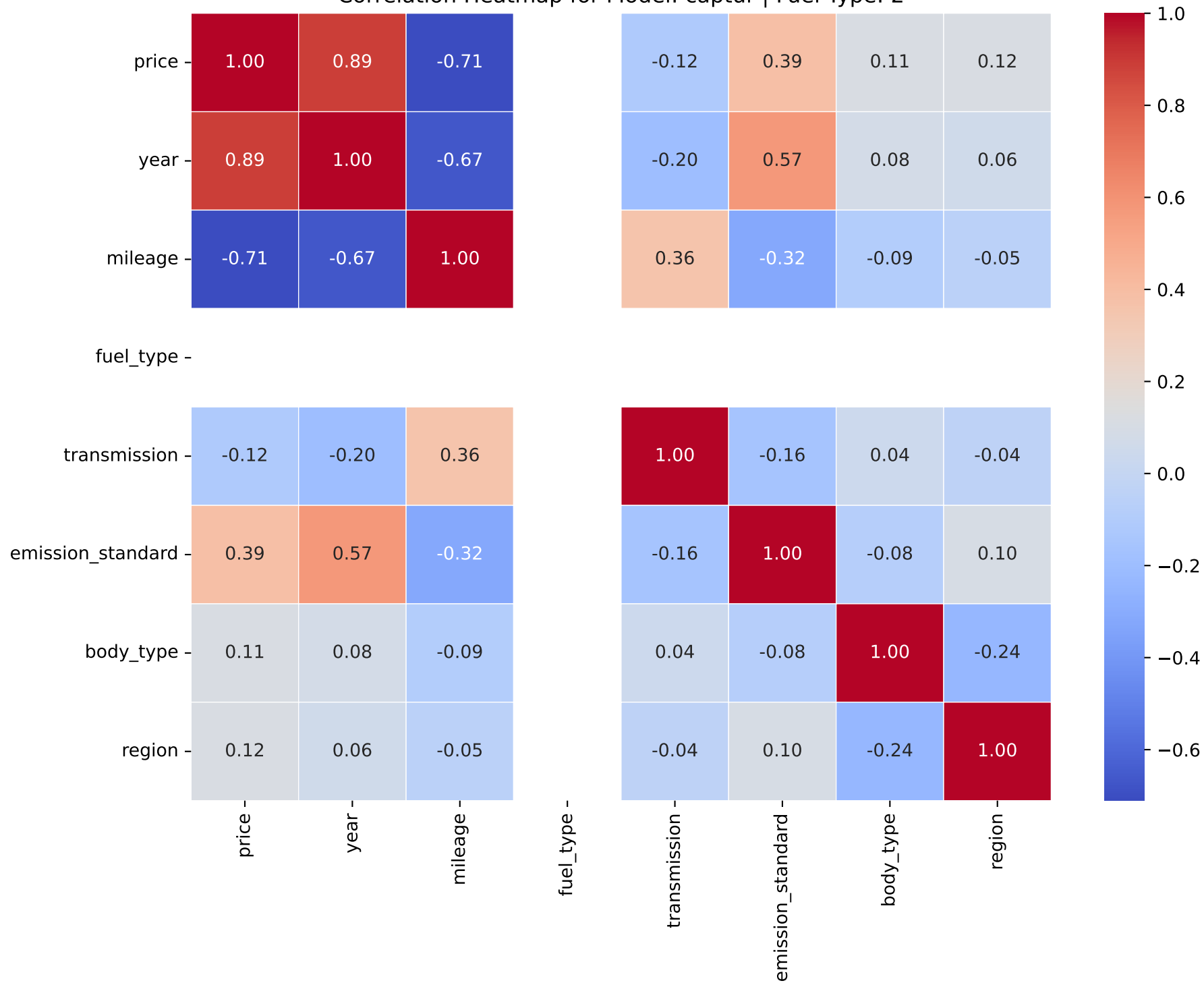
Correlation Heatmap for Model: captur | Fuel Type: 2
