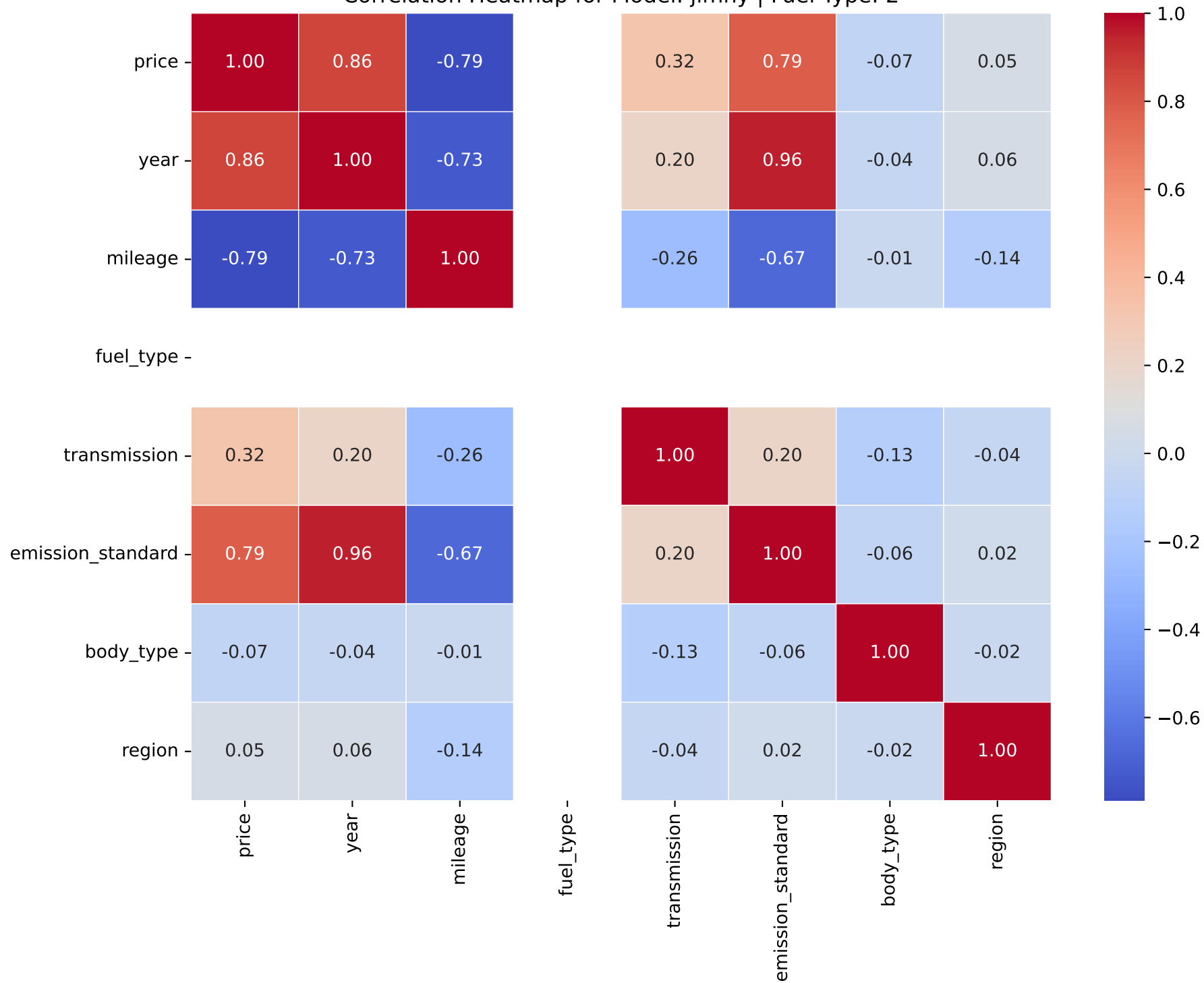
Correlation Heatmap for Model: jimny | Fuel Type: 2
