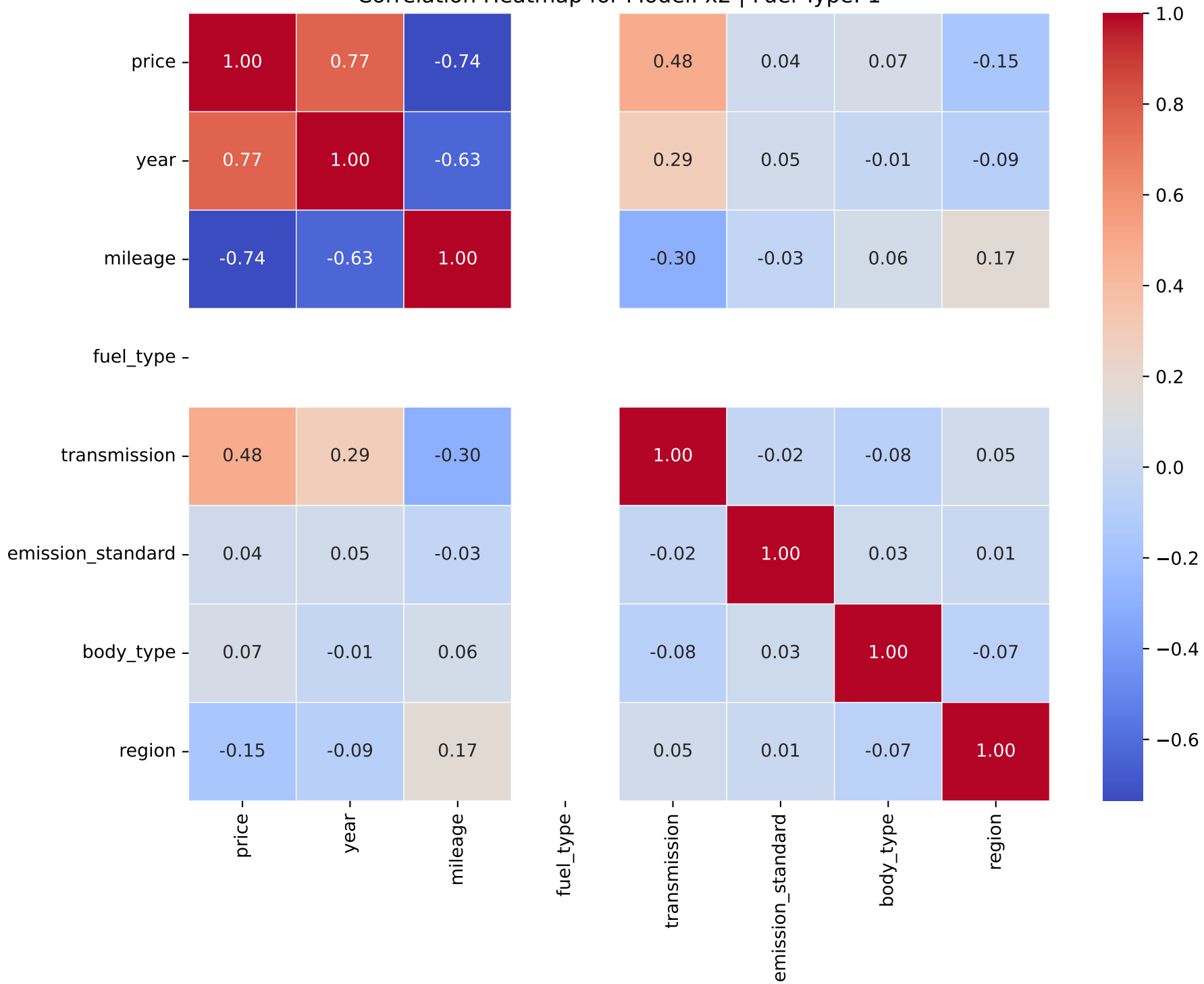
Correlation Heatmap for Model: x2 | Fuel Type: 1
