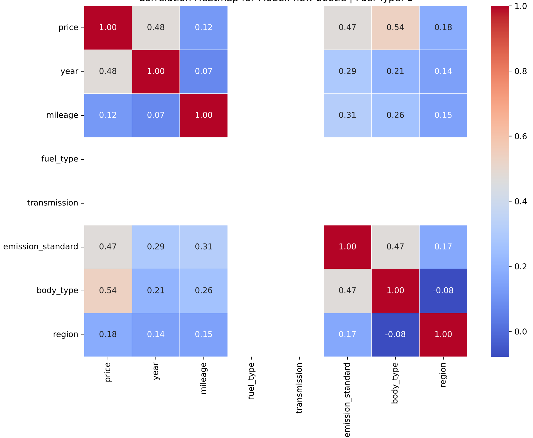
Correlation Heatmap for Model: new beetle | Fuel Type: 1
