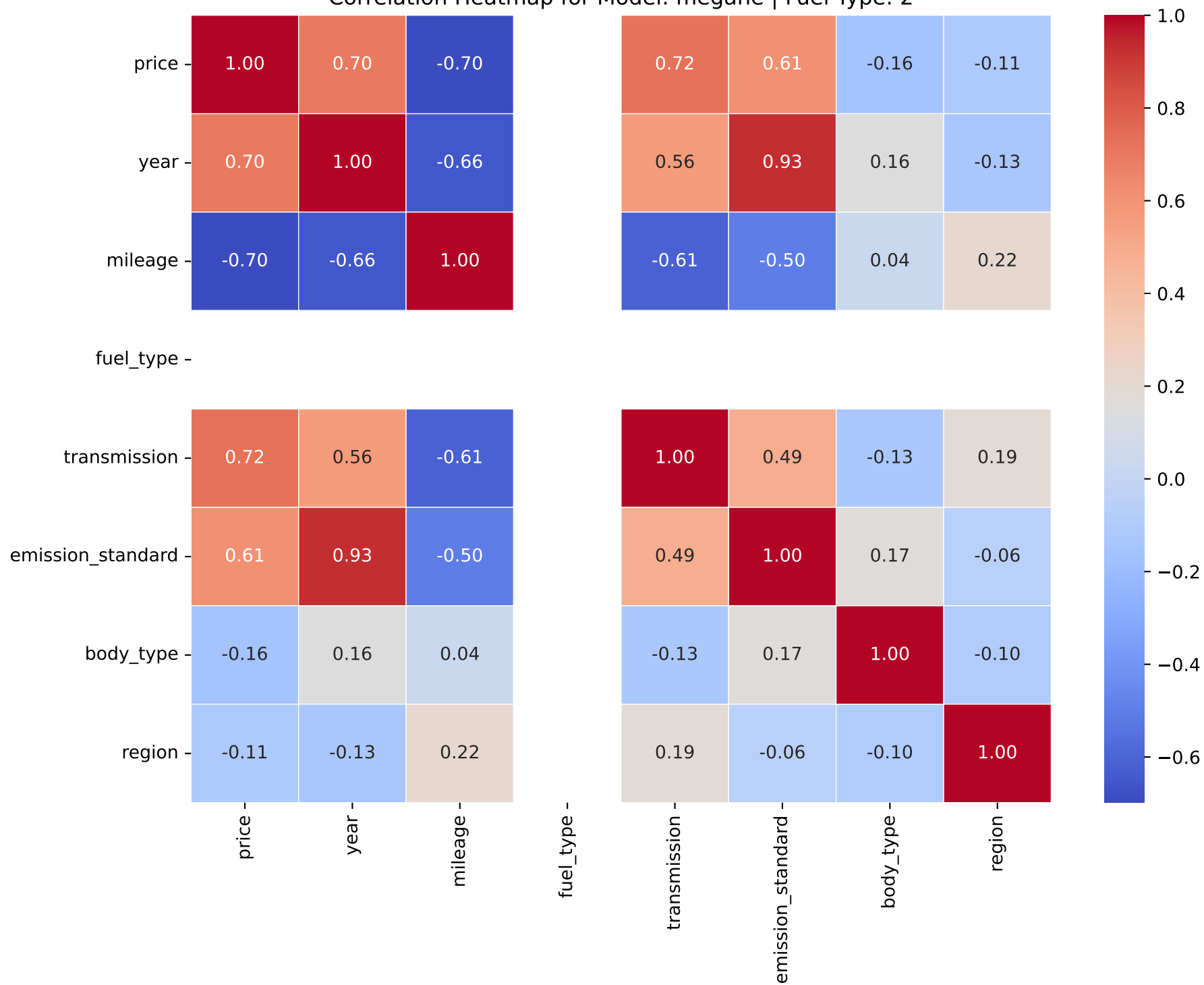
Correlation Heatmap for Model: megane | Fuel Type: 2
