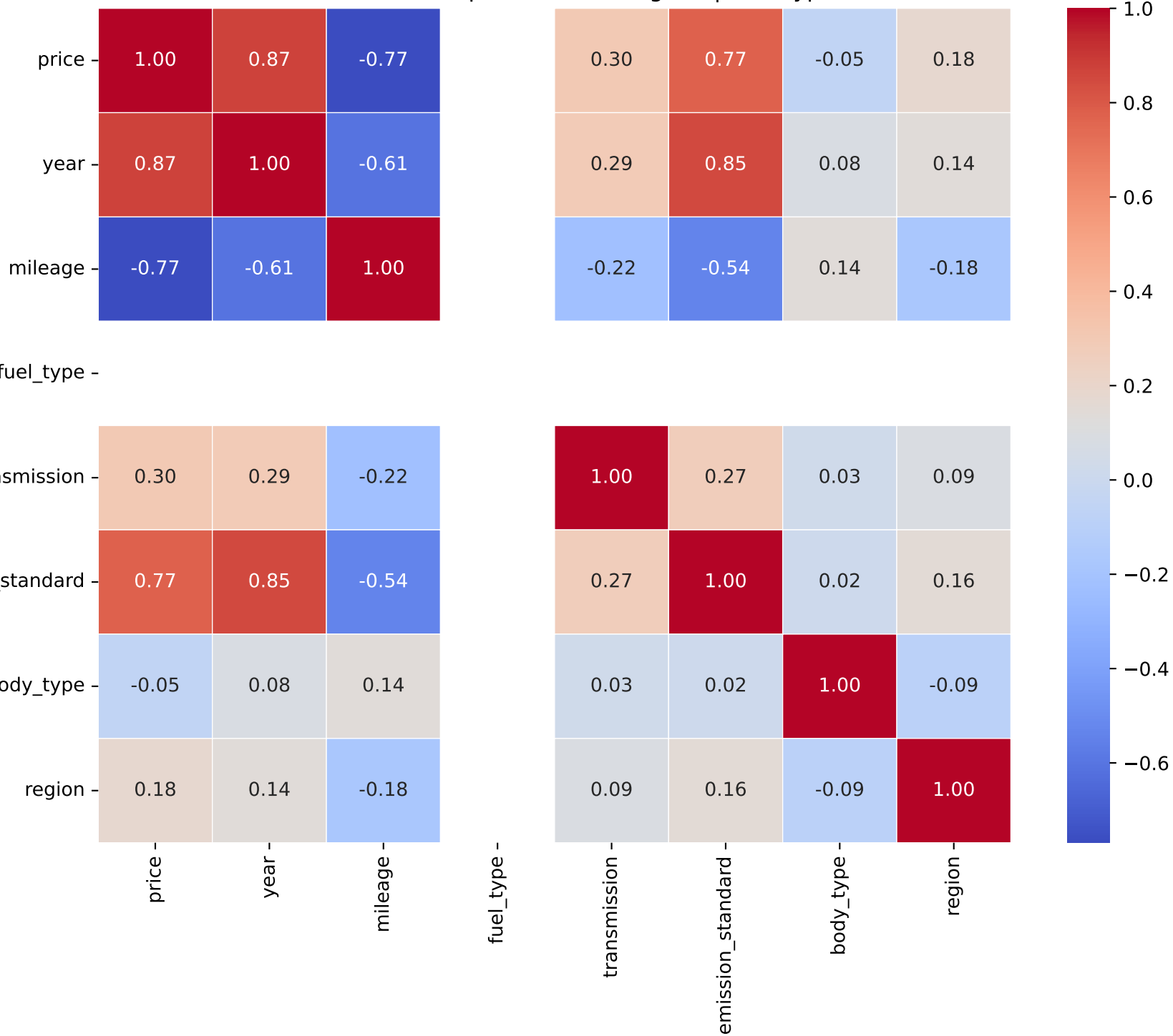
Correlation Heatmap for Model: megane | Fuel Type: 1
