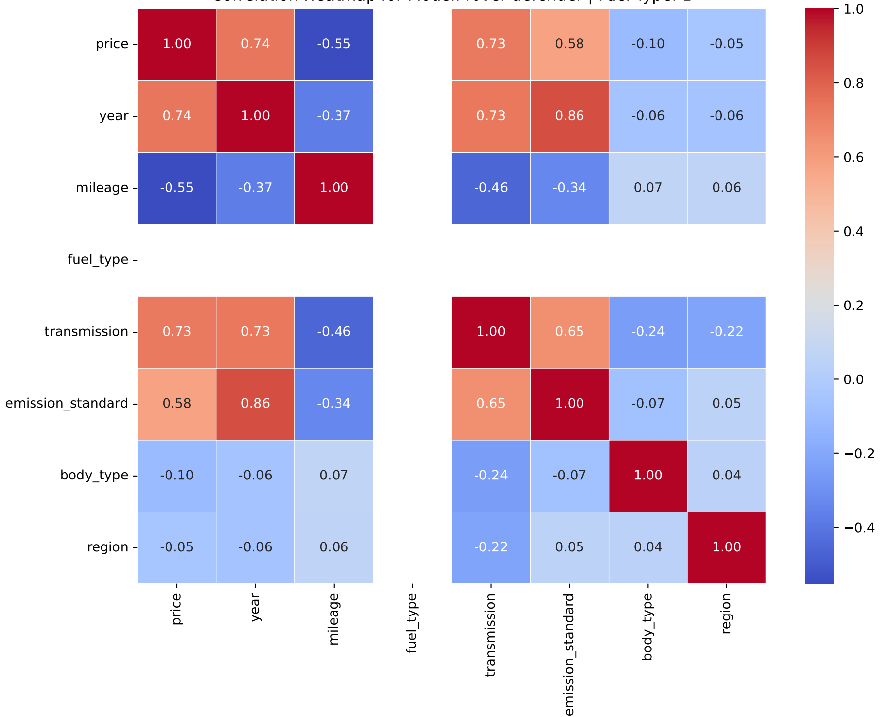
Correlation Heatmap for Model: rover defender | Fuel Type: 1
