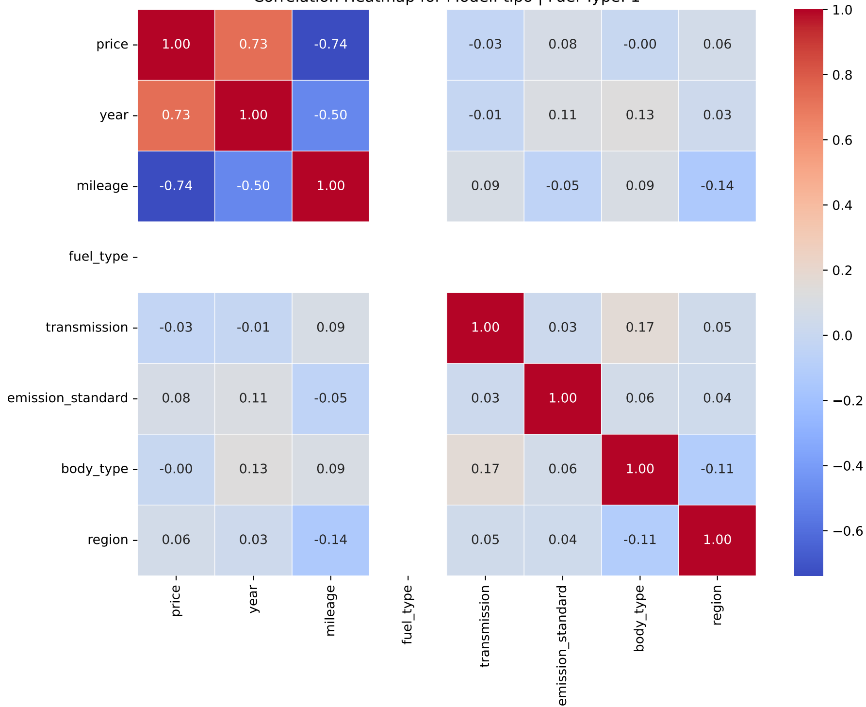
Correlation Heatmap for Model: tipo | Fuel Type: 1
