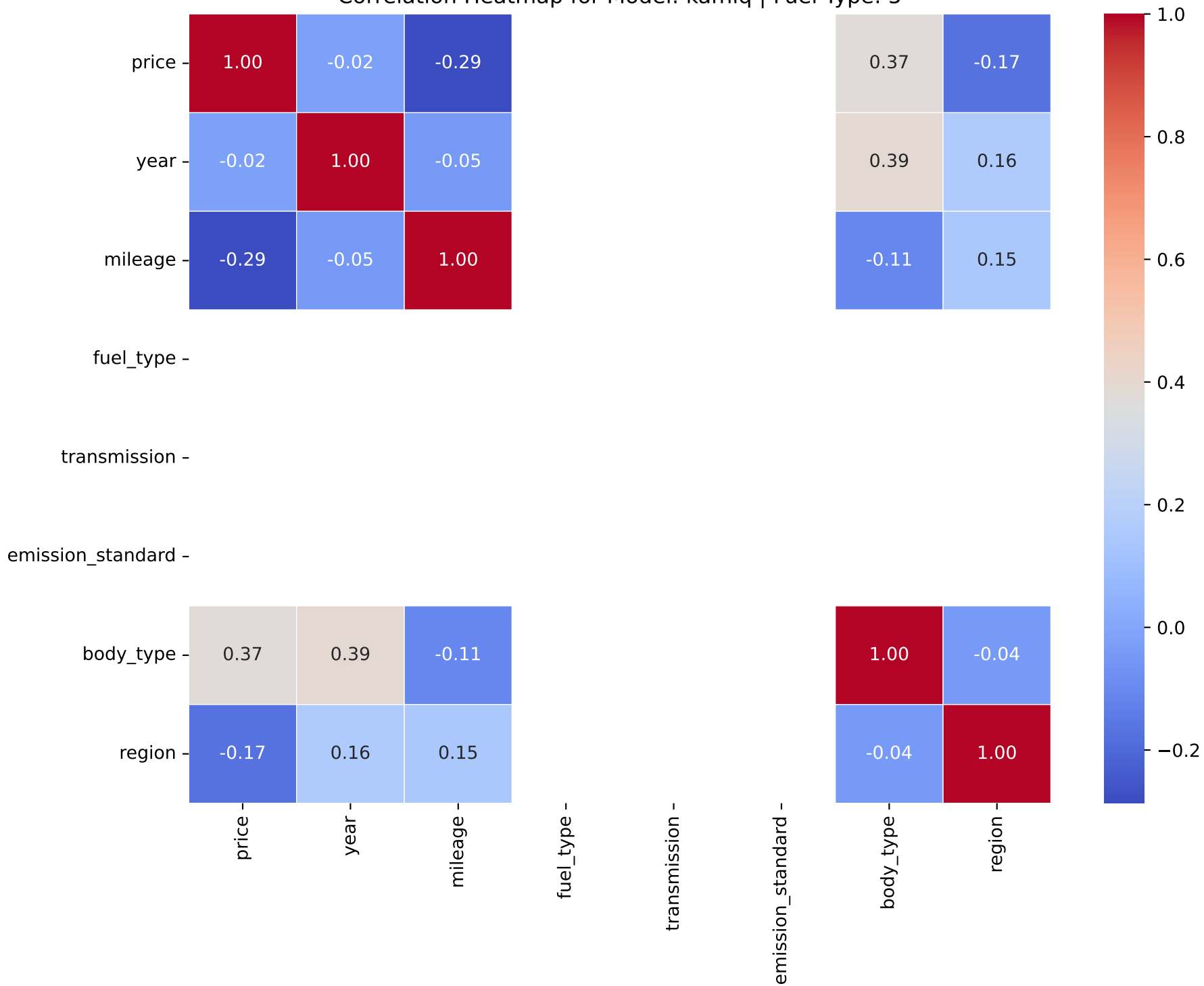
Correlation Heatmap for Model: kamiq | Fuel Type: 5
