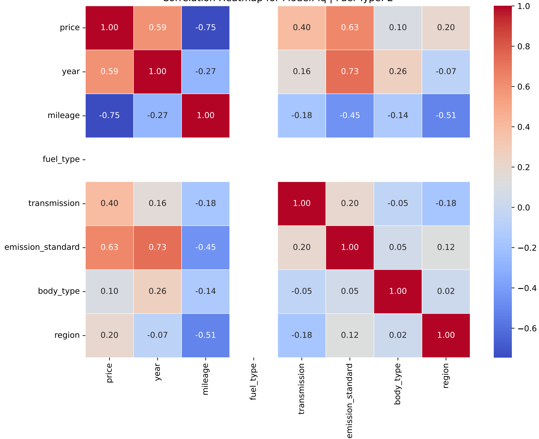
Correlation Heatmap for Model: iq | Fuel Type: 2
