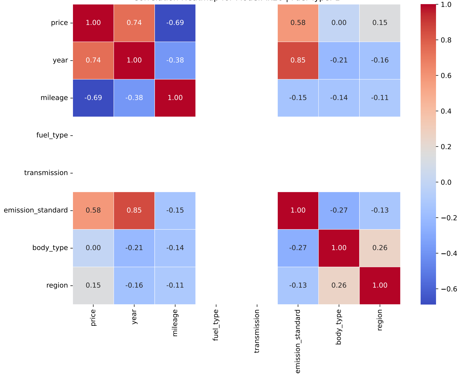
Correlation Heatmap for Model: ix20 | Fuel Type: 1
