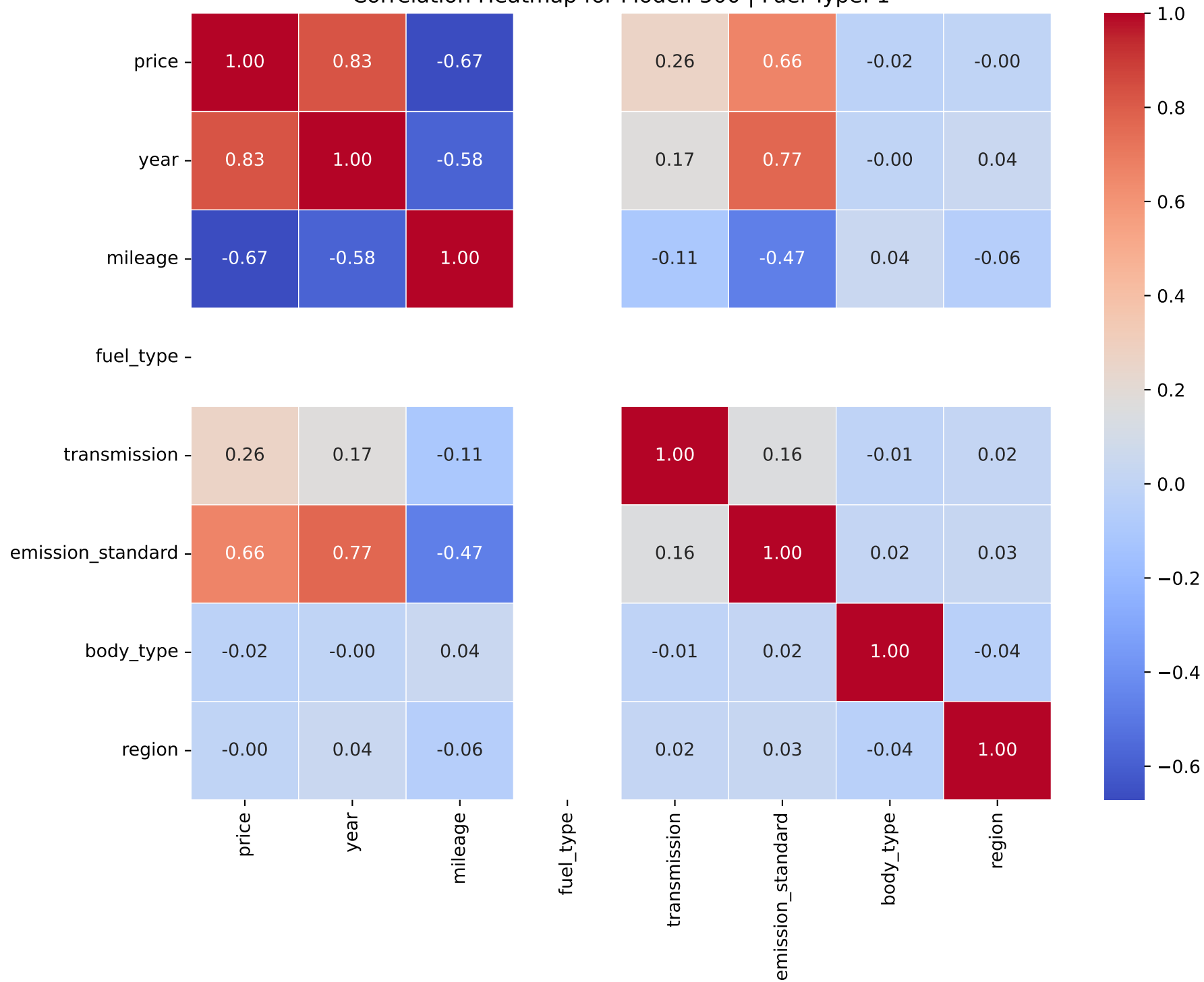
Correlation Heatmap for Model: 500 | Fuel Type: 1
