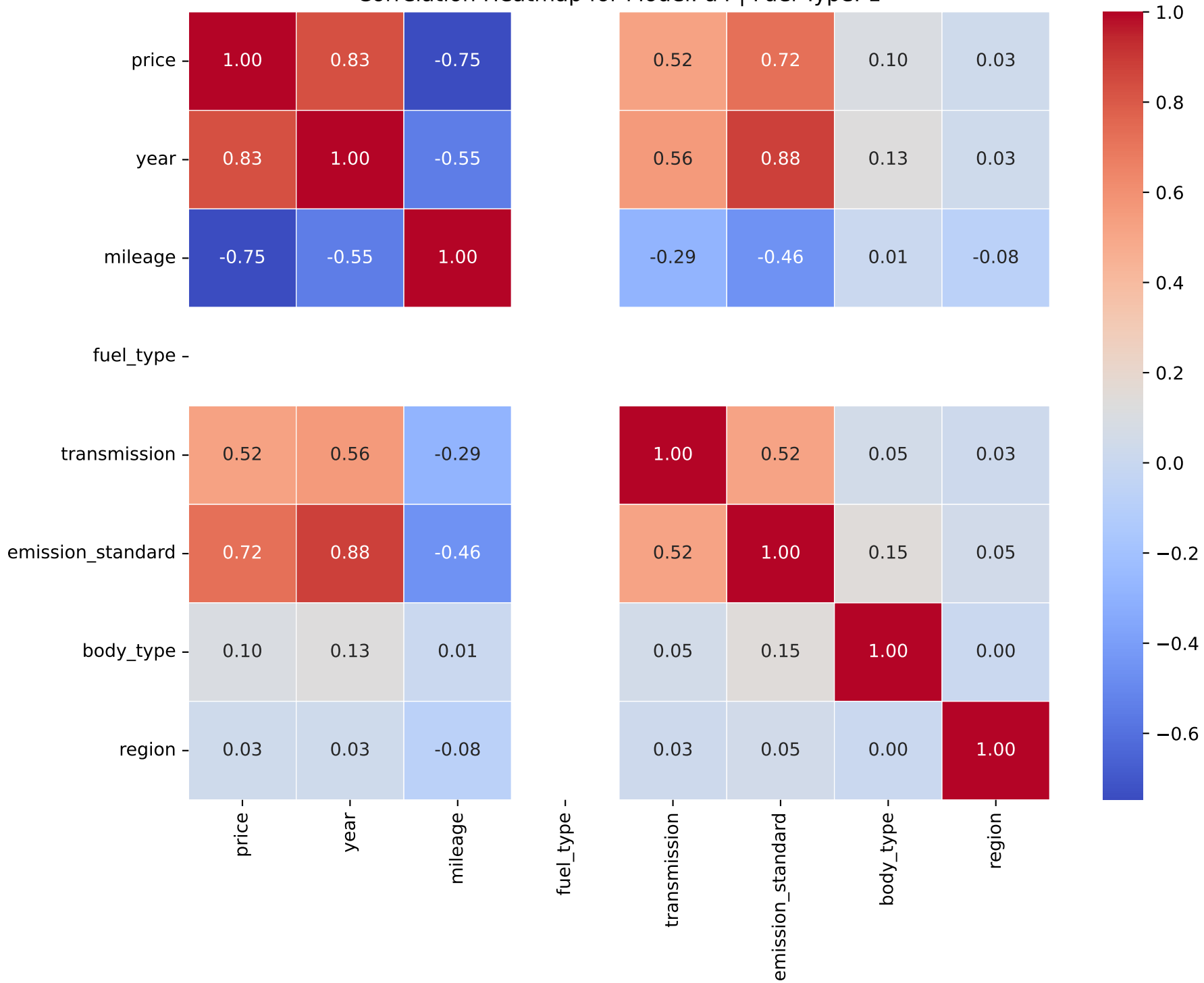
Correlation Heatmap for Model: a4 | Fuel Type: 1
