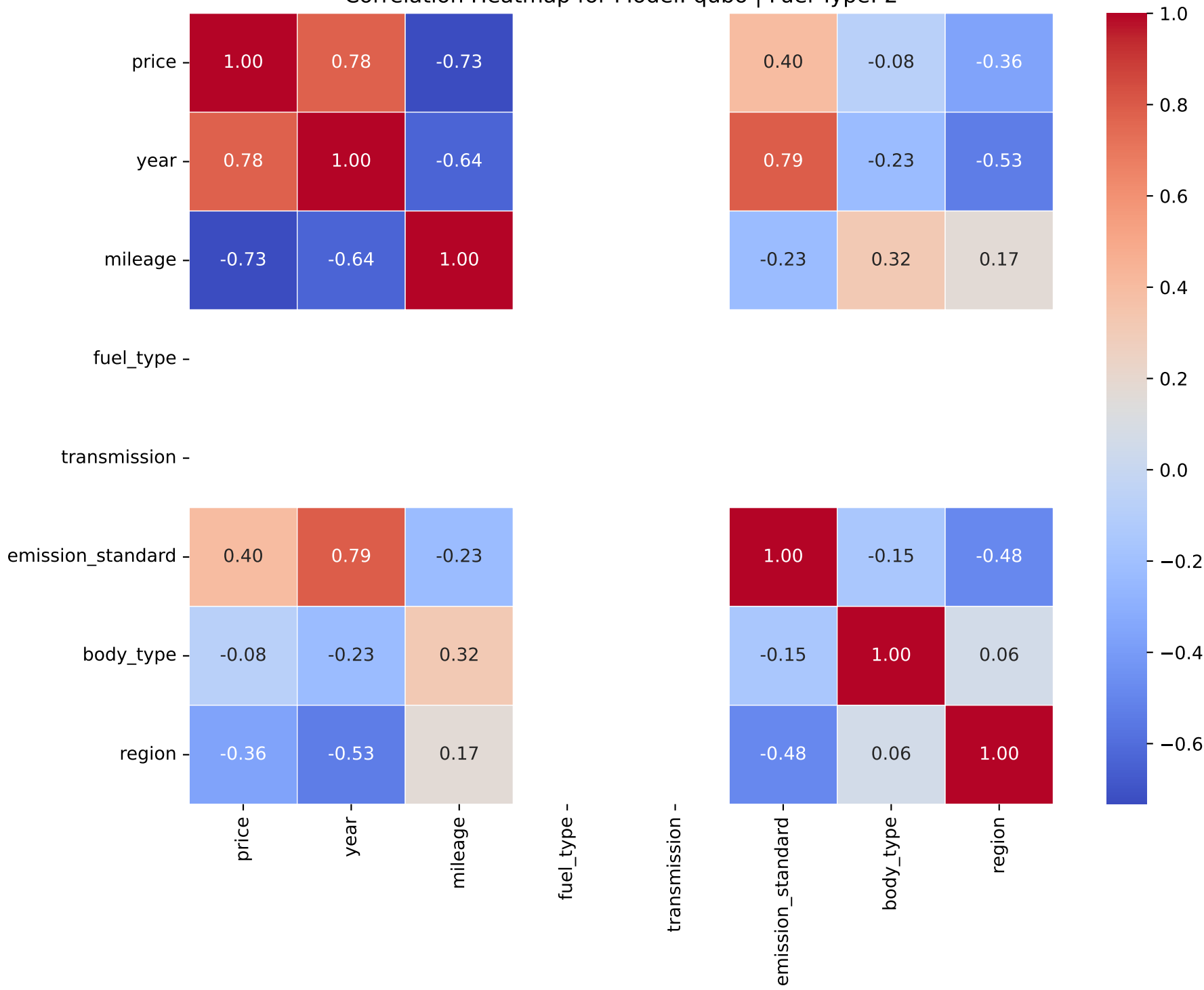
Correlation Heatmap for Model: qubo | Fuel Type: 2
