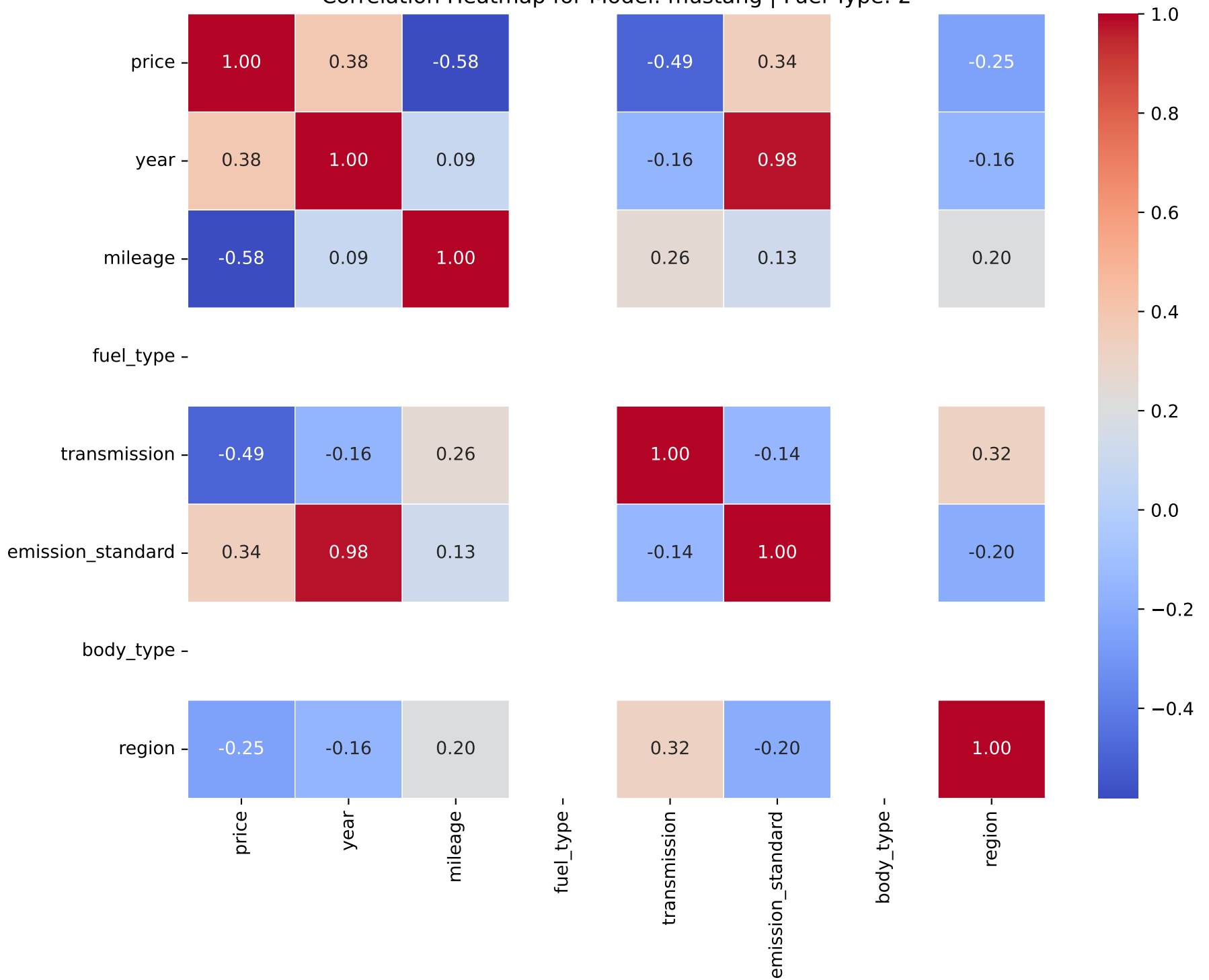
Correlation Heatmap for Model: mustang | Fuel Type: 2
