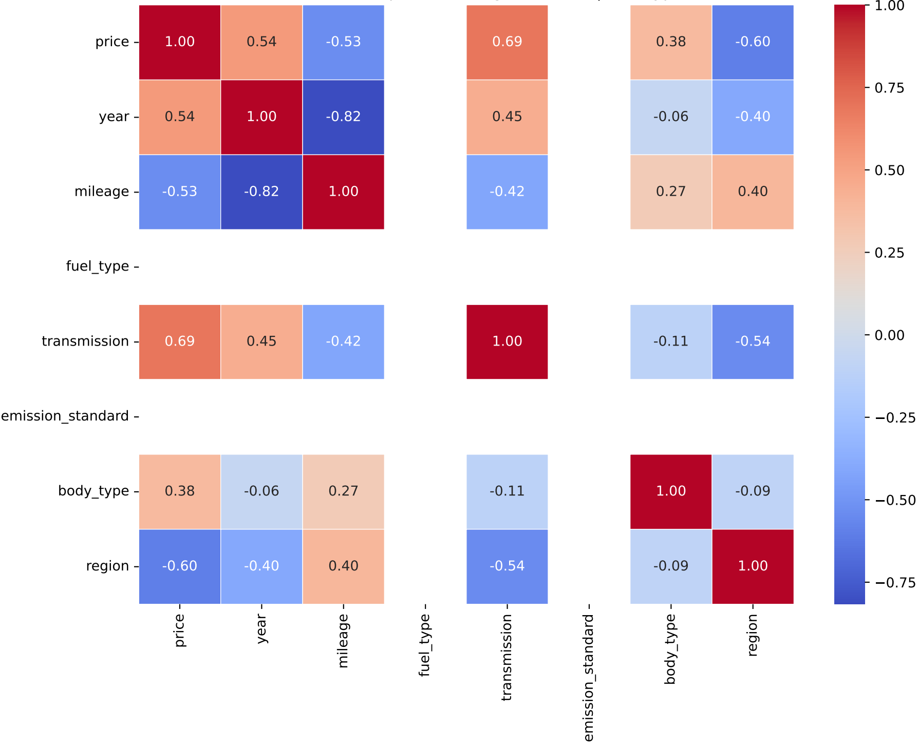
Correlation Heatmap for Model: grandland x | Fuel Type: 2
