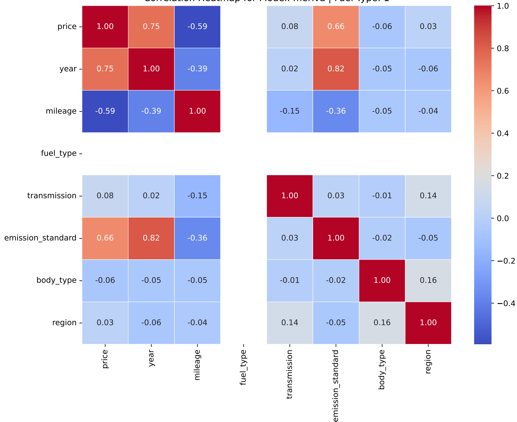
Correlation Heatmap for Model: meriva | Fuel Type: 1
