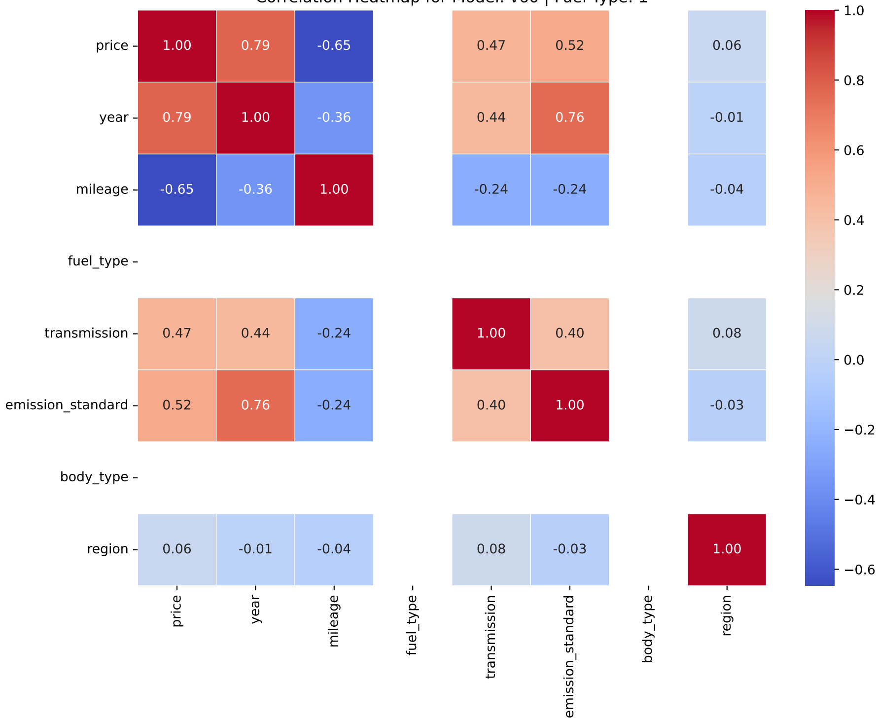
Correlation Heatmap for Model: v60 | Fuel Type: 1
