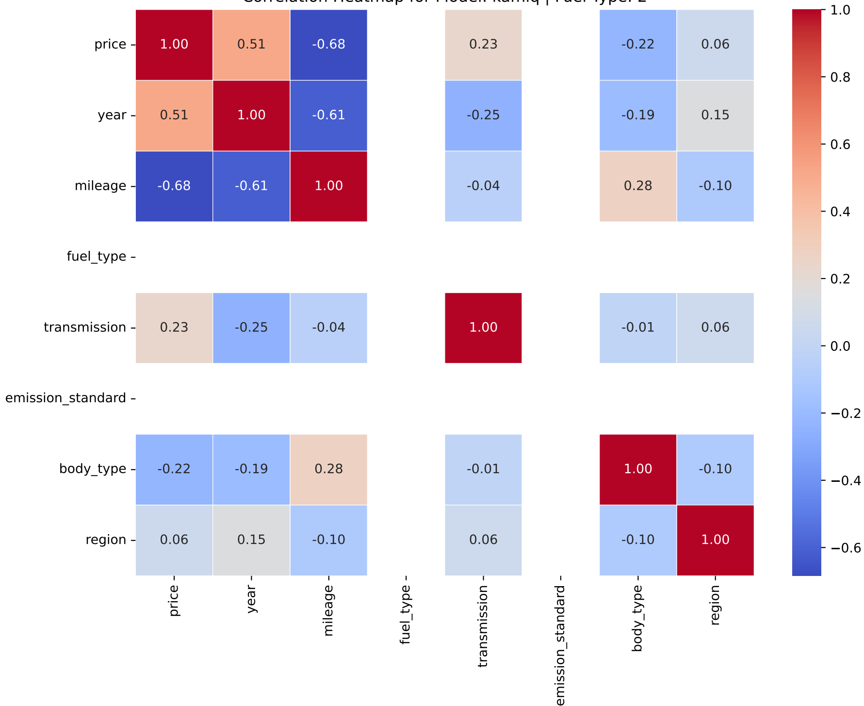
Correlation Heatmap for Model: kamiq | Fuel Type: 2
