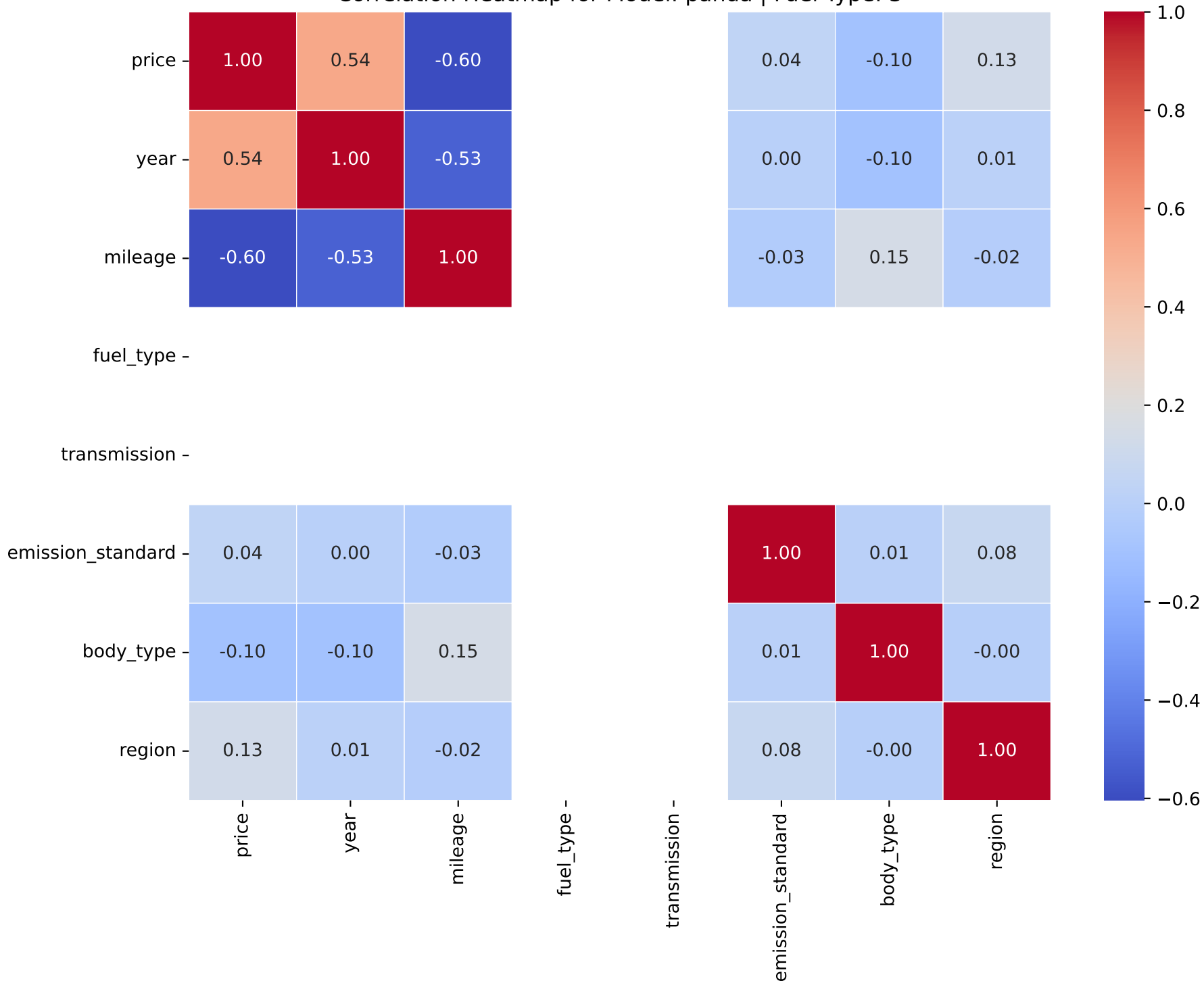
Correlation Heatmap for Model: panda | Fuel Type: 3
