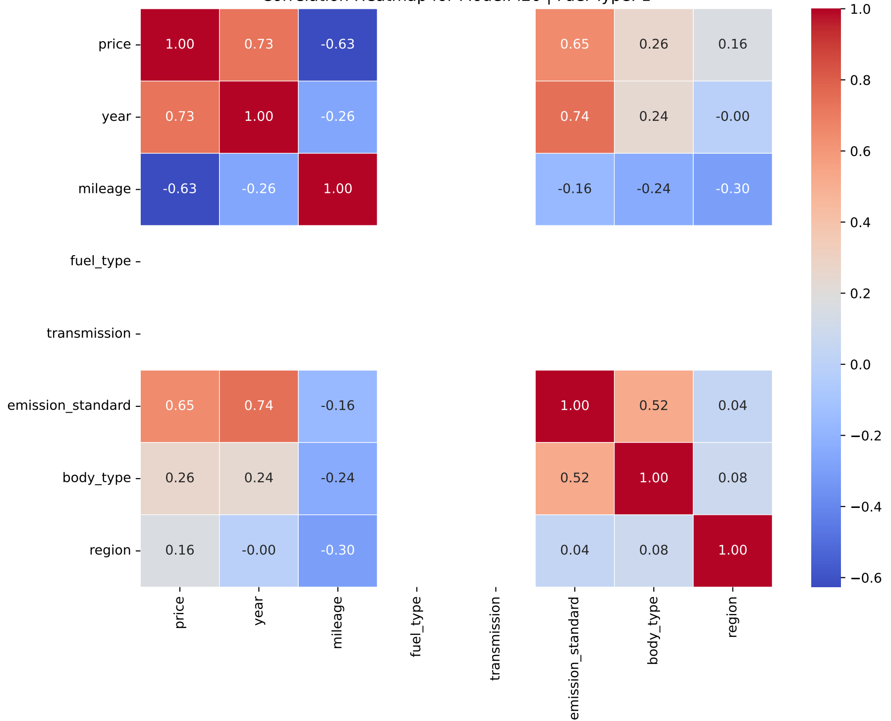
Correlation Heatmap for Model: i20 | Fuel Type: 1
