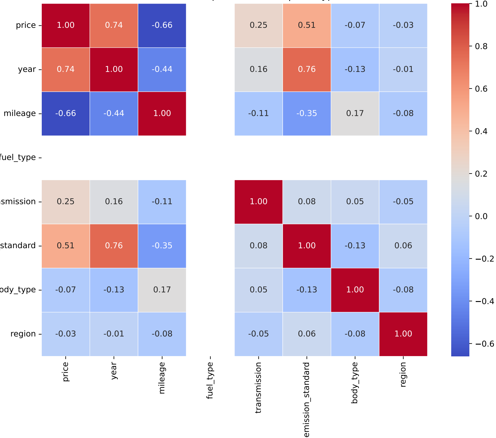
Correlation Heatmap for Model: a1 | Fuel Type: 1
