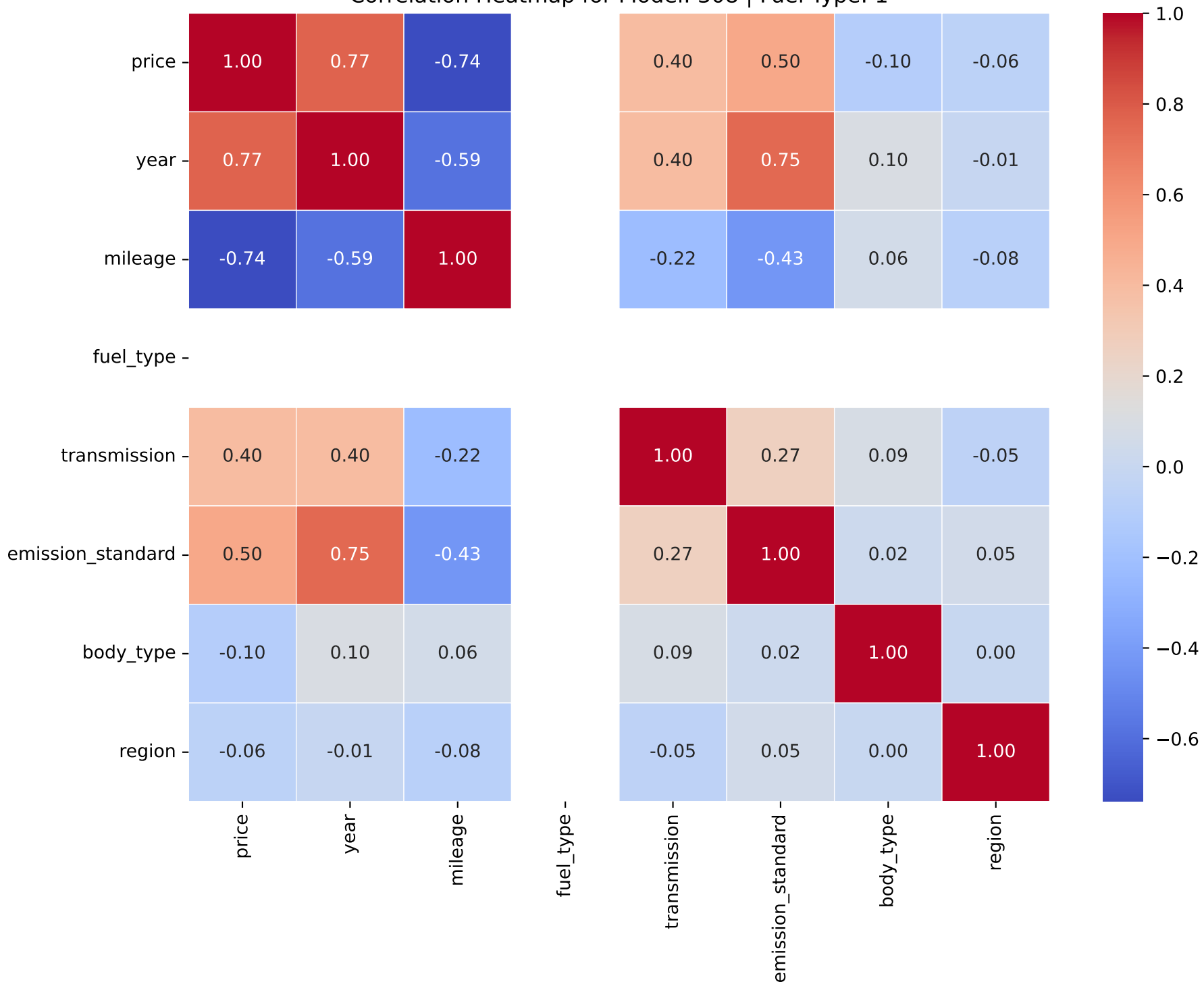
Correlation Heatmap for Model: 308 | Fuel Type: 1
