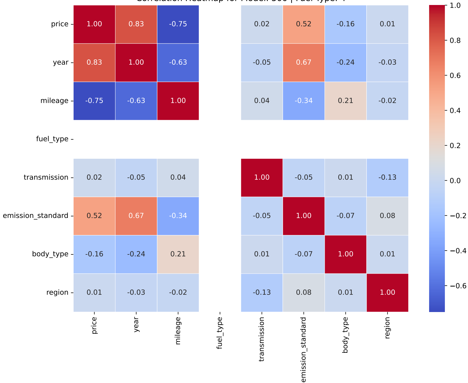
Correlation Heatmap for Model: 500 | Fuel Type: 4
