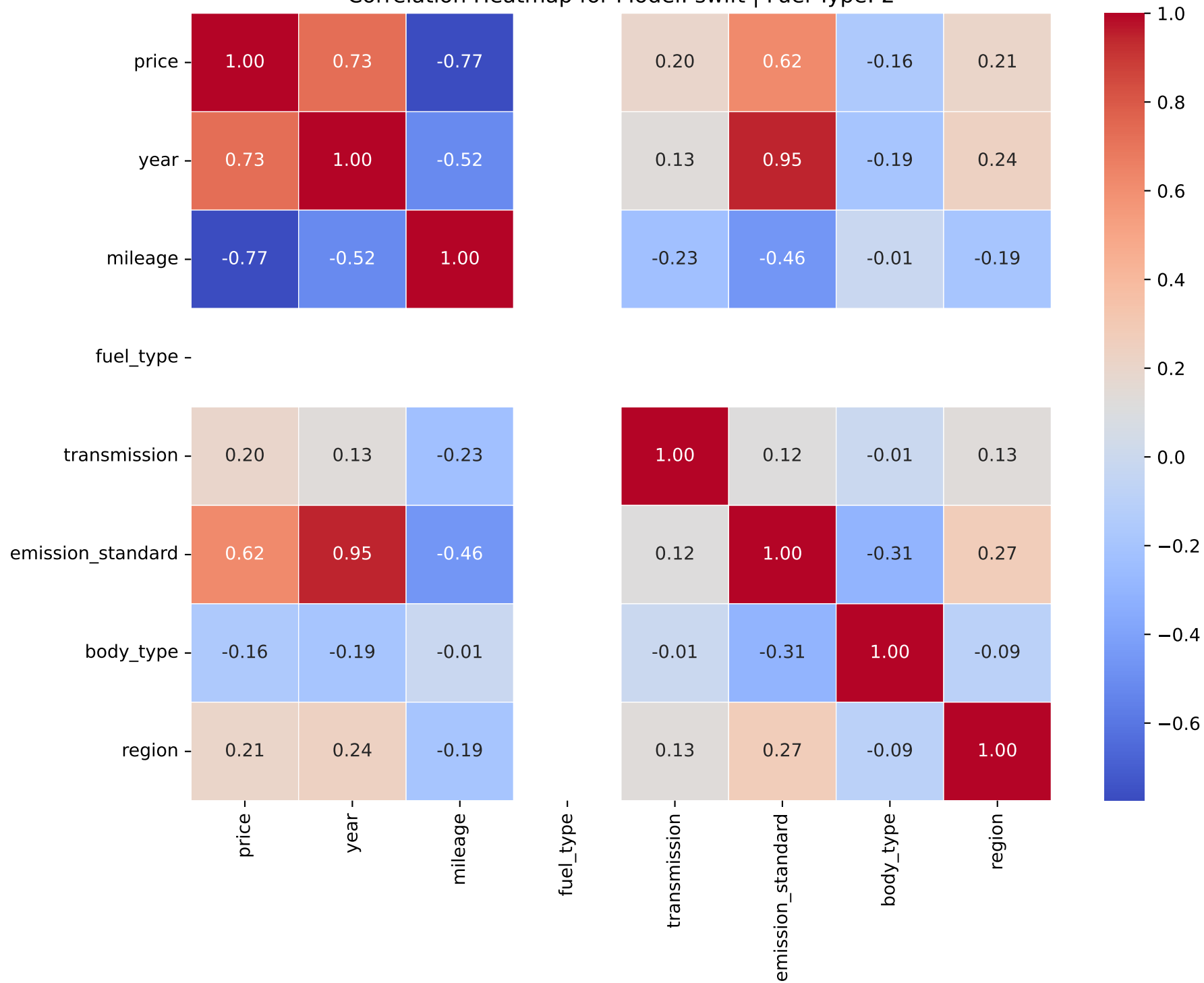
Correlation Heatmap for Model: swift | Fuel Type: 2
