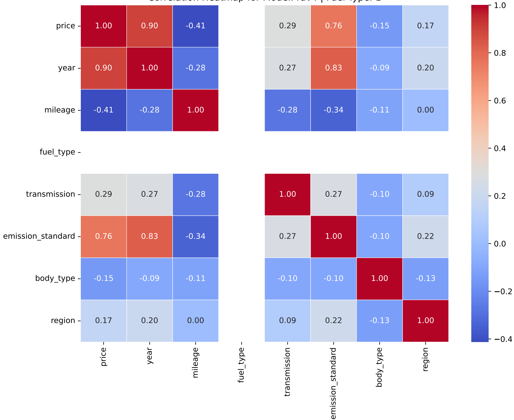
Correlation Heatmap for Model: rav4 | Fuel Type: 1
