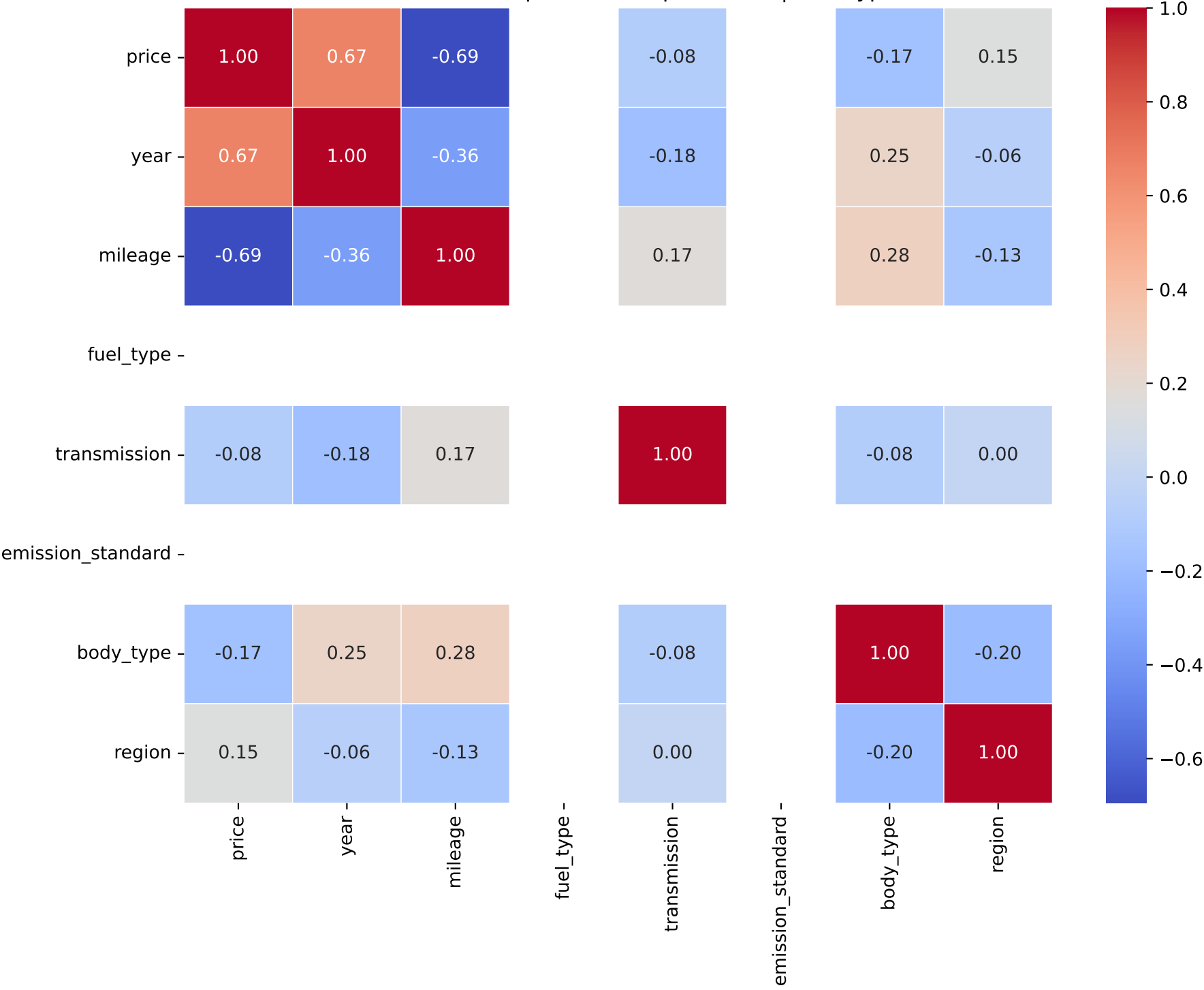
Correlation Heatmap for Model: panamera | Fuel Type: 3
