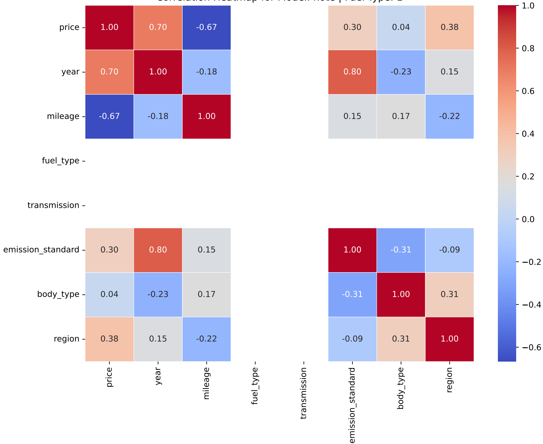
Correlation Heatmap for Model: note | Fuel Type: 1
