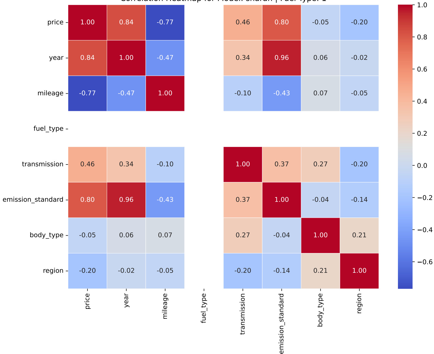
Correlation Heatmap for Model: sharan | Fuel Type: 1
