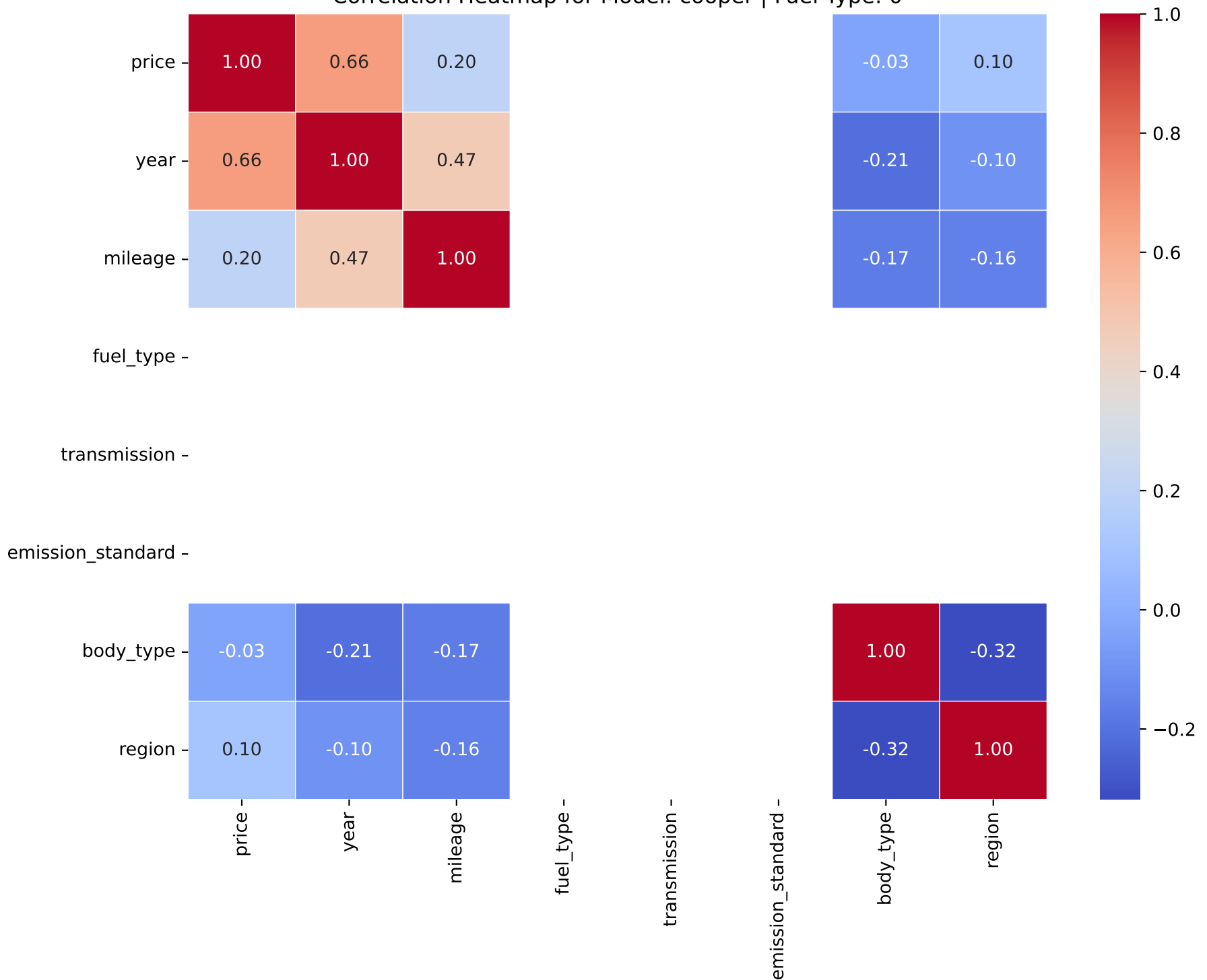
Correlation Heatmap for Model: cooper | Fuel Type: 0
