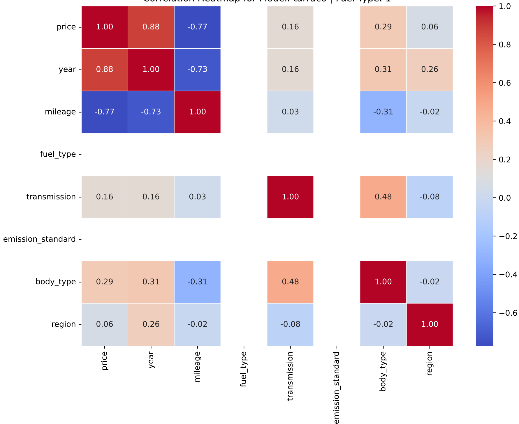
Correlation Heatmap for Model: tarraco | Fuel Type: 1
