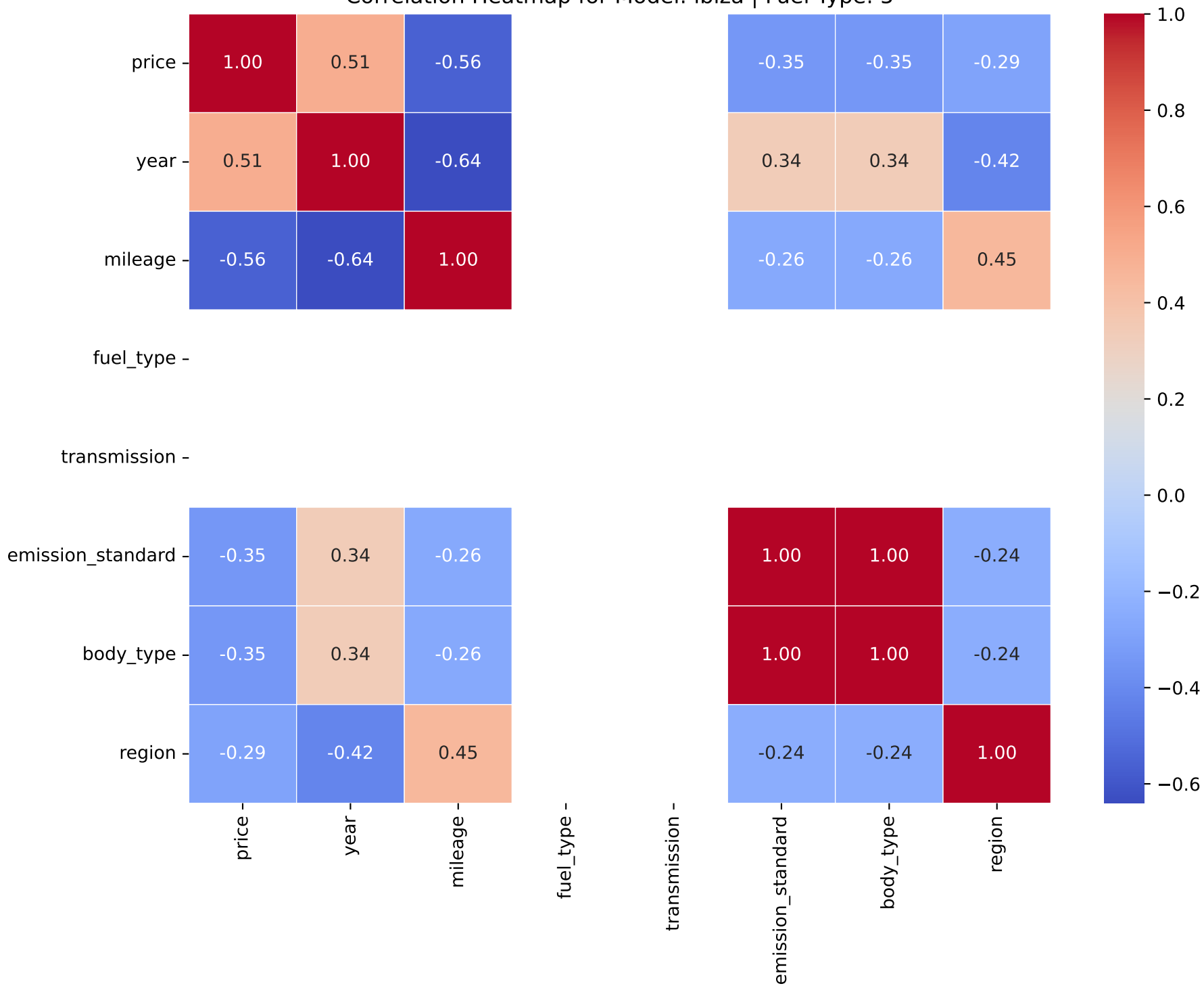
Correlation Heatmap for Model: ibiza | Fuel Type: 5
