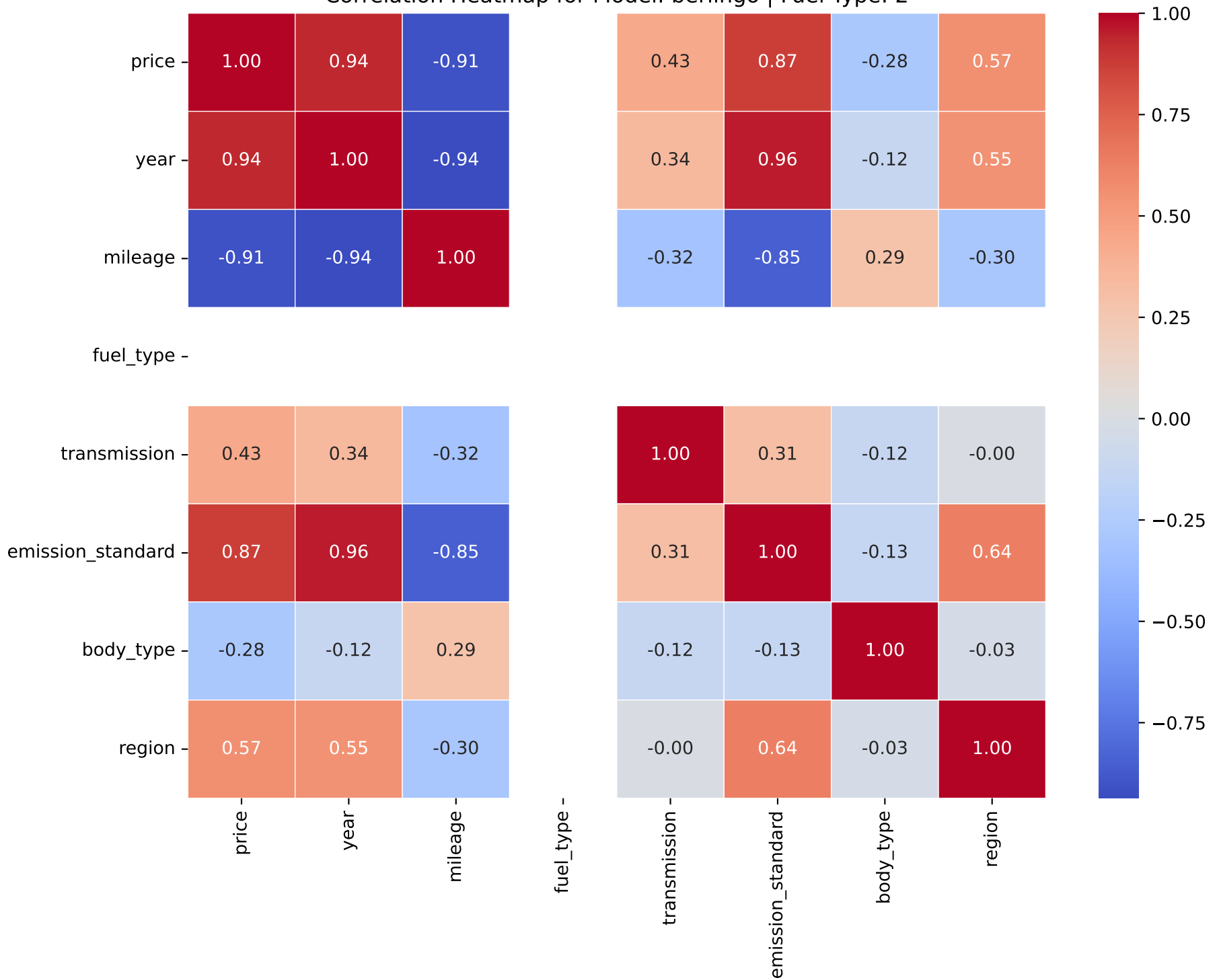
Correlation Heatmap for Model: berlingo | Fuel Type: 2
