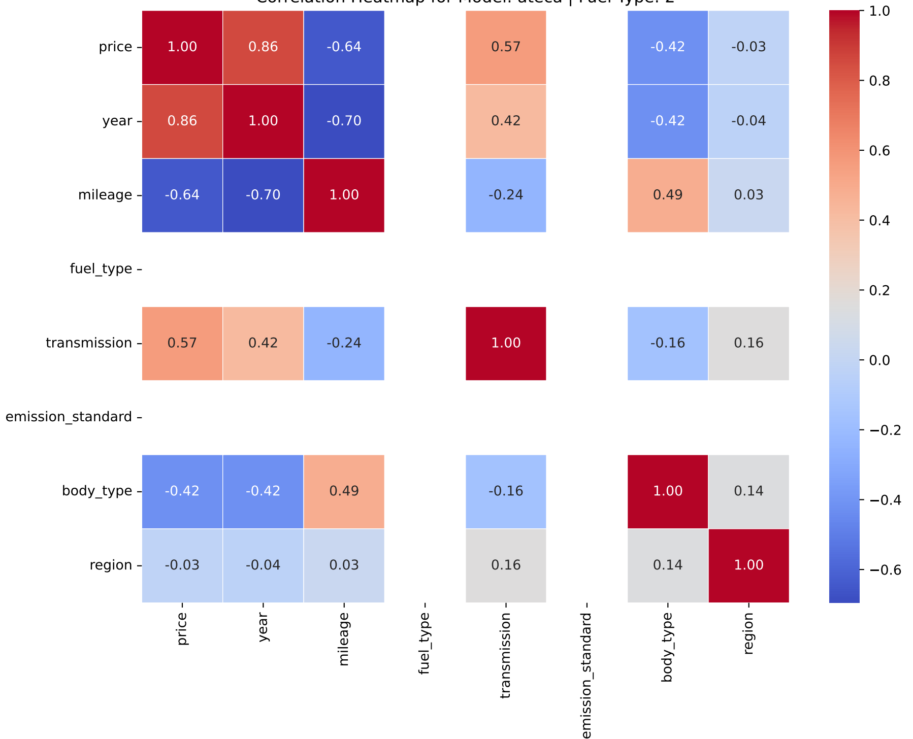
Correlation Heatmap for Model: ateca | Fuel Type: 2
