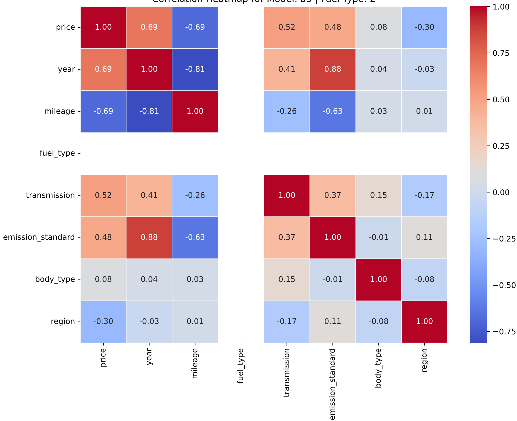
Correlation Heatmap for Model: a3 | Fuel Type: 2
