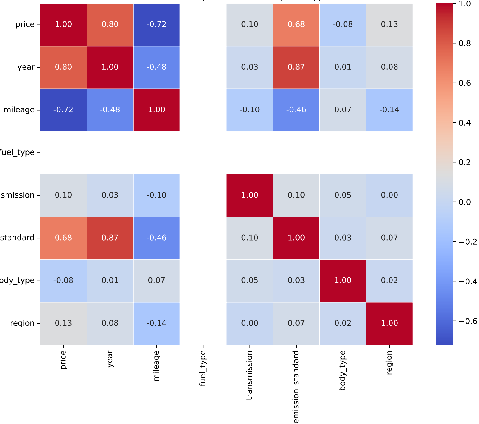
Correlation Heatmap for Model: clio | Fuel Type: 1
