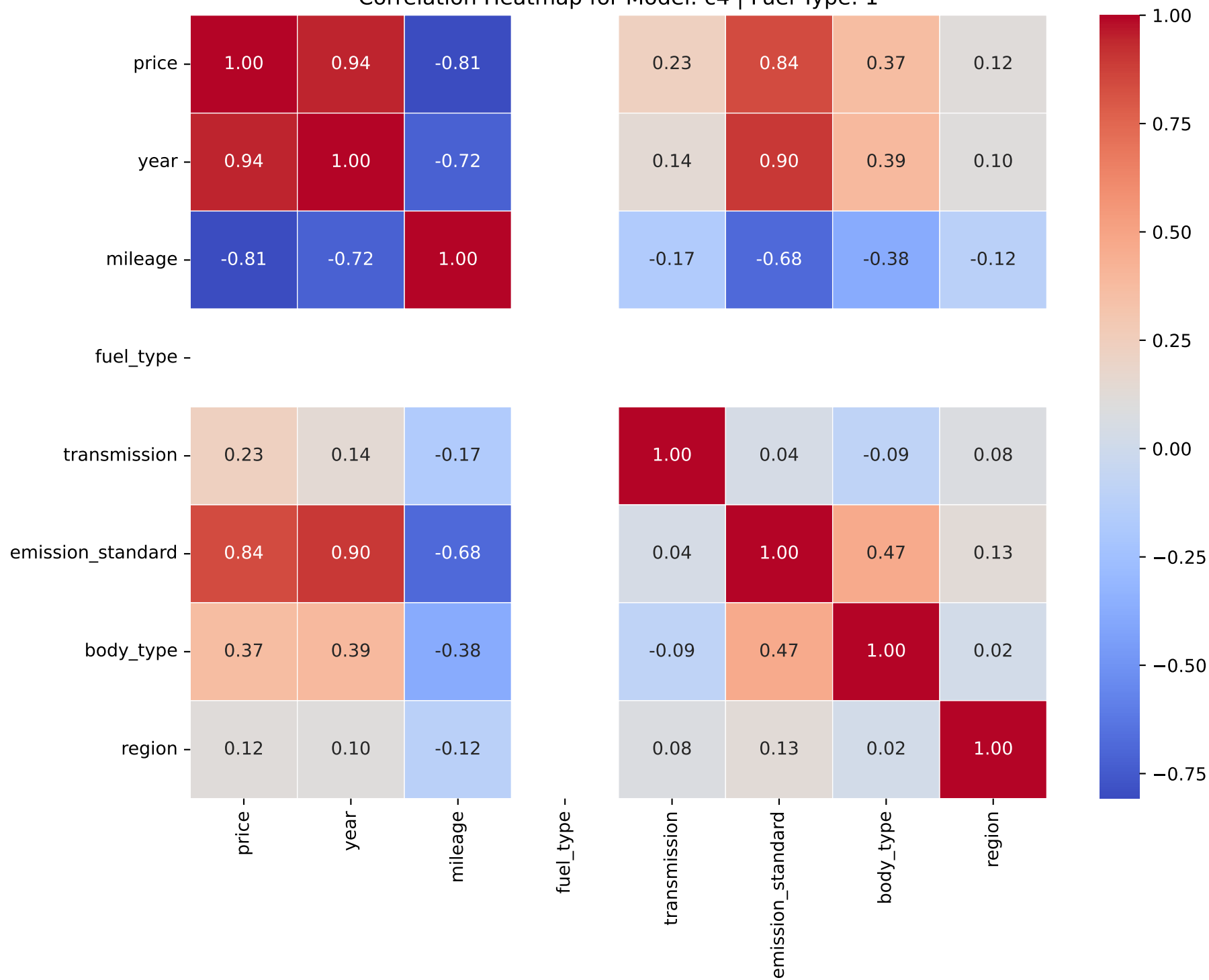
Correlation Heatmap for Model: c4 | Fuel Type: 1
