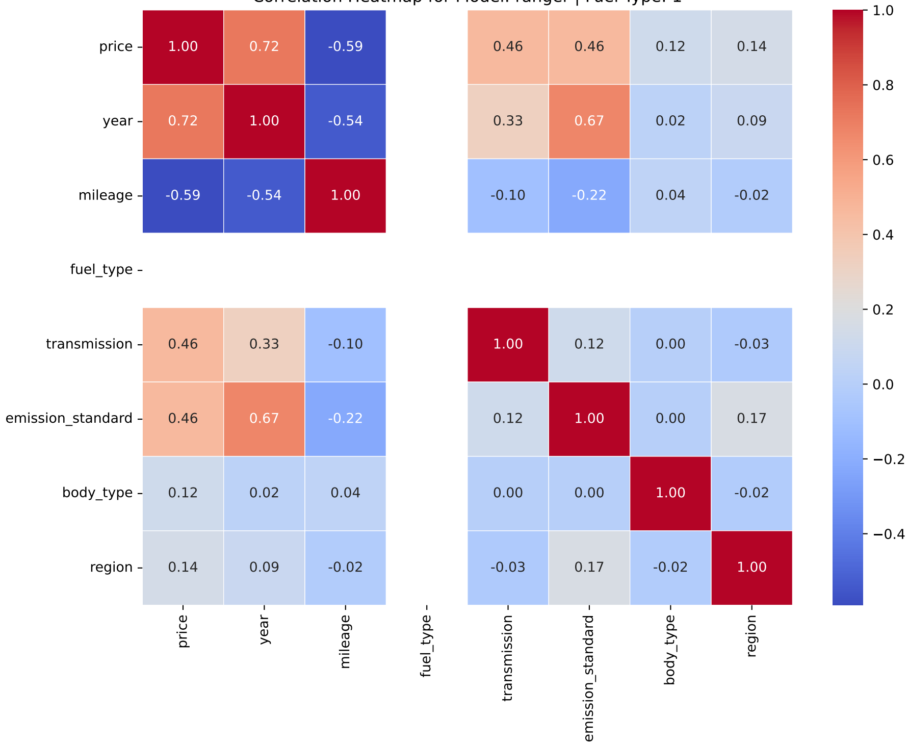
Correlation Heatmap for Model: ranger | Fuel Type: 1
