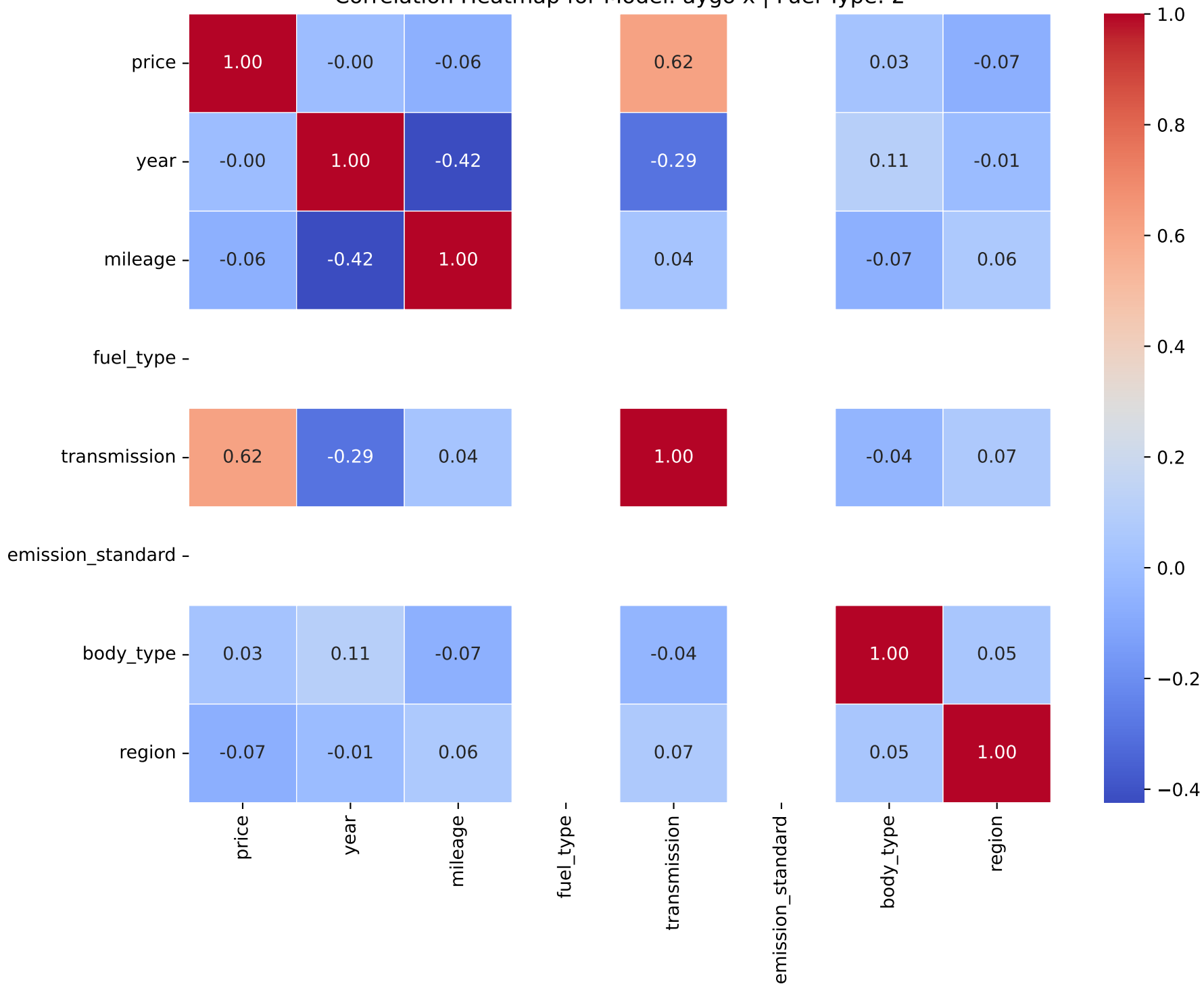
Correlation Heatmap for Model: aygo x | Fuel Type: 2
