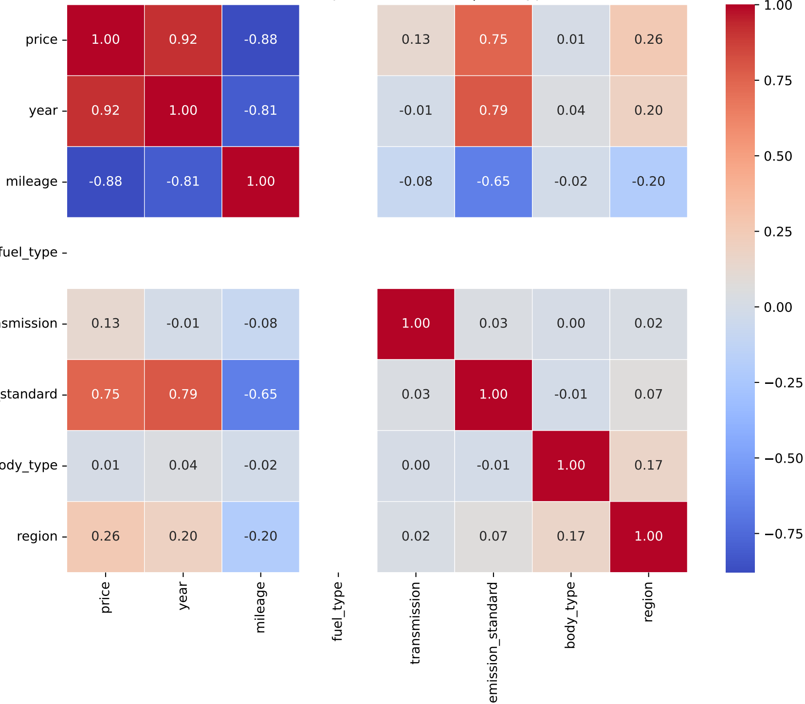
Correlation Heatmap for Model: ibiza | Fuel Type: 2
