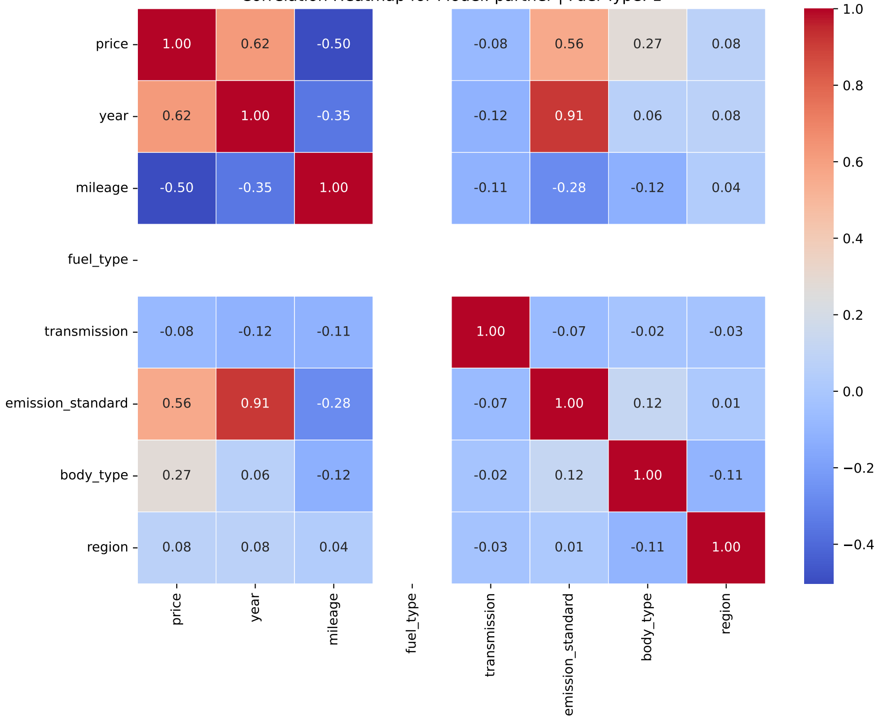
Correlation Heatmap for Model: partner | Fuel Type: 1
