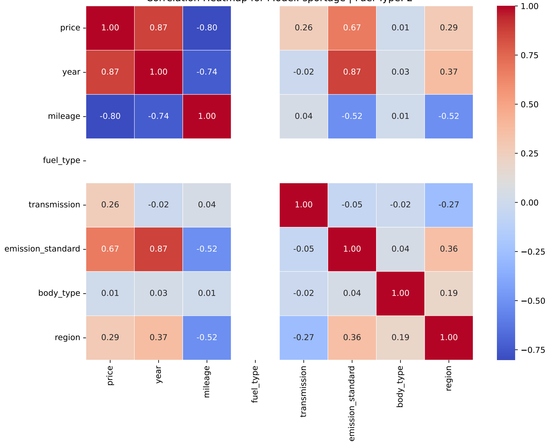
Correlation Heatmap for Model: sportage | Fuel Type: 2
