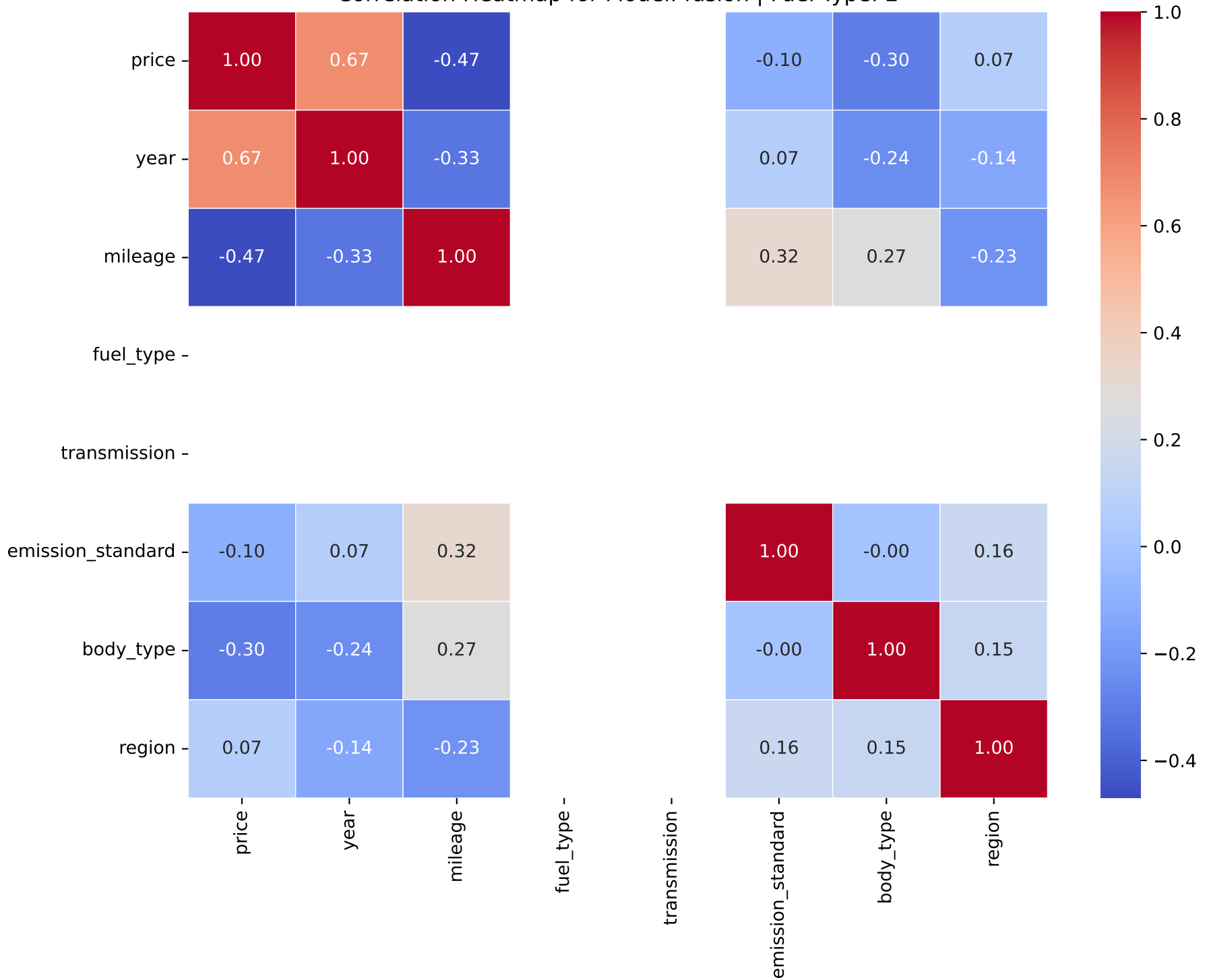
Correlation Heatmap for Model: fusion | Fuel Type: 2
