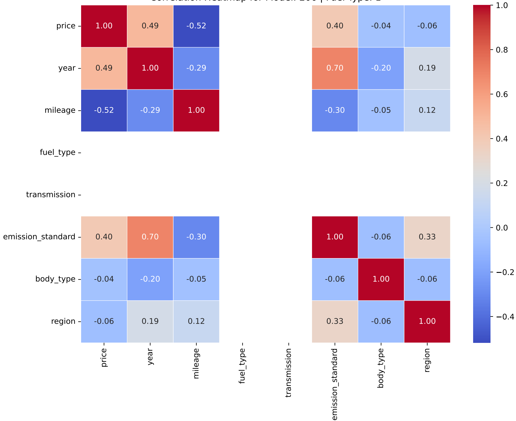
Correlation Heatmap for Model: 206 | Fuel Type: 1
