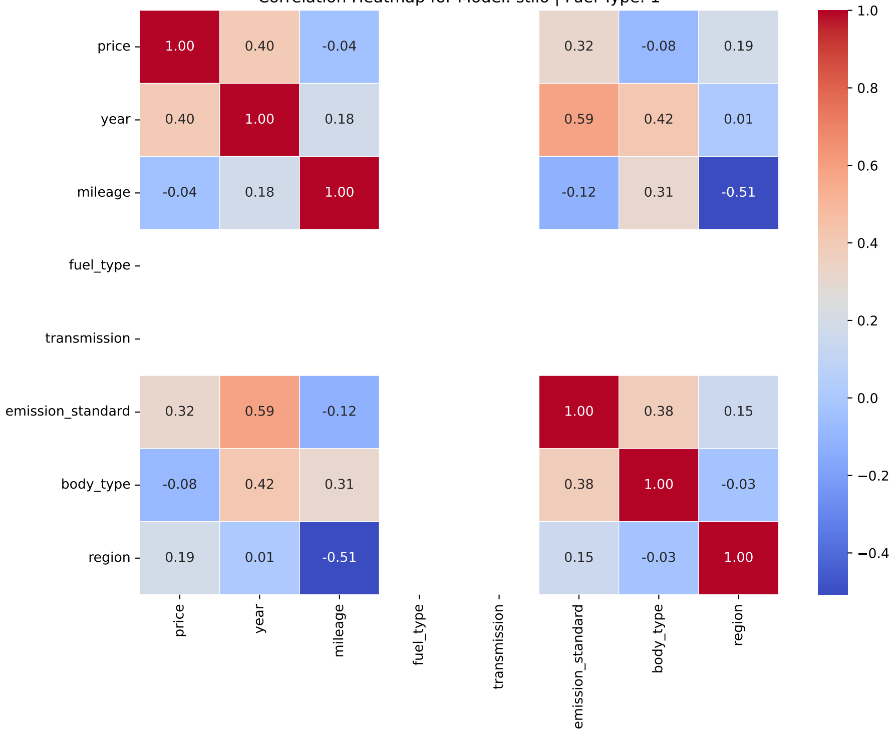
Correlation Heatmap for Model: stilo | Fuel Type: 1
