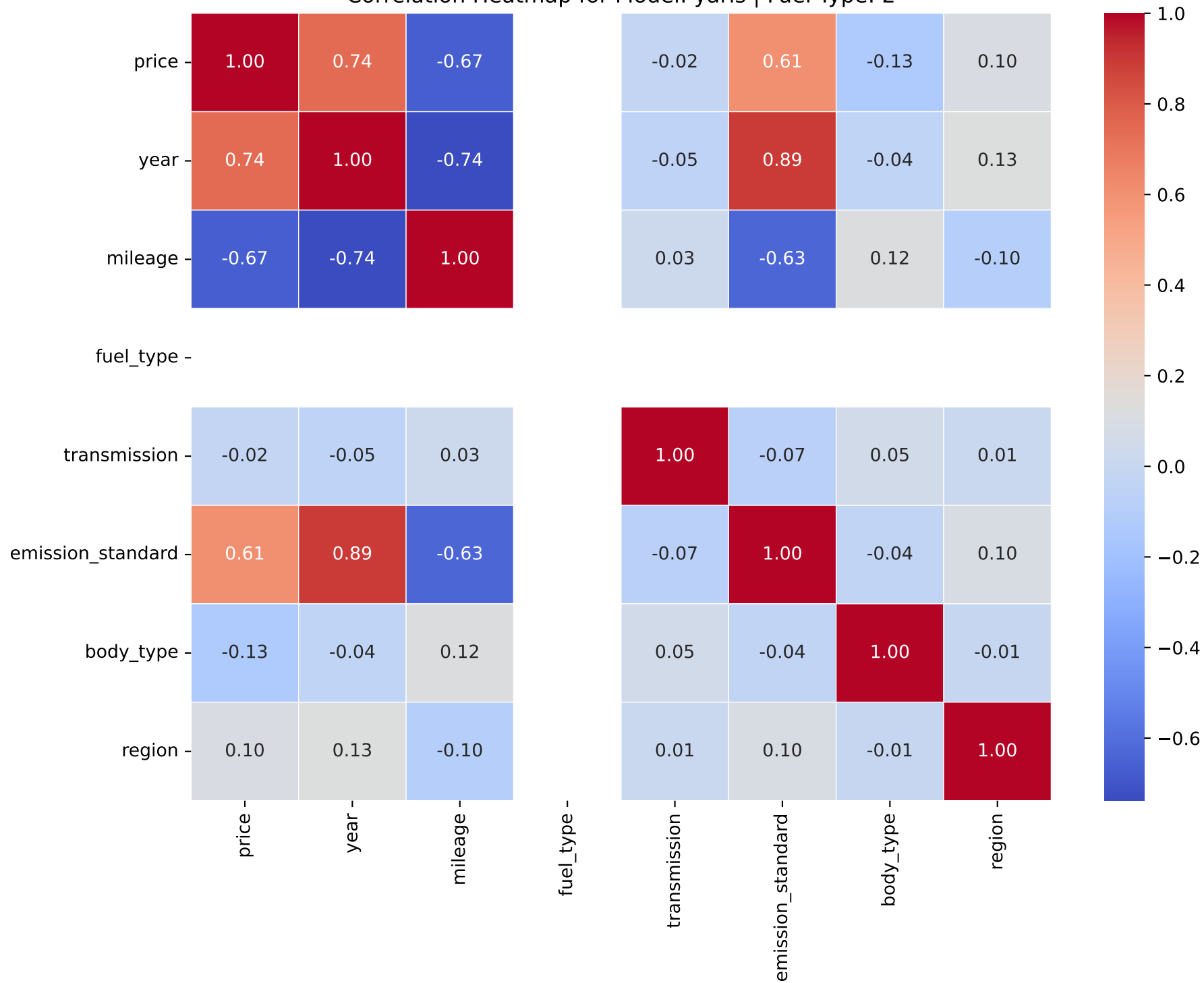
Correlation Heatmap for Model: yaris | Fuel Type: 2
