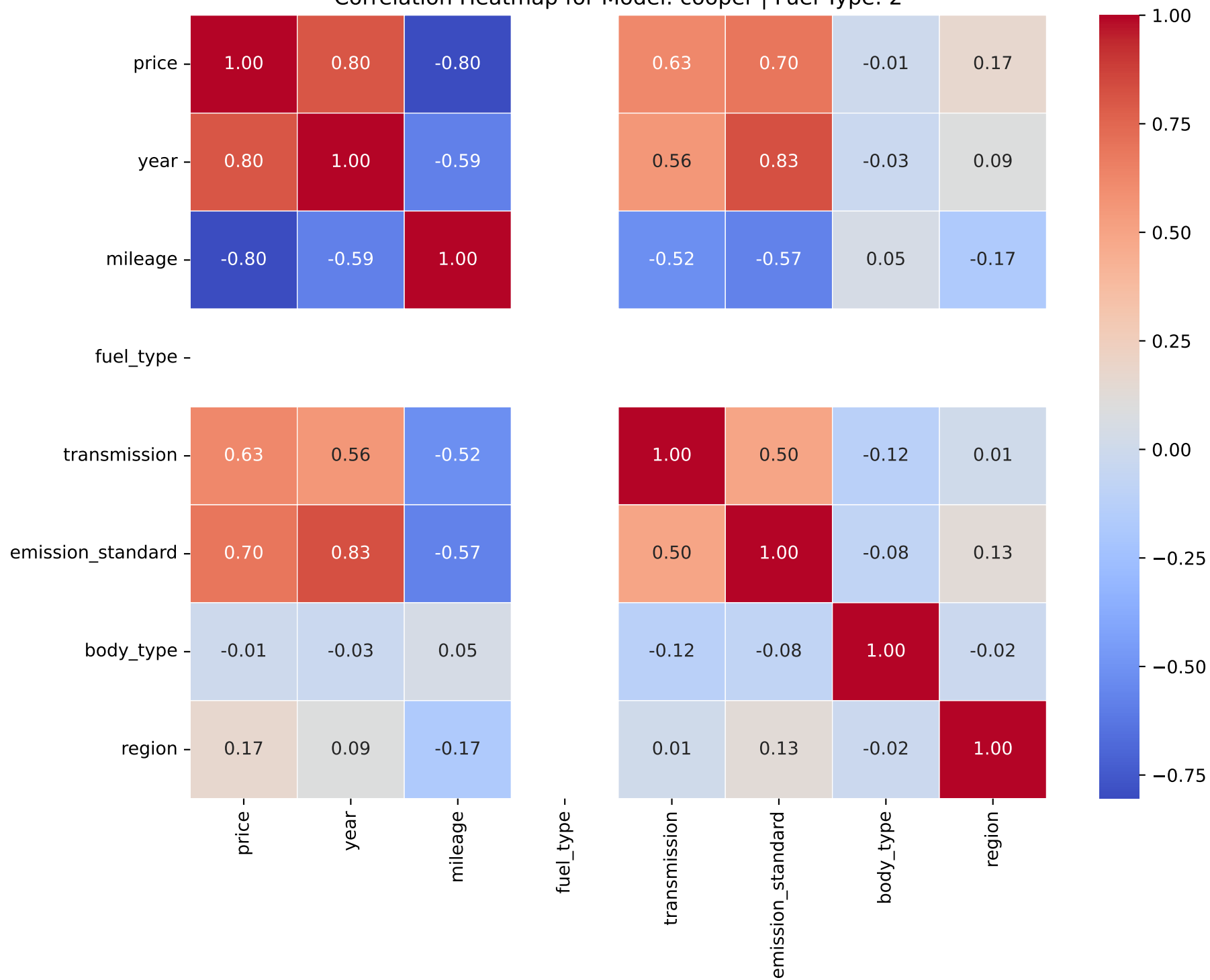
Correlation Heatmap for Model: cooper | Fuel Type: 2
