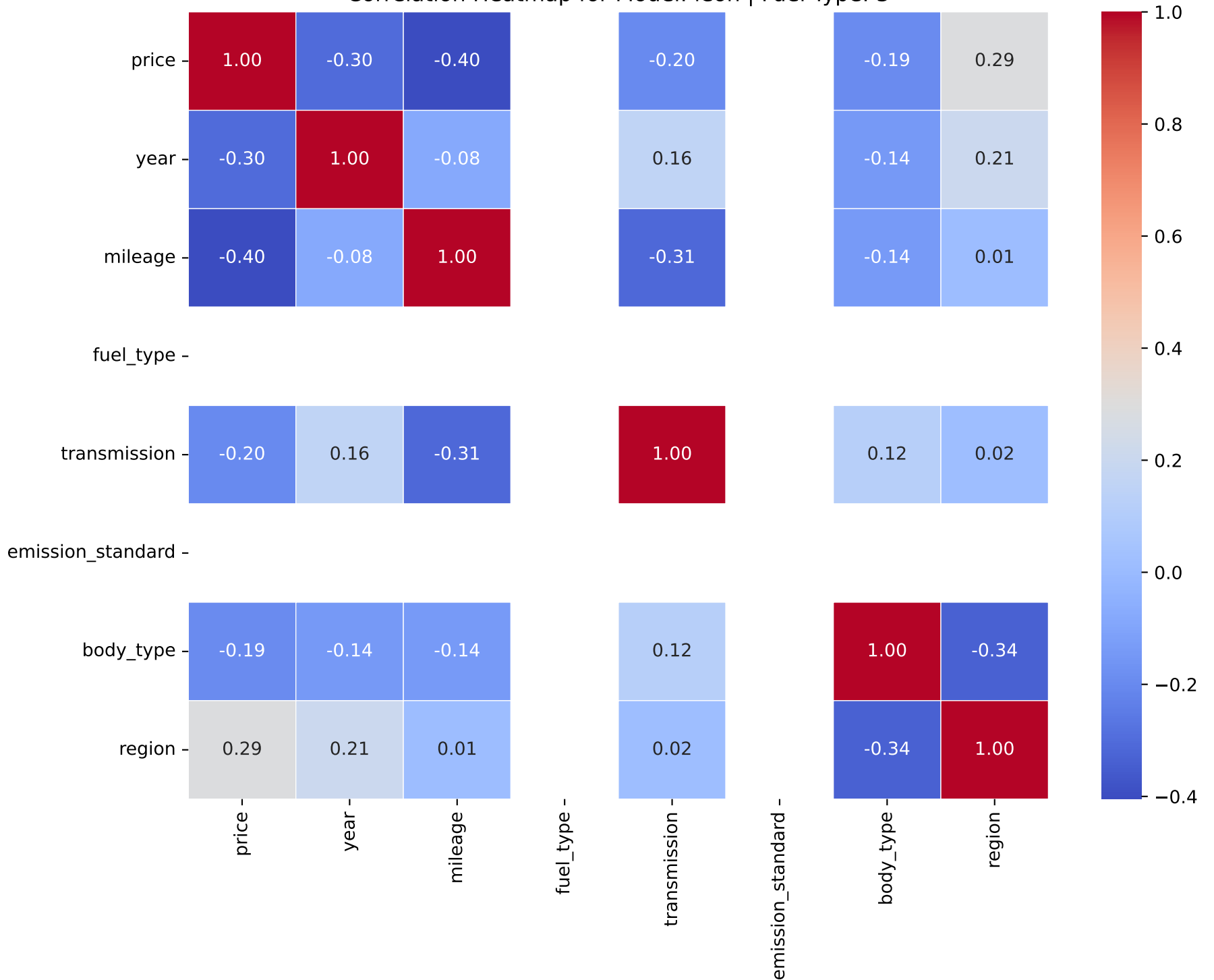
Correlation Heatmap for Model: leon | Fuel Type: 3
