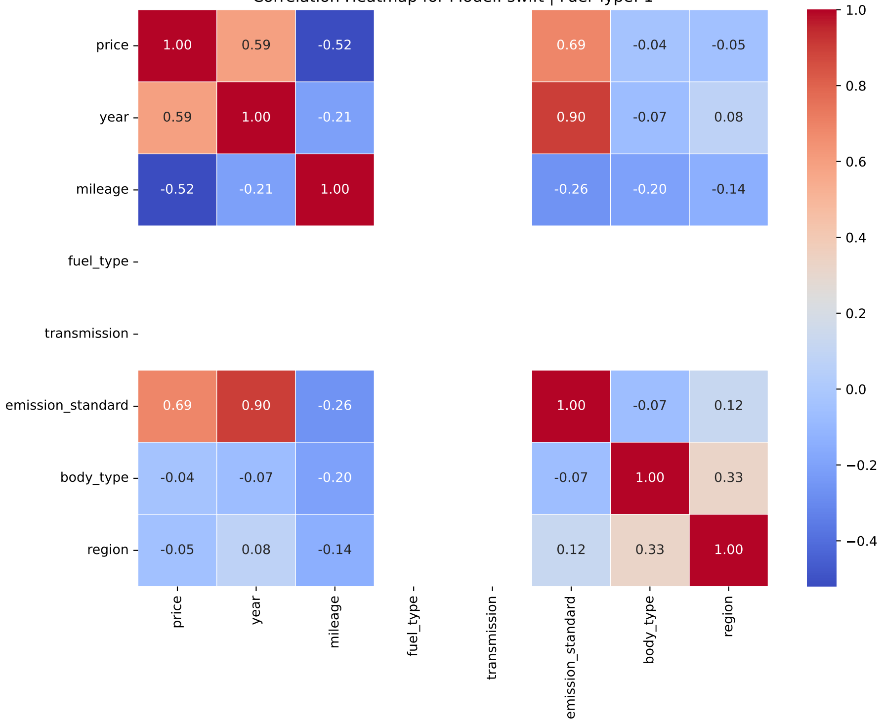
Correlation Heatmap for Model: swift | Fuel Type: 1
