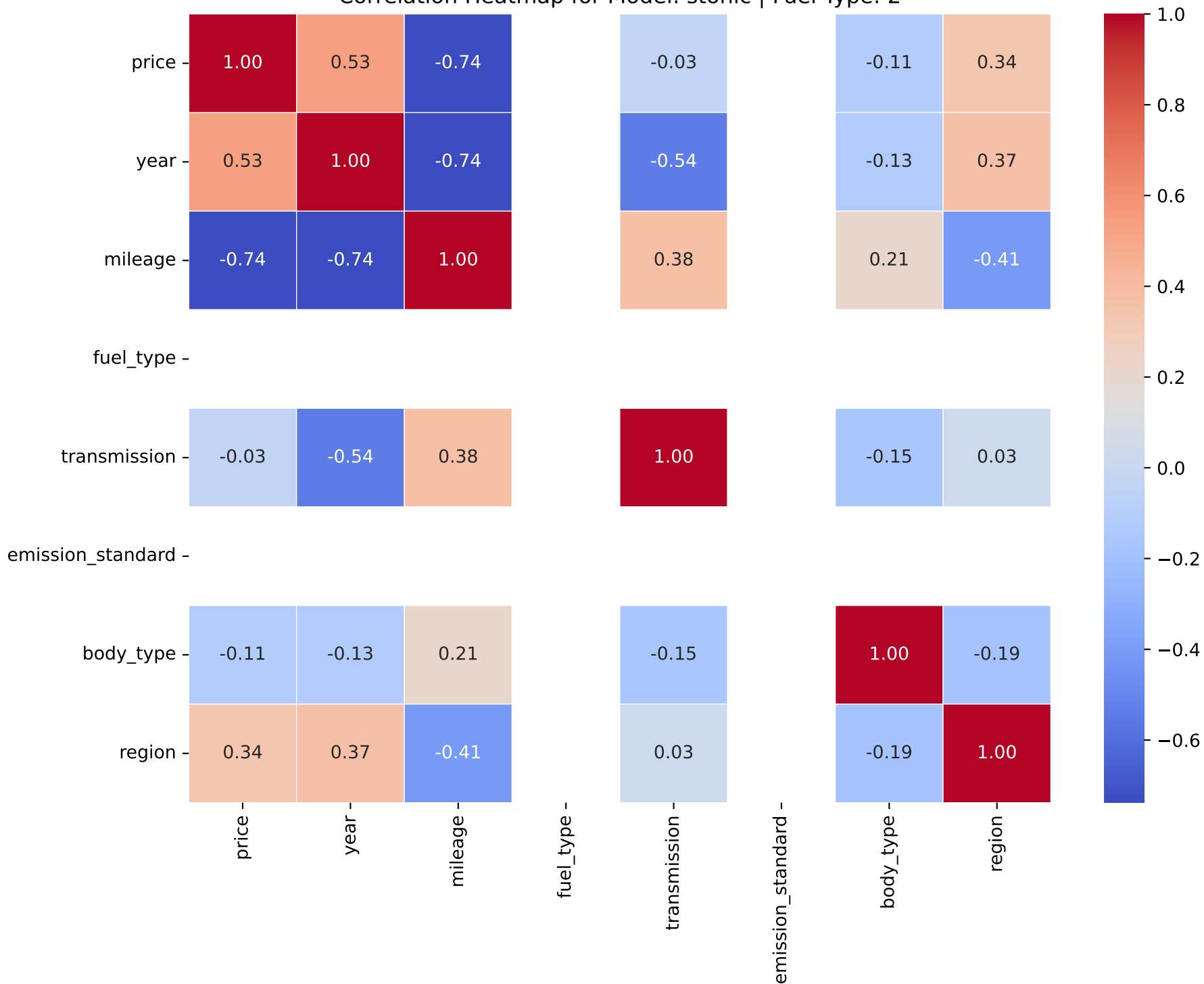
Correlation Heatmap for Model: stonic | Fuel Type: 2
