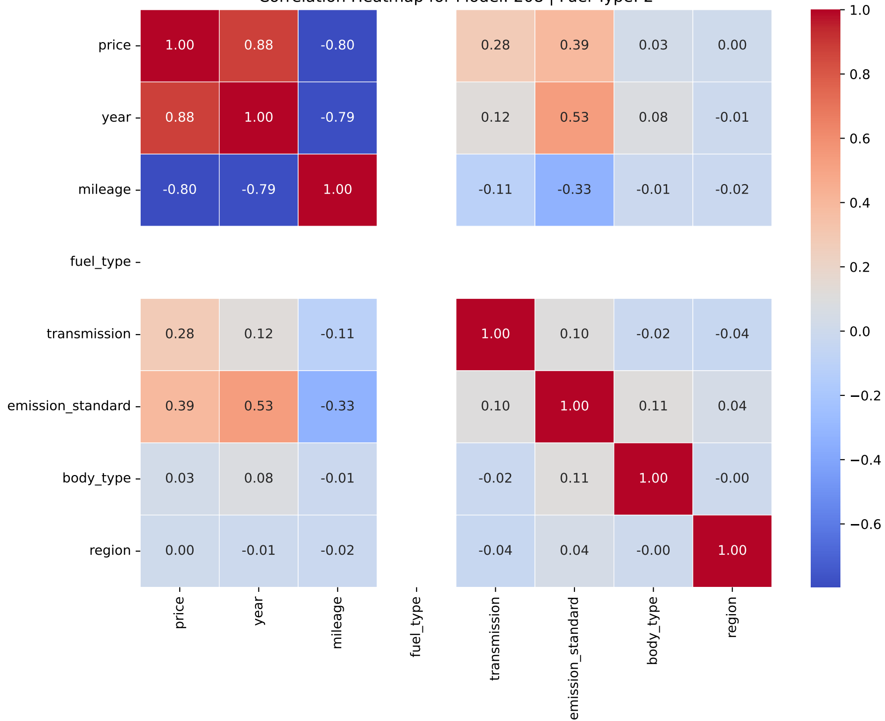
Correlation Heatmap for Model: 208 | Fuel Type: 2
