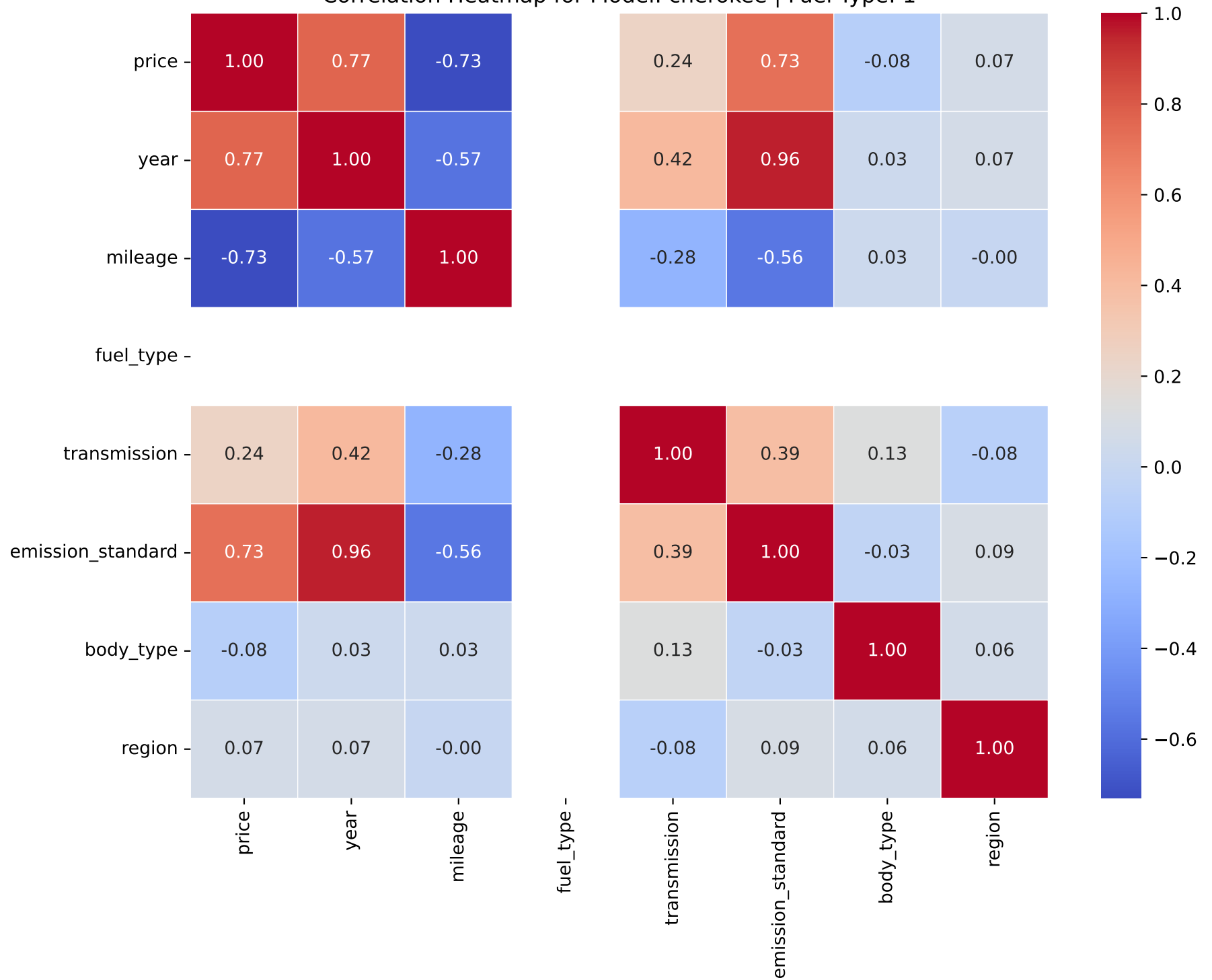
Correlation Heatmap for Model: cherokee | Fuel Type: 1
