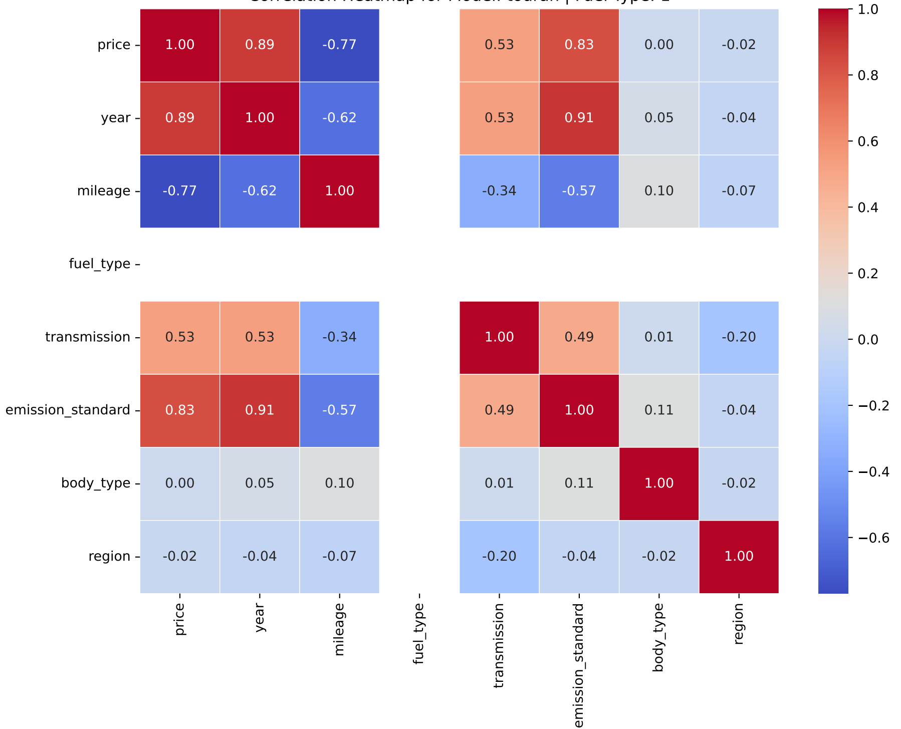
Correlation Heatmap for Model: touran | Fuel Type: 1
