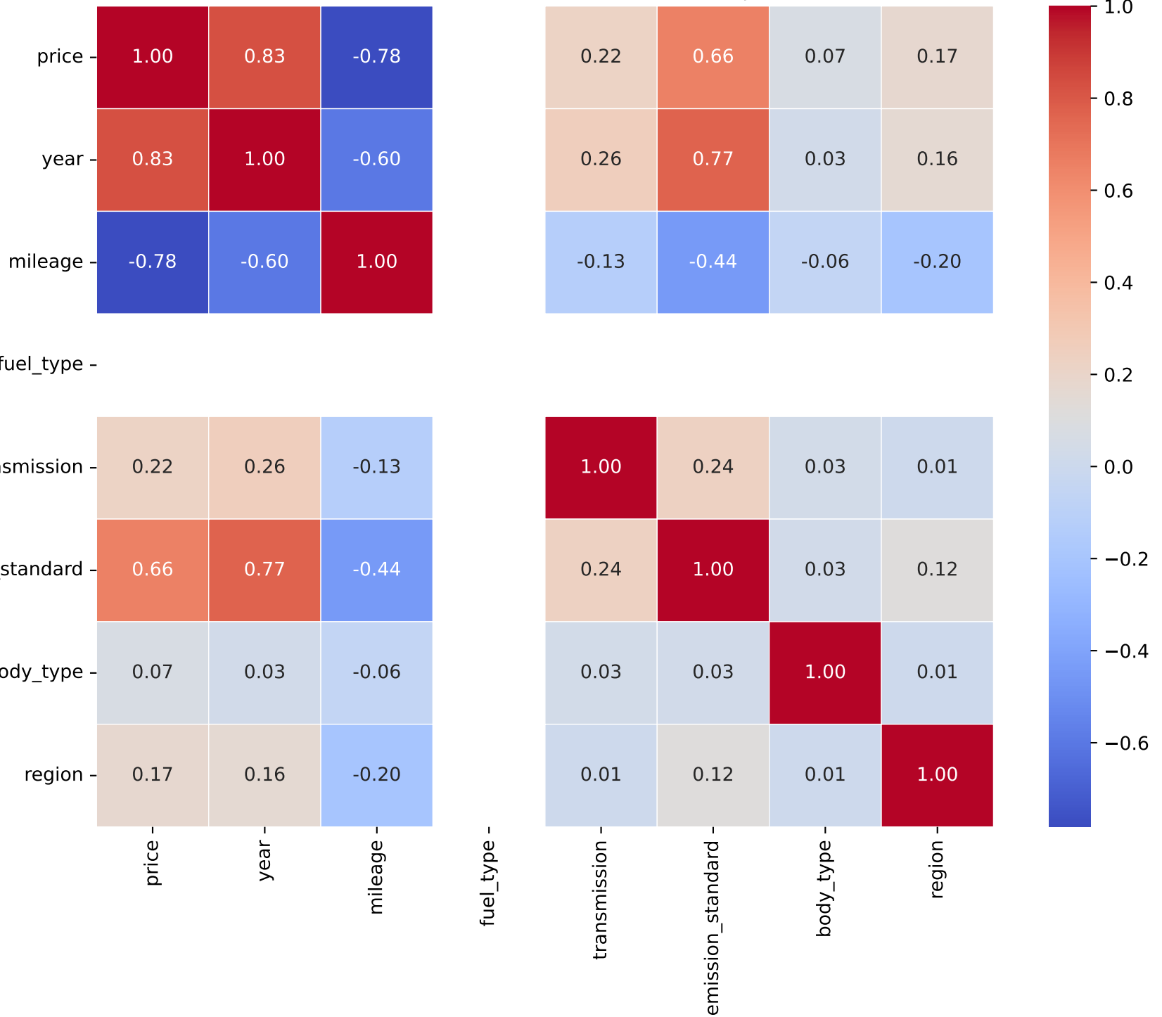
Correlation Heatmap for Model: romeo giulietta | Fuel Type: 1
