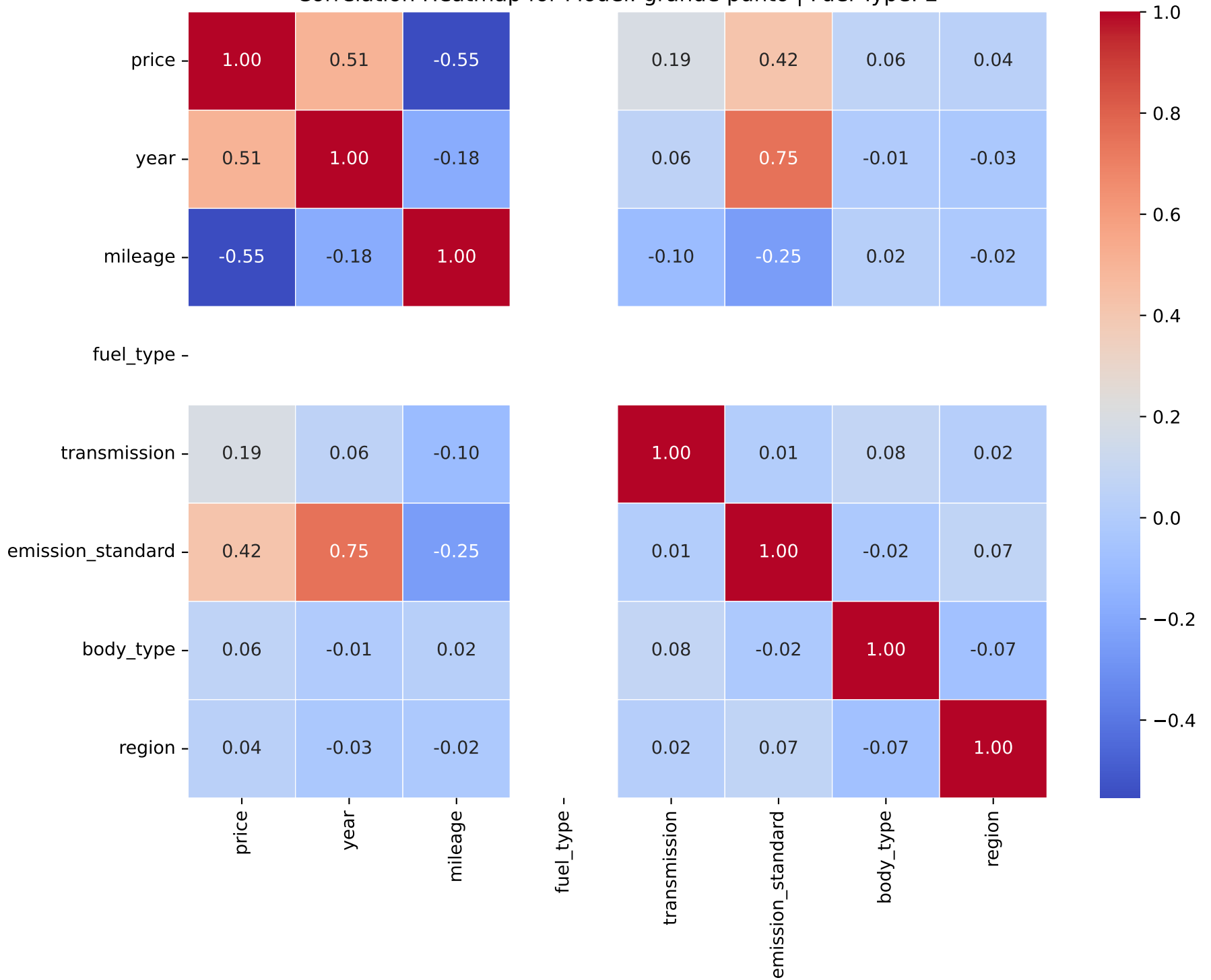
Correlation Heatmap for Model: grande punto | Fuel Type: 2
