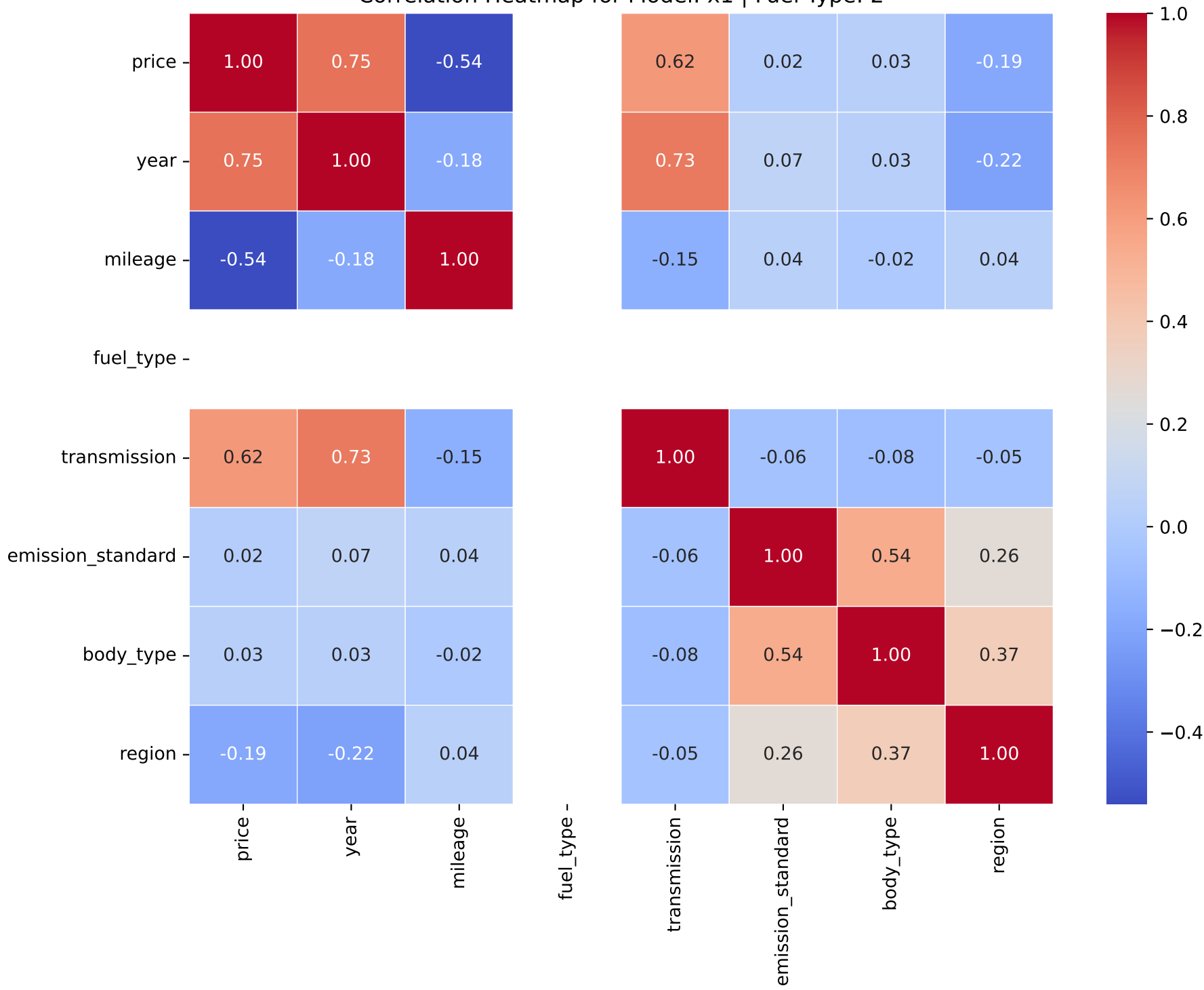
Correlation Heatmap for Model: x1 | Fuel Type: 2
