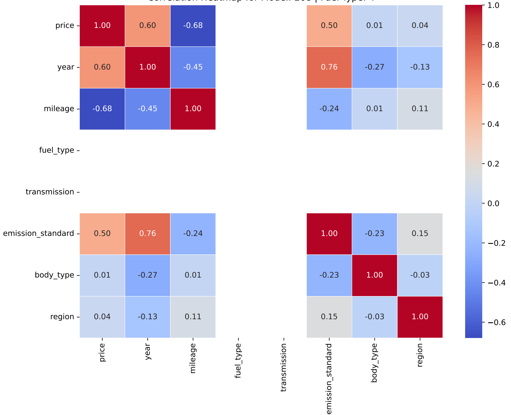
Correlation Heatmap for Model: 208 | Fuel Type: 4
