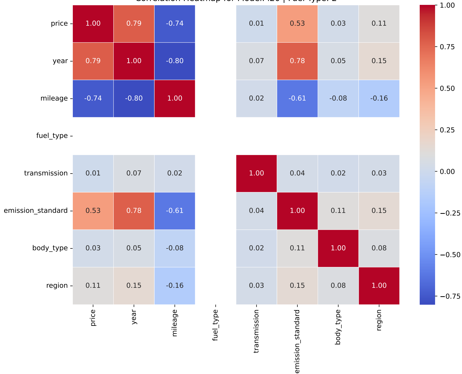
Correlation Heatmap for Model: i20 | Fuel Type: 2
