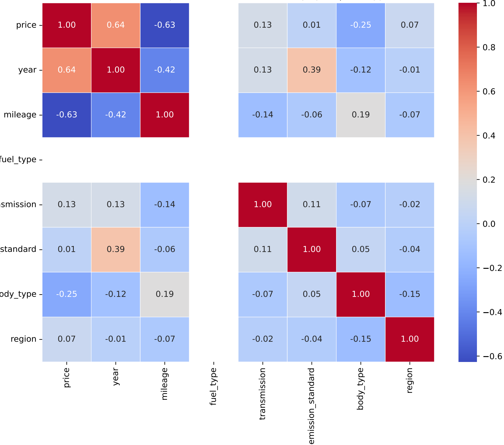
Correlation Heatmap for Model: rover discovery sport | Fuel Type: 1
