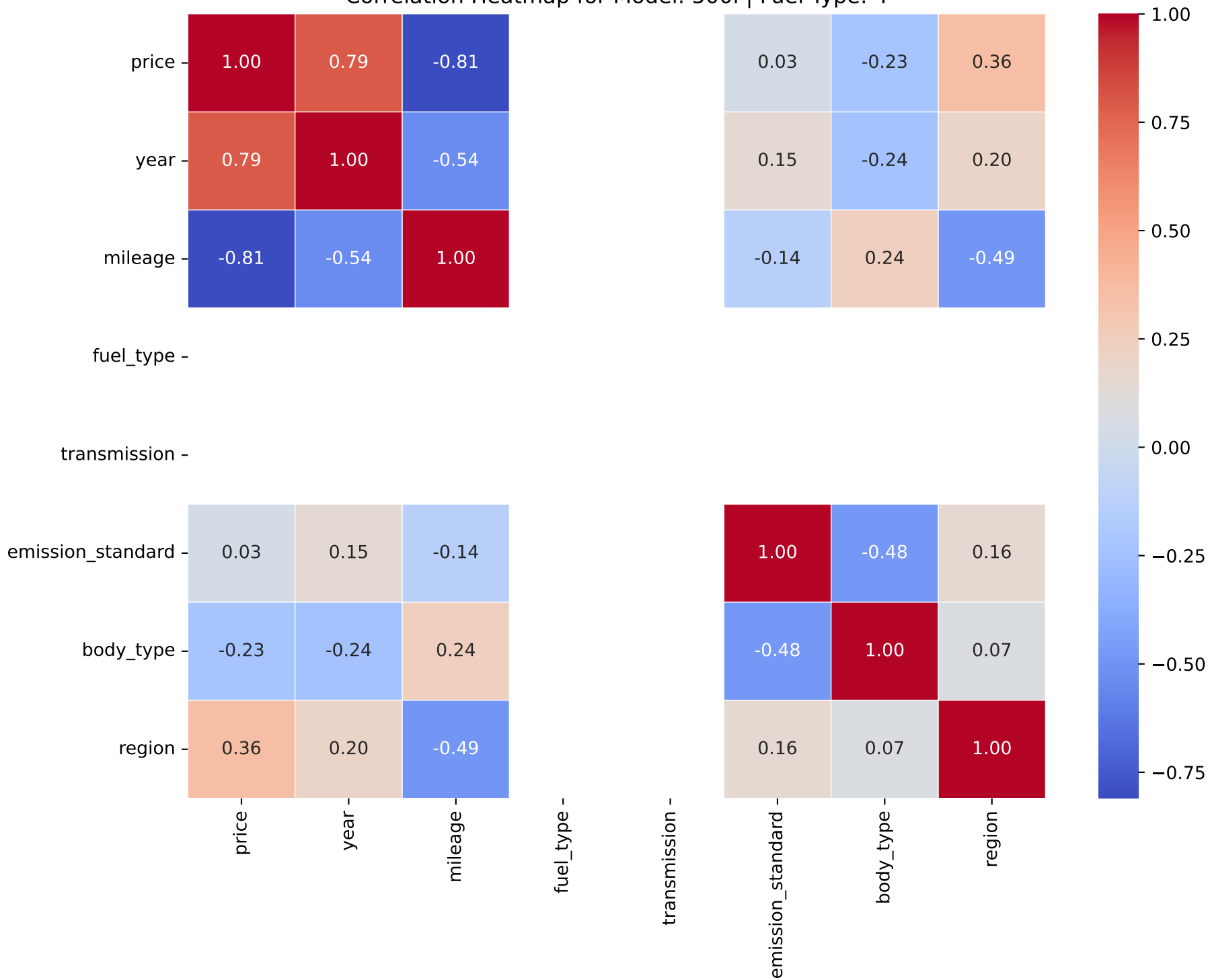
Correlation Heatmap for Model: 500I | Fuel Type: 4
