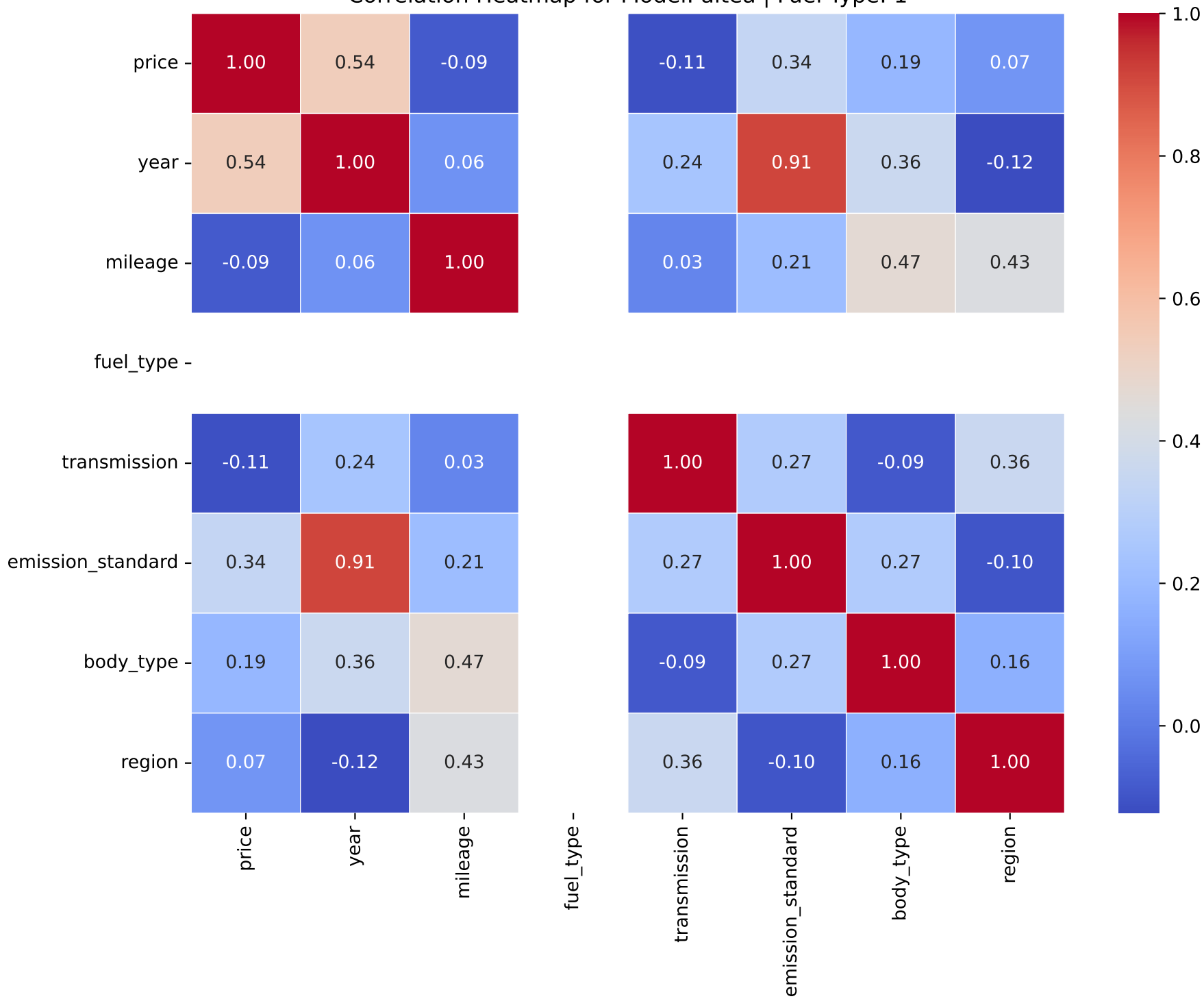
Correlation Heatmap for Model: altea | Fuel Type: 1
