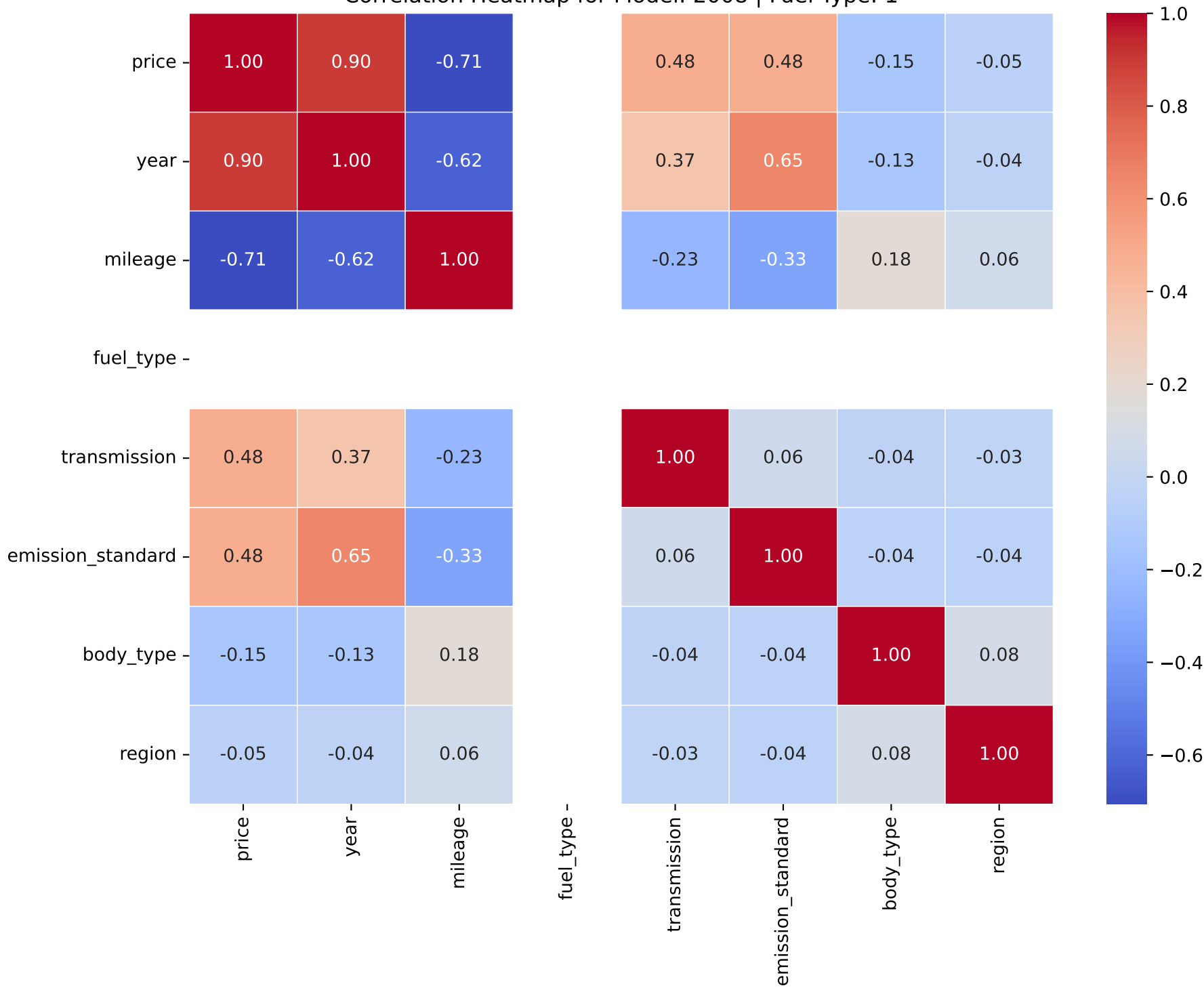
Correlation Heatmap for Model: 2008 | Fuel Type: 1
