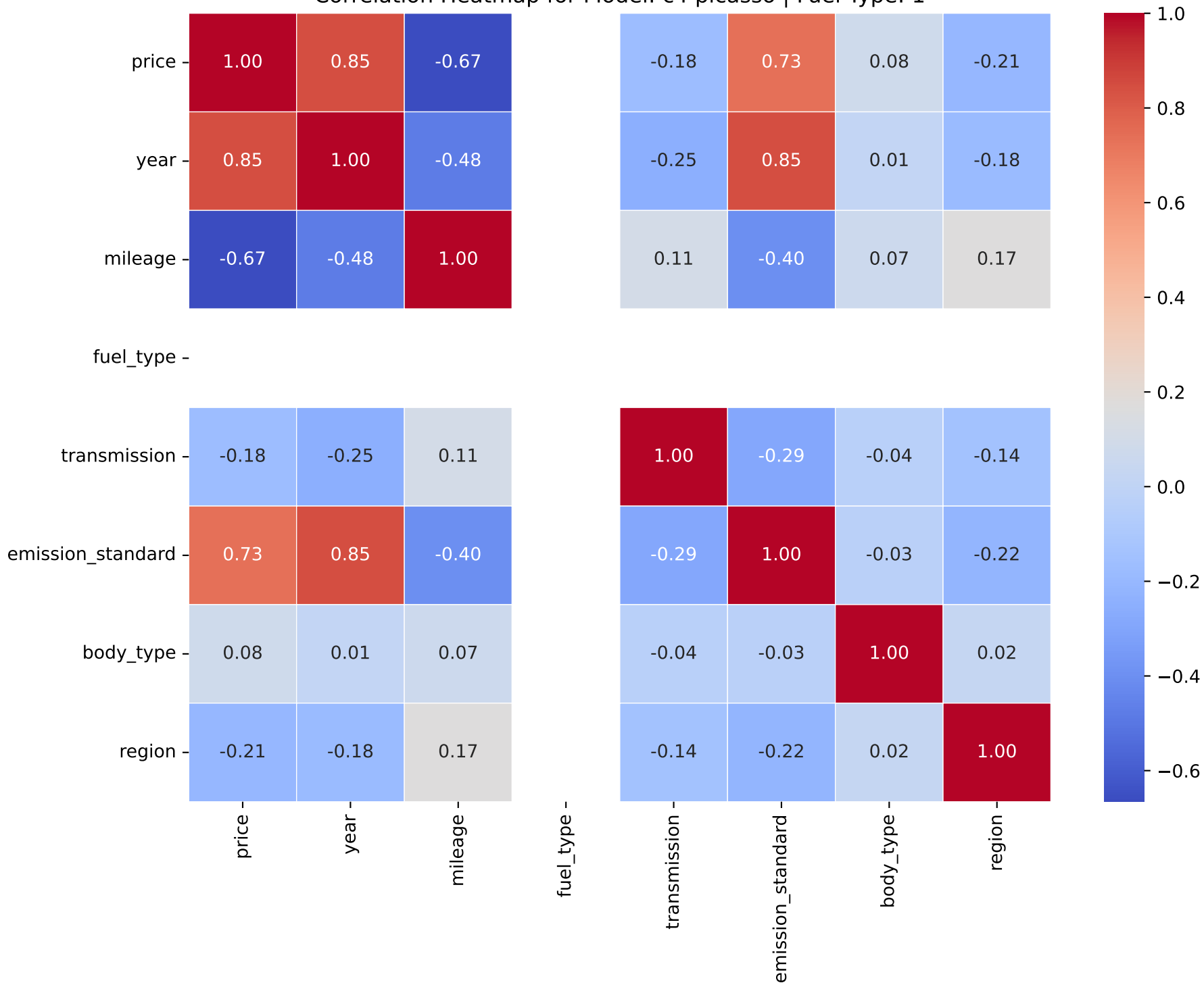
Correlation Heatmap for Model: c4 picasso | Fuel Type: 1
