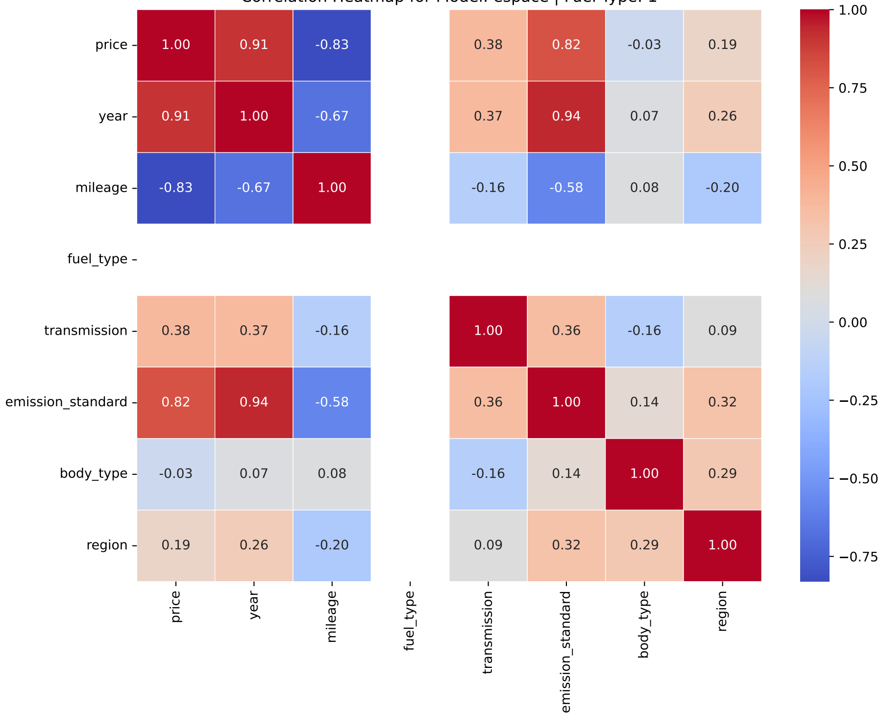
Correlation Heatmap for Model: espace | Fuel Type: 1
