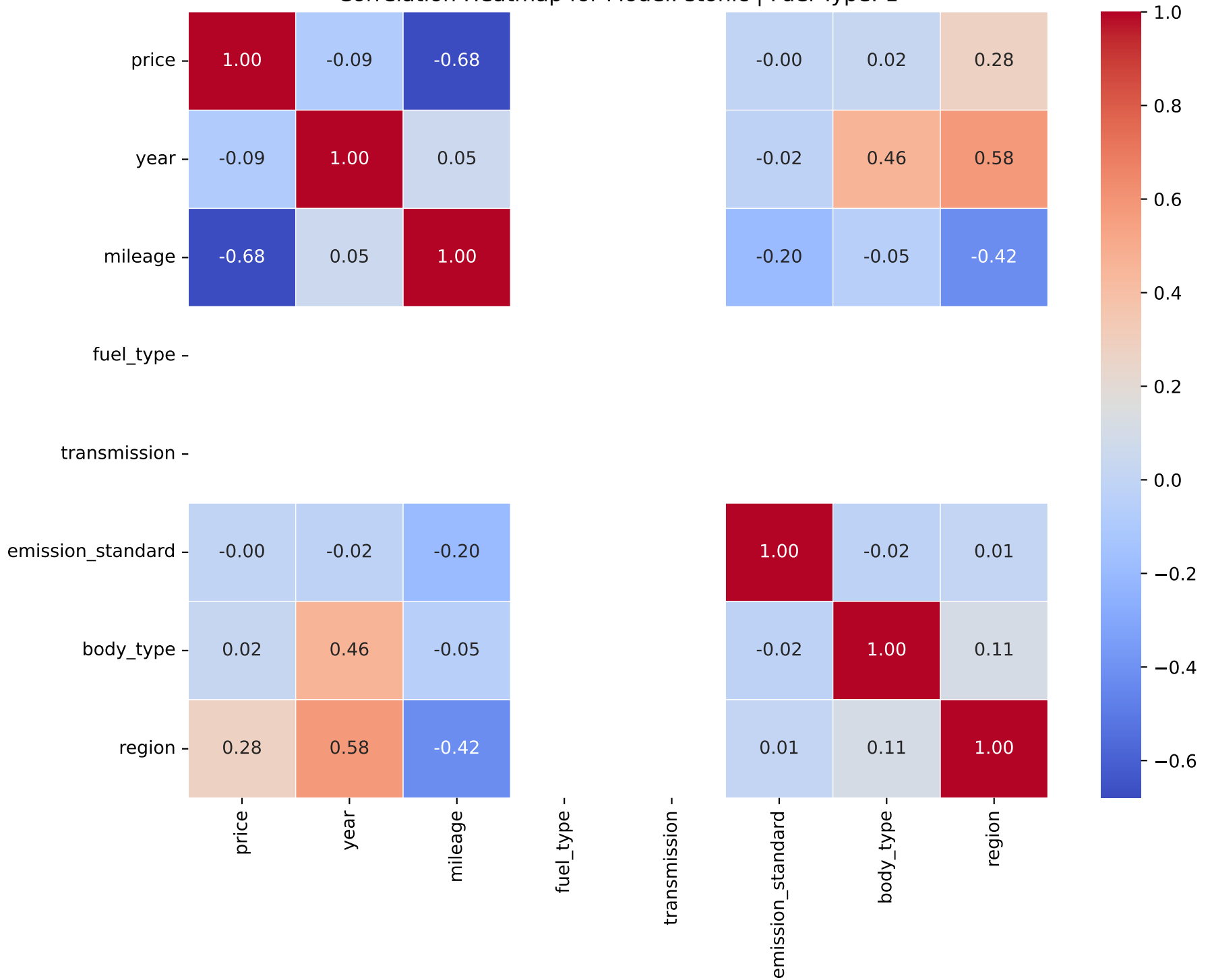
Correlation Heatmap for Model: stonic | Fuel Type: 1
