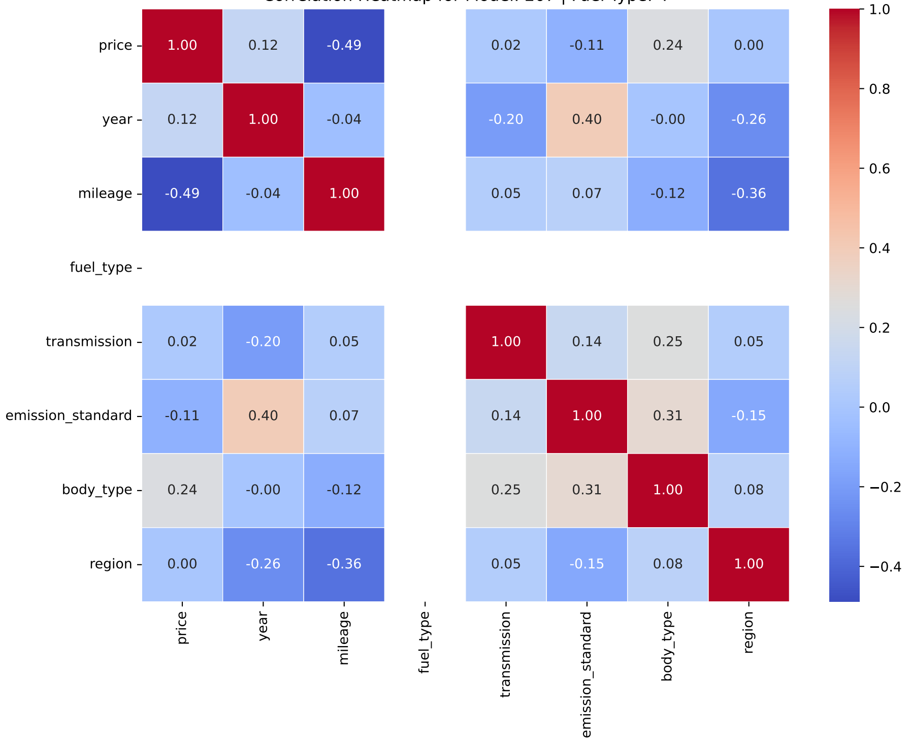
Correlation Heatmap for Model: 207 | Fuel Type: 4
