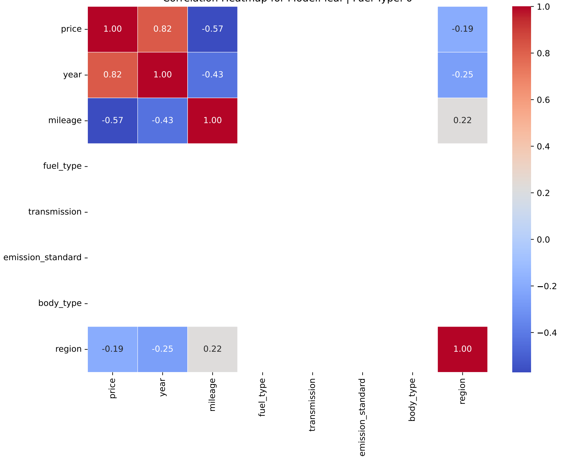
Correlation Heatmap for Model: leaf | Fuel Type: 0
