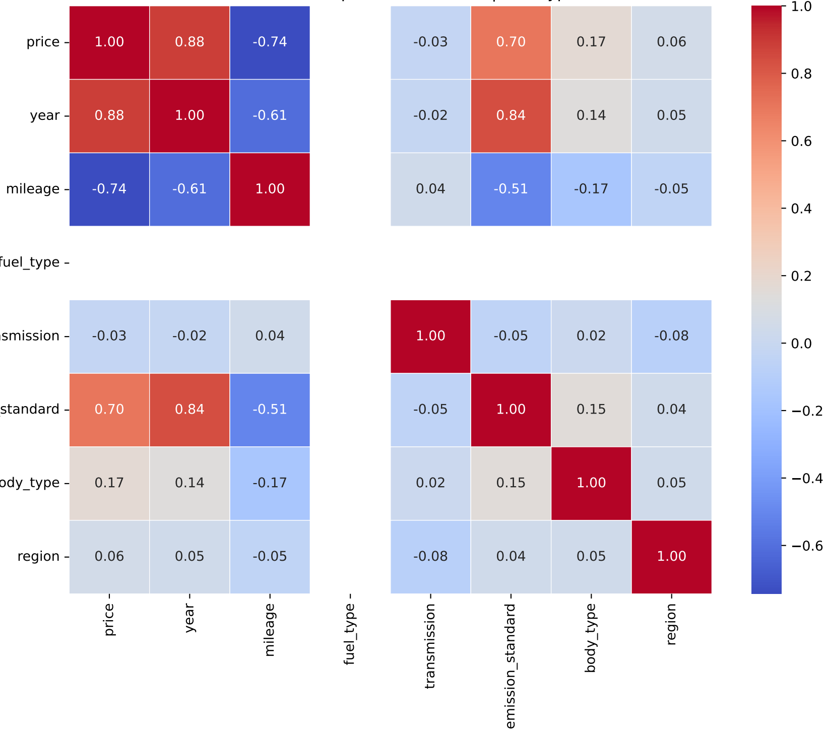
Correlation Heatmap for Model: corsa | Fuel Type: 1
