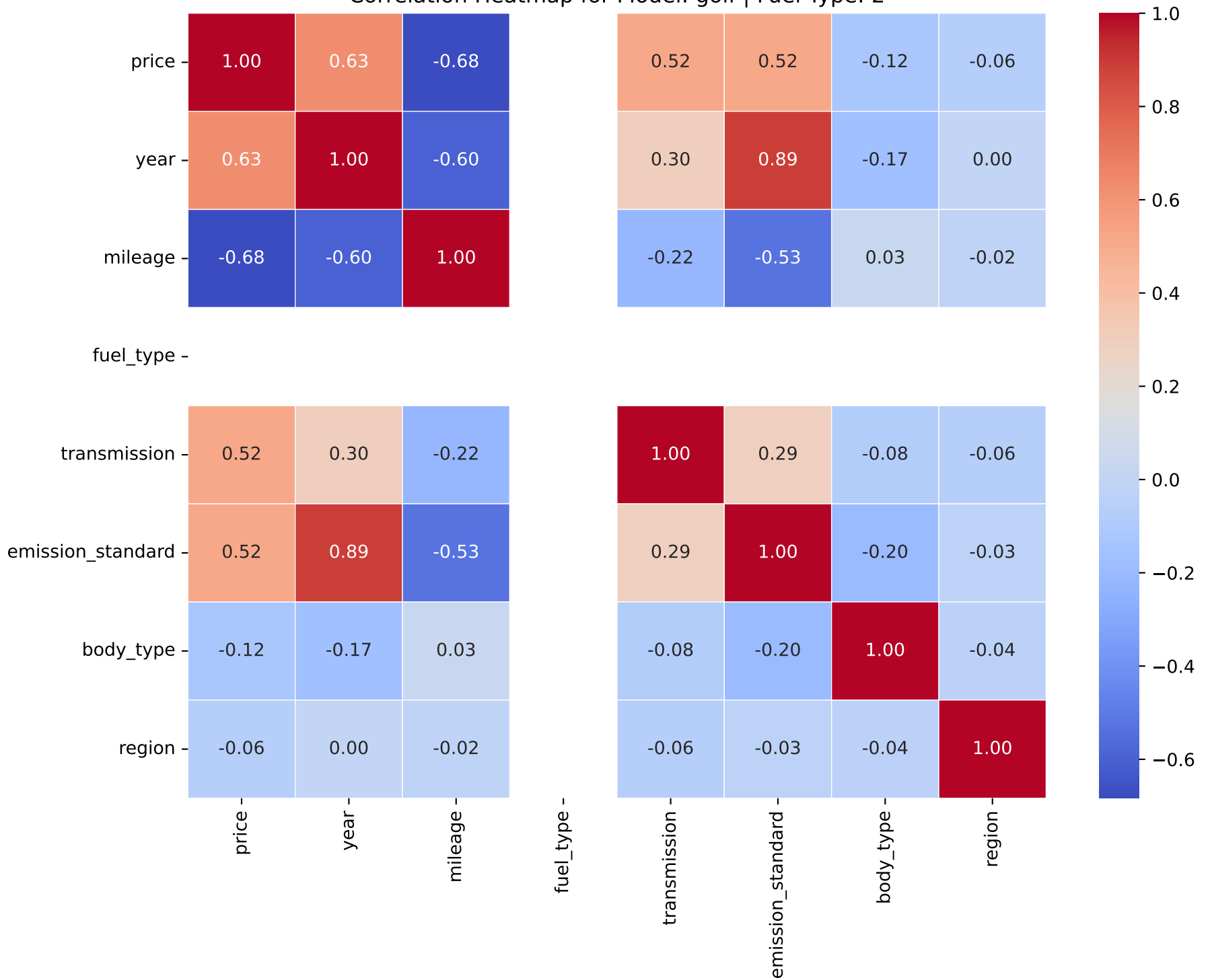
Correlation Heatmap for Model: golf | Fuel Type: 2
