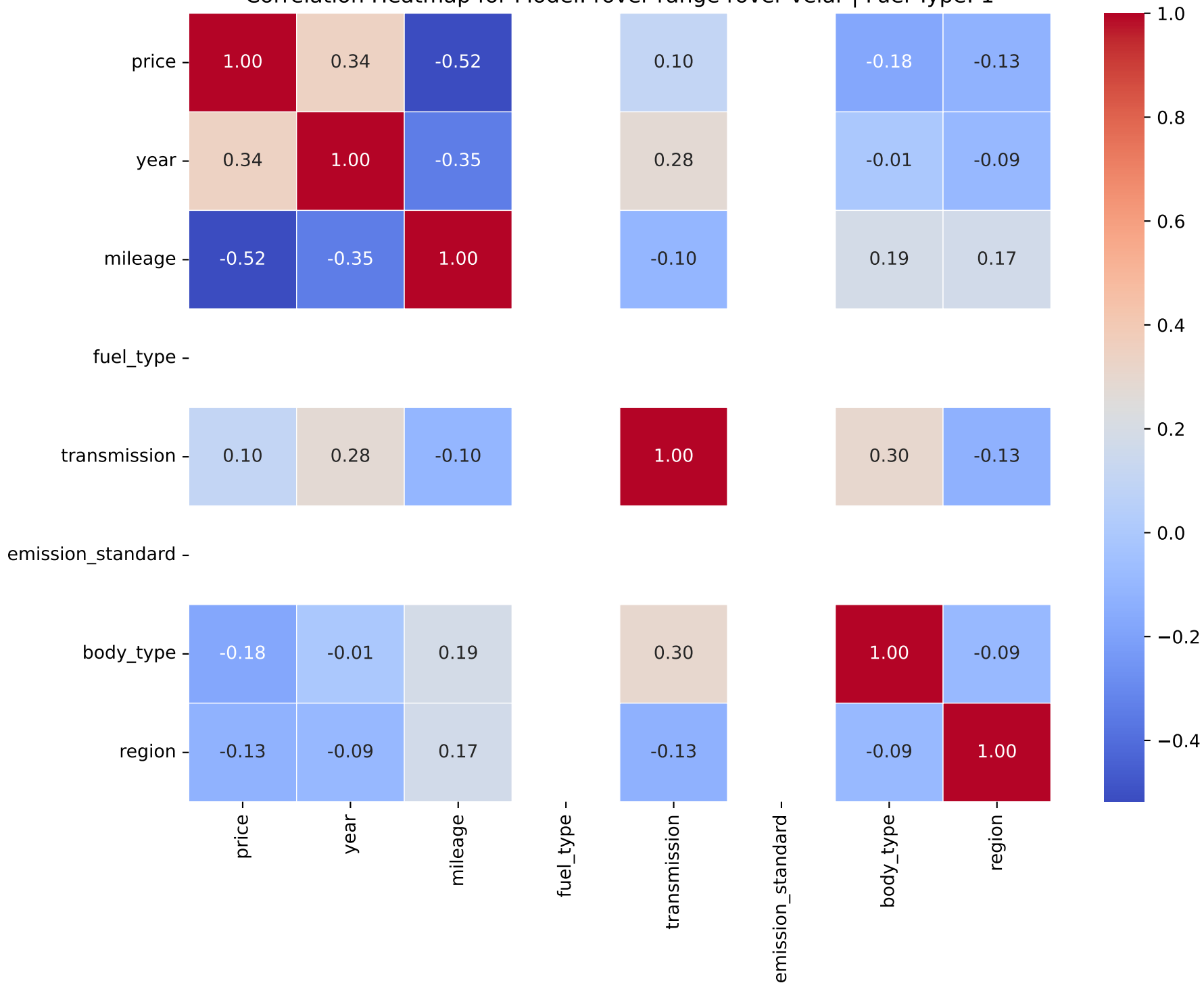
Correlation Heatmap for Model: rover range rover velar | Fuel Type: 1
