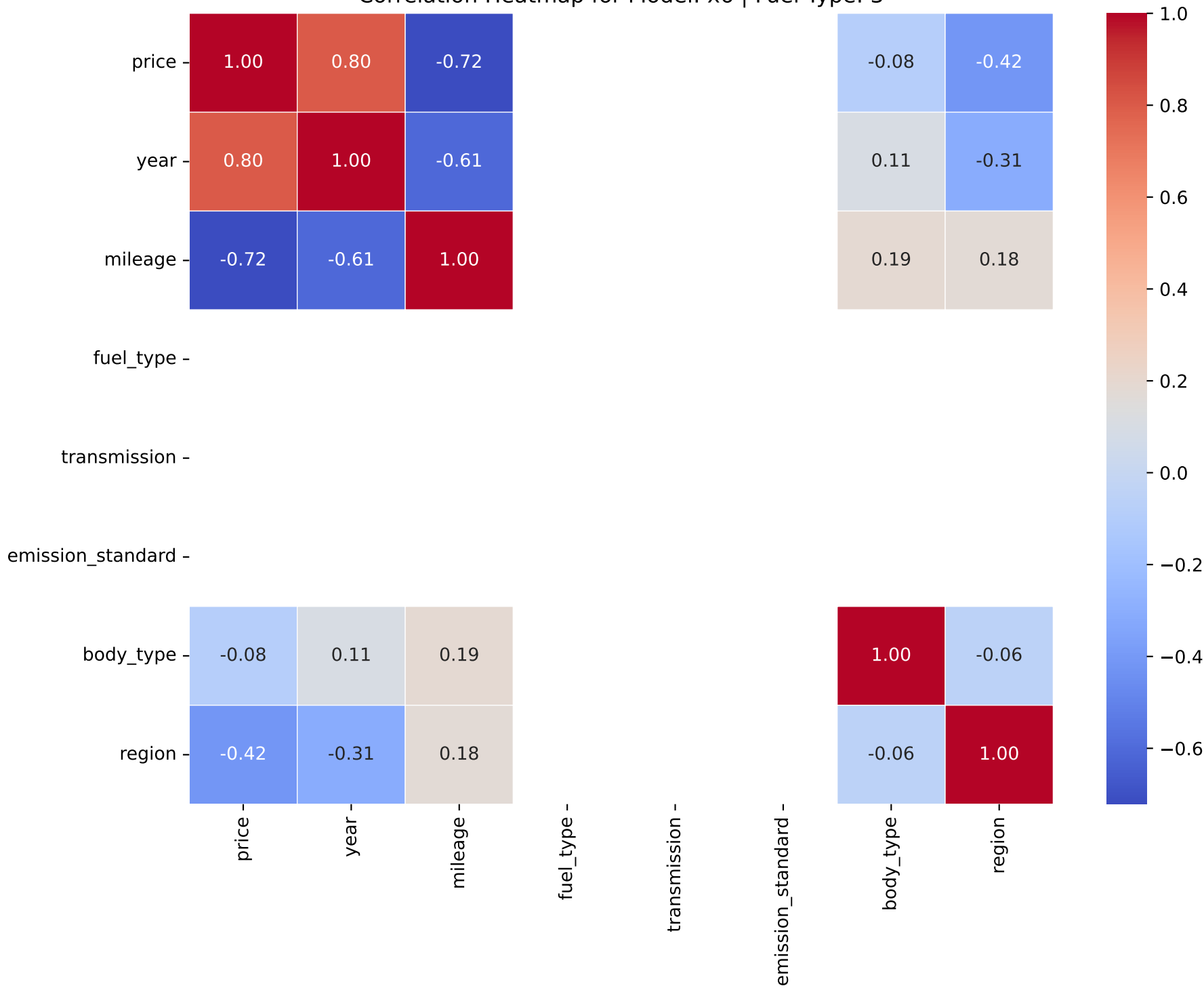
Correlation Heatmap for Model: x6 | Fuel Type: 3
