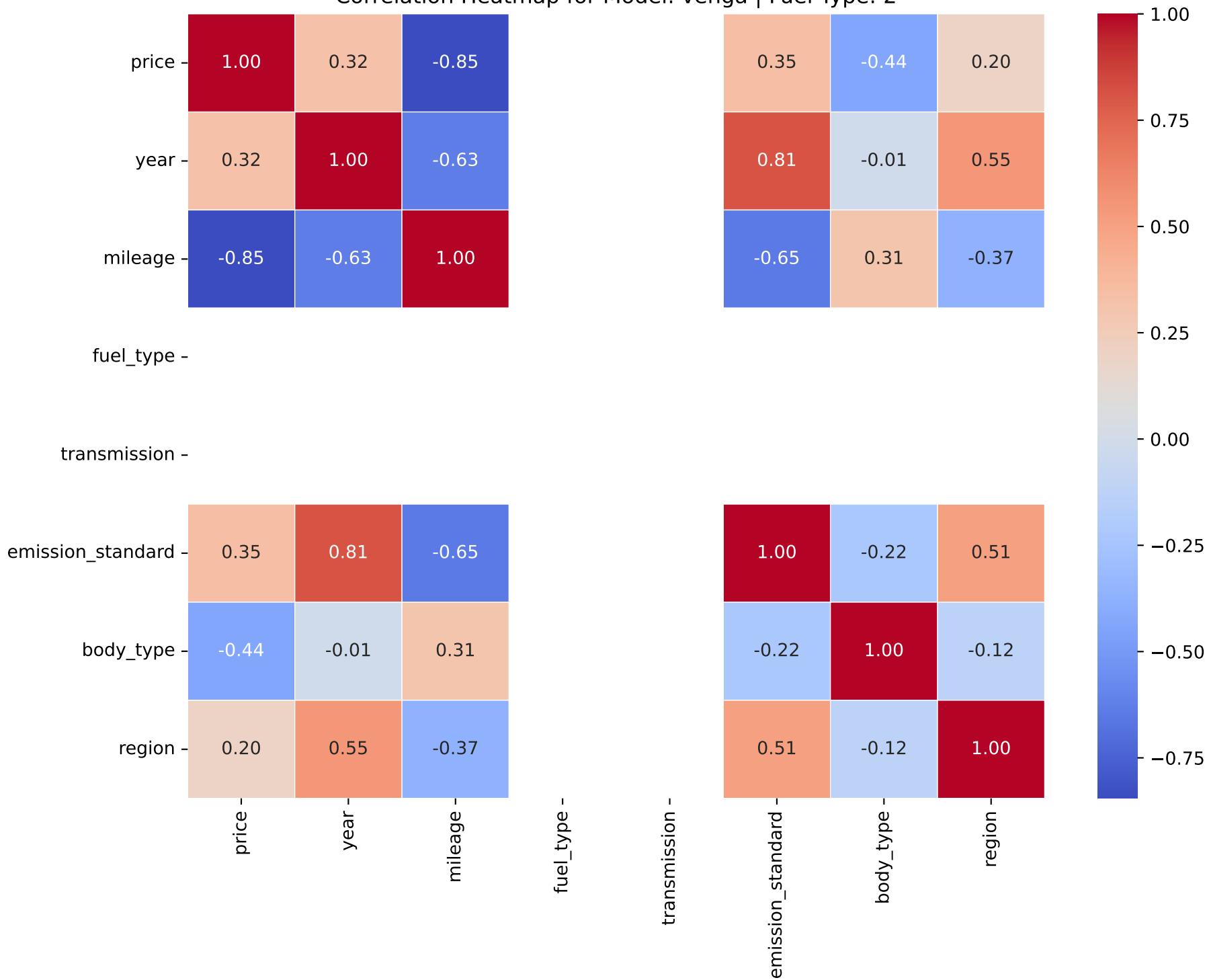
Correlation Heatmap for Model: venga | Fuel Type: 2
