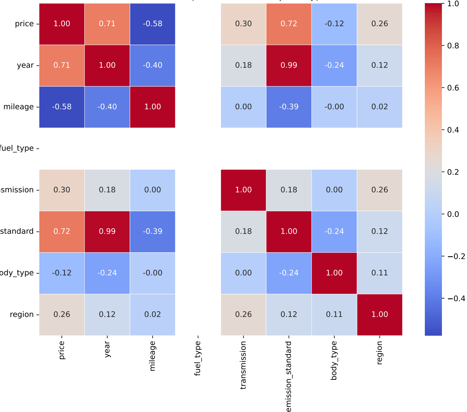
Correlation Heatmap for Model: vitara | Fuel Type: 1
