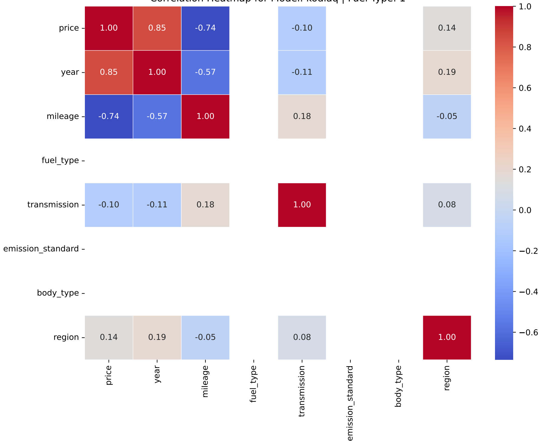
Correlation Heatmap for Model: kodiaq | Fuel Type: 1
