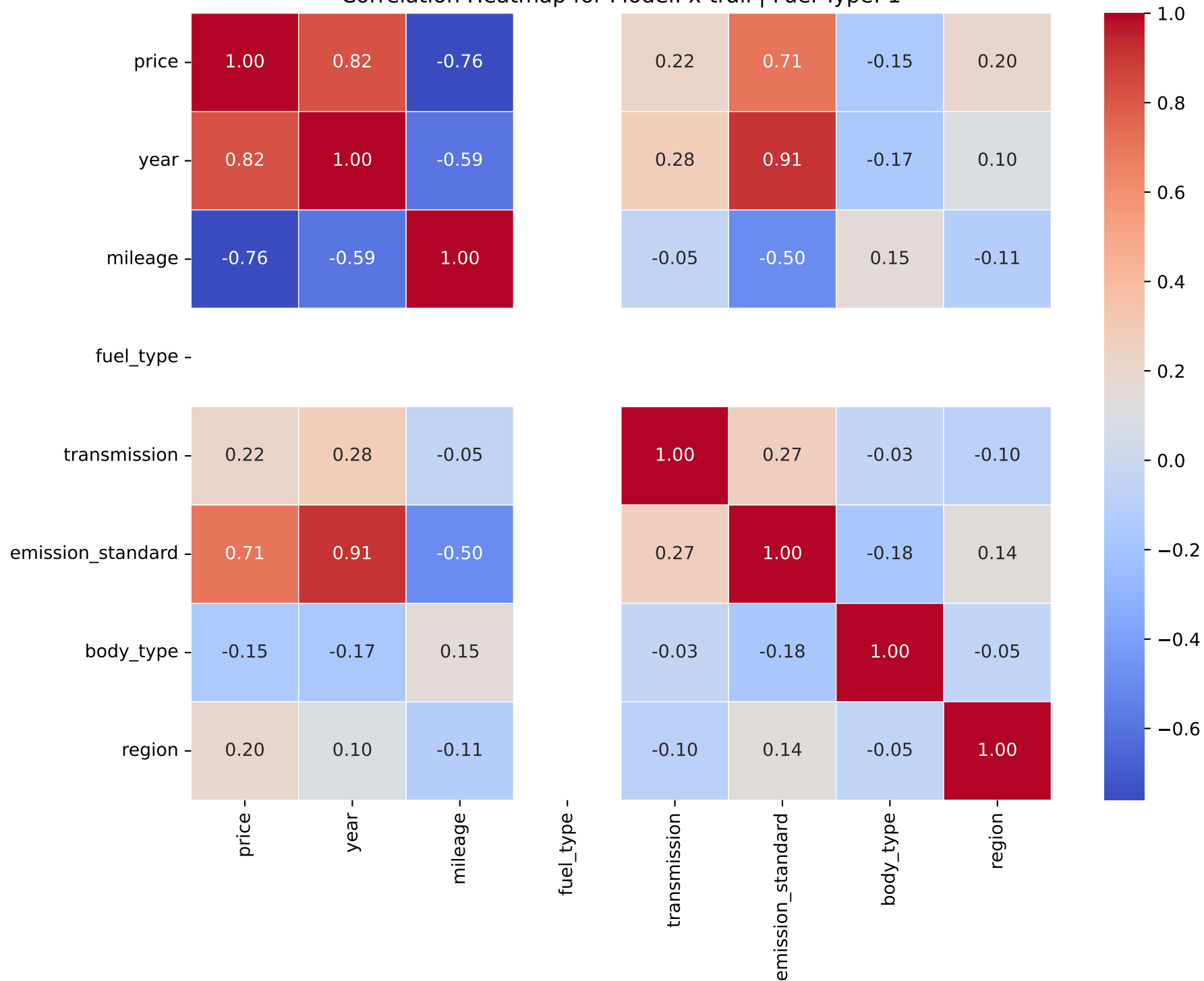
Correlation Heatmap for Model: x-trail | Fuel Type: 1
