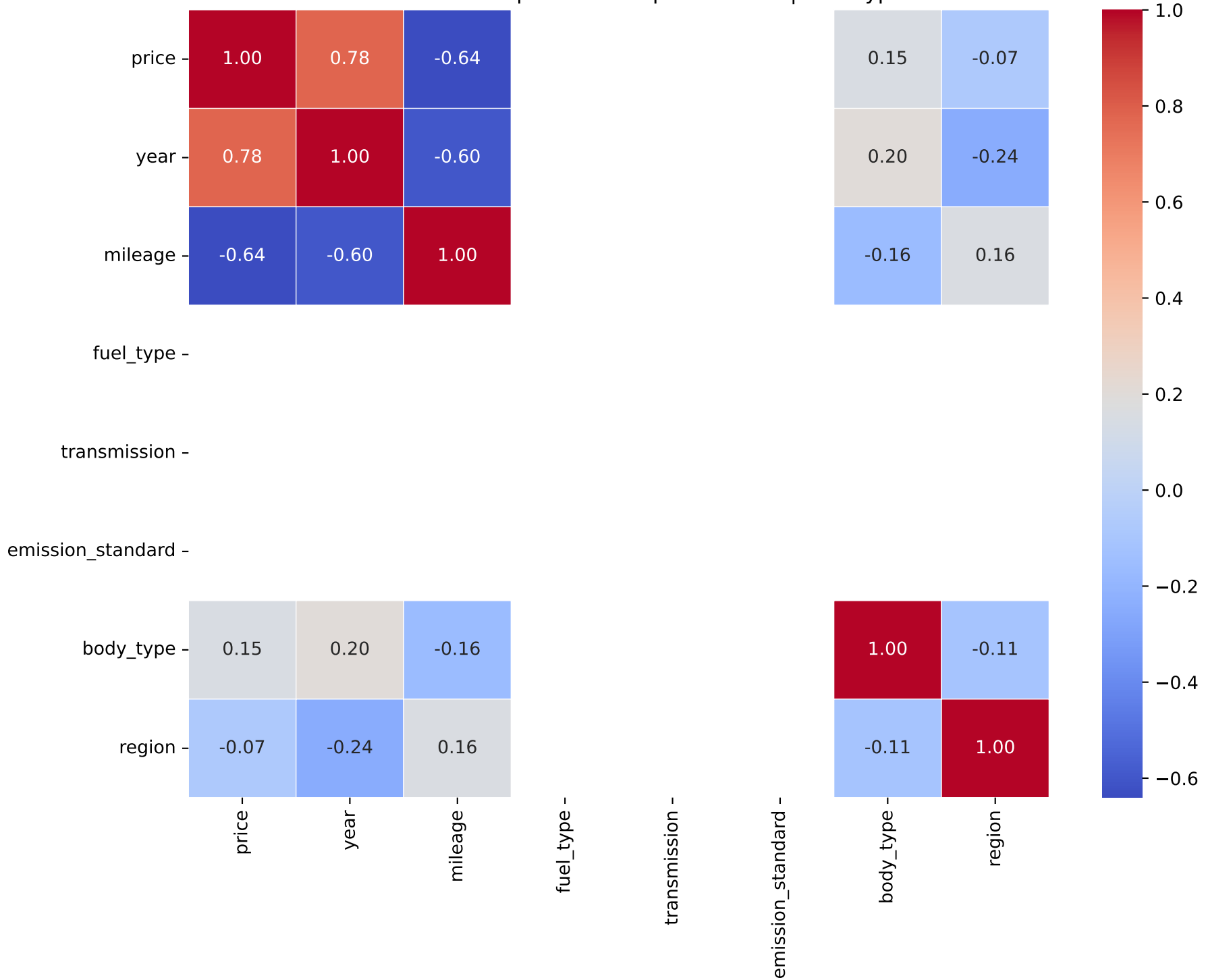
Correlation Heatmap for Model: panda cross | Fuel Type: 3
