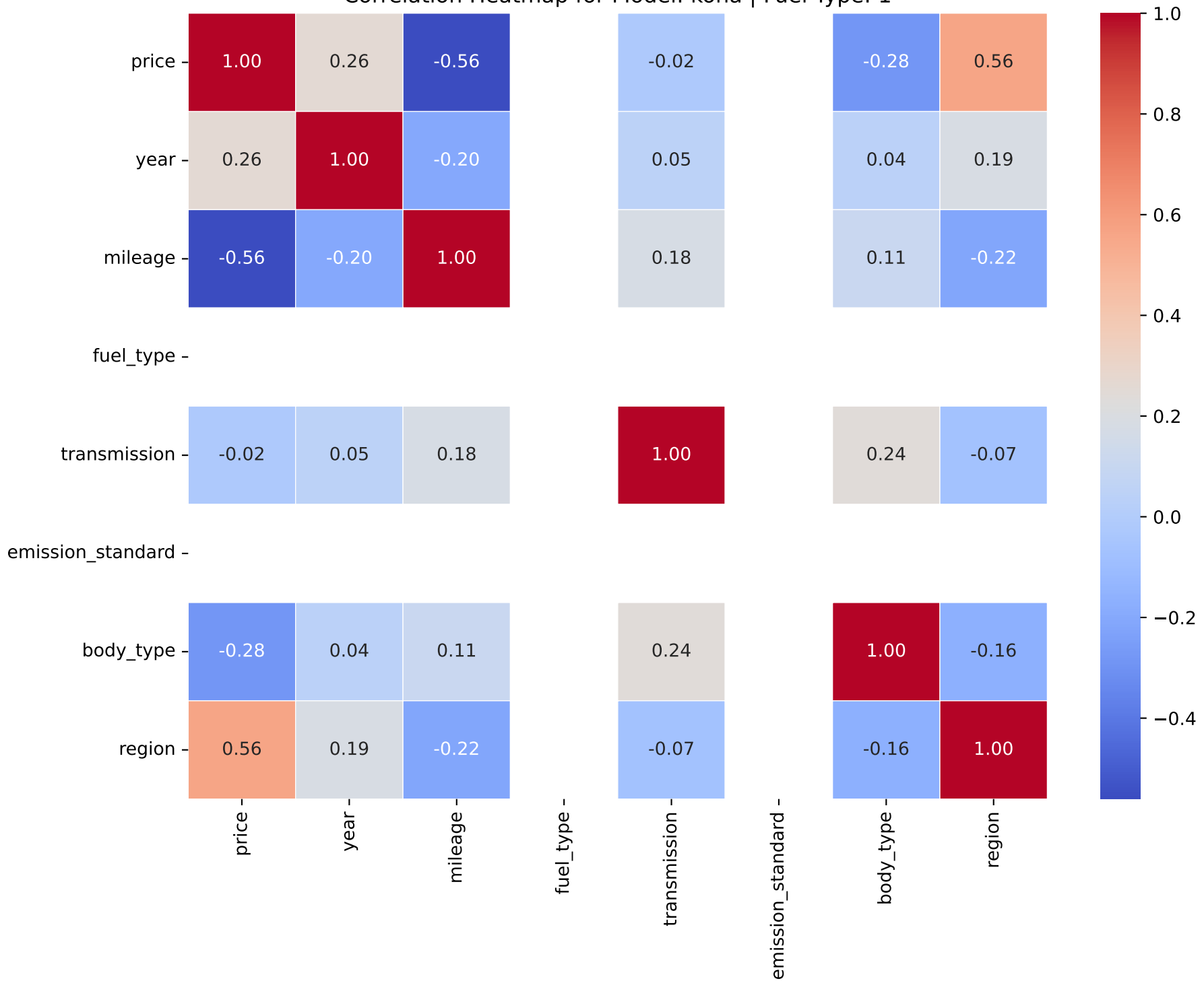
Correlation Heatmap for Model: kona | Fuel Type: 1
