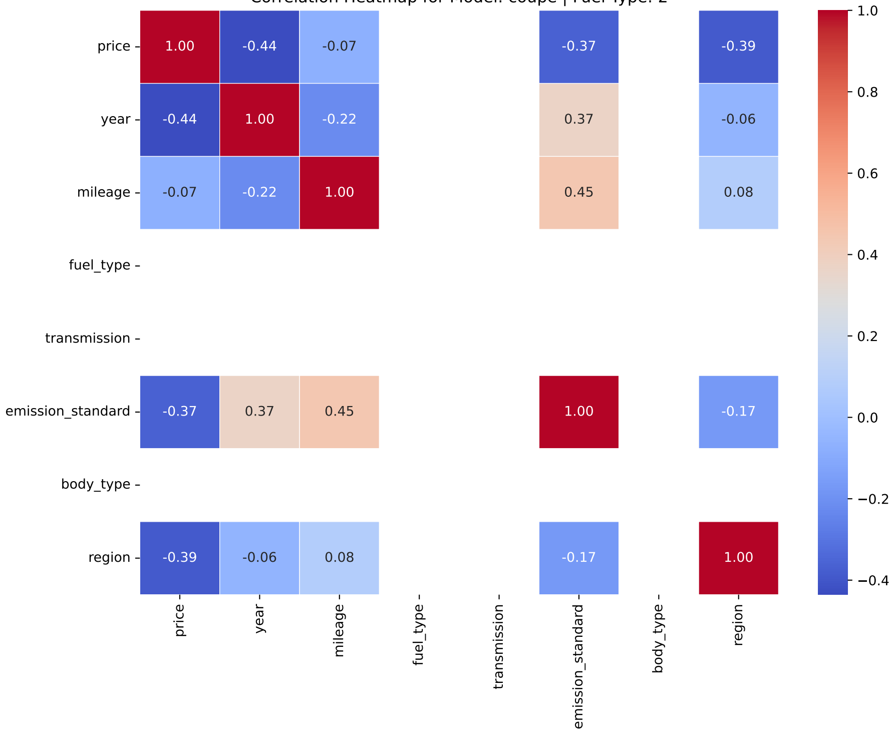
Correlation Heatmap for Model: coupe | Fuel Type: 2
