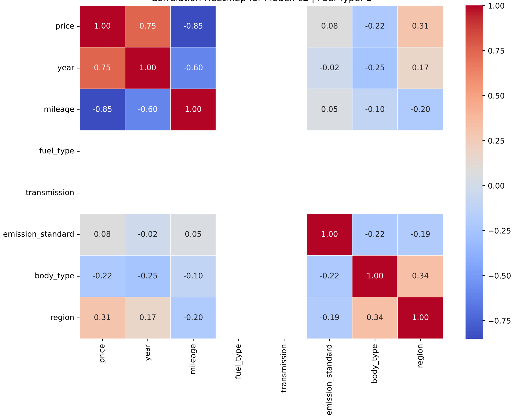
Correlation Heatmap for Model: c2 | Fuel Type: 1
