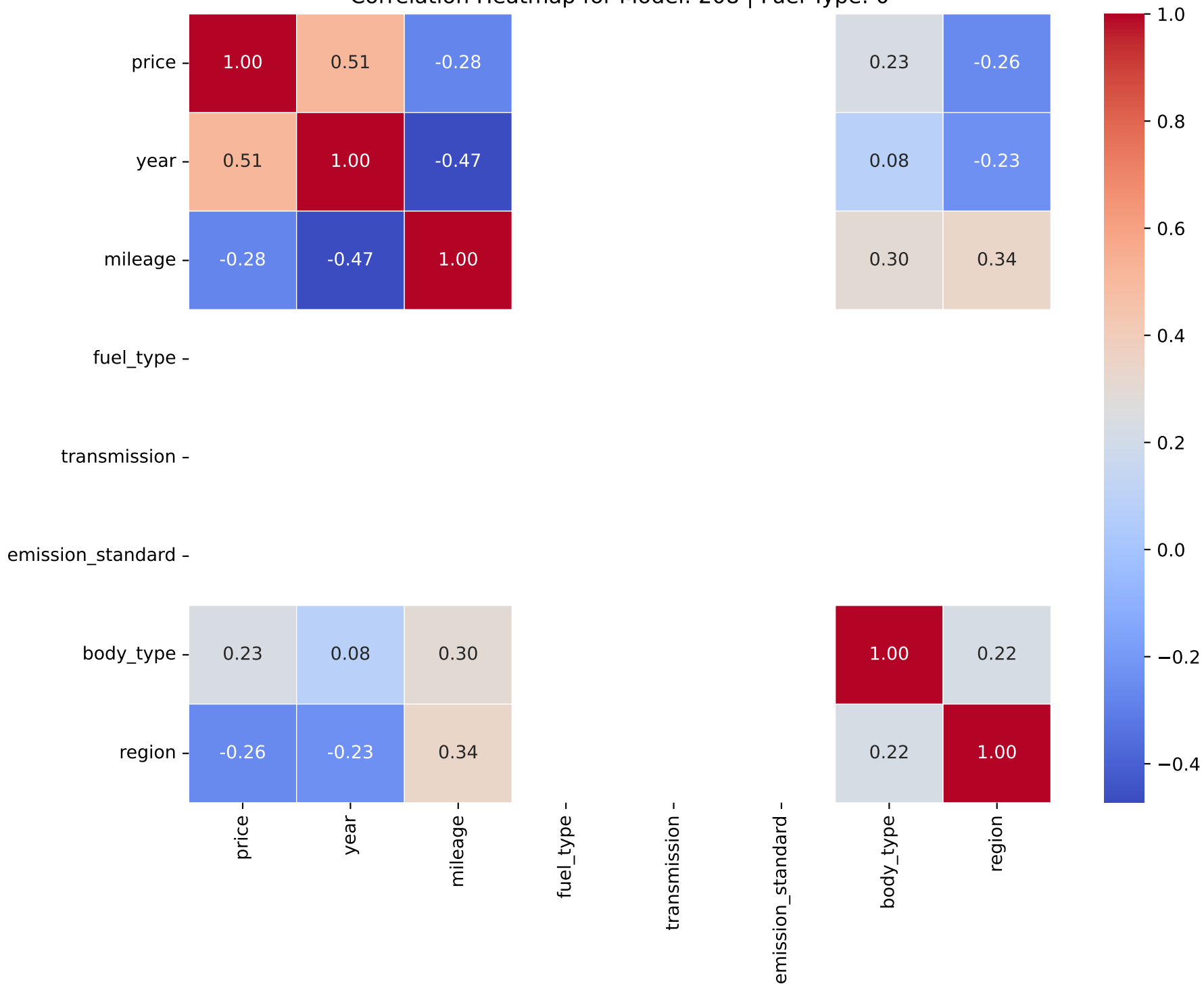
Correlation Heatmap for Model: 208 | Fuel Type: 0
