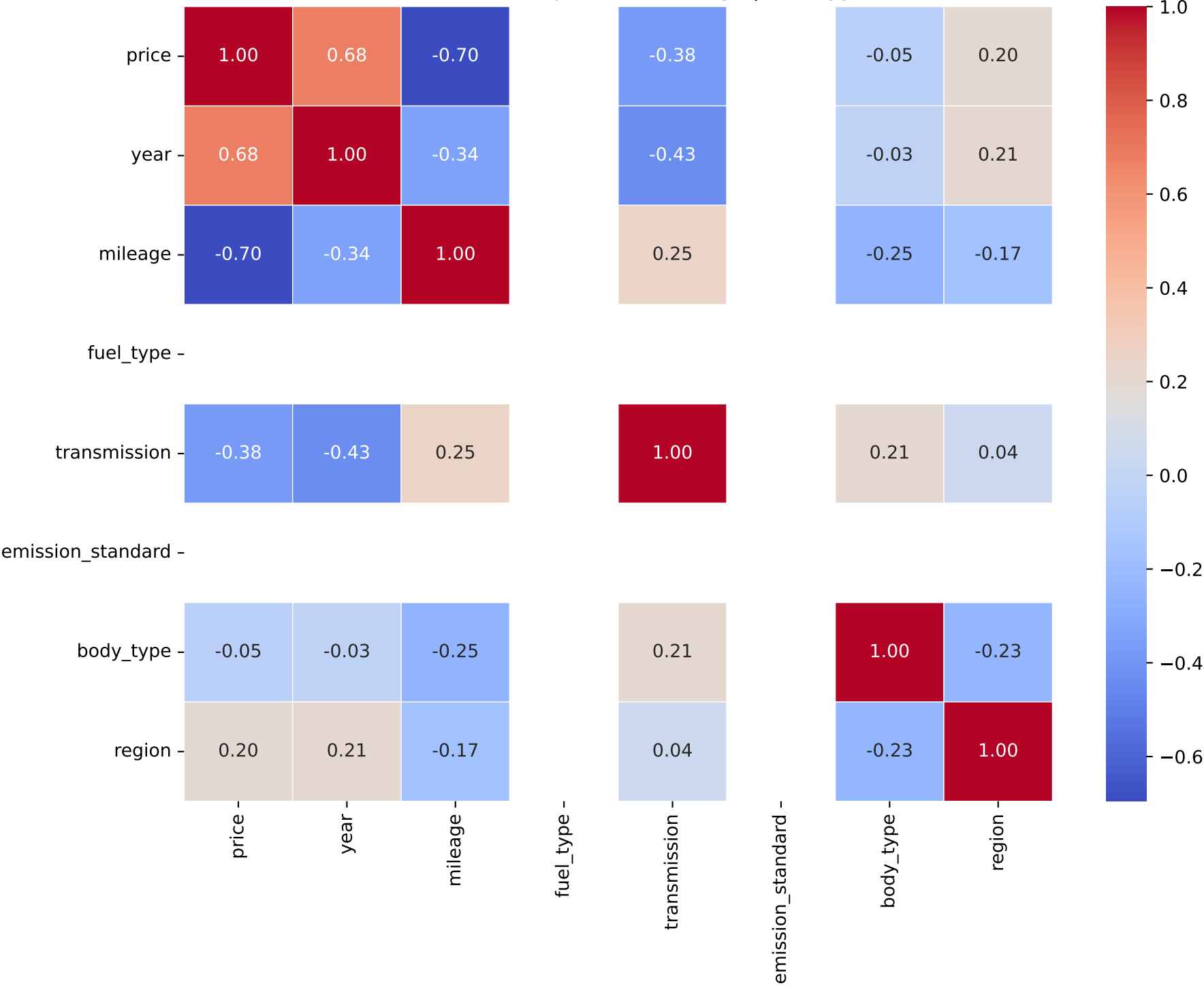
Correlation Heatmap for Model: edge | Fuel Type: 1
