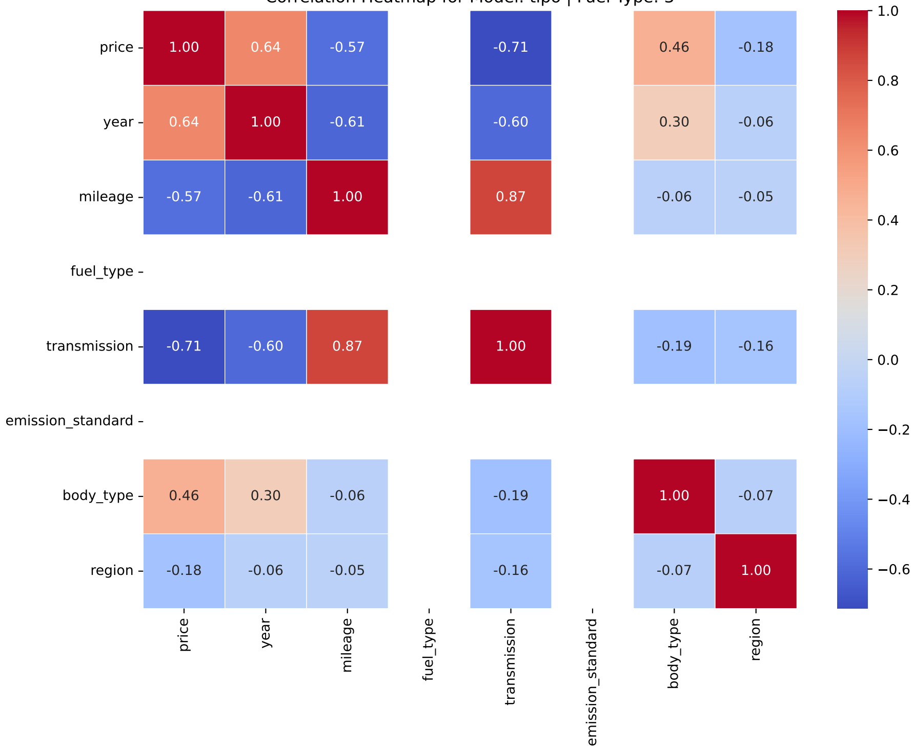
Correlation Heatmap for Model: tipo | Fuel Type: 3
