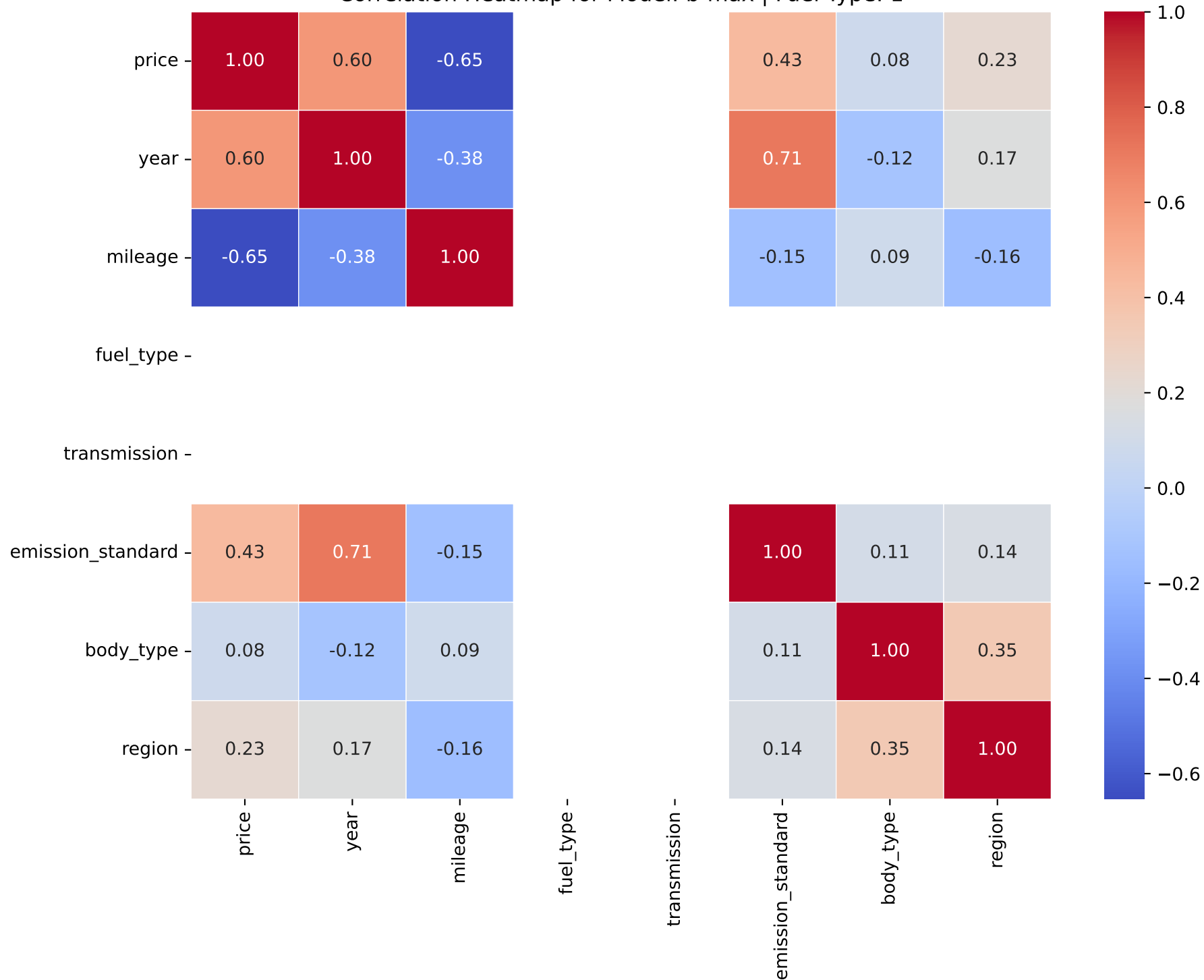
Correlation Heatmap for Model: b-max | Fuel Type: 1
