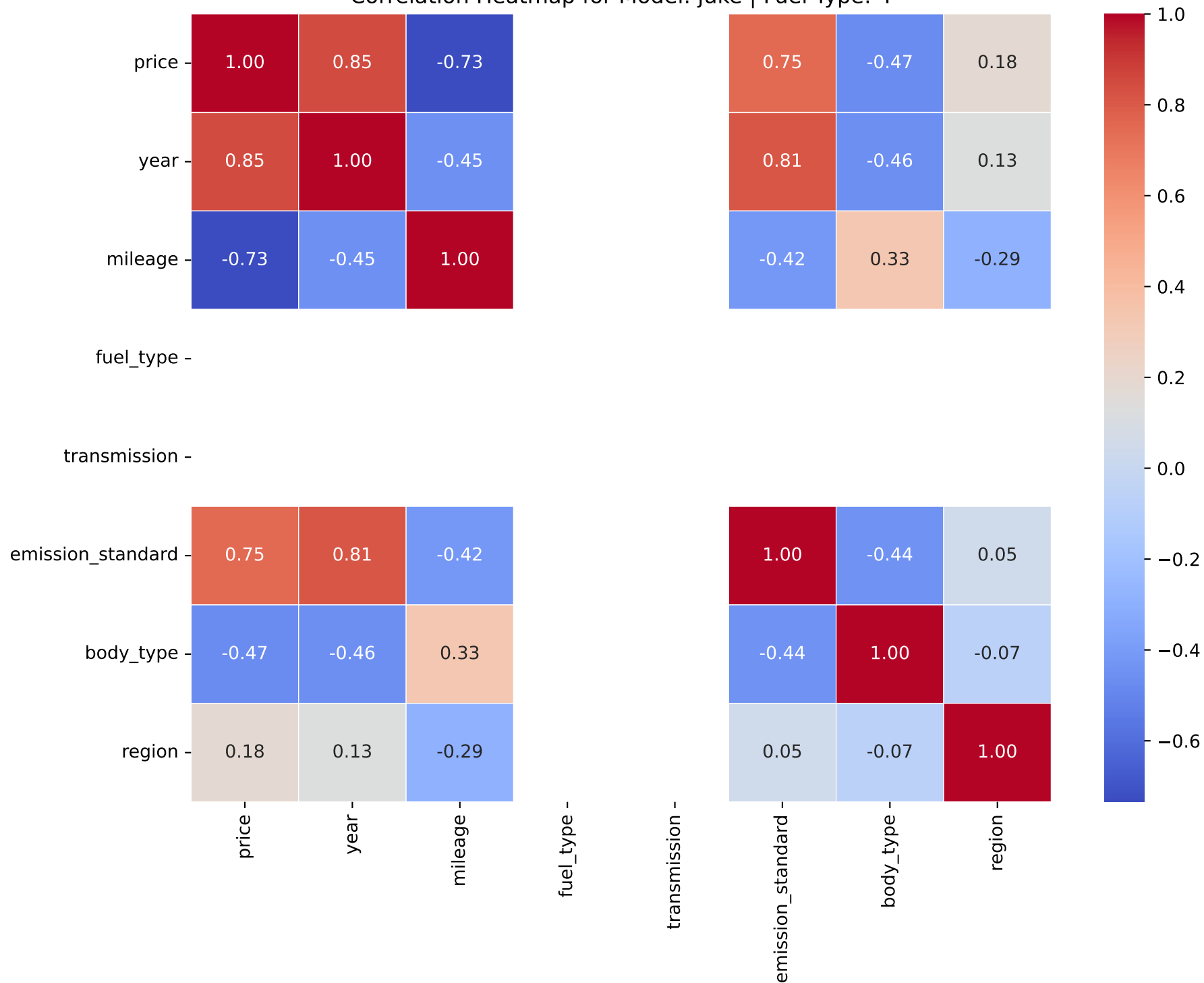
Correlation Heatmap for Model: juke | Fuel Type: 4
