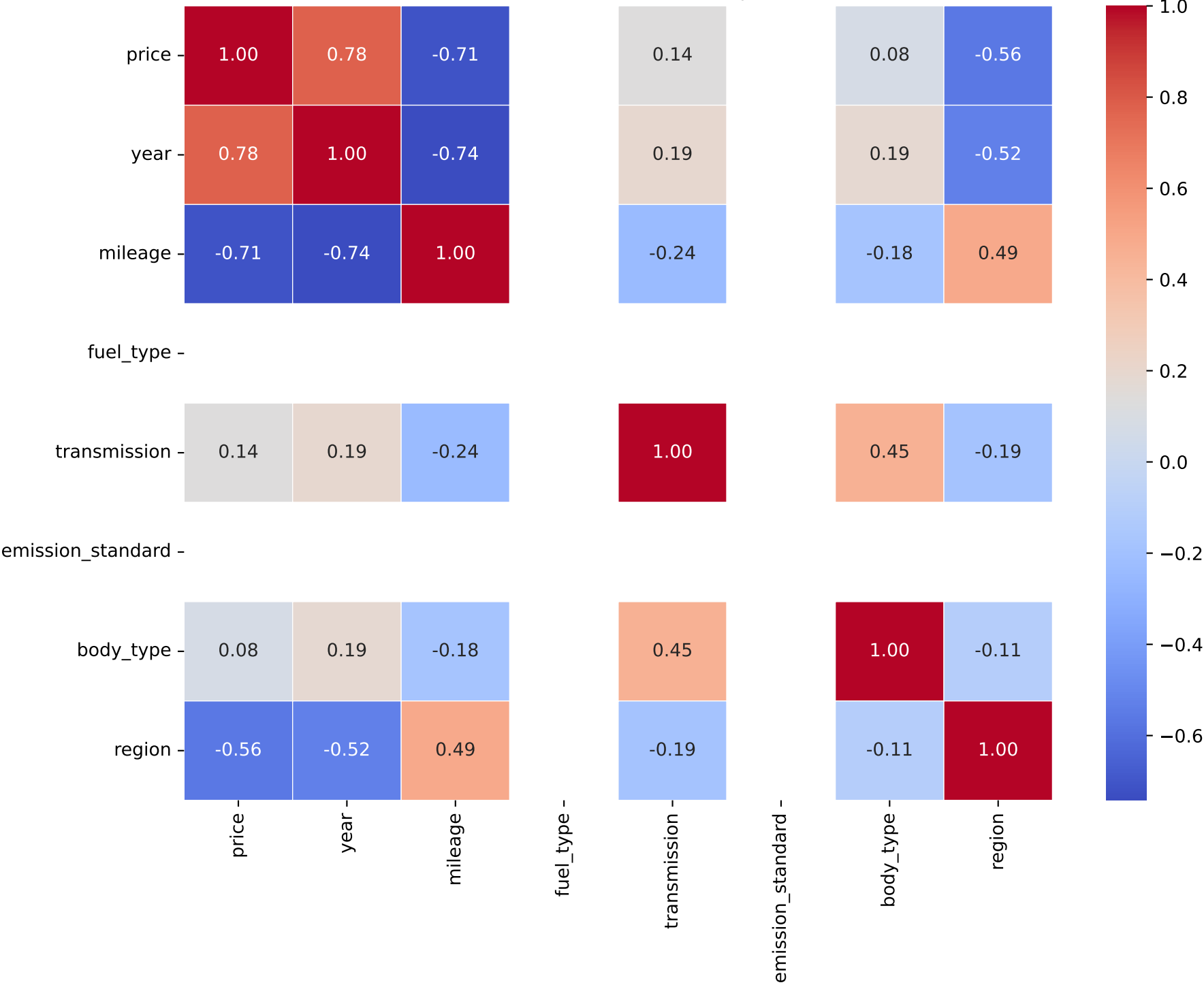
Correlation Heatmap for Model: q3 | Fuel Type: 3
