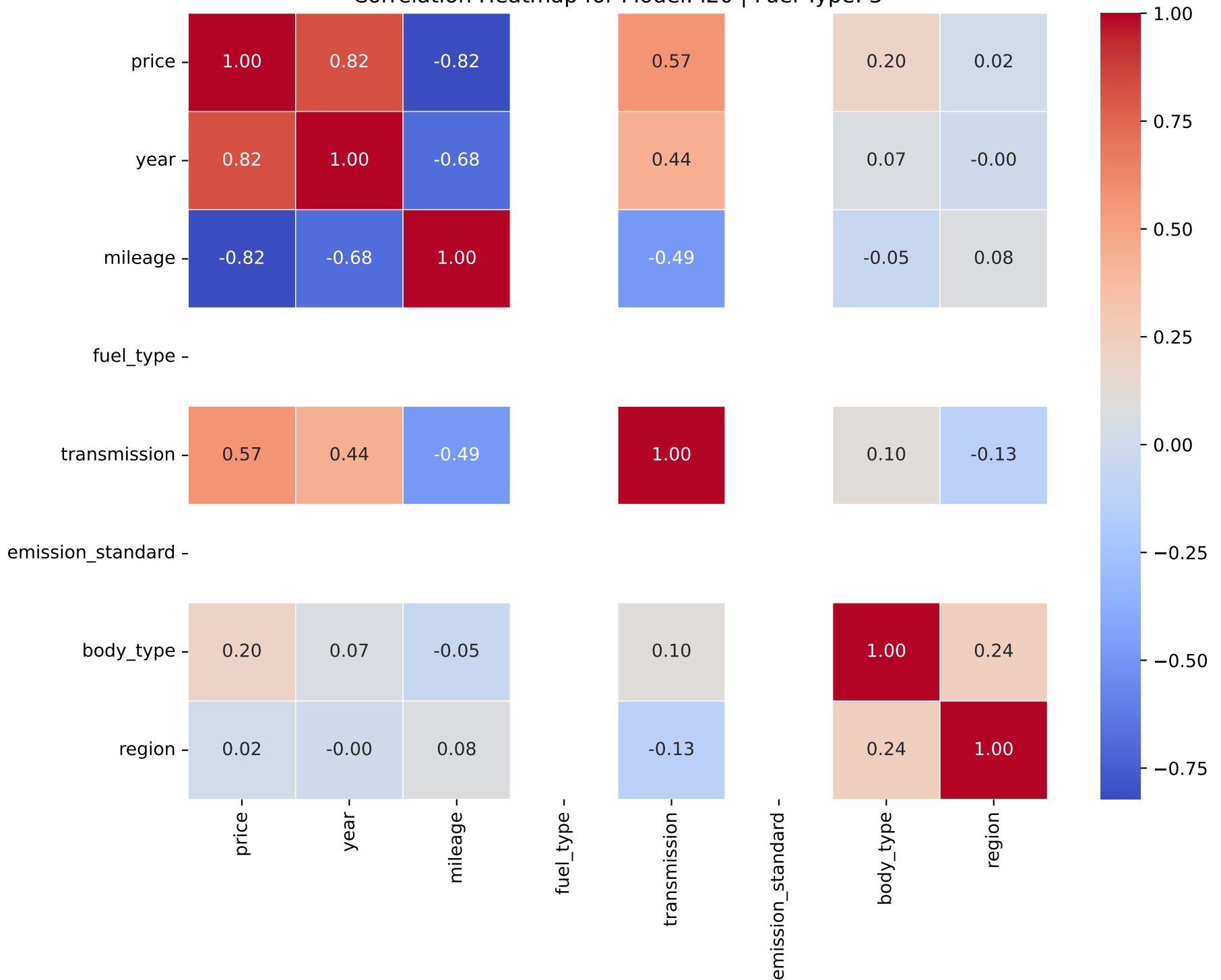
Correlation Heatmap for Model: i20 | Fuel Type: 3
