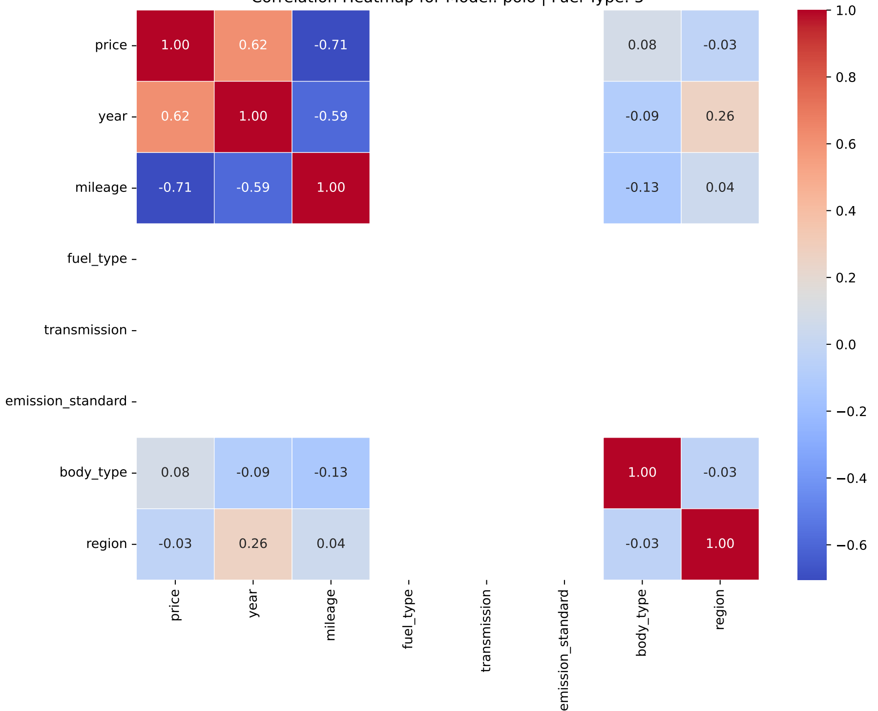
Correlation Heatmap for Model: polo | Fuel Type: 5
