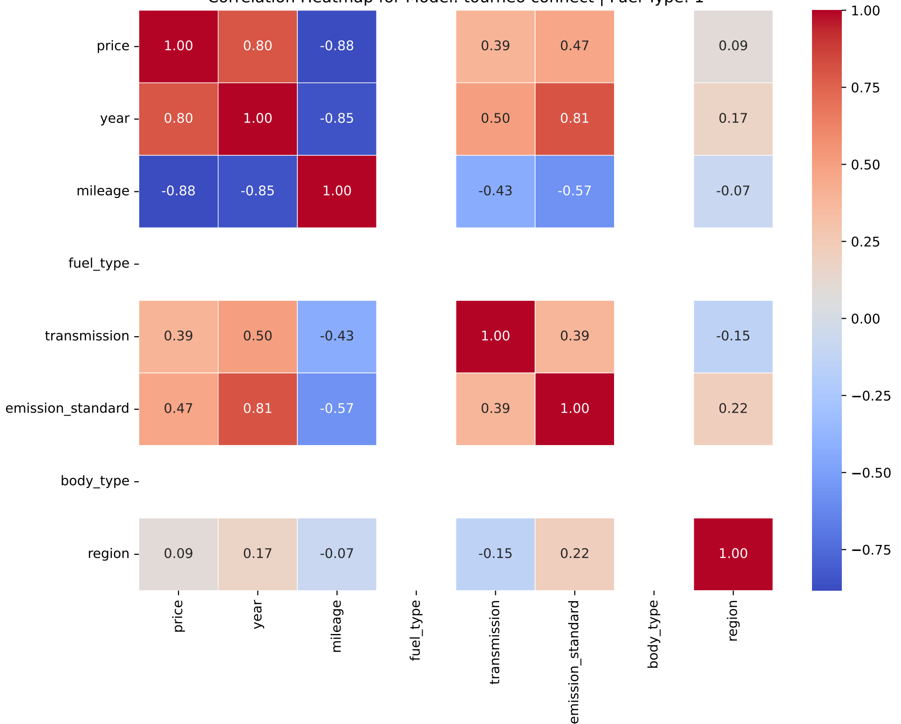
Correlation Heatmap for Model: tourneo connect | Fuel Type: 1
