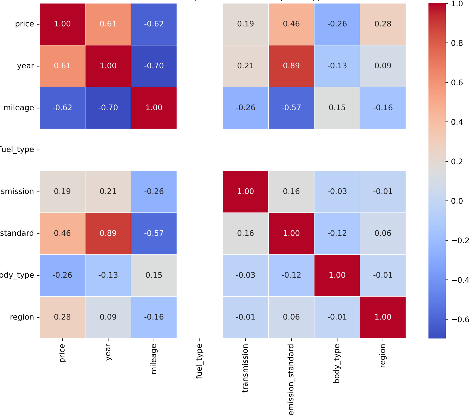
Correlation Heatmap for Model: focus | Fuel Type: 2
