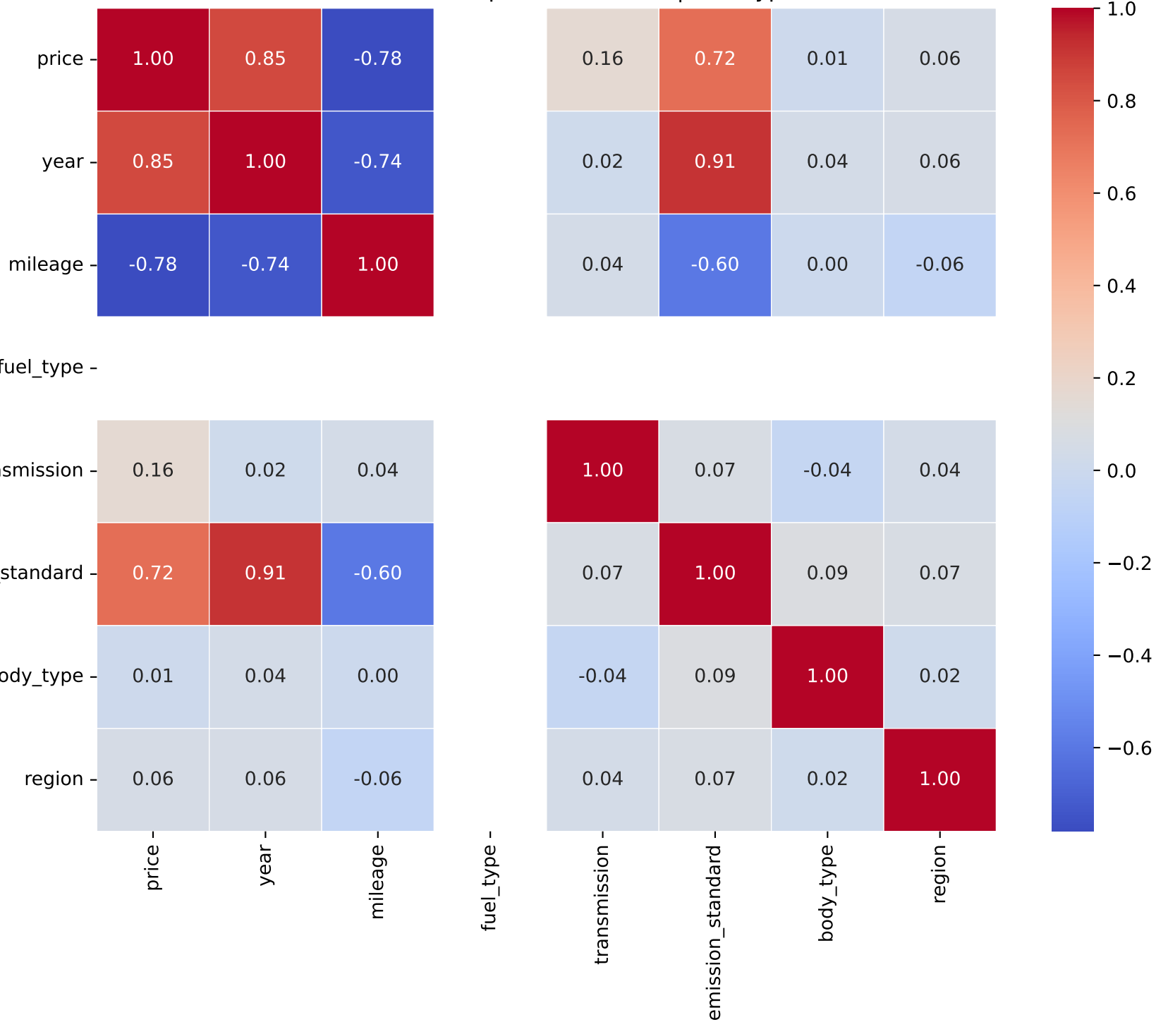
Correlation Heatmap for Model: clio | Fuel Type: 2
