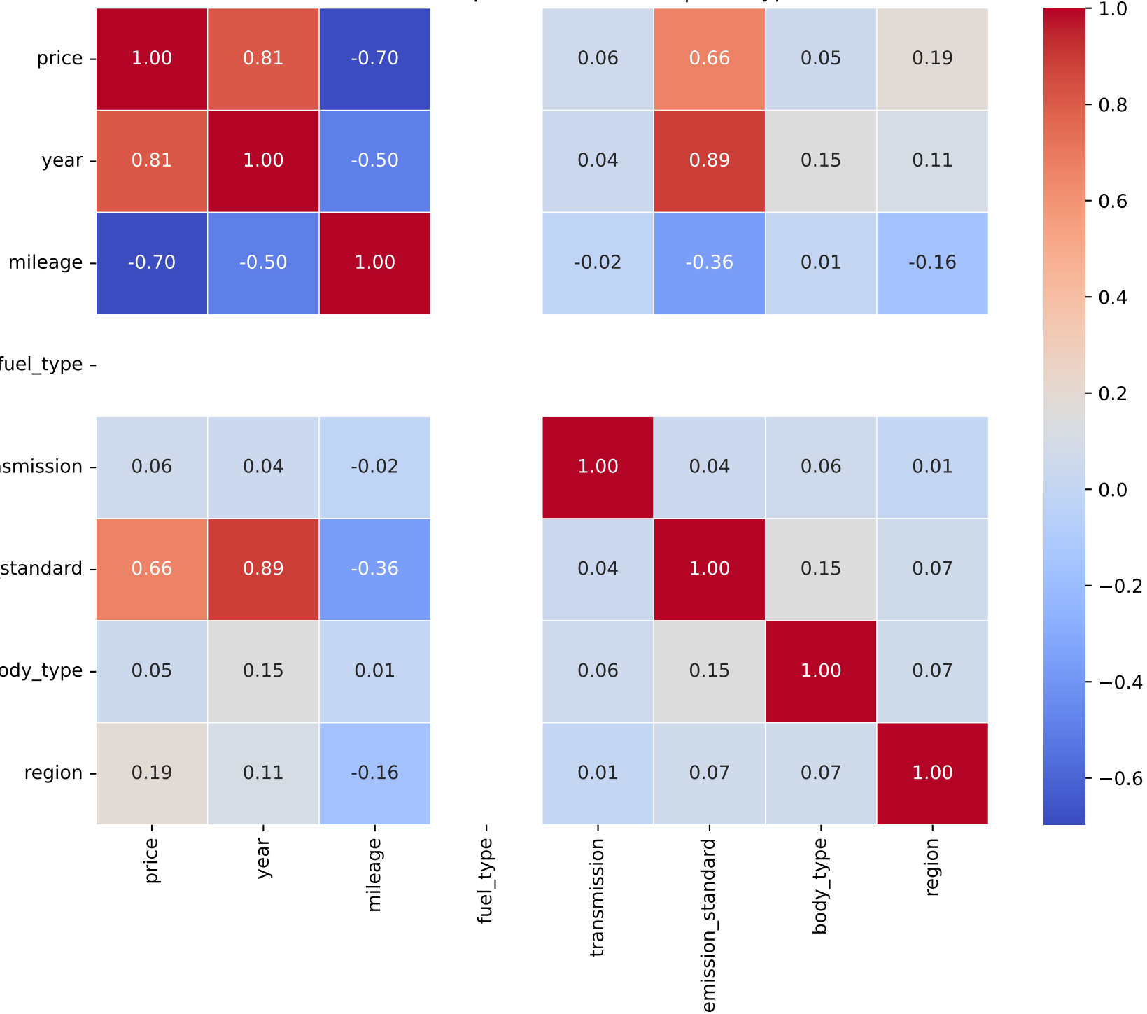
Correlation Heatmap for Model: fiesta | Fuel Type: 2
