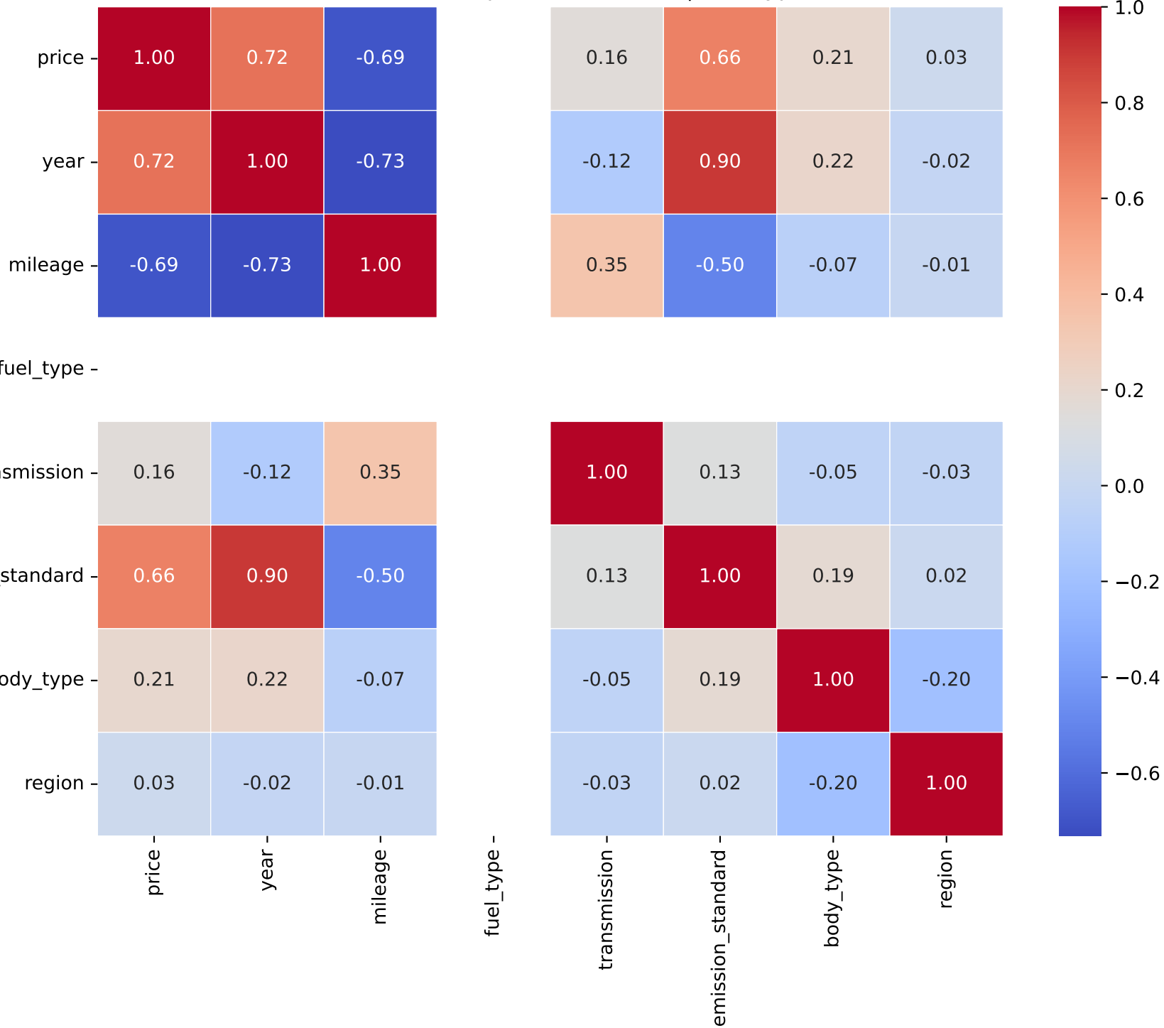
Correlation Heatmap for Model: leon | Fuel Type: 2
