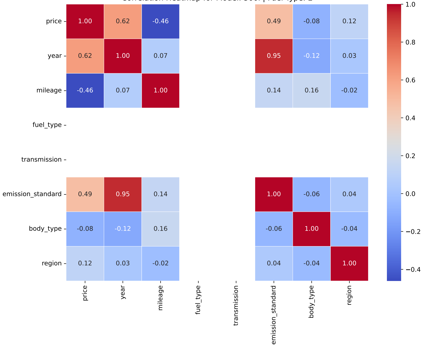
Correlation Heatmap for Model: 500I | Fuel Type: 2
