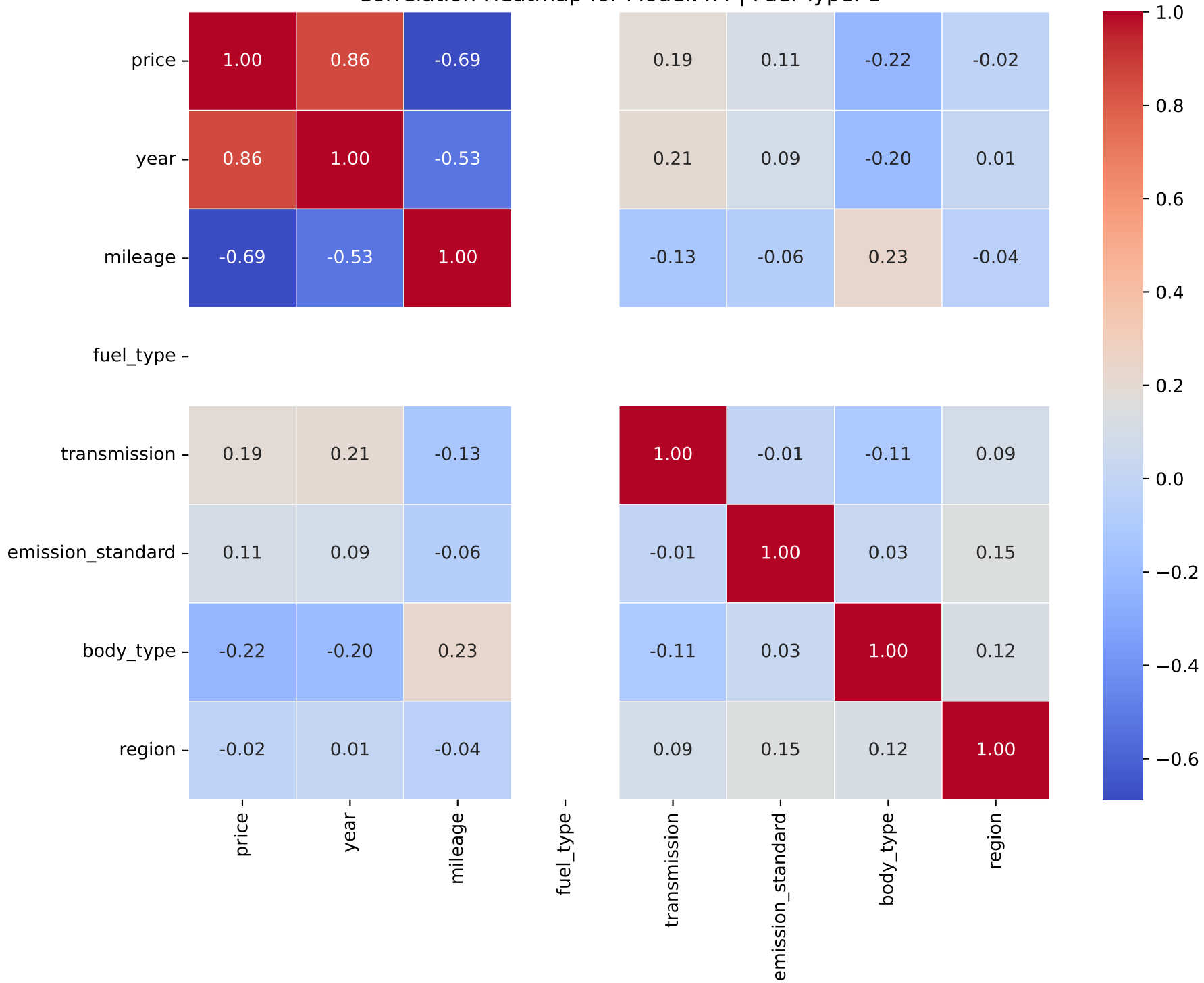
Correlation Heatmap for Model: x4 | Fuel Type: 1
