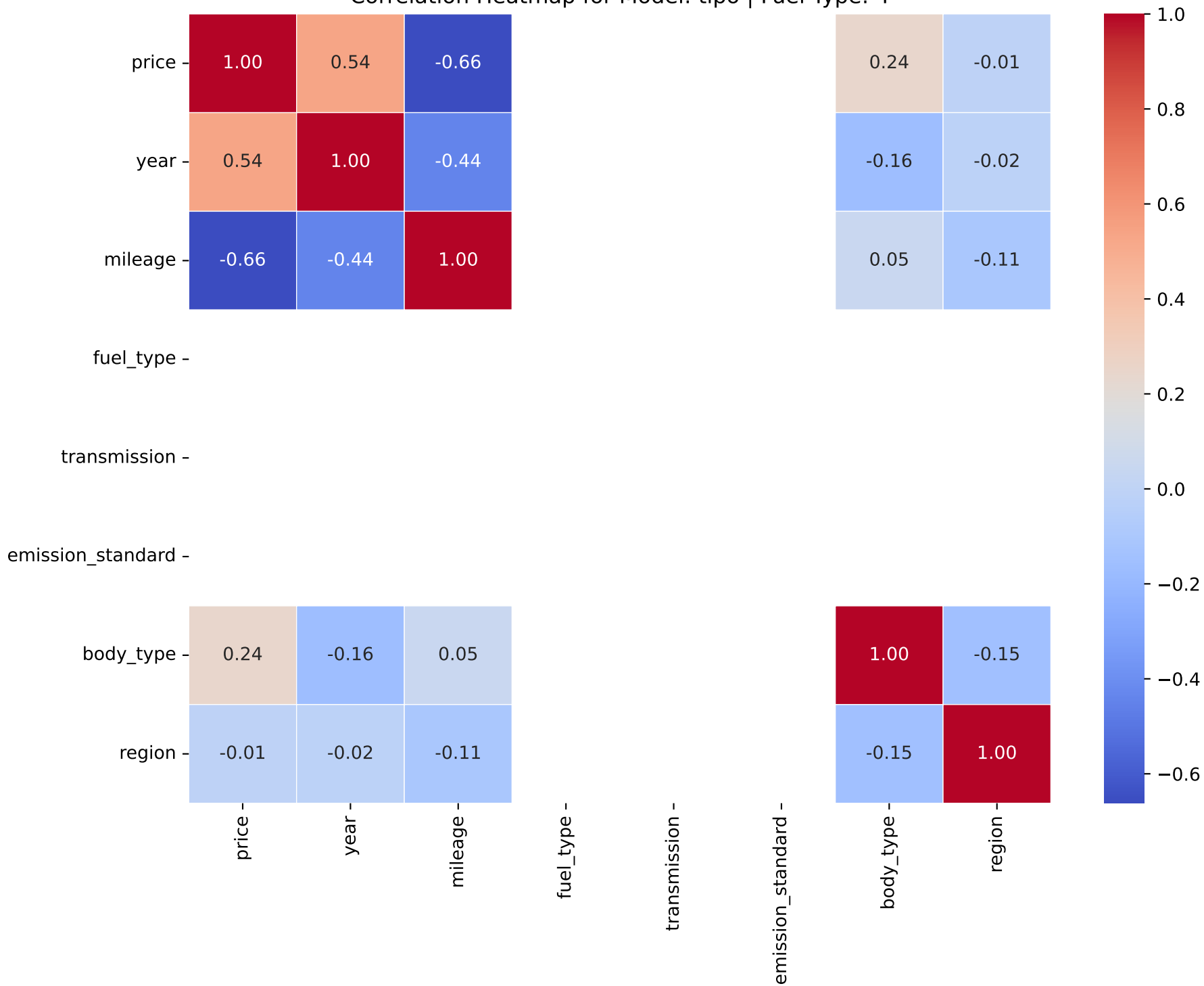
Correlation Heatmap for Model: tipo | Fuel Type: 4
