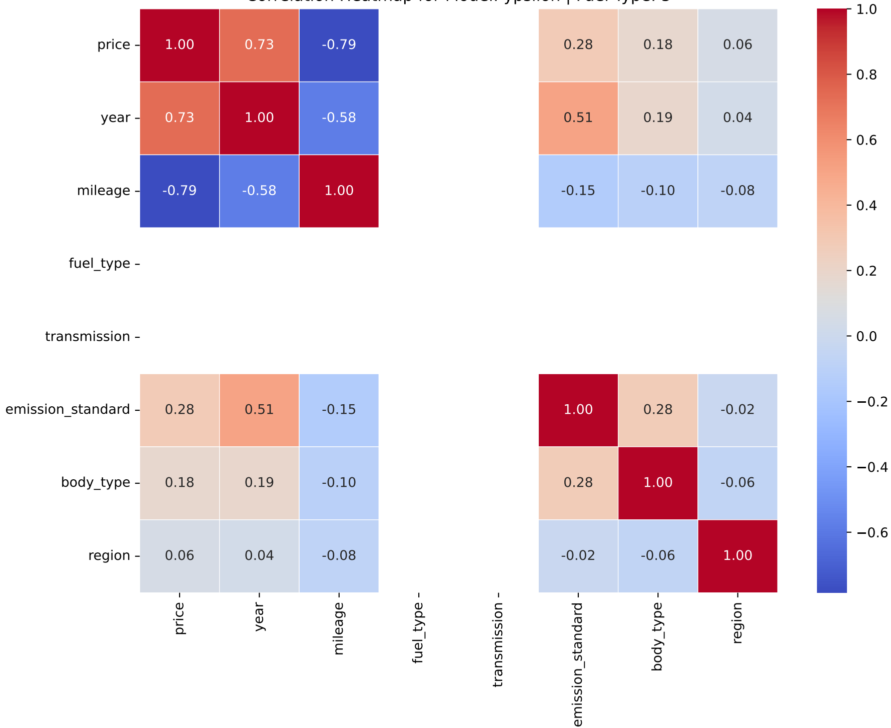
Correlation Heatmap for Model: ypsilon | Fuel Type: 5
