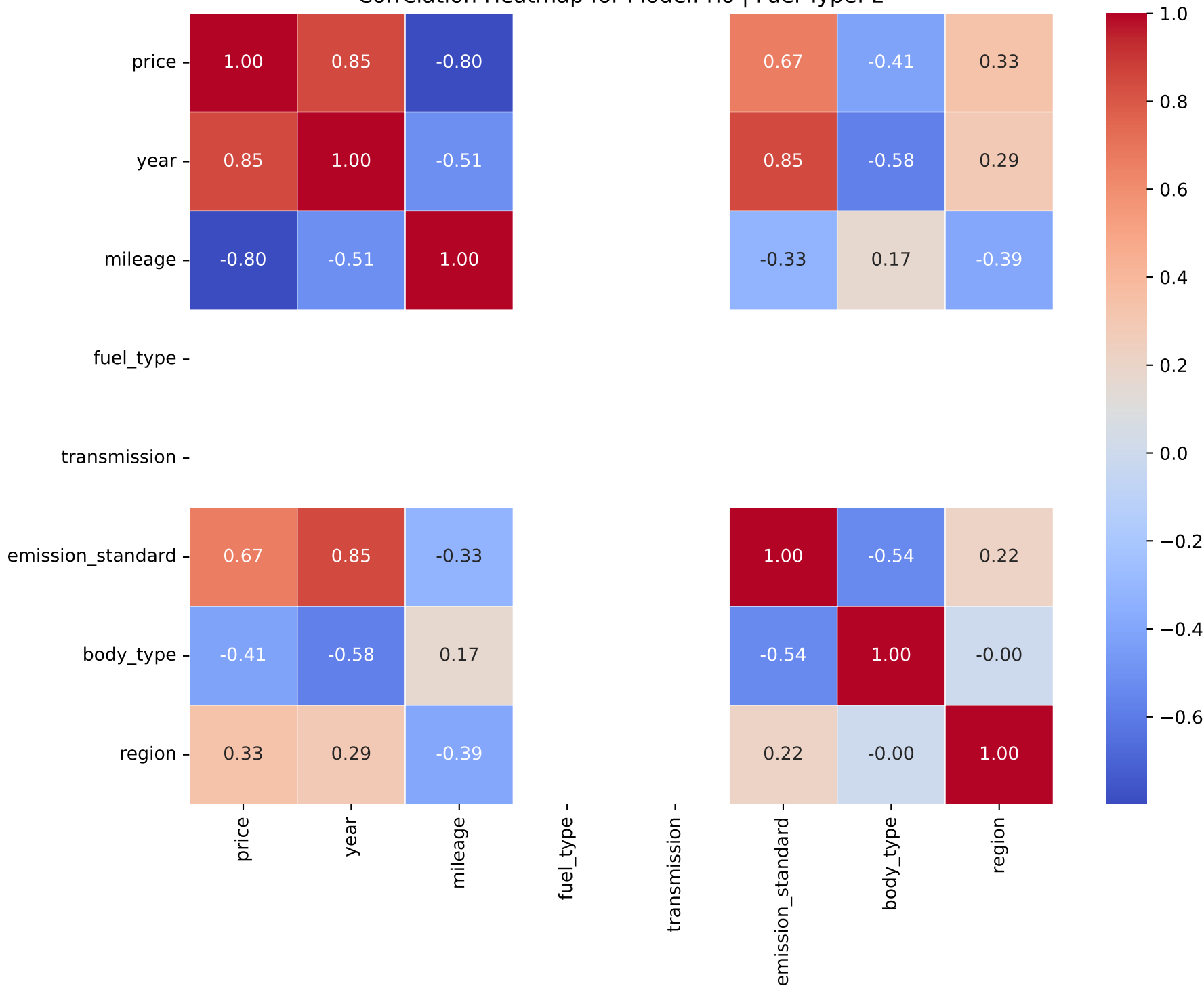
Correlation Heatmap for Model: rio | Fuel Type: 2
