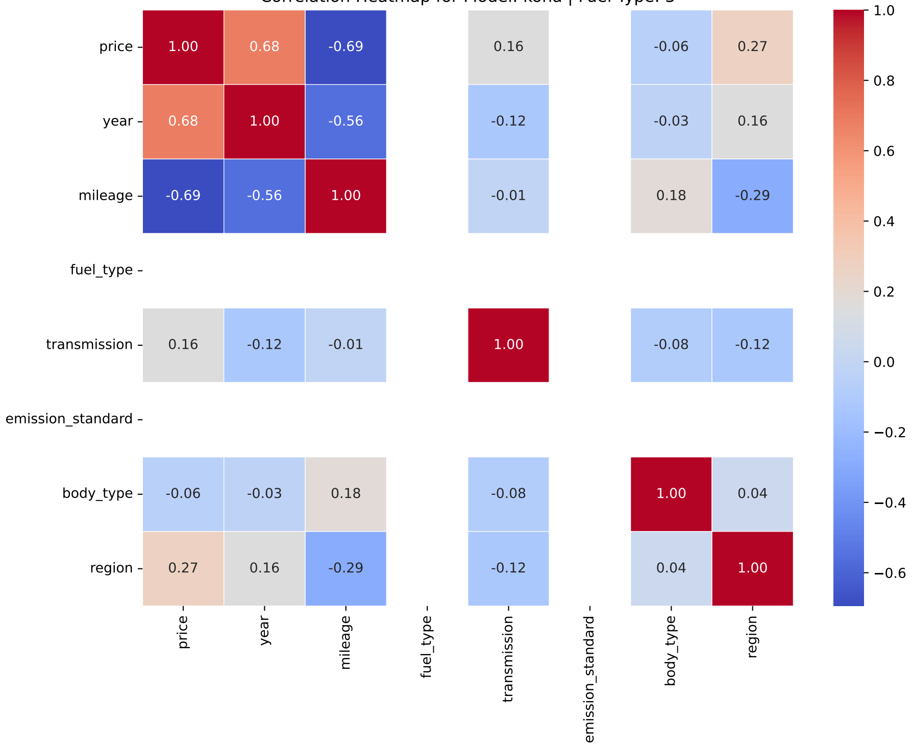
Correlation Heatmap for Model: kona | Fuel Type: 3
