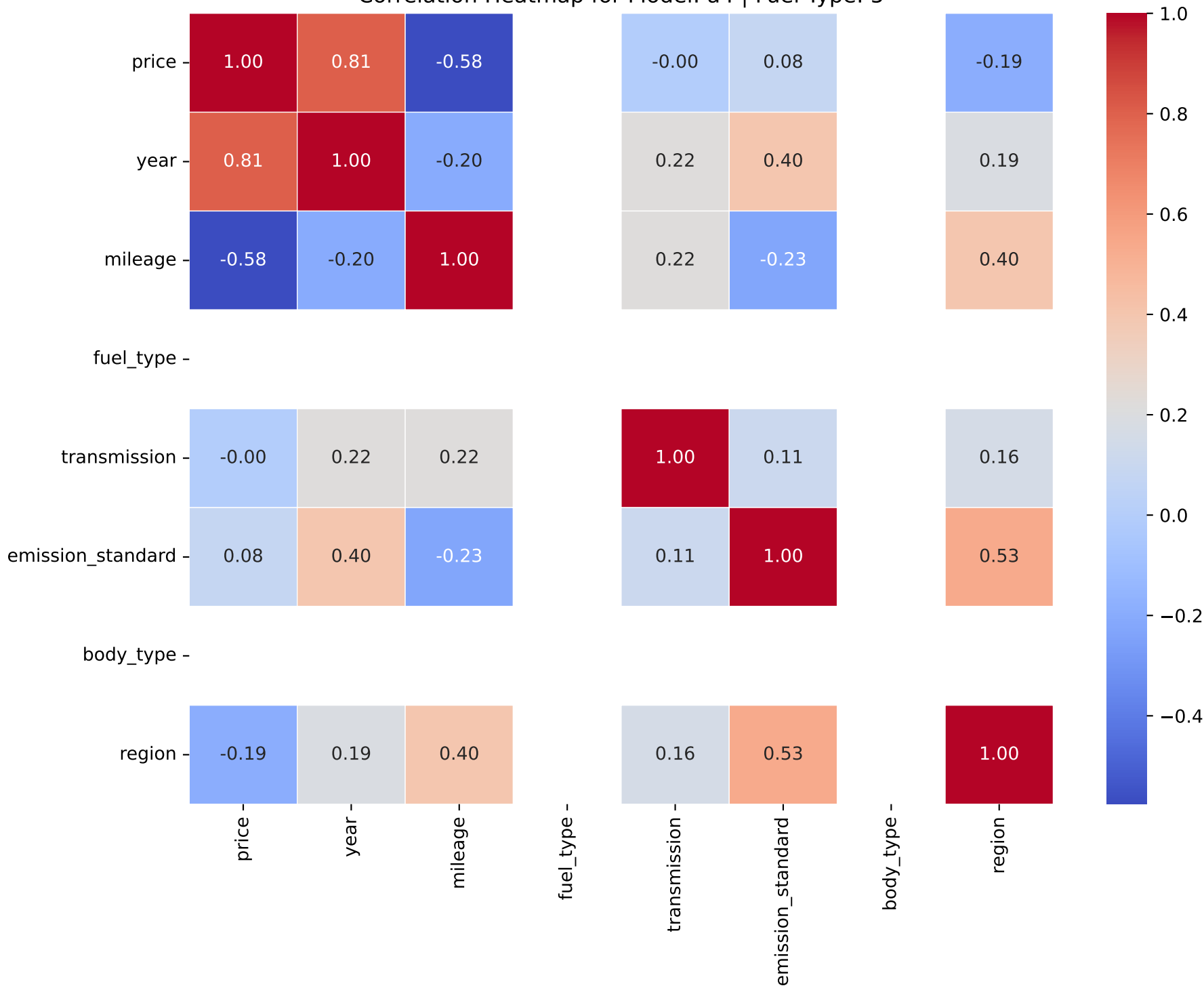
Correlation Heatmap for Model: a4 | Fuel Type: 5
