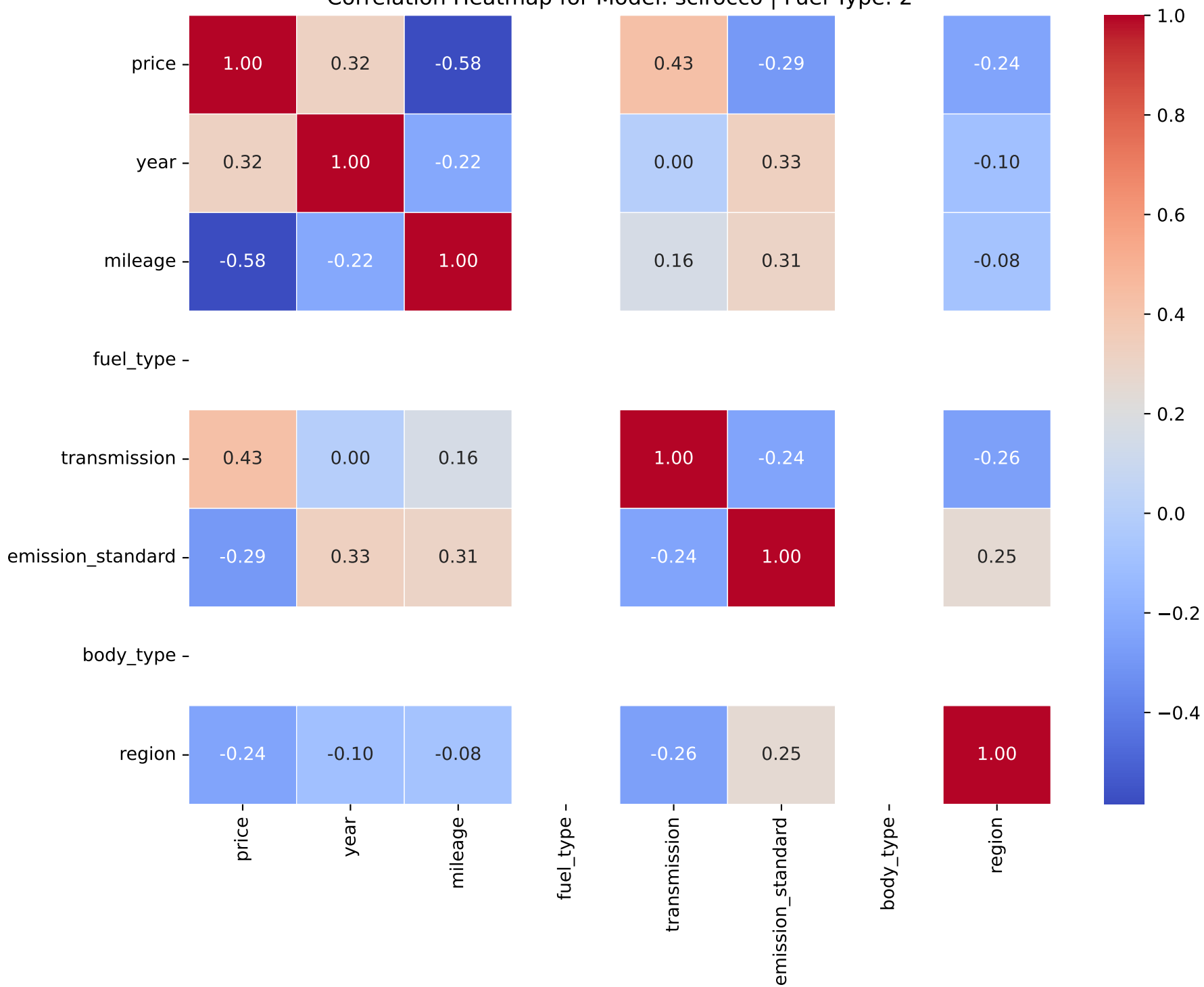
Correlation Heatmap for Model: scirocco | Fuel Type: 2
