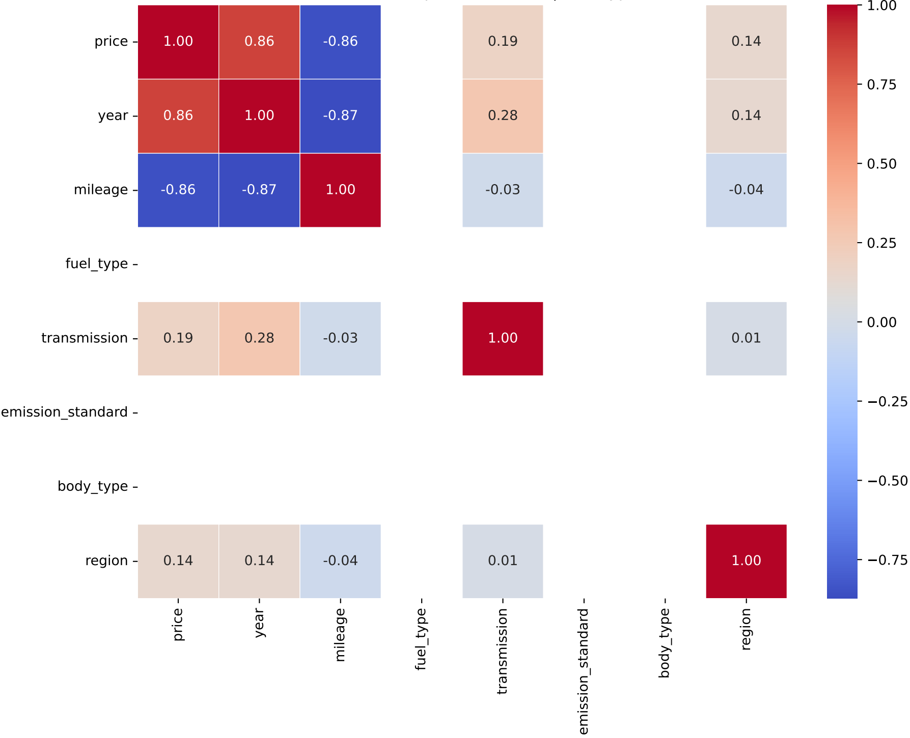
Correlation Heatmap for Model: x2 | Fuel Type: 2
