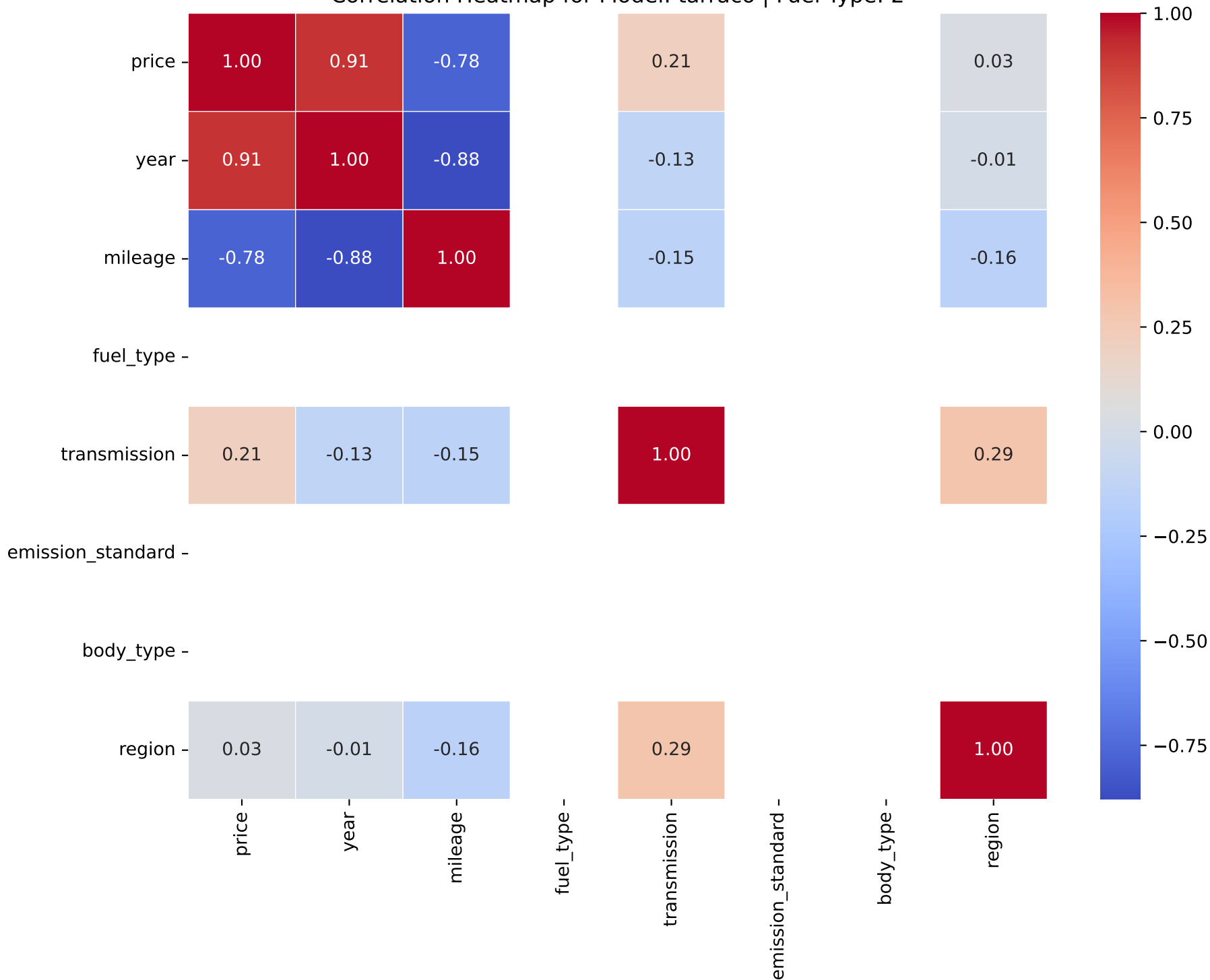
Correlation Heatmap for Model: tarraco | Fuel Type: 2
