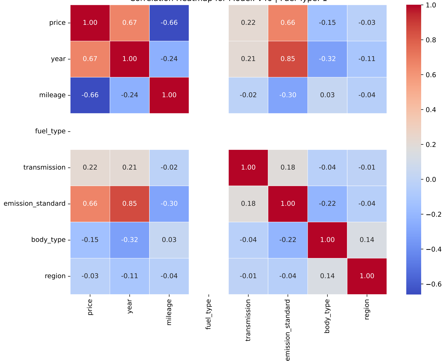
Correlation Heatmap for Model: v40 | Fuel Type: 1
