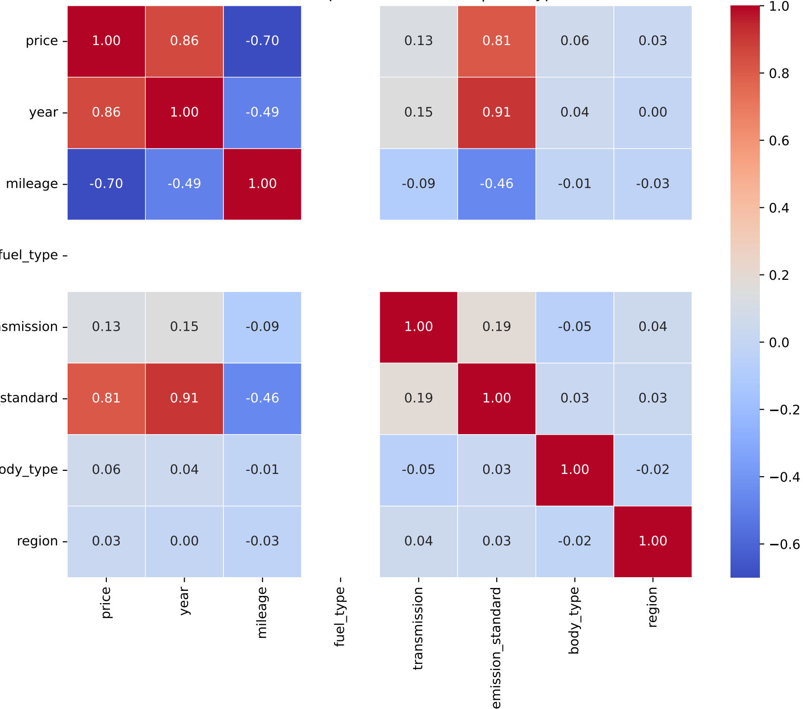
Correlation Heatmap for Model: c-max | Fuel Type: 1
