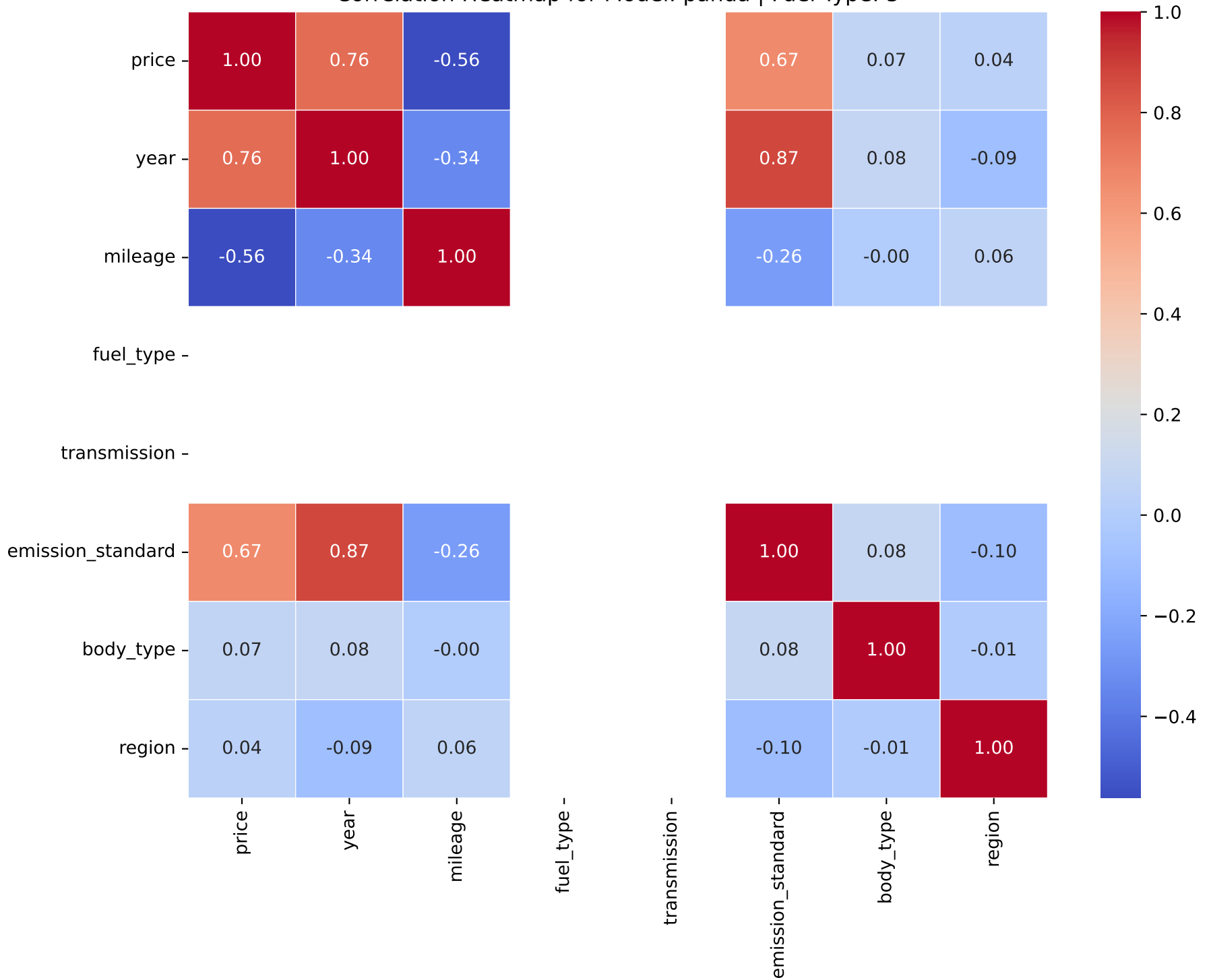
Correlation Heatmap for Model: panda | Fuel Type: 5
