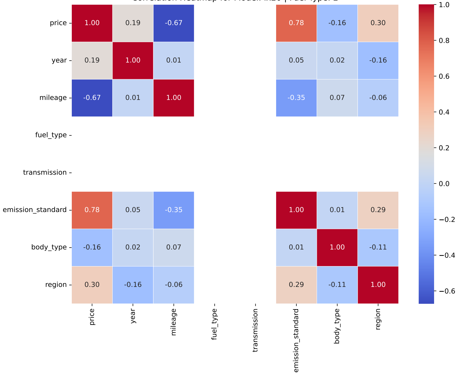
Correlation Heatmap for Model: ix20 | Fuel Type: 2
