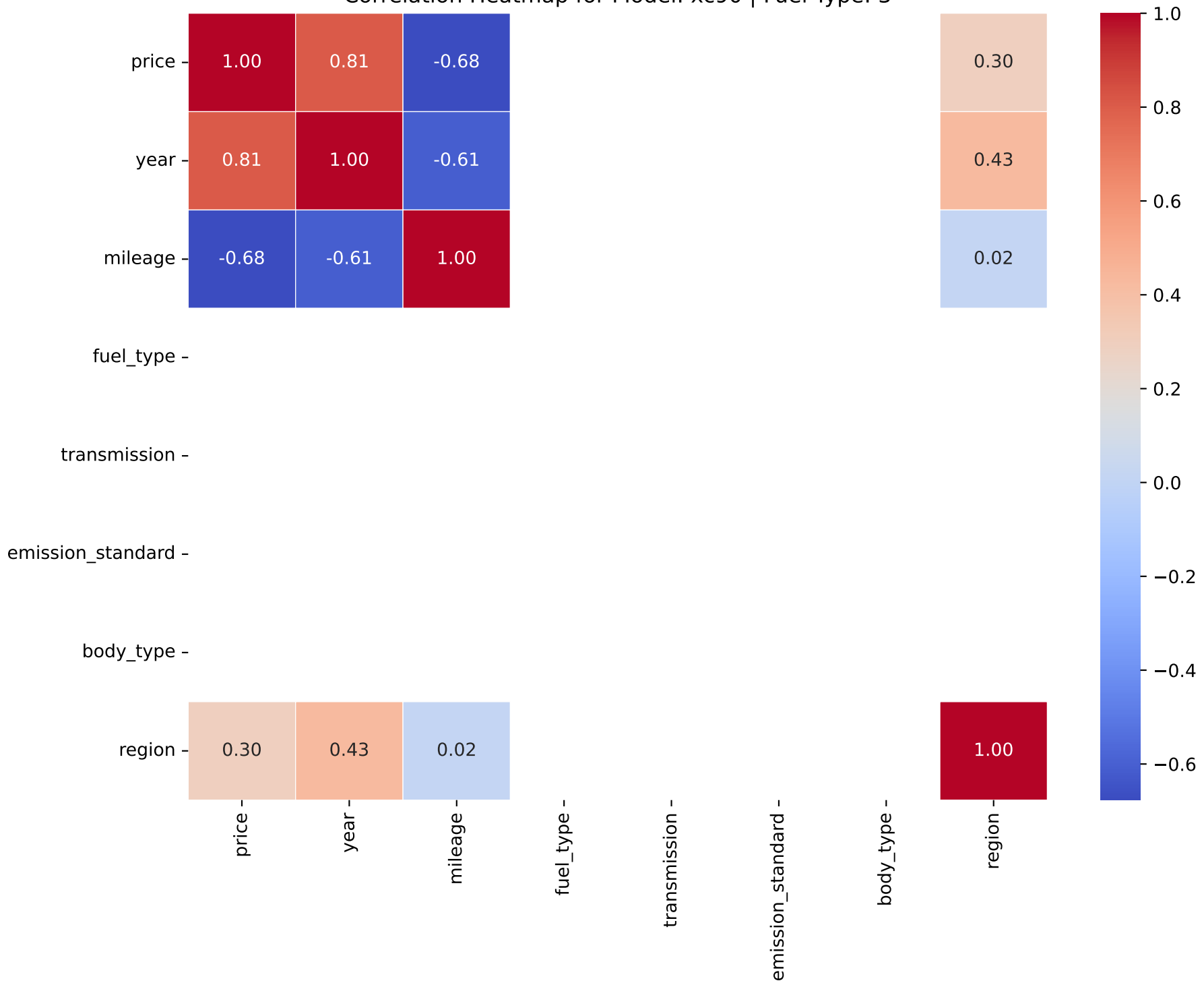
Correlation Heatmap for Model: xc90 | Fuel Type: 3
