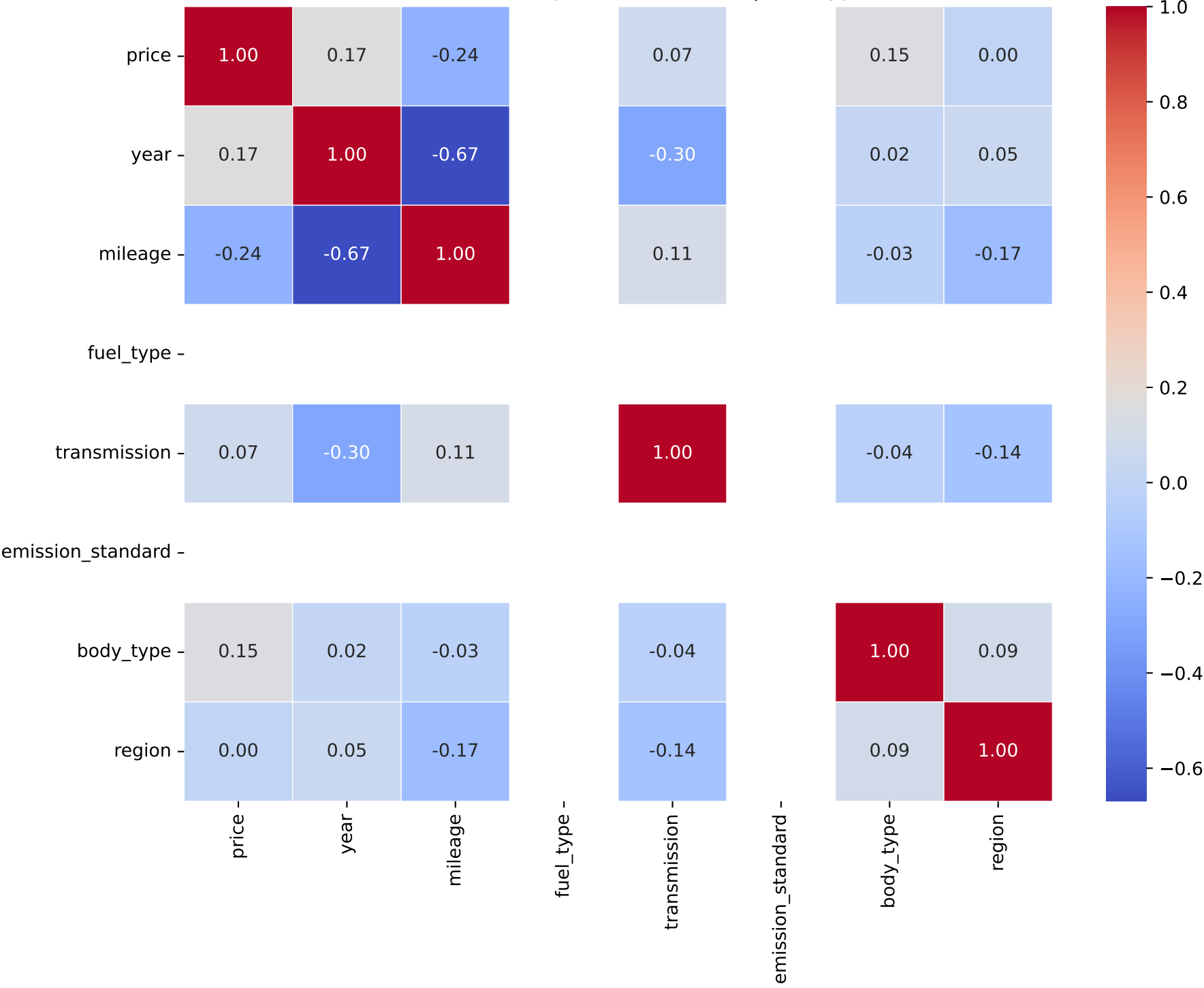
Correlation Heatmap for Model: 500x | Fuel Type: 3
