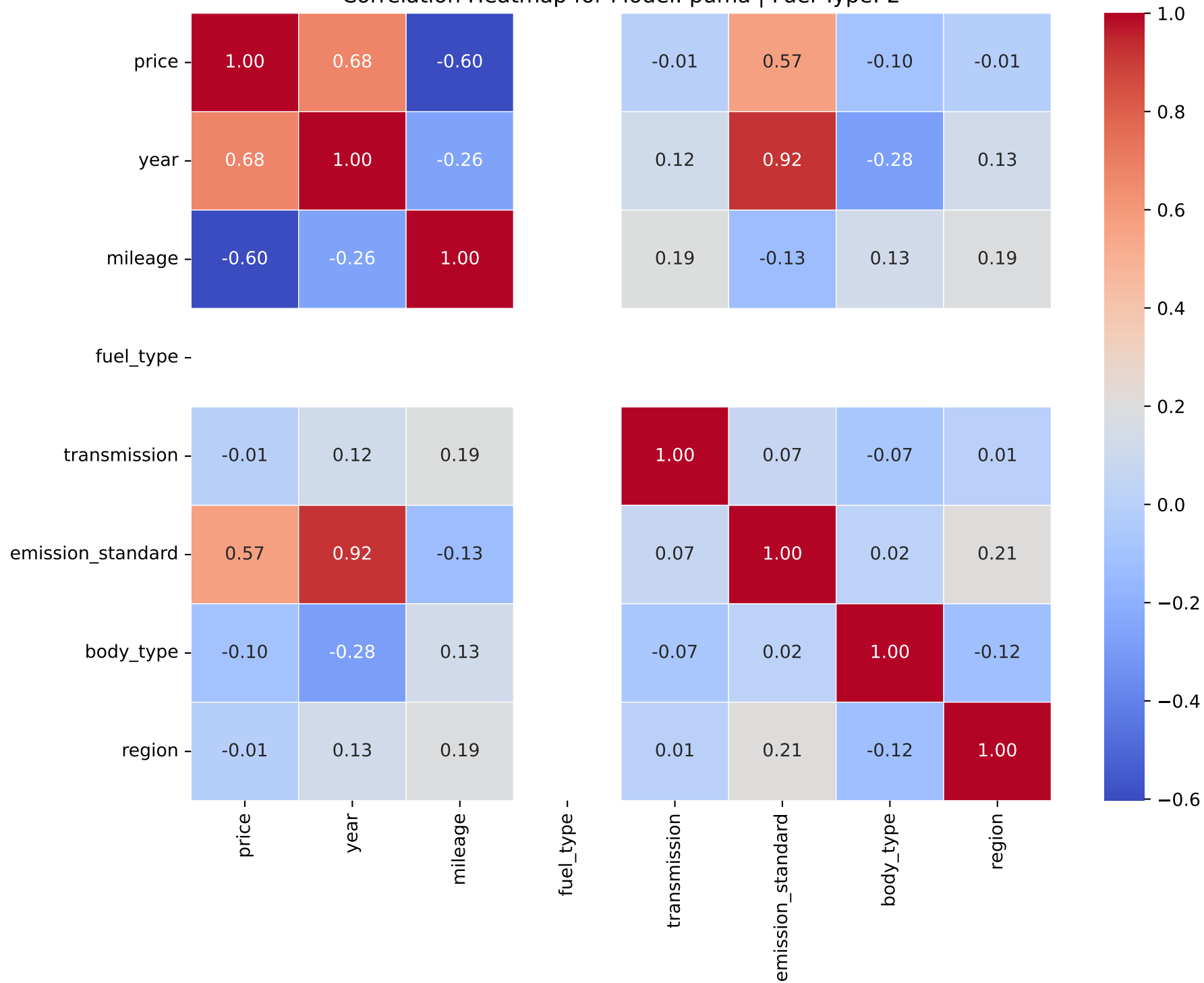
Correlation Heatmap for Model: puma | Fuel Type: 2
