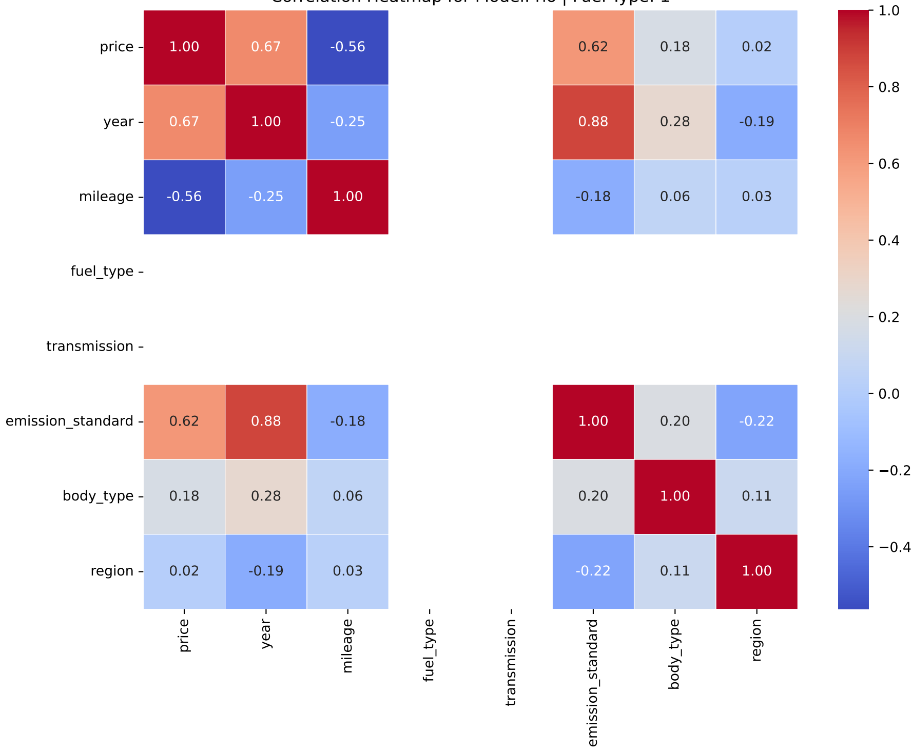
Correlation Heatmap for Model: rio | Fuel Type: 1
