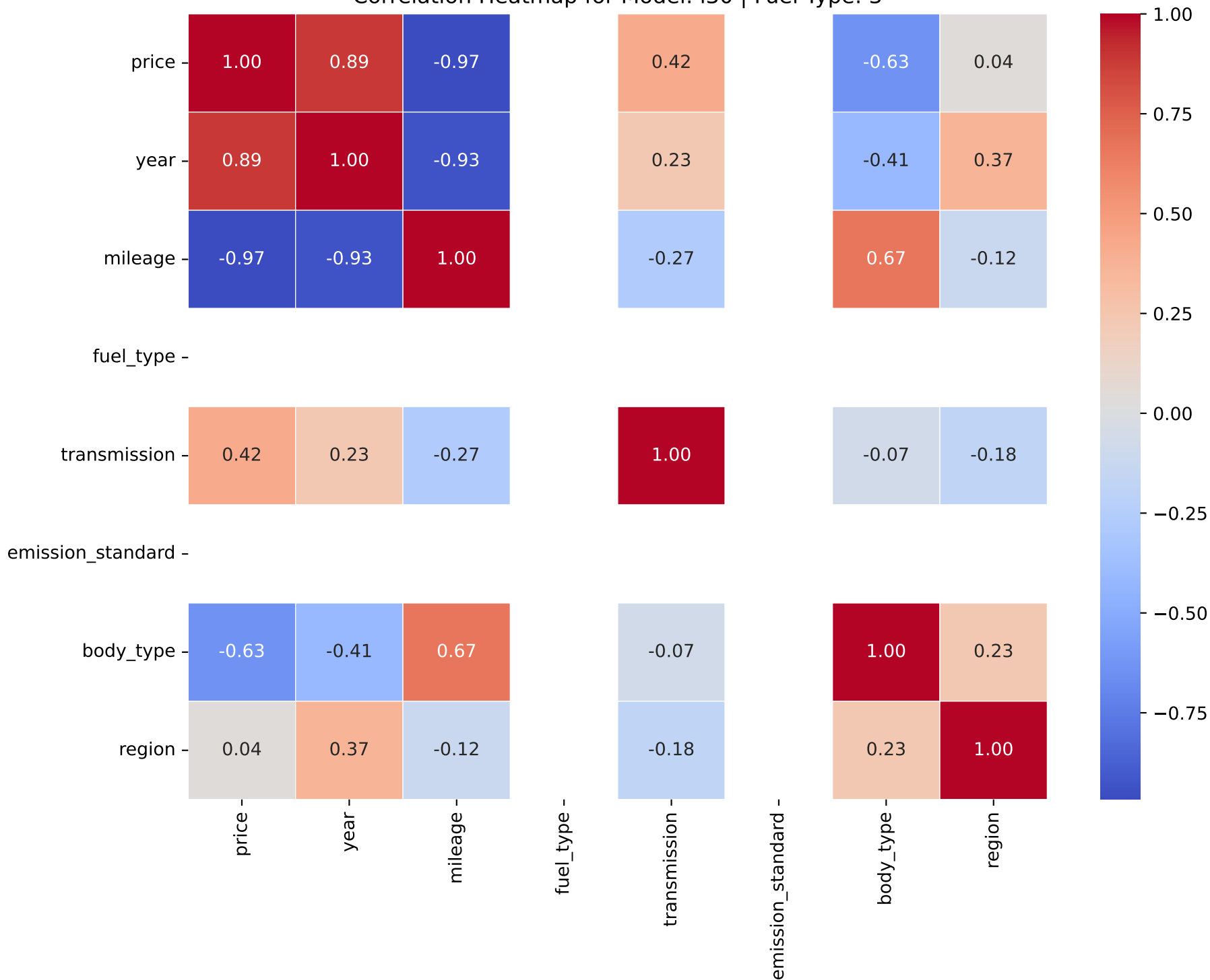
Correlation Heatmap for Model: i30 | Fuel Type: 3
