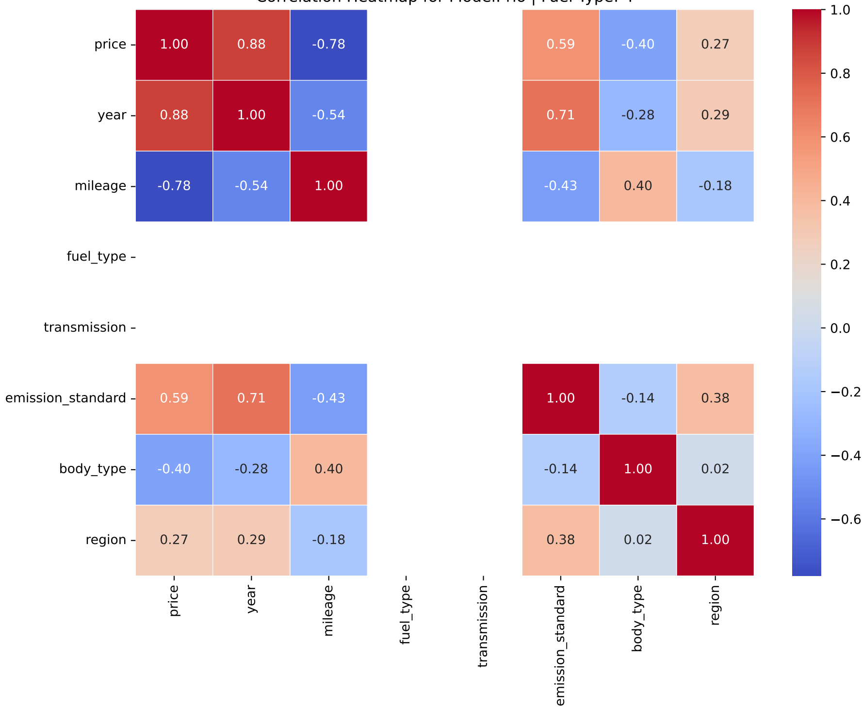
Correlation Heatmap for Model: rio | Fuel Type: 4
