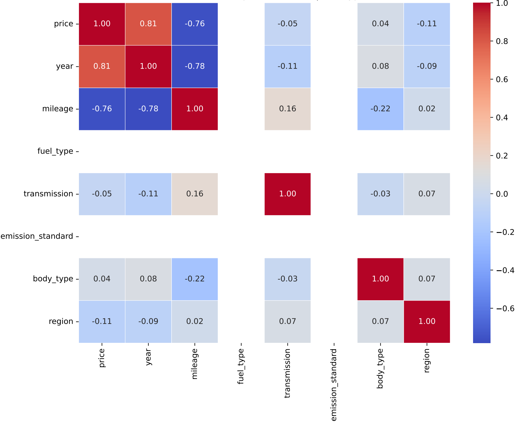
Correlation Heatmap for Model: x4 | Fuel Type: 3
