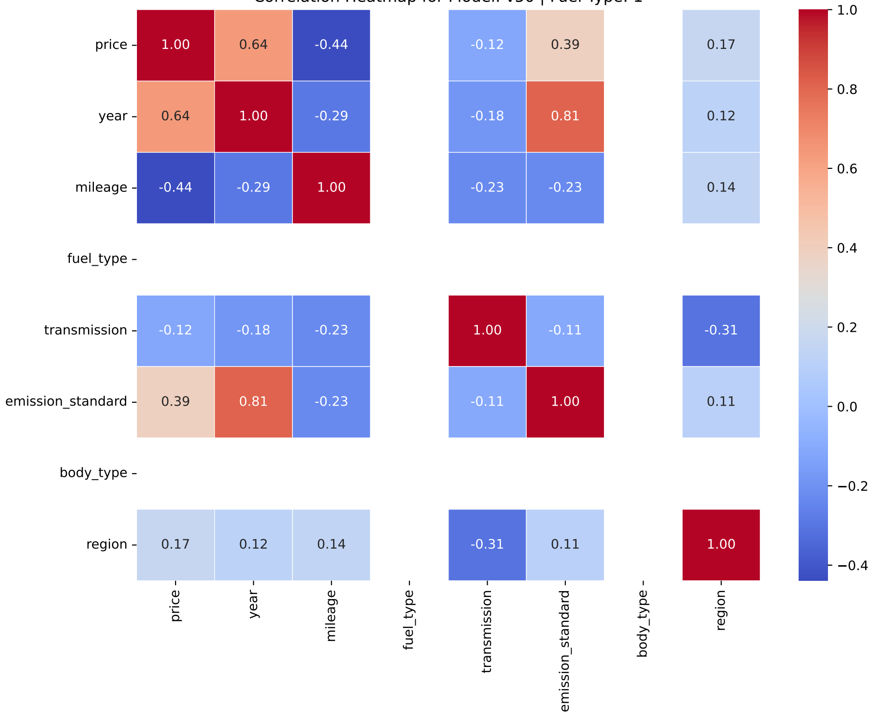
Correlation Heatmap for Model: v50 | Fuel Type: 1
