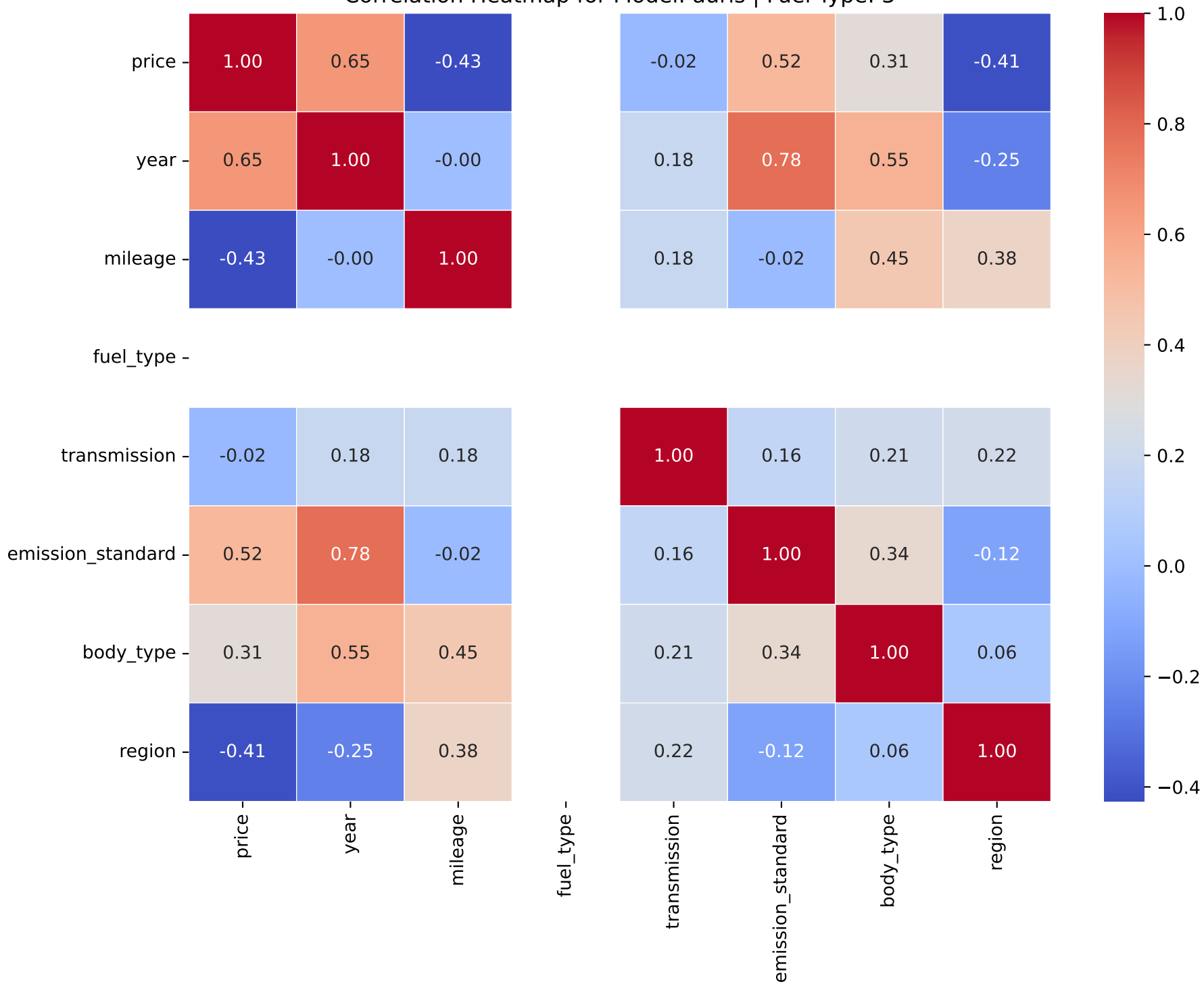
Correlation Heatmap for Model: auris | Fuel Type: 3
