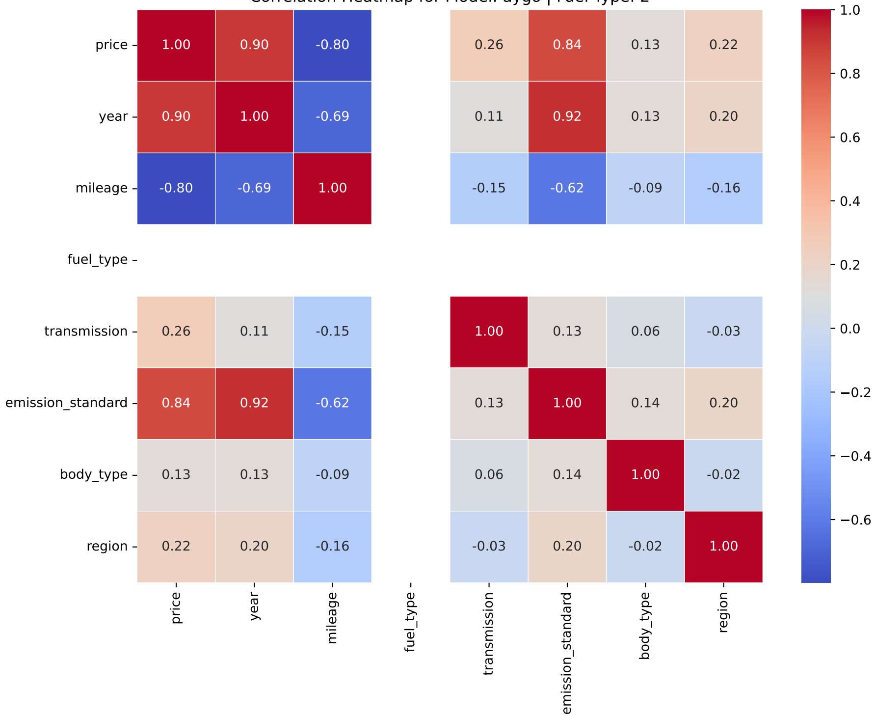
Correlation Heatmap for Model: aygo | Fuel Type: 2
