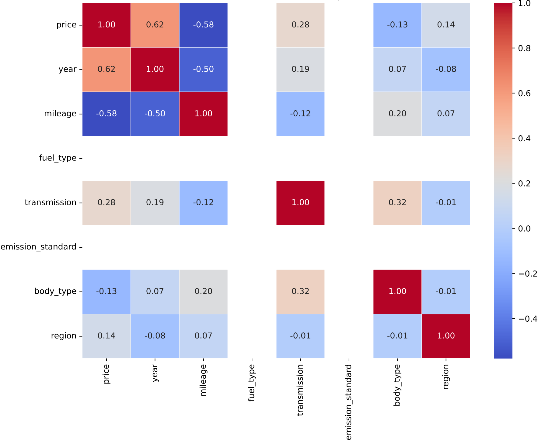
Correlation Heatmap for Model: focus | Fuel Type: 3
