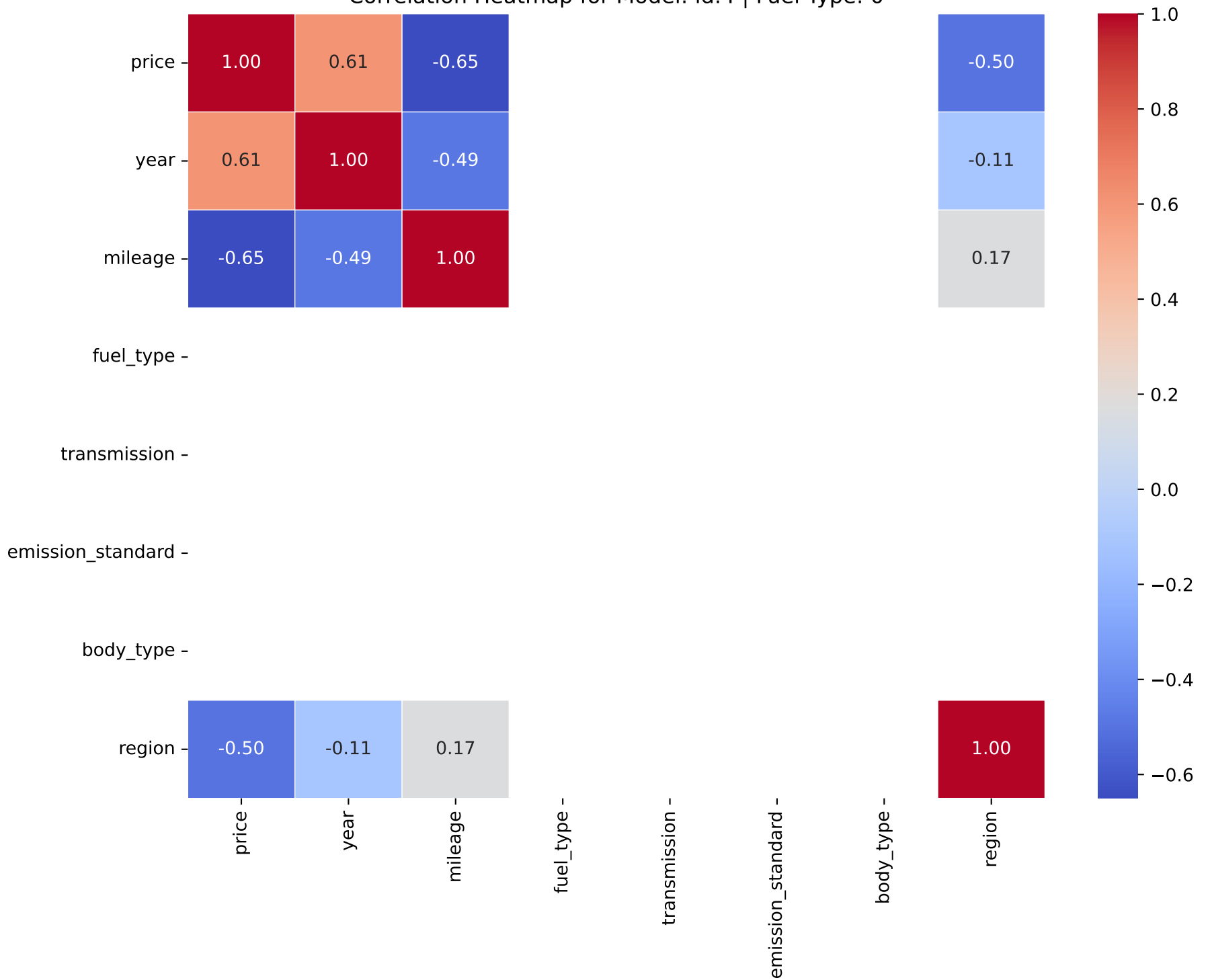
Correlation Heatmap for Model: id.4 | Fuel Type: 0
