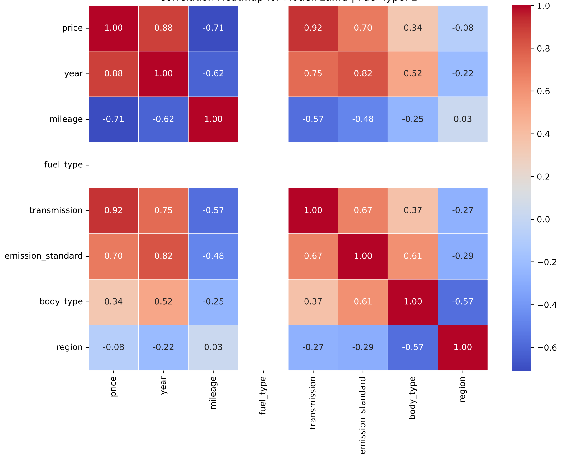
Correlation Heatmap for Model: zafira | Fuel Type: 2
