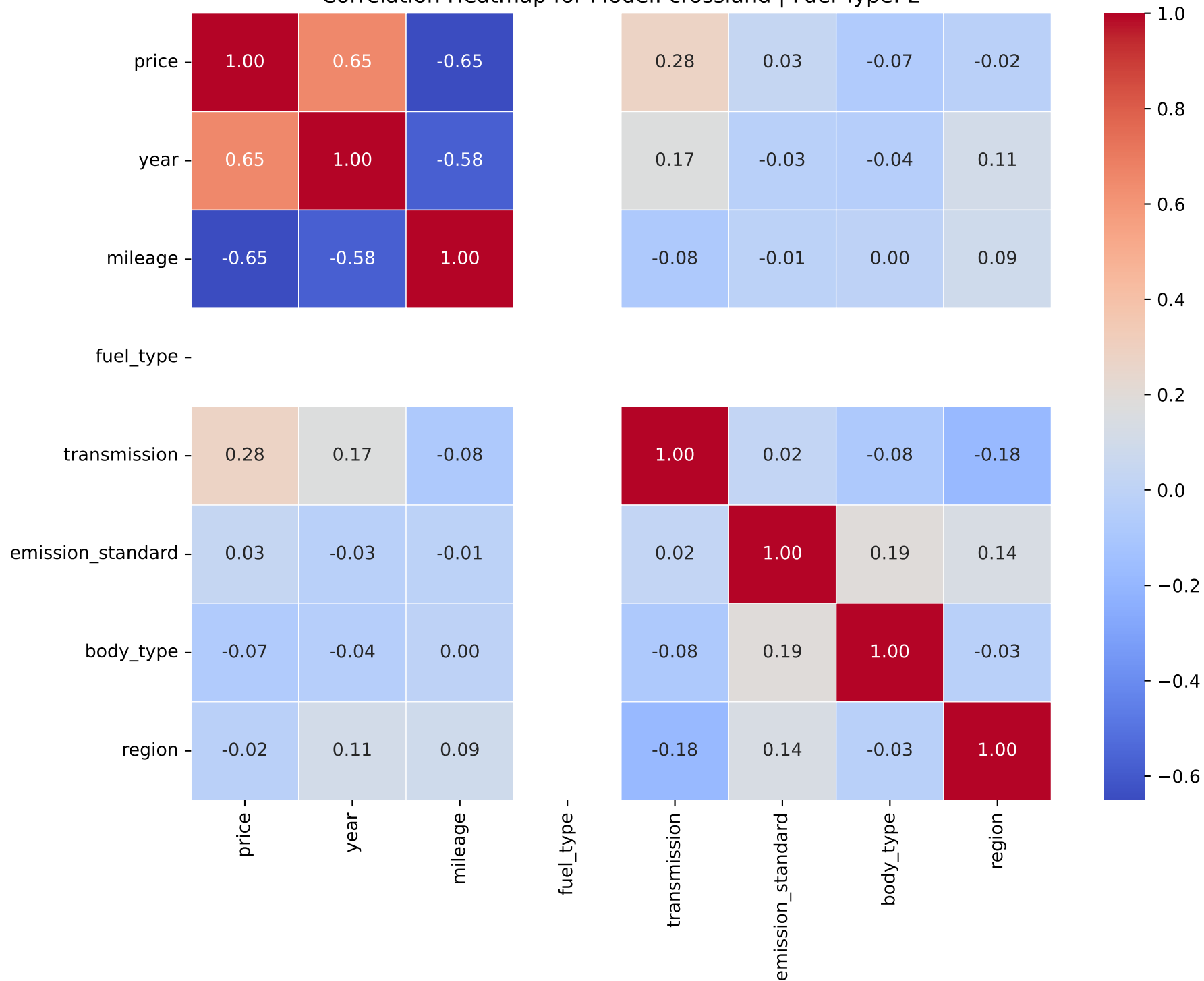
Correlation Heatmap for Model: crossland | Fuel Type: 2
