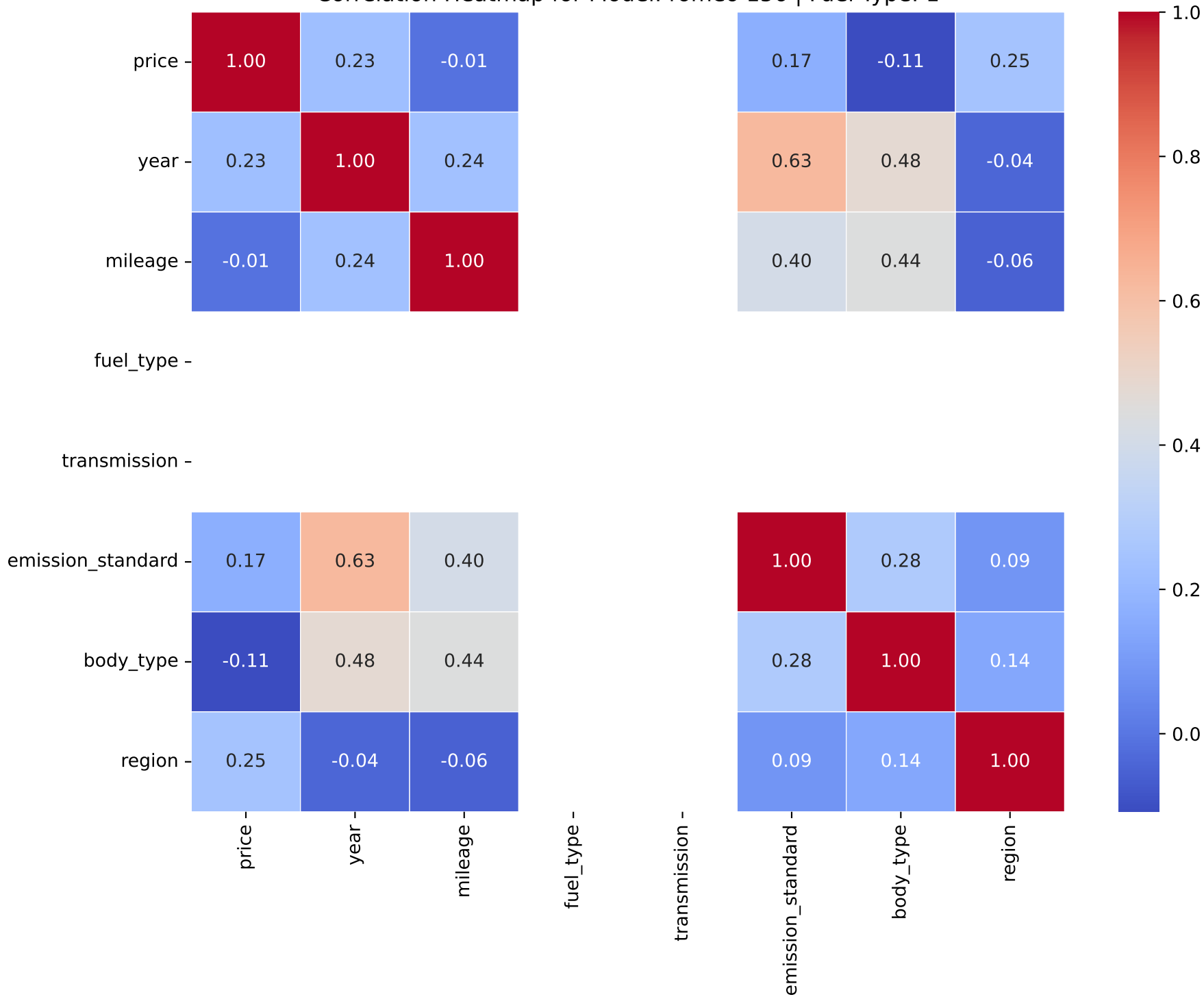
Correlation Heatmap for Model: romeo 156 | Fuel Type: 1
