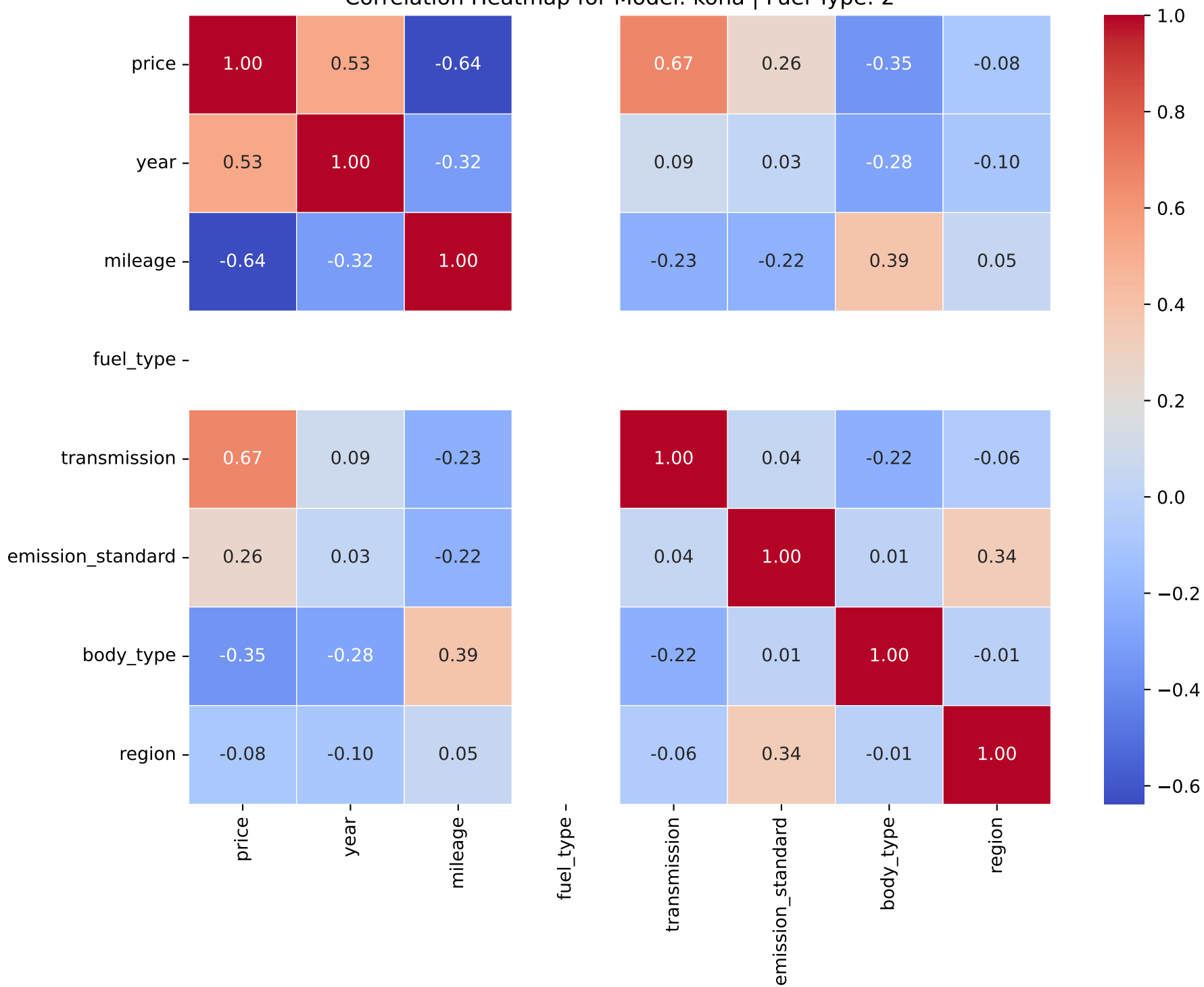
Correlation Heatmap for Model: kona | Fuel Type: 2
