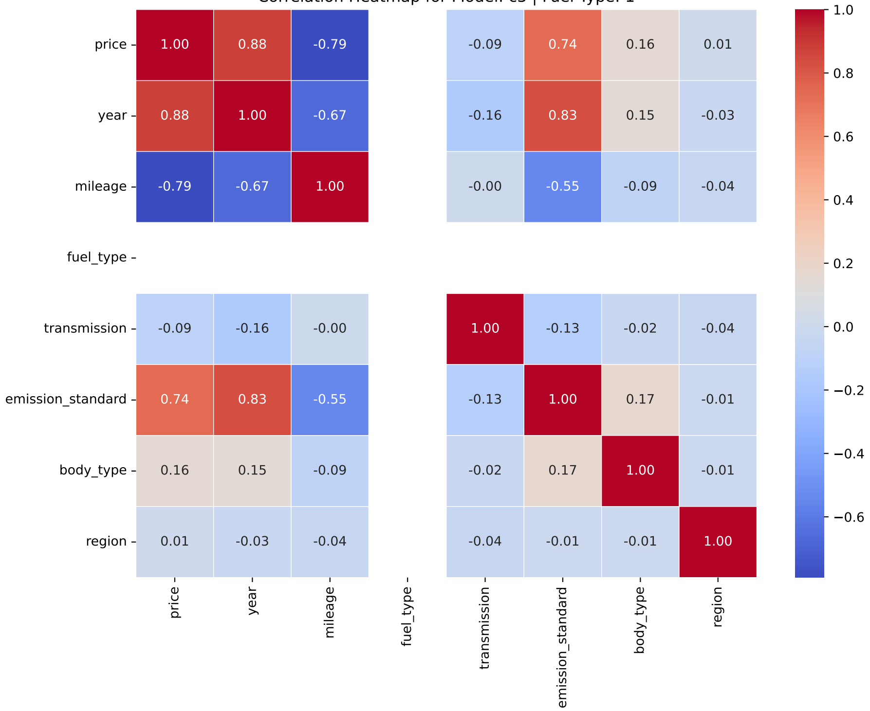
Correlation Heatmap for Model: c3 | Fuel Type: 1
