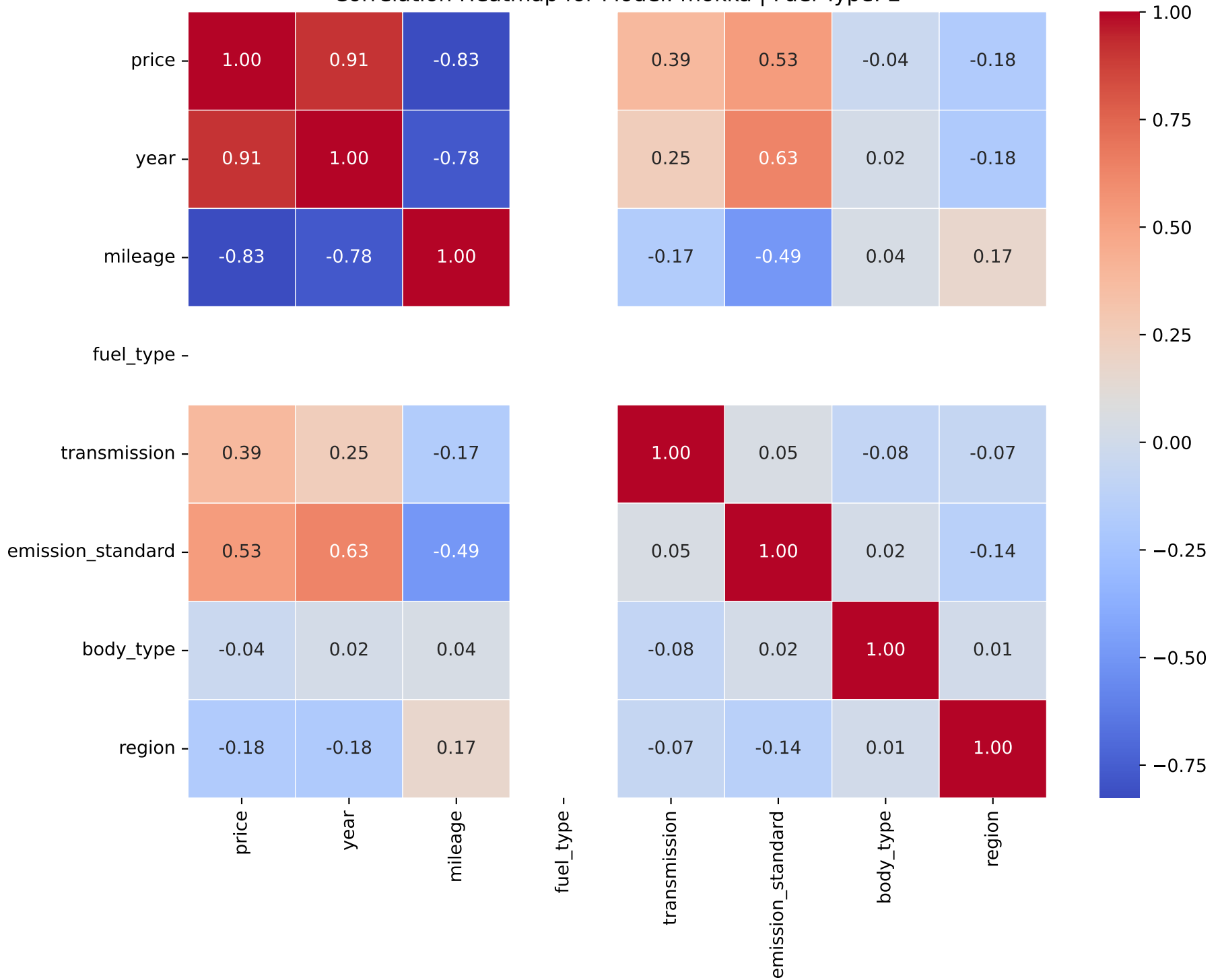
Correlation Heatmap for Model: mokka | Fuel Type: 2
