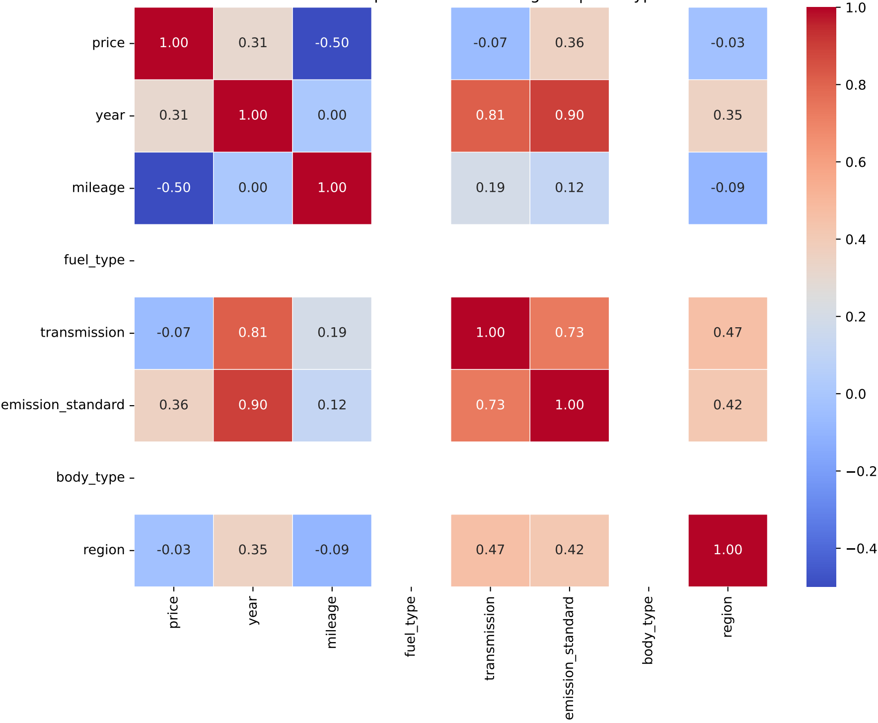
Correlation Heatmap for Model: romeo giulia | Fuel Type: 2
