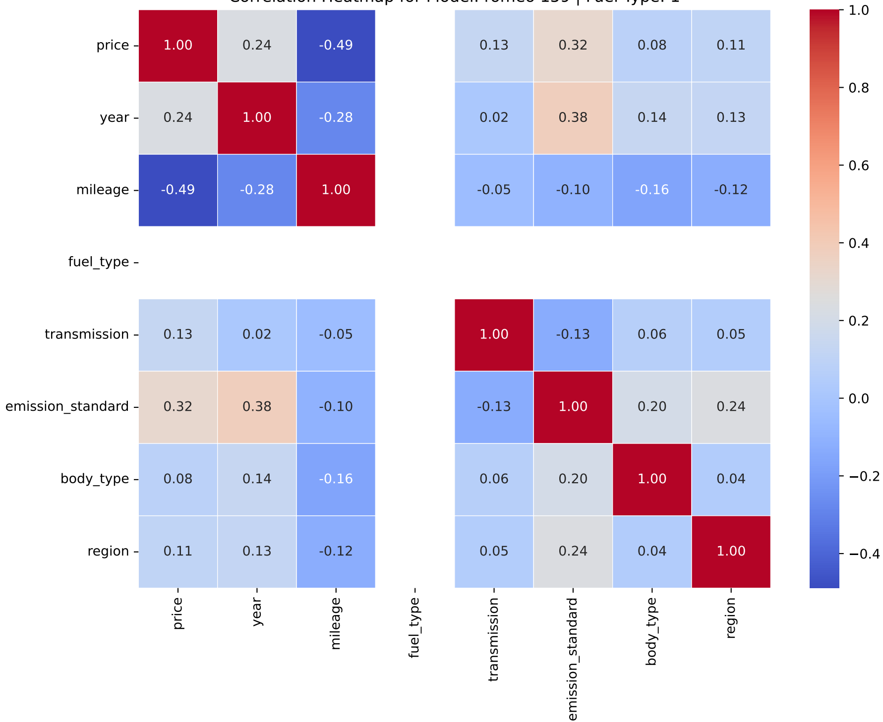
Correlation Heatmap for Model: romeo 159 | Fuel Type: 1
