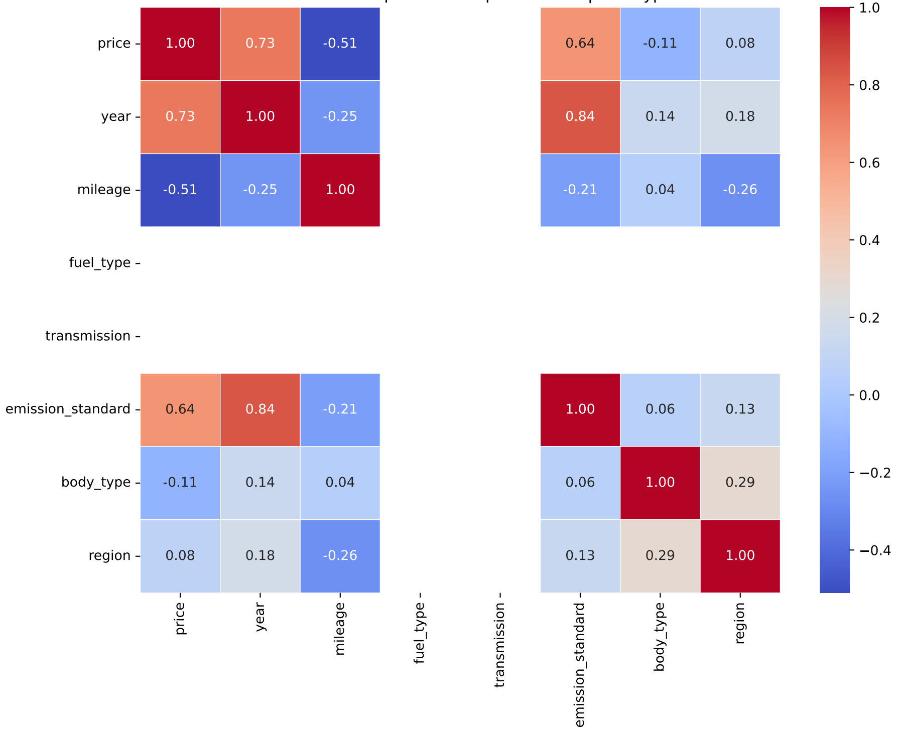
Correlation Heatmap for Model: panda cross | Fuel Type: 1
