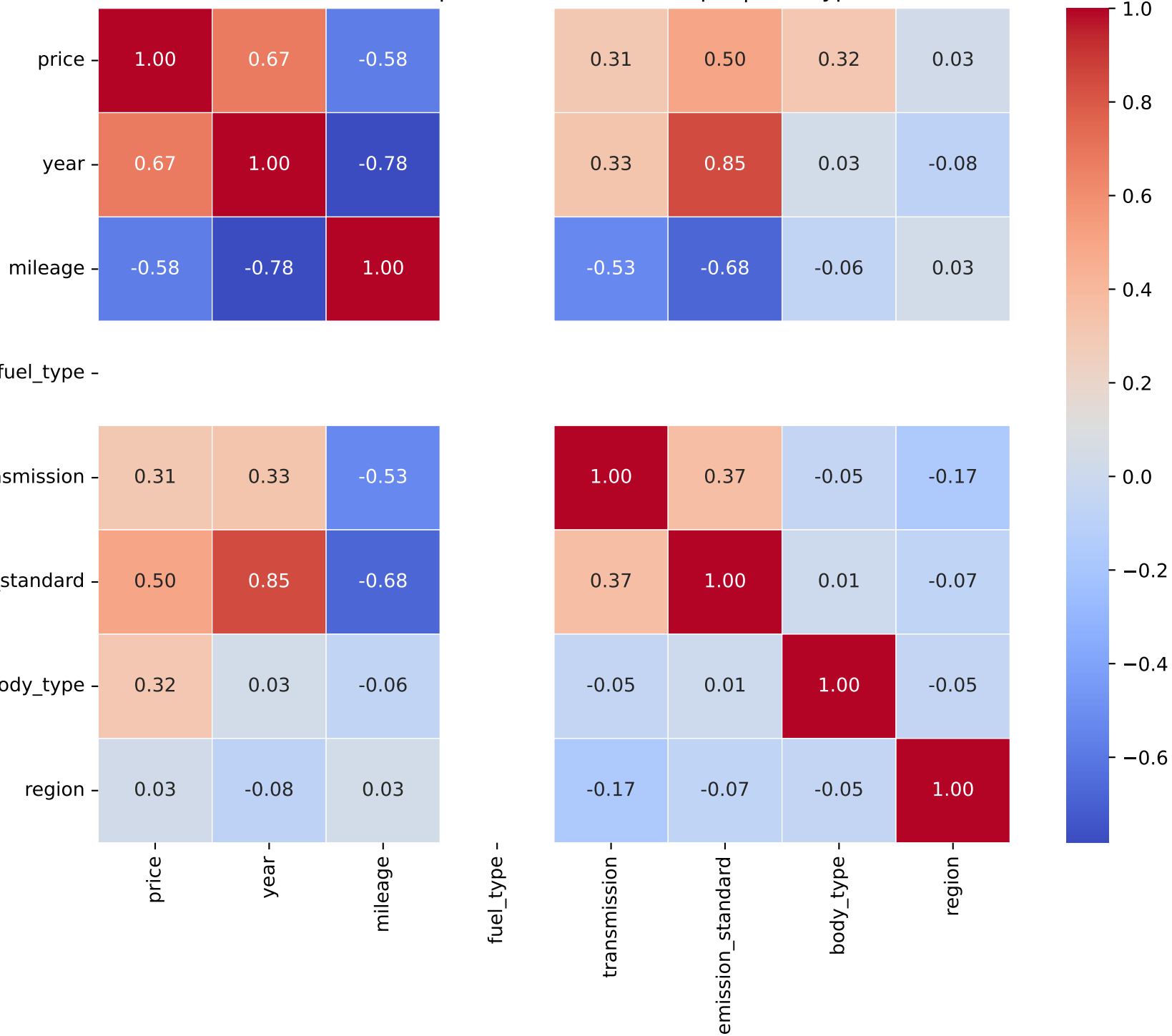
Correlation Heatmap for Model: rover evoque | Fuel Type: 1
