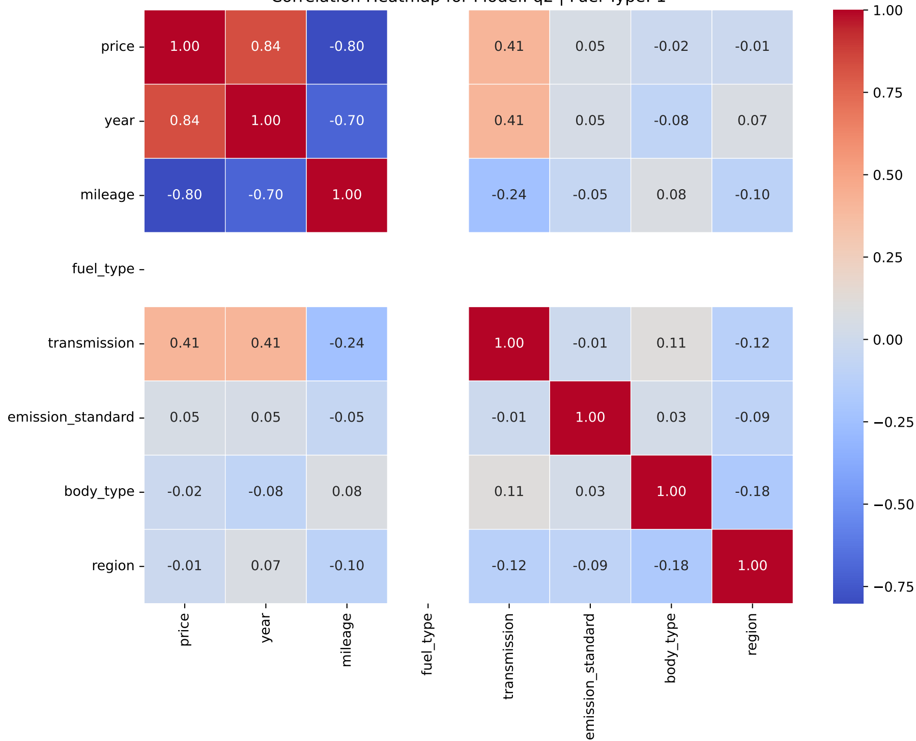
Correlation Heatmap for Model: q2 | Fuel Type: 1
