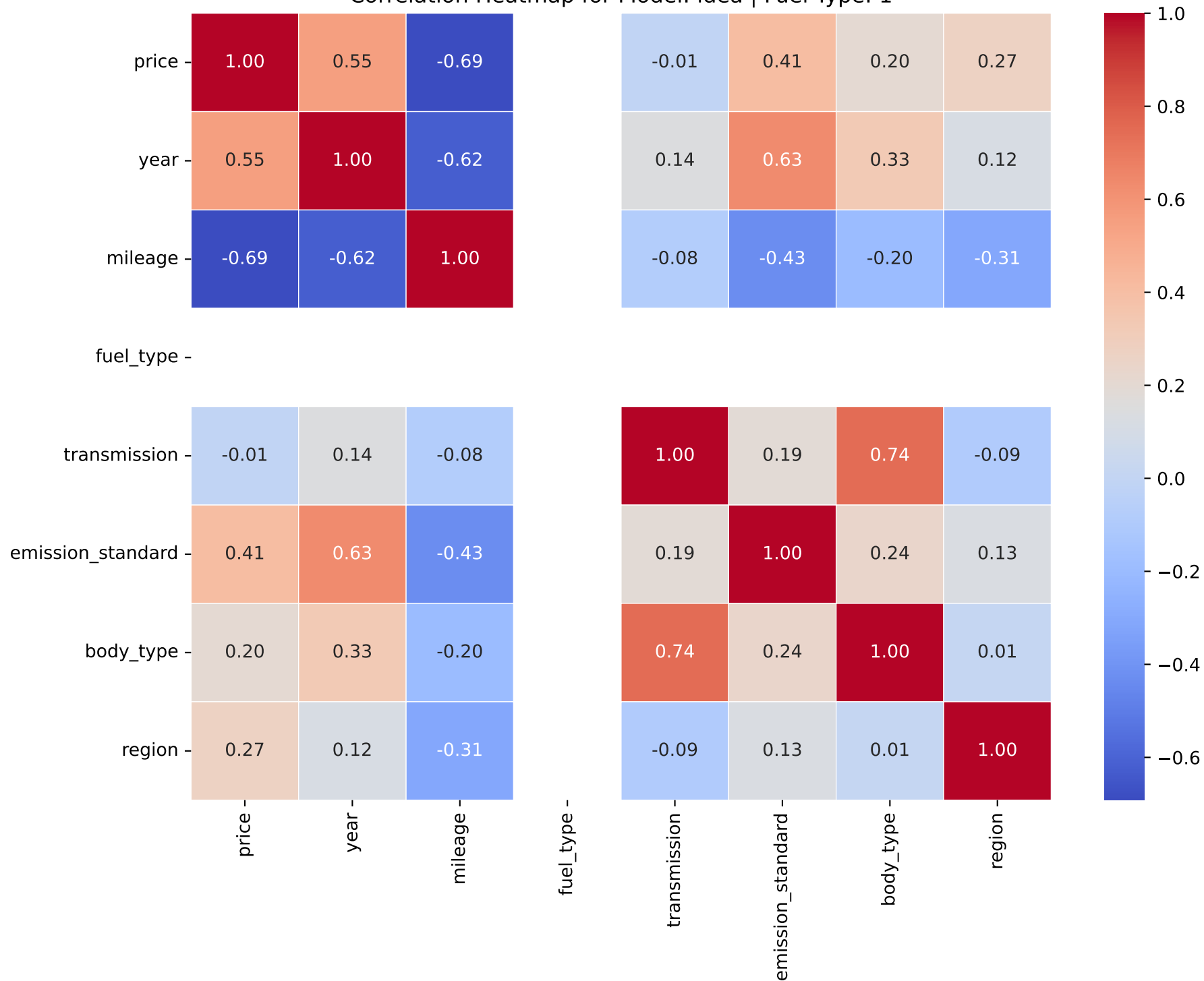
Correlation Heatmap for Model: idea | Fuel Type: 1
