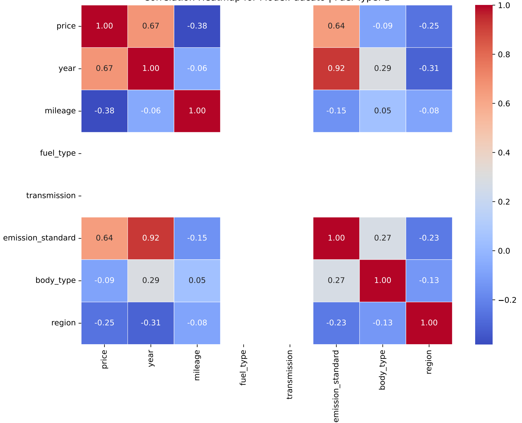
Correlation Heatmap for Model: ducato | Fuel Type: 1
