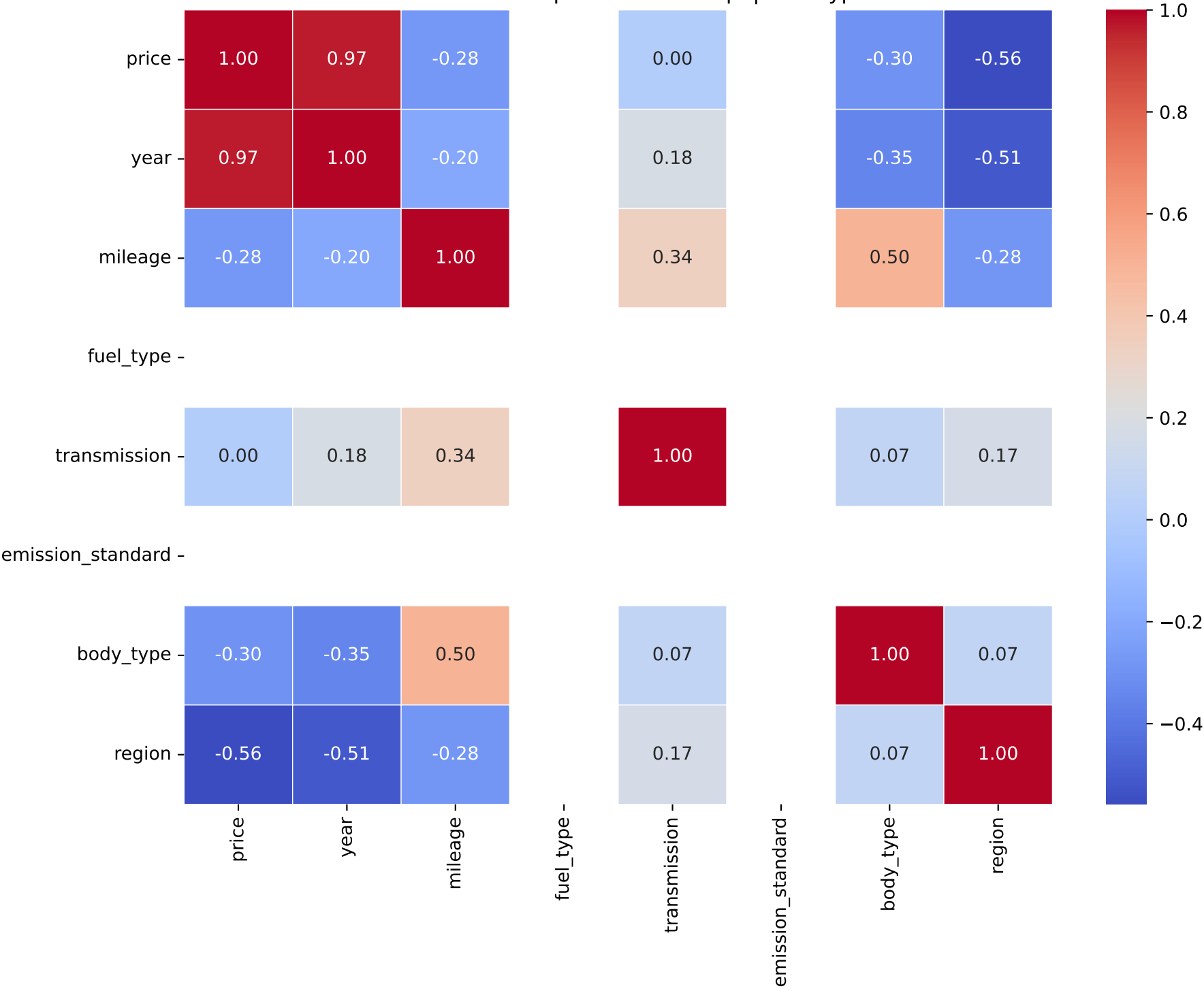
Correlation Heatmap for Model: rs q3 | Fuel Type: 2
