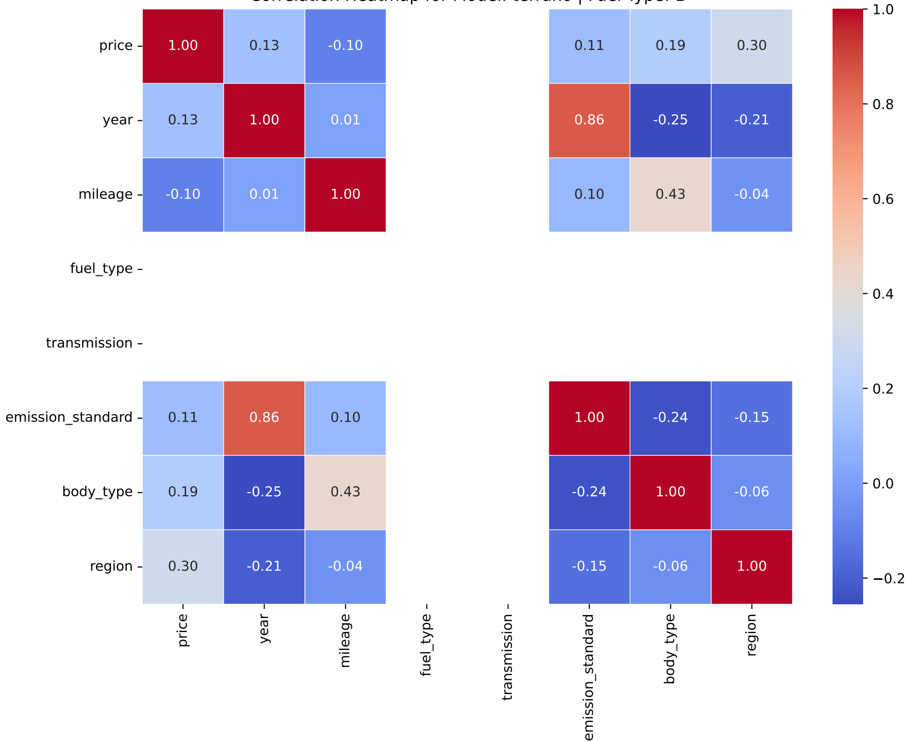
Correlation Heatmap for Model: terrano | Fuel Type: 1
