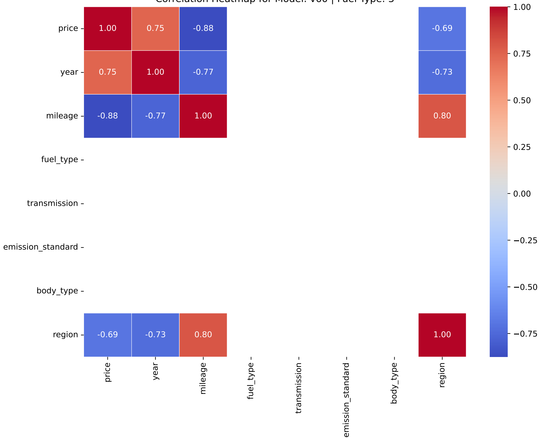
Correlation Heatmap for Model: v60 | Fuel Type: 3
