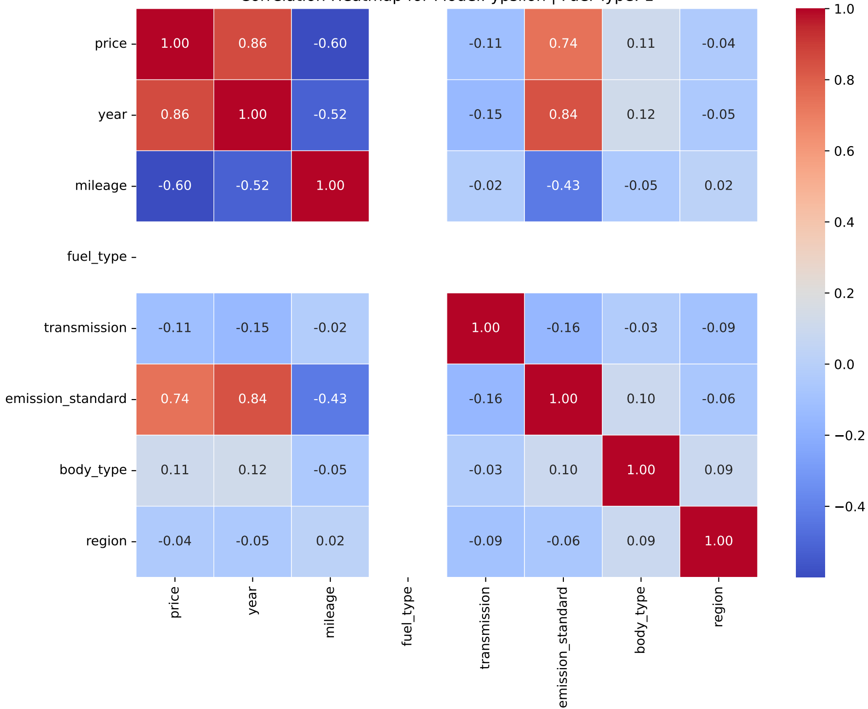
Correlation Heatmap for Model: ypsilon | Fuel Type: 1
