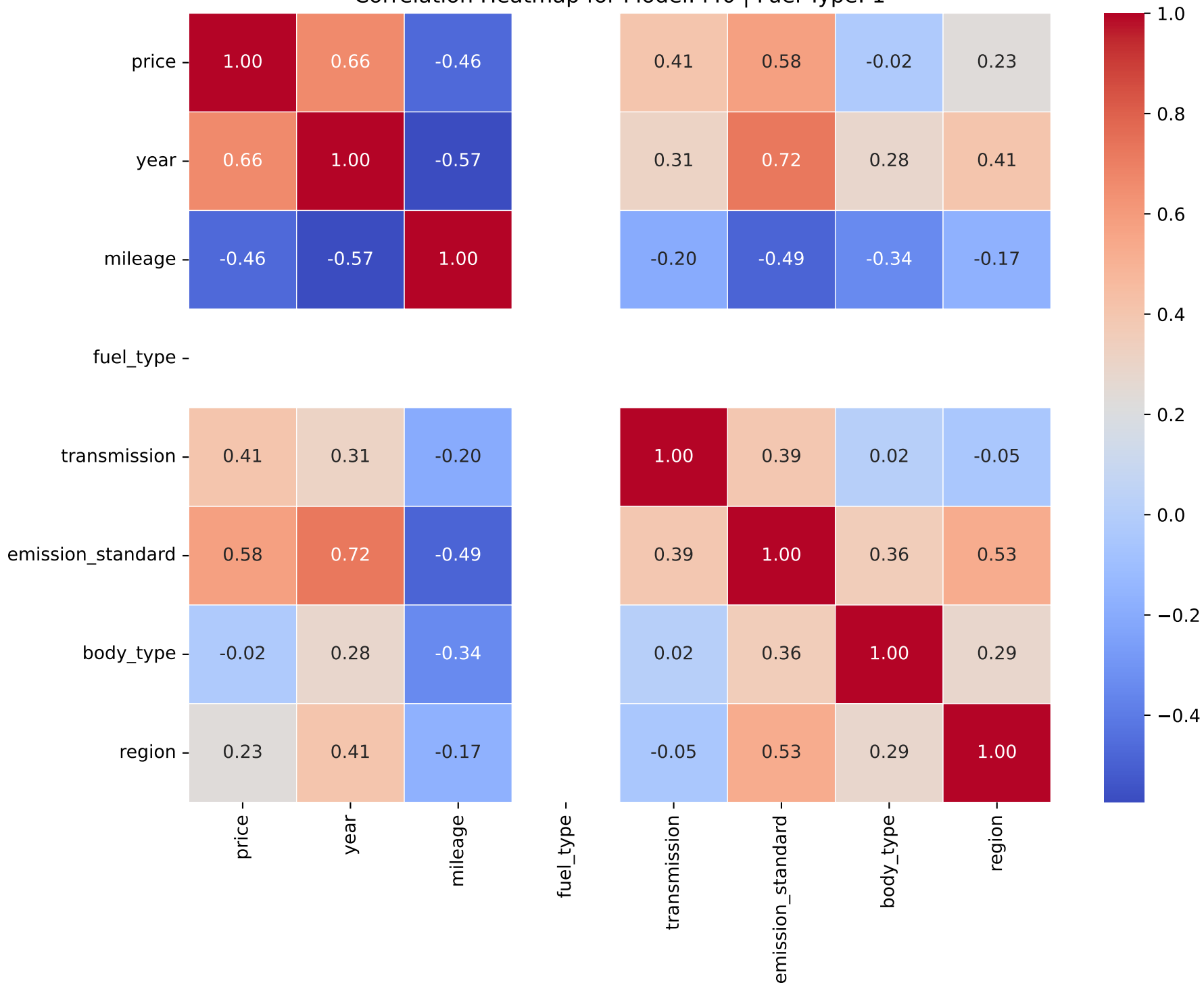
Correlation Heatmap for Model: i40 | Fuel Type: 1
