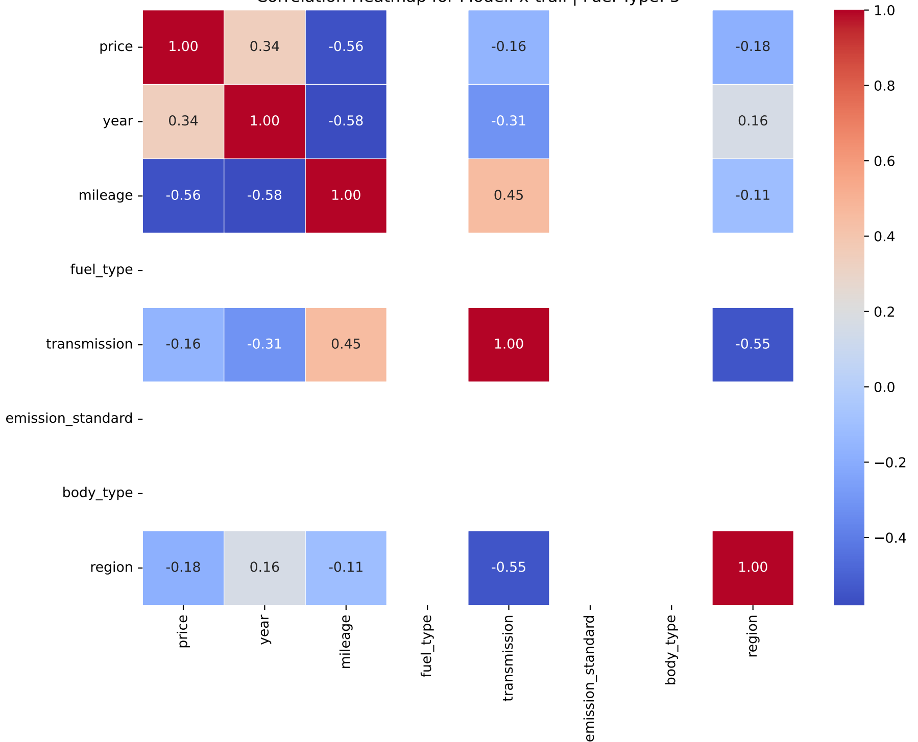
Correlation Heatmap for Model: x-trail | Fuel Type: 3
