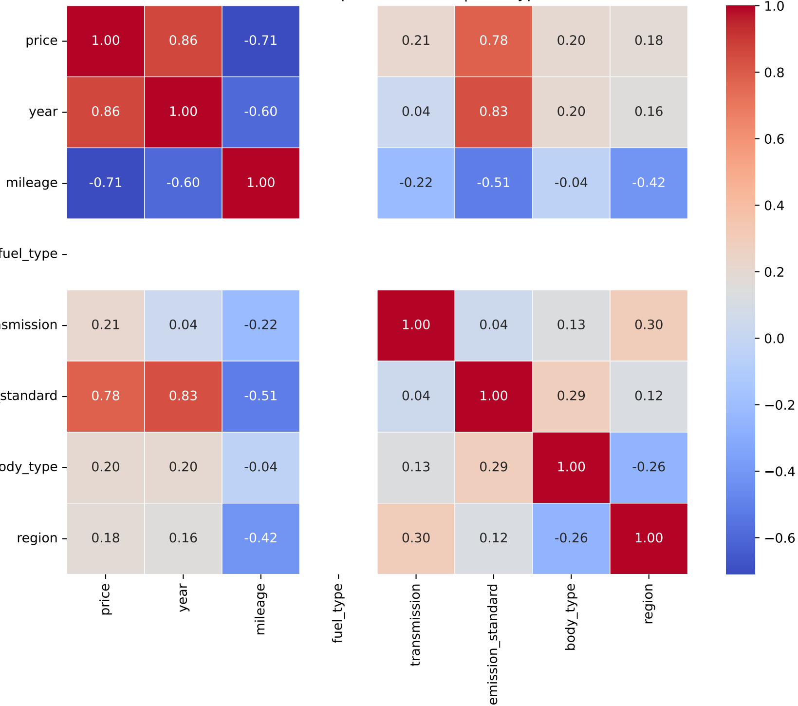
Correlation Heatmap for Model: a7 | Fuel Type: 1
