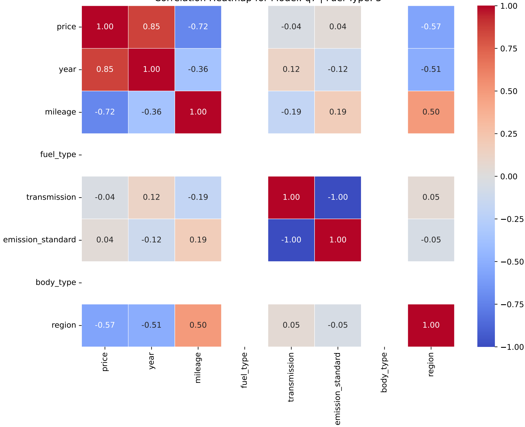
Correlation Heatmap for Model: q7 | Fuel Type: 3
