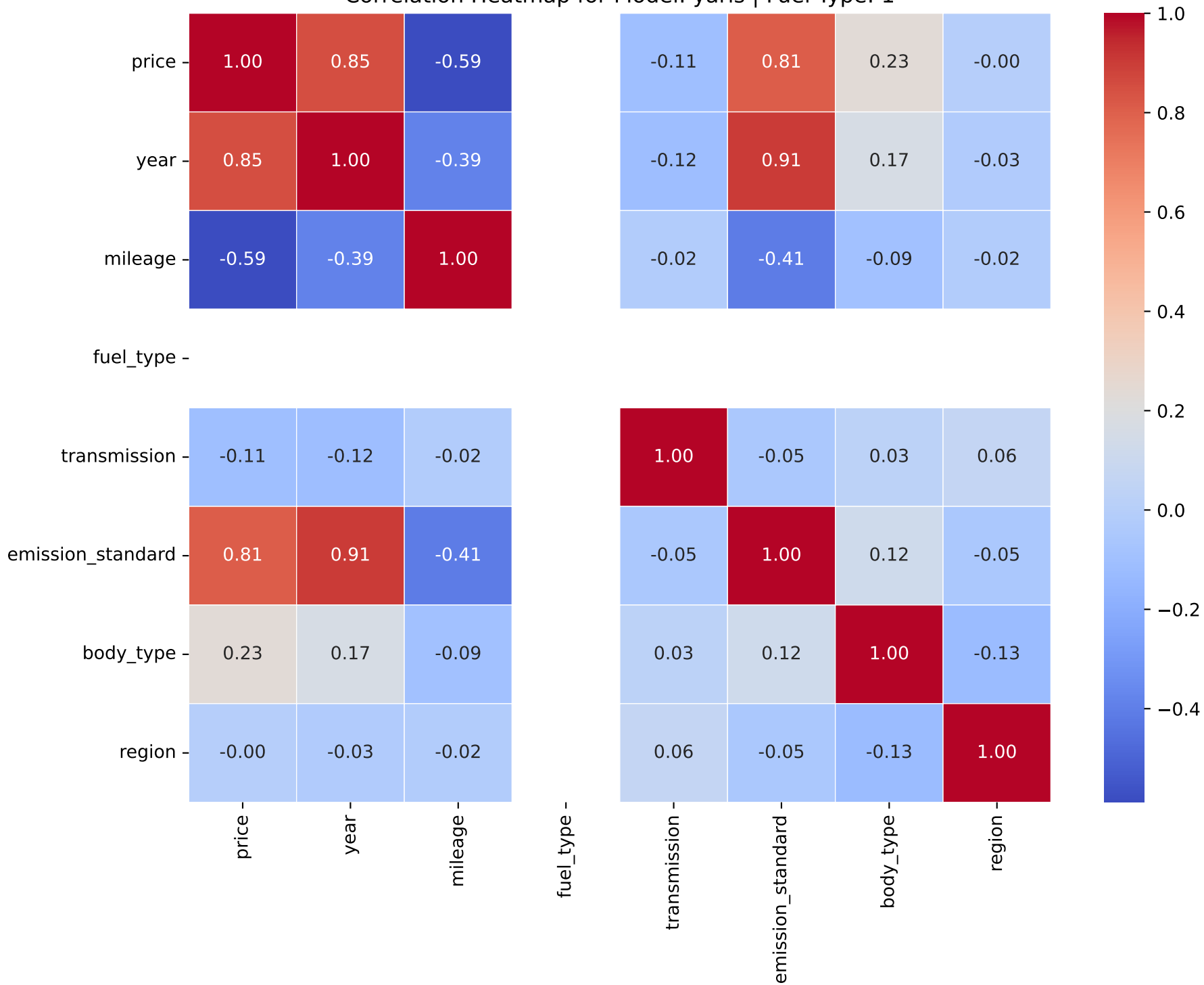
Correlation Heatmap for Model: yaris | Fuel Type: 1
