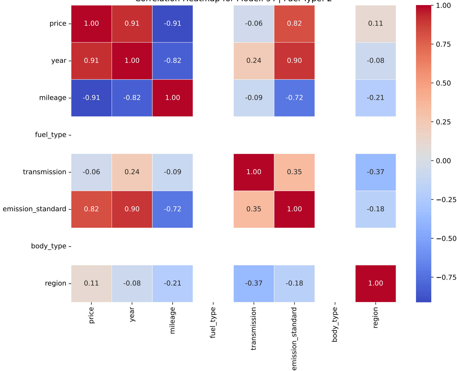
Correlation Heatmap for Model: s4 | Fuel Type: 2
