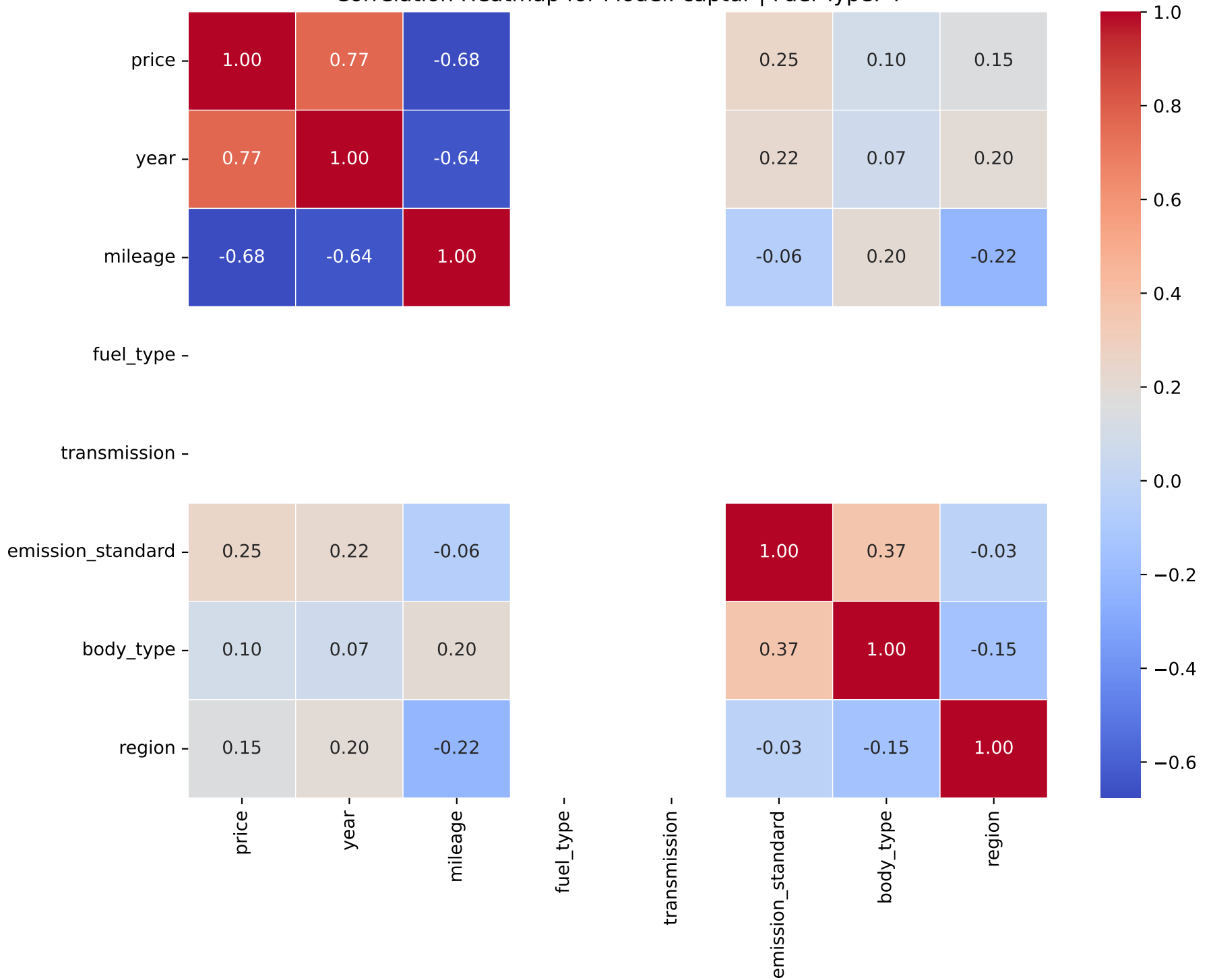
Correlation Heatmap for Model: captur | Fuel Type: 4
