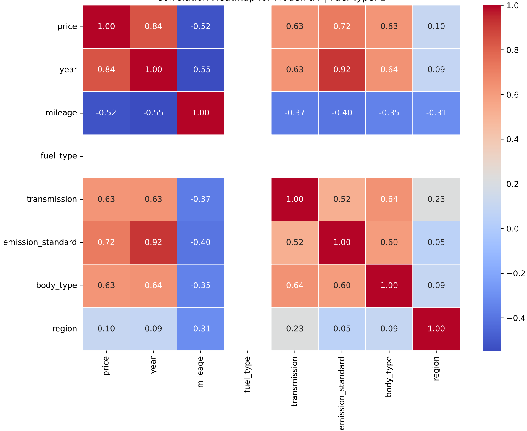
Correlation Heatmap for Model: a4 | Fuel Type: 2
