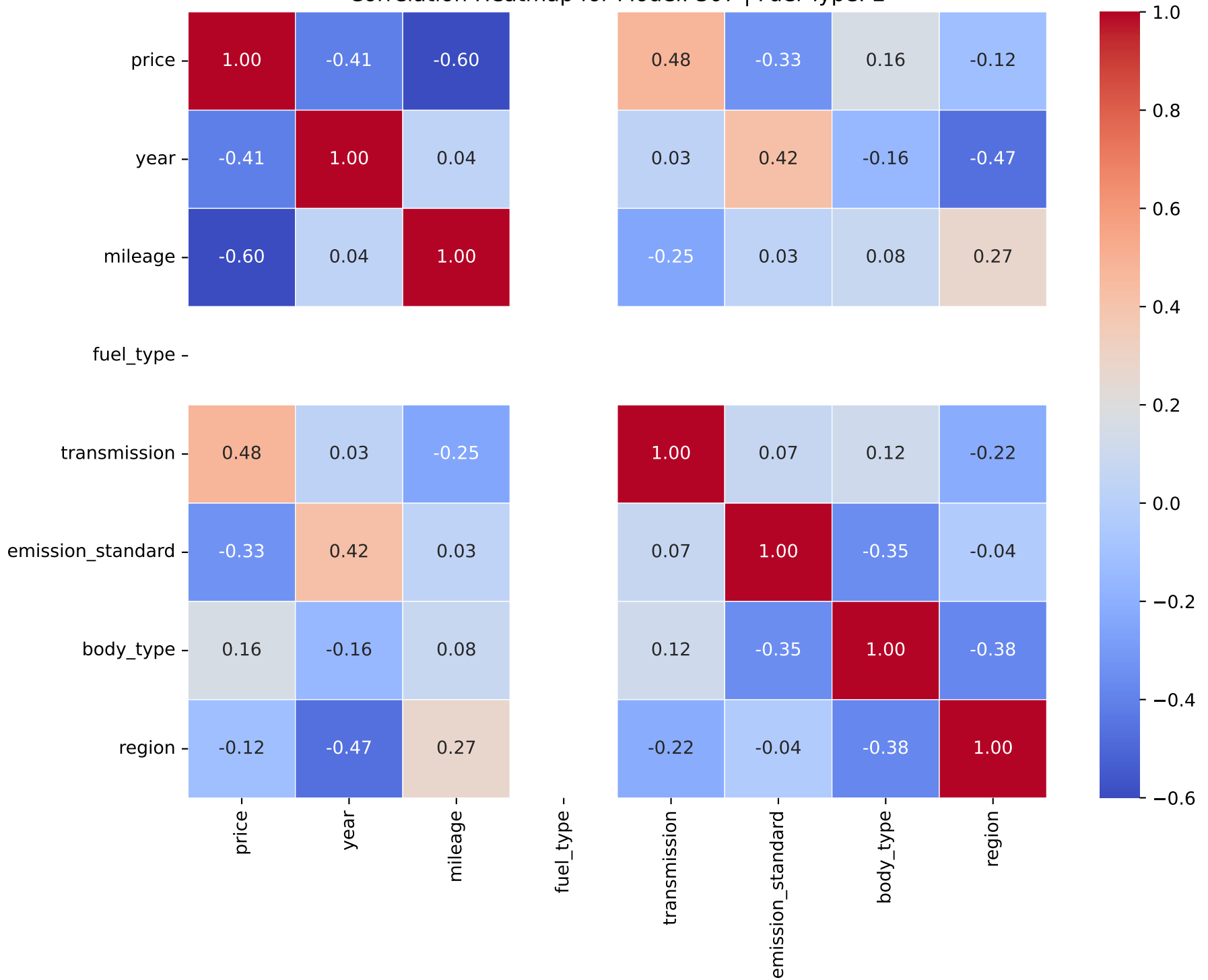
Correlation Heatmap for Model: 307 | Fuel Type: 2
