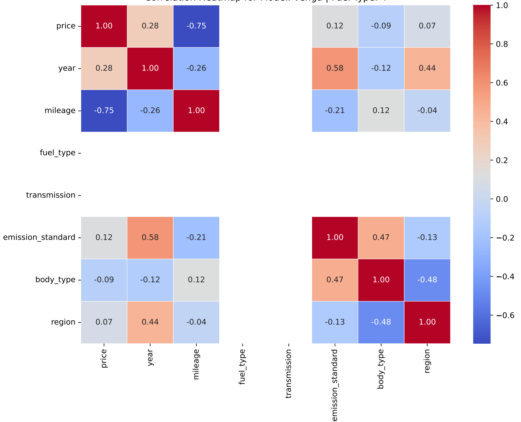
Correlation Heatmap for Model: venga | Fuel Type: 4
