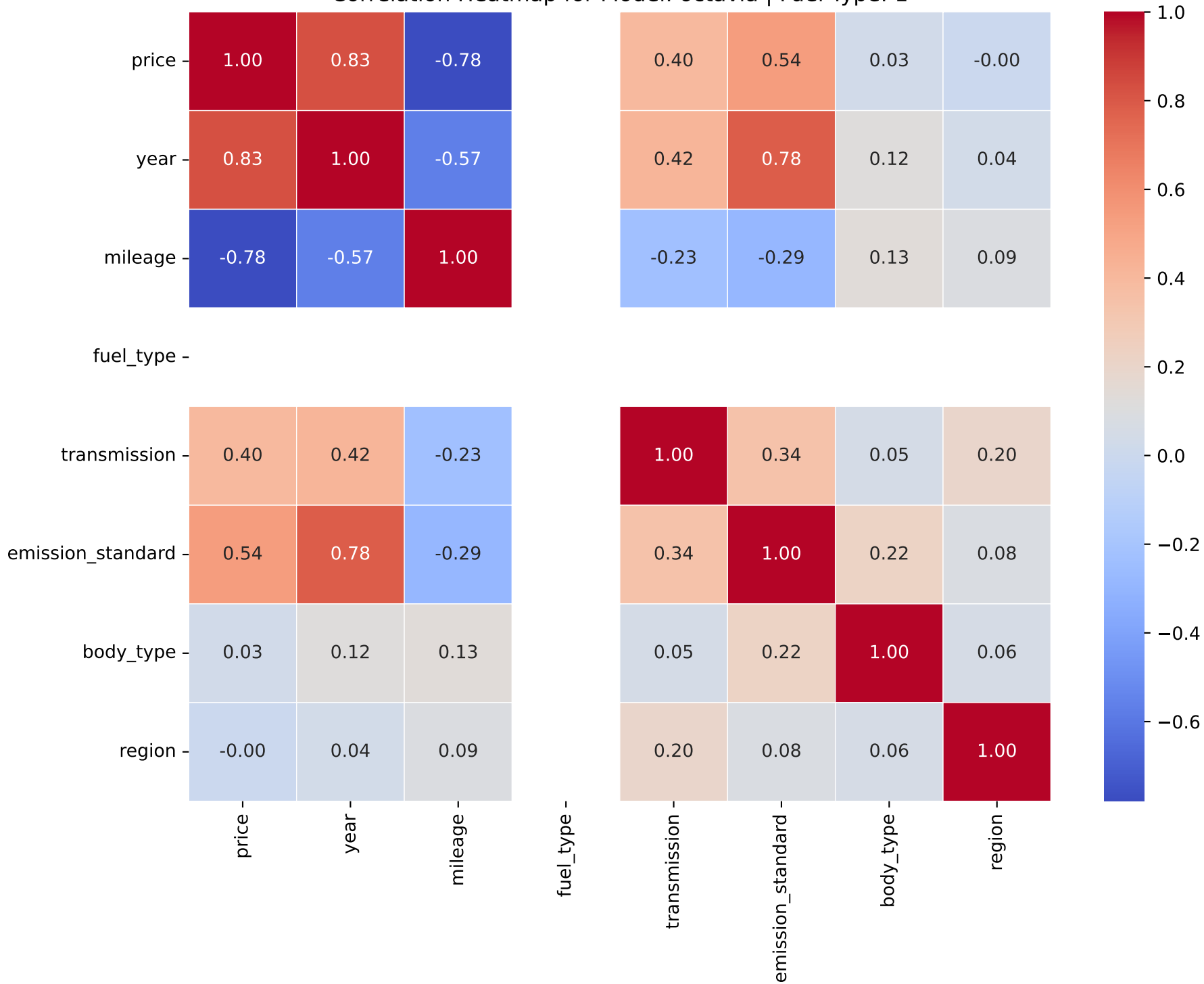
Correlation Heatmap for Model: octavia | Fuel Type: 1
