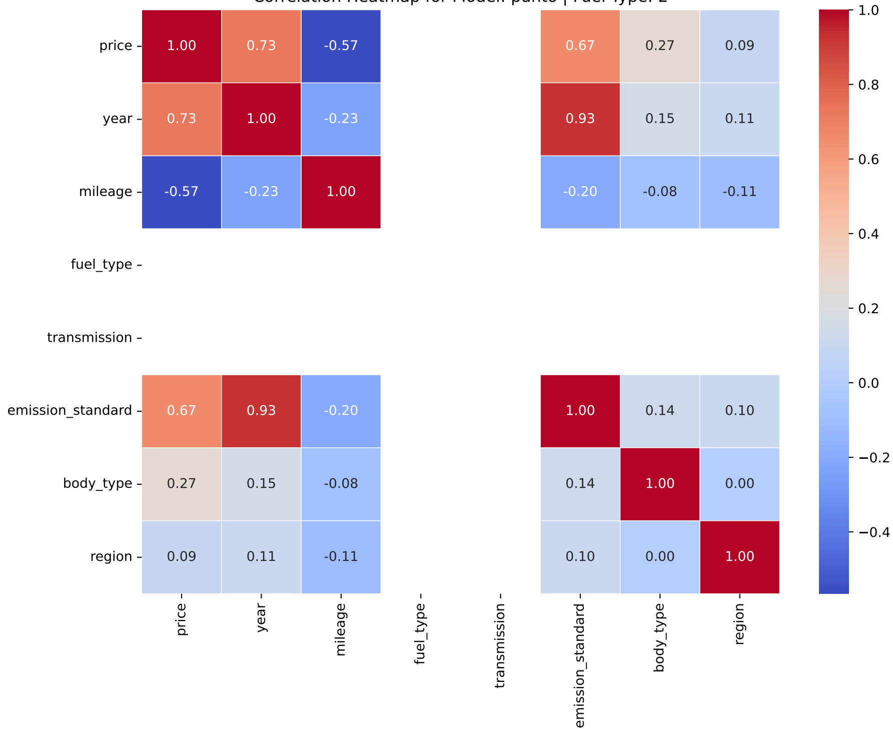
Correlation Heatmap for Model: punto | Fuel Type: 2
