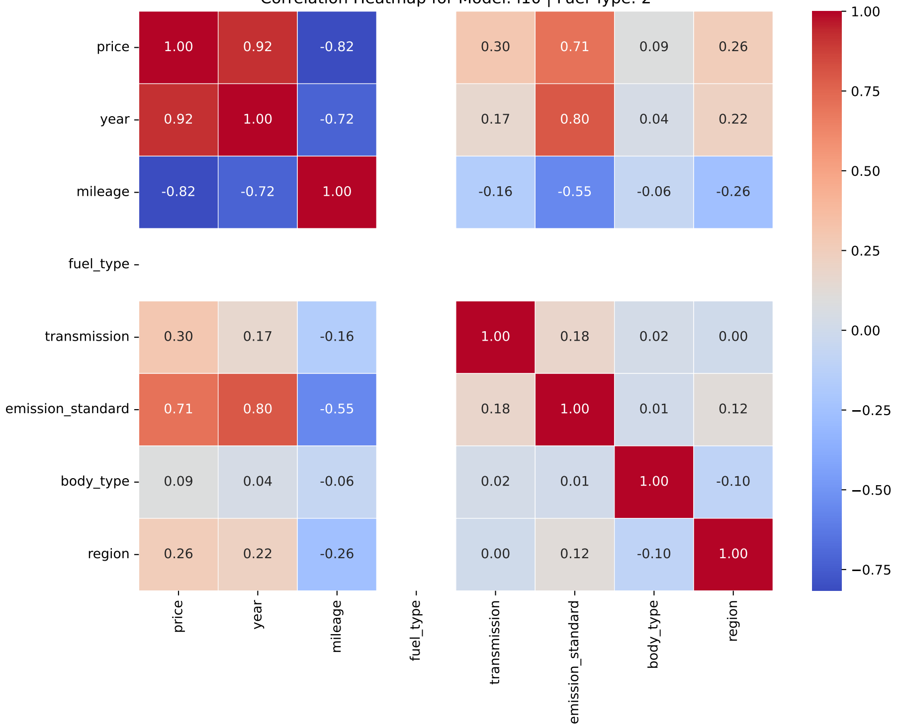
Correlation Heatmap for Model: i10 | Fuel Type: 2
