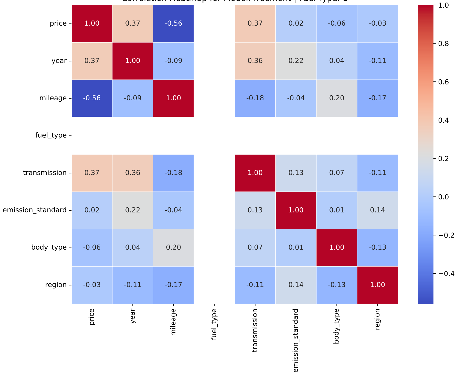
Correlation Heatmap for Model: freemont | Fuel Type: 1
