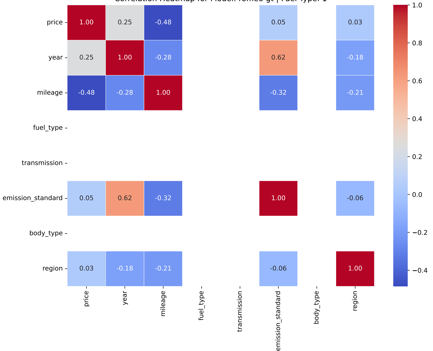
Correlation Heatmap for Model: romeo gt | Fuel Type: 1
