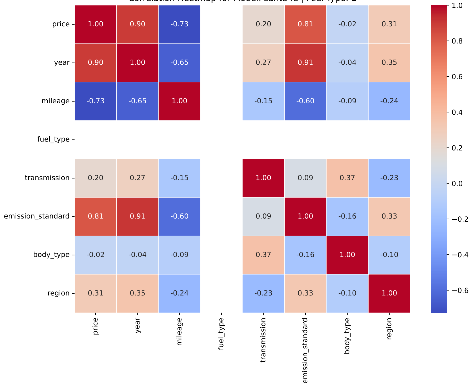
Correlation Heatmap for Model: santa fe | Fuel Type: 1
