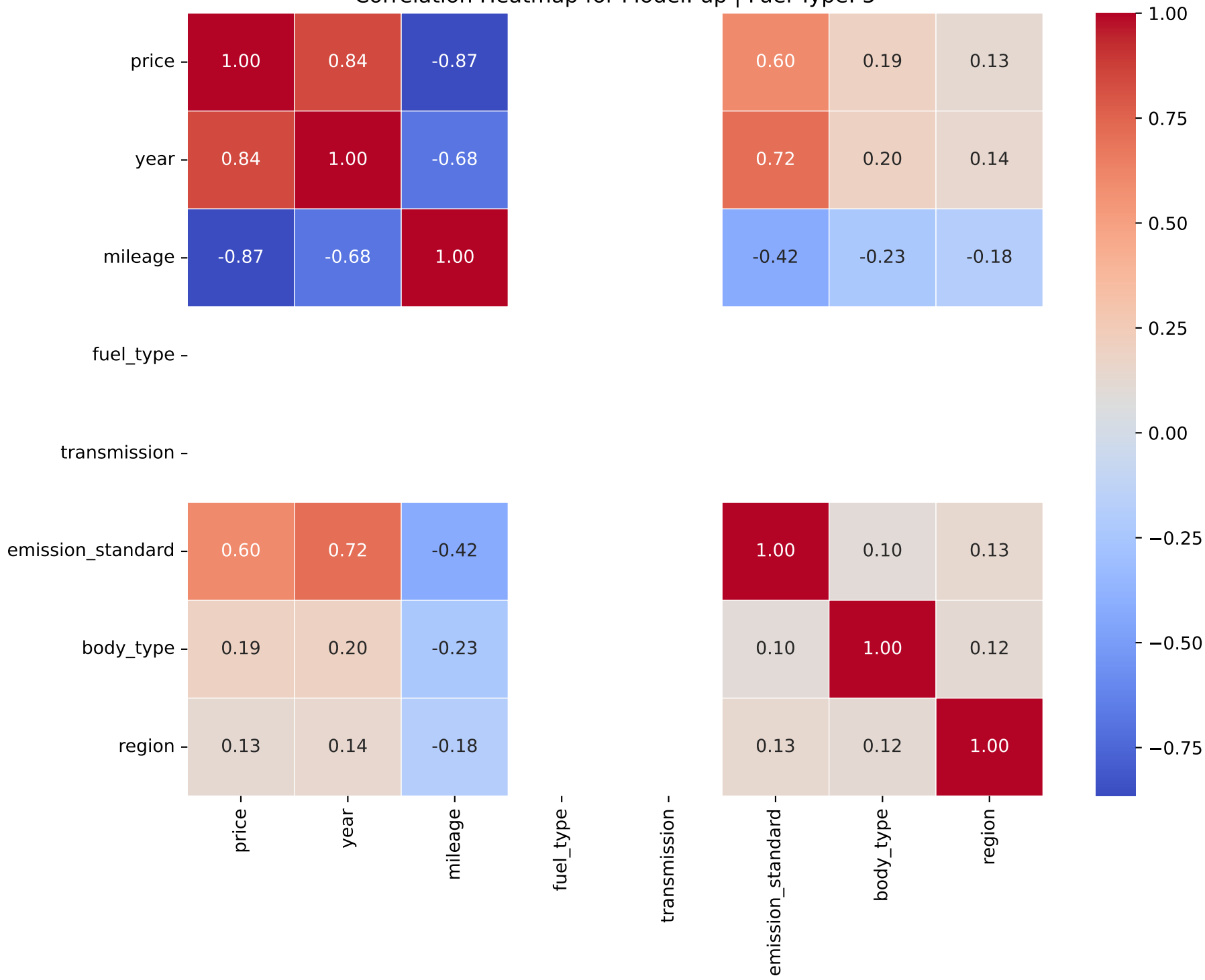
Correlation Heatmap for Model: up | Fuel Type: 5
