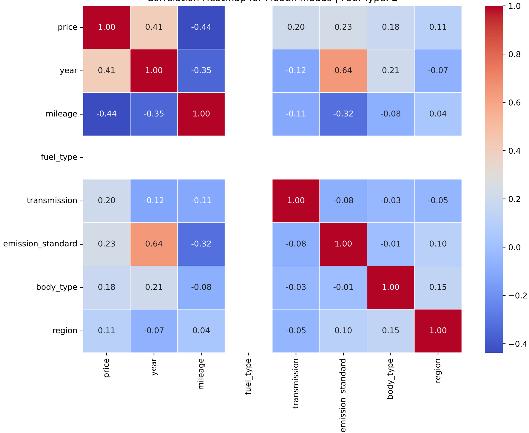
Correlation Heatmap for Model: modus | Fuel Type: 2
