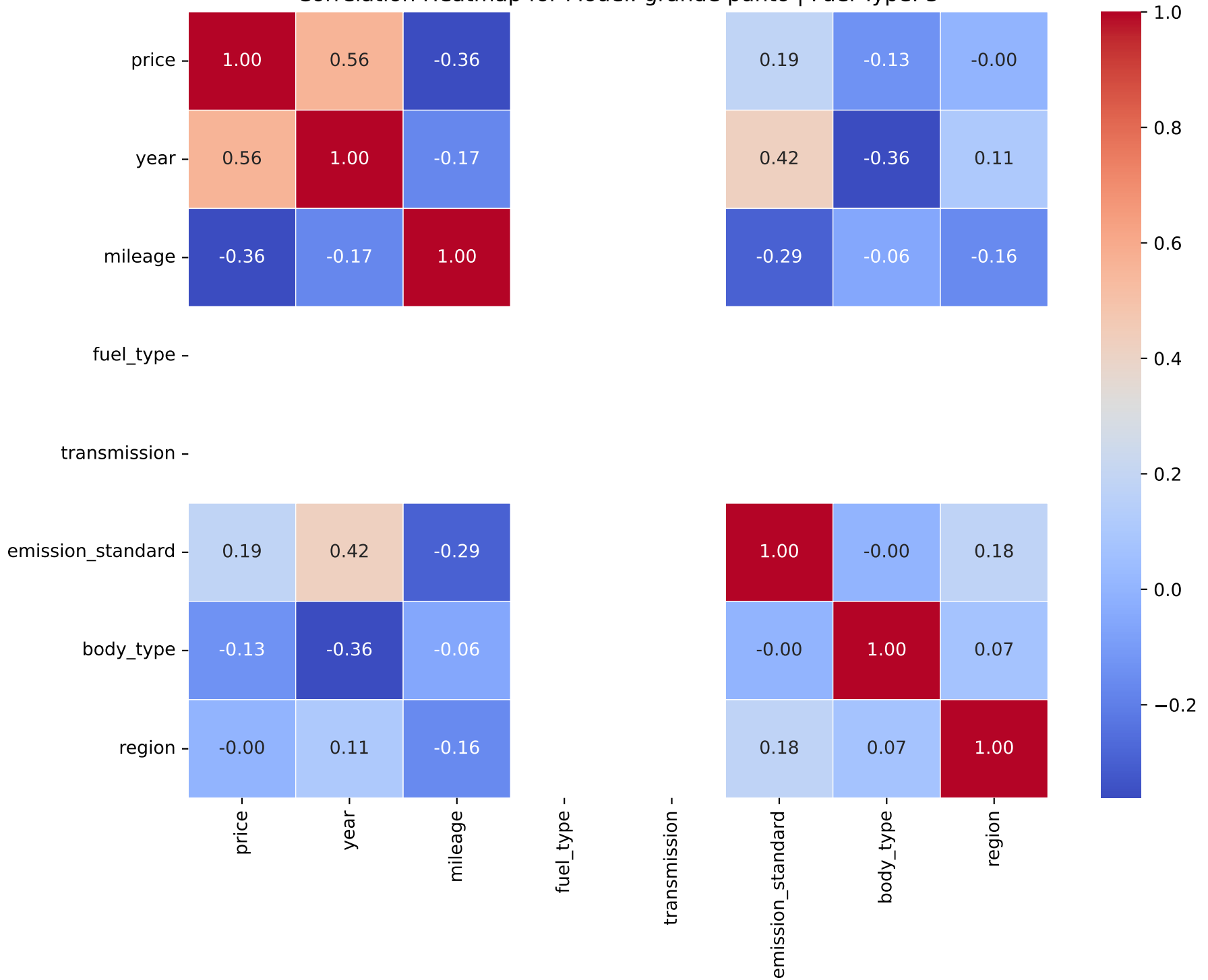
Correlation Heatmap for Model: grande punto | Fuel Type: 5
