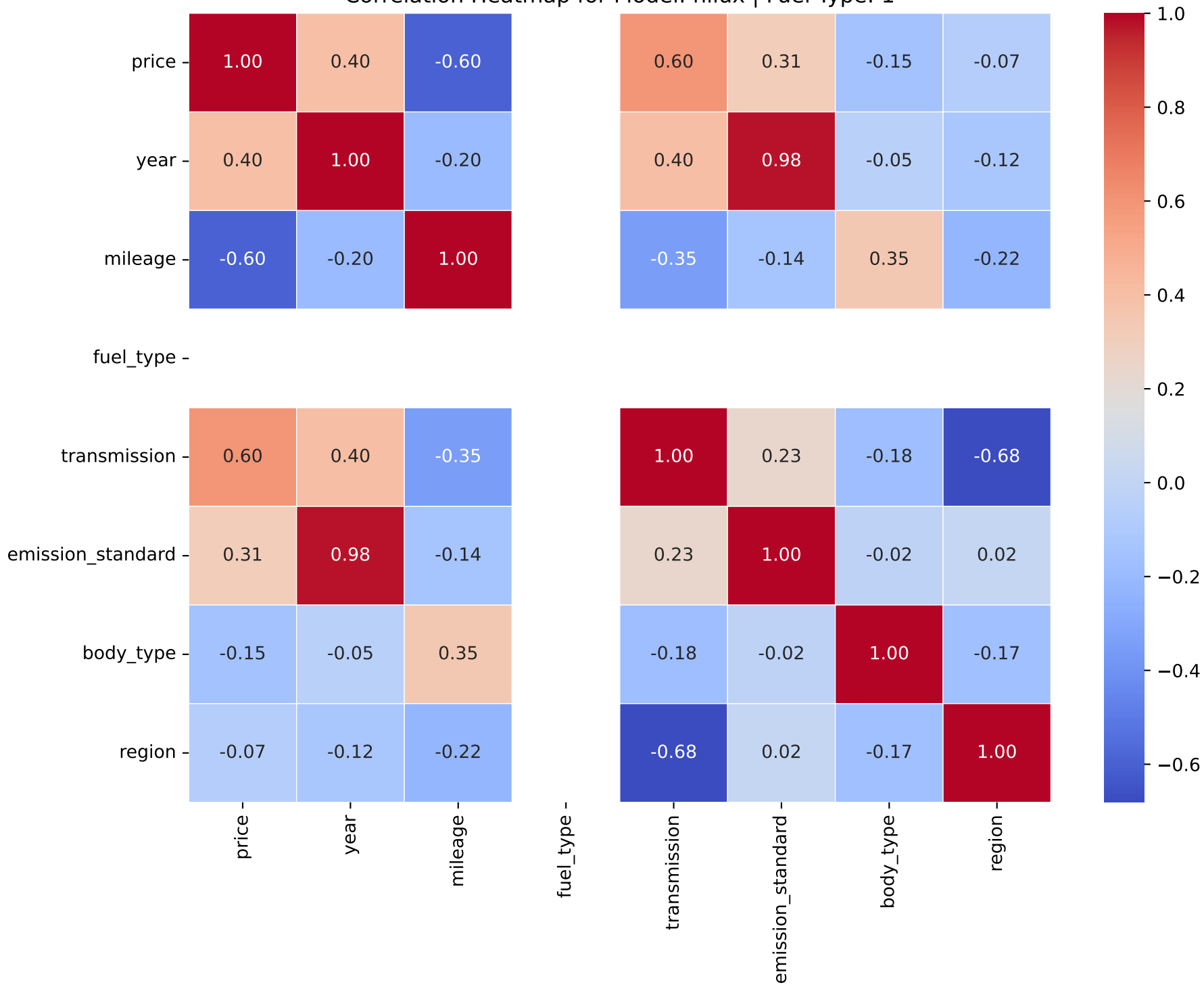
Correlation Heatmap for Model: hilux | Fuel Type: 1
