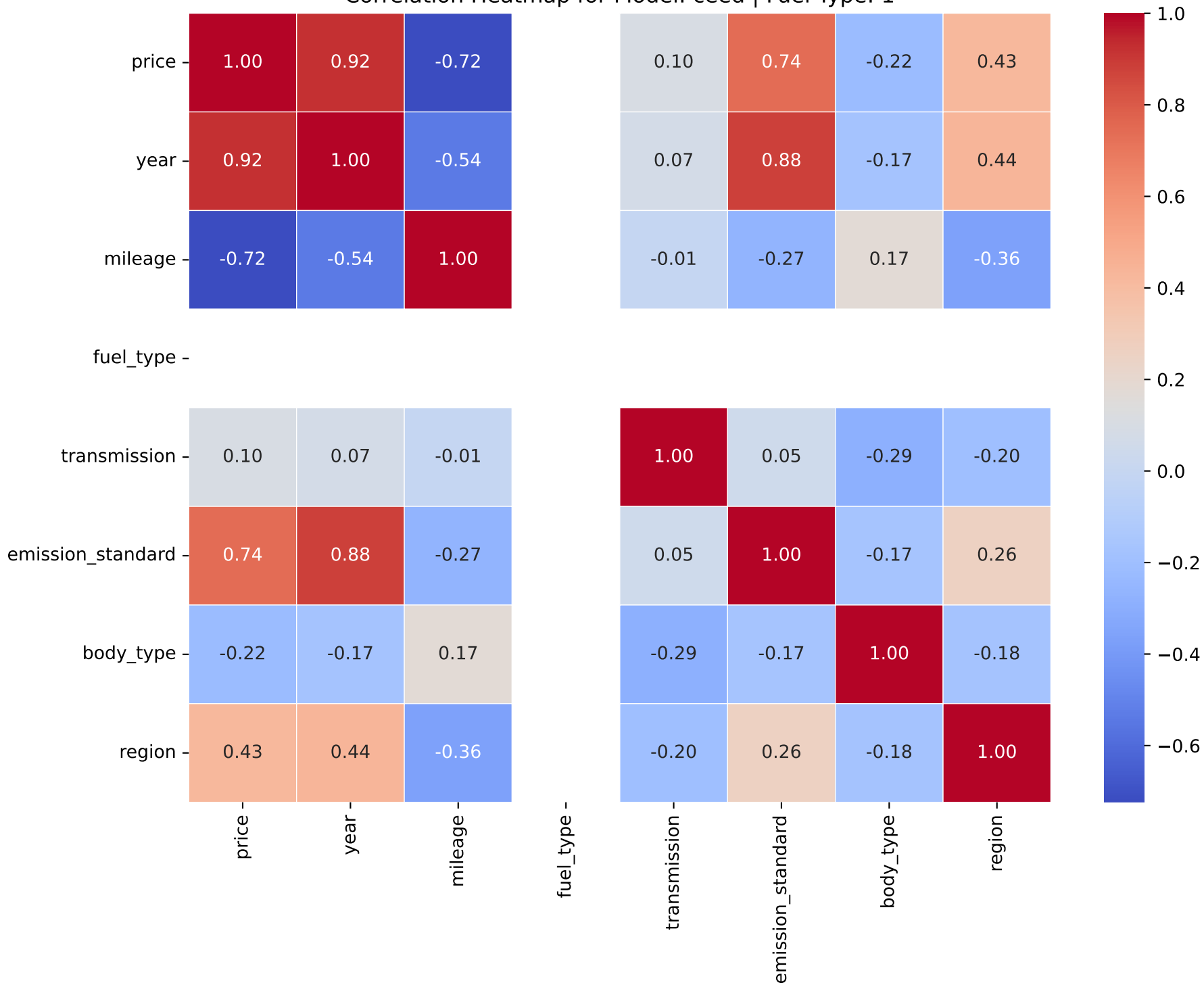
Correlation Heatmap for Model: ceed | Fuel Type: 1
