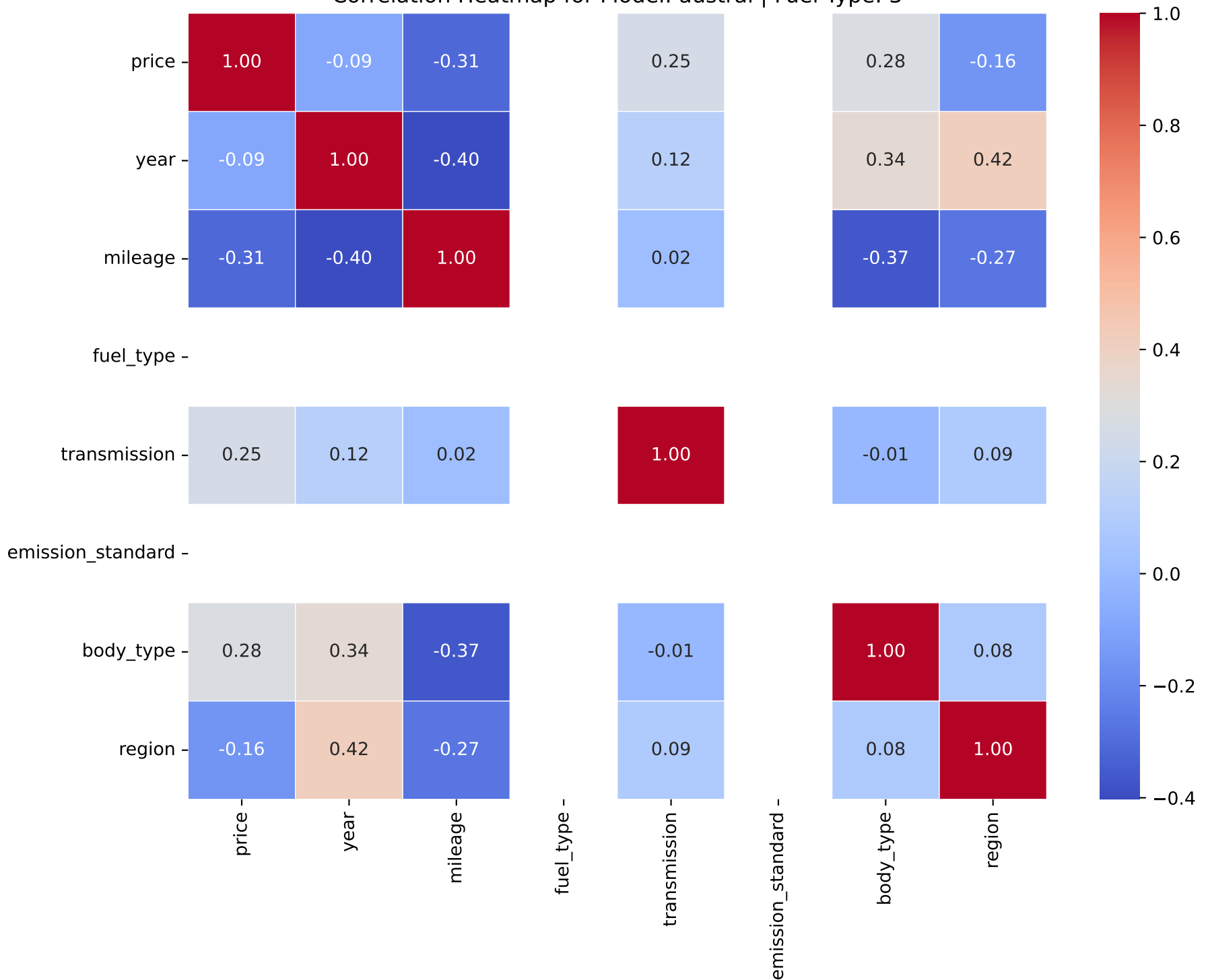
Correlation Heatmap for Model: austral | Fuel Type: 3
