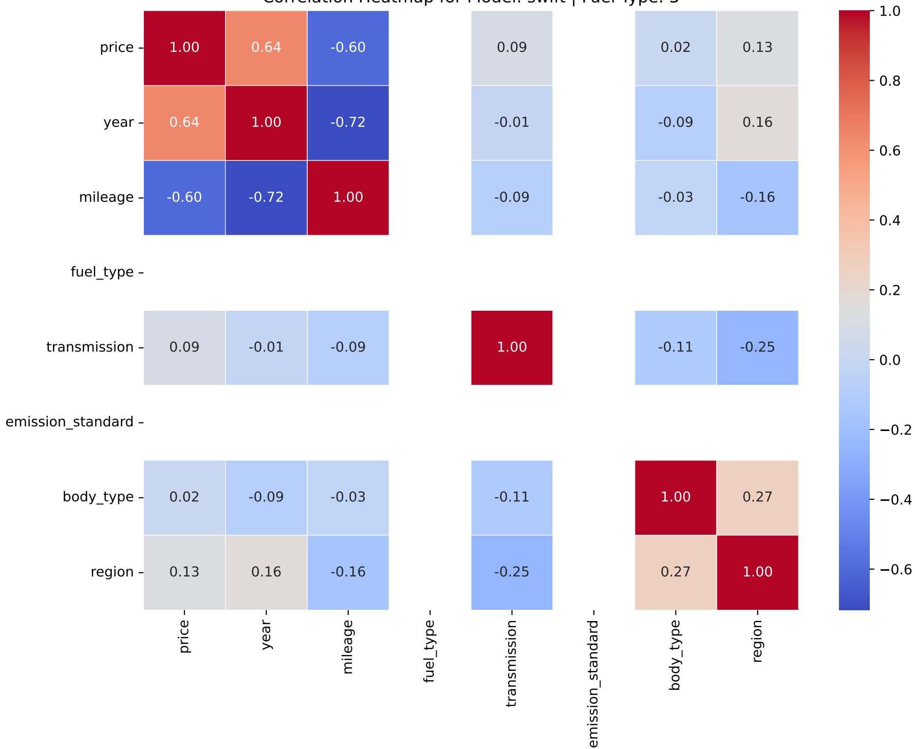
Correlation Heatmap for Model: swift | Fuel Type: 3
