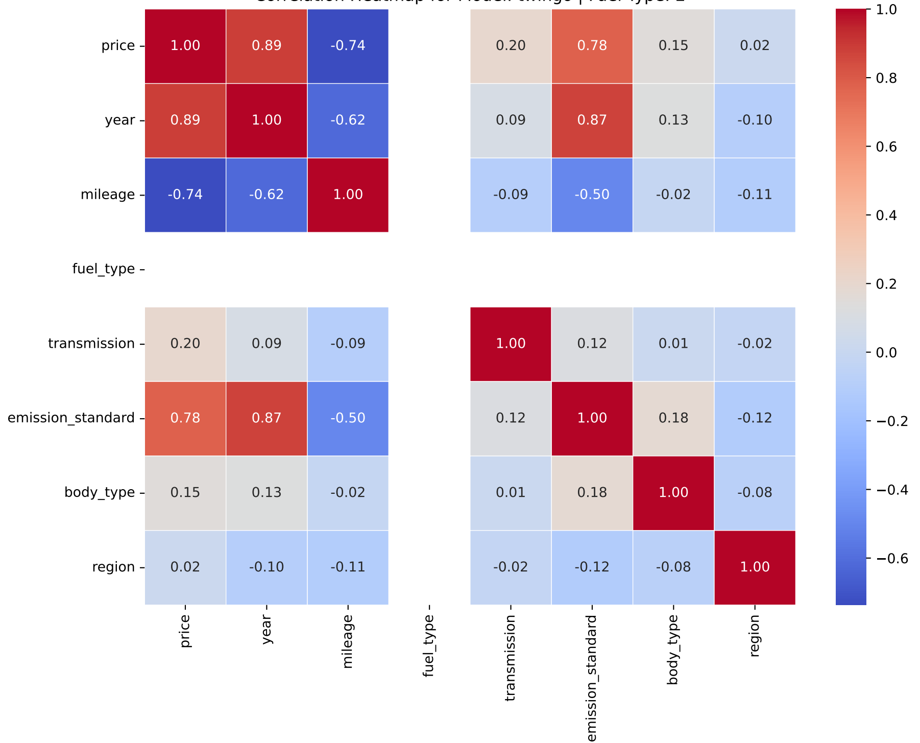
Correlation Heatmap for Model: twingo | Fuel Type: 2
