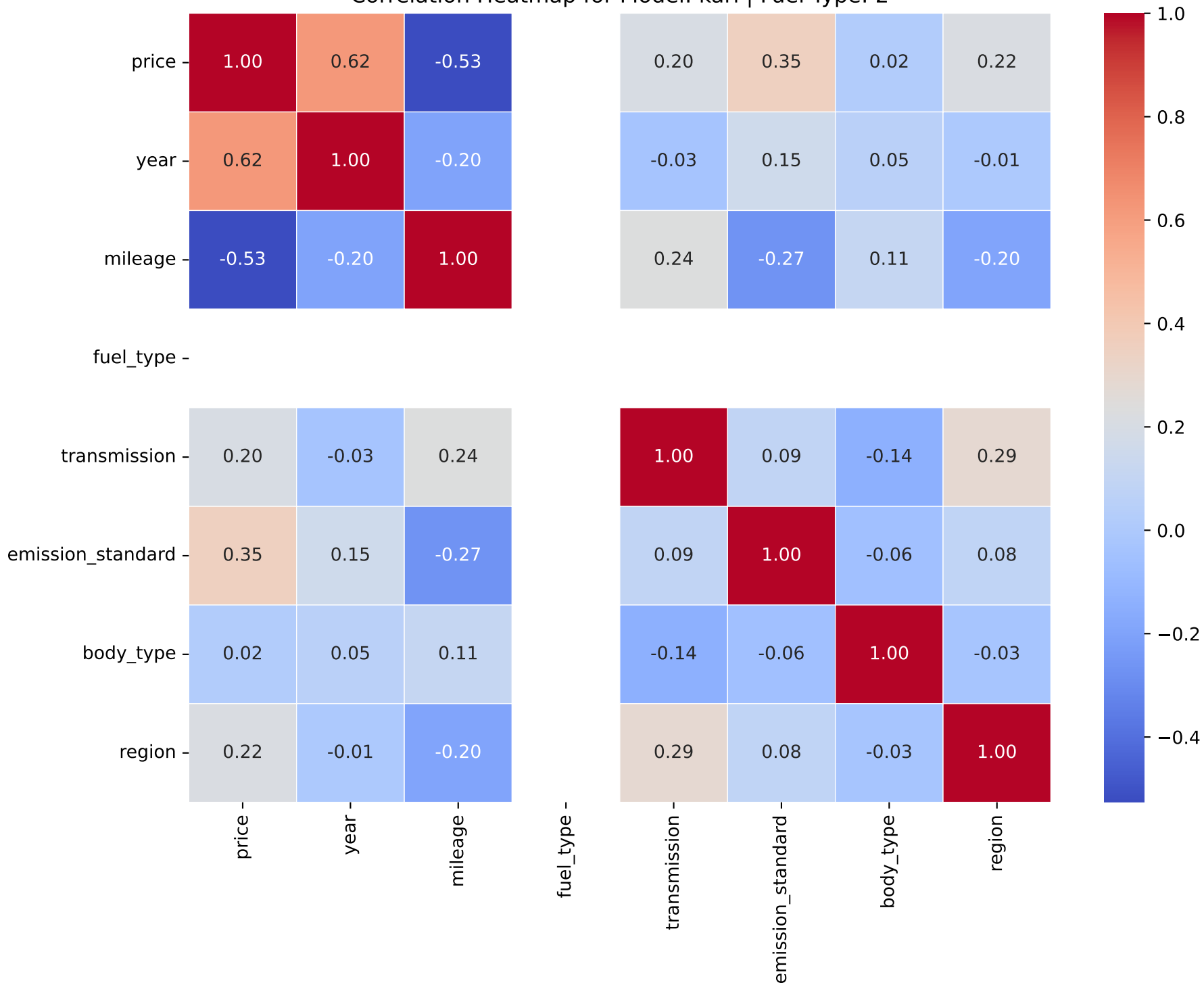
Correlation Heatmap for Model: karl | Fuel Type: 2
