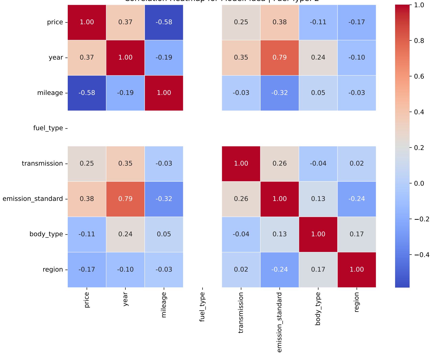
Correlation Heatmap for Model: idea | Fuel Type: 2
