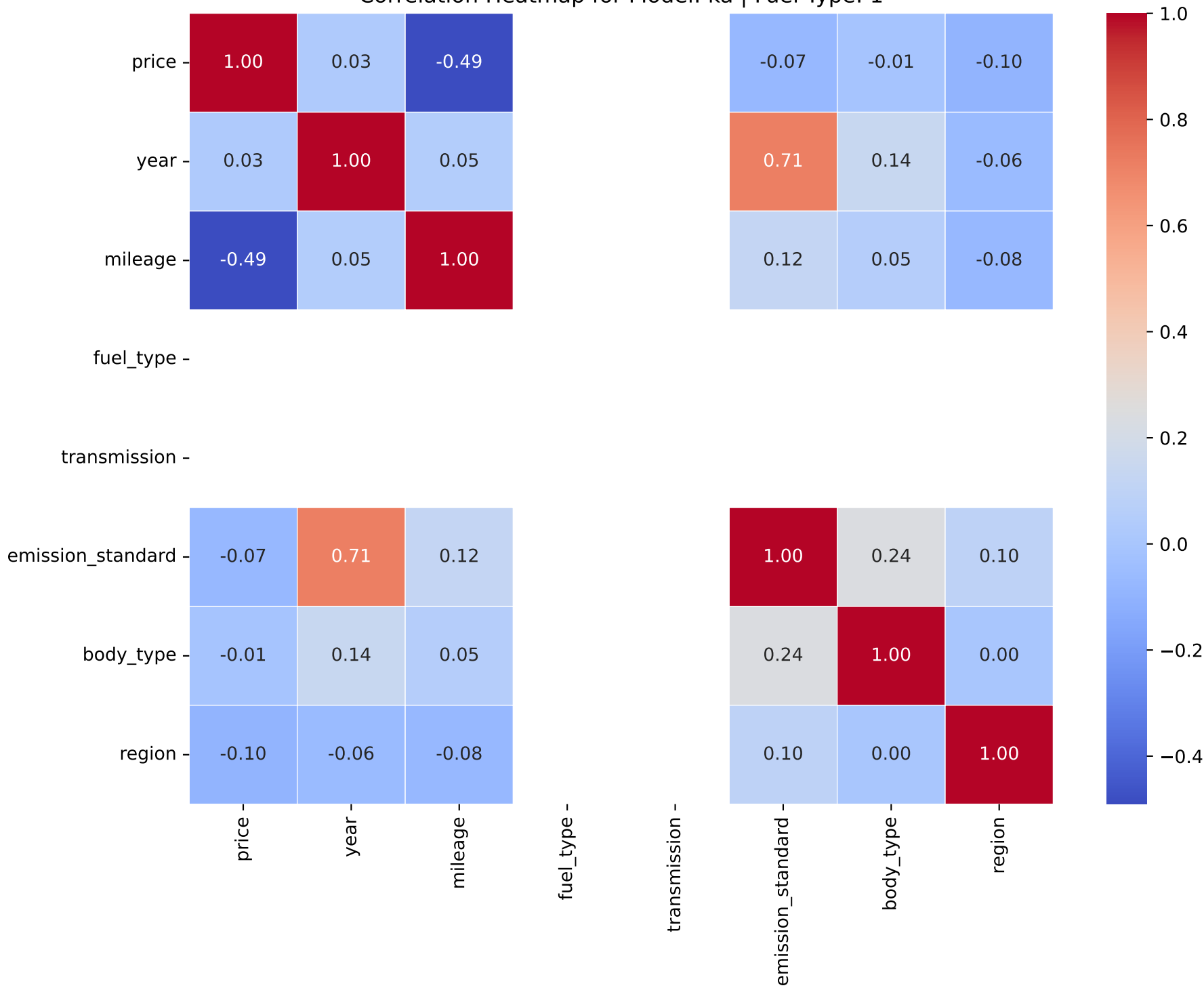
Correlation Heatmap for Model: ka | Fuel Type: 1
