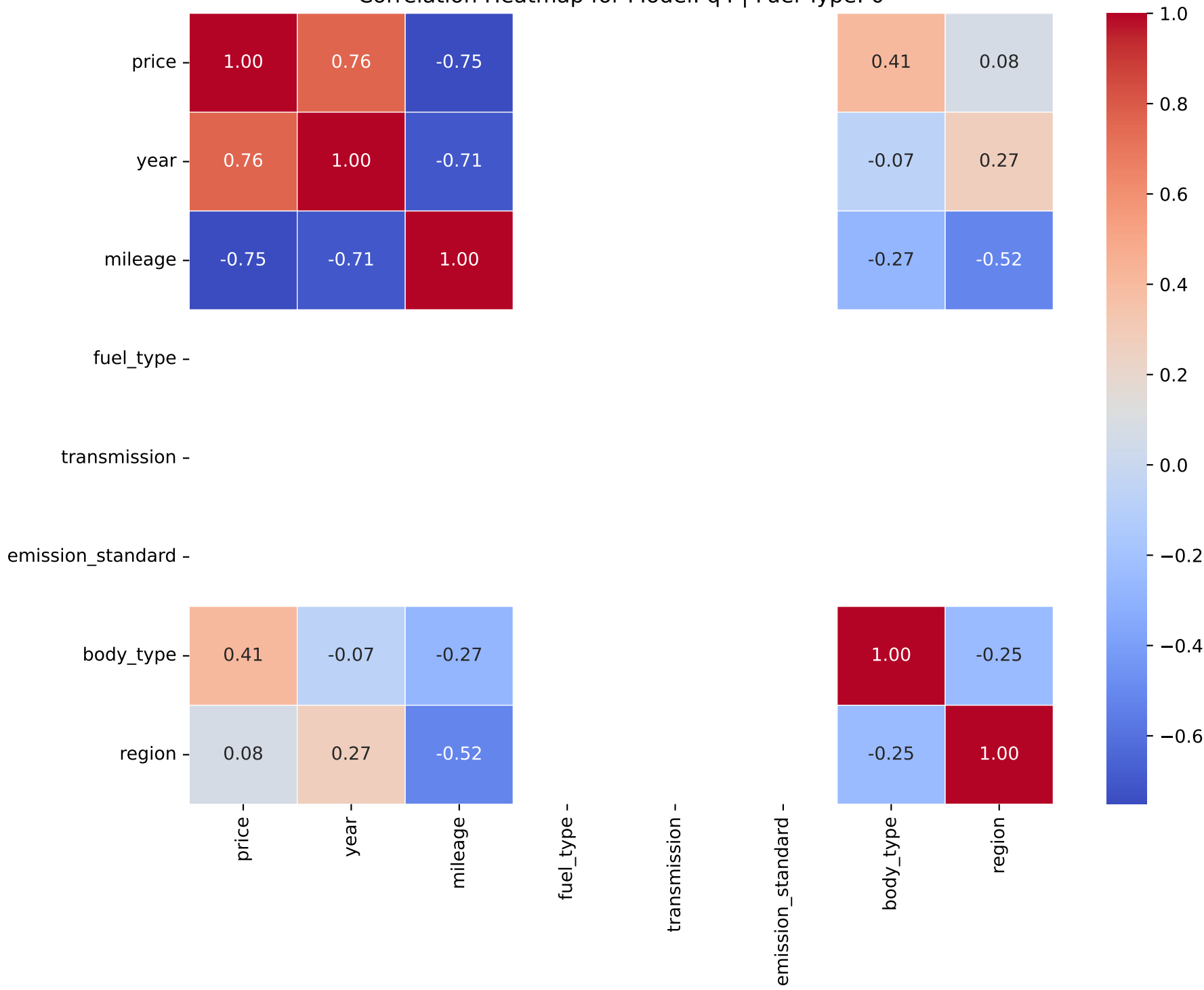
Correlation Heatmap for Model: q4 | Fuel Type: 0
