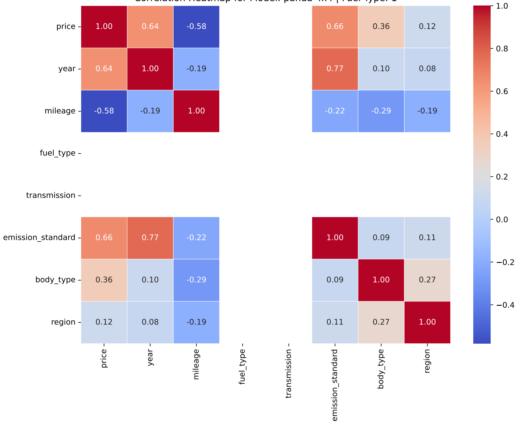
Correlation Heatmap for Model: panda 4x4 | Fuel Type: 1
