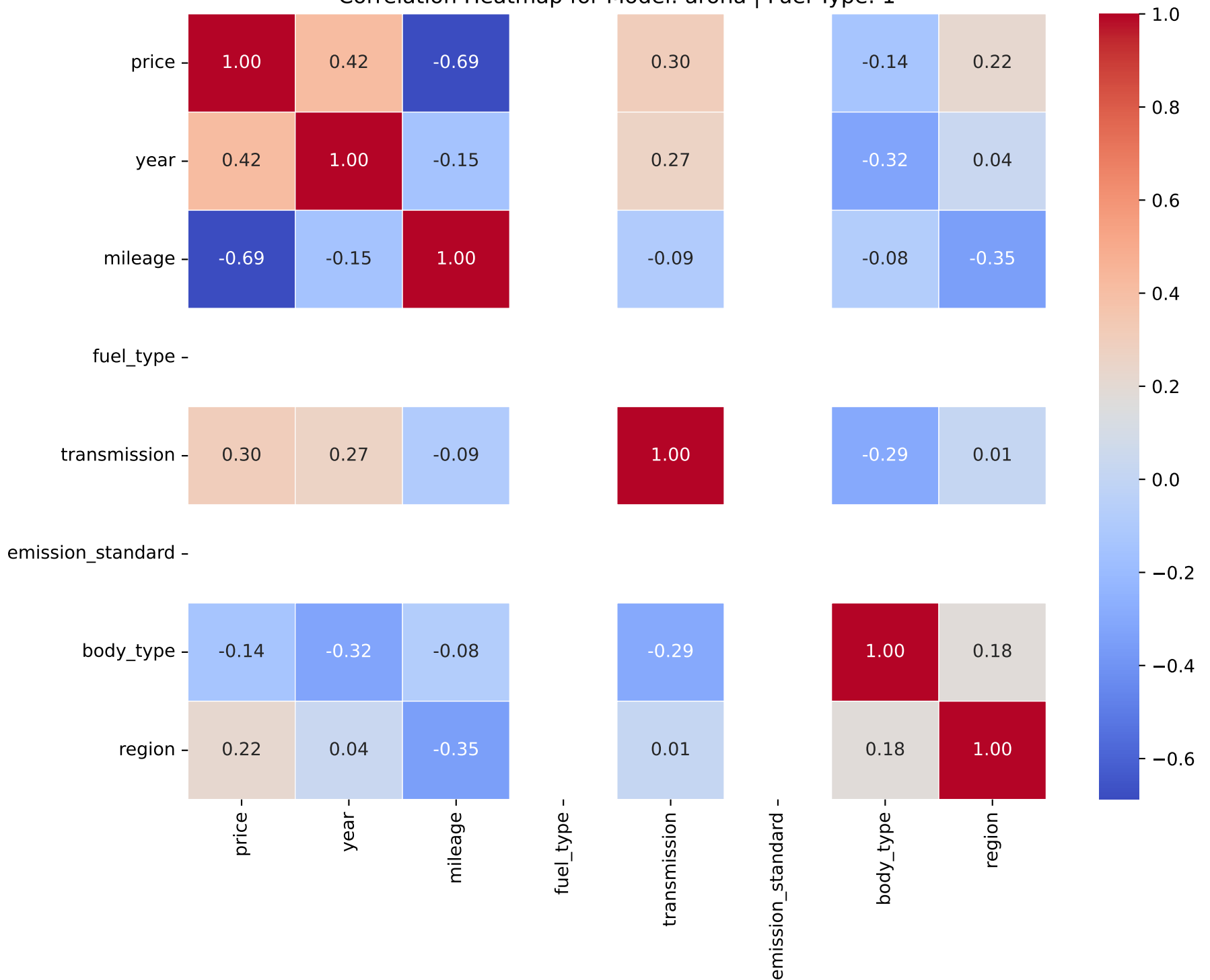
Correlation Heatmap for Model: arona | Fuel Type: 1
