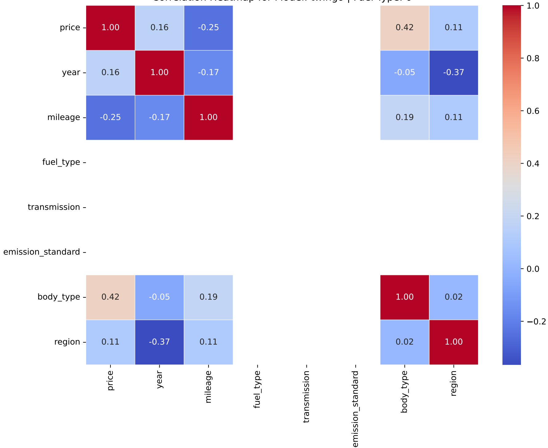
Correlation Heatmap for Model: twingo | Fuel Type: 0
