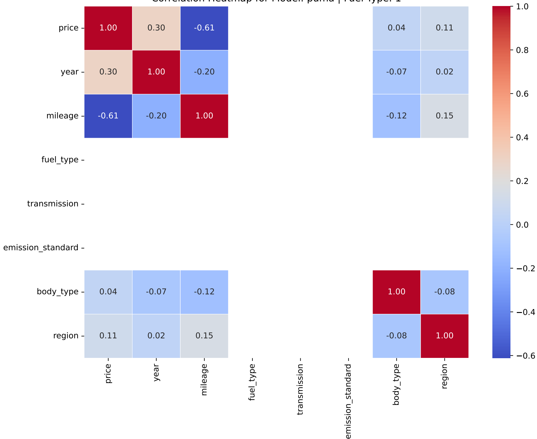
Correlation Heatmap for Model: puma | Fuel Type: 1
