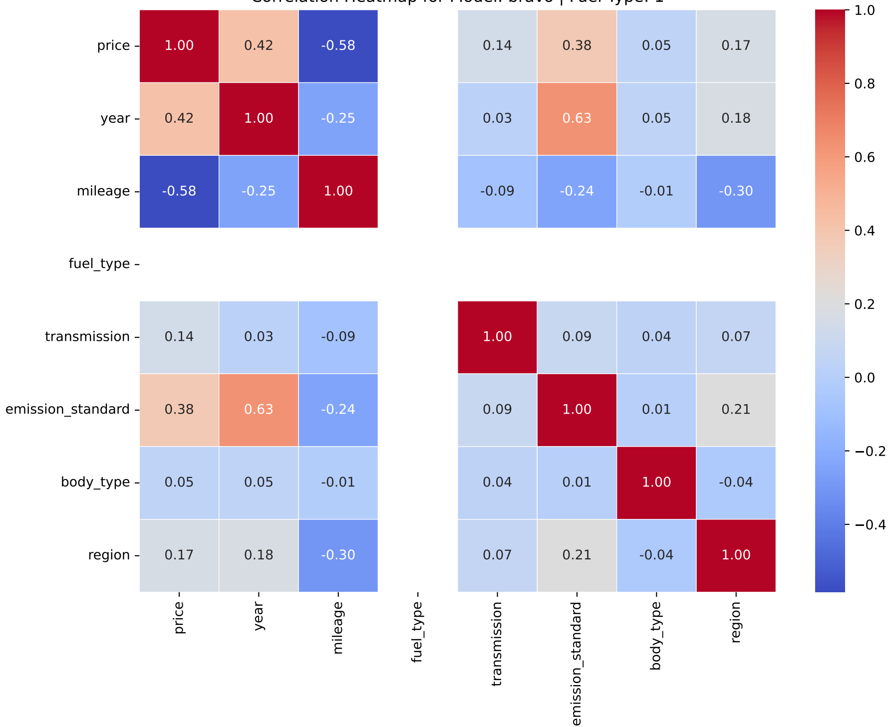
Correlation Heatmap for Model: bravo | Fuel Type: 1
