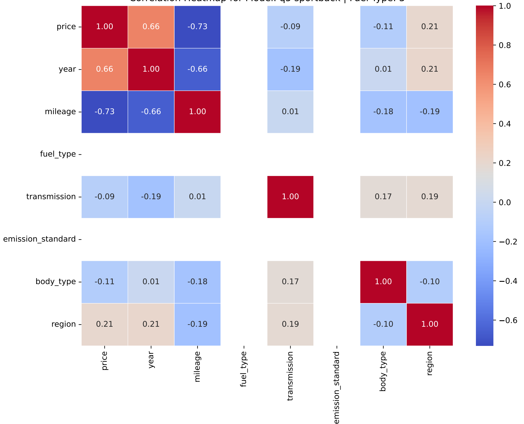
Correlation Heatmap for Model: q5 sportback | Fuel Type: 3
