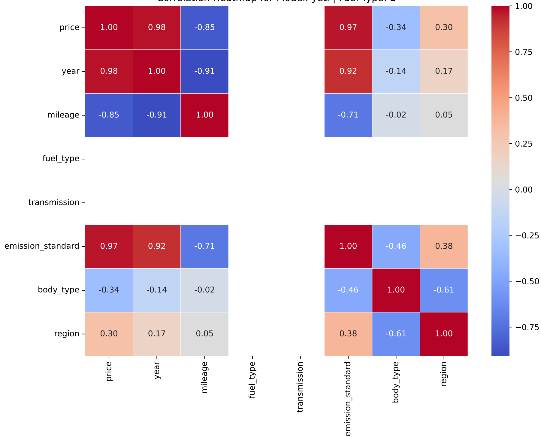
Correlation Heatmap for Model: yeti | Fuel Type: 2
