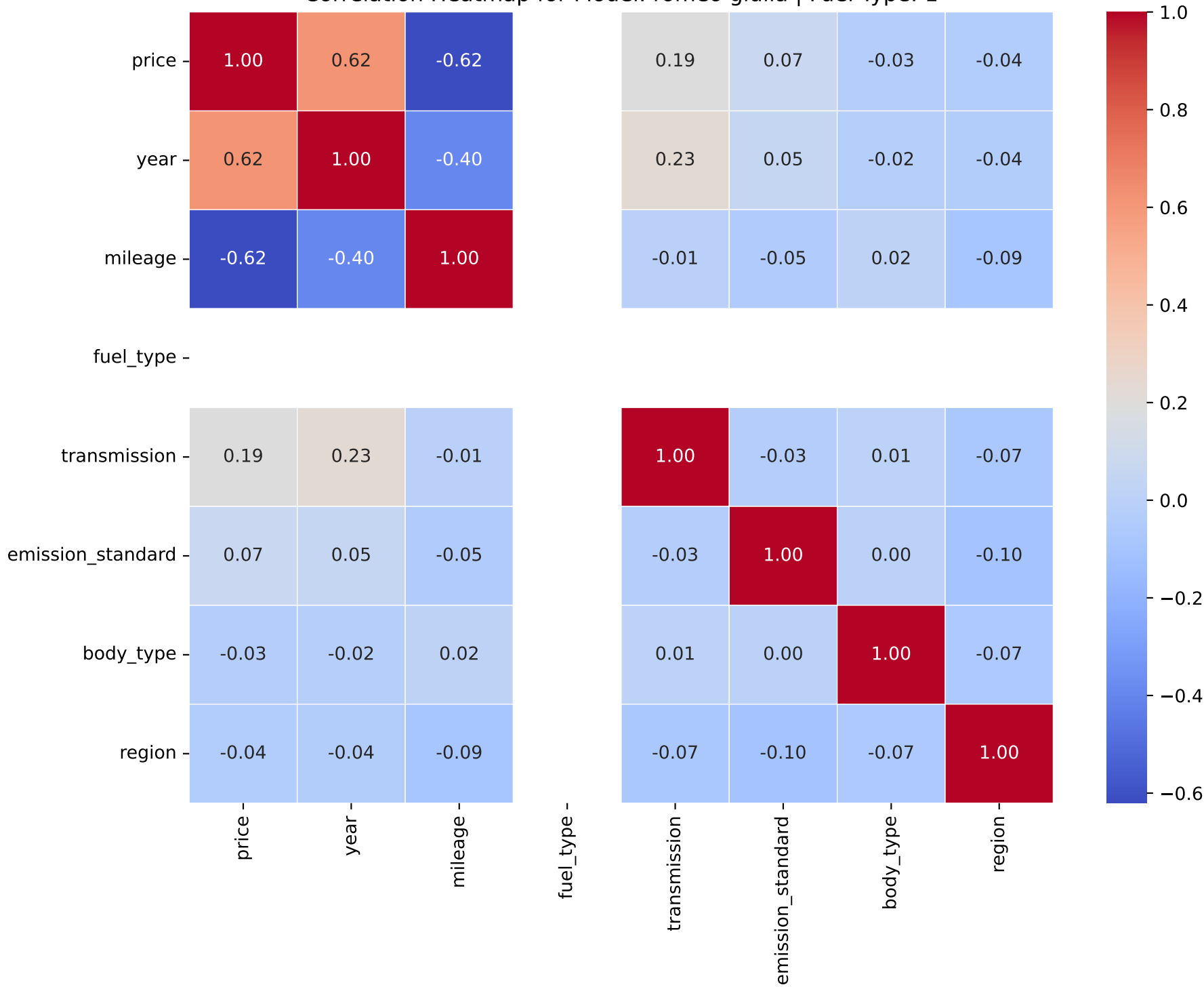
Correlation Heatmap for Model: romeo giulia | Fuel Type: 1
