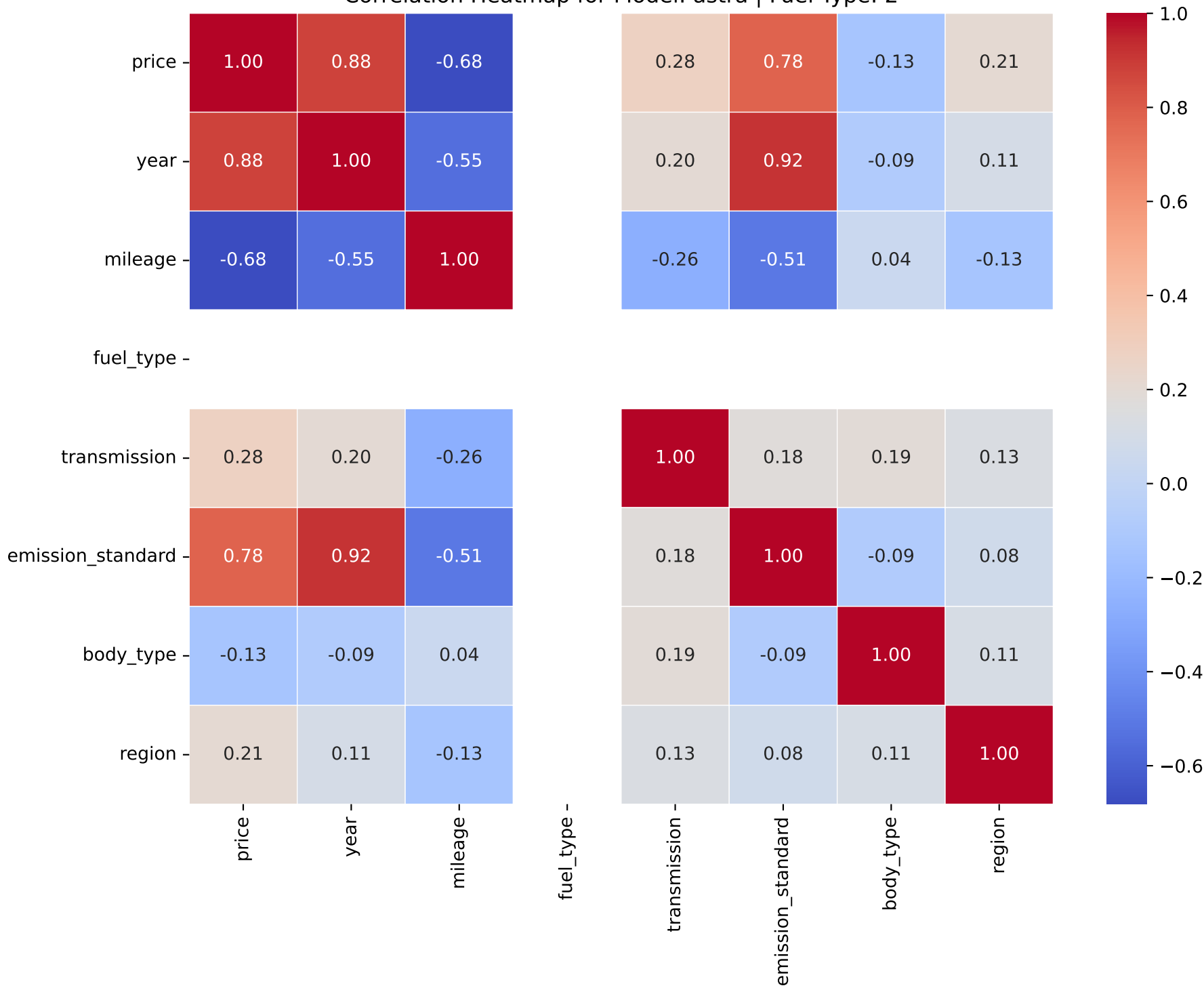
Correlation Heatmap for Model: astra | Fuel Type: 2
