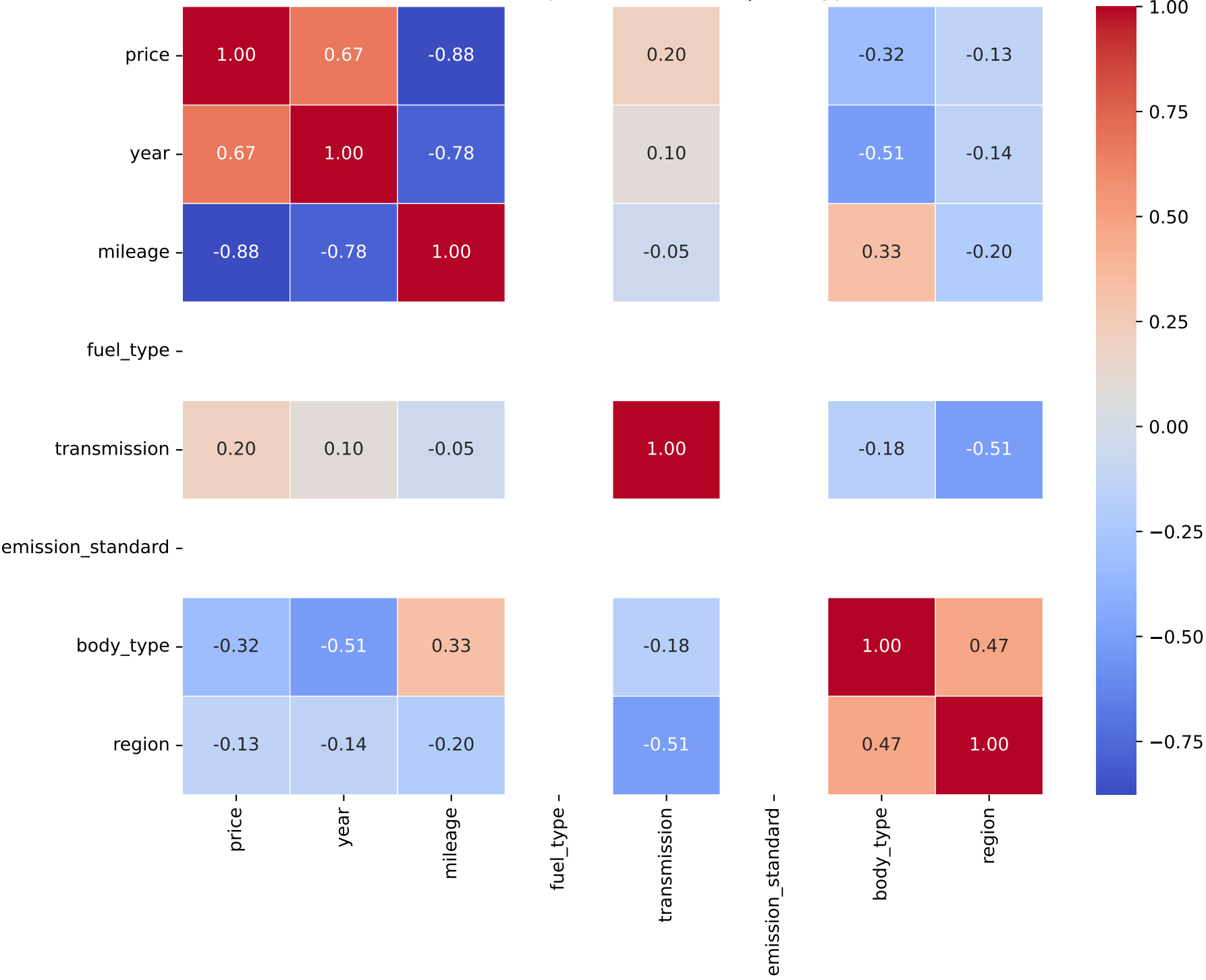
Correlation Heatmap for Model: scala | Fuel Type: 2
