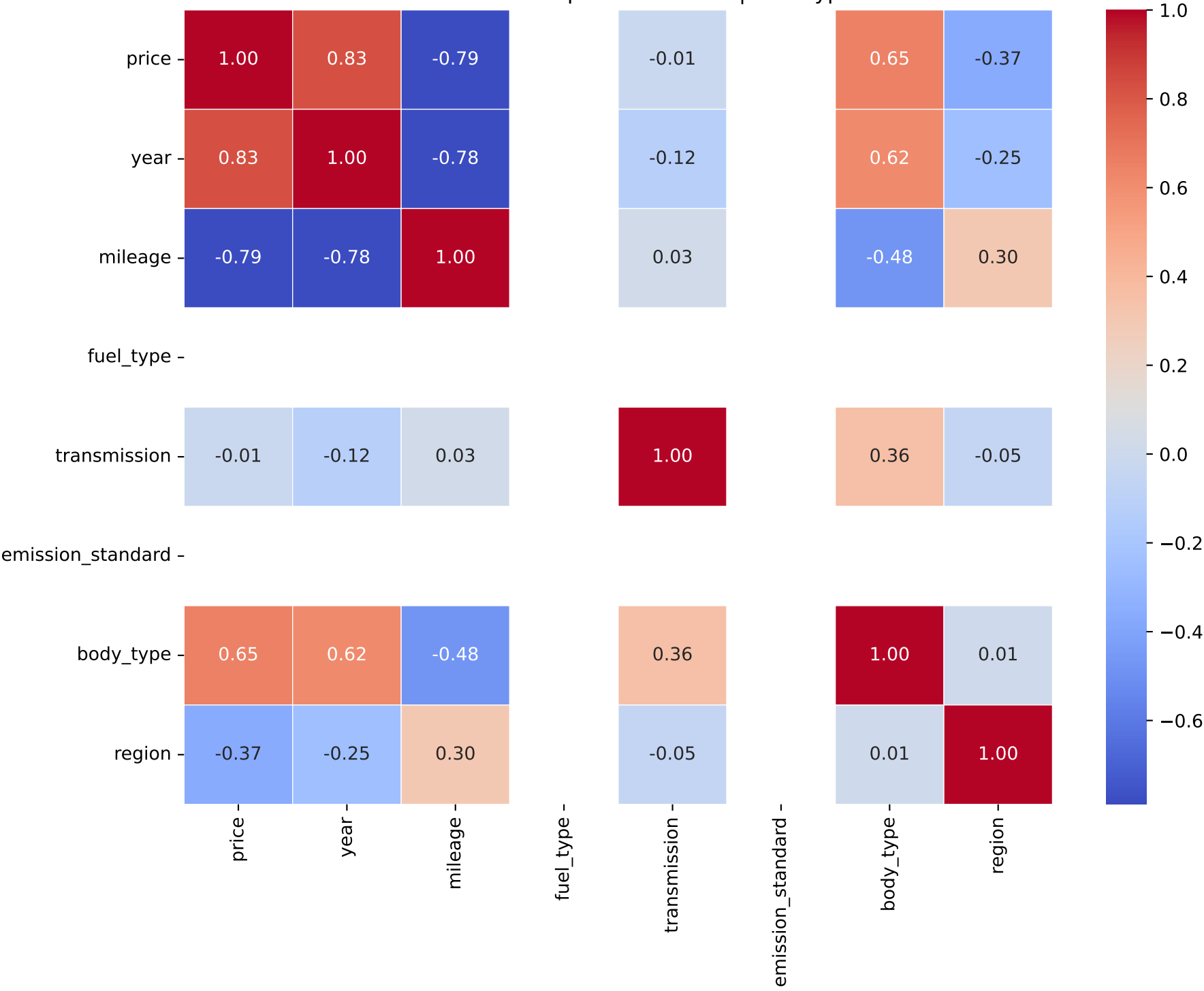
Correlation Heatmap for Model: a5 | Fuel Type: 3
