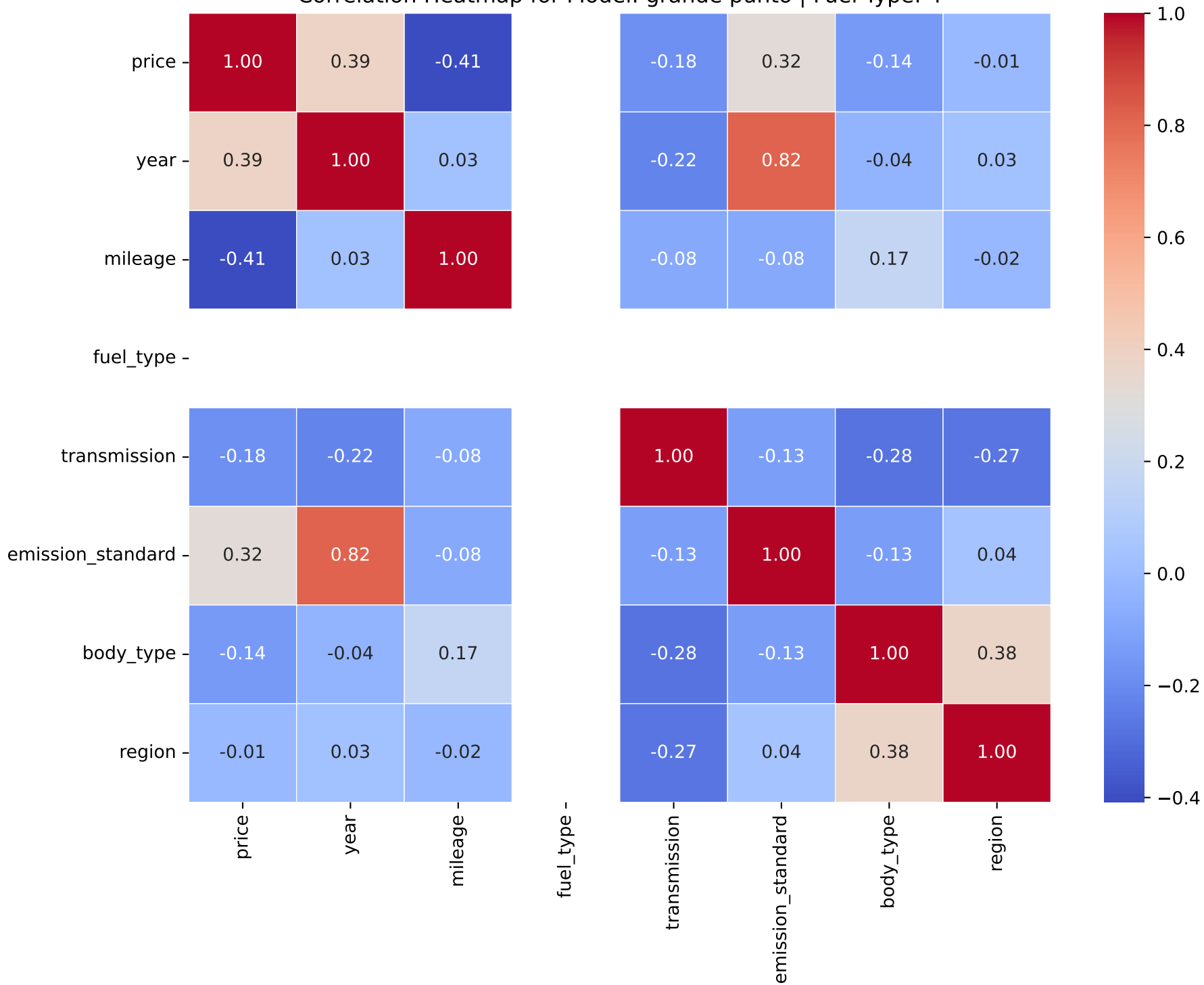
Correlation Heatmap for Model: grande punto | Fuel Type: 4
