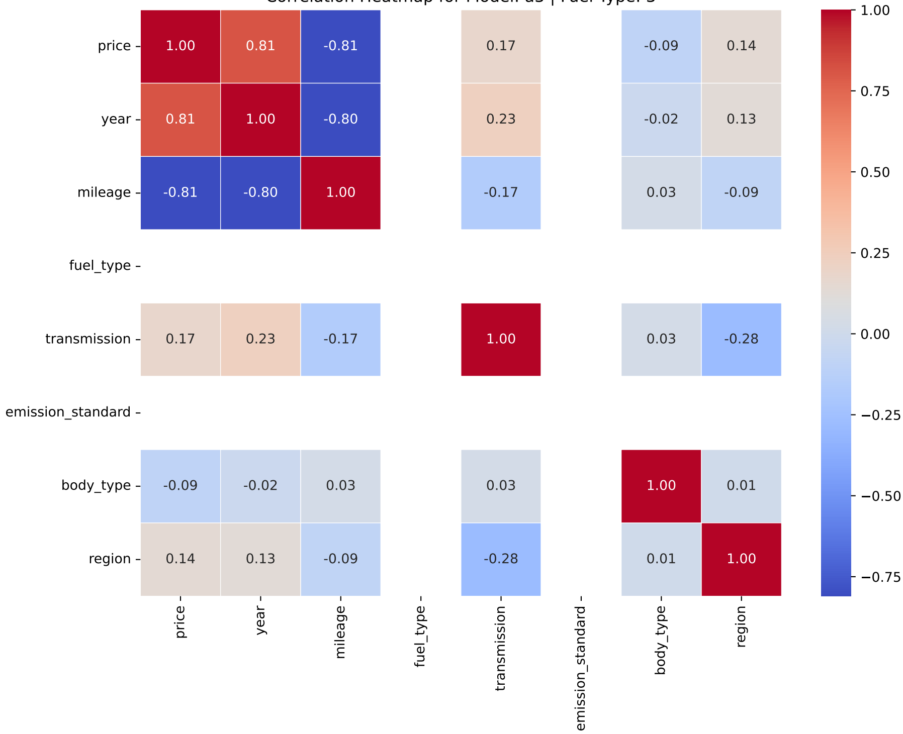
Correlation Heatmap for Model: a3 | Fuel Type: 3
