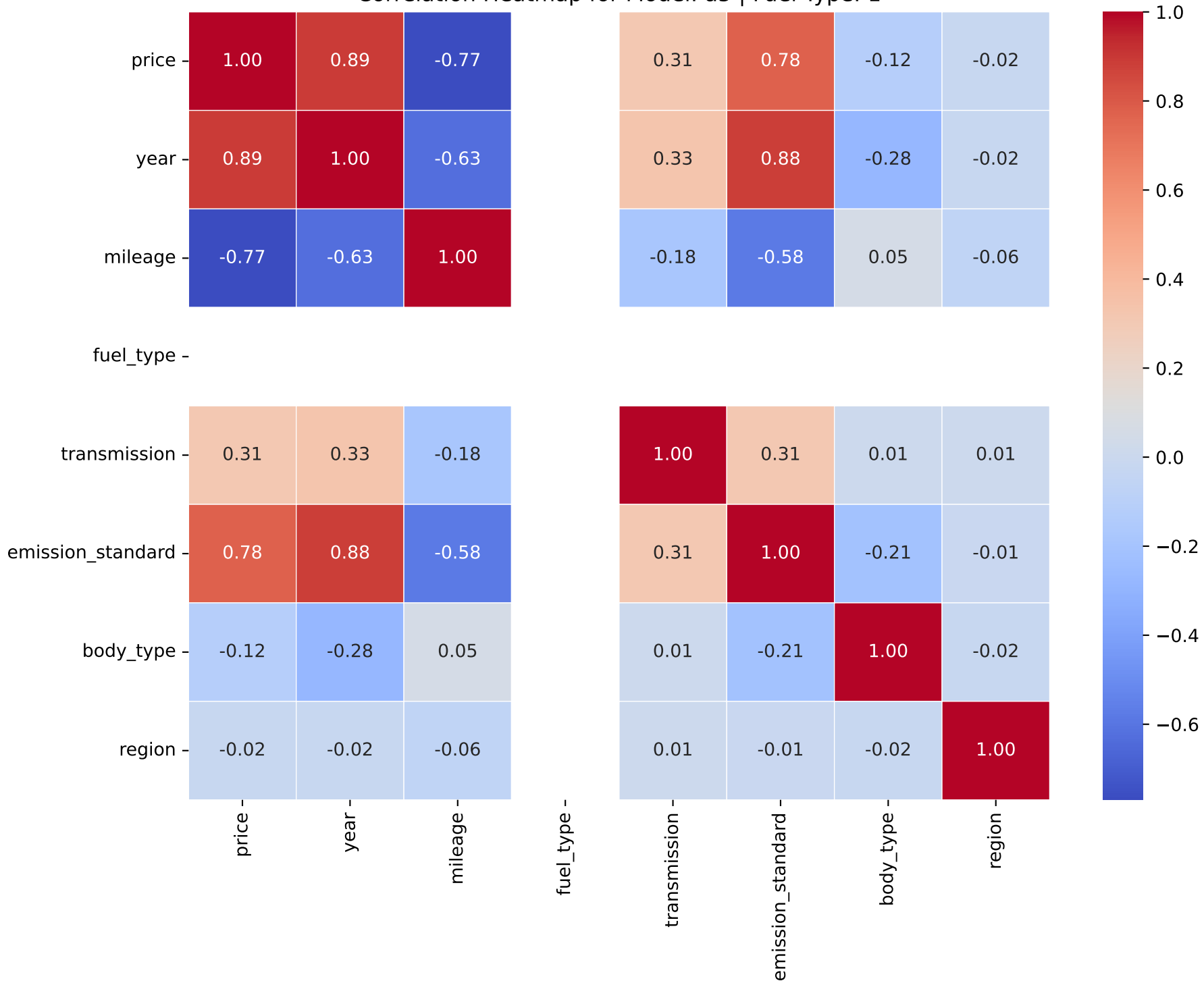
Correlation Heatmap for Model: a5 | Fuel Type: 1
