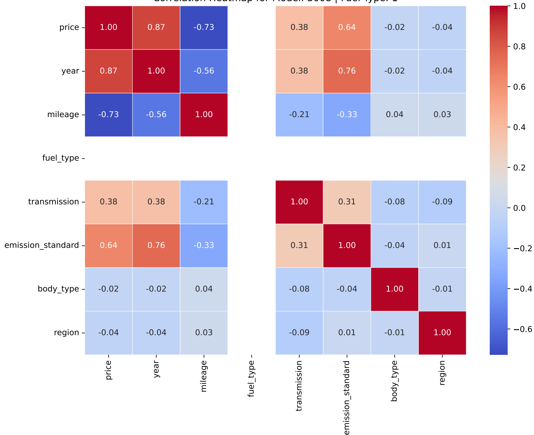
Correlation Heatmap for Model: 3008 | Fuel Type: 1
