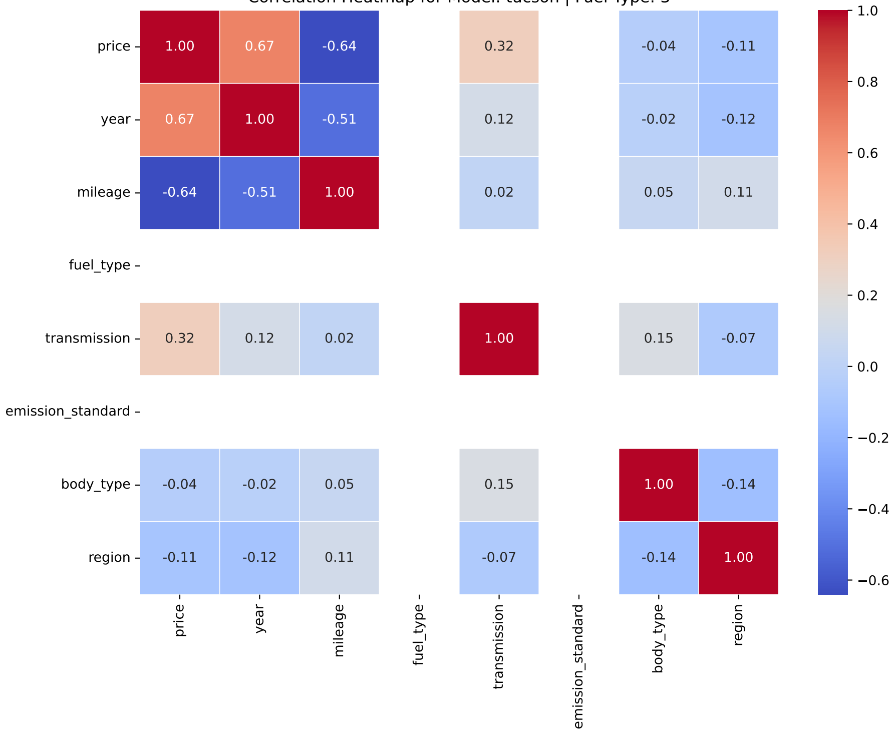
Correlation Heatmap for Model: tucson | Fuel Type: 3
