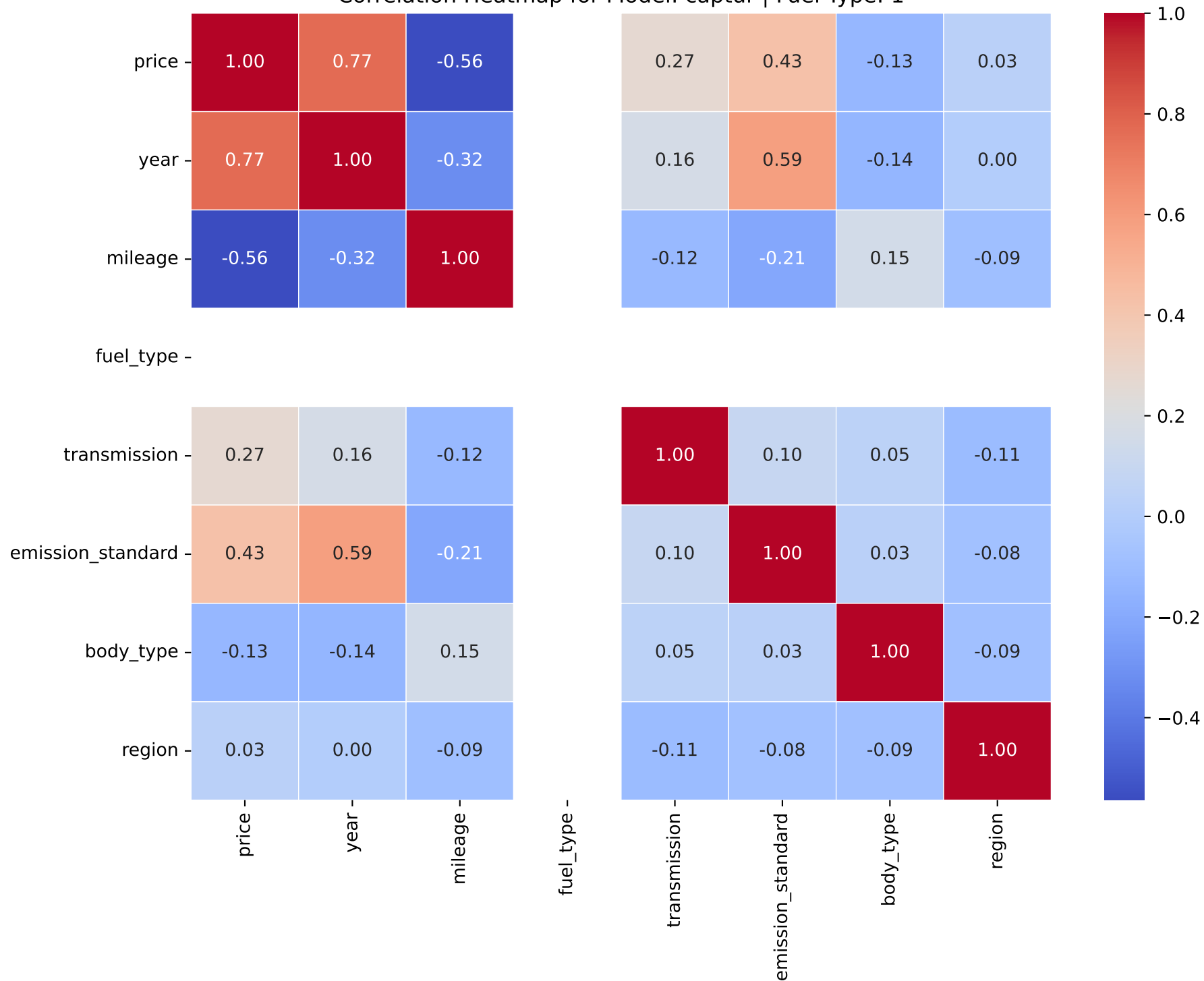
Correlation Heatmap for Model: captur | Fuel Type: 1
