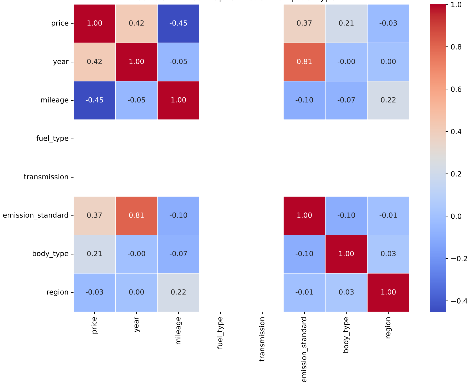
Correlation Heatmap for Model: 207 | Fuel Type: 1
