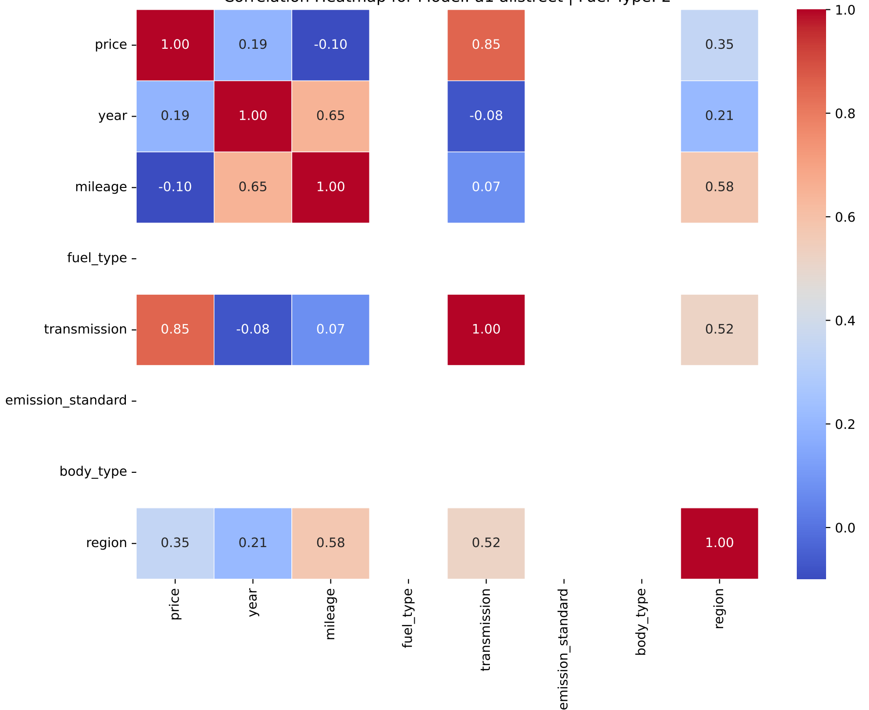
Correlation Heatmap for Model: a1 allstreet | Fuel Type: 2
