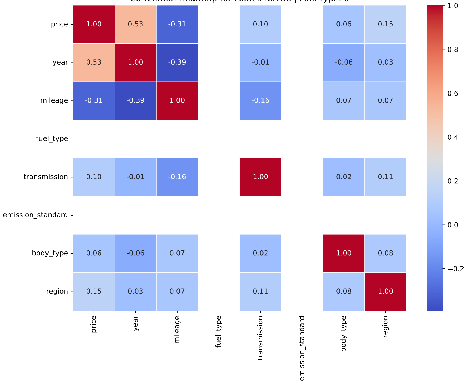
Correlation Heatmap for Model: fortwo | Fuel Type: 0
