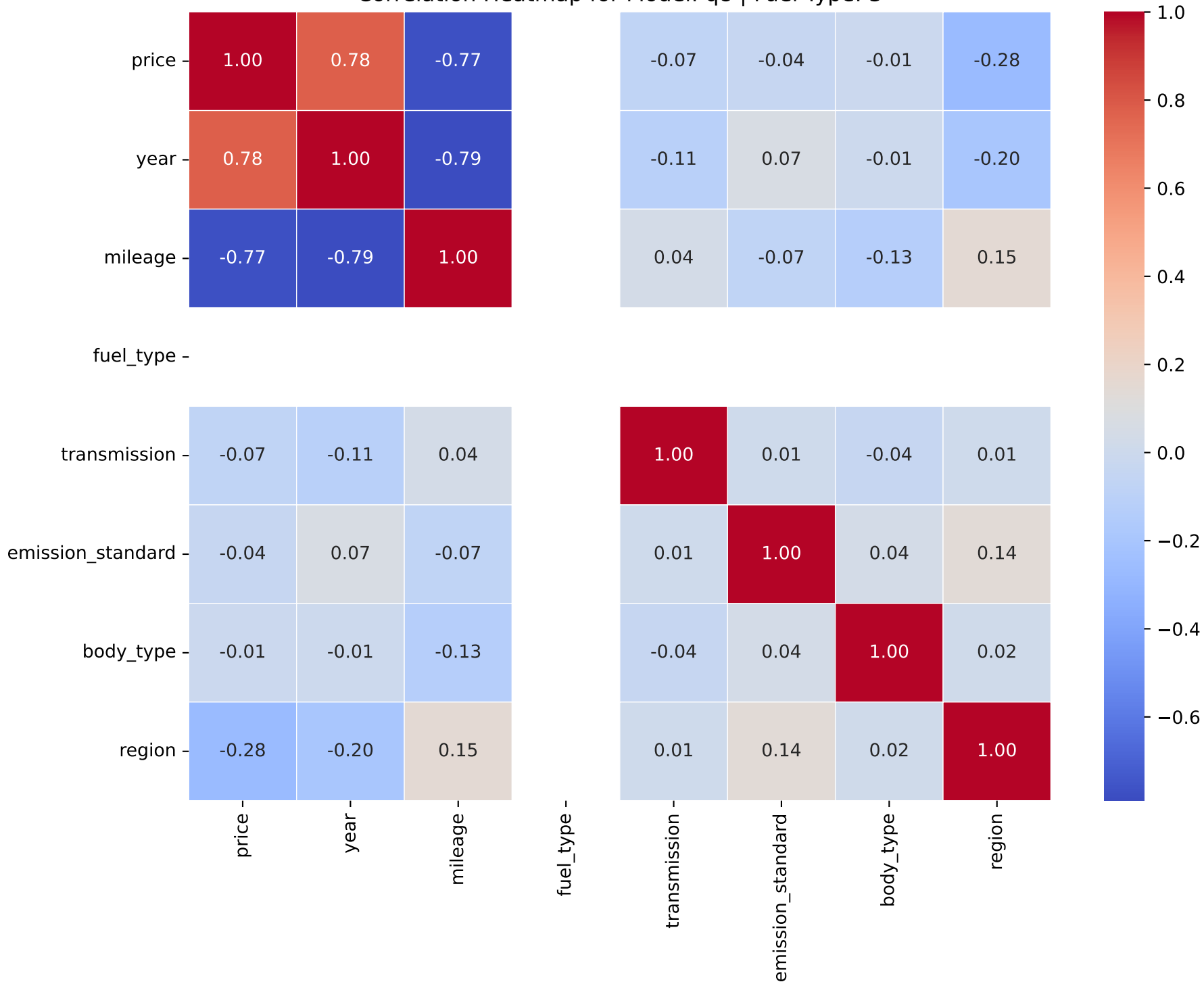
Correlation Heatmap for Model: q8 | Fuel Type: 3
