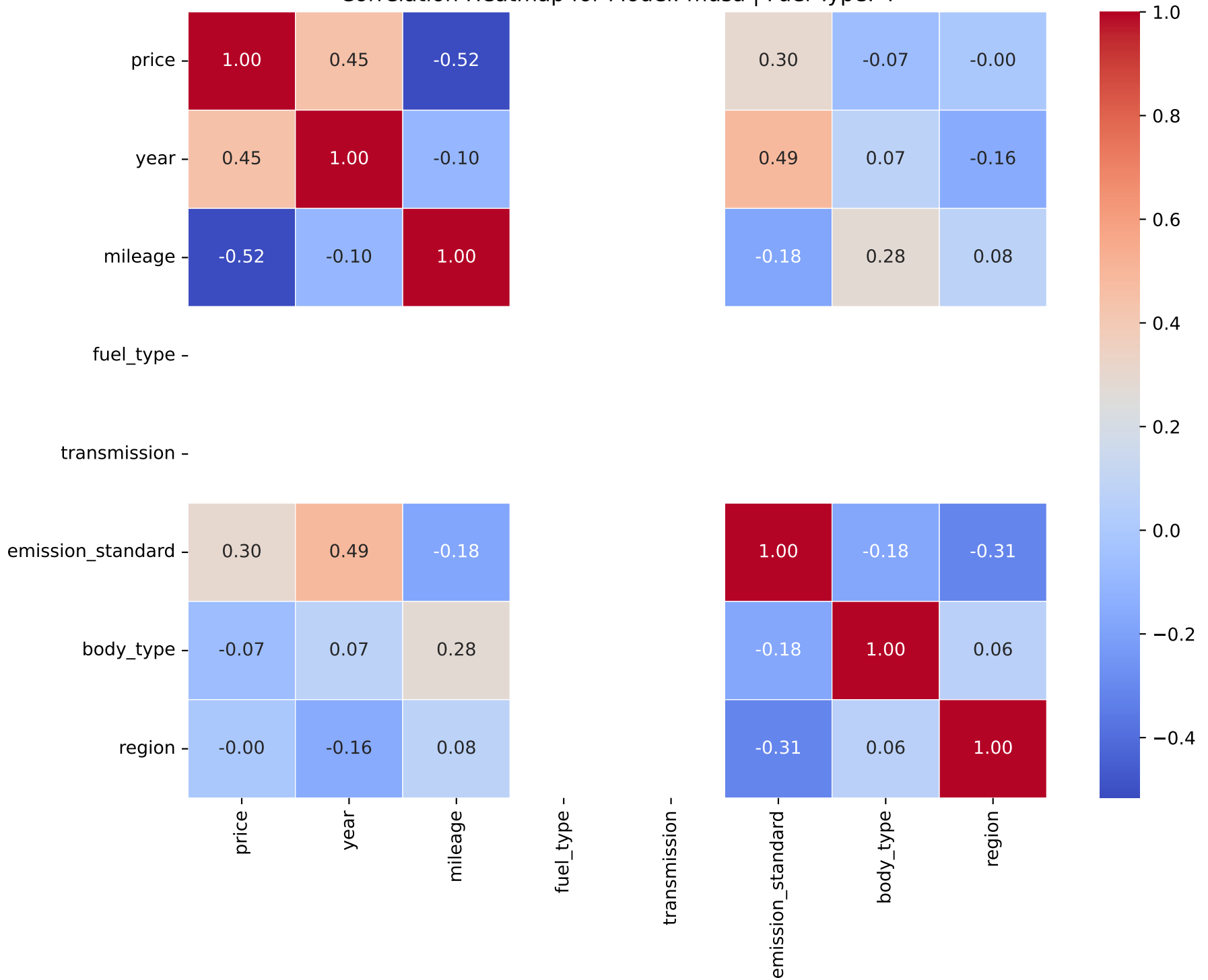
Correlation Heatmap for Model: musa | Fuel Type: 4
