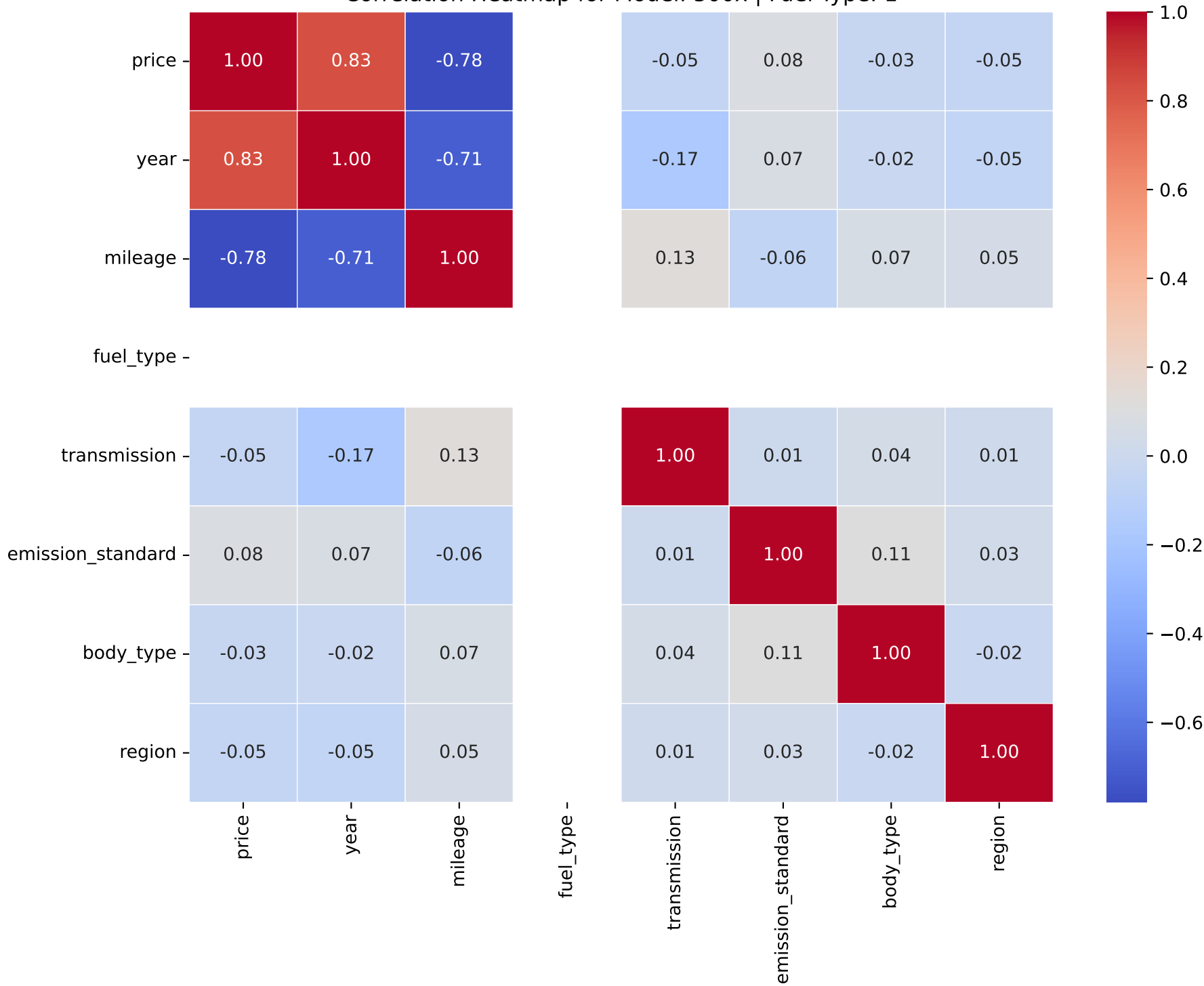
Correlation Heatmap for Model: 500x | Fuel Type: 1
