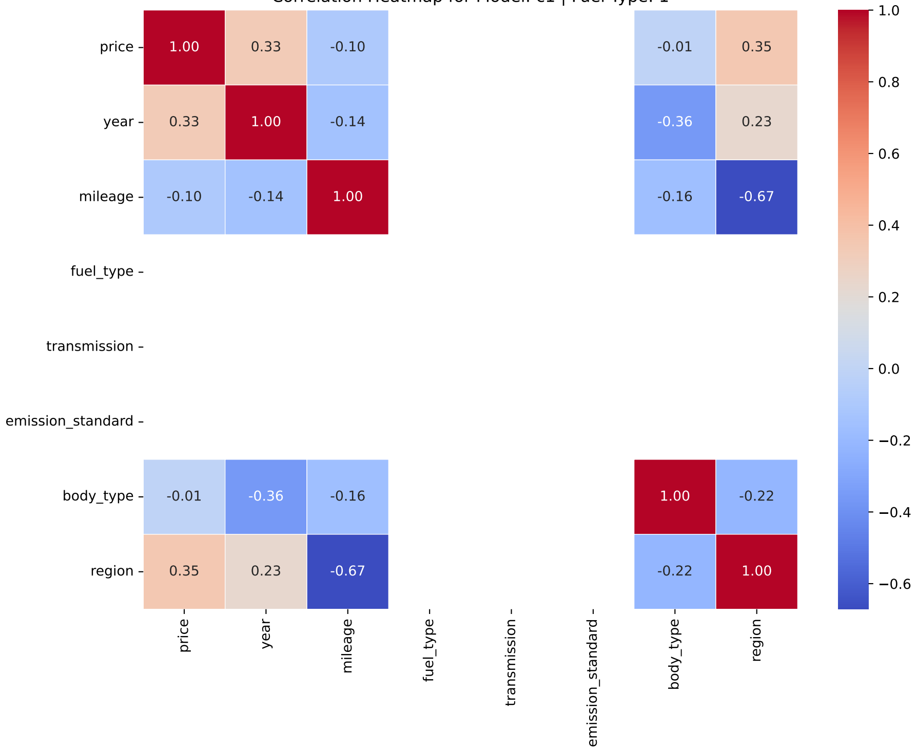
Correlation Heatmap for Model: c1 | Fuel Type: 1
