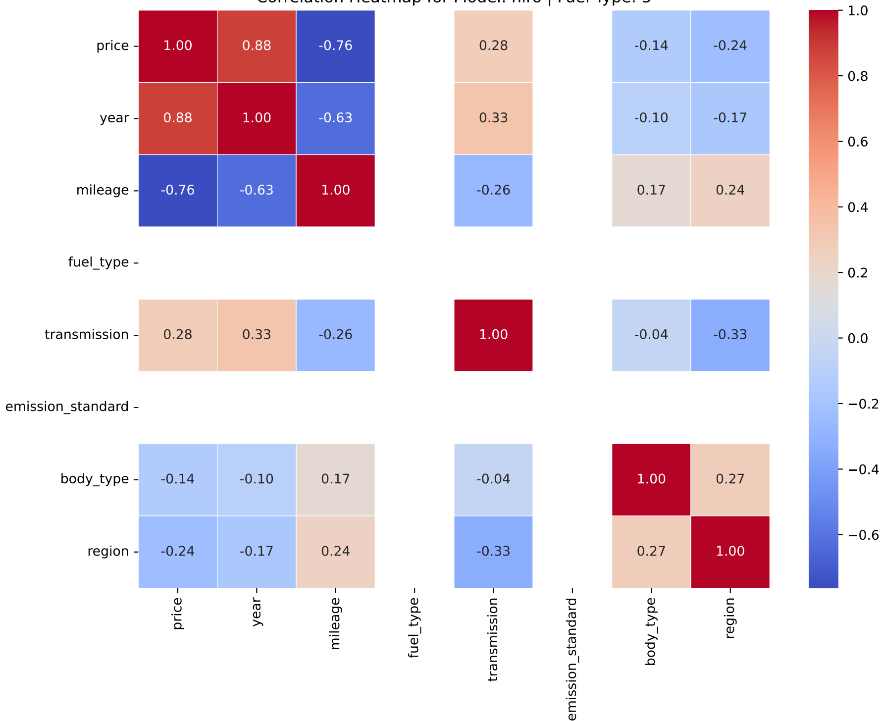
Correlation Heatmap for Model: niro | Fuel Type: 3
