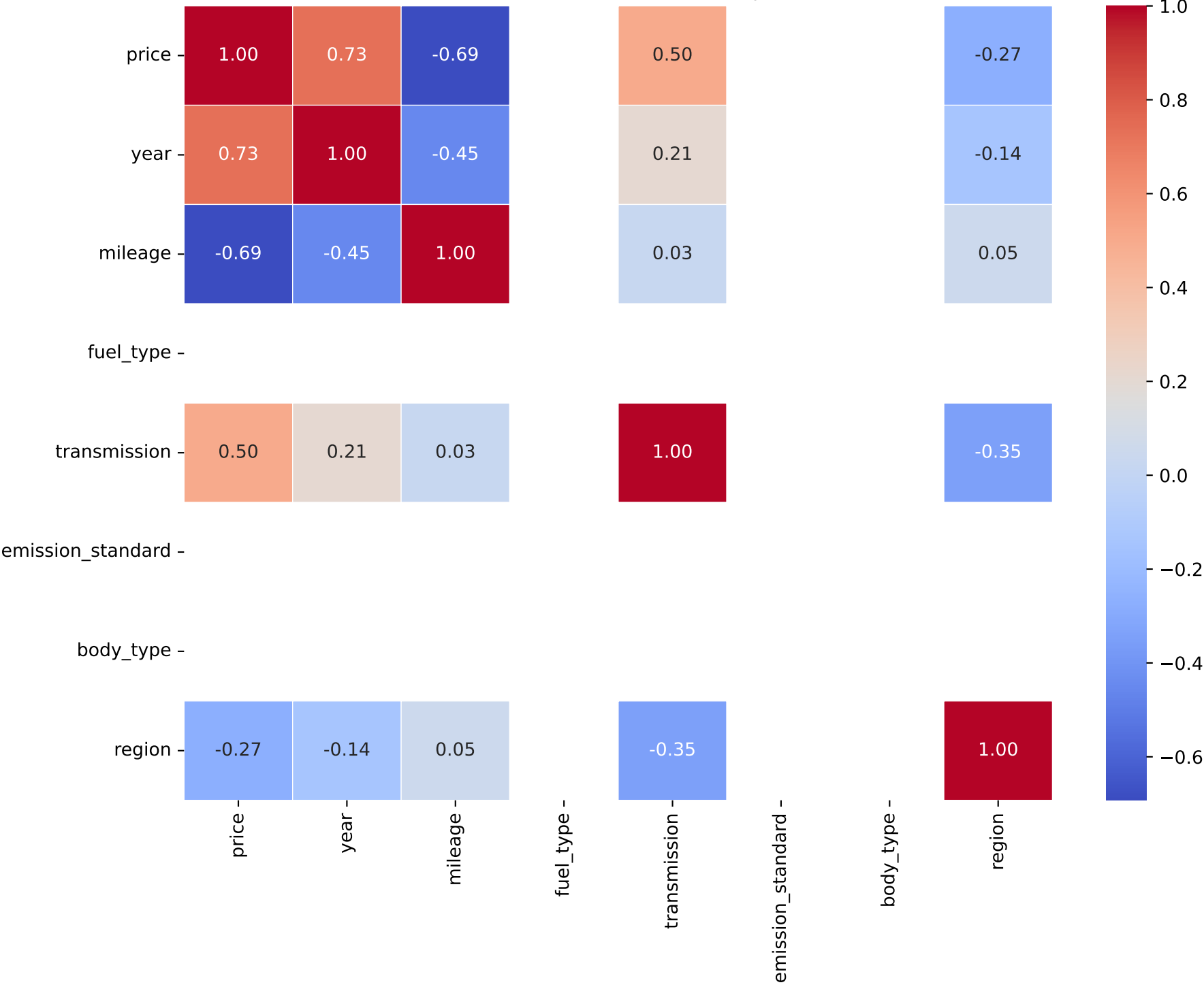
Correlation Heatmap for Model: ioniq | Fuel Type: 3
