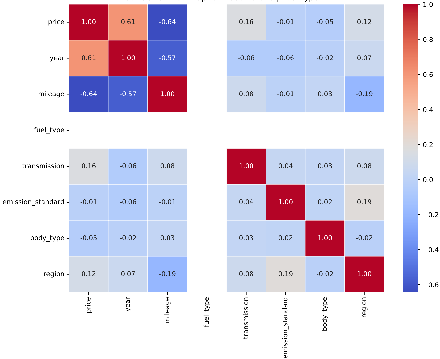
Correlation Heatmap for Model: arona | Fuel Type: 2
