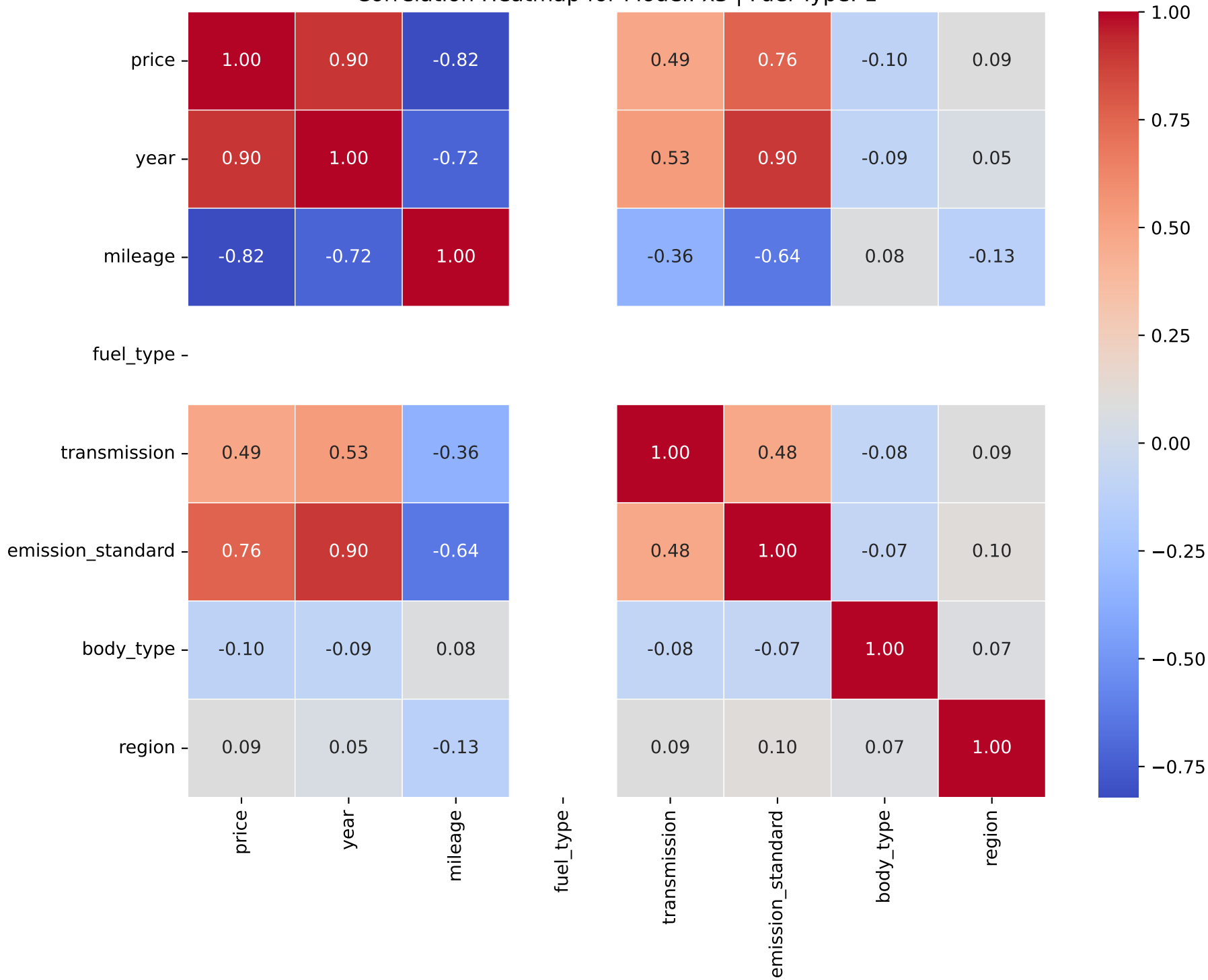
Correlation Heatmap for Model: x3 | Fuel Type: 1
