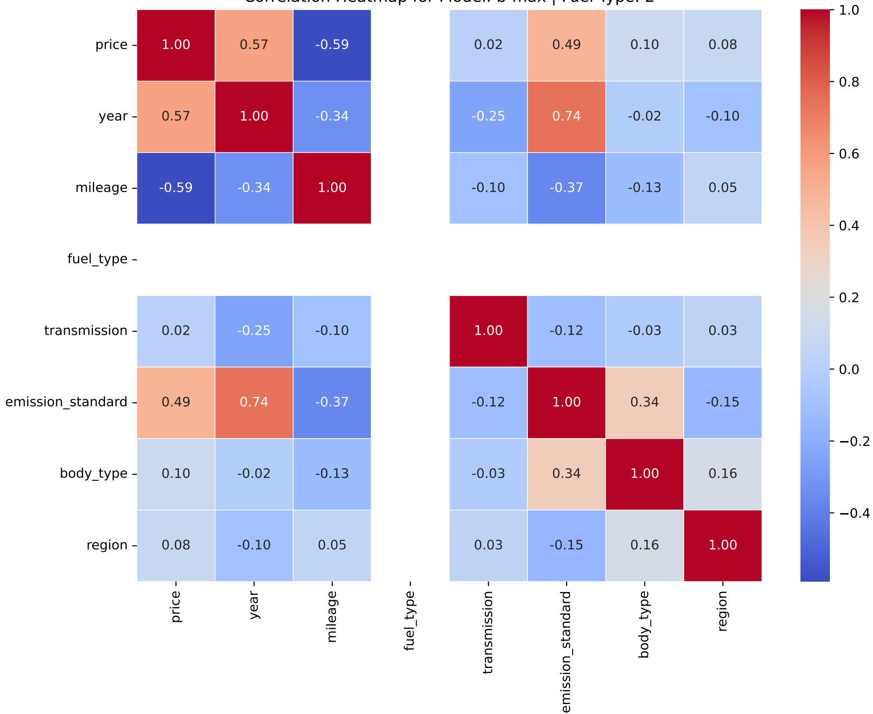
Correlation Heatmap for Model: b-max | Fuel Type: 2
