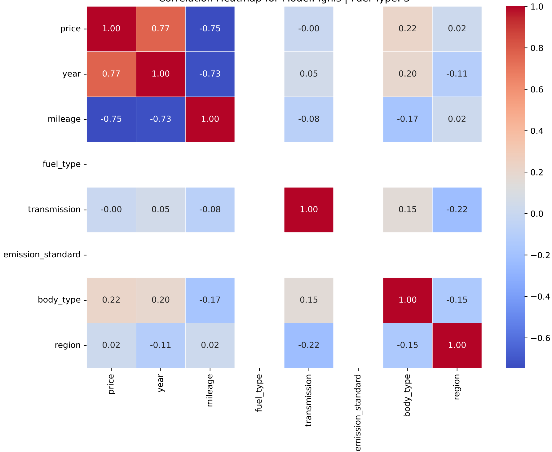
Correlation Heatmap for Model: ignis | Fuel Type: 3
