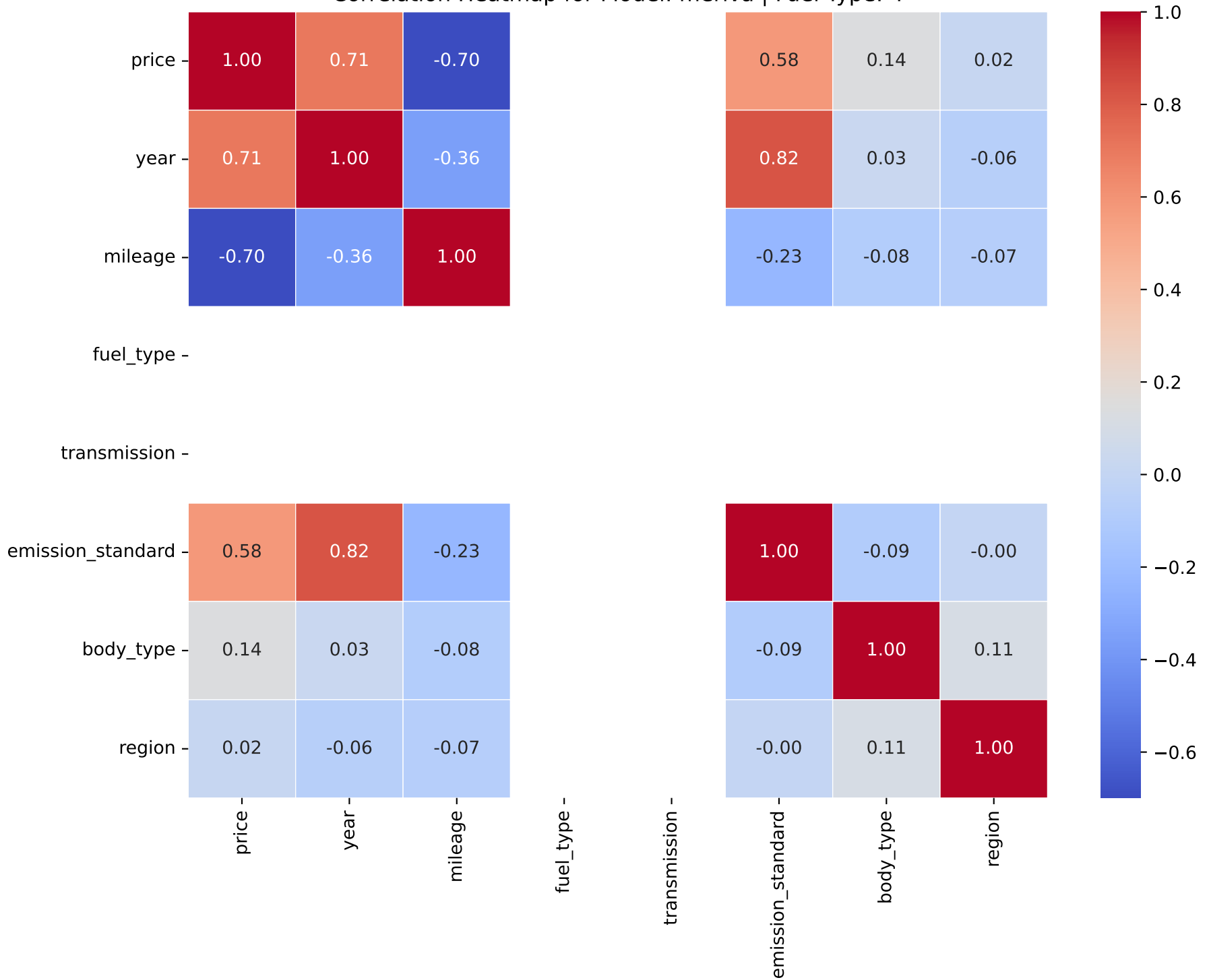
Correlation Heatmap for Model: meriva | Fuel Type: 4
