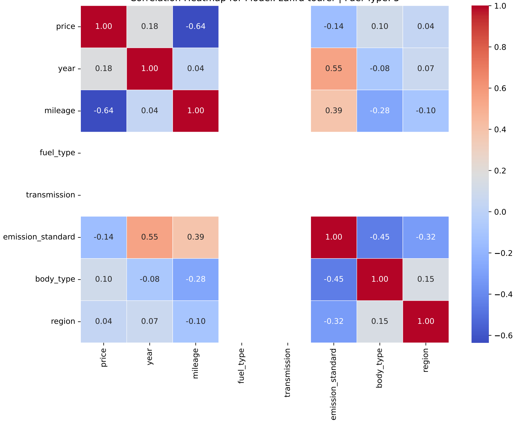
Correlation Heatmap for Model: zafira tourer | Fuel Type: 5
