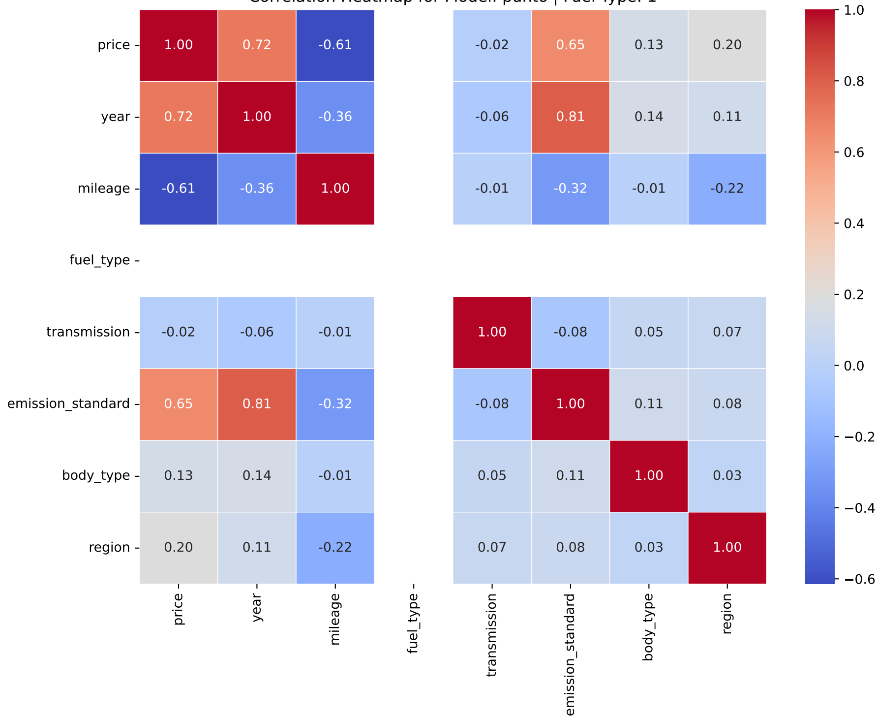
Correlation Heatmap for Model: punto | Fuel Type: 1
