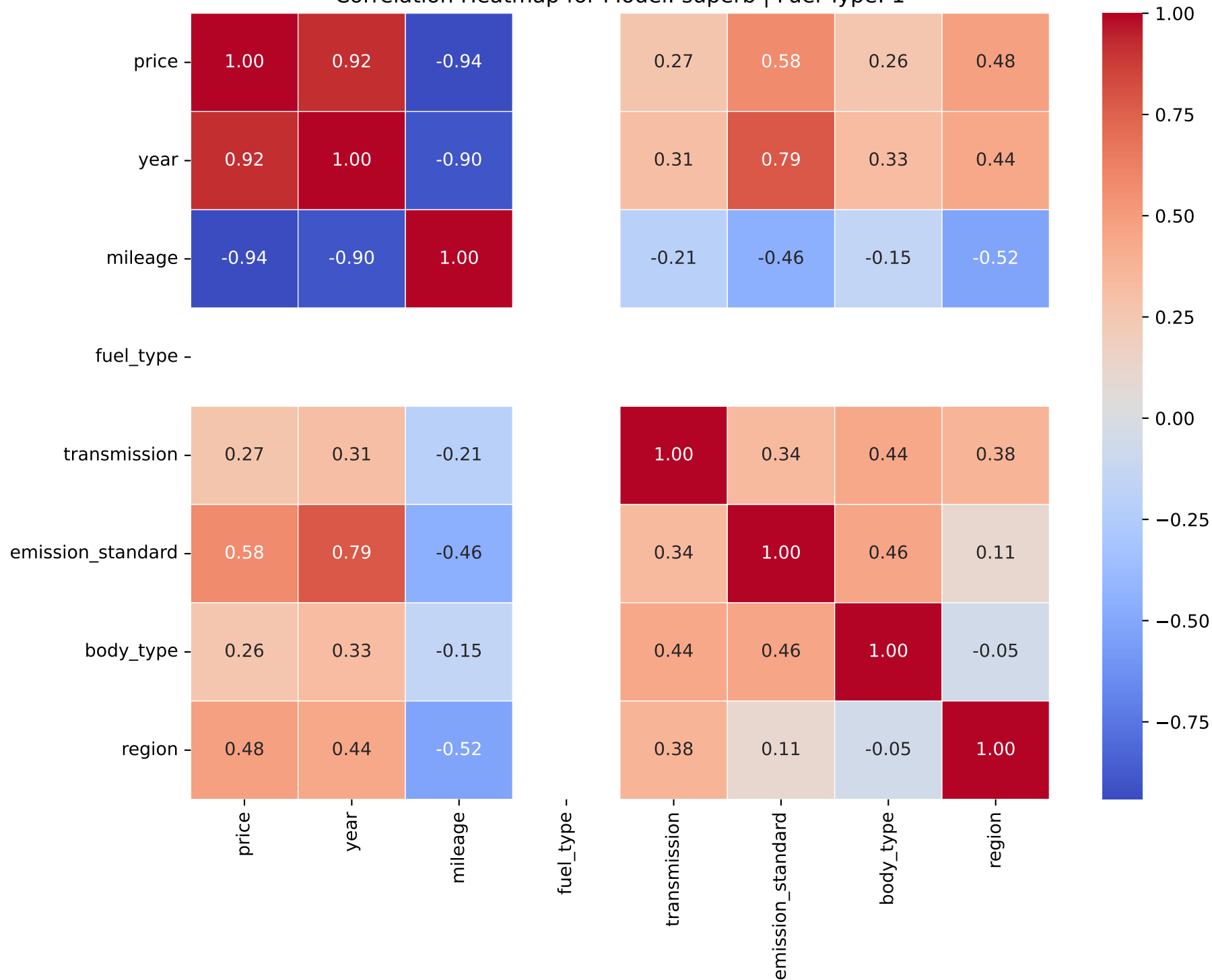
Correlation Heatmap for Model: superb | Fuel Type: 1
