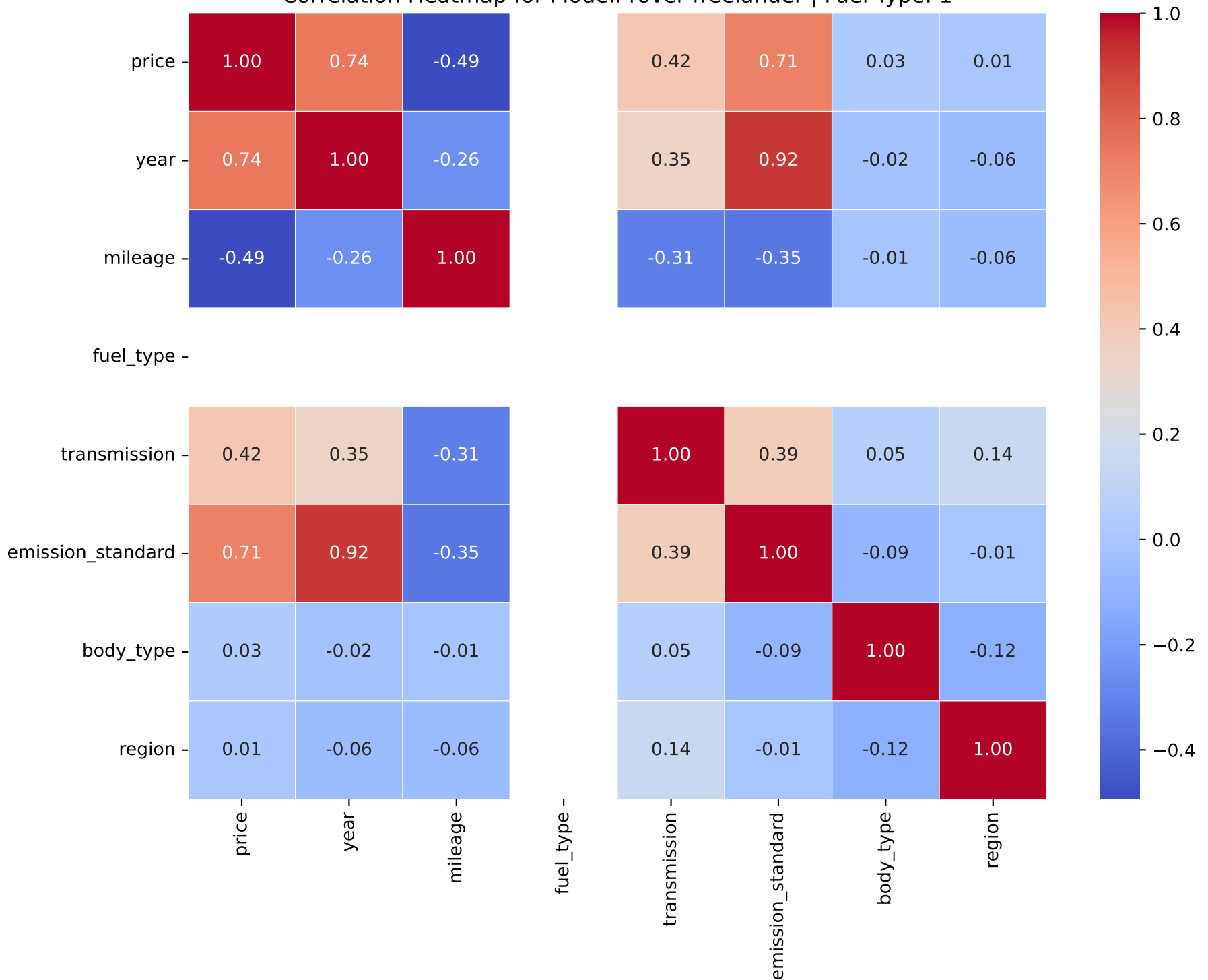
Correlation Heatmap for Model: rover freelander | Fuel Type: 1
