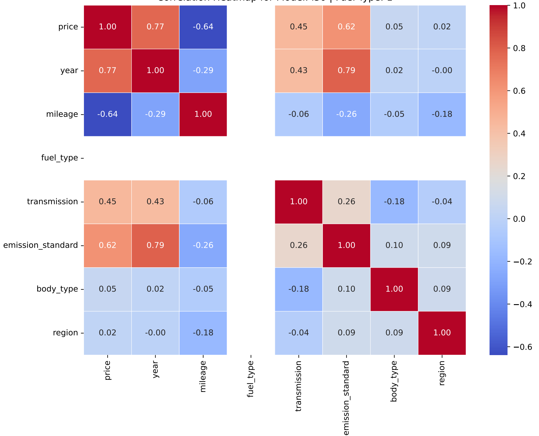
Correlation Heatmap for Model: i30 | Fuel Type: 1
