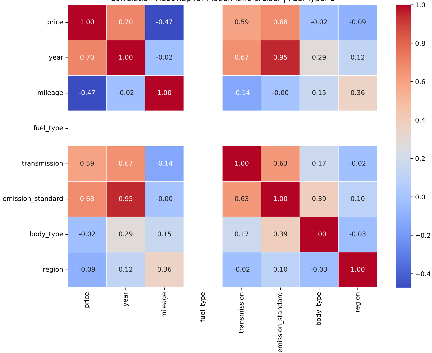
Correlation Heatmap for Model: land cruiser | Fuel Type: 1
