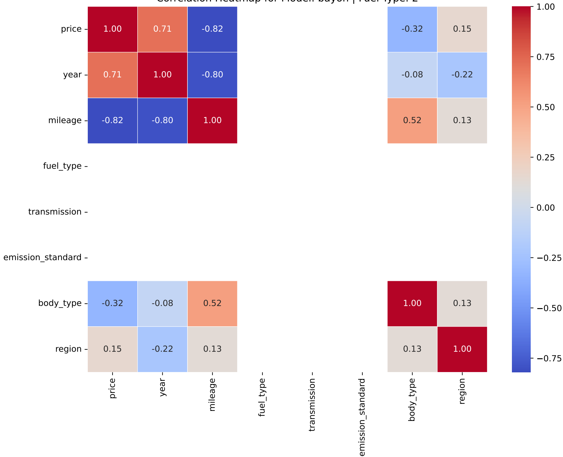
Correlation Heatmap for Model: bayon | Fuel Type: 2
