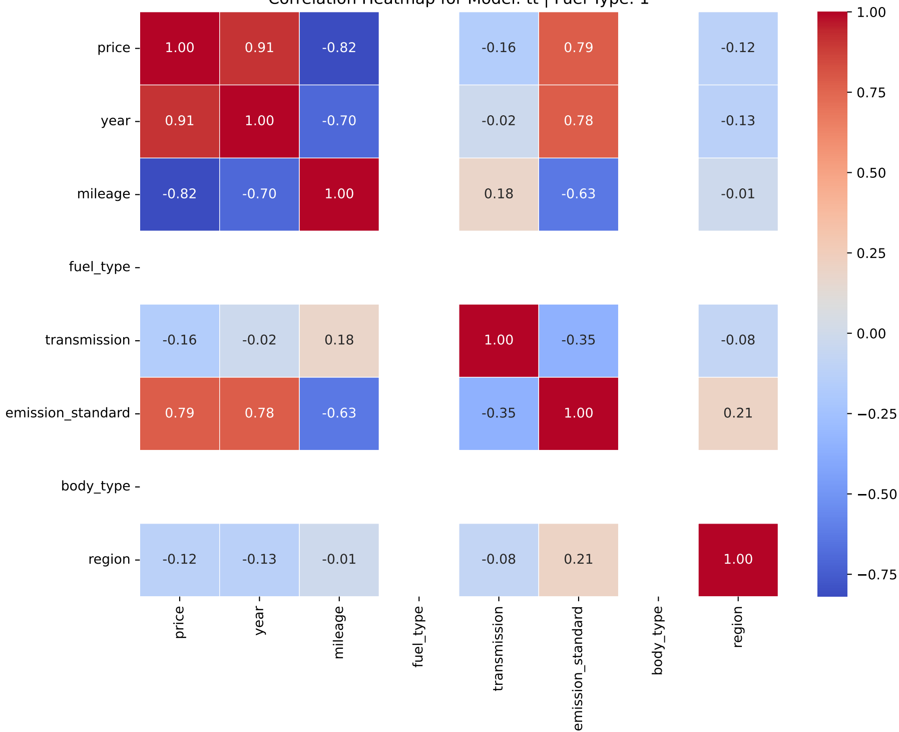
Correlation Heatmap for Model: tt | Fuel Type: 1
