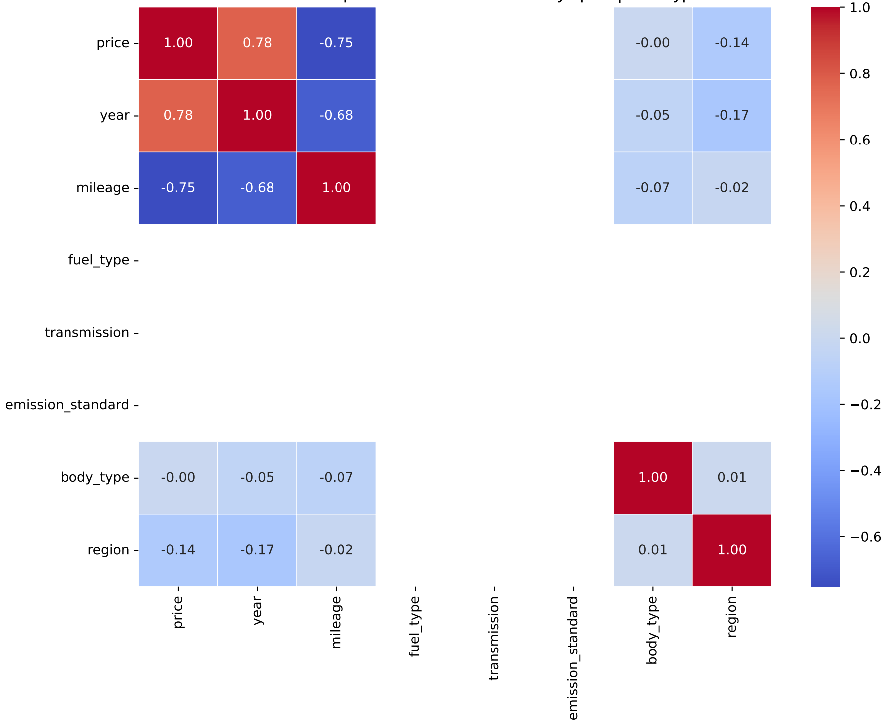
Correlation Heatmap for Model: rover discovery sport | Fuel Type: 3
