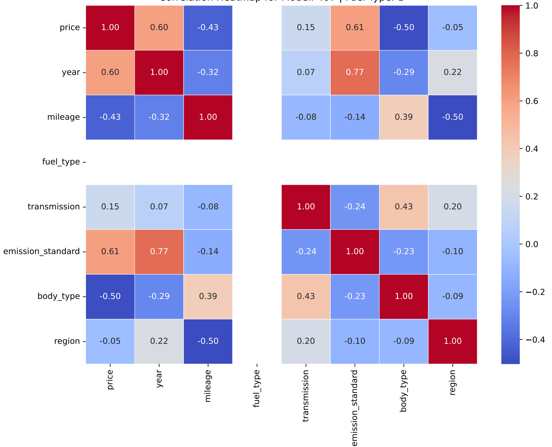
Correlation Heatmap for Model: 407 | Fuel Type: 1
