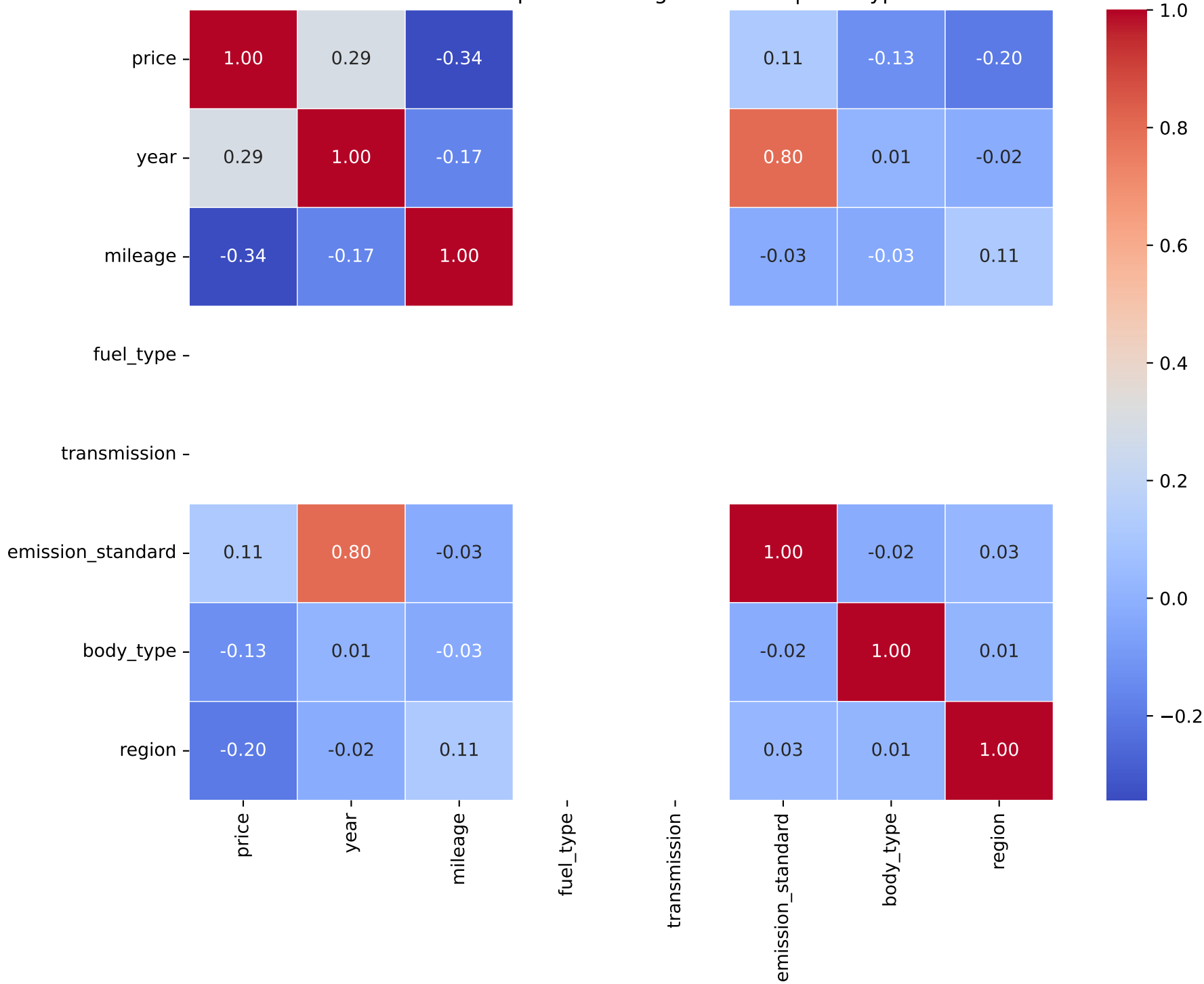
Correlation Heatmap for Model: grand vitara | Fuel Type: 1
