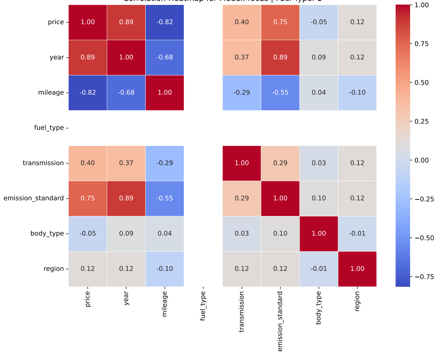
Correlation Heatmap for Model: focus | Fuel Type: 1
