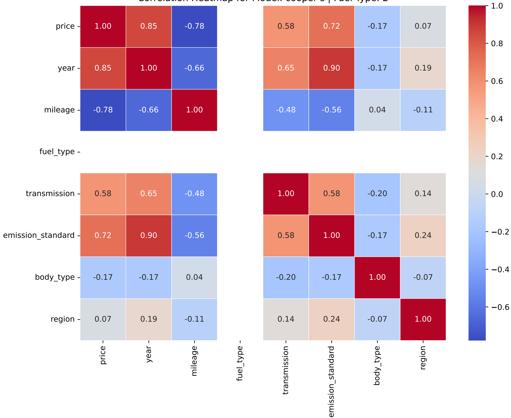
Correlation Heatmap for Model: cooper s | Fuel Type: 2
