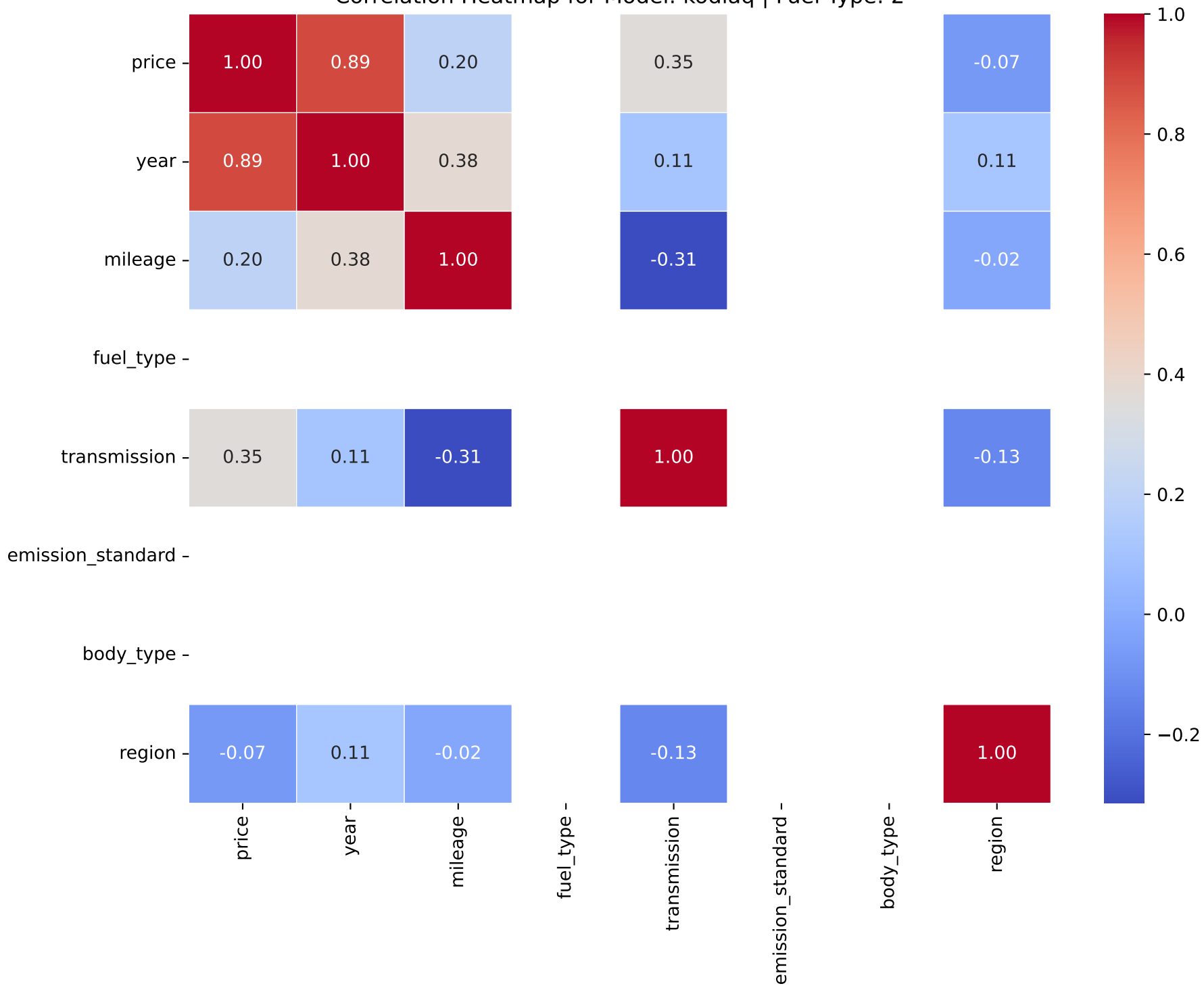
Correlation Heatmap for Model: kodiaq | Fuel Type: 2
