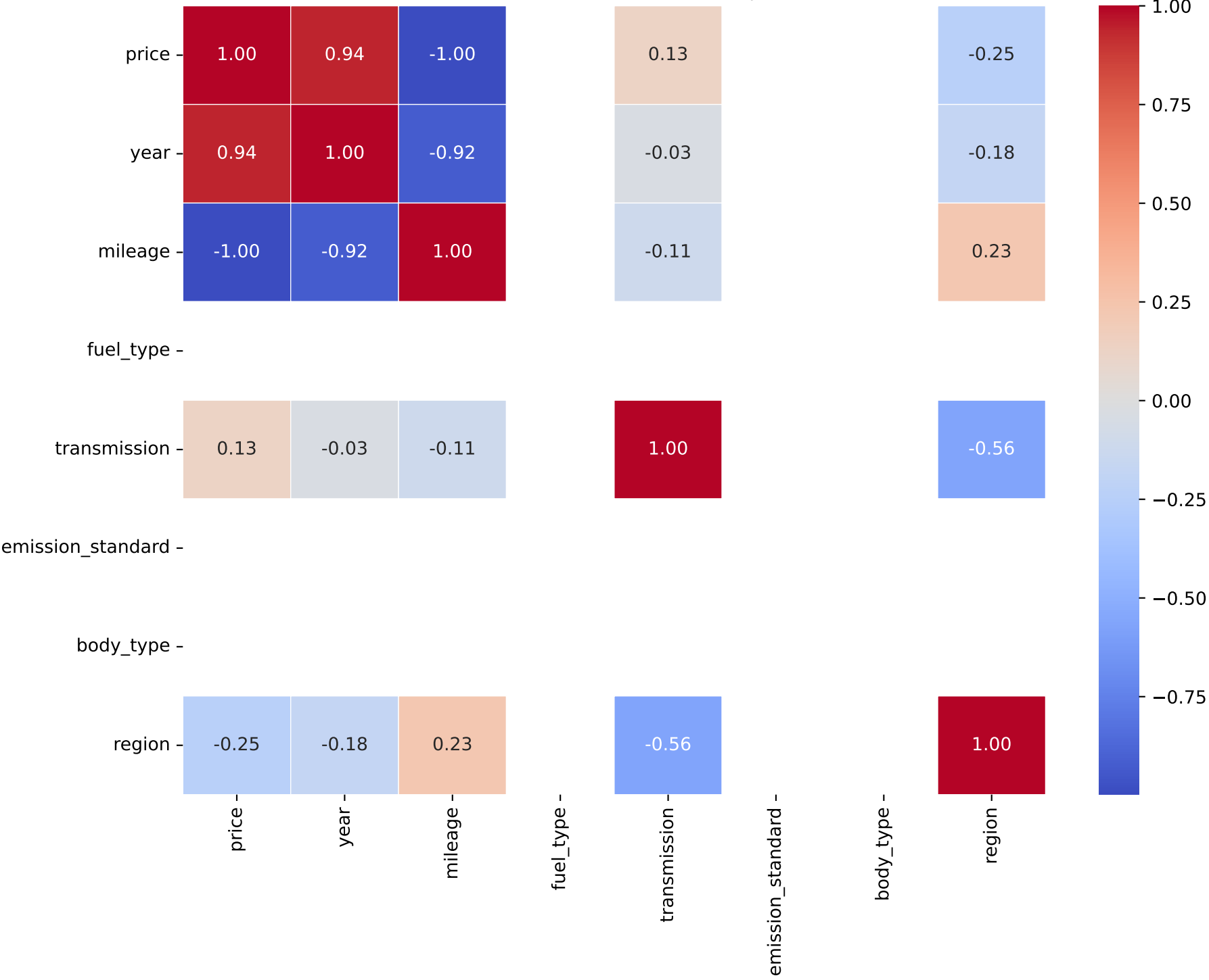
Correlation Heatmap for Model: scala | Fuel Type: 1
