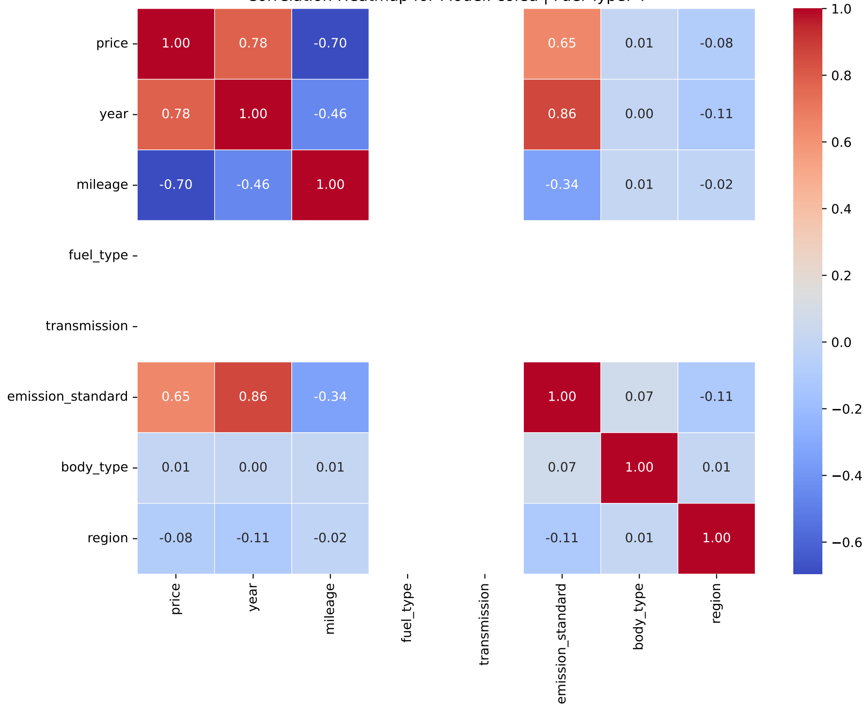
Correlation Heatmap for Model: corsa | Fuel Type: 4
