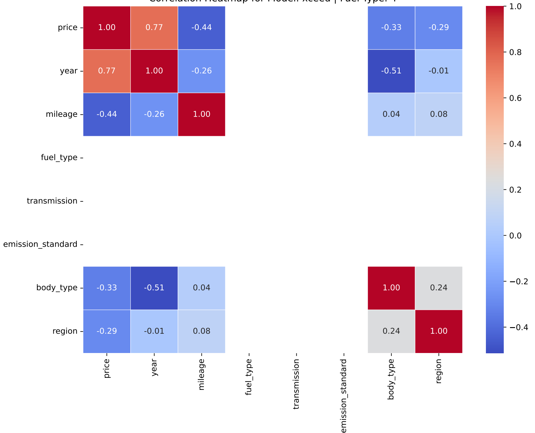
Correlation Heatmap for Model: xceed | Fuel Type: 4
