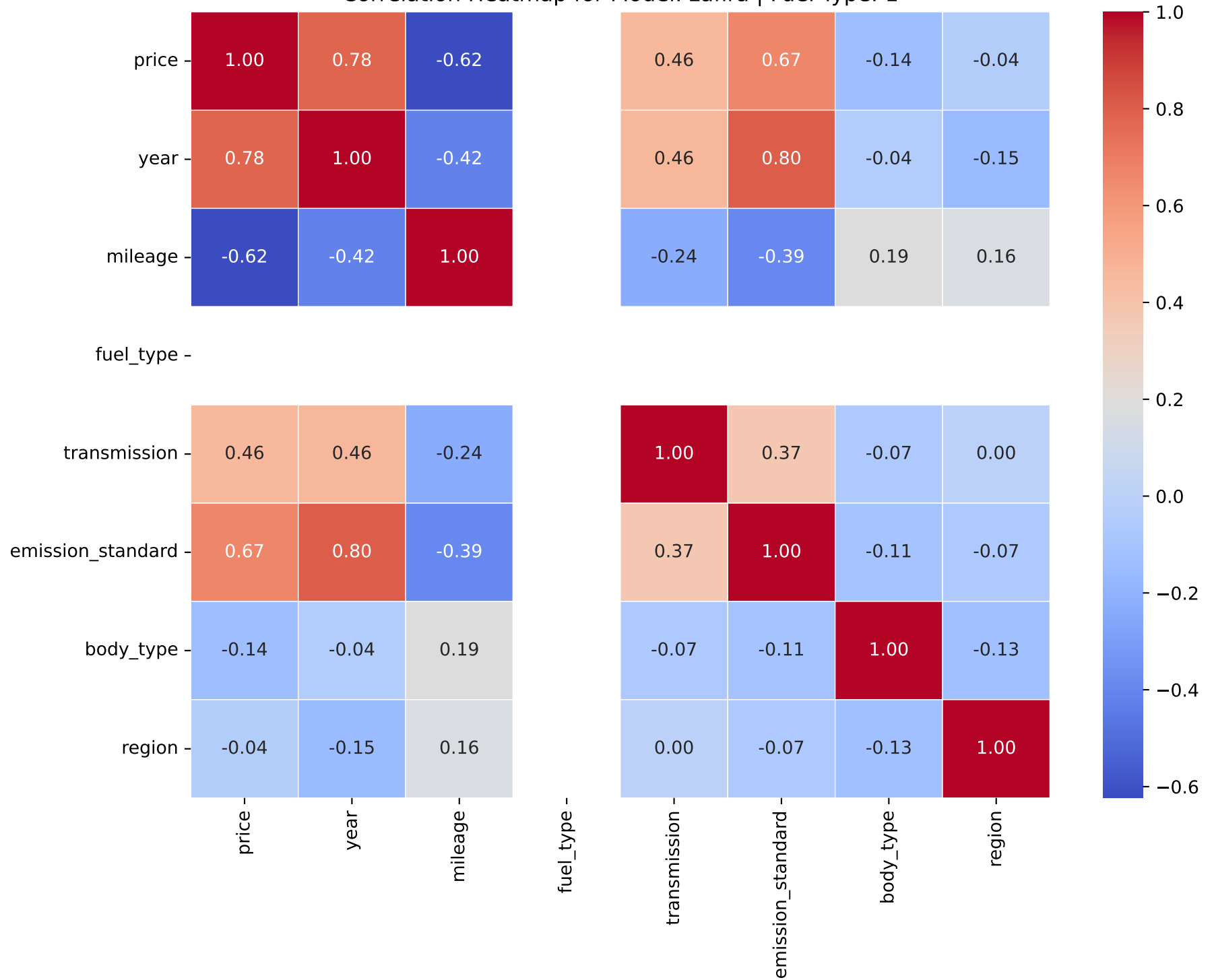
Correlation Heatmap for Model: zafira | Fuel Type: 1
