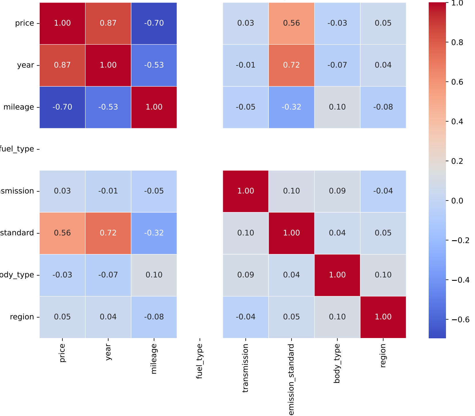
Correlation Heatmap for Model: tucson | Fuel Type: 1
