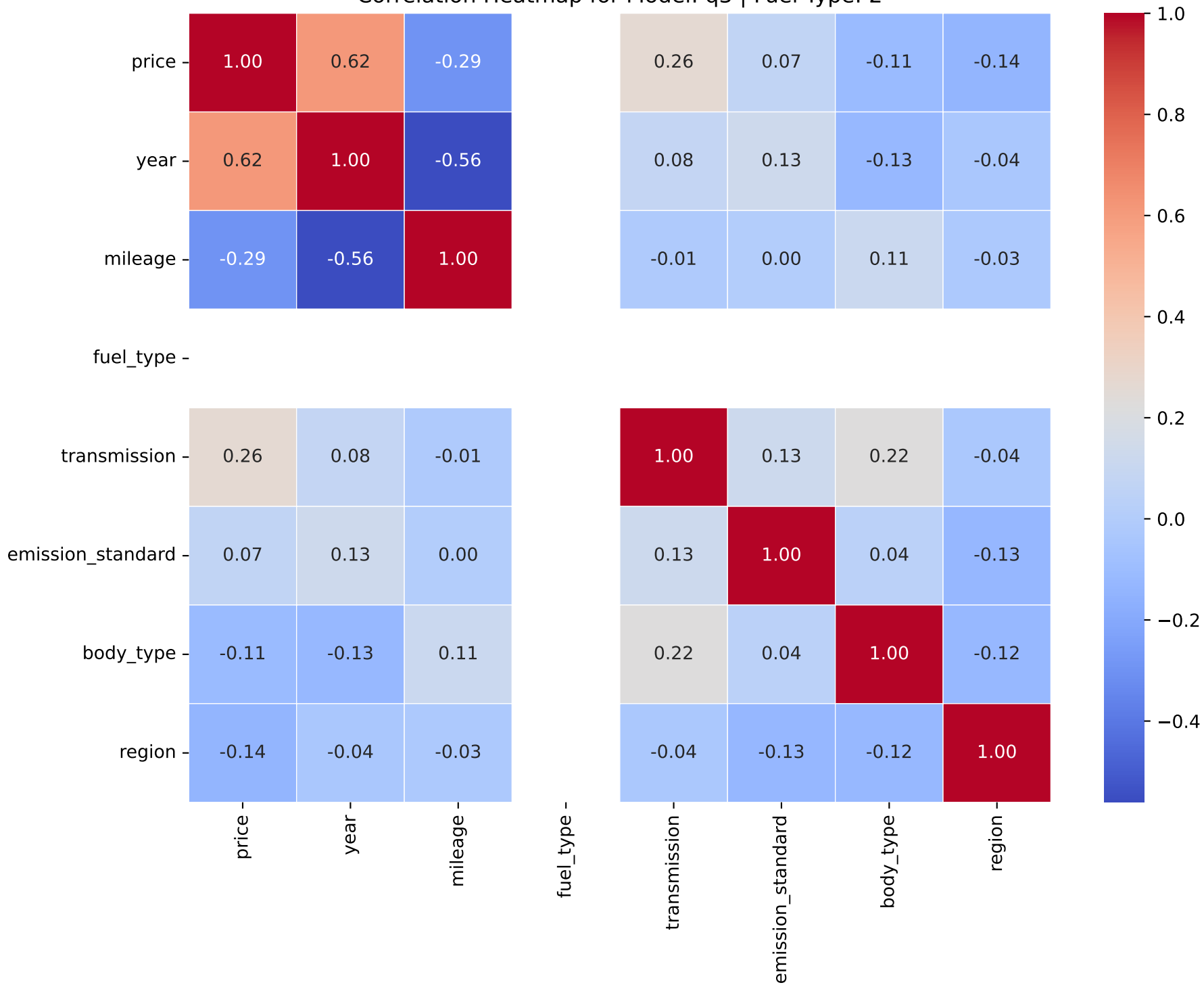
Correlation Heatmap for Model: q3 | Fuel Type: 2
