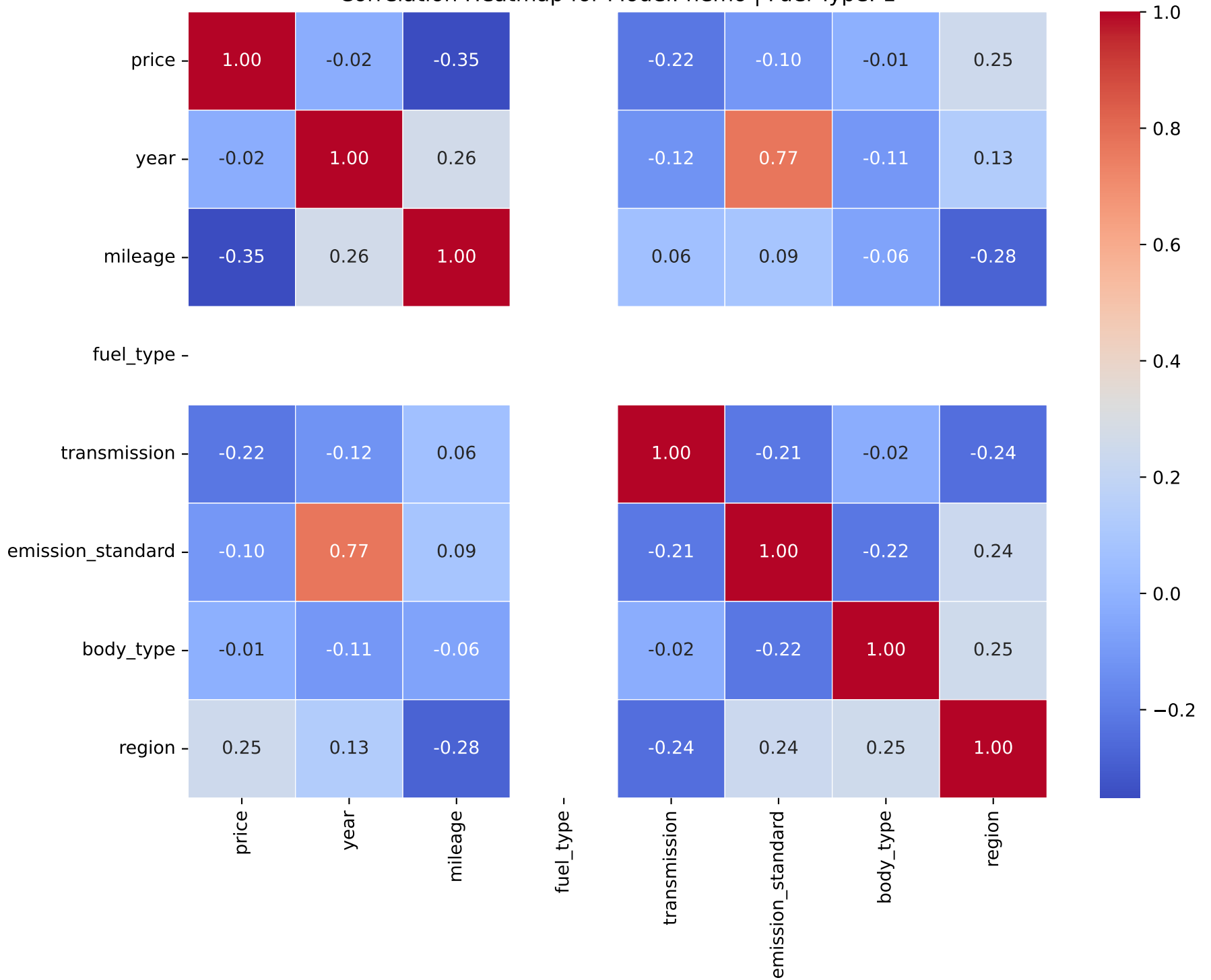
Correlation Heatmap for Model: nemo | Fuel Type: 1
