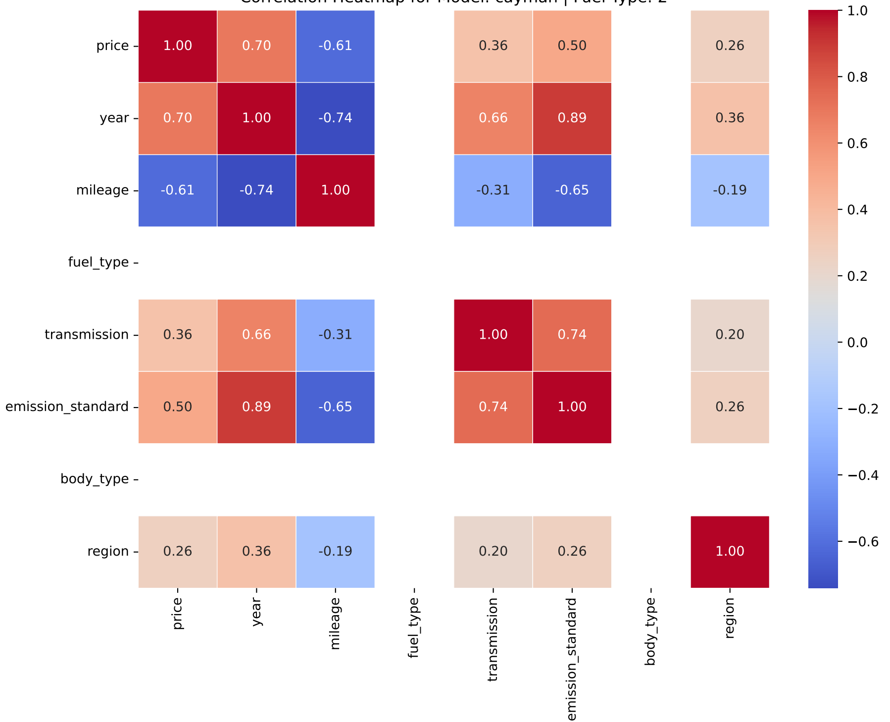
Correlation Heatmap for Model: cayman | Fuel Type: 2
