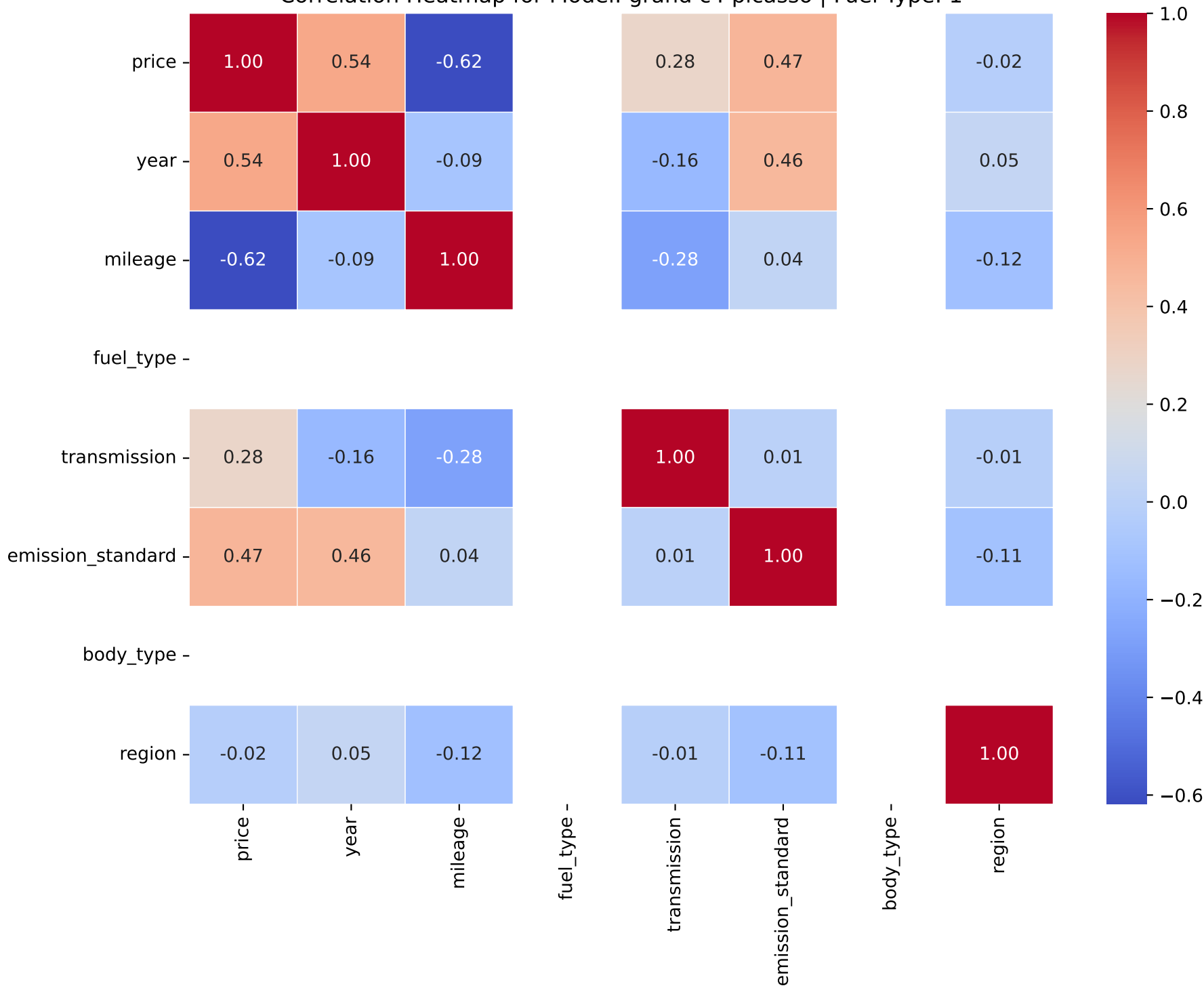
Correlation Heatmap for Model: grand c4 picasso | Fuel Type: 1
