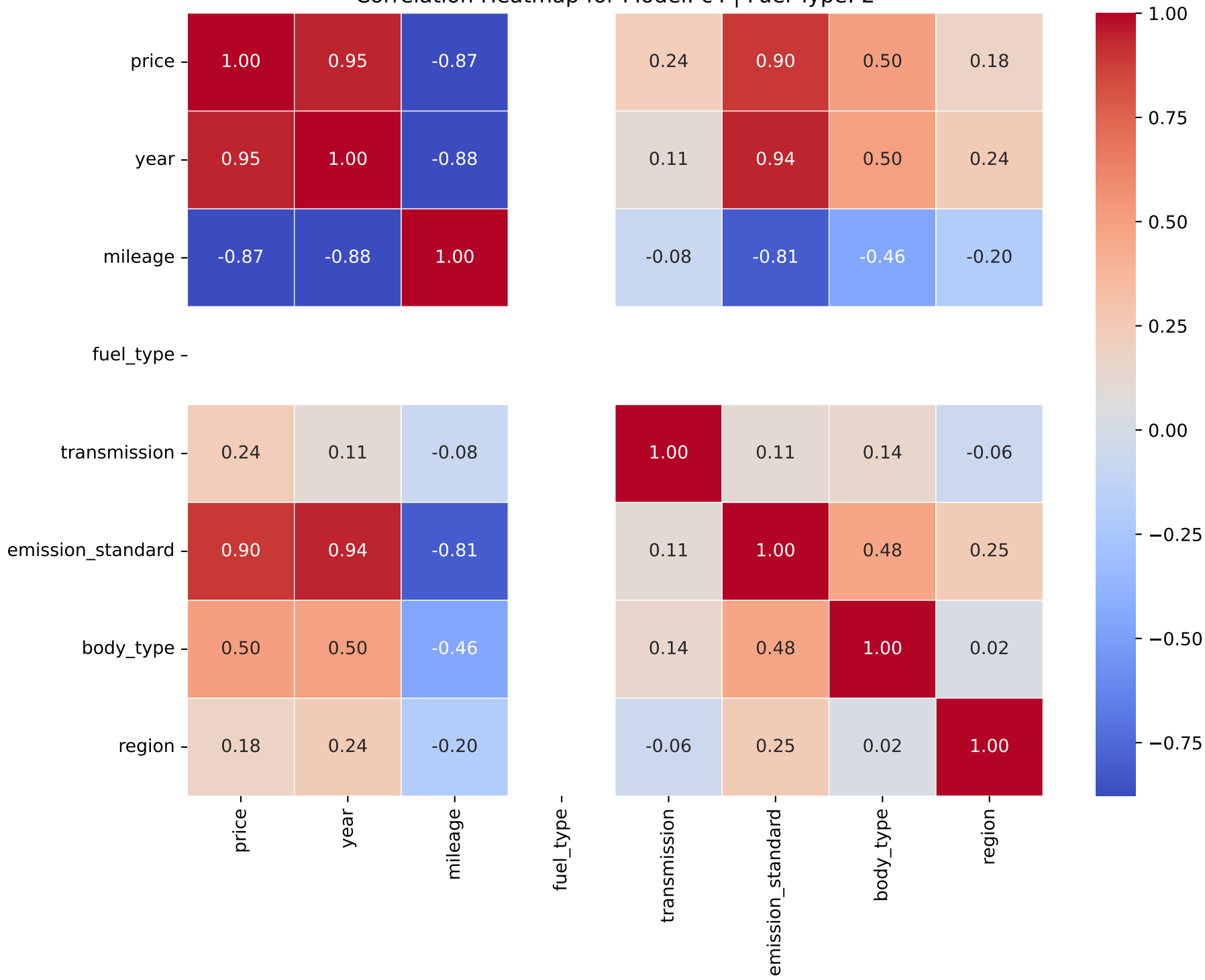
Correlation Heatmap for Model: c4 | Fuel Type: 2
