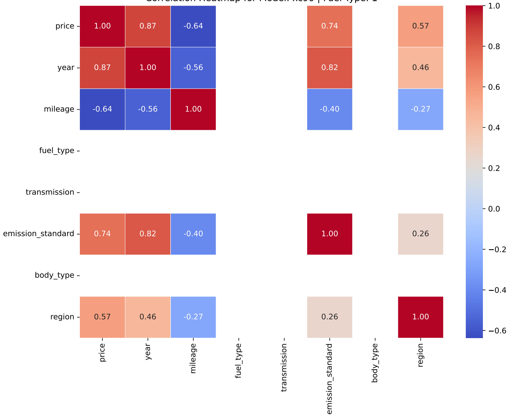
Correlation Heatmap for Model: xc90 | Fuel Type: 1
