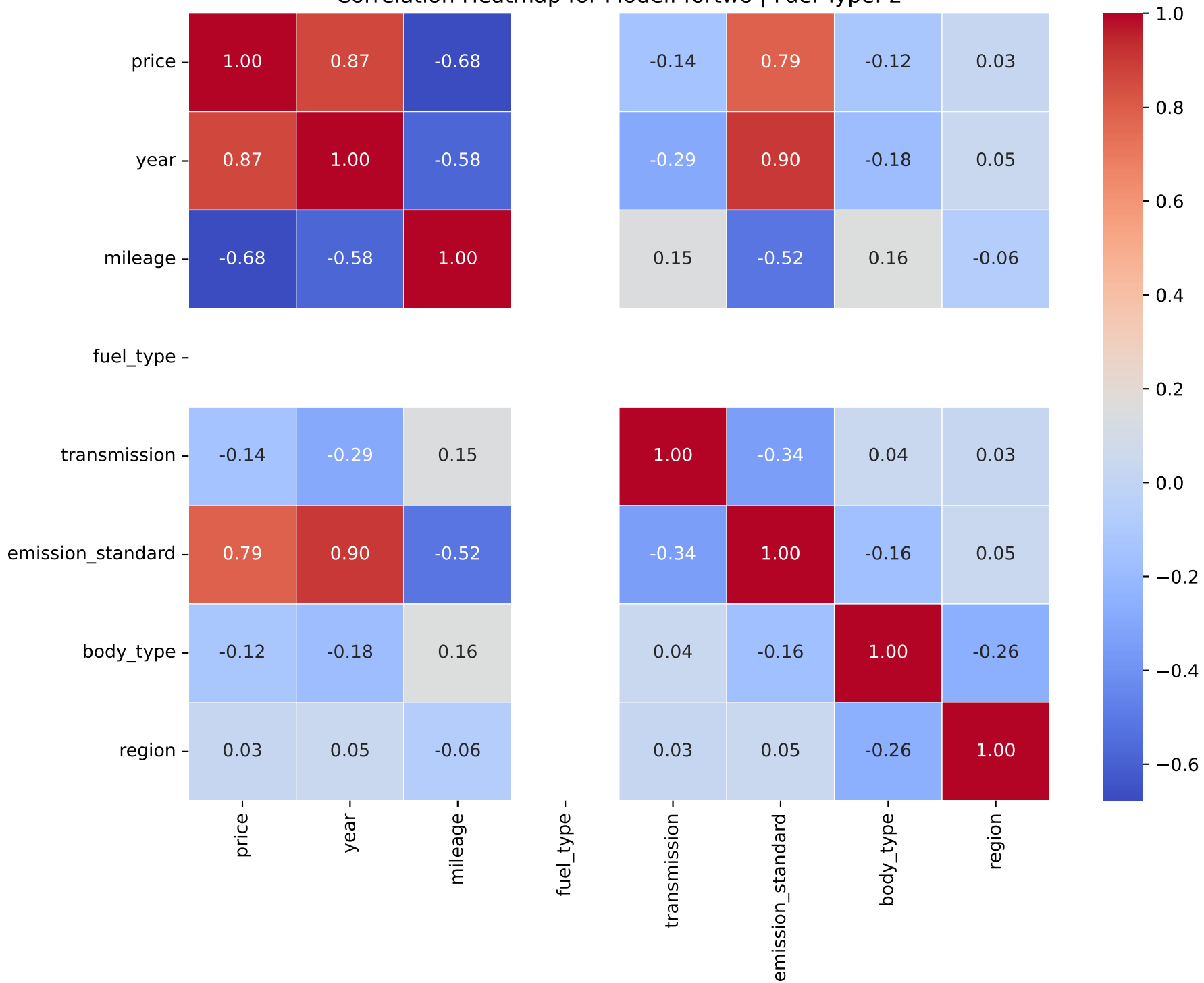
Correlation Heatmap for Model: fortwo | Fuel Type: 2
