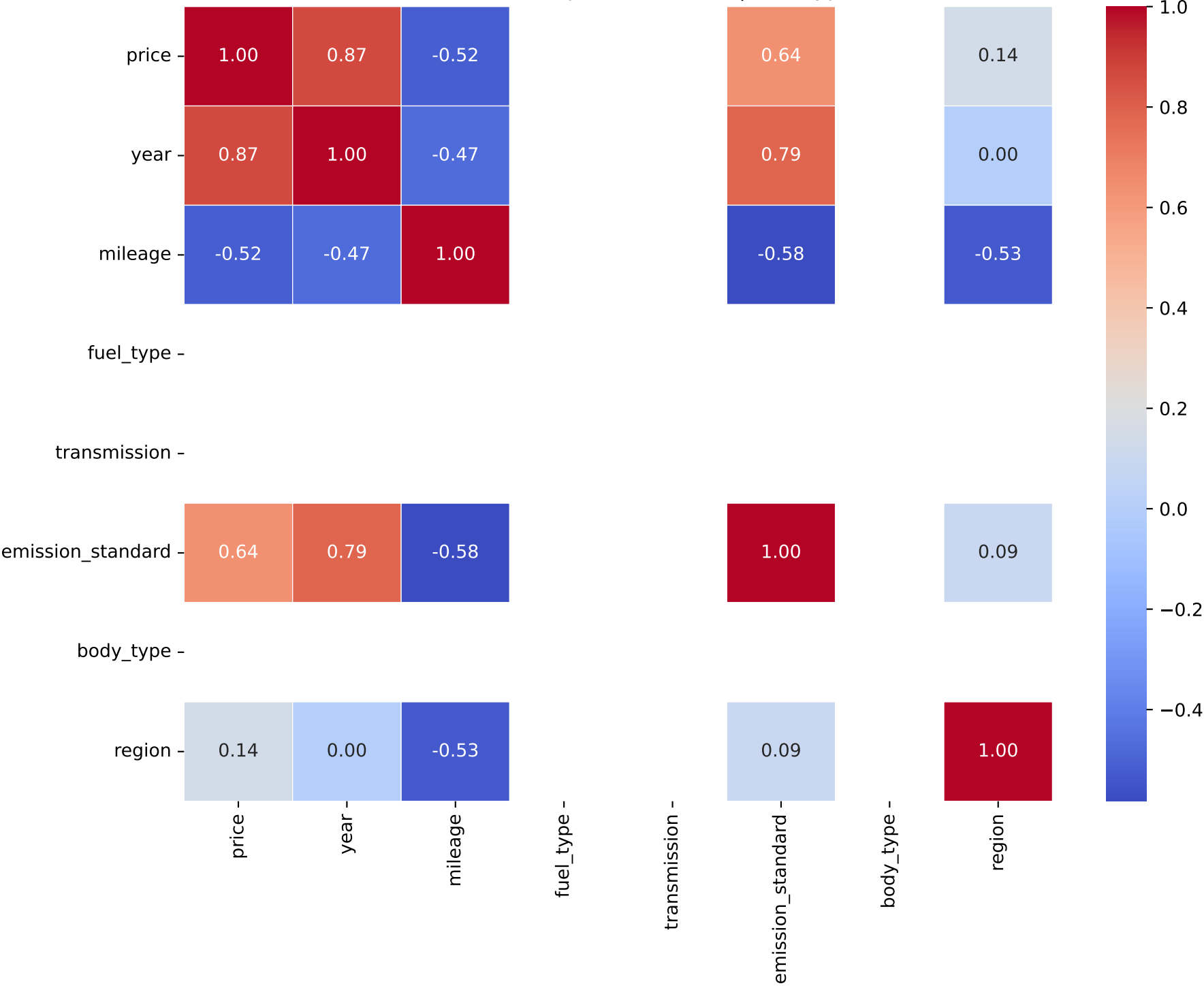
Correlation Heatmap for Model: a8 | Fuel Type: 1
