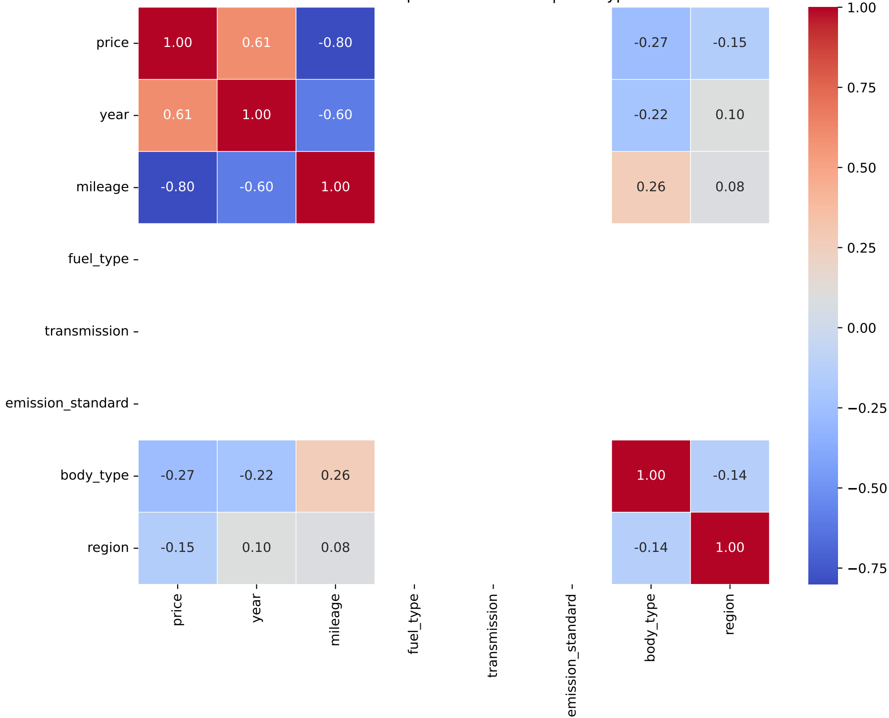
Correlation Heatmap for Model: 3008 | Fuel Type: 3
