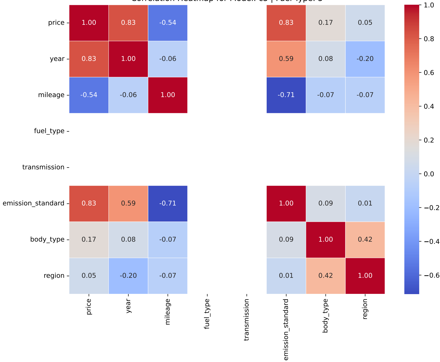
Correlation Heatmap for Model: c3 | Fuel Type: 5
