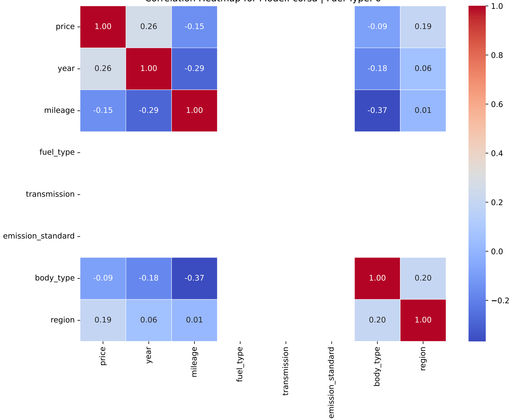
Correlation Heatmap for Model: corsa | Fuel Type: 0
