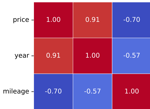
Correlation Heatmap for Model: micra | Fuel Type: 2
