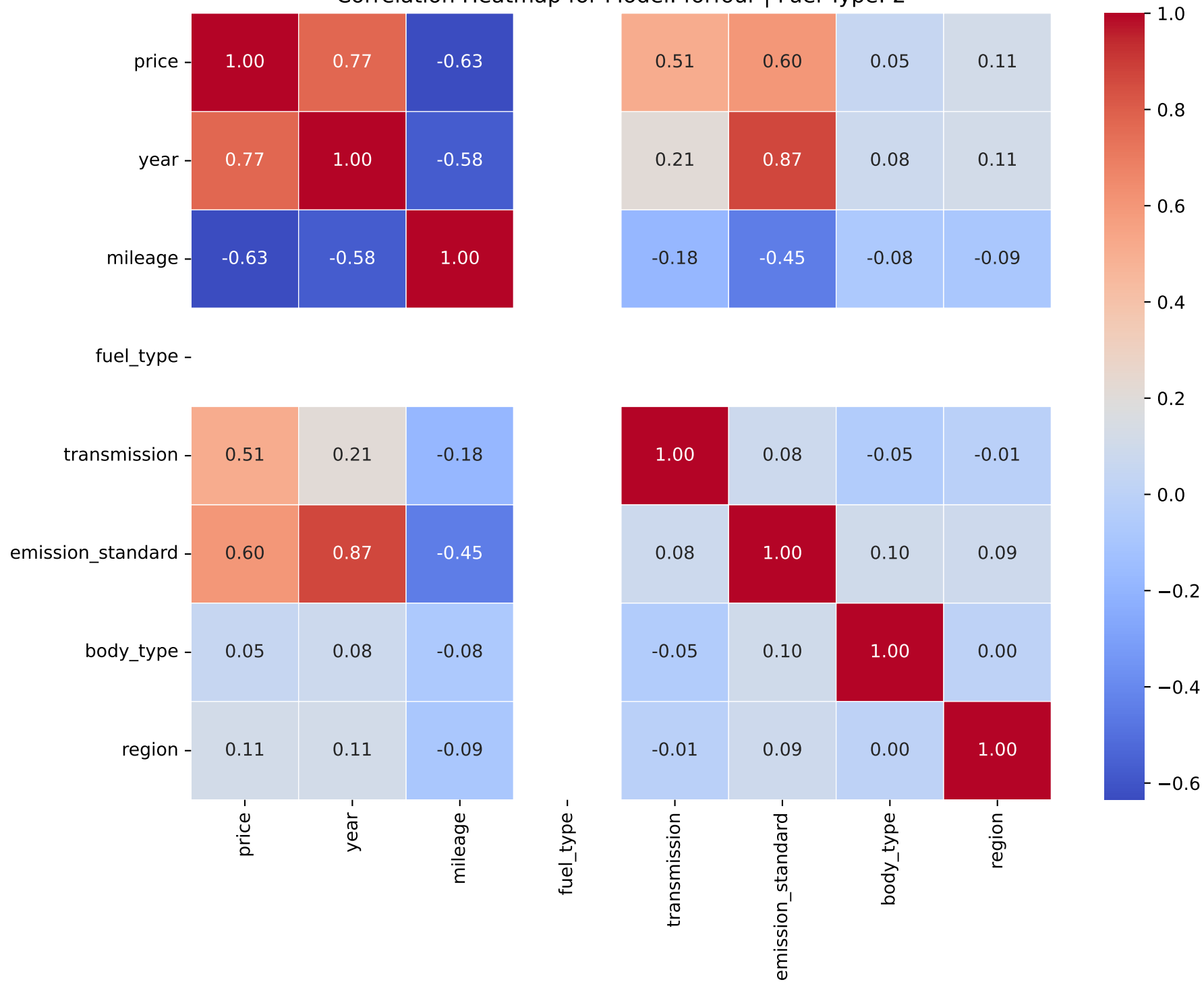
Correlation Heatmap for Model: forfour | Fuel Type: 2
