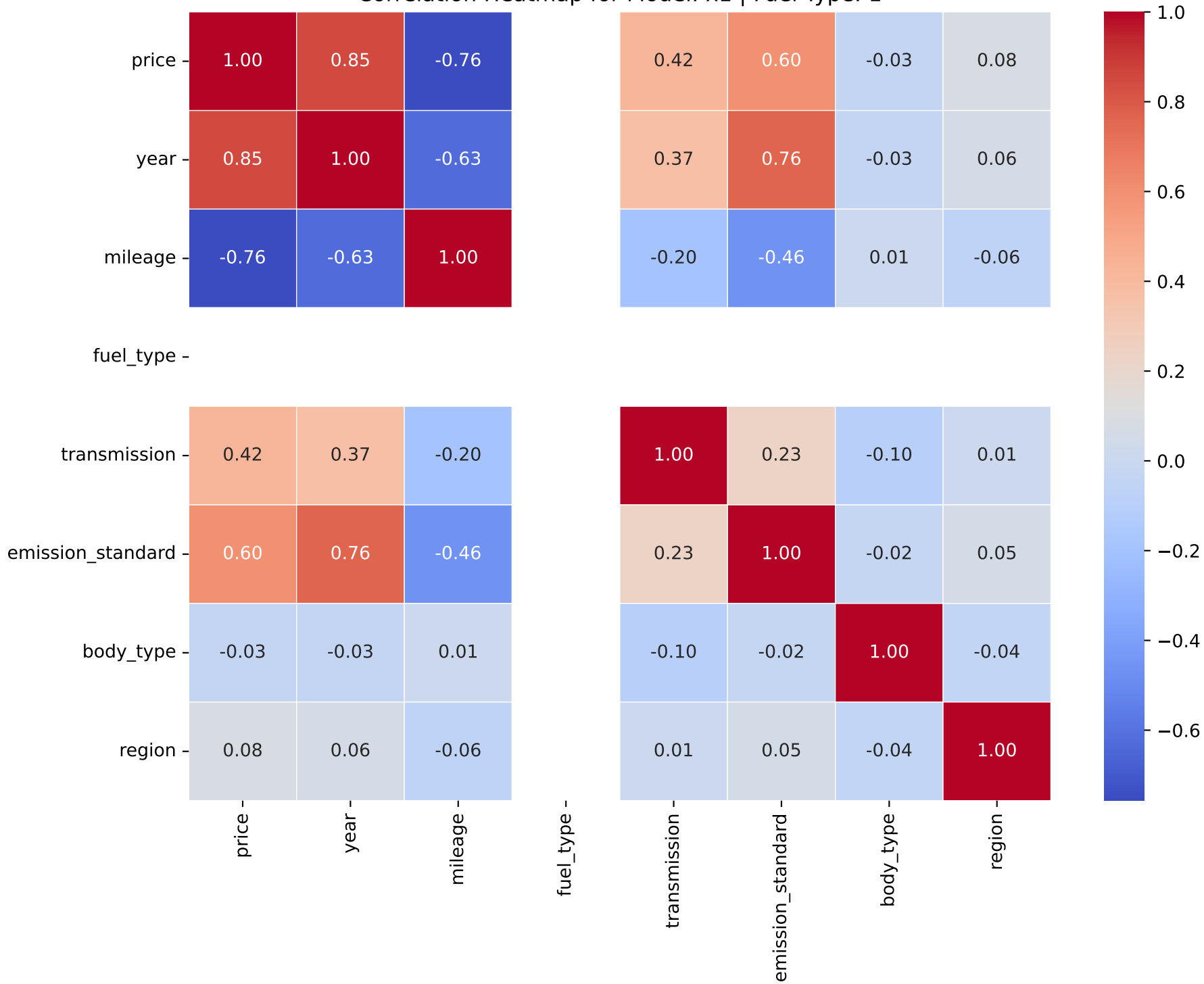
Correlation Heatmap for Model: x1 | Fuel Type: 1
