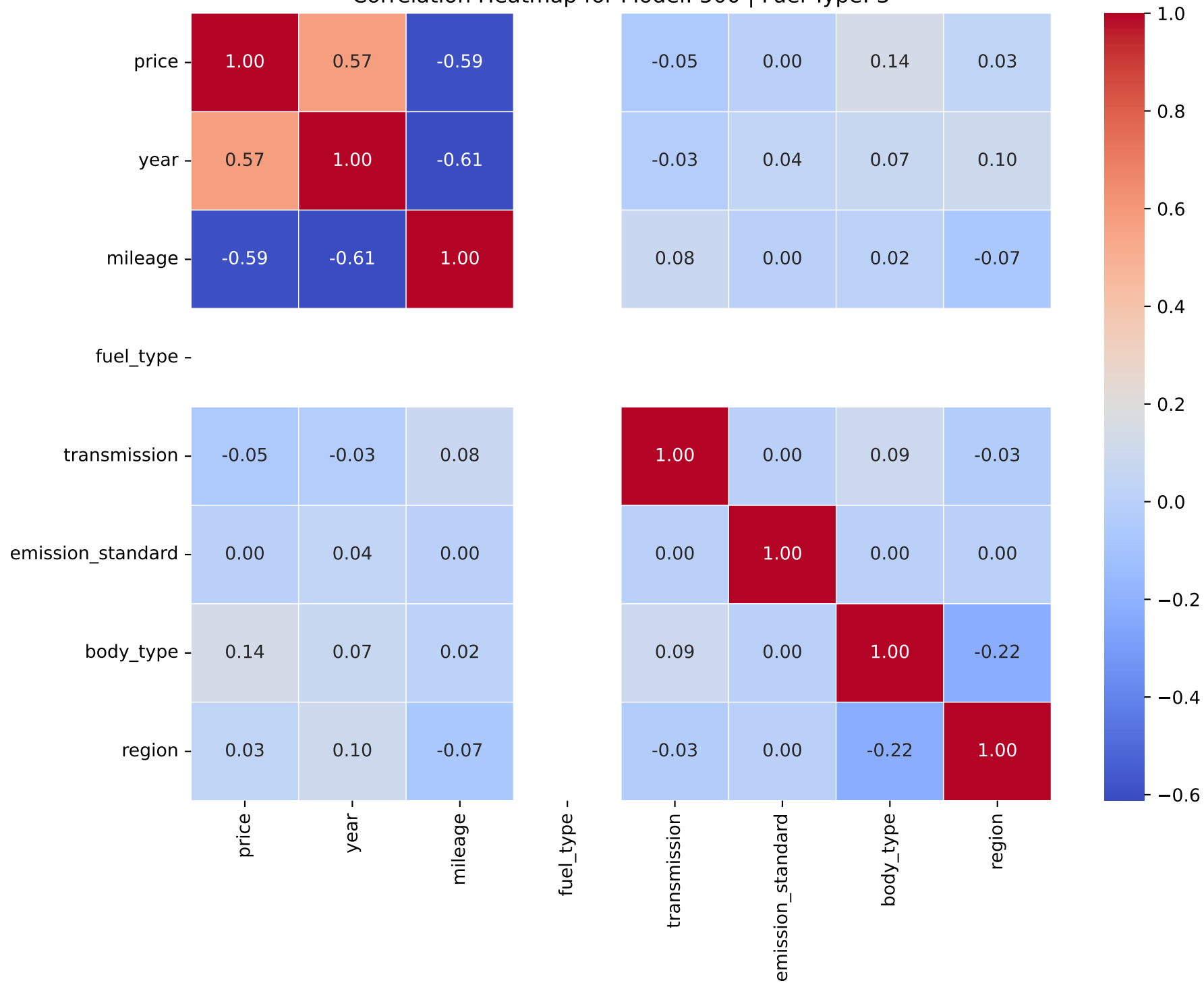
Correlation Heatmap for Model: 500 | Fuel Type: 3
