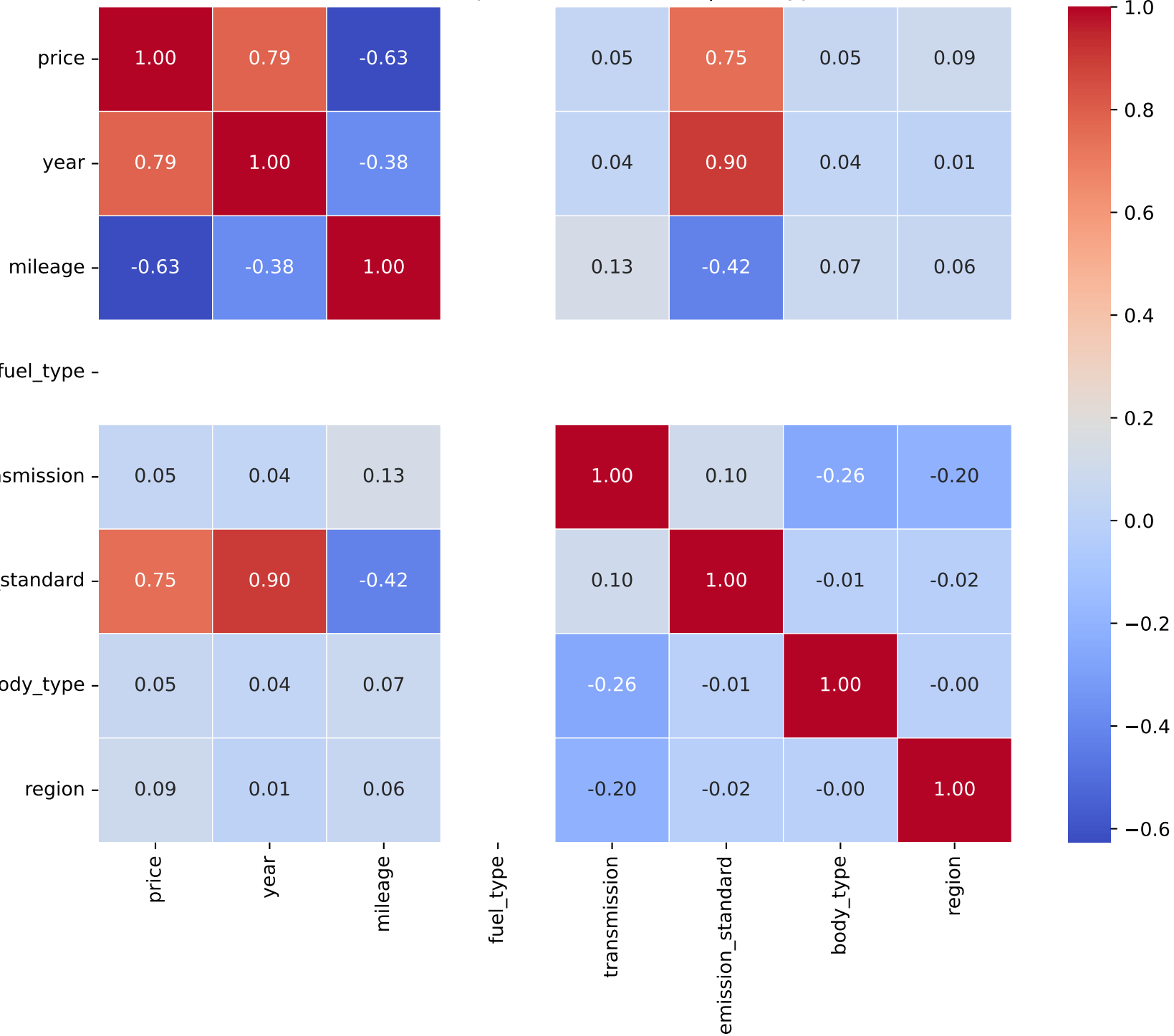
Correlation Heatmap for Model: navara | Fuel Type: 1
