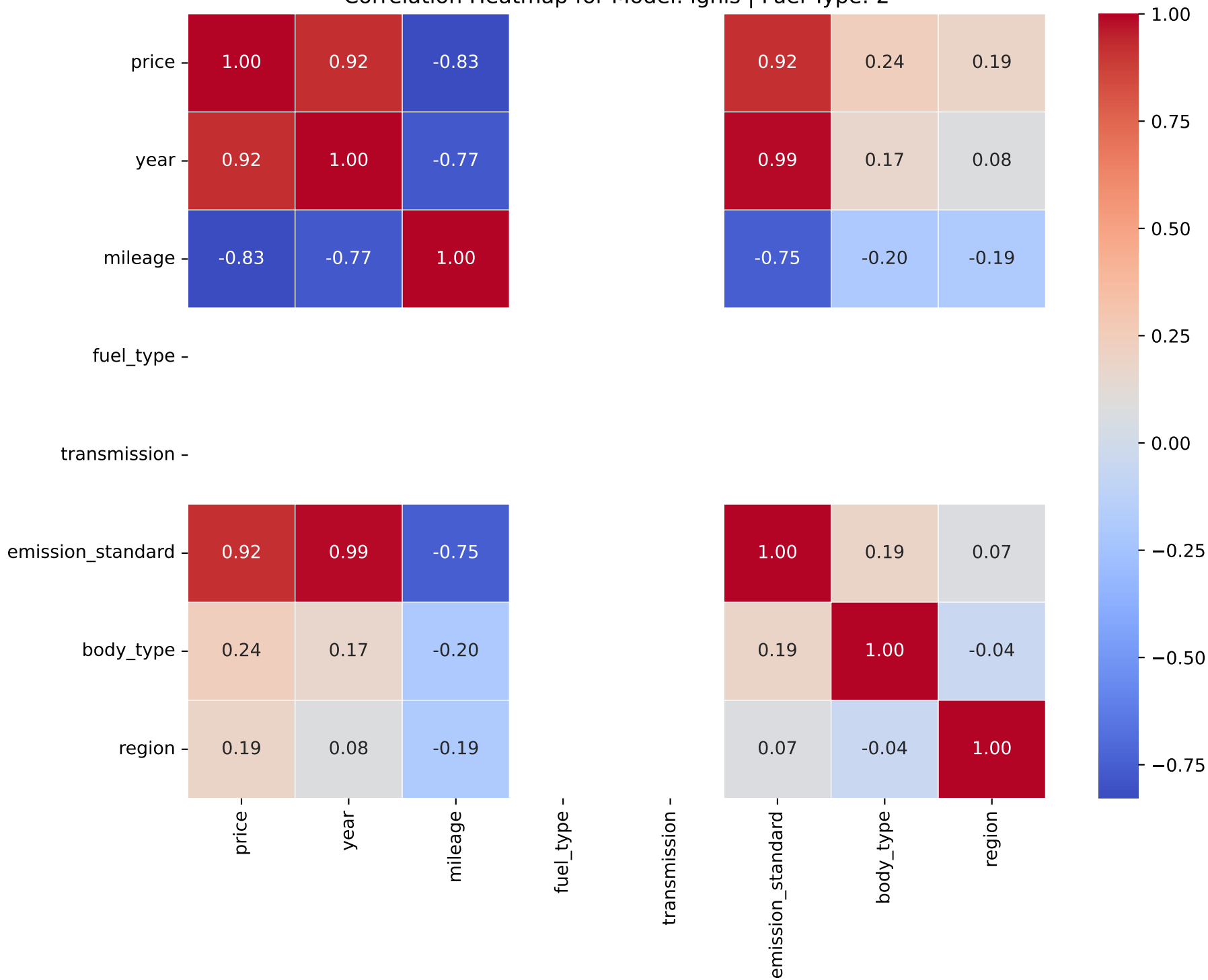
Correlation Heatmap for Model: ignis | Fuel Type: 2
