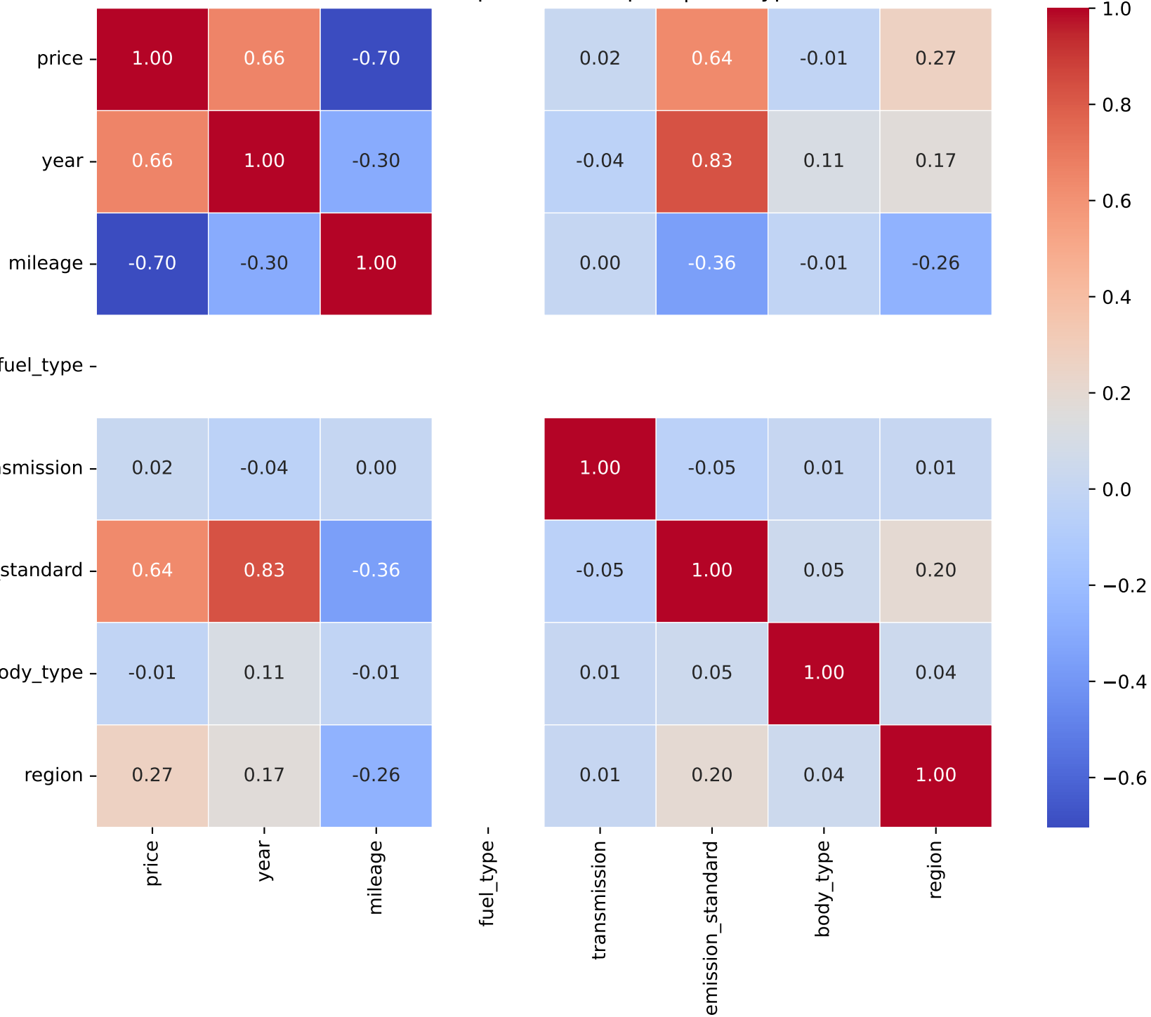
Correlation Heatmap for Model: qubo | Fuel Type: 1
