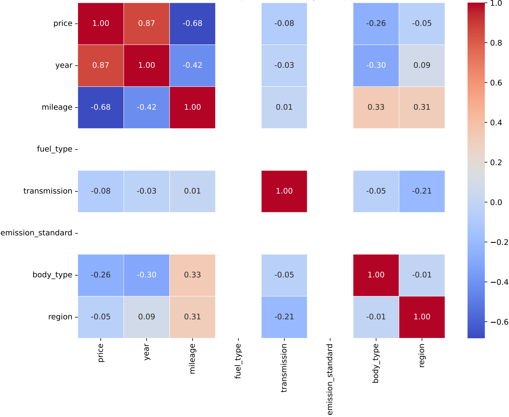
Correlation Heatmap for Model: x5 | Fuel Type: 3
