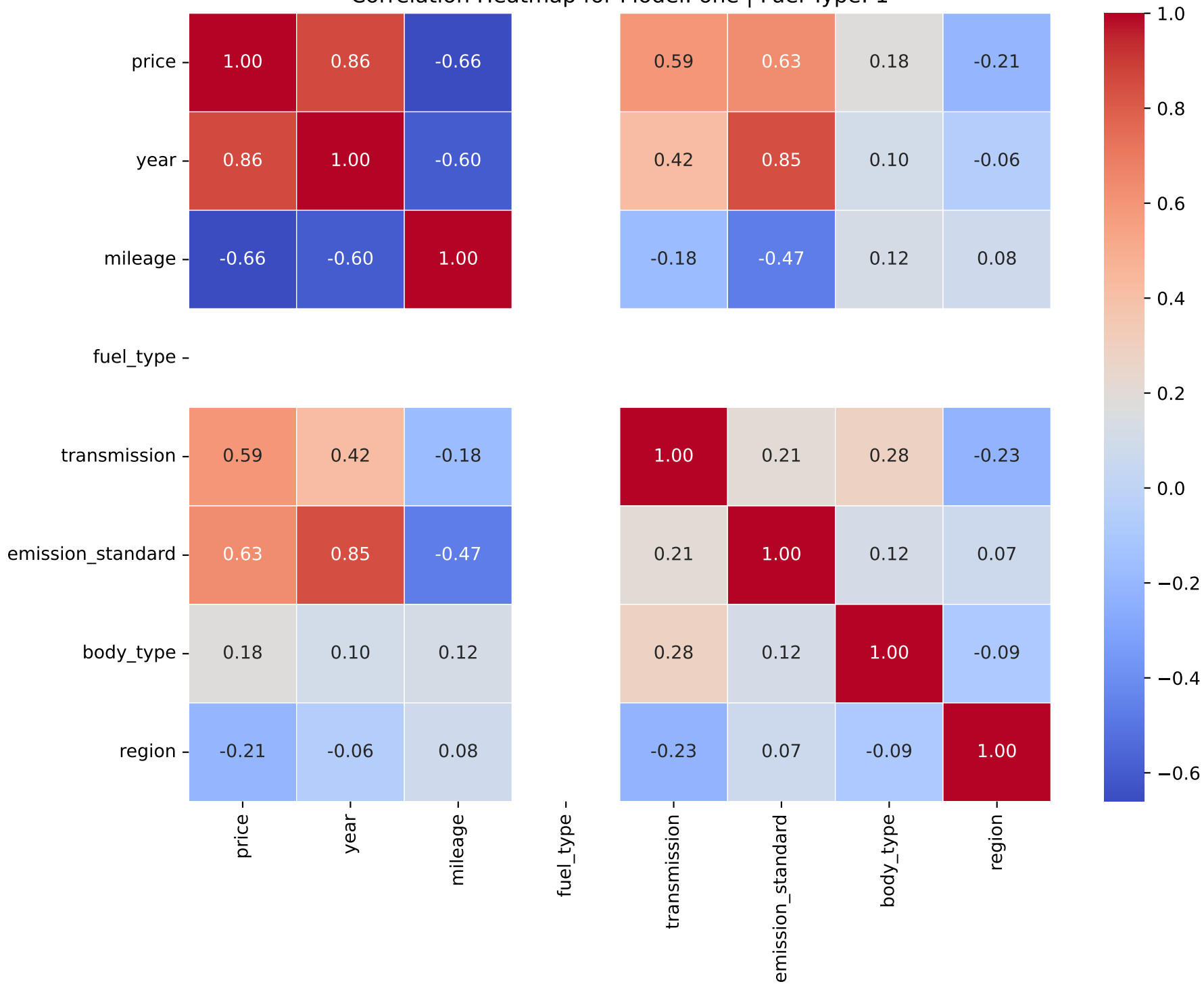
Correlation Heatmap for Model: one | Fuel Type: 1
