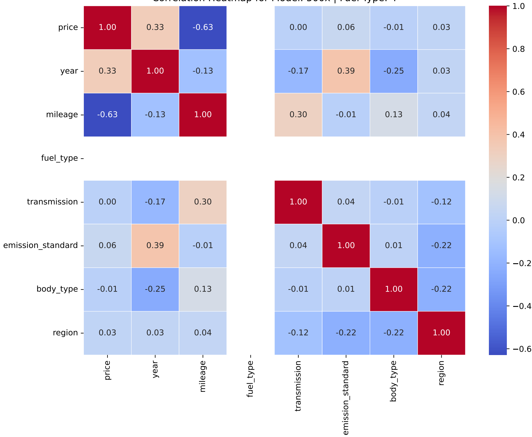
Correlation Heatmap for Model: 500x | Fuel Type: 4
