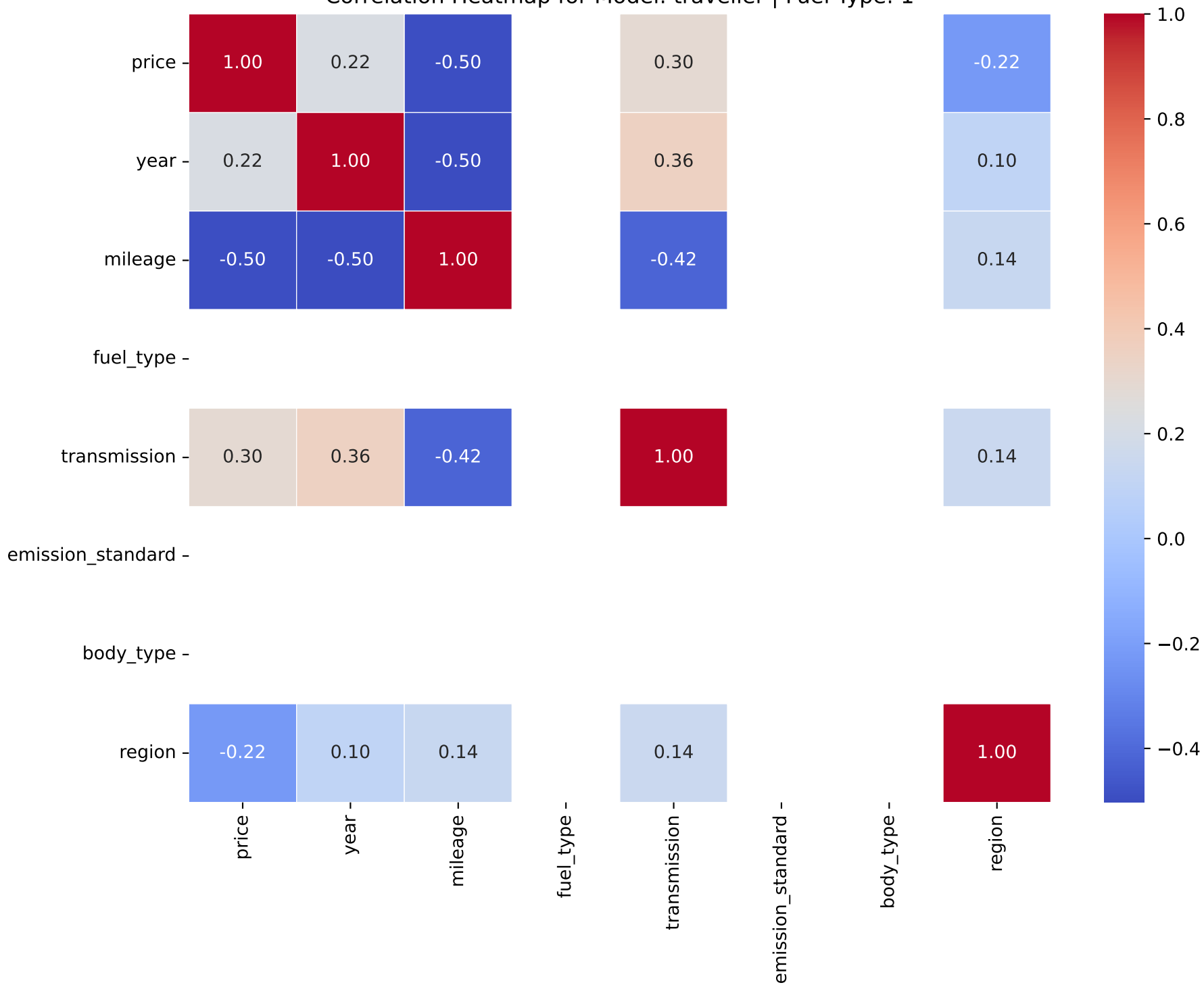
Correlation Heatmap for Model: traveller | Fuel Type: 1
