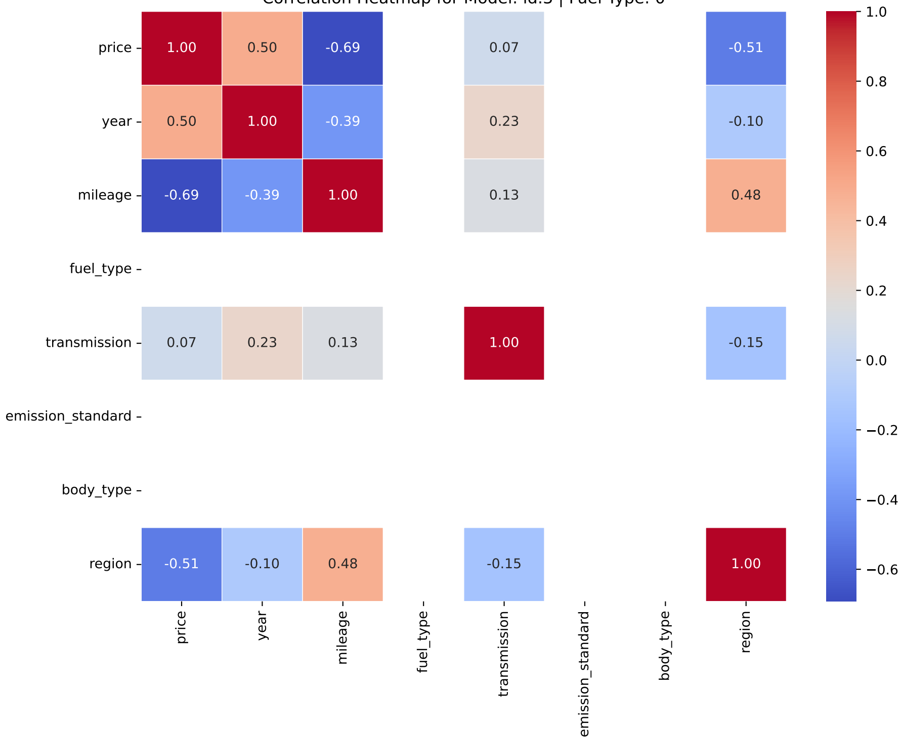
Correlation Heatmap for Model: id.3 | Fuel Type: 0
