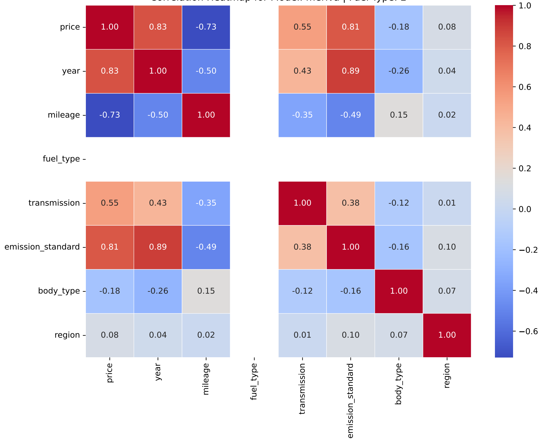
Correlation Heatmap for Model: meriva | Fuel Type: 2
