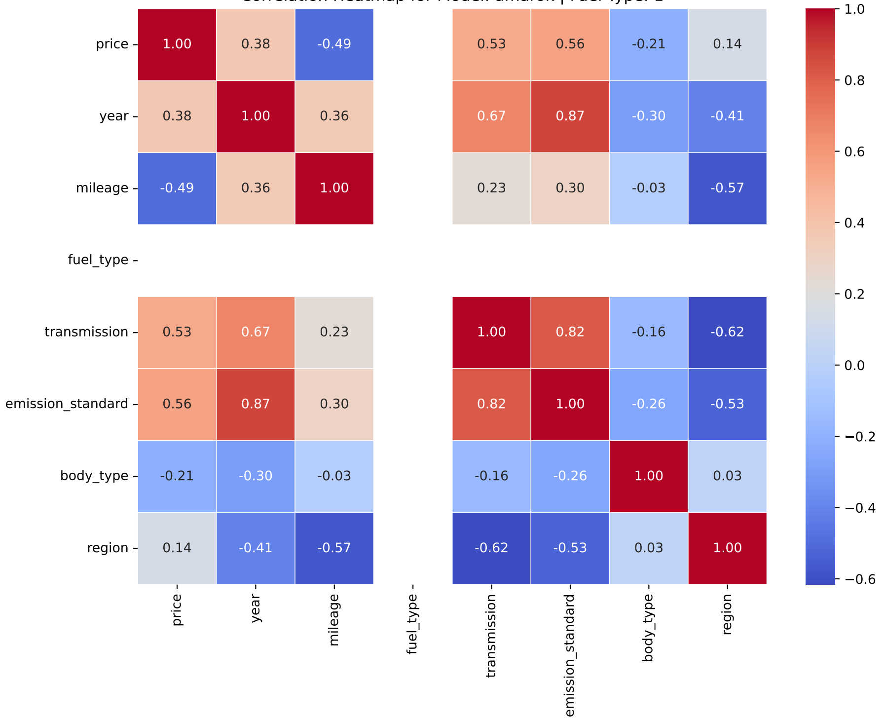
Correlation Heatmap for Model: amarok | Fuel Type: 1
