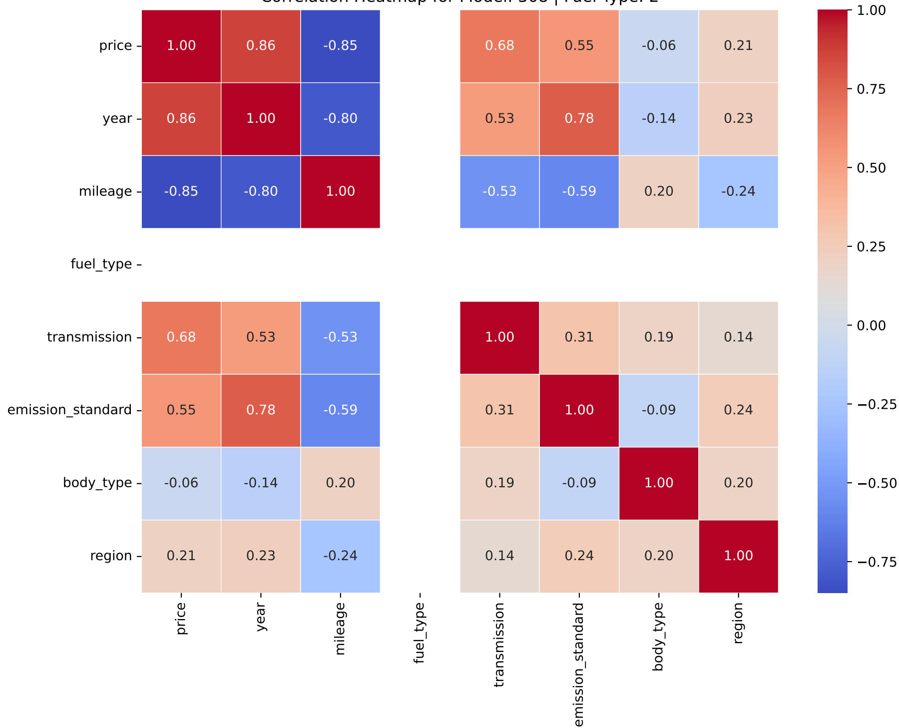
Correlation Heatmap for Model: 308 | Fuel Type: 2
