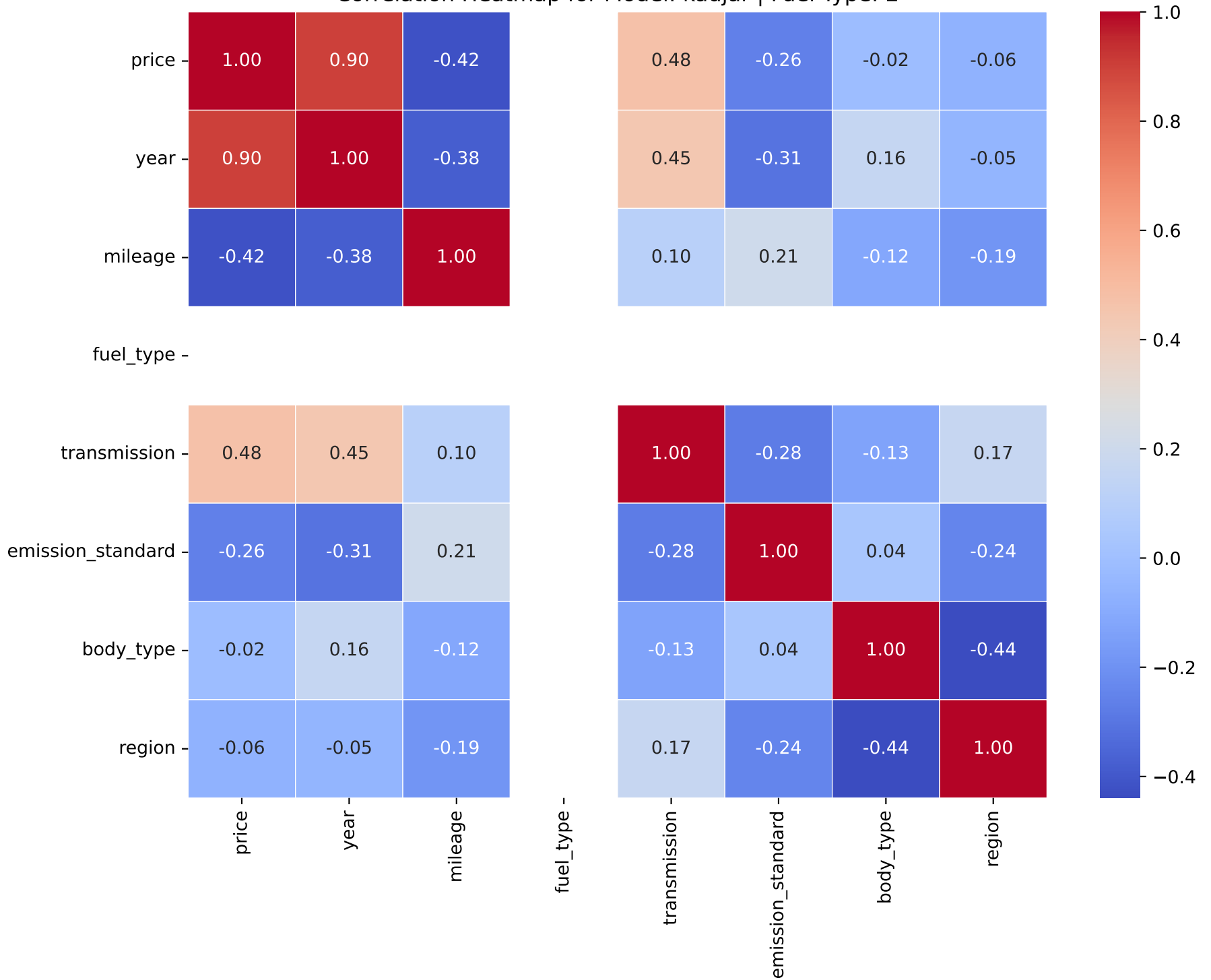
Correlation Heatmap for Model: kadjar | Fuel Type: 2
