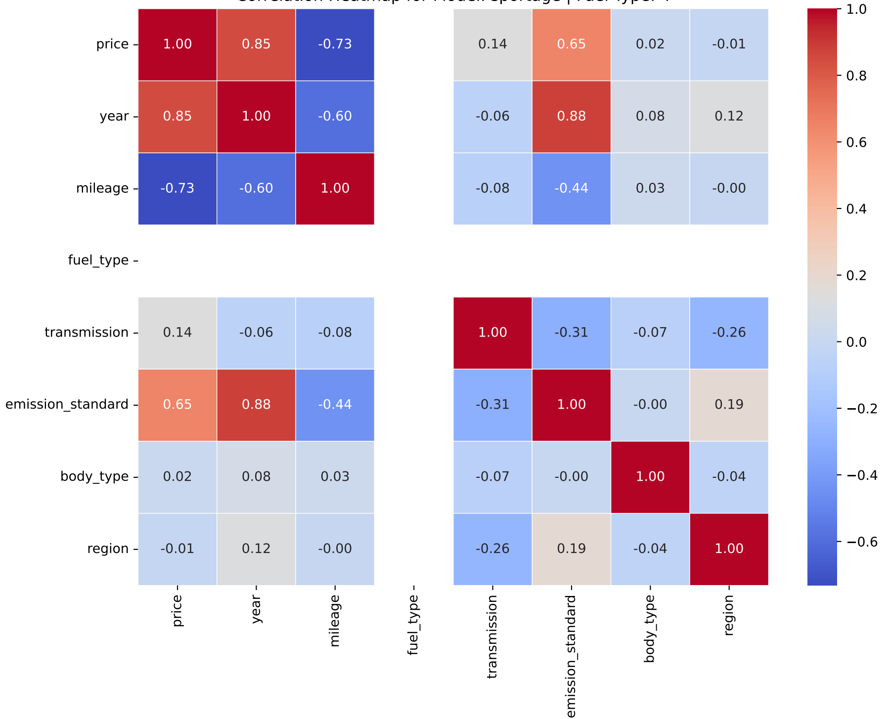
Correlation Heatmap for Model: sportage | Fuel Type: 4
