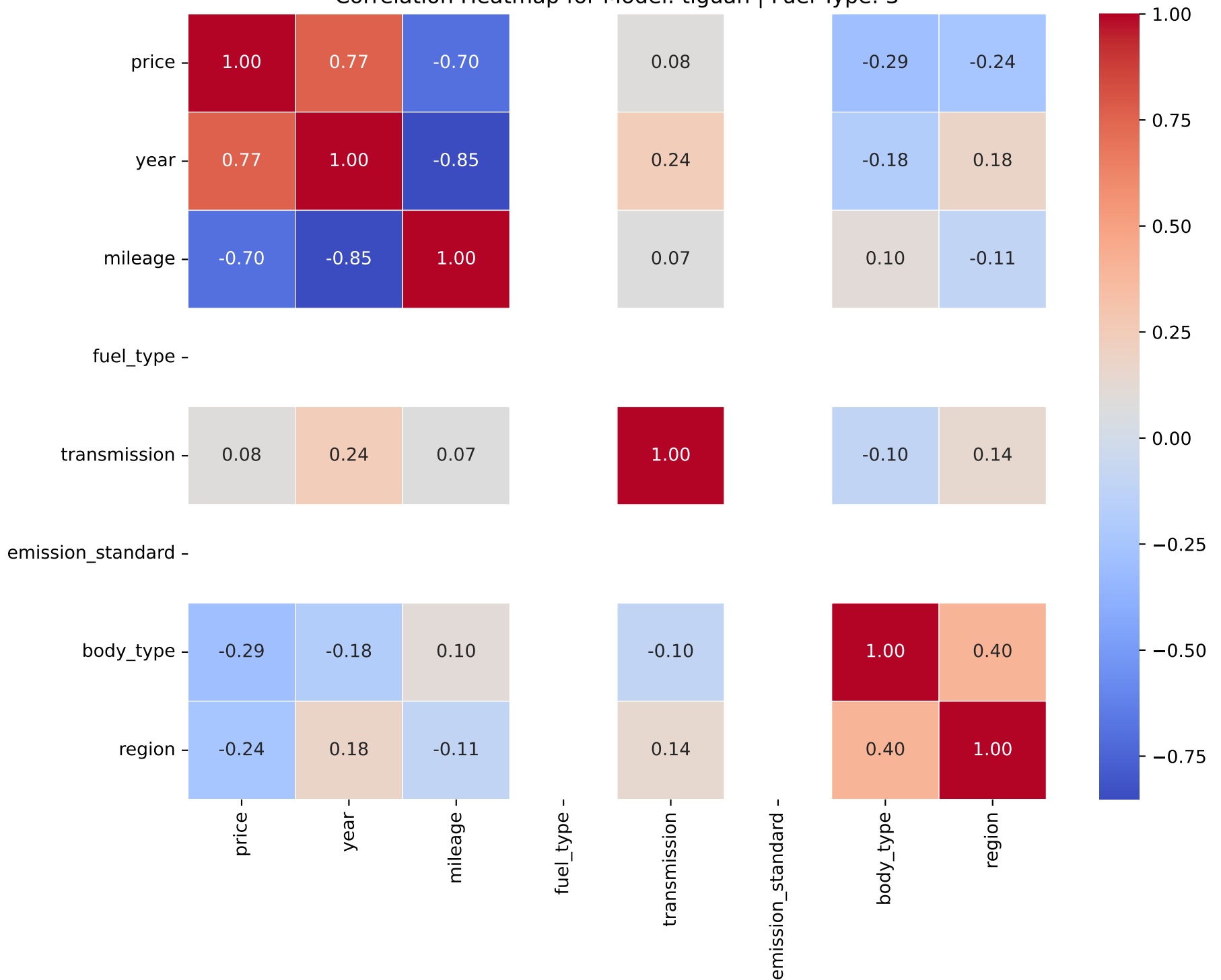
Correlation Heatmap for Model: tiguan | Fuel Type: 3
