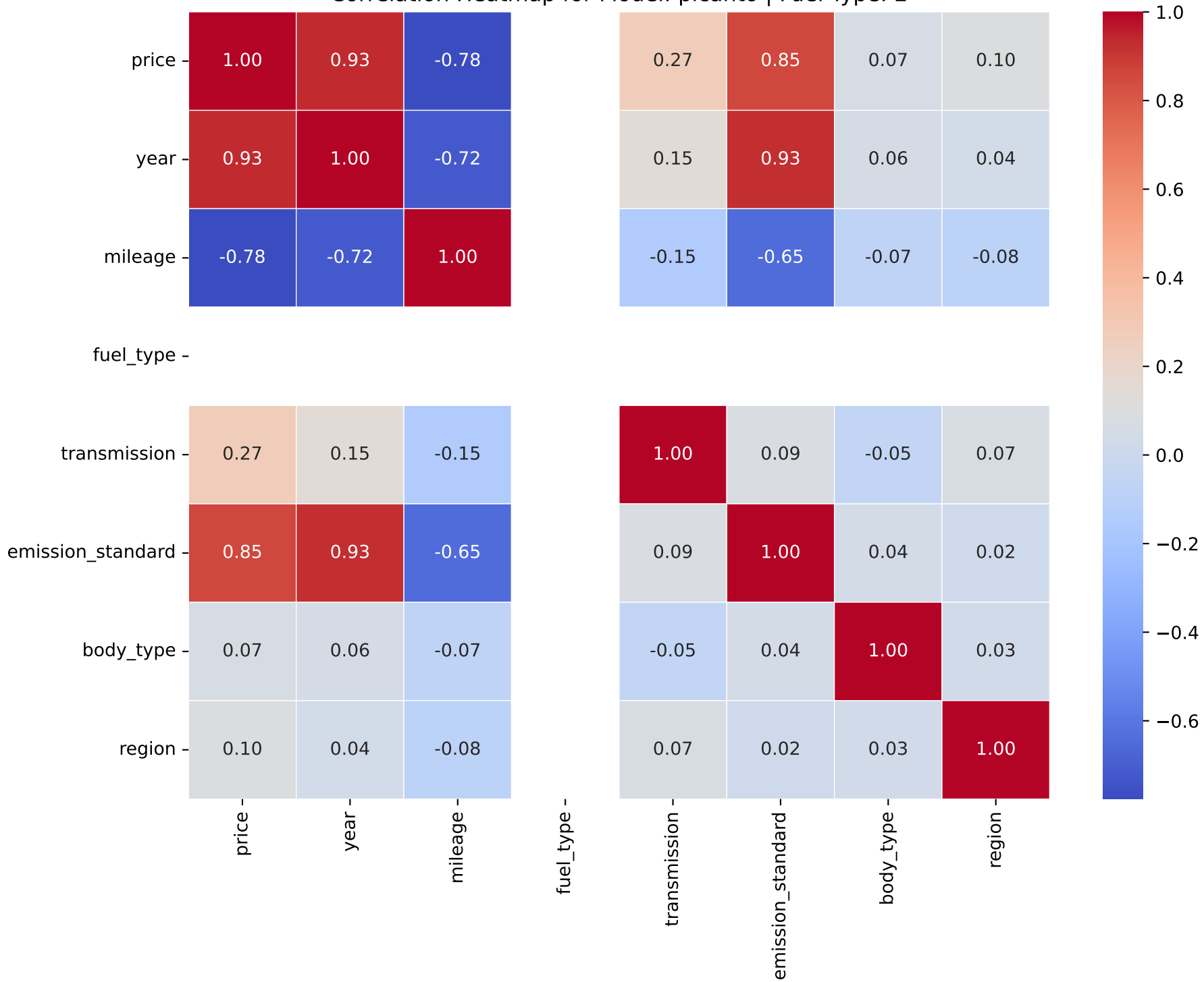
Correlation Heatmap for Model: picanto | Fuel Type: 2
