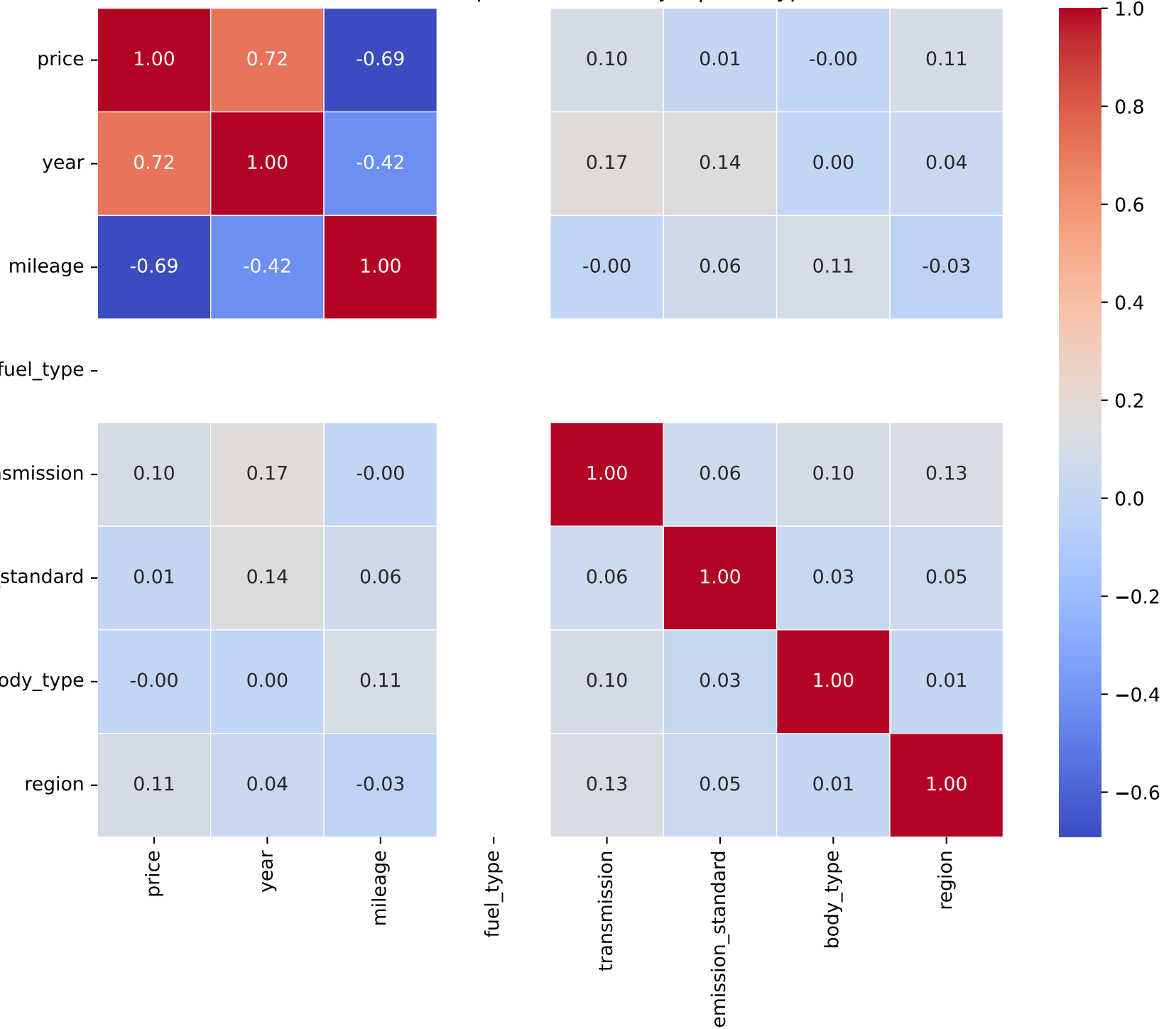
Correlation Heatmap for Model: kadjar | Fuel Type: 1
