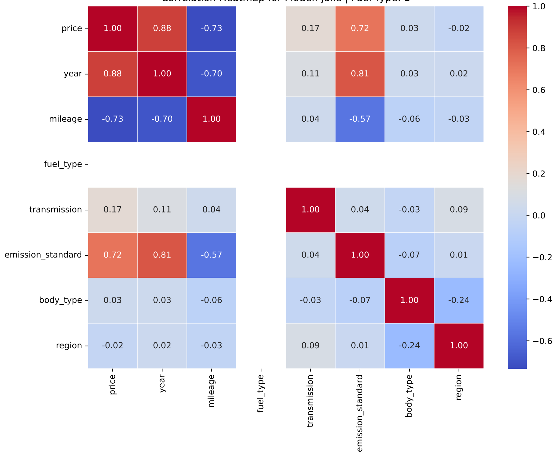
Correlation Heatmap for Model: juke | Fuel Type: 2
