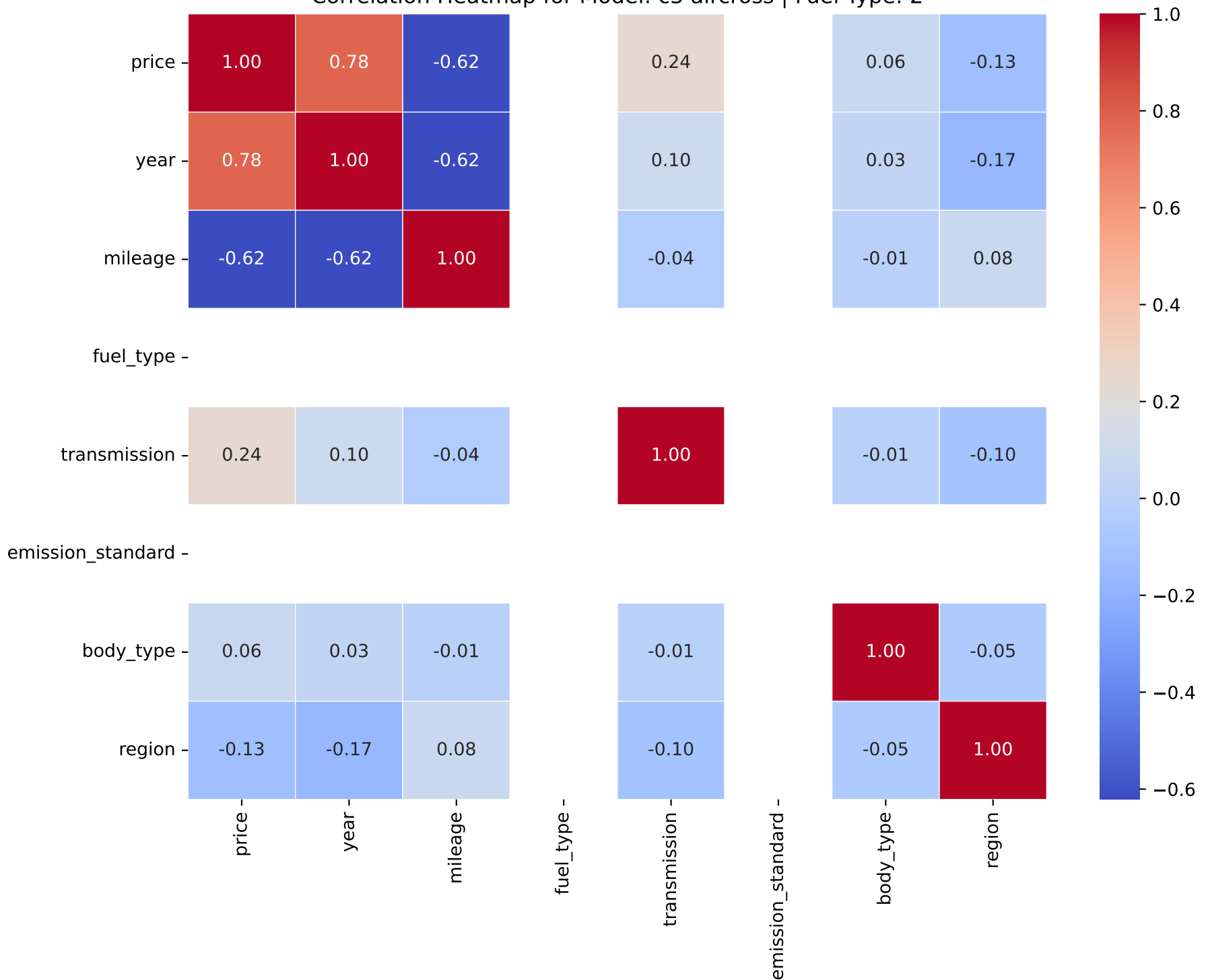
Correlation Heatmap for Model: c3 aircross | Fuel Type: 2
