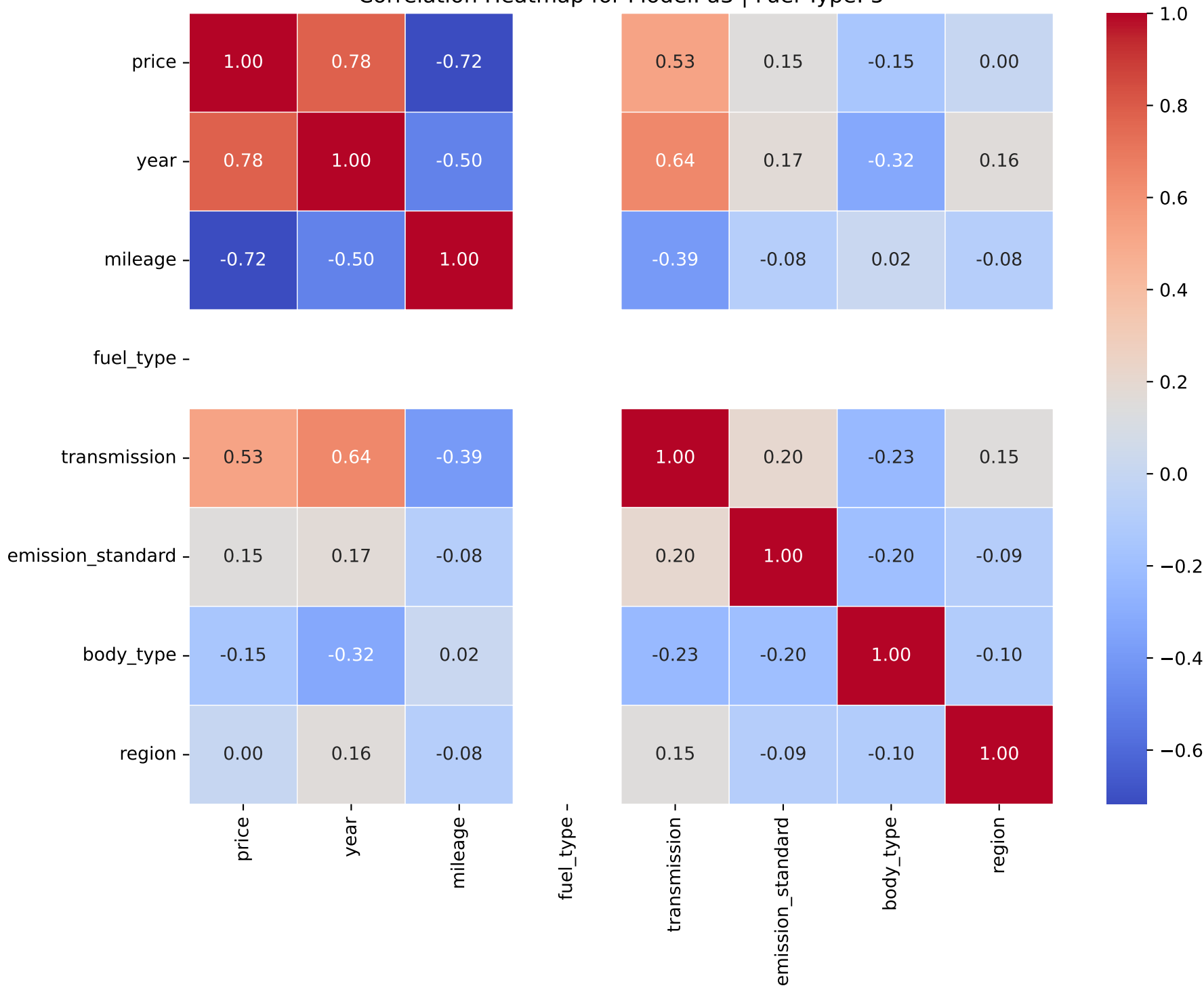
Correlation Heatmap for Model: a3 | Fuel Type: 5
