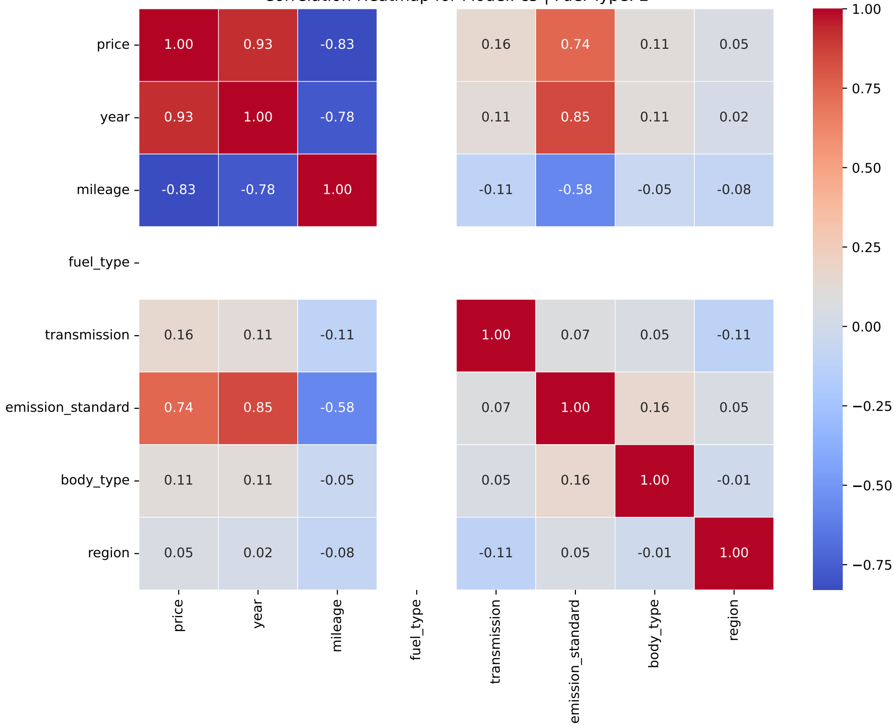
Correlation Heatmap for Model: c3 | Fuel Type: 2
