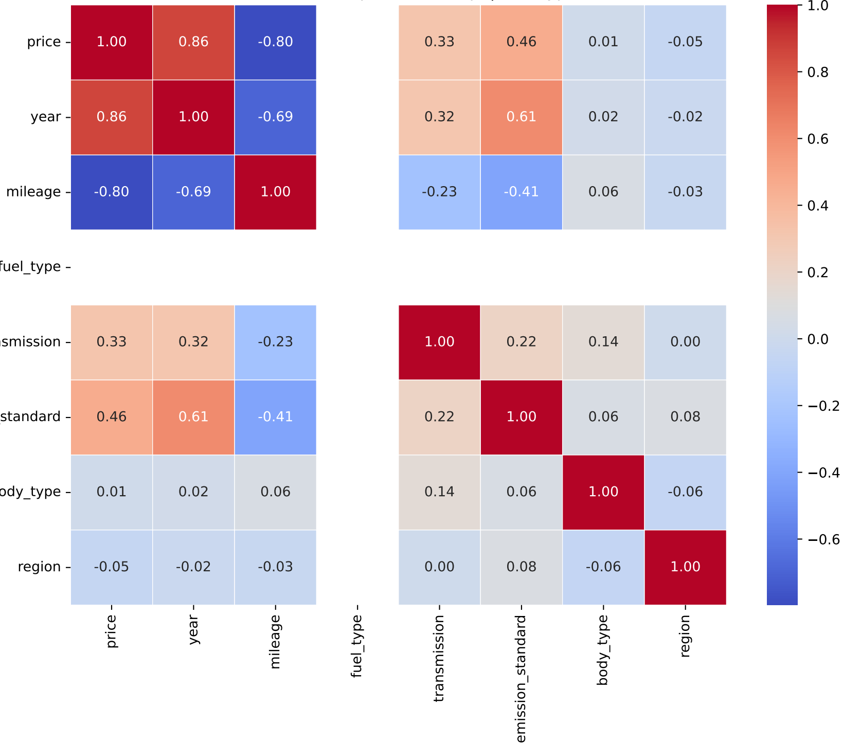
Correlation Heatmap for Model: q3 | Fuel Type: 1
