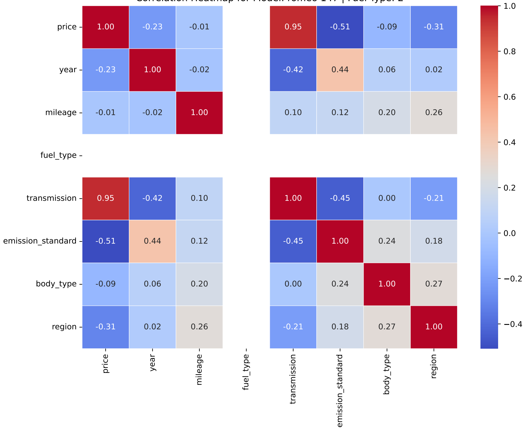
Correlation Heatmap for Model: romeo 147 | Fuel Type: 2
