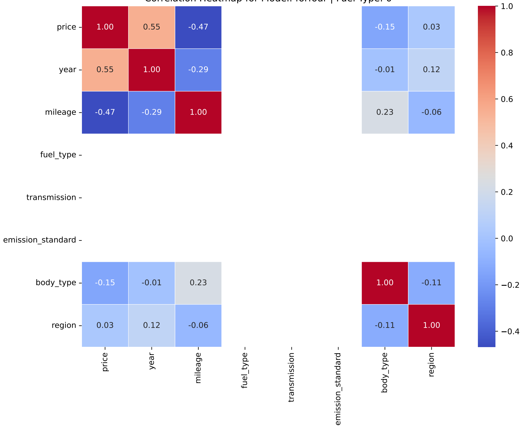
Correlation Heatmap for Model: forfour | Fuel Type: 0
