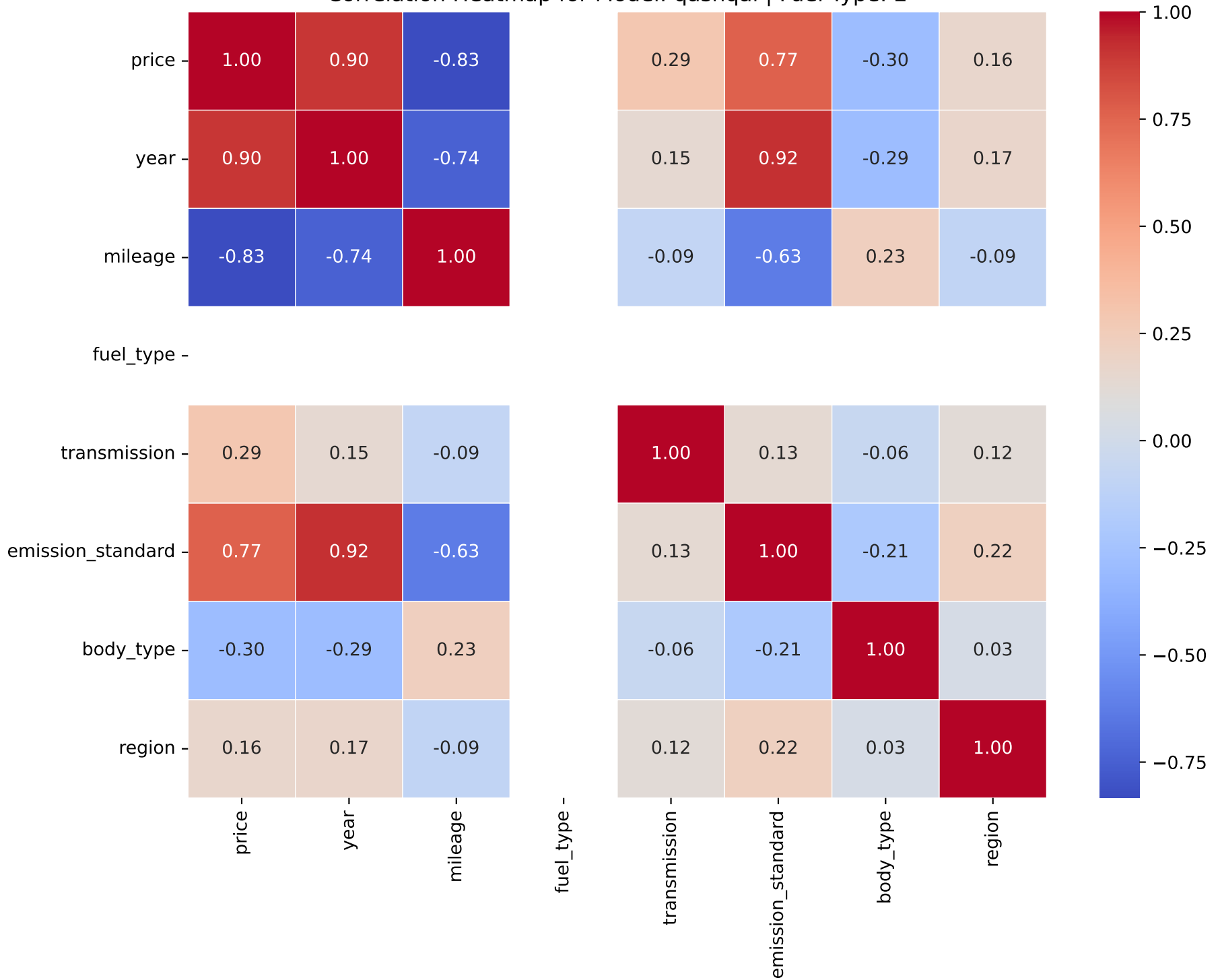
Correlation Heatmap for Model: qashqai | Fuel Type: 2
