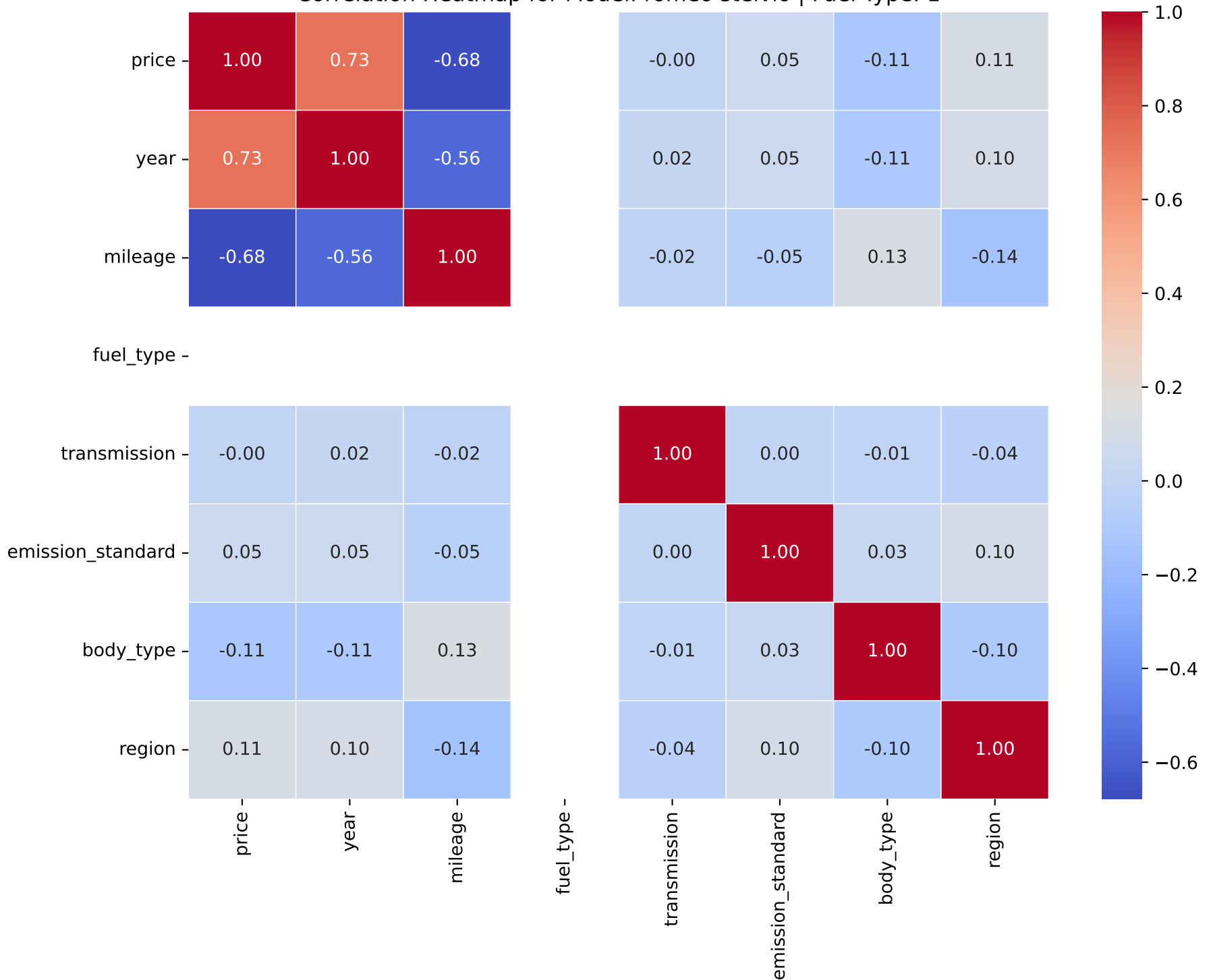
Correlation Heatmap for Model: romeo stelvio | Fuel Type: 1
