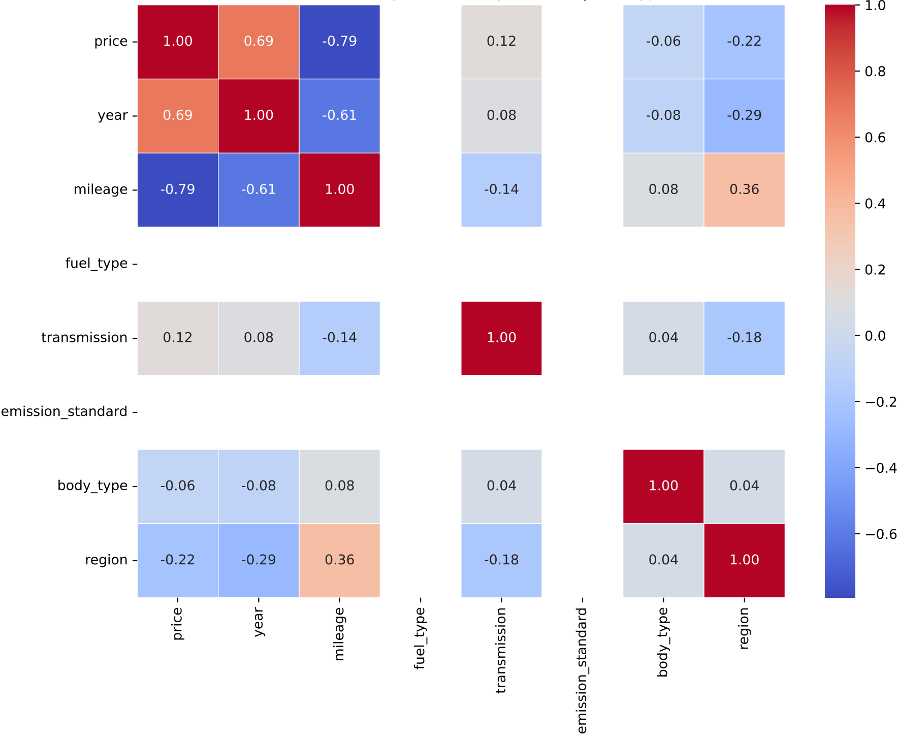
Correlation Heatmap for Model: grandland | Fuel Type: 1
