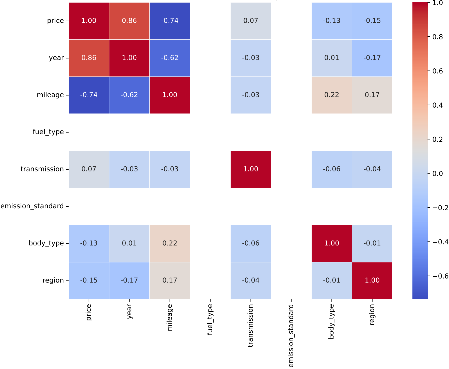
Correlation Heatmap for Model: x3 | Fuel Type: 3
