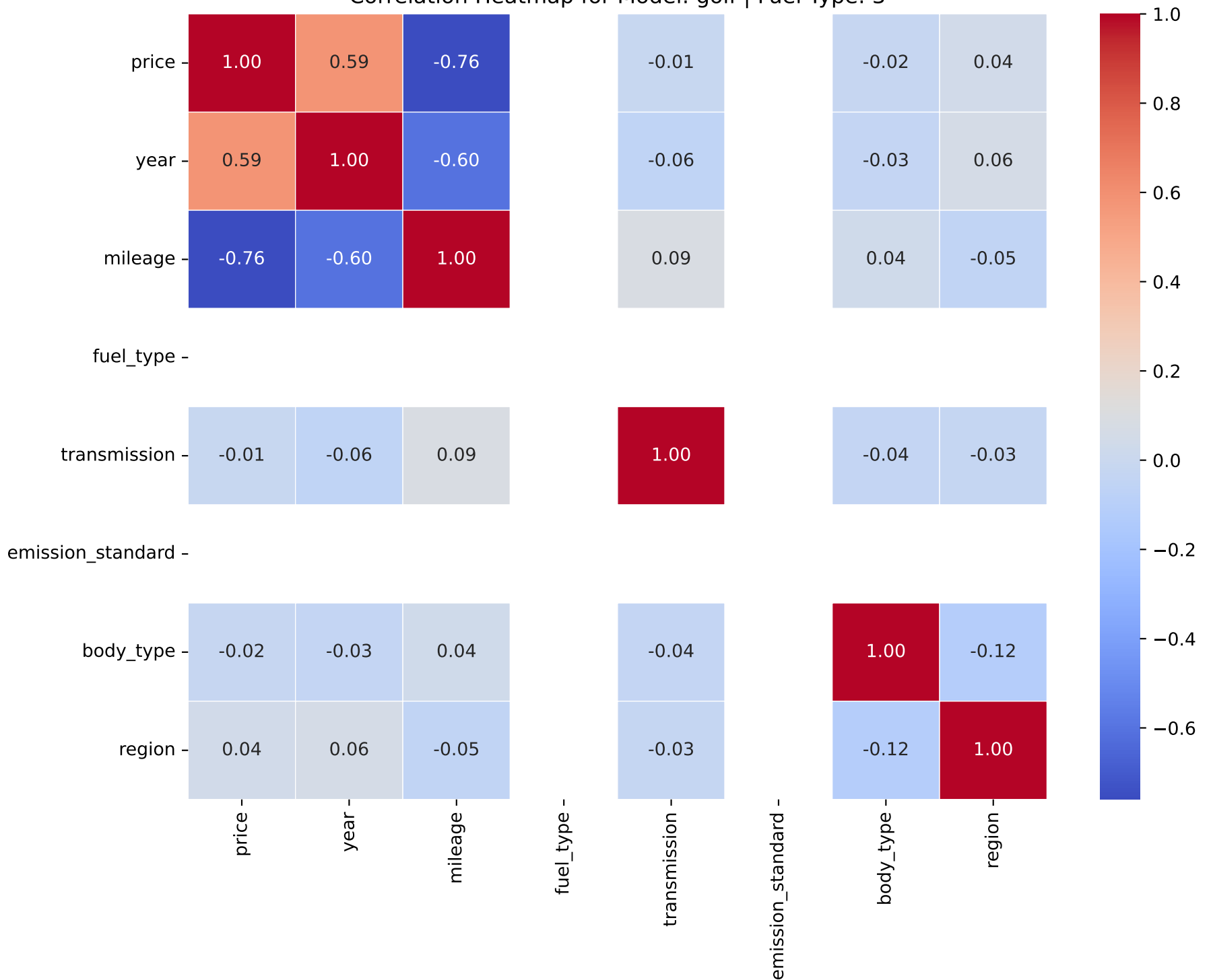
Correlation Heatmap for Model: golf | Fuel Type: 3
