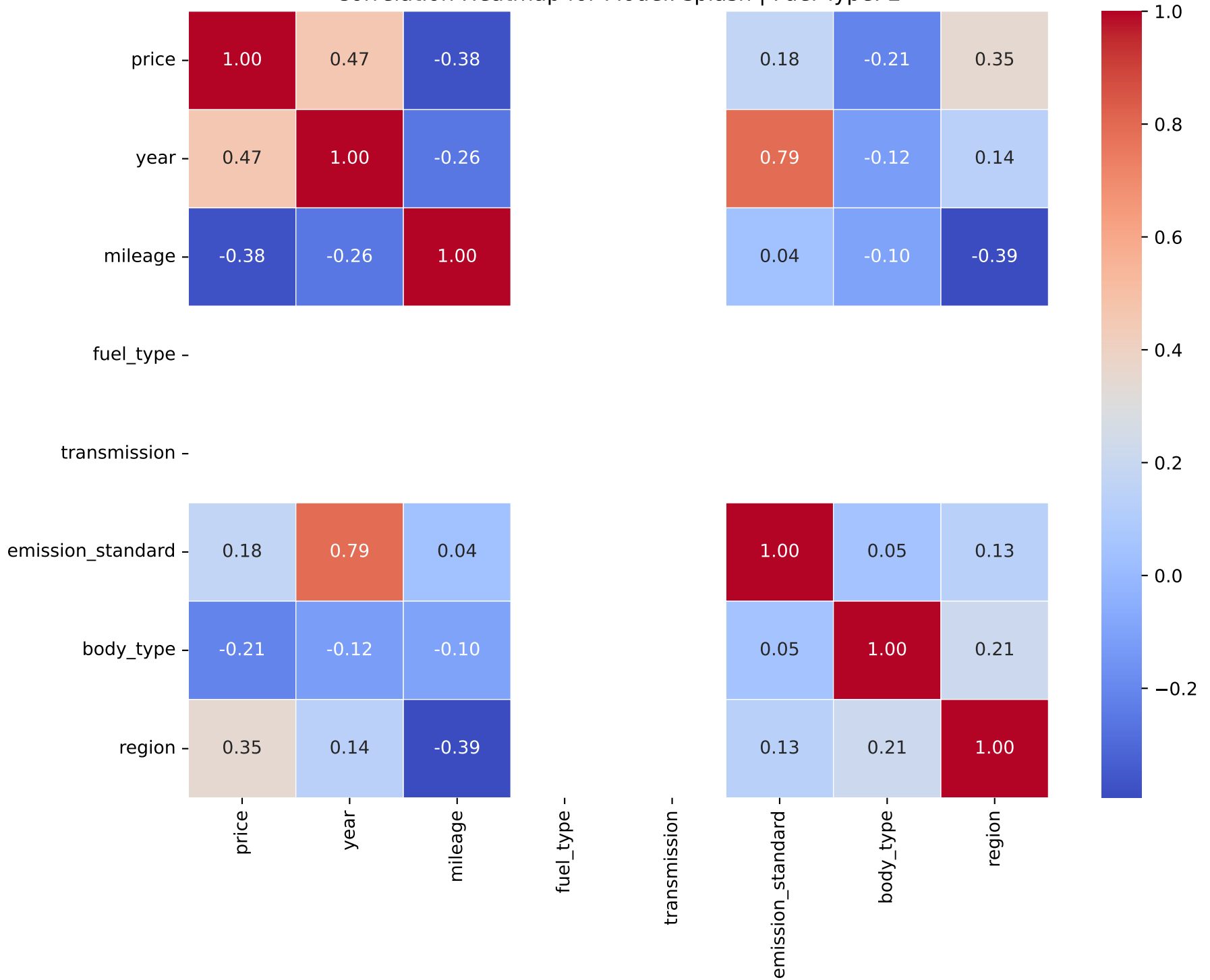
Correlation Heatmap for Model: splash | Fuel Type: 2
