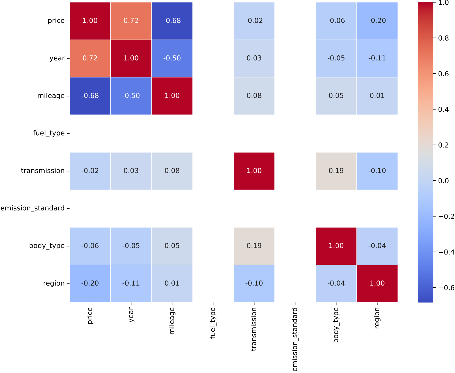
Correlation Heatmap for Model: q5 | Fuel Type: 3
