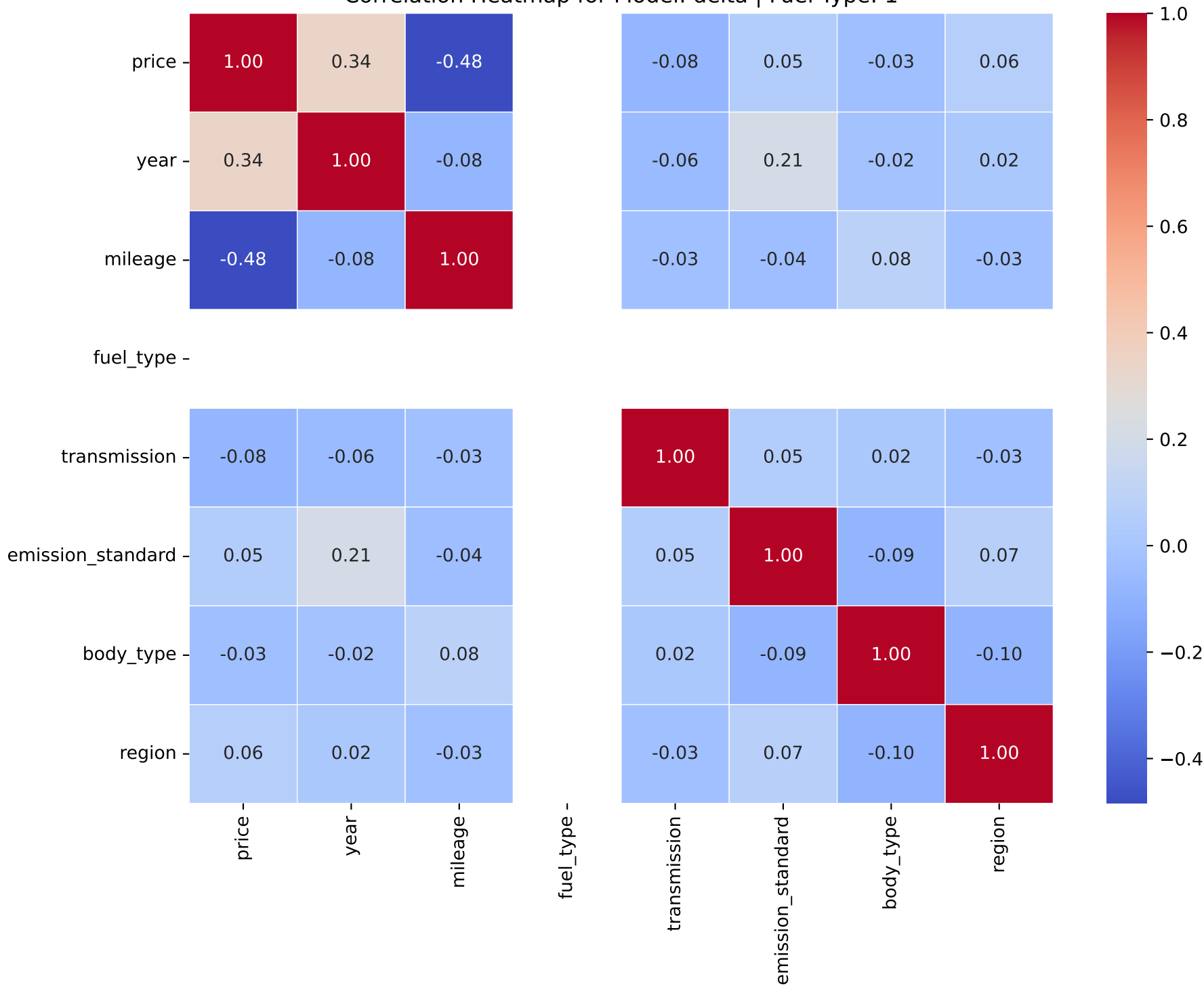
Correlation Heatmap for Model: delta | Fuel Type: 1
