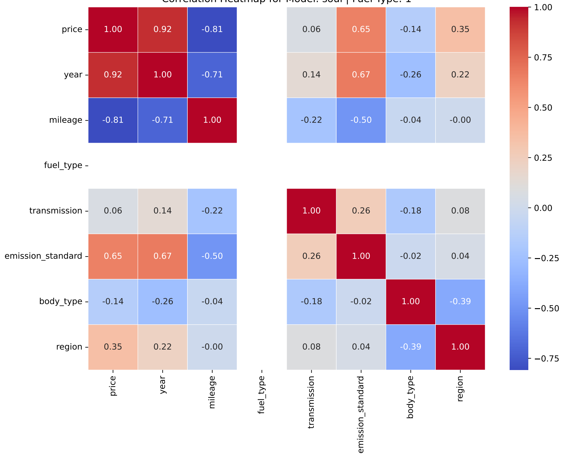
Correlation Heatmap for Model: soul | Fuel Type: 1
