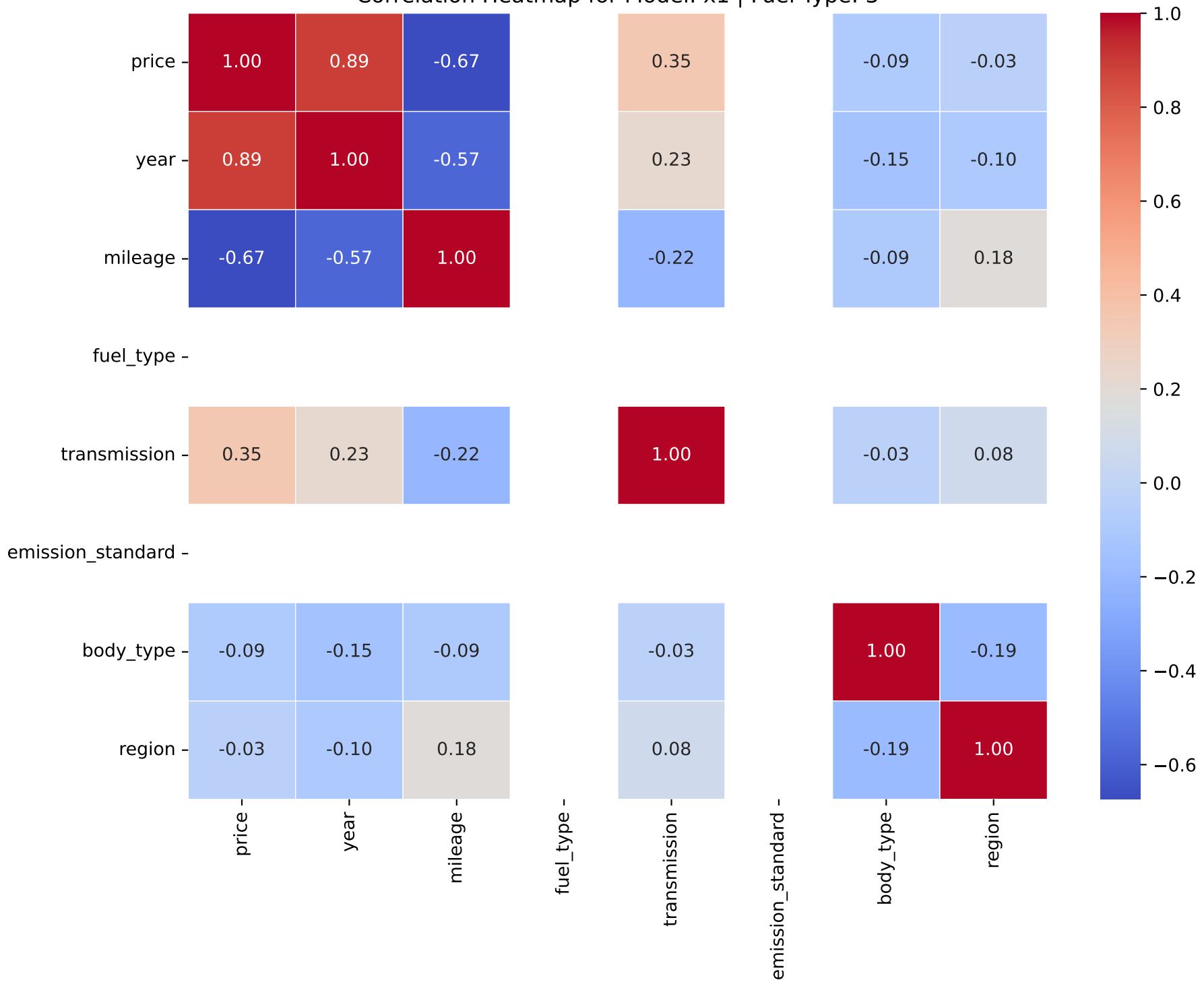
Correlation Heatmap for Model: x1 | Fuel Type: 3
