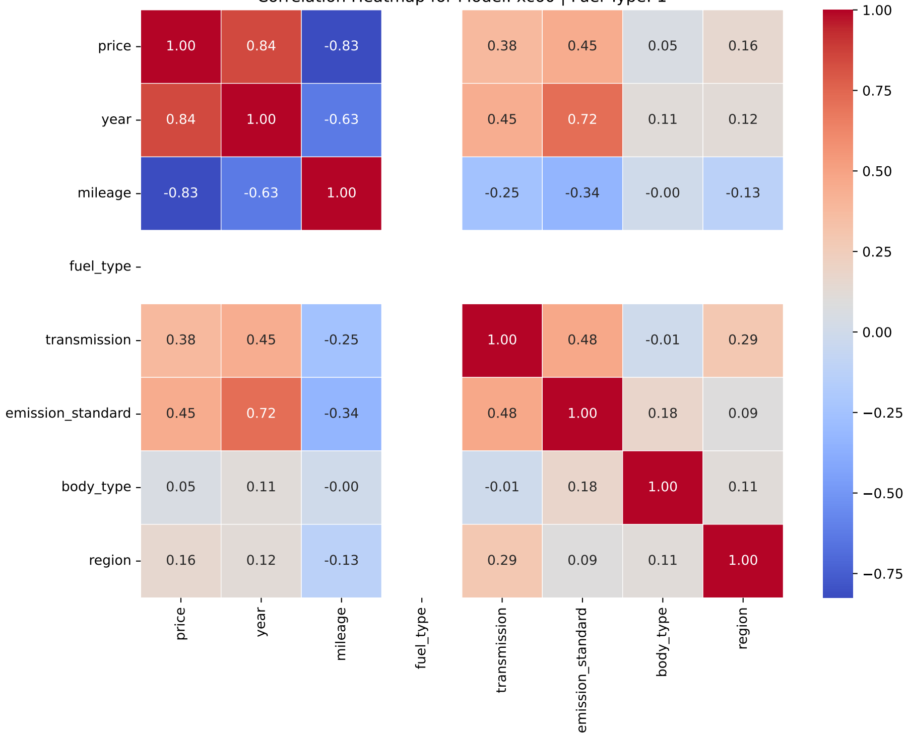
Correlation Heatmap for Model: xc60 | Fuel Type: 1
