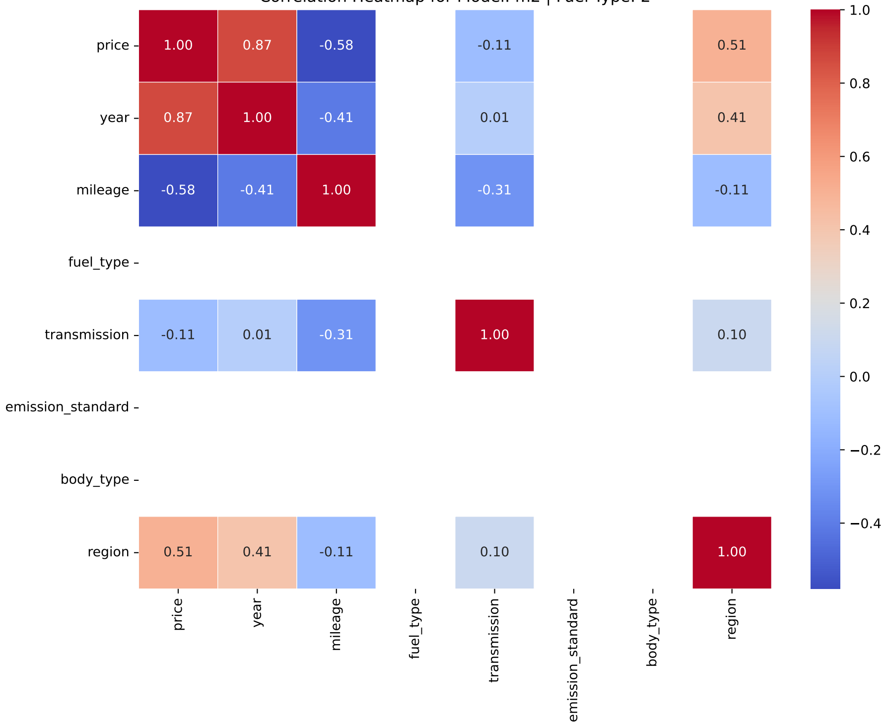
Correlation Heatmap for Model: m2 | Fuel Type: 2
