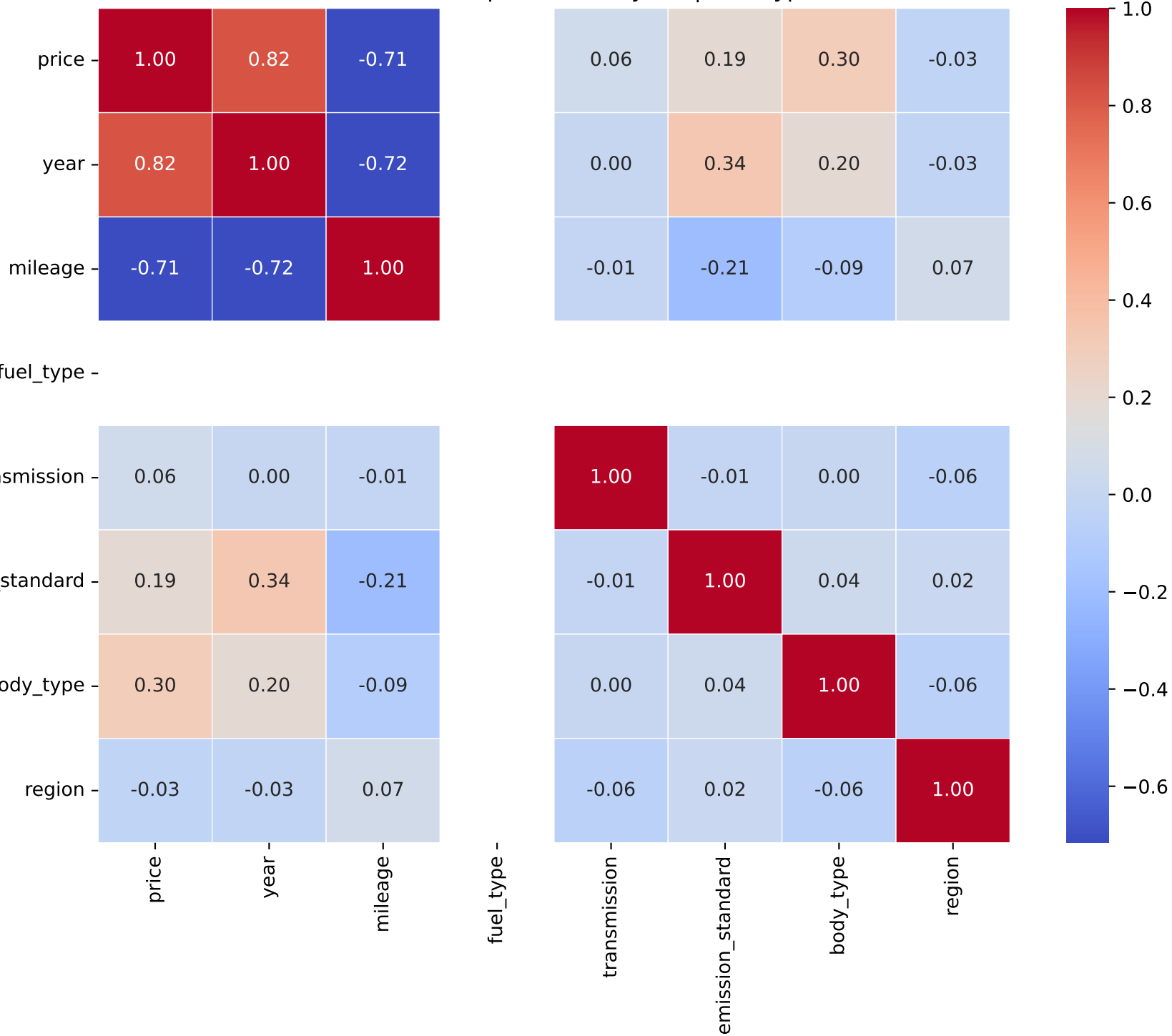
Correlation Heatmap for Model: yaris | Fuel Type: 3
