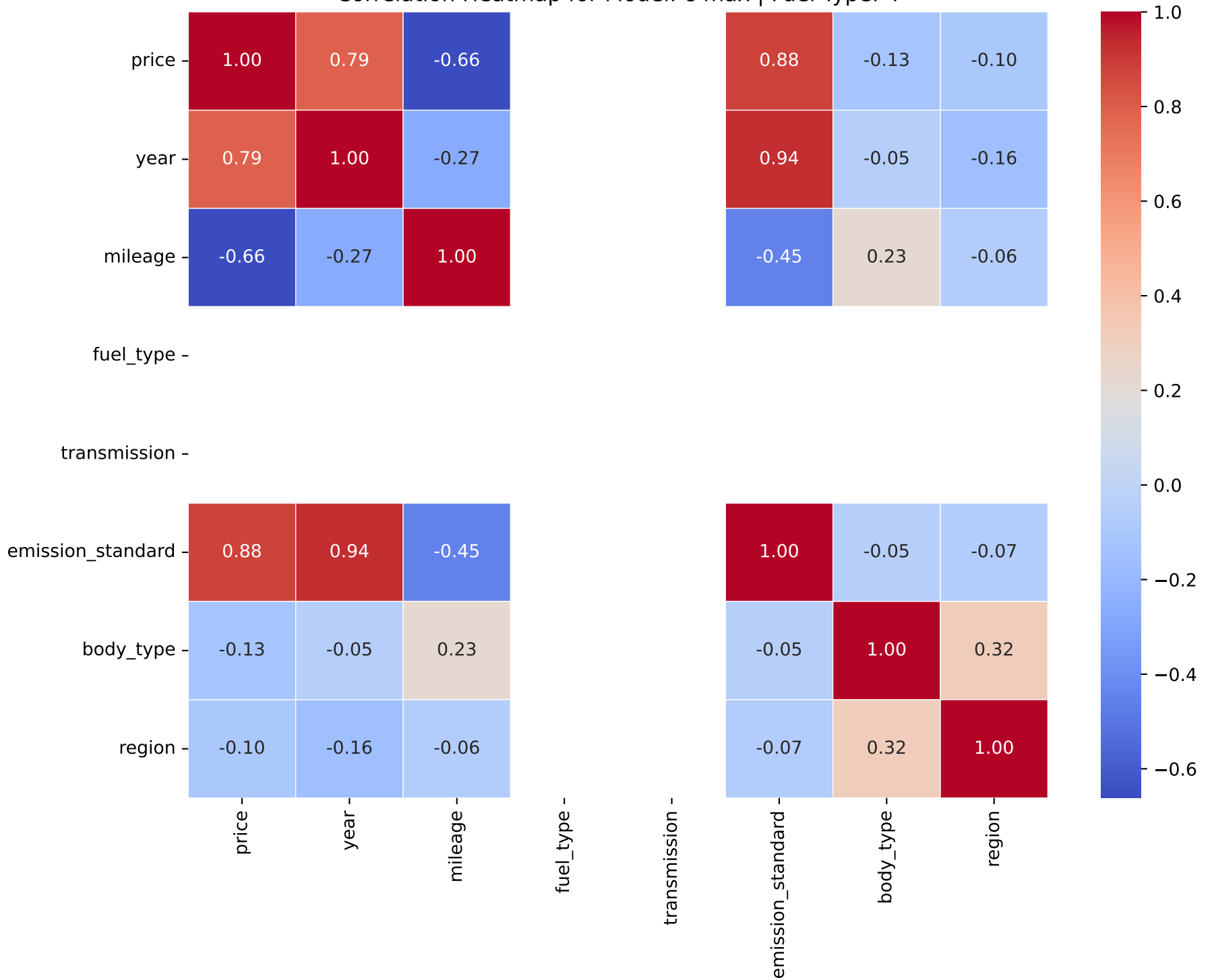
Correlation Heatmap for Model: c-max | Fuel Type: 4
