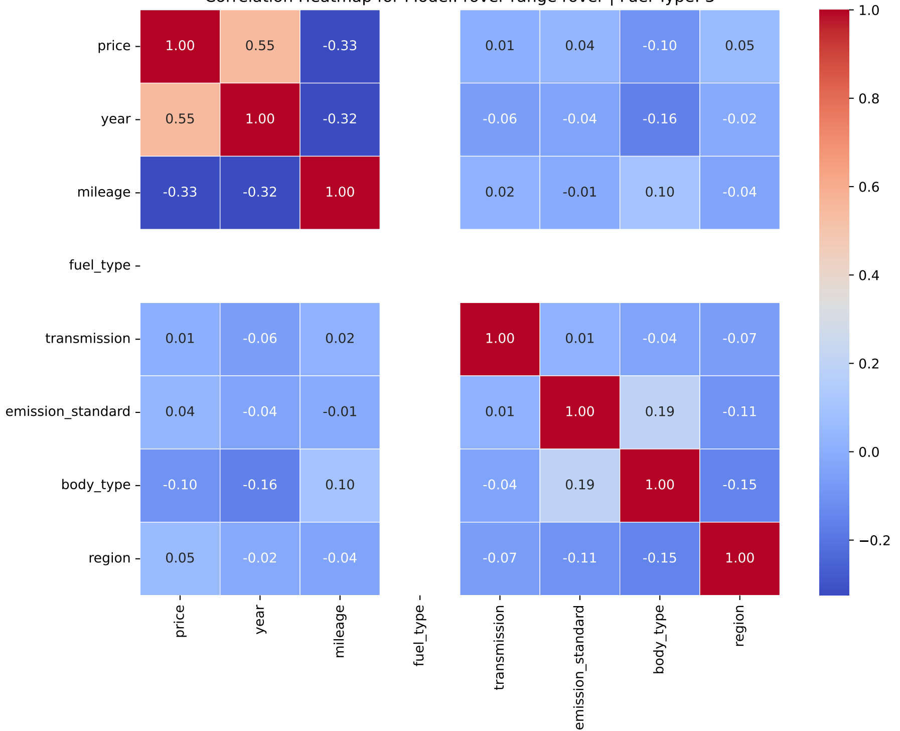
Correlation Heatmap for Model: rover range rover | Fuel Type: 3
