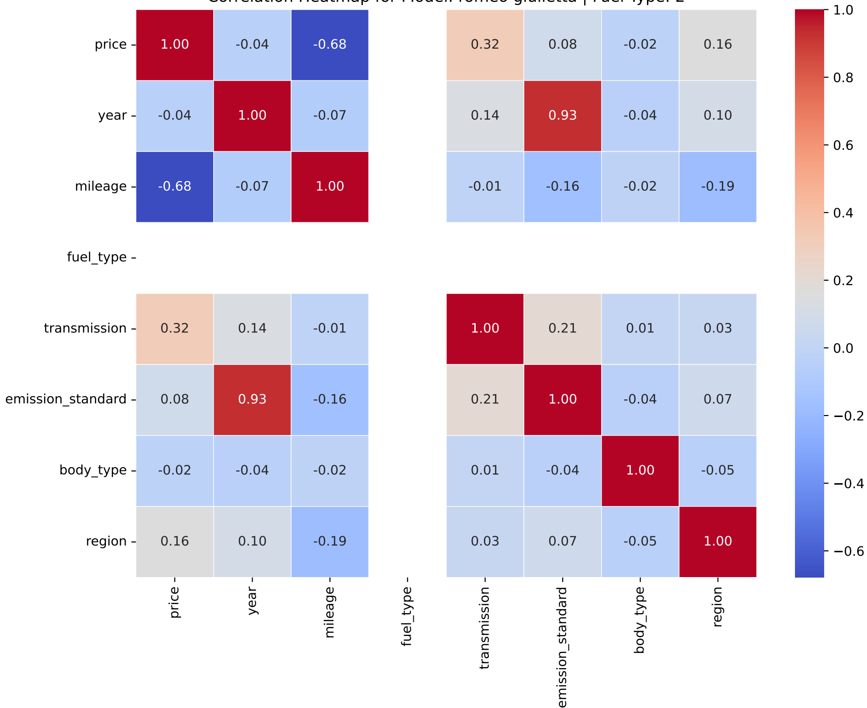
Correlation Heatmap for Model: romeo giulietta | Fuel Type: 2
