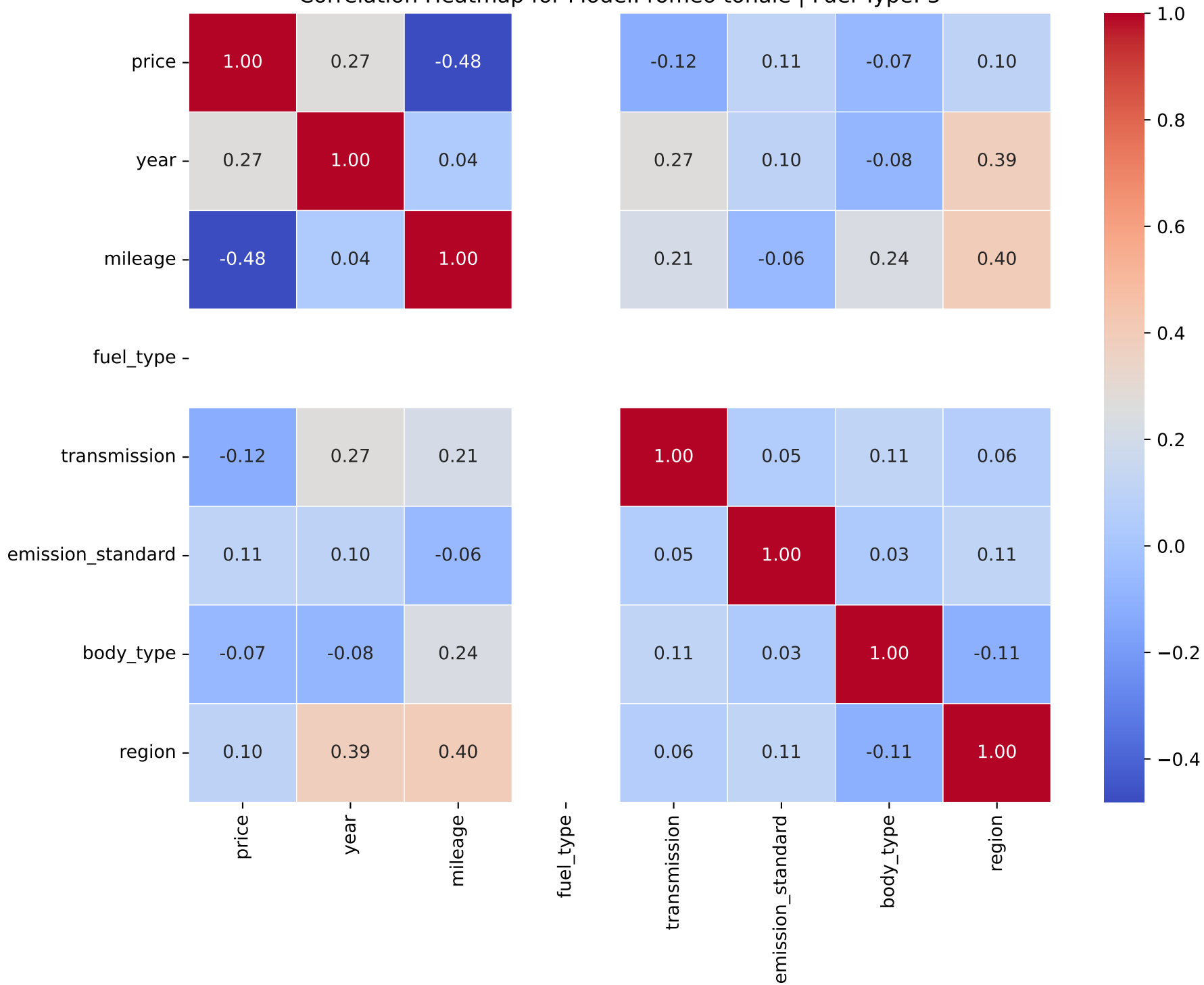
Correlation Heatmap for Model: romeo tonale | Fuel Type: 3
