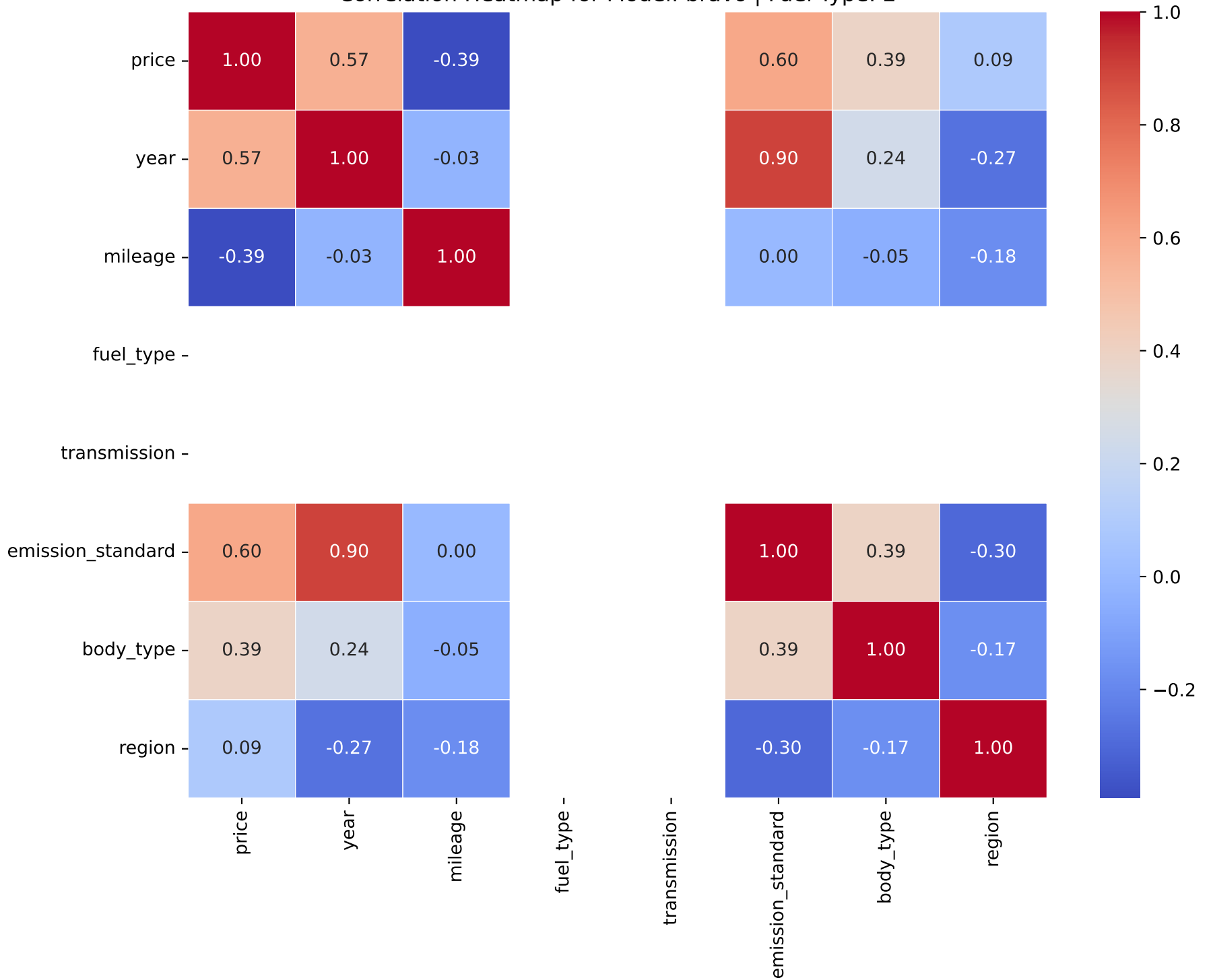
Correlation Heatmap for Model: bravo | Fuel Type: 2
