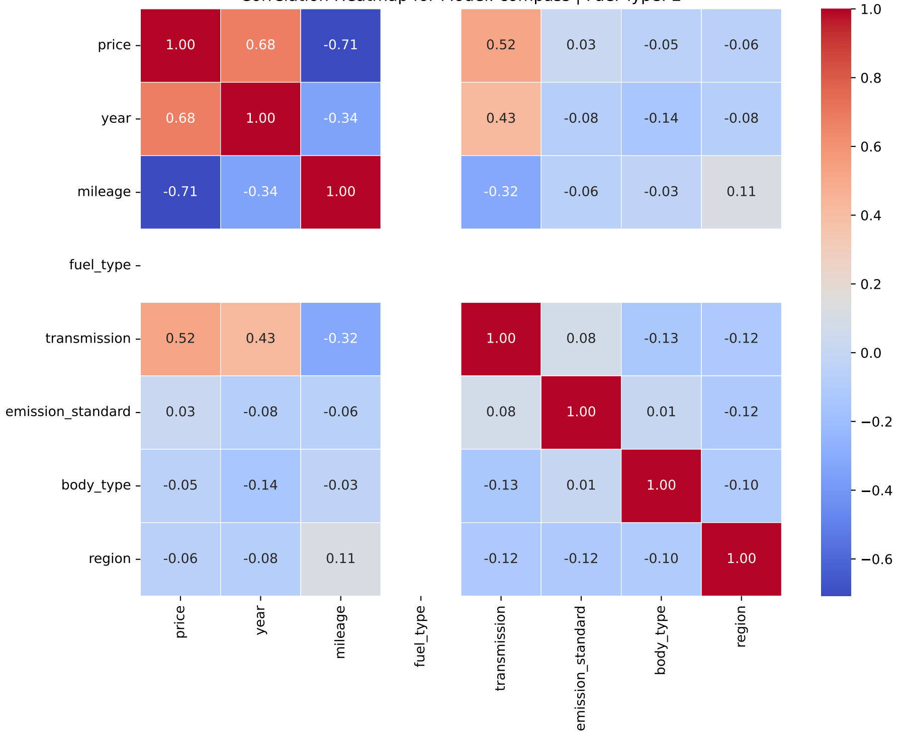
Correlation Heatmap for Model: compass | Fuel Type: 2
