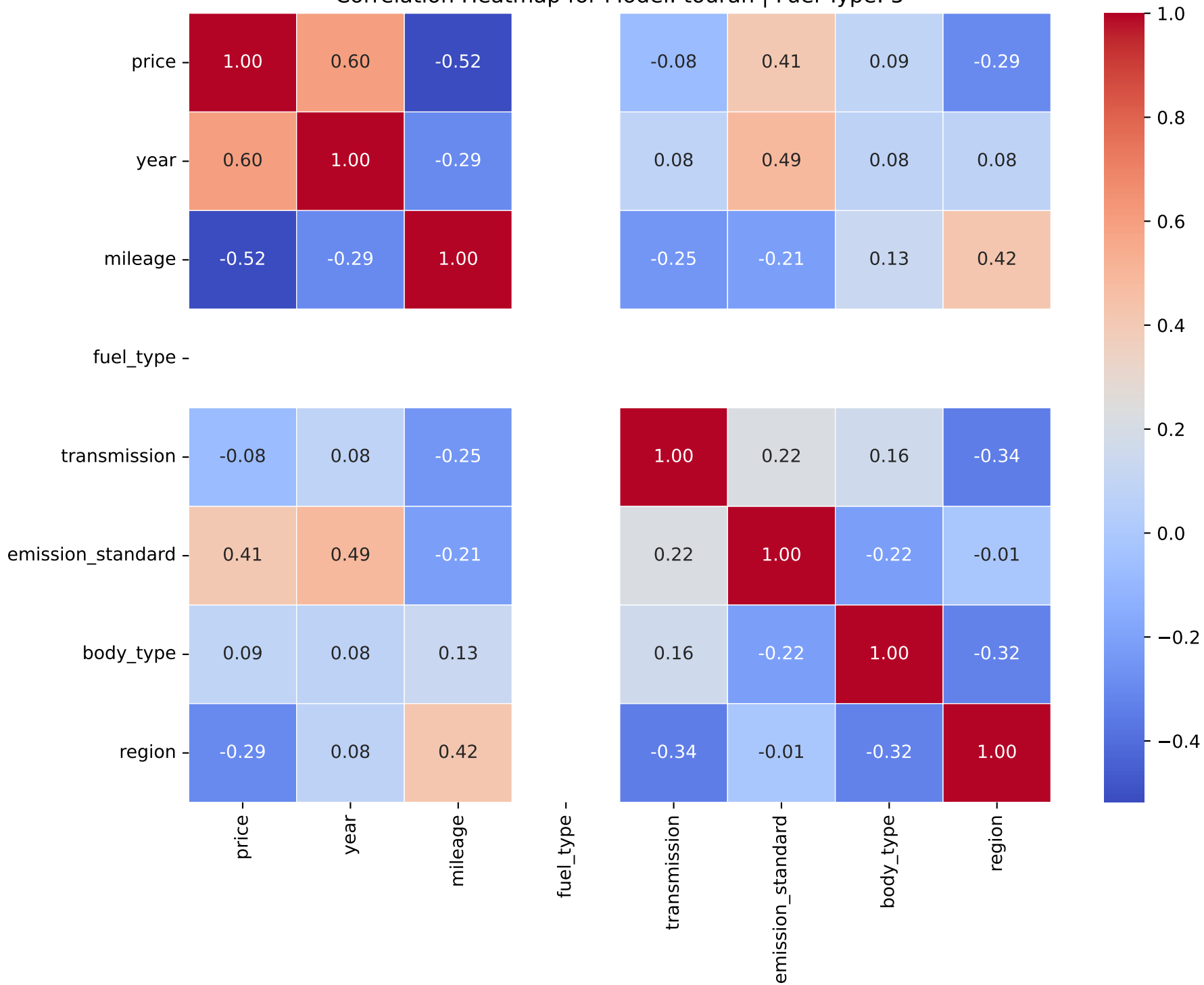
Correlation Heatmap for Model: touran | Fuel Type: 5
