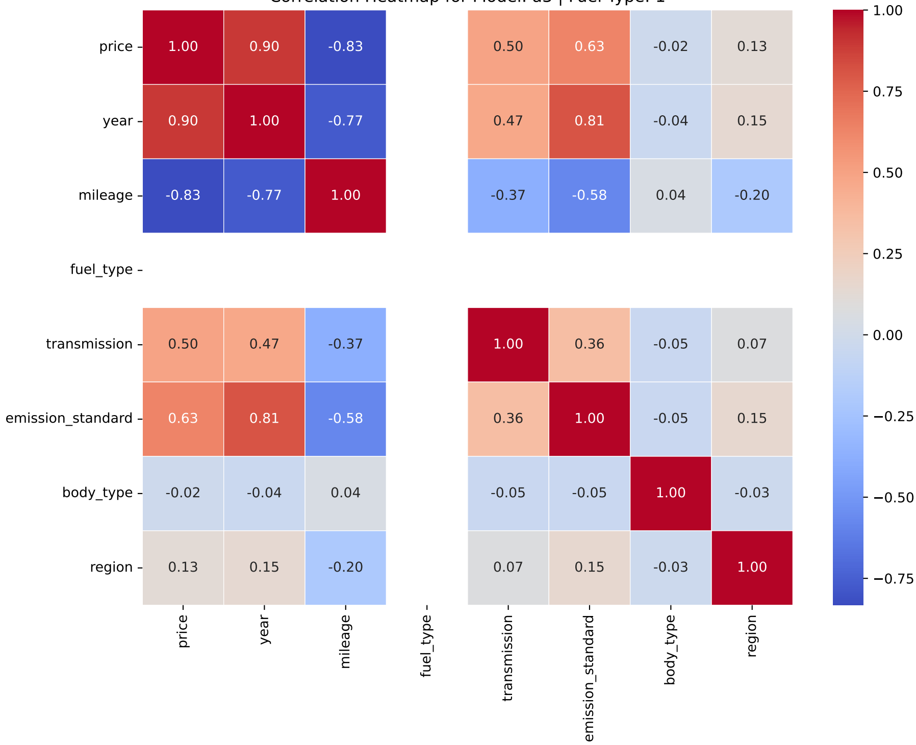
Correlation Heatmap for Model: a3 | Fuel Type: 1
