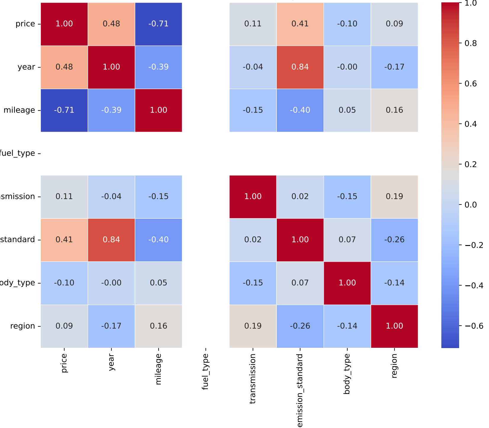
Correlation Heatmap for Model: antara | Fuel Type: 1
