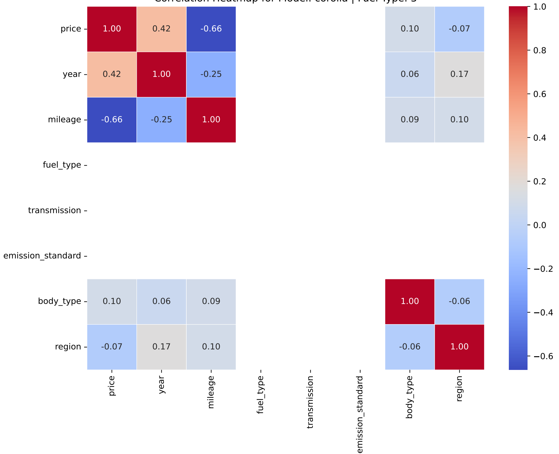
Correlation Heatmap for Model: corolla | Fuel Type: 3
