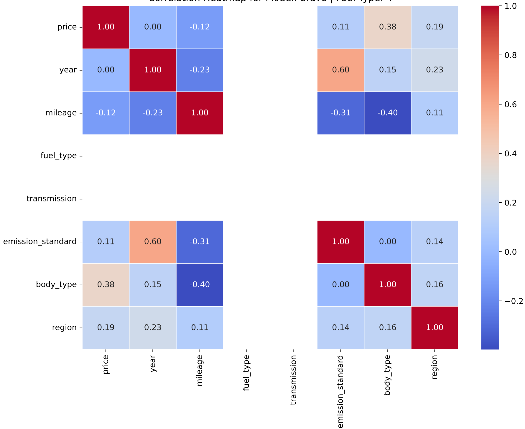
Correlation Heatmap for Model: bravo | Fuel Type: 4
