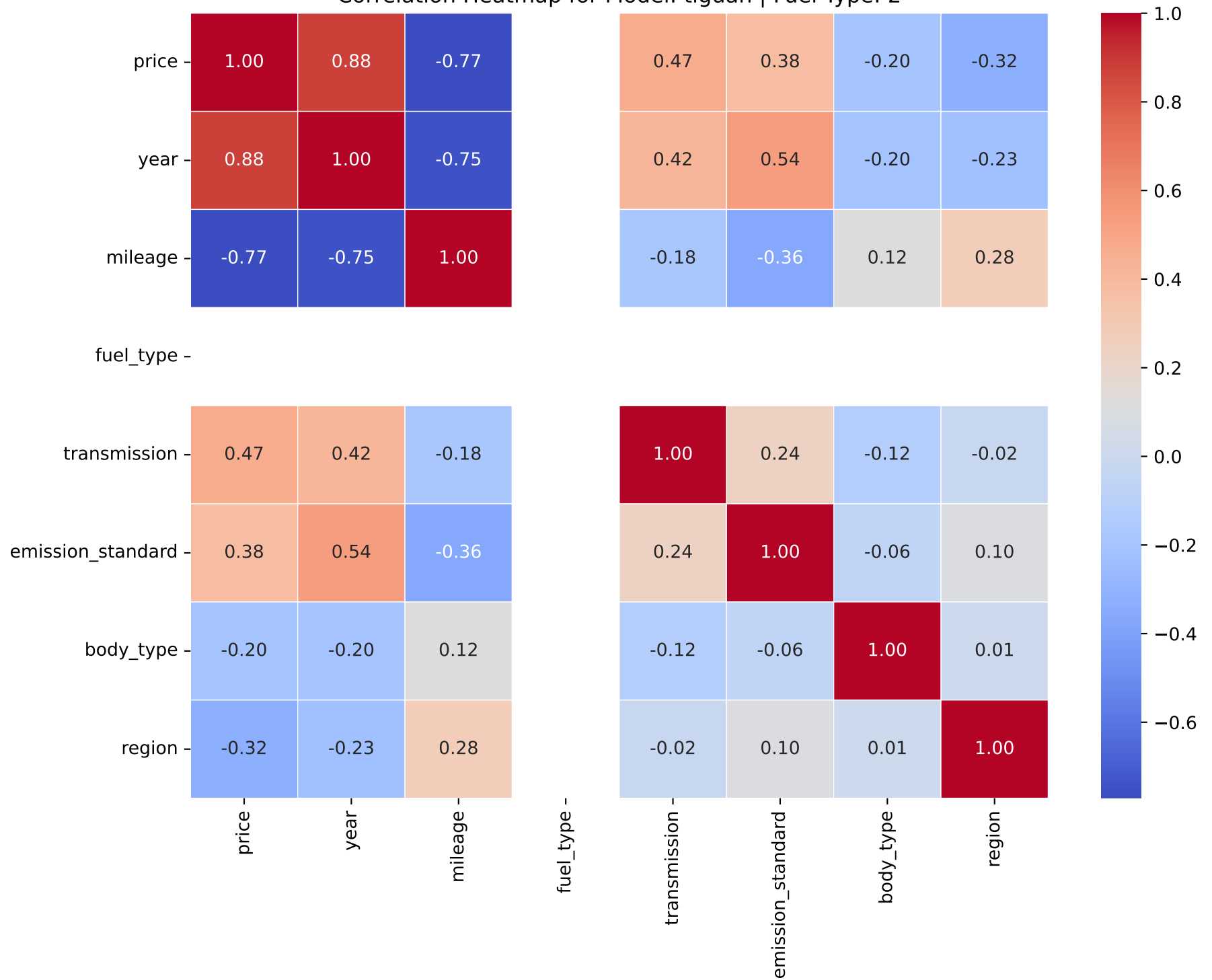
Correlation Heatmap for Model: tiguan | Fuel Type: 2
