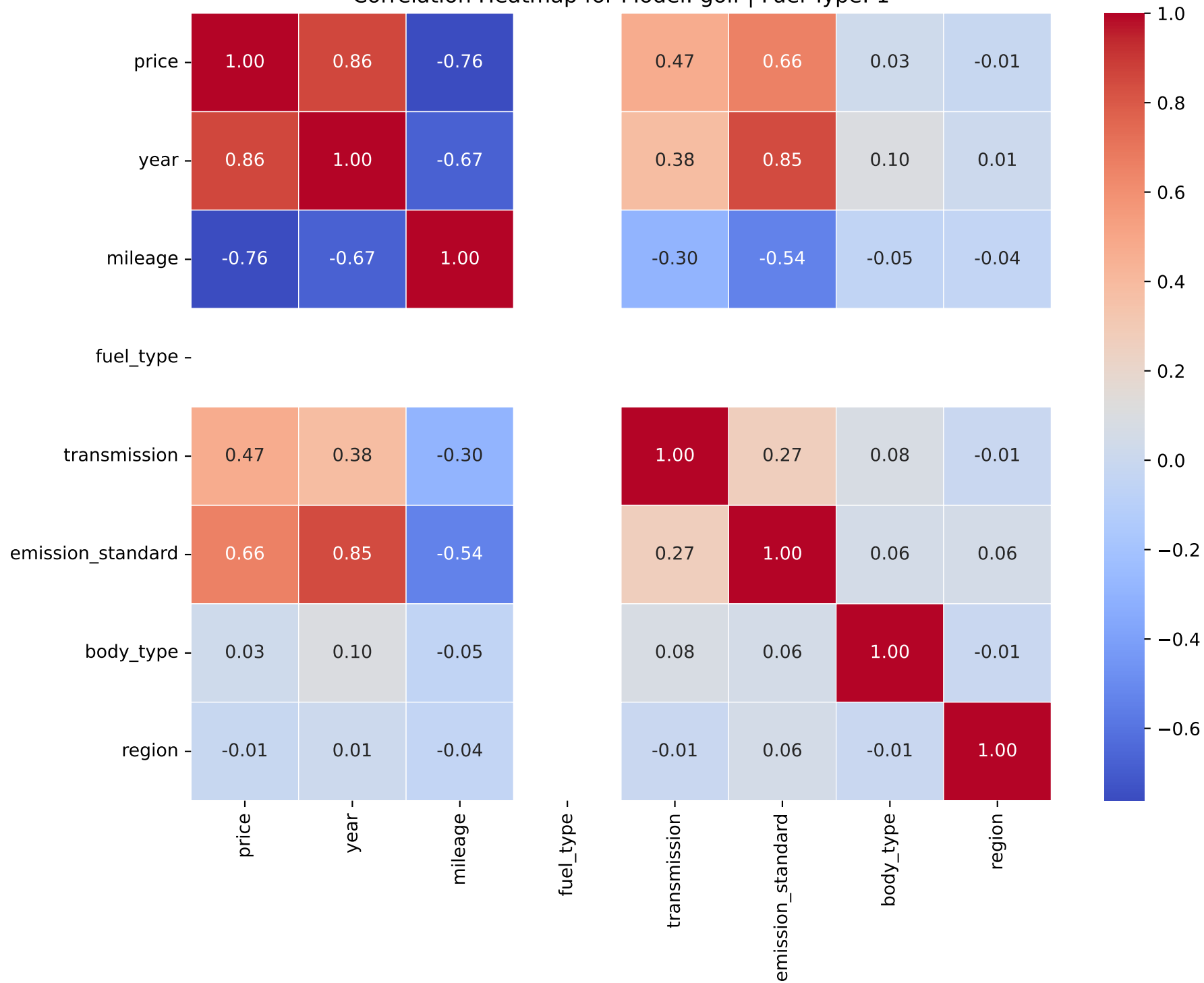
Correlation Heatmap for Model: golf | Fuel Type: 1
