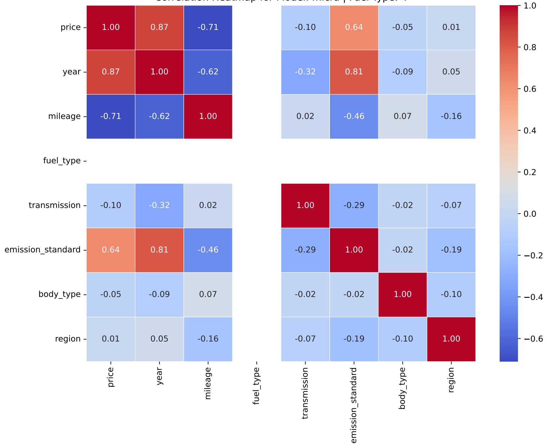
Correlation Heatmap for Model: micra | Fuel Type: 4
