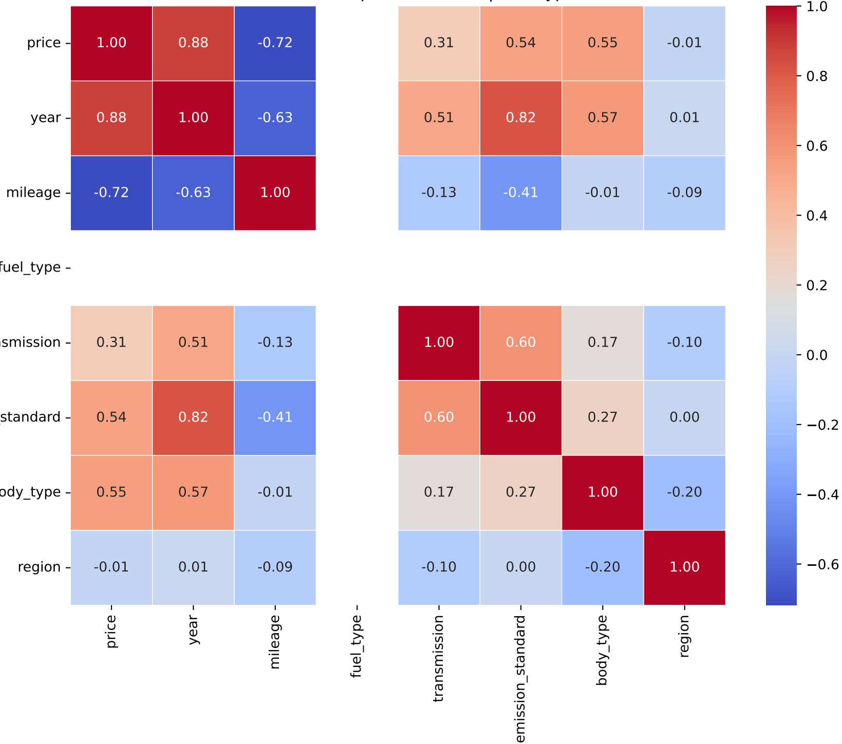
Correlation Heatmap for Model: s3 | Fuel Type: 2
