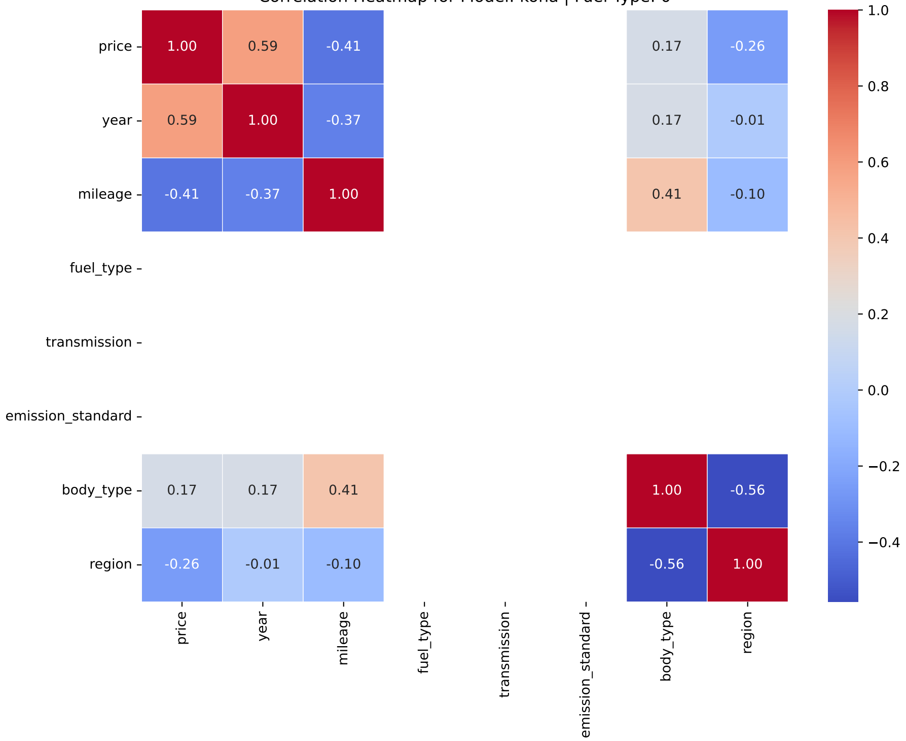
Correlation Heatmap for Model: kona | Fuel Type: 0
