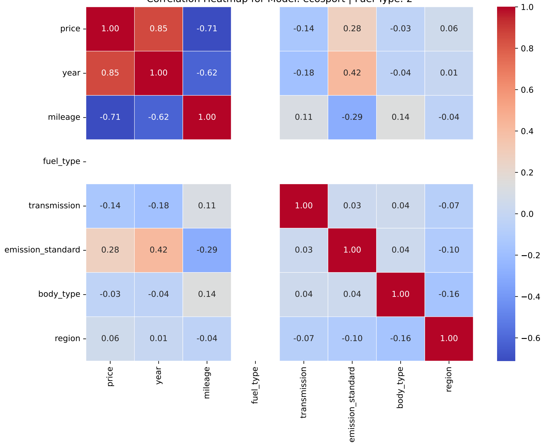
Correlation Heatmap for Model: ecosport | Fuel Type: 2
