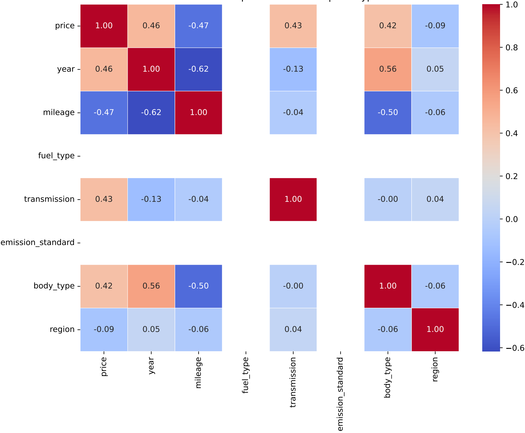
Correlation Heatmap for Model: 5008 | Fuel Type: 2
