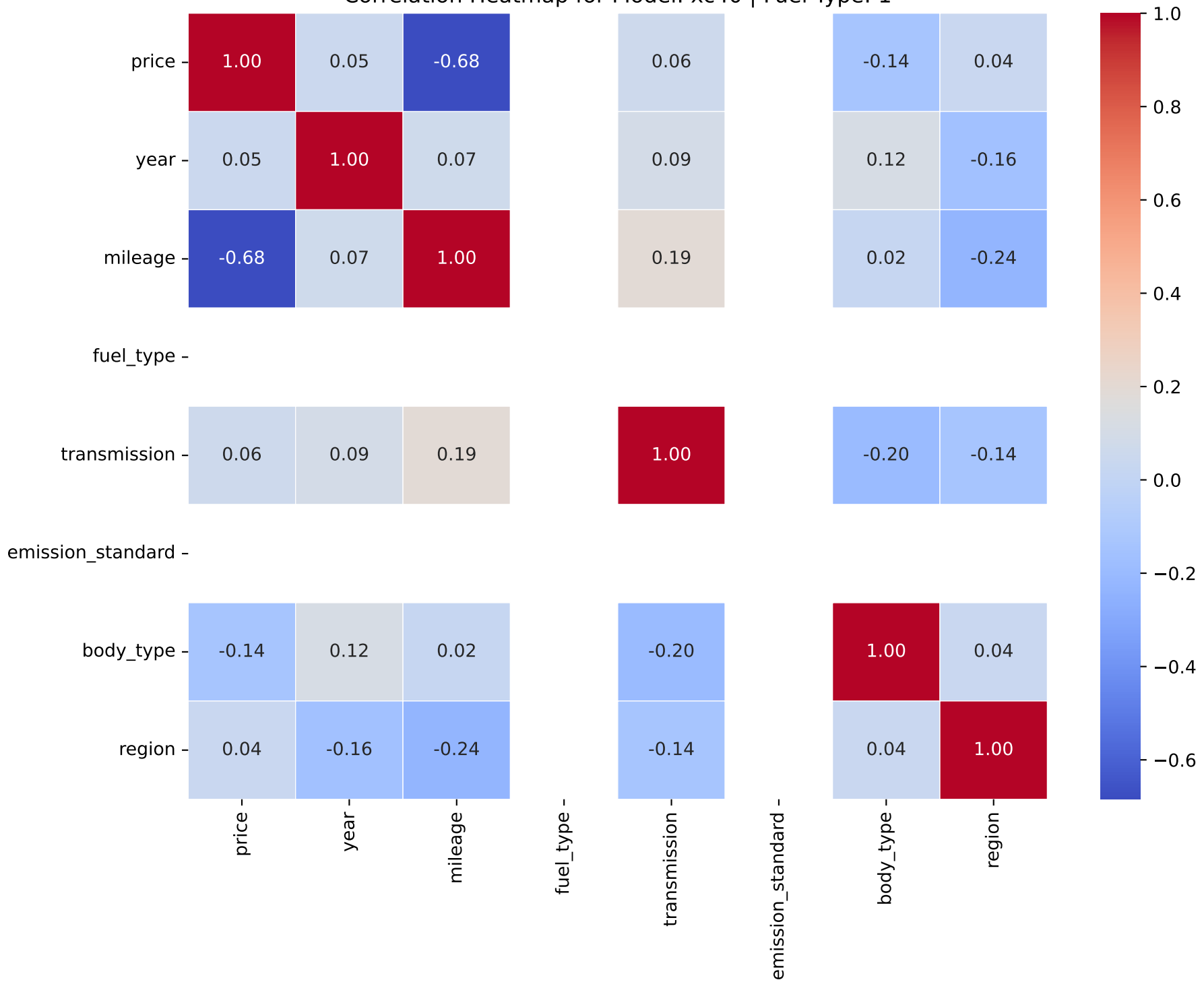
Correlation Heatmap for Model: xc40 | Fuel Type: 1
