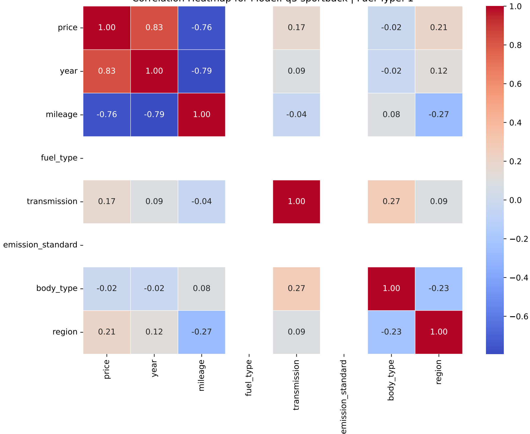
Correlation Heatmap for Model: q3 sportback | Fuel Type: 1
