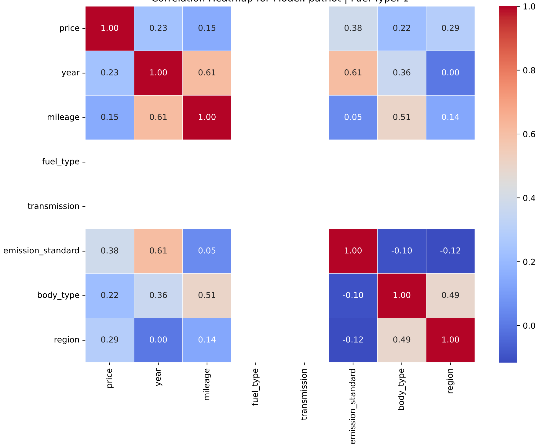
Correlation Heatmap for Model: patriot | Fuel Type: 1
