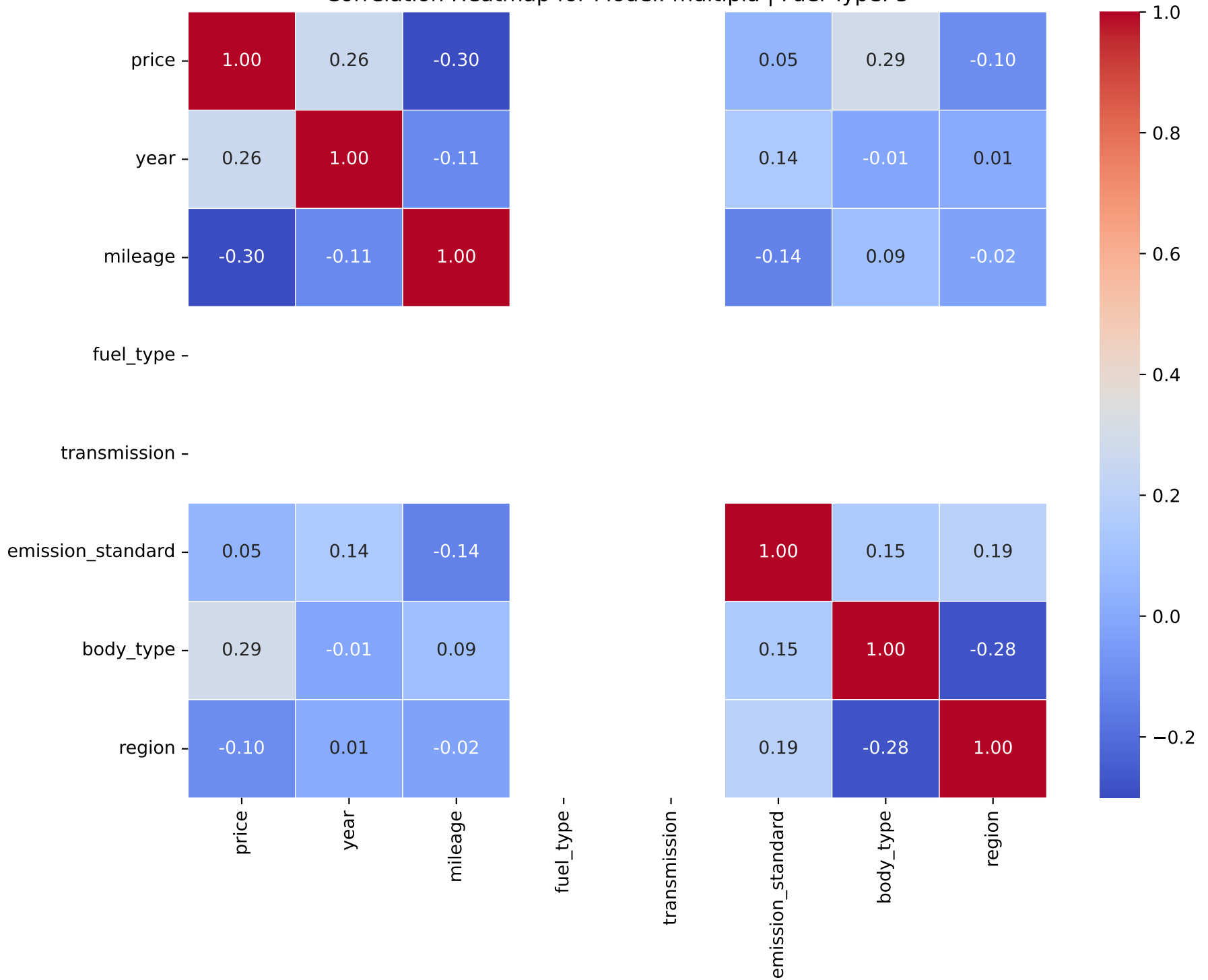
Correlation Heatmap for Model: multipla | Fuel Type: 5
