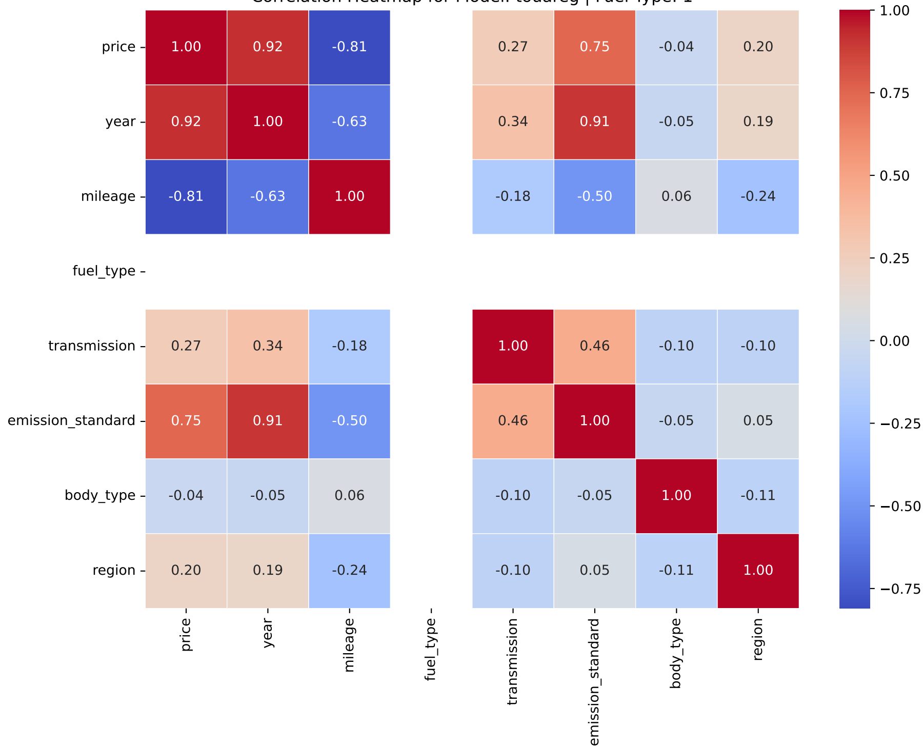
Correlation Heatmap for Model: touareg | Fuel Type: 1
