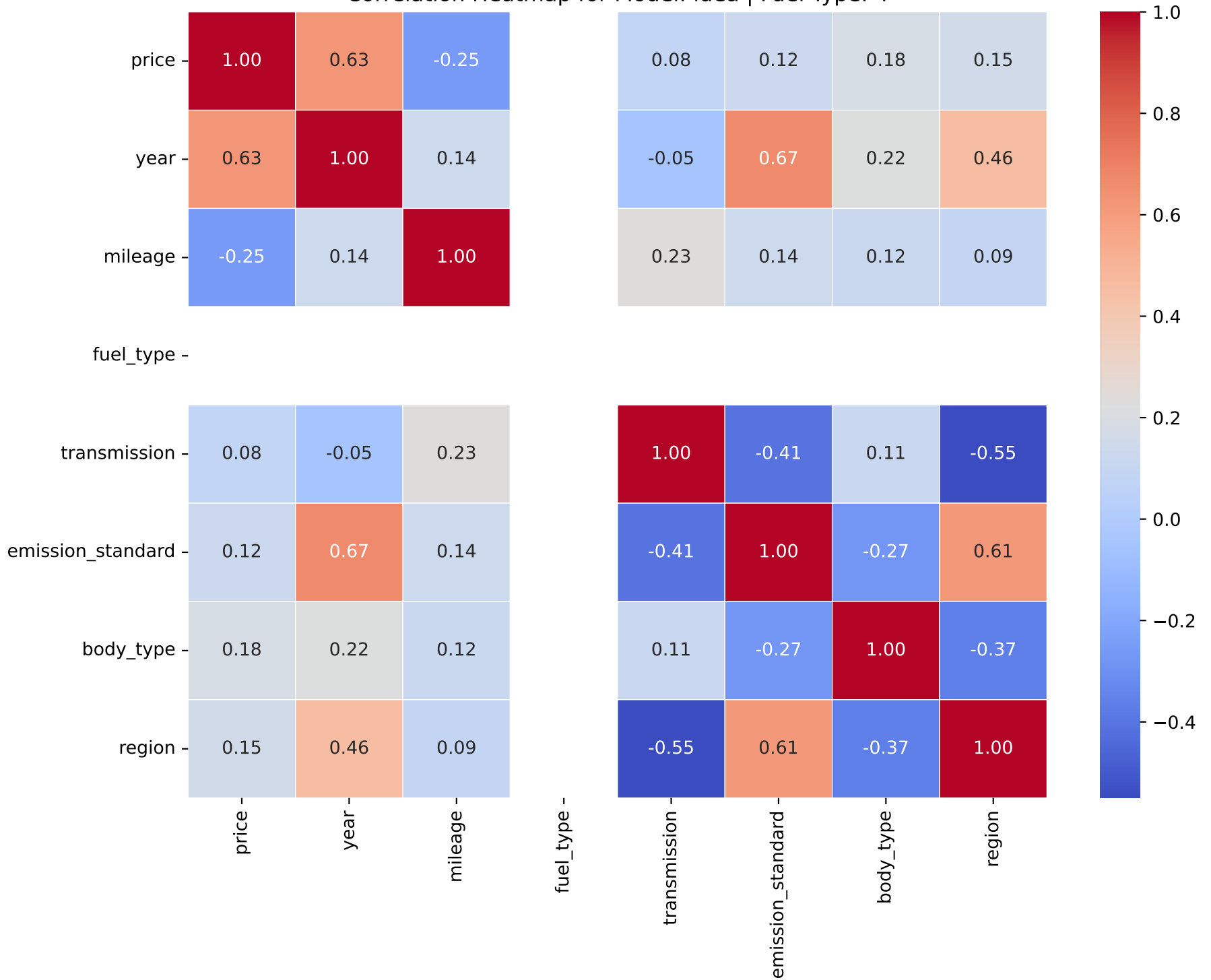
Correlation Heatmap for Model: idea | Fuel Type: 4
