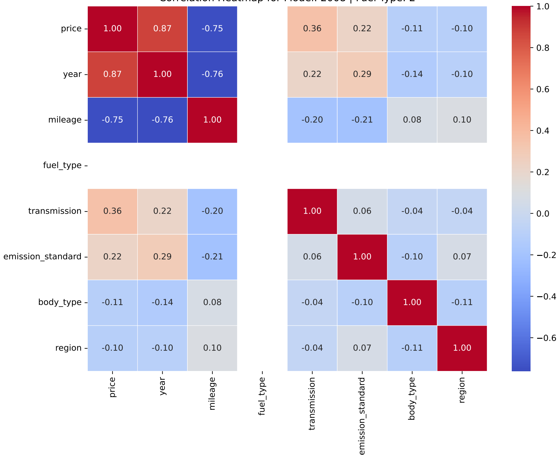
Correlation Heatmap for Model: 2008 | Fuel Type: 2
