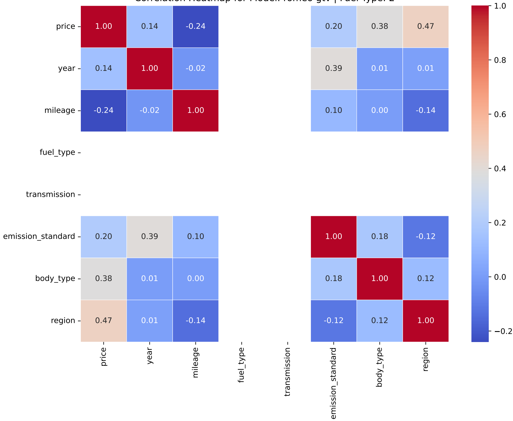
Correlation Heatmap for Model: romeo gtv | Fuel Type: 2
