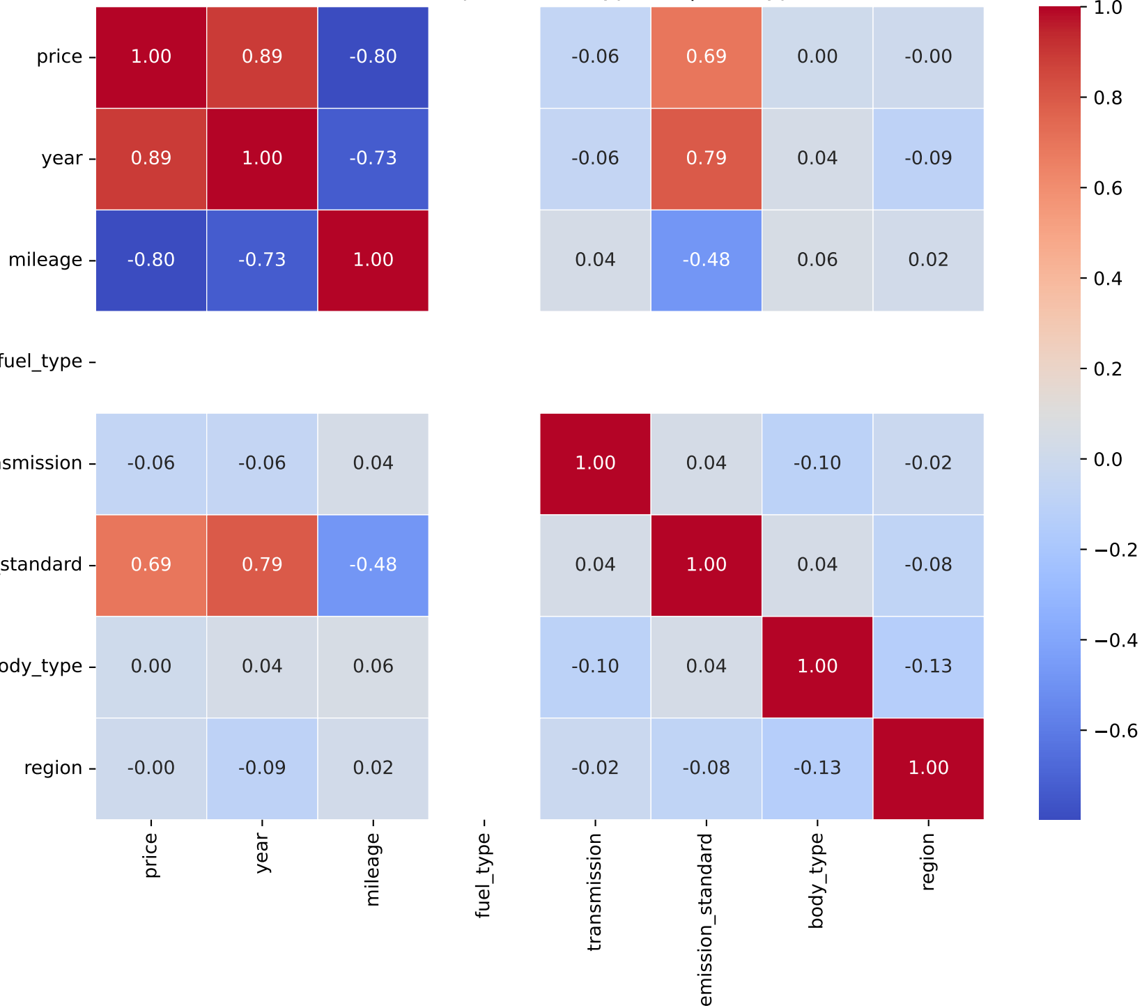
Correlation Heatmap for Model: ypsilon | Fuel Type: 4
