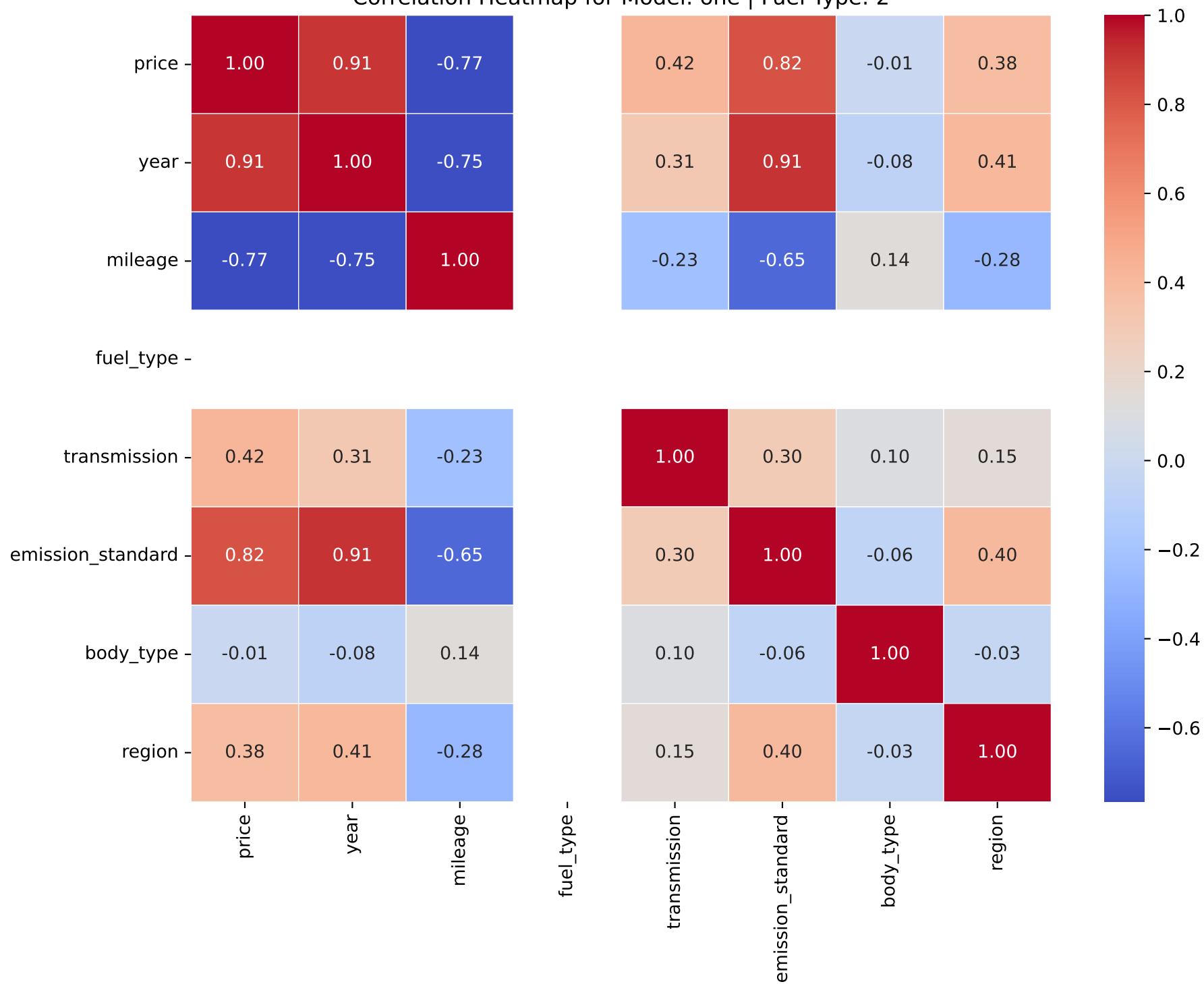
Correlation Heatmap for Model: one | Fuel Type: 2
