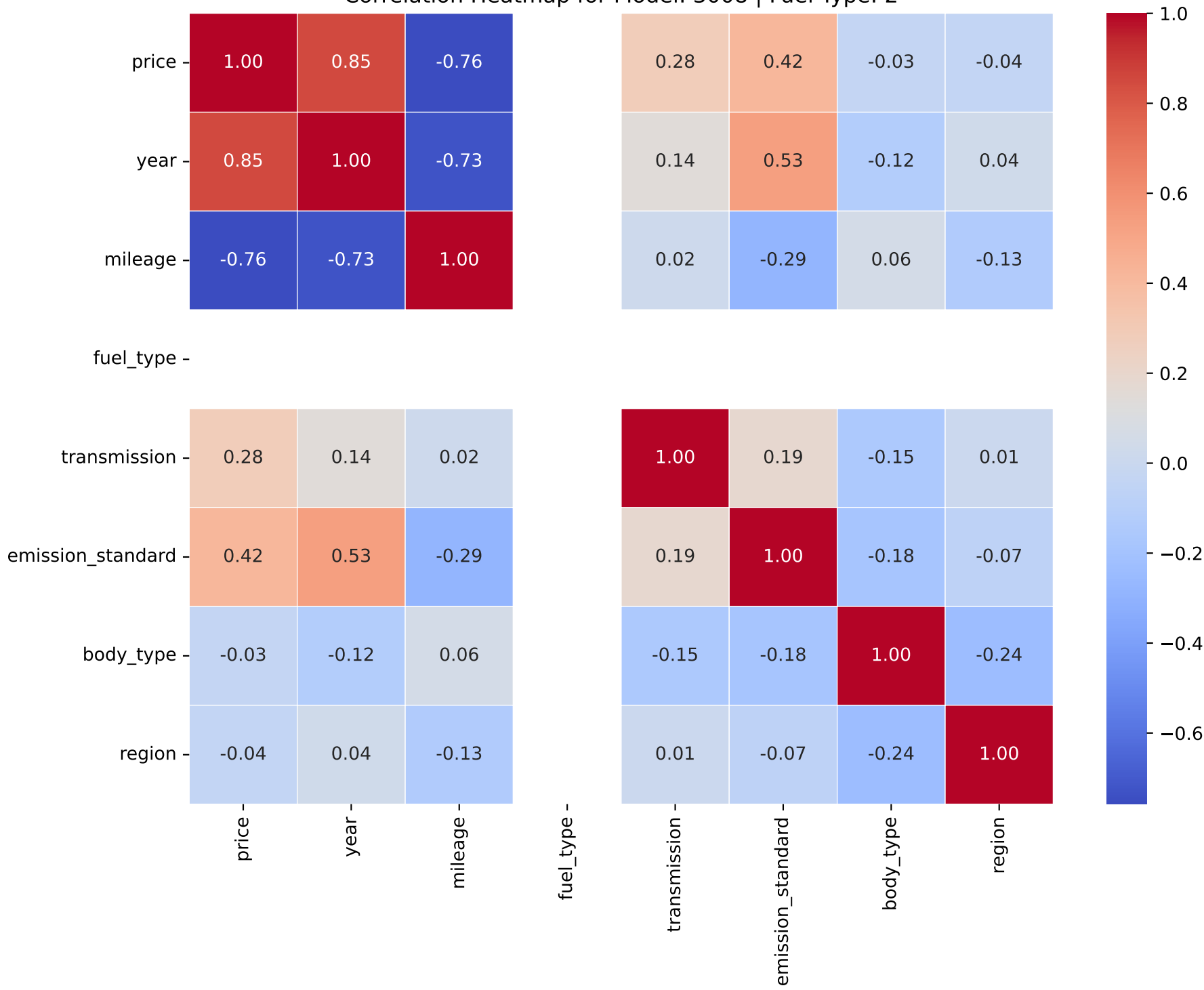
Correlation Heatmap for Model: 3008 | Fuel Type: 2
