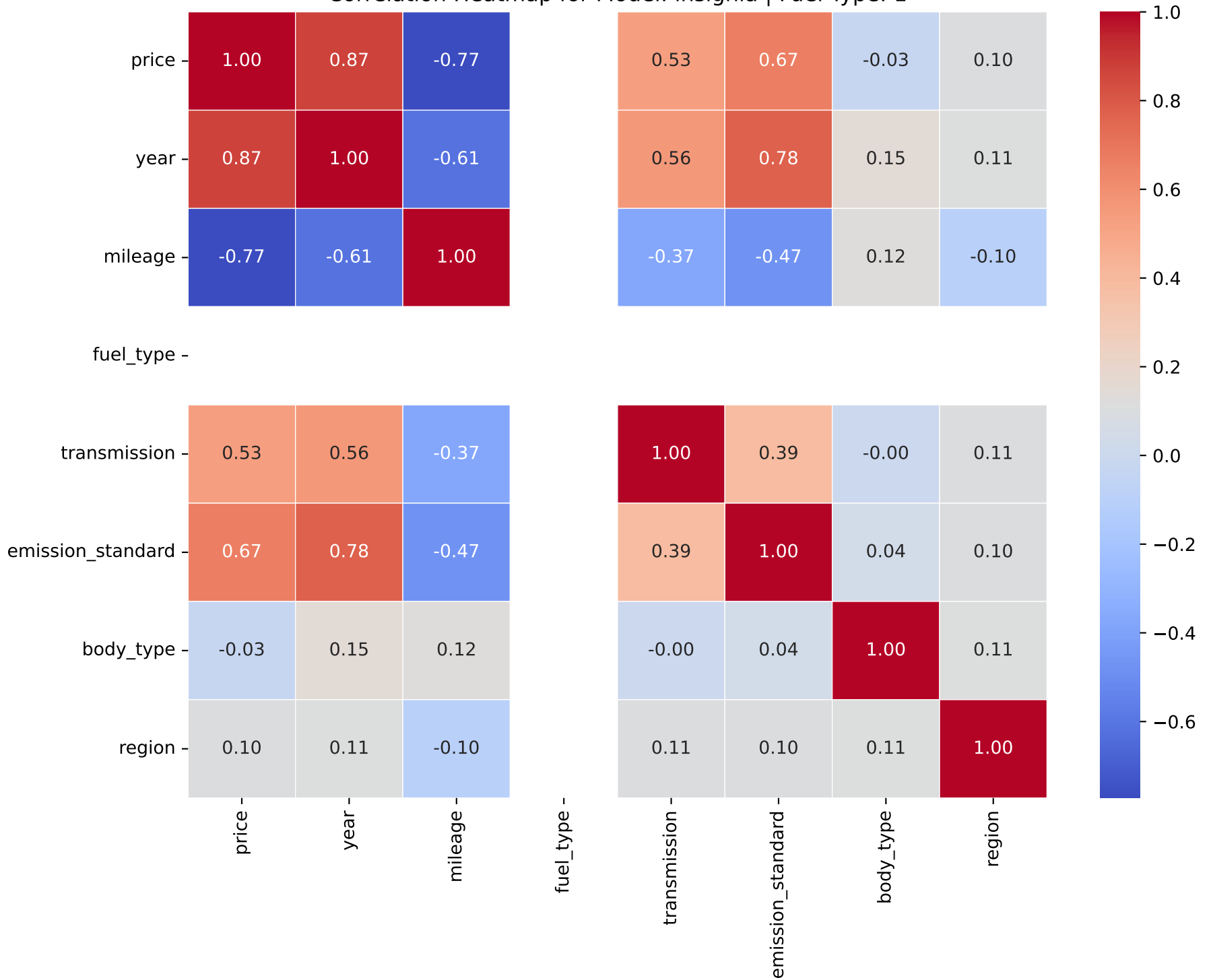
Correlation Heatmap for Model: insignia | Fuel Type: 1
