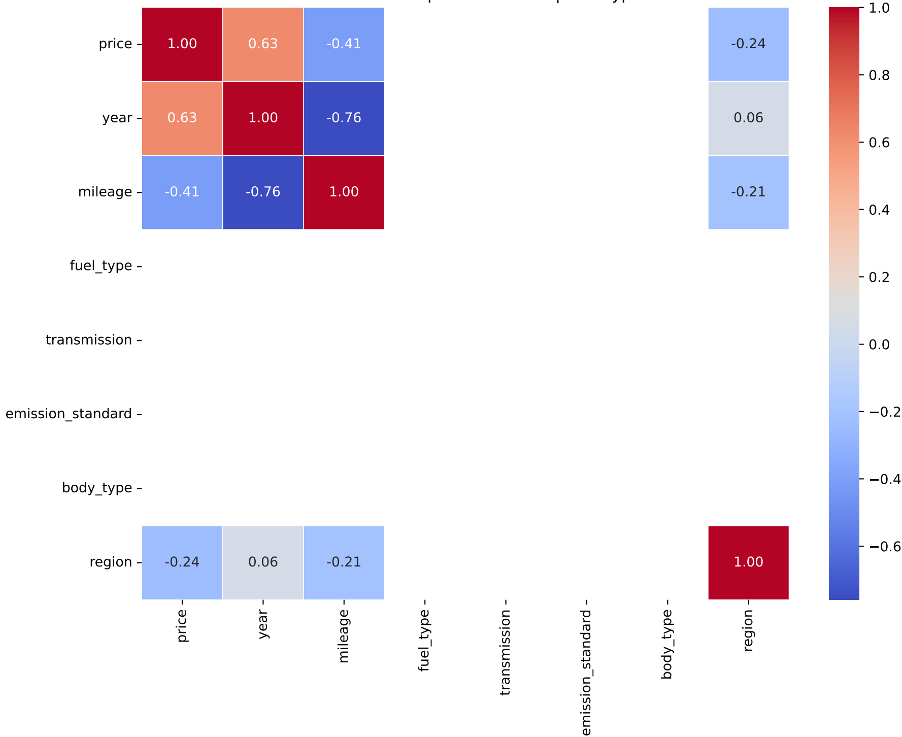
Correlation Heatmap for Model: a7 | Fuel Type: 3
