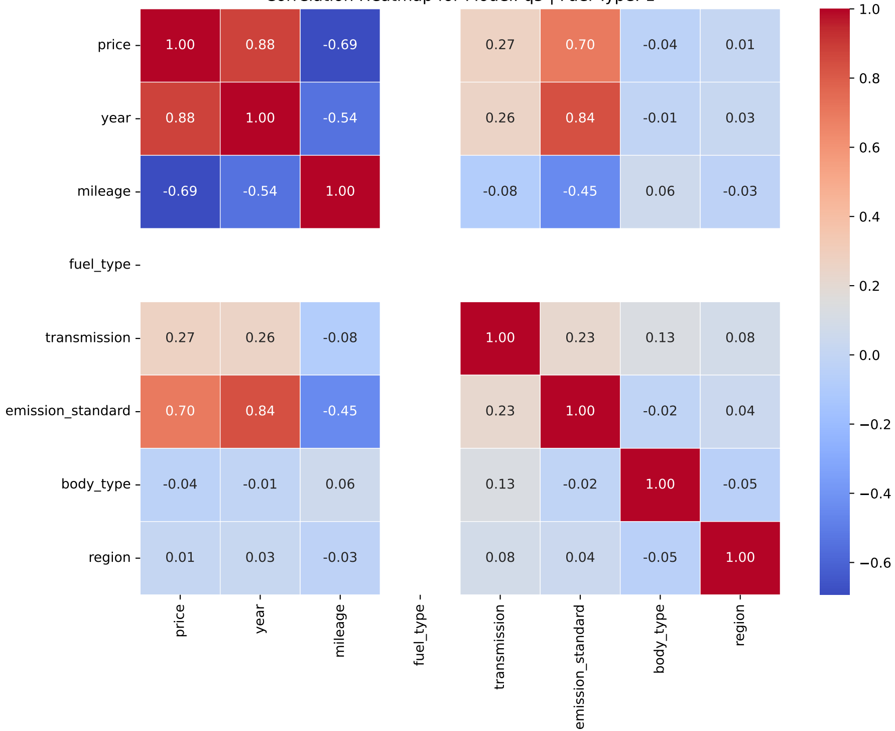
Correlation Heatmap for Model: q5 | Fuel Type: 1
