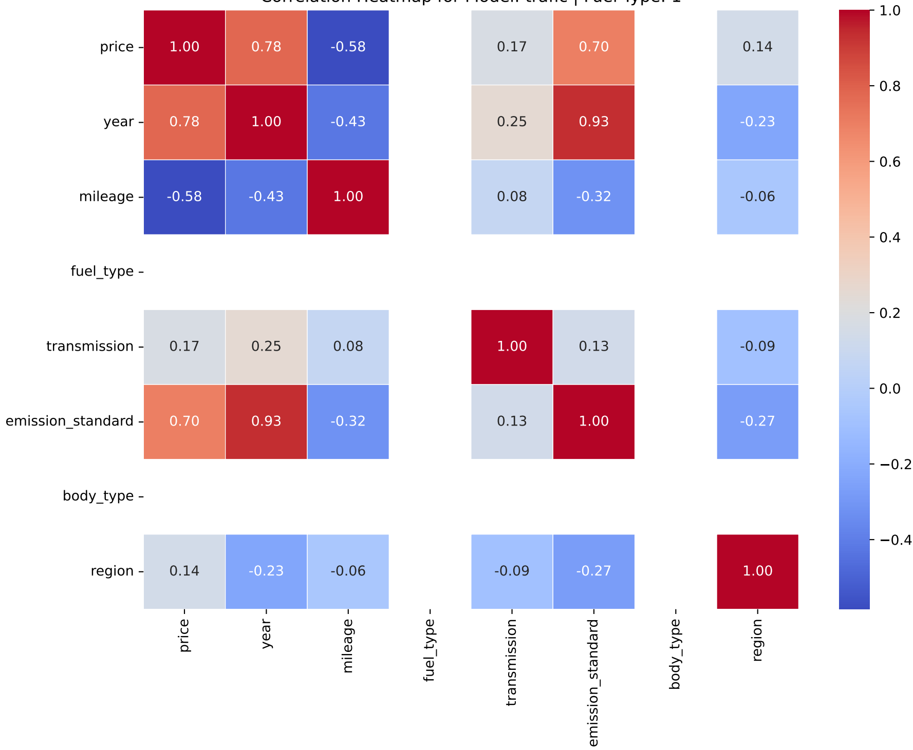
Correlation Heatmap for Model: traffic | Fuel Type: 1
