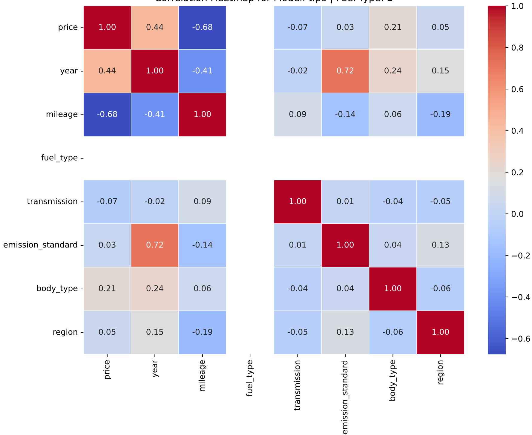
Correlation Heatmap for Model: tipo | Fuel Type: 2
