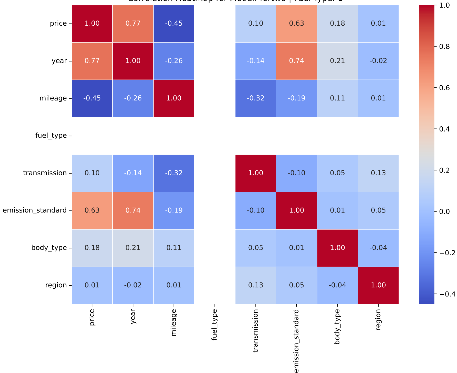
Correlation Heatmap for Model: fortwo | Fuel Type: 1
