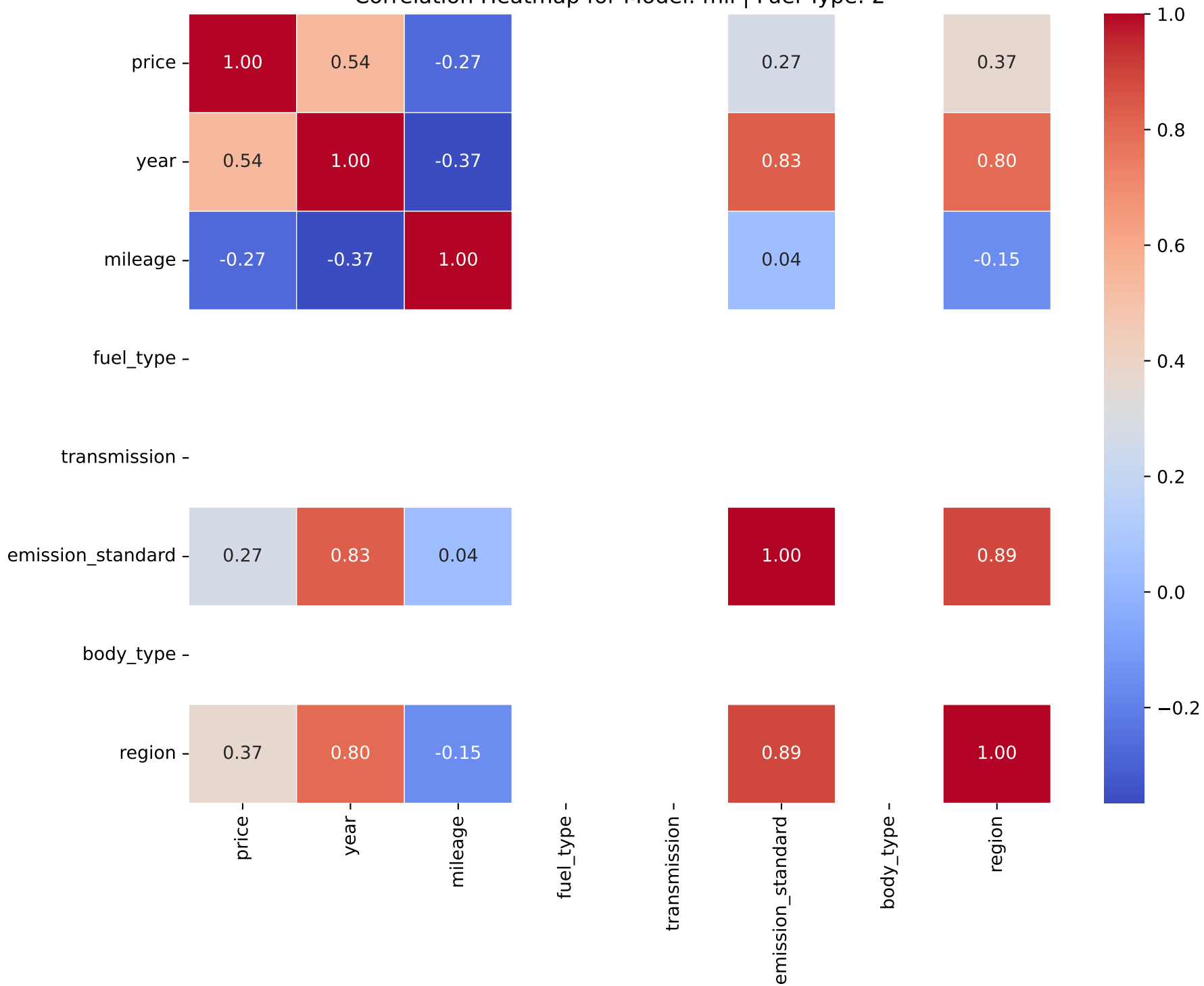
Correlation Heatmap for Model: mii | Fuel Type: 2
