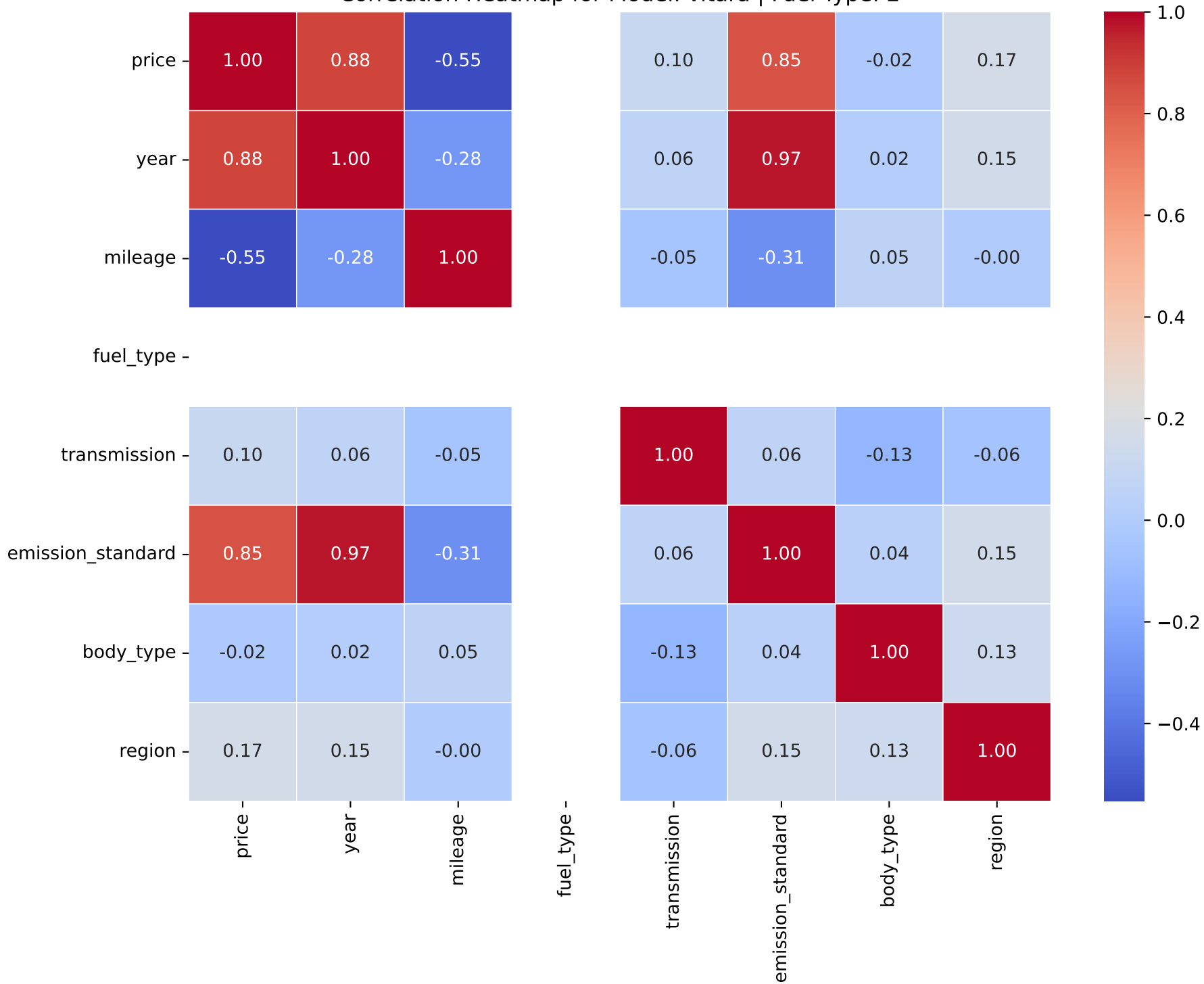
Correlation Heatmap for Model: vitara | Fuel Type: 2
