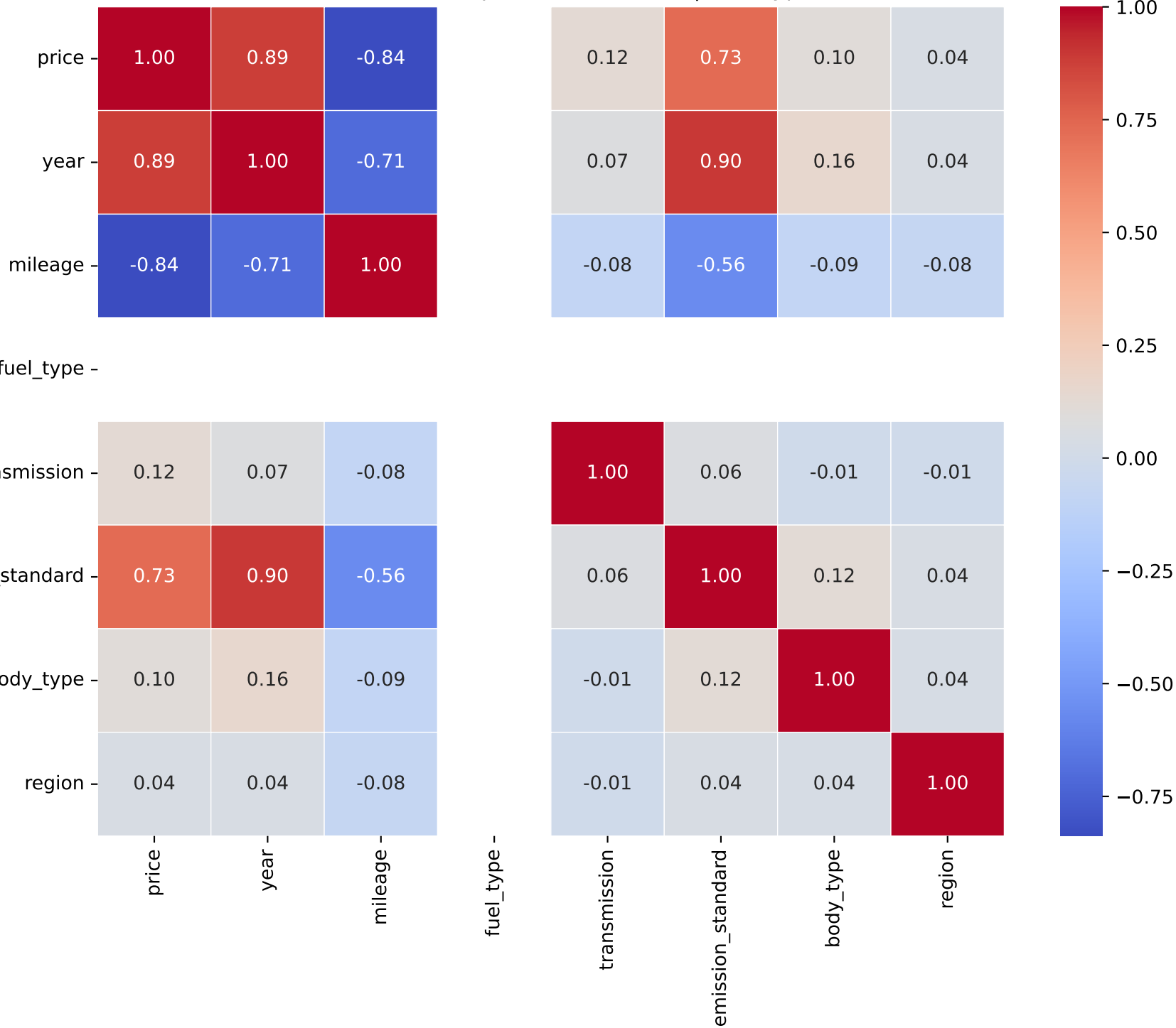
Correlation Heatmap for Model: corsa | Fuel Type: 2
