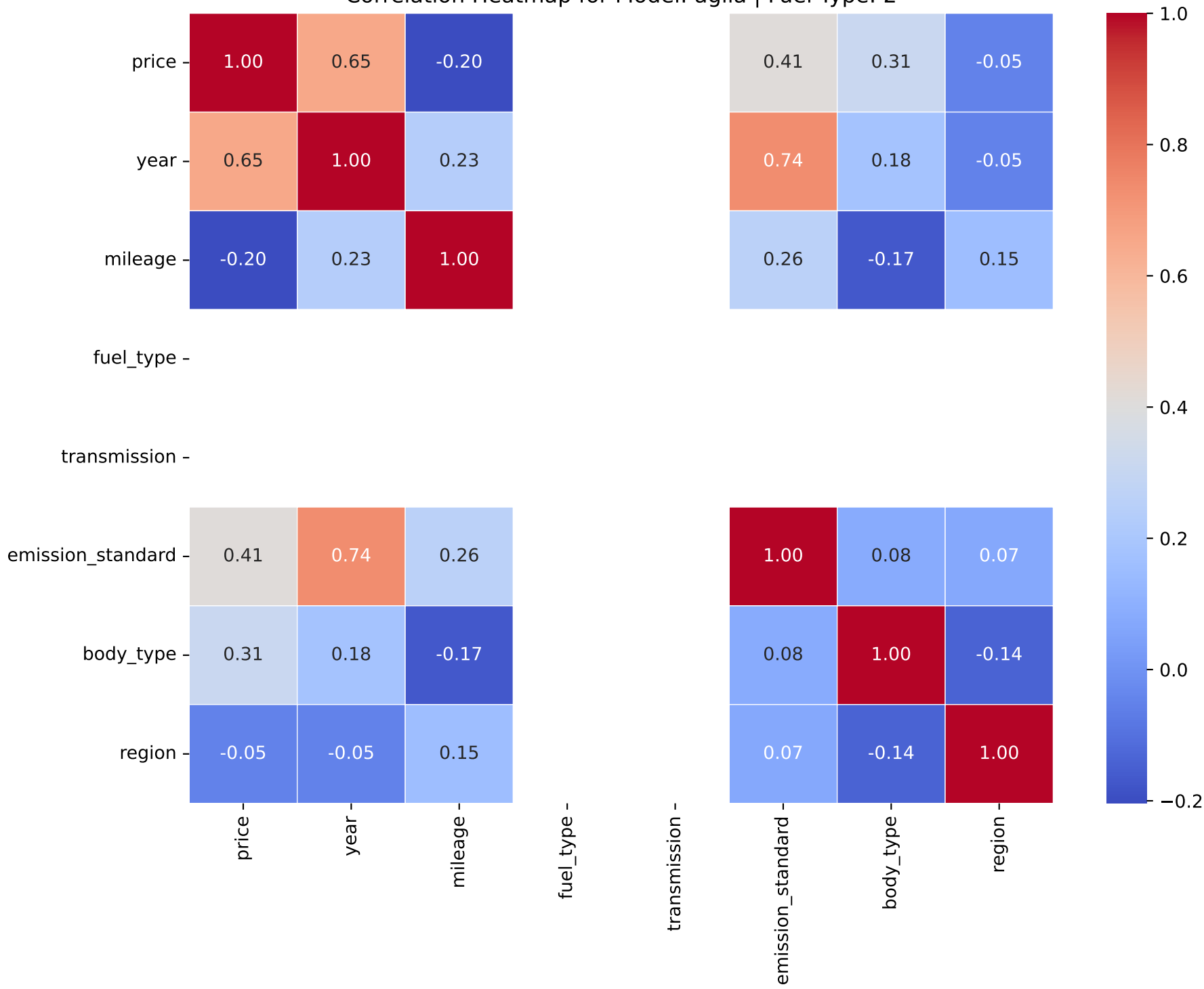
Correlation Heatmap for Model: agila | Fuel Type: 2
