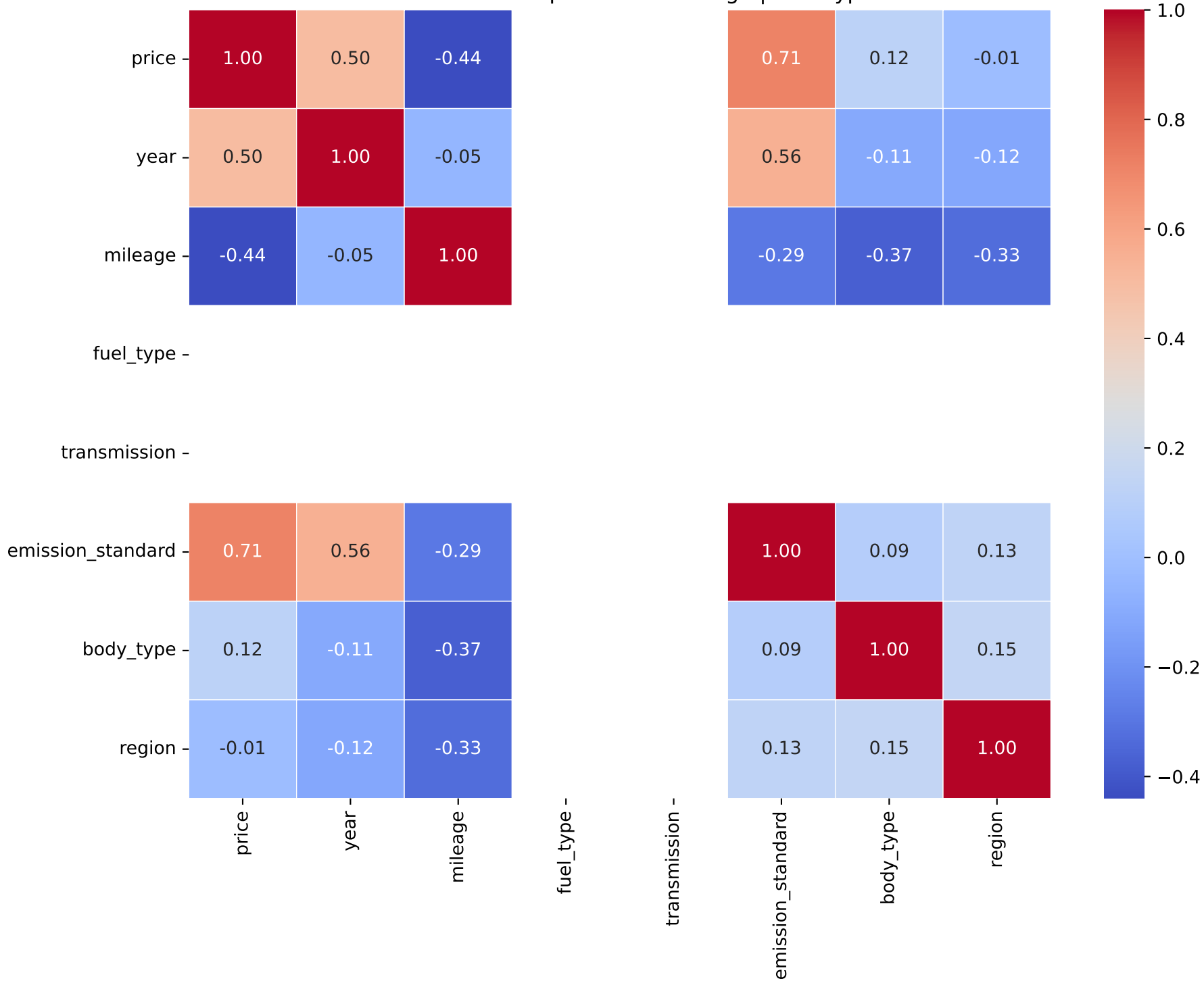
Correlation Heatmap for Model: venga | Fuel Type: 1
