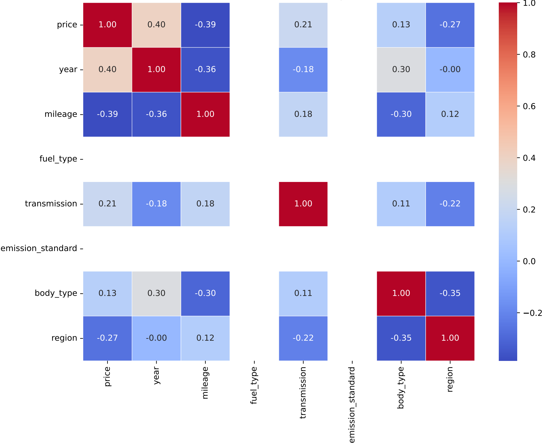
Correlation Heatmap for Model: 2008 | Fuel Type: 0
