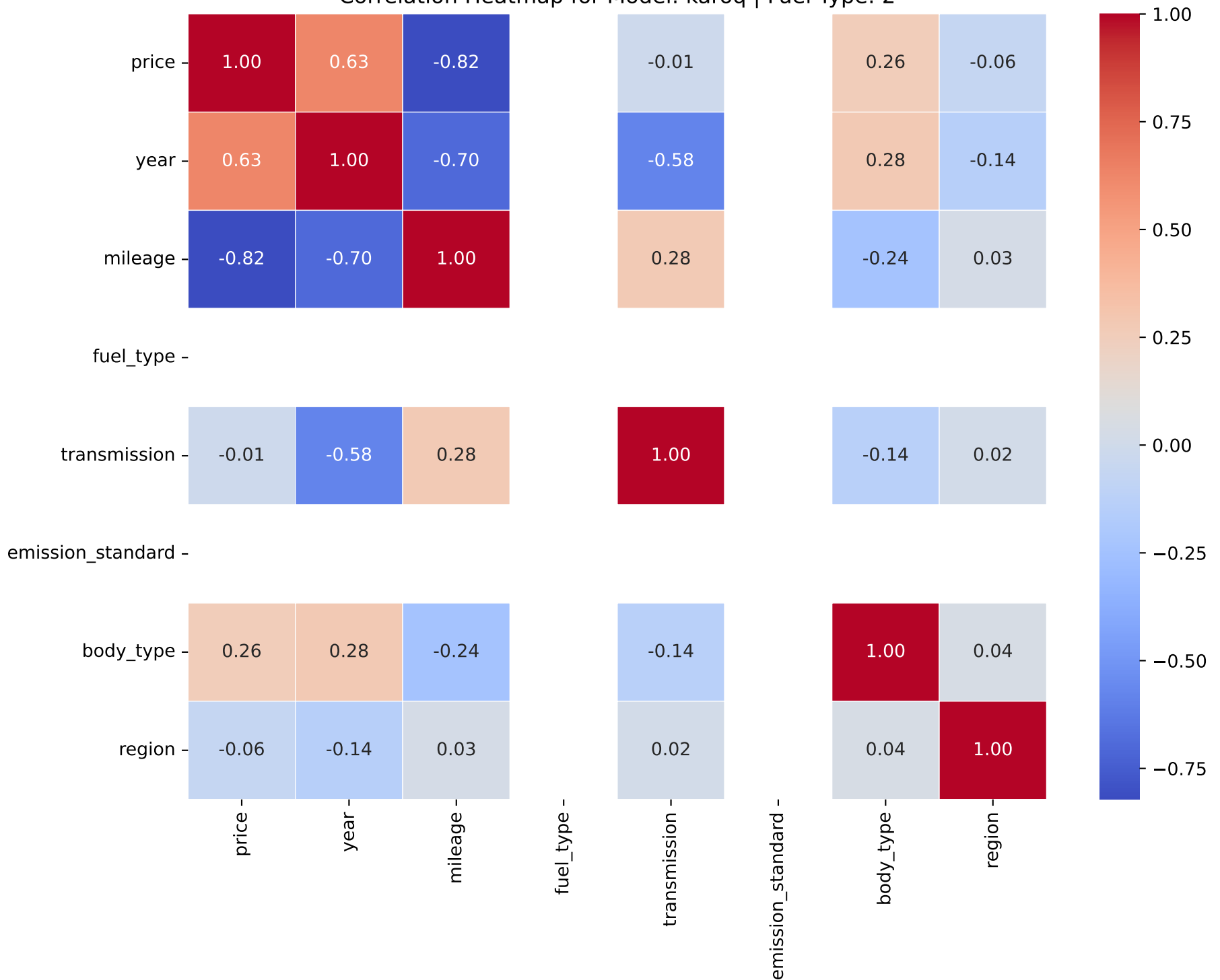
Correlation Heatmap for Model: karoq | Fuel Type: 2
