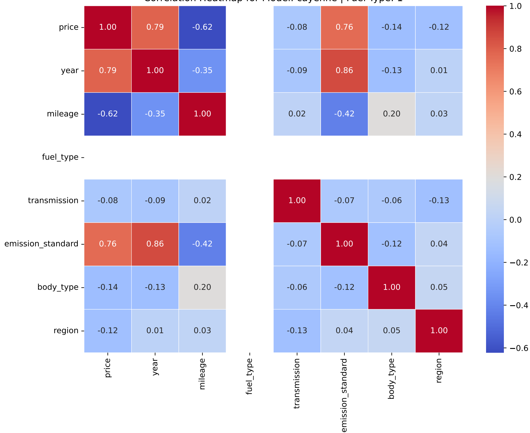
Correlation Heatmap for Model: cayenne | Fuel Type: 1
