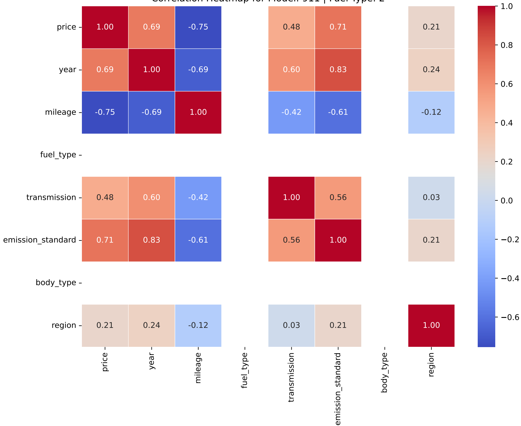
Correlation Heatmap for Model: 911 | Fuel Type: 2
