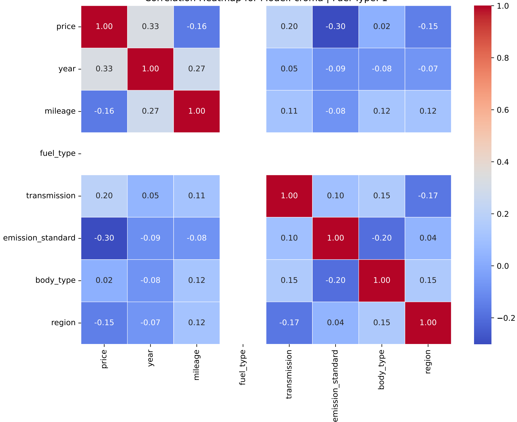
Correlation Heatmap for Model: croma | Fuel Type: 1
