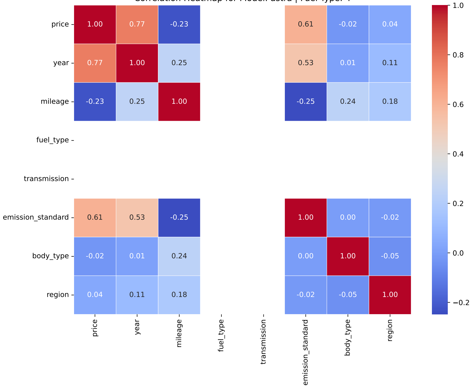
Correlation Heatmap for Model: astra | Fuel Type: 4
