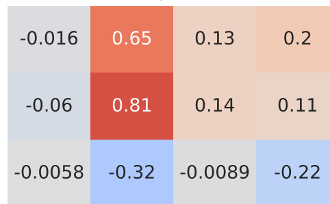
Pearson Correlation - Model: punto | Fuel: 1
