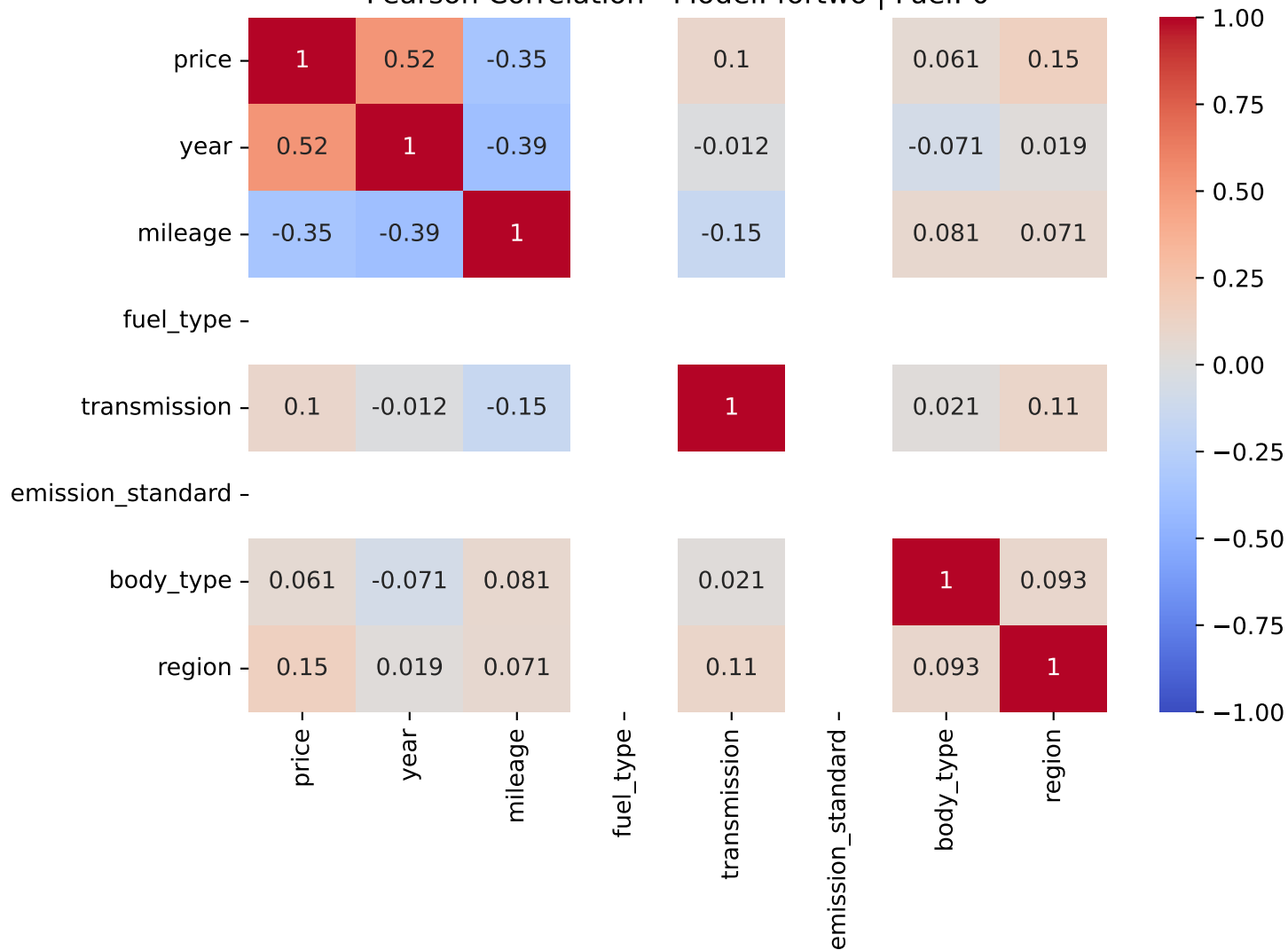
Pearson Correlation - Model: fortwo | Fuel: 0
