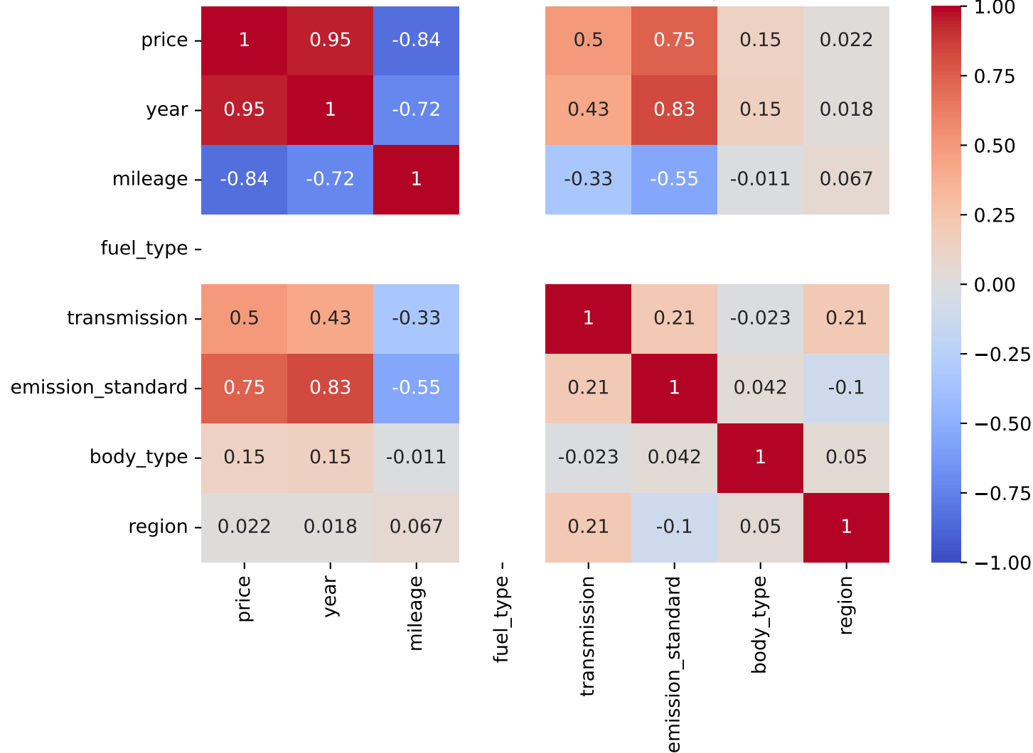
Pearson Correlation - Model: picanto | Fuel: 4
