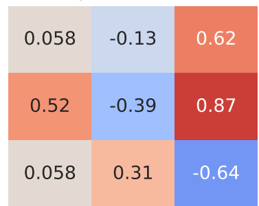
Spearman Correlation - Model: yeti | Fuel: 1
