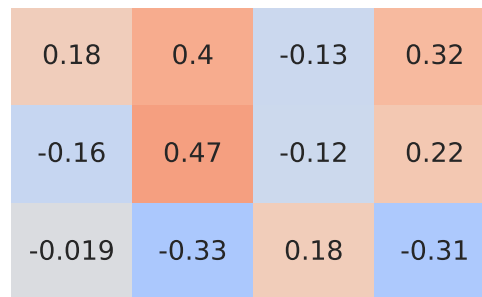
Spearman Correlation - Model: 108 | Fuel: 2
