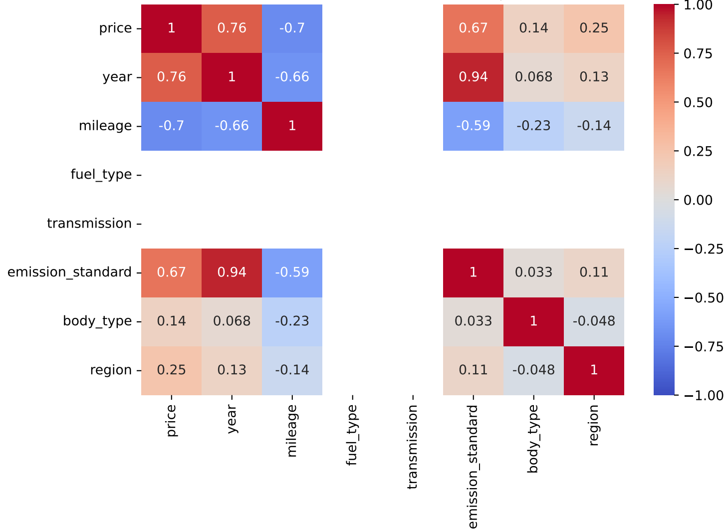
Pearson Correlation - Model: kangoo | Fuel: 1
