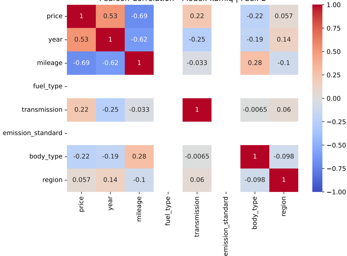
Pearson Correlation - Model: kamiq | Fuel: 2
