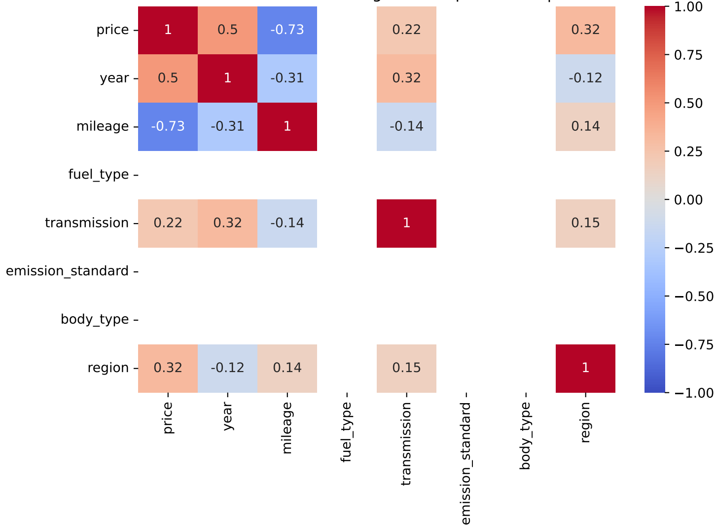
Pearson Correlation - Model: grand c4 spacetourer | Fuel: 1
