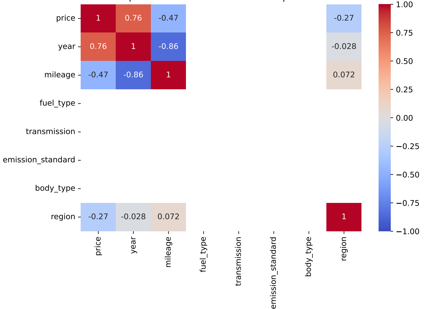
Spearman Correlation - Model: a7 | Fuel: 3
