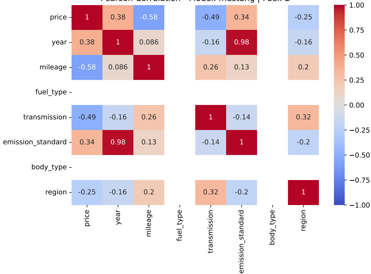
Pearson Correlation - Model: mustang | Fuel: 2
