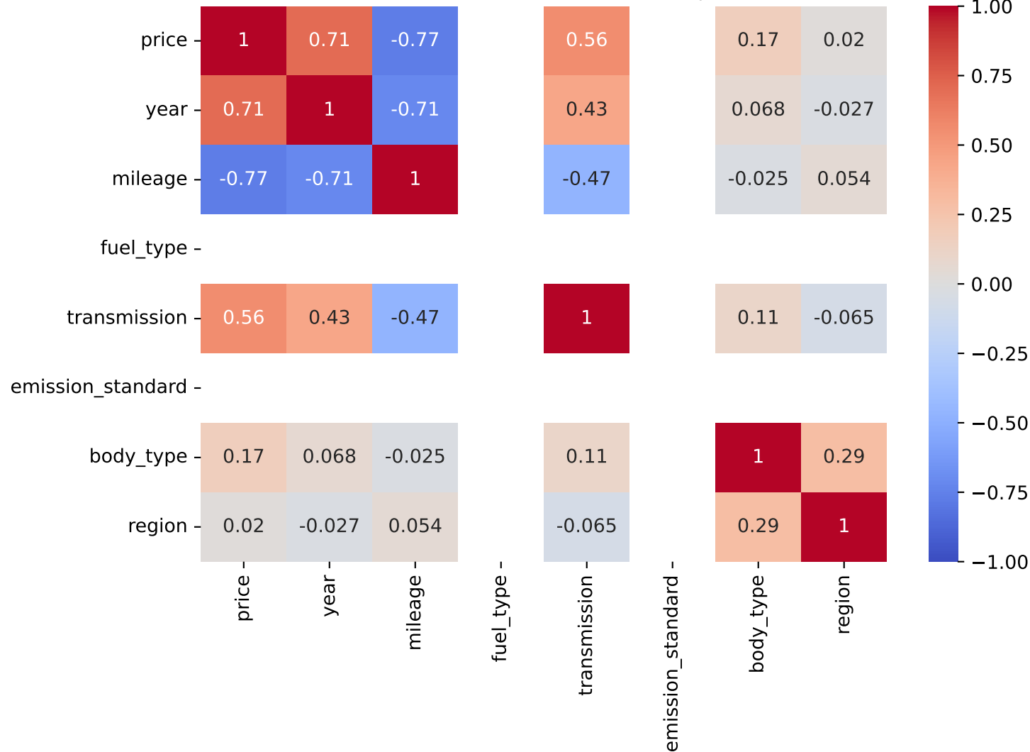
Spearman Correlation - Model: i20 | Fuel: 3
