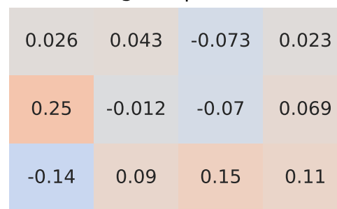
Pearson Correlation - Model: renegade | Fuel: 3
