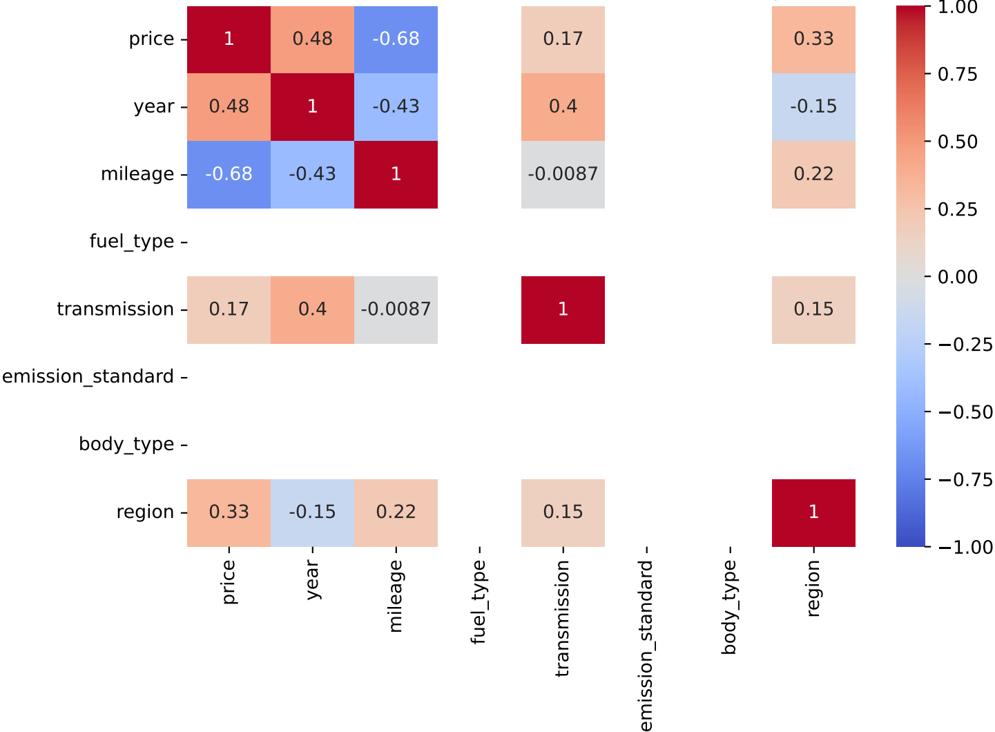
Spearman Correlation - Model: grand c4 spacetourer | Fuel: 1
