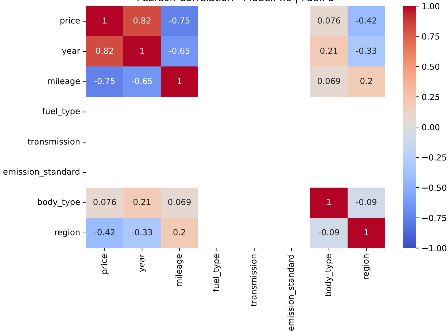
Pearson Correlation - Model: x6 | Fuel: 3
