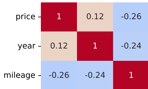
Spearman Correlation - Model: romeo 156 | Fuel: 2
