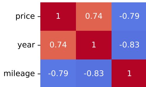
Spearman Correlation - Model: rover evoque | Fuel: 1
