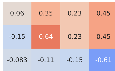
Spearman Correlation - Model: verso | Fuel: 1
