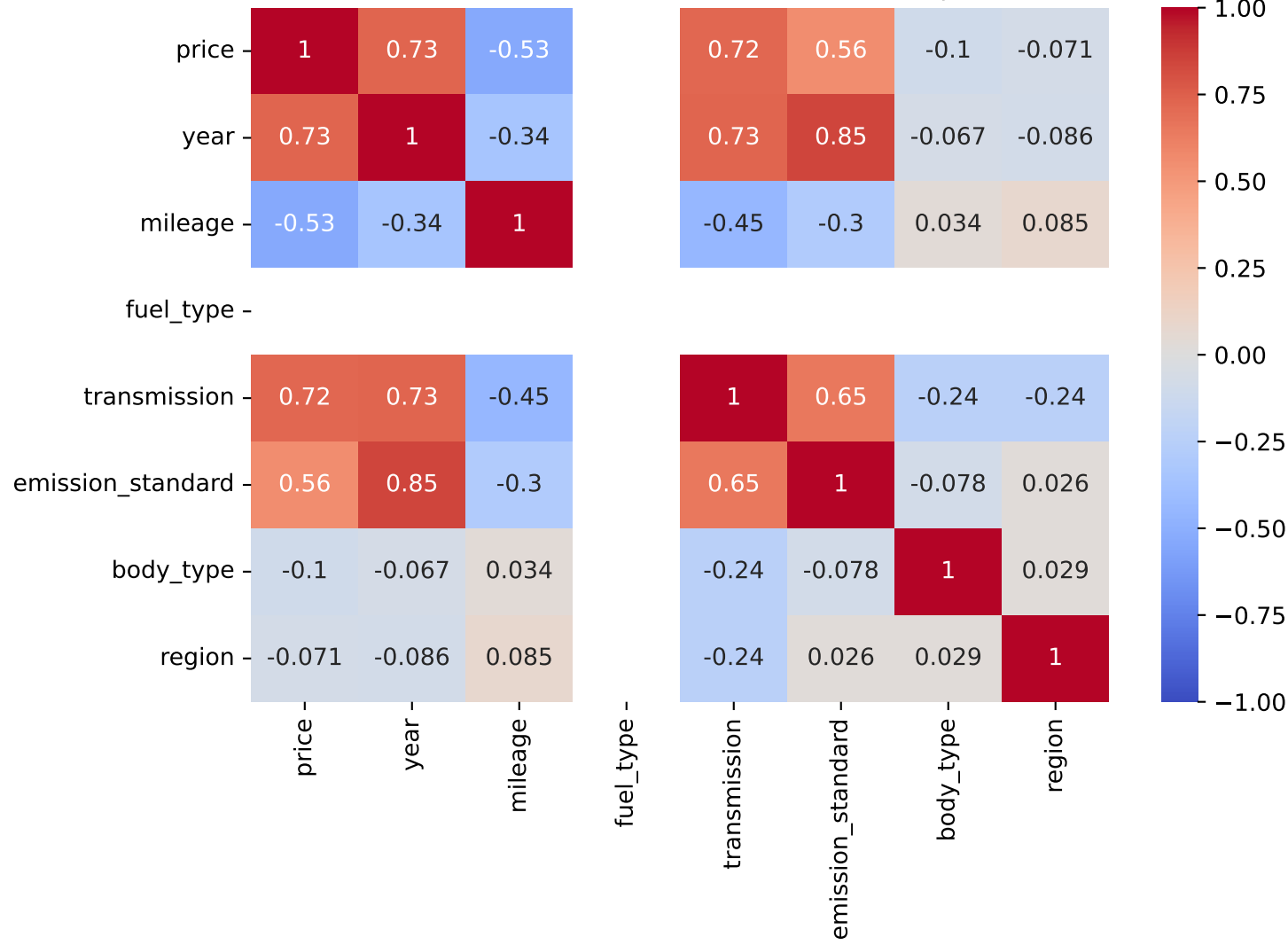
Pearson Correlation - Model: rover defender | Fuel: 1
