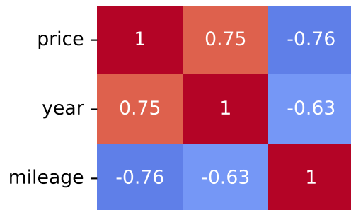
Spearman Correlation - Model: romeo mito | Fuel: 1
