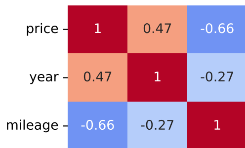
Pearson Correlation - Model: hilux | Fuel: 1
