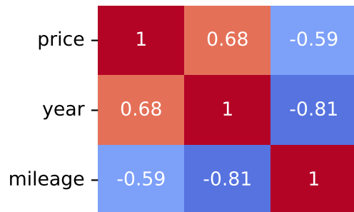
Pearson Correlation - Model: rover evoque | Fuel: 1
