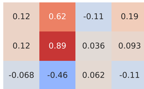
Pearson Correlation - Model: ibiza | Fuel: 1
