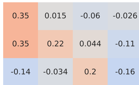
Pearson Correlation - Model: freemont | Fuel: 1
