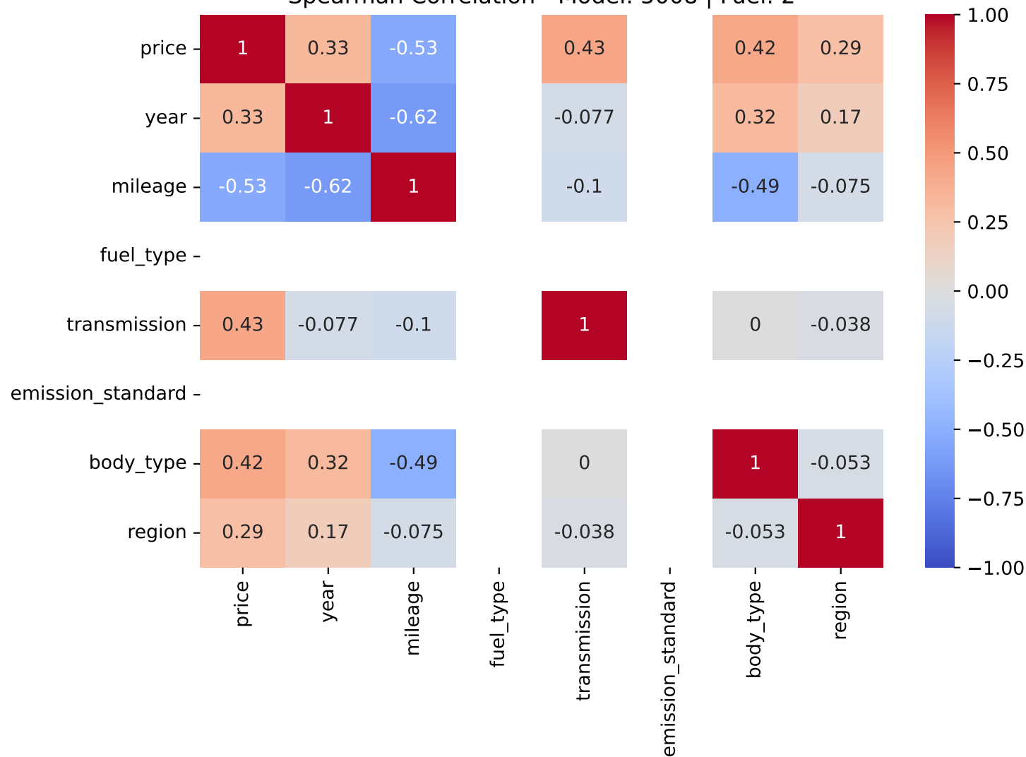
Spearman Correlation - Model: 5008 | Fuel: 2
