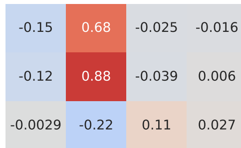
Pearson Correlation - Model: ka | Fuel: 2
