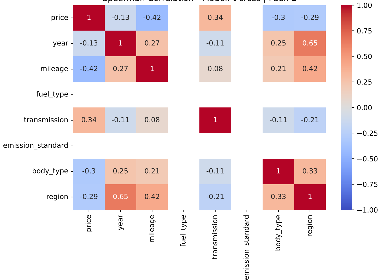
Spearman Correlation - Model: t-cross | Fuel: 1
