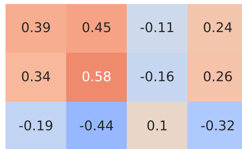
Pearson Correlation - Model: countryman | Fuel: 2
