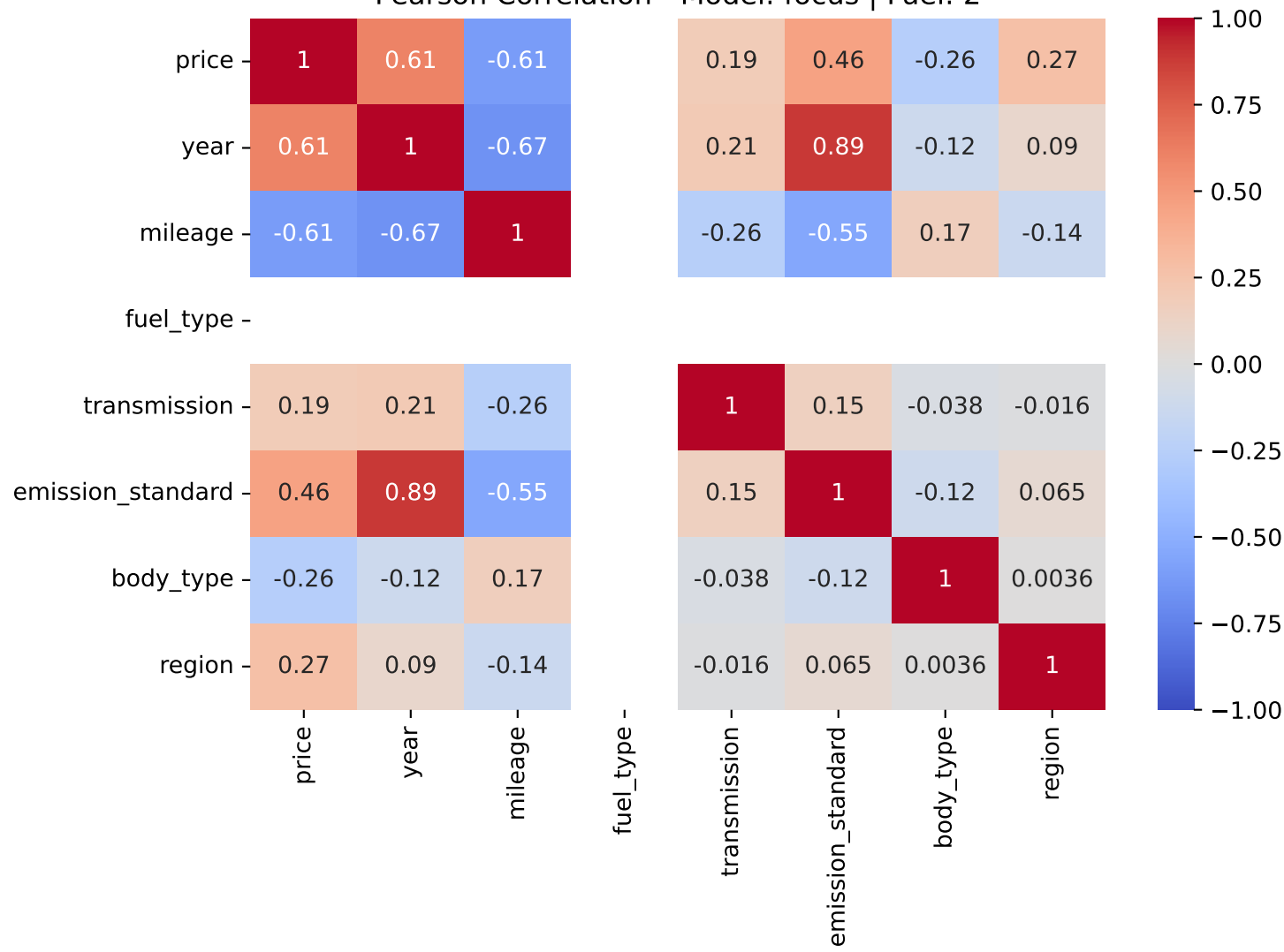
Pearson Correlation - Model: focus | Fuel: 2
