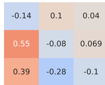
Pearson Correlation - Model: zafira tourer | Fuel: 5
