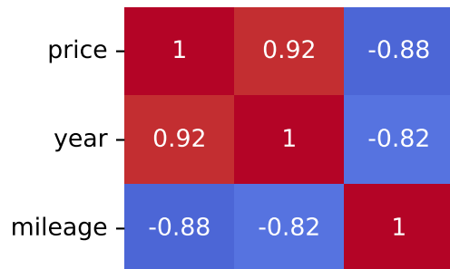
Pearson Correlation - Model: ibiza | Fuel: 2
