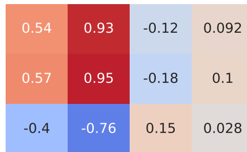
Pearson Correlation - Model: koleos | Fuel: 1
