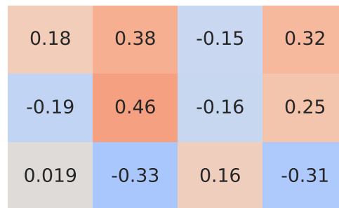
Pearson Correlation - Model: 108 | Fuel: 2
