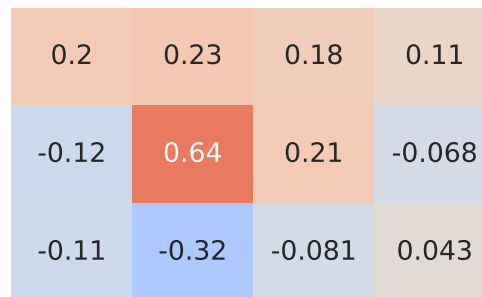
Pearson Correlation - Model: modus | Fuel: 2
