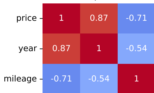
Spearman Correlation - Model: q5 | Fuel: 1
