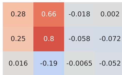
Spearman Correlation - Model: v40 | Fuel: 1
