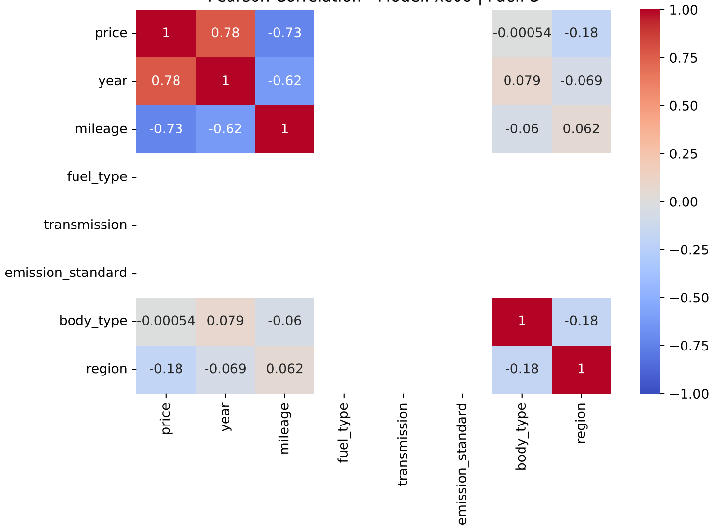
Pearson Correlation - Model: xc60 | Fuel: 3
