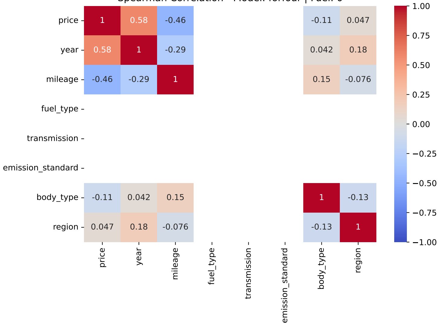
Spearman Correlation - Model: forfour | Fuel: 0
