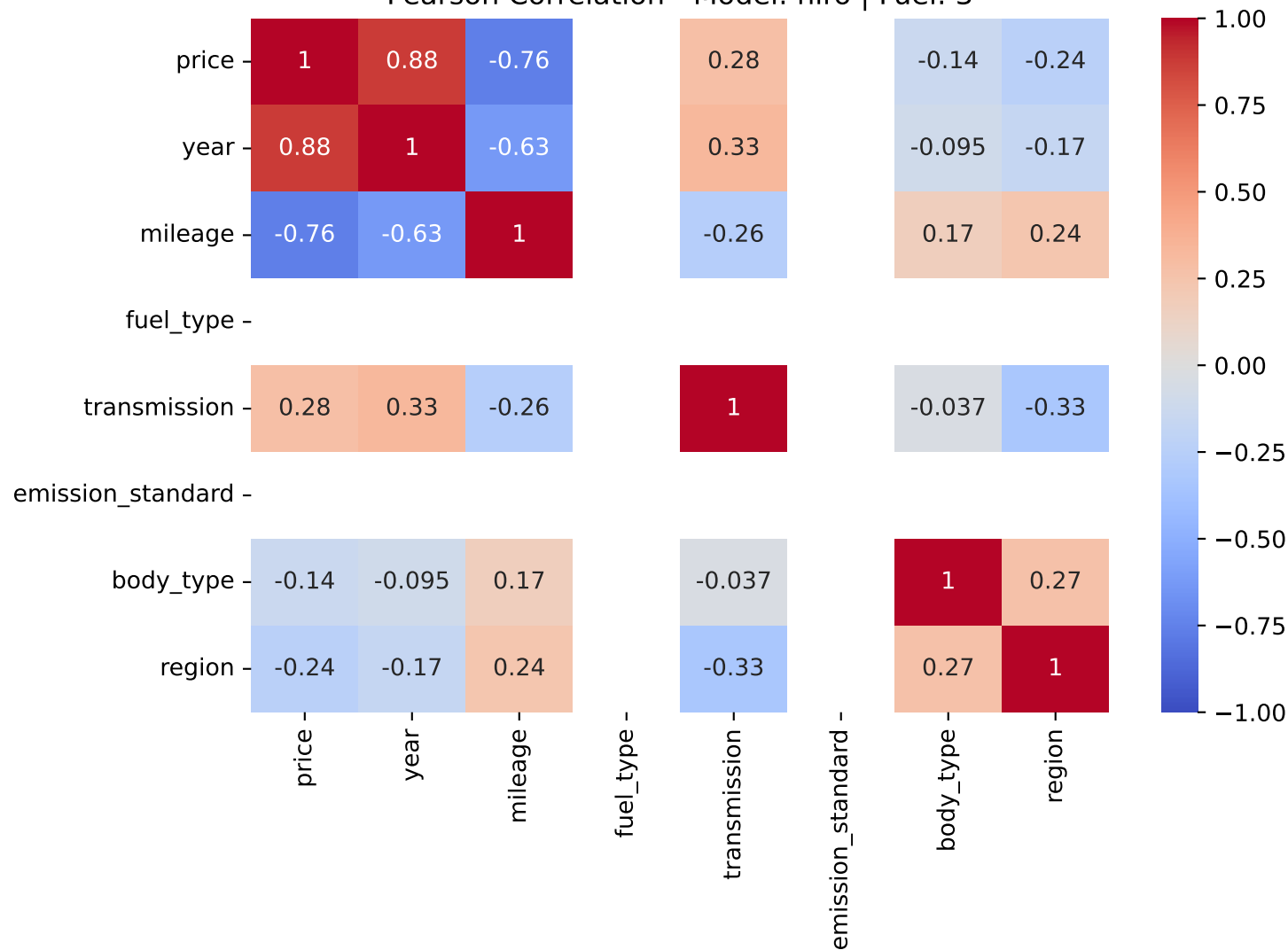
Pearson Correlation - Model: niro | Fuel: 3
