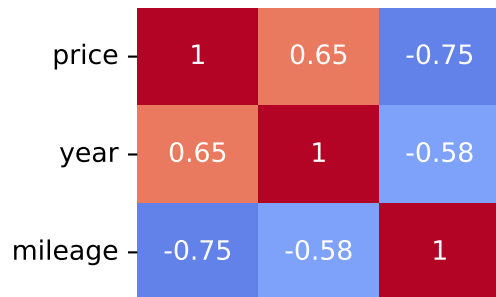
Spearman Correlation - Model: x2 | Fuel: 1
