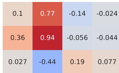
Pearson Correlation - Model: grand cherokee | Fuel: 1
