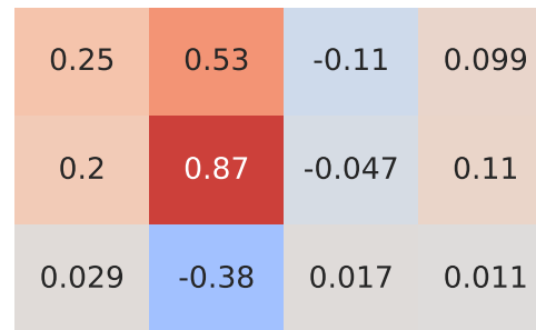
Spearman Correlation - Model: romeo mito | Fuel: 2
