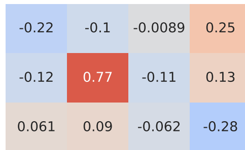
Pearson Correlation - Model: nemo | Fuel: 1
