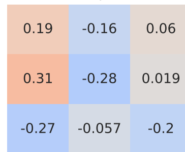
Spearman Correlation - Model: grande punto | Fuel: 5
