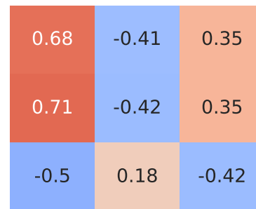
Spearman Correlation - Model: rio | Fuel: 2
