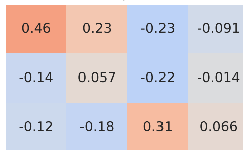
Spearman Correlation - Model: kona | Fuel: 2
