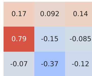
Spearman Correlation - Model: sedici | Fuel: 2
