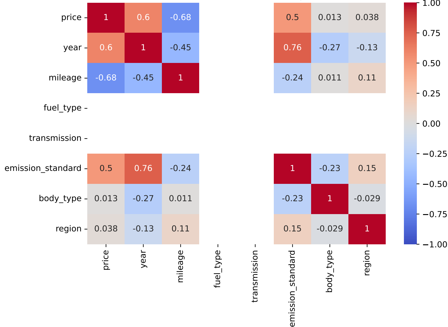
Pearson Correlation - Model: 208 | Fuel: 4
