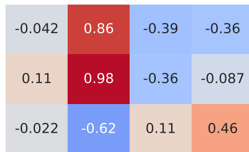
Pearson Correlation - Model: octavia | Fuel: 2
