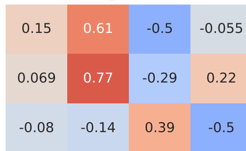
Pearson Correlation - Model: 407 | Fuel: 1
