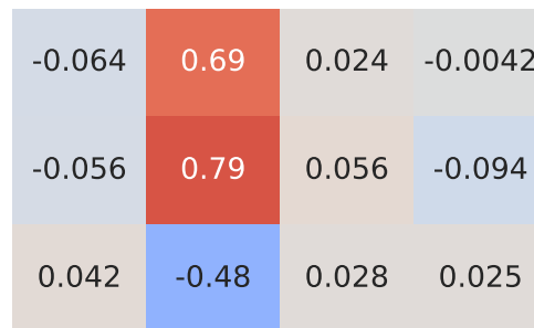
Pearson Correlation - Model: ypsilon | Fuel: 4
