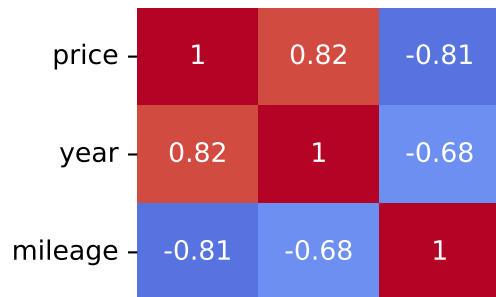
Pearson Correlation - Model: panda | Fuel: 4
