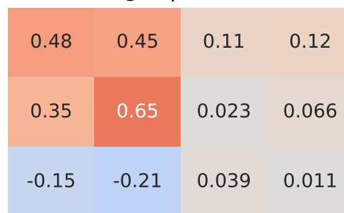
Pearson Correlation - Model: ranger | Fuel: 1
