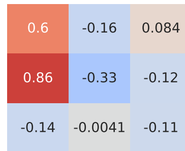
Spearman Correlation - Model: ix20 | Fuel: 1
