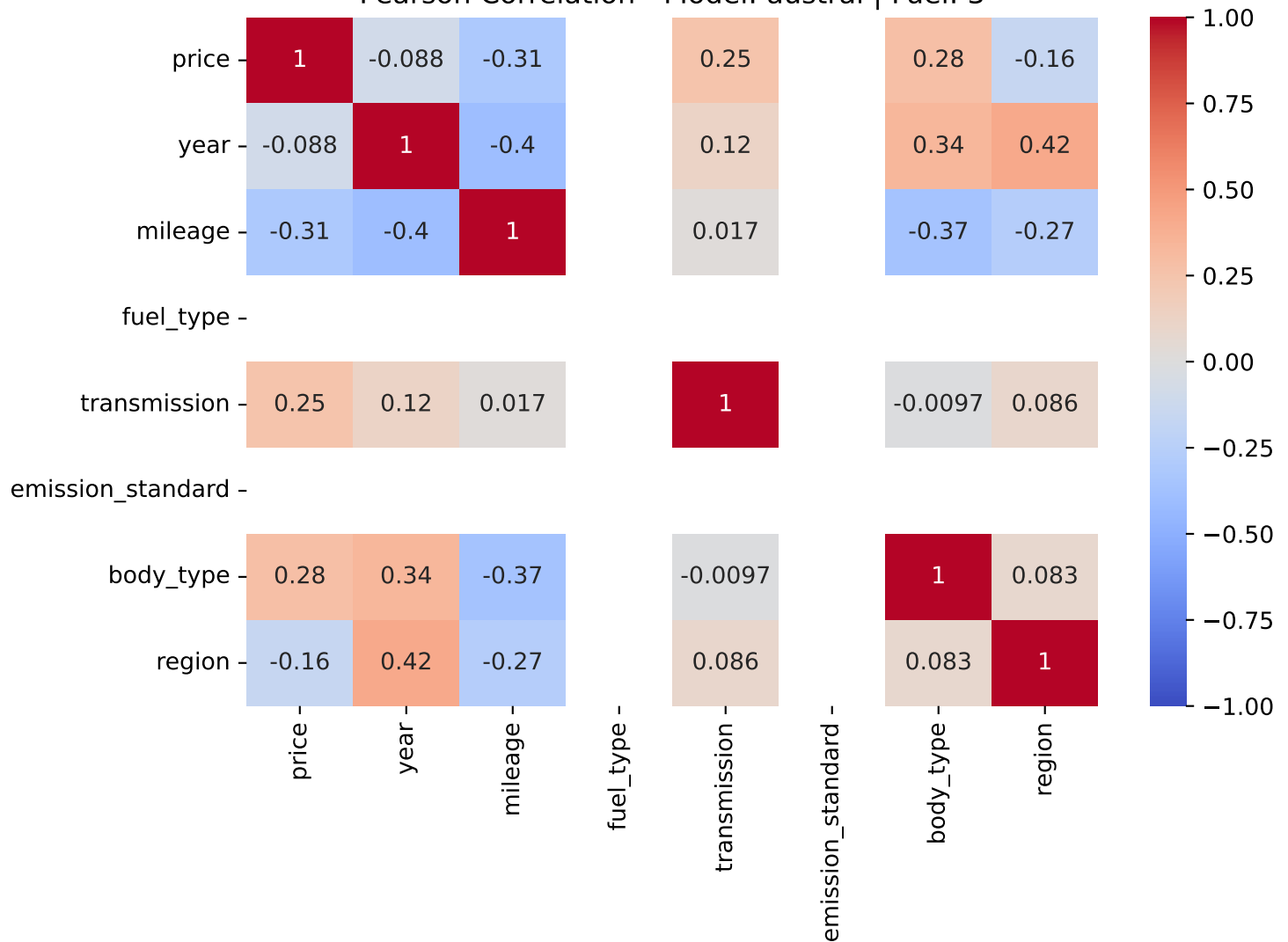
Pearson Correlation - Model: austral | Fuel: 3
