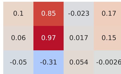
Pearson Correlation - Model: vitara | Fuel: 2
