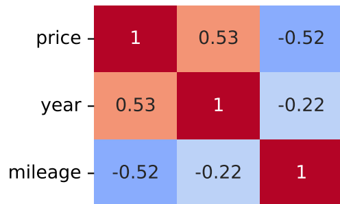
Spearman Correlation - Model: c3 picasso | Fuel: 1
