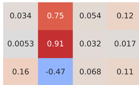
Spearman Correlation - Model: navara | Fuel: 1
