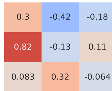
Spearman Correlation - Model: sx4 | Fuel: 1
