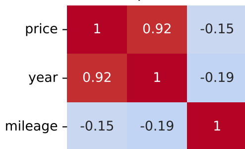
Spearman Correlation - Model: zafira | Fuel: 2
