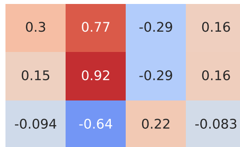
Pearson Correlation - Model: qashqai | Fuel: 2
