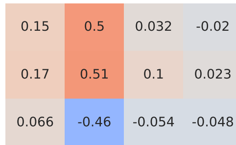
Spearman Correlation - Model: juke | Fuel: 2
