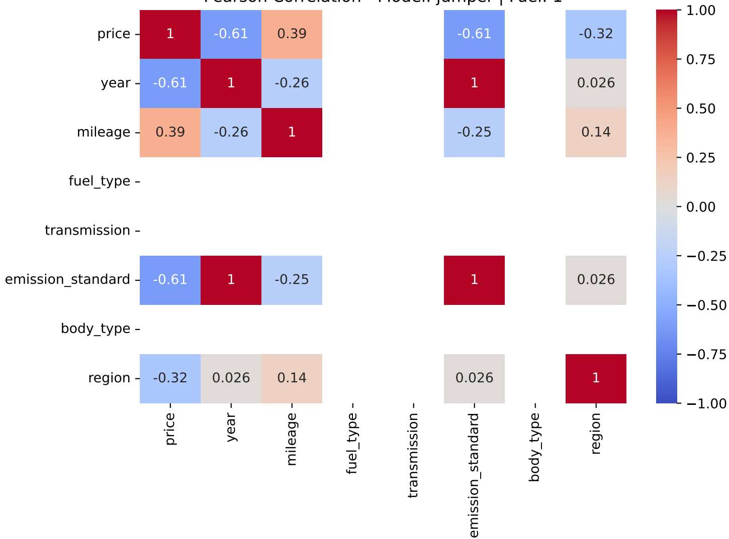
Pearson Correlation - Model: jumper | Fuel: 1
