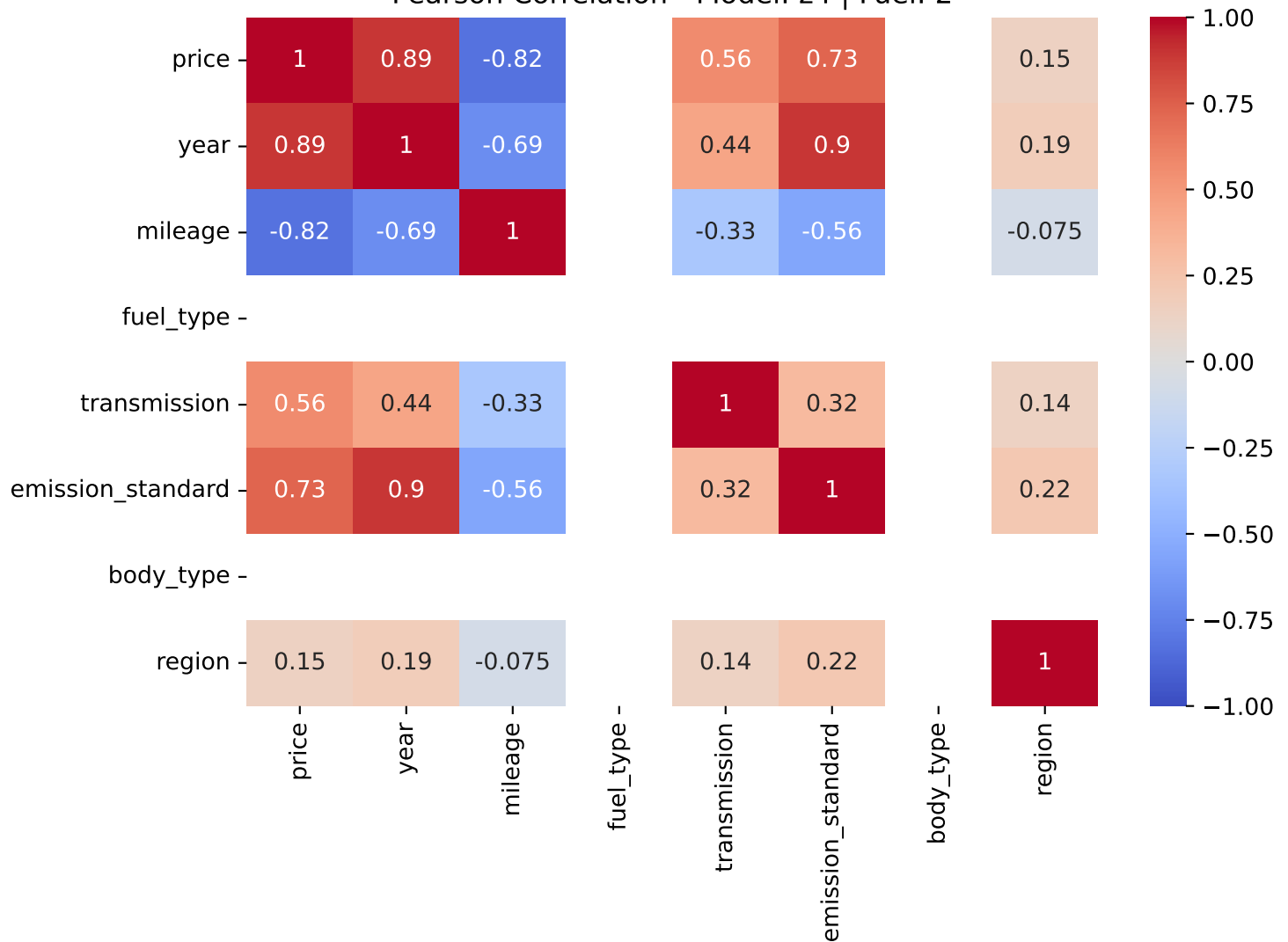
Pearson Correlation - Model: z4 | Fuel: 2
