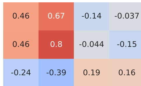
Pearson Correlation - Model: zafira | Fuel: 1
