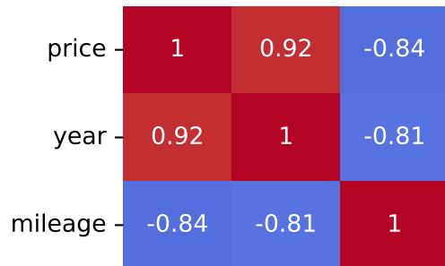
Pearson Correlation - Model: fabia | Fuel: 2
