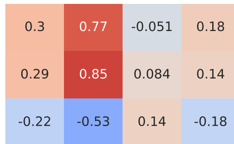
Pearson Correlation - Model: megane | Fuel: 1
