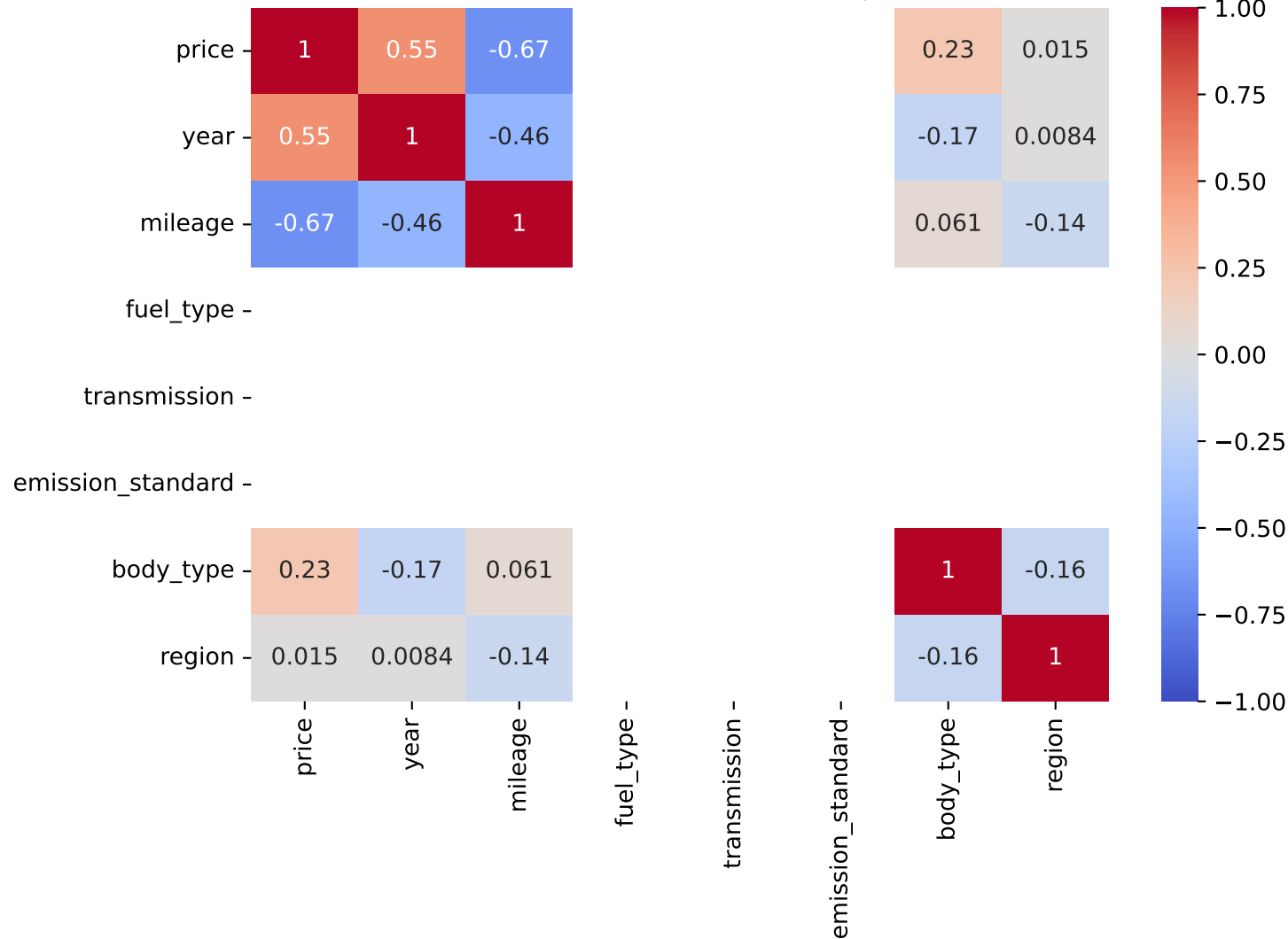
Pearson Correlation - Model: tipo | Fuel: 4
