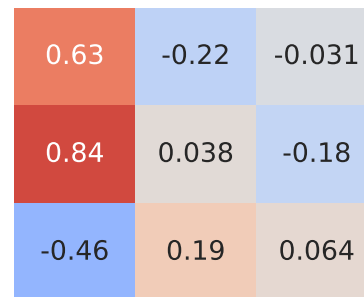
Spearman Correlation - Model: c-max | Fuel: 2
