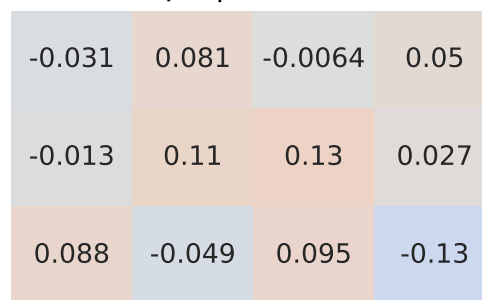
Pearson Correlation - Model: tipo | Fuel: 1
