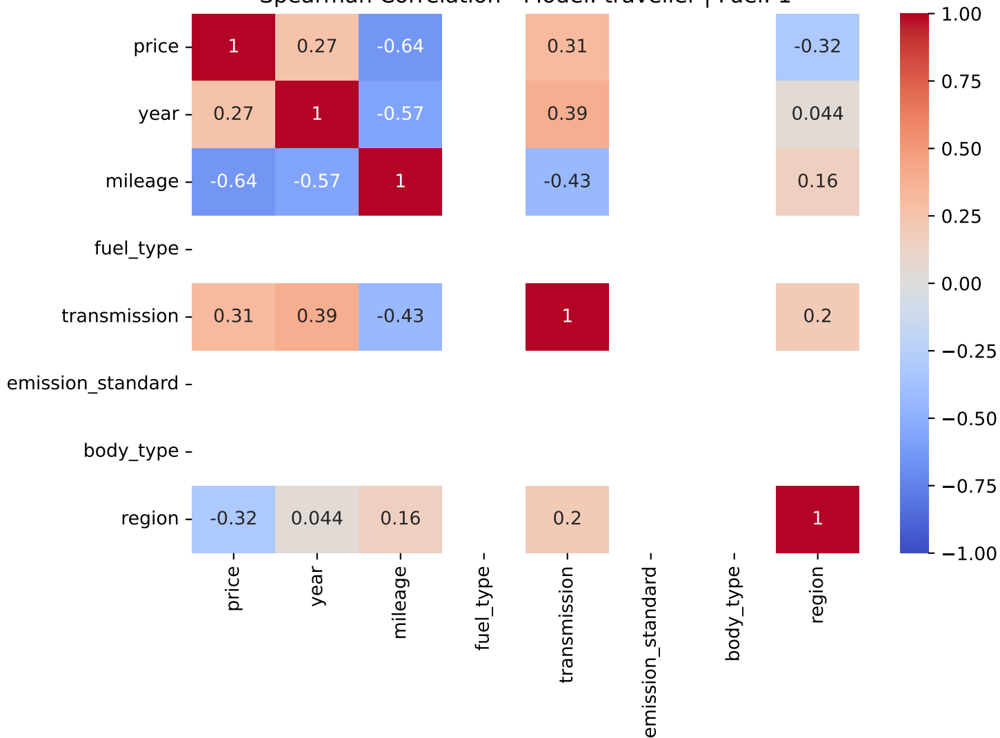
Spearman Correlation - Model: traveller | Fuel: 1
