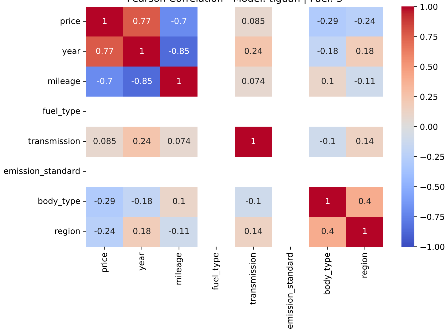
Pearson Correlation - Model: tiguan | Fuel: 3
