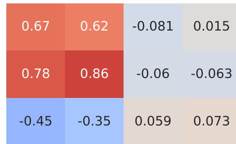
Spearman Correlation - Model: rover defender | Fuel: 1
