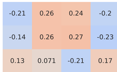
Spearman Correlation - Model: rs3 | Fuel: 2
