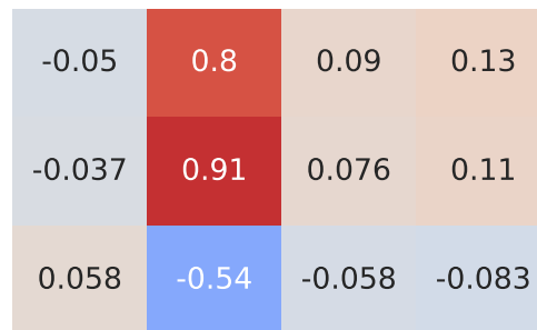
Pearson Correlation - Model: fiesta | Fuel: 1
