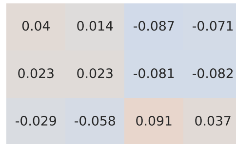
Spearman Correlation - Model: c-hr | Fuel: 3
