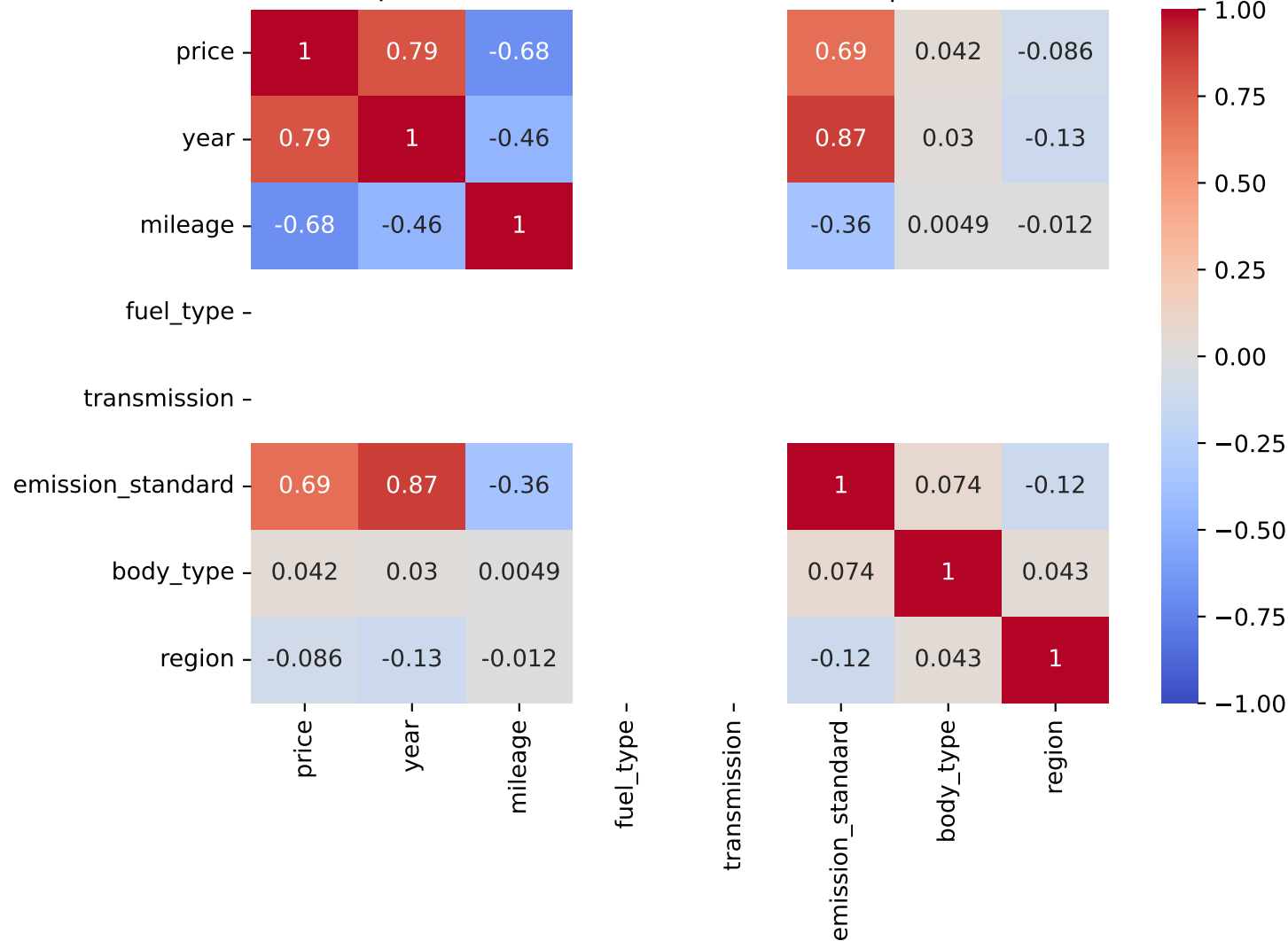
Spearman Correlation - Model: corsa | Fuel: 4
