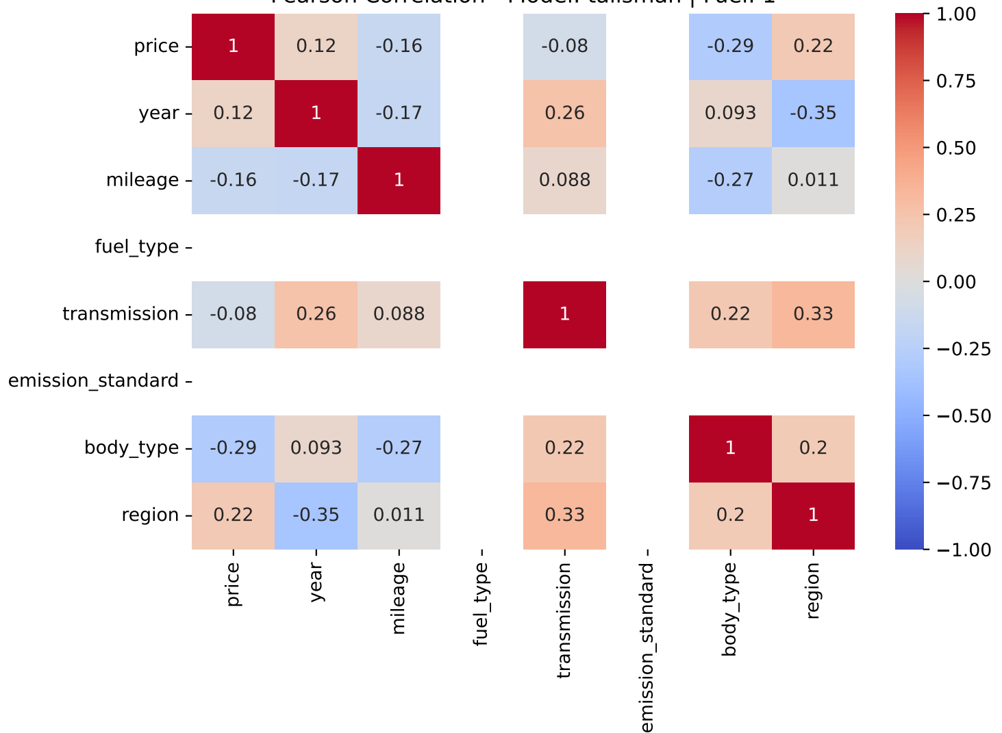
Pearson Correlation - Model: talisman | Fuel: 1
