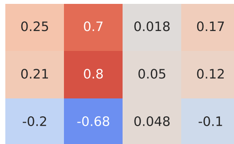
Spearman Correlation - Model: caddy | Fuel: 1
