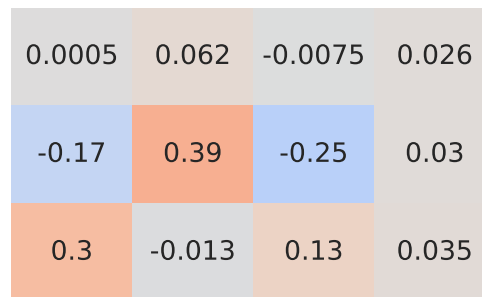
Pearson Correlation - Model: 500x | Fuel: 4
