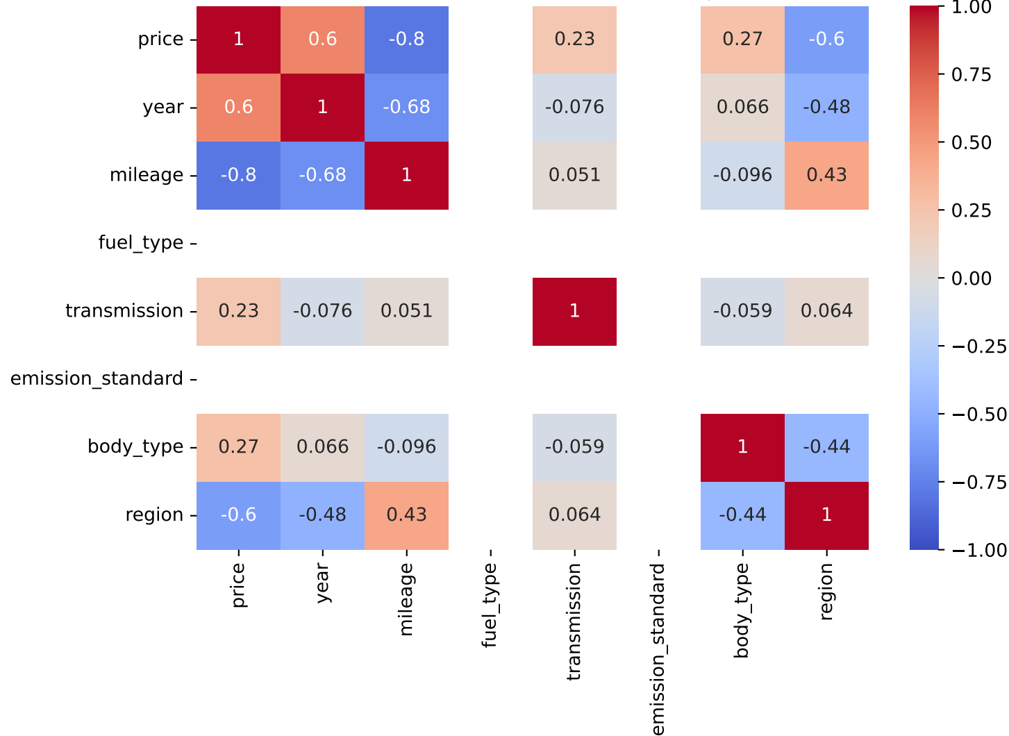
Pearson Correlation - Model: renegade | Fuel: 4
