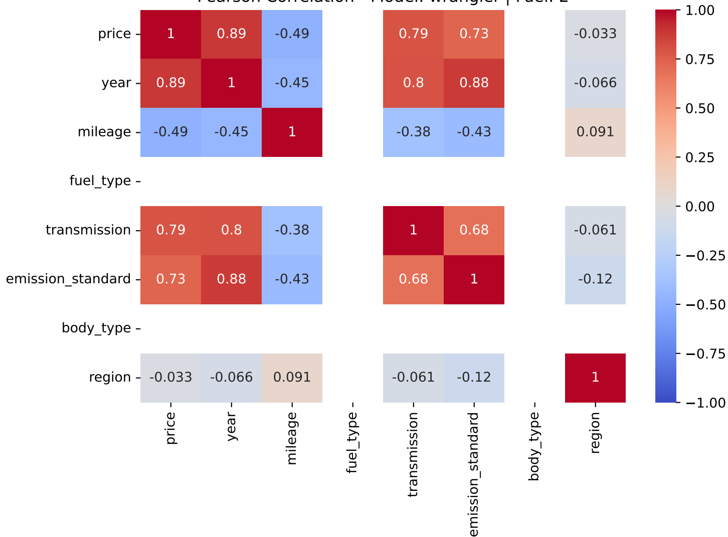
Pearson Correlation - Model: wrangler | Fuel: 2
