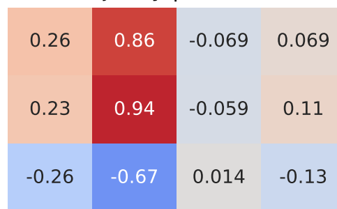
Spearman Correlation - Model: jimny | Fuel: 2
