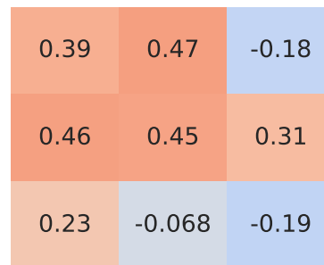
Spearman Correlation - Model: alto | Fuel: 2
