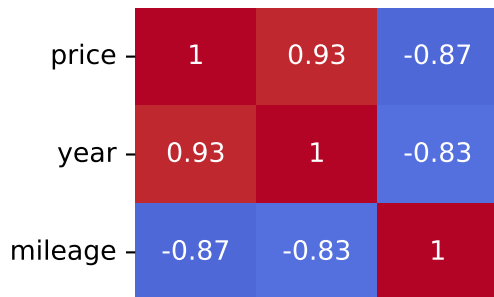
Spearman Correlation - Model: sportage | Fuel: 2
