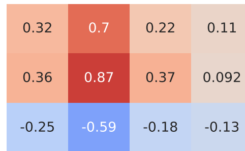
Pearson Correlation - Model: leon | Fuel: 1
