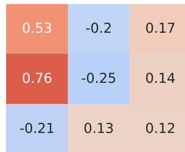
Pearson Correlation - Model: sx4 | Fuel: 2
