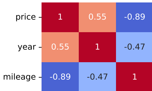
Spearman Correlation - Model: soul | Fuel: 1
