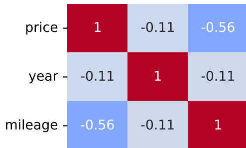
Pearson Correlation - Model: b-max | Fuel: 4
