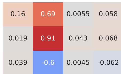
Pearson Correlation - Model: clio | Fuel: 2
