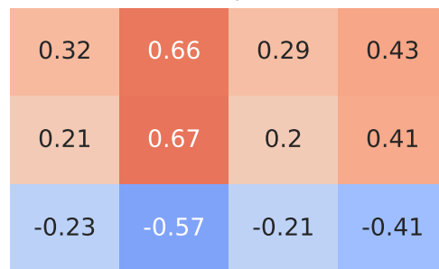
Spearman Correlation - Model: superb | Fuel: 1
