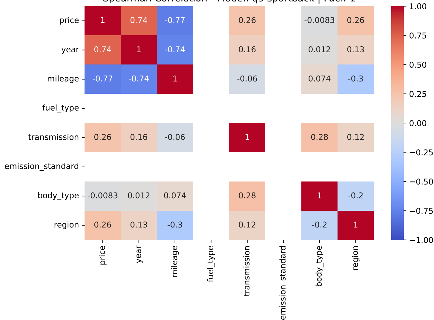
Spearman Correlation - Model: q3 sportback | Fuel: 1
