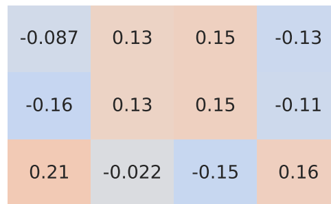
Pearson Correlation - Model: mokka | Fuel: 4
