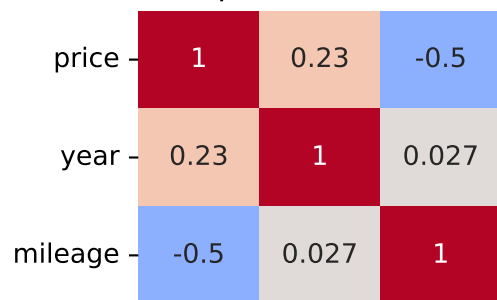
Spearman Correlation - Model: romeo tonale | Fuel: 3
