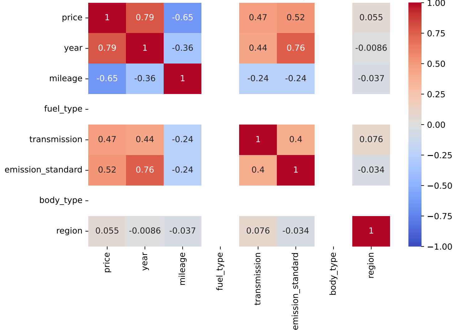
Pearson Correlation - Model: v60 | Fuel: 1
