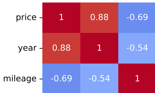
Pearson Correlation - Model: q5 | Fuel: 1
