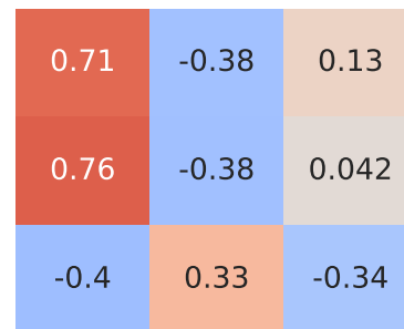
Spearman Correlation - Model: juke | Fuel: 4
