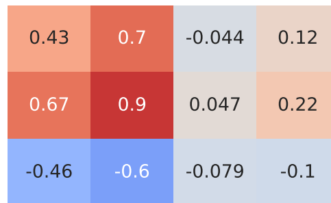
Pearson Correlation - Model: rover discovery | Fuel: 1
