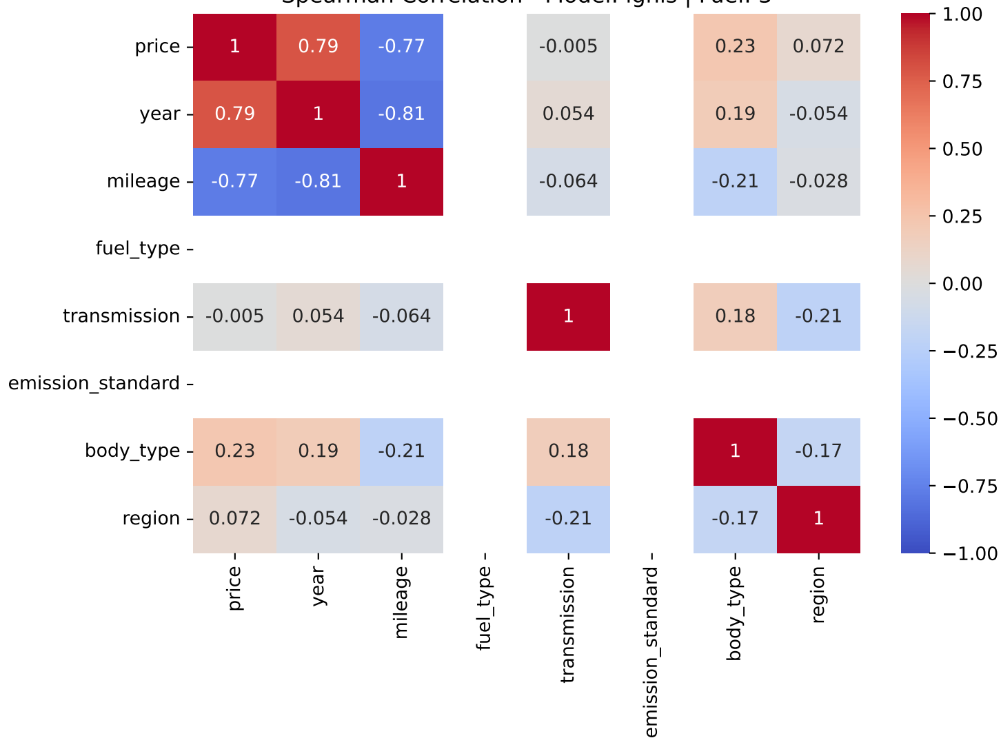
Spearman Correlation - Model: ignis | Fuel: 3
