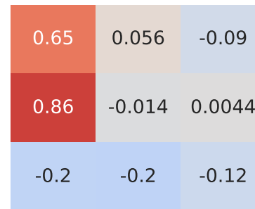
Spearman Correlation - Model: swift | Fuel: 1
