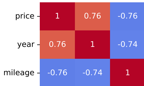
Pearson Correlation - Model: caddy | Fuel: 1
