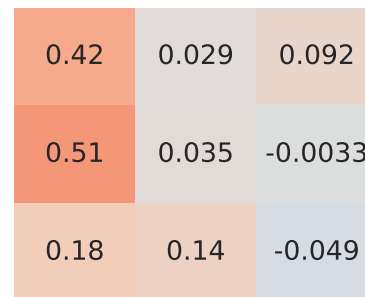
Spearman Correlation - Model: 500I | Fuel: 2
