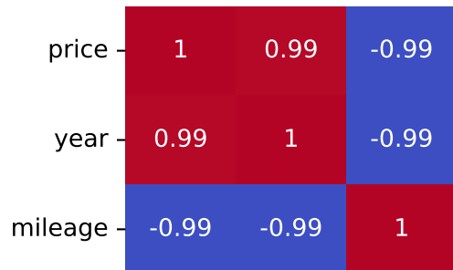
Spearman Correlation - Model: yeti | Fuel: 2
