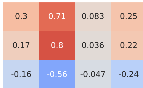
Pearson Correlation - Model: i10 | Fuel: 2
