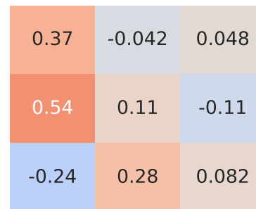
Spearman Correlation - Model: musa | Fuel: 4
