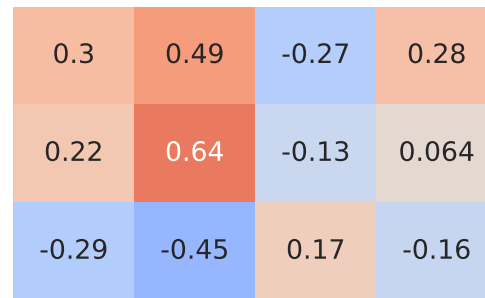
Spearman Correlation - Model: focus | Fuel: 2
