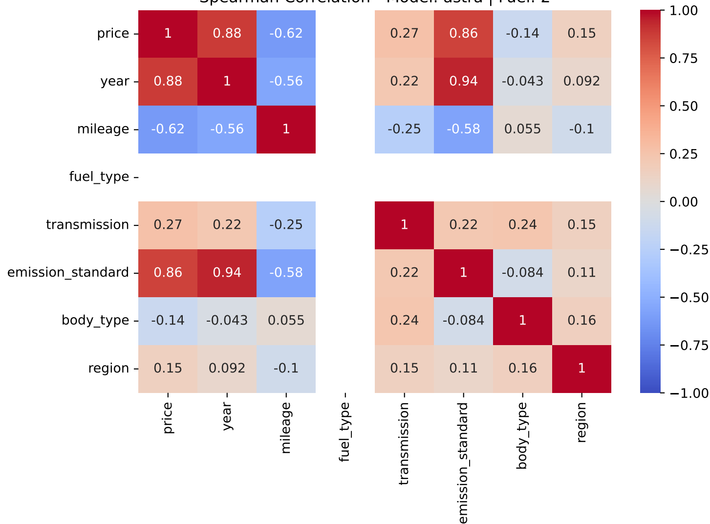
Spearman Correlation - Model: astra | Fuel: 2
