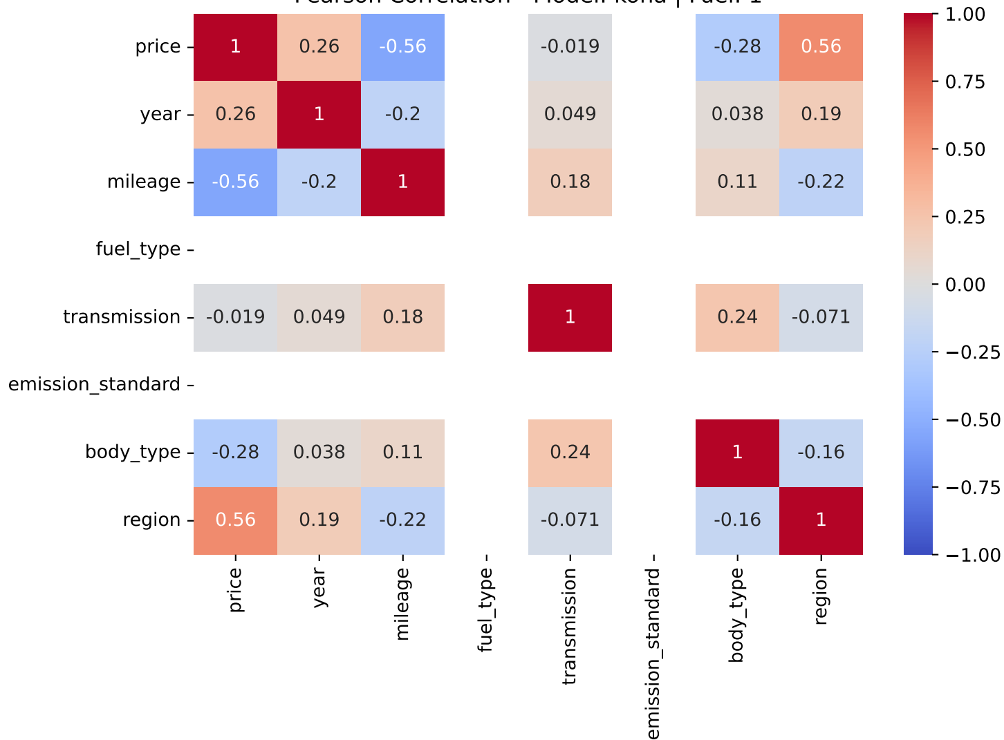
Pearson Correlation - Model: kona | Fuel: 1
