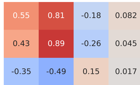
Pearson Correlation - Model: meriva | Fuel: 2
