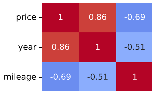
Spearman Correlation - Model: mondeo | Fuel: 1
