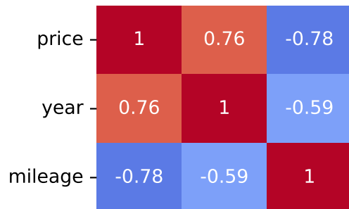
Spearman Correlation - Model: 308 | Fuel: 1
