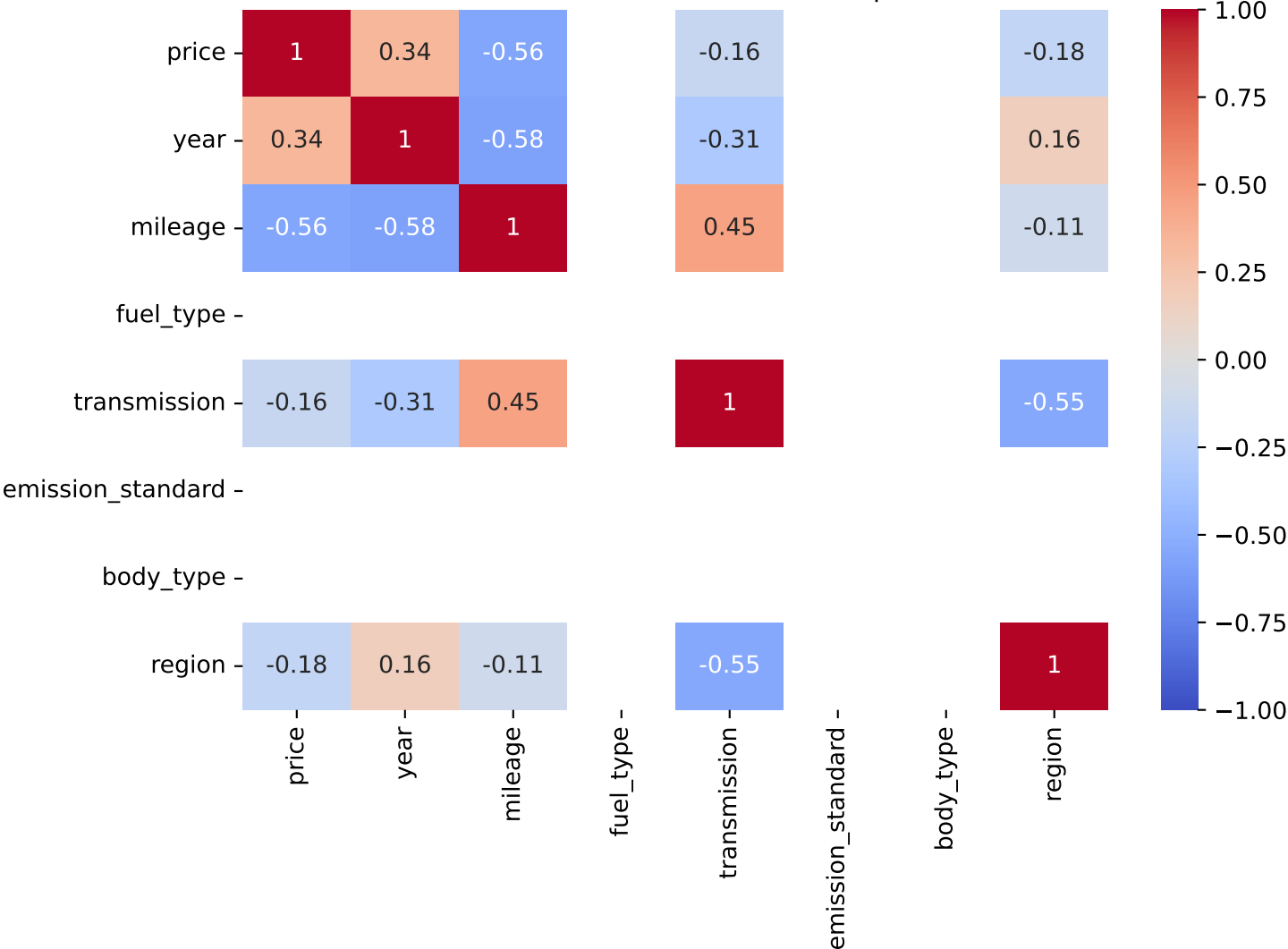
Pearson Correlation - Model: x-trail | Fuel: 3
