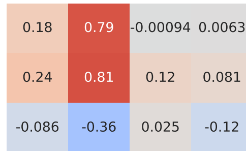
Spearman Correlation - Model: x6 | Fuel: 1
