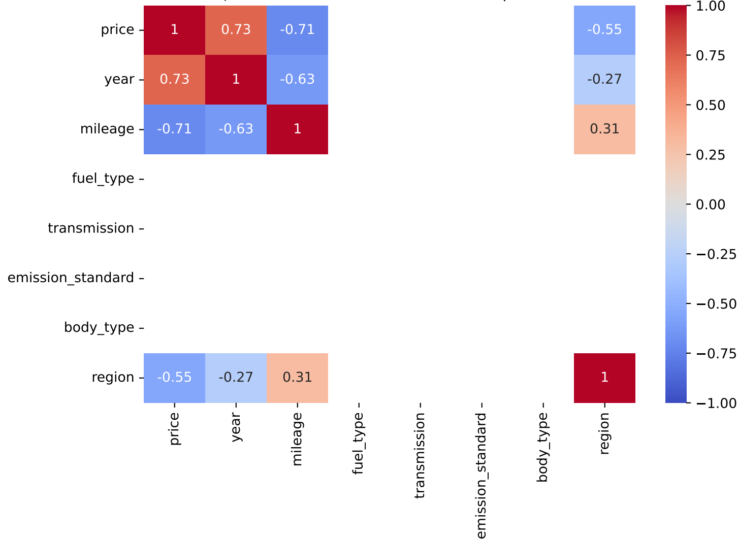
Spearman Correlation - Model: id.4 | Fuel: 0
