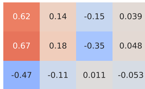
Spearman Correlation - Model: a3 | Fuel: 5
