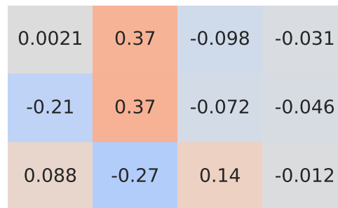
Spearman Correlation - Model: compass | Fuel: 1
