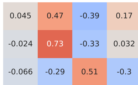
Spearman Correlation - Model: adam | Fuel: 2
