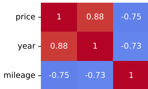
Spearman Correlation - Model: tiguan | Fuel: 2
