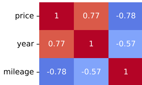
Spearman Correlation - Model: 500I | Fuel: 4
