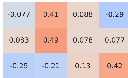
Pearson Correlation - Model: touran | Fuel: 5
