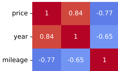
Pearson Correlation - Model: tiguan | Fuel: 1
