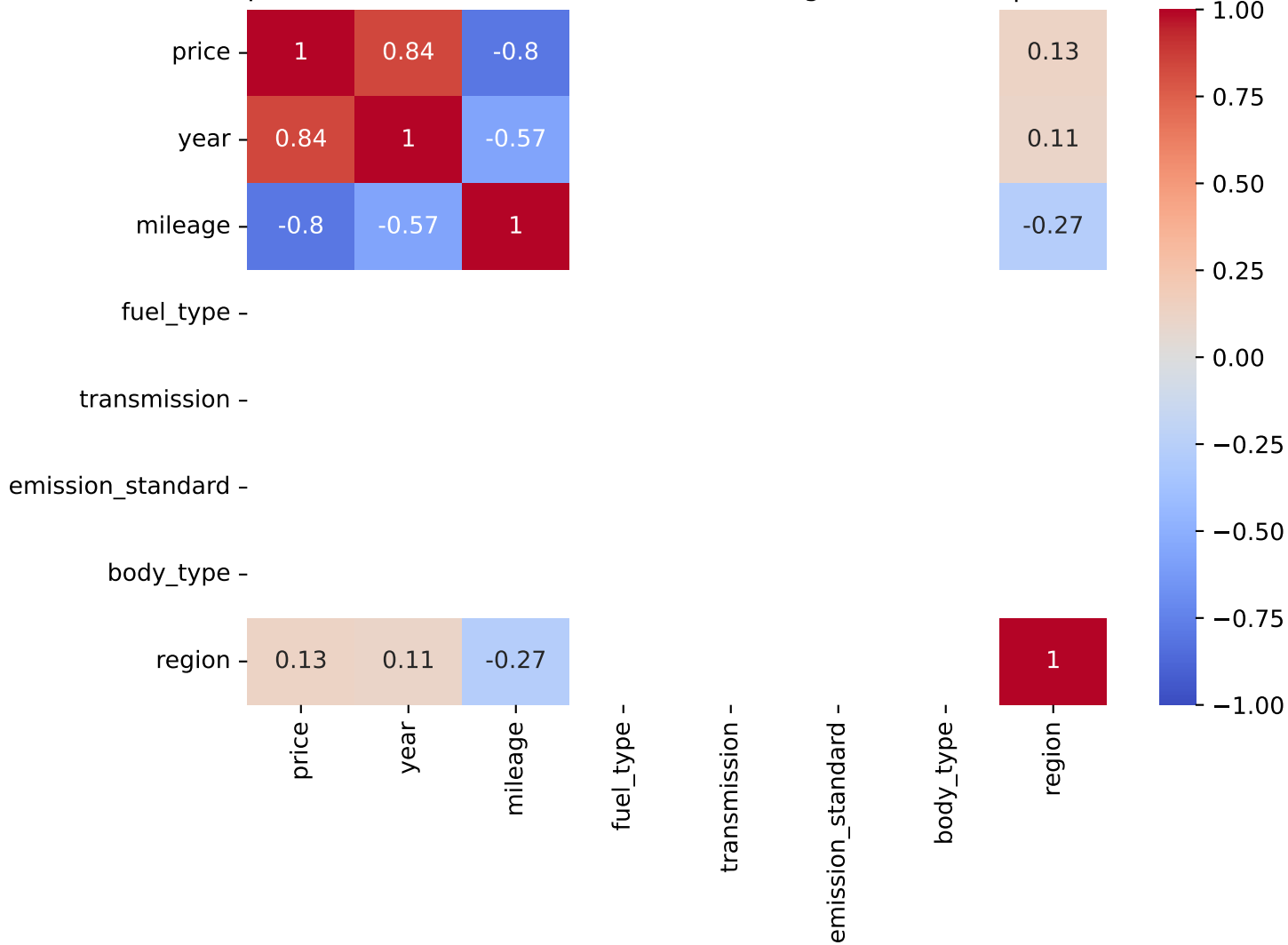
Spearman Correlation - Model: rover range rover velar | Fuel: 3
