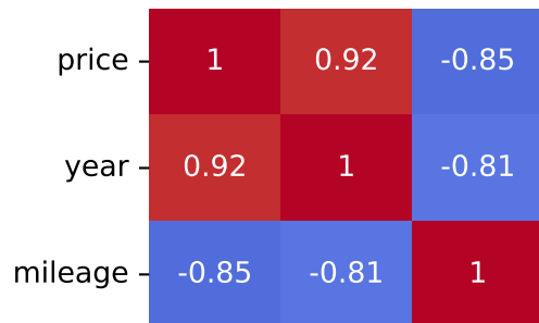
Spearman Correlation - Model: corsa | Fuel: 2
