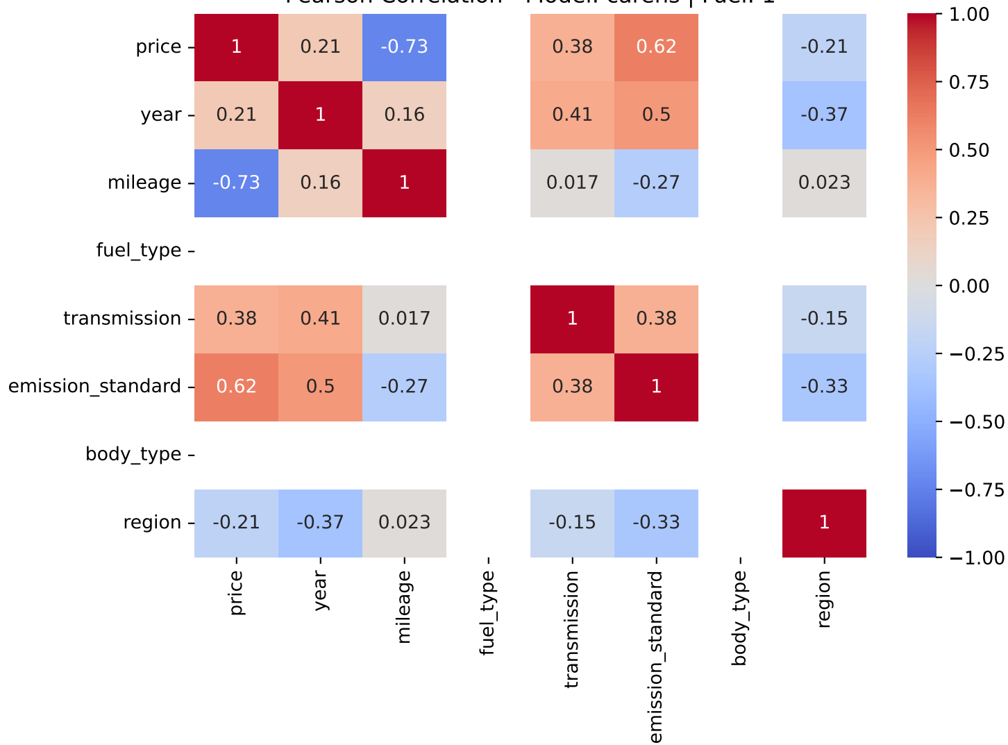
Pearson Correlation - Model: carens | Fuel: 1
