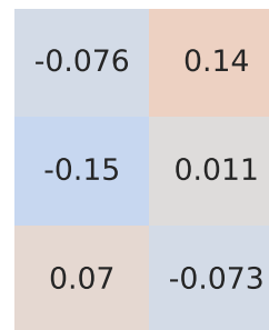
Spearman Correlation - Model: arona | Fuel: 5
