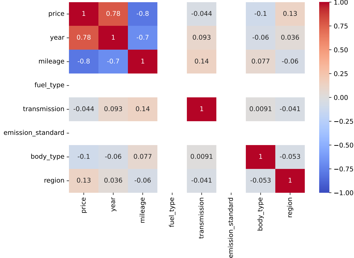
Spearman Correlation - Model: crossland | Fuel: 1
