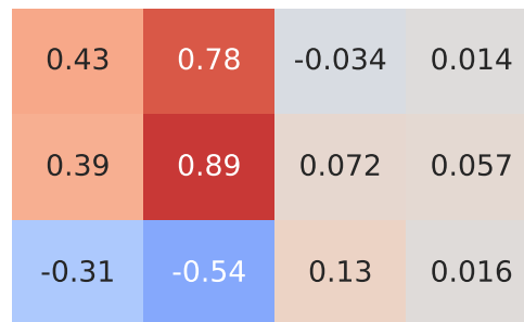
Pearson Correlation - Model: astra | Fuel: 1
