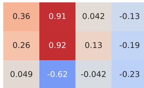
Spearman Correlation - Model: sharan | Fuel: 1
