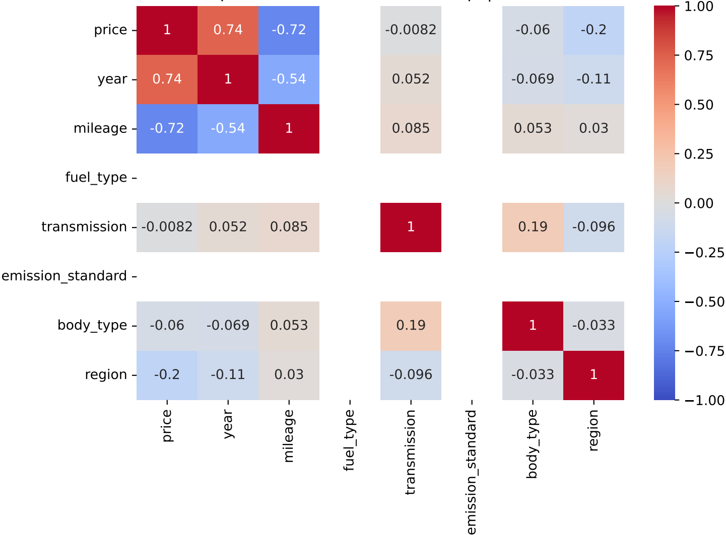
Spearman Correlation - Model: q5 | Fuel: 3
