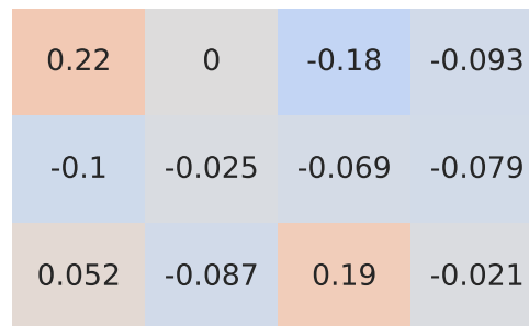
Spearman Correlation - Model: karoq | Fuel: 1
