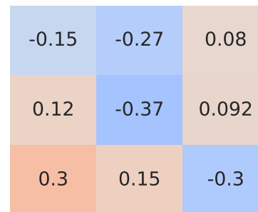
Spearman Correlation - Model: fusion | Fuel: 2
