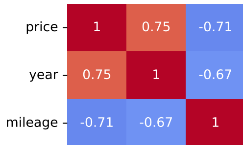
Pearson Correlation - Model: 500x | Fuel: 2
