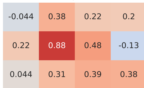
Spearman Correlation - Model: altea | Fuel: 1
