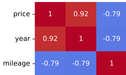
Spearman Correlation - Model: one | Fuel: 2
