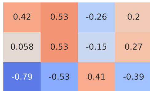
Spearman Correlation - Model: tucson | Fuel: 2
