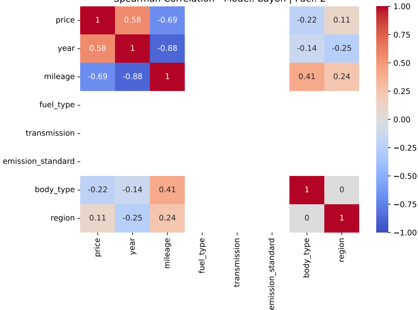
Spearman Correlation - Model: bayon | Fuel: 2
