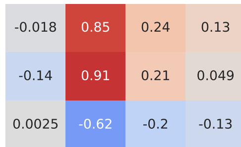
Spearman Correlation - Model: c1 | Fuel: 2
