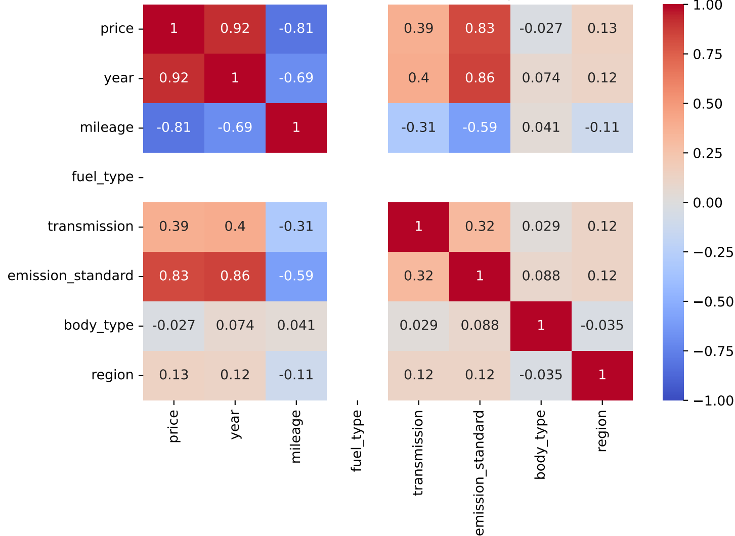
Spearman Correlation - Model: focus | Fuel: 1
