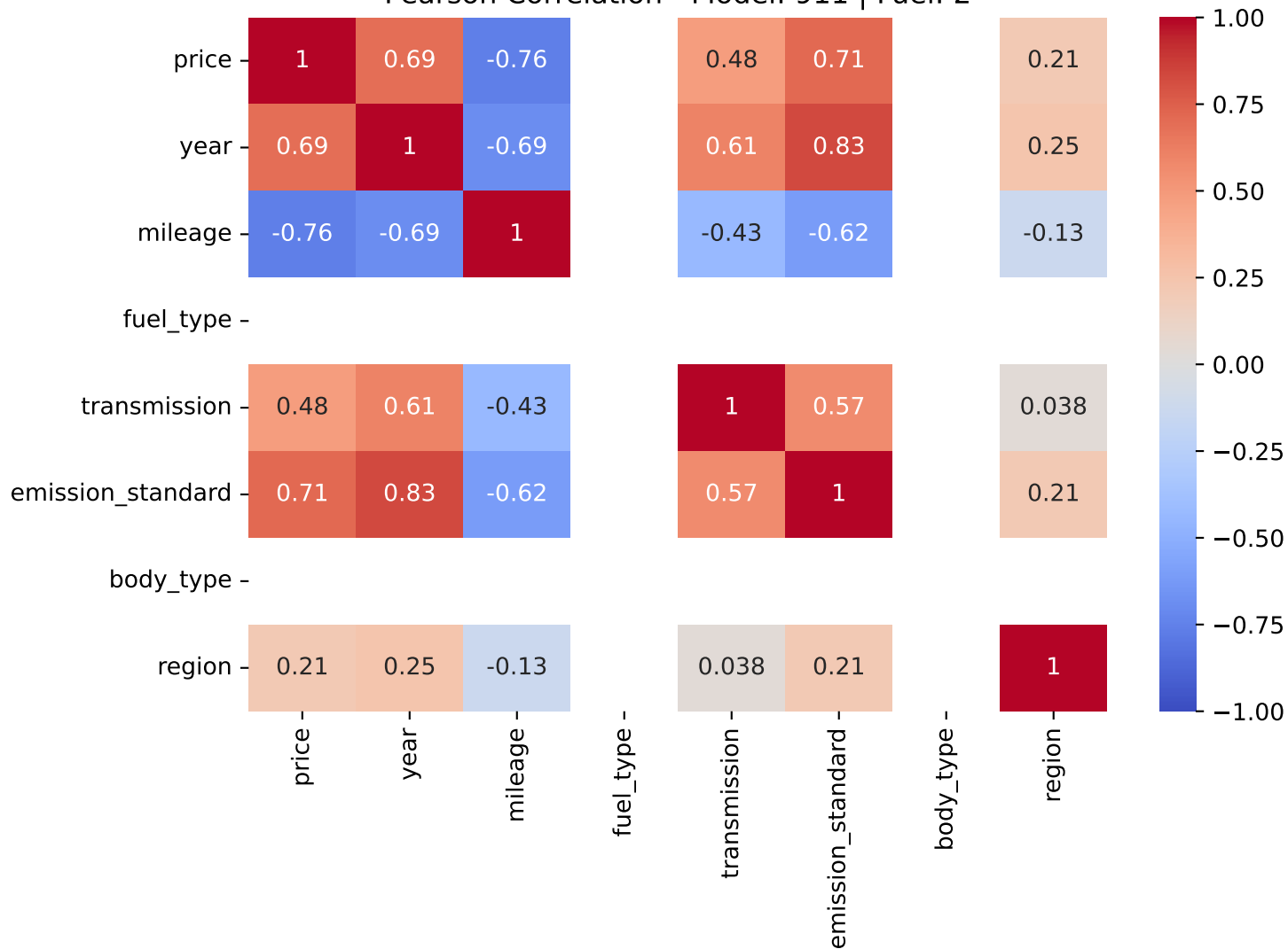
Pearson Correlation - Model: 911 | Fuel: 2
