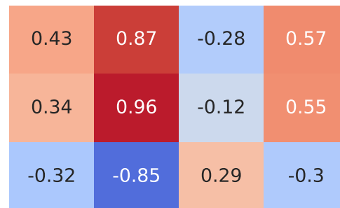
Pearson Correlation - Model: berlingo | Fuel: 2
