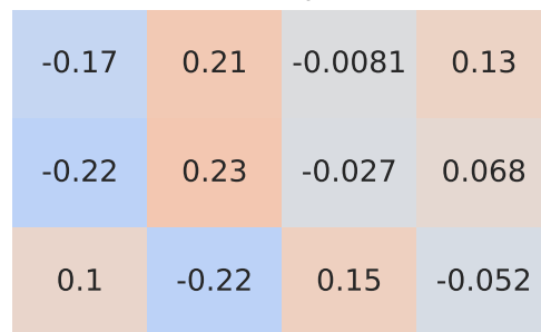
Spearman Correlation - Model: ecosport | Fuel: 2
