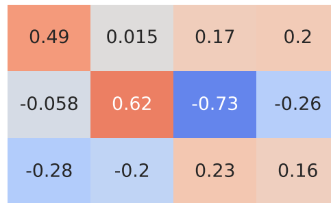
Pearson Correlation - Model: romeo 156 | Fuel: 2
