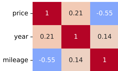
Spearman Correlation - Model: fusion | Fuel: 1
