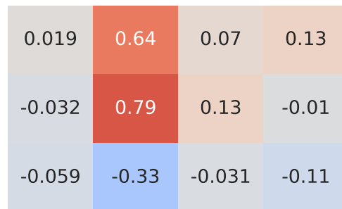
Spearman Correlation - Model: berlingo | Fuel: 1
