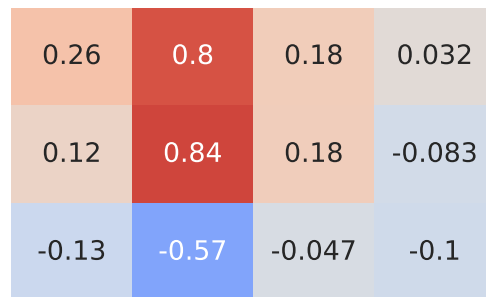
Spearman Correlation - Model: twingo | Fuel: 2
