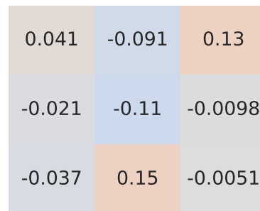
Spearman Correlation - Model: panda | Fuel: 3
