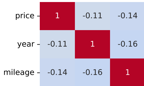
Spearman Correlation - Model: bravo | Fuel: 4
