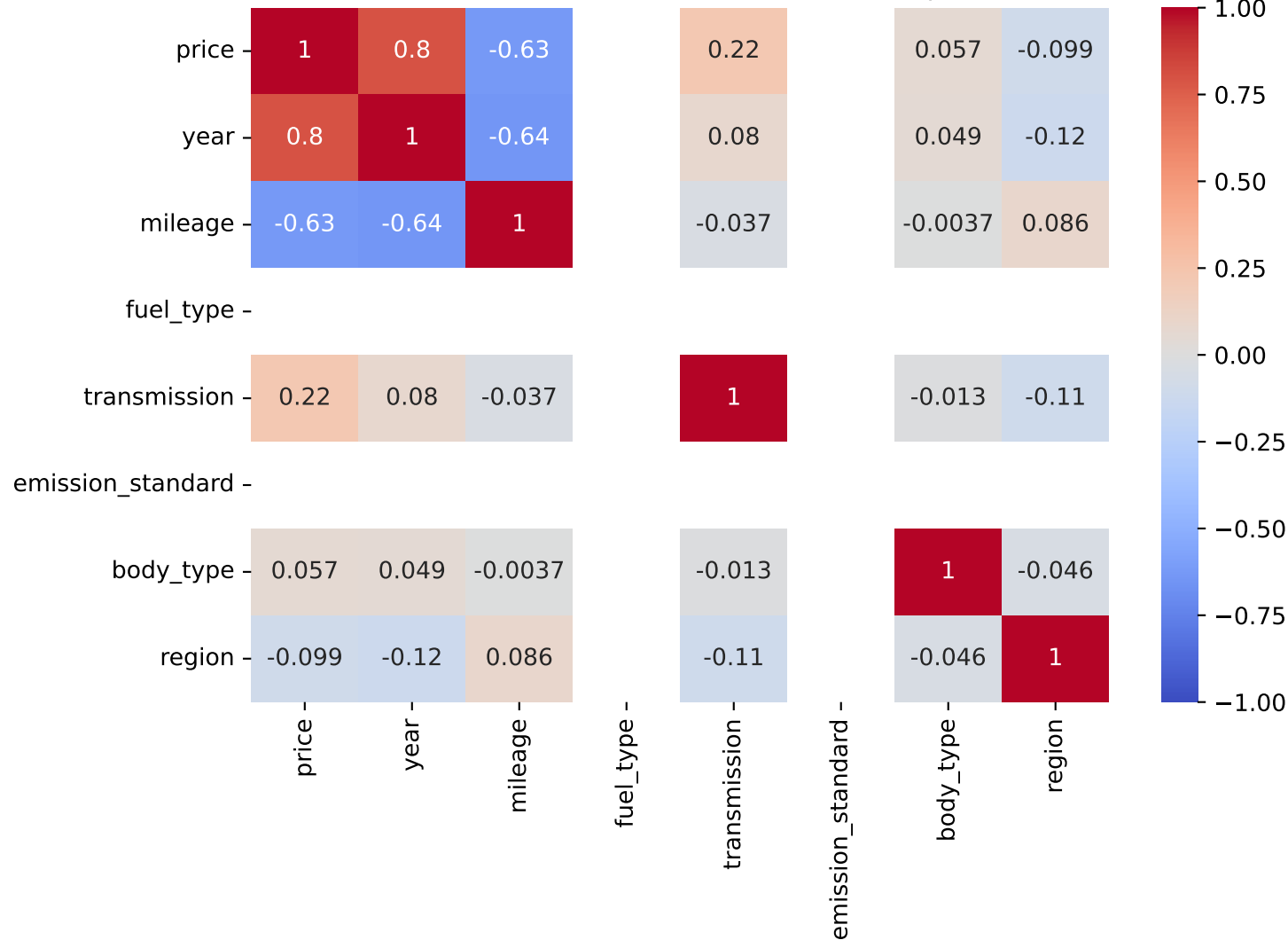
Spearman Correlation - Model: c3 aircross | Fuel: 2
