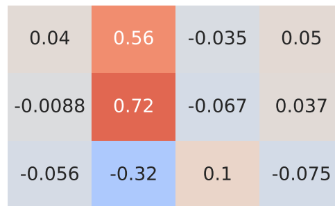
Pearson Correlation - Model: tucson | Fuel: 1
