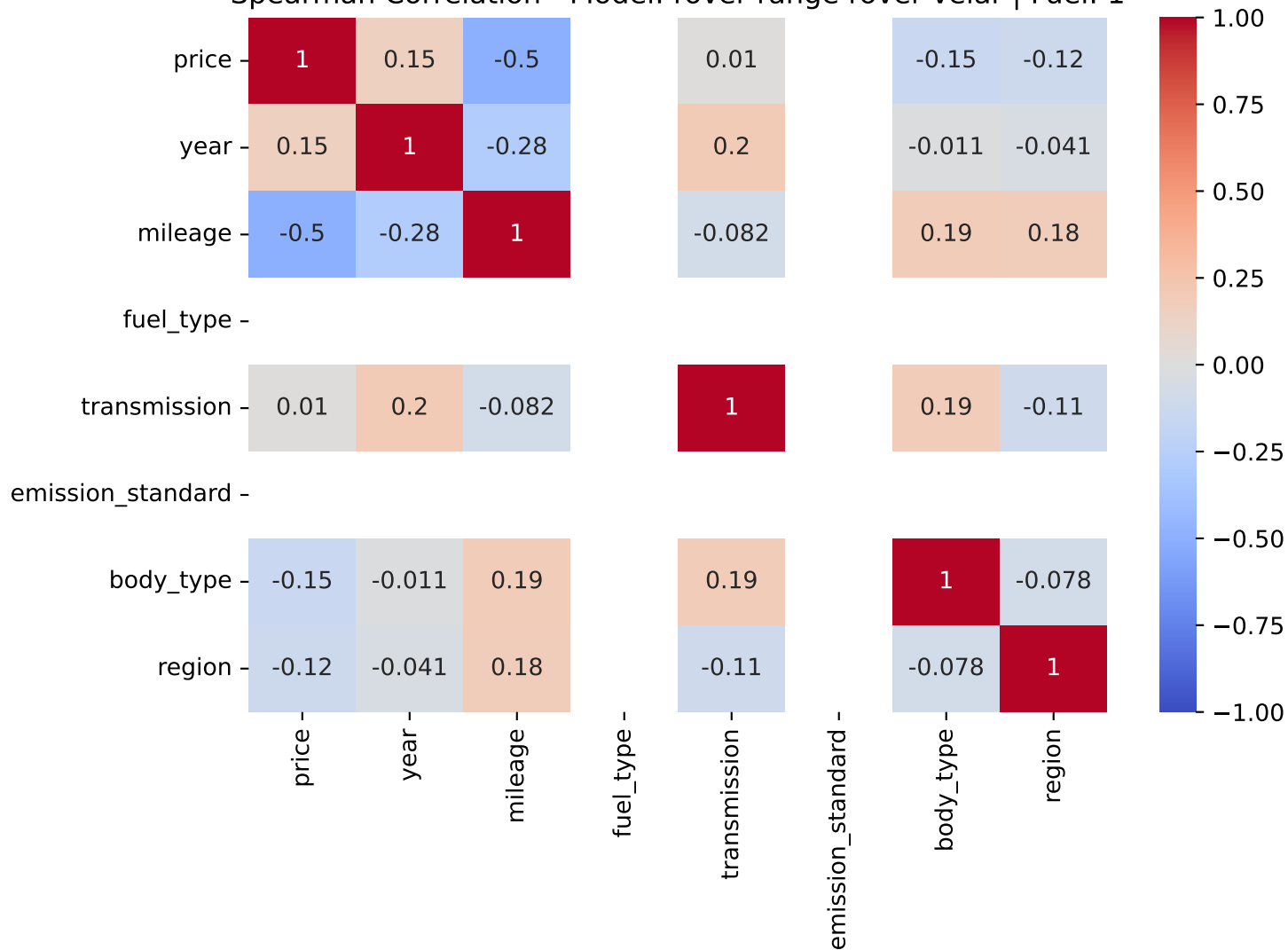
Spearman Correlation - Model: rover range rover velar | Fuel: 1
