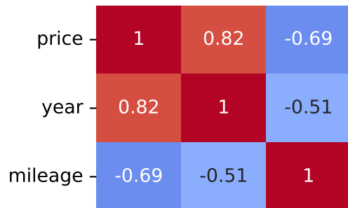
Spearman Correlation - Model: rio | Fuel: 4
