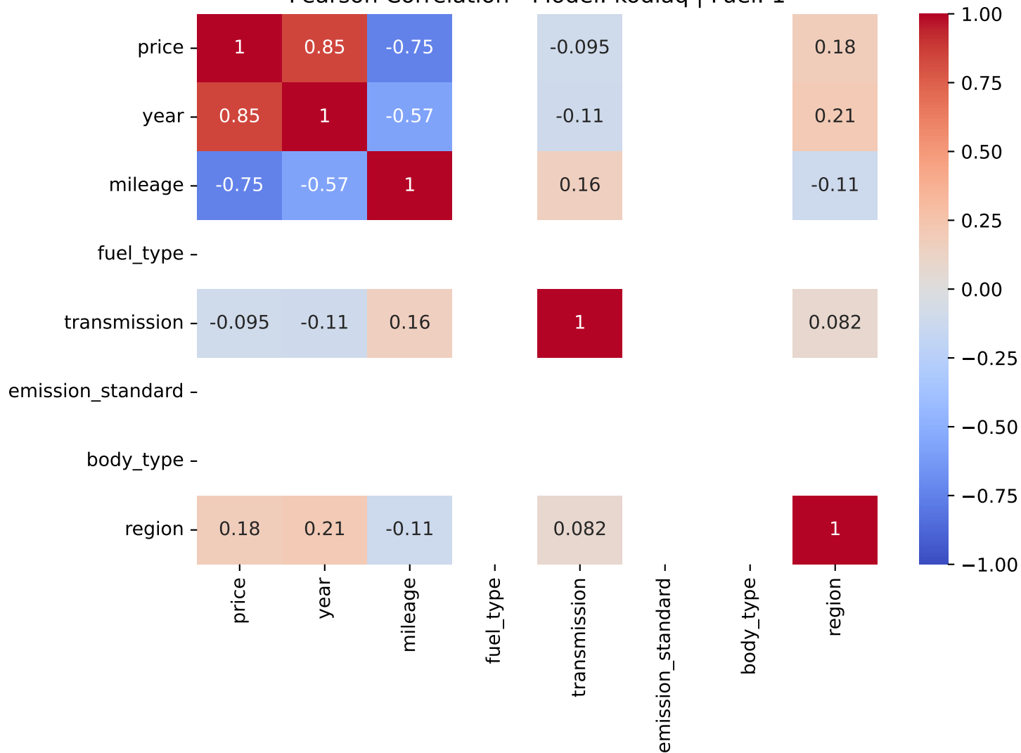
Pearson Correlation - Model: kodiaq | Fuel: 1
