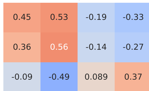
Spearman Correlation - Model: tiguan | Fuel: 2
