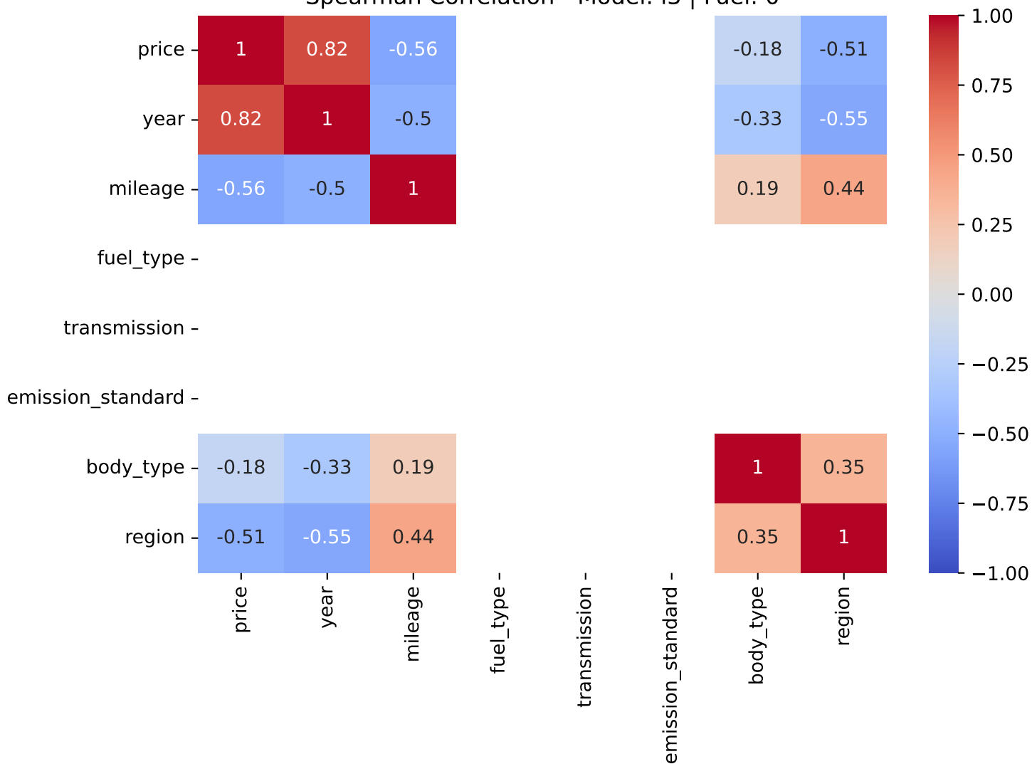
Spearman Correlation - Model: i3 | Fuel: 0
