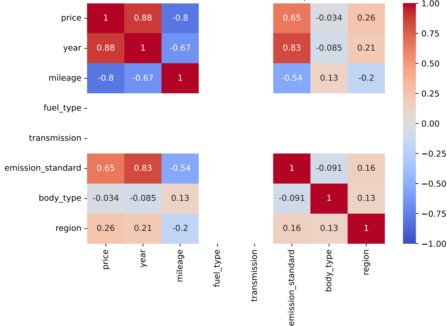
Pearson Correlation - Model: fiesta | Fuel: 4
