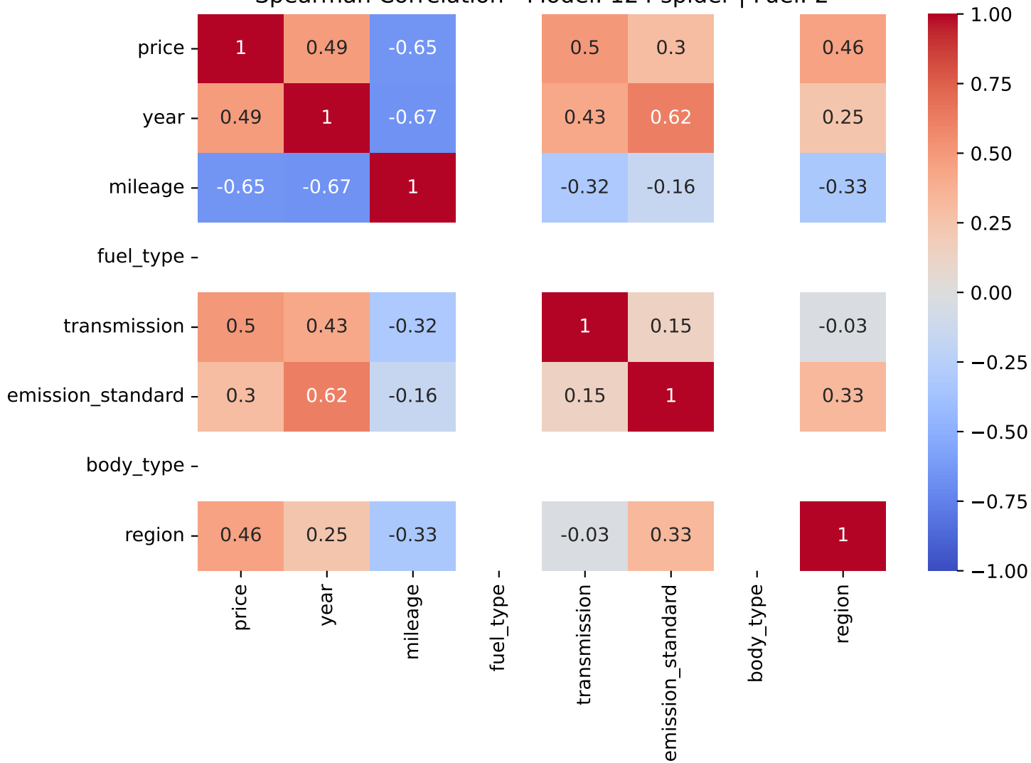
Spearman Correlation - Model: 124 spider | Fuel: 2
