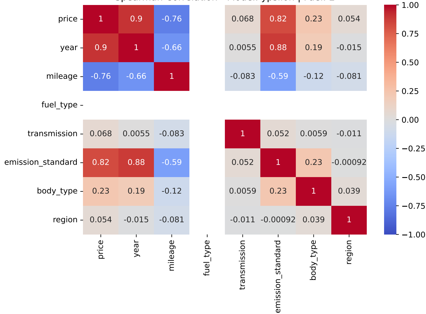
Spearman Correlation - Model: ypsilon | Fuel: 2
