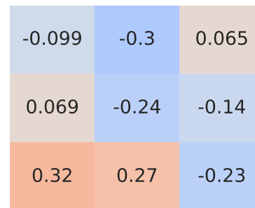
Pearson Correlation - Model: fusion | Fuel: 2
