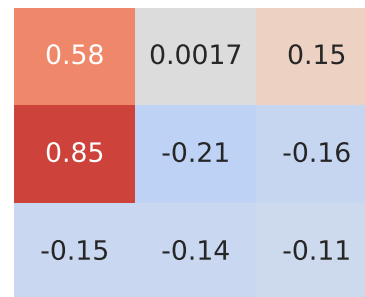
Pearson Correlation - Model: ix20 | Fuel: 1
