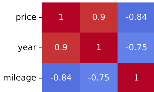
Pearson Correlation - Model: qashqai | Fuel: 2
