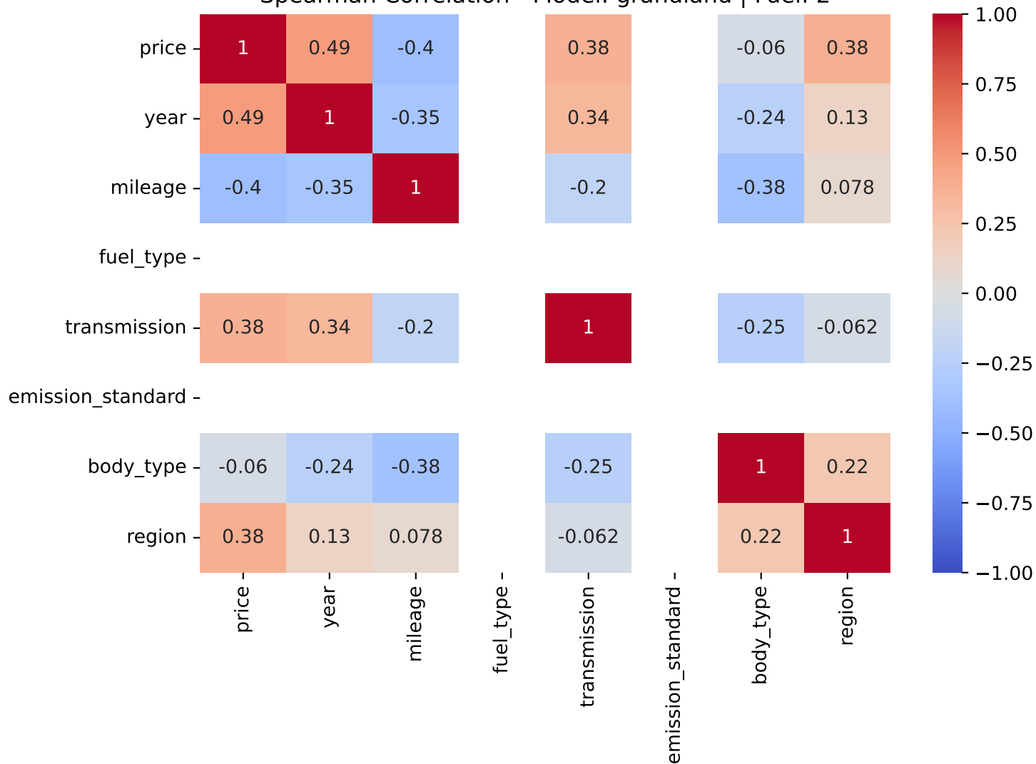
Spearman Correlation - Model: grandland | Fuel: 2
