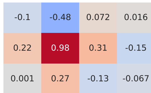
Pearson Correlation - Model: delta | Fuel: 2
