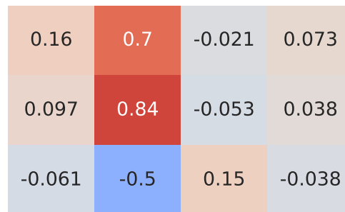
Spearman Correlation - Model: 500 | Fuel: 2
