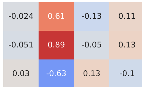
Pearson Correlation - Model: yaris | Fuel: 2
