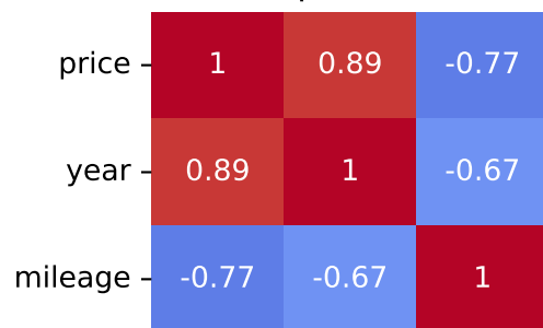
Spearman Correlation - Model: passat | Fuel: 1
