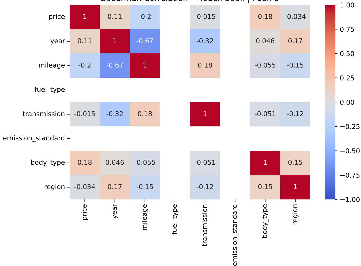
Spearman Correlation - Model: 500x | Fuel: 3
