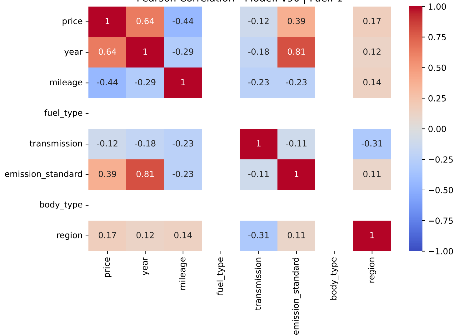
Pearson Correlation - Model: v50 | Fuel: 1
