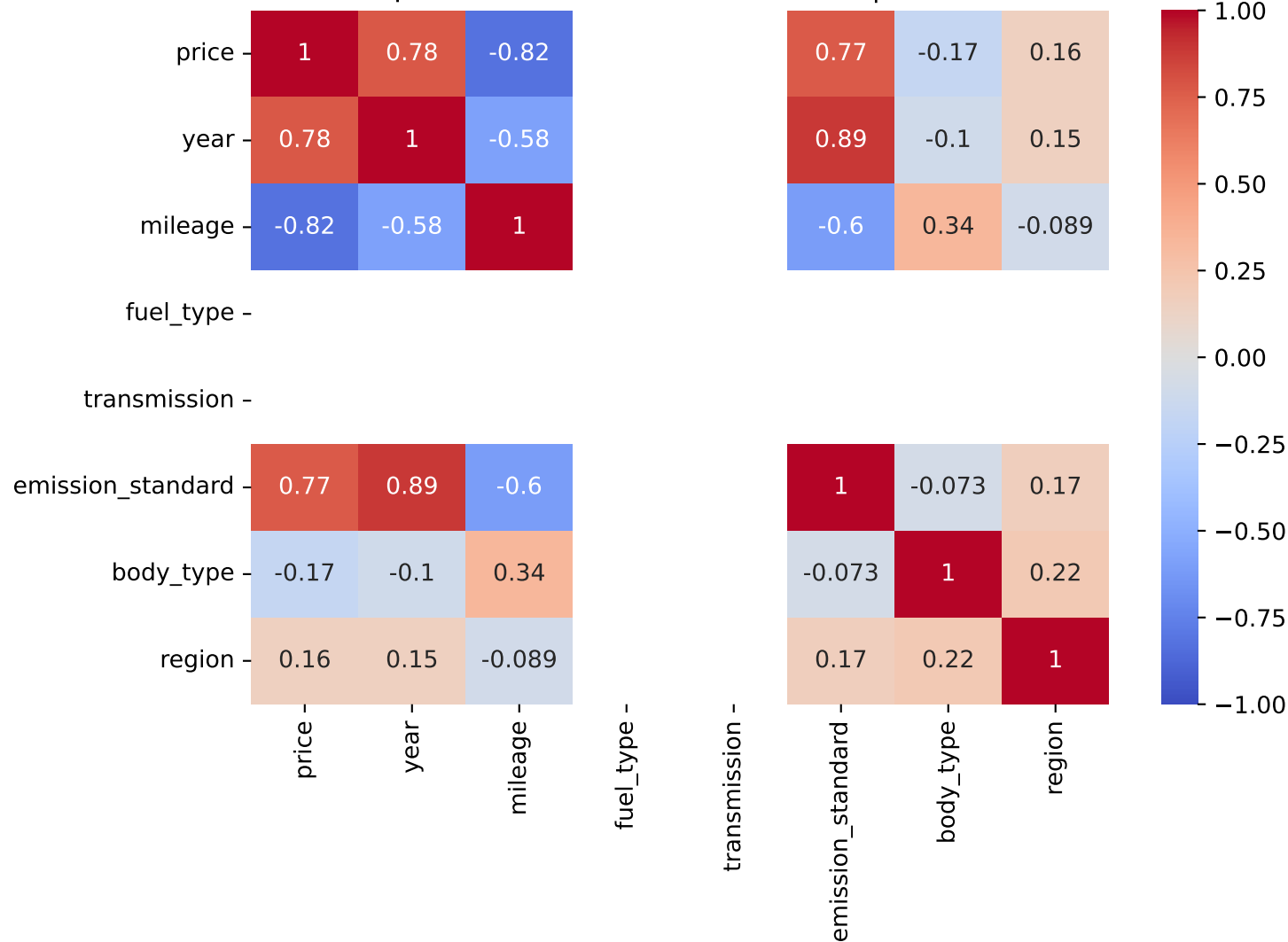
Spearman Correlation - Model: i20 | Fuel: 4
