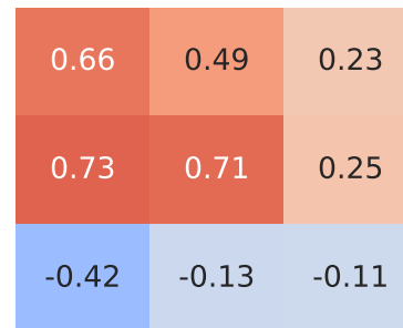
Pearson Correlation - Model: polo | Fuel: 4
