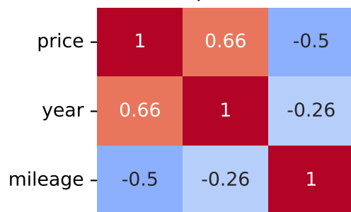
Spearman Correlation - Model: punto | Fuel: 4
