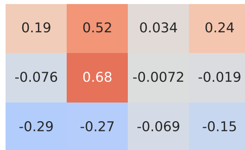
Pearson Correlation - Model: modus | Fuel: 1
