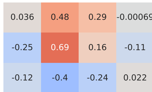
Spearman Correlation - Model: b-max | Fuel: 2
