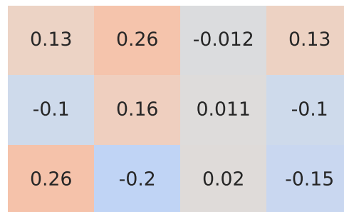
Spearman Correlation - Model: karl | Fuel: 2
