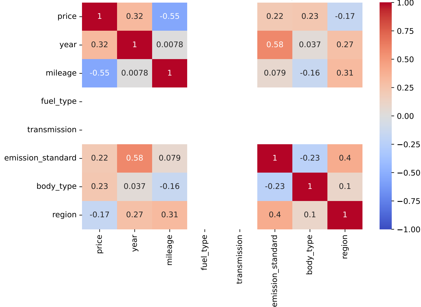
Spearman Correlation - Model: jimny | Fuel: 1
