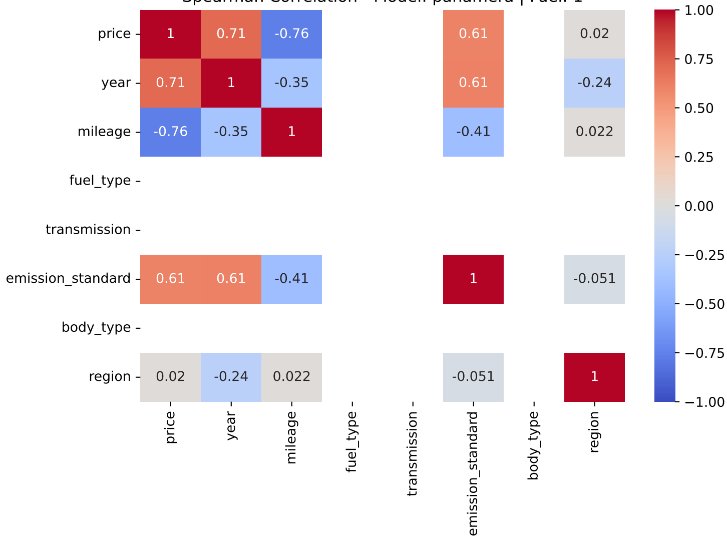
Spearman Correlation - Model: panamera | Fuel: 1
