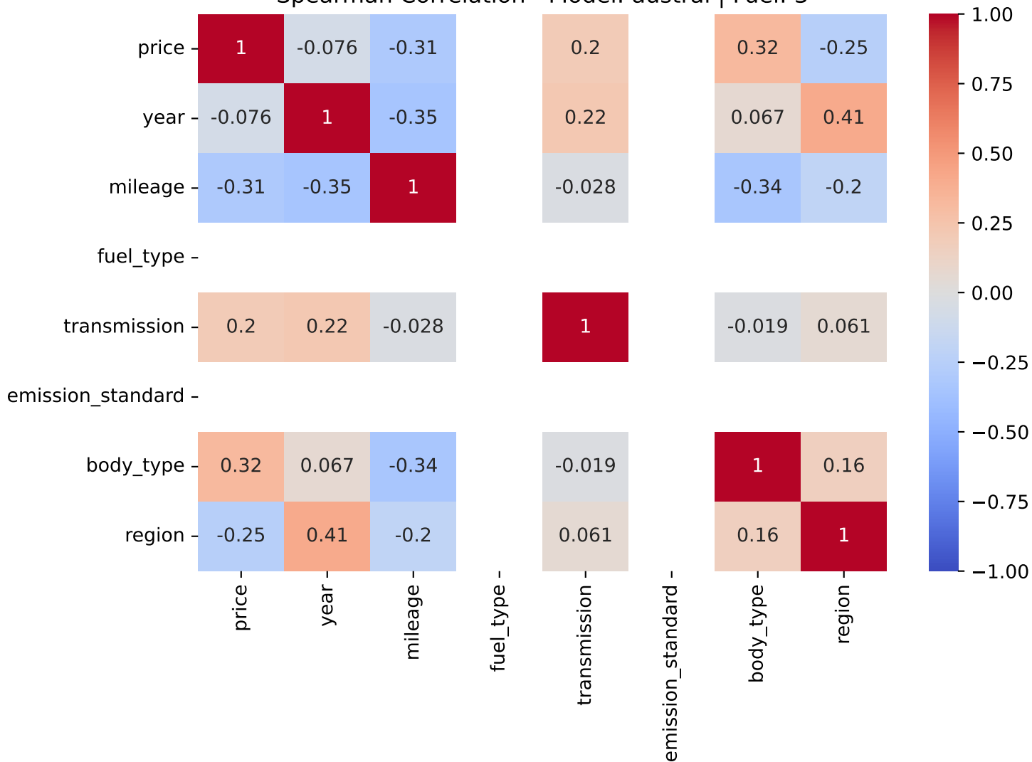
Spearman Correlation - Model: austral | Fuel: 3
