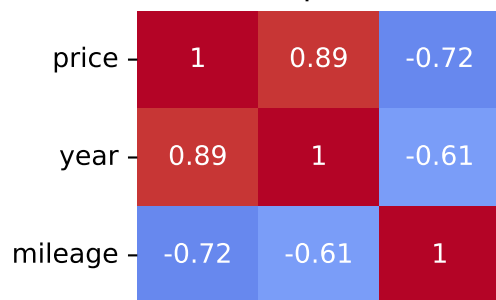
Spearman Correlation - Model: up | Fuel: 2
