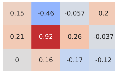
Spearman Correlation - Model: delta | Fuel: 2
