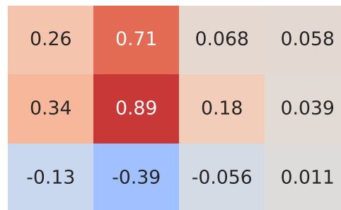
Pearson Correlation - Model: a6 | Fuel: 1
