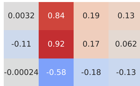
Pearson Correlation - Model: c1 | Fuel: 2
