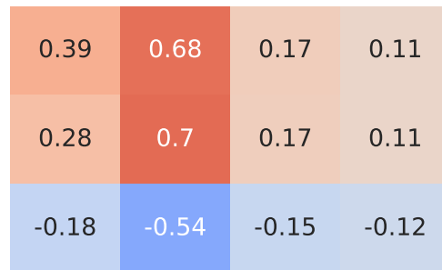
Spearman Correlation - Model: polo | Fuel: 2
