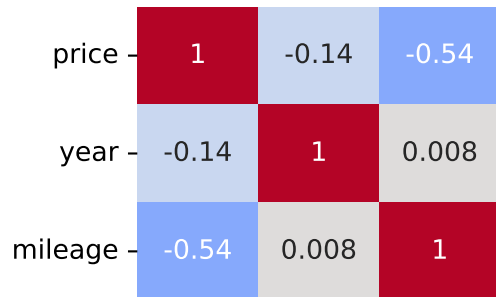
Spearman Correlation - Model: b-max | Fuel: 4
