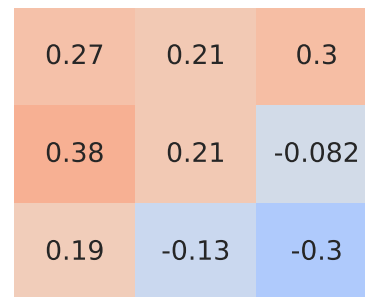
Pearson Correlation - Model: fusion | Fuel: 1
