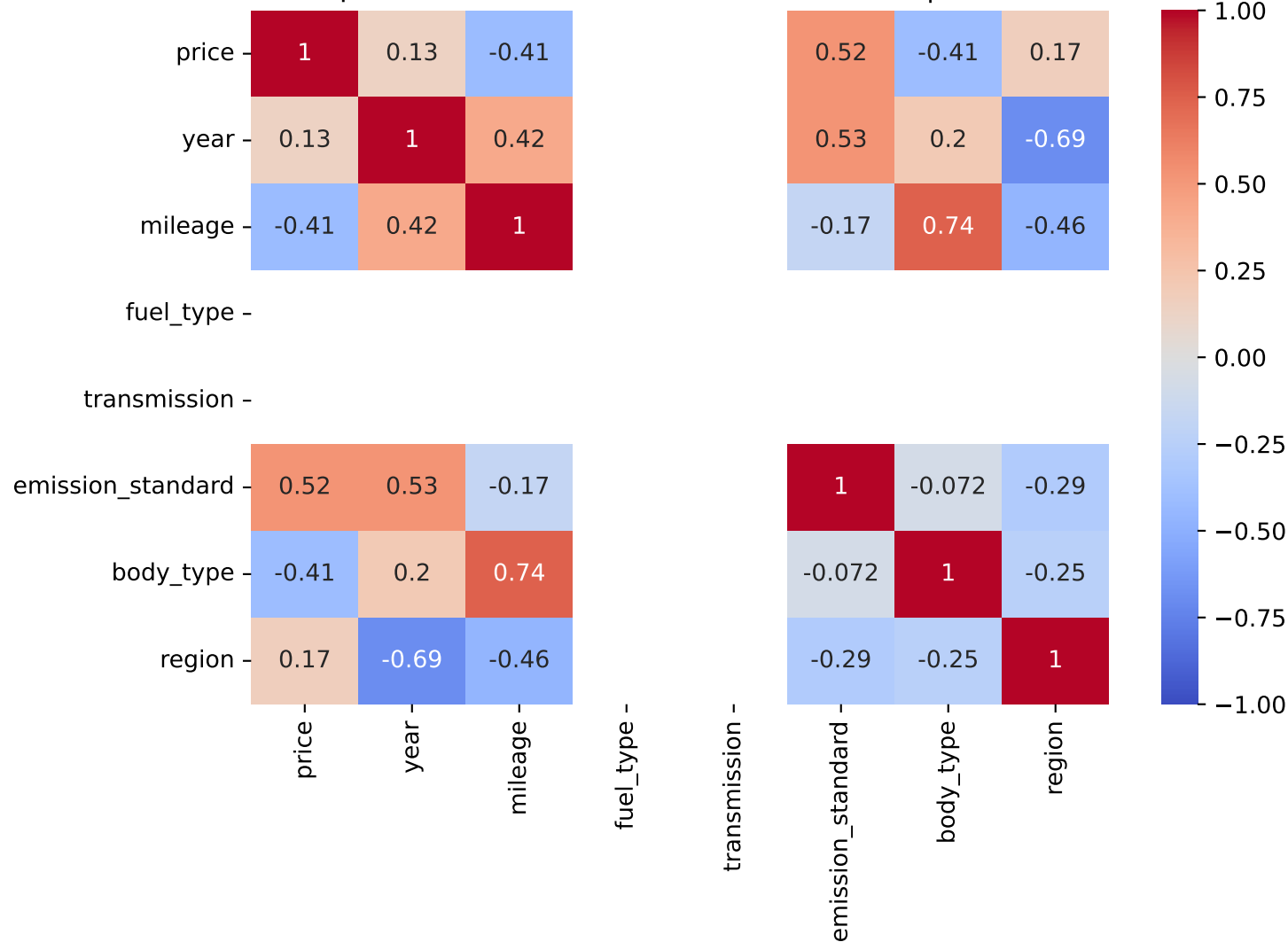
Spearman Correlation - Model: c4 aircross | Fuel: 1
