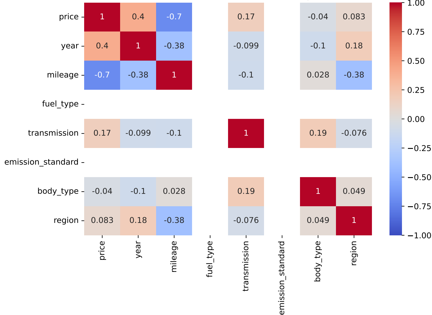
Pearson Correlation - Model: crossland x | Fuel: 2
