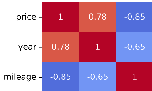
Spearman Correlation - Model: c-max | Fuel: 2
