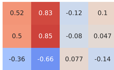
Spearman Correlation - Model: x3 | Fuel: 1
