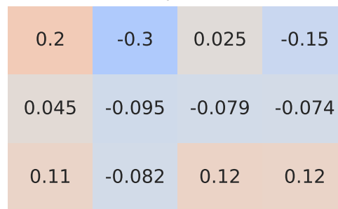
Pearson Correlation - Model: cromax | Fuel: 1
