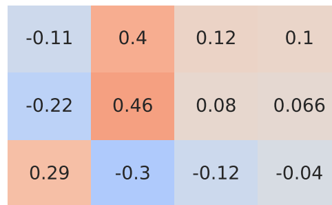
Spearman Correlation - Model: captur | Fuel: 2
