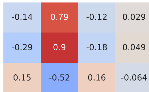
Pearson Correlation - Model: fortwo | Fuel: 2
