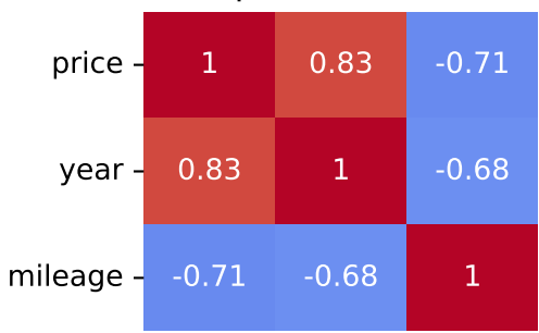
Spearman Correlation - Model: grand scenic | Fuel: 1
