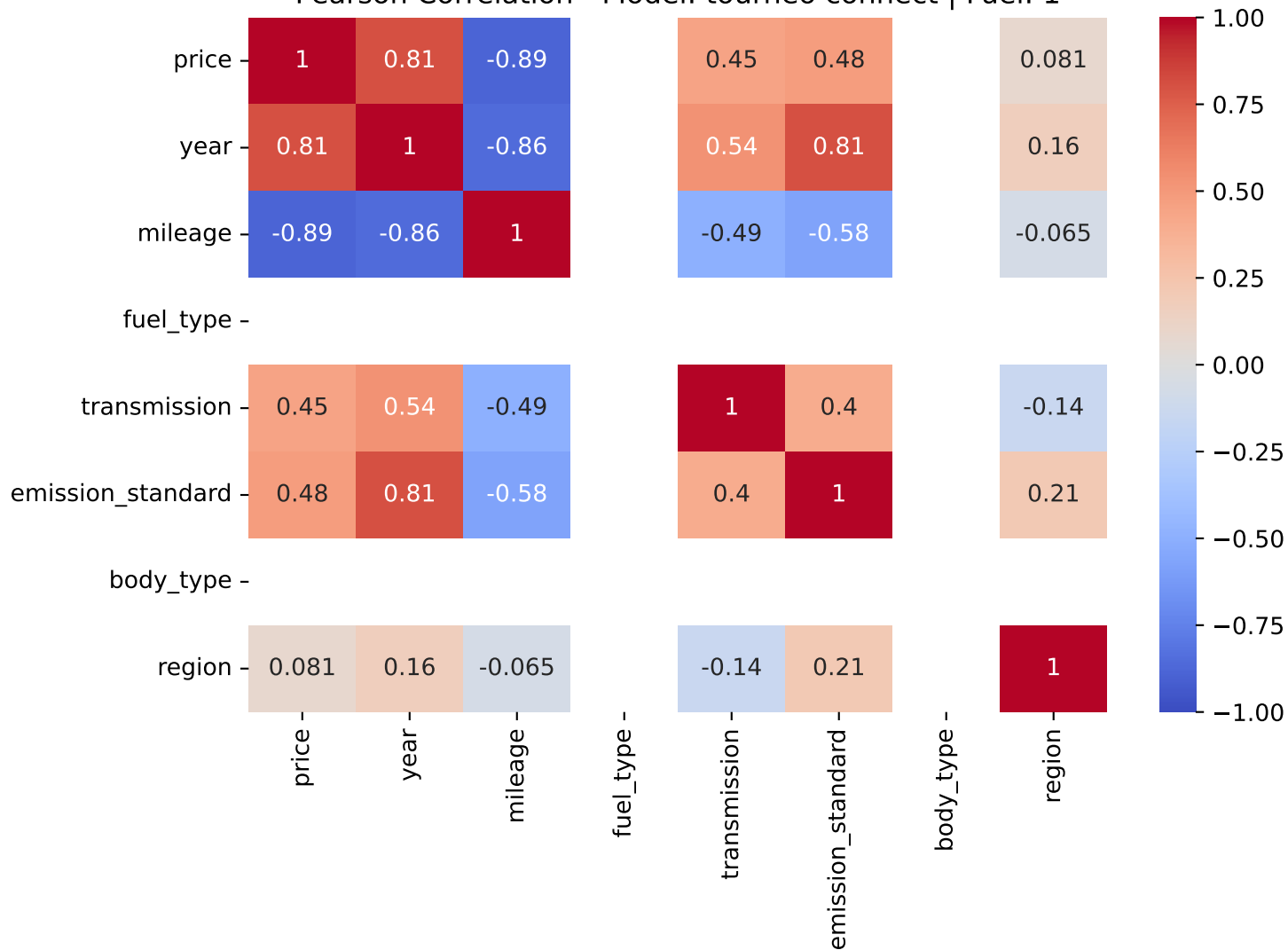
Pearson Correlation - Model: torneo connect | Fuel: 1
