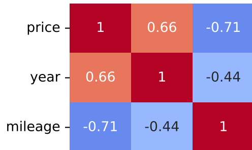
Pearson Correlation - Model: qubo | Fuel: 5
