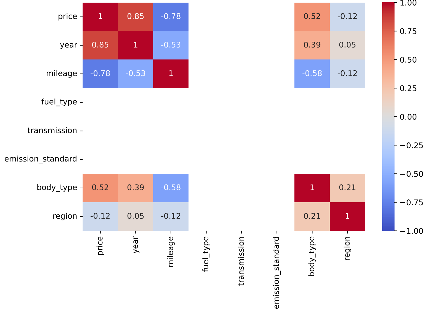
Pearson Correlation - Model: karl | Fuel: 4
