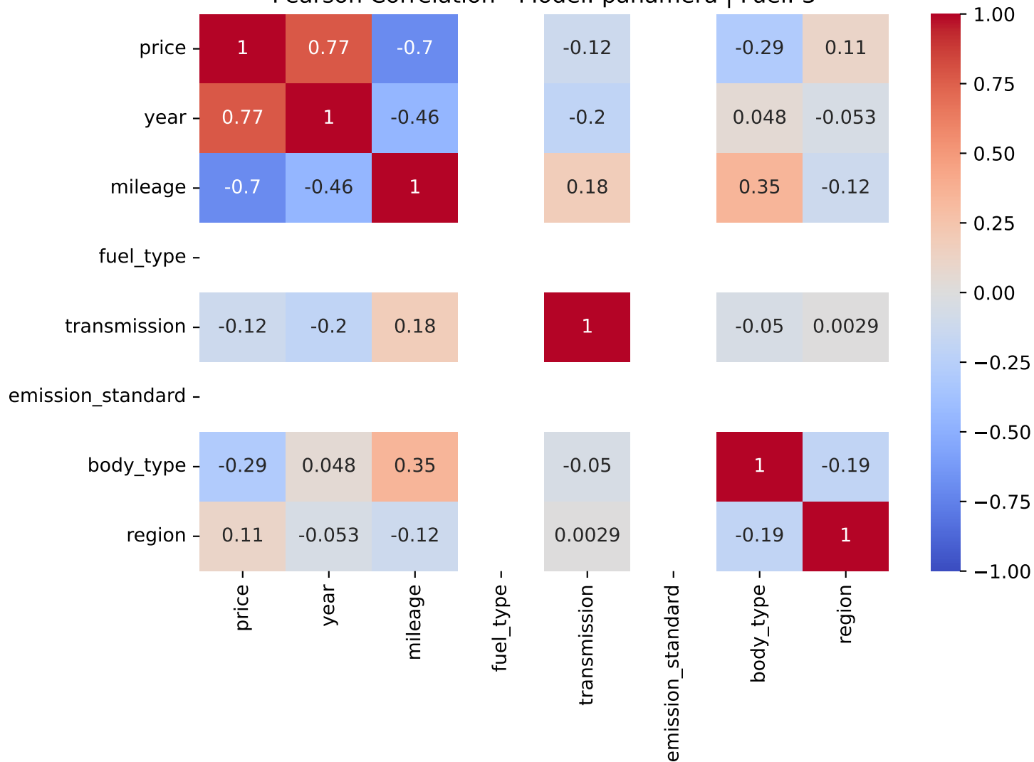
Pearson Correlation - Model: panamera | Fuel: 3
