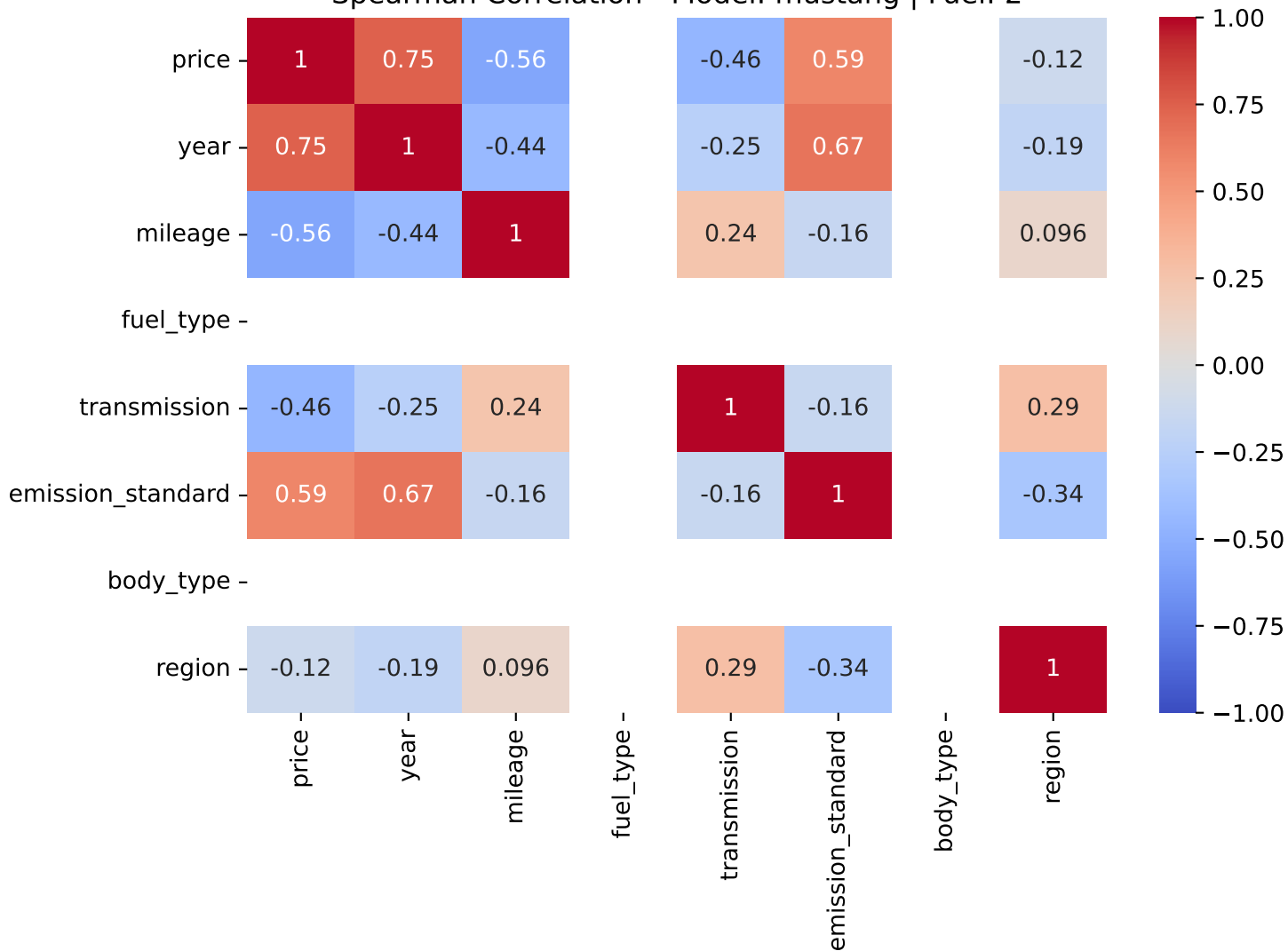
Spearman Correlation - Model: mustang | Fuel: 2
