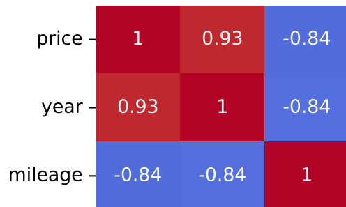
Spearman Correlation - Model: c3 | Fuel: 2
