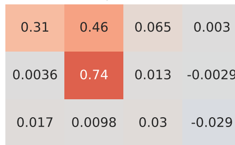
Pearson Correlation - Model: 107 | Fuel: 2
