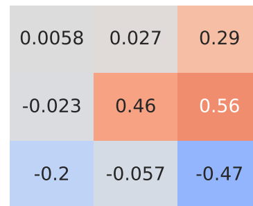
Pearson Correlation - Model: stonic | Fuel: 1
