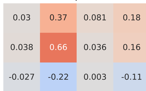
Spearman Correlation - Model: musa | Fuel: 1
