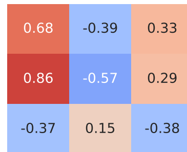
Pearson Correlation - Model: rio | Fuel: 2
