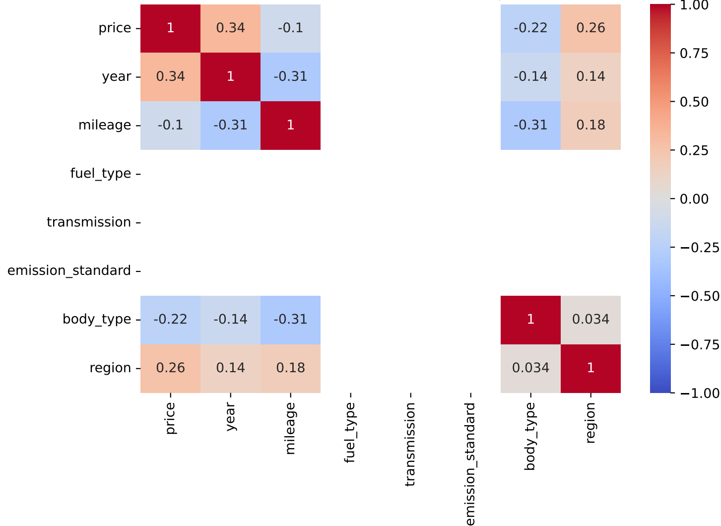
Spearman Correlation - Model: corsa | Fuel: 0
