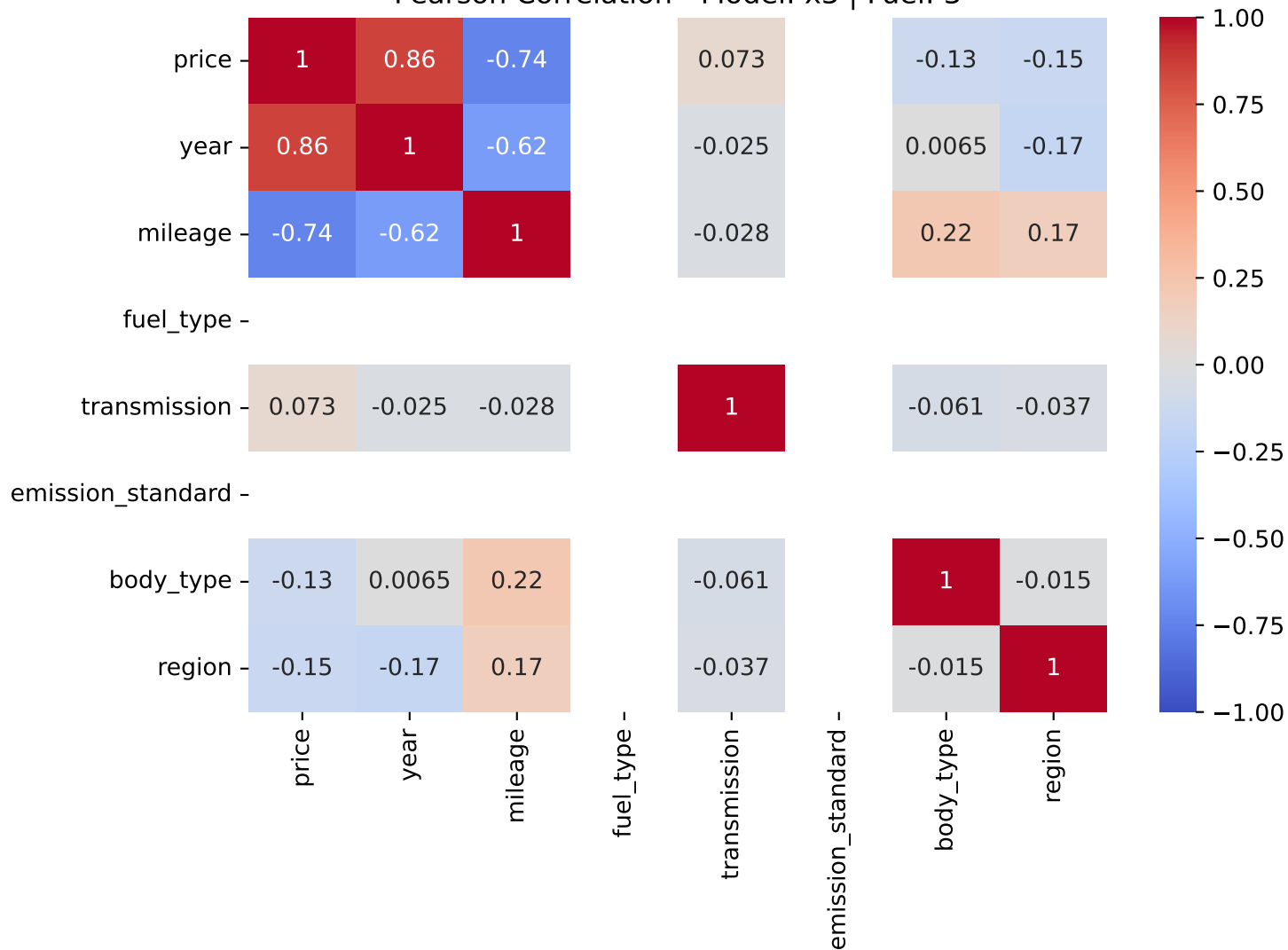
Pearson Correlation - Model: x3 | Fuel: 3
