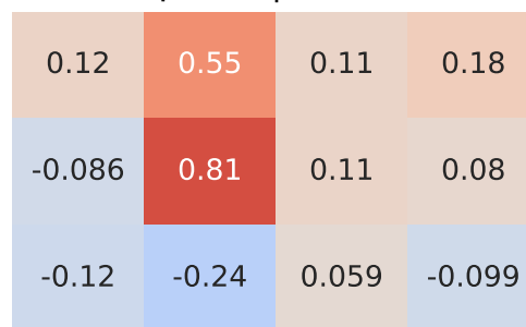
Spearman Correlation - Model: punto | Fuel: 4
