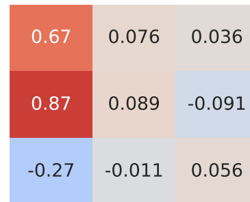
Pearson Correlation - Model: panda | Fuel: 5
