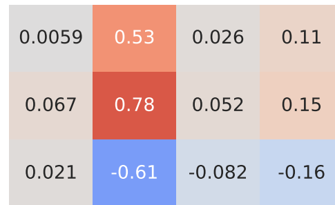
Pearson Correlation - Model: i20 | Fuel: 2
