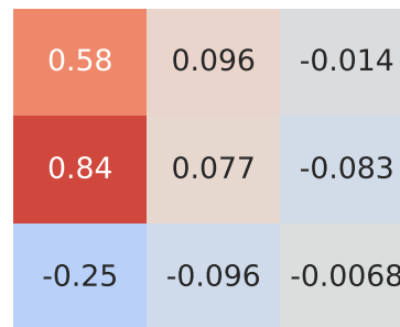
Spearman Correlation - Model: meriva | Fuel: 4
