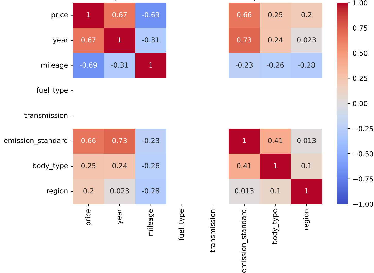
Spearman Correlation - Model: i20 | Fuel: 1
