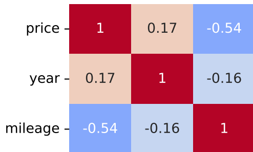
Spearman Correlation - Model: 500x | Fuel: 4
