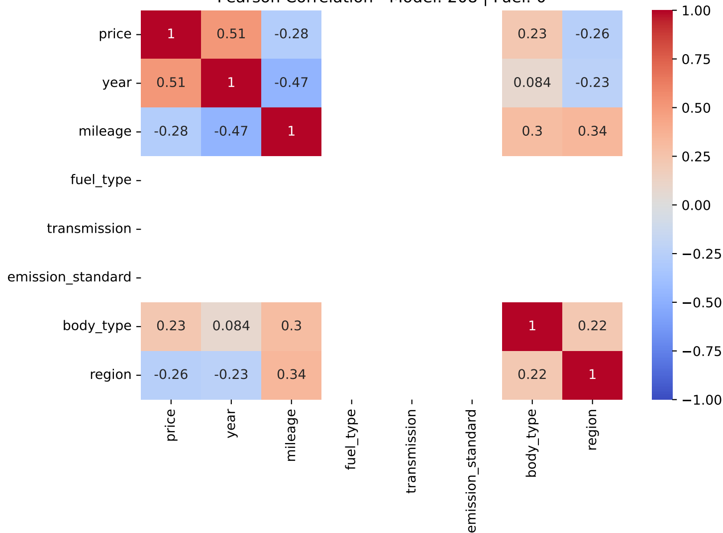
Pearson Correlation - Model: 208 | Fuel: 0
