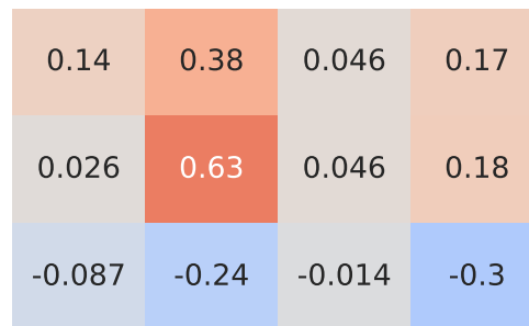
Pearson Correlation - Model: bravo | Fuel: 1
