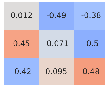
Spearman Correlation - Model: ibiza | Fuel: 5
