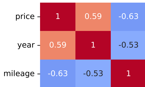
Pearson Correlation - Model: puma | Fuel: 3
