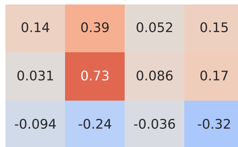
Spearman Correlation - Model: bravo | Fuel: 1
