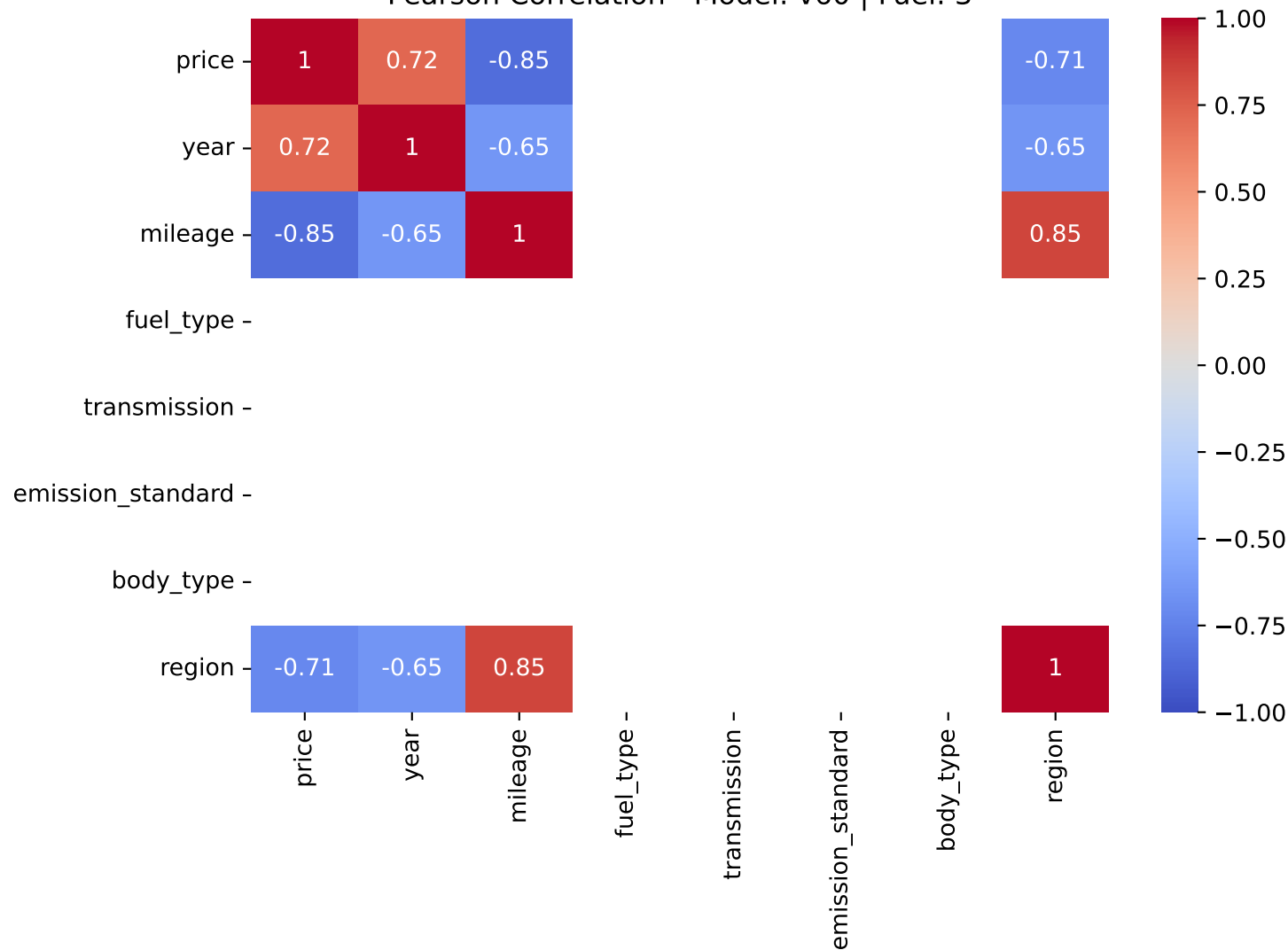
Pearson Correlation - Model: v60 | Fuel: 3
