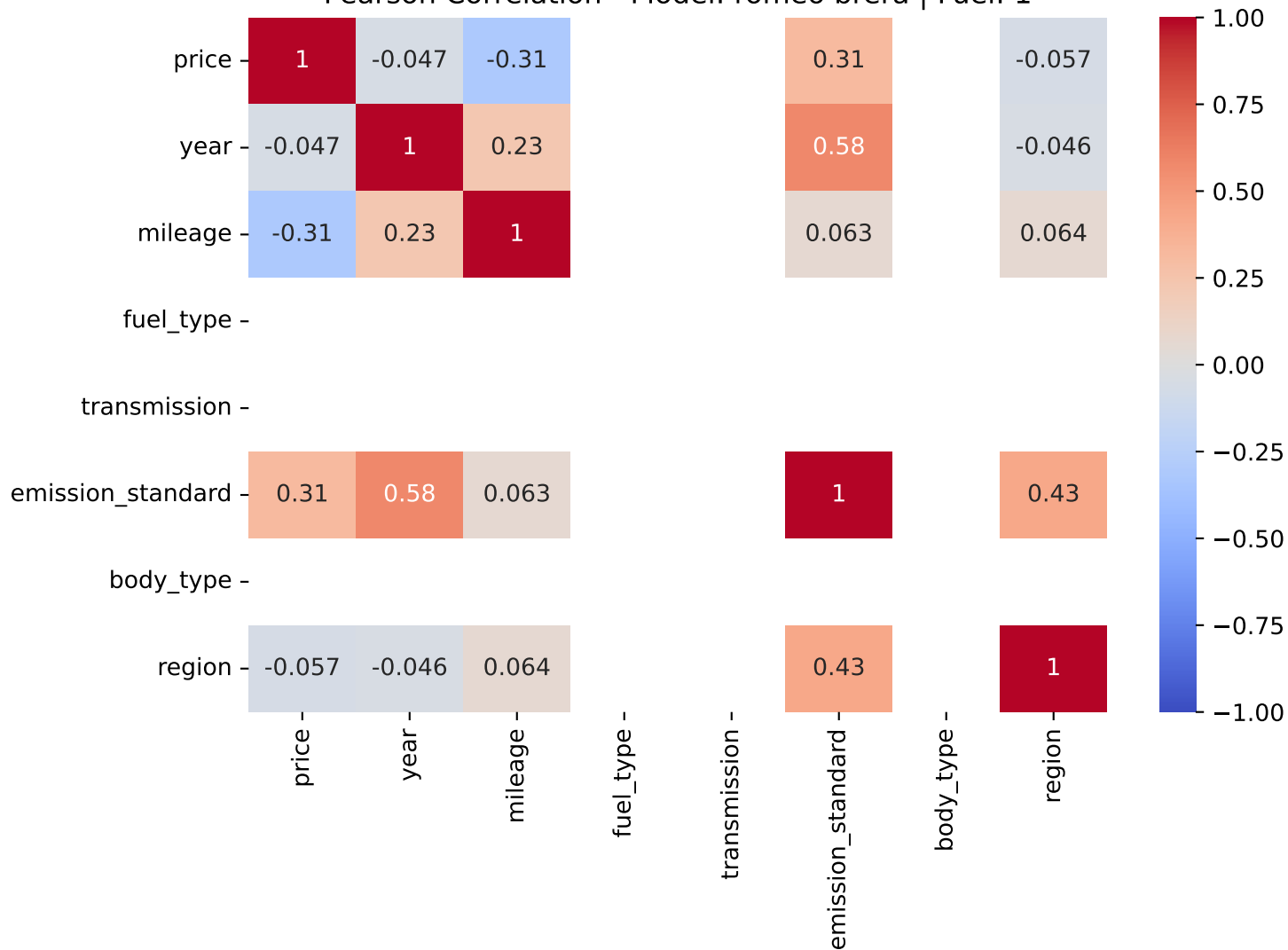
Pearson Correlation - Model: romeo brera | Fuel: 1
