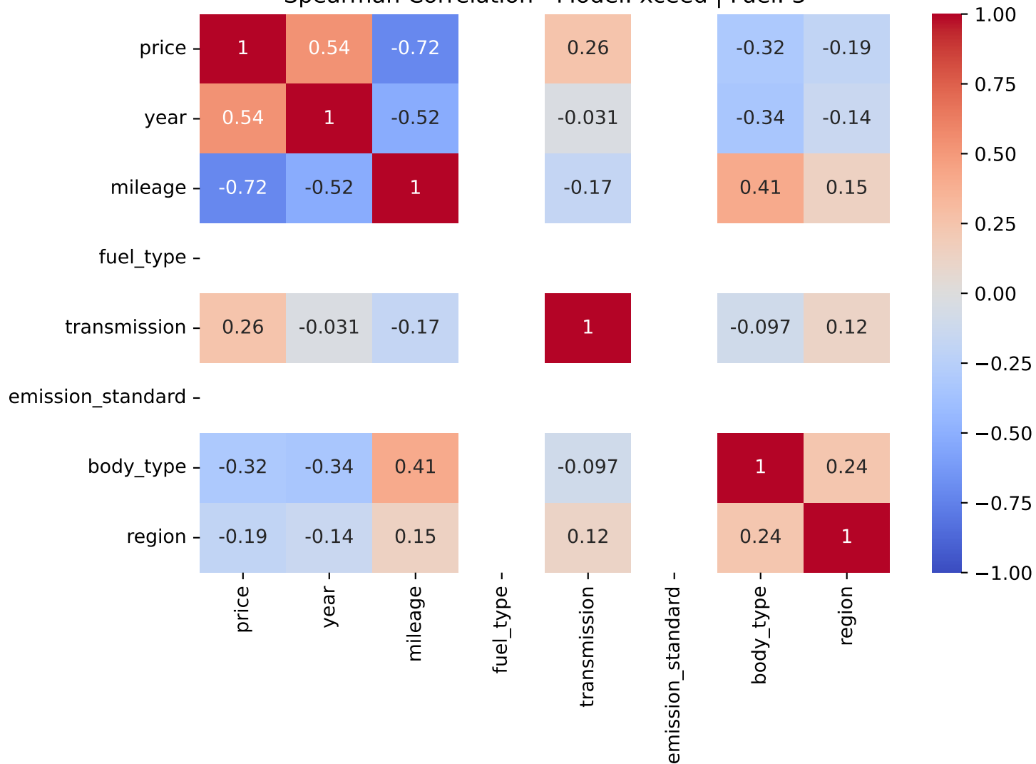
Spearman Correlation - Model: xceed | Fuel: 3
