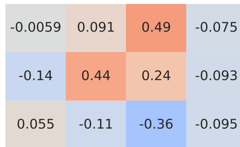
Pearson Correlation - Model: c2 | Fuel: 2
