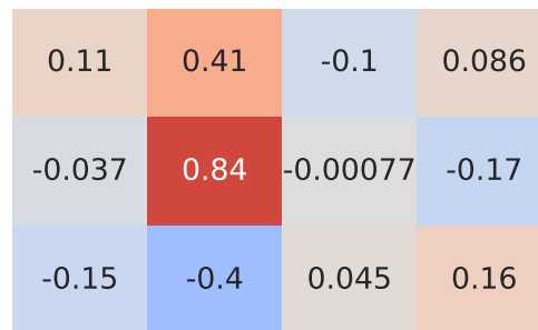
Pearson Correlation - Model: antara | Fuel: 1
