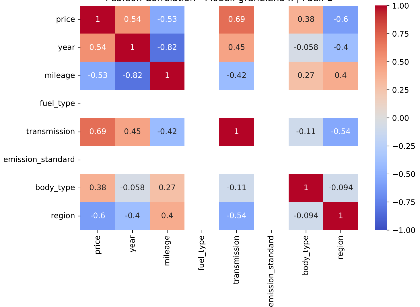
Pearson Correlation - Model: grandland x | Fuel: 2
