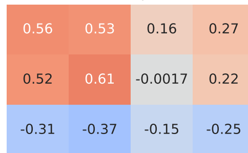
Spearman Correlation - Model: clubman | Fuel: 1
