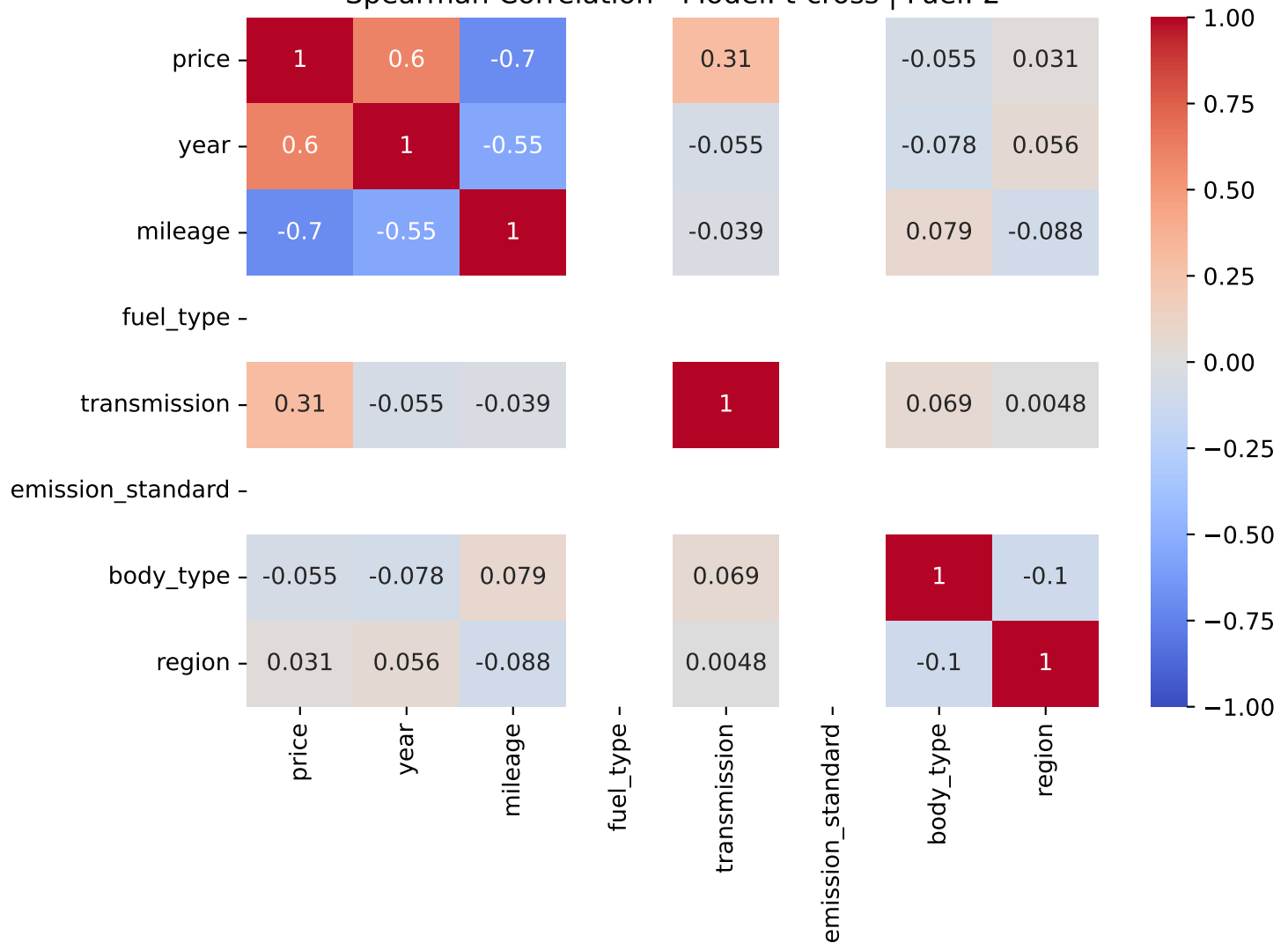
Spearman Correlation - Model: t-cross | Fuel: 2
