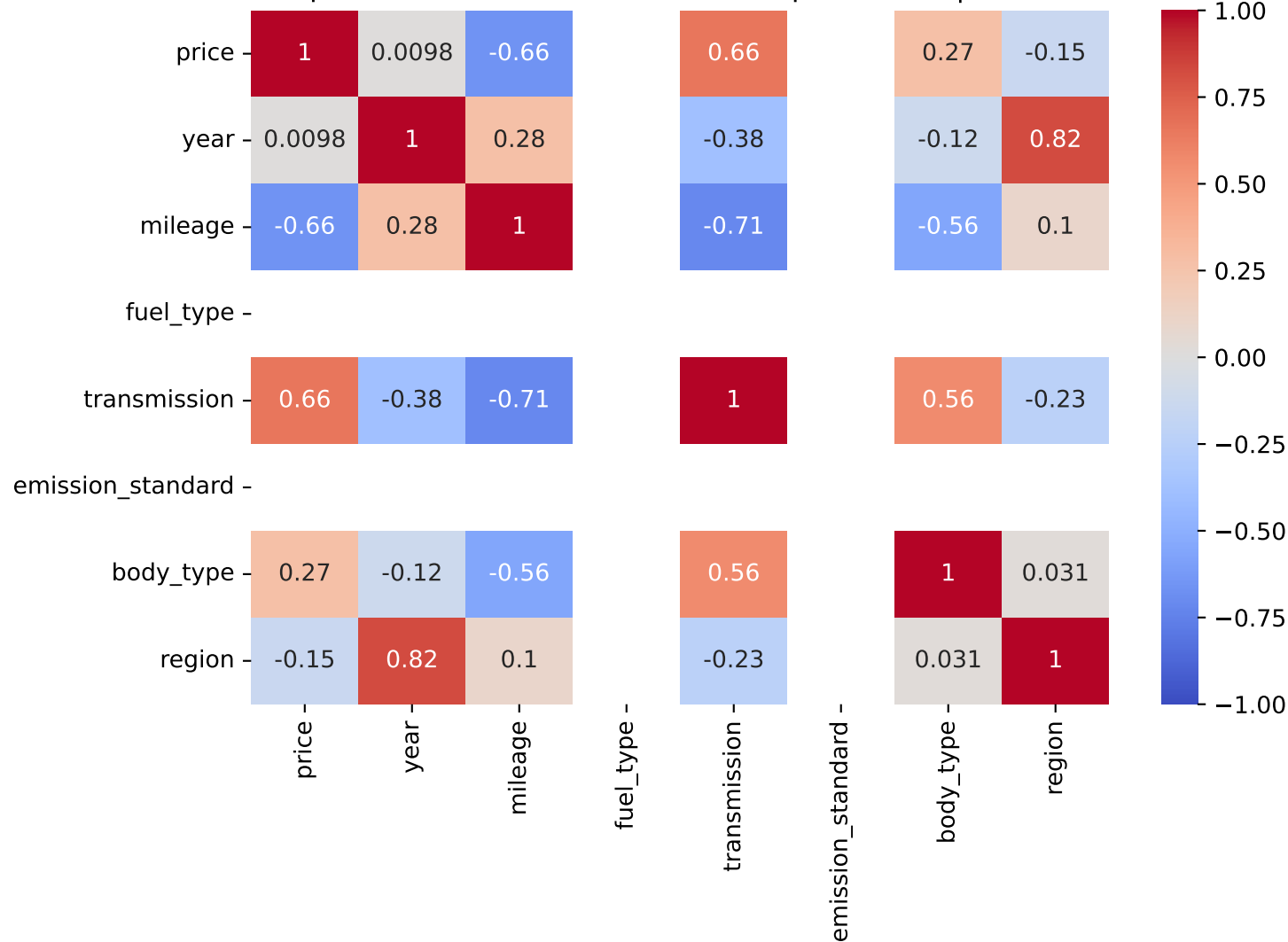
Spearman Correlation - Model: c4 spacetourer | Fuel: 1
