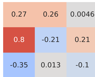
Spearman Correlation - Model: 206 | Fuel: 2
