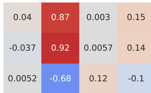
Spearman Correlation - Model: yaris | Fuel: 2
