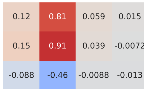
Pearson Correlation - Model: c-max | Fuel: 1
