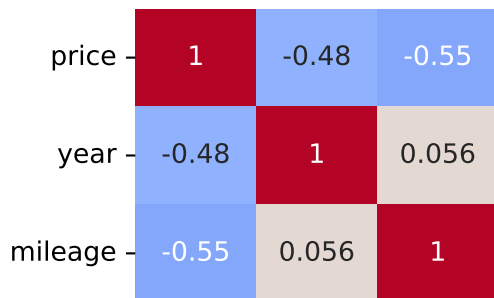
Spearman Correlation - Model: delta | Fuel: 2
