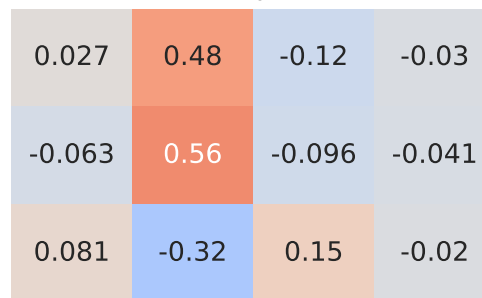
Pearson Correlation - Model: compass | Fuel: 1
