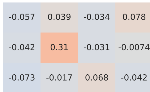
Spearman Correlation - Model: delta | Fuel: 1
