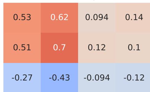
Spearman Correlation - Model: countryman | Fuel: 1
