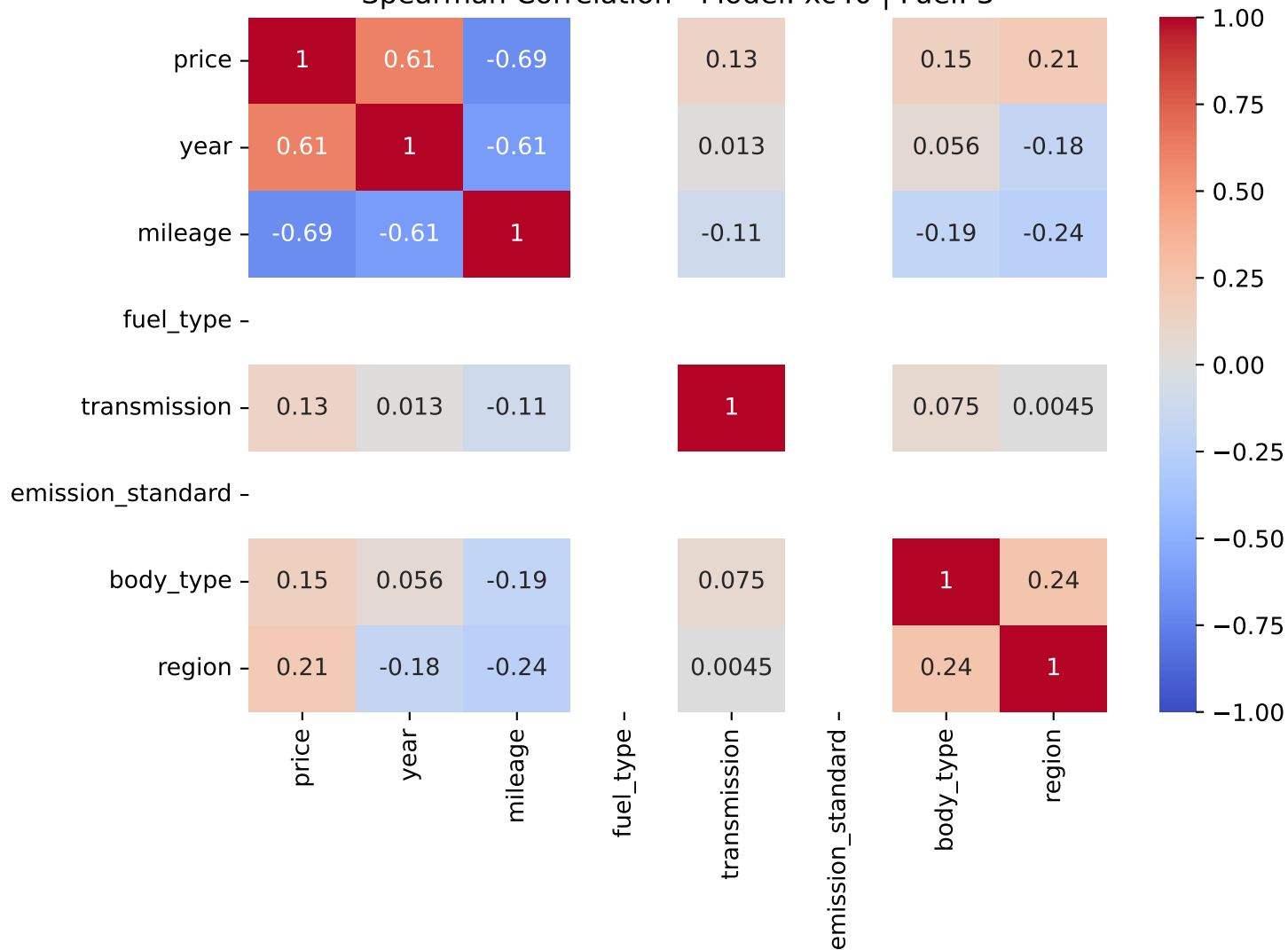
Spearman Correlation - Model: xc40 | Fuel: 3
