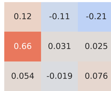
Spearman Correlation - Model: grand vitara | Fuel: 1
