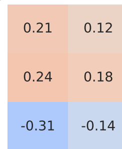
Pearson Correlation - Model: bayon | Fuel: 3
