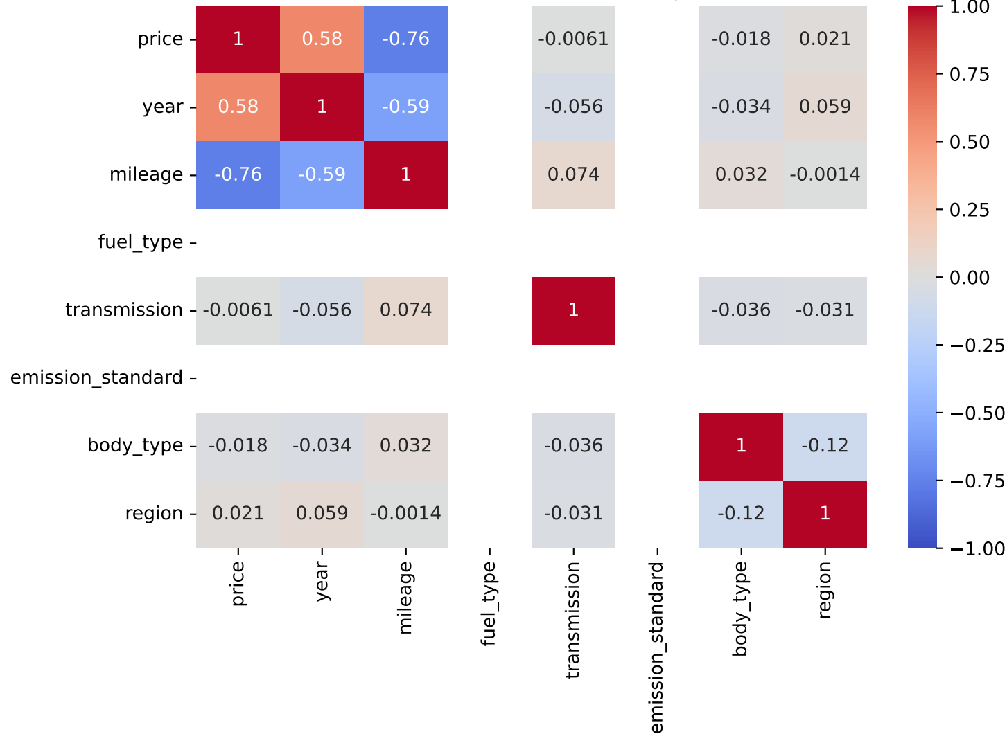
Pearson Correlation - Model: golf | Fuel: 3
