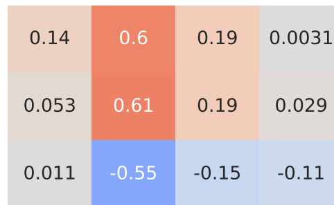
Spearman Correlation - Model: a1 | Fuel: 2
