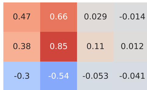
Pearson Correlation - Model: golf | Fuel: 1
