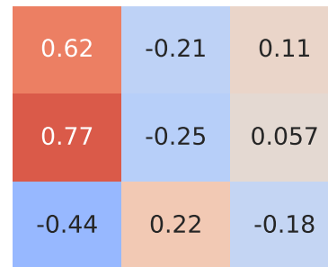
Pearson Correlation - Model: i10 | Fuel: 4
