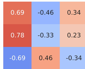
Spearman Correlation - Model: swift | Fuel: 4
