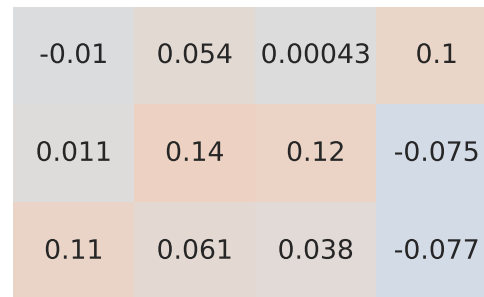
Pearson Correlation - Model: macan | Fuel: 1
