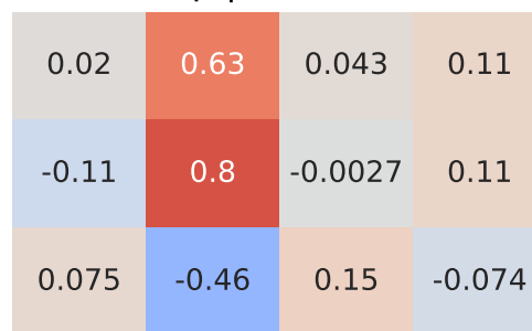
Pearson Correlation - Model: up | Fuel: 2
