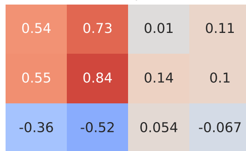
Spearman Correlation - Model: insignia | Fuel: 1
