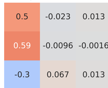
Pearson Correlation - Model: juke | Fuel: 1
