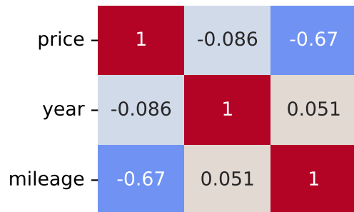
Pearson Correlation - Model: stonic | Fuel: 1
