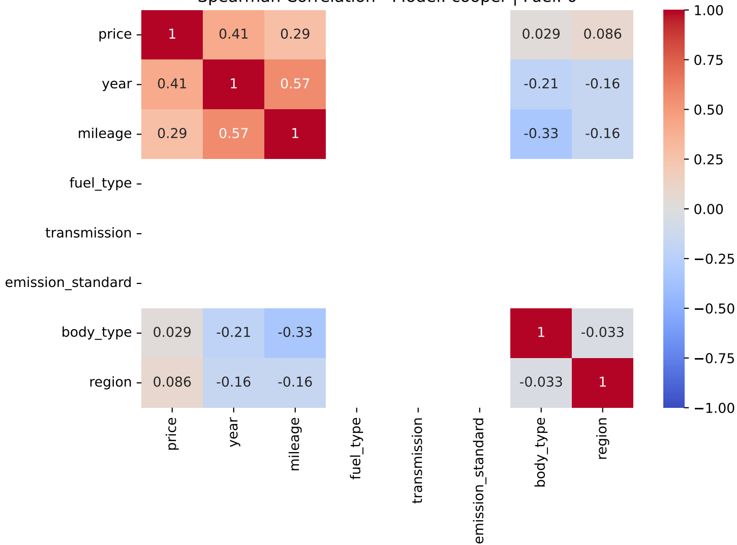
Spearman Correlation - Model: cooper | Fuel: 0
