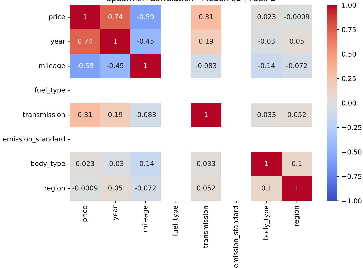
Spearman Correlation - Model: q2 | Fuel: 2
