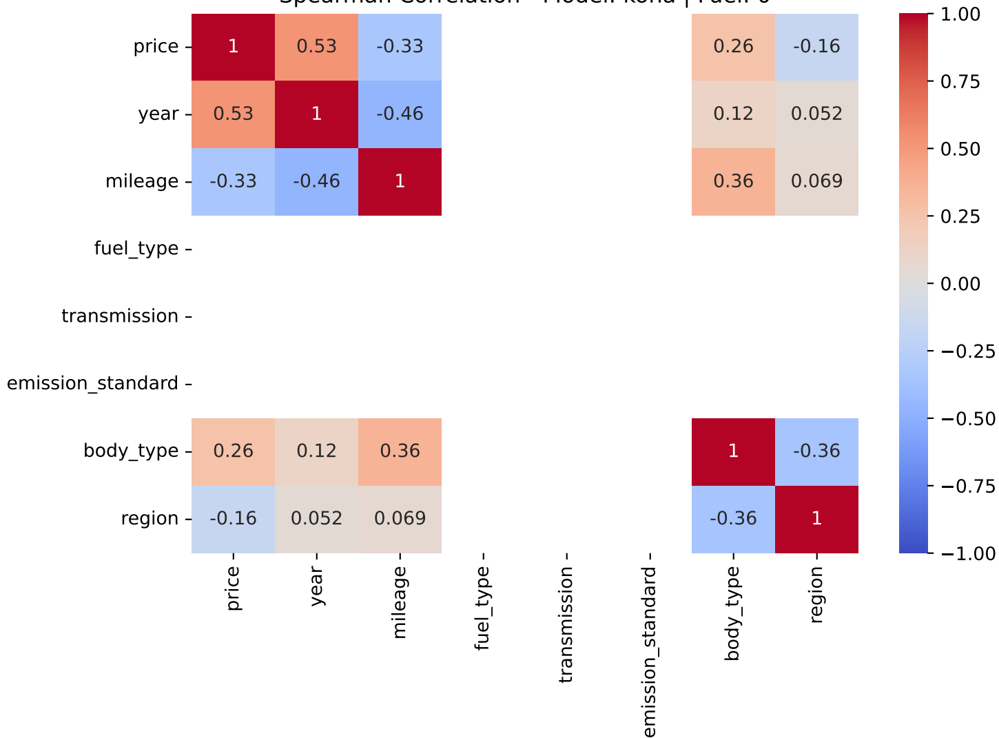
Spearman Correlation - Model: kona | Fuel: 0
