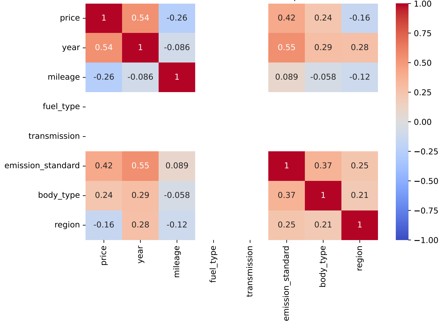
Pearson Correlation - Model: alto | Fuel: 2
