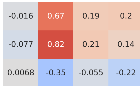
Spearman Correlation - Model: punto | Fuel: 1
