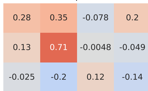
Spearman Correlation - Model: musa | Fuel: 2
