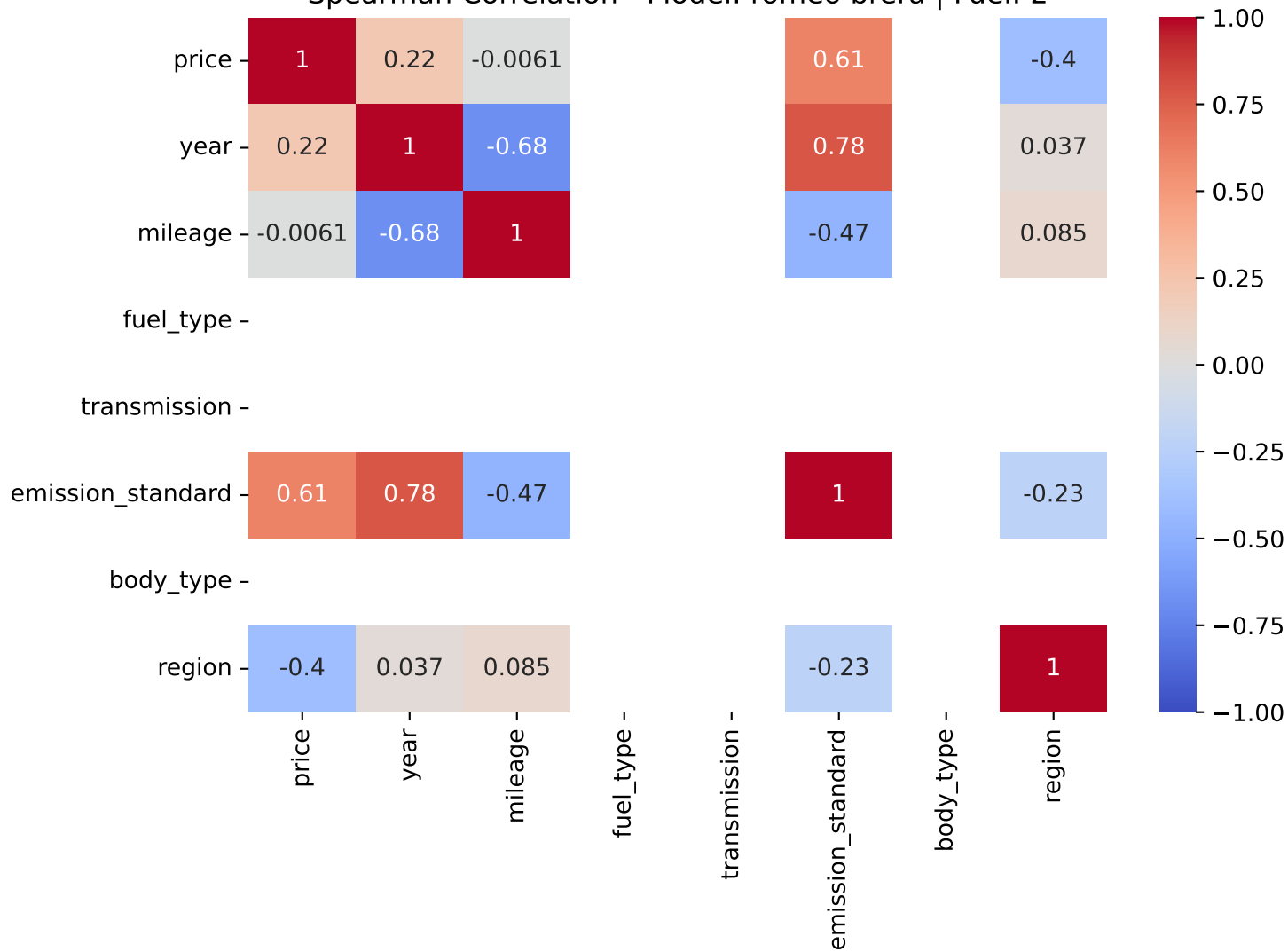
Spearman Correlation - Model: romeo brera | Fuel: 2
