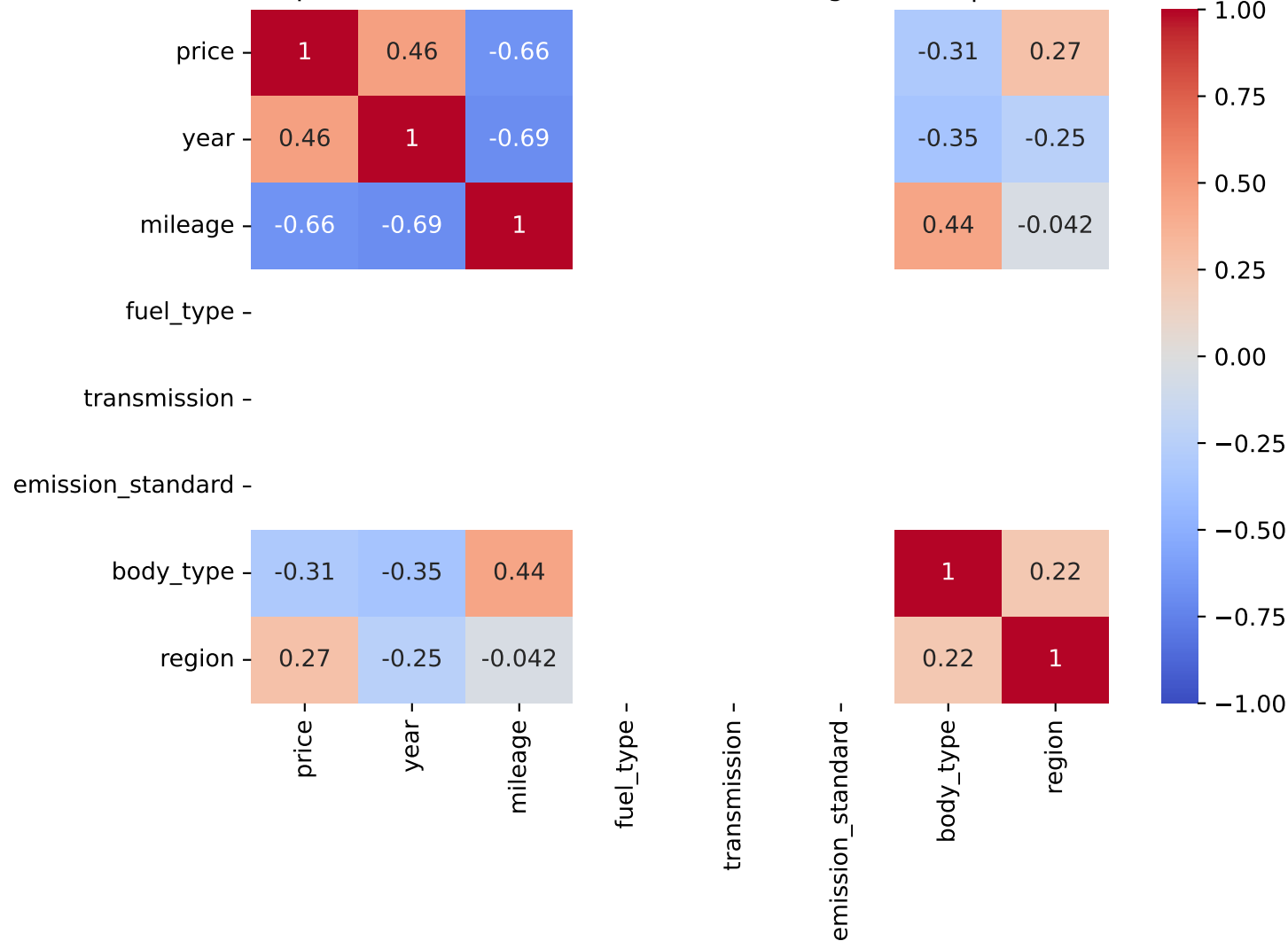
Spearman Correlation - Model: mustang mach-e | Fuel: 0
