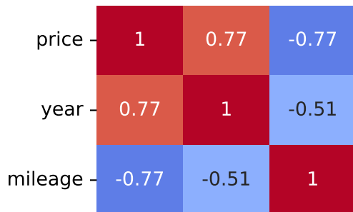
Spearman Correlation - Model: adam | Fuel: 2
