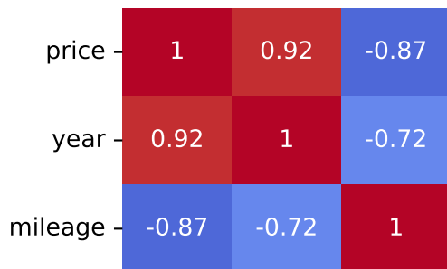
Pearson Correlation - Model: octavia | Fuel: 2
