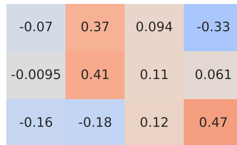
Spearman Correlation - Model: touran | Fuel: 5
