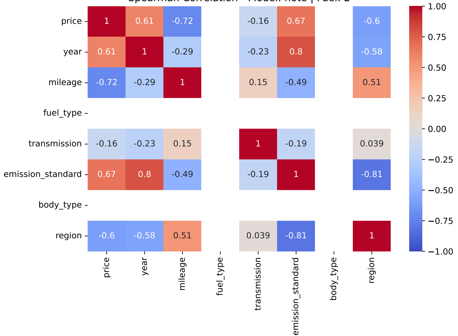
Spearman Correlation - Model: note | Fuel: 2
