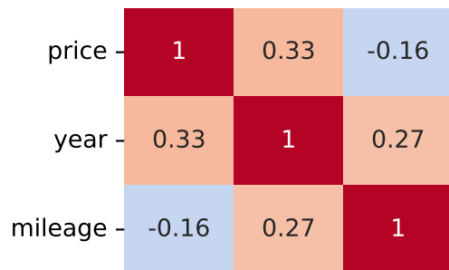
Pearson Correlation - Model: cromax | Fuel: 1
