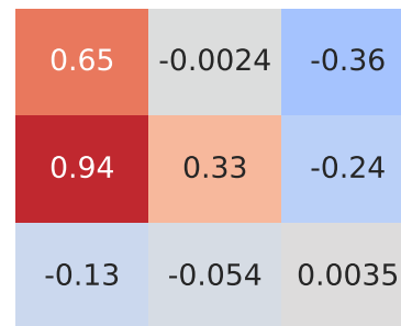
Spearman Correlation - Model: ducato | Fuel: 1
