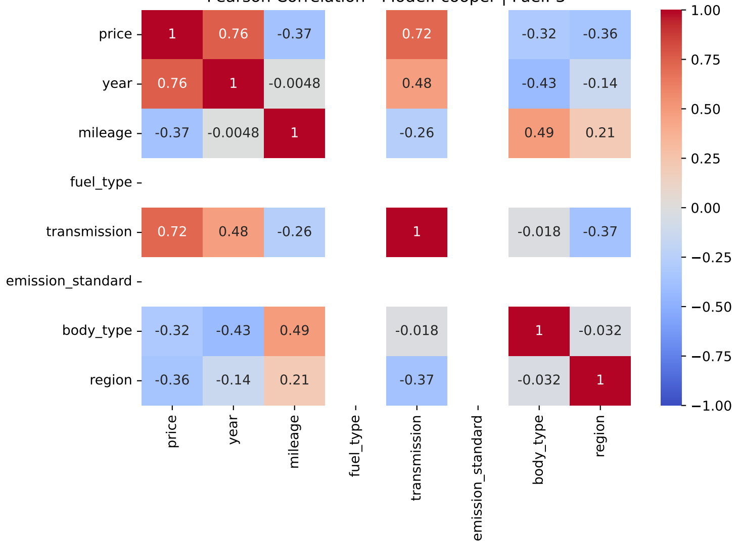
Pearson Correlation - Model: cooper | Fuel: 3
