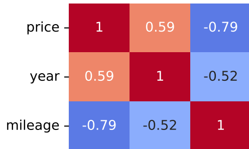
Pearson Correlation - Model: celerio | Fuel: 2
