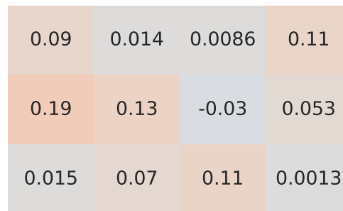
Spearman Correlation - Model: kadjar | Fuel: 1
