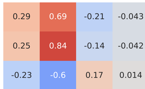
Pearson Correlation - Model: 508 | Fuel: 1
