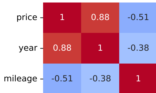
Spearman Correlation - Model: q7 | Fuel: 1
