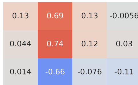
Pearson Correlation - Model: a1 | Fuel: 2
