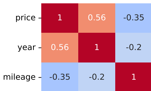
Pearson Correlation - Model: a5 | Fuel: 2
