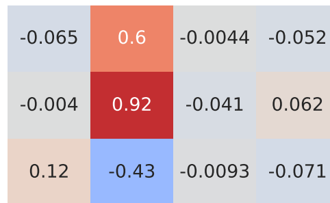
Pearson Correlation - Model: dobro | Fuel: 1
