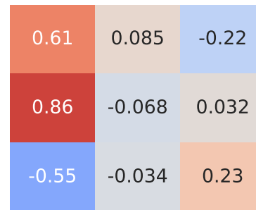
Spearman Correlation - Model: grand vitara | Fuel: 2
