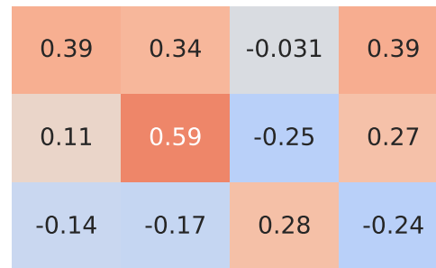
Spearman Correlation - Model: a5 | Fuel: 2
