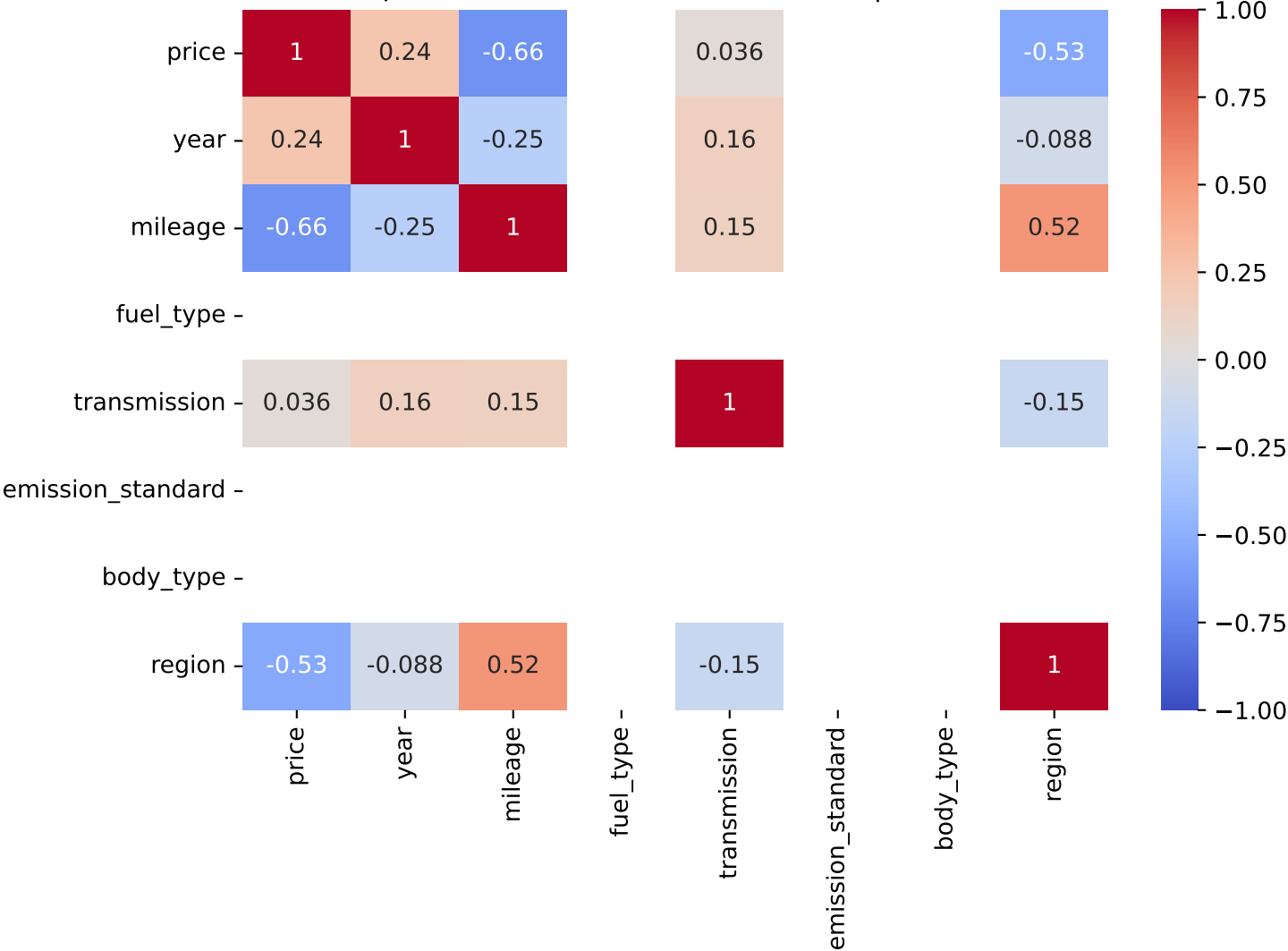
Spearman Correlation - Model: id.3 | Fuel: 0
