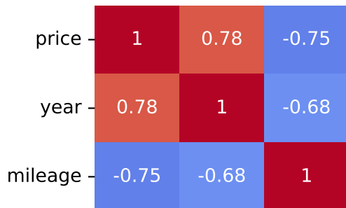
Pearson Correlation - Model: rover discovery sport | Fuel: 3
