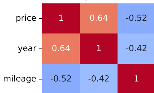
Spearman Correlation - Model: vivaro | Fuel: 1
