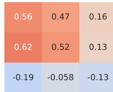
Spearman Correlation - Model: polo | Fuel: 4
