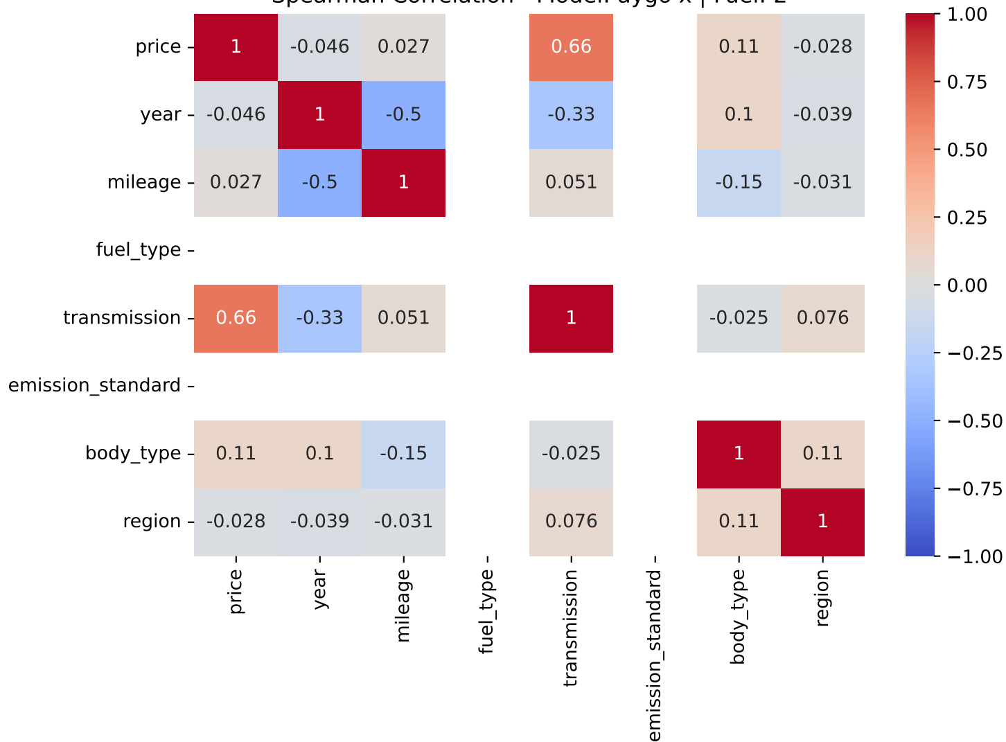
Spearman Correlation - Model: aygo x | Fuel: 2
