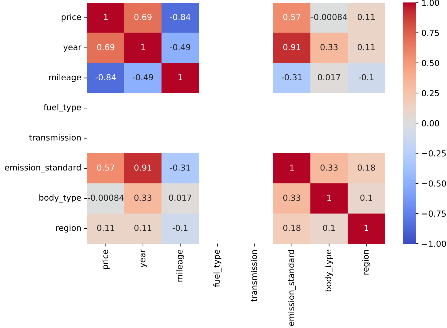
Pearson Correlation - Model: romeo mito | Fuel: 4
