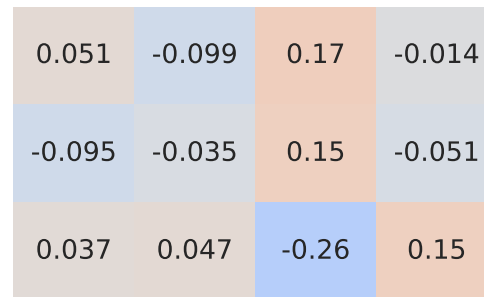
Pearson Correlation - Model: kuga | Fuel: 2
