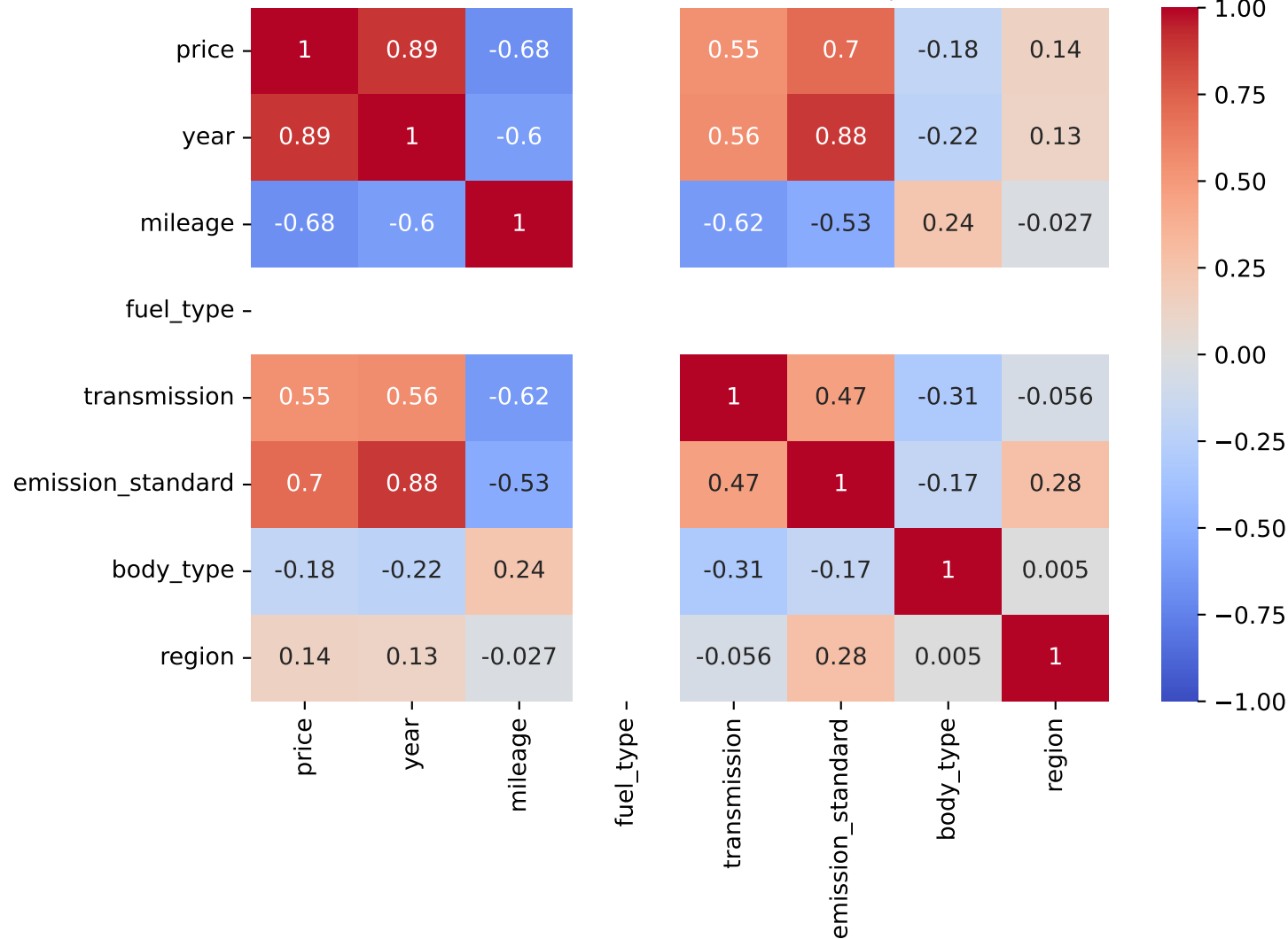
Pearson Correlation - Model: sorento | Fuel: 1
