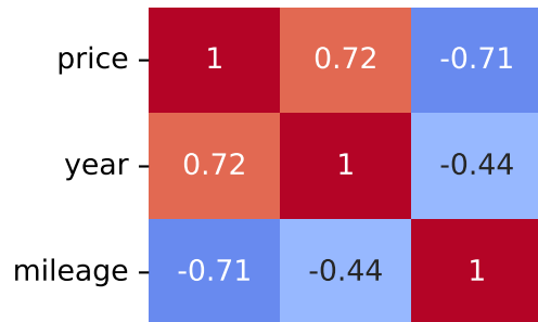
Pearson Correlation - Model: berlingo | Fuel: 1
