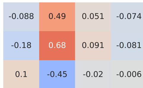
Pearson Correlation - Model: 208 | Fuel: 1
