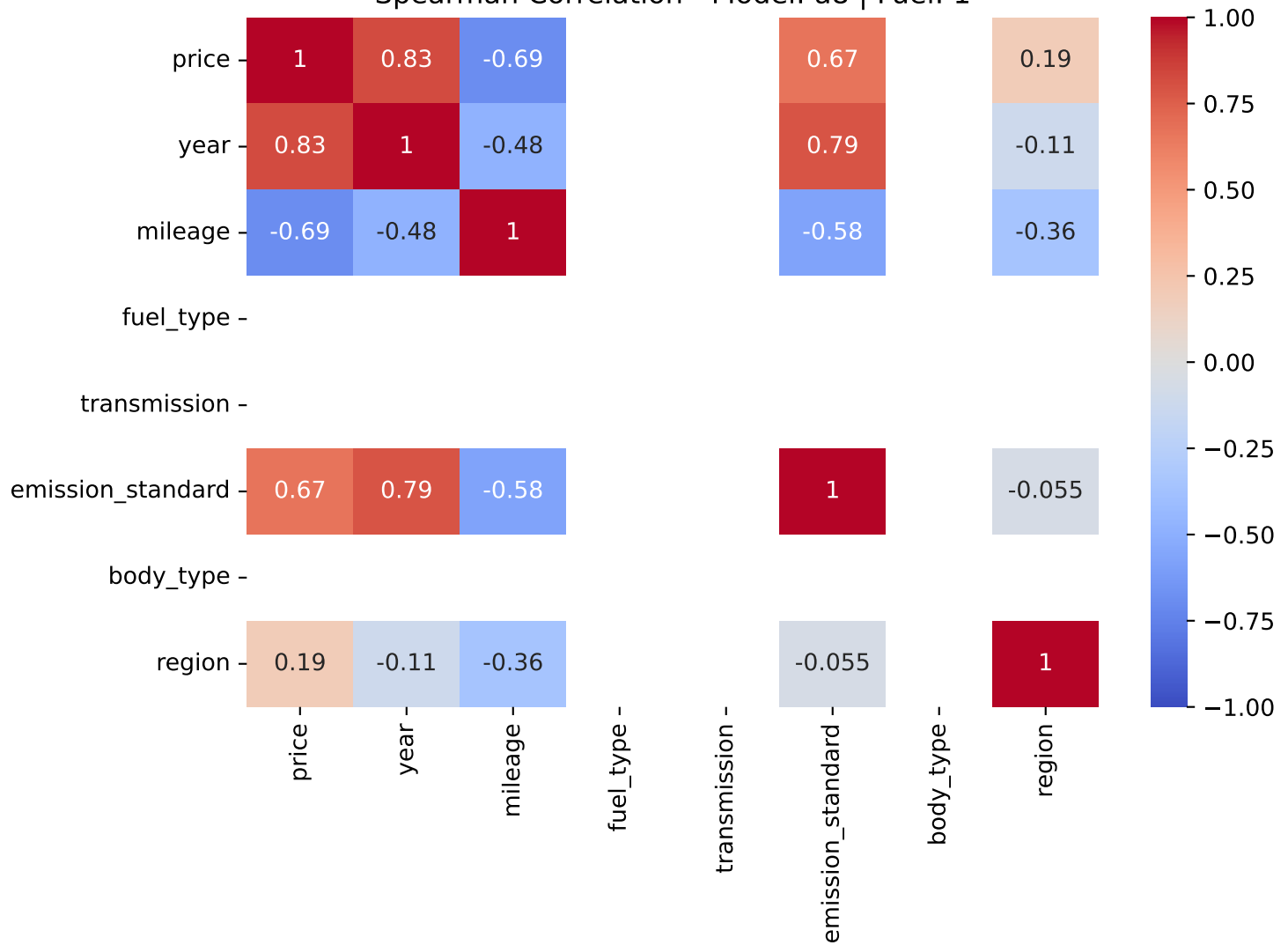
Spearman Correlation - Model: a8 | Fuel: 1
