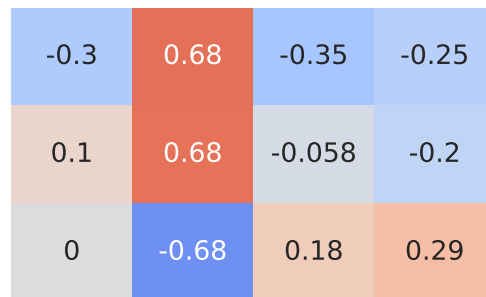
Spearman Correlation - Model: octavia | Fuel: 2
