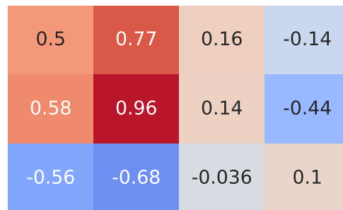
Pearson Correlation - Model: m3 | Fuel: 2
