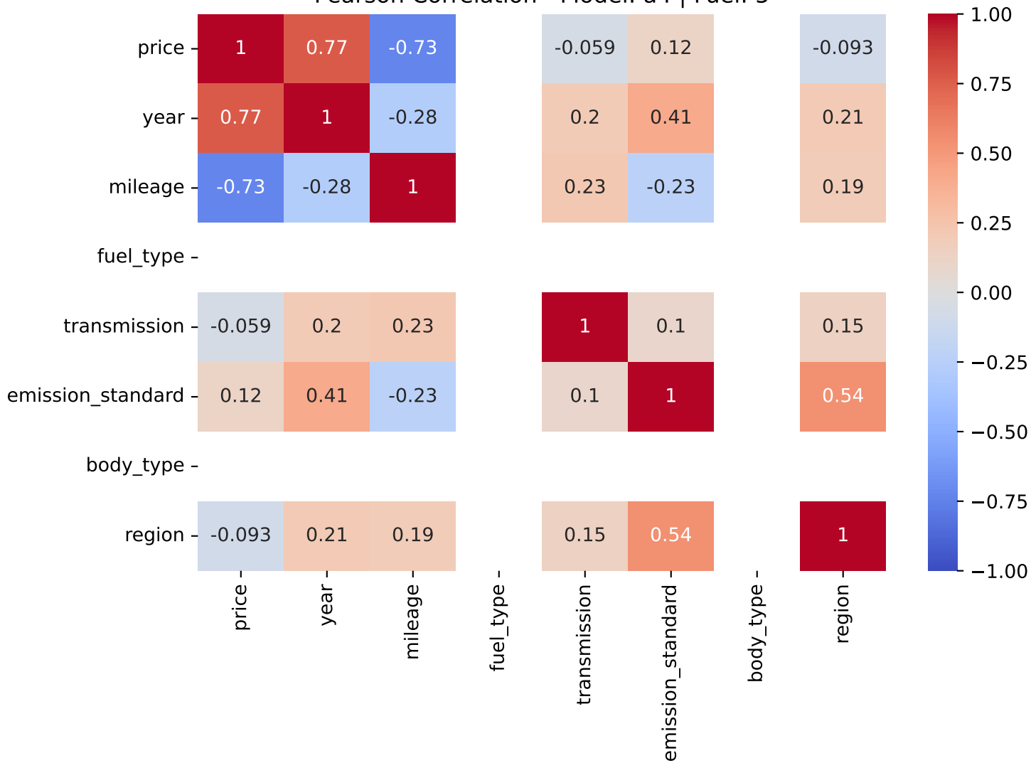
Pearson Correlation - Model: a4 | Fuel: 5
