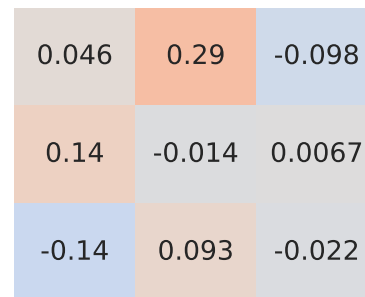
Pearson Correlation - Model: multipla | Fuel: 5
