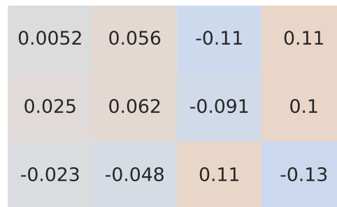
Spearman Correlation - Model: romeo stelvio | Fuel: 1
