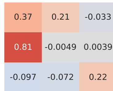
Pearson Correlation - Model: 207 | Fuel: 1
