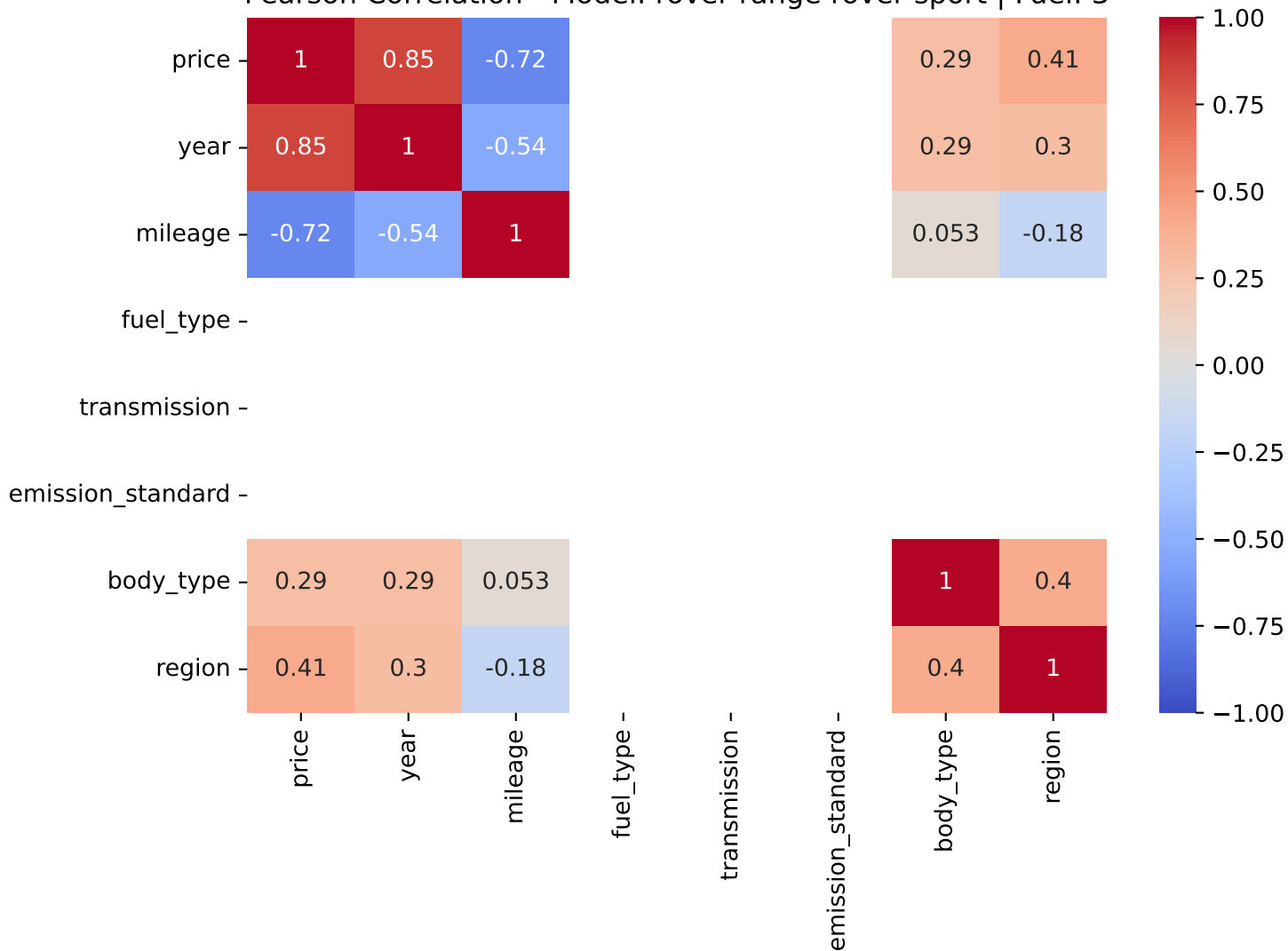
Pearson Correlation - Model: rover range rover sport | Fuel: 3
