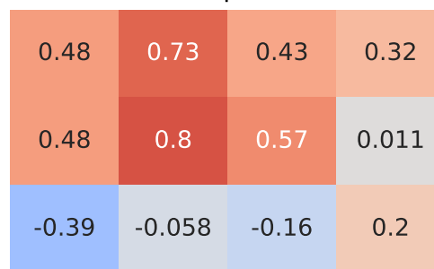
Spearman Correlation - Model: zafira | Fuel: 2
