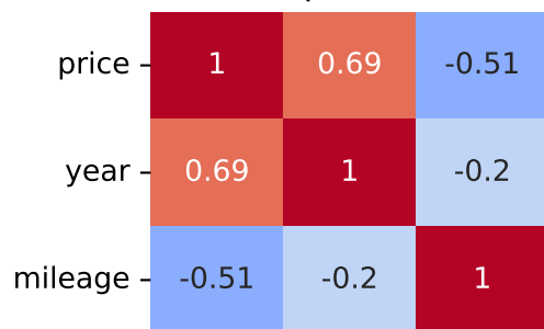
Spearman Correlation - Model: vitara | Fuel: 2
