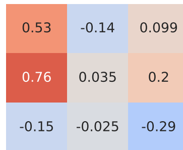
Spearman Correlation - Model: panda cross | Fuel: 1
