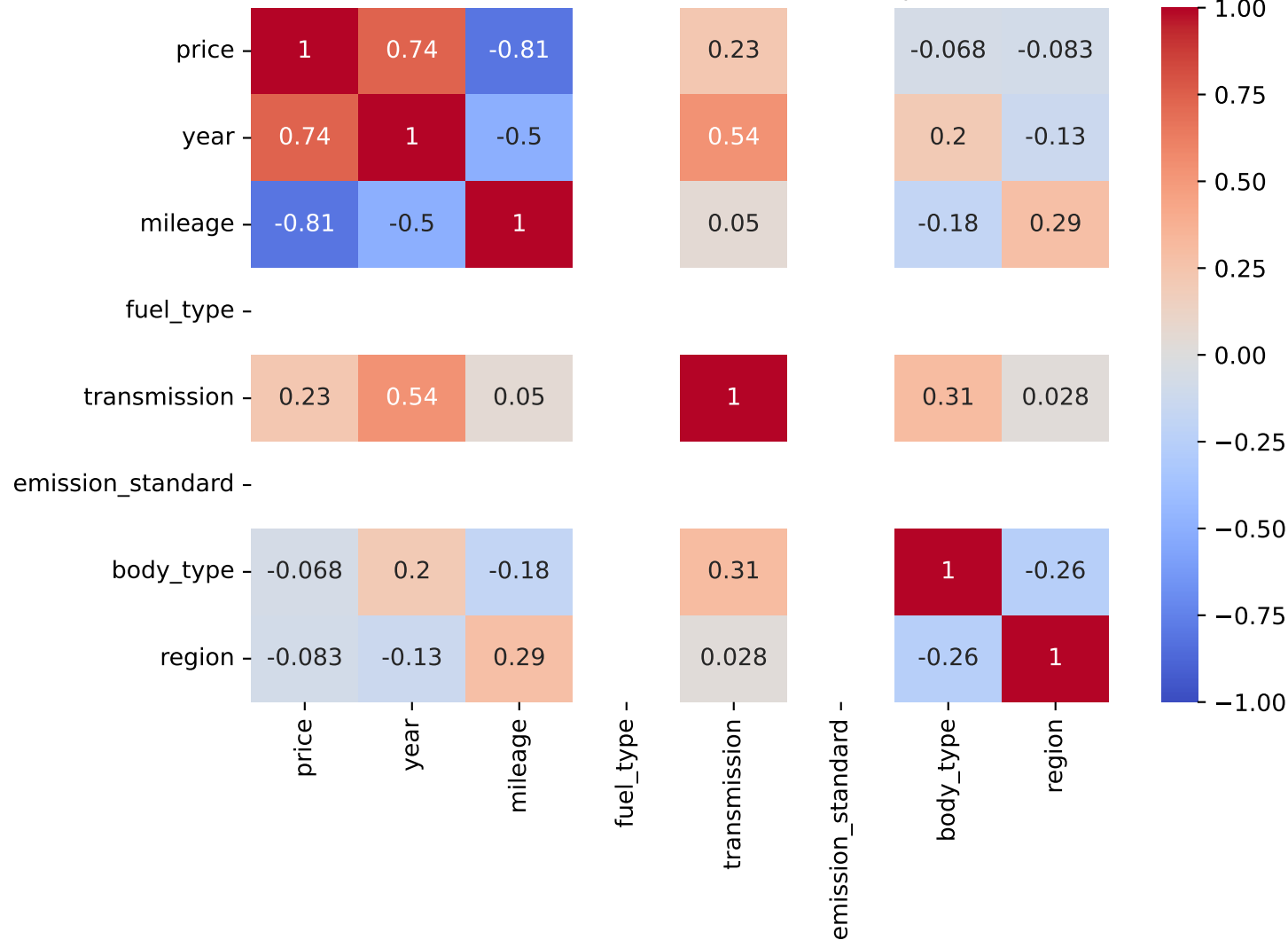
Spearman Correlation - Model: octavia | Fuel: 5
