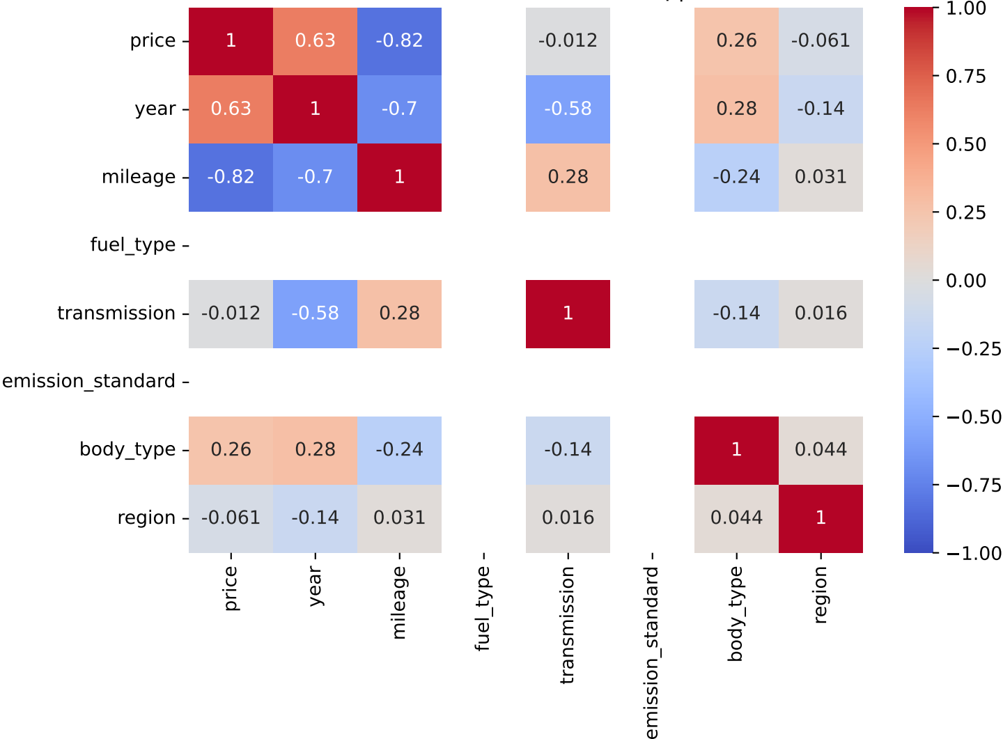
Pearson Correlation - Model: karoq | Fuel: 2
