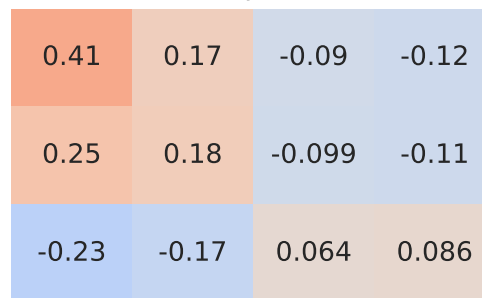
Spearman Correlation - Model: 2008 | Fuel: 2
