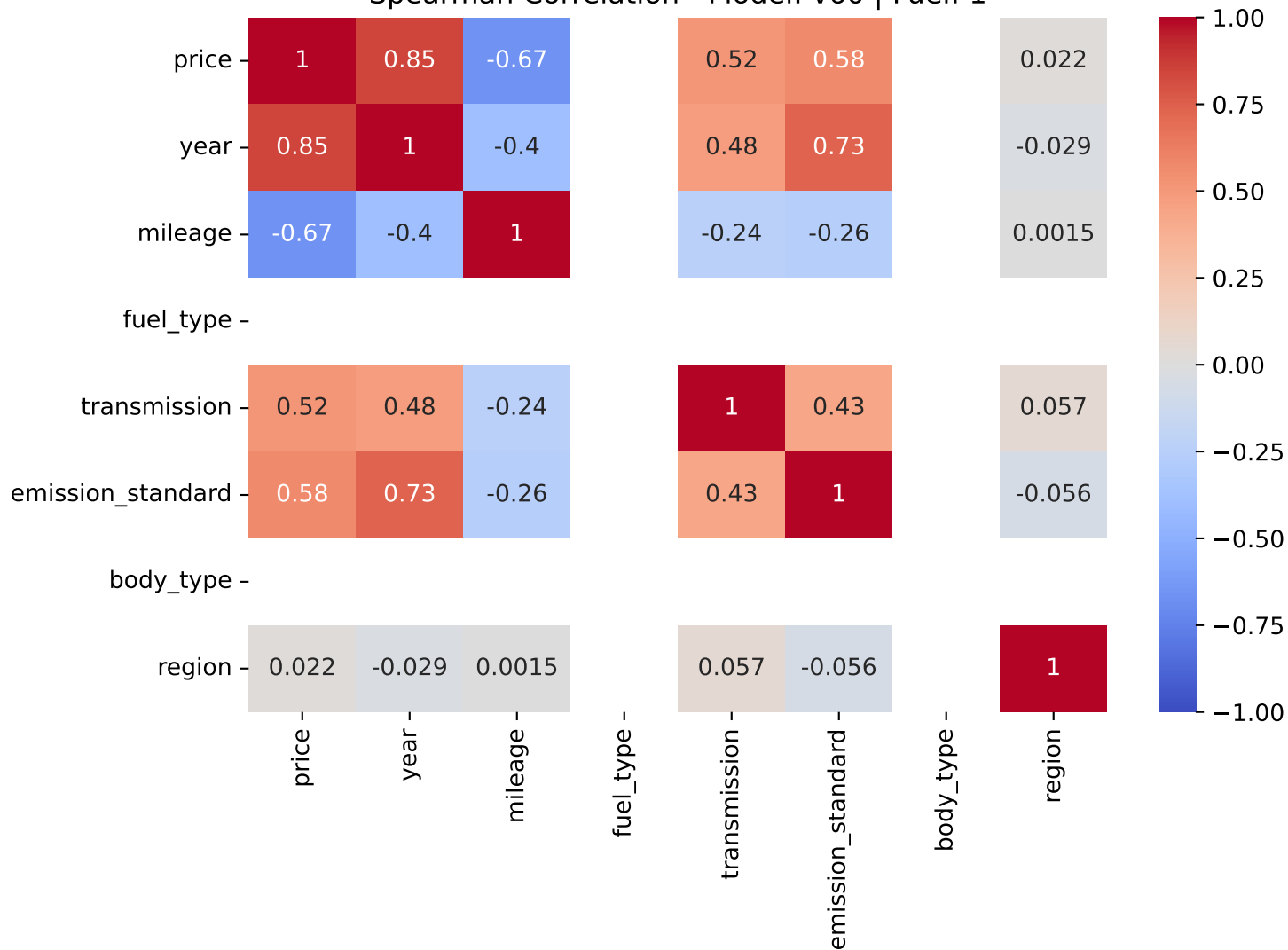
Spearman Correlation - Model: v60 | Fuel: 1
