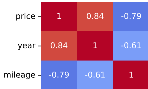
Spearman Correlation - Model: romeo giulietta | Fuel: 1
