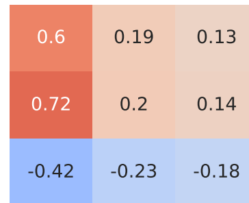
Pearson Correlation - Model: up | Fuel: 5
