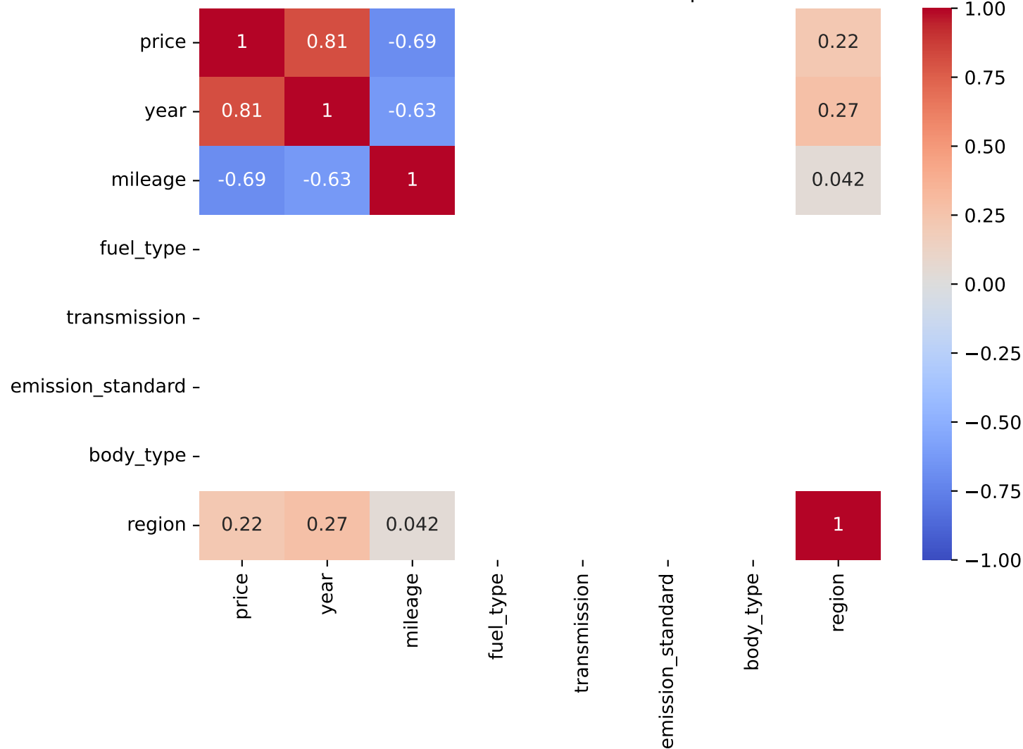
Pearson Correlation - Model: xc90 | Fuel: 3
