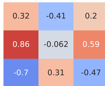
Spearman Correlation - Model: venga | Fuel: 2
