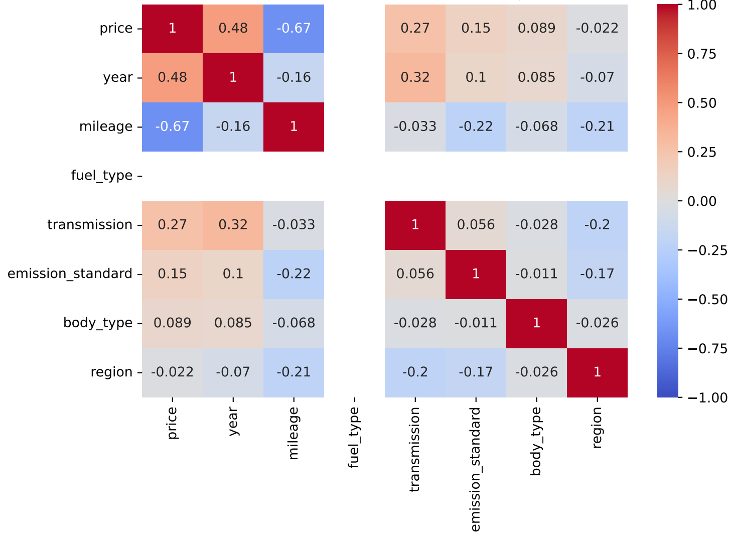
Pearson Correlation - Model: crossland x | Fuel: 1
