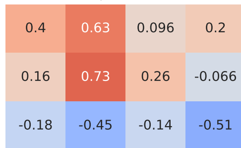
Pearson Correlation - Model: iq | Fuel: 2
