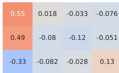
Spearman Correlation - Model: compass | Fuel: 2
