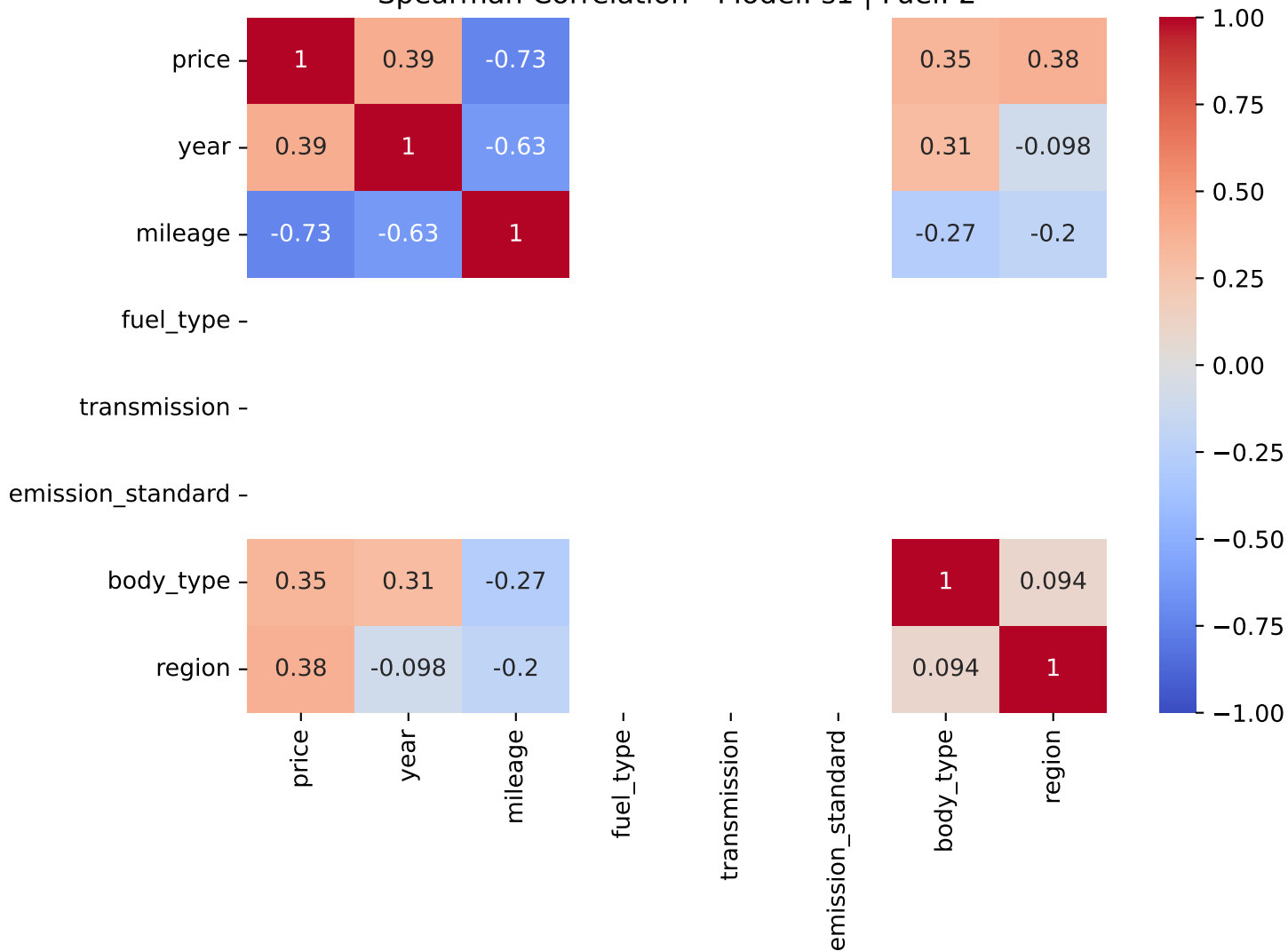
Spearman Correlation - Model: s1 | Fuel: 2
