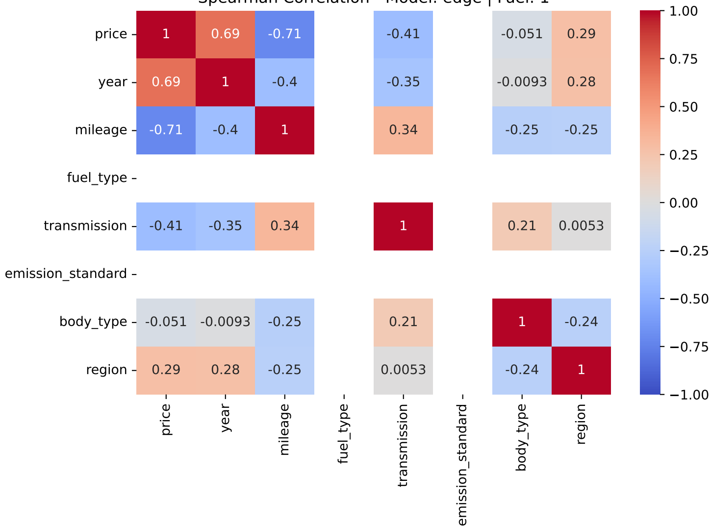
Spearman Correlation - Model: edge | Fuel: 1
