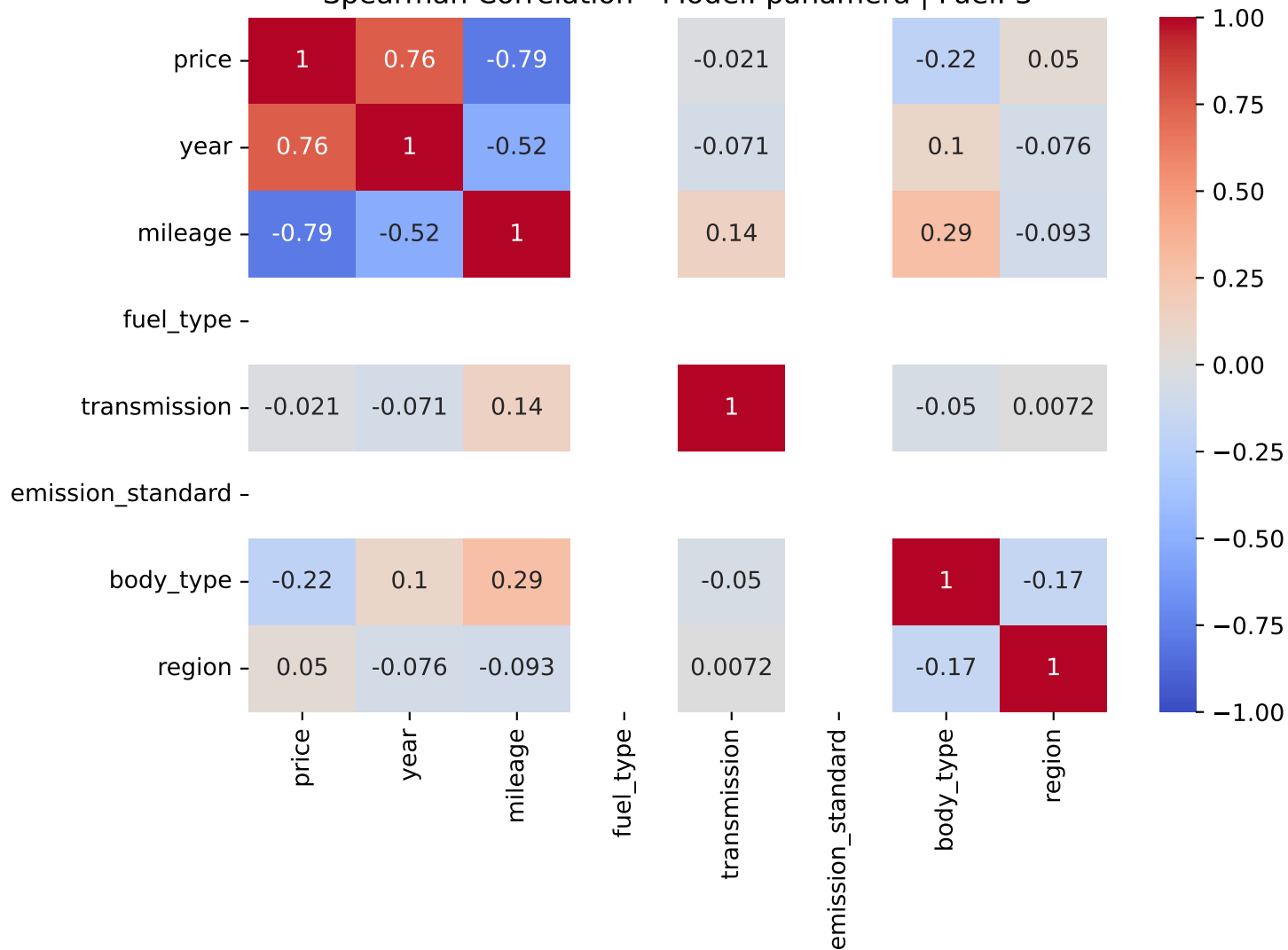
Spearman Correlation - Model: panamera | Fuel: 3
