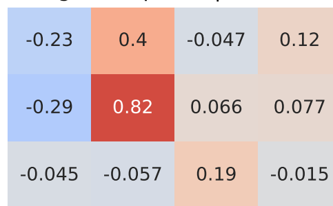
Spearman Correlation - Model: grande punto | Fuel: 4
