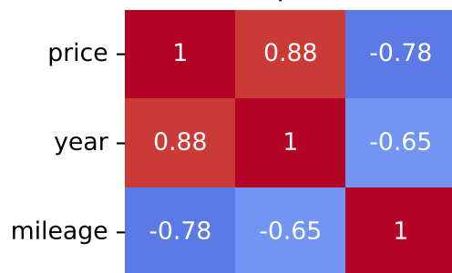
Spearman Correlation - Model: x1 | Fuel: 1
