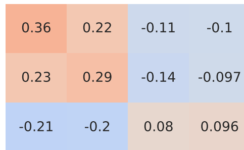
Pearson Correlation - Model: 2008 | Fuel: 2
