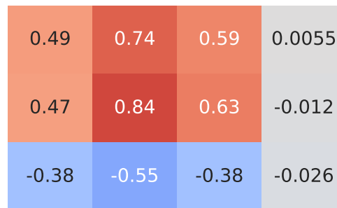
Pearson Correlation - Model: 5008 | Fuel: 1
