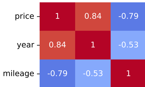
Spearman Correlation - Model: fabia | Fuel: 1
