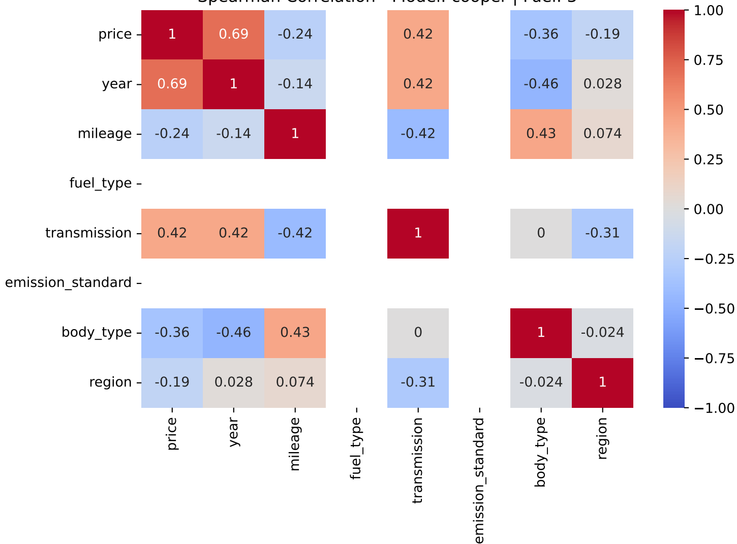
Spearman Correlation - Model: cooper | Fuel: 3
