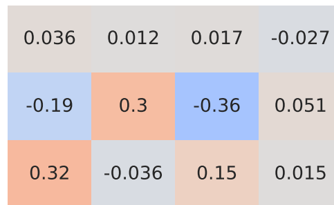
Spearman Correlation - Model: 500x | Fuel: 4
