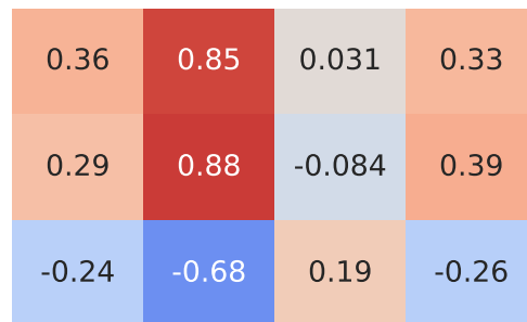
Spearman Correlation - Model: one | Fuel: 2
