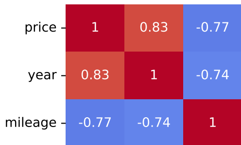
Pearson Correlation - Model: clio | Fuel: 2
