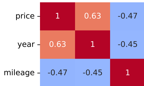
Pearson Correlation - Model: arkana | Fuel: 3
