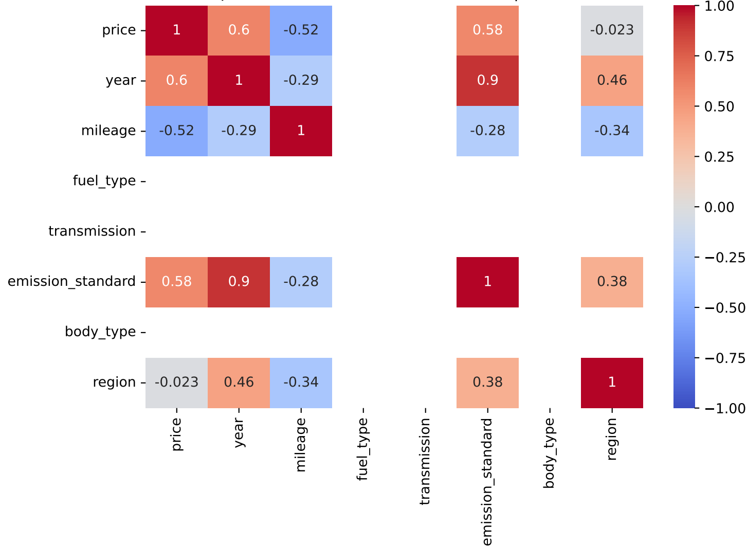
Spearman Correlation - Model: delta | Fuel: 4
