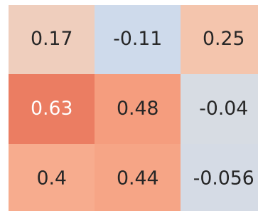
Pearson Correlation - Model: romeo 156 | Fuel: 1
