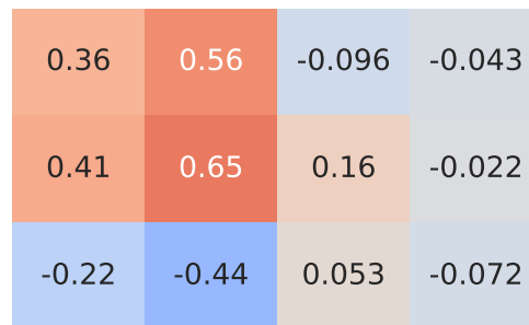
Spearman Correlation - Model: 308 | Fuel: 1
