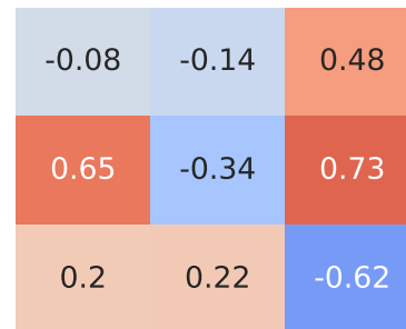
Pearson Correlation - Model: yeti | Fuel: 1
