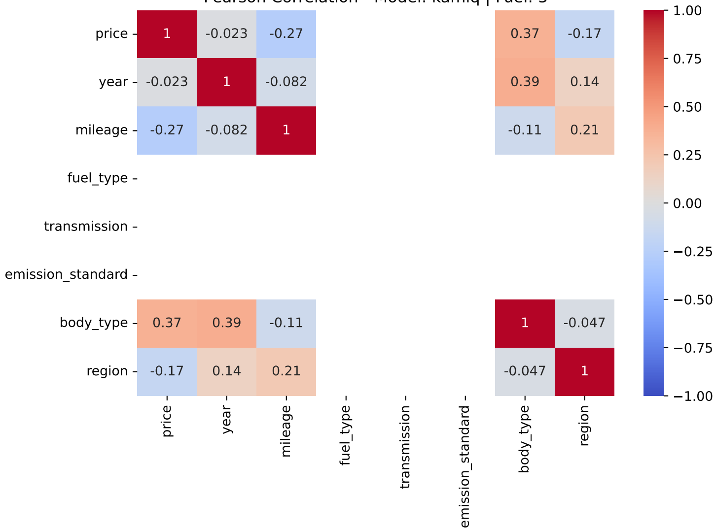
Pearson Correlation - Model: kamiq | Fuel: 5
