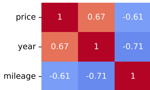
Pearson Correlation - Model: t-roc | Fuel: 2
