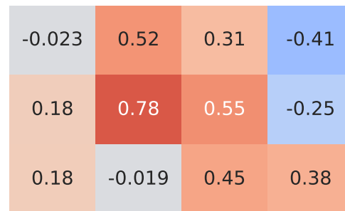
Pearson Correlation - Model: auris | Fuel: 3
