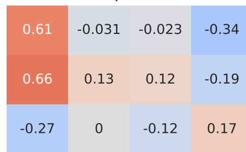
Spearman Correlation - Model: x1 | Fuel: 2
