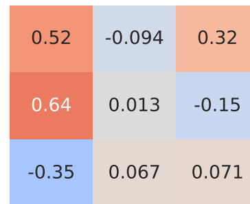
Spearman Correlation - Model: multipa | Fuel: 1
