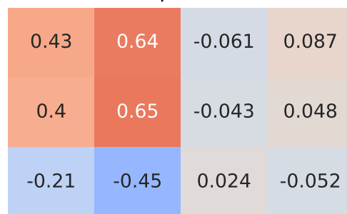
Spearman Correlation - Model: x1 | Fuel: 1
