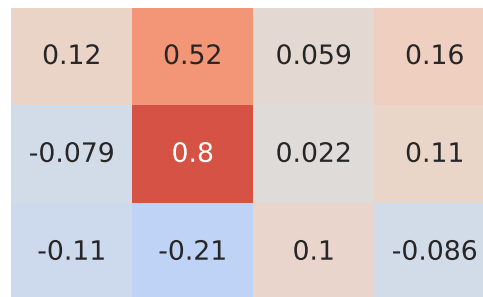
Pearson Correlation - Model: punto | Fuel: 4
