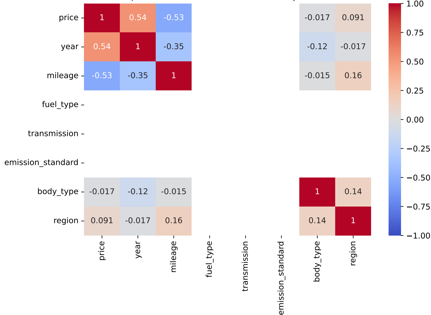
Spearman Correlation - Model: clio | Fuel: 3
