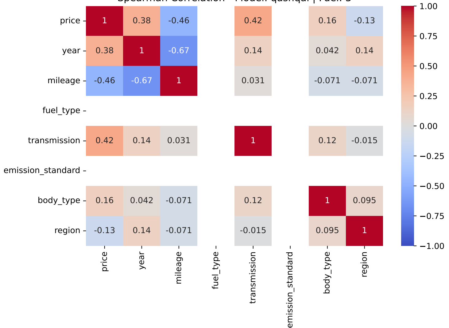
Spearman Correlation - Model: qashqai | Fuel: 3
