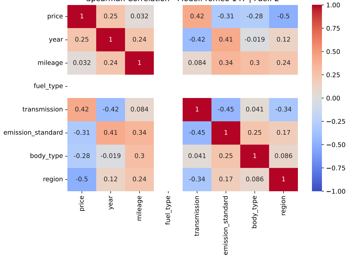
Spearman Correlation - Model: romeo 147 | Fuel: 2
