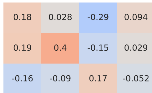
Spearman Correlation - Model: rover discovery sport | Fuel: 1
