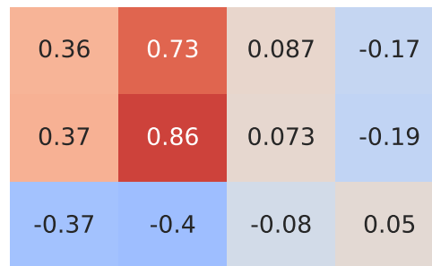
Spearman Correlation - Model: c3 | Fuel: 4
