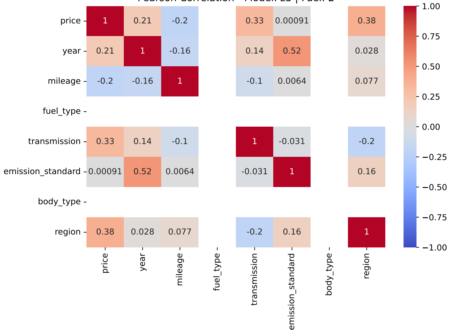
Pearson Correlation - Model: z3 | Fuel: 2
