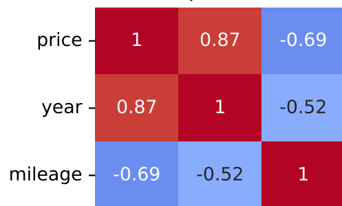
Spearman Correlation - Model: scenic | Fuel: 1
