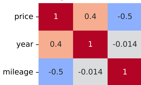
Spearman Correlation - Model: grande punto | Fuel: 4
