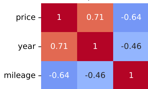
Spearman Correlation - Model: tipo | Fuel: 2
