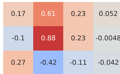
Pearson Correlation - Model: leon | Fuel: 2
