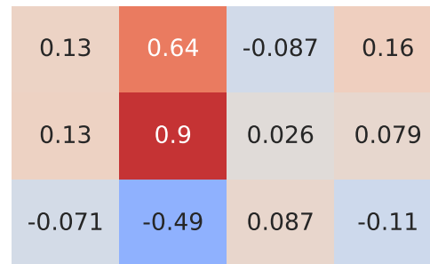
Spearman Correlation - Model: ibiza | Fuel: 1
