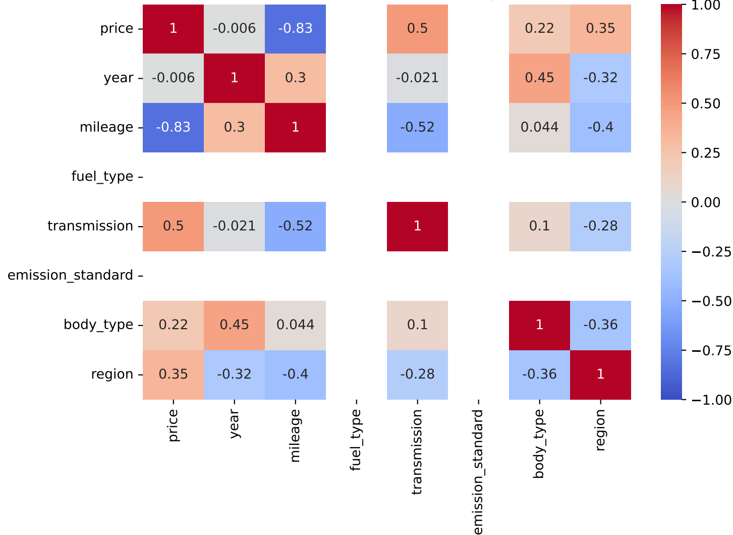
Pearson Correlation - Model: v90 | Fuel: 1
