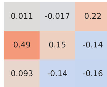
Pearson Correlation - Model: romeo 147 | Fuel: 1
