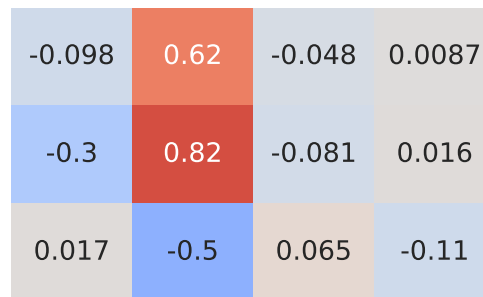
Pearson Correlation - Model: micra | Fuel: 4
