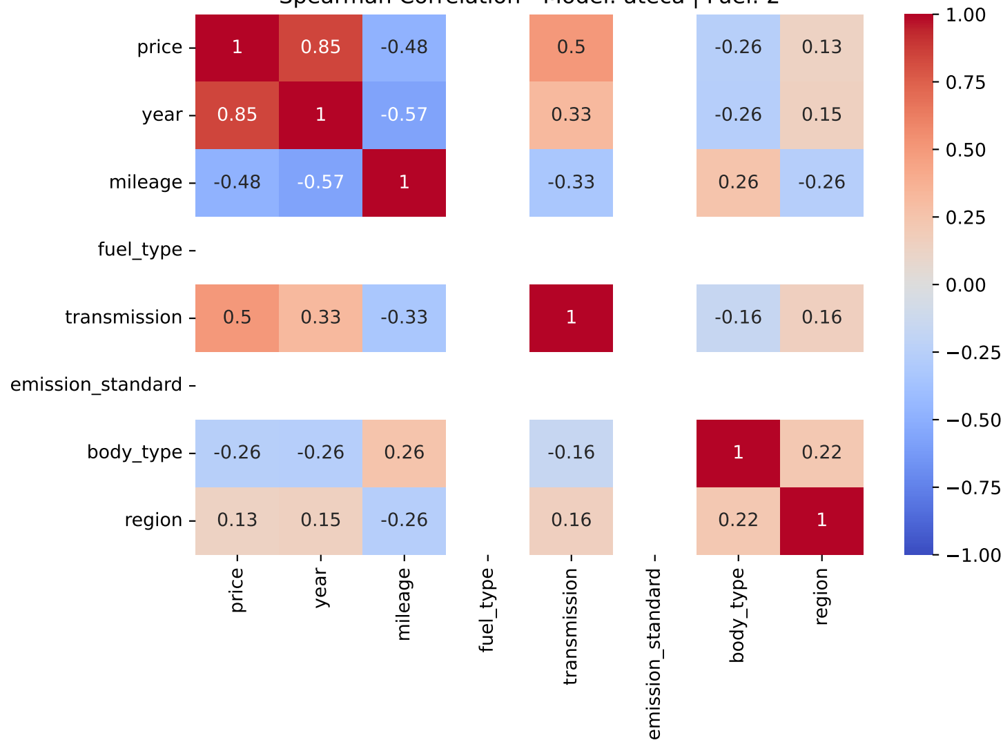
Spearman Correlation - Model: ateca | Fuel: 2
