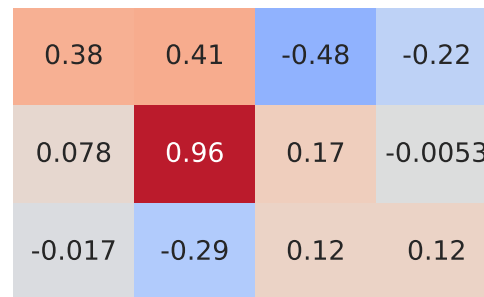
Pearson Correlation - Model: transit | Fuel: 1
