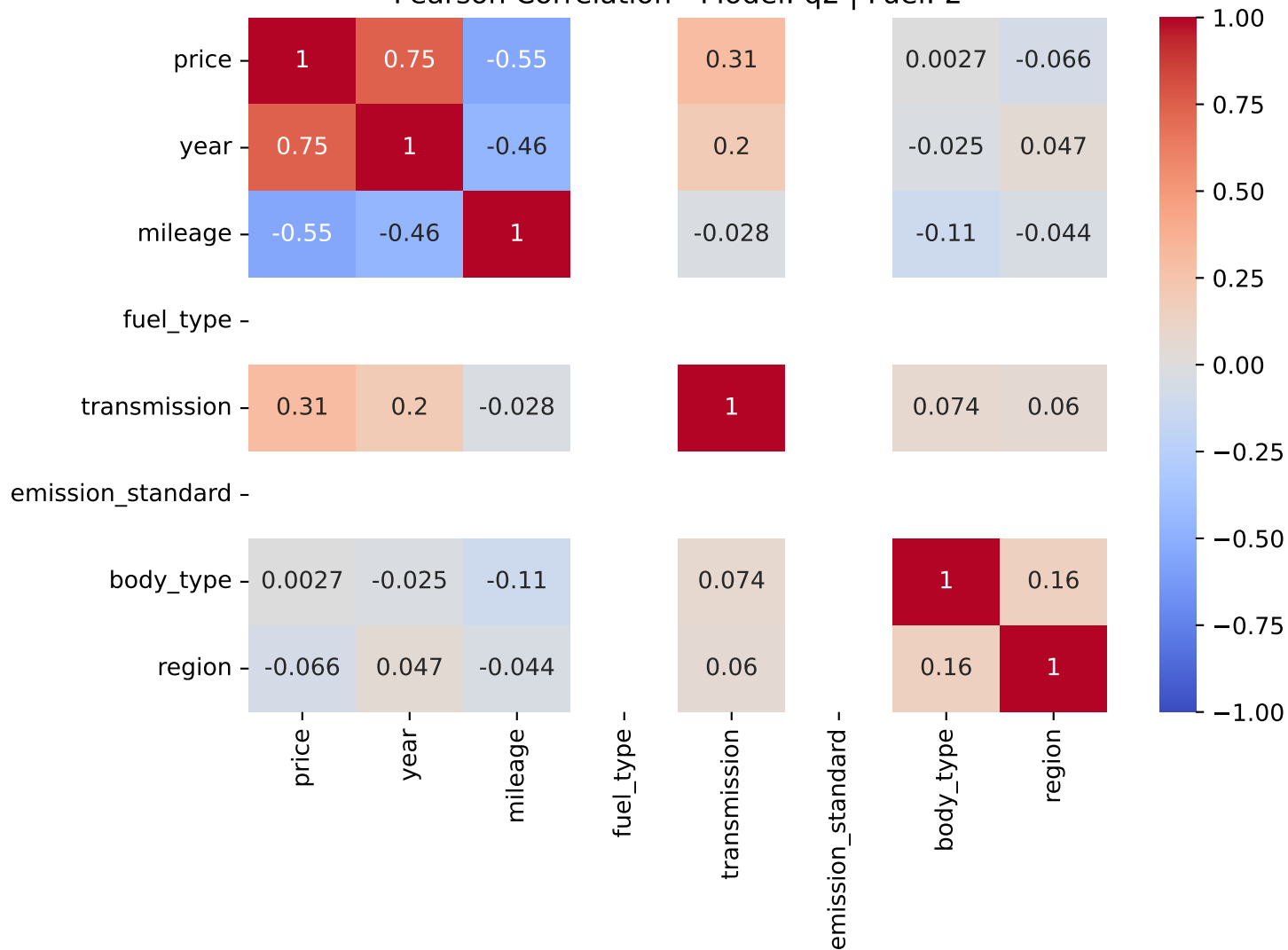
Pearson Correlation - Model: q2 | Fuel: 2
