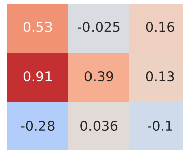
Spearman Correlation - Model: romeo mito | Fuel: 4
