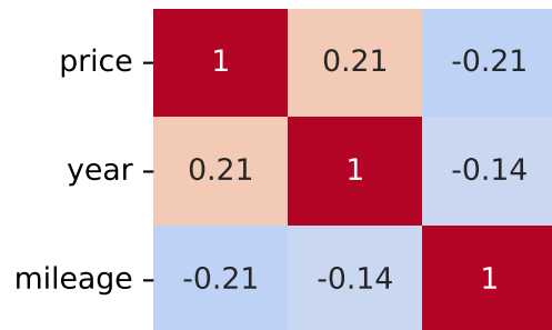
Spearman Correlation - Model: multipa | Fuel: 5
