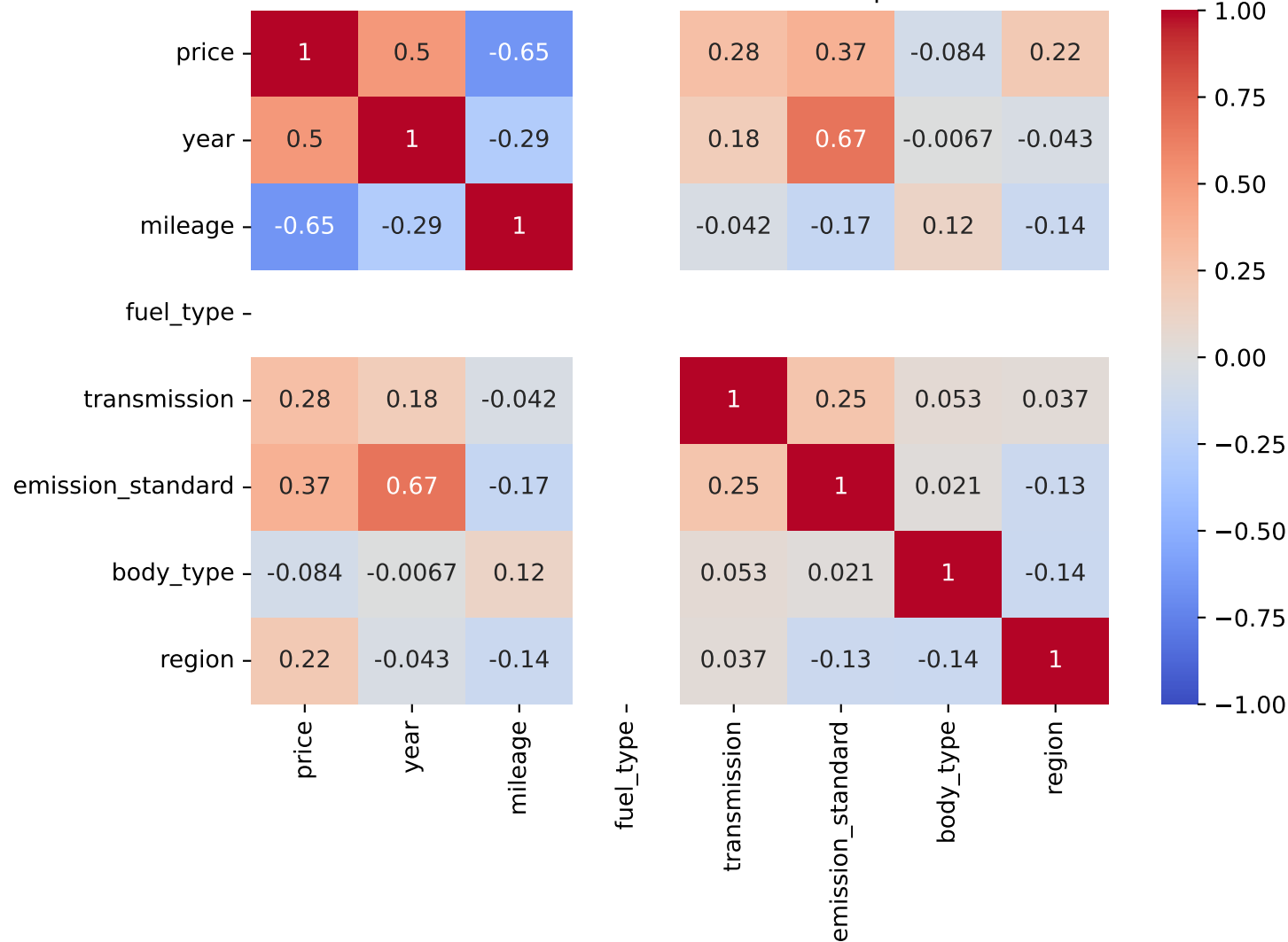
Pearson Correlation - Model: musa | Fuel: 2
