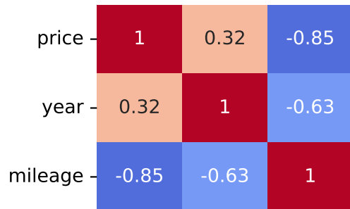
Pearson Correlation - Model: vengs | Fuel: 2
