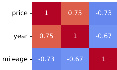
Spearman Correlation - Model: 500x | Fuel: 2
