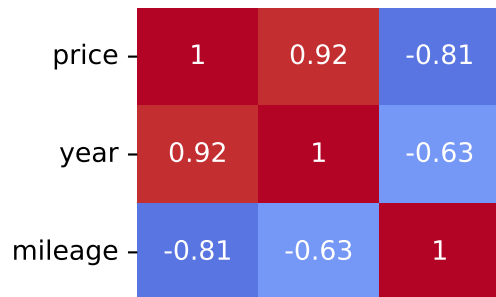
Pearson Correlation - Model: touareg | Fuel: 1
