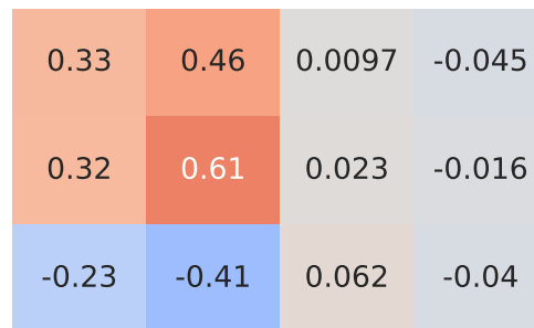
Pearson Correlation - Model: q3 | Fuel: 1
