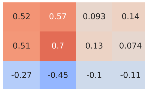
Pearson Correlation - Model: countryman | Fuel: 1
