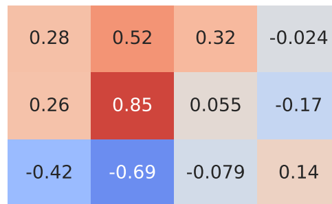
Pearson Correlation - Model: rover evoque | Fuel: 1
