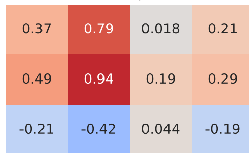
Spearman Correlation - Model: mondeo | Fuel: 1
