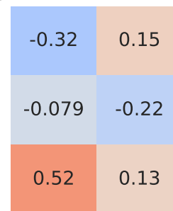
Pearson Correlation - Model: bayon | Fuel: 2
