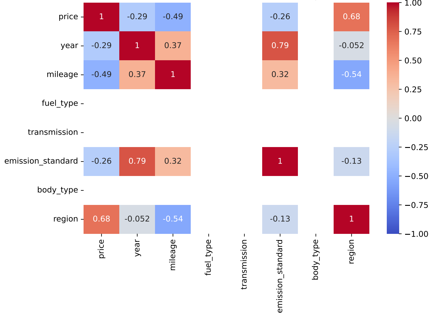
Spearman Correlation - Model: romeo spider | Fuel: 2
