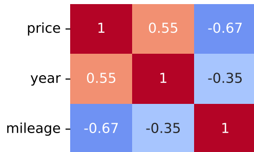
Spearman Correlation - Model: b-max | Fuel: 2
