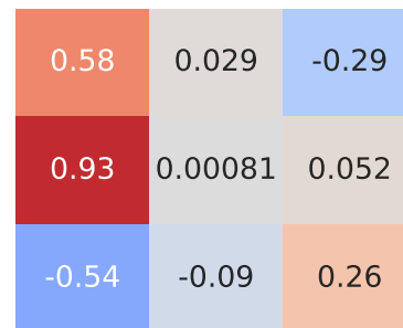
Pearson Correlation - Model: grand vitara | Fuel: 2
