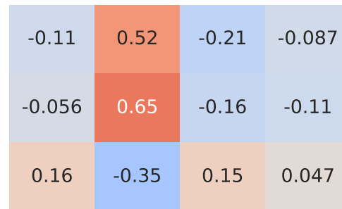
Spearman Correlation - Model: mokka | Fuel: 1
