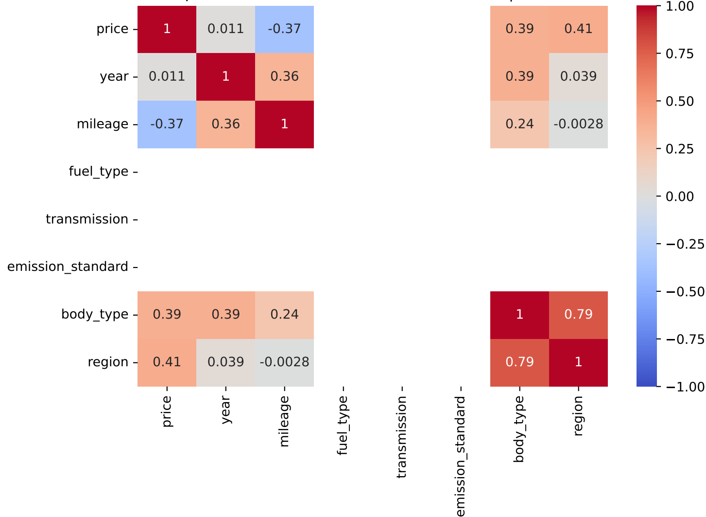
Spearman Correlation - Model: new beetle | Fuel: 2
