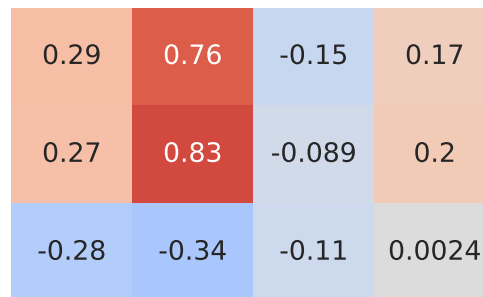
Pearson Correlation - Model: rav4 | Fuel: 1
