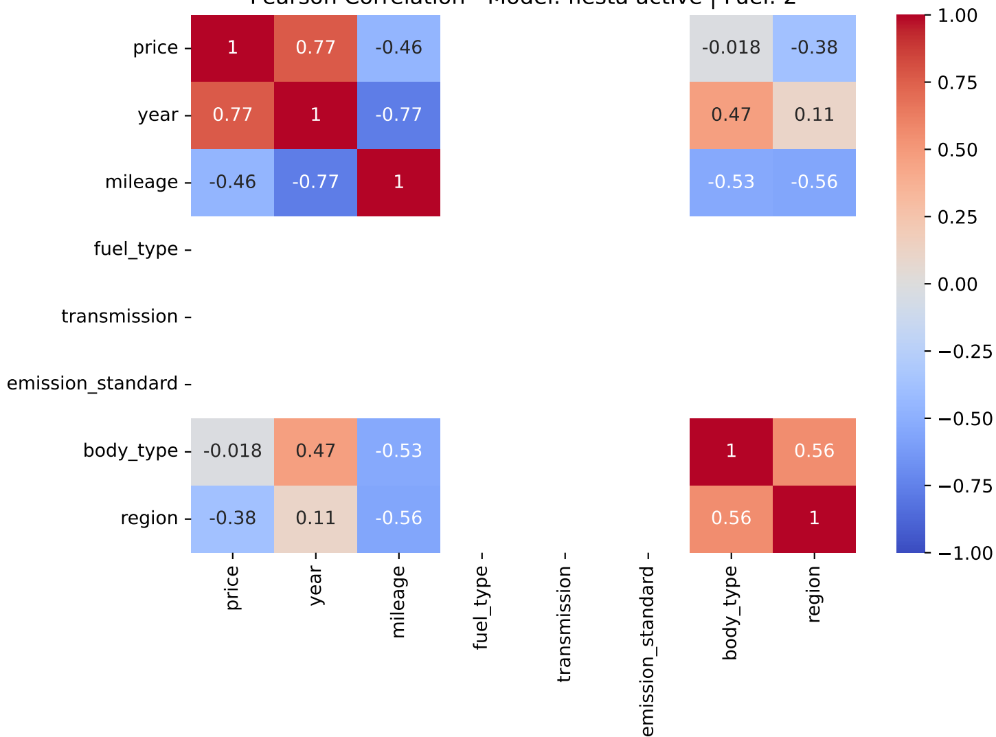
Pearson Correlation - Model: fiesta active | Fuel: 2
