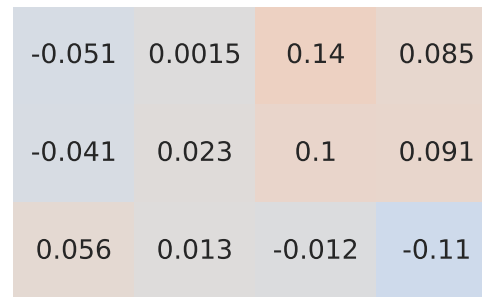
Spearman Correlation - Model: 500 | Fuel: 3
