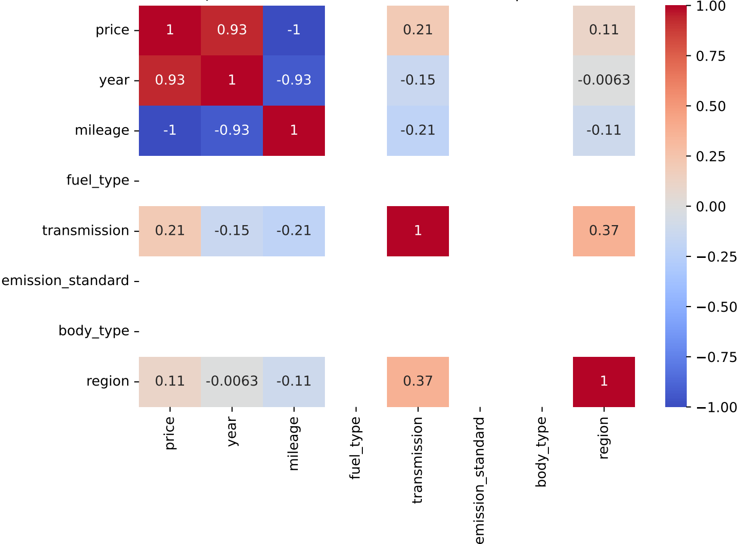
Spearman Correlation - Model: tarraco | Fuel: 2
