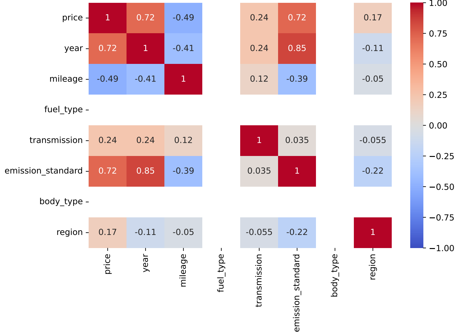
Spearman Correlation - Model: traffic | Fuel: 1
