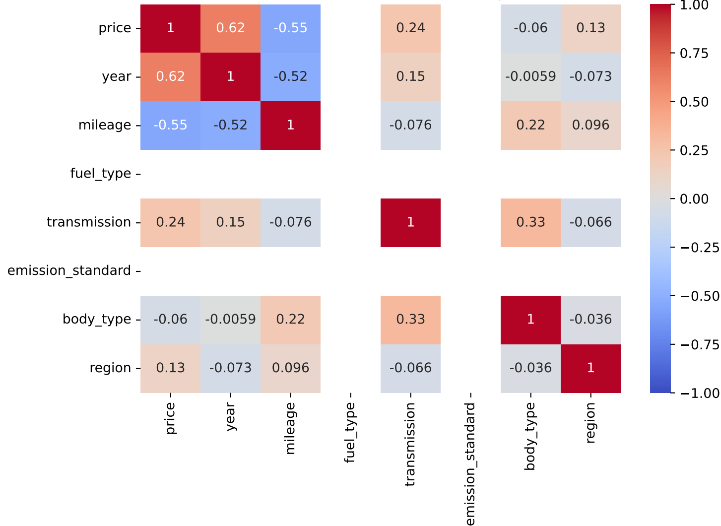
Spearman Correlation - Model: focus | Fuel: 3
