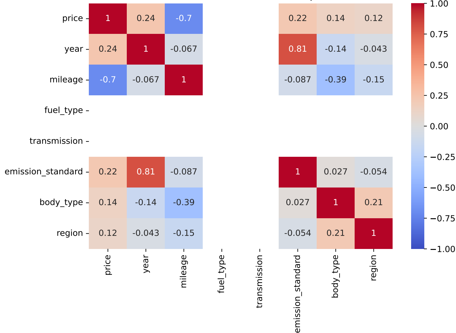
Pearson Correlation - Model: sedici | Fuel: 2
