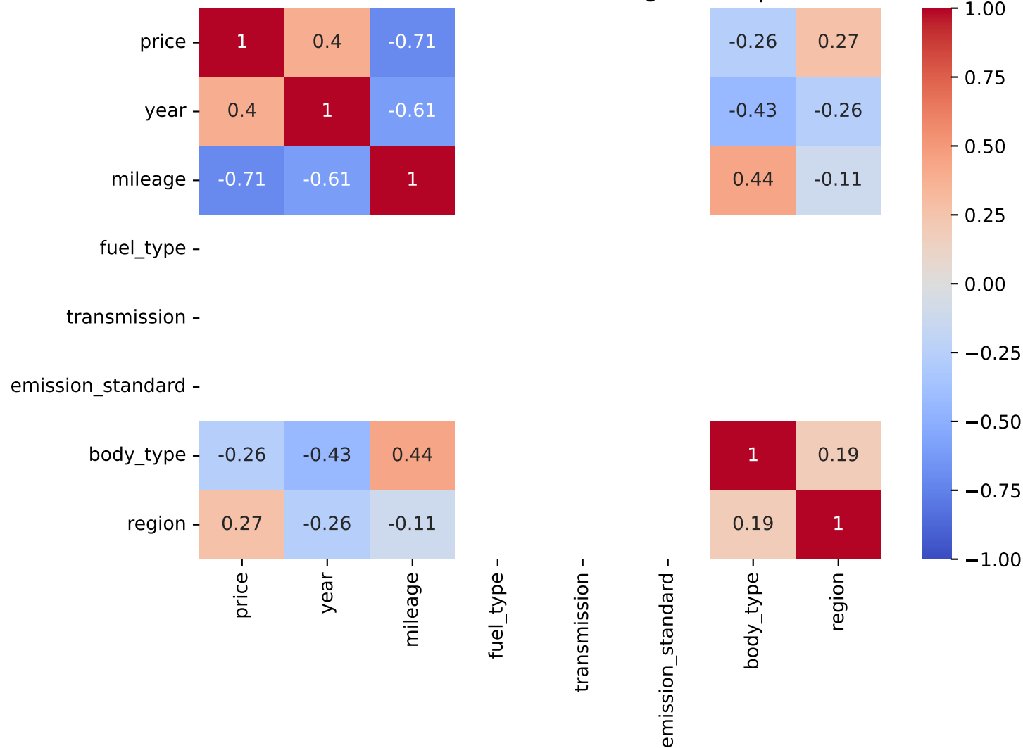
Pearson Correlation - Model: mustang mach-e | Fuel: 0
