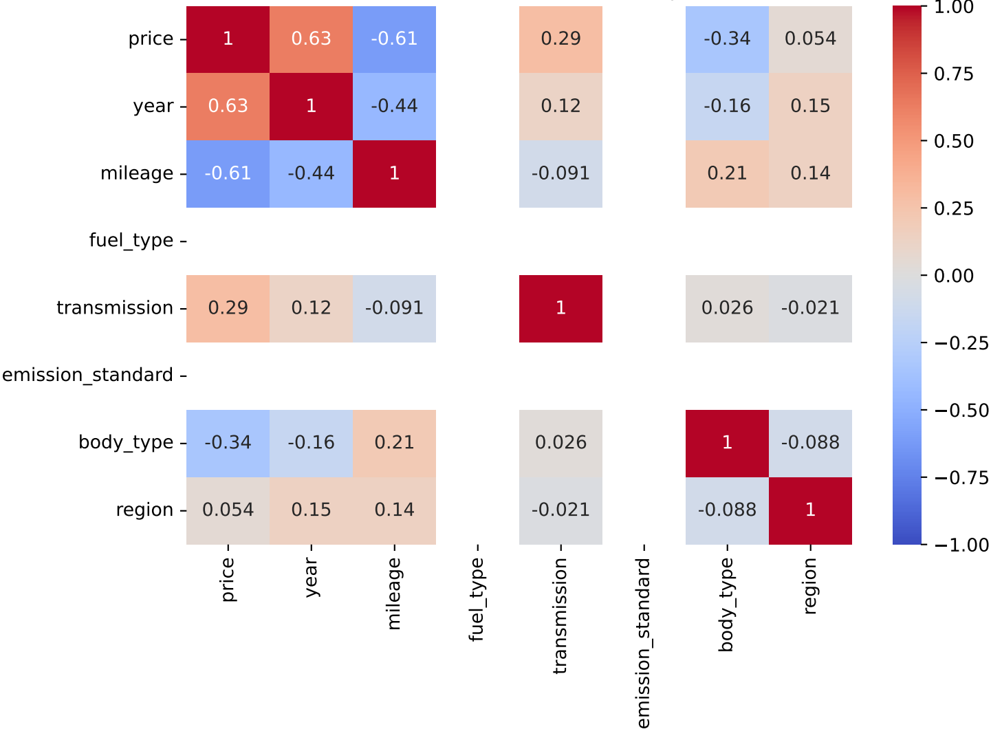
Pearson Correlation - Model: fiesta | Fuel: 3
