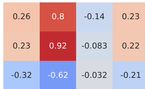
Spearman Correlation - Model: swift | Fuel: 2
