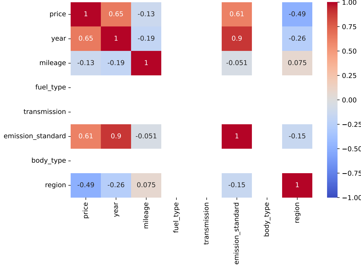
Spearman Correlation - Model: dobro | Fuel: 2
