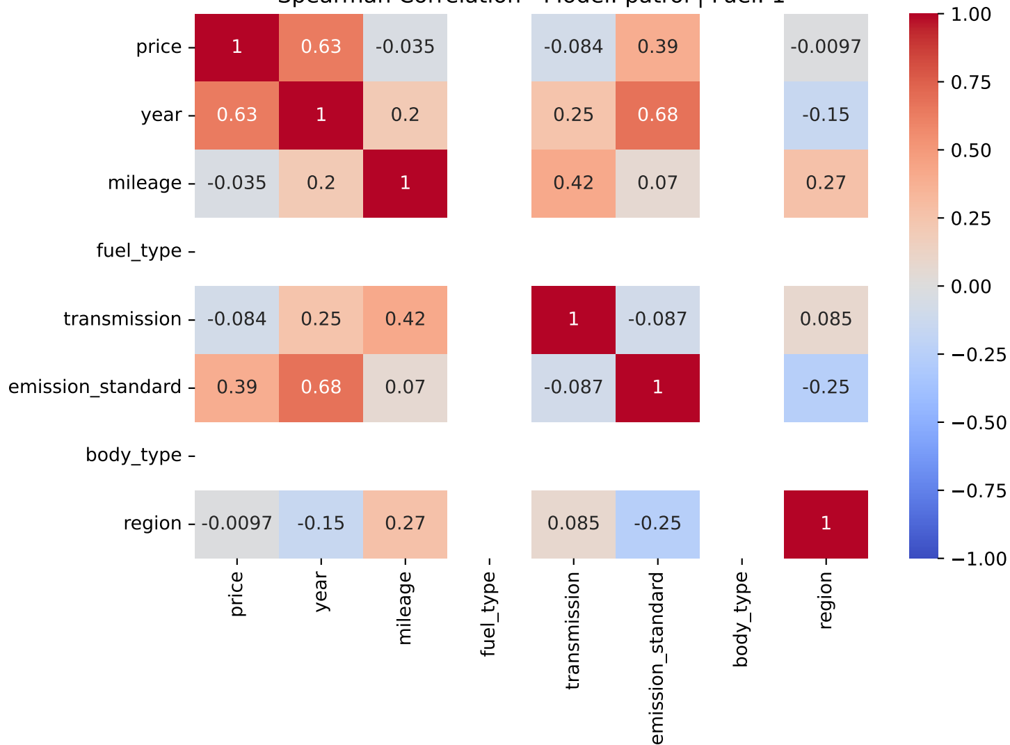
Spearman Correlation - Model: patrol | Fuel: 1
