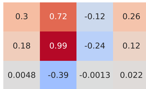
Pearson Correlation - Model: vitara | Fuel: 1
