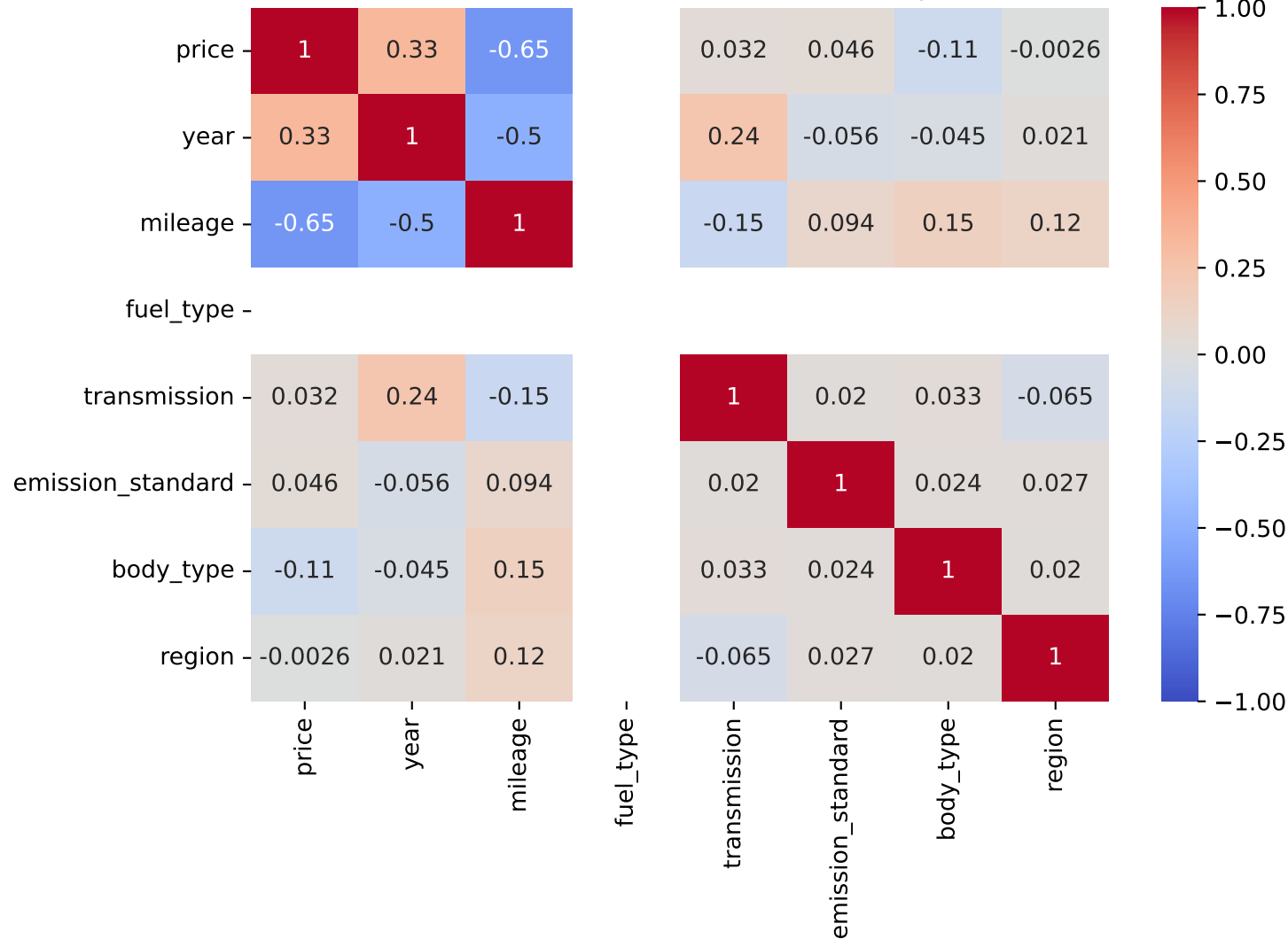
Spearman Correlation - Model: renegade | Fuel: 3
