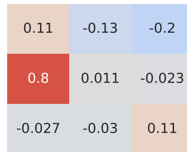
Pearson Correlation - Model: grand vitara | Fuel: 1
