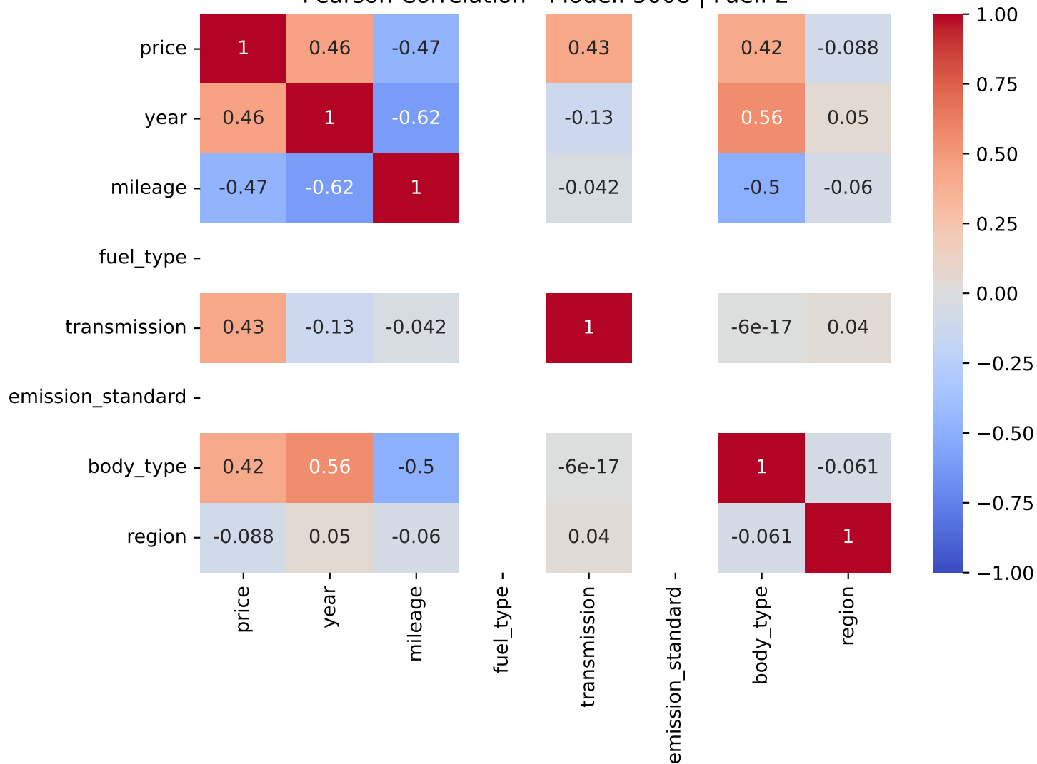
Pearson Correlation - Model: 5008 | Fuel: 2
