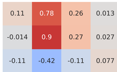
Pearson Correlation - Model: micra | Fuel: 2
