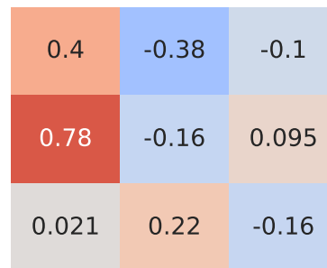
Pearson Correlation - Model: sx4 | Fuel: 1
