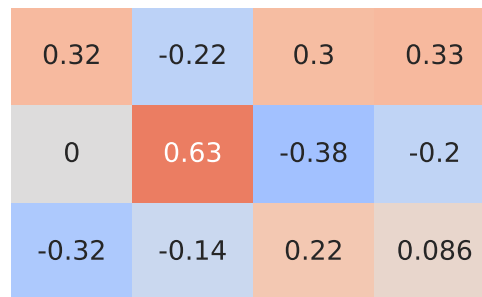
Spearman Correlation - Model: romeo 156 | Fuel: 2
