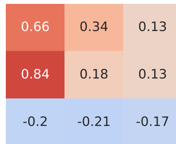
Spearman Correlation - Model: panda 4x4 | Fuel: 1
