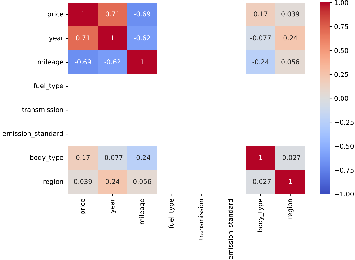
Spearman Correlation - Model: polo | Fuel: 5
