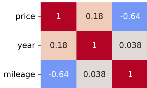
Pearson Correlation - Model: zafira tourer | Fuel: 5
