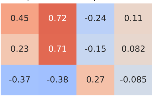
Spearman Correlation - Model: grand scenic | Fuel: 1
