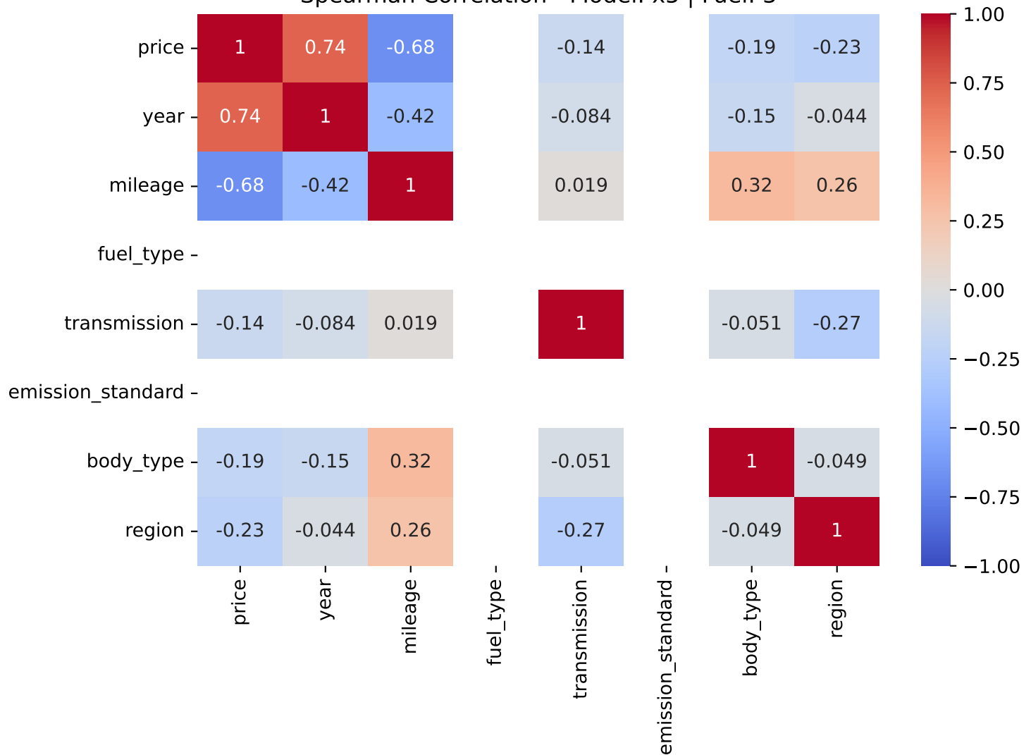
Spearman Correlation - Model: x5 | Fuel: 3
