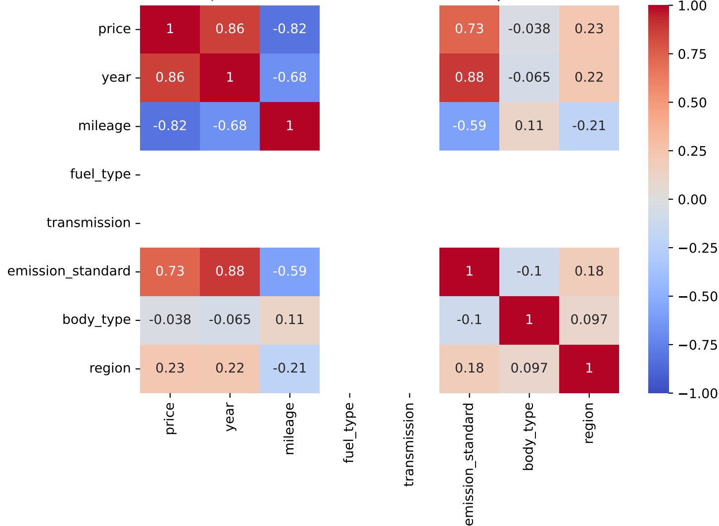
Spearman Correlation - Model: fiesta | Fuel: 4
