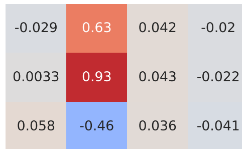
Pearson Correlation - Model: panda | Fuel: 1
