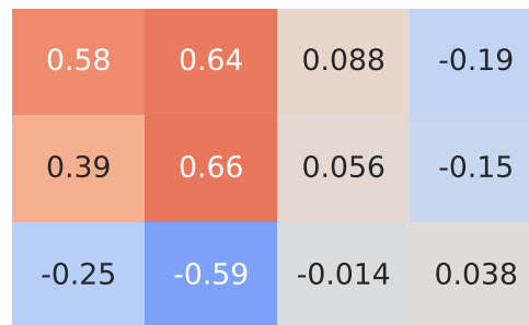
Spearman Correlation - Model: a3 | Fuel: 2
