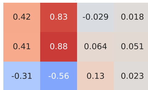
Spearman Correlation - Model: astra | Fuel: 1
