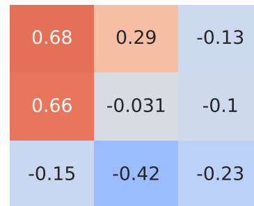
Spearman Correlation - Model: venga | Fuel: 1
