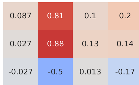
Spearman Correlation - Model: fiesta | Fuel: 2
