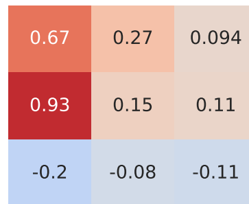
Pearson Correlation - Model: punto | Fuel: 2
