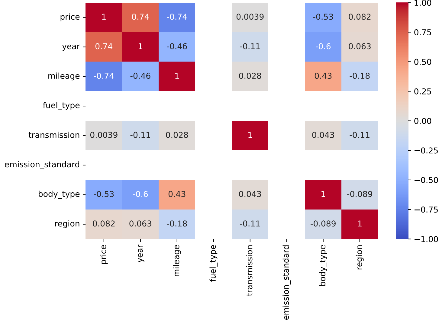
Pearson Correlation - Model: c4 cactus | Fuel: 2
