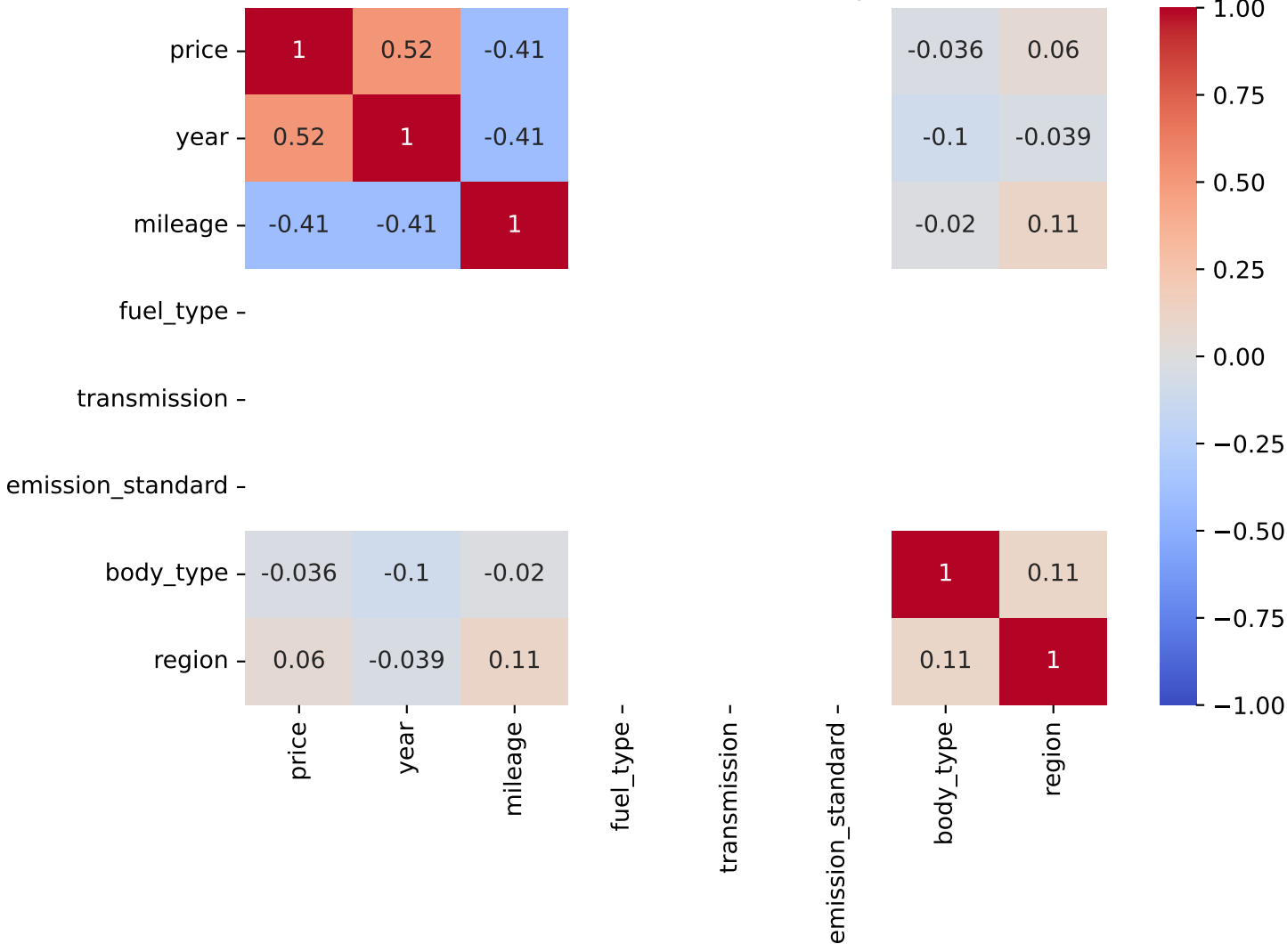
Pearson Correlation - Model: clio | Fuel: 3
