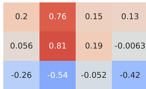
Spearman Correlation - Model: a7 | Fuel: 1
