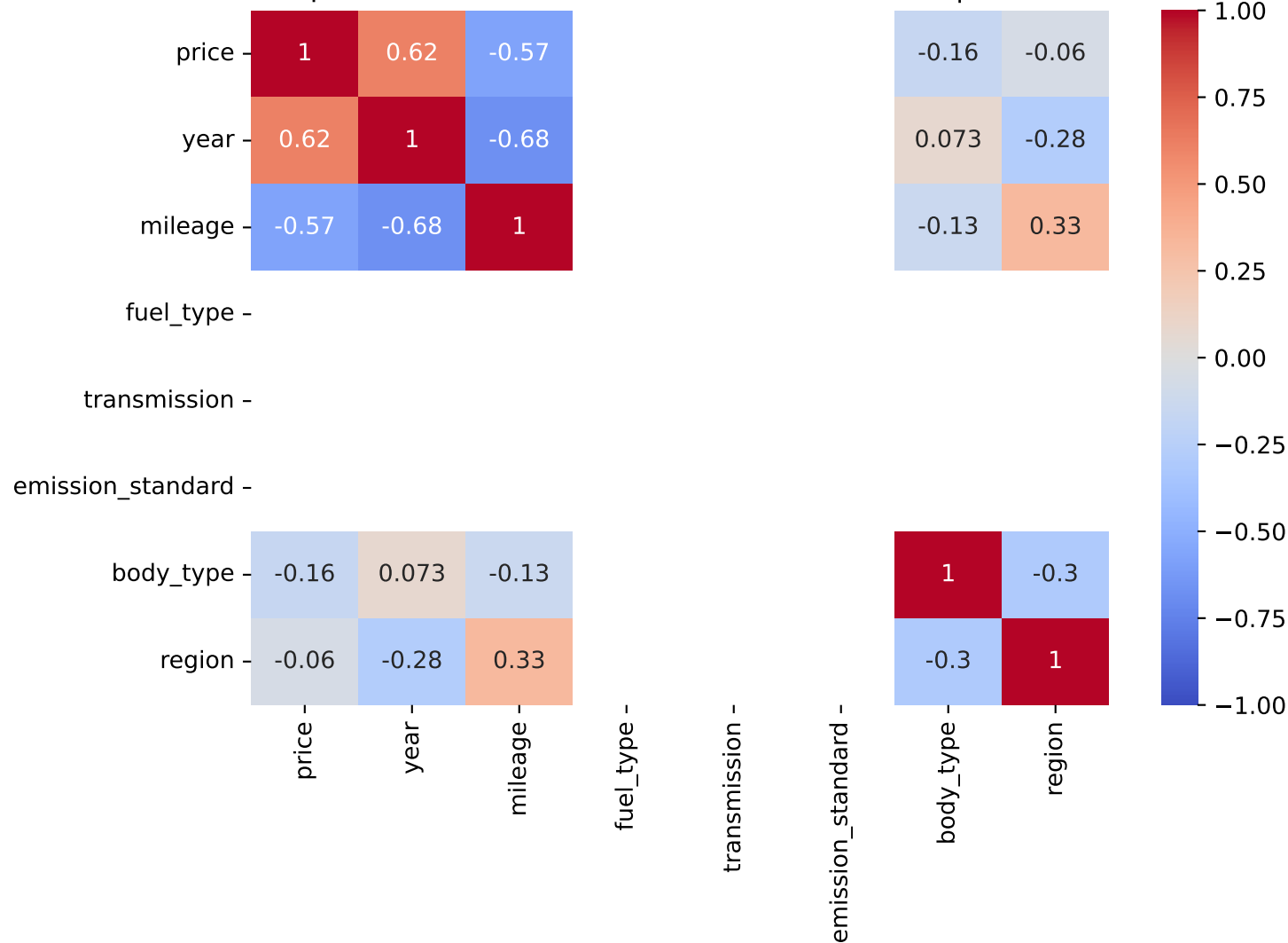
Spearman Correlation - Model: rover defender | Fuel: 3
