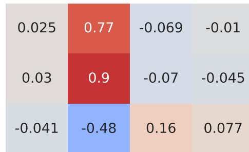
Pearson Correlation - Model: rover range rover sport | Fuel: 1
