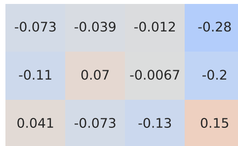
Pearson Correlation - Model: q8 | Fuel: 3
