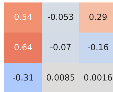
Pearson Correlation - Model: multipa | Fuel: 1
