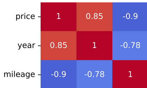
Pearson Correlation - Model: m3 | Fuel: 2
