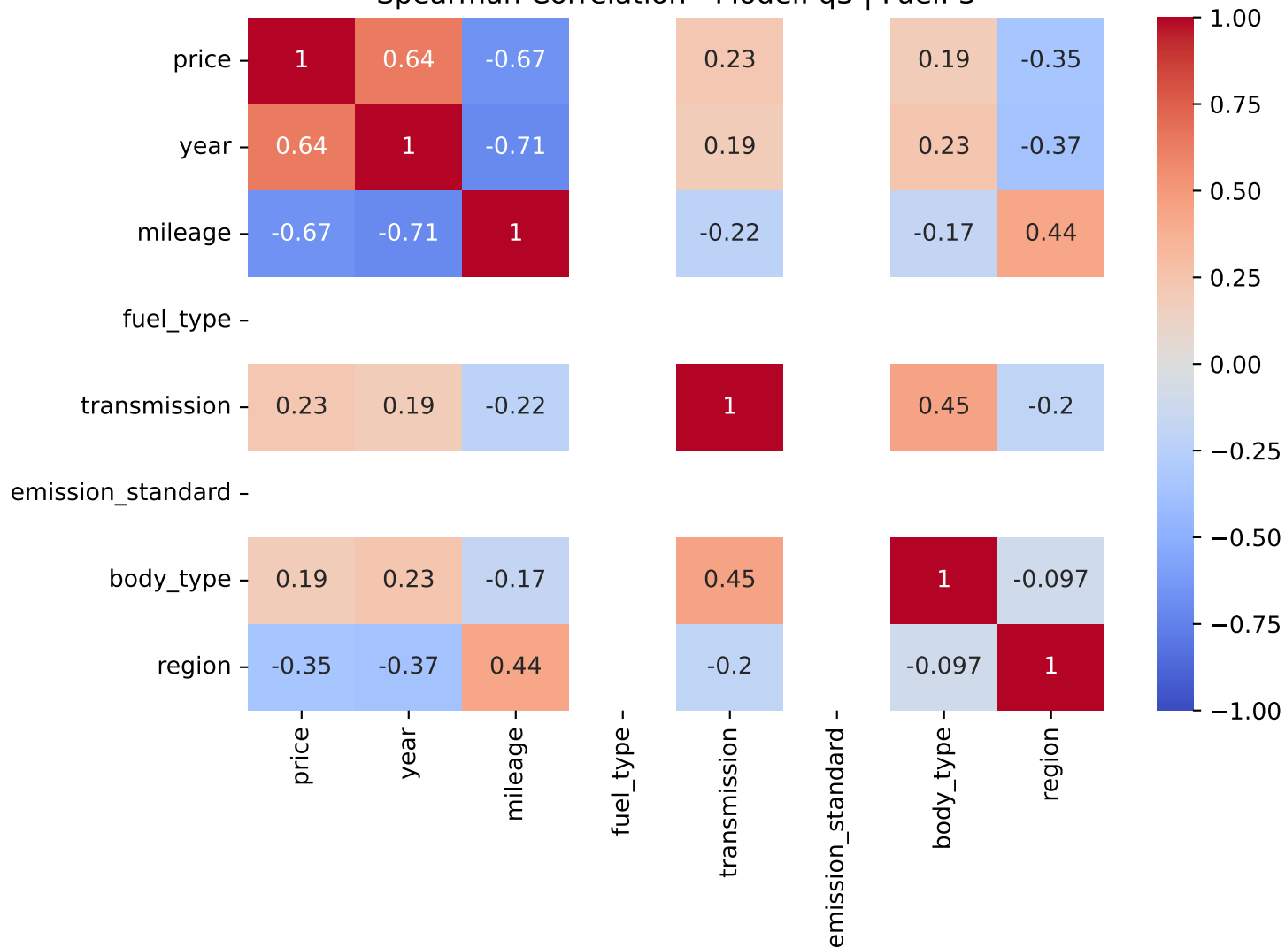
Spearman Correlation - Model: q3 | Fuel: 3
