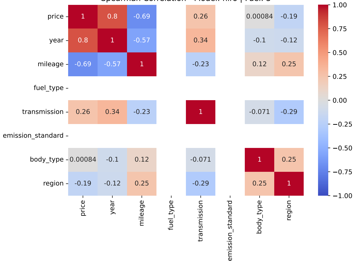
Spearman Correlation - Model: niro | Fuel: 3
