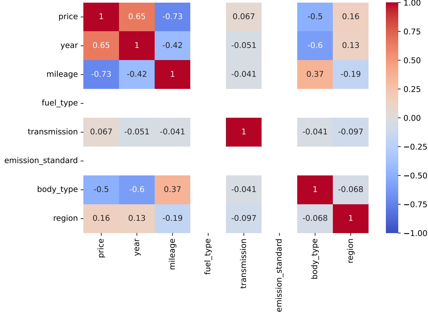
Spearman Correlation - Model: c4 cactus | Fuel: 2
