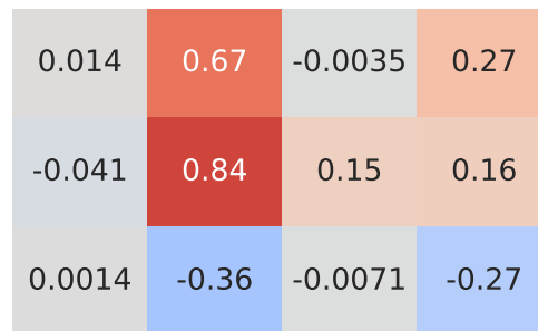
Spearman Correlation - Model: qubo | Fuel: 1
