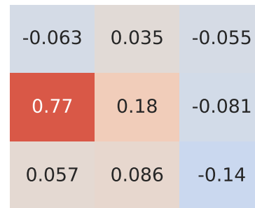
Spearman Correlation - Model: ka | Fuel: 1
