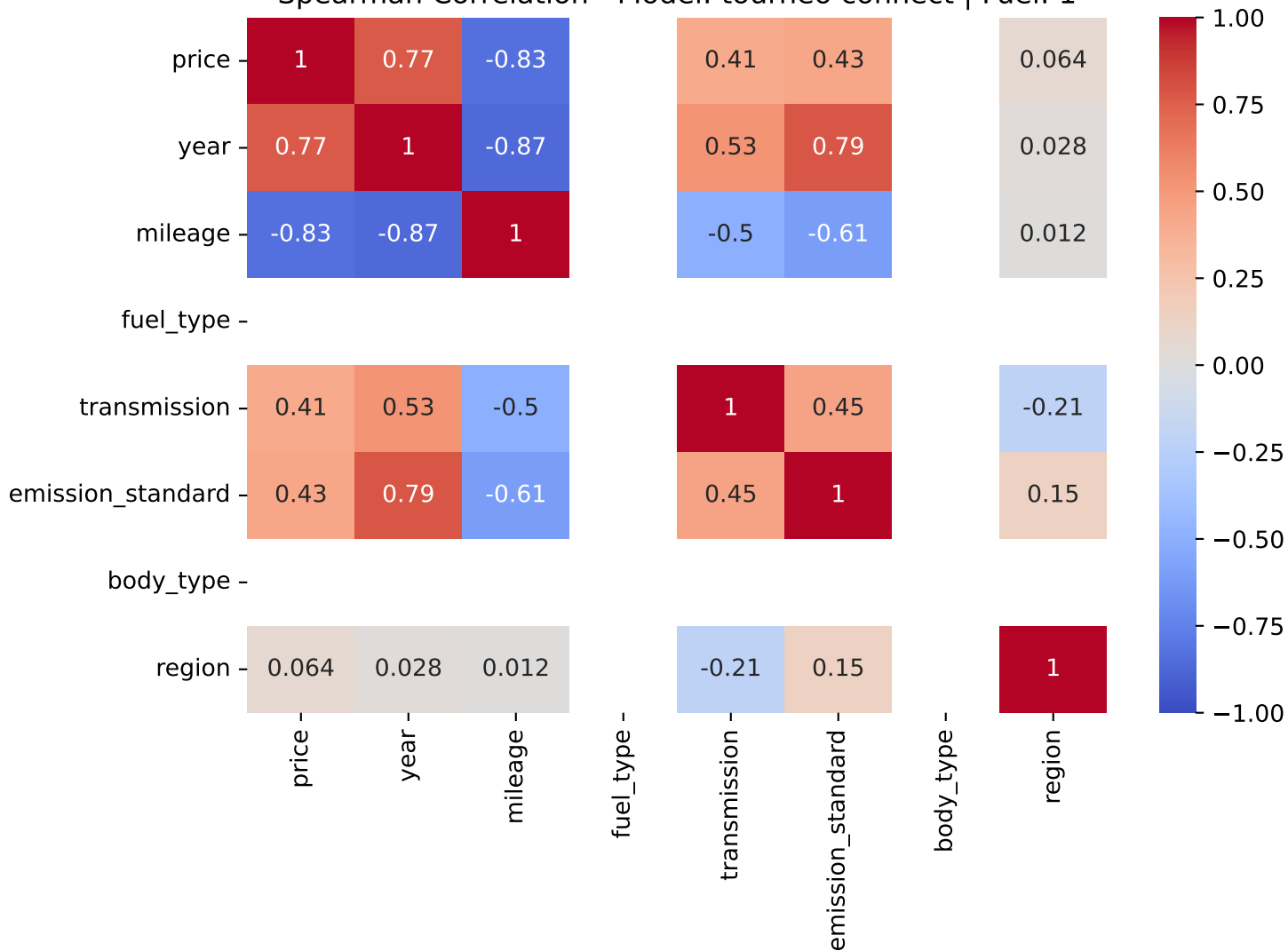
Spearman Correlation - Model: tourneo connect | Fuel: 1
