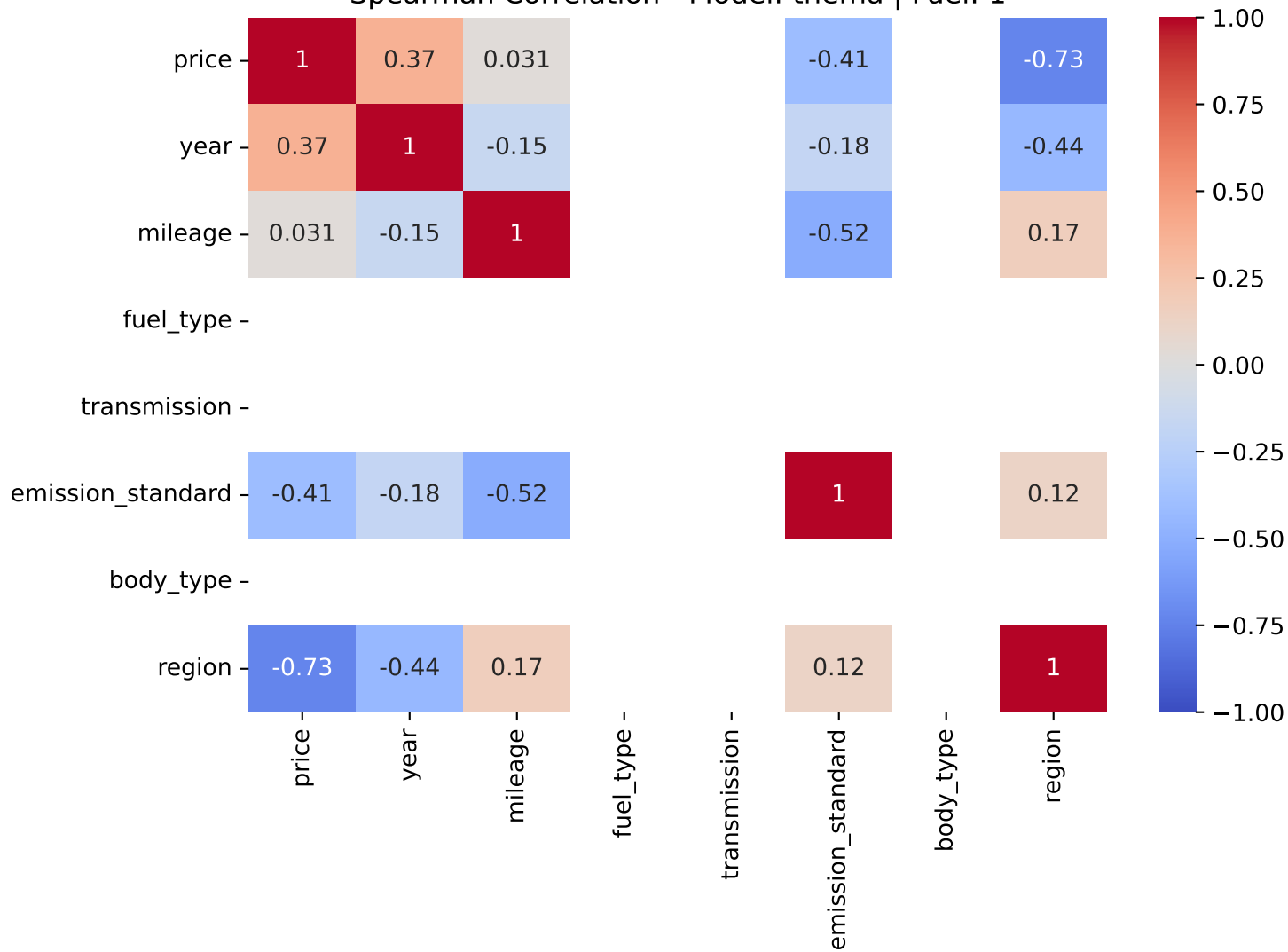
Spearman Correlation - Model: thema | Fuel: 1
