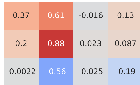
Spearman Correlation - Model: romeo giulietta | Fuel: 2
