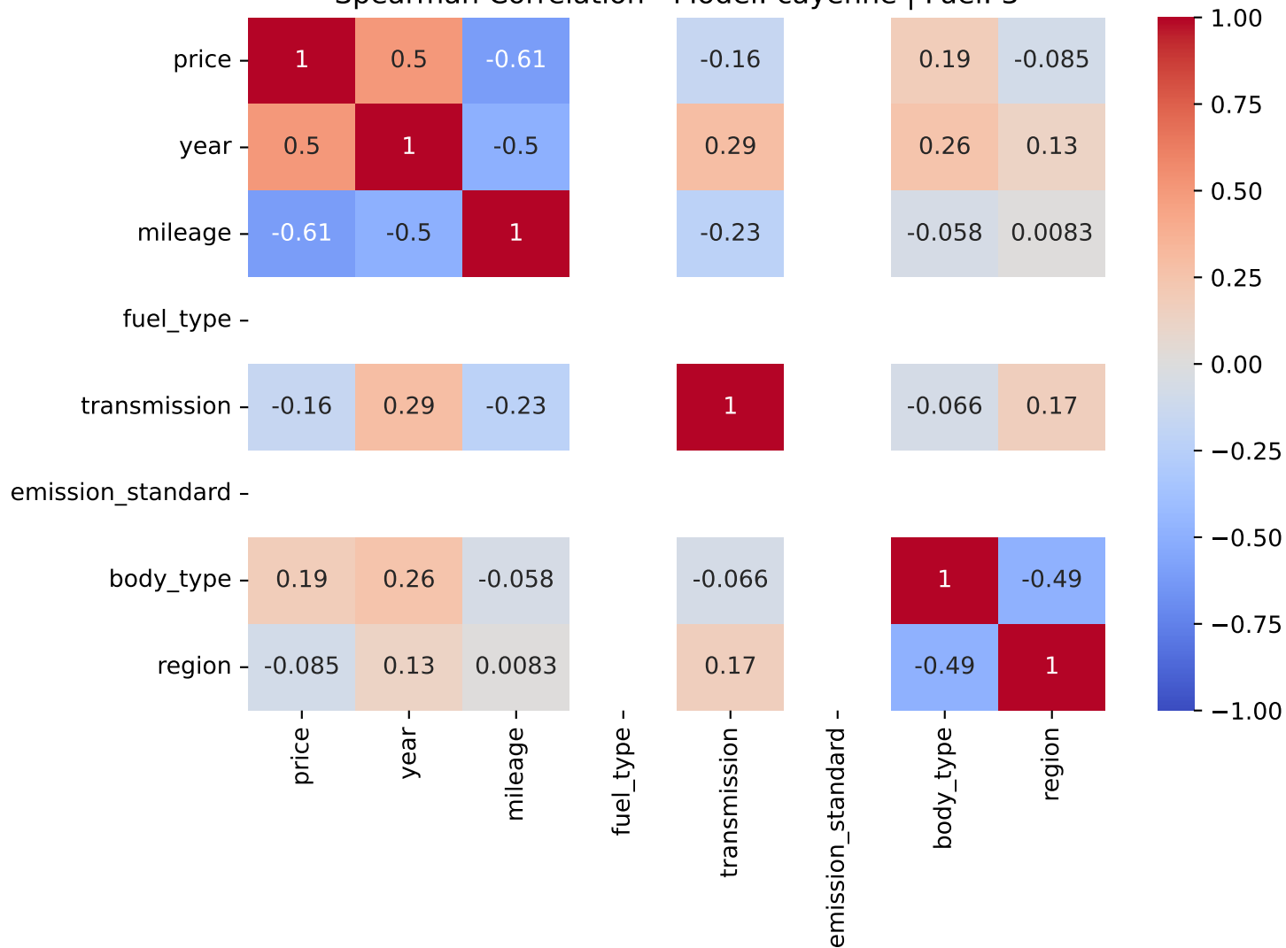
Spearman Correlation - Model: cayenne | Fuel: 3
