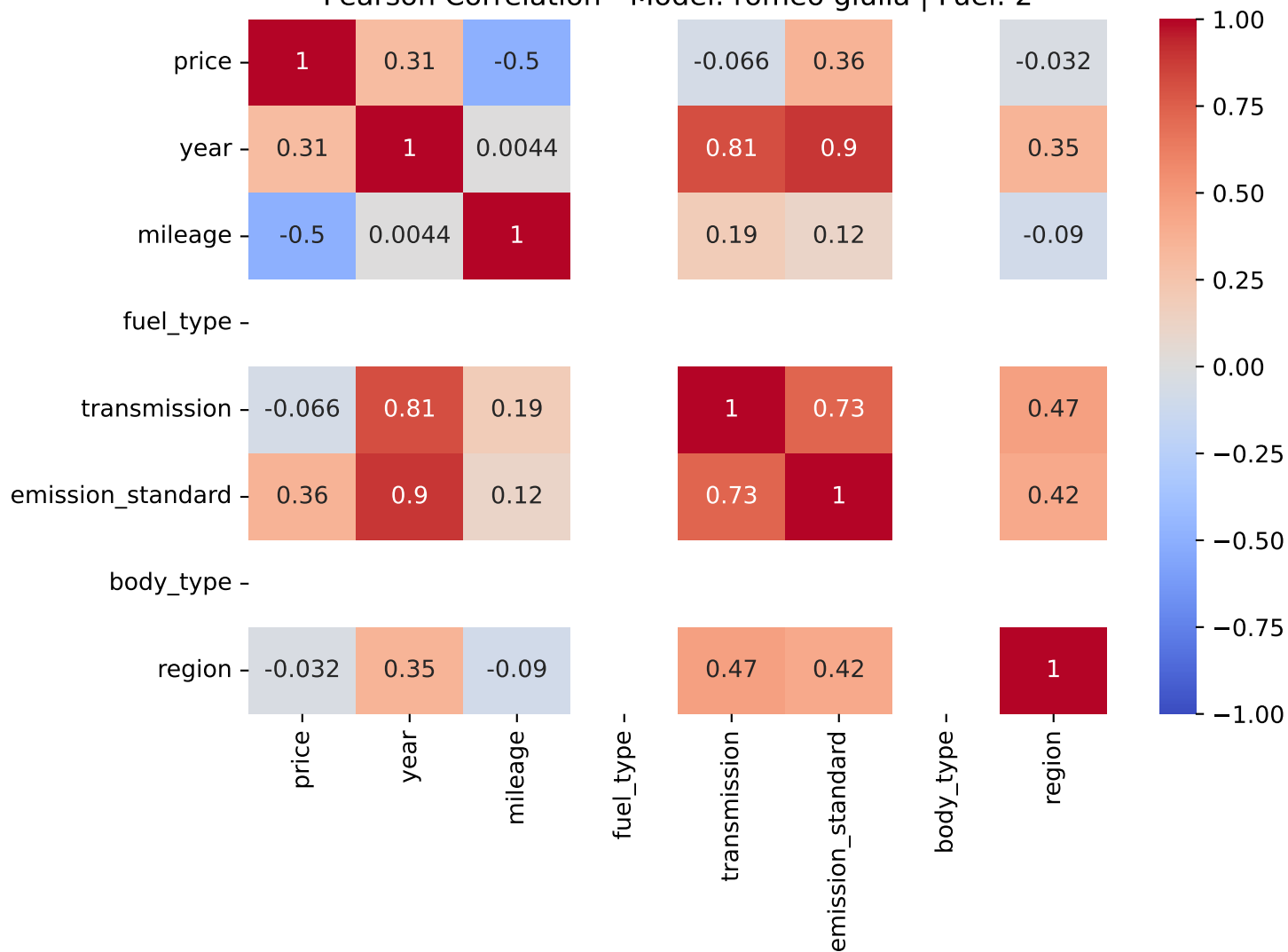
Pearson Correlation - Model: romeo giulia | Fuel: 2
