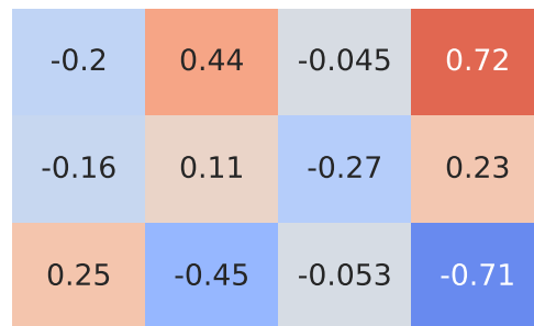
Pearson Correlation - Model: rifter | Fuel: 1
