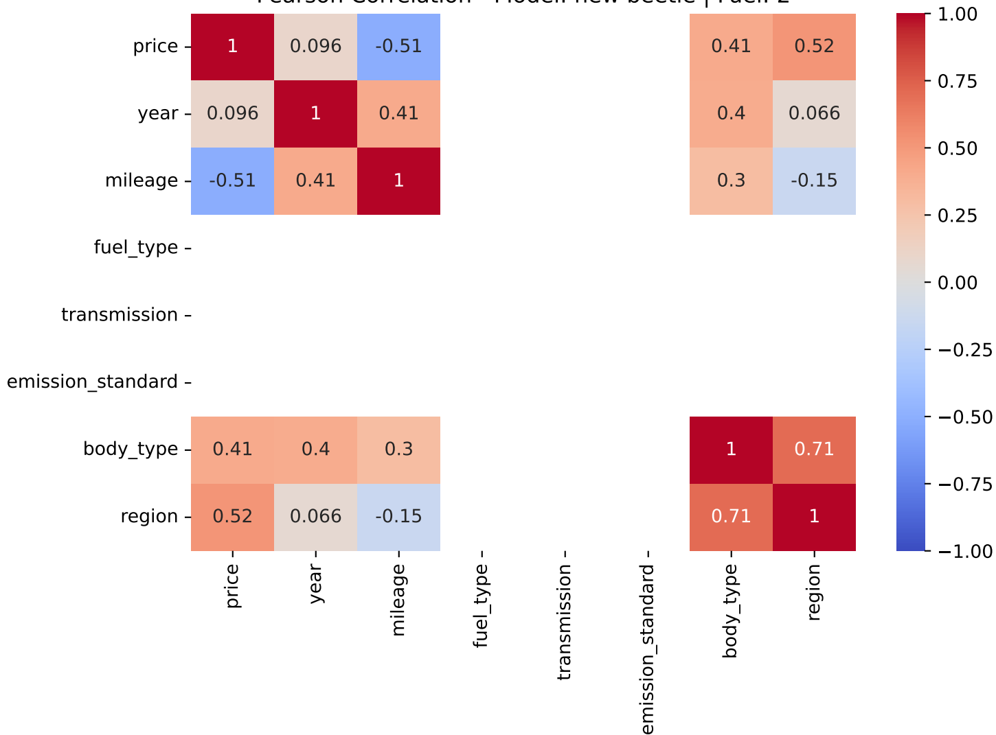
Pearson Correlation - Model: new beetle | Fuel: 2
