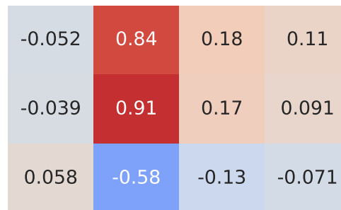
Spearman Correlation - Model: fiesta | Fuel: 1
