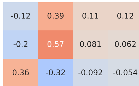
Pearson Correlation - Model: captur | Fuel: 2
