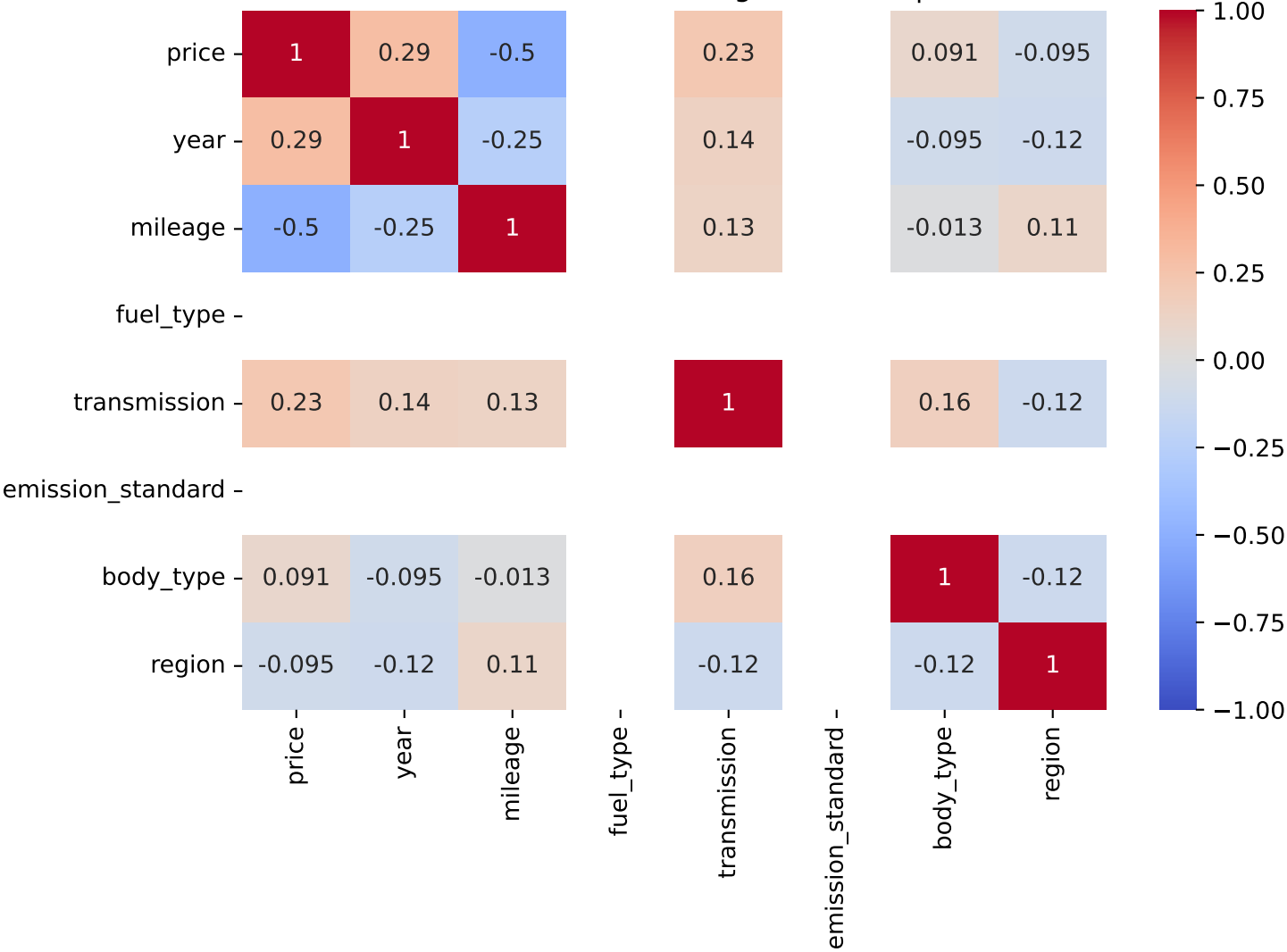
Pearson Correlation - Model: grandland x | Fuel: 1
