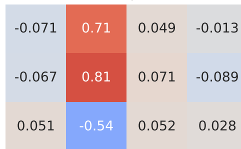
Spearman Correlation - Model: ypsilon | Fuel: 4
