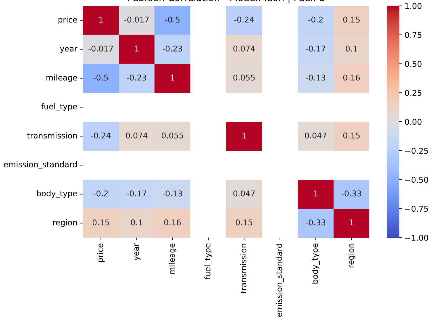
Pearson Correlation - Model: leon | Fuel: 3
