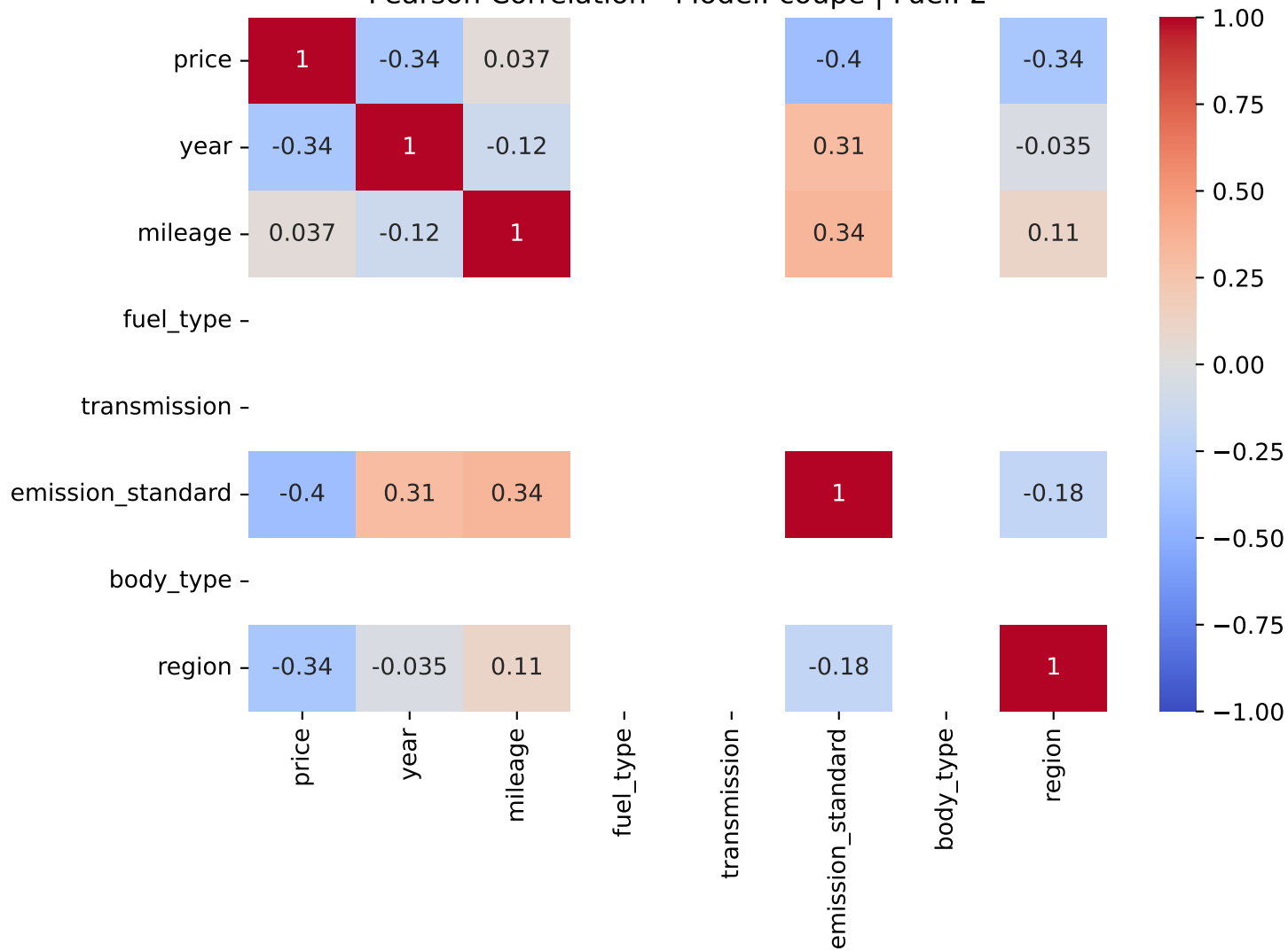
Pearson Correlation - Model: coupe | Fuel: 2
