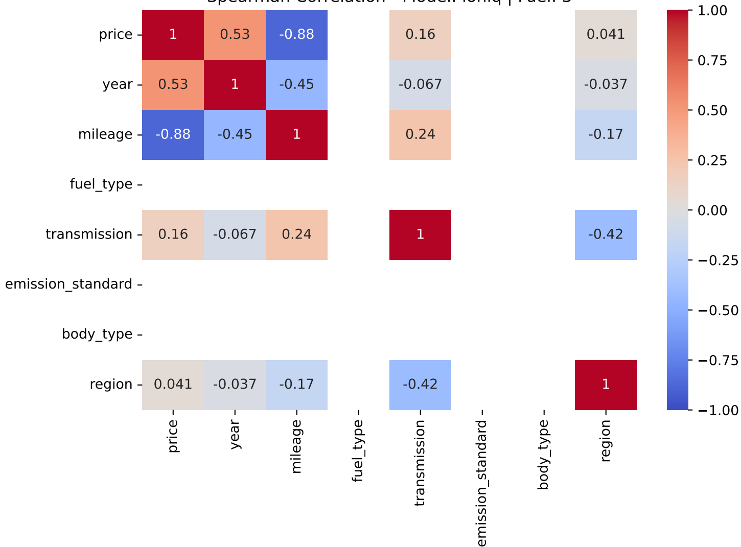
Spearman Correlation - Model: ioniq | Fuel: 3
