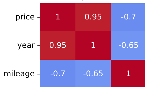
Spearman Correlation - Model: micra | Fuel: 2
