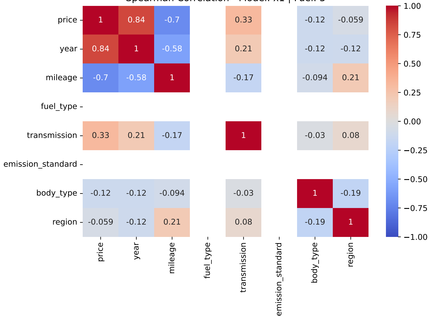
Spearman Correlation - Model: x1 | Fuel: 3
