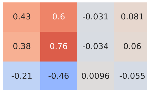
Pearson Correlation - Model: x1 | Fuel: 1
