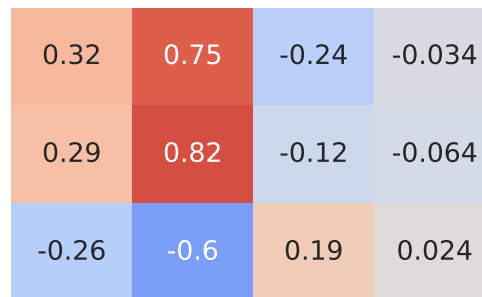
Spearman Correlation - Model: 508 | Fuel: 1
