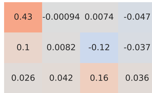
Spearman Correlation - Model: t-roc | Fuel: 2
