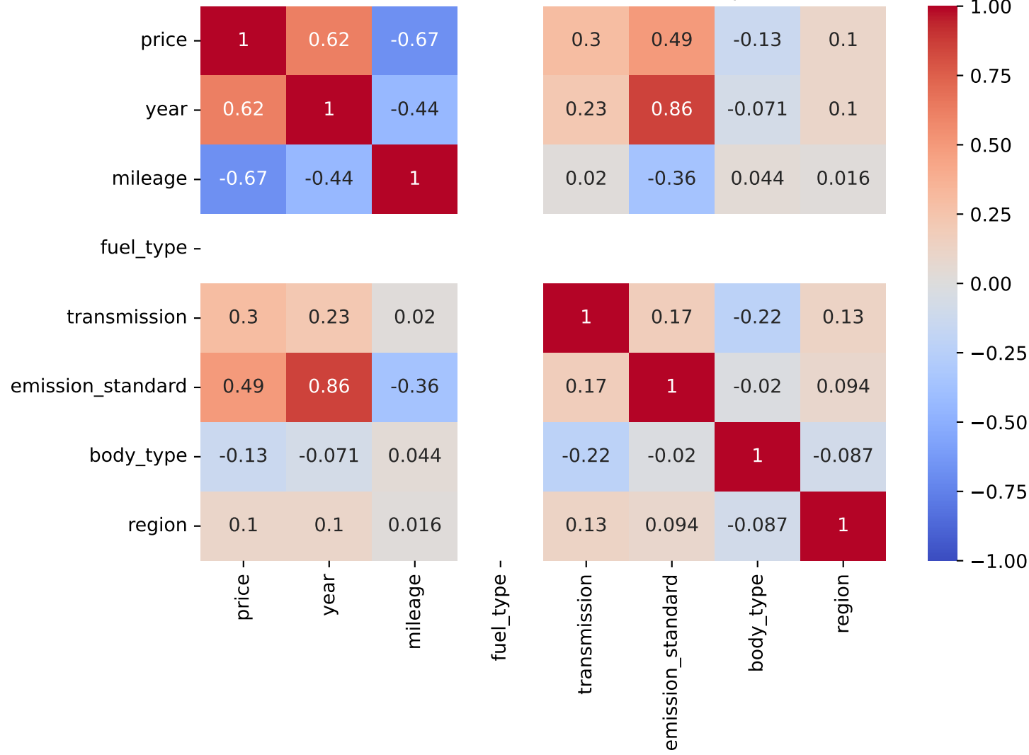
Pearson Correlation - Model: romeo mito | Fuel: 2
