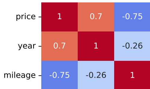
Pearson Correlation - Model: note | Fuel: 1
