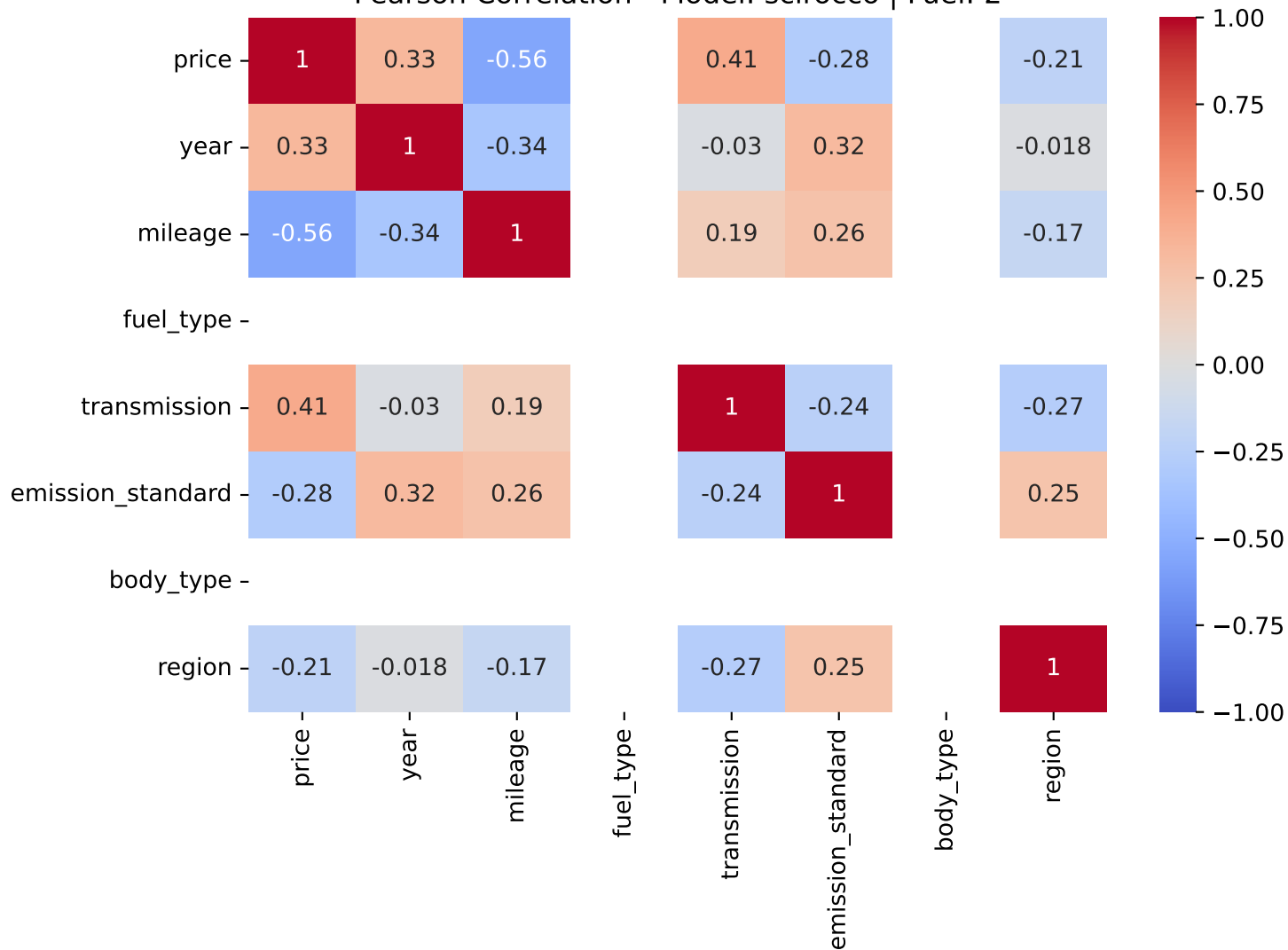
Pearson Correlation - Model: scirocco | Fuel: 2
