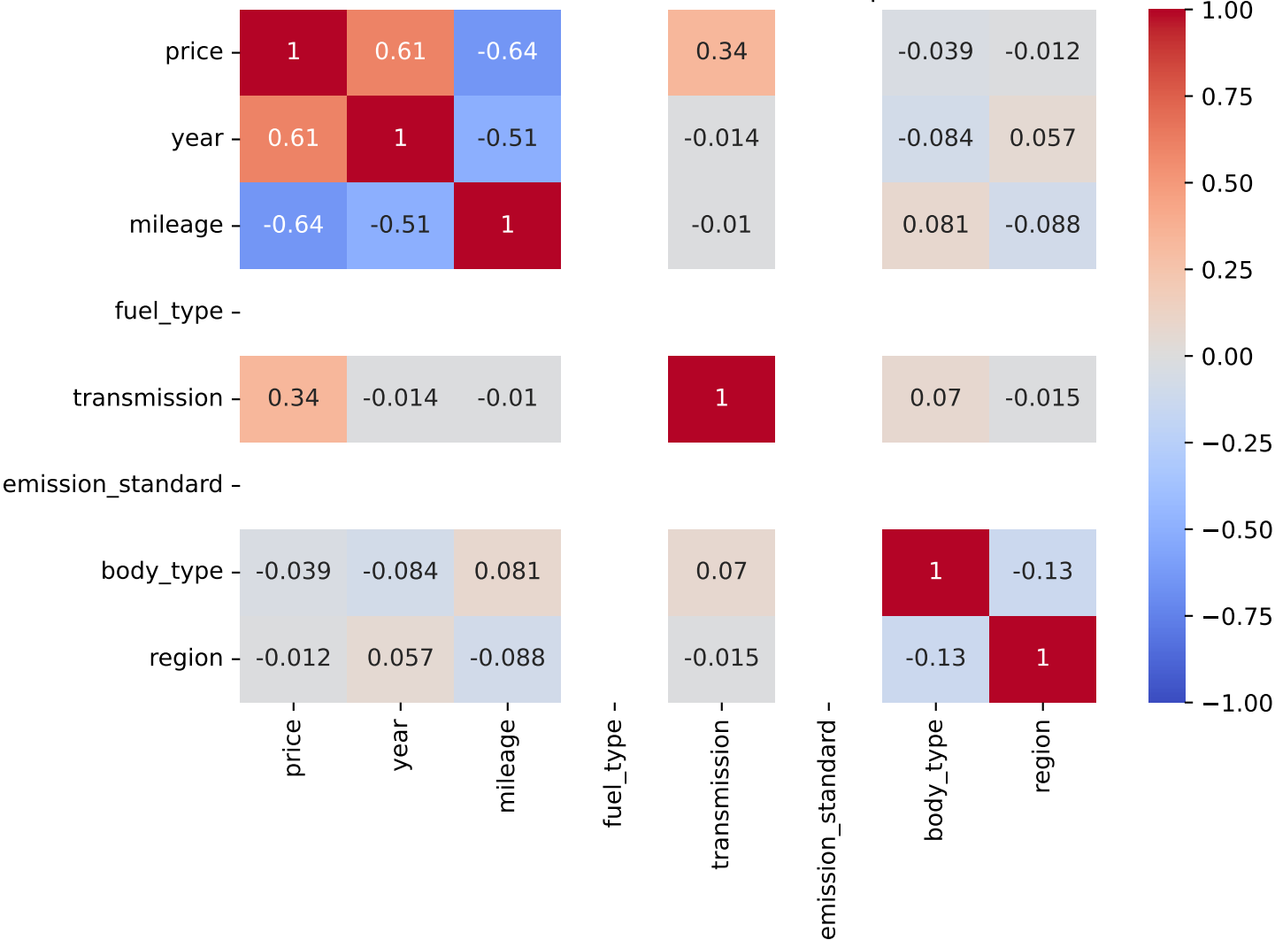
Pearson Correlation - Model: t-cross | Fuel: 2
