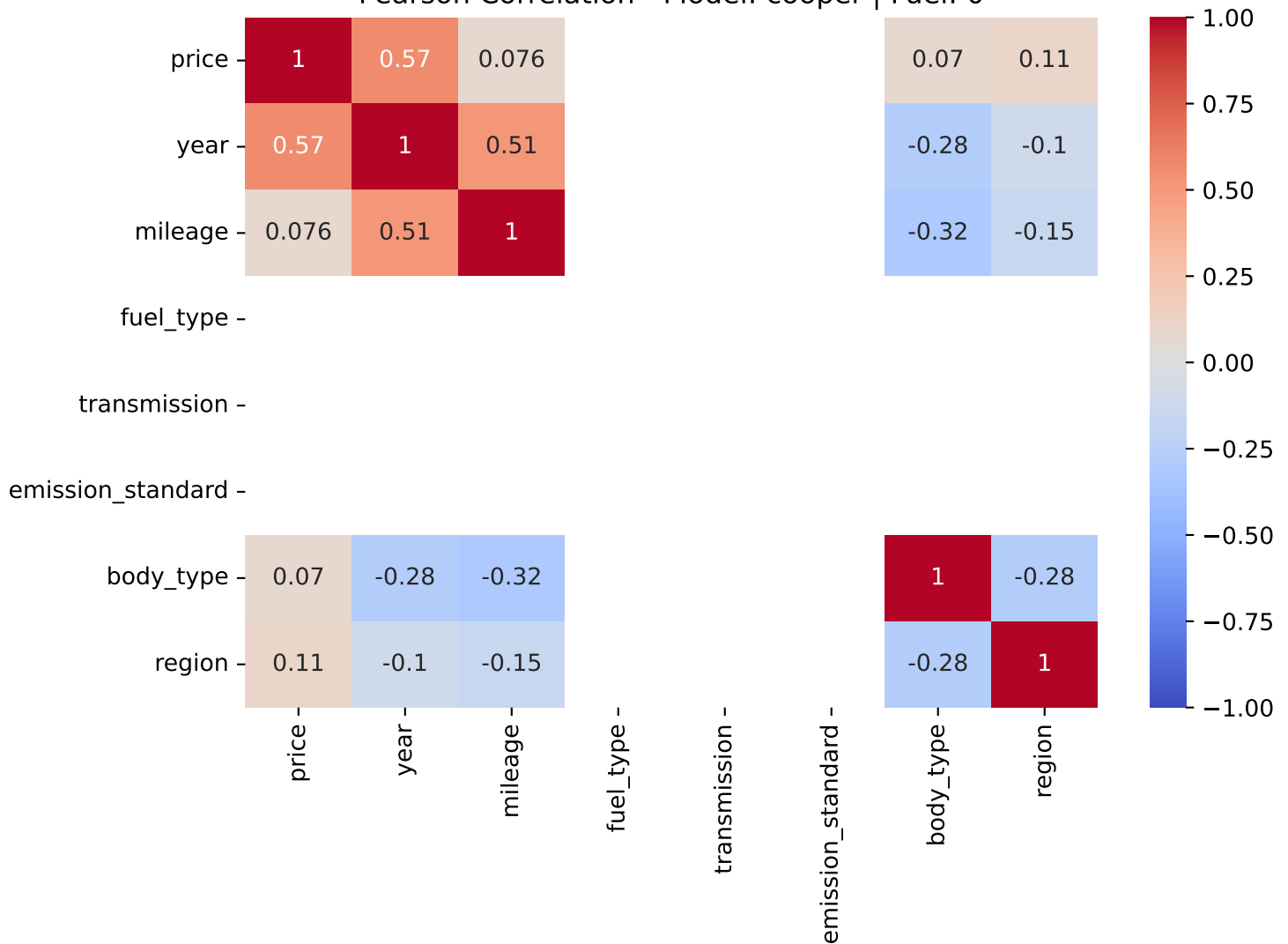
Pearson Correlation - Model: cooper | Fuel: 0
