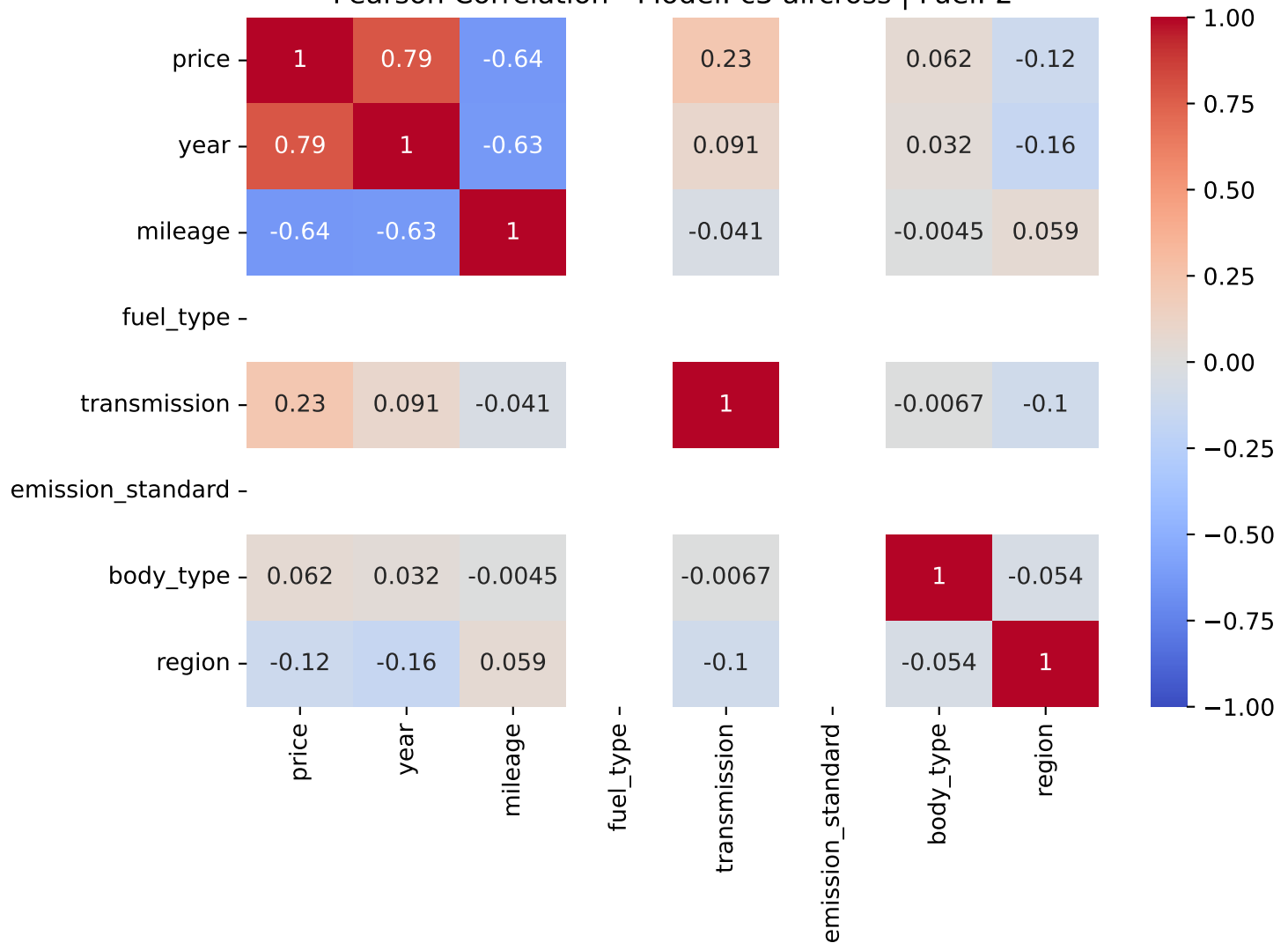
Pearson Correlation - Model: c3 aircross | Fuel: 2
