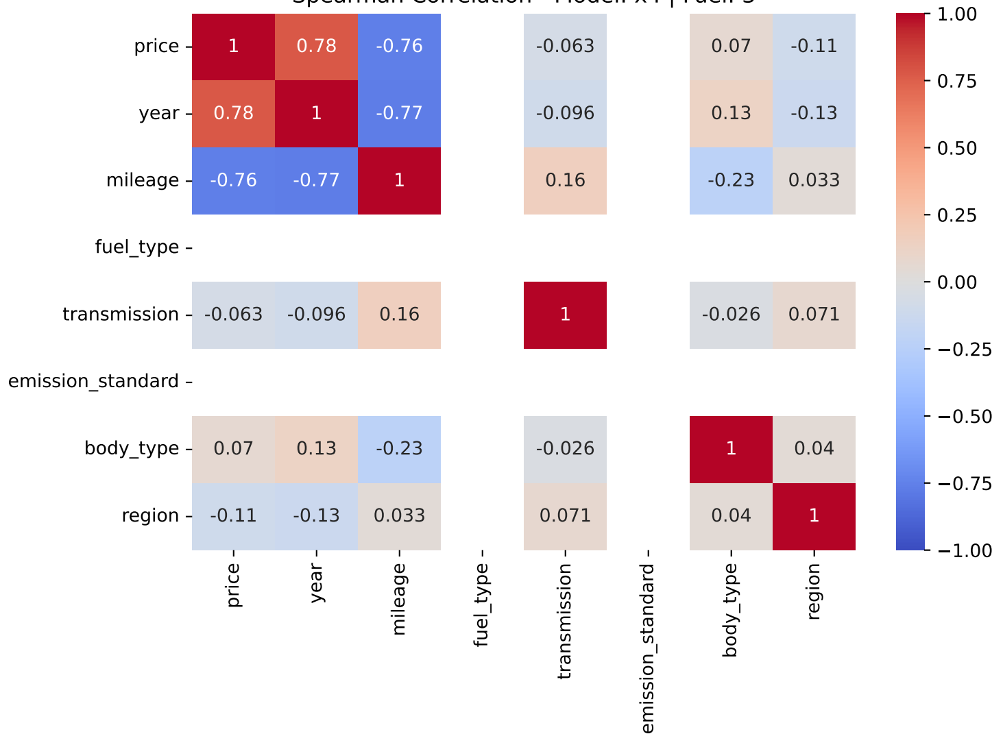
Spearman Correlation - Model: x4 | Fuel: 3
