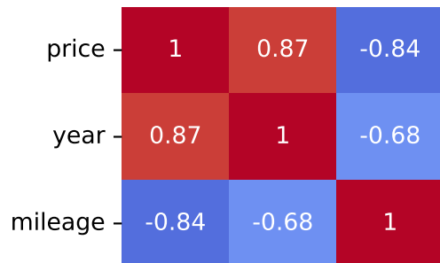
Spearman Correlation - Model: golf | Fuel: 5
