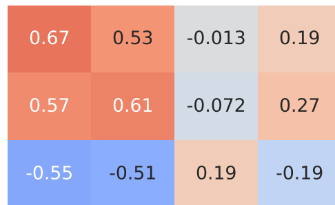
Spearman Correlation - Model: 308 | Fuel: 2
