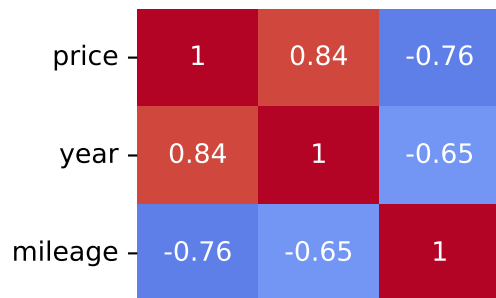
Spearman Correlation - Model: tiguan | Fuel: 1
