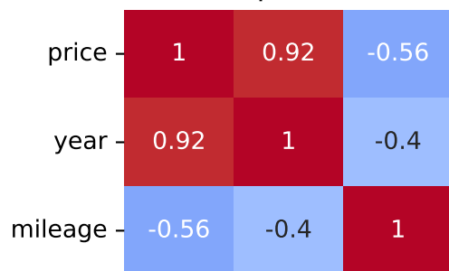
Spearman Correlation - Model: auris | Fuel: 1
