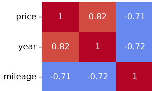
Pearson Correlation - Model: yaris | Fuel: 3
