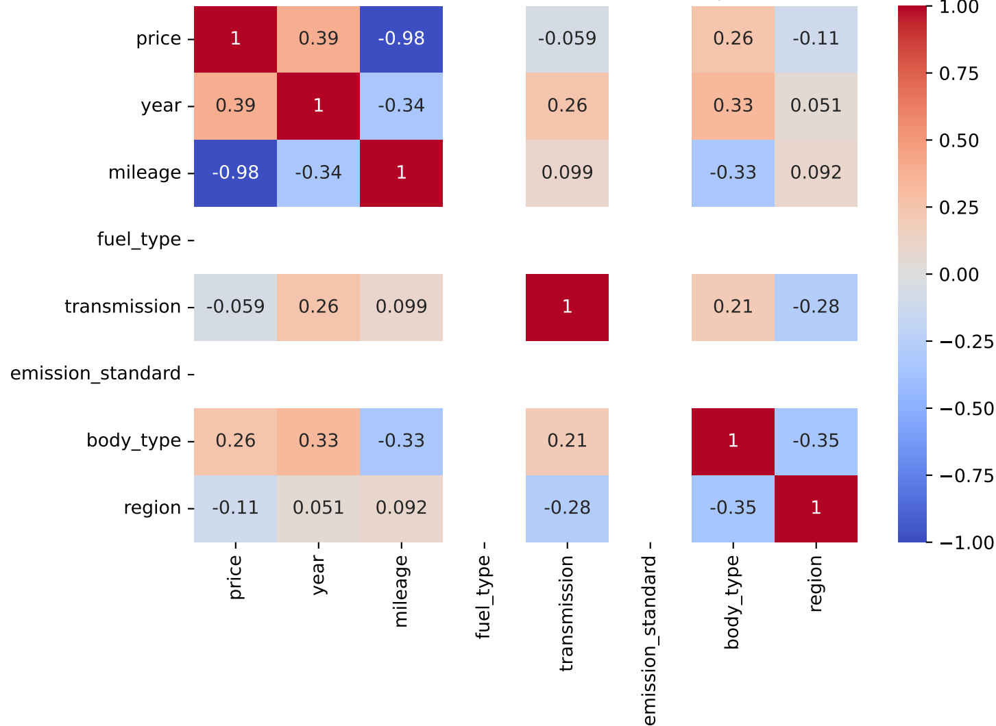
Spearman Correlation - Model: c5 aircross | Fuel: 2
