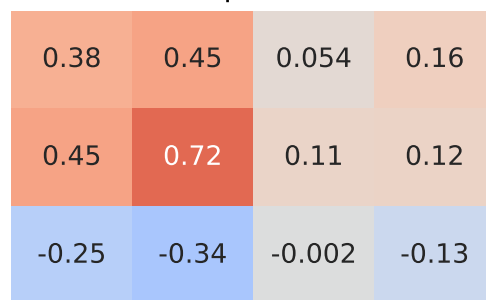
Pearson Correlation - Model: xc60 | Fuel: 1
