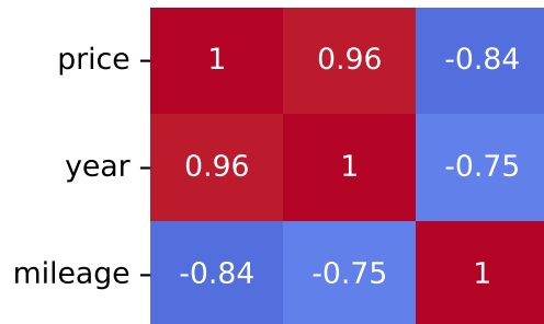
Spearman Correlation - Model: picanto | Fuel: 4
