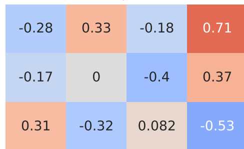
Spearman Correlation - Model: rifter | Fuel: 1
