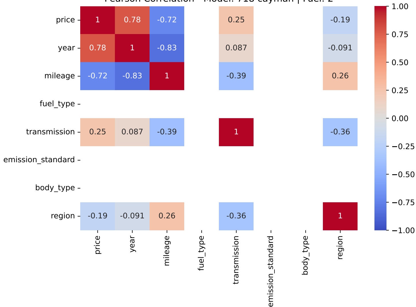
Pearson Correlation - Model: 718 cayman | Fuel: 2
