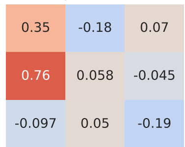
Spearman Correlation - Model: sedici | Fuel: 1
