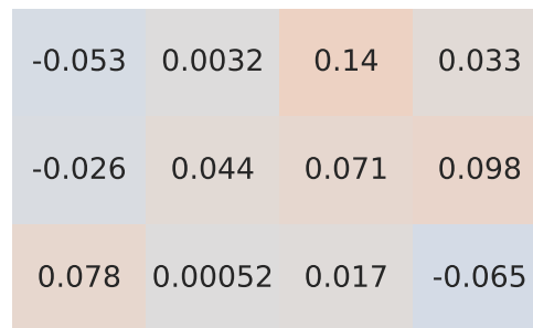
Pearson Correlation - Model: 500 | Fuel: 3
