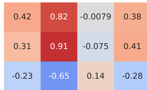
Pearson Correlation - Model: one | Fuel: 2
