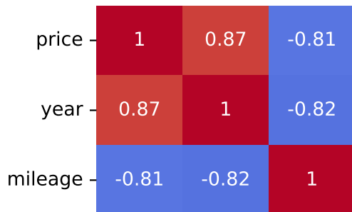
Spearman Correlation - Model: 208 | Fuel: 2
