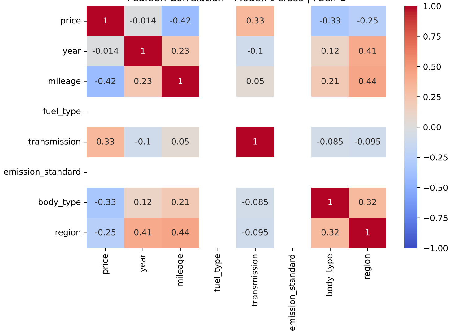
Pearson Correlation - Model: t-cross | Fuel: 1
