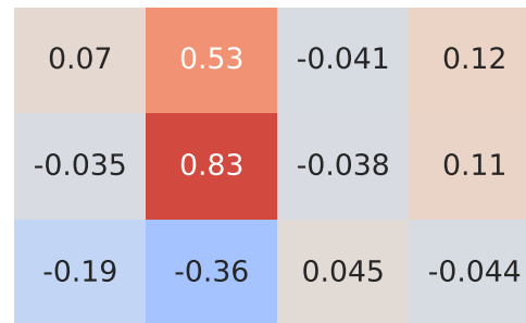
Spearman Correlation - Model: romeo giulietta | Fuel: 4
