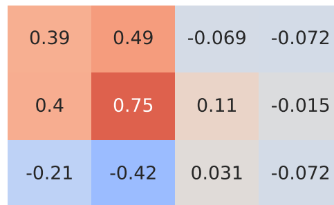
Pearson Correlation - Model: 308 | Fuel: 1
