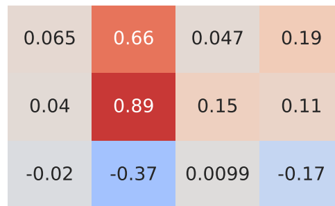
Pearson Correlation - Model: fiesta | Fuel: 2
