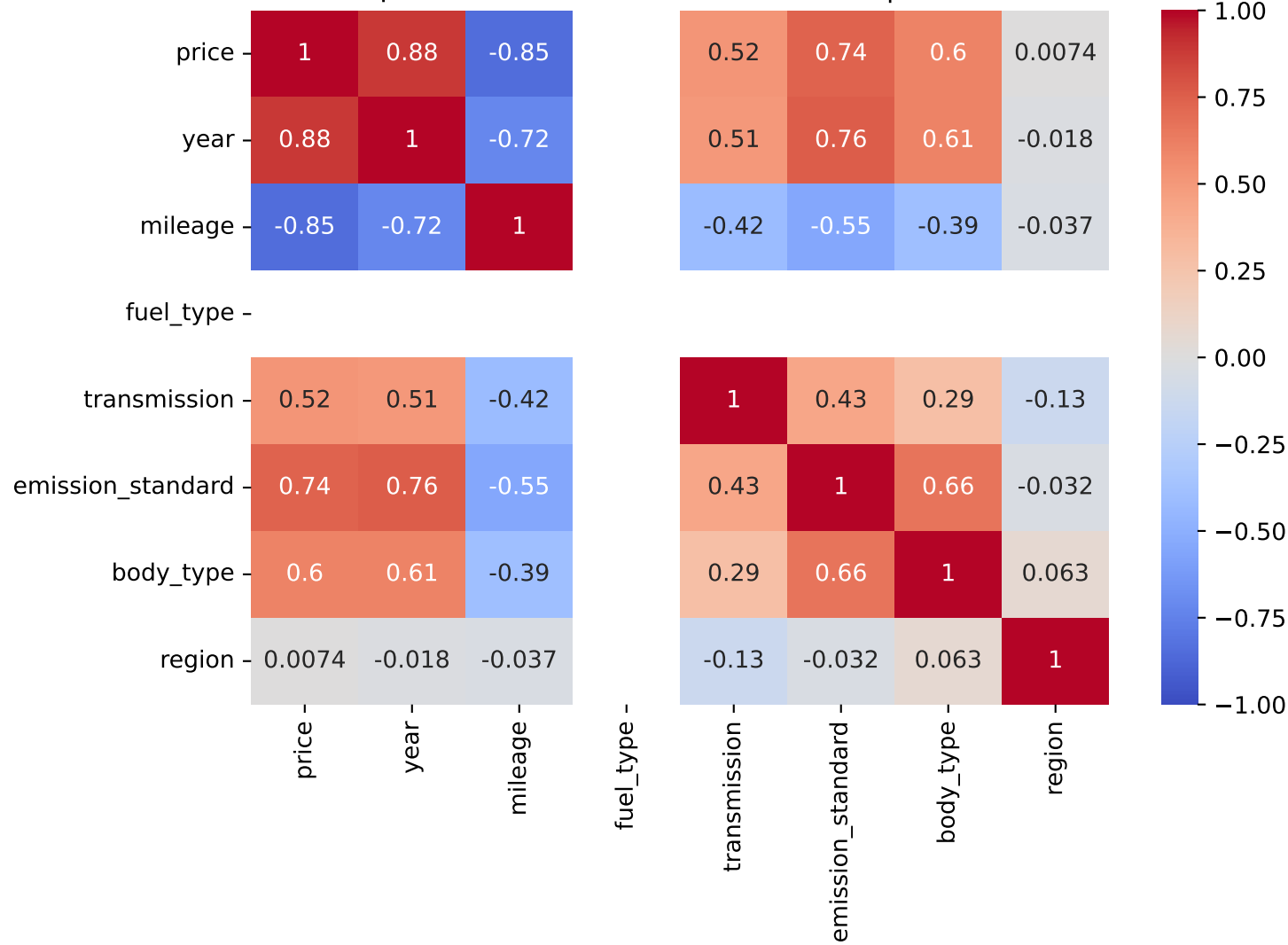
Spearman Correlation - Model: 5008 | Fuel: 1
