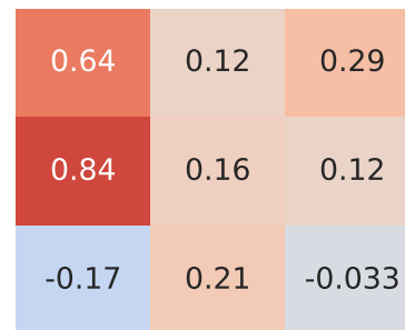
Spearman Correlation - Model: punto | Fuel: 5
