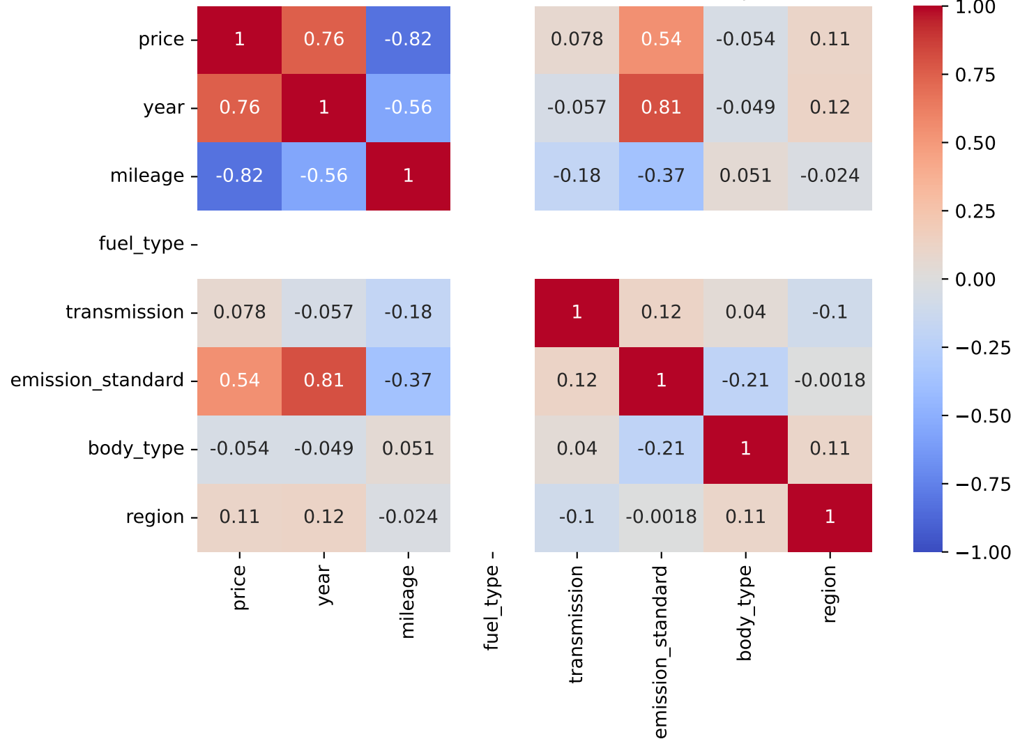
Pearson Correlation - Model: romeo giulietta | Fuel: 4
