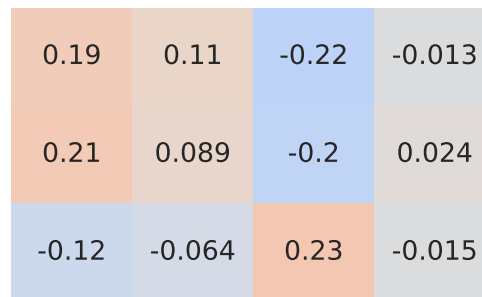
Pearson Correlation - Model: x4 | Fuel: 1
