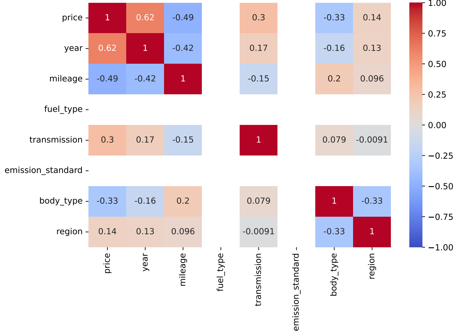
Spearman Correlation - Model: fiesta | Fuel: 3
