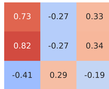
Spearman Correlation - Model: rio | Fuel: 4
