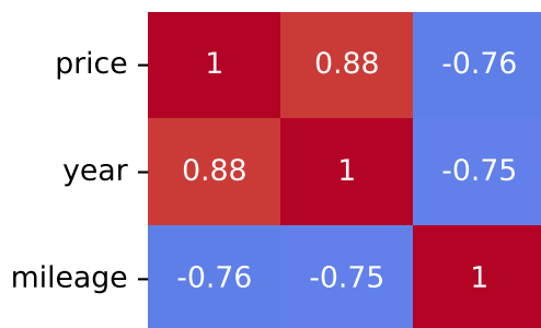
Pearson Correlation - Model: tiguau | Fuel: 2
