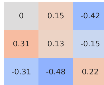
Spearman Correlation - Model: celerio | Fuel: 2
