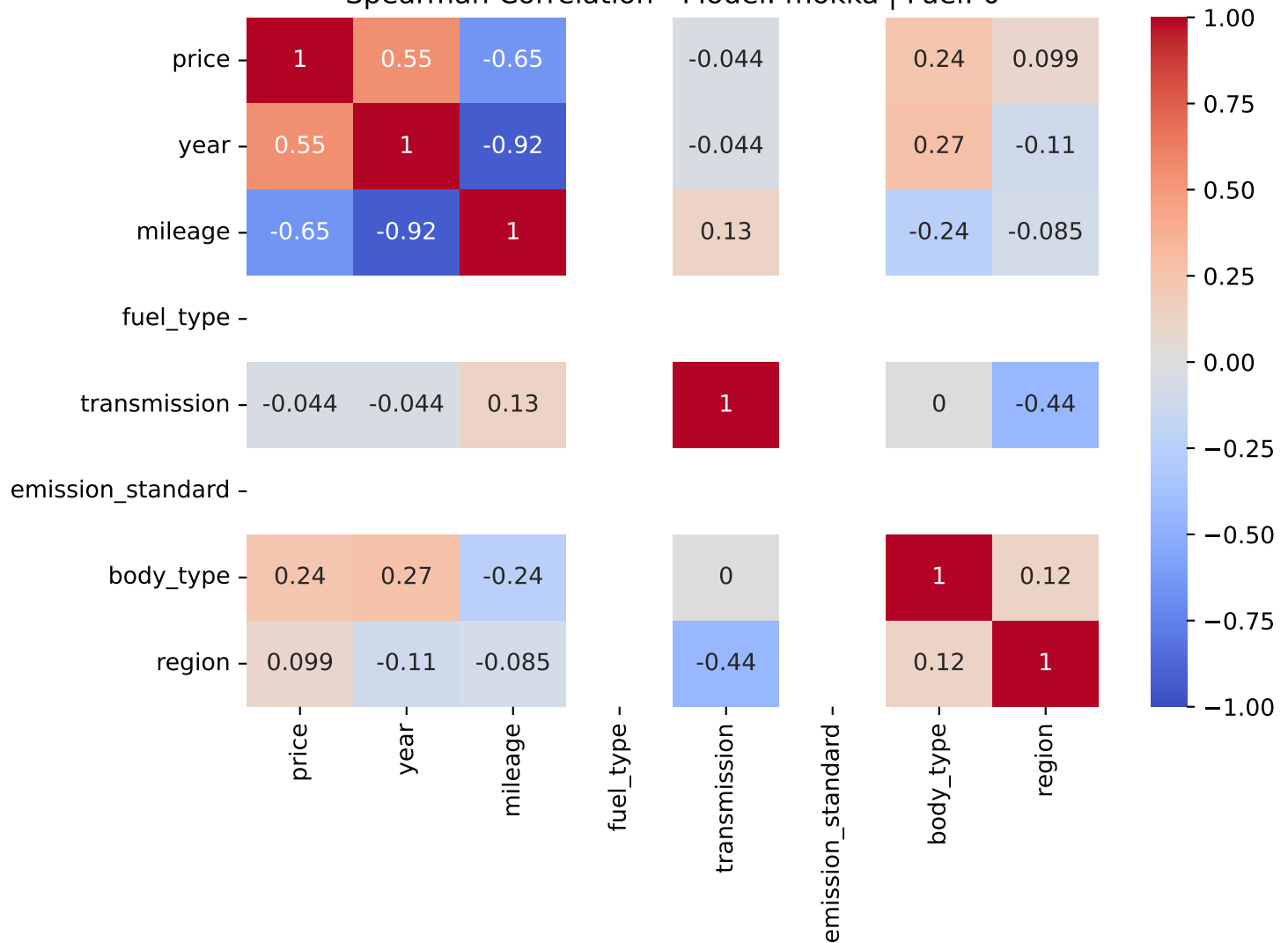
Spearman Correlation - Model: mokka | Fuel: 0
