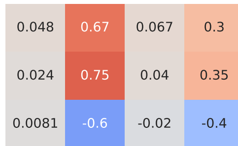
Spearman Correlation - Model: sportage | Fuel: 2
