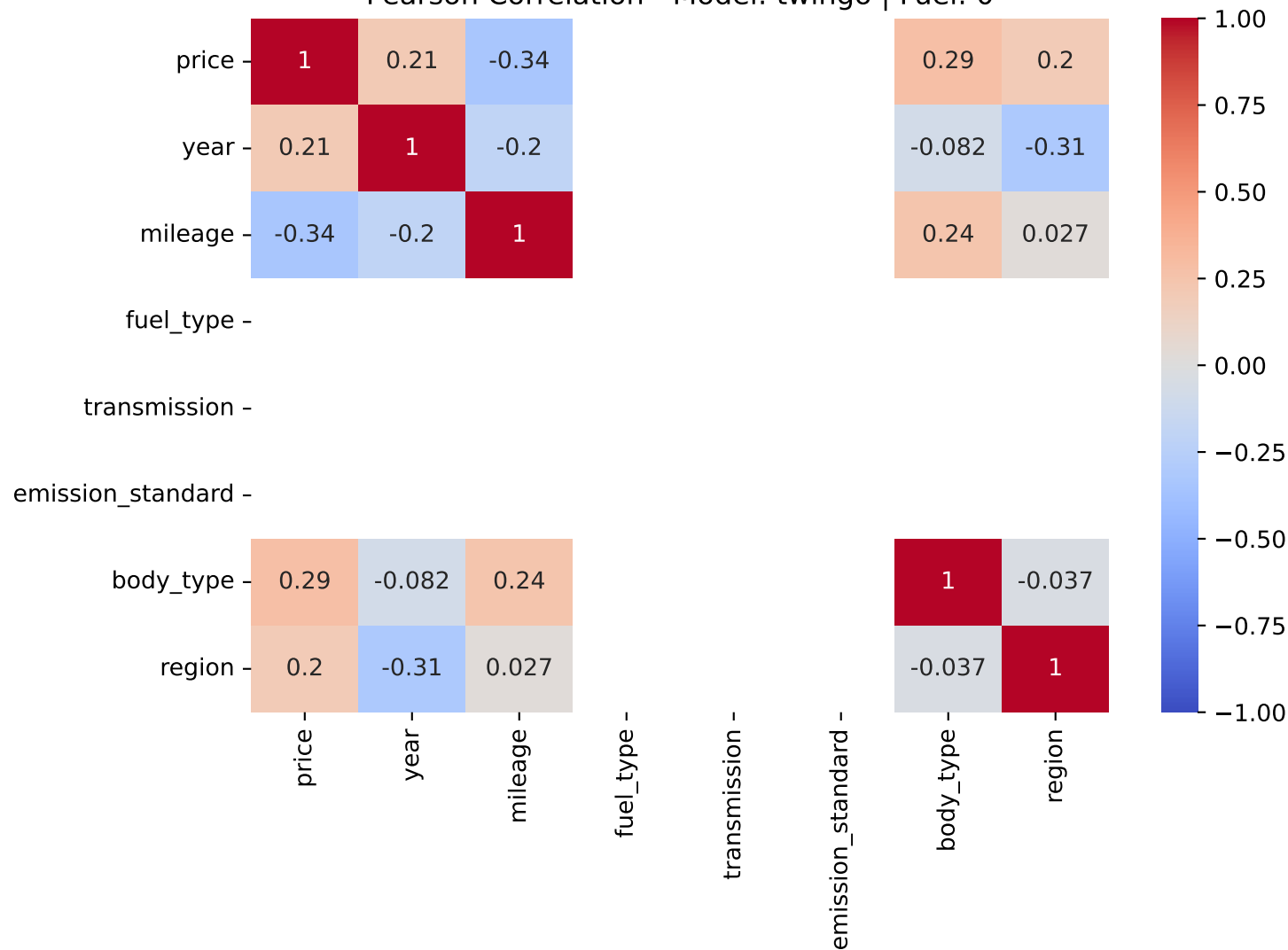
Pearson Correlation - Model: twingo | Fuel: 0
