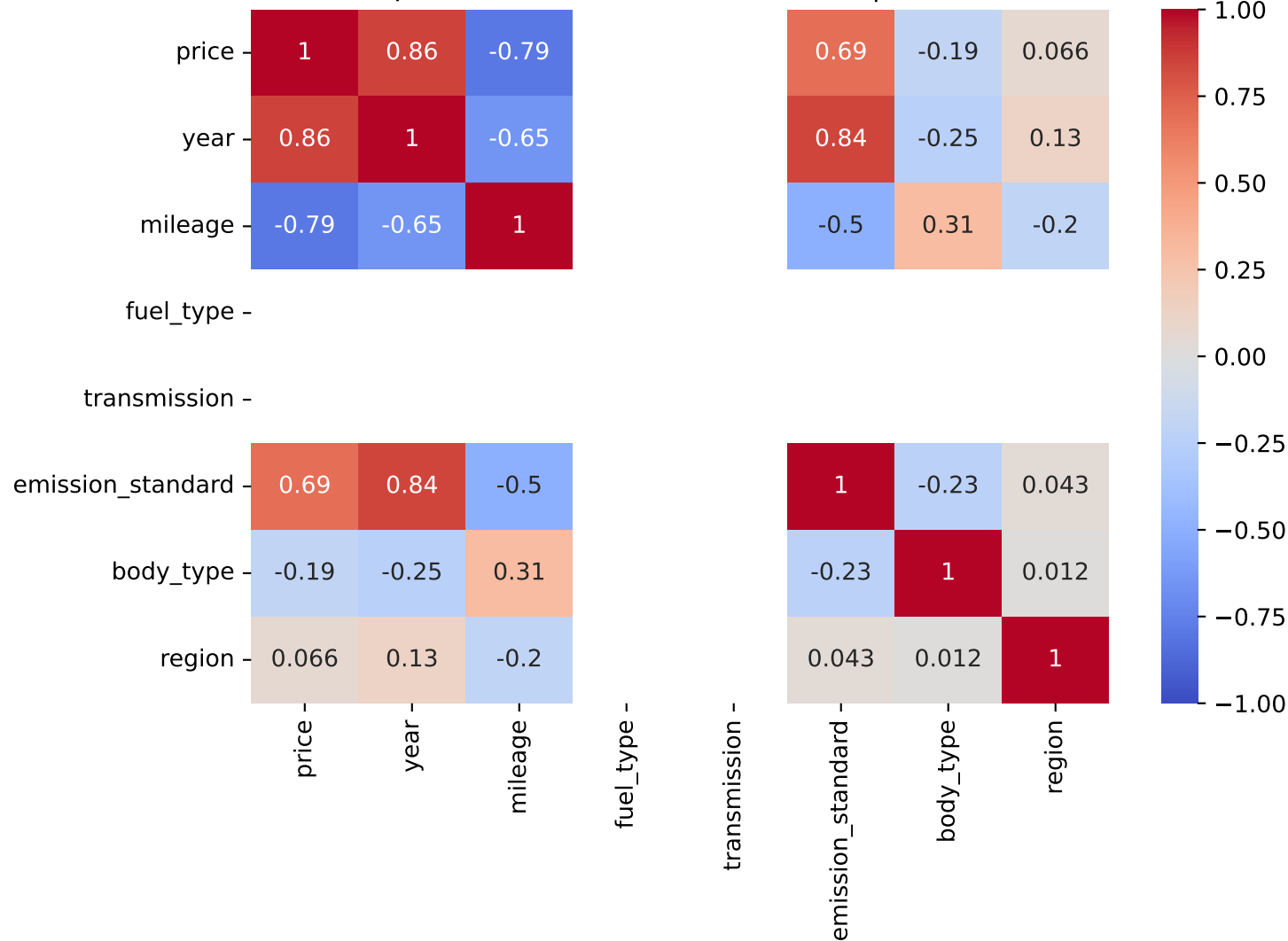
Spearman Correlation - Model: i10 | Fuel: 4
