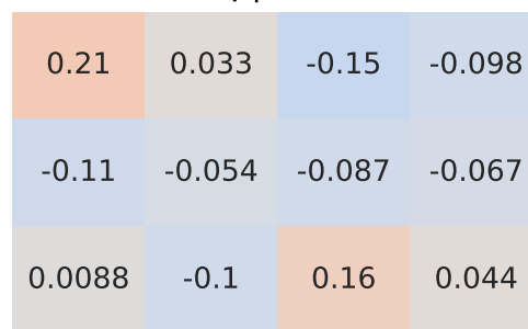
Pearson Correlation - Model: karoq | Fuel: 1
