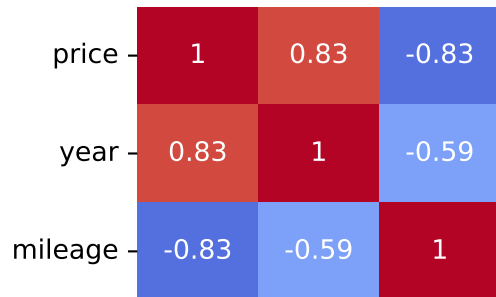
Pearson Correlation - Model: i20 | Fuel: 4
