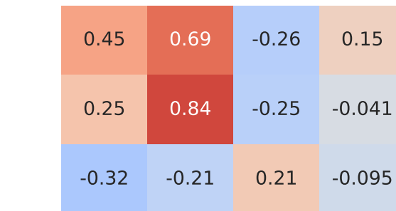
Pearson Correlation - Model: grand scenic | Fuel: 1
