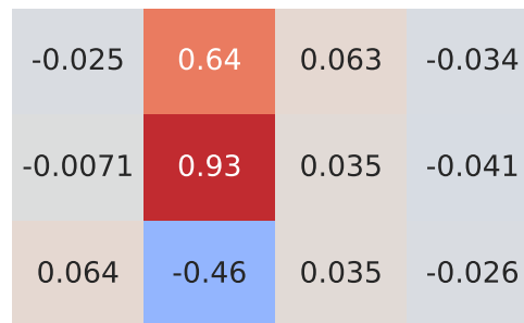
Spearman Correlation - Model: panda | Fuel: 1
