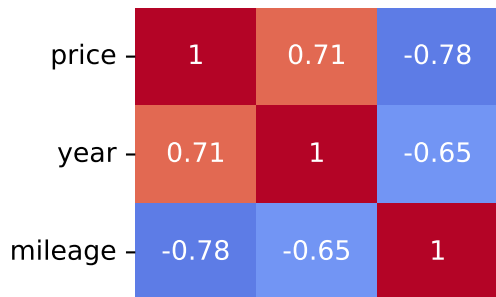
Spearman Correlation - Model: qubo | Fuel: 2
