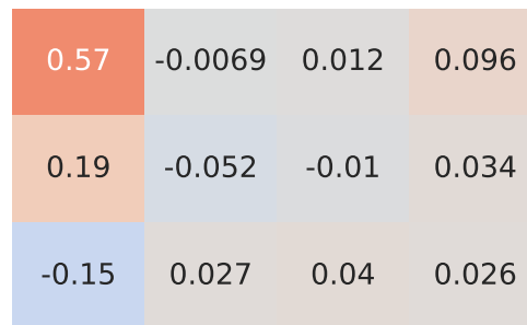
Pearson Correlation - Model: ypsilon | Fuel: 3
