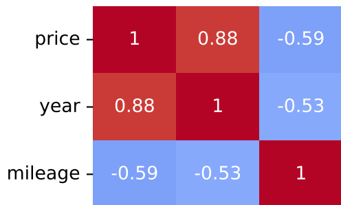
Spearman Correlation - Model: ypsilon | Fuel: 1
