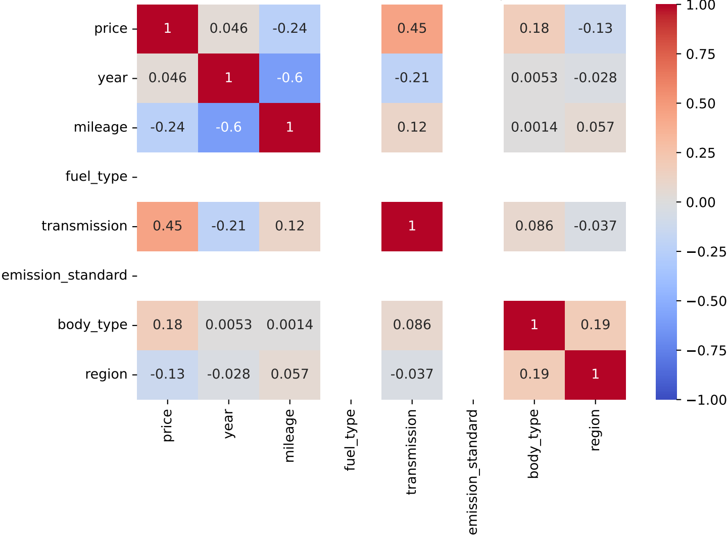
Spearman Correlation - Model: taigo | Fuel: 2
