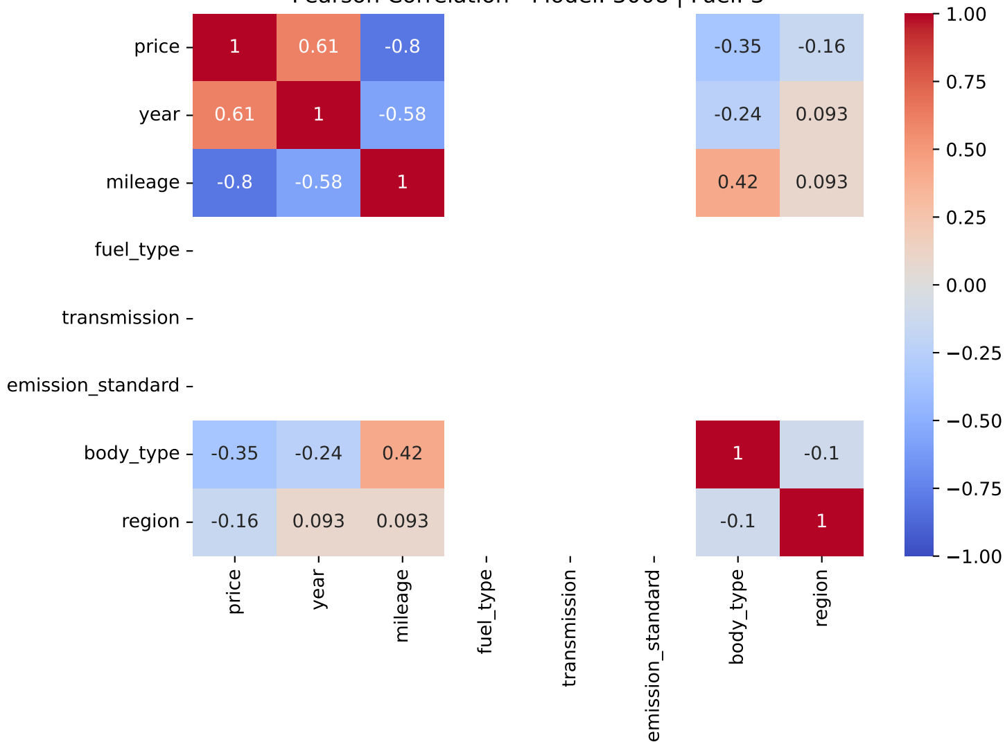
Pearson Correlation - Model: 3008 | Fuel: 3
