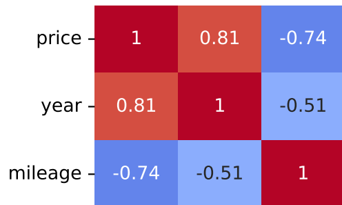
Spearman Correlation - Model: berlingo | Fuel: 1
