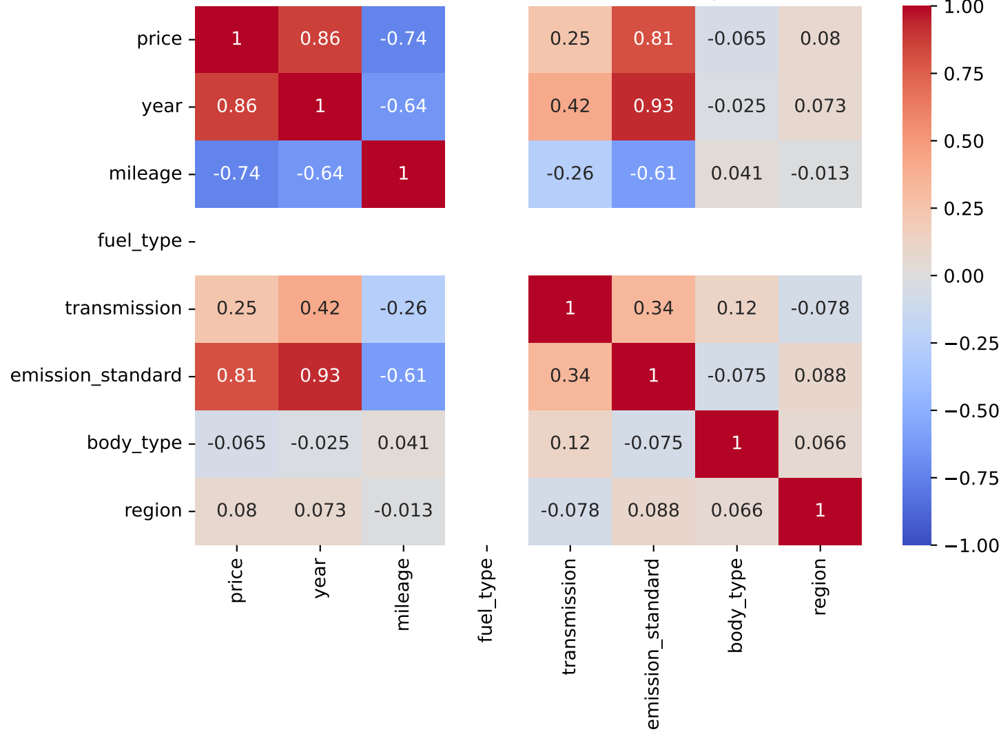
Spearman Correlation - Model: cherokee | Fuel: 1
