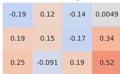
Spearman Correlation - Model: romeo tonale | Fuel: 3
