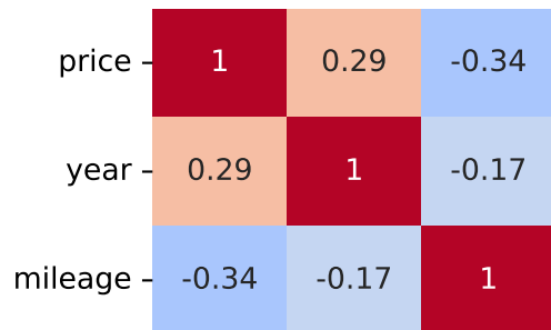
Pearson Correlation - Model: grand vitara | Fuel: 1
