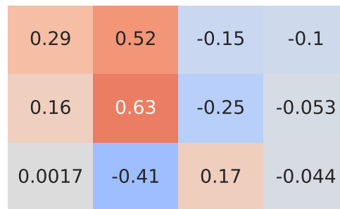
Pearson Correlation - Model: 3008 | Fuel: 2
