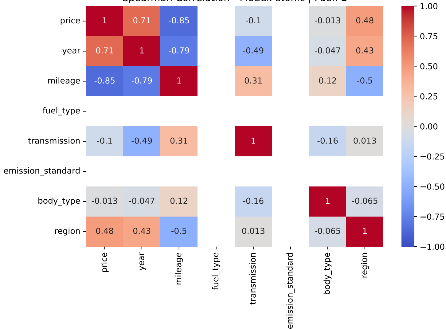
Spearman Correlation - Model: stonic | Fuel: 2
