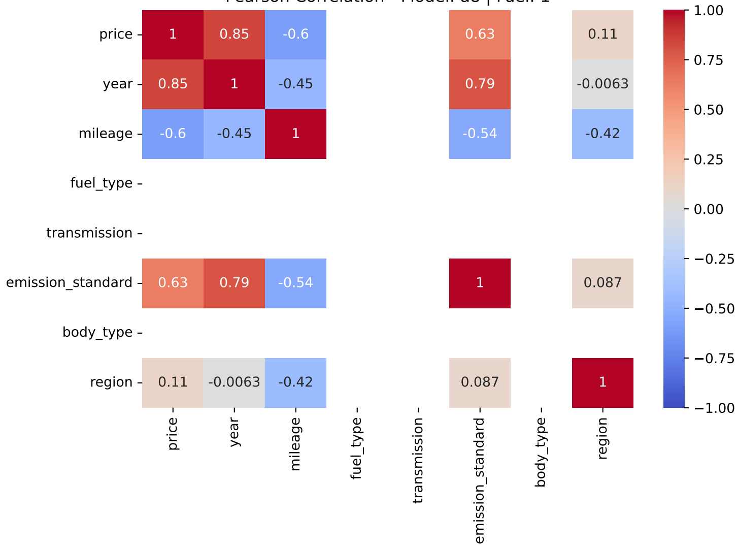
Pearson Correlation - Model: a8 | Fuel: 1
