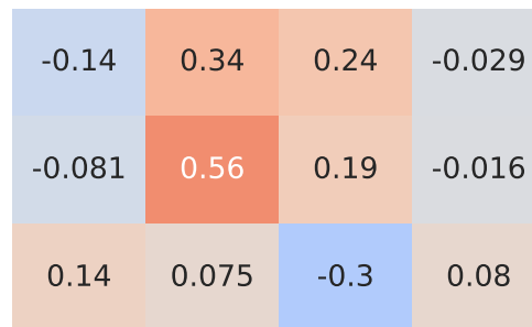
Pearson Correlation - Model: rs3 | Fuel: 2
