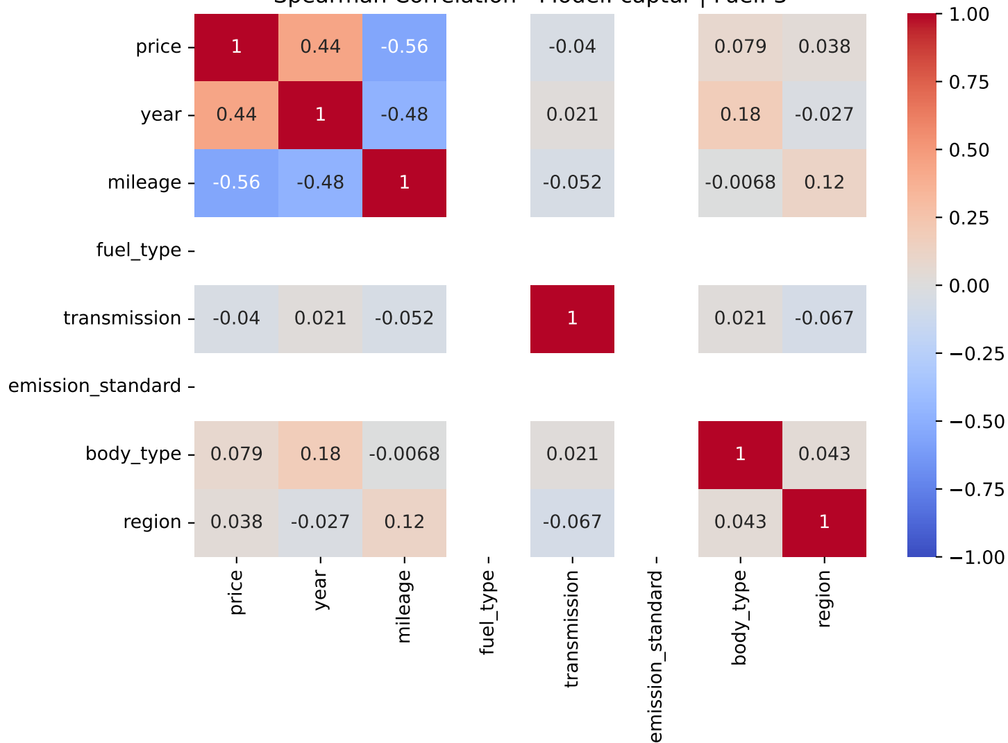
Spearman Correlation - Model: captur | Fuel: 3
