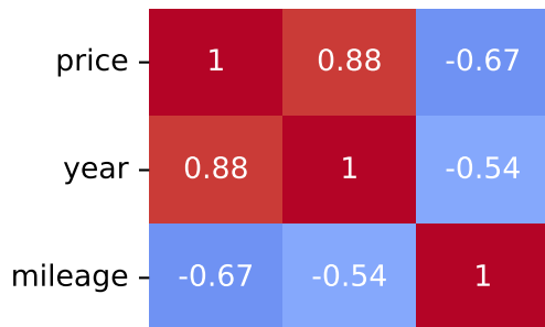
Pearson Correlation - Model: scenic | Fuel: 1
