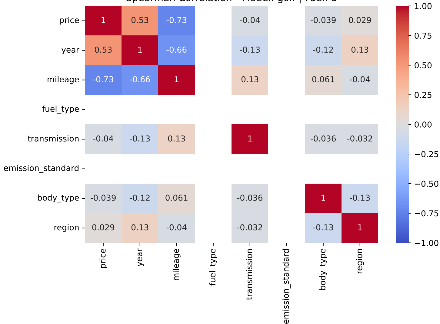
Spearman Correlation - Model: golf | Fuel: 3
