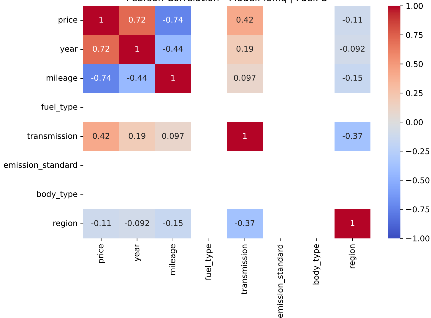
Pearson Correlation - Model: ioniq | Fuel: 3
