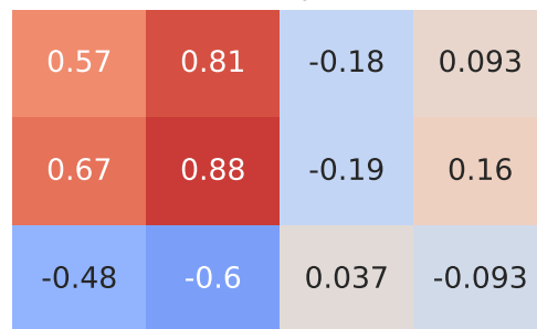
Spearman Correlation - Model: cooper s | Fuel: 2
