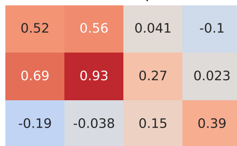
Spearman Correlation - Model: land cruiser | Fuel: 1
