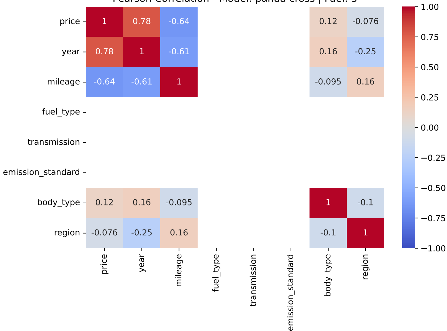
Pearson Correlation - Model: panda cross | Fuel: 3
