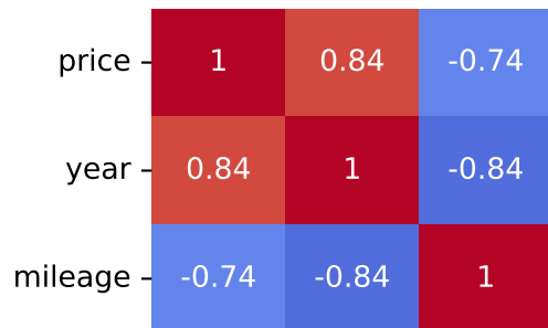
Spearman Correlation - Model: a3 | Fuel: 2
