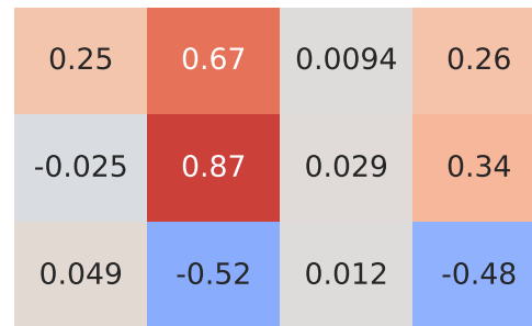
Pearson Correlation - Model: sportage | Fuel: 2
