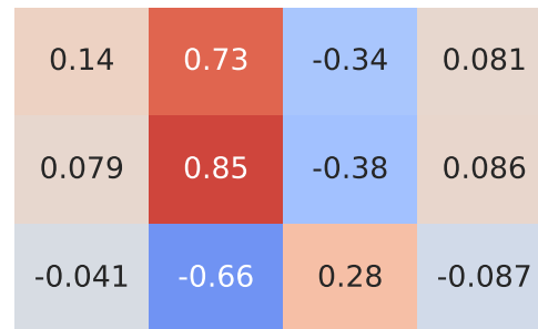
Pearson Correlation - Model: fabia | Fuel: 2
