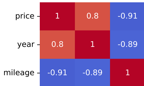
Spearman Correlation - Model: octavia | Fuel: 2
