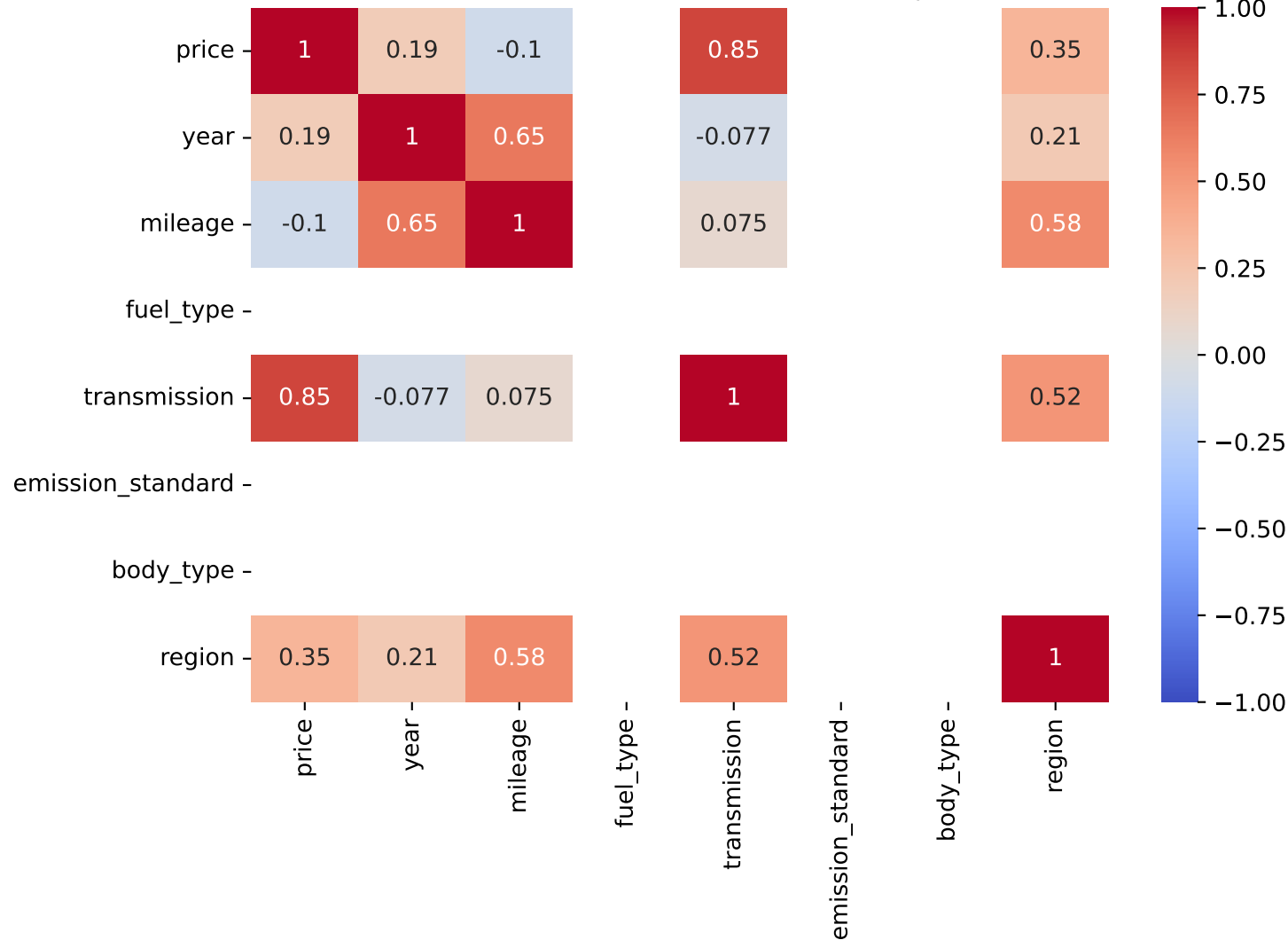
Pearson Correlation - Model: a1 allstreet | Fuel: 2
