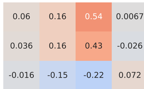
Spearman Correlation - Model: yaris | Fuel: 3
