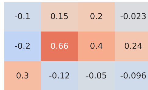
Spearman Correlation - Model: idea | Fuel: 4
