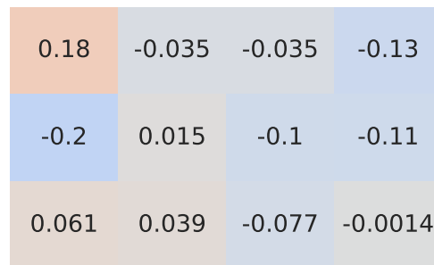
Spearman Correlation - Model: xc40 | Fuel: 2
