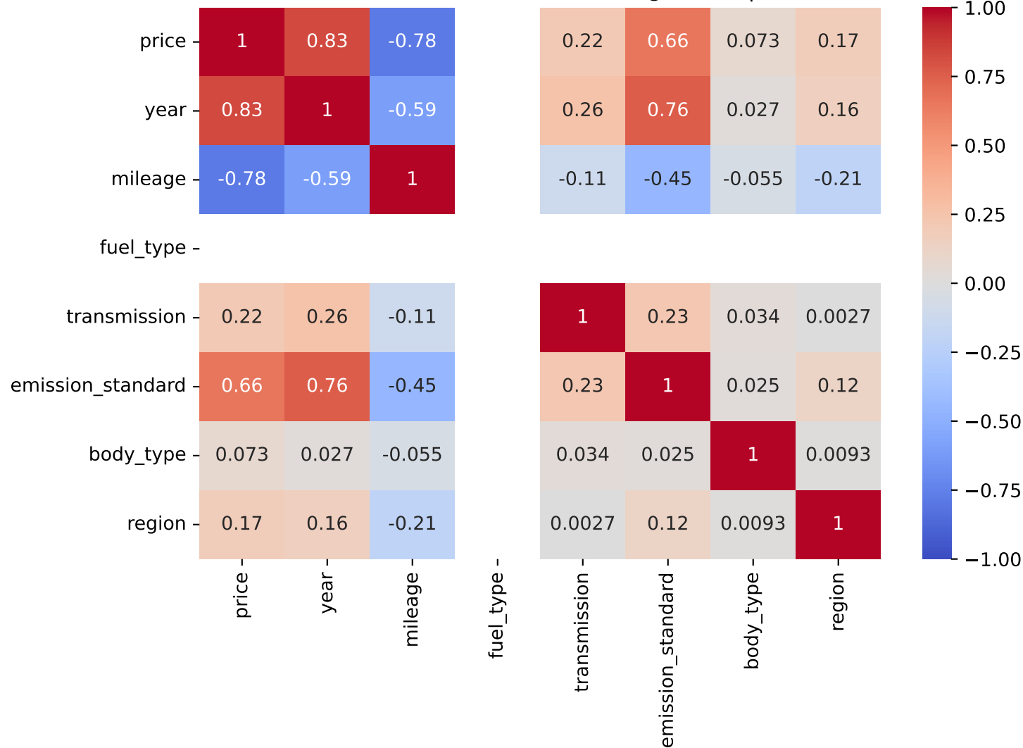
Pearson Correlation - Model: romeo giulietta | Fuel: 1
