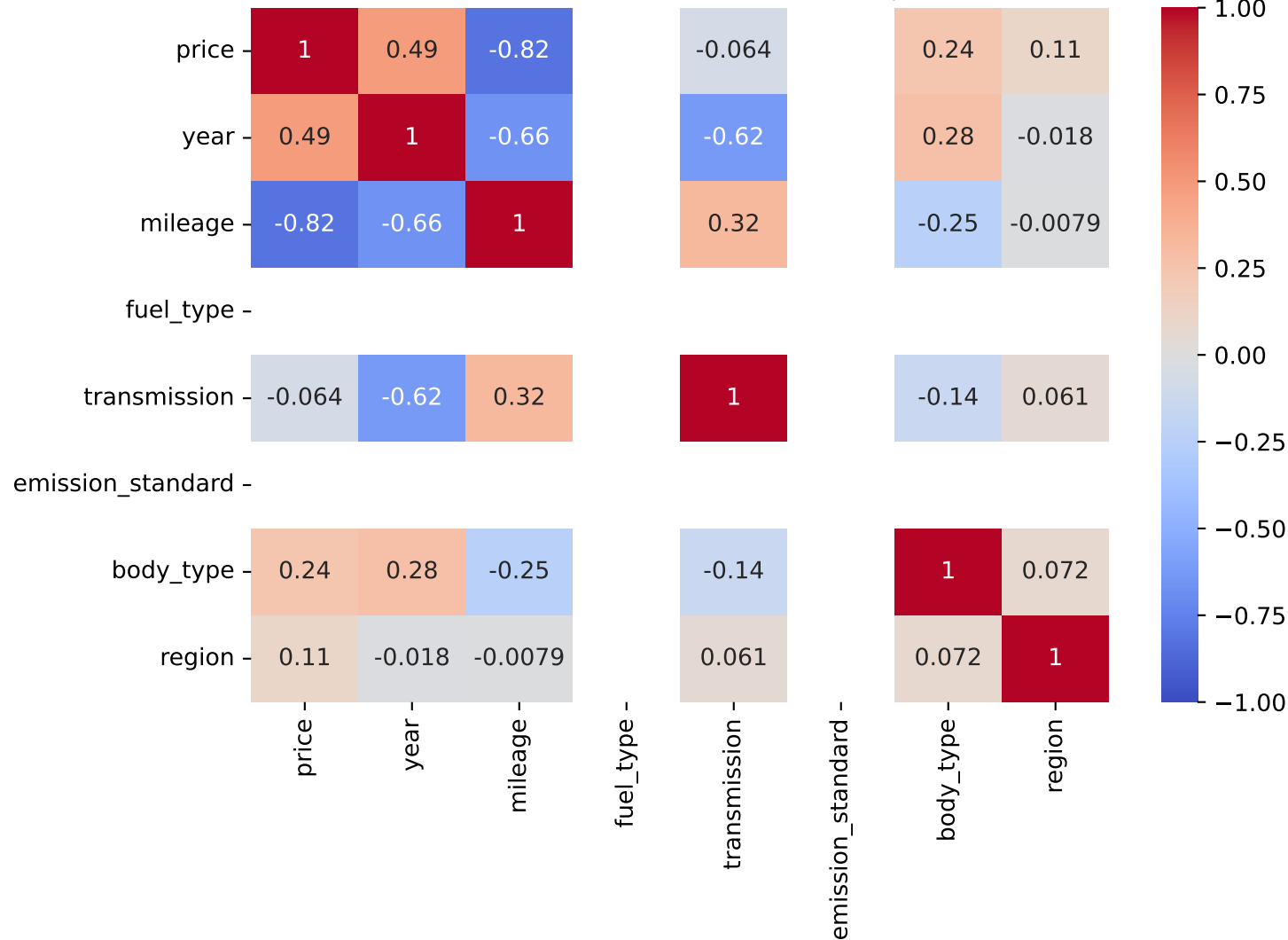
Spearman Correlation - Model: karoq | Fuel: 2
