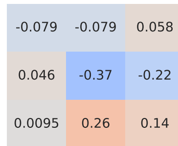
Pearson Correlation - Model: panda cross | Fuel: 2
