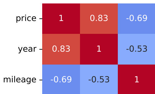
Pearson Correlation - Model: tt | Fuel: 2
