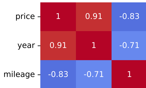
Spearman Correlation - Model: x3 | Fuel: 1
