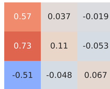
Pearson Correlation - Model: panda | Fuel: 4
