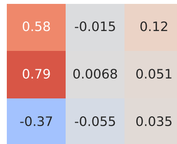
Pearson Correlation - Model: ix20 | Fuel: 4
