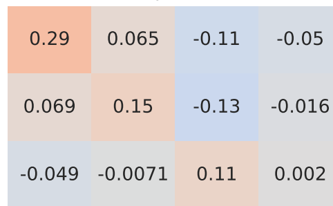
Spearman Correlation - Model: q3 | Fuel: 2
