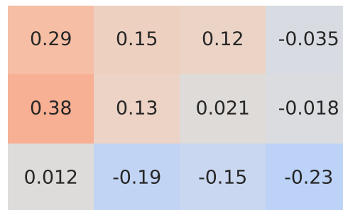
Spearman Correlation - Model: crossland x | Fuel: 1
