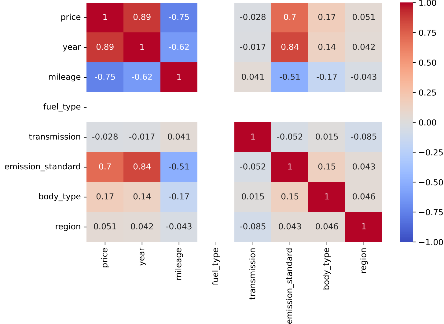
Pearson Correlation - Model: corsa | Fuel: 1
