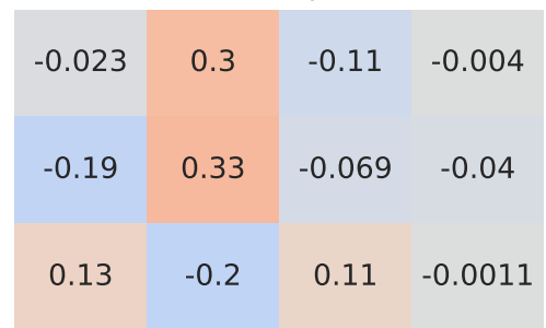
Spearman Correlation - Model: renegade | Fuel: 1
