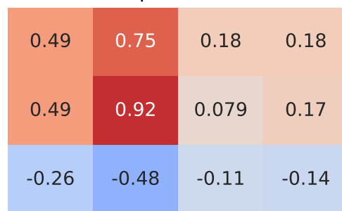
Pearson Correlation - Model: tt | Fuel: 2
