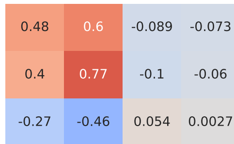
Pearson Correlation - Model: tiguan | Fuel: 1
