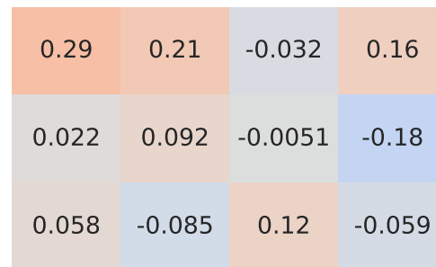
Pearson Correlation - Model: ix35 | Fuel: 1
