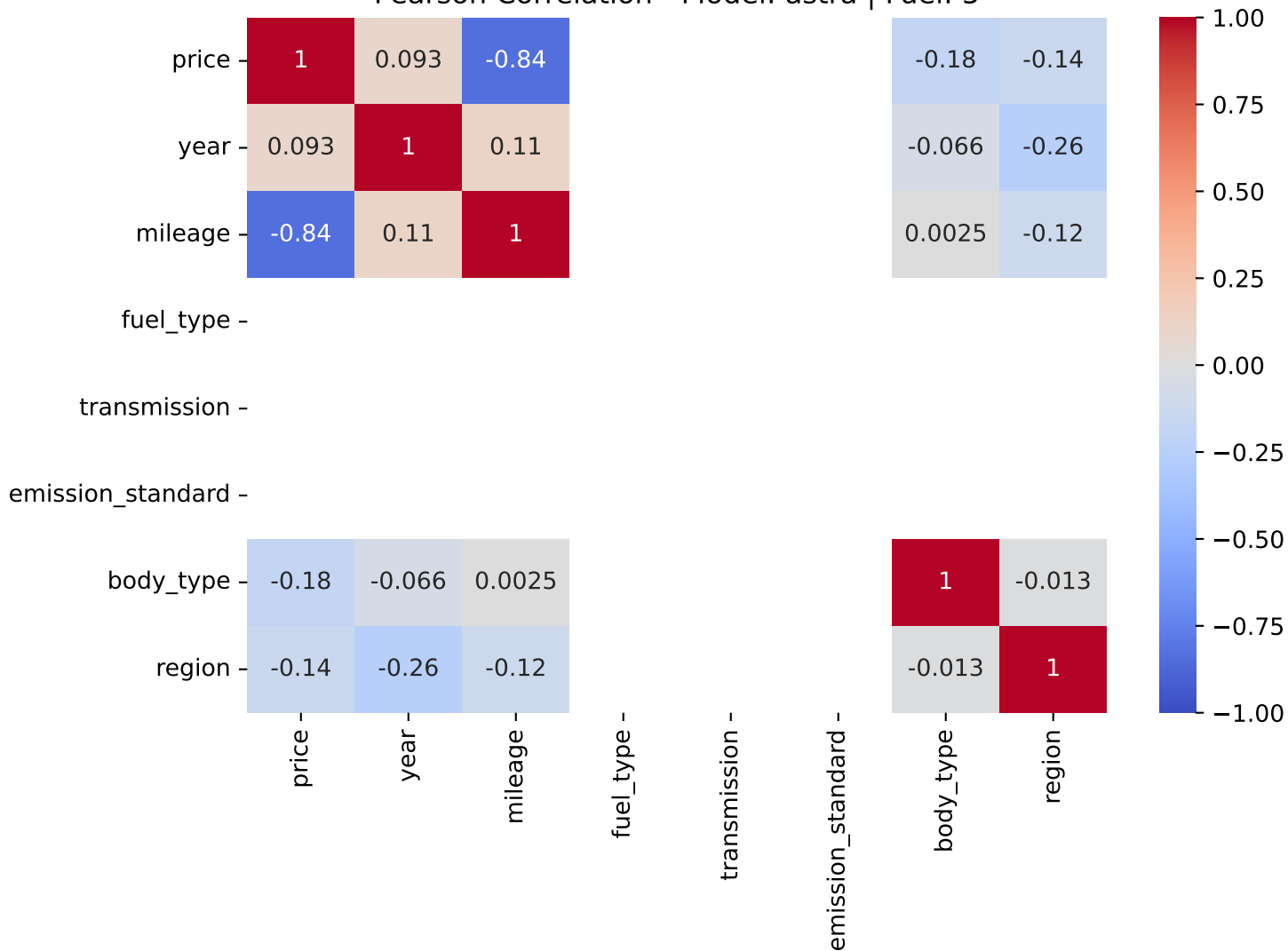
Pearson Correlation - Model: astra | Fuel: 5
