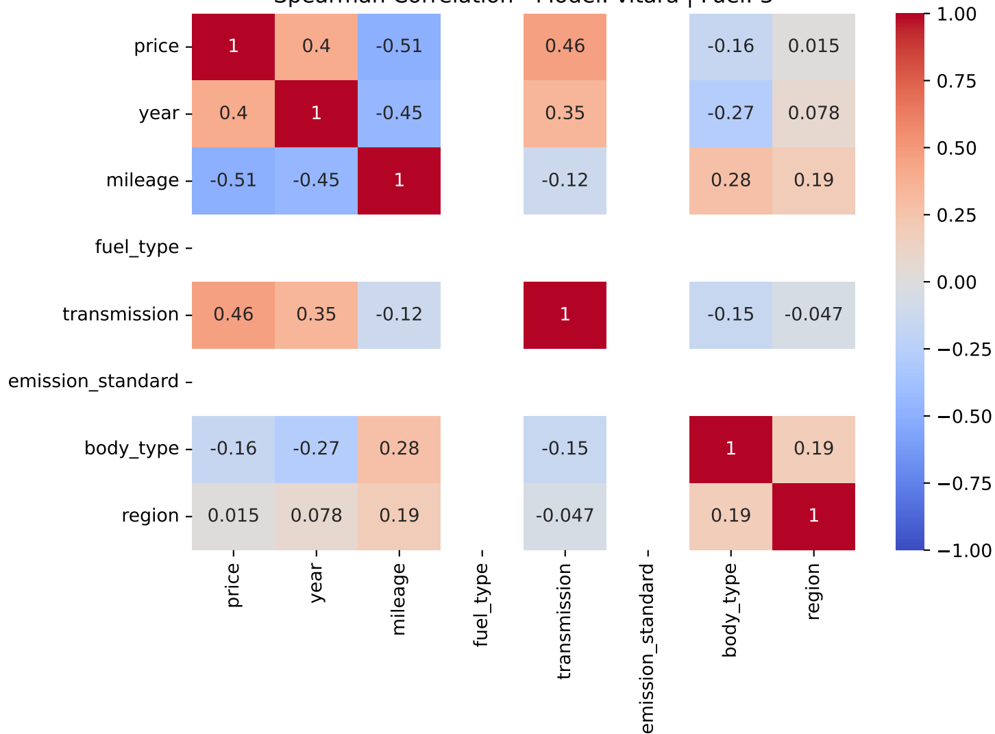
Spearman Correlation - Model: vitara | Fuel: 3
