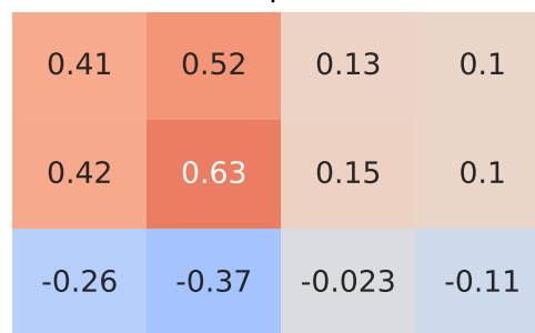
Spearman Correlation - Model: xc60 | Fuel: 1
