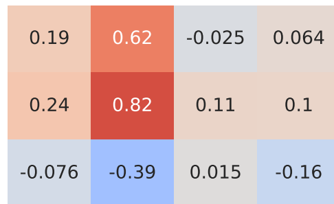
Pearson Correlation - Model: x6 | Fuel: 1
