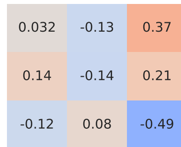
Pearson Correlation - Model: 500I | Fuel: 4
