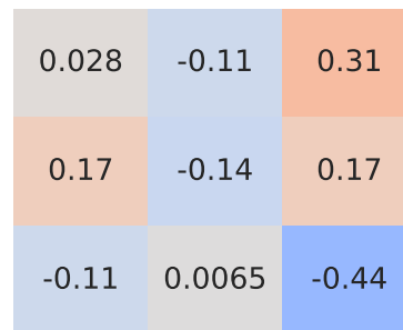
Spearman Correlation - Model: 500I | Fuel: 4
