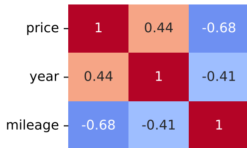
Pearson Correlation - Model: tipo | Fuel: 2
