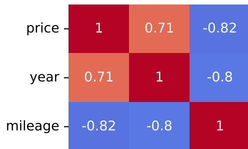
Pearson Correlation - Model: bayon | Fuel: 2
