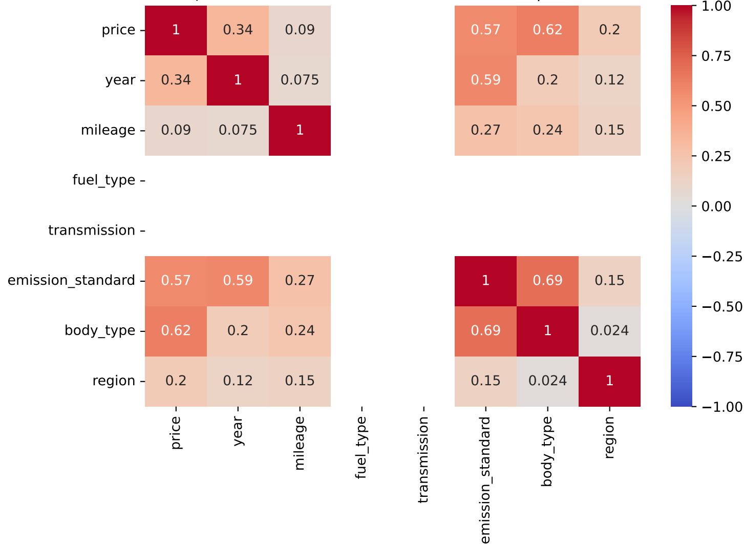
Spearman Correlation - Model: new beetle | Fuel: 1
