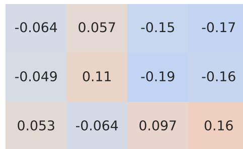
Pearson Correlation - Model: c3 aircross | Fuel: 1
