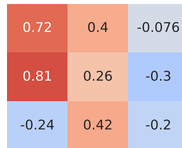
Pearson Correlation - Model: astra gtc | Fuel: 1
