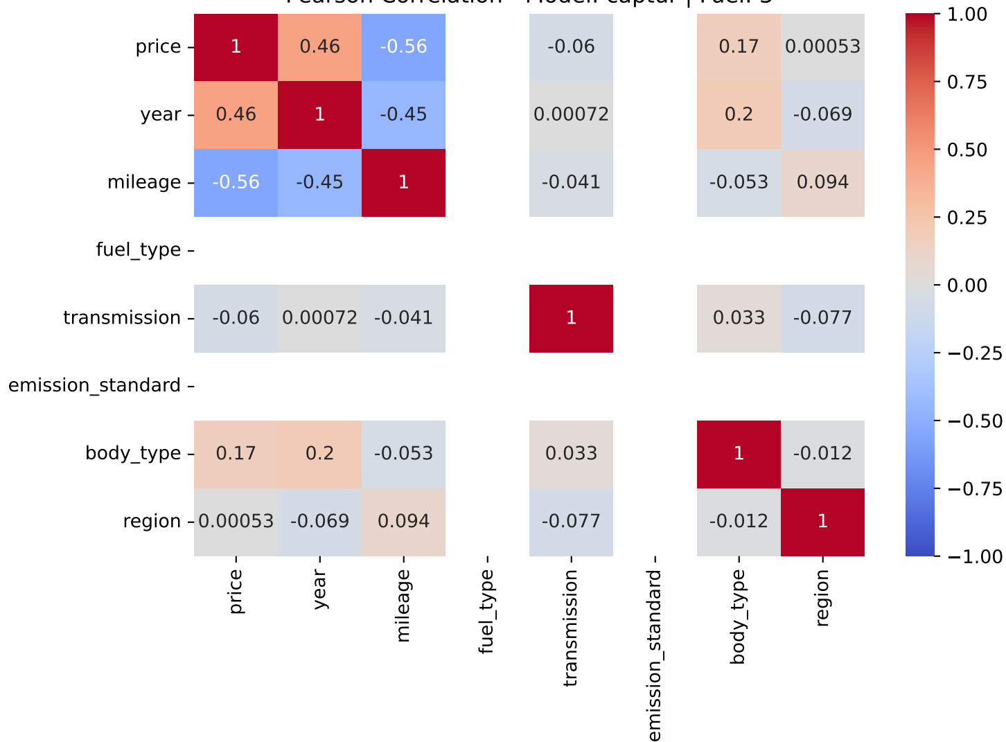
Pearson Correlation - Model: captur | Fuel: 3
