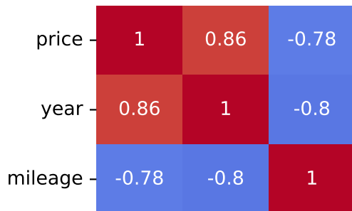
Spearman Correlation - Model: clio | Fuel: 2
