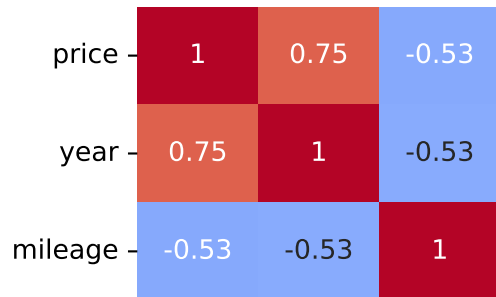
Spearman Correlation - Model: panda cross | Fuel: 3
