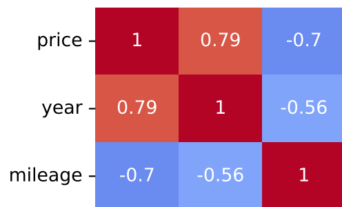
Pearson Correlation - Model: c3 | Fuel: 4
