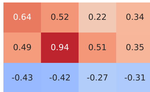
Pearson Correlation - Model: clubman | Fuel: 2
