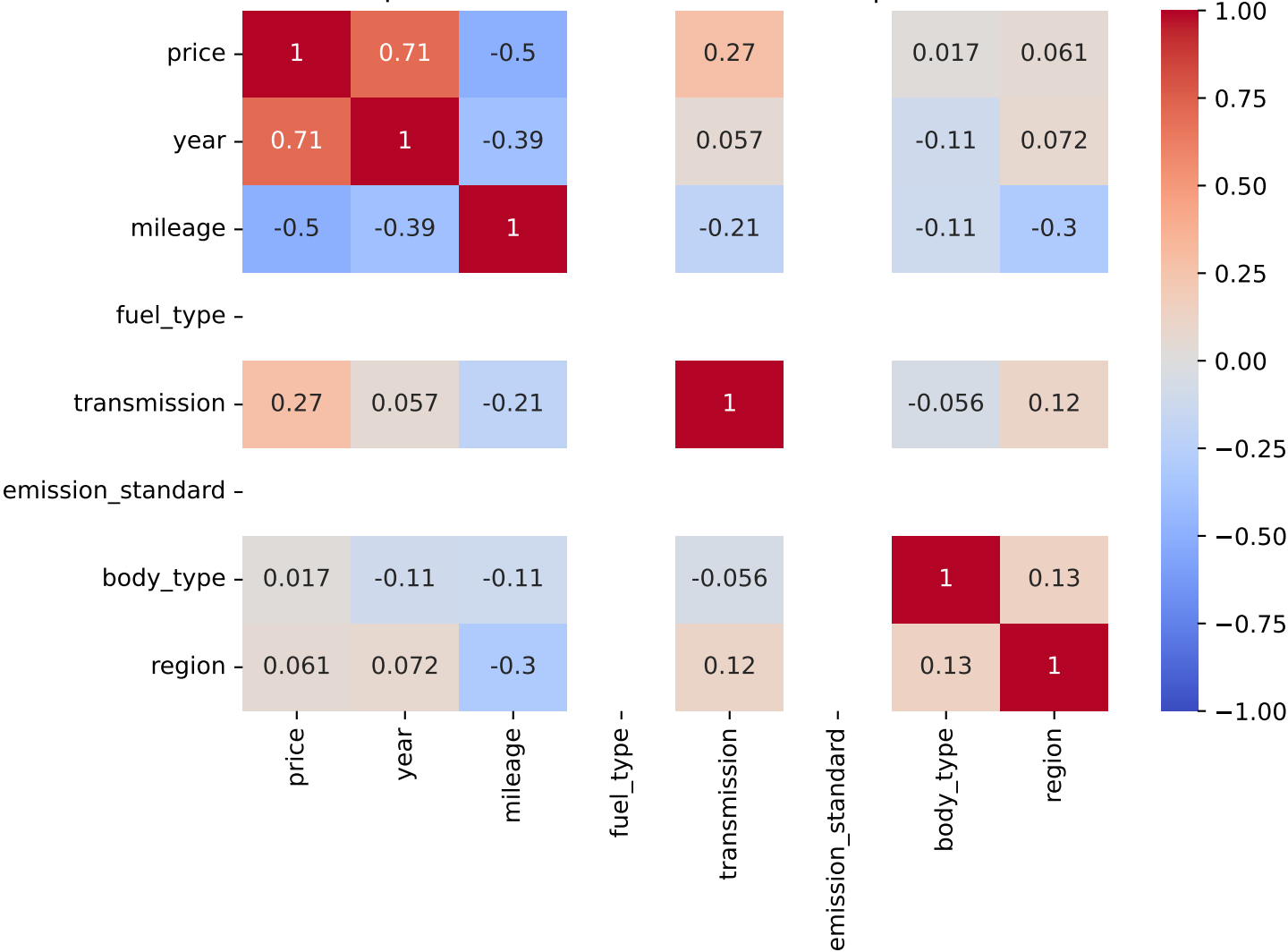
Spearman Correlation - Model: zoe | Fuel: 0
