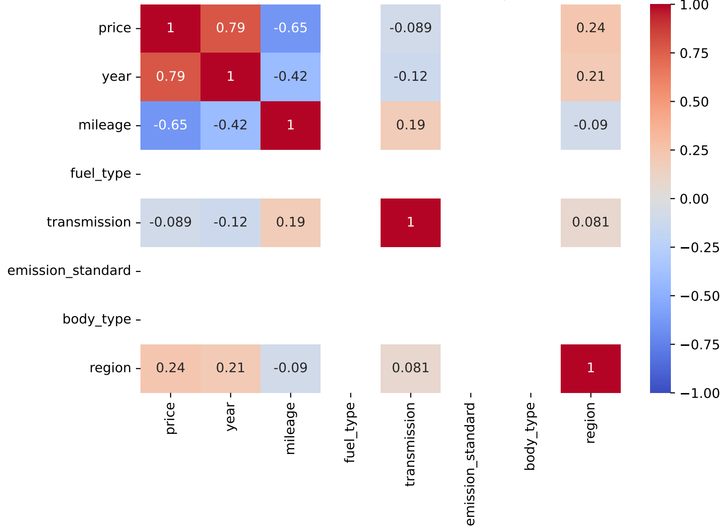
Spearman Correlation - Model: kodiaq | Fuel: 1
