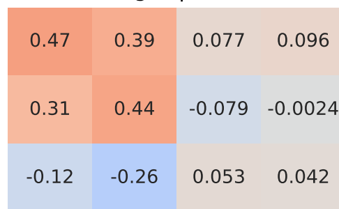
Spearman Correlation - Model: ranger | Fuel: 1
