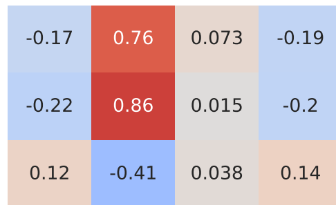
Spearman Correlation - Model: c4 picasso | Fuel: 1
