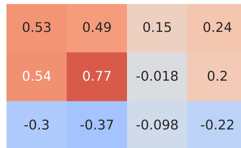
Pearson Correlation - Model: clubman | Fuel: 1
