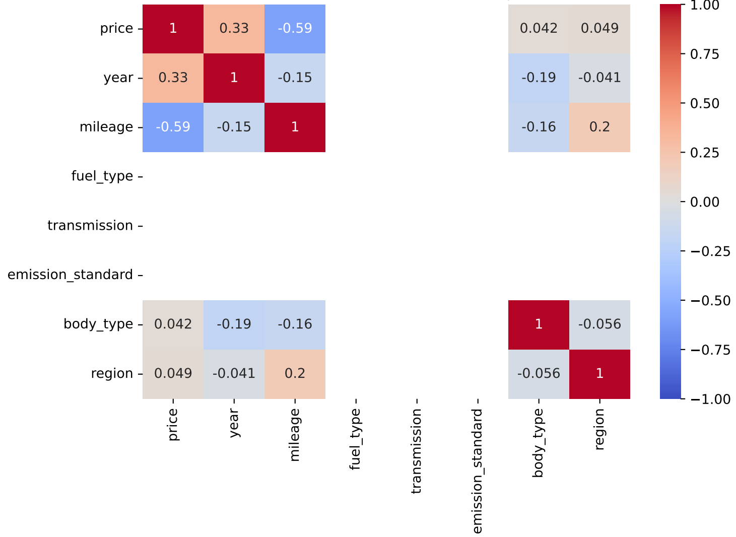
Spearman Correlation - Model: puma | Fuel: 1
