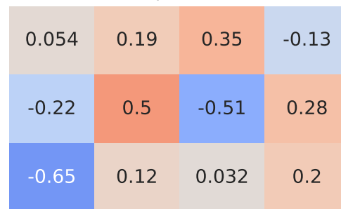
Pearson Correlation - Model: stilo | Fuel: 2
