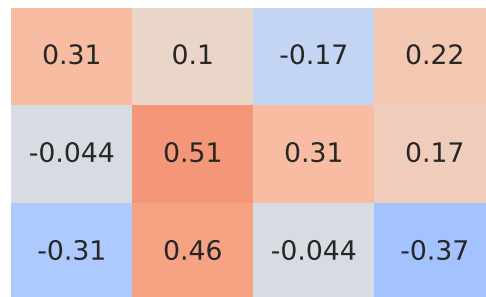
Spearman Correlation - Model: zafira tourer | Fuel: 1
