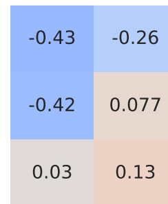
Spearman Correlation - Model: xceed | Fuel: 4
