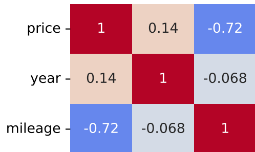
Spearman Correlation - Model: venga | Fuel: 4
