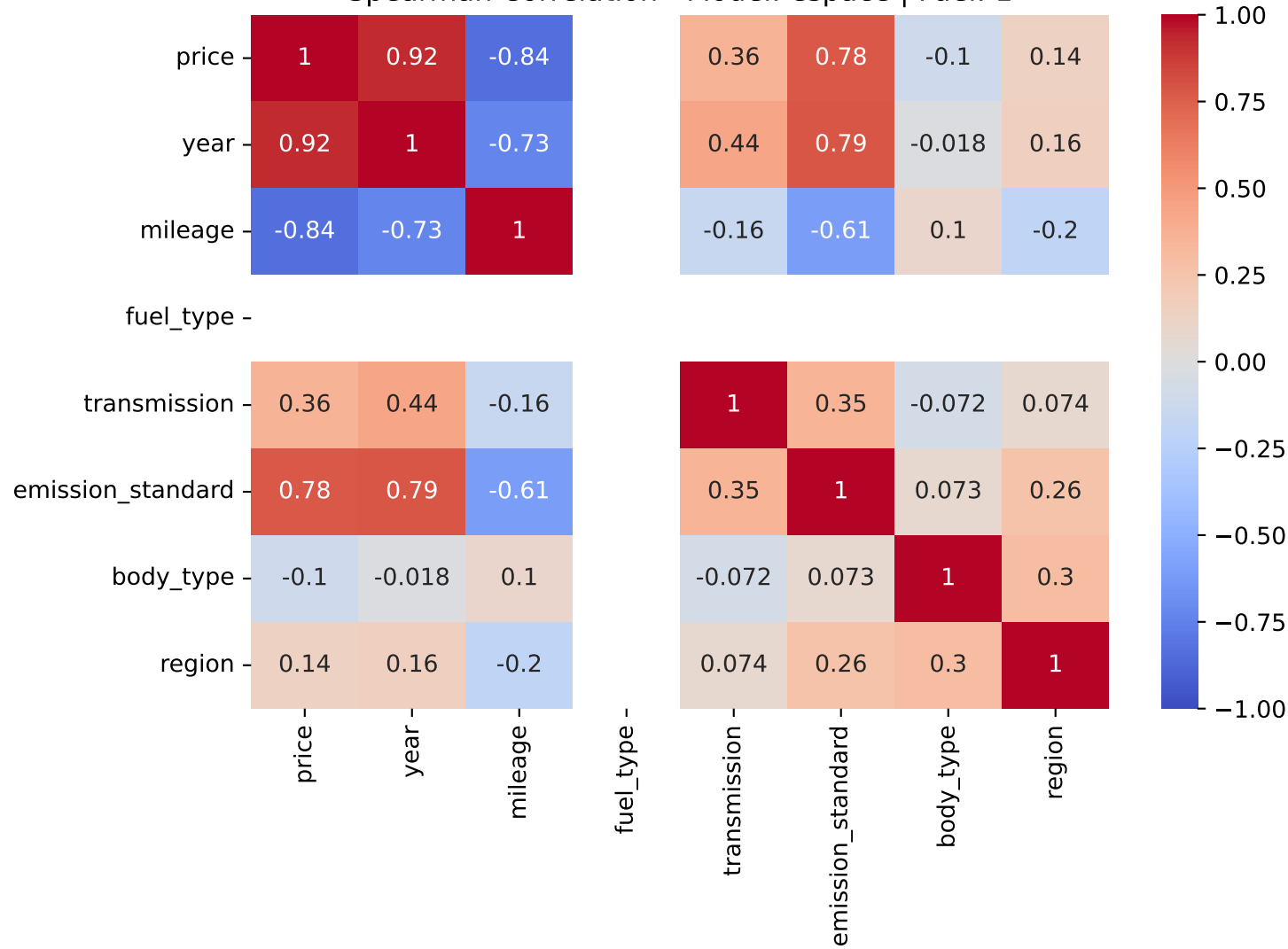
Spearman Correlation - Model: espace | Fuel: 1
