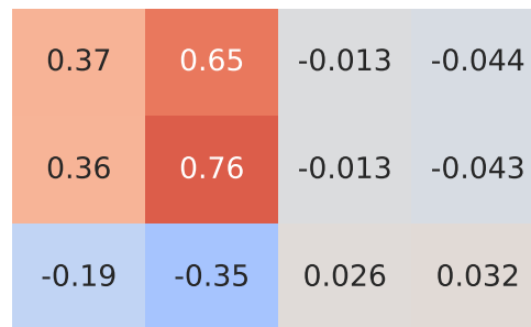
Pearson Correlation - Model: 3008 | Fuel: 1
