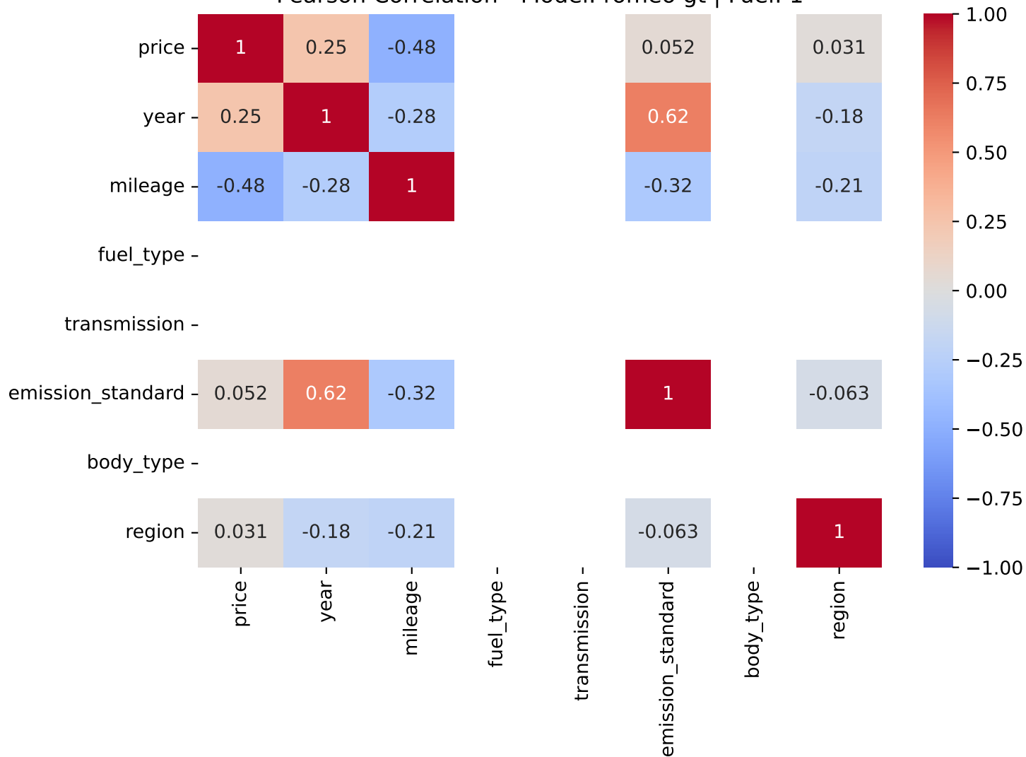
Pearson Correlation - Model: romeo gt | Fuel: 1
