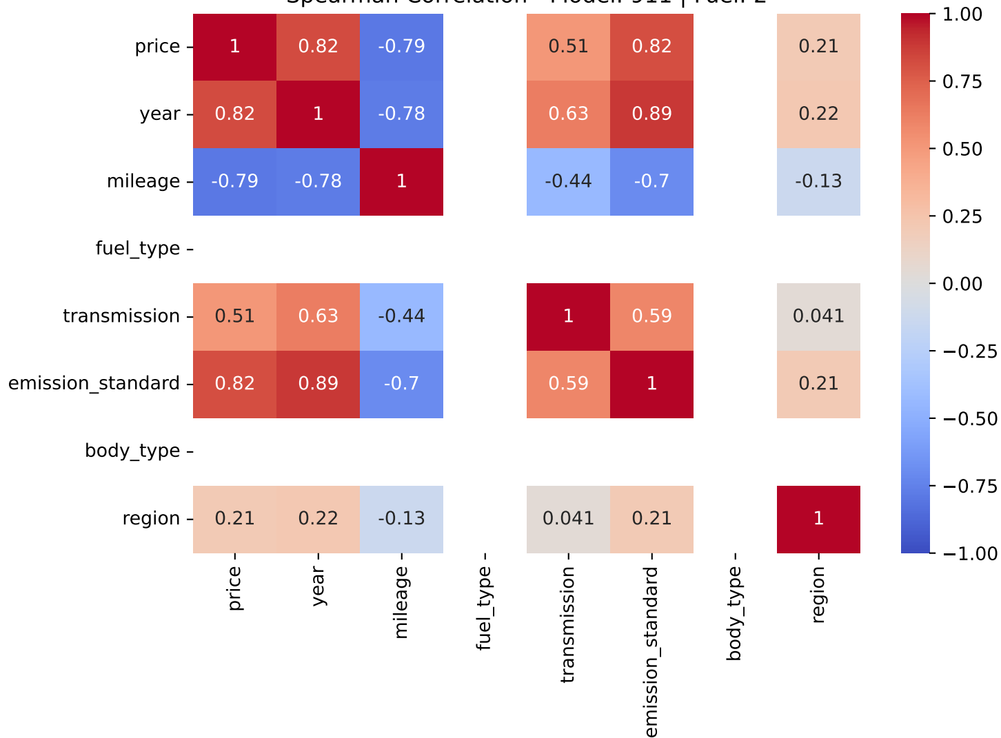
Spearman Correlation - Model: 911 | Fuel: 2
