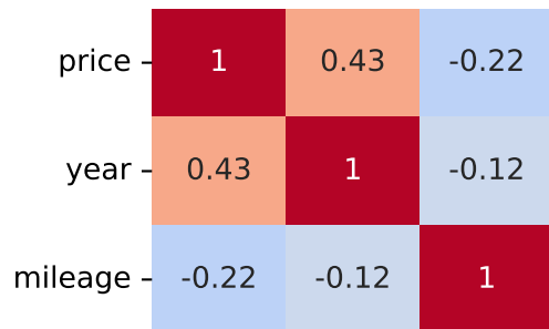
Spearman Correlation - Model: alto | Fuel: 2
