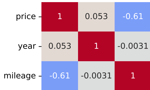
Spearman Correlation - Model: stonic | Fuel: 1
