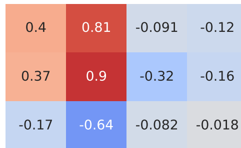
Spearman Correlation - Model: galaxy | Fuel: 1
