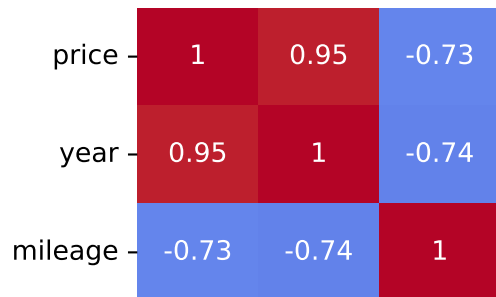
Spearman Correlation - Model: s3 | Fuel: 2
