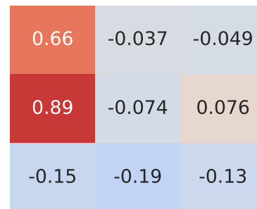
Pearson Correlation - Model: swift | Fuel: 1
