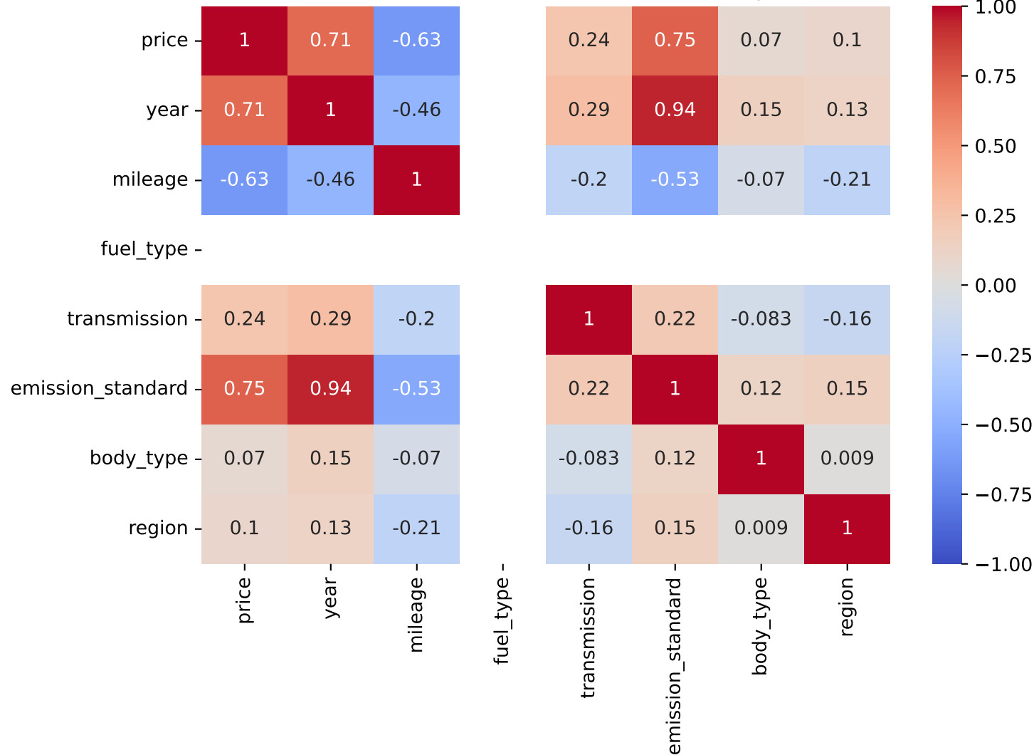
Pearson Correlation - Model: transit connect | Fuel: 1
