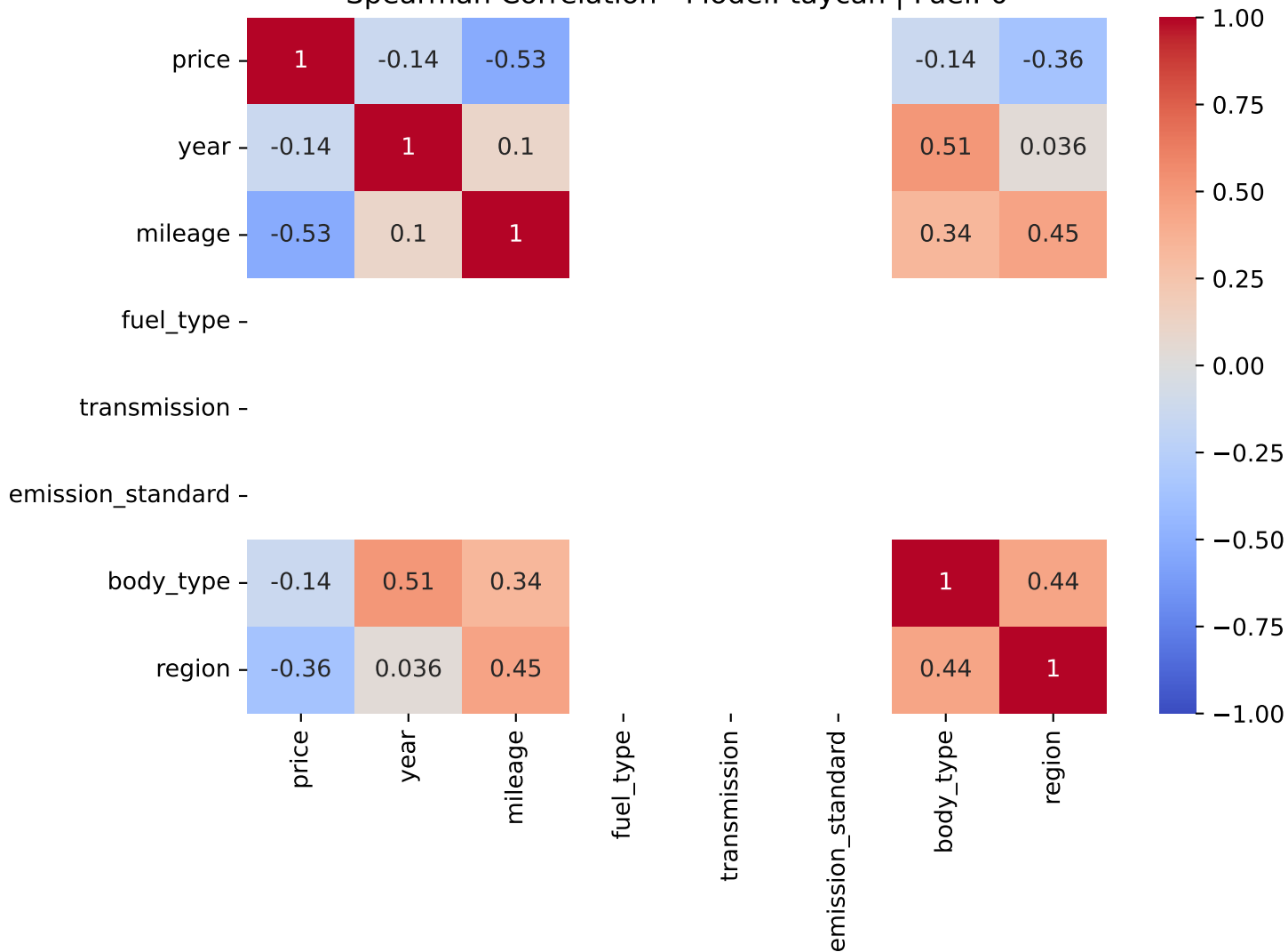
Spearman Correlation - Model: taycan | Fuel: 0
