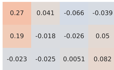
Spearman Correlation - Model: crossland | Fuel: 2
