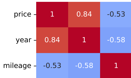
Pearson Correlation - Model: a4 | Fuel: 2
