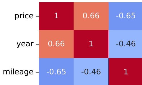
Pearson Correlation - Model: rover discovery sport | Fuel: 1
