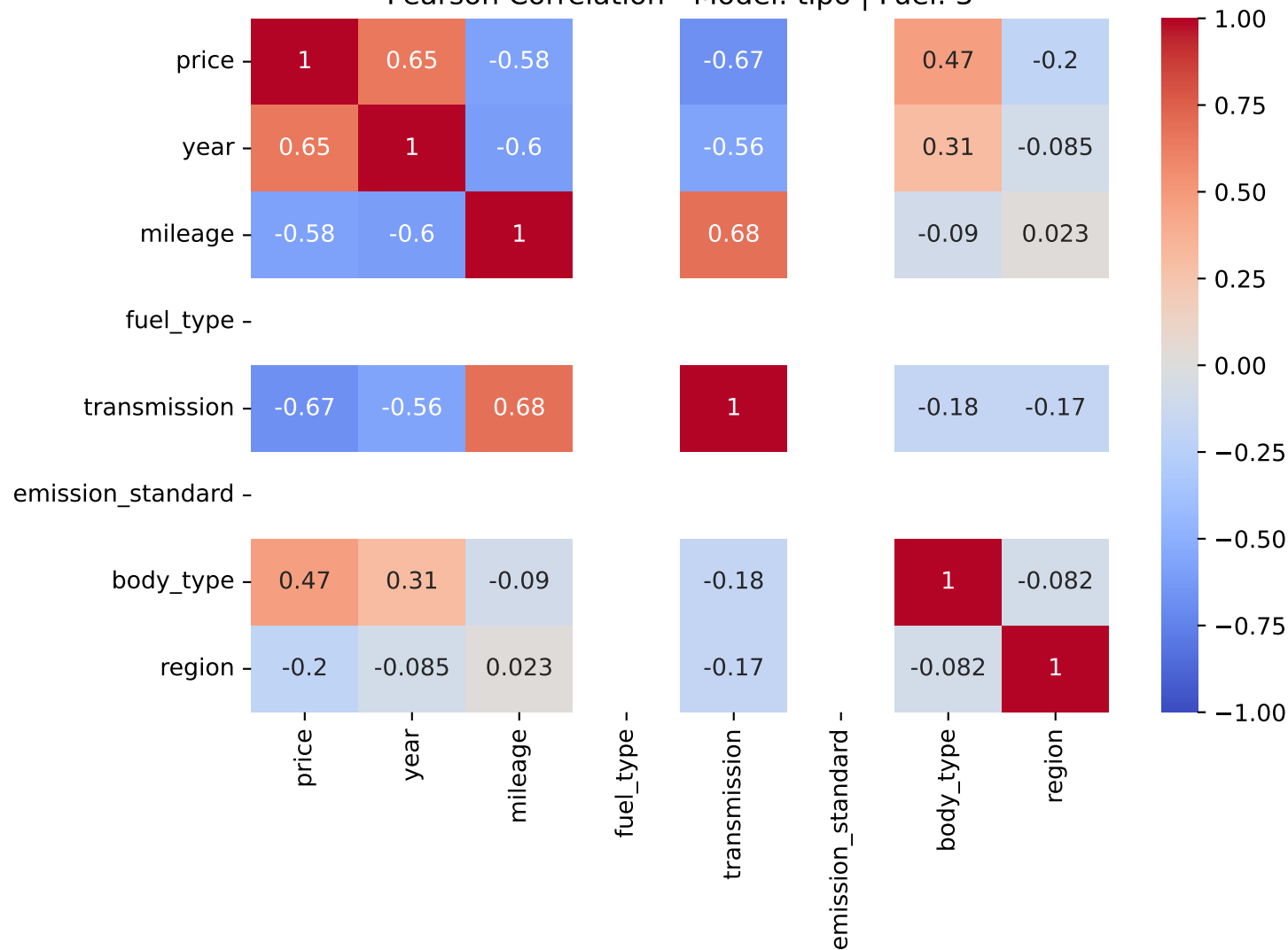
Pearson Correlation - Model: tipo | Fuel: 3
