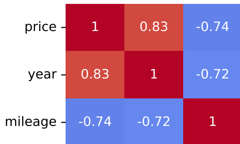
Spearman Correlation - Model: 3008 | Fuel: 2
