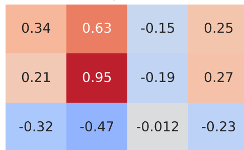
Pearson Correlation - Model: swift | Fuel: 2
