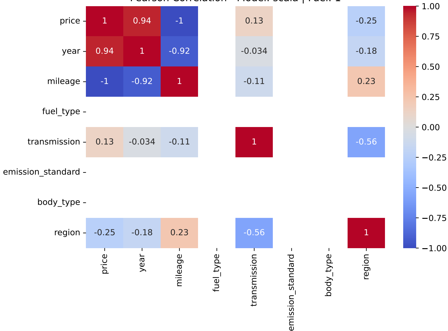
Pearson Correlation - Model: scala | Fuel: 1
