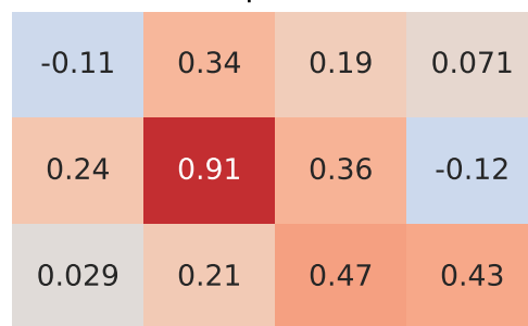
Pearson Correlation - Model: altea | Fuel: 1
