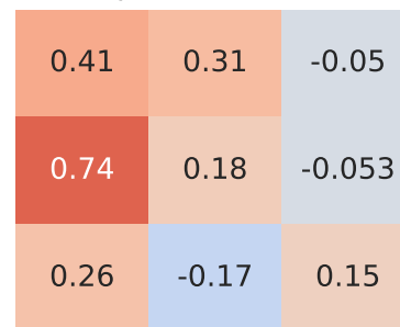
Pearson Correlation - Model: agila | Fuel: 2
