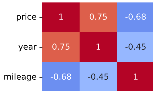
Spearman Correlation - Model: 500l | Fuel: 1
