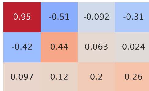
Pearson Correlation - Model: romeo 147 | Fuel: 2
