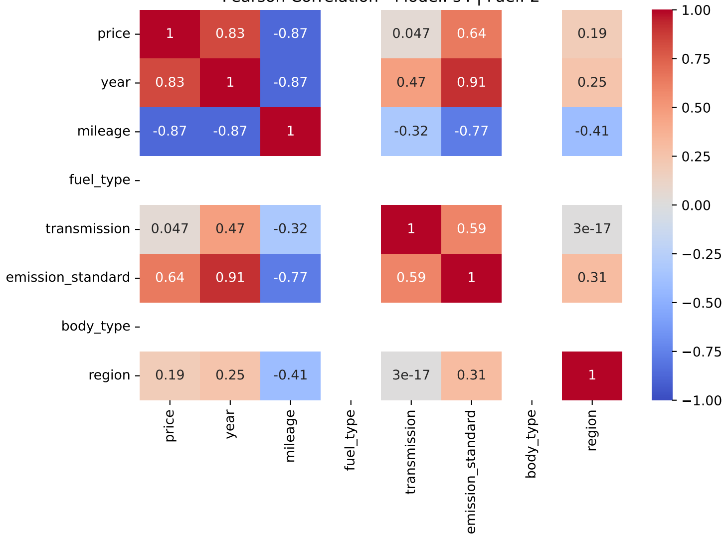
Pearson Correlation - Model: s4 | Fuel: 2
