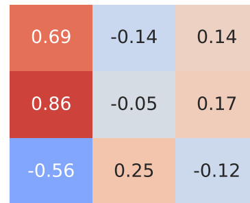
Pearson Correlation - Model: i20 | Fuel: 4
