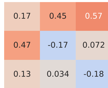
Spearman Correlation - Model: romeo gtv | Fuel: 2
