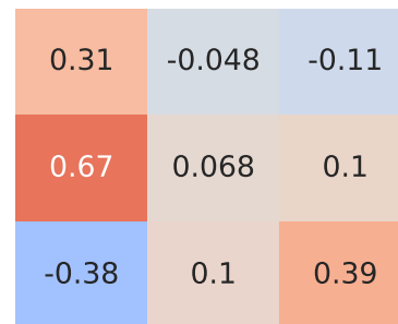
Pearson Correlation - Model: 500l | Fuel: 5
