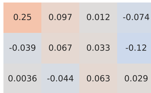
Spearman Correlation - Model: 500x | Fuel: 2
