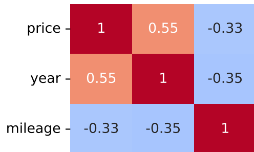
Pearson Correlation - Model: rover range rover | Fuel: 3
