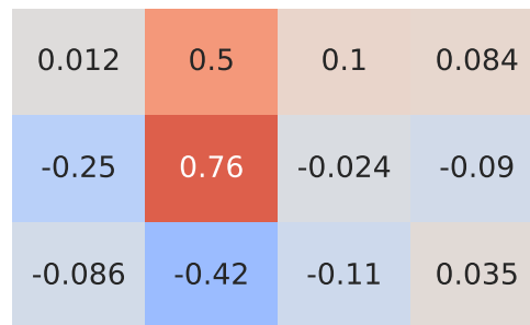
Pearson Correlation - Model: b-max | Fuel: 2
