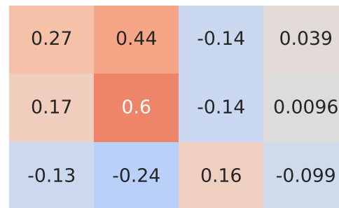
Pearson Correlation - Model: captur | Fuel: 1
