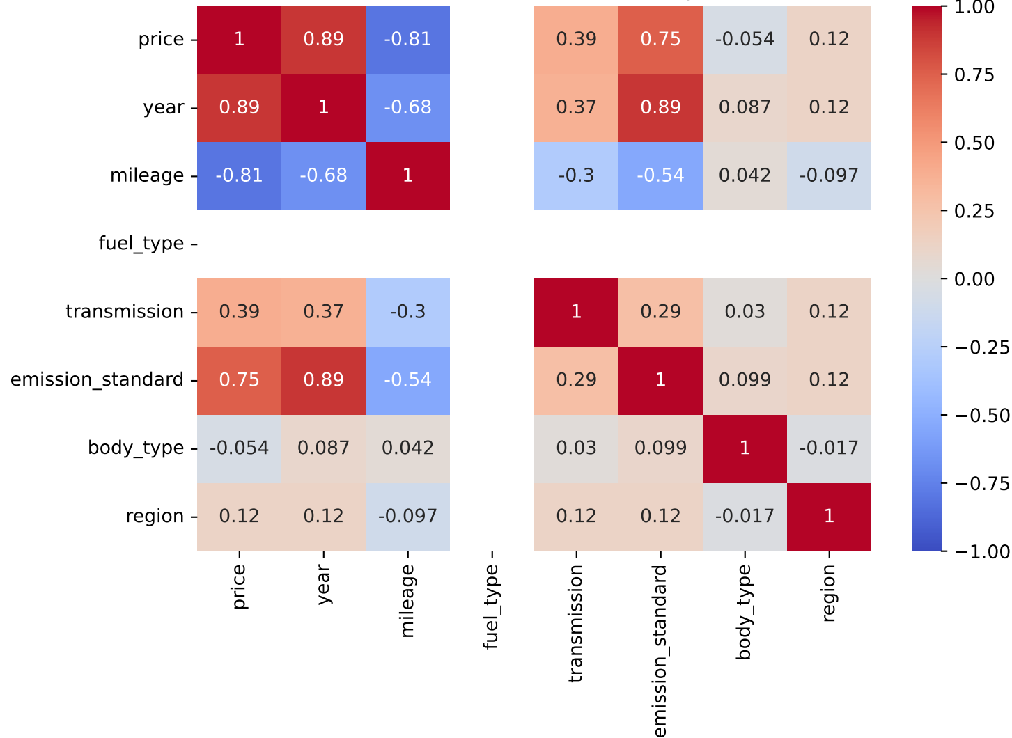
Pearson Correlation - Model: focus | Fuel: 1
