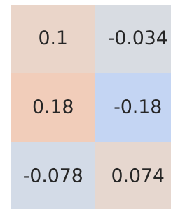
Spearman Correlation - Model: panda cross | Fuel: 3
