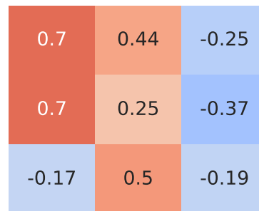
Spearman Correlation - Model: astra gtc | Fuel: 1
