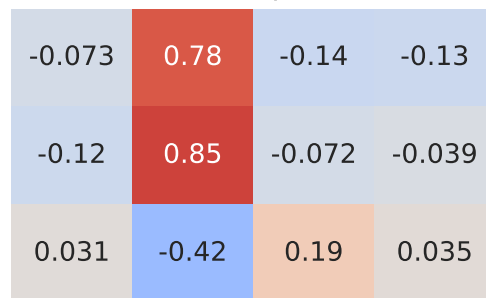
Spearman Correlation - Model: cayenne | Fuel: 1
