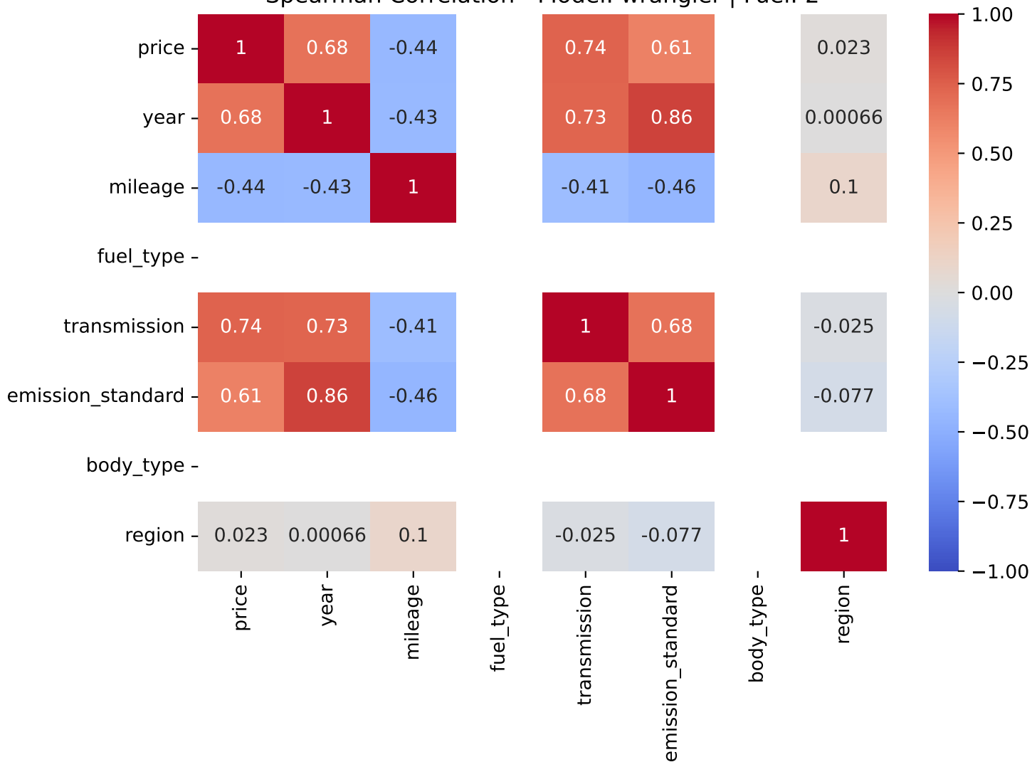
Spearman Correlation - Model: wrangler | Fuel: 2
