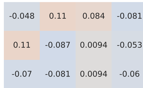
Spearman Correlation - Model: a6 | Fuel: 3
