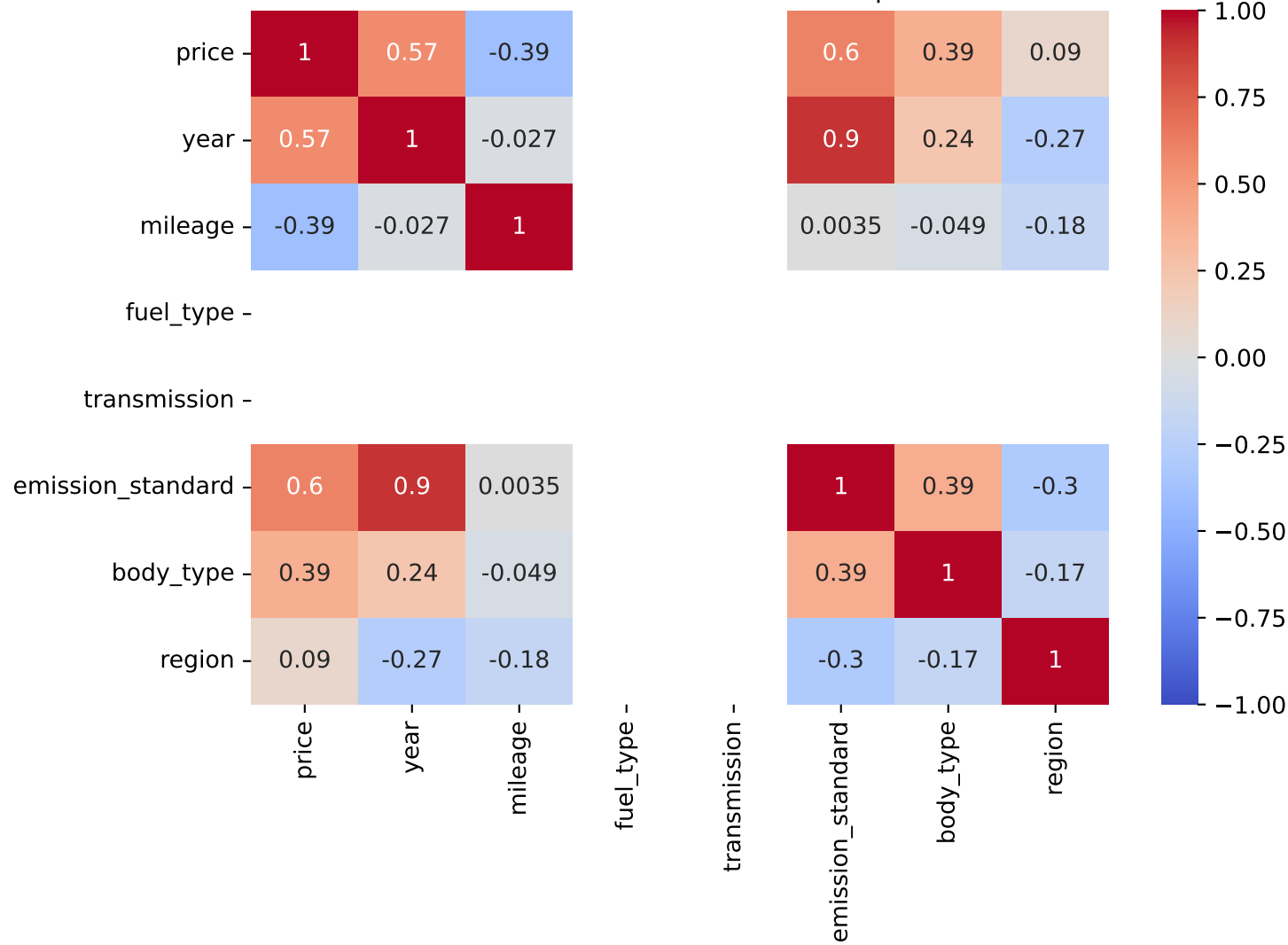
Pearson Correlation - Model: bravo | Fuel: 2
