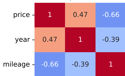
Spearman Correlation - Model: stonic | Fuel: 4
