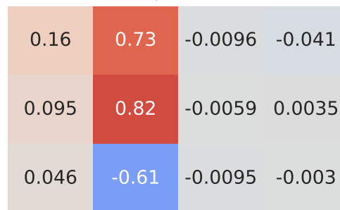
Pearson Correlation - Model: juke | Fuel: 2
