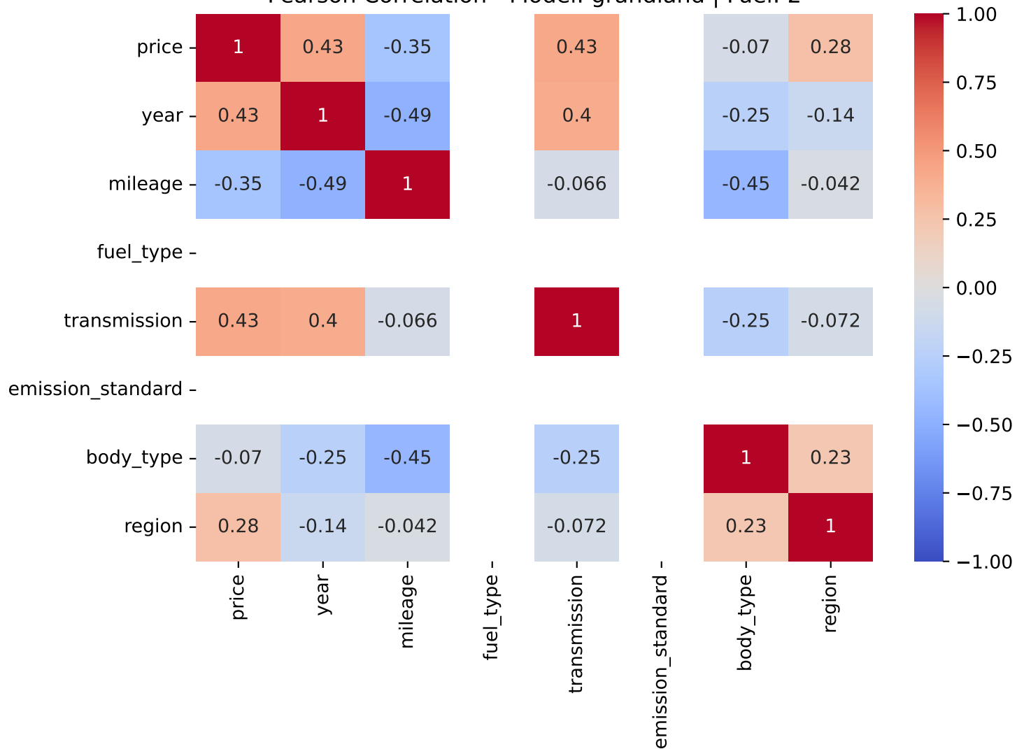
Pearson Correlation - Model: grandland | Fuel: 2
