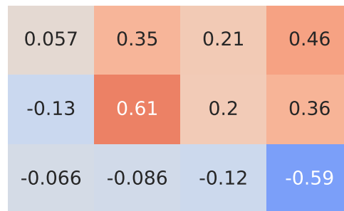
Pearson Correlation - Model: verso | Fuel: 1
