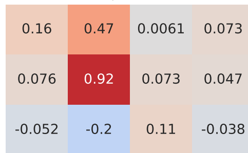
Pearson Correlation - Model: 500 | Fuel: 2
