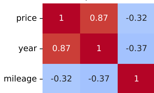
Spearman Correlation - Model: kadjar | Fuel: 2
