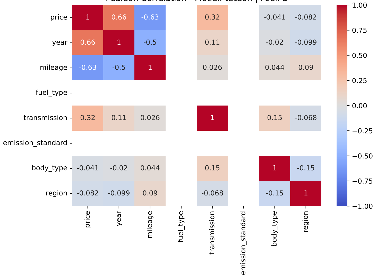
Pearson Correlation - Model: tucson | Fuel: 3
