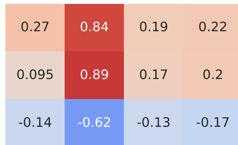
Spearman Correlation - Model: aygo | Fuel: 2
