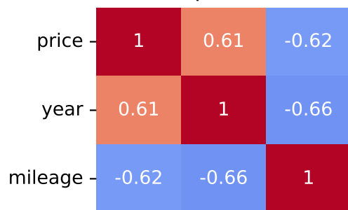
Spearman Correlation - Model: arona | Fuel: 2
