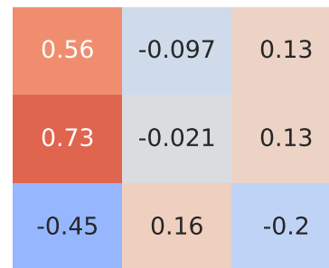
Spearman Correlation - Model: romeo mito | Fuel: 1
