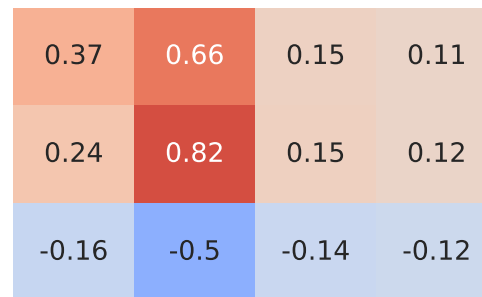
Pearson Correlation - Model: polo | Fuel: 2
