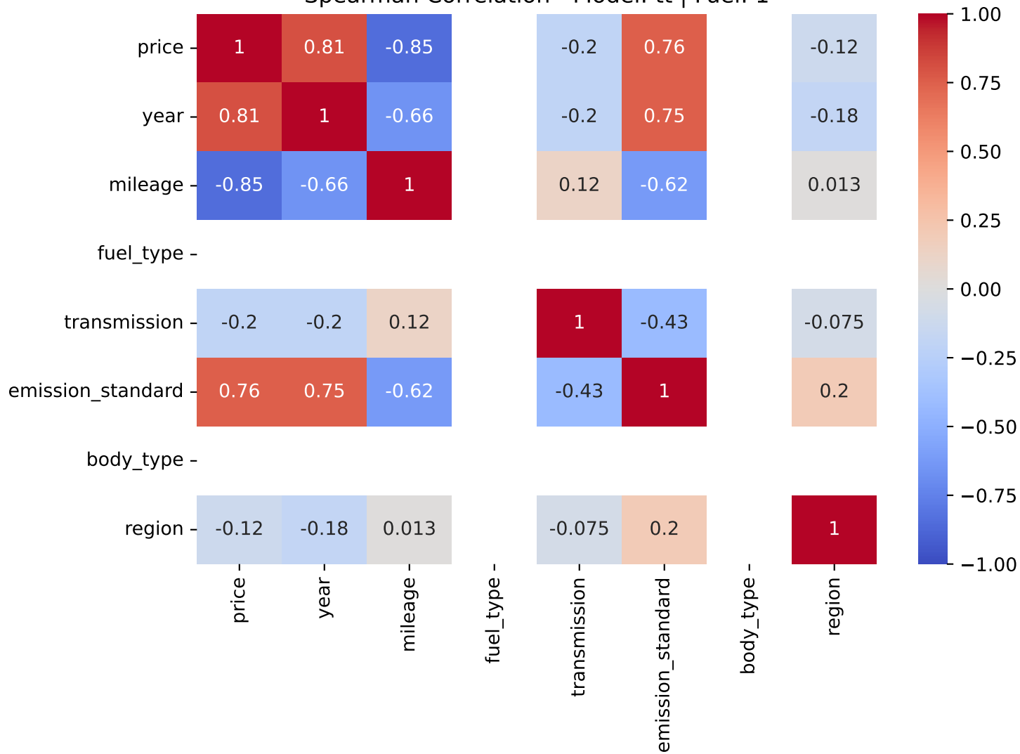
Spearman Correlation - Model: tt | Fuel: 1
