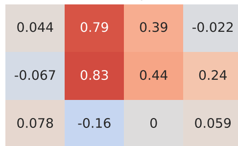
Spearman Correlation - Model: panamera | Fuel: 2
