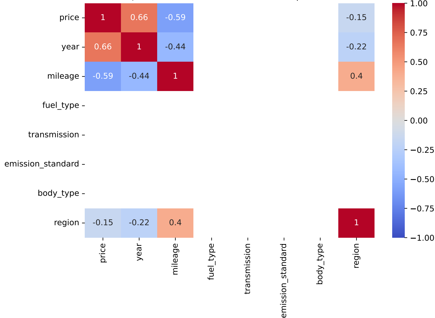
Spearman Correlation - Model: leaf | Fuel: 0
