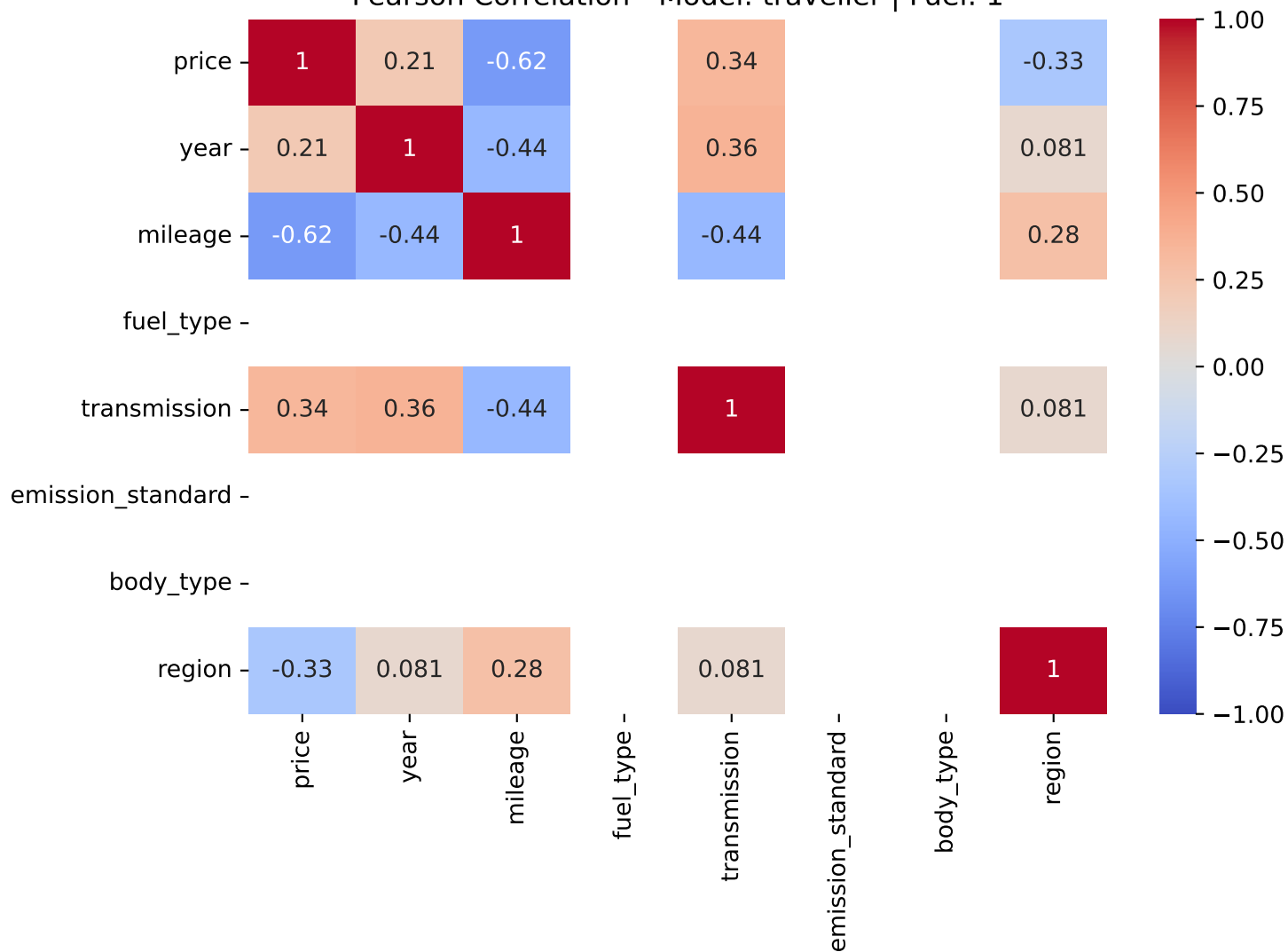
Pearson Correlation - Model: traveller | Fuel: 1
