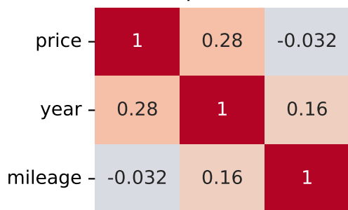
Spearman Correlation - Model: phedra | Fuel: 1
