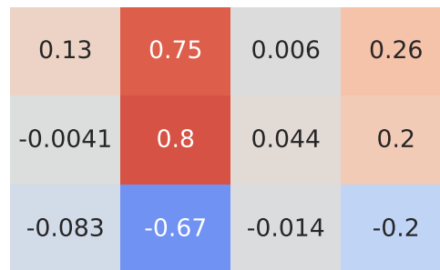
Pearson Correlation - Model: ibiza | Fuel: 2
