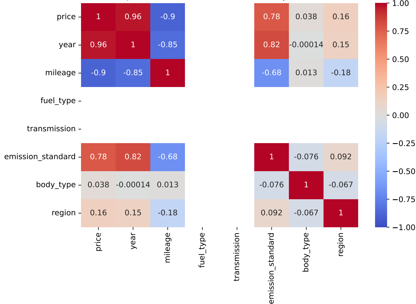
Spearman Correlation - Model: clio | Fuel: 4
