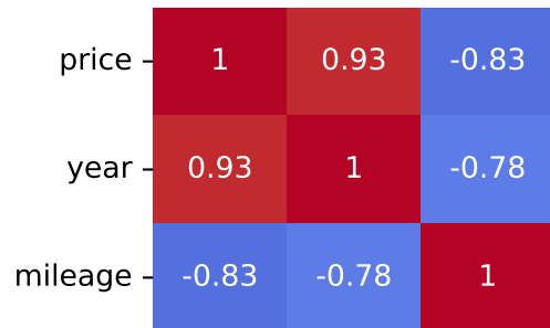
Pearson Correlation - Model: c3 | Fuel: 2
