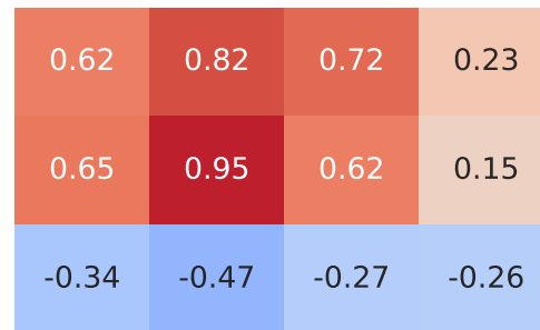
Spearman Correlation - Model: a4 | Fuel: 2
