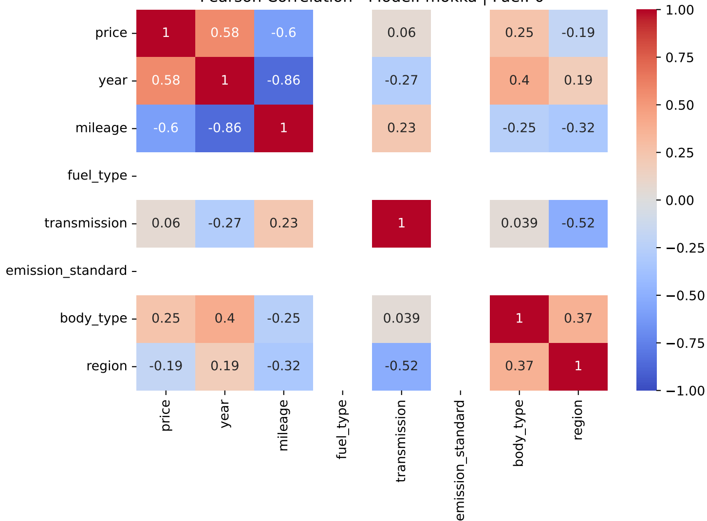
Pearson Correlation - Model: mokka | Fuel: 0
