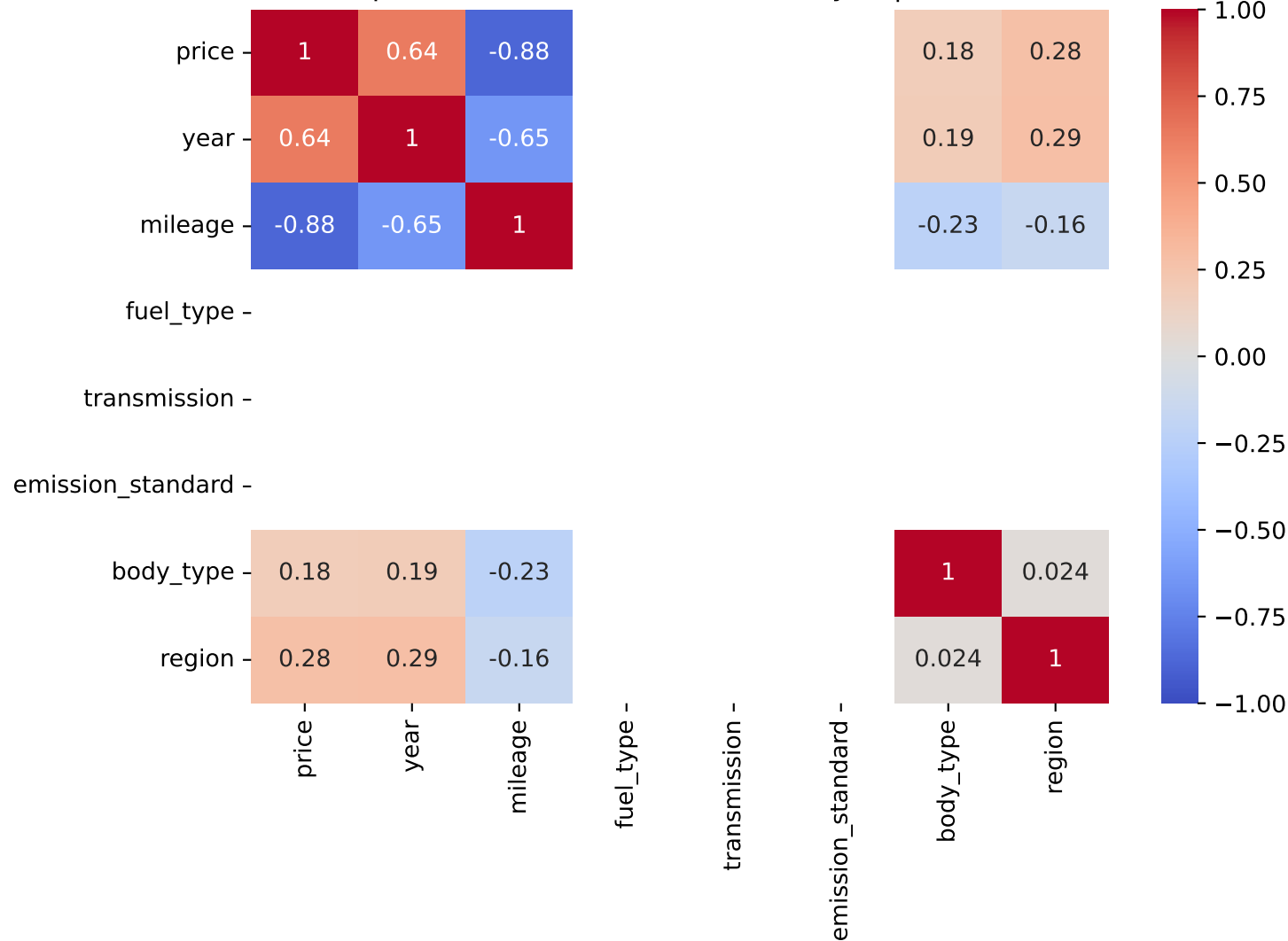
Spearman Correlation - Model: bayon | Fuel: 3
