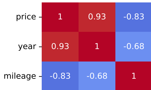
Spearman Correlation - Model: scenic | Fuel: 2
