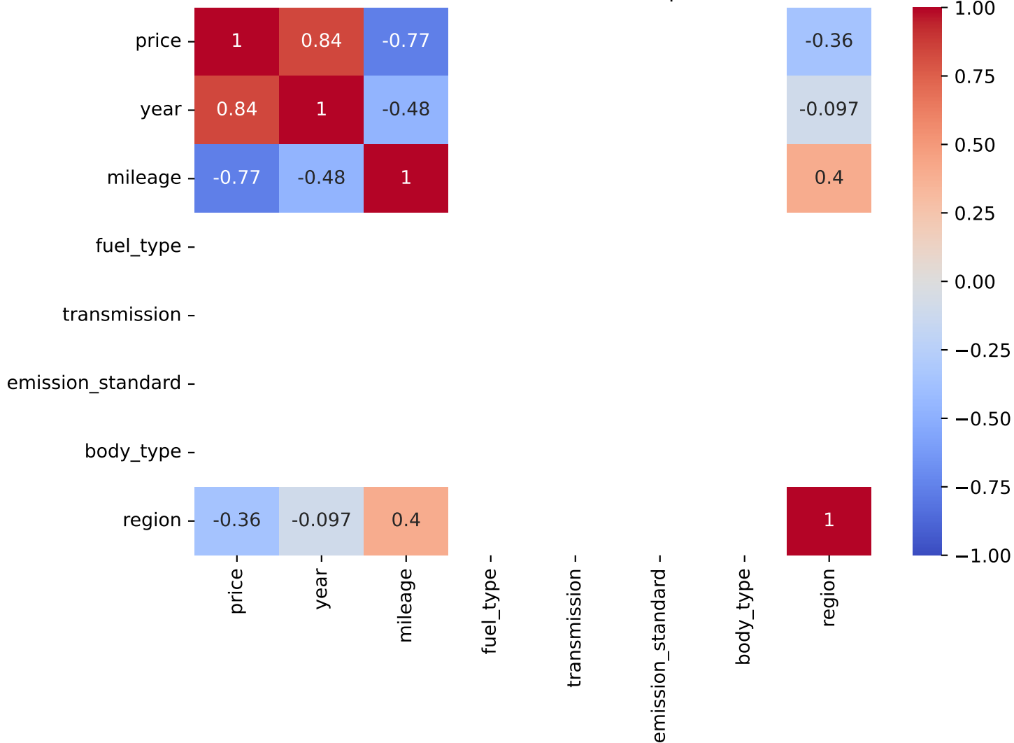
Pearson Correlation - Model: a8 | Fuel: 3
