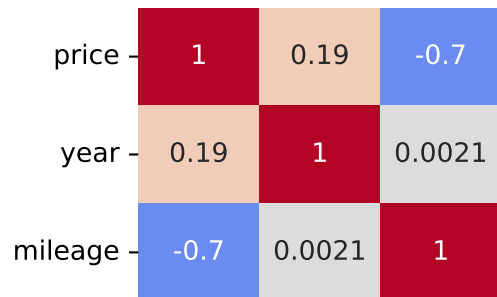
Pearson Correlation - Model: ix20 | Fuel: 2
