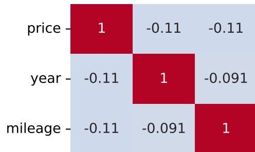
Pearson Correlation - Model: a2 | Fuel: 1
