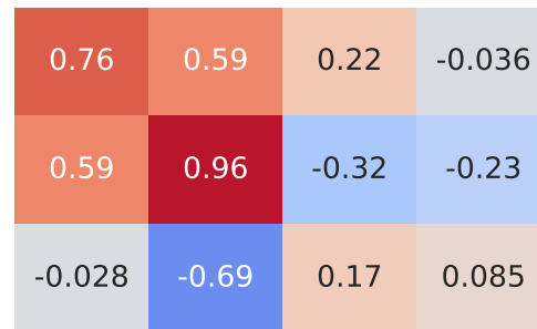
Spearman Correlation - Model: a6 | Fuel: 2
