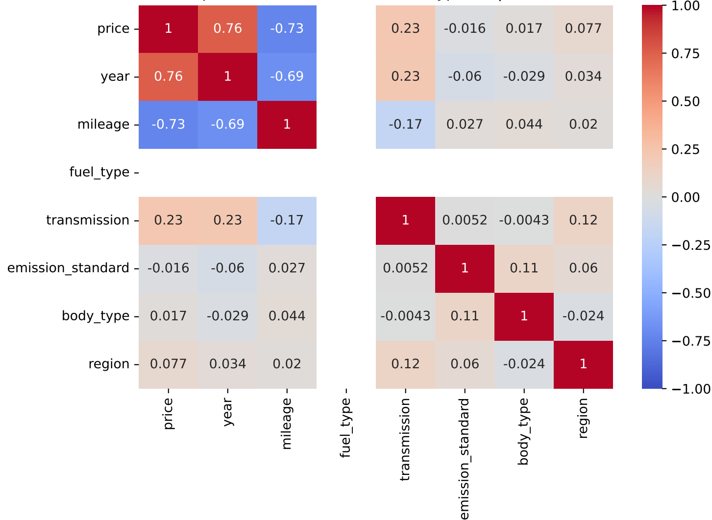
Spearman Correlation - Model: ypsilon | Fuel: 3
