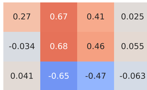
Spearman Correlation - Model: c4 | Fuel: 2
