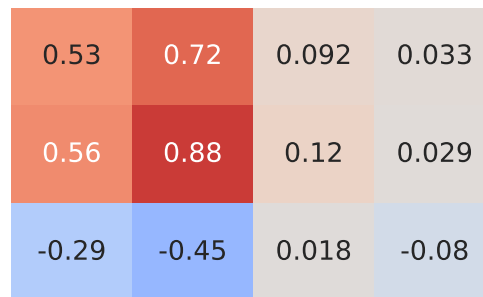
Pearson Correlation - Model: a4 | Fuel: 1
