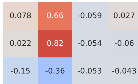
Pearson Correlation - Model: meriva | Fuel: 1
