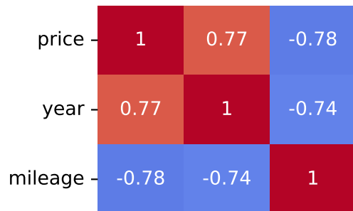
Spearman Correlation - Model: caddy | Fuel: 1
