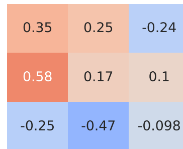
Spearman Correlation - Model: golf | Fuel: 4
