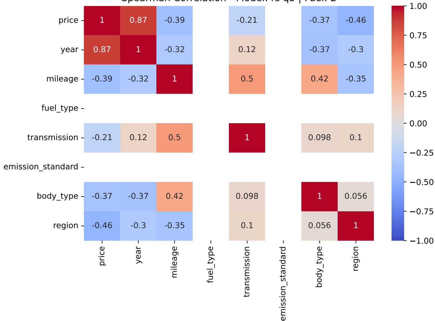
Spearman Correlation - Model: rs q3 | Fuel: 2
