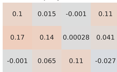
Pearson Correlation - Model: kadjar | Fuel: 1
