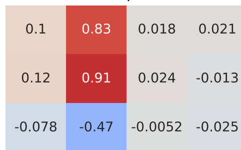
Spearman Correlation - Model: c-max | Fuel: 1
