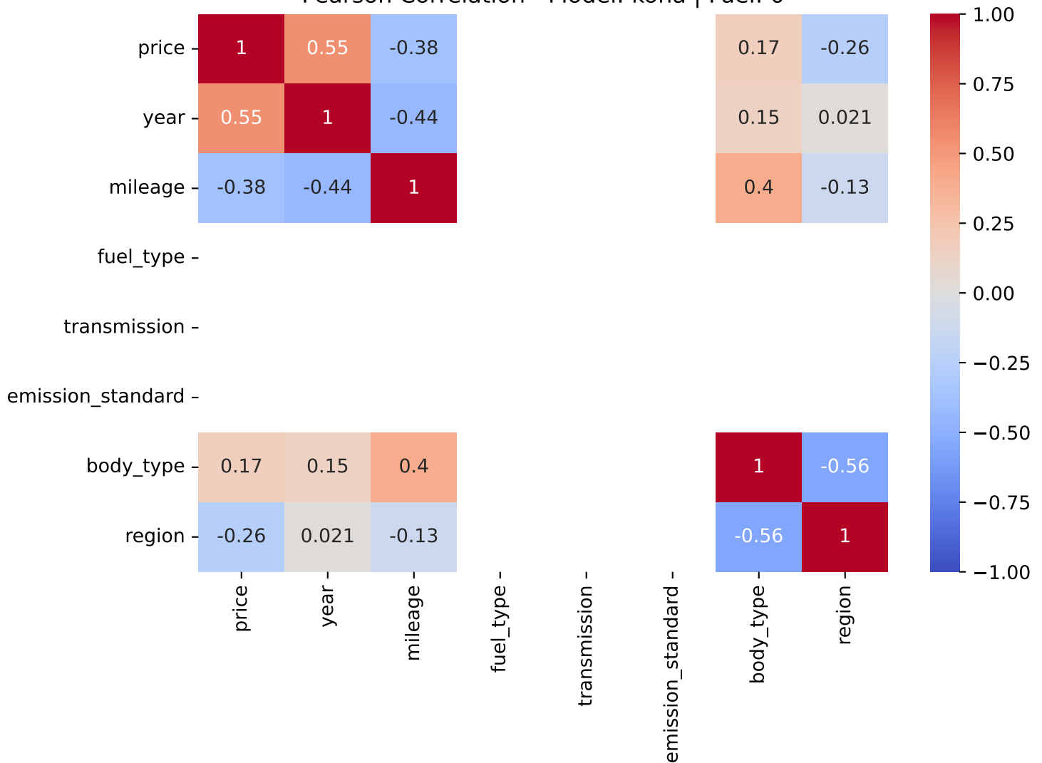
Pearson Correlation - Model: kona | Fuel: 0
