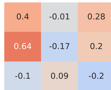
Spearman Correlation - Model: b-max | Fuel: 1
