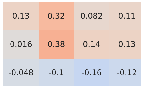
Pearson Correlation - Model: romeo 159 | Fuel: 1
