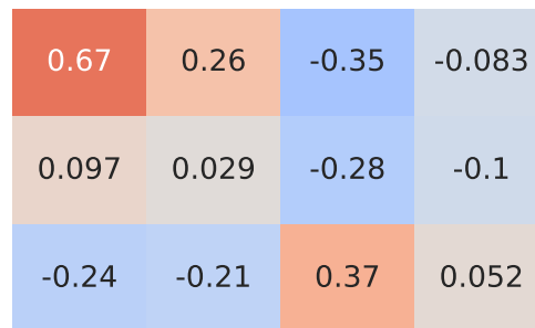
Pearson Correlation - Model: kona | Fuel: 2
