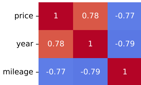
Pearson Correlation - Model: q8 | Fuel: 3
