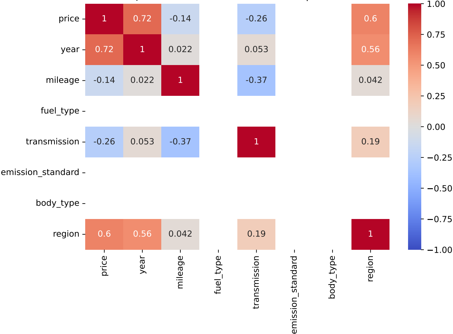
Spearman Correlation - Model: m2 | Fuel: 2
