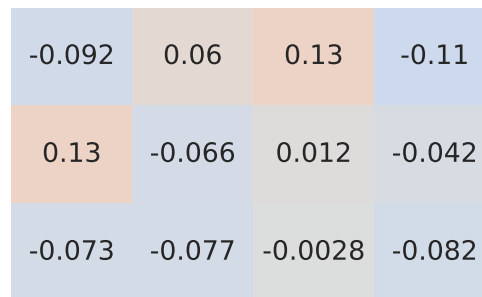
Pearson Correlation - Model: a6 | Fuel: 3
