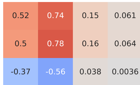
Spearman Correlation - Model: picanto | Fuel: 4
