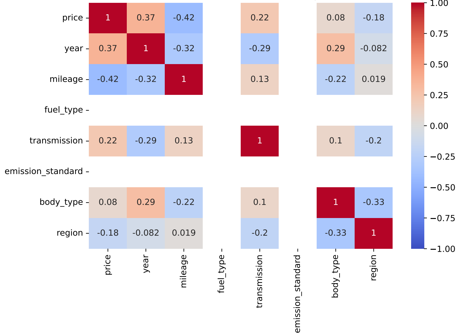
Spearman Correlation - Model: 2008 | Fuel: 0
