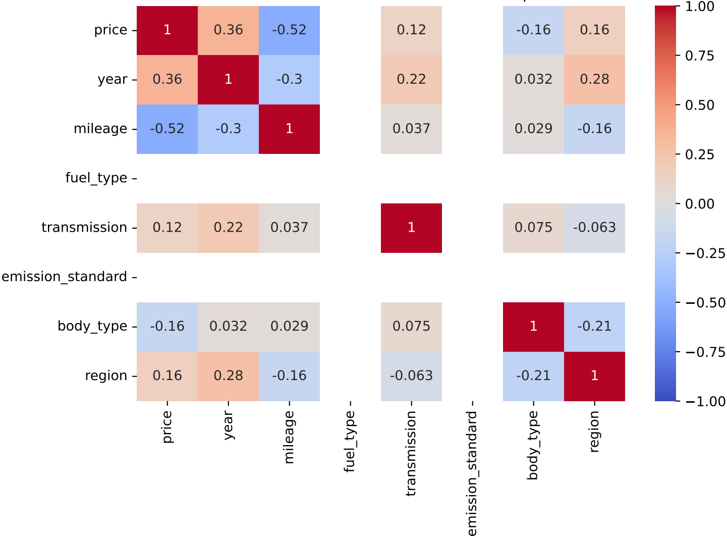
Pearson Correlation - Model: romeo tonale | Fuel: 1
