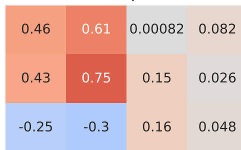
Spearman Correlation - Model: octavia | Fuel: 1
