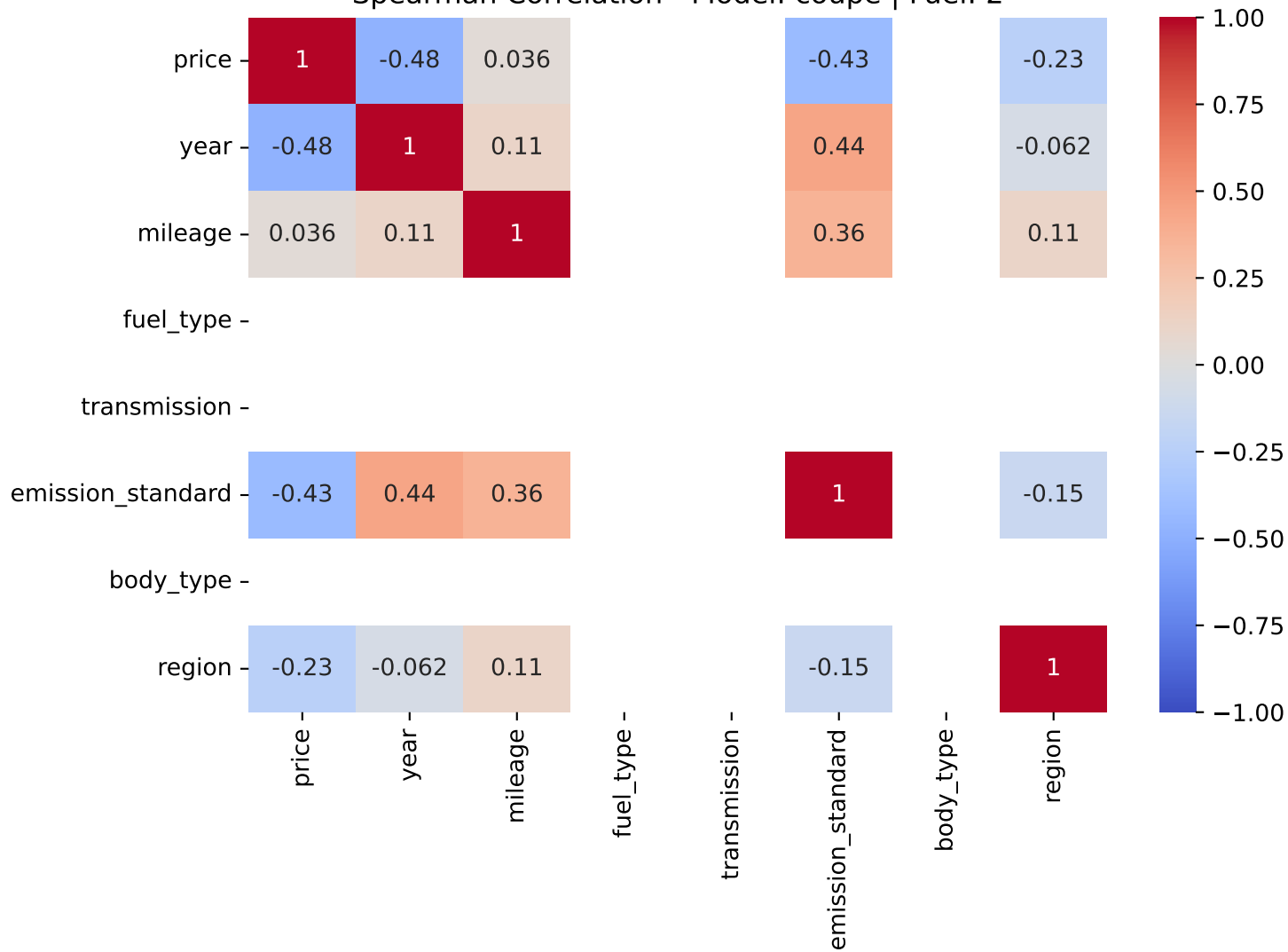
Spearman Correlation - Model: coupe | Fuel: 2
