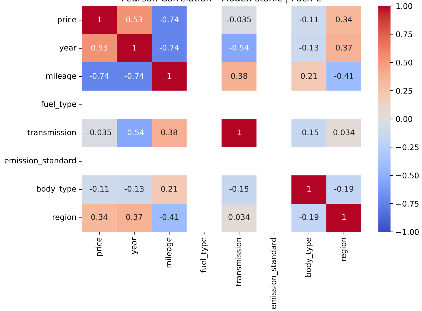
Pearson Correlation - Model: stonic | Fuel: 2
