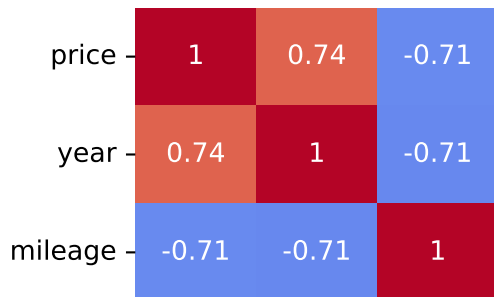
Pearson Correlation - Model: rover discovery | Fuel: 1
