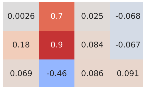
Pearson Correlation - Model: cayenne | Fuel: 2
