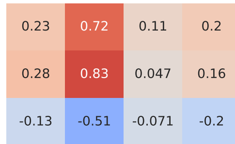
Spearman Correlation - Model: romeo giulietta | Fuel: 1
