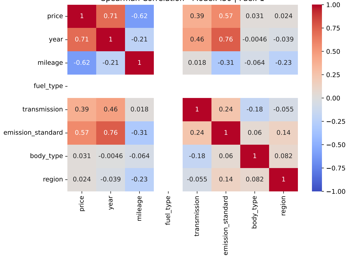
Spearman Correlation - Model: i30 | Fuel: 1
