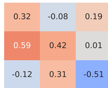
Pearson Correlation - Model: stilo | Fuel: 1
