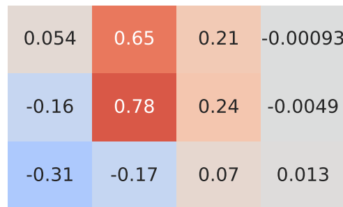
Spearman Correlation - Model: fortwo | Fuel: 1
