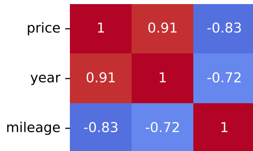
Pearson Correlation - Model: 5008 | Fuel: 1
