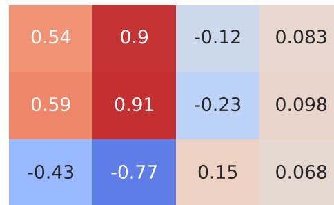
Spearman Correlation - Model: koleos | Fuel: 1
