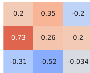
Pearson Correlation - Model: golf | Fuel: 4
