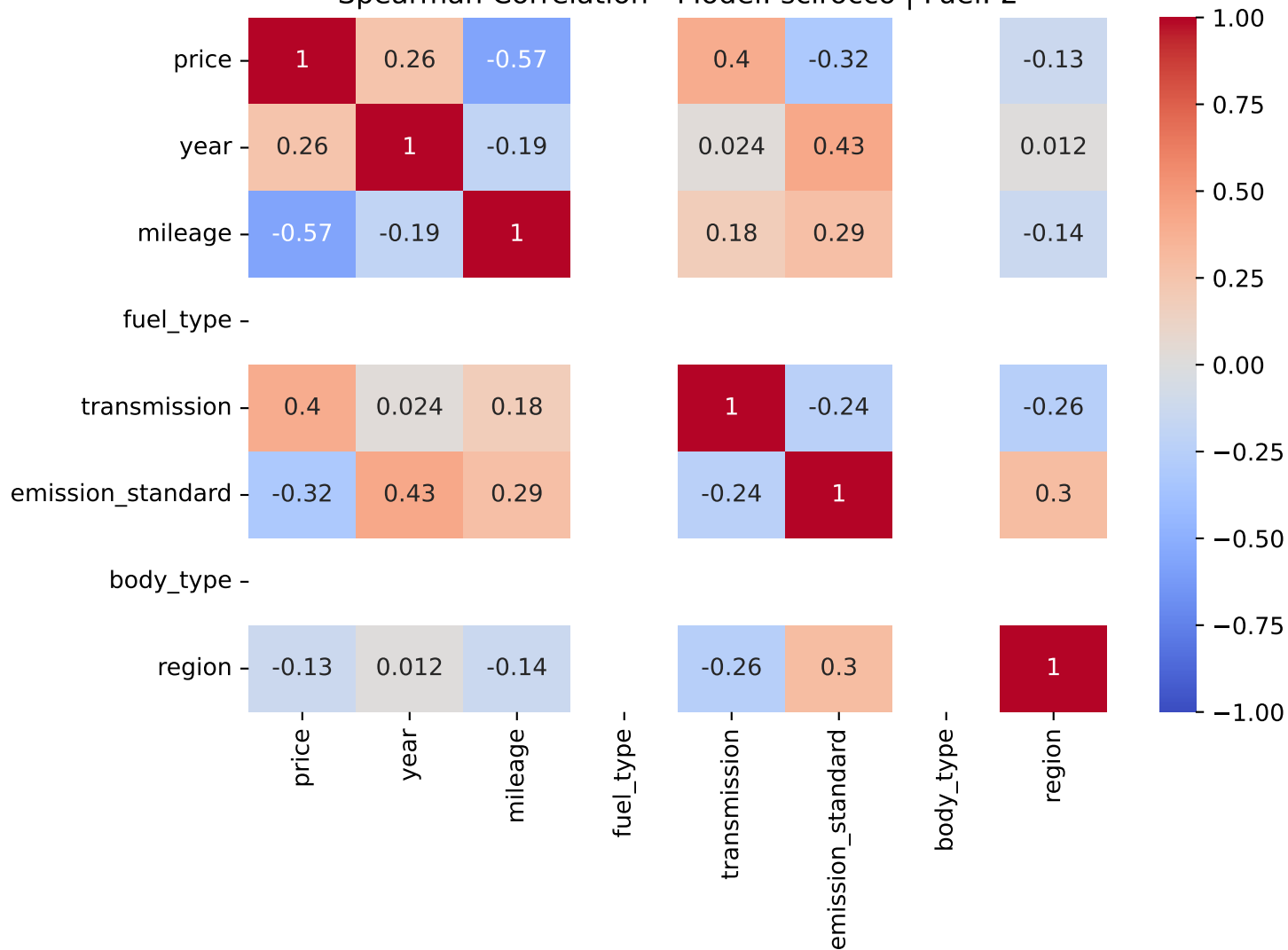
Spearman Correlation - Model: scirocco | Fuel: 2
