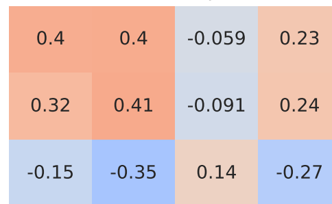
Spearman Correlation - Model: countryman | Fuel: 2
