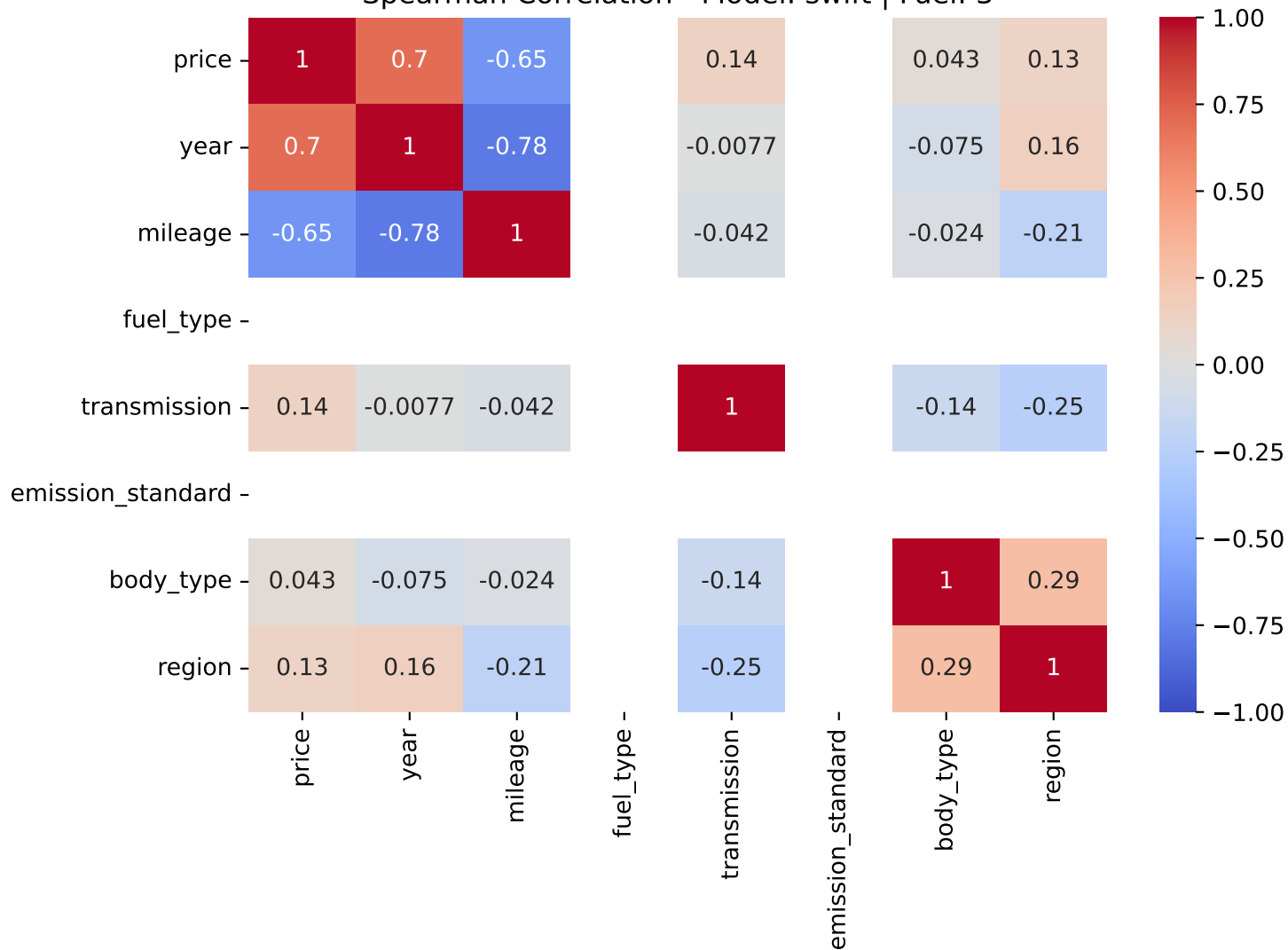
Spearman Correlation - Model: swift | Fuel: 3
