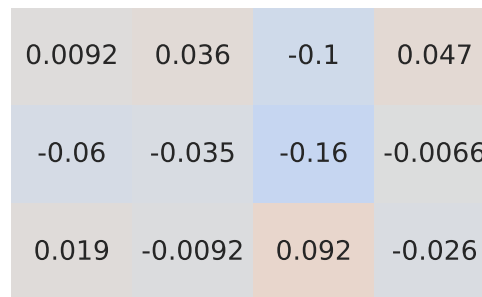
Pearson Correlation - Model: rover range rover | Fuel: 3
