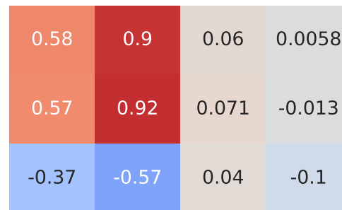
Spearman Correlation - Model: touran | Fuel: 1
