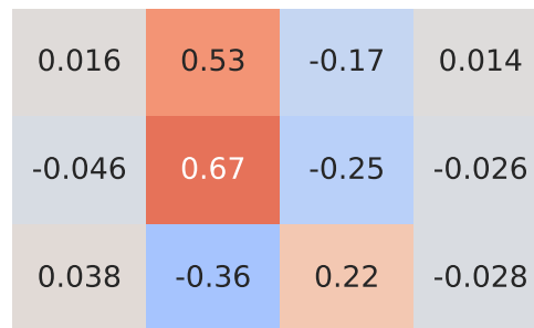
Pearson Correlation - Model: 500 | Fuel: 4
