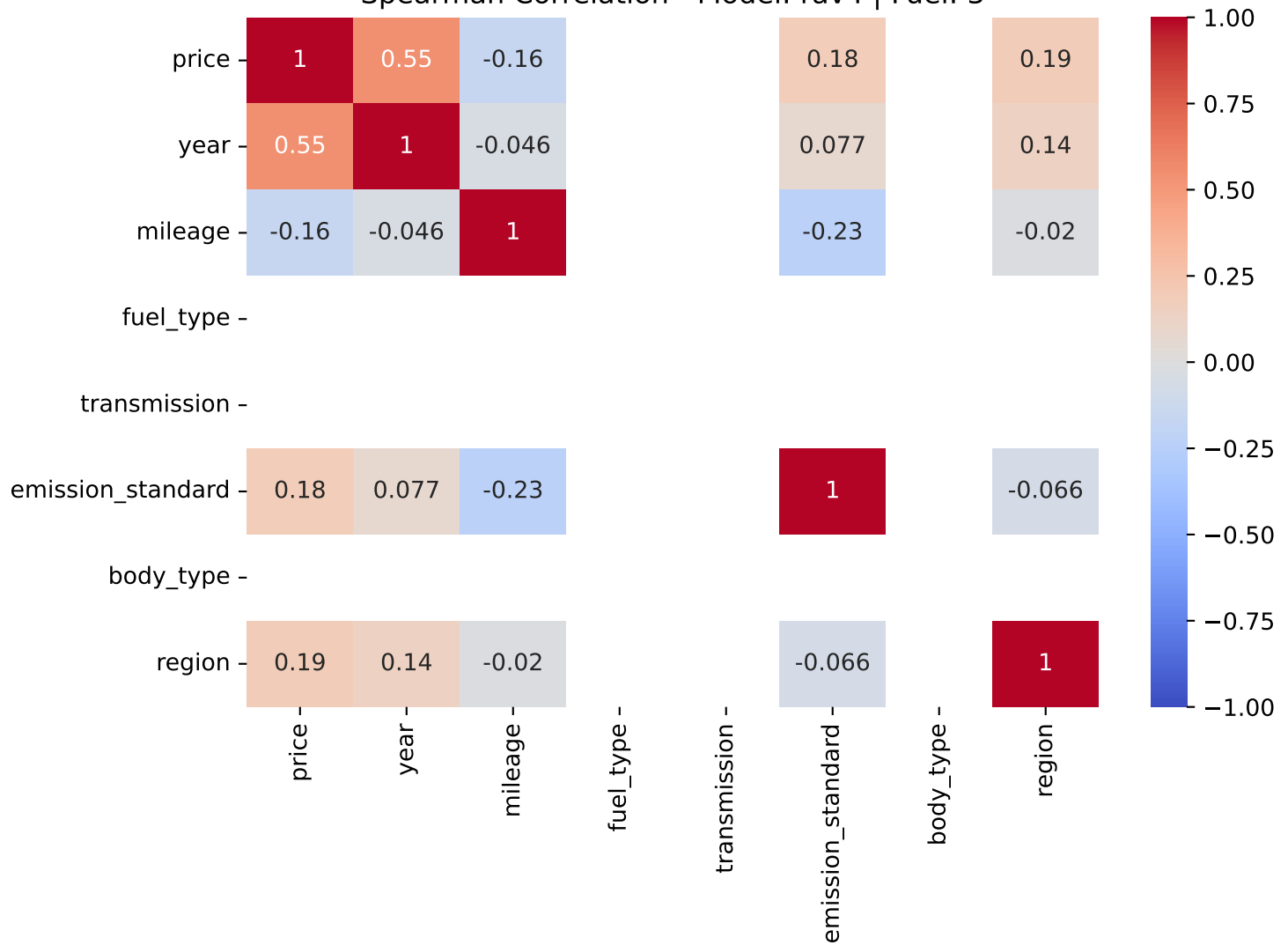
Spearman Correlation - Model: rav4 | Fuel: 3
