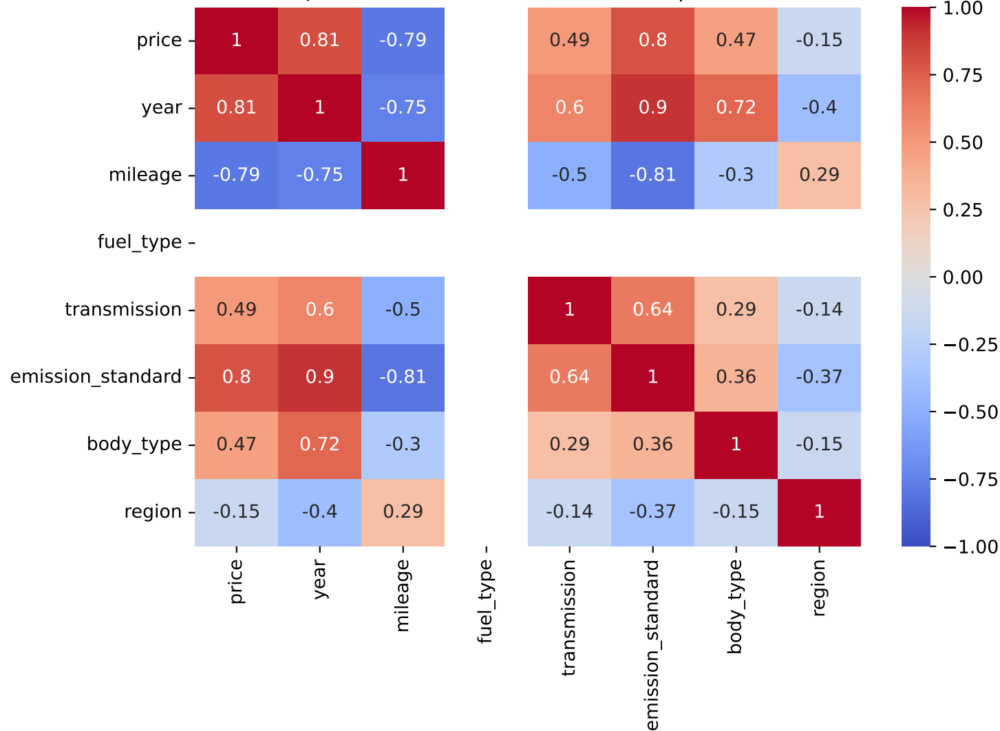
Spearman Correlation - Model: m3 | Fuel: 2
