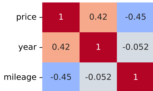
Pearson Correlation - Model: 207 | Fuel: 1
