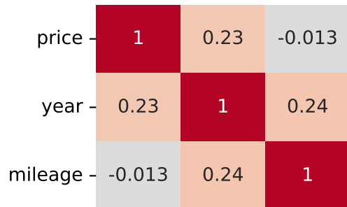
Pearson Correlation - Model: romeo 156 | Fuel: 1
