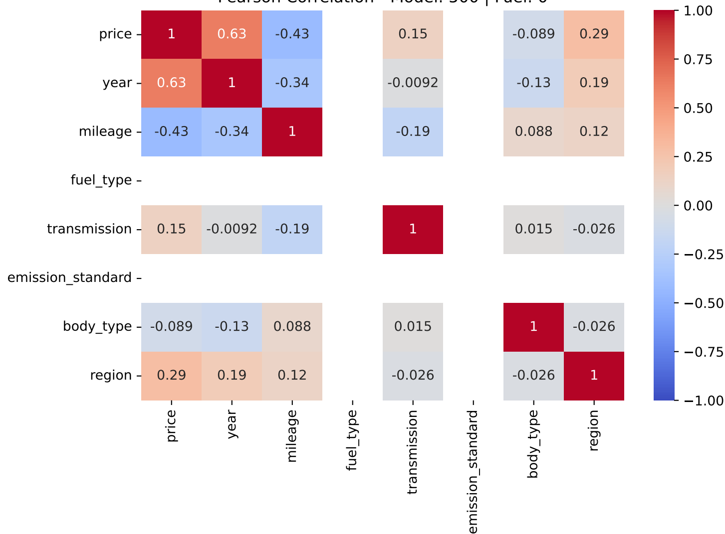
Pearson Correlation - Model: 500 | Fuel: 0
