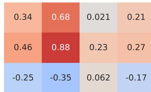
Pearson Correlation - Model: mondeo | Fuel: 1
