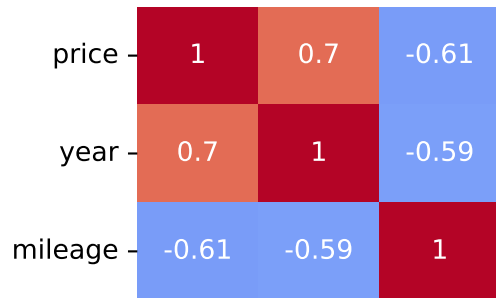
Spearman Correlation - Model: fiesta active | Fuel: 2
