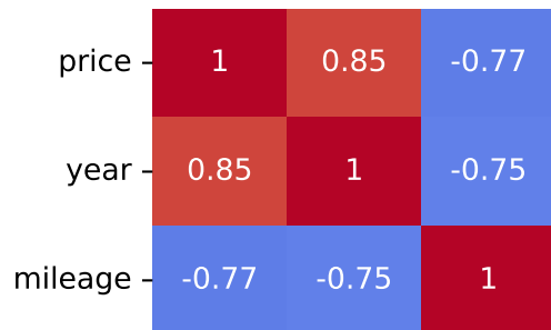
Spearman Correlation - Model: rs3 | Fuel: 2
