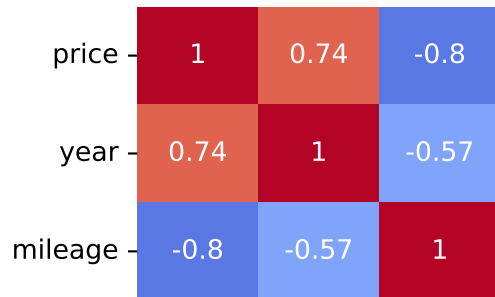
Pearson Correlation - Model: c4 cactus | Fuel: 1
