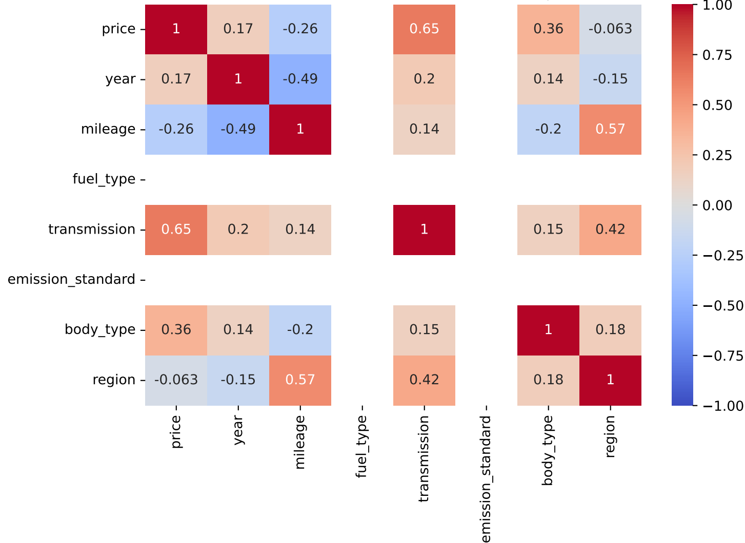
Spearman Correlation - Model: a1 citycarver | Fuel: 2
