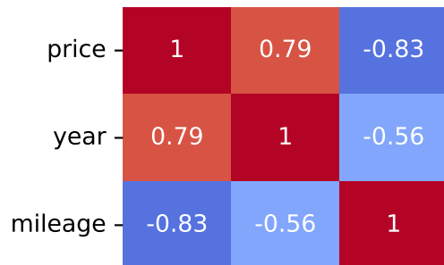
Pearson Correlation - Model: 500I | Fuel: 4
