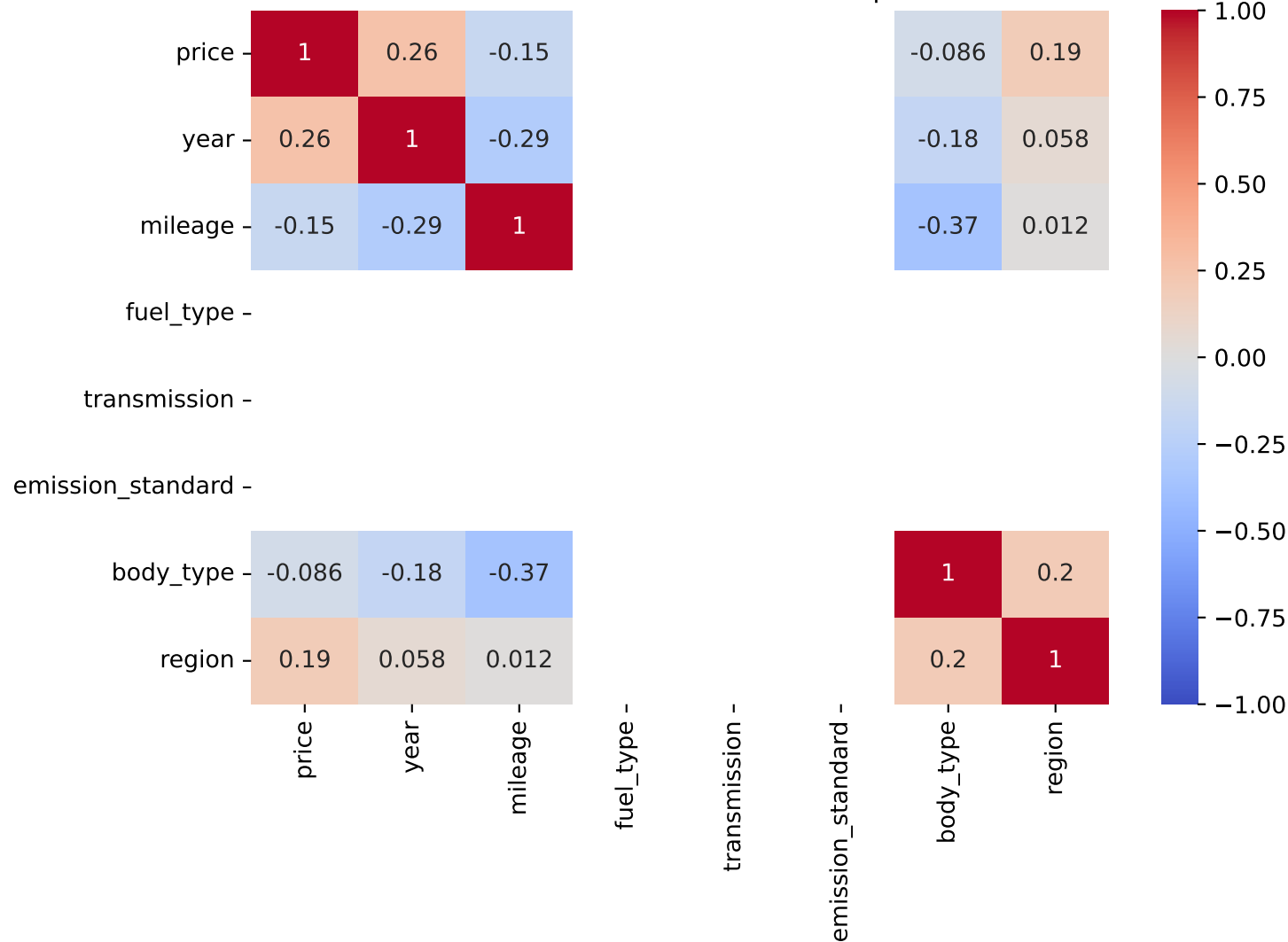
Pearson Correlation - Model: corsa | Fuel: 0
