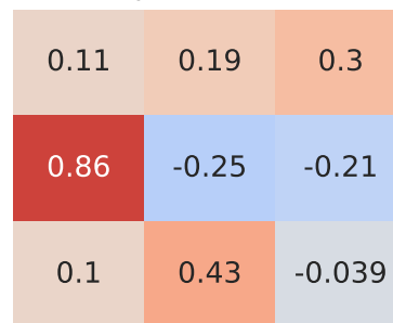
Pearson Correlation - Model: terrano | Fuel: 1
