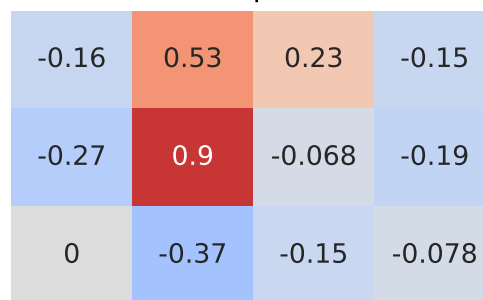
Spearman Correlation - Model: vivaro | Fuel: 1
