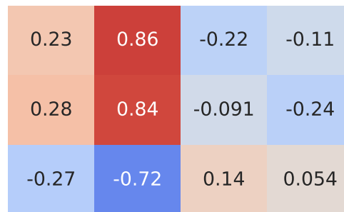
Spearman Correlation - Model: fabia | Fuel: 1
