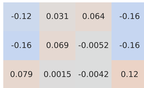
Spearman Correlation - Model: macan | Fuel: 2
