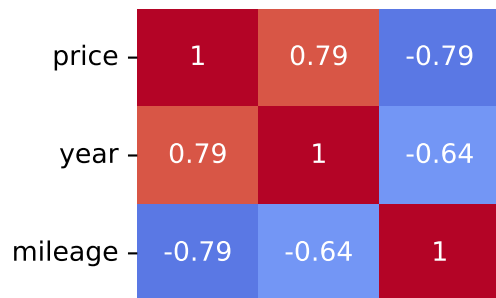
Spearman Correlation - Model: q2 | Fuel: 1
