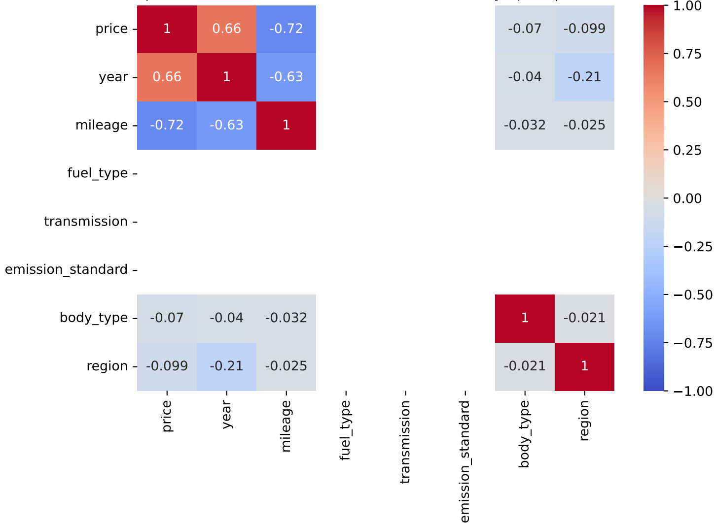
Spearman Correlation - Model: rover discovery sport | Fuel: 3
