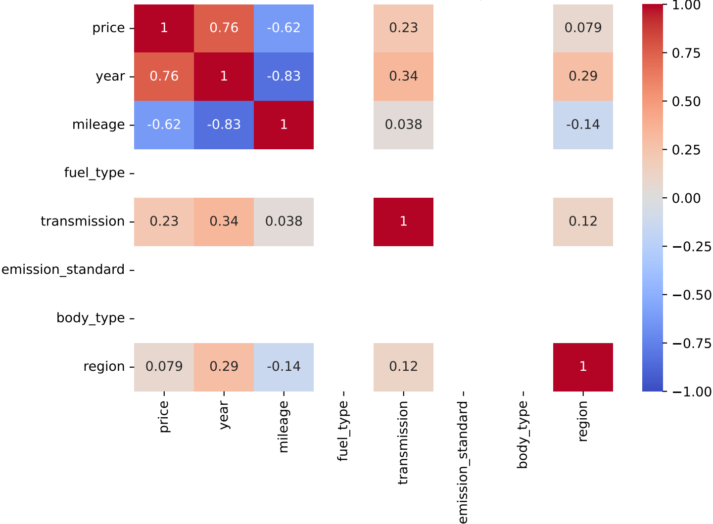
Spearman Correlation - Model: x2 | Fuel: 2
