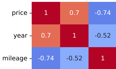
Spearman Correlation - Model: compass | Fuel: 1
