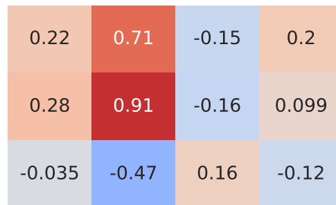
Pearson Correlation - Model: x-trail | Fuel: 1
