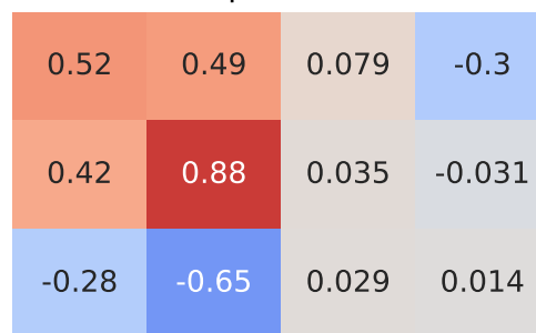
Pearson Correlation - Model: a3 | Fuel: 2
