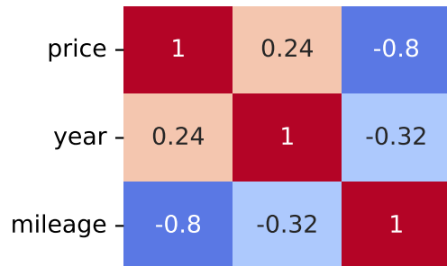
Pearson Correlation - Model: yeti | Fuel: 1
