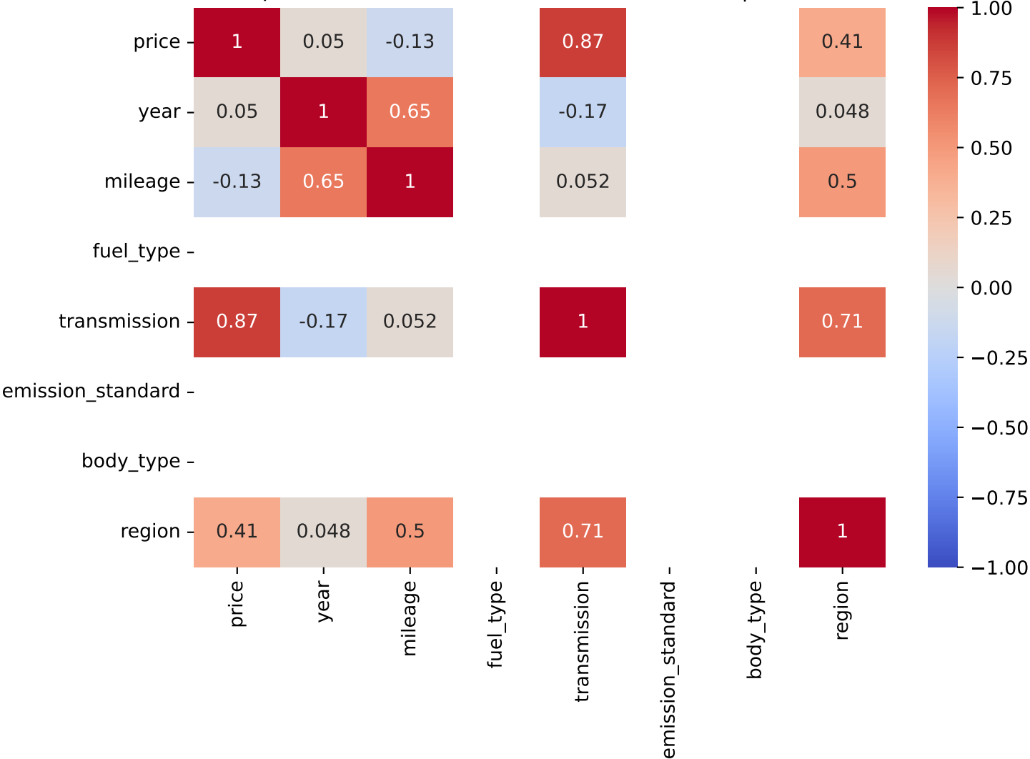
Spearman Correlation - Model: a1 allstreet | Fuel: 2
