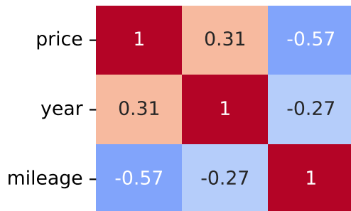
Spearman Correlation - Model: 206 | Fuel: 2
