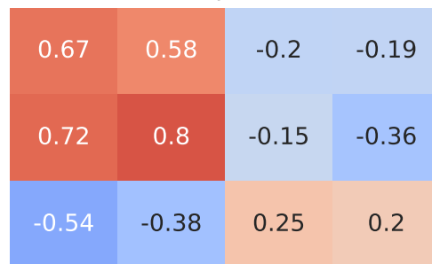
Spearman Correlation - Model: hilux | Fuel: 1
