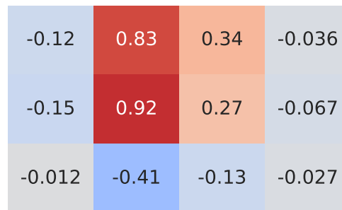
Spearman Correlation - Model: yaris | Fuel: 1
