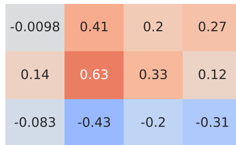
Pearson Correlation - Model: idea | Fuel: 1
