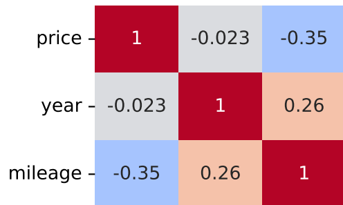
Pearson Correlation - Model: nemo | Fuel: 1
