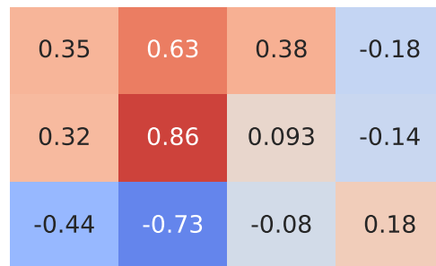
Spearman Correlation - Model: rover evoque | Fuel: 1
