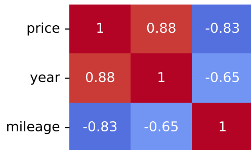
Pearson Correlation - Model: soul | Fuel: 1
