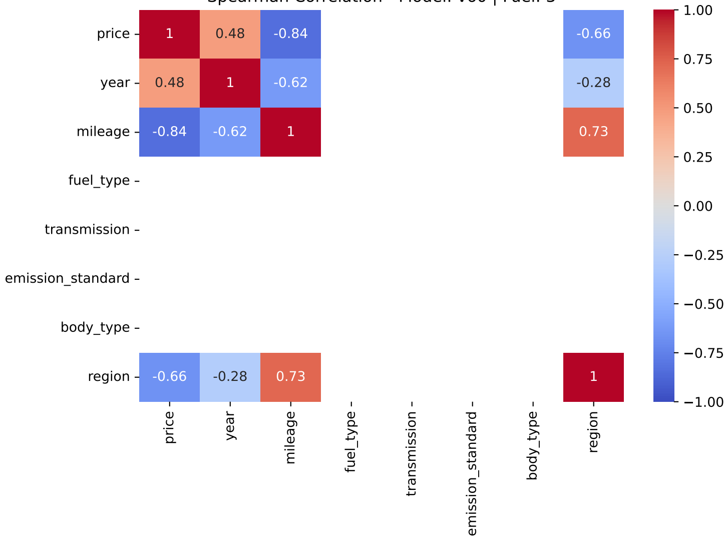
Spearman Correlation - Model: v60 | Fuel: 3
