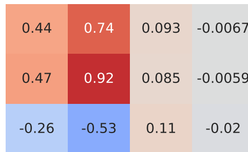
Pearson Correlation - Model: passat | Fuel: 1
