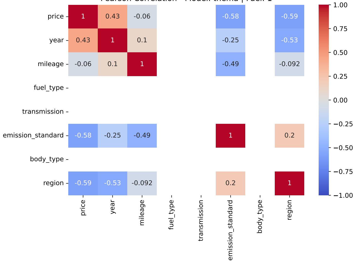
Pearson Correlation - Model: thema | Fuel: 1
