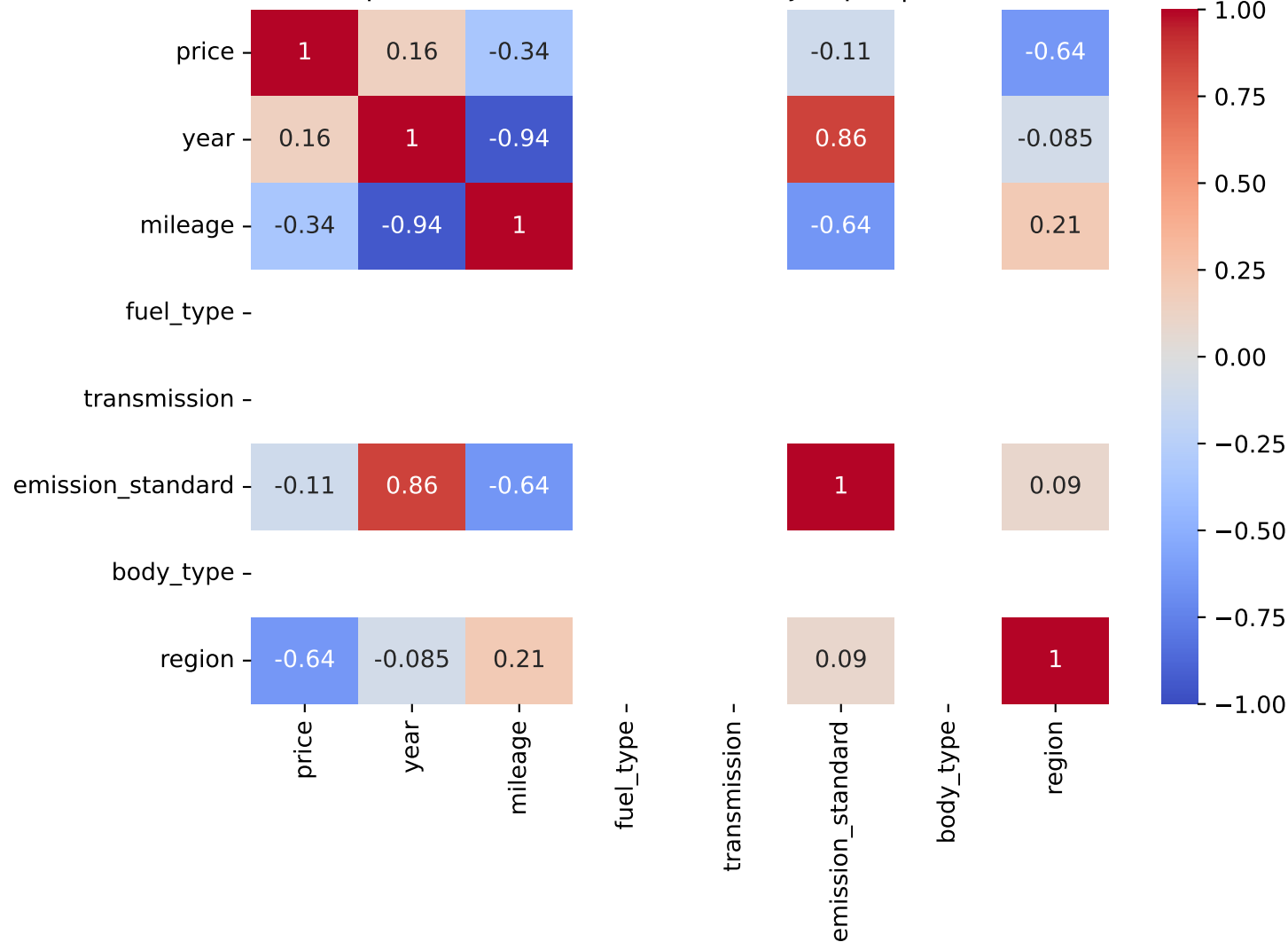
Spearman Correlation - Model: jumper | Fuel: 1
