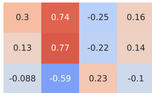
Spearman Correlation - Model: qashqai | Fuel: 2
