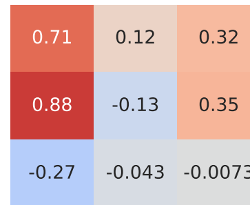
Pearson Correlation - Model: c3 picasso | Fuel: 2
