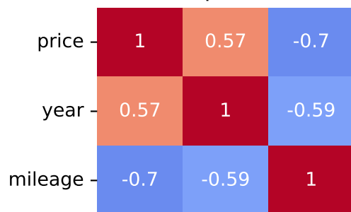
Spearman Correlation - Model: idea | Fuel: 1
