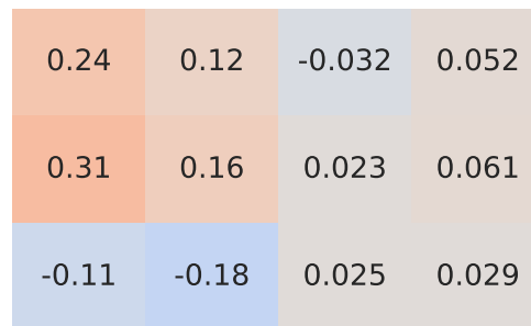
Pearson Correlation - Model: c5 aircross | Fuel: 1
