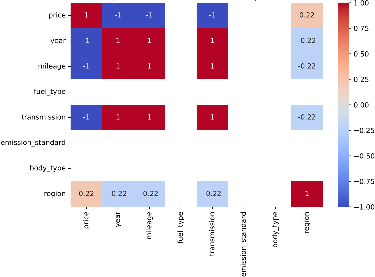
Spearman Correlation - Model: v40 | Fuel: 2
