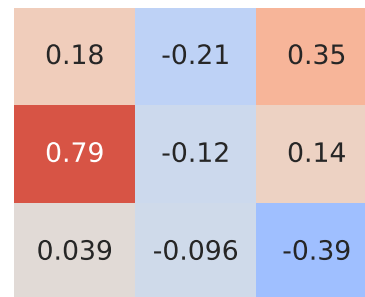
Pearson Correlation - Model: splash | Fuel: 2
