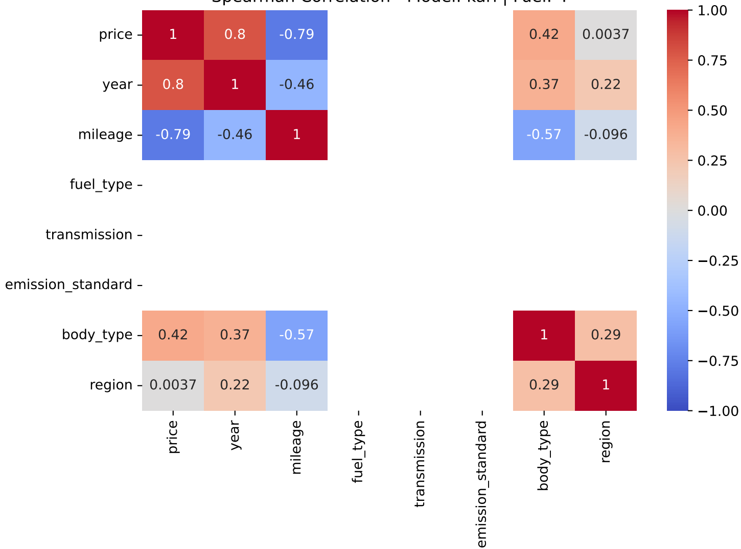
Spearman Correlation - Model: karl | Fuel: 4
