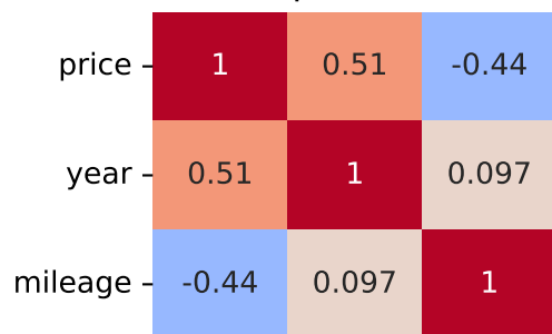
Spearman Correlation - Model: amarak | Fuel: 1
