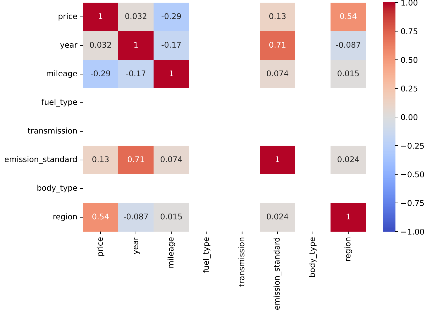
Pearson Correlation - Model: c30 | Fuel: 1
