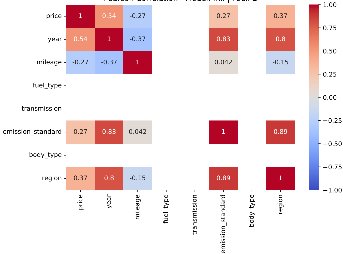
Pearson Correlation - Model: mii | Fuel: 2
