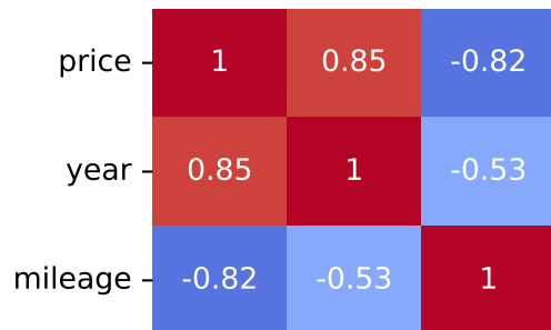
Pearson Correlation - Model: rio | Fuel: 2
