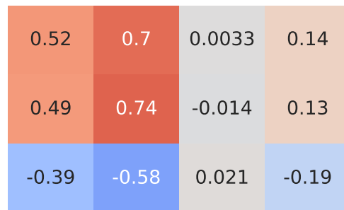
Spearman Correlation - Model: a3 | Fuel: 1
