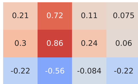
Spearman Correlation - Model: transit connect | Fuel: 1
