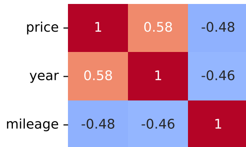
Spearman Correlation - Model: arkana | Fuel: 3
