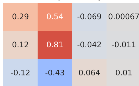
Spearman Correlation - Model: rover range rover | Fuel: 1
