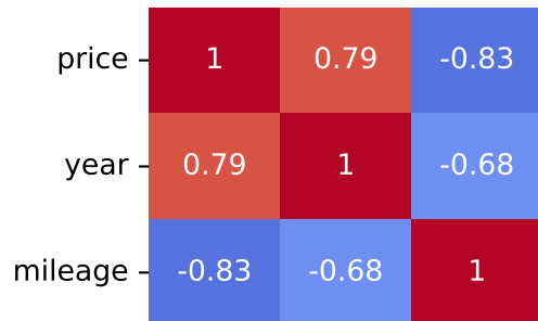
Pearson Correlation - Model: c-max | Fuel: 2
