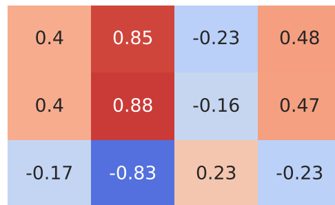
Spearman Correlation - Model: berlingo | Fuel: 2
