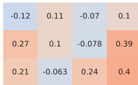
Pearson Correlation - Model: romeo tonale | Fuel: 3
