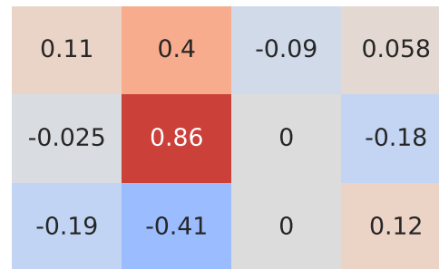
Spearman Correlation - Model: antara | Fuel: 1
