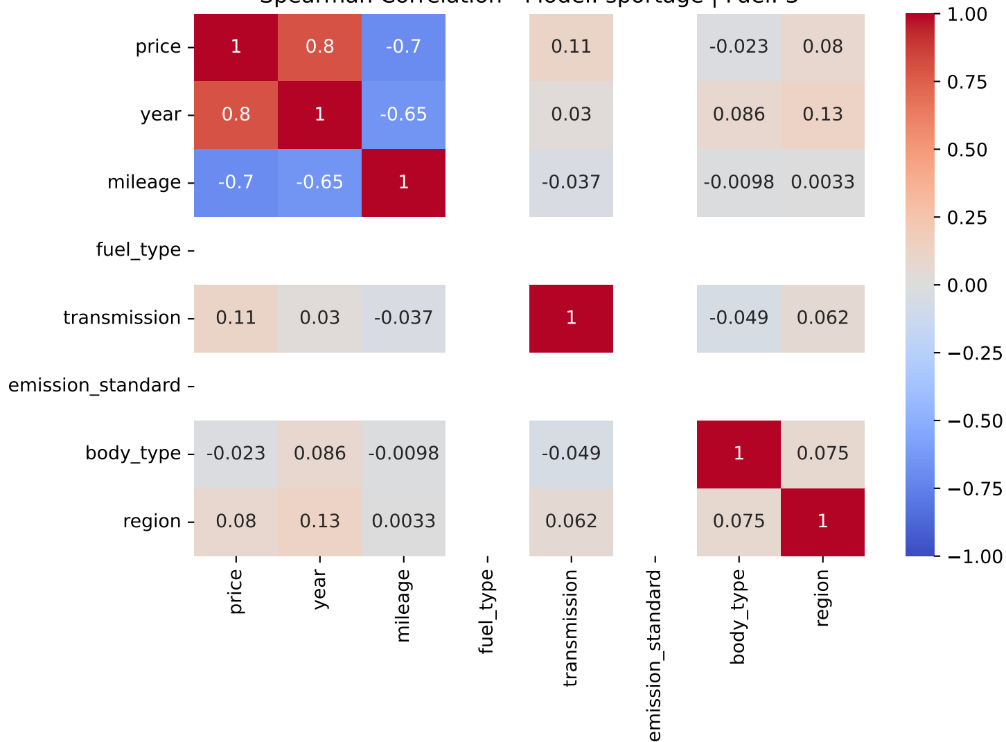
Spearman Correlation - Model: sportage | Fuel: 3
