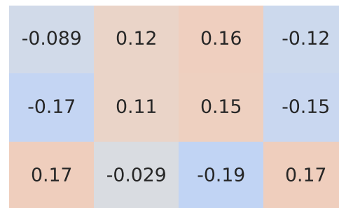
Spearman Correlation - Model: mokka | Fuel: 4
