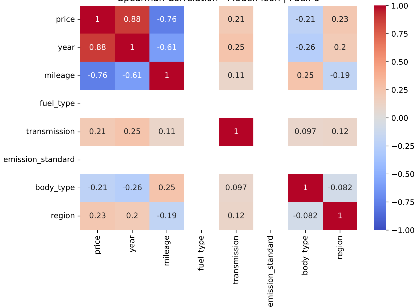
Spearman Correlation - Model: leon | Fuel: 5
