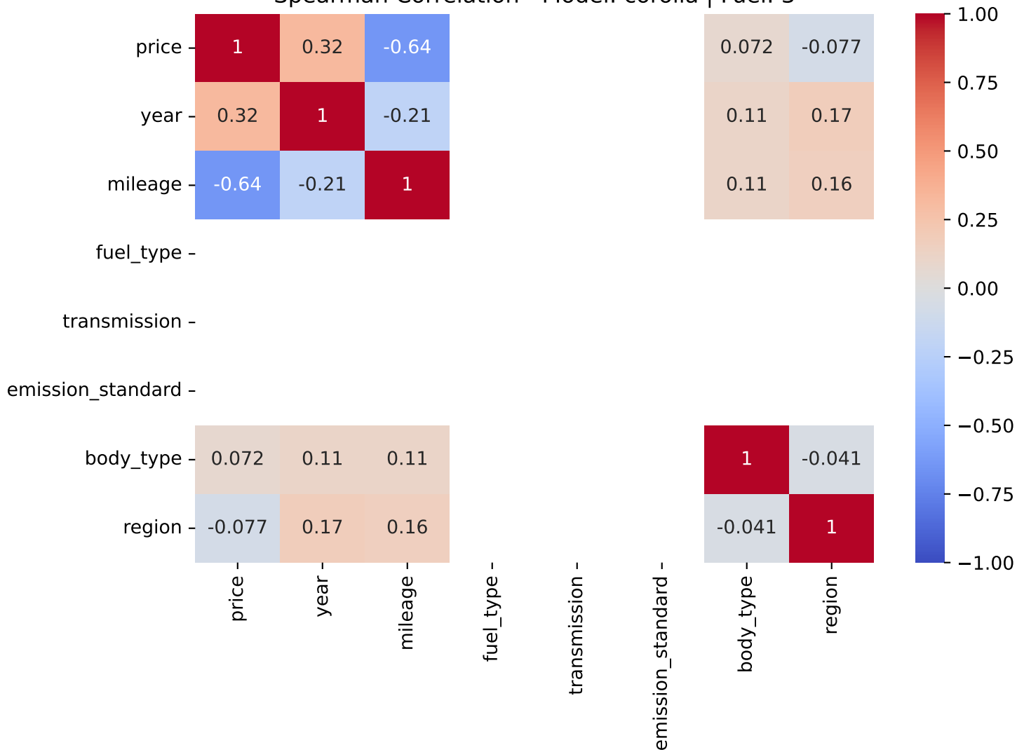
Spearman Correlation - Model: corolla | Fuel: 3
