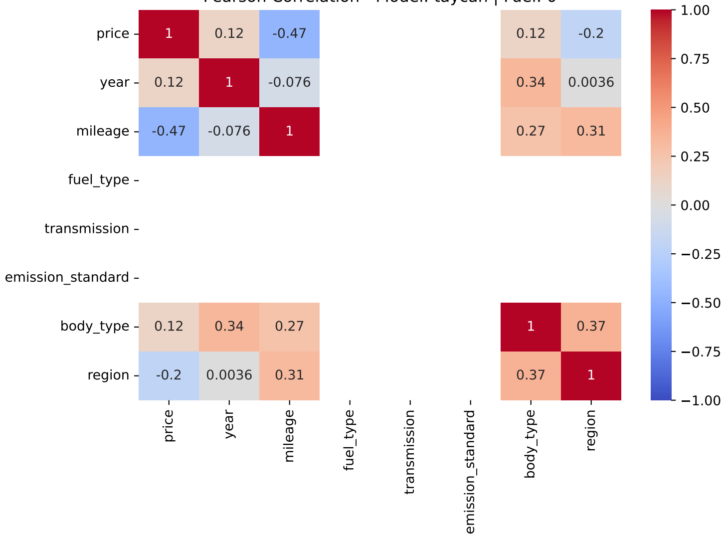
Pearson Correlation - Model: taycan | Fuel: 0
