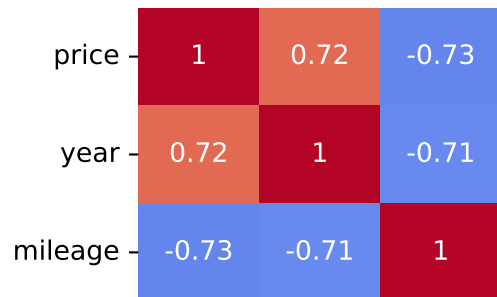
Pearson Correlation - Model: leon | Fuel: 2
