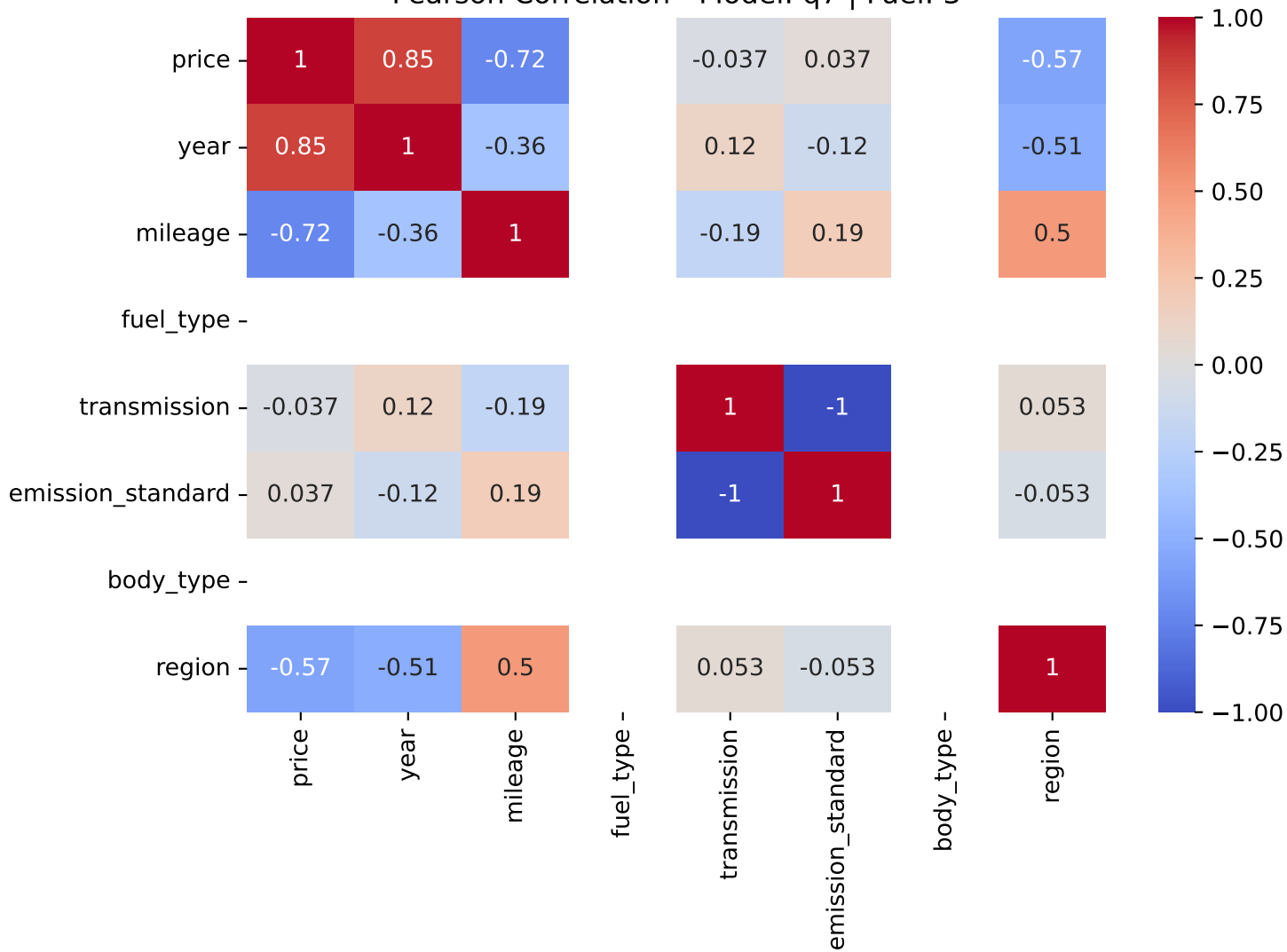
Pearson Correlation - Model: q7 | Fuel: 3
