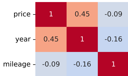
Spearman Correlation - Model: multipa | Fuel: 1
