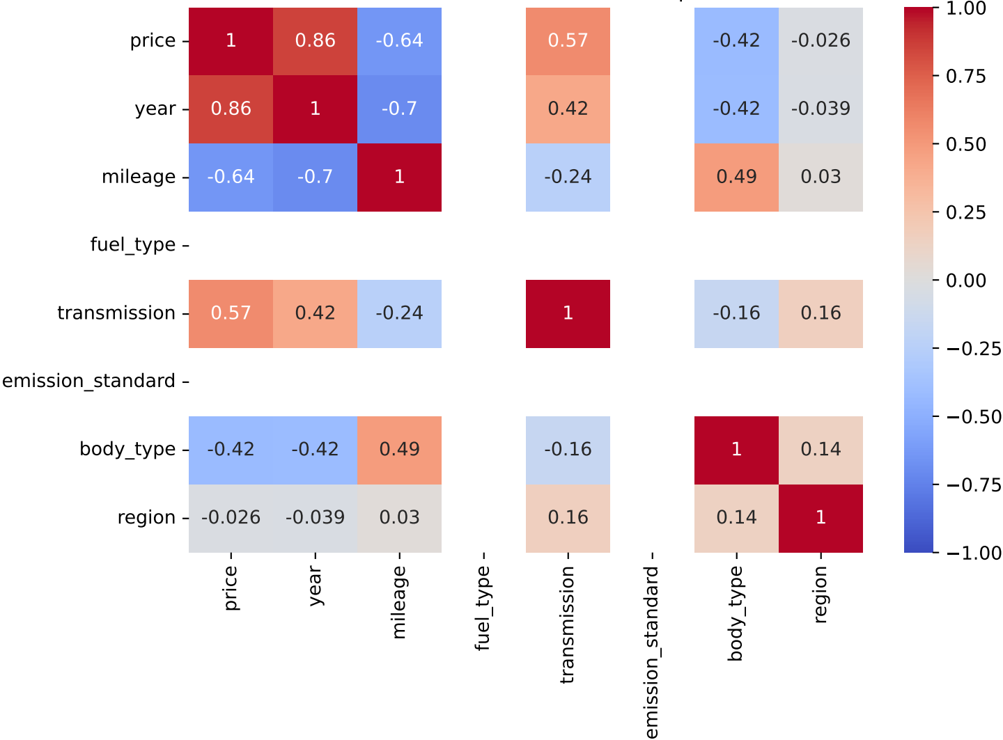
Pearson Correlation - Model: ateca | Fuel: 2
