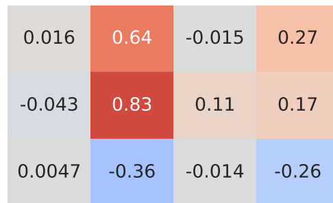
Pearson Correlation - Model: qubo | Fuel: 1
