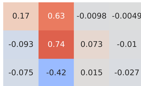
Spearman Correlation - Model: sportage | Fuel: 4
