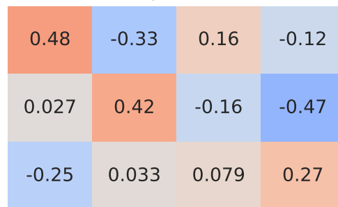
Pearson Correlation - Model: 307 | Fuel: 2
