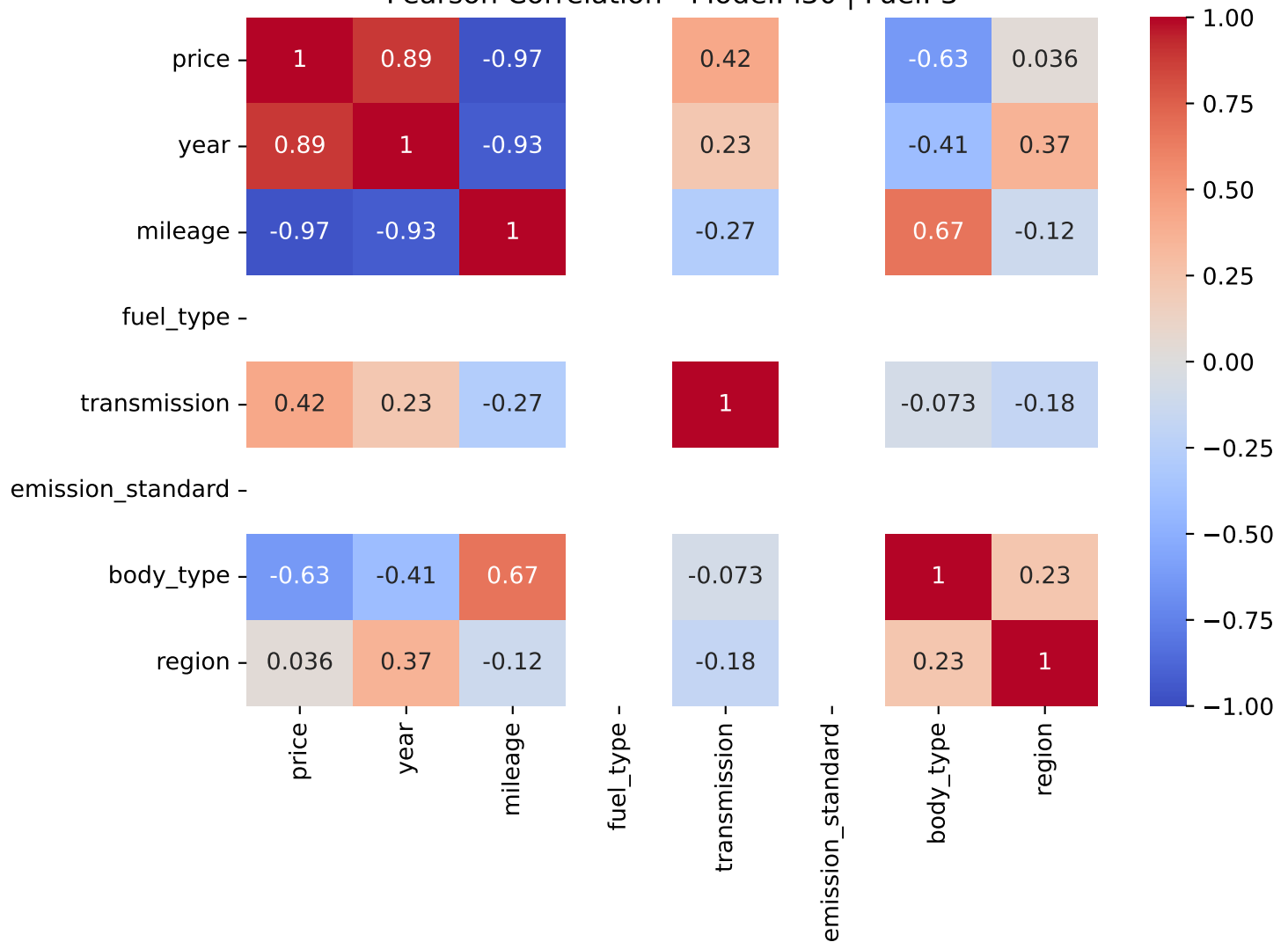
Pearson Correlation - Model: i30 | Fuel: 3
