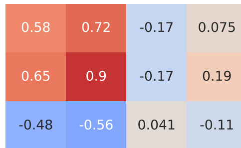
Pearson Correlation - Model: cooper s | Fuel: 2
