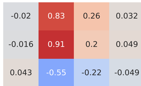
Spearman Correlation - Model: corsa | Fuel: 1
