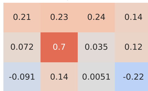
Pearson Correlation - Model: 207 | Fuel: 2
