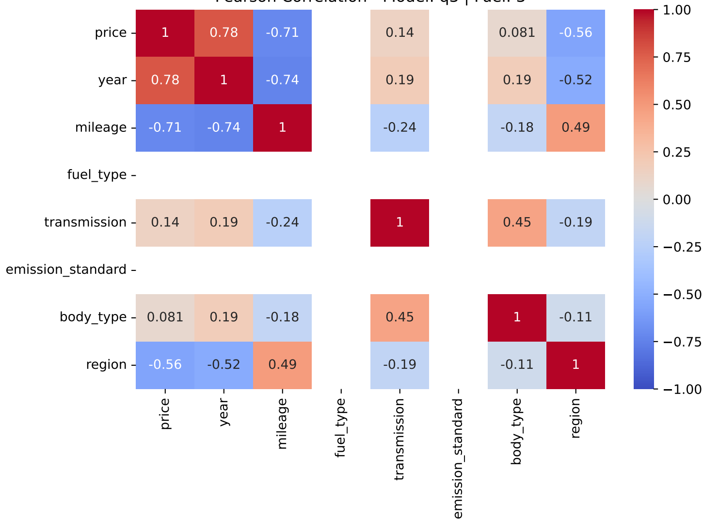
Pearson Correlation - Model: q3 | Fuel: 3
