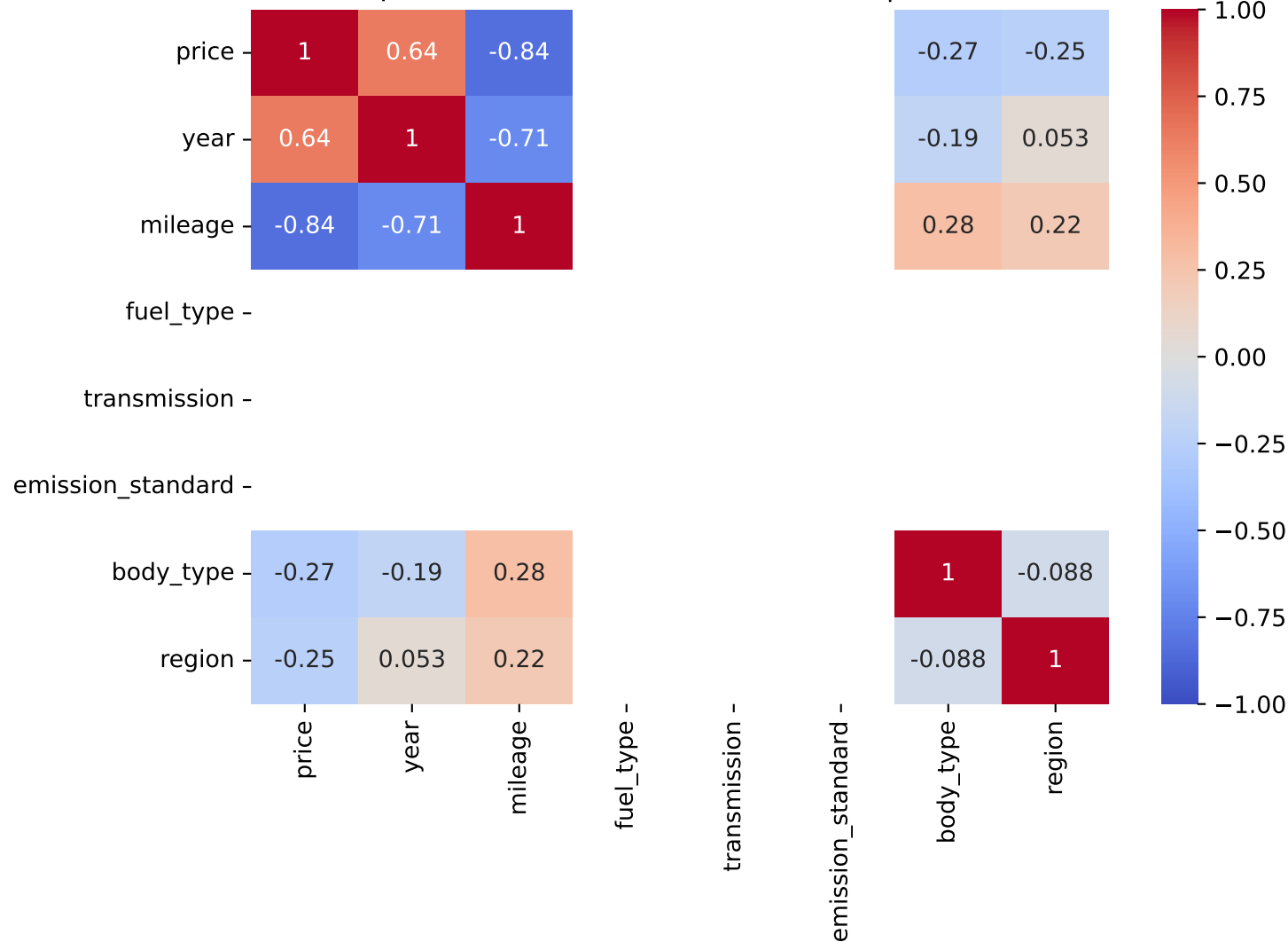
Spearman Correlation - Model: 3008 | Fuel: 3
