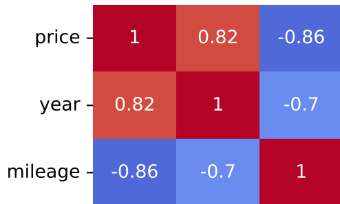
Spearman Correlation - Model: up | Fuel: 5
