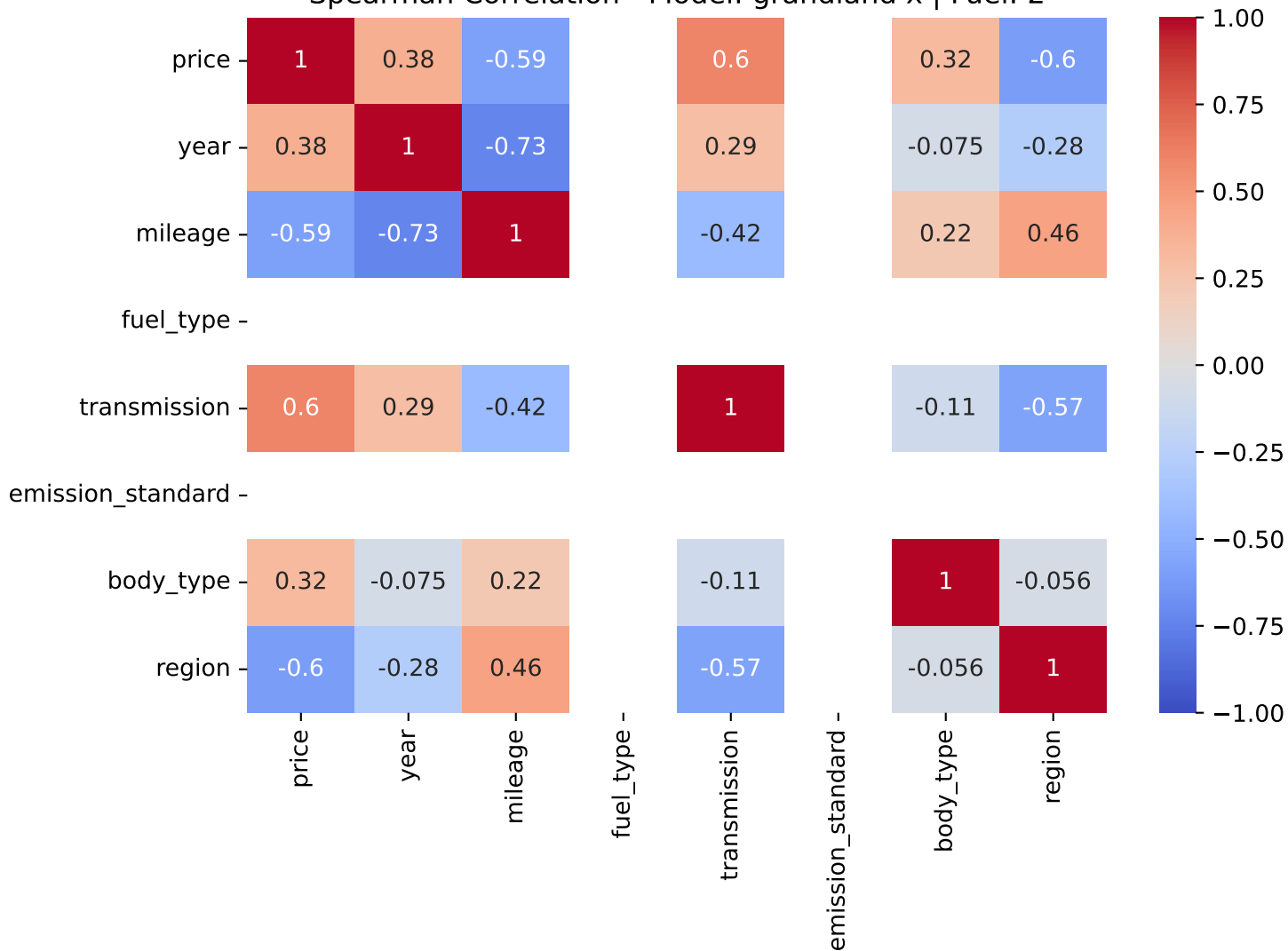
Spearman Correlation - Model: grandland x | Fuel: 2
