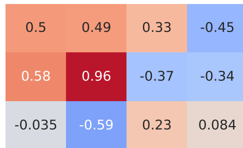
Pearson Correlation - Model: a6 | Fuel: 2
