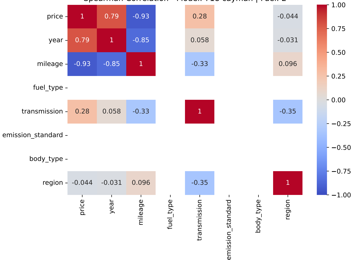
Spearman Correlation - Model: 718 cayman | Fuel: 2
