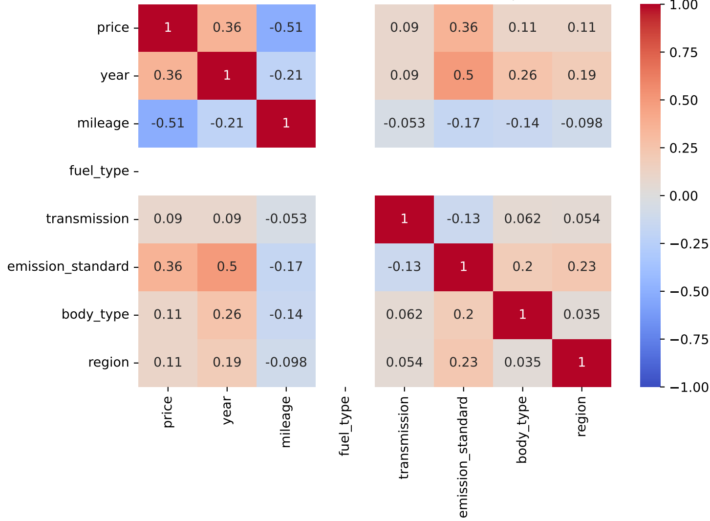
Spearman Correlation - Model: romeo 159 | Fuel: 1
