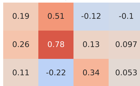
Spearman Correlation - Model: c5 | Fuel: 1
