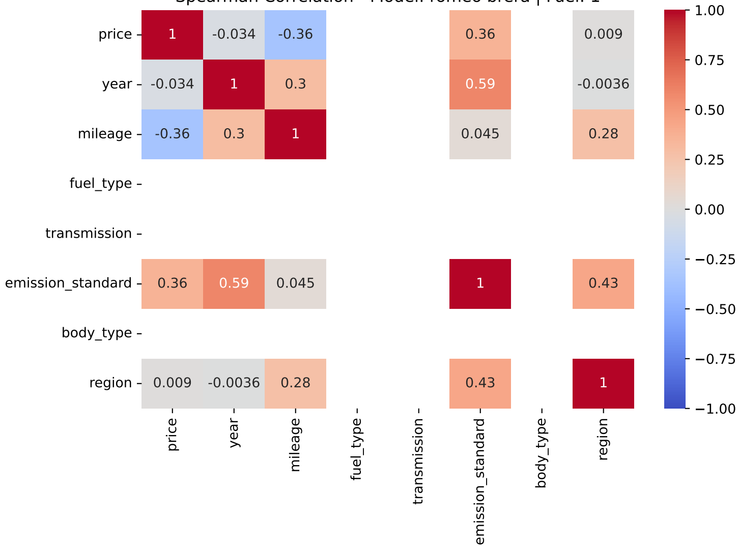
Spearman Correlation - Model: romeo brera | Fuel: 1
