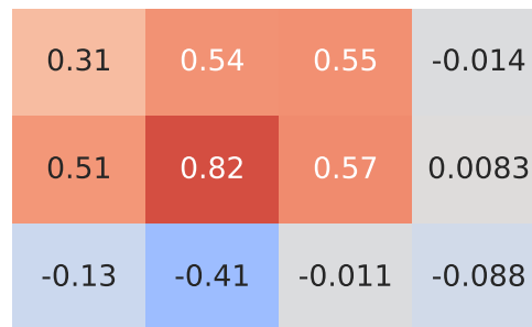
Pearson Correlation - Model: s3 | Fuel: 2
