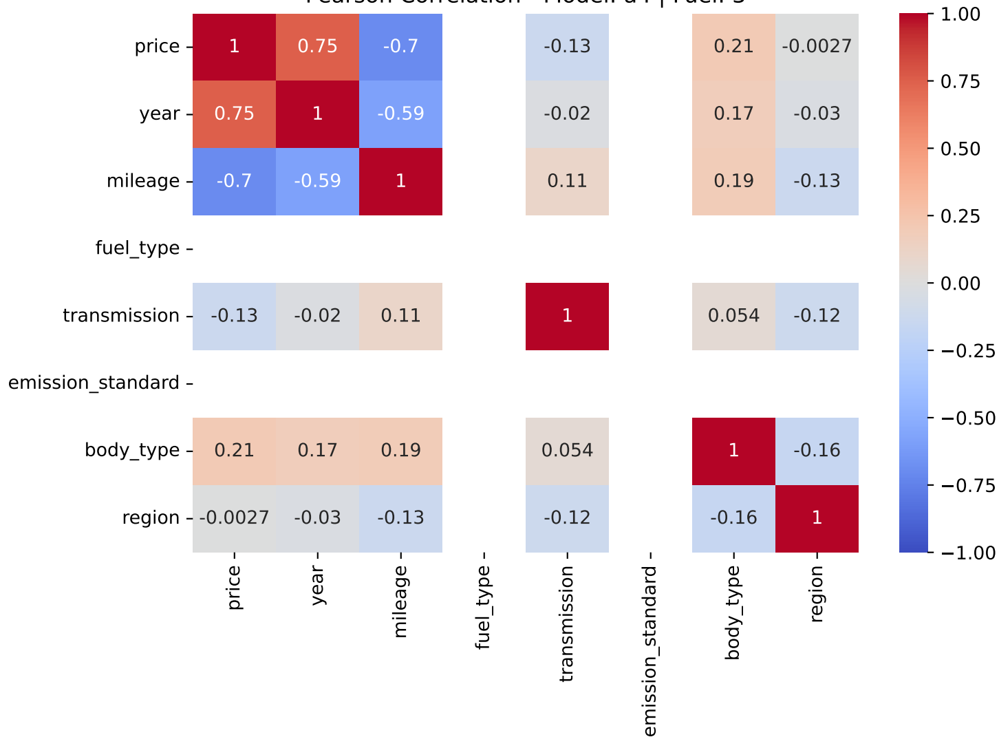
Pearson Correlation - Model: a4 | Fuel: 3
