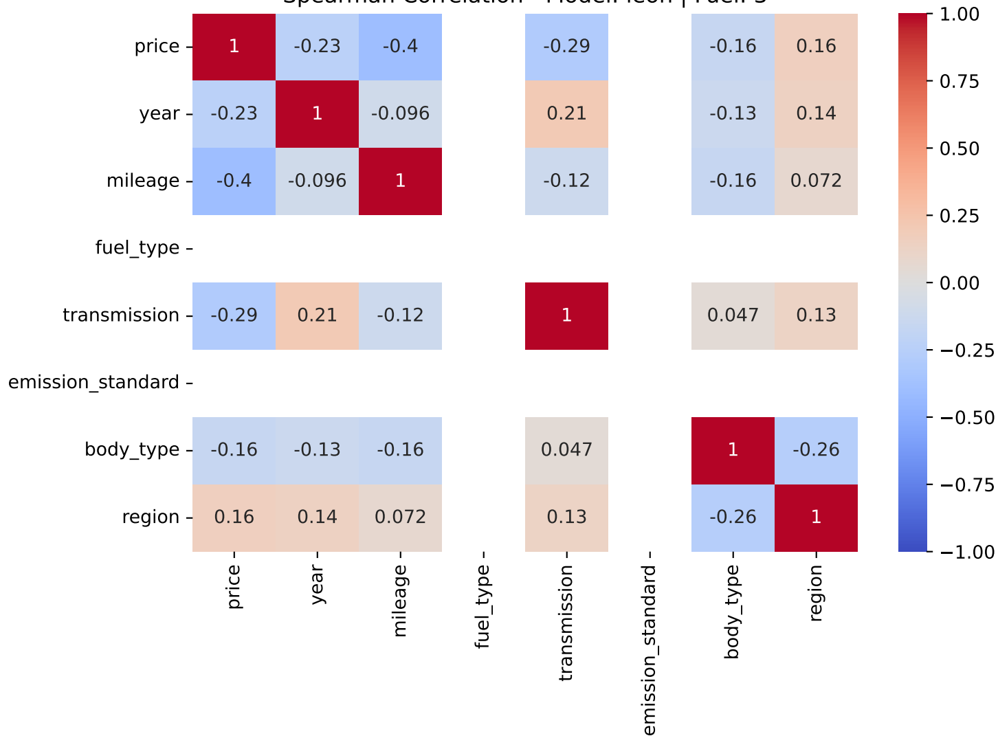
Spearman Correlation - Model: leon | Fuel: 3
