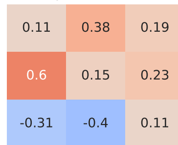
Pearson Correlation - Model: bravo | Fuel: 4
