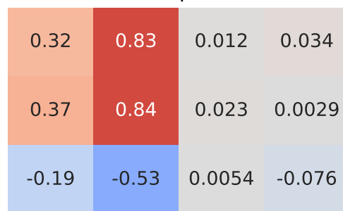
Spearman Correlation - Model: scenic | Fuel: 1
