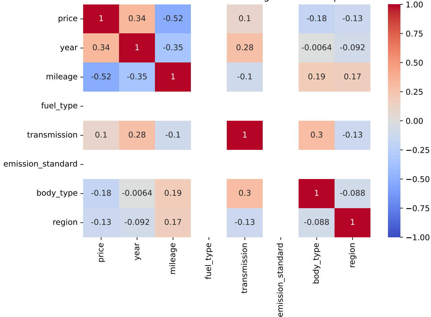
Pearson Correlation - Model: rover range rover velar | Fuel: 1
