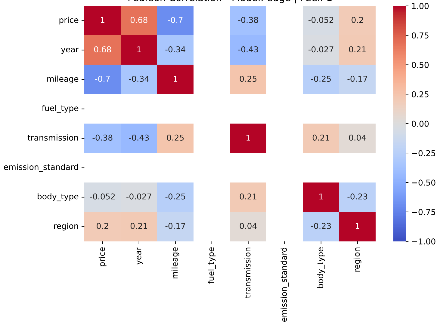
Pearson Correlation - Model: edge | Fuel: 1
