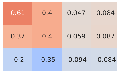
Spearman Correlation - Model: forfour | Fuel: 2
