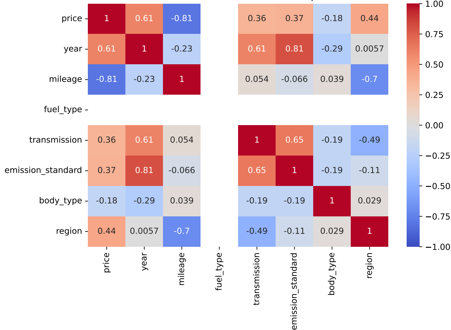
Pearson Correlation - Model: amarok | Fuel: 1
