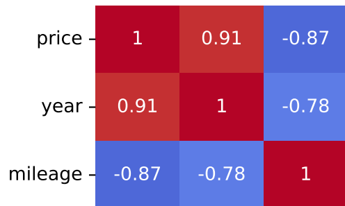
Pearson Correlation - Model: 508 | Fuel: 1
