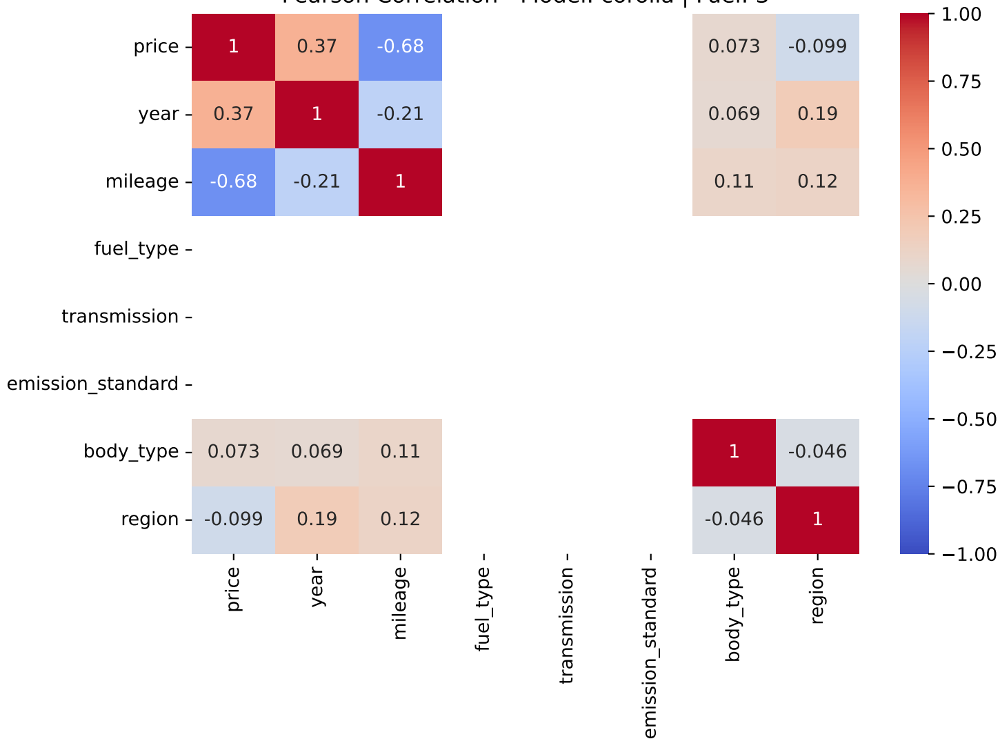
Pearson Correlation - Model: corolla | Fuel: 3
