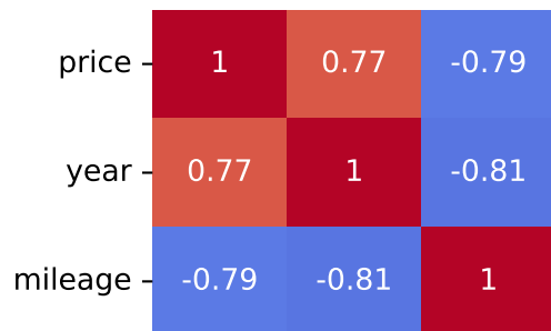
Spearman Correlation - Model: q8 | Fuel: 3
