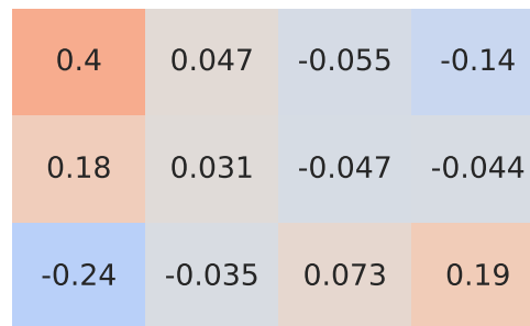
Spearman Correlation - Model: x2 | Fuel: 1
