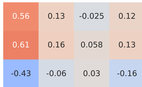
Spearman Correlation - Model: golf | Fuel: 5
