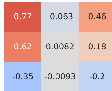
Spearman Correlation - Model: ix20 | Fuel: 2
