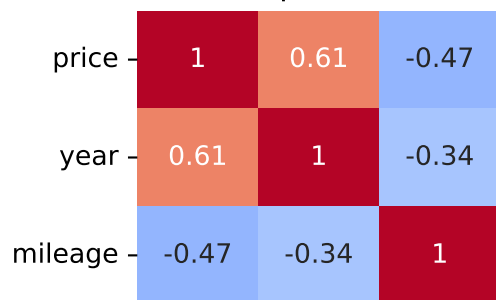
Spearman Correlation - Model: musa | Fuel: 1
