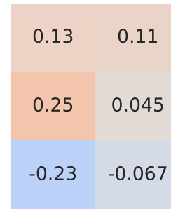
Spearman Correlation - Model: countryman | Fuel: 3
