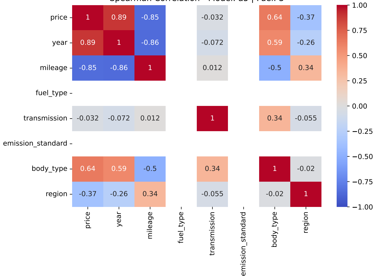
Spearman Correlation - Model: a5 | Fuel: 3
