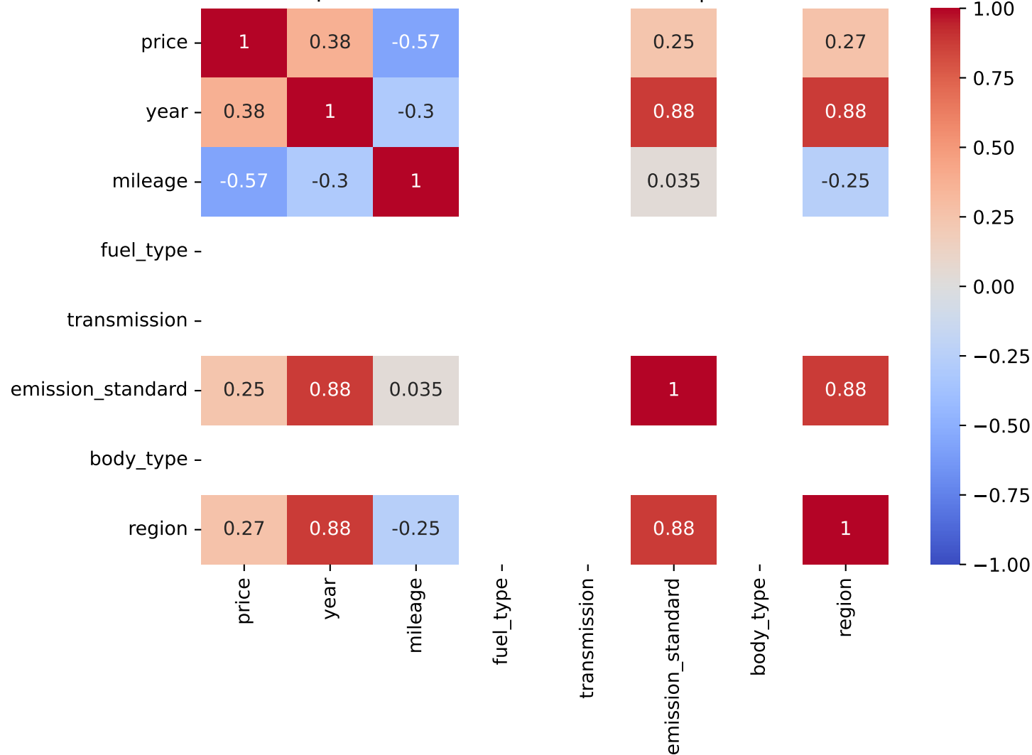
Spearman Correlation - Model: mii | Fuel: 2
