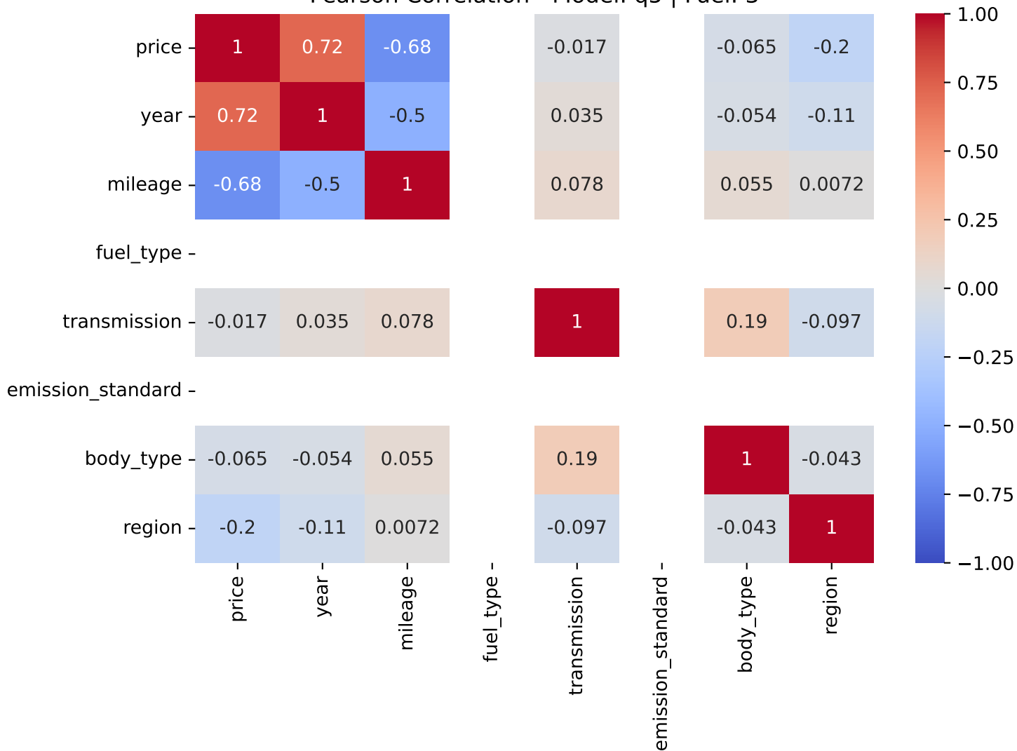
Pearson Correlation - Model: q5 | Fuel: 3
