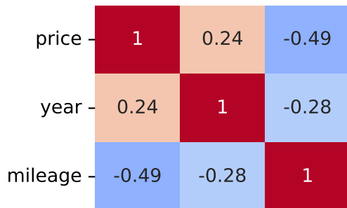
Pearson Correlation - Model: romeo 159 | Fuel: 1
