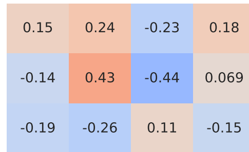
Pearson Correlation - Model: c4 cactus | Fuel: 1
