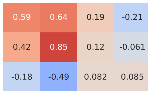
Pearson Correlation - Model: one | Fuel: 1
