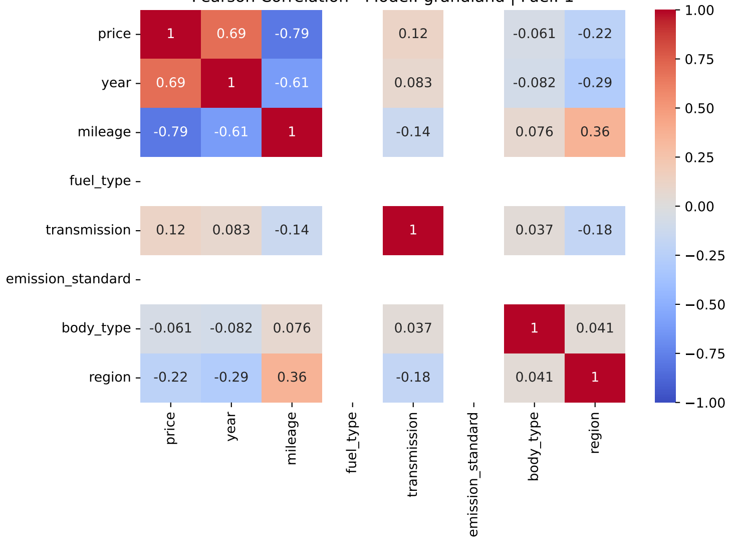
Pearson Correlation - Model: grandland | Fuel: 1
