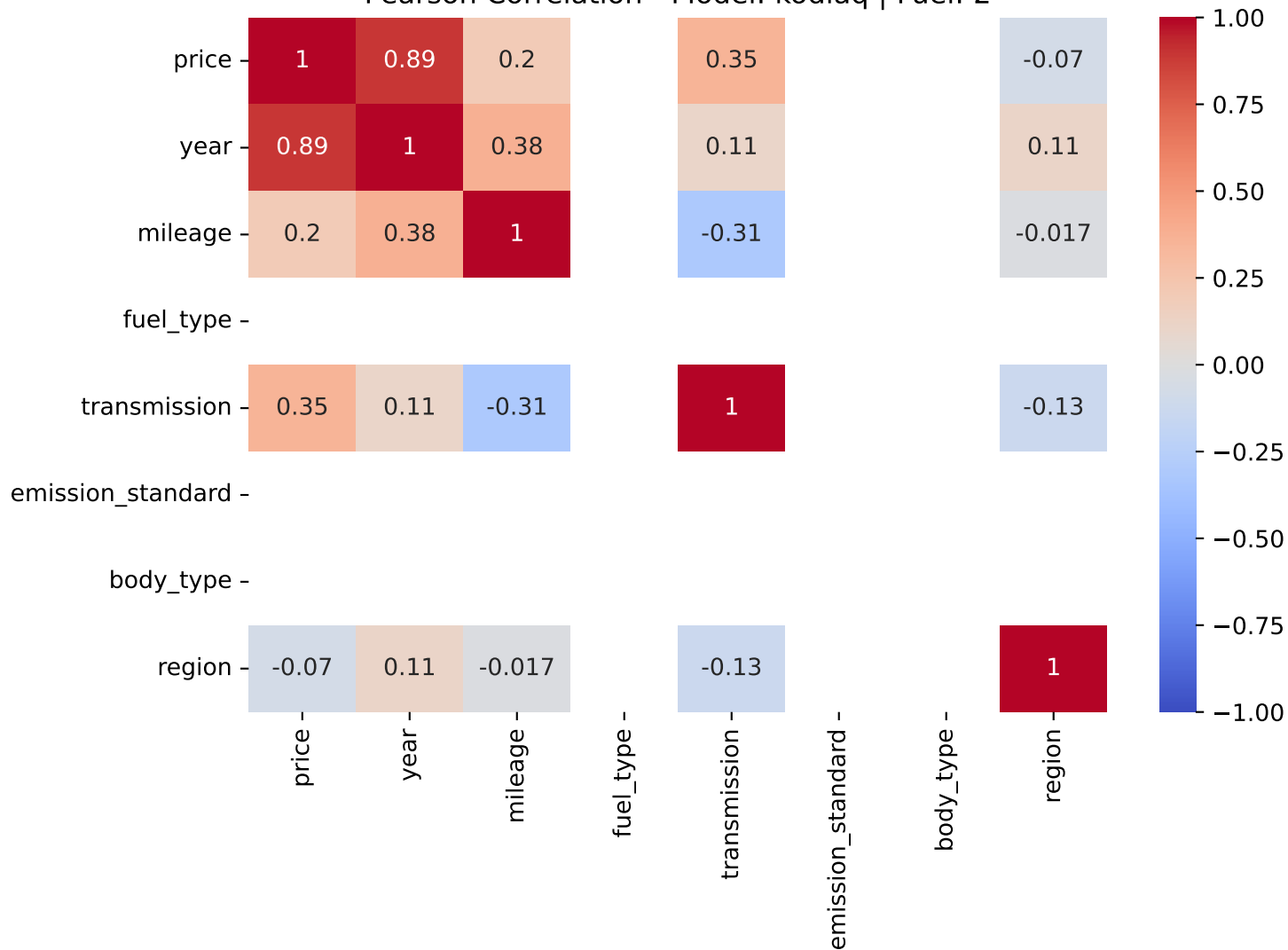
Pearson Correlation - Model: kodiaq | Fuel: 2
