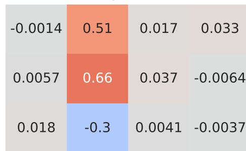
Pearson Correlation - Model: 500I | Fuel: 1
