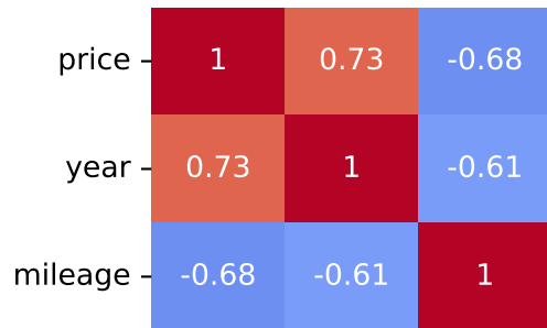
Spearman Correlation - Model: focus | Fuel: 2
