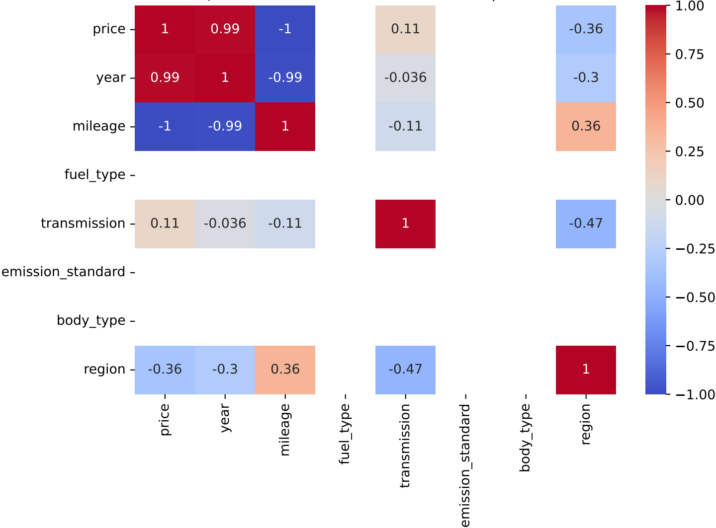
Spearman Correlation - Model: scala | Fuel: 1
