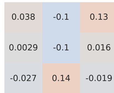
Pearson Correlation - Model: panda | Fuel: 3
