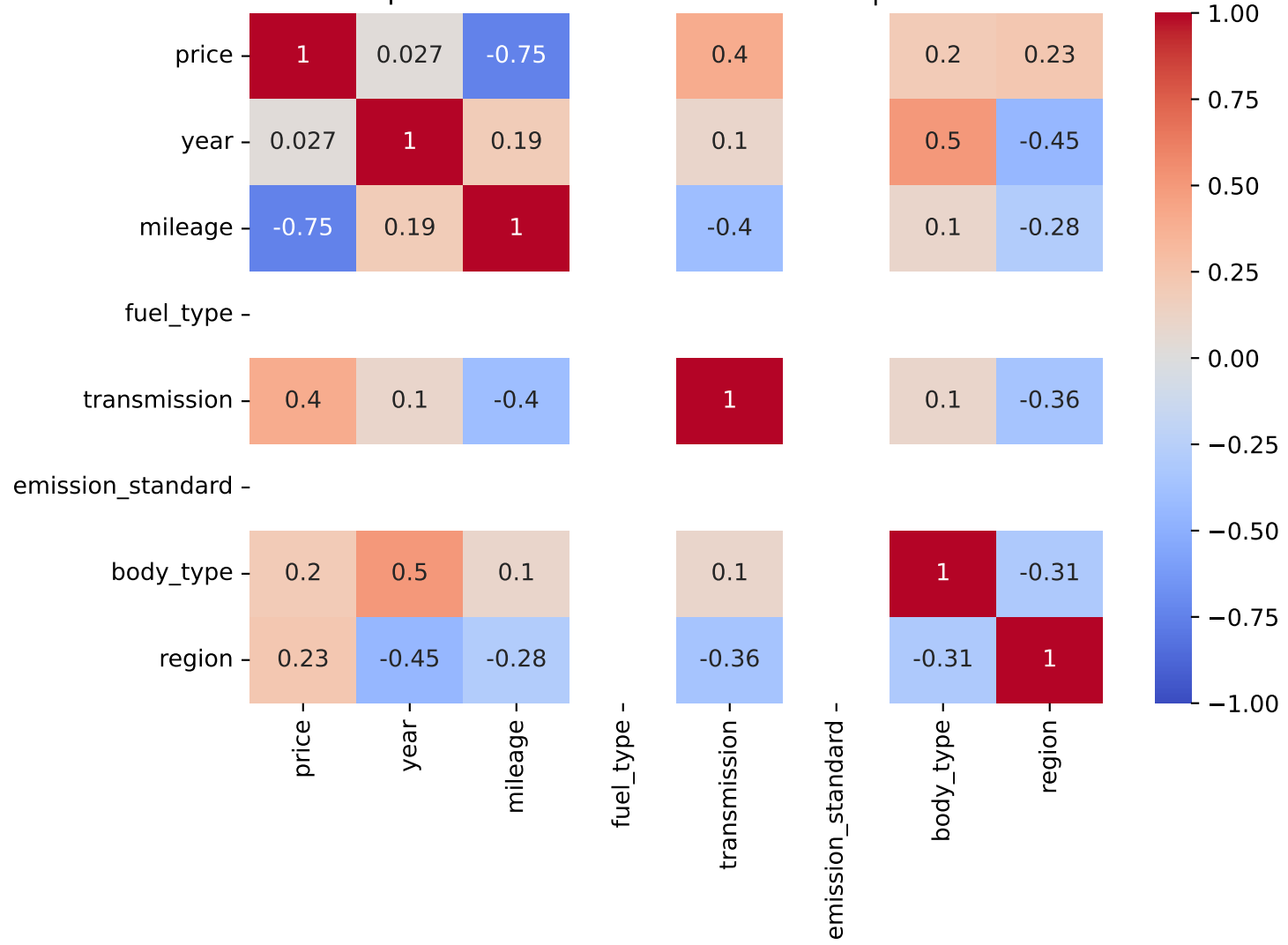
Spearman Correlation - Model: v90 | Fuel: 1
