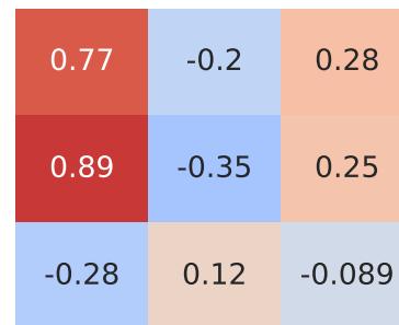
Spearman Correlation - Model: q7 | Fuel: 1
