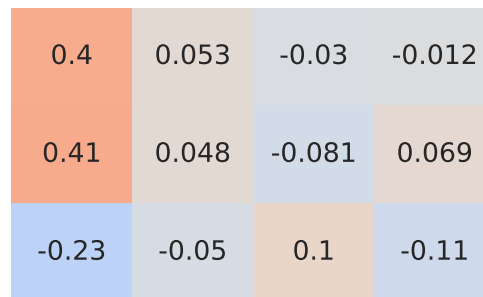
Pearson Correlation - Model: q2 | Fuel: 1
