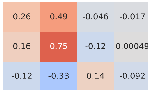
Pearson Correlation - Model: a1 | Fuel: 1
