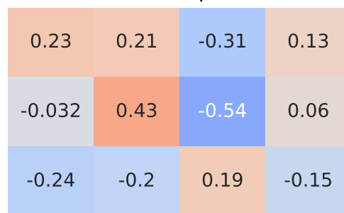
Spearman Correlation - Model: c4 cactus | Fuel: 1
