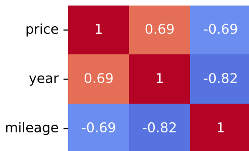
Pearson Correlation - Model: a3 | Fuel: 2
