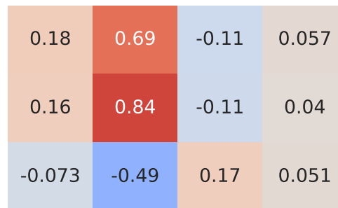
Pearson Correlation - Model: x5 | Fuel: 1
