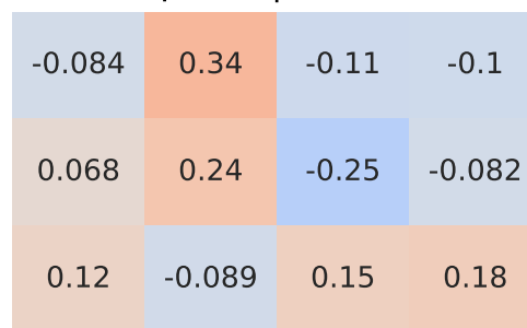
Spearman Correlation - Model: puma | Fuel: 2
