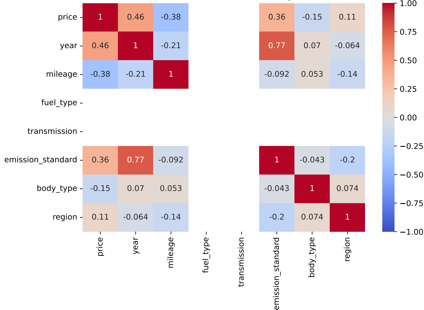
Pearson Correlation - Model: sedici | Fuel: 1
