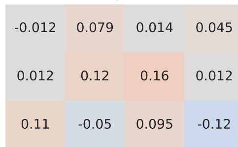
Spearman Correlation - Model: tipo | Fuel: 1
