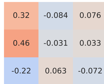
Pearson Correlation - Model: ecosport | Fuel: 1
