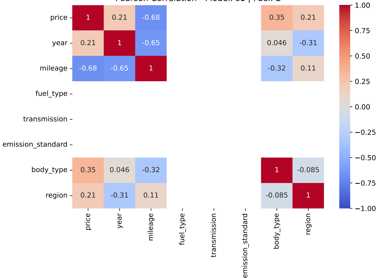
Pearson Correlation - Model: s1 | Fuel: 2
