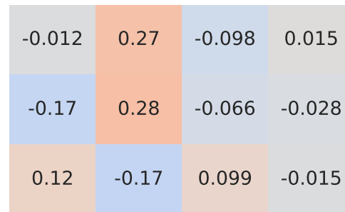
Pearson Correlation - Model: renegade | Fuel: 1
