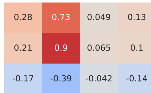
Pearson Correlation - Model: polo | Fuel: 1
