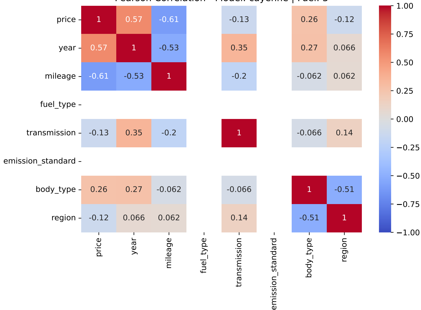
Pearson Correlation - Model: cayenne | Fuel: 3
