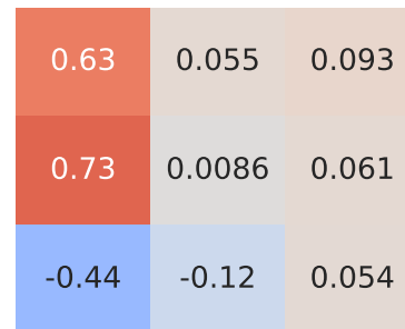
Spearman Correlation - Model: ix20 | Fuel: 4
