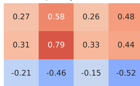
Pearson Correlation - Model: superb | Fuel: 1
