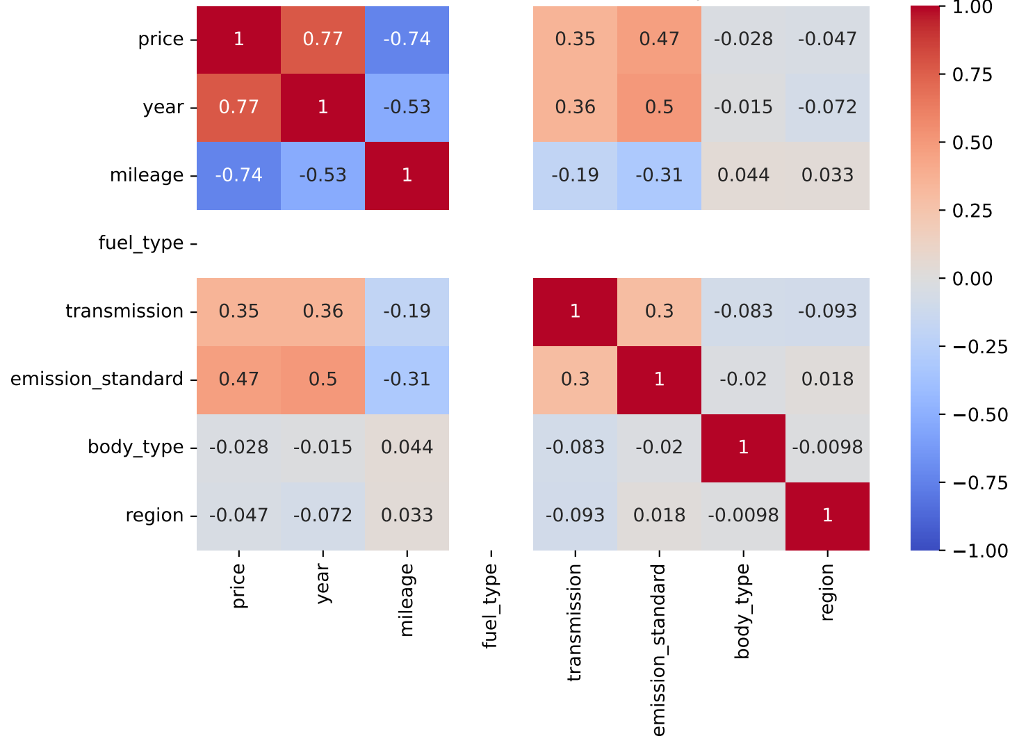
Spearman Correlation - Model: 3008 | Fuel: 1
