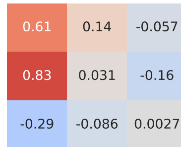
Pearson Correlation - Model: meriva | Fuel: 4
