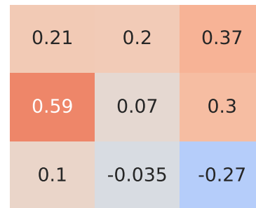
Spearman Correlation - Model: a2 | Fuel: 1
