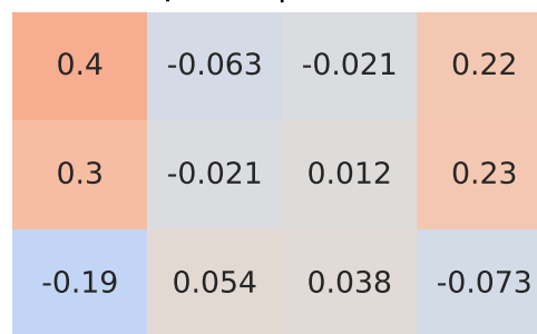
Spearman Correlation - Model: puma | Fuel: 3
