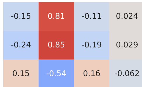
Spearman Correlation - Model: fortwo | Fuel: 2
