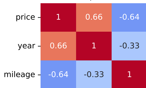
Spearman Correlation - Model: x1 | Fuel: 2
