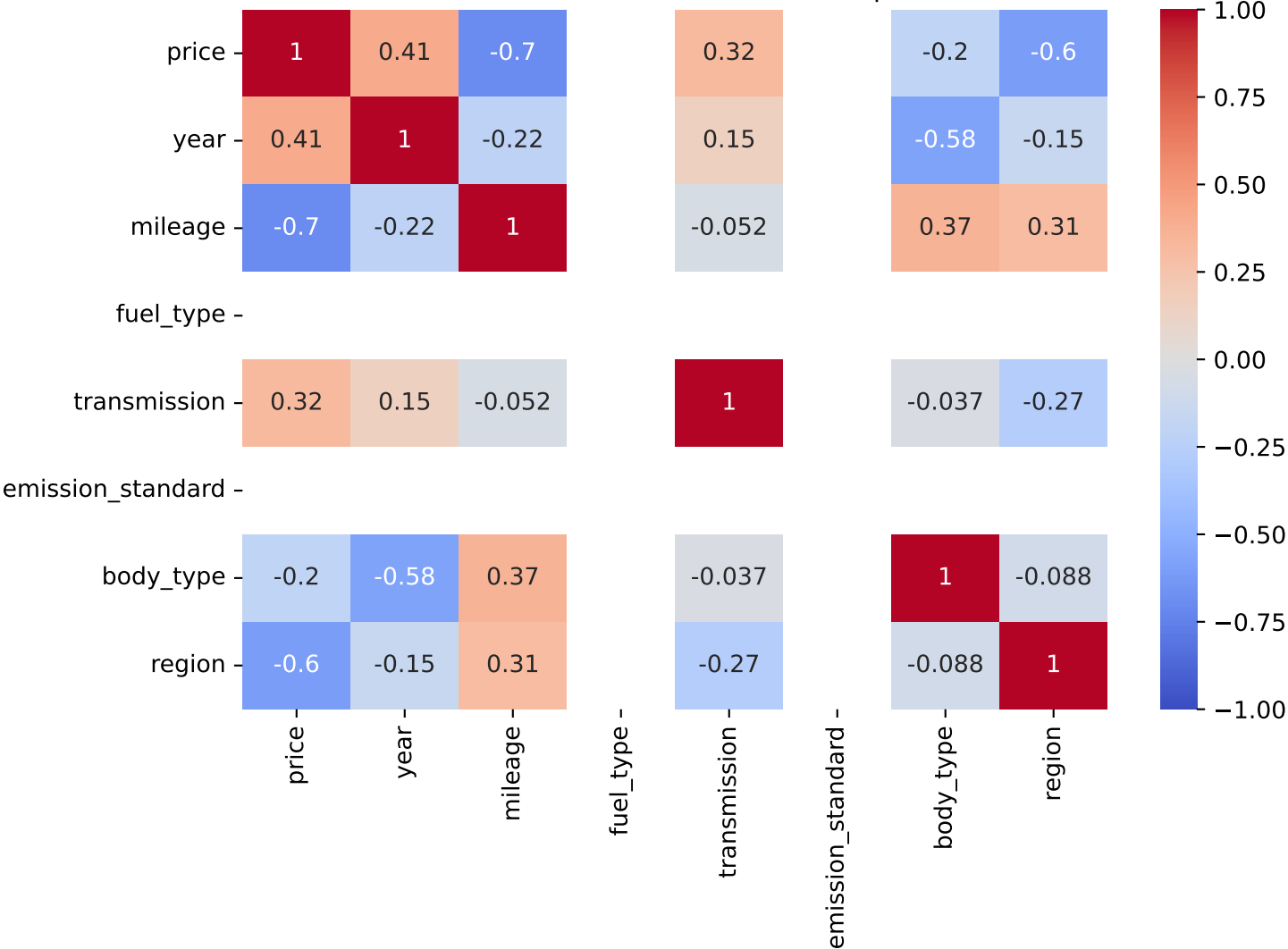
Pearson Correlation - Model: stonic | Fuel: 3
