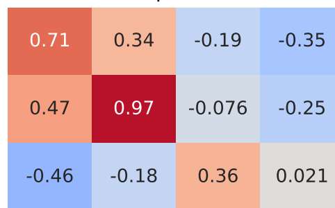
Pearson Correlation - Model: hilux | Fuel: 1
