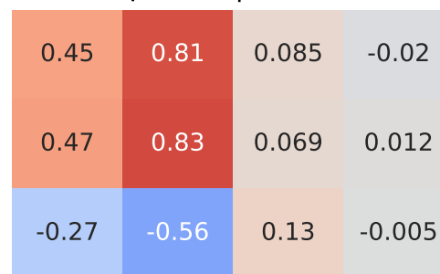
Spearman Correlation - Model: passat | Fuel: 1
