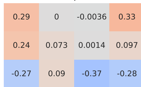
Spearman Correlation - Model: stonic | Fuel: 4
