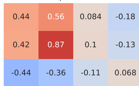
Pearson Correlation - Model: c3 | Fuel: 4
