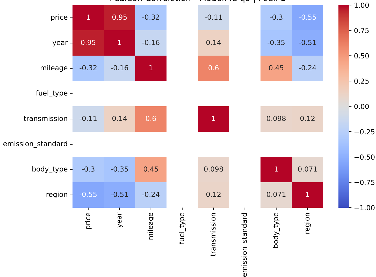
Pearson Correlation - Model: rs q3 | Fuel: 2
