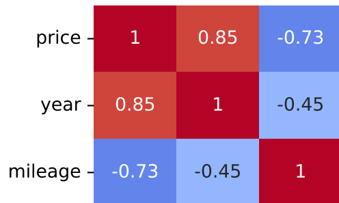
Pearson Correlation - Model: juke | Fuel: 4
