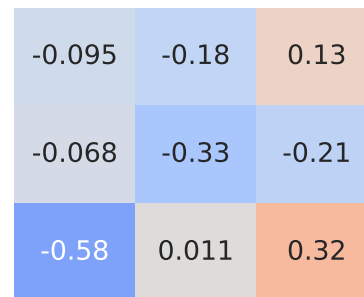
Spearman Correlation - Model: 206 | Fuel: 4
