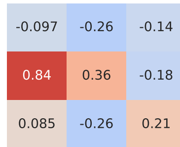
Spearman Correlation - Model: b-max | Fuel: 4
