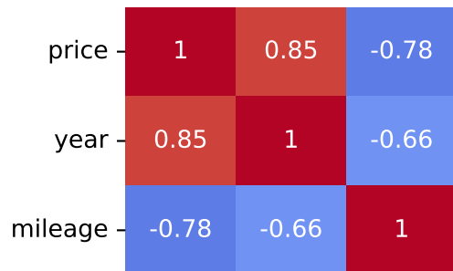
Pearson Correlation - Model: cooper s | Fuel: 2
