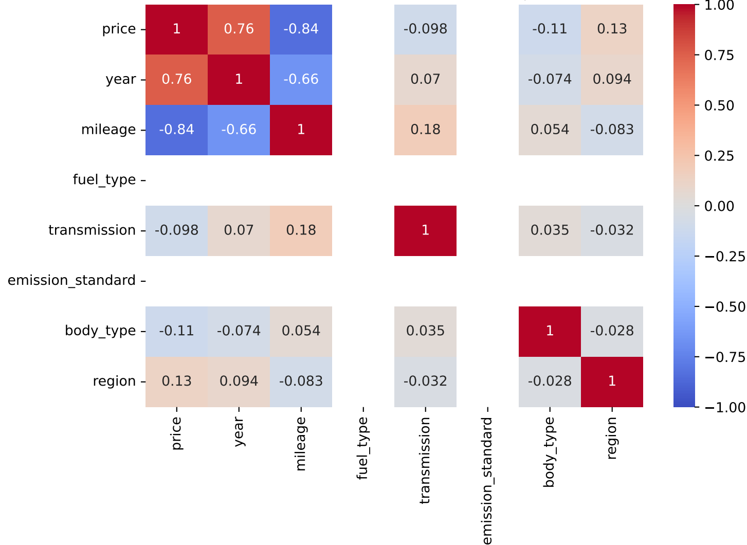
Pearson Correlation - Model: crossland | Fuel: 1
