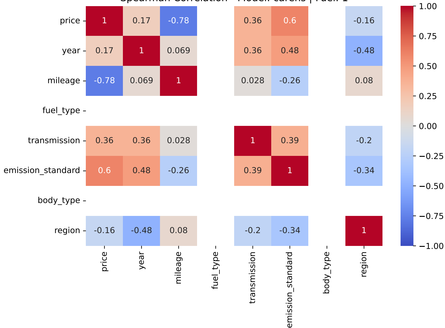
Spearman Correlation - Model: carens | Fuel: 1
