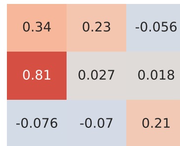
Spearman Correlation - Model: 207 | Fuel: 1
