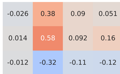
Spearman Correlation - Model: grande punto | Fuel: 1
