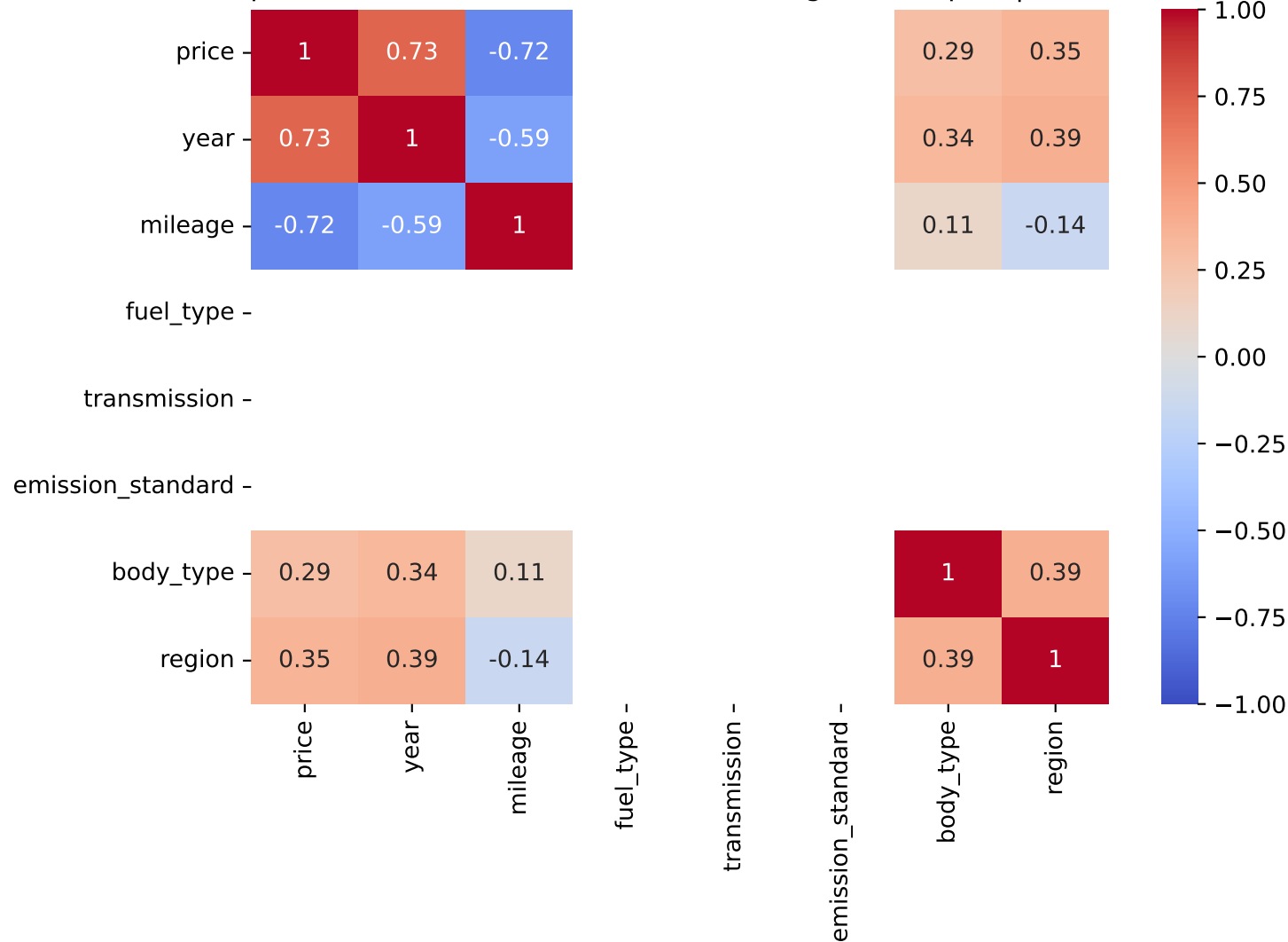
Spearman Correlation - Model: rover range rover sport | Fuel: 3
