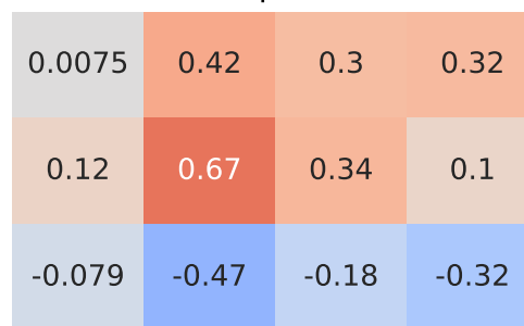
Spearman Correlation - Model: idea | Fuel: 1
