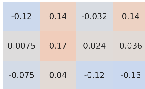
Spearman Correlation - Model: arkana | Fuel: 3
