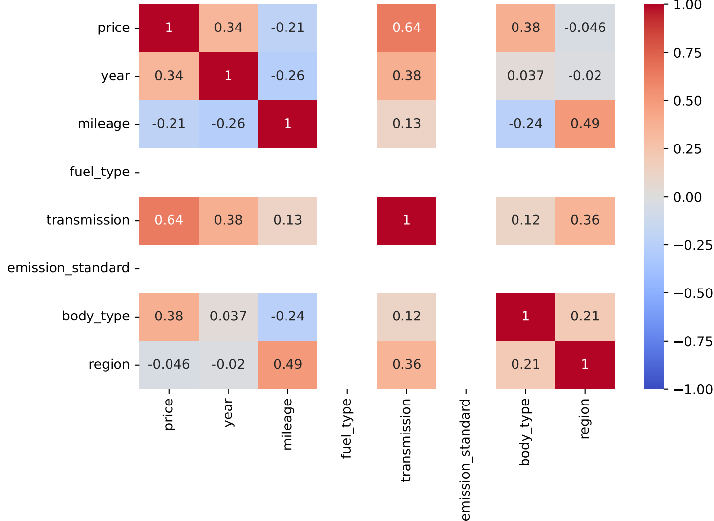
Pearson Correlation - Model: a1 citycarver | Fuel: 2
