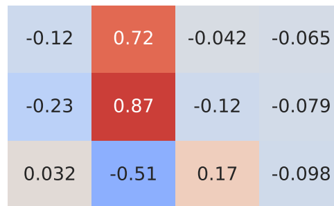
Spearman Correlation - Model: micra | Fuel: 4
