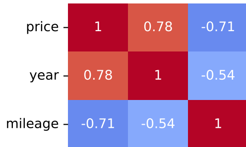
Spearman Correlation - Model: tucson | Fuel: 1
