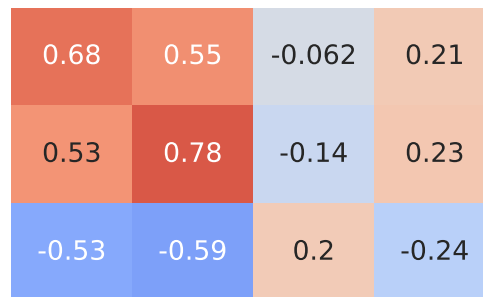
Pearson Correlation - Model: 308 | Fuel: 2
