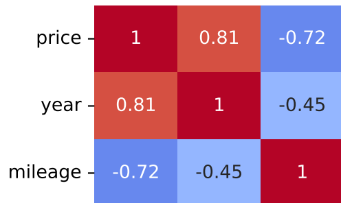
Pearson Correlation - Model: grand cherokee | Fuel: 1
