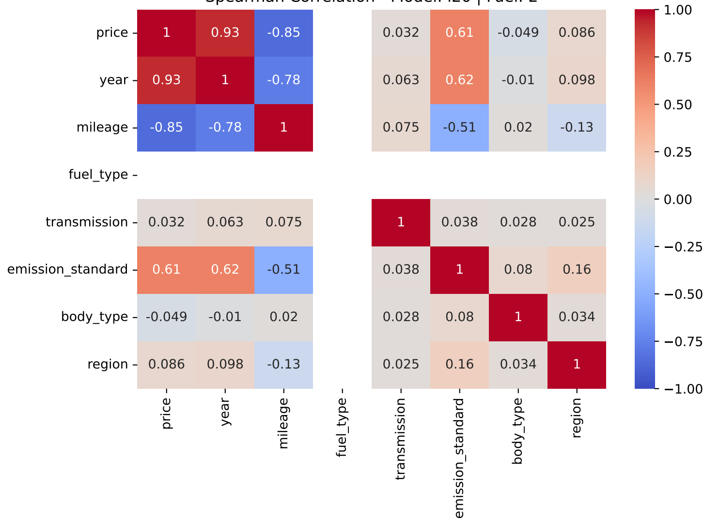
Spearman Correlation - Model: i20 | Fuel: 2
