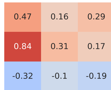
Pearson Correlation - Model: panda 4x4 | Fuel: 2
