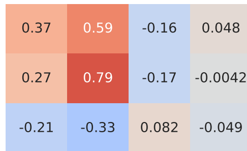
Pearson Correlation - Model: sportage | Fuel: 1
