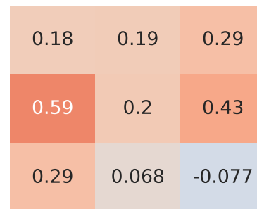
Pearson Correlation - Model: a2 | Fuel: 1
