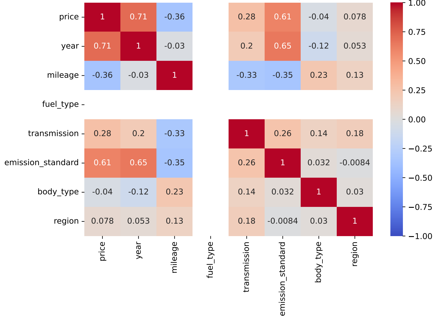
Spearman Correlation - Model: astra | Fuel: 4
