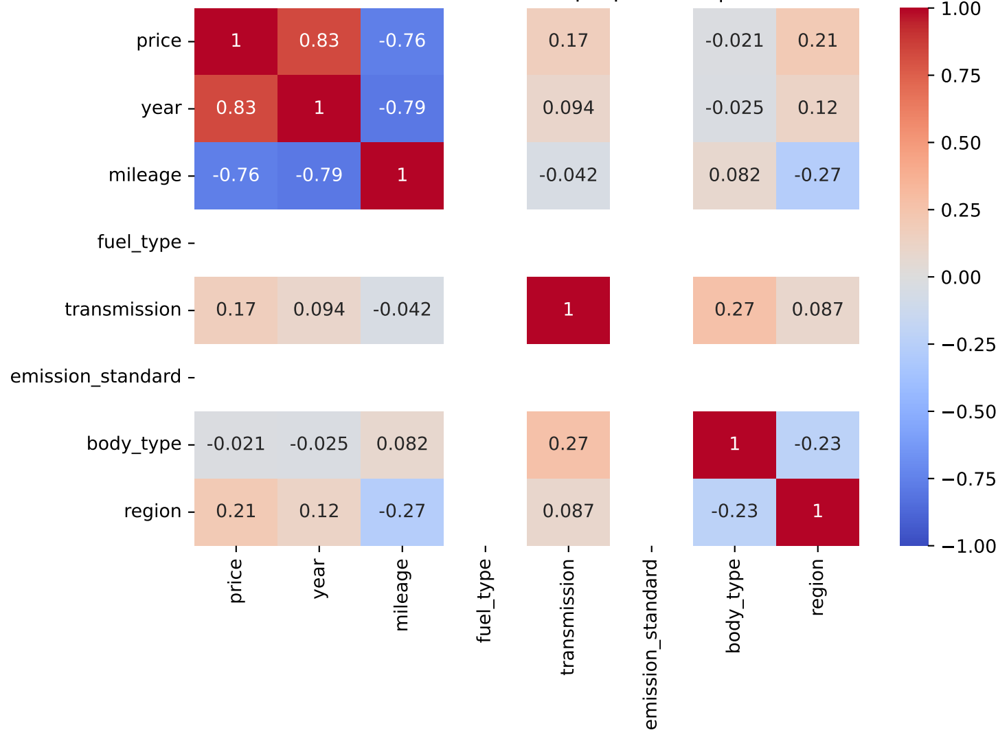
Pearson Correlation - Model: q3 sportback | Fuel: 1
