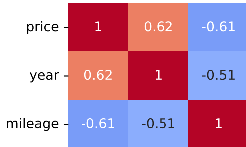
Pearson Correlation - Model: renegade | Fuel: 2
