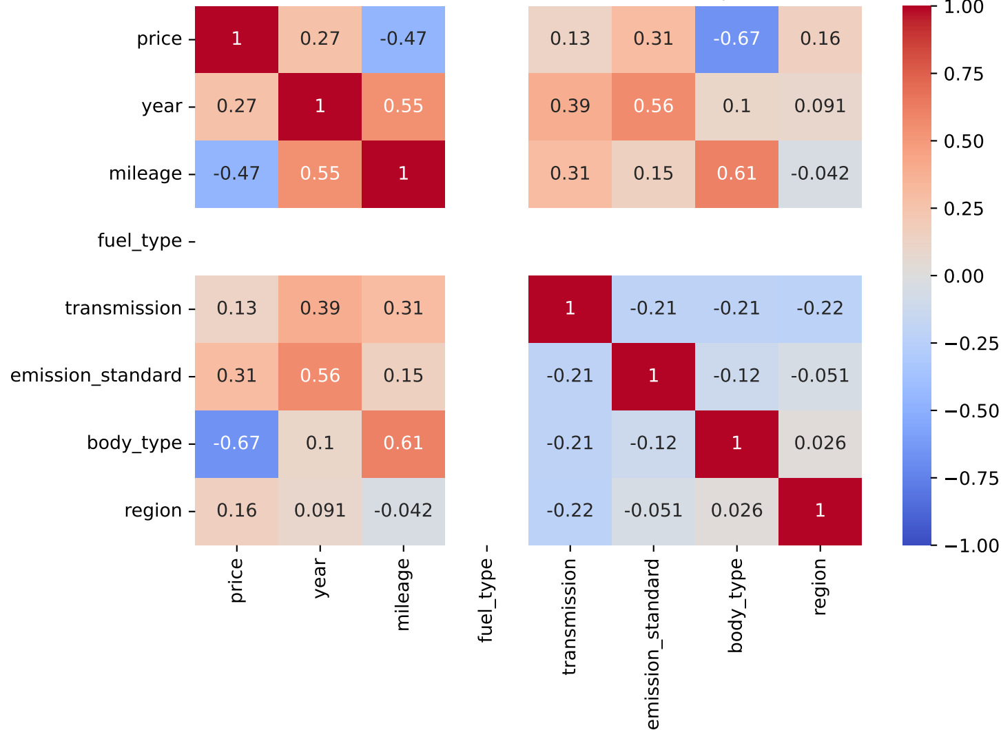
Spearman Correlation - Model: romeo 159 | Fuel: 2
