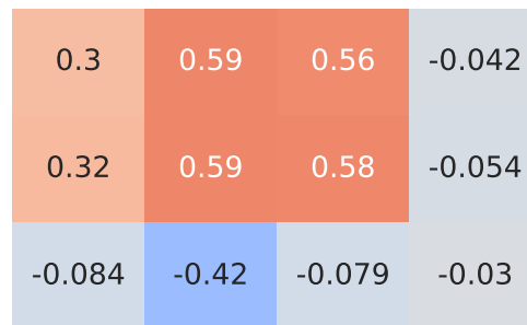
Spearman Correlation - Model: s3 | Fuel: 2
