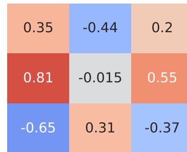
Pearson Correlation - Model: vengs | Fuel: 2
