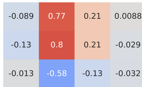
Spearman Correlation - Model: c3 | Fuel: 1
