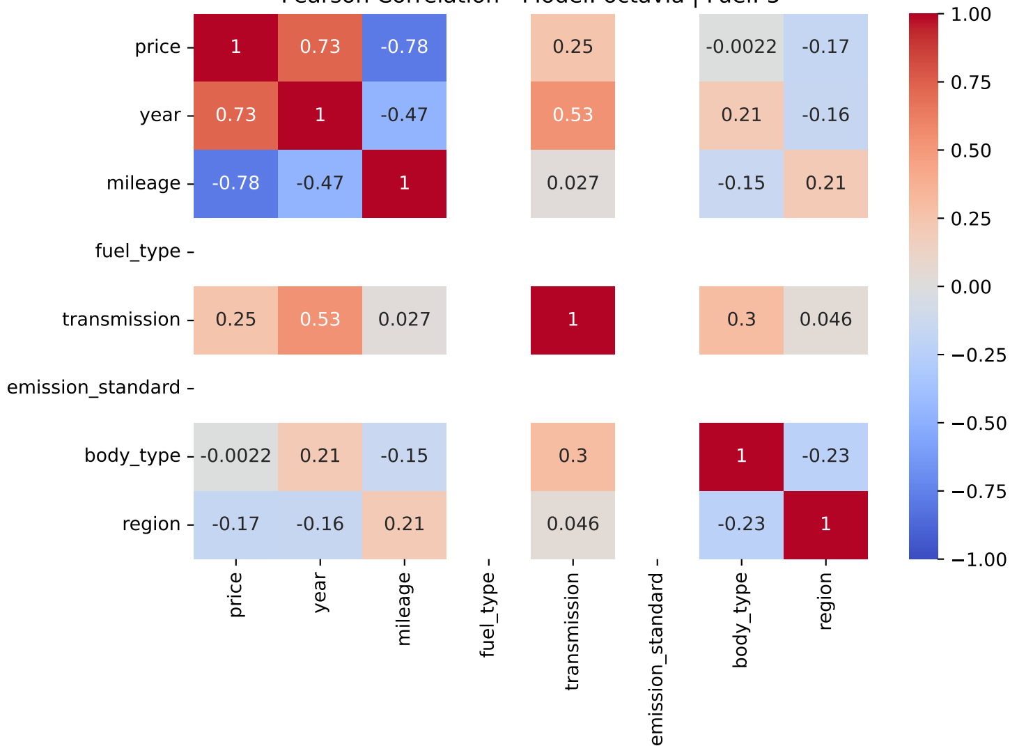
Pearson Correlation - Model: octavia | Fuel: 5
