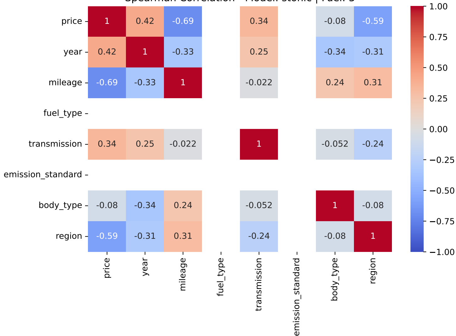
Spearman Correlation - Model: stonic | Fuel: 3
