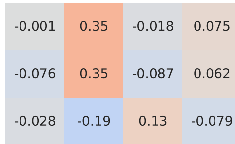
Spearman Correlation - Model: tucson | Fuel: 1
