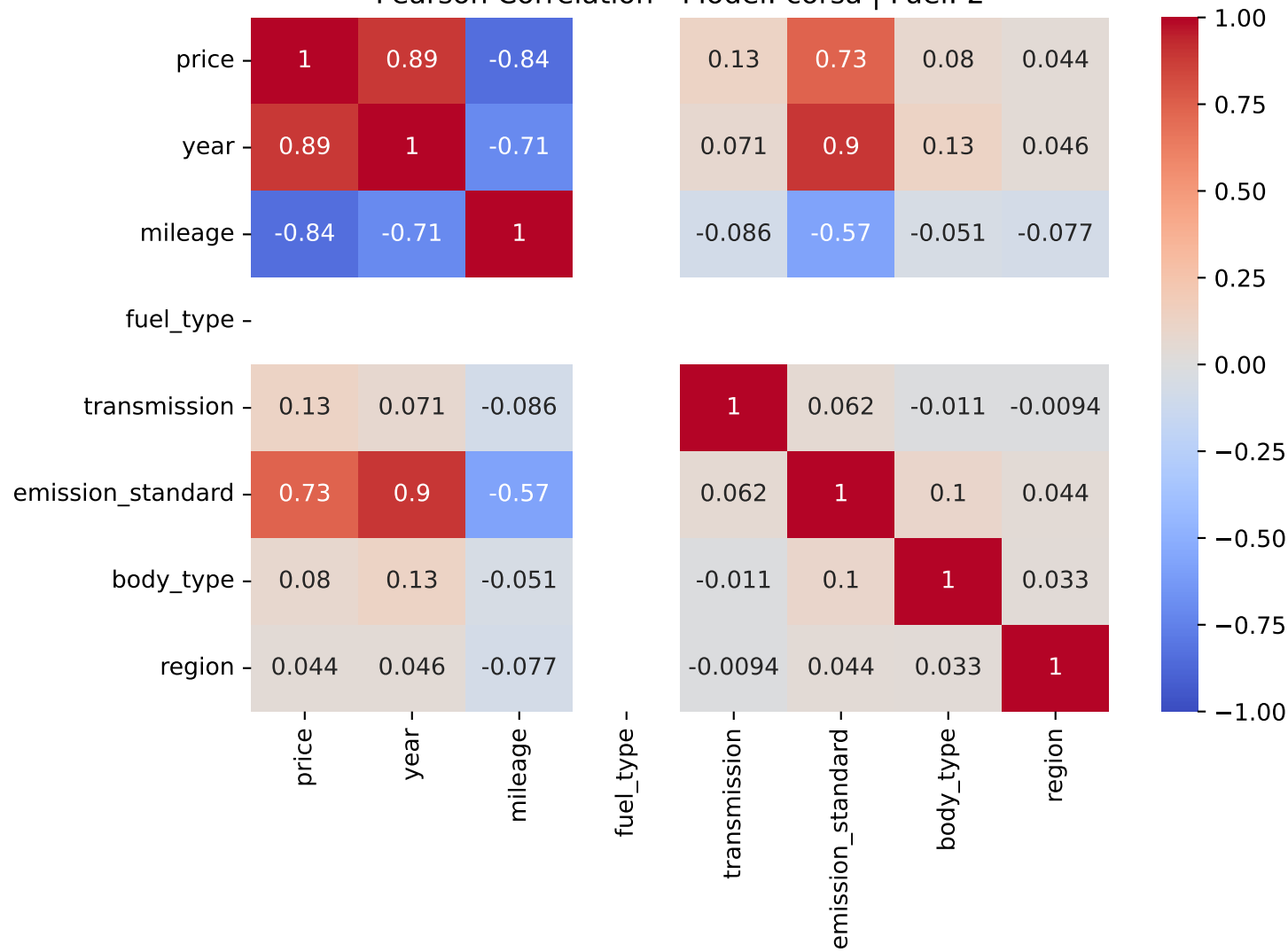
Pearson Correlation - Model: corsa | Fuel: 2
