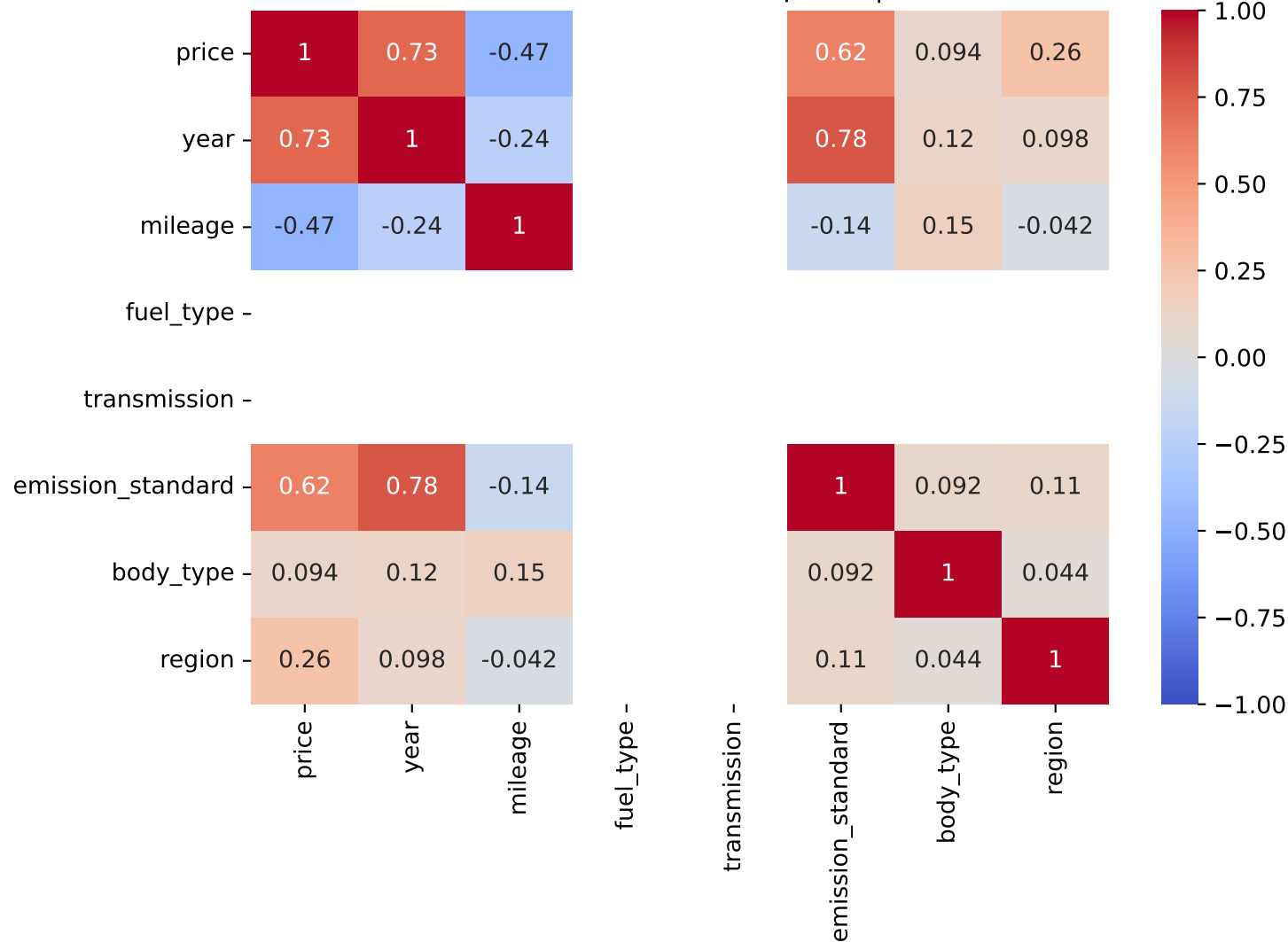
Pearson Correlation - Model: punto | Fuel: 5
