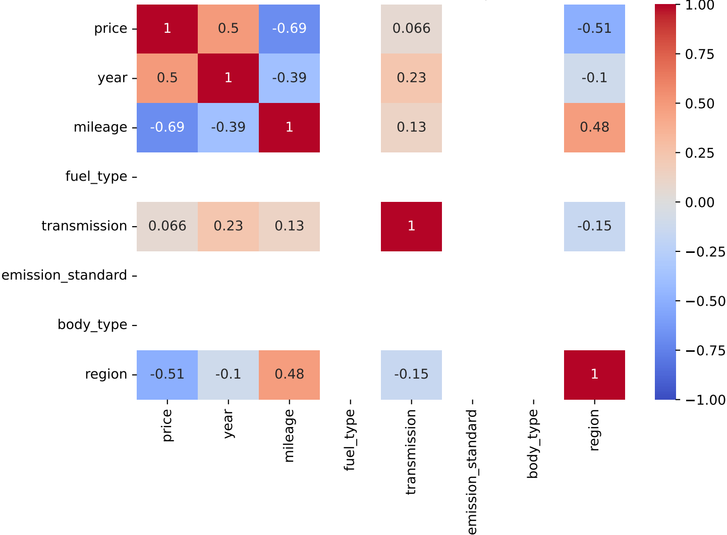
Pearson Correlation - Model: id.3 | Fuel: 0
