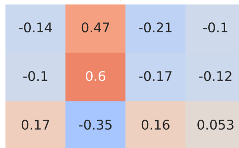
Pearson Correlation - Model: mokka | Fuel: 1
