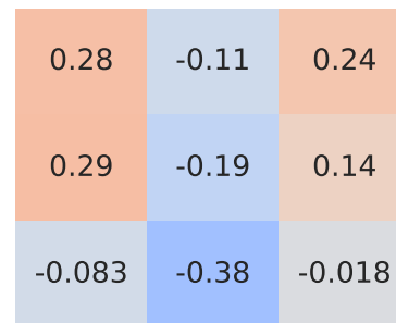
Spearman Correlation - Model: c2 | Fuel: 1
