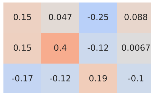
Pearson Correlation - Model: rover discovery sport | Fuel: 1
