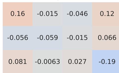
Pearson Correlation - Model: arona | Fuel: 2
