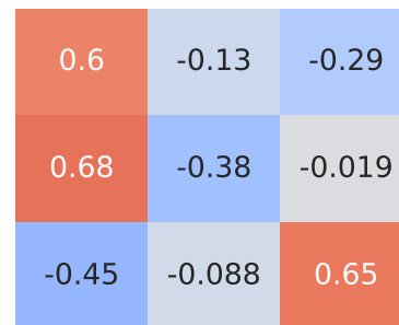
Spearman Correlation - Model: ka | Fuel: 4
