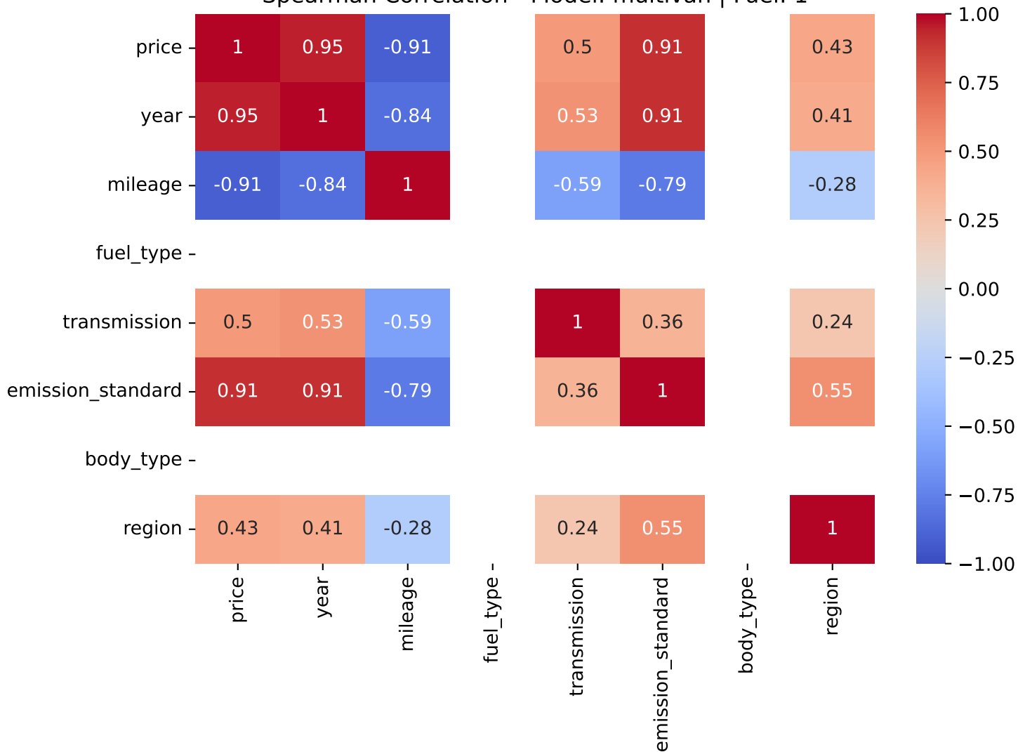
Spearman Correlation - Model: multivan | Fuel: 1
