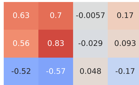
Pearson Correlation - Model: cooper | Fuel: 2
