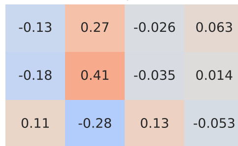
Pearson Correlation - Model: ecosport | Fuel: 2
