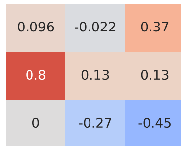
Spearman Correlation - Model: splash | Fuel: 2
