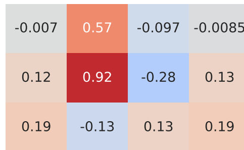
Pearson Correlation - Model: puma | Fuel: 2
