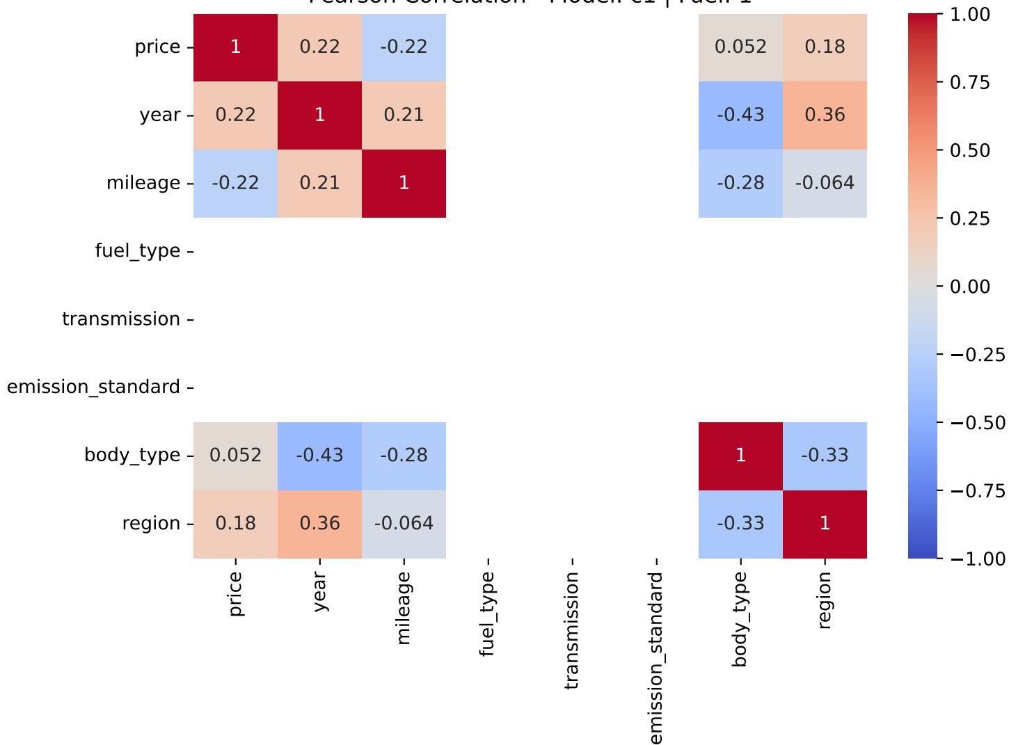
Pearson Correlation - Model: c1 | Fuel: 1
