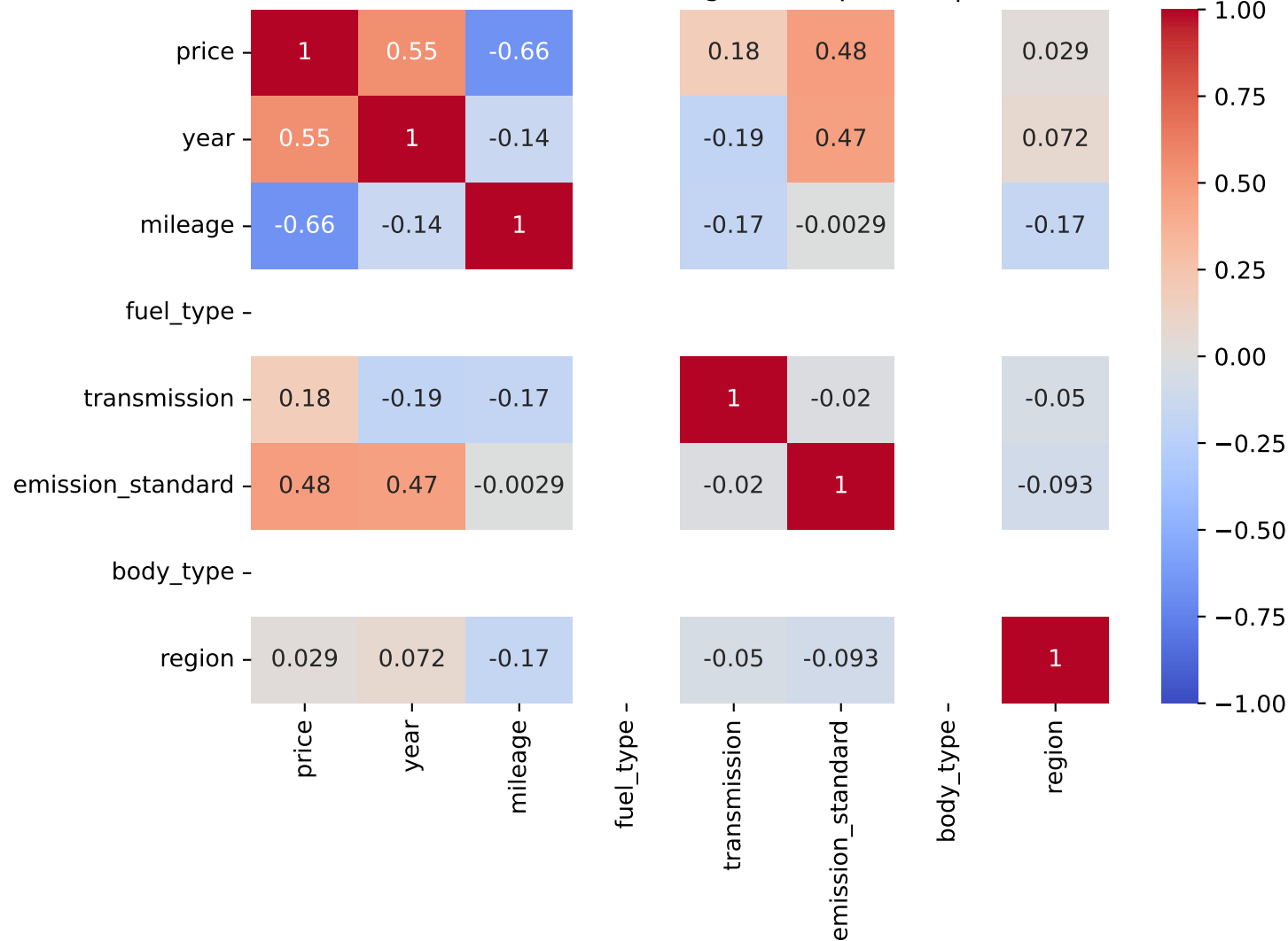
Pearson Correlation - Model: grand c4 picasso | Fuel: 1
