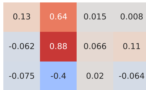
Pearson Correlation - Model: sportage | Fuel: 4
