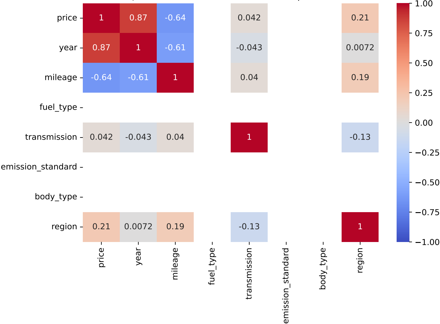
Spearman Correlation - Model: m4 | Fuel: 2
