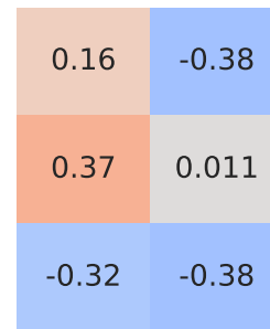
Spearman Correlation - Model: fiesta active | Fuel: 2
