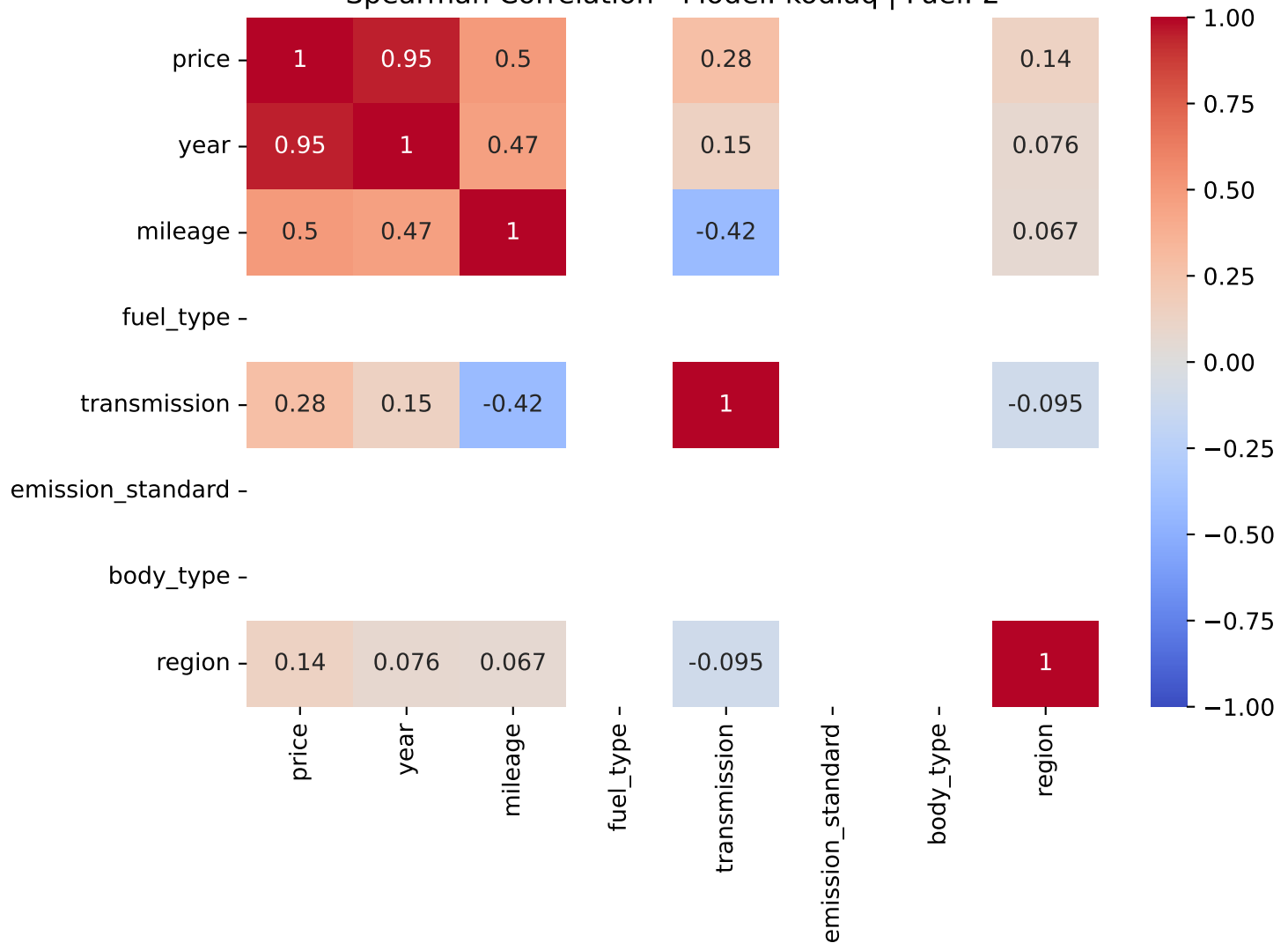
Spearman Correlation - Model: kodiaq | Fuel: 2
