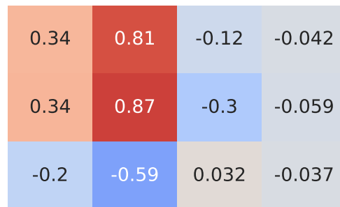
Spearman Correlation - Model: a5 | Fuel: 1
