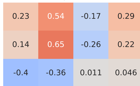
Pearson Correlation - Model: soul | Fuel: 1
