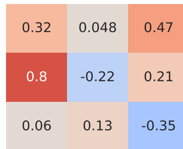
Pearson Correlation - Model: note | Fuel: 1
