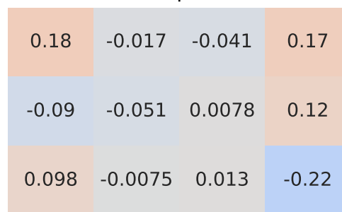
Spearman Correlation - Model: arona | Fuel: 2
