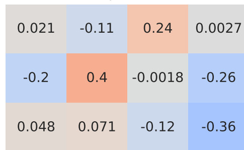
Pearson Correlation - Model: 207 | Fuel: 4
