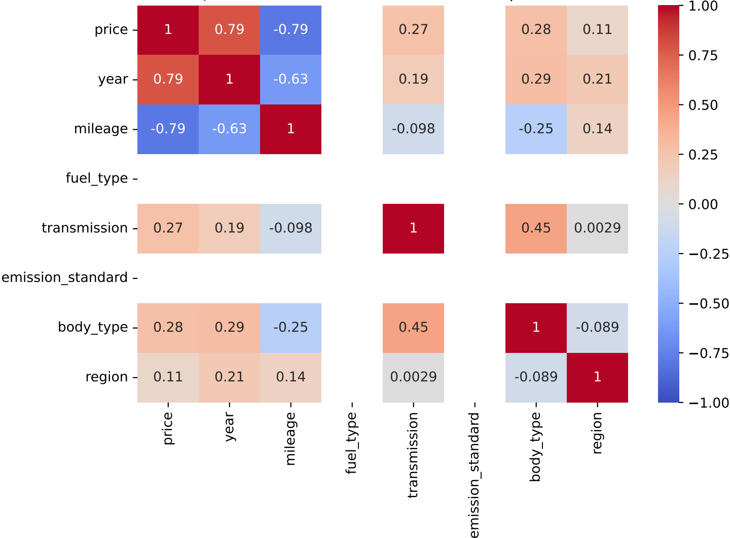
Spearman Correlation - Model: tarraco | Fuel: 1
