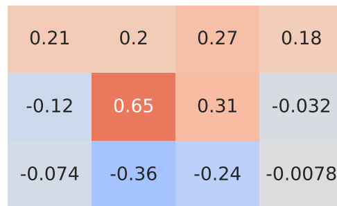
Spearman Correlation - Model: modus | Fuel: 2
