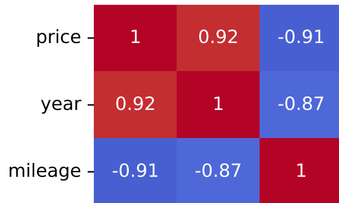
Pearson Correlation - Model: tucson | Fuel: 2
