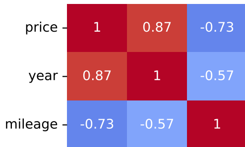
Pearson Correlation - Model: 3008 | Fuel: 1
