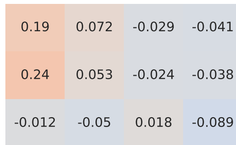
Pearson Correlation - Model: romeo giulia | Fuel: 1
