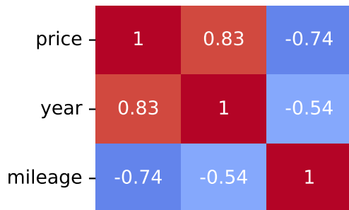
Pearson Correlation - Model: a4 | Fuel: 1
