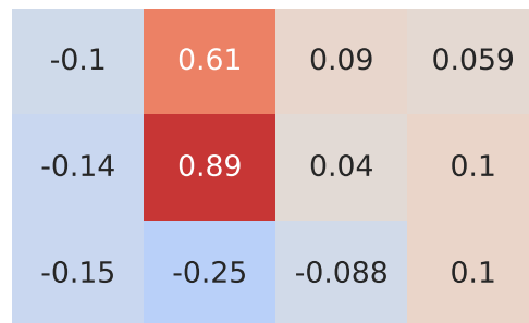
Spearman Correlation - Model: partner | Fuel: 1
