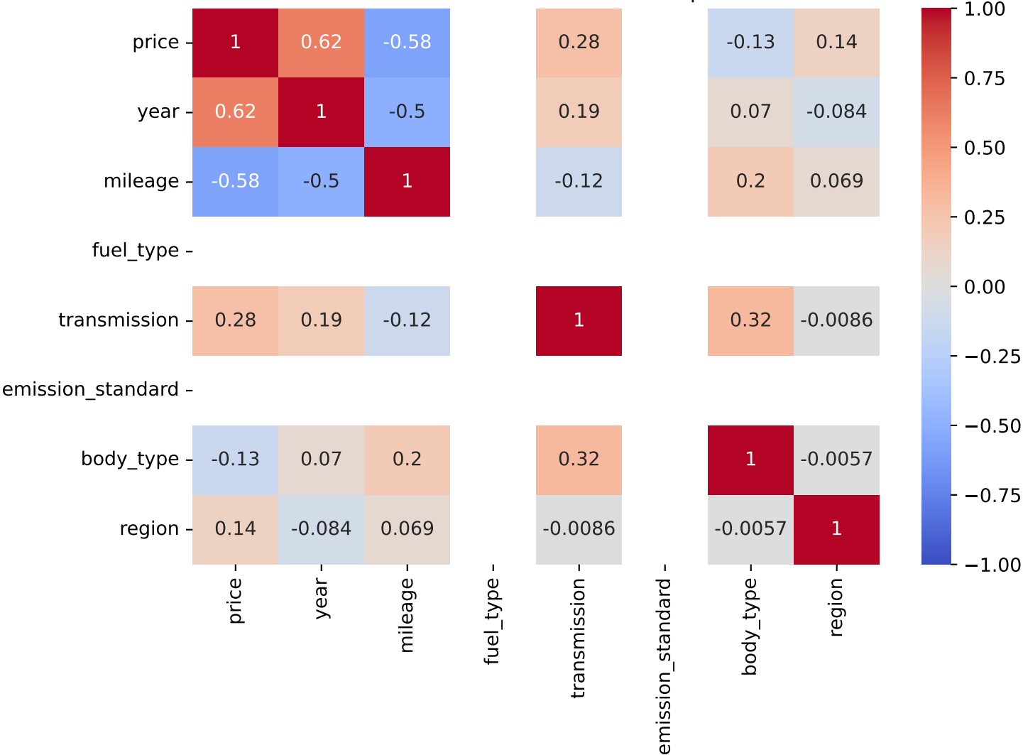
Pearson Correlation - Model: focus | Fuel: 3
