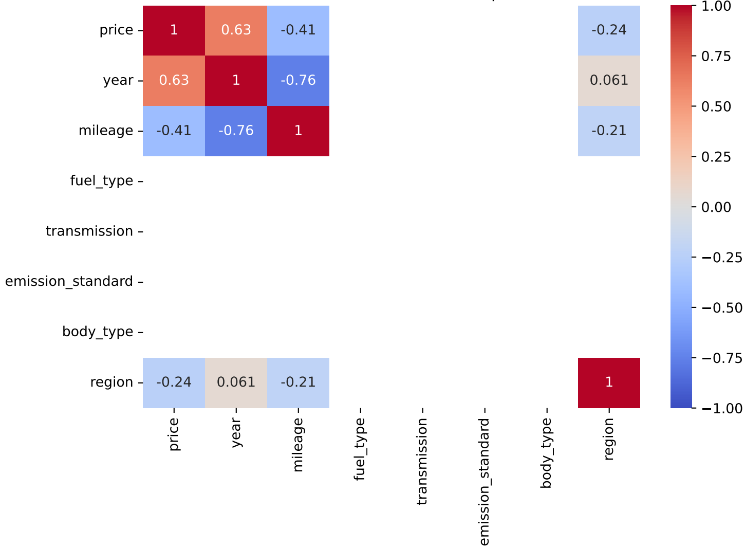
Pearson Correlation - Model: a7 | Fuel: 3
