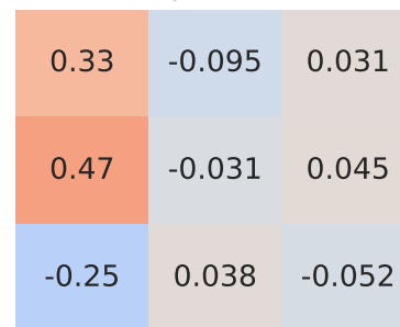
Spearman Correlation - Model: ecosport | Fuel: 1
