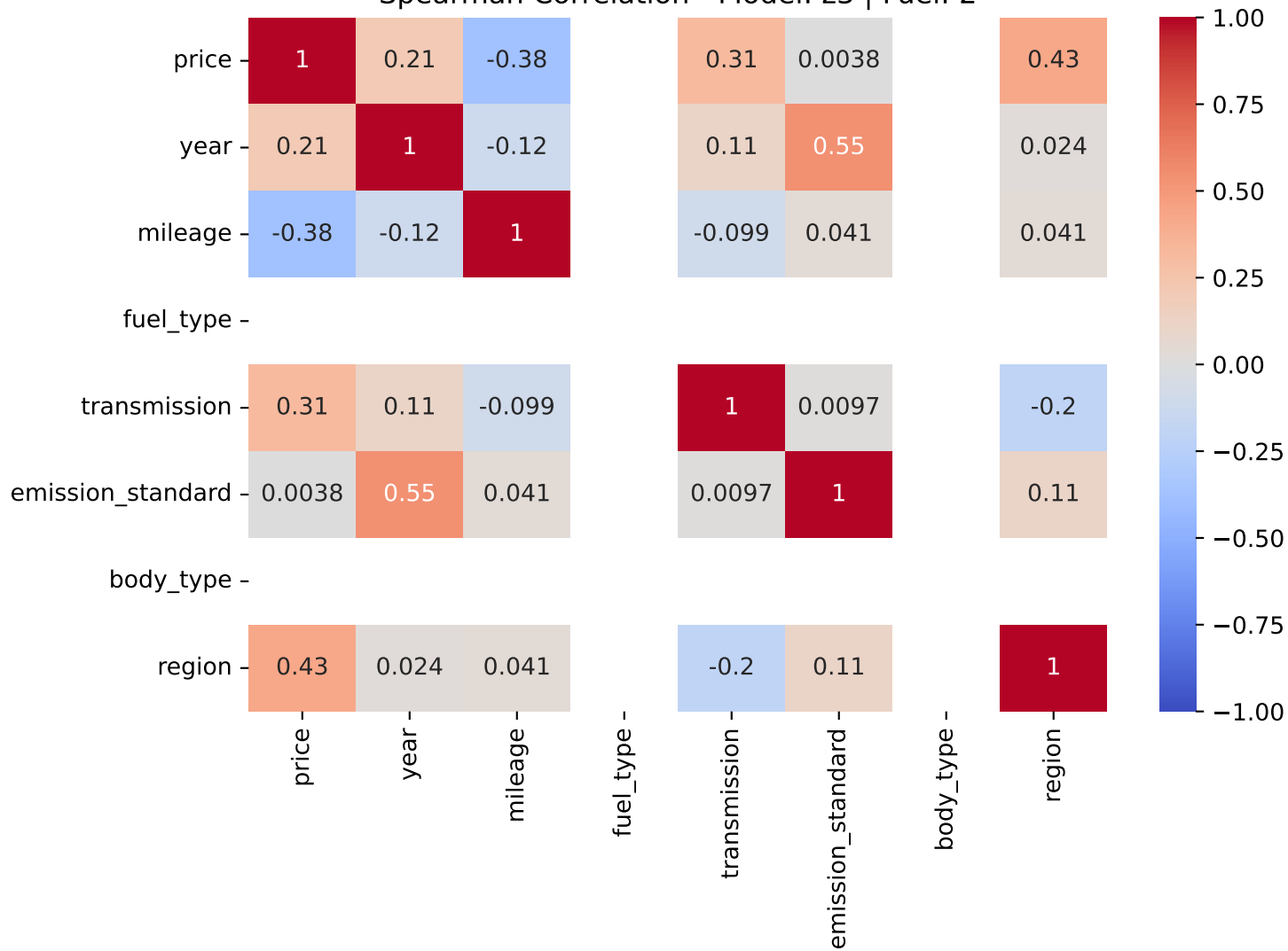
Spearman Correlation - Model: z3 | Fuel: 2
