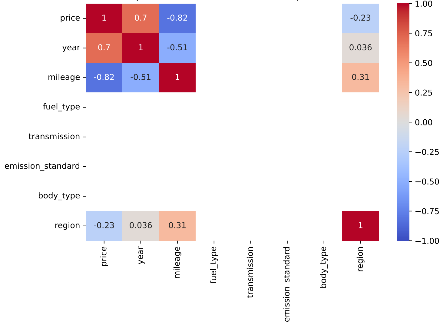
Spearman Correlation - Model: a8 | Fuel: 3
