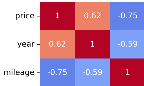
Spearman Correlation - Model: romeo giulietta | Fuel: 2
