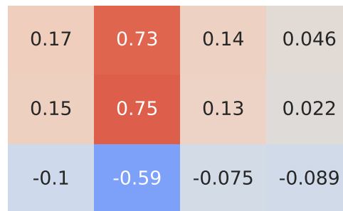
Spearman Correlation - Model: c3 | Fuel: 2
