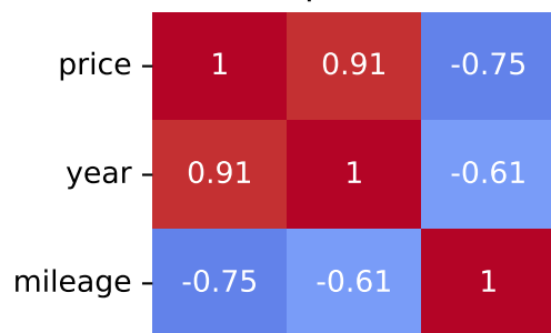
Spearman Correlation - Model: s-max | Fuel: 1
