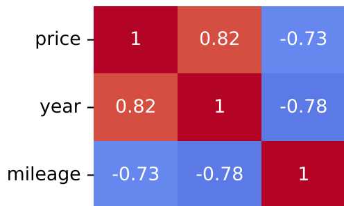
Spearman Correlation - Model: 2008 | Fuel: 2
