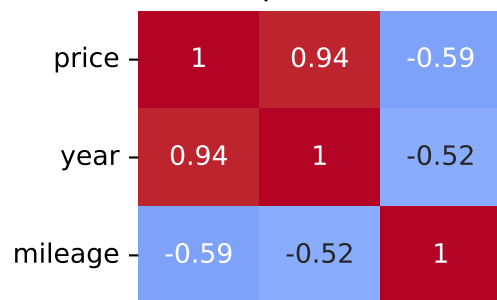
Spearman Correlation - Model: touareg | Fuel: 1
