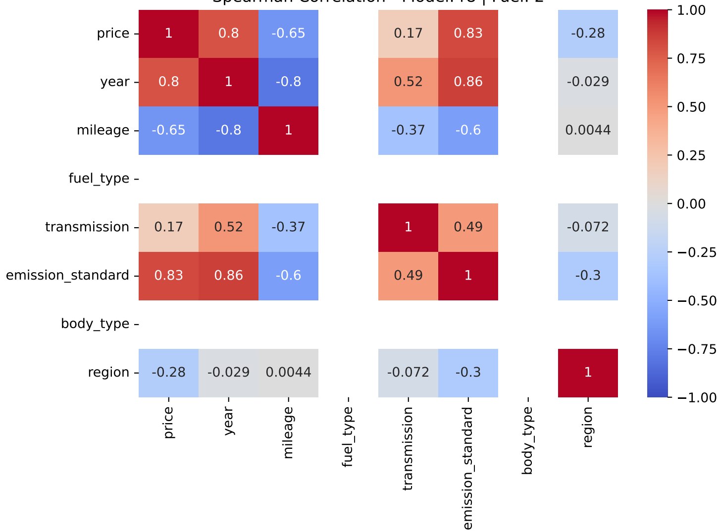
Spearman Correlation - Model: r8 | Fuel: 2
