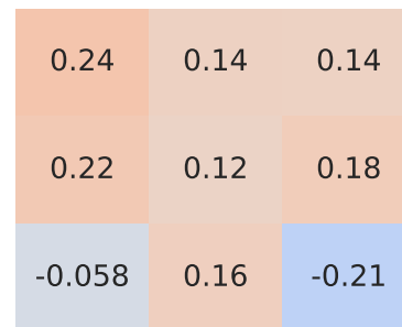
Pearson Correlation - Model: captur | Fuel: 4
