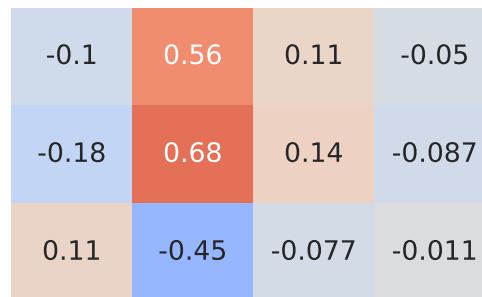
Spearman Correlation - Model: 208 | Fuel: 1
