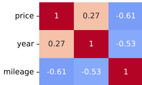
Pearson Correlation - Model: panda cross | Fuel: 2
