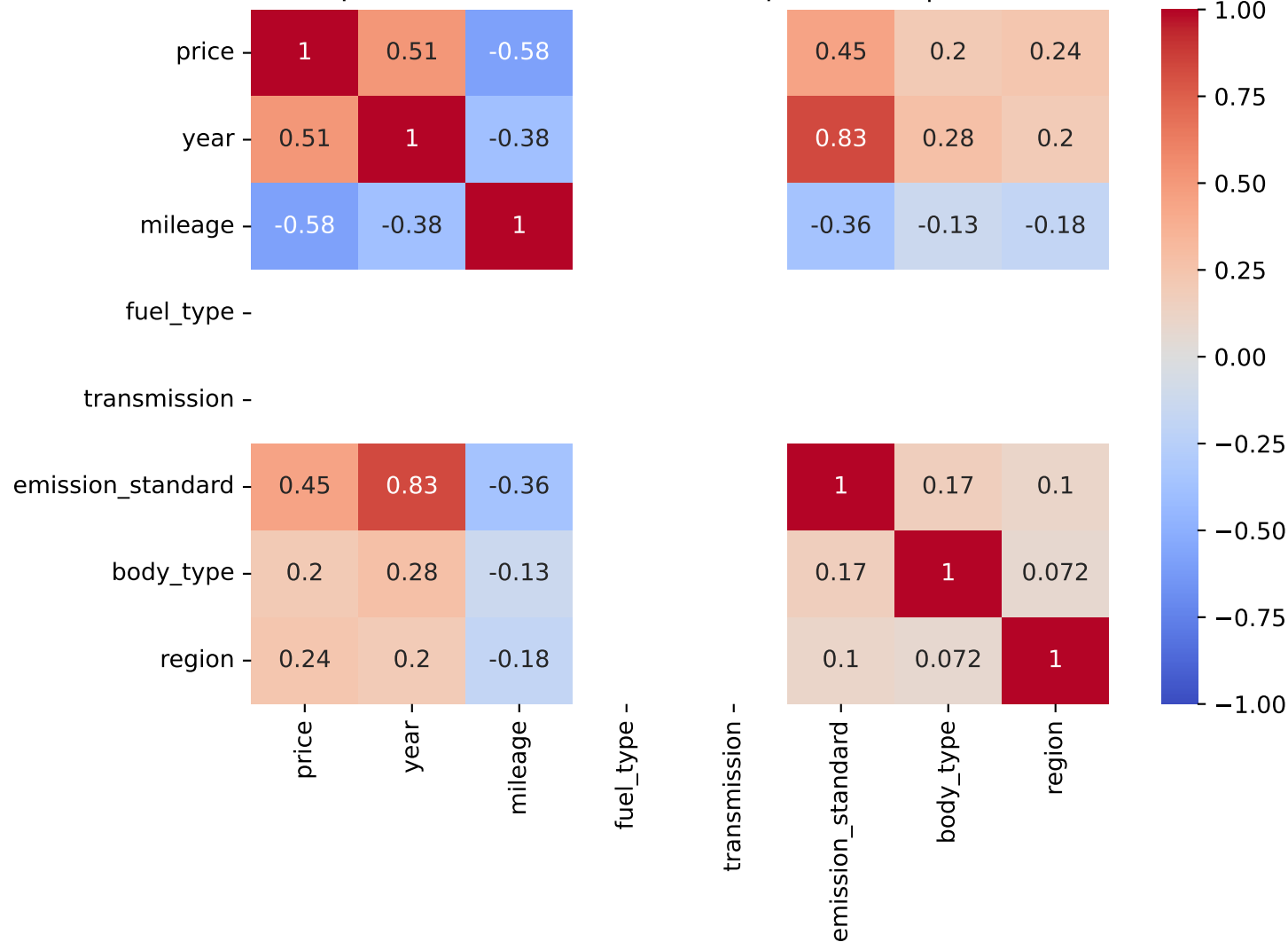
Spearman Correlation - Model: panda 4x4 | Fuel: 2
