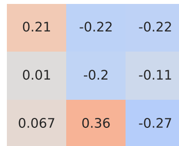
Spearman Correlation - Model: romeo stelvio | Fuel: 2
