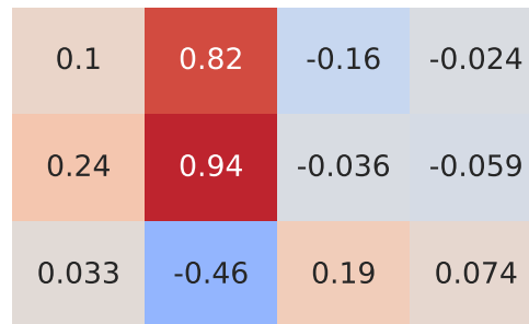
Spearman Correlation - Model: grand cherokee | Fuel: 1
