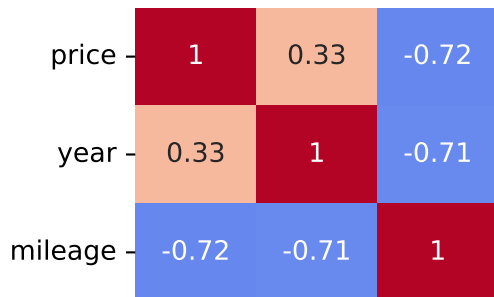
Spearman Correlation - Model: venga | Fuel: 2
