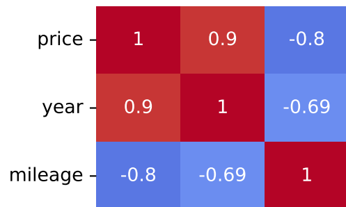
Pearson Correlation - Model: aygo | Fuel: 2
