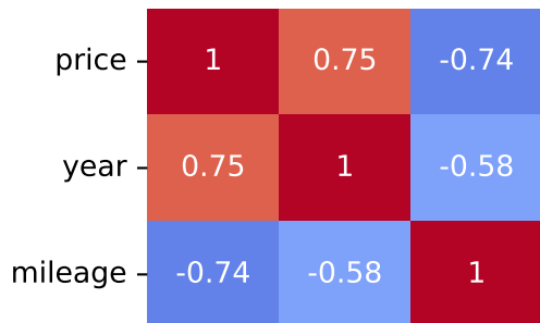
Pearson Correlation - Model: c3 aircross | Fuel: 1
