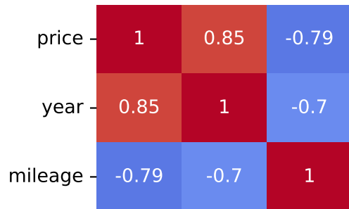
Spearman Correlation - Model: c-hr | Fuel: 3
