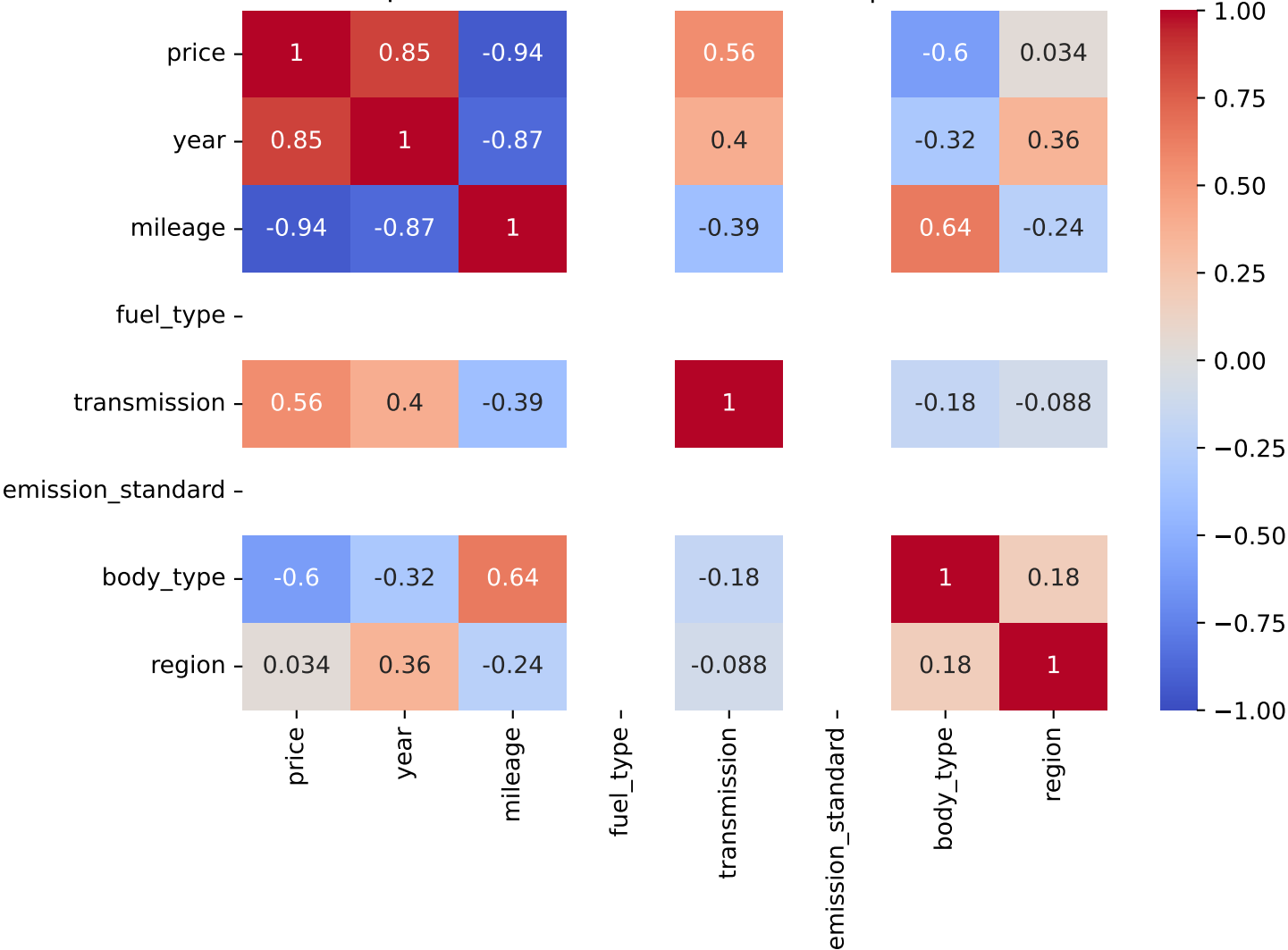
Spearman Correlation - Model: i30 | Fuel: 3
