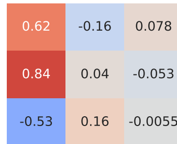
Pearson Correlation - Model: c-max | Fuel: 2
