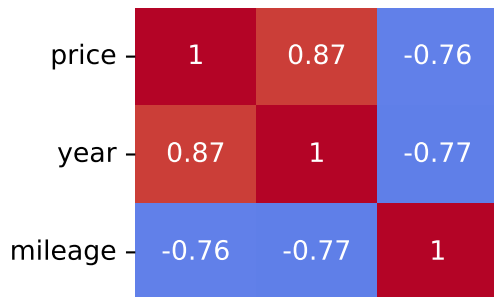
Pearson Correlation - Model: 2008 | Fuel: 2
