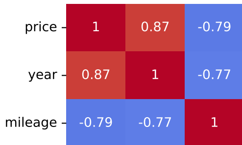
Pearson Correlation - Model: 3008 | Fuel: 2
