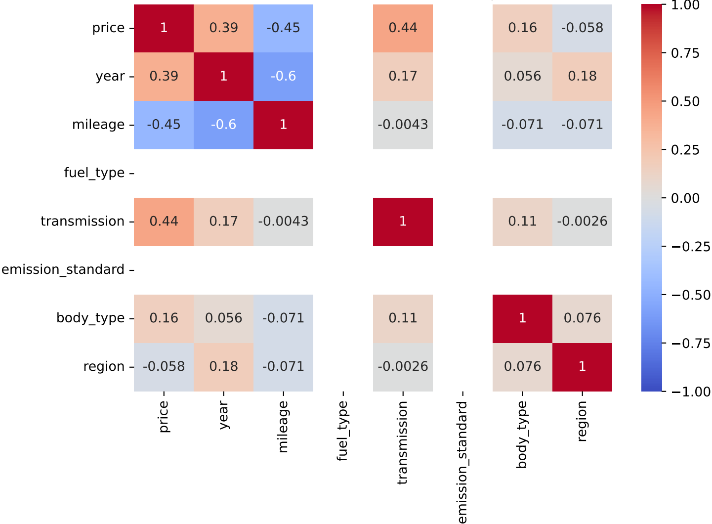
Pearson Correlation - Model: qashqai | Fuel: 3
