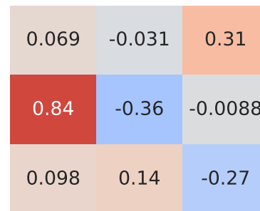
Spearman Correlation - Model: note | Fuel: 1
