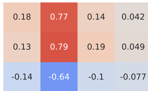
Spearman Correlation - Model: corsa | Fuel: 2
