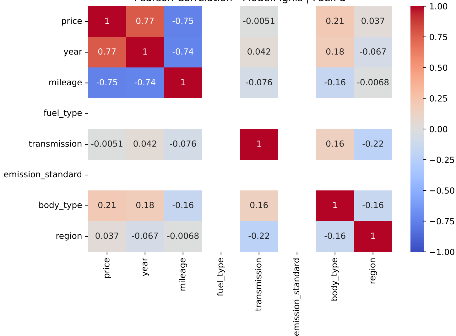
Pearson Correlation - Model: ignis | Fuel: 3
