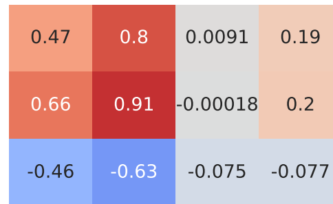
Spearman Correlation - Model: rover discovery | Fuel: 1
