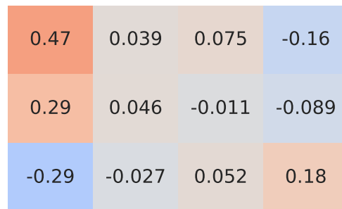
Pearson Correlation - Model: x2 | Fuel: 1
