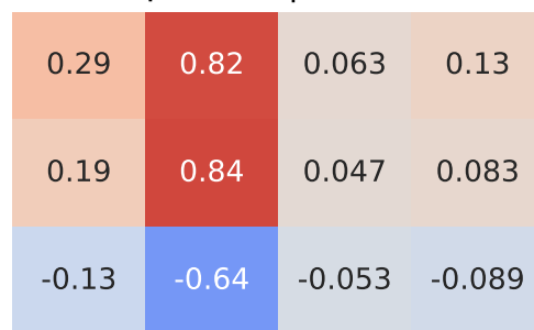
Spearman Correlation - Model: picanto | Fuel: 2
