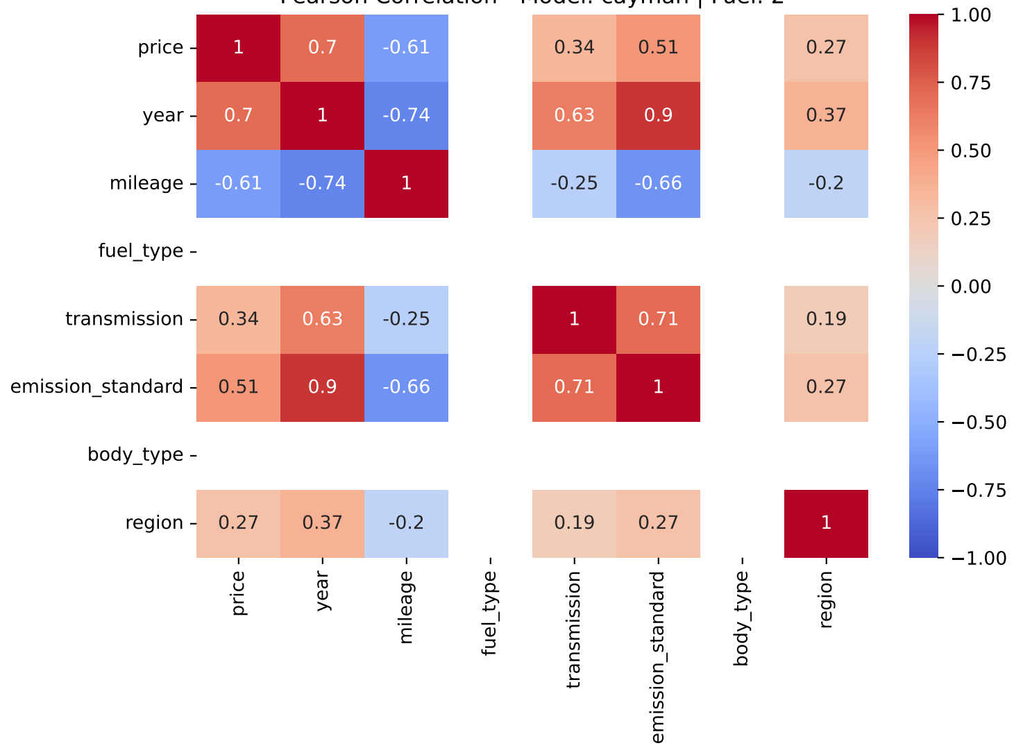
Pearson Correlation - Model: cayman | Fuel: 2
