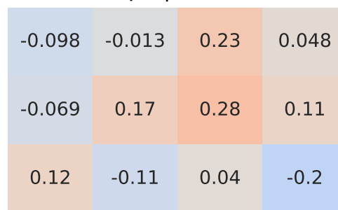
Spearman Correlation - Model: tipo | Fuel: 2
