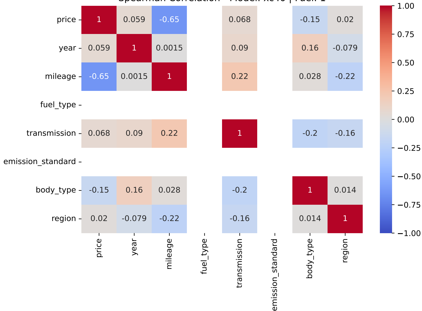
Spearman Correlation - Model: xc40 | Fuel: 1
