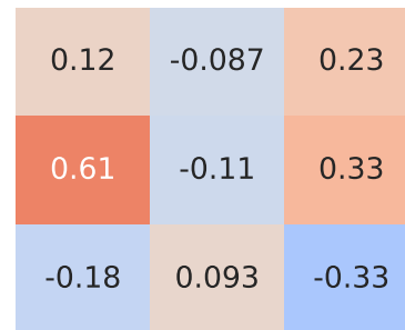
Pearson Correlation - Model: venga | Fuel: 4
