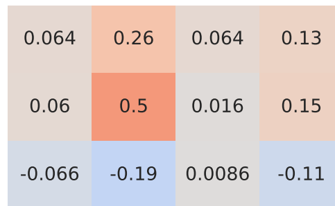
Pearson Correlation - Model: musa | Fuel: 1
