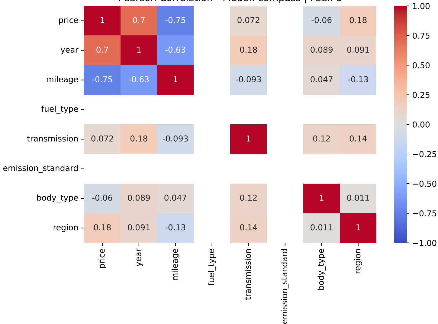
Pearson Correlation - Model: compass | Fuel: 3
