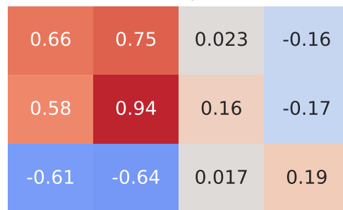
Spearman Correlation - Model: megane | Fuel: 2
