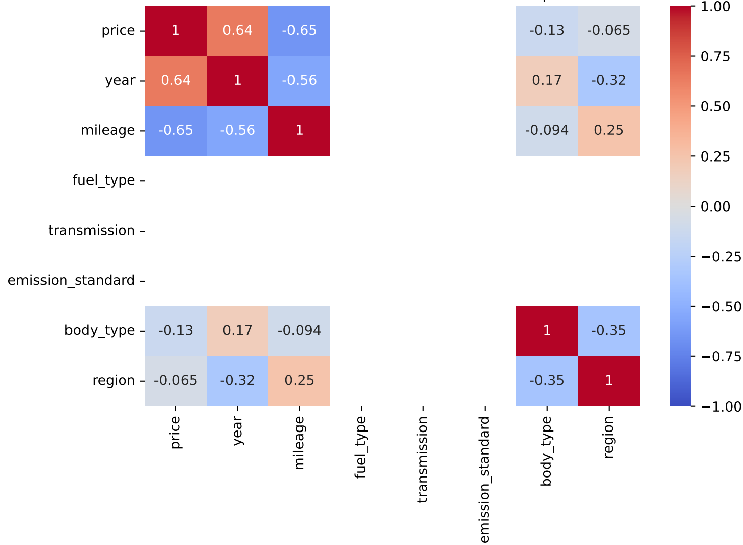
Pearson Correlation - Model: rover defender | Fuel: 3
