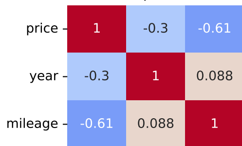
Spearman Correlation - Model: 307 | Fuel: 2
