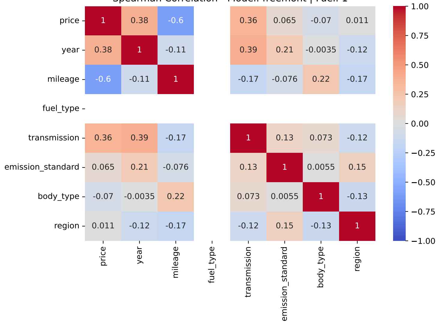
Spearman Correlation - Model: freemont | Fuel: 1
