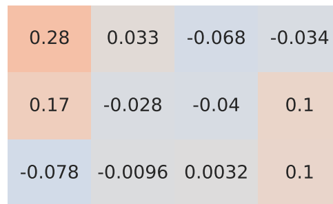
Pearson Correlation - Model: crossland | Fuel: 2
