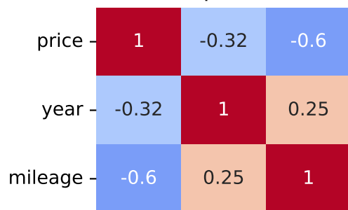
Spearman Correlation - Model: stilo | Fuel: 2
