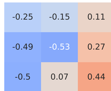
Pearson Correlation - Model: 206 | Fuel: 4
