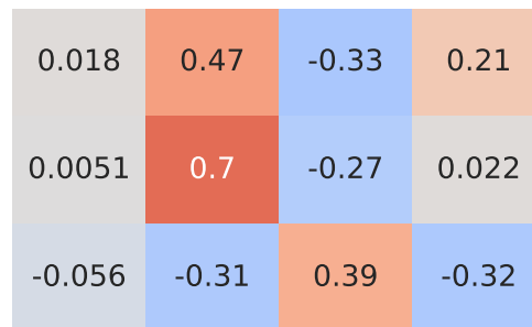
Pearson Correlation - Model: adam | Fuel: 2
