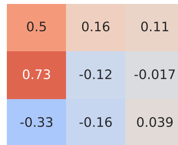
Spearman Correlation - Model: 208 | Fuel: 4
