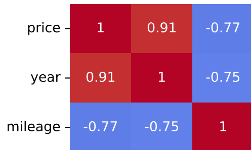
Pearson Correlation - Model: one | Fuel: 2
