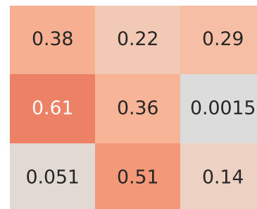
Pearson Correlation - Model: patriot | Fuel: 1
