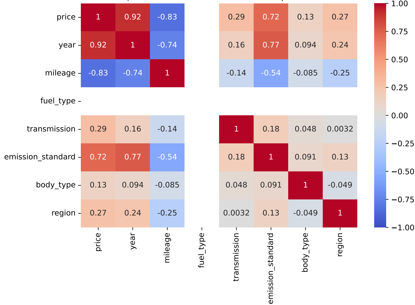
Spearman Correlation - Model: i10 | Fuel: 2
