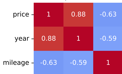
Spearman Correlation - Model: sorento | Fuel: 1
