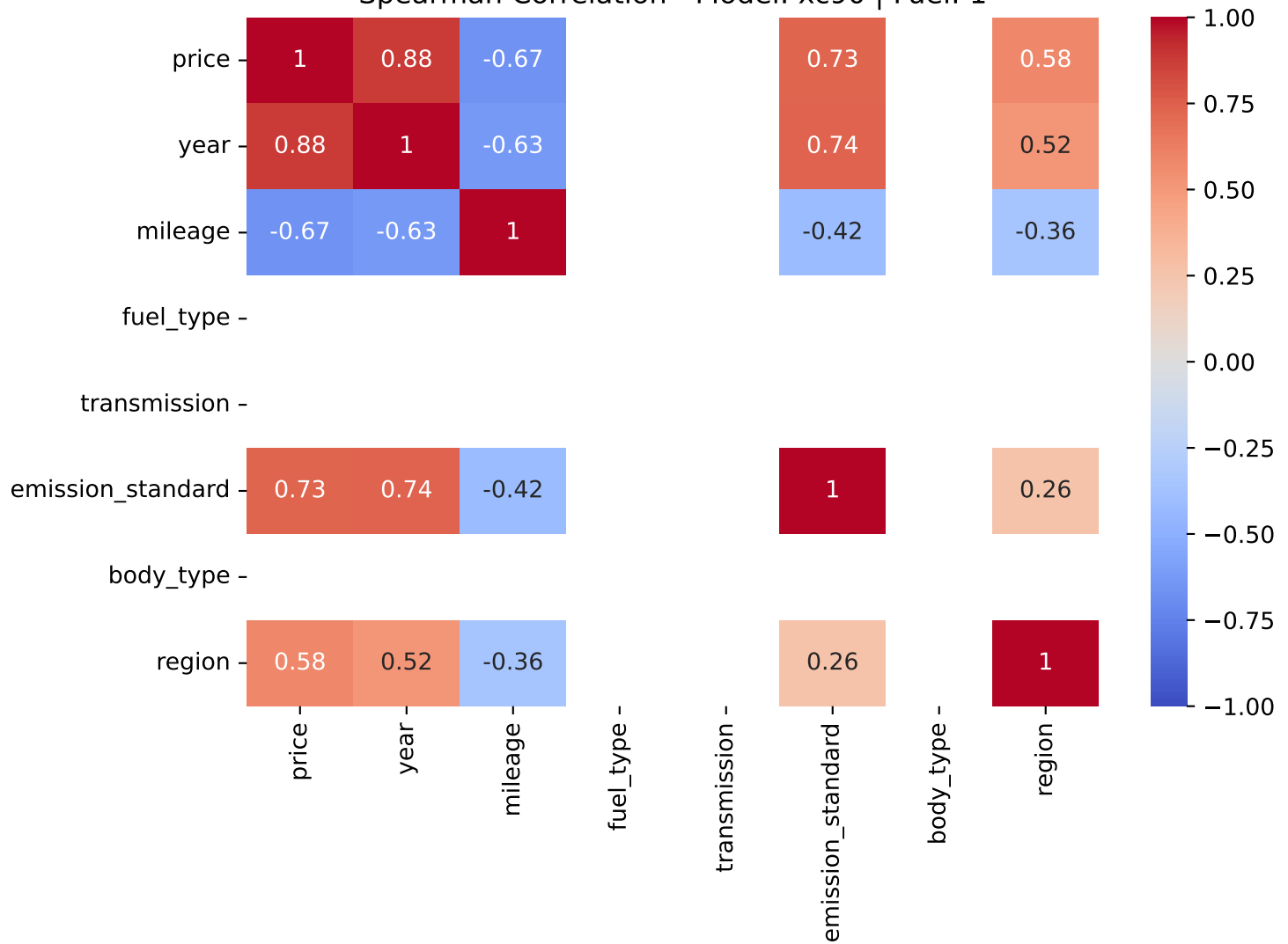
Spearman Correlation - Model: xc90 | Fuel: 1
