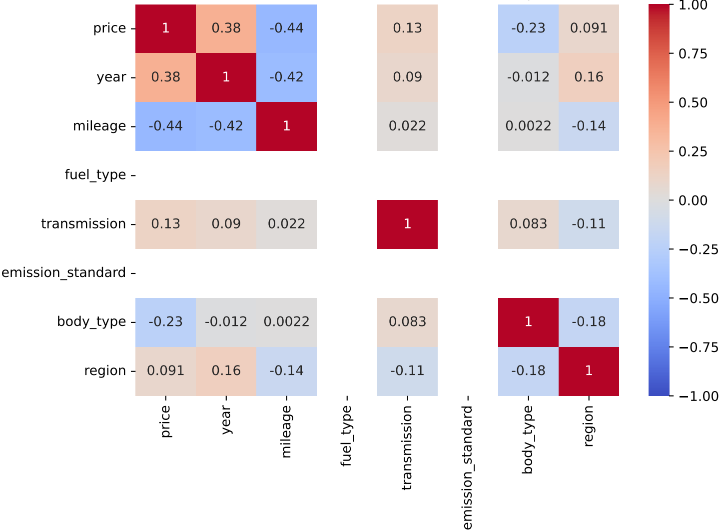
Spearman Correlation - Model: romeo tonale | Fuel: 1
