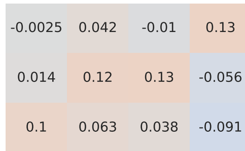
Spearman Correlation - Model: macan | Fuel: 1
