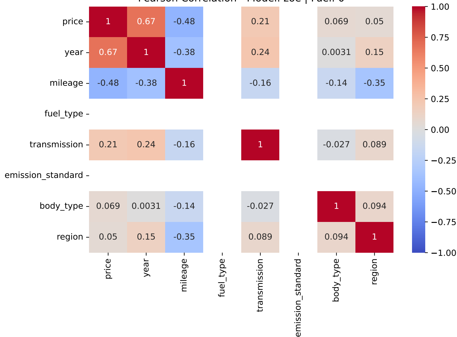
Pearson Correlation - Model: zoe | Fuel: 0
