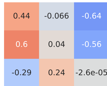
Pearson Correlation - Model: mii | Fuel: 5
