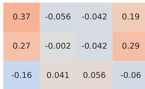
Pearson Correlation - Model: puma | Fuel: 3
