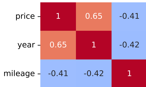
Spearman Correlation - Model: romeo stelvio | Fuel: 2
