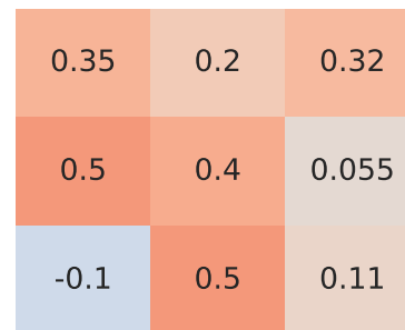
Spearman Correlation - Model: patriot | Fuel: 1
