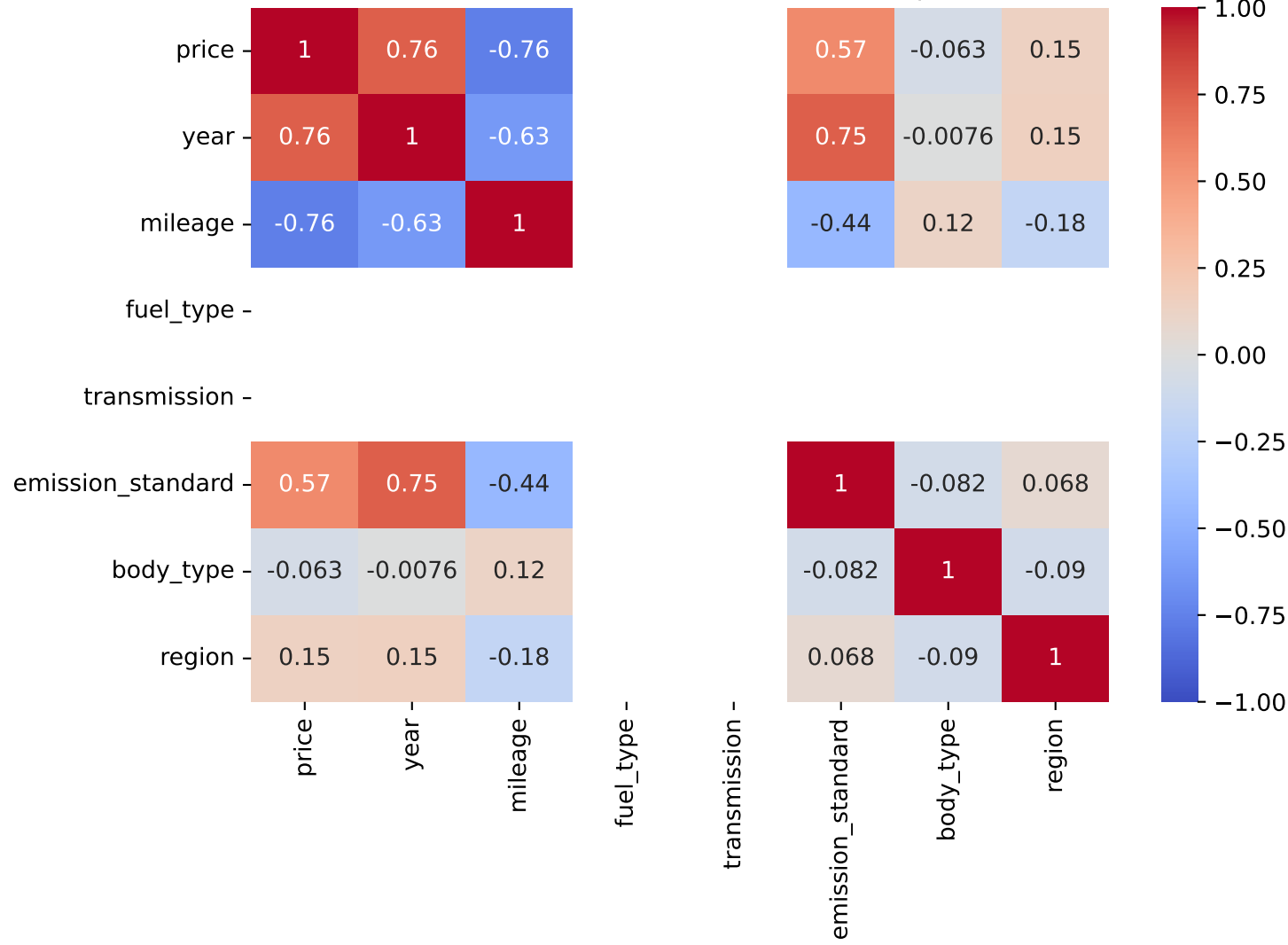
Pearson Correlation - Model: romeo mito | Fuel: 1
