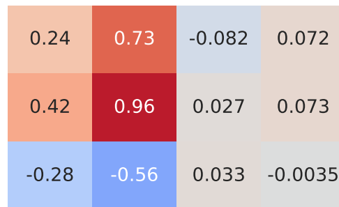
Pearson Correlation - Model: cherokee | Fuel: 1
