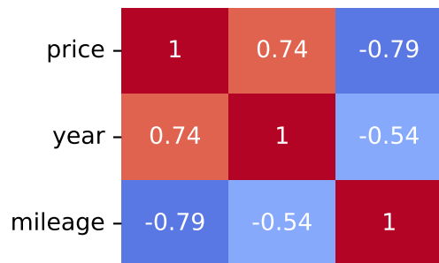
Pearson Correlation - Model: swift | Fuel: 2
