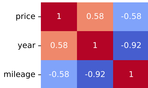
Spearman Correlation - Model: c4 | Fuel: 2
