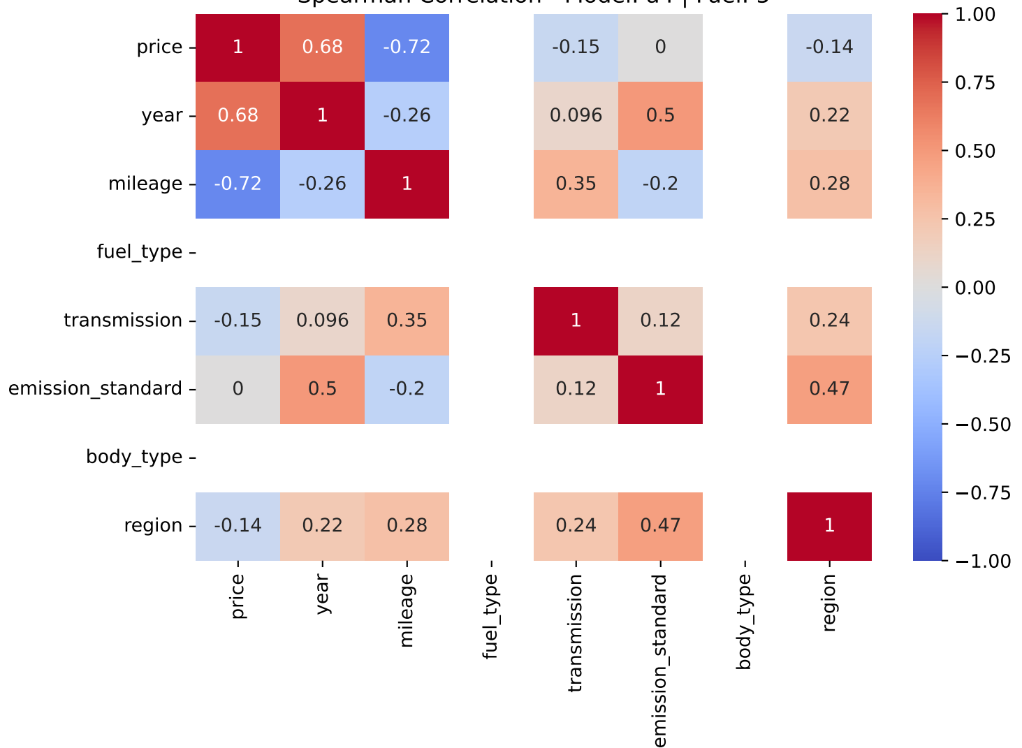
Spearman Correlation - Model: a4 | Fuel: 5
