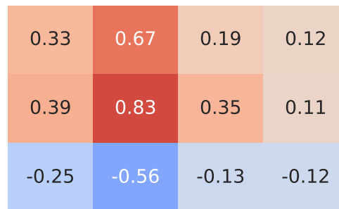
Spearman Correlation - Model: leon | Fuel: 1
