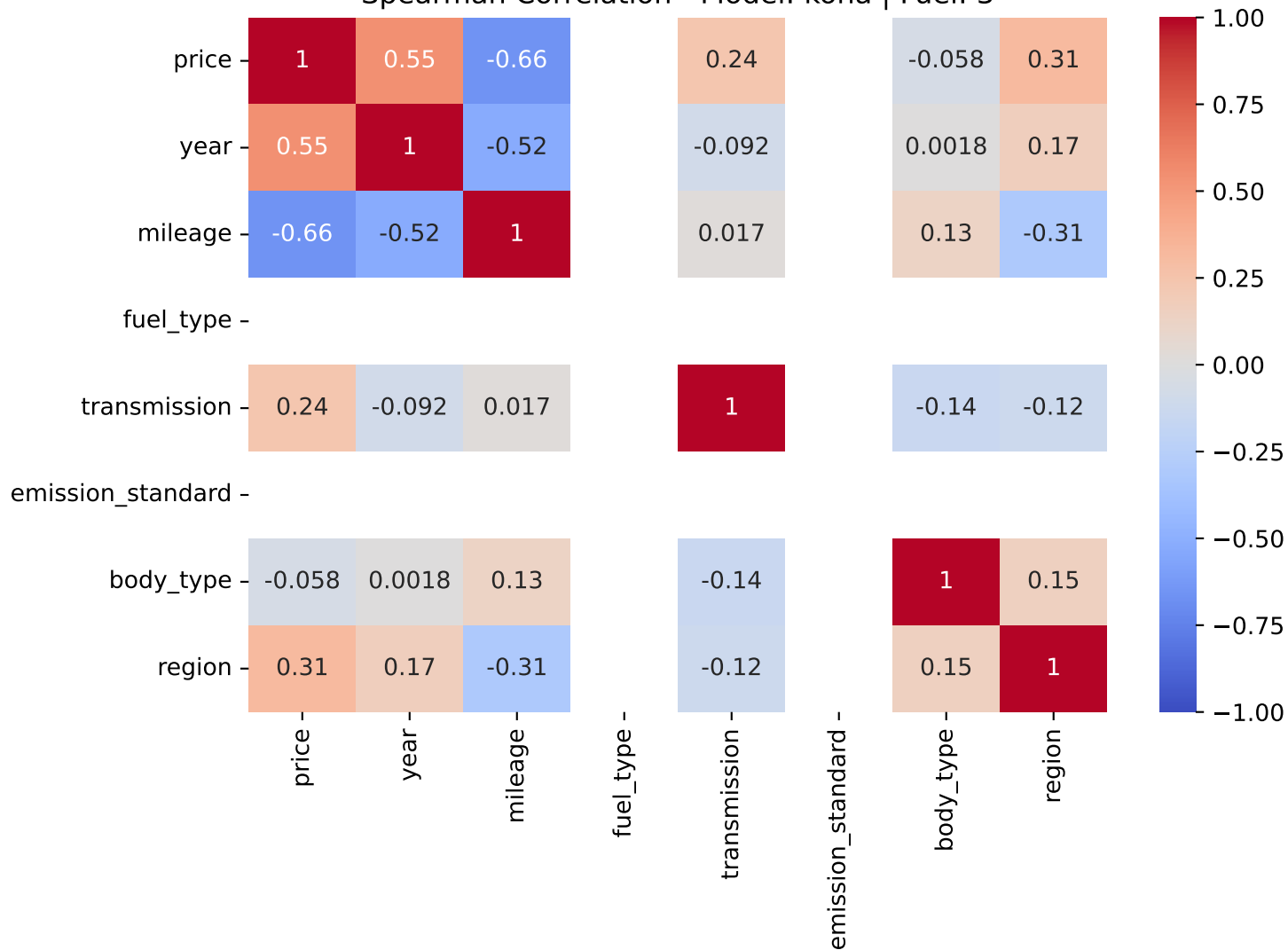
Spearman Correlation - Model: kona | Fuel: 3
