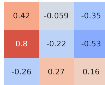
Pearson Correlation - Model: qubo | Fuel: 2
