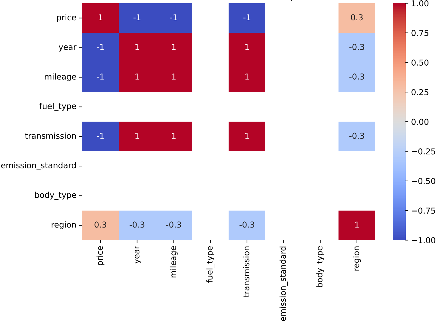
Pearson Correlation - Model: v40 | Fuel: 2
