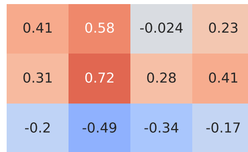
Pearson Correlation - Model: i40 | Fuel: 1
