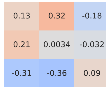
Pearson Correlation - Model: celerio | Fuel: 2
