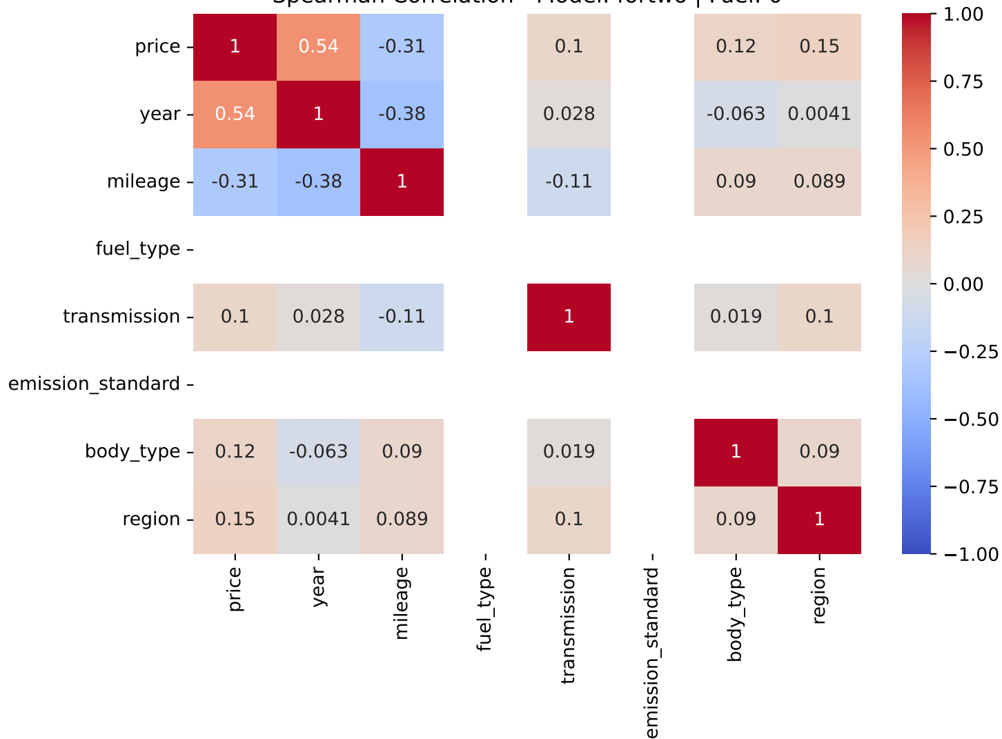
Spearman Correlation - Model: fortwo | Fuel: 0
