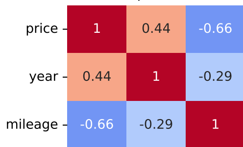
Spearman Correlation - Model: musa | Fuel: 2
