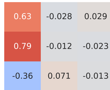
Spearman Correlation - Model: juke | Fuel: 1
