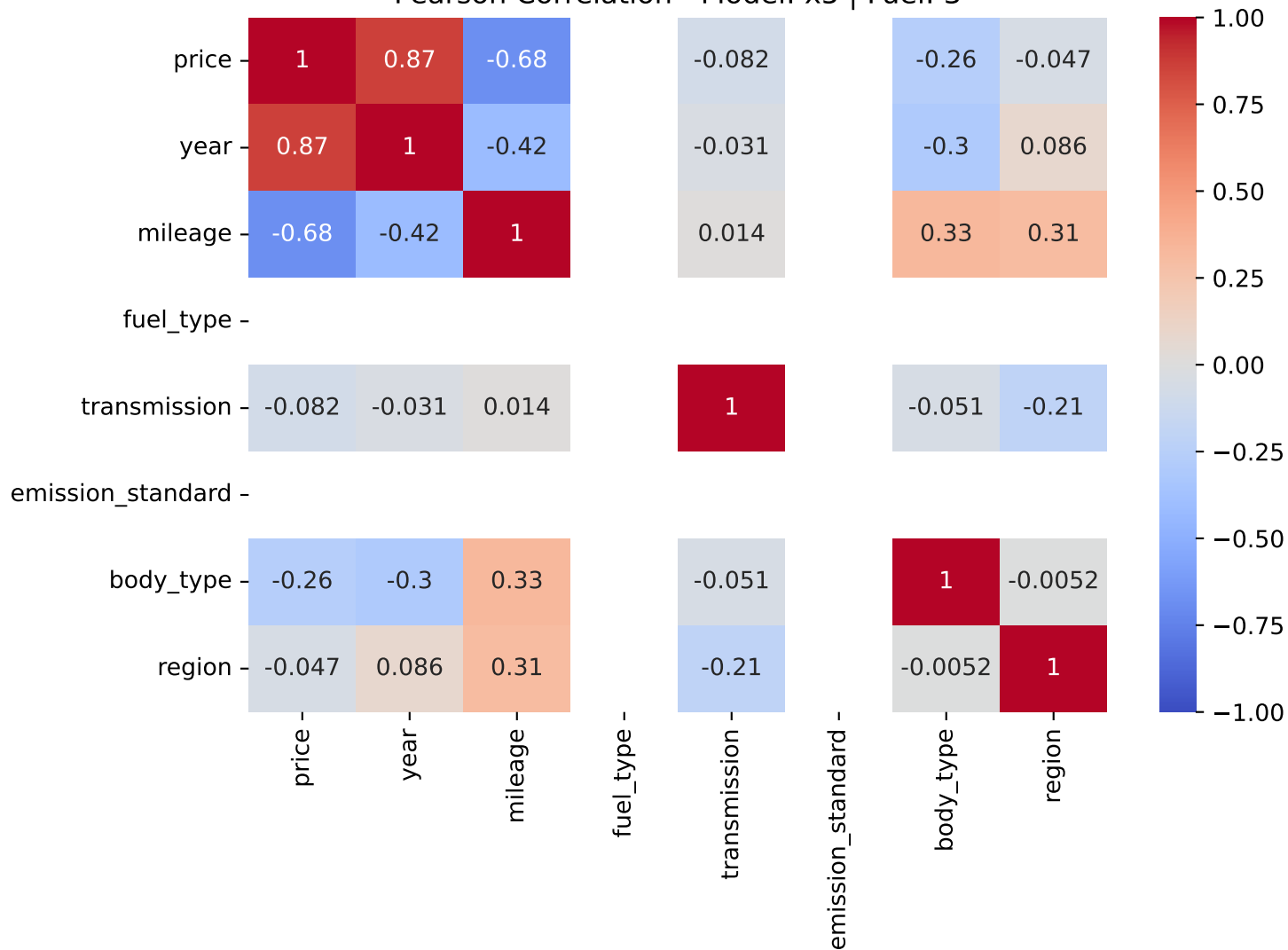
Pearson Correlation - Model: x5 | Fuel: 3
