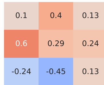
Spearman Correlation - Model: bravo | Fuel: 4
