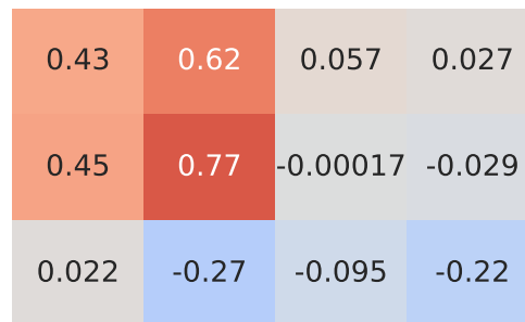
Pearson Correlation - Model: i30 | Fuel: 1
