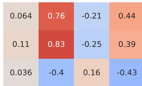
Spearman Correlation - Model: ceed | Fuel: 1
