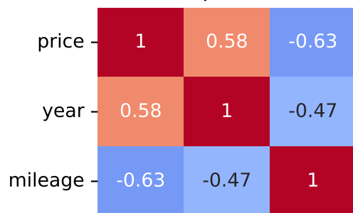
Spearman Correlation - Model: kuga | Fuel: 3
