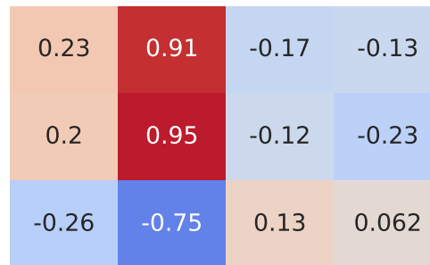
Pearson Correlation - Model: fabia | Fuel: 1
