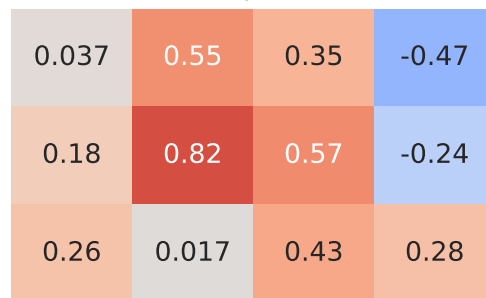
Spearman Correlation - Model: auris | Fuel: 3
