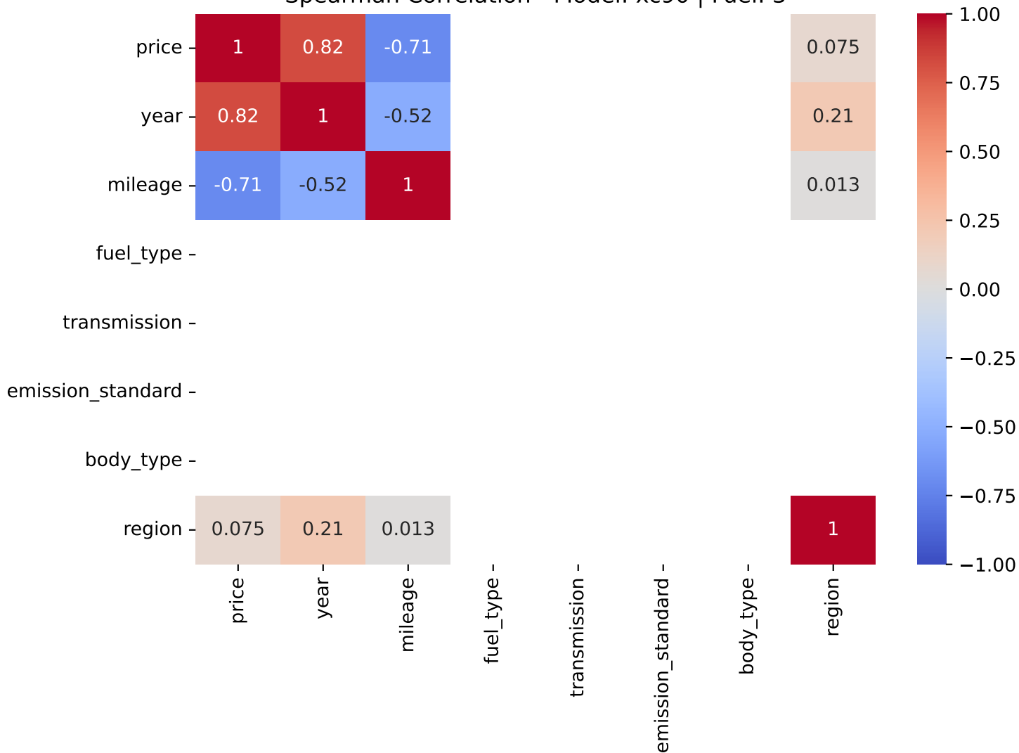
Spearman Correlation - Model: xc90 | Fuel: 3
