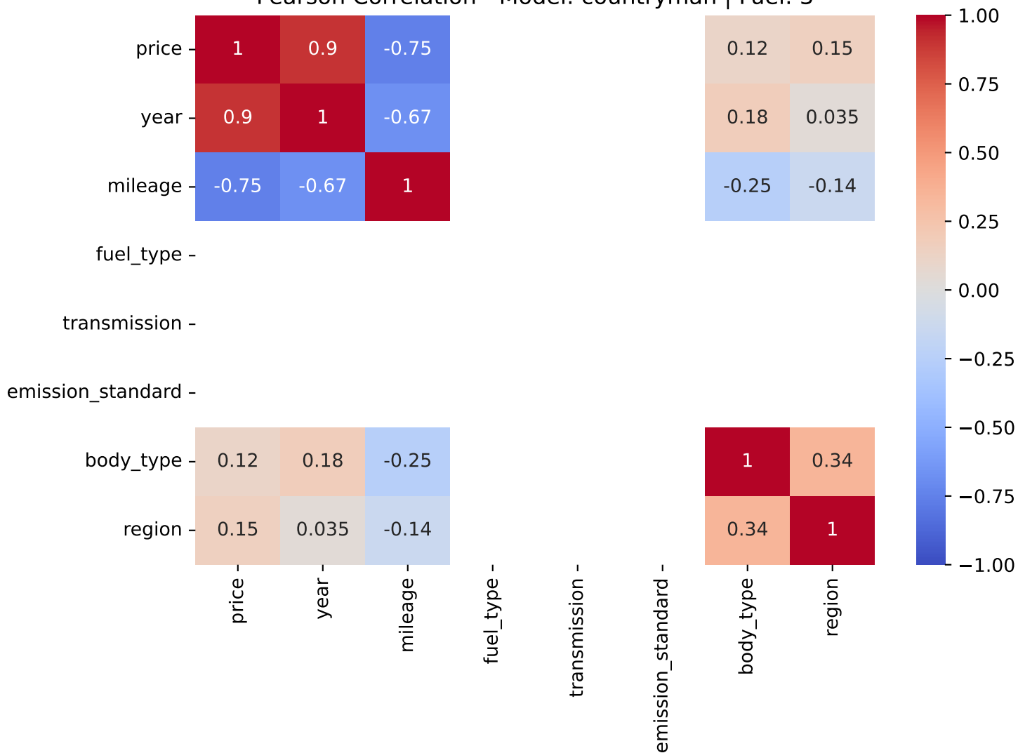
Pearson Correlation - Model: countryman | Fuel: 3
