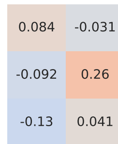
Pearson Correlation - Model: polo | Fuel: 5
