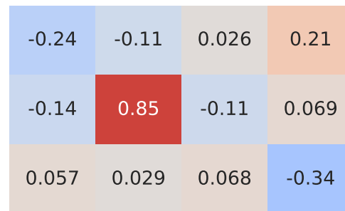
Spearman Correlation - Model: nemo | Fuel: 1
