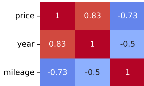
Pearson Correlation - Model: meriva | Fuel: 2
