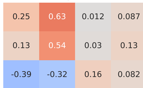
Pearson Correlation - Model: astra | Fuel: 4
