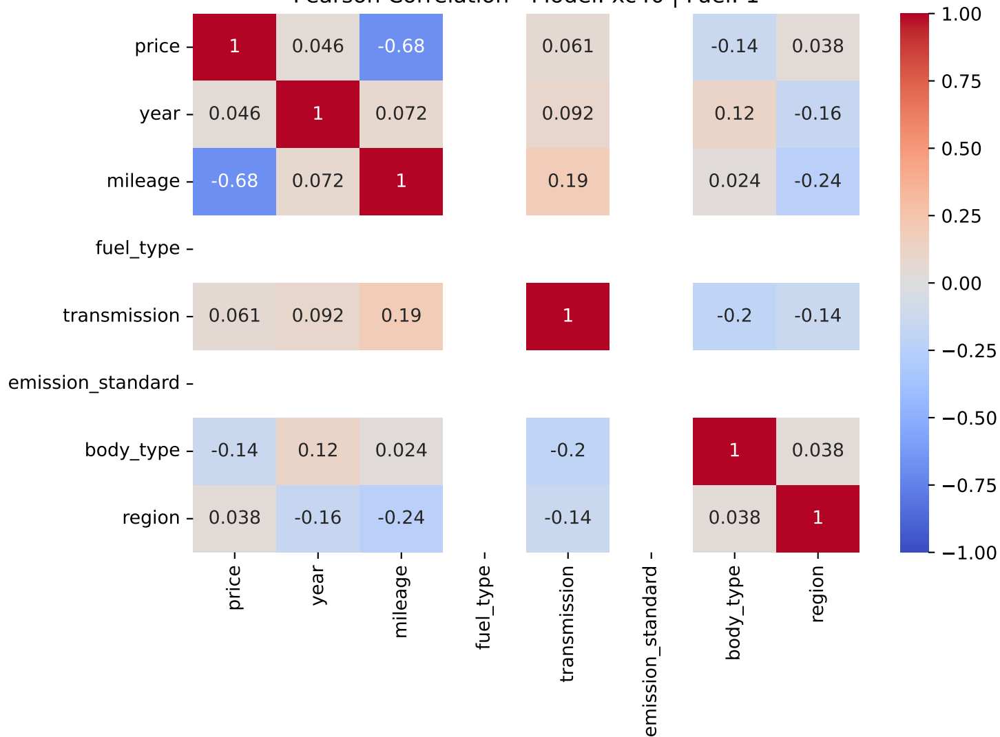
Pearson Correlation - Model: xc40 | Fuel: 1
