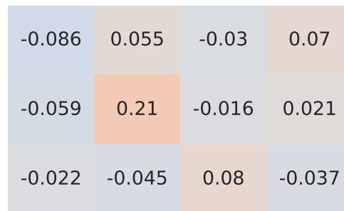
Pearson Correlation - Model: delta | Fuel: 1
