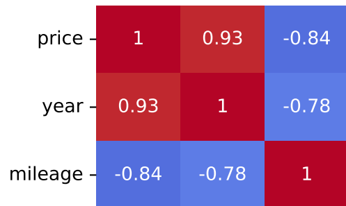
Spearman Correlation - Model: a3 | Fuel: 1
