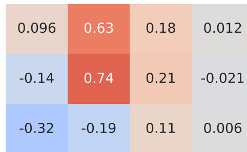
Pearson Correlation - Model: fortwo | Fuel: 1
