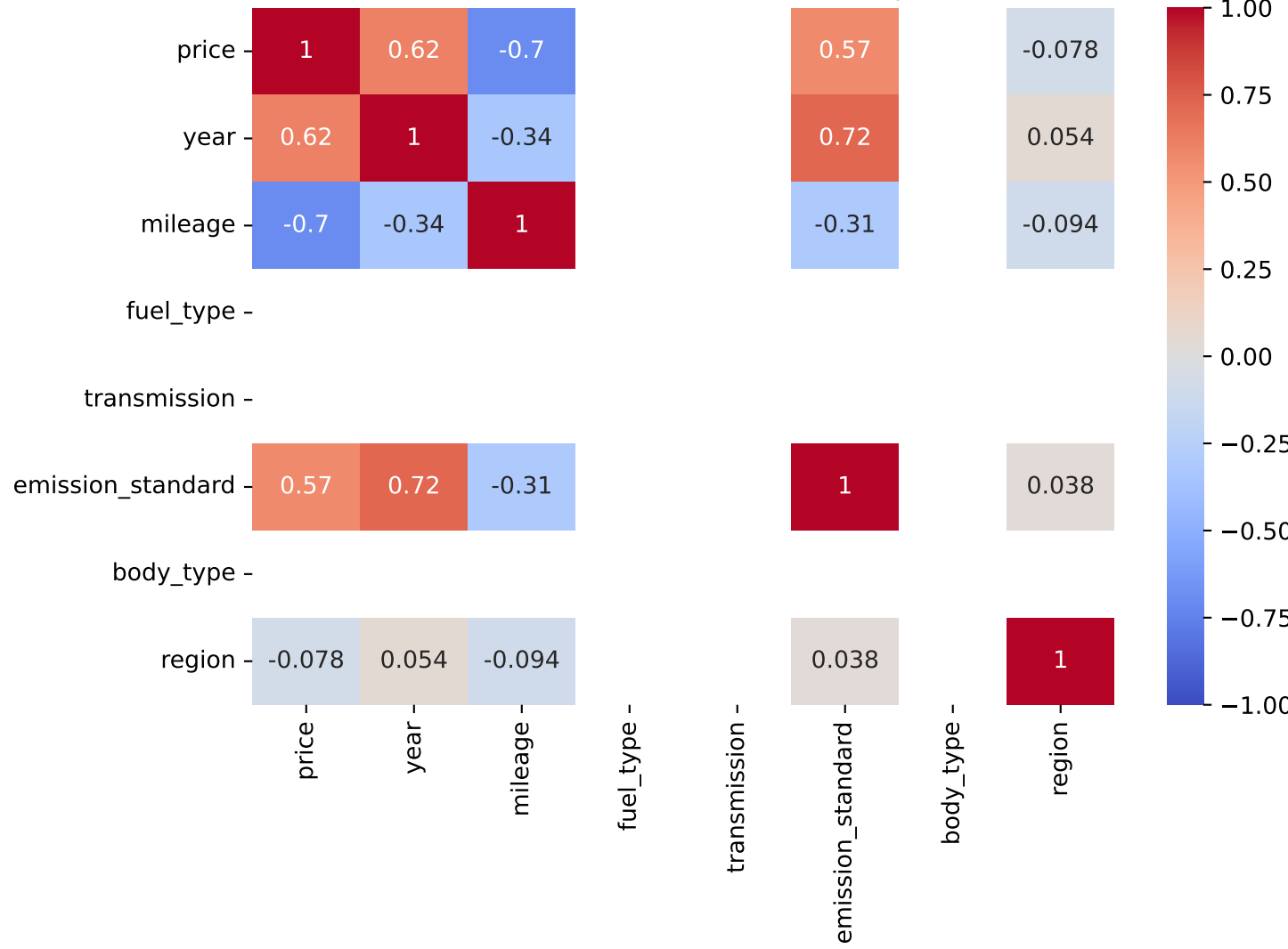
Spearman Correlation - Model: zafira | Fuel: 5
