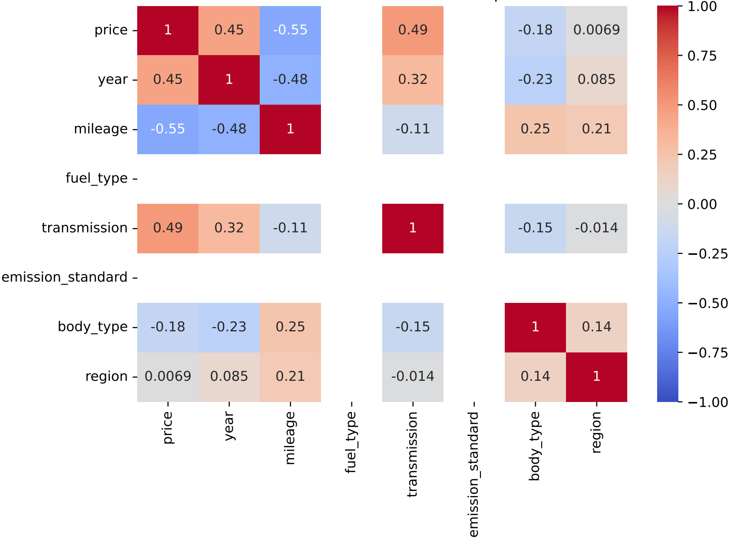
Pearson Correlation - Model: vitara | Fuel: 3
