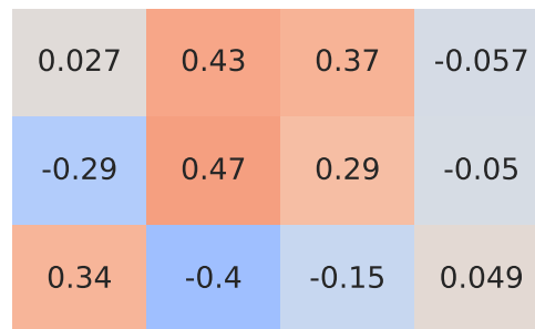
Spearman Correlation - Model: leon | Fuel: 2
