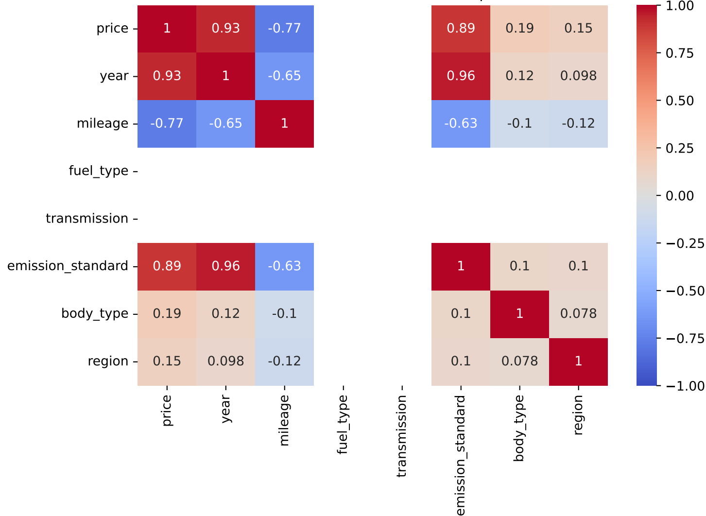
Pearson Correlation - Model: micra | Fuel: 1
