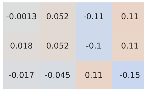
Pearson Correlation - Model: romeo stelvio | Fuel: 1
