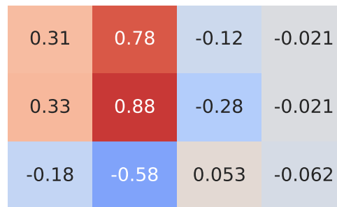
Pearson Correlation - Model: a5 | Fuel: 1
