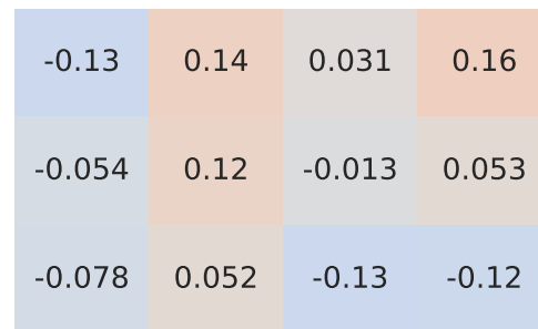
Pearson Correlation - Model: arkana | Fuel: 3
