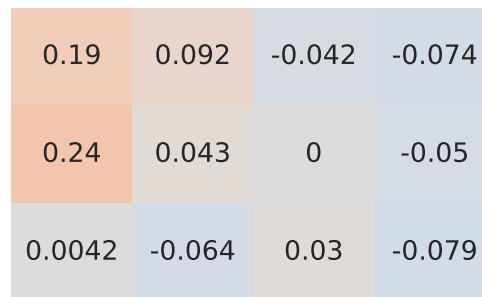
Spearman Correlation - Model: romeo giulia | Fuel: 1
