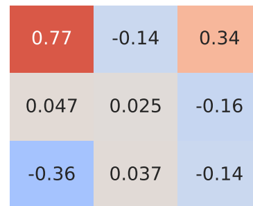
Pearson Correlation - Model: ix20 | Fuel: 2
