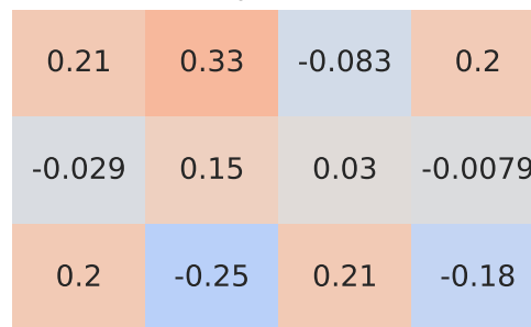
Pearson Correlation - Model: karl | Fuel: 2
