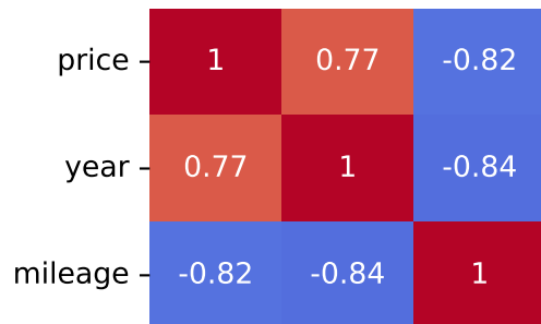
Spearman Correlation - Model: karoq | Fuel: 1
