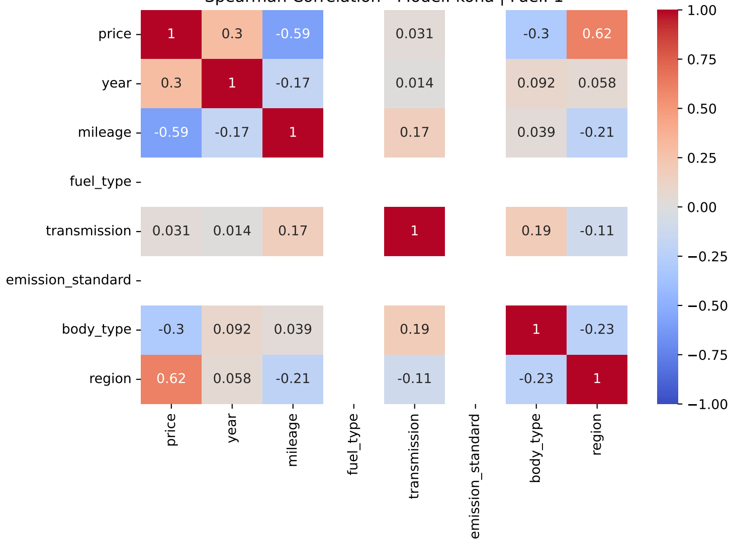
Spearman Correlation - Model: kona | Fuel: 1
