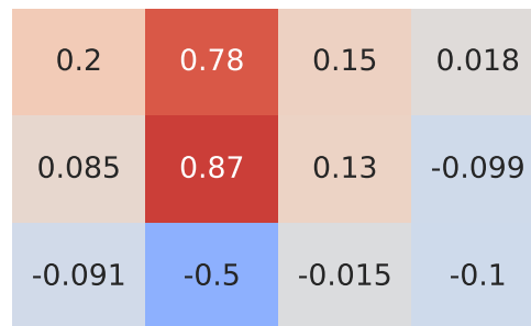
Pearson Correlation - Model: twingo | Fuel: 2
