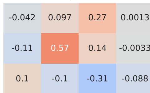
Spearman Correlation - Model: c2 | Fuel: 2
