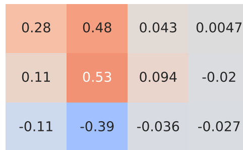
Spearman Correlation - Model: 208 | Fuel: 2
