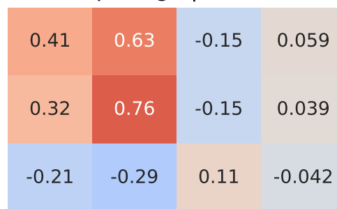
Spearman Correlation - Model: sportage | Fuel: 1
