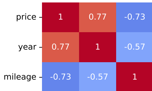
Pearson Correlation - Model: cherokee | Fuel: 1
