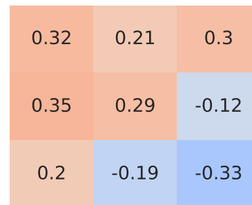
Spearman Correlation - Model: fusion | Fuel: 1
