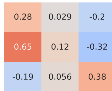
Pearson Correlation - Model: 307 | Fuel: 1
