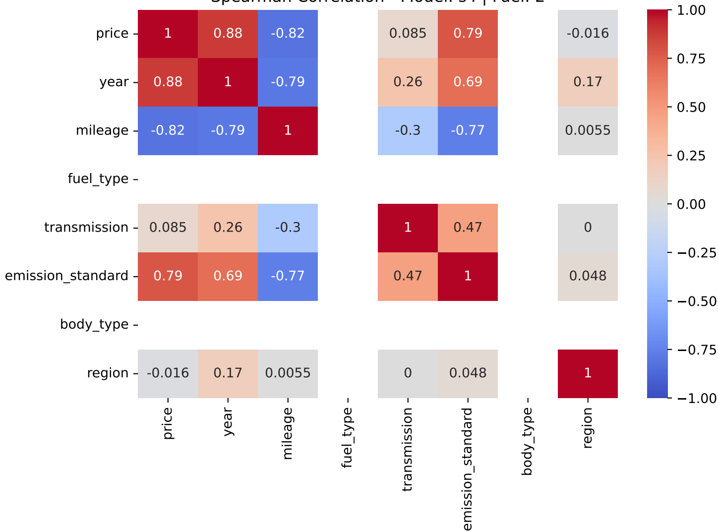
Spearman Correlation - Model: s4 | Fuel: 2
