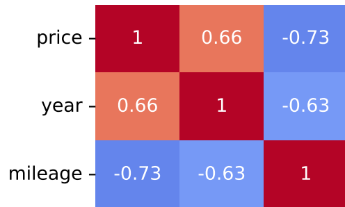
Spearman Correlation - Model: grand vitara | Fuel: 2
