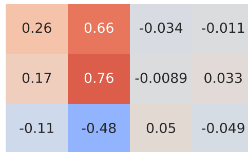
Pearson Correlation - Model: 500 | Fuel: 1
