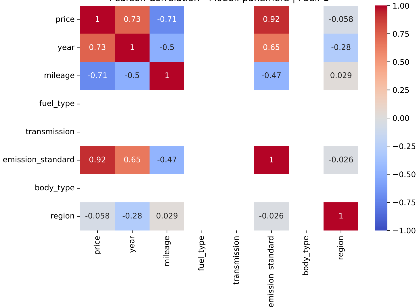
Pearson Correlation - Model: panamera | Fuel: 1
