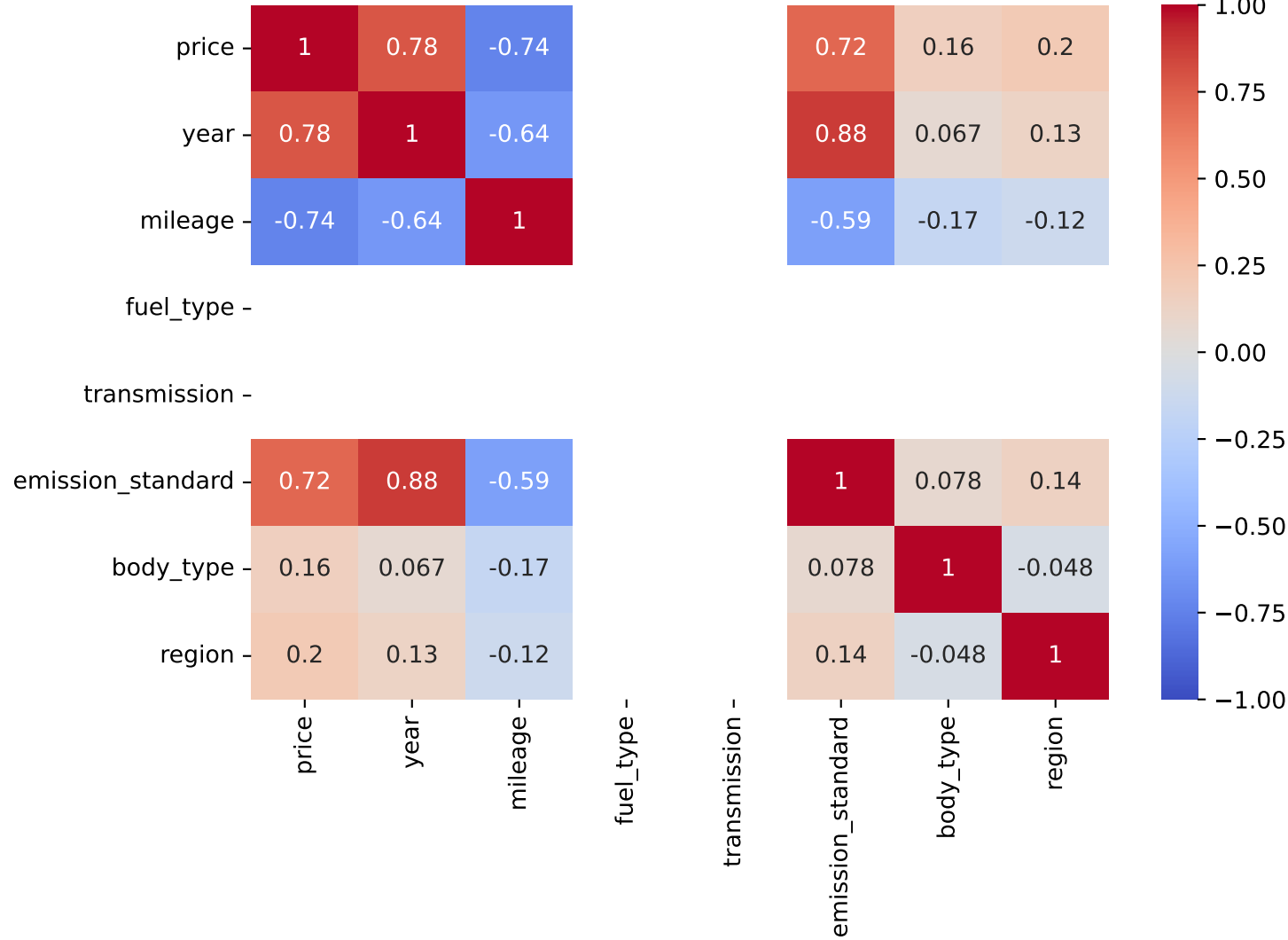
Spearman Correlation - Model: kangoo | Fuel: 1
