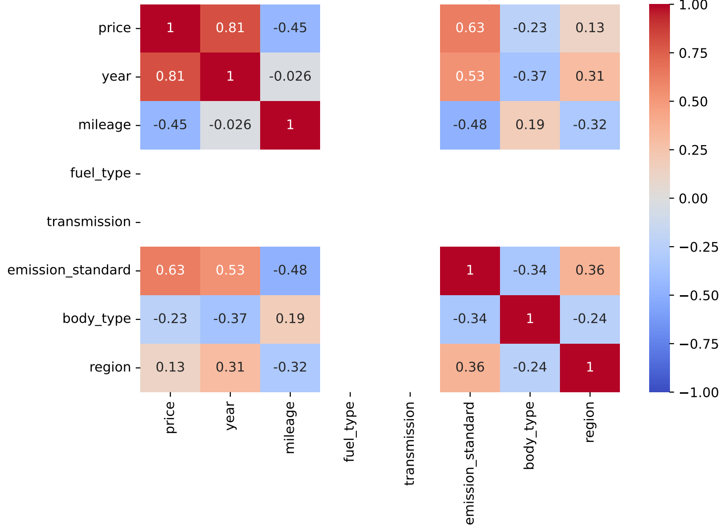
Pearson Correlation - Model: focus | Fuel: 4
