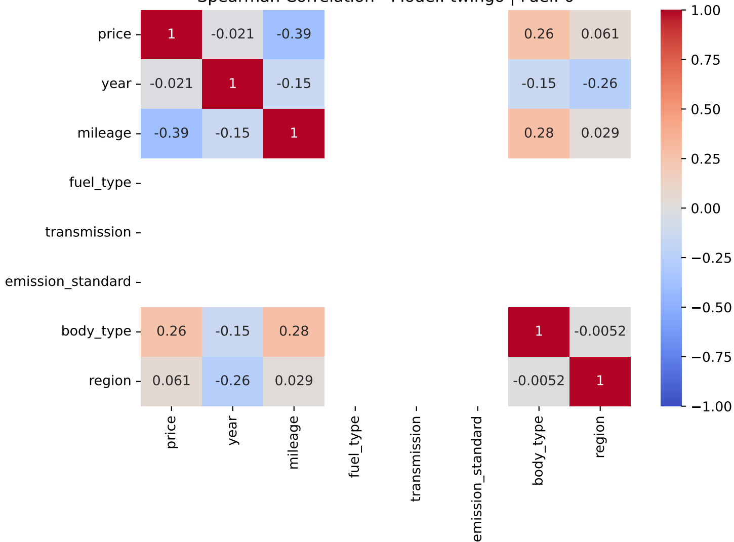
Spearman Correlation - Model: twingo | Fuel: 0
