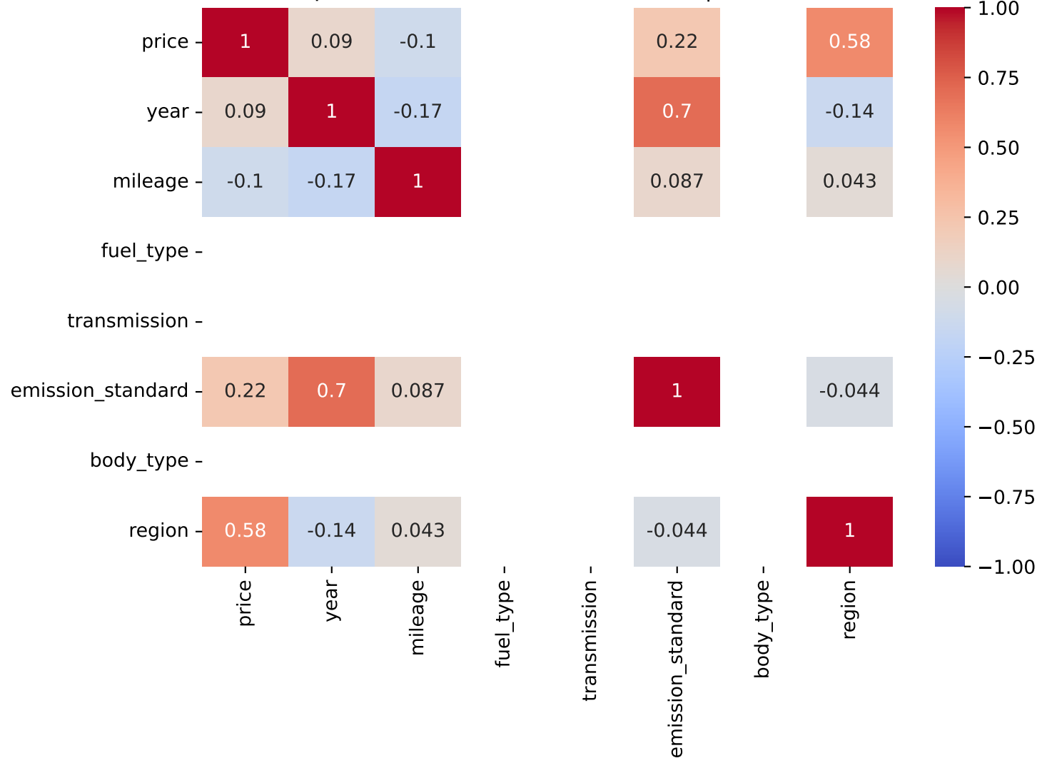
Spearman Correlation - Model: c30 | Fuel: 1
