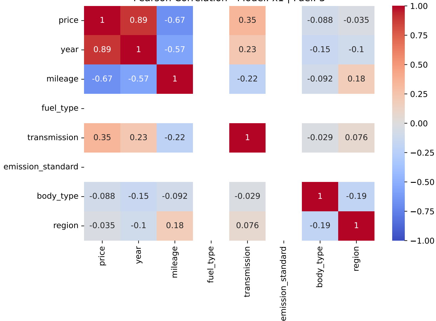
Pearson Correlation - Model: x1 | Fuel: 3
