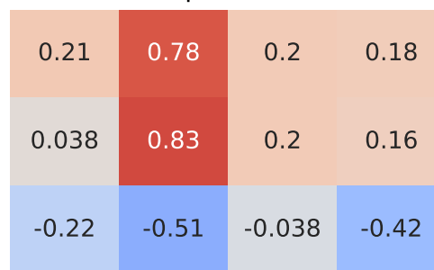
Pearson Correlation - Model: a7 | Fuel: 1
