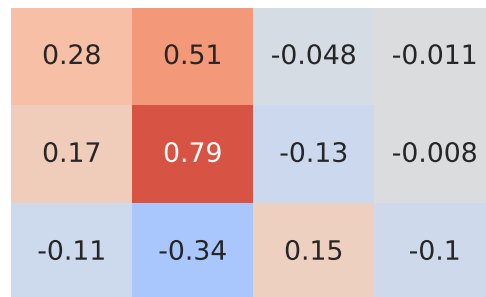
Spearman Correlation - Model: a1 | Fuel: 1
