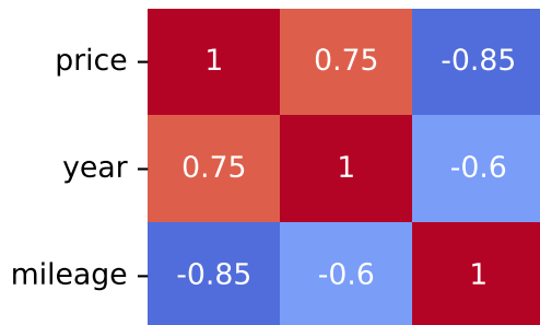
Pearson Correlation - Model: c2 | Fuel: 1
