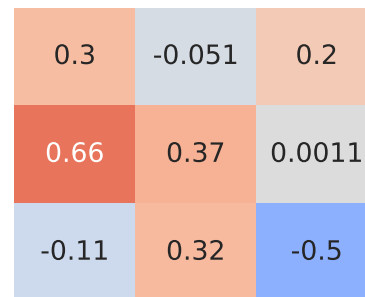
Spearman Correlation - Model: stilo | Fuel: 1
