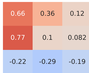
Pearson Correlation - Model: panda 4x4 | Fuel: 1
