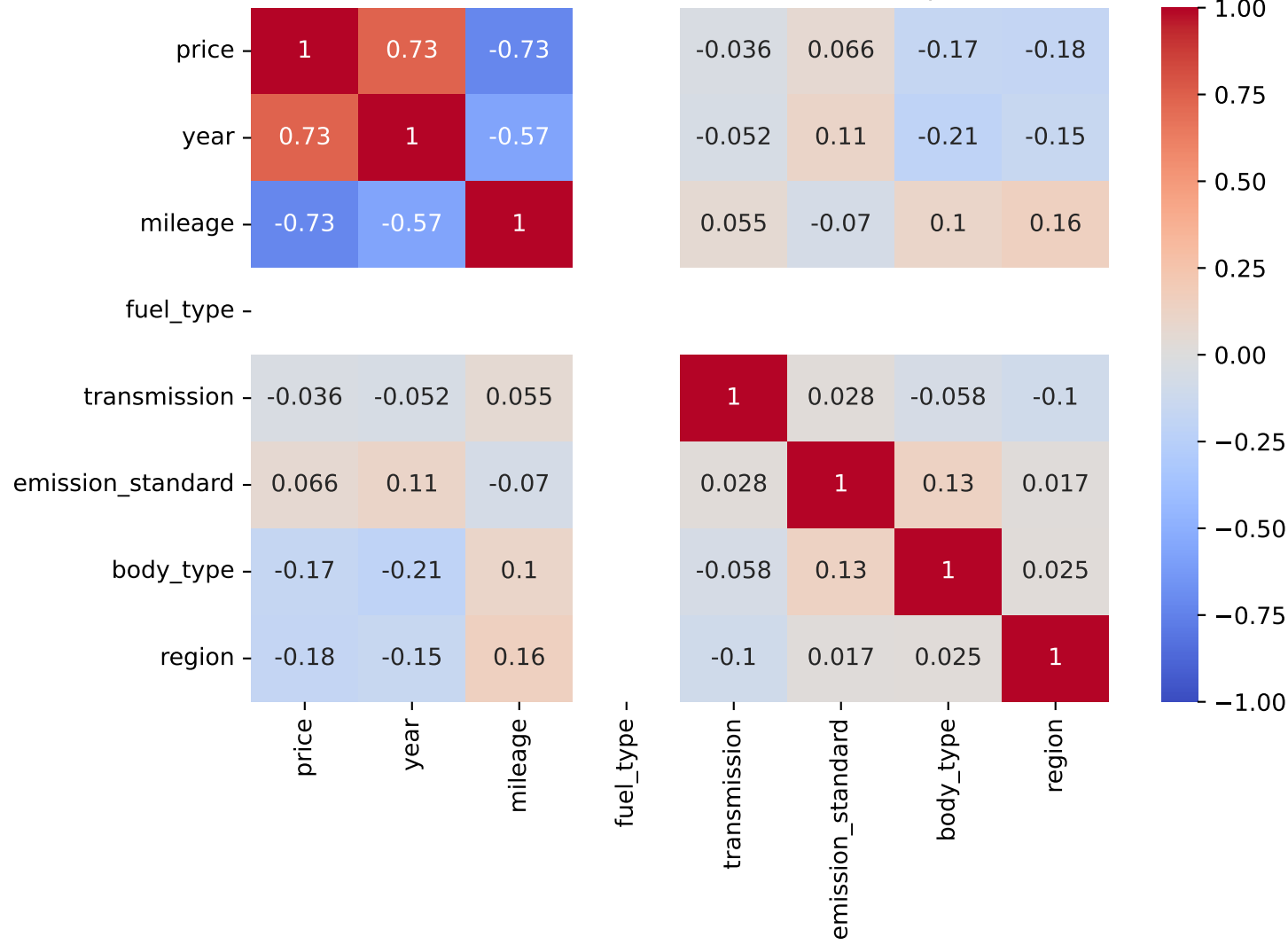
Spearman Correlation - Model: c3 aircross | Fuel: 1
