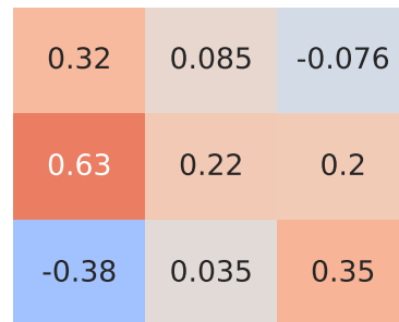
Spearman Correlation - Model: 500I | Fuel: 5
