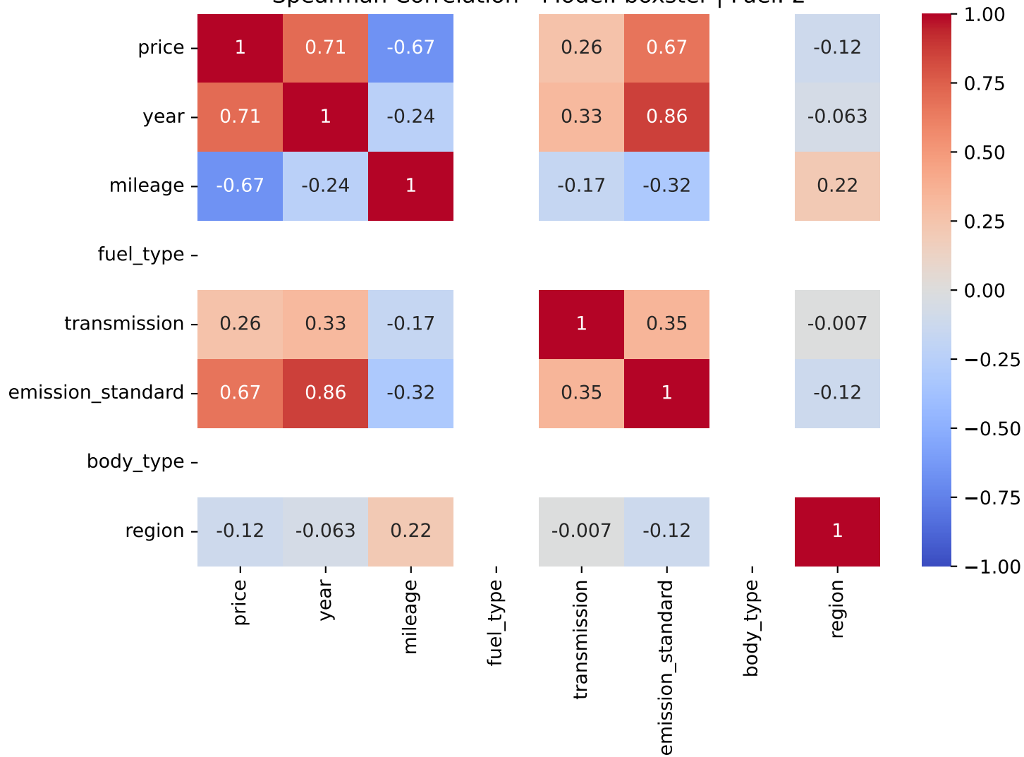
Spearman Correlation - Model: boxster | Fuel: 2
