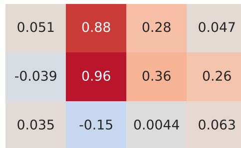
Pearson Correlation - Model: panamera | Fuel: 2
