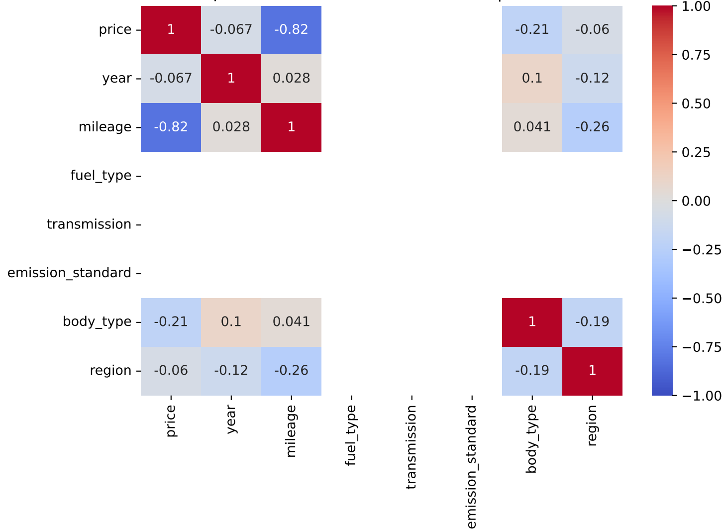
Spearman Correlation - Model: astra | Fuel: 5
