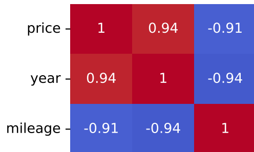
Pearson Correlation - Model: berlingo | Fuel: 2
