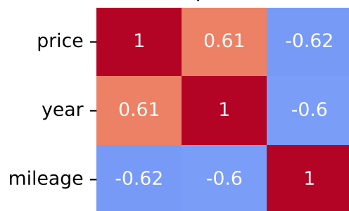
Spearman Correlation - Model: puma | Fuel: 3
