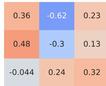
Spearman Correlation - Model: c3 picasso | Fuel: 4
