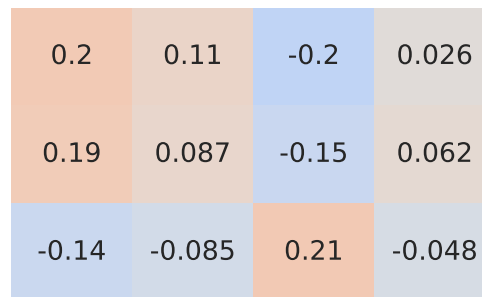
Spearman Correlation - Model: x4 | Fuel: 1
