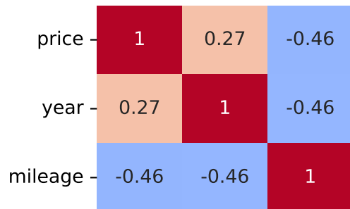
Pearson Correlation - Model: golf | Fuel: 4
