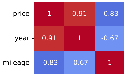
Pearson Correlation - Model: espace | Fuel: 1
