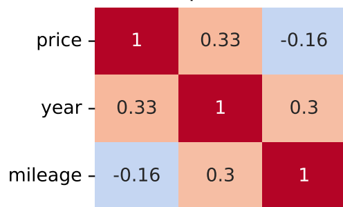
Spearman Correlation - Model: croma | Fuel: 1
