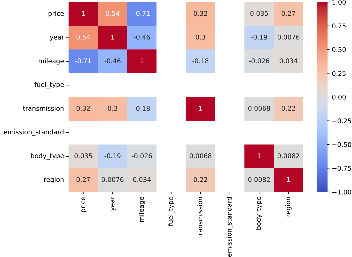
Pearson Correlation - Model: ateca | Fuel: 1
