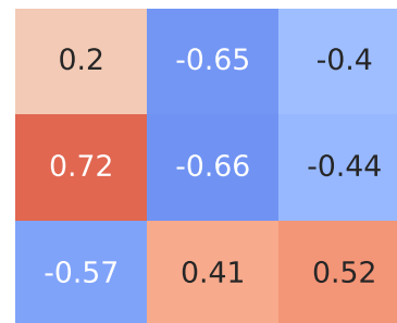
Pearson Correlation - Model: ibiza | Fuel: 5
