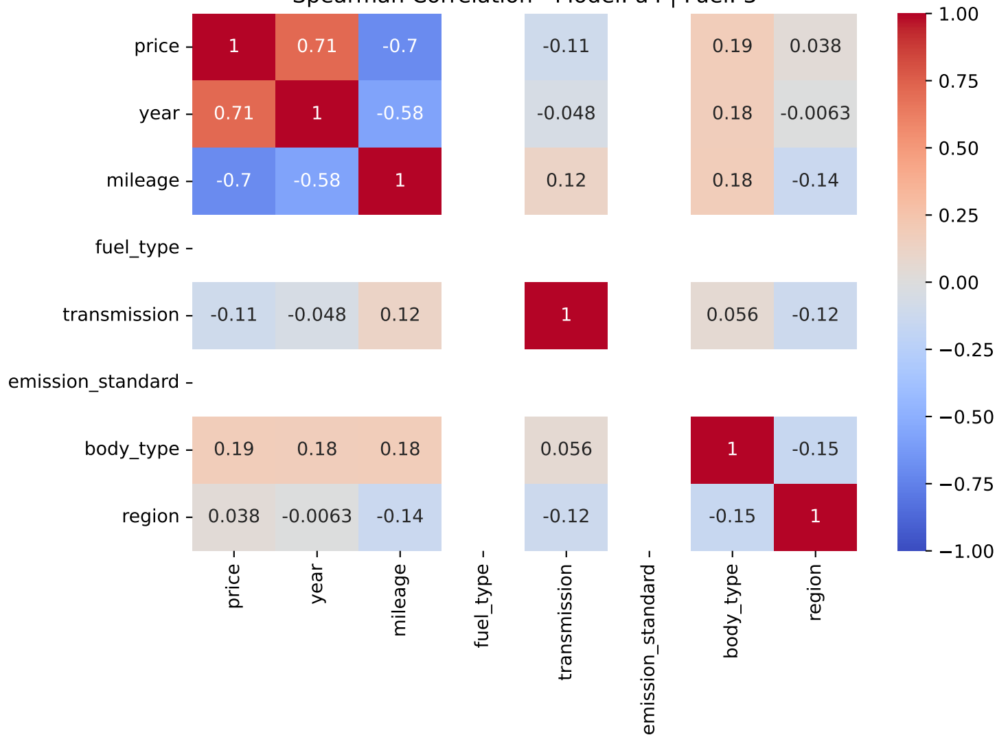
Spearman Correlation - Model: a4 | Fuel: 3
