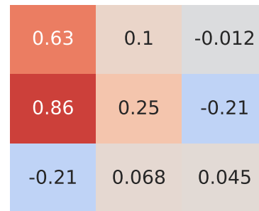
Spearman Correlation - Model: rio | Fuel: 1
