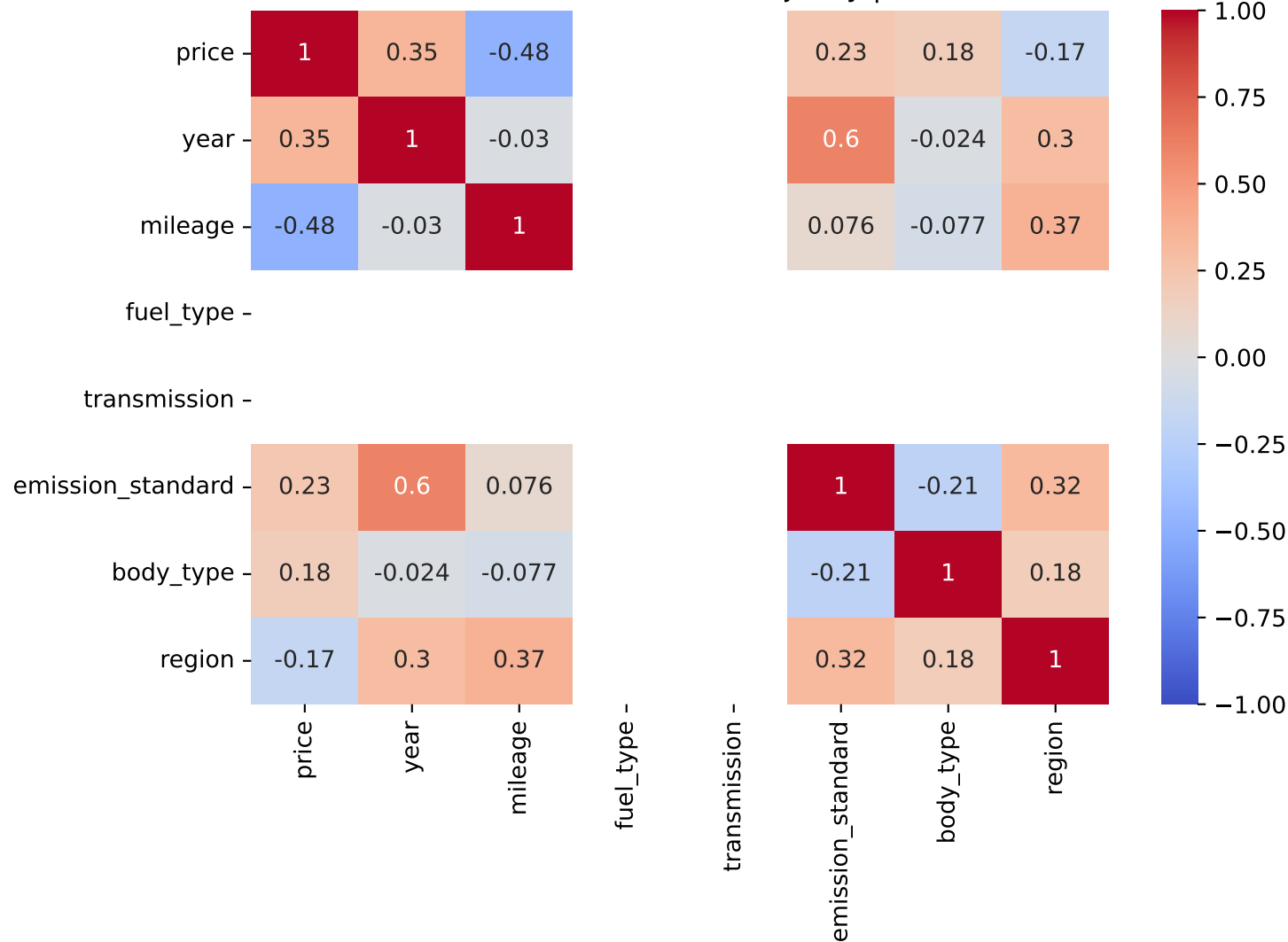
Pearson Correlation - Model: jimny | Fuel: 1
