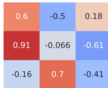
Pearson Correlation - Model: c4 aircross | Fuel: 1
