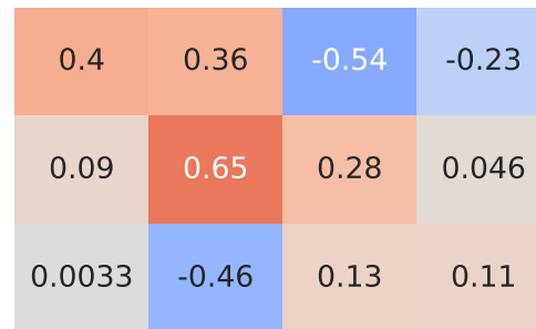
Spearman Correlation - Model: transit | Fuel: 1
