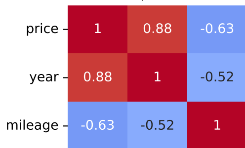
Spearman Correlation - Model: kuga | Fuel: 2
