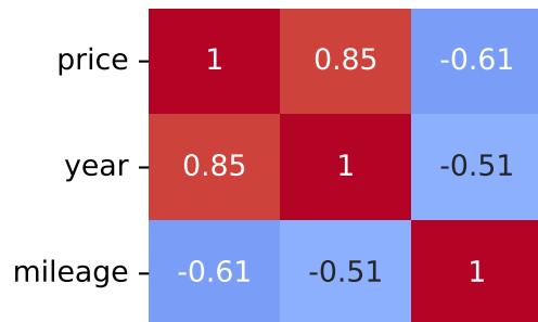
Spearman Correlation - Model: c2 | Fuel: 1
