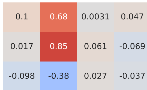
Spearman Correlation - Model: meriva | Fuel: 1
