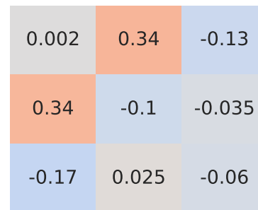
Spearman Correlation - Model: multipa | Fuel: 5
