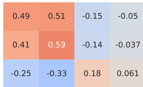
Spearman Correlation - Model: 2008 | Fuel: 1
