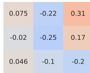
Pearson Correlation - Model: c2 | Fuel: 1
