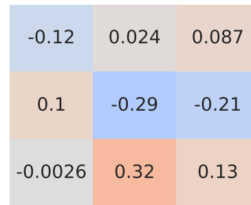
Spearman Correlation - Model: panda cross | Fuel: 2
