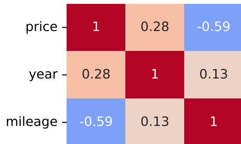
Pearson Correlation - Model: fusion | Fuel: 1
