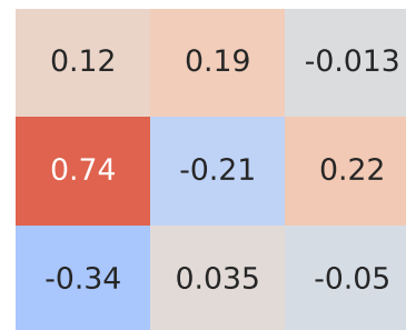
Pearson Correlation - Model: 206 | Fuel: 2
