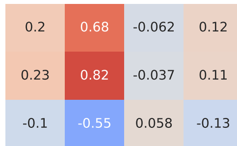
Pearson Correlation - Model: kuga | Fuel: 1
