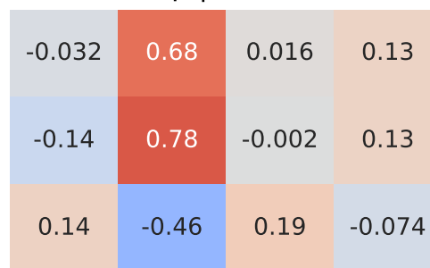
Spearman Correlation - Model: up | Fuel: 2
