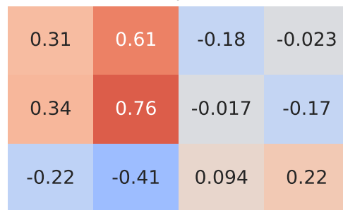
Spearman Correlation - Model: zafira | Fuel: 1
