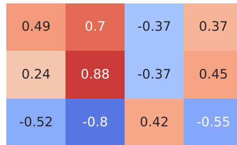
Pearson Correlation - Model: tucson | Fuel: 2
