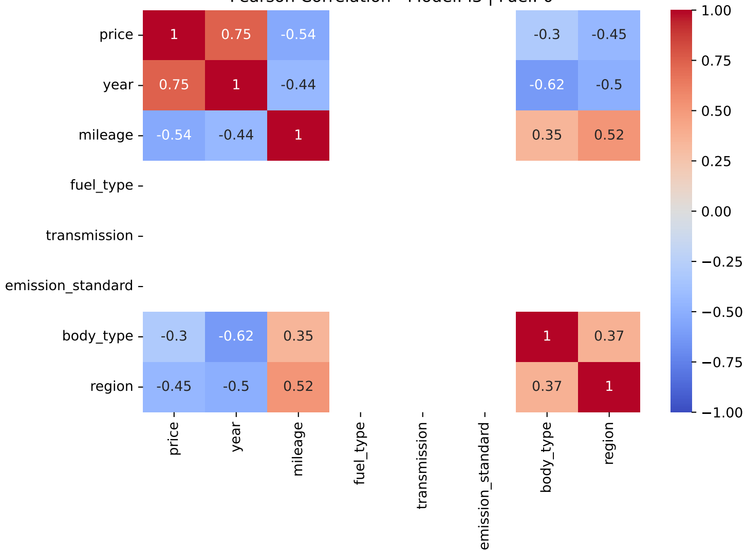
Pearson Correlation - Model: i3 | Fuel: 0
