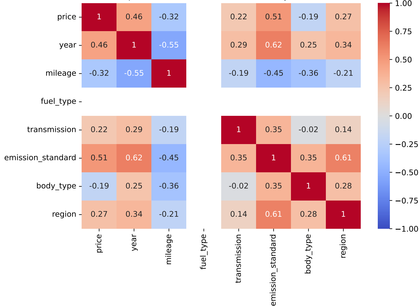
Spearman Correlation - Model: i40 | Fuel: 1
