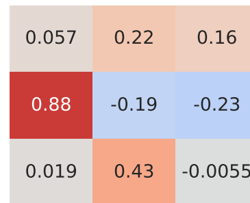
Spearman Correlation - Model: terrano | Fuel: 1
