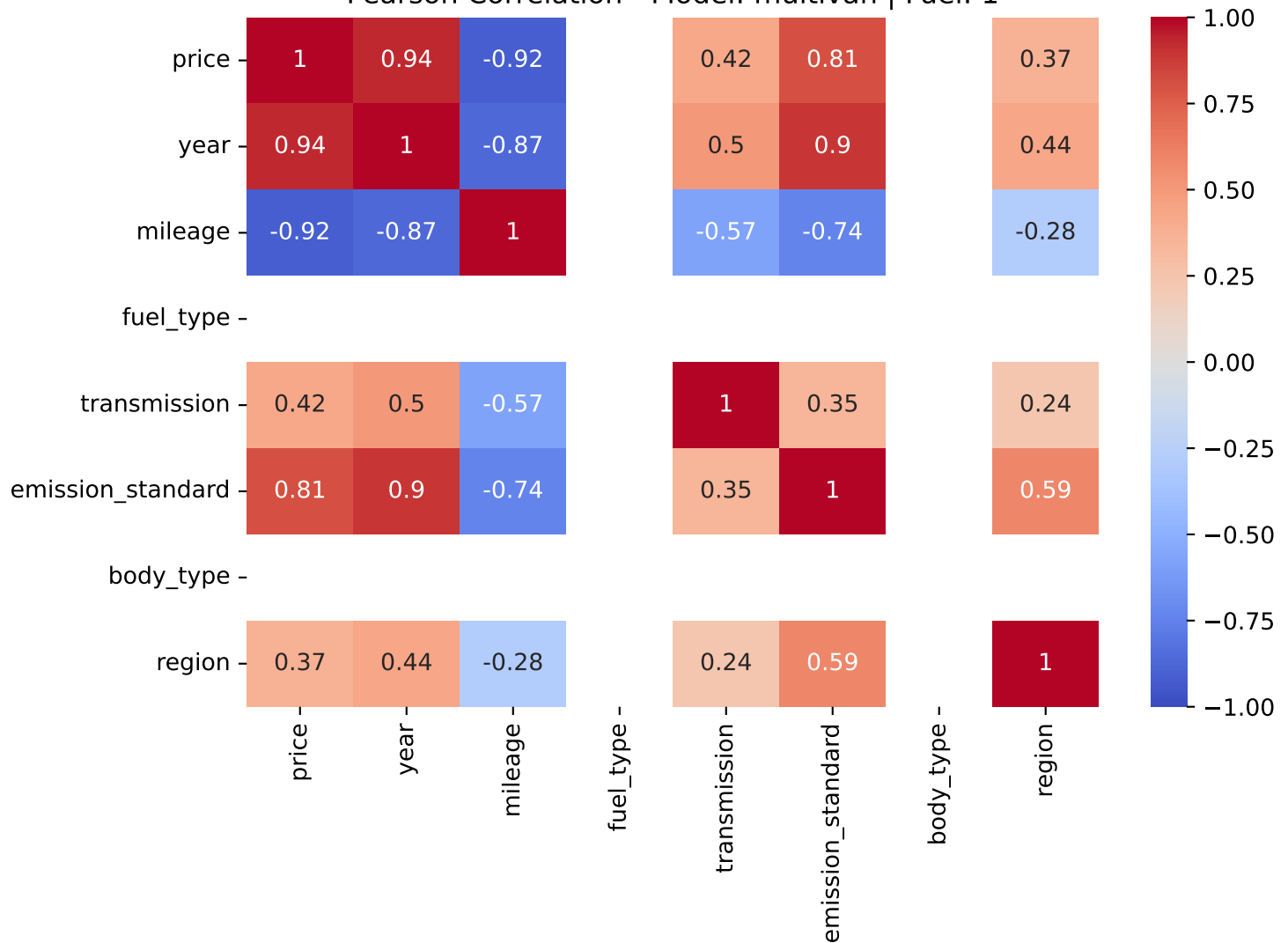
Pearson Correlation - Model: multivan | Fuel: 1
