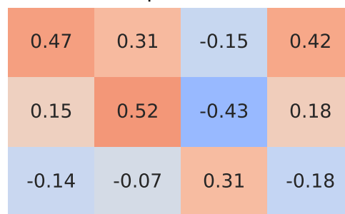
Pearson Correlation - Model: a5 | Fuel: 2
