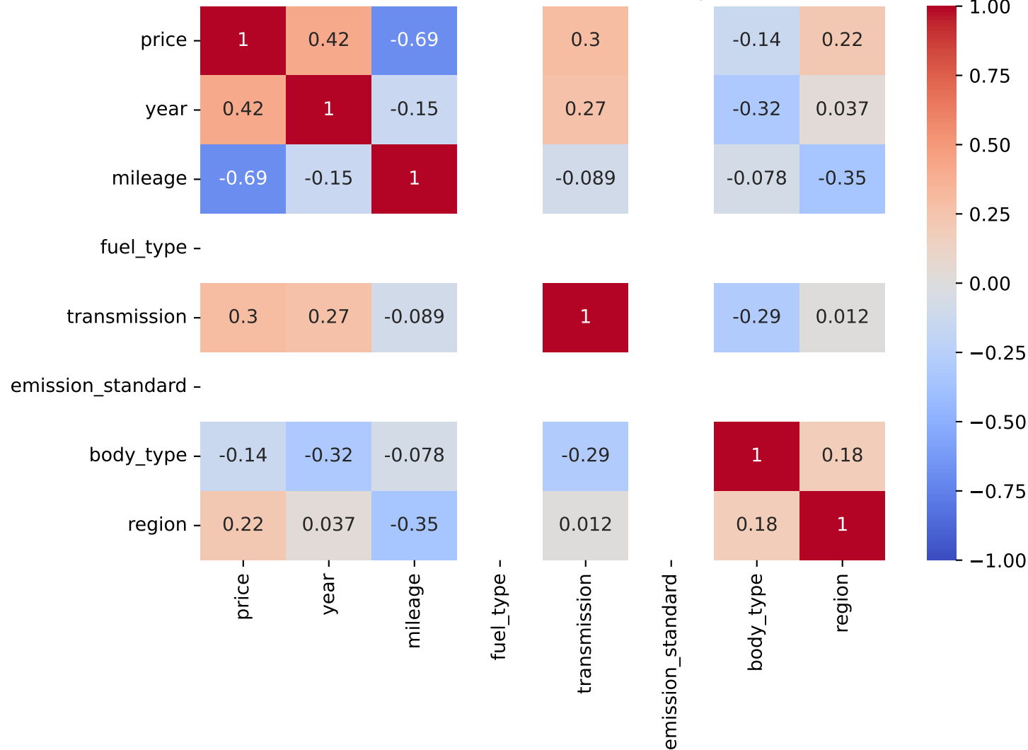
Pearson Correlation - Model: arona | Fuel: 1
