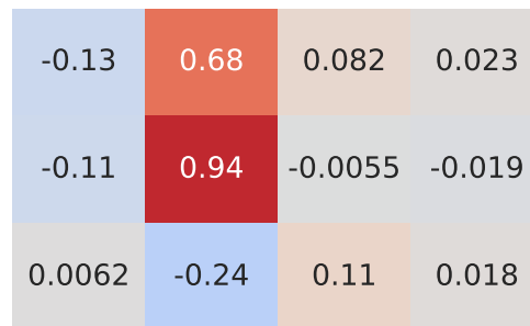
Spearman Correlation - Model: ka | Fuel: 2
