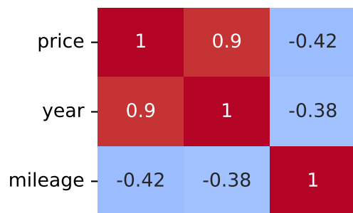
Pearson Correlation - Model: kadjar | Fuel: 2
