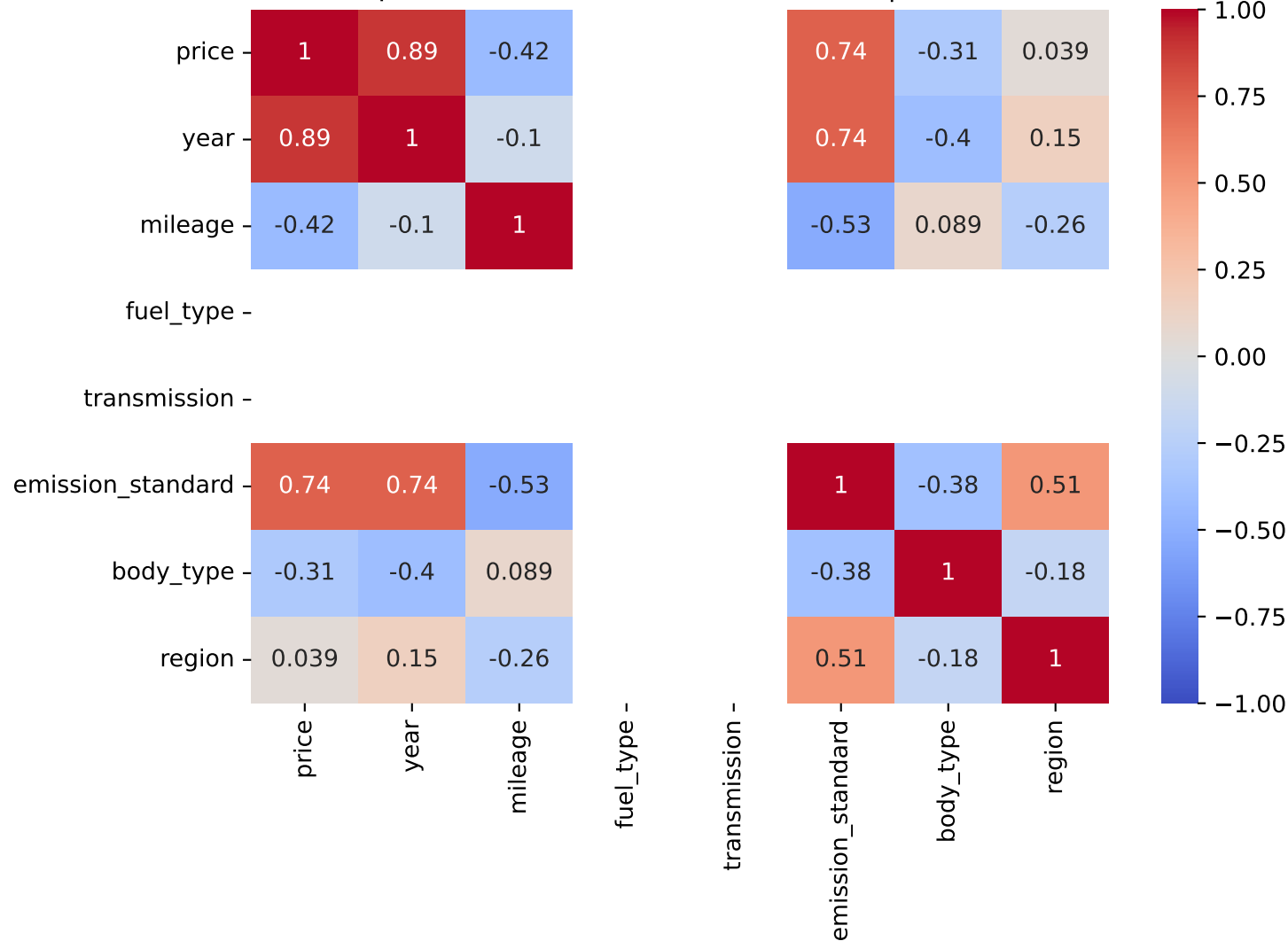
Spearman Correlation - Model: focus | Fuel: 4
