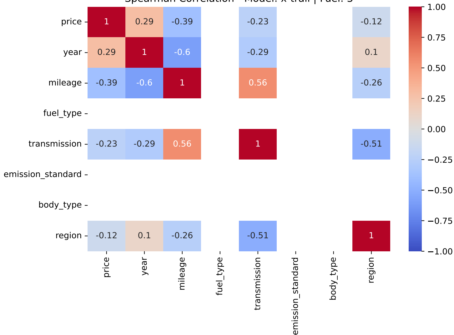
Spearman Correlation - Model: x-trail | Fuel: 3
