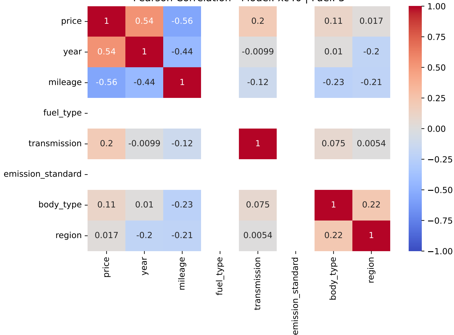
Pearson Correlation - Model: xc40 | Fuel: 3
