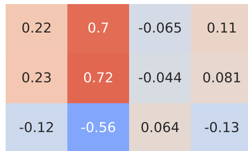
Spearman Correlation - Model: kuga | Fuel: 1
