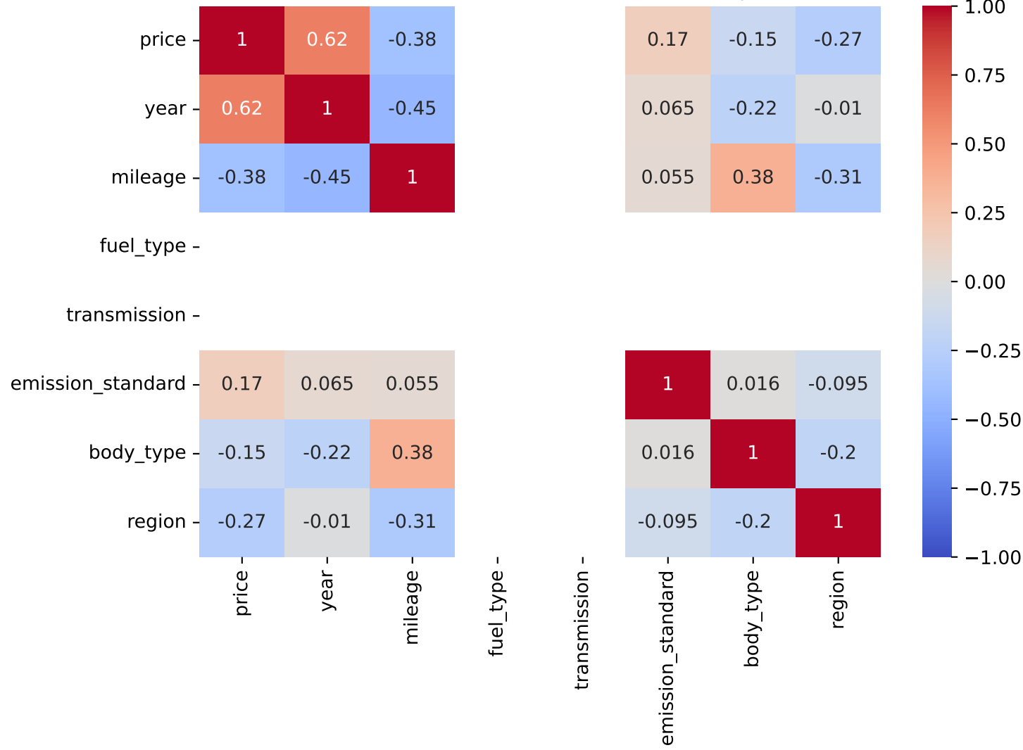
Pearson Correlation - Model: romeo stelvio | Fuel: 2
