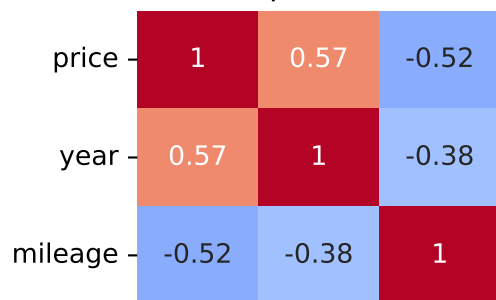
Spearman Correlation - Model: modus | Fuel: 1
