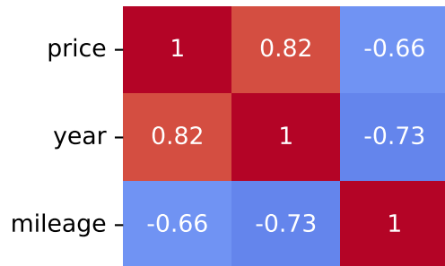
Spearman Correlation - Model: rover discovery | Fuel: 1
