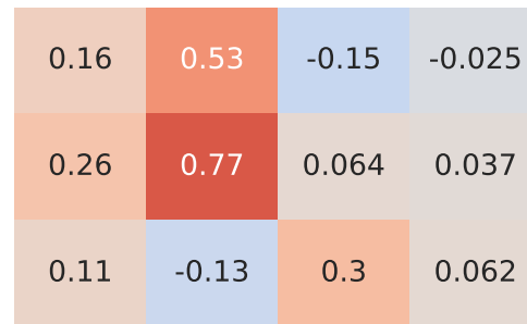
Pearson Correlation - Model: c5 | Fuel: 1
