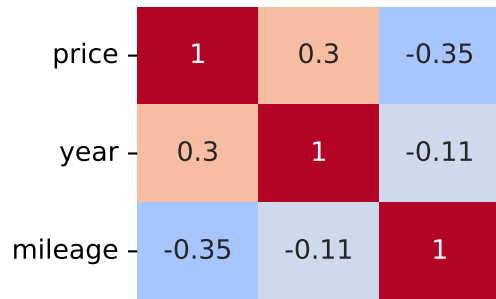
Spearman Correlation - Model: grand vitara | Fuel: 1
