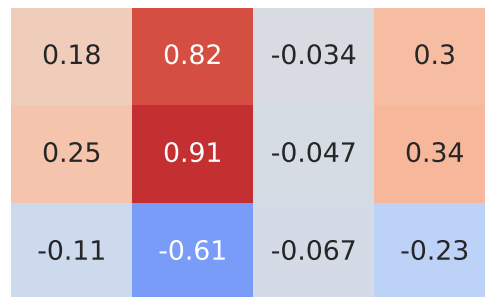
Pearson Correlation - Model: santa fe | Fuel: 1
