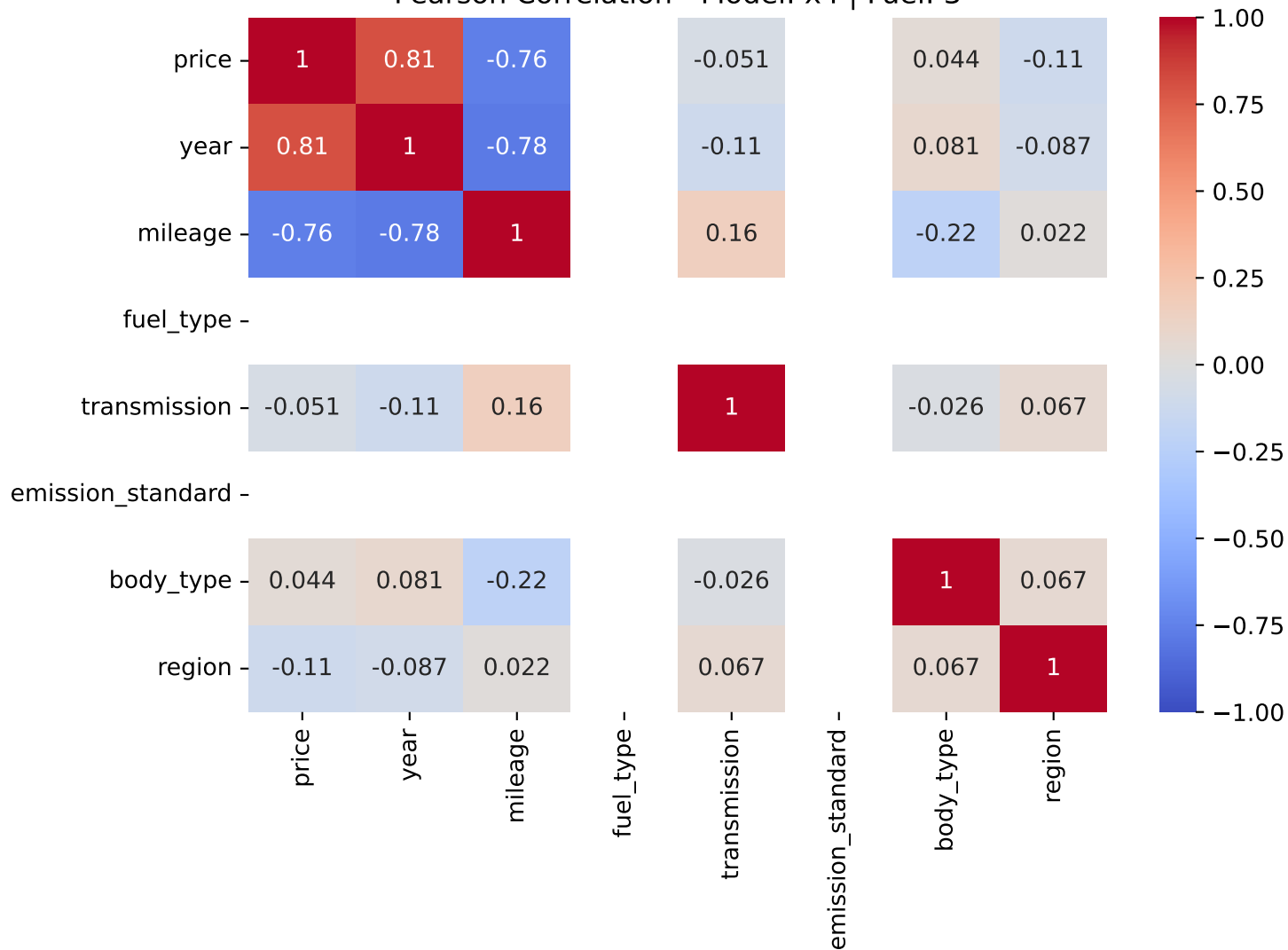
Pearson Correlation - Model: x4 | Fuel: 3
