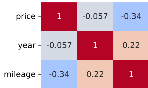
Spearman Correlation - Model: nemo | Fuel: 1
