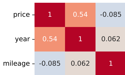
Pearson Correlation - Model: altea | Fuel: 1
