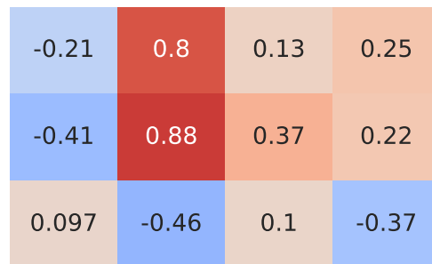
Pearson Correlation - Model: auris | Fuel: 1
