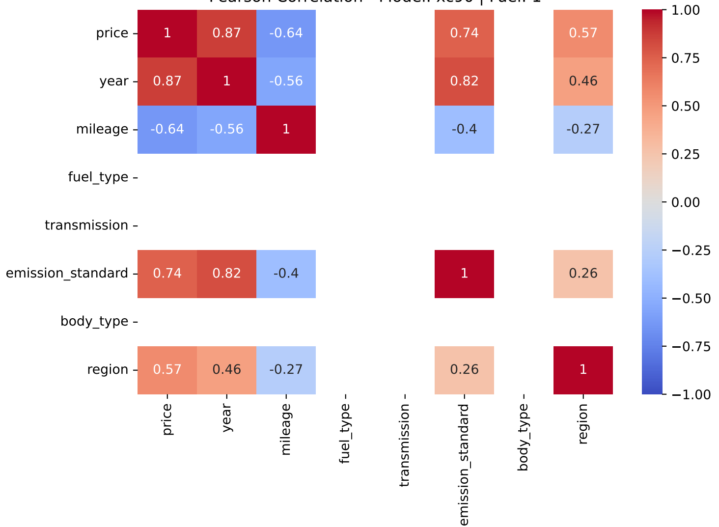
Pearson Correlation - Model: xc90 | Fuel: 1
