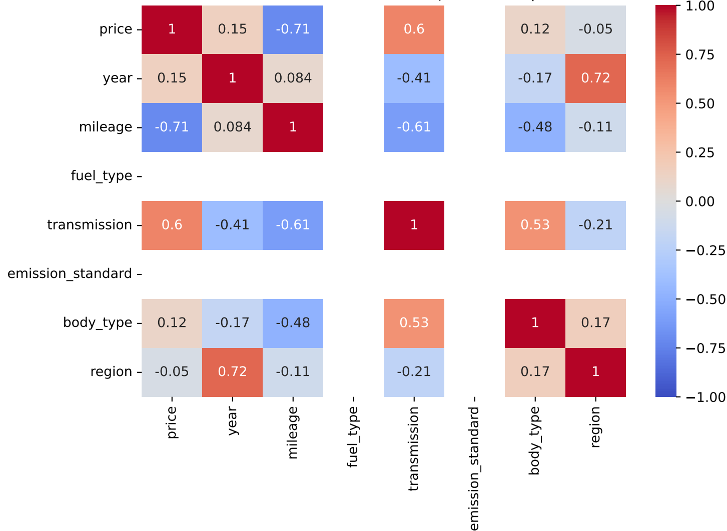
Pearson Correlation - Model: c4 spacetourer | Fuel: 1
