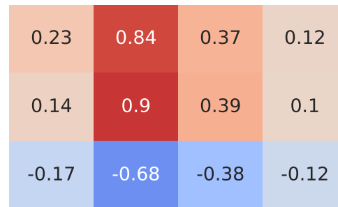
Pearson Correlation - Model: c4 | Fuel: 1
