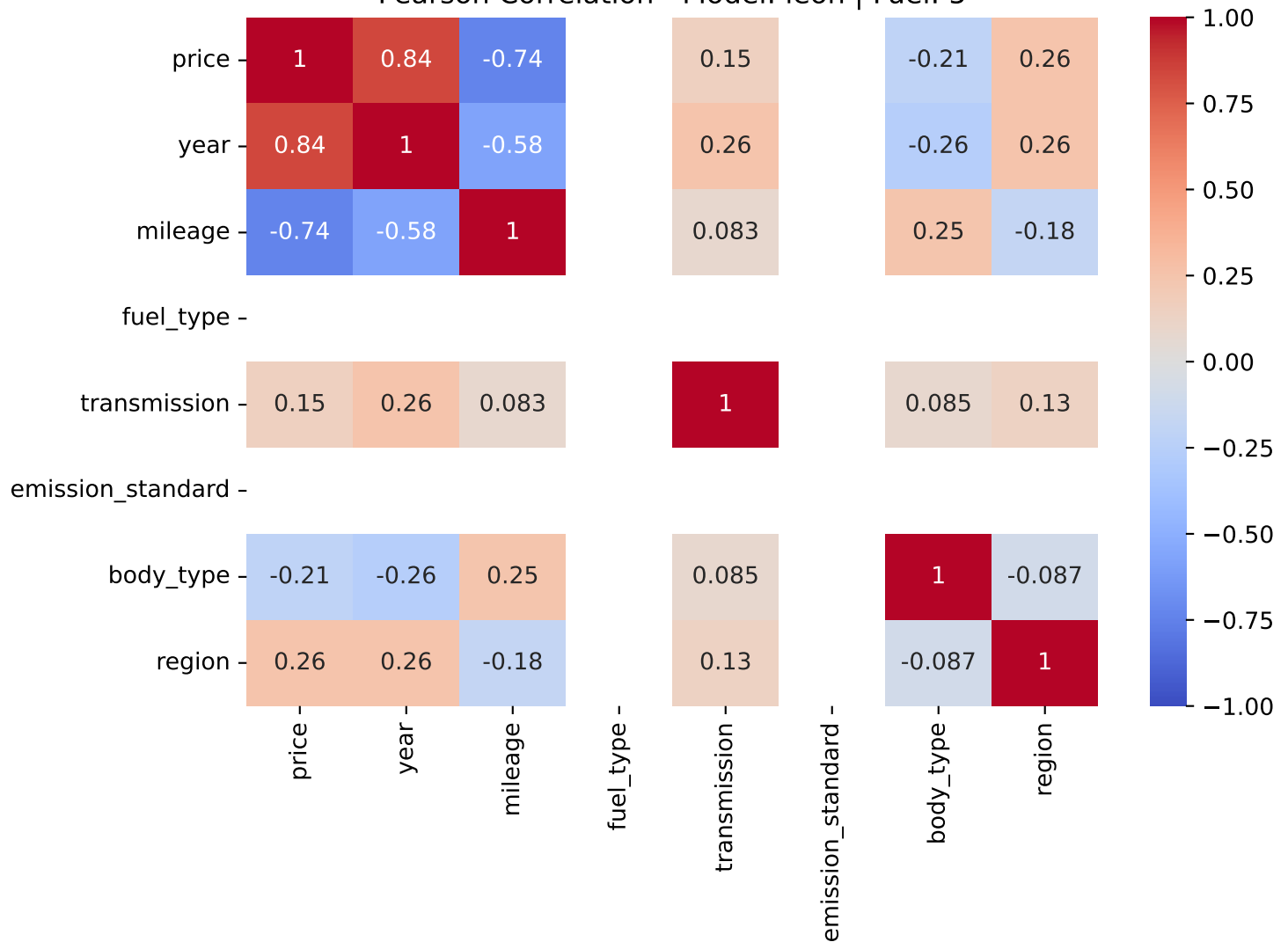
Pearson Correlation - Model: leon | Fuel: 5
