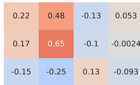
Spearman Correlation - Model: captur | Fuel: 1
