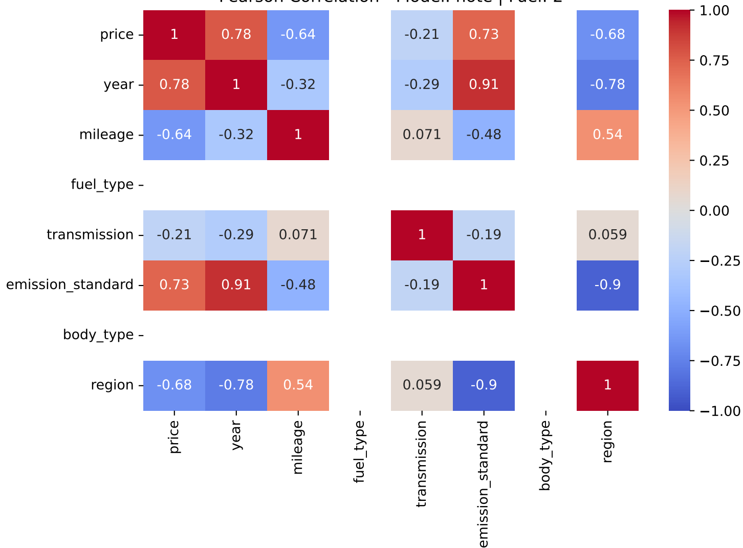
Pearson Correlation - Model: note | Fuel: 2
