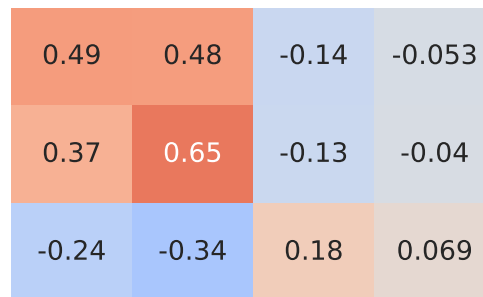
Pearson Correlation - Model: 2008 | Fuel: 1
