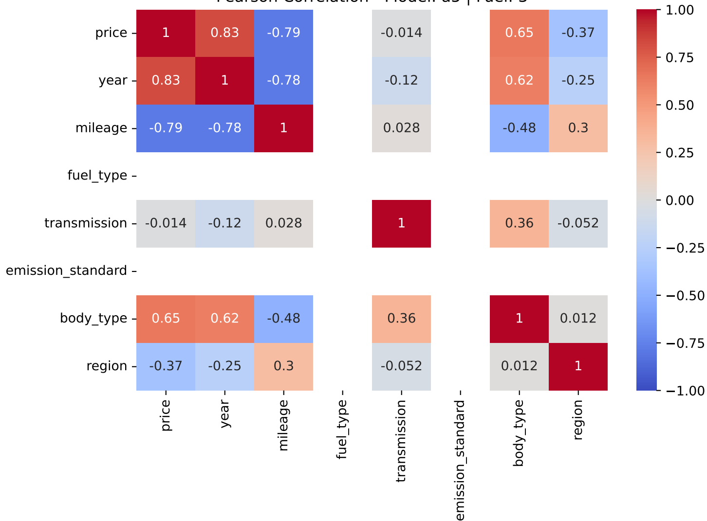
Pearson Correlation - Model: a5 | Fuel: 3
