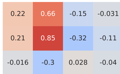
Pearson Correlation - Model: v40 | Fuel: 1
