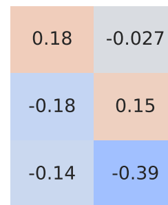
Pearson Correlation - Model: q4 | Fuel: 0
