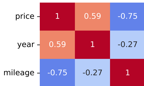
Pearson Correlation - Model: iq | Fuel: 2
