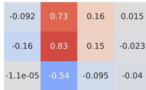
Pearson Correlation - Model: c3 | Fuel: 1
