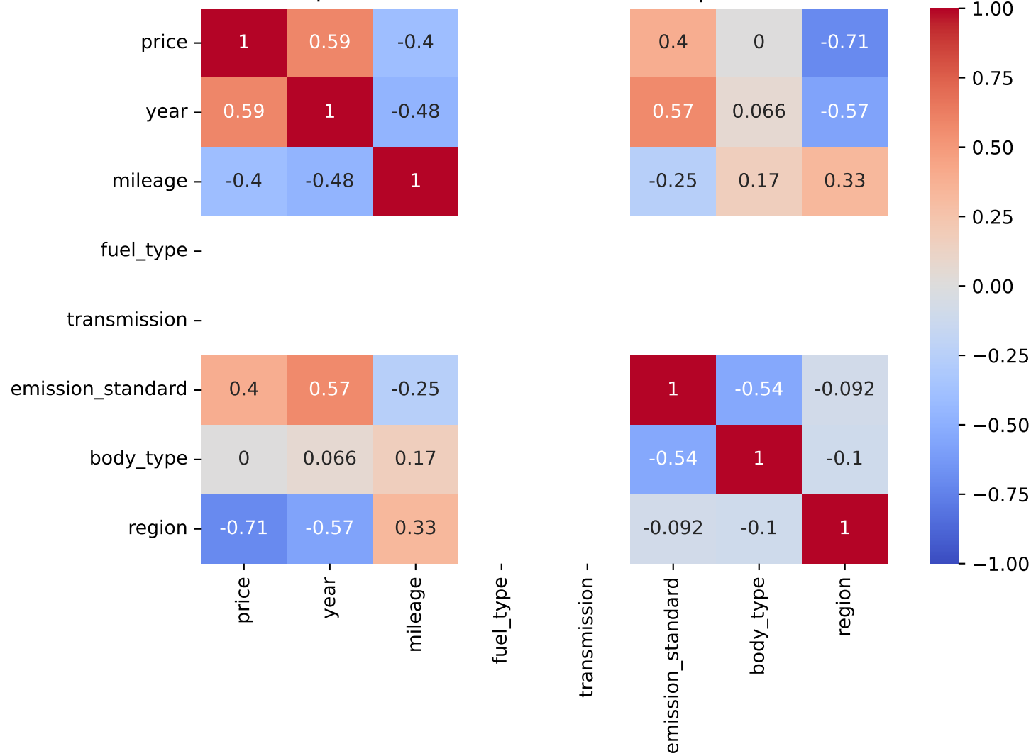
Spearman Correlation - Model: mii | Fuel: 5
