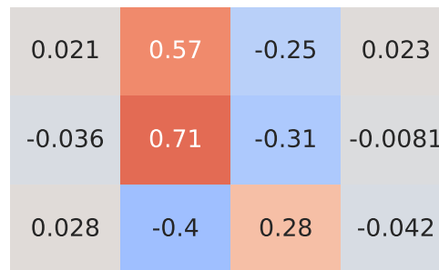
Spearman Correlation - Model: 500 | Fuel: 4
