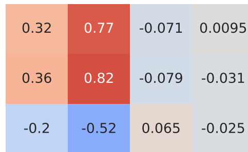
Spearman Correlation - Model: qashqai | Fuel: 1
