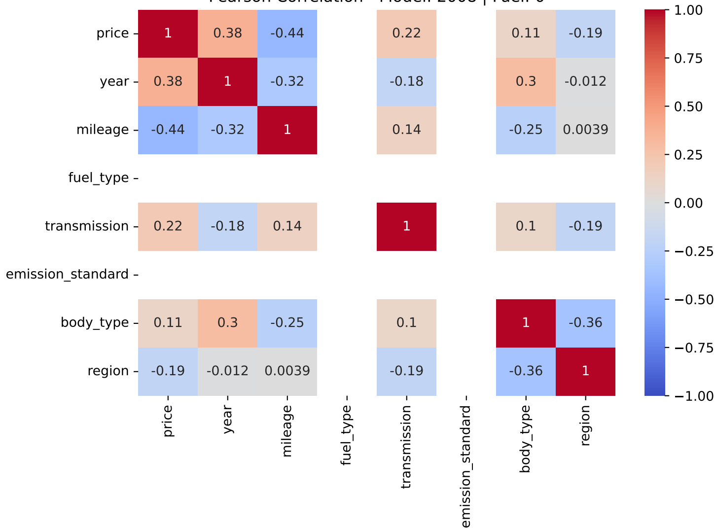
Pearson Correlation - Model: 2008 | Fuel: 0
