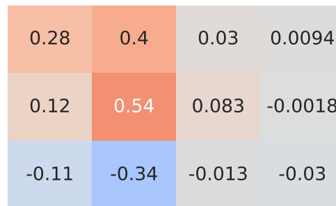
Pearson Correlation - Model: 208 | Fuel: 2
