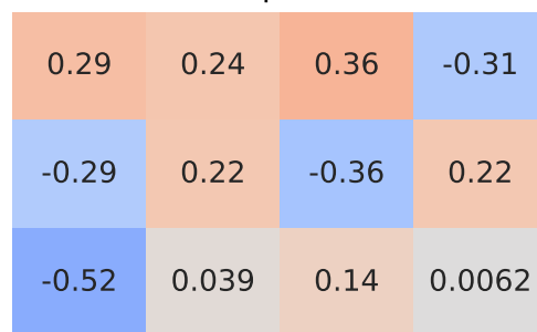
Spearman Correlation - Model: stilo | Fuel: 2
