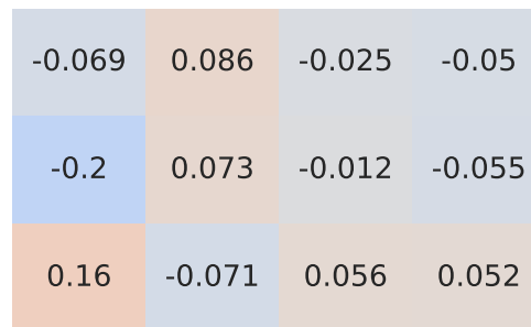
Spearman Correlation - Model: 500x | Fuel: 1
