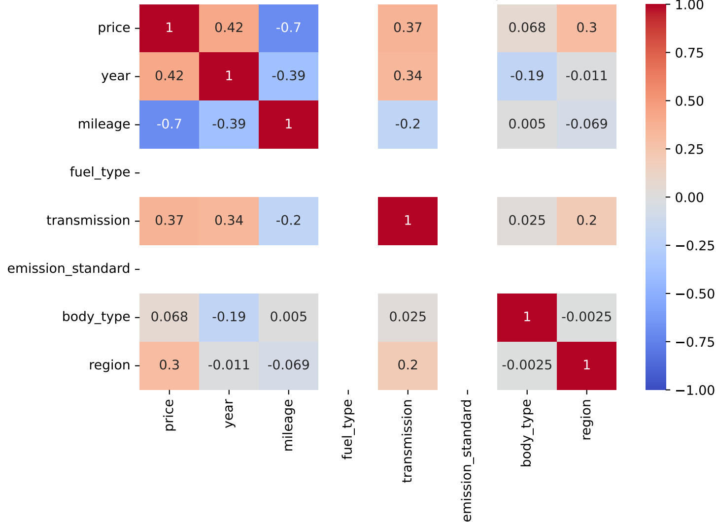
Spearman Correlation - Model: ateca | Fuel: 1
