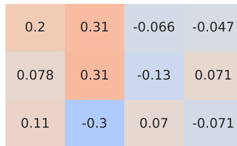
Spearman Correlation - Model: 3008 | Fuel: 2
