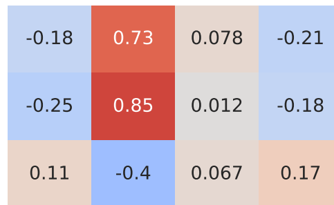
Pearson Correlation - Model: c4 picasso | Fuel: 1
