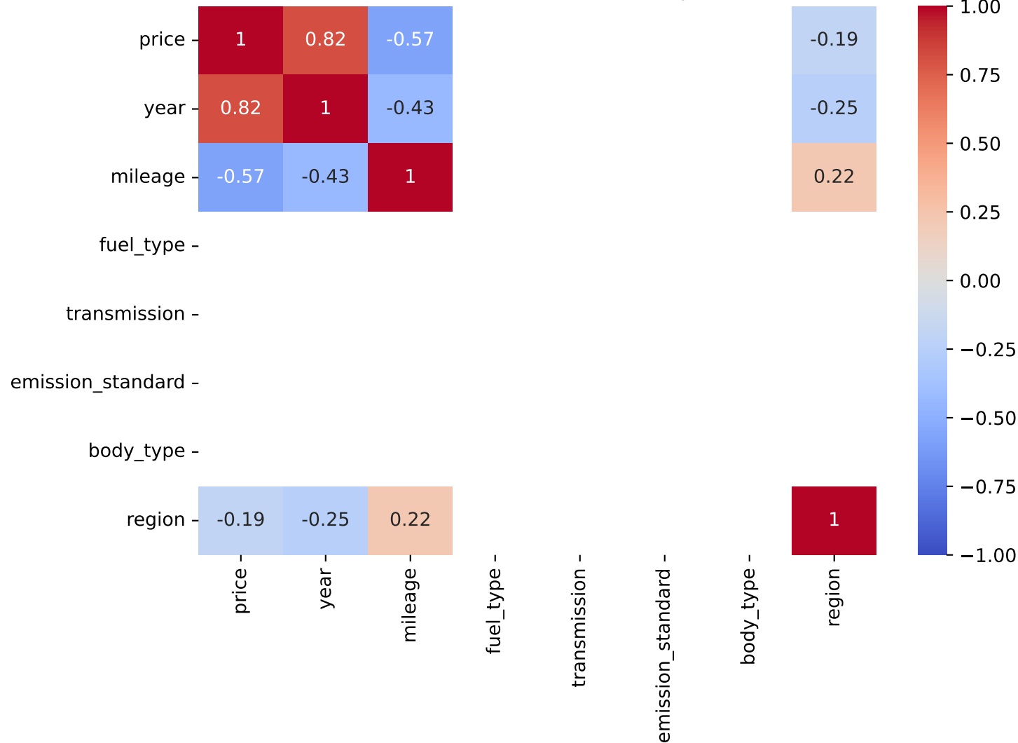
Pearson Correlation - Model: leaf | Fuel: 0
