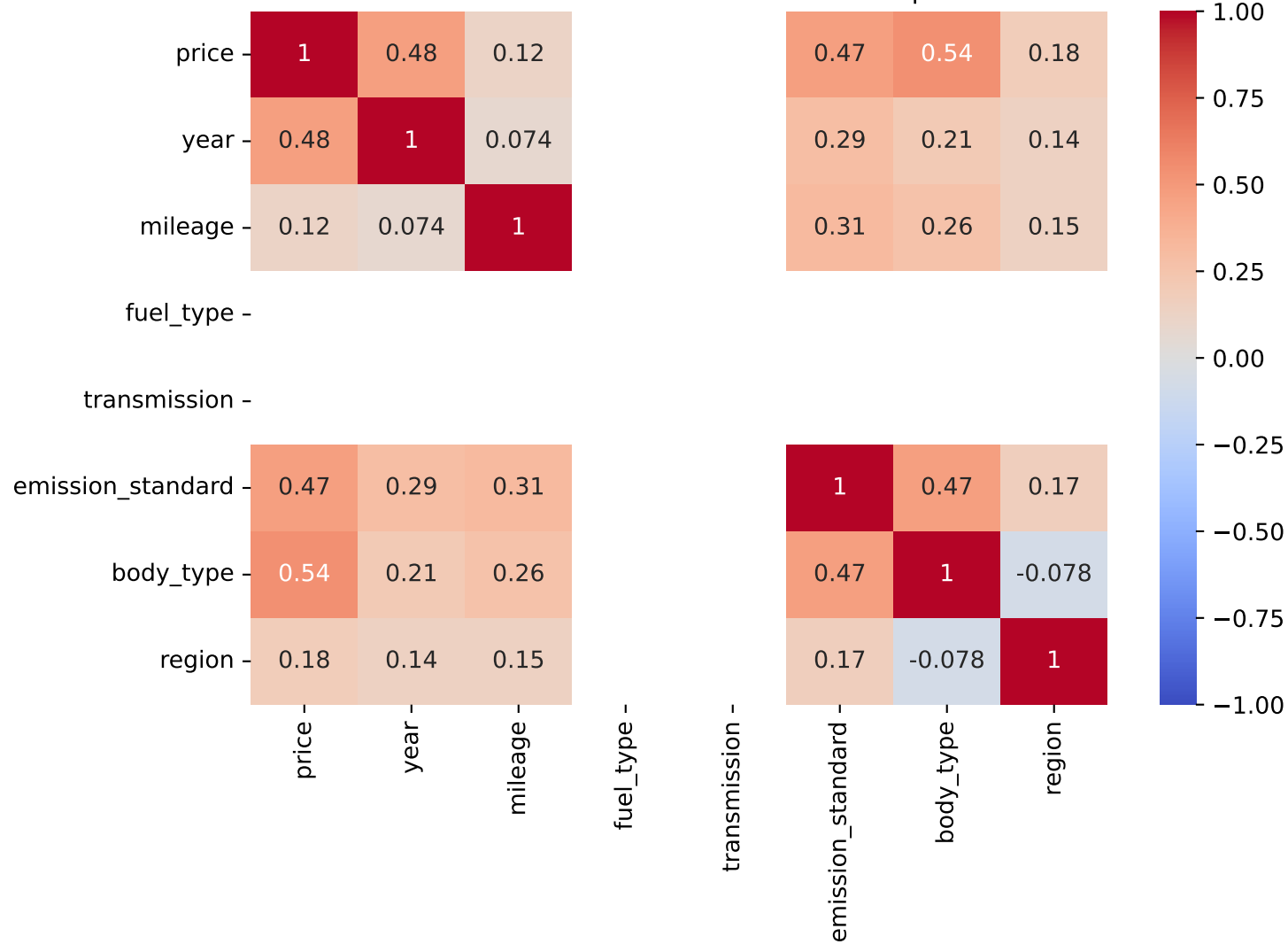
Pearson Correlation - Model: new beetle | Fuel: 1
