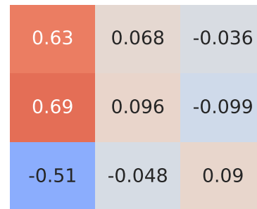
Spearman Correlation - Model: panda | Fuel: 4
