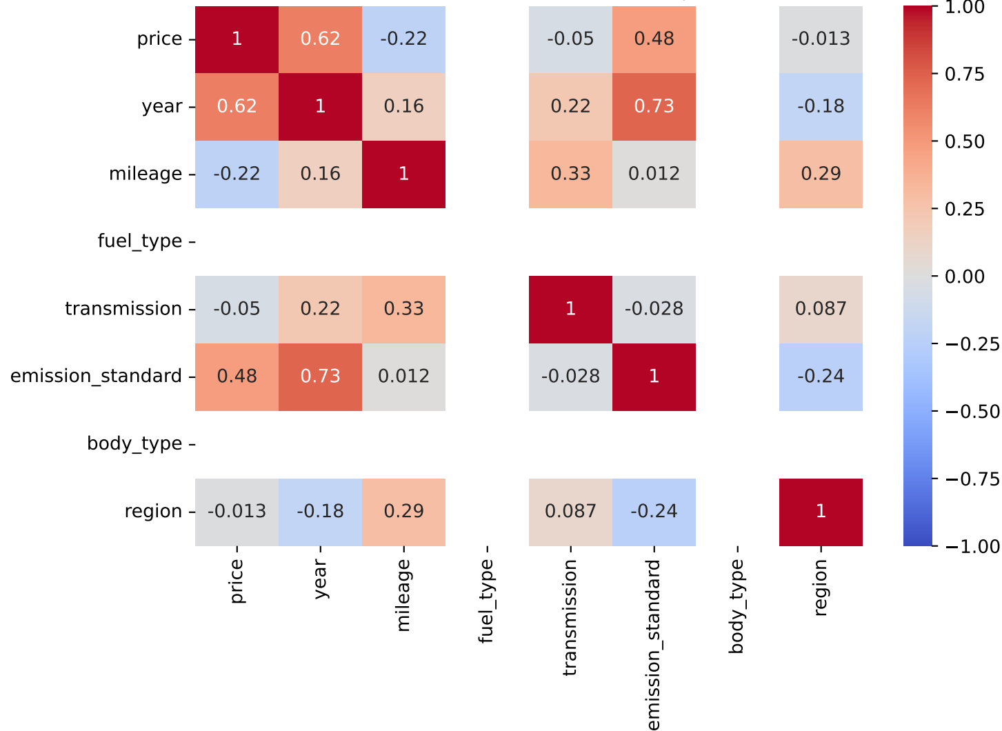
Pearson Correlation - Model: patrol | Fuel: 1
