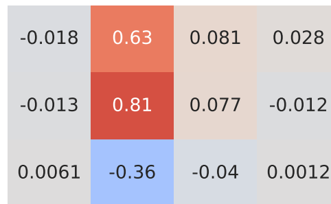
Spearman Correlation - Model: 500l | Fuel: 1
