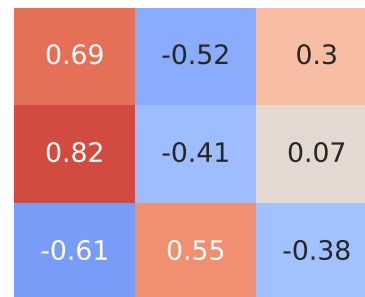
Pearson Correlation - Model: swift | Fuel: 4
