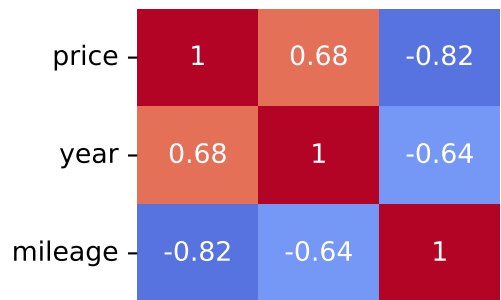
Spearman Correlation - Model: yeti | Fuel: 1
