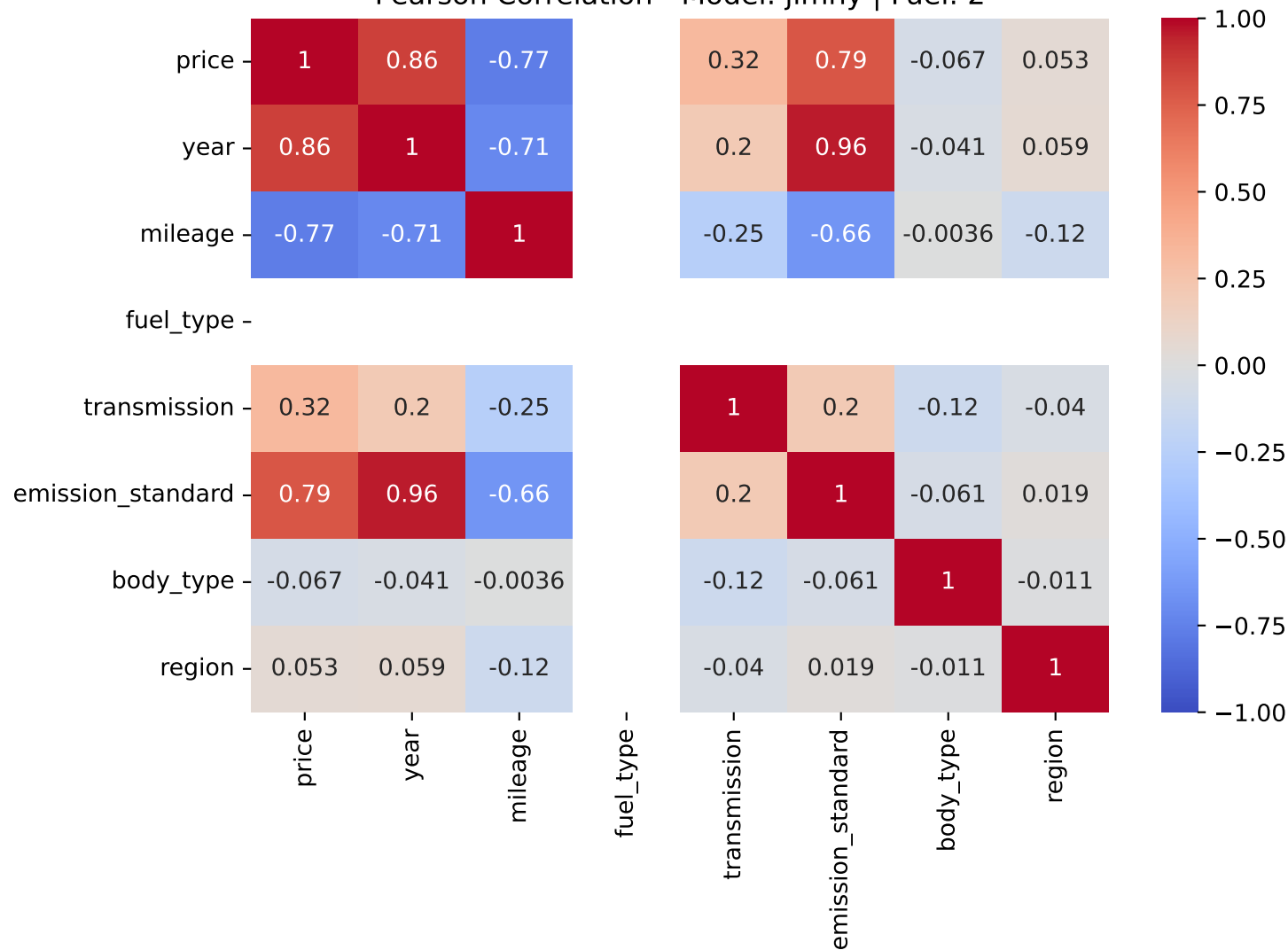
Pearson Correlation - Model: jimny | Fuel: 2
