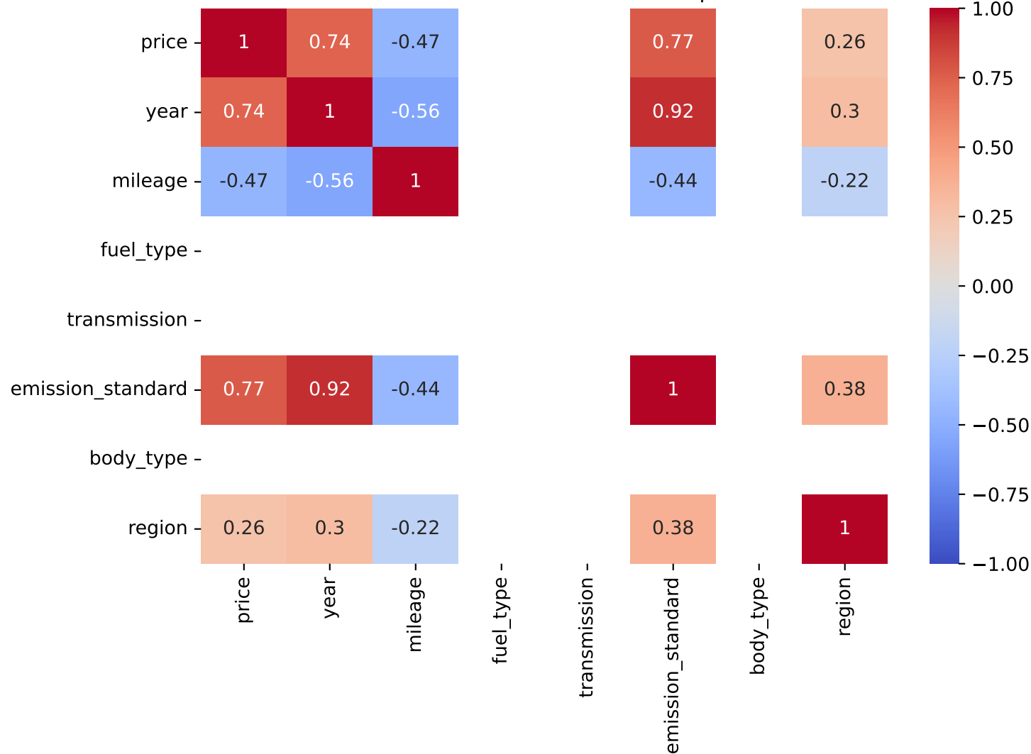
Pearson Correlation - Model: dobrolo | Fuel: 5
