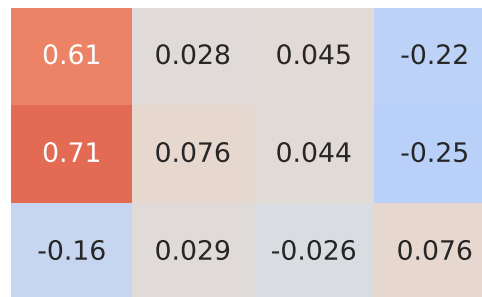
Pearson Correlation - Model: x1 | Fuel: 2
