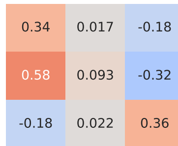
Spearman Correlation - Model: 307 | Fuel: 1
