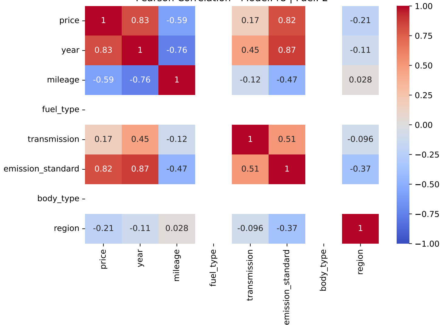
Pearson Correlation - Model: r8 | Fuel: 2
