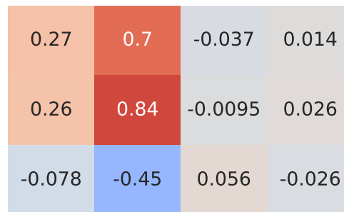
Pearson Correlation - Model: q5 | Fuel: 1
