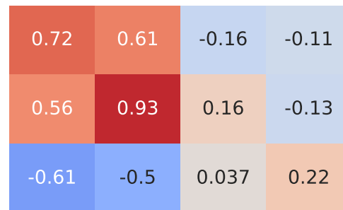
Pearson Correlation - Model: megane | Fuel: 2
