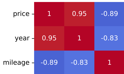
Pearson Correlation - Model: clio | Fuel: 4
