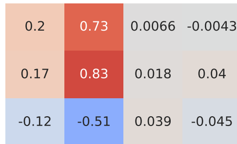
Spearman Correlation - Model: 500 | Fuel: 1
