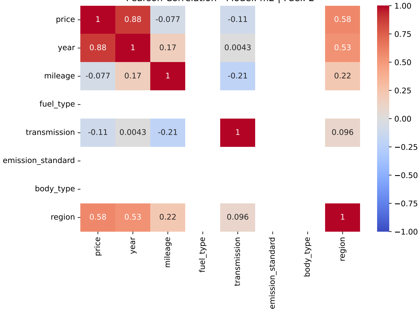
Pearson Correlation - Model: m2 | Fuel: 2
