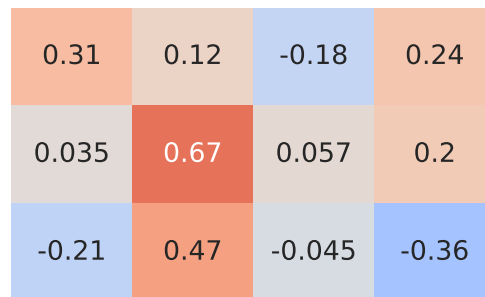
Pearson Correlation - Model: zafira tourer | Fuel: 1
