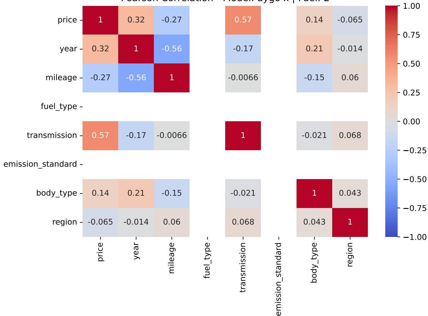
Pearson Correlation - Model: aygo x | Fuel: 2
