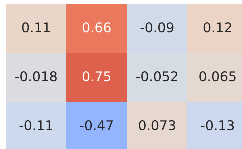
Spearman Correlation - Model: clio | Fuel: 1
