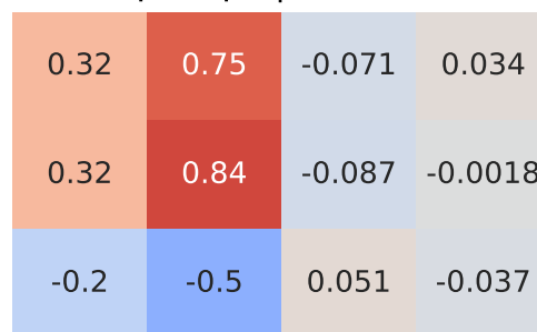
Pearson Correlation - Model: qashqai | Fuel: 1
