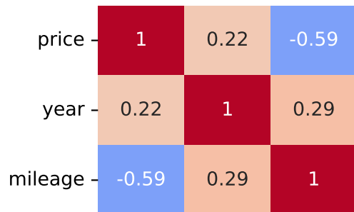
Spearman Correlation - Model: zafira tourer | Fuel: 1
