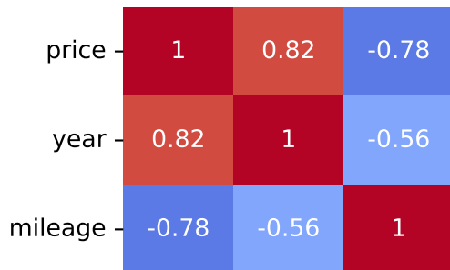
Pearson Correlation - Model: octavia | Fuel: 1
