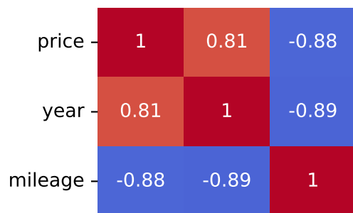
Pearson Correlation - Model: karoq | Fuel: 1
