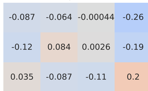
Spearman Correlation - Model: q8 | Fuel: 3
