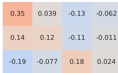
Pearson Correlation - Model: t-roc | Fuel: 1
