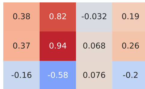
Pearson Correlation - Model: espace | Fuel: 1
