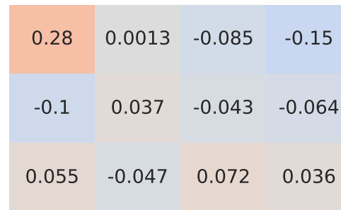
Pearson Correlation - Model: renegade | Fuel: 2
