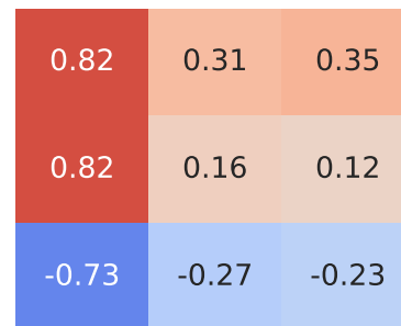
Spearman Correlation - Model: ignis | Fuel: 2
