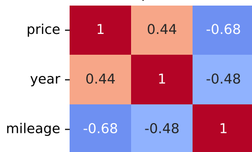
Spearman Correlation - Model: puma | Fuel: 2
