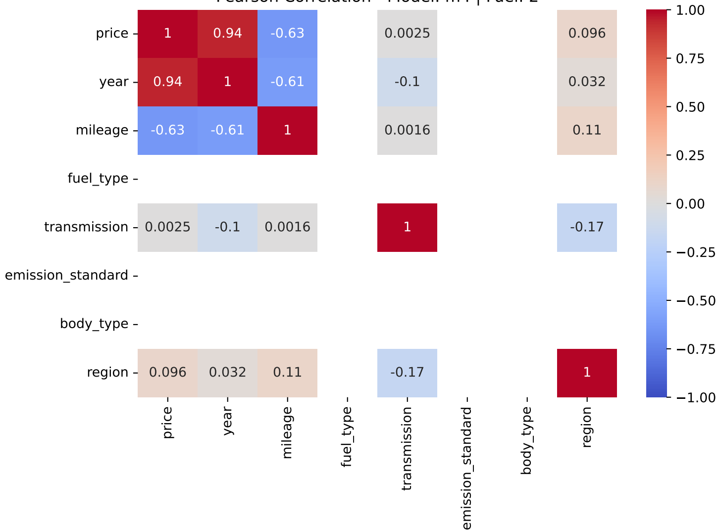
Pearson Correlation - Model: m4 | Fuel: 2
