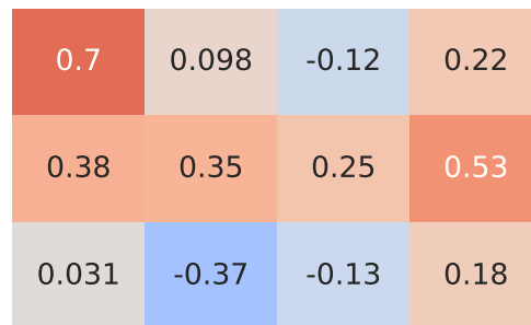
Pearson Correlation - Model: phedra | Fuel: 1
