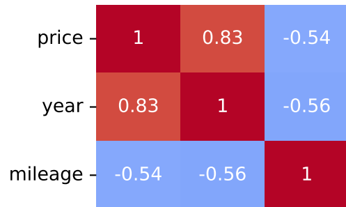
Spearman Correlation - Model: a4 | Fuel: 2
