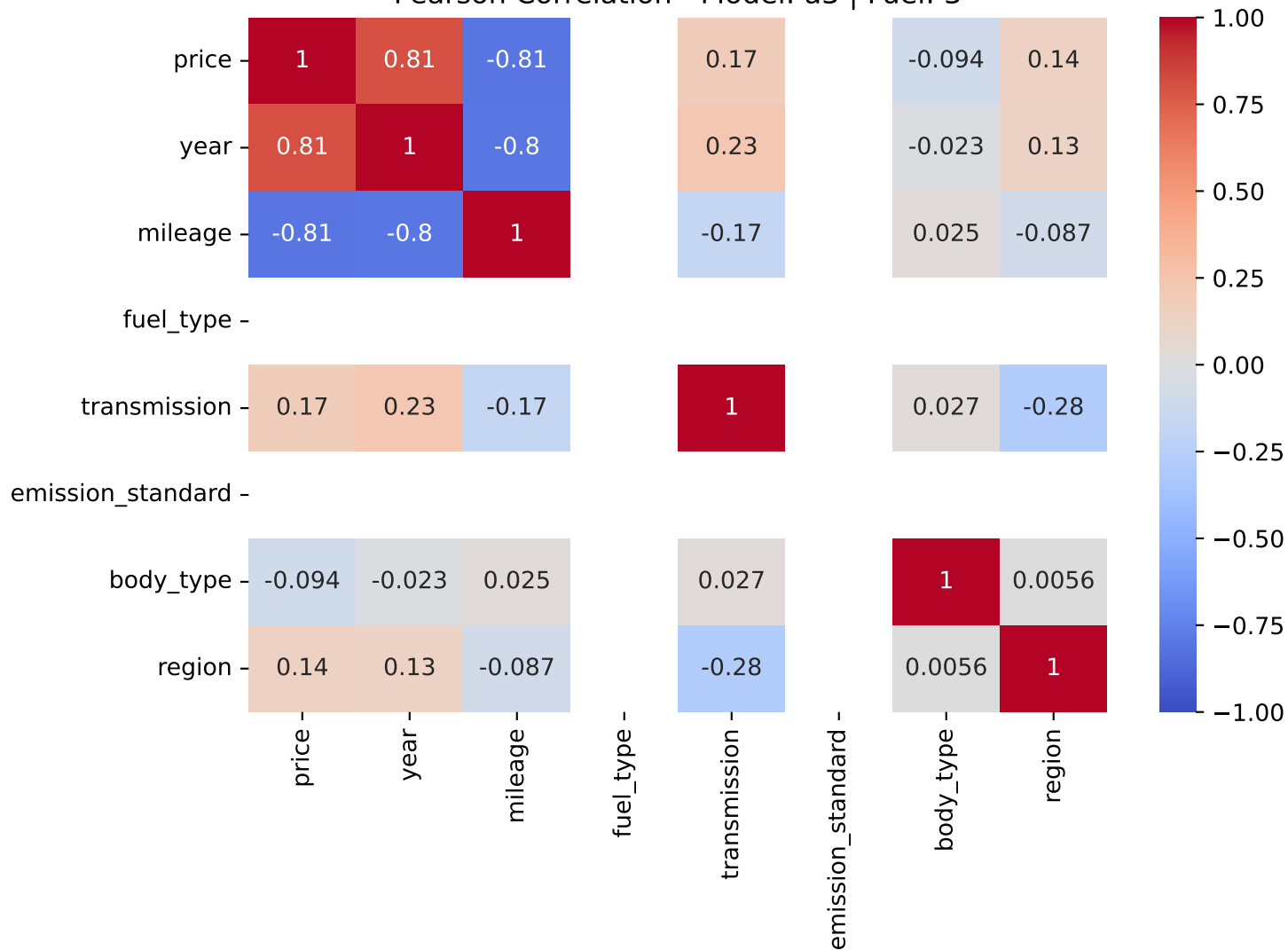
Pearson Correlation - Model: a3 | Fuel: 3
