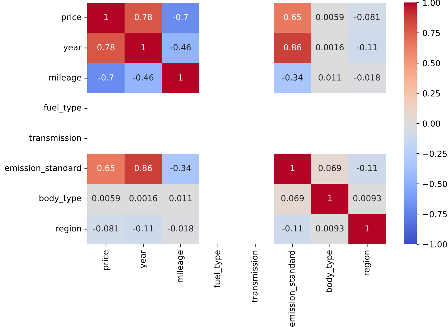
Pearson Correlation - Model: corsa | Fuel: 4
