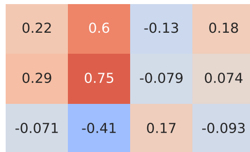
Spearman Correlation - Model: x-trail | Fuel: 1
