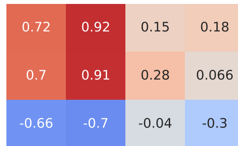
Spearman Correlation - Model: scenic | Fuel: 2
