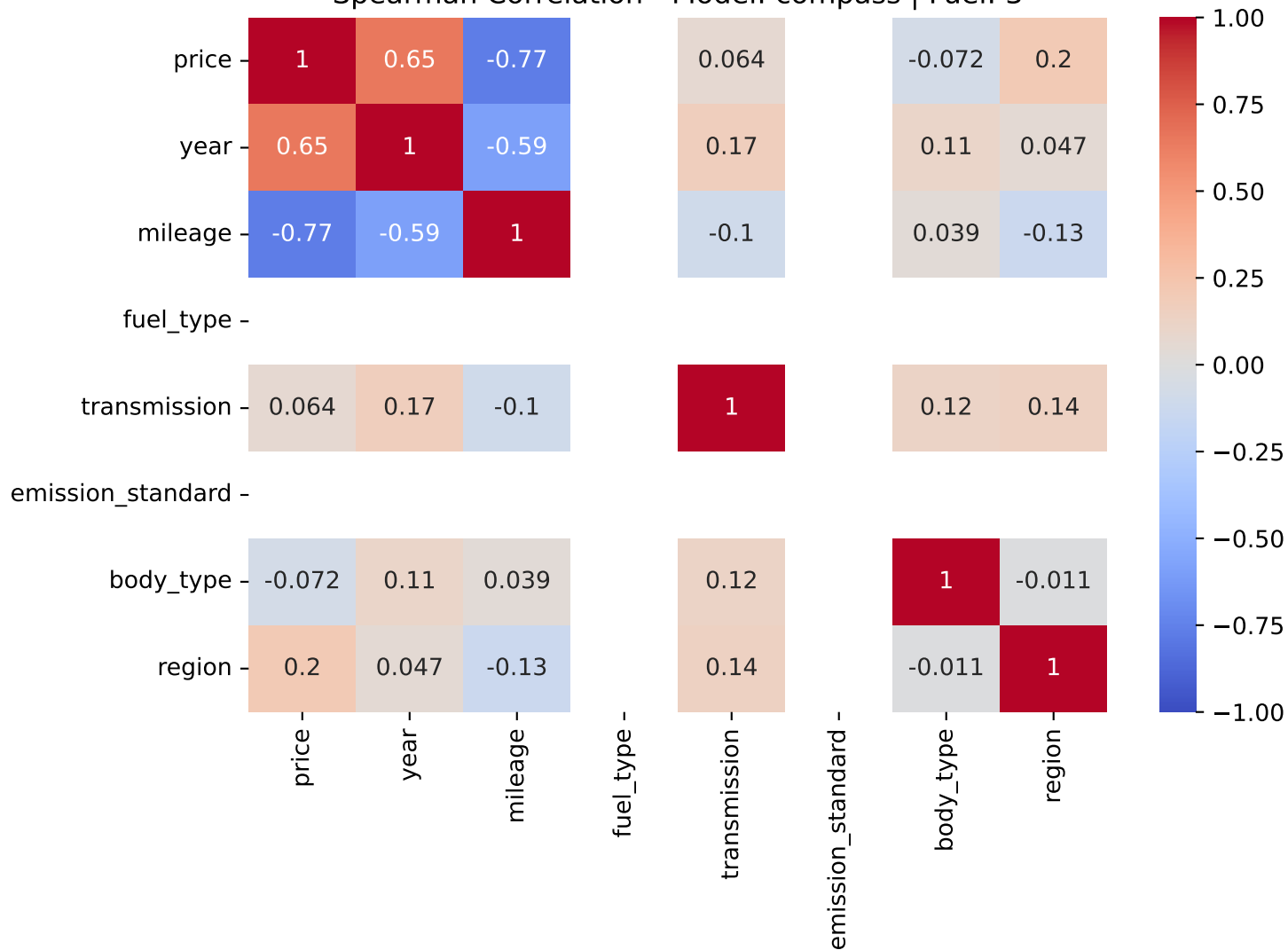
Spearman Correlation - Model: compass | Fuel: 3
