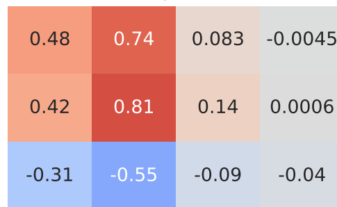
Spearman Correlation - Model: golf | Fuel: 1
