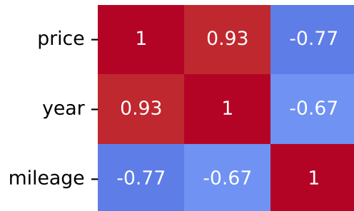
Spearman Correlation - Model: x5 | Fuel: 1
