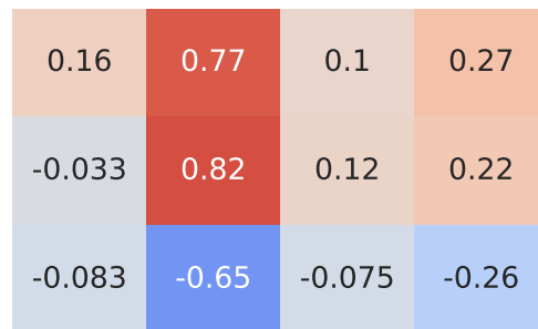
Spearman Correlation - Model: ibiza | Fuel: 2
