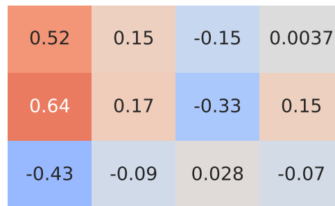
Pearson Correlation - Model: a3 | Fuel: 5
