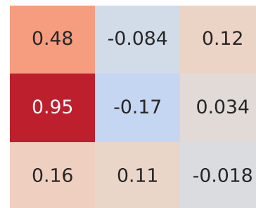
Pearson Correlation - Model: 500I | Fuel: 2
