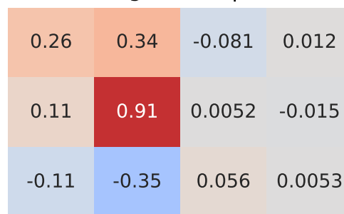
Pearson Correlation - Model: rover range rover | Fuel: 1
