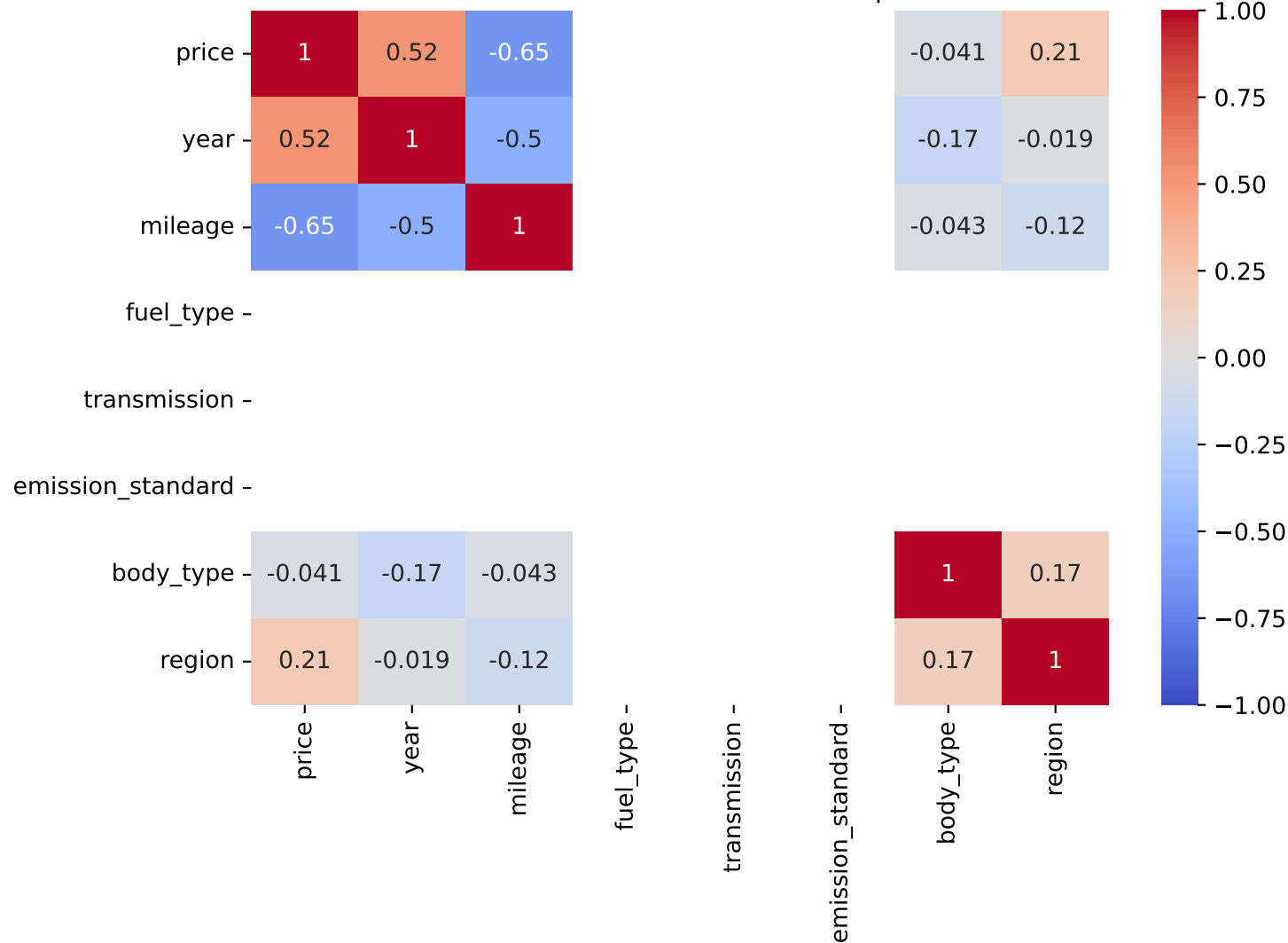
Pearson Correlation - Model: arona | Fuel: 5
