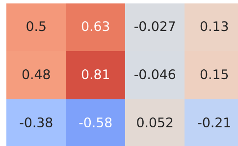
Pearson Correlation - Model: a3 | Fuel: 1
