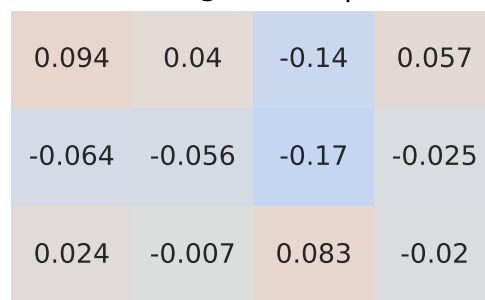
Spearman Correlation - Model: rover range rover | Fuel: 3
