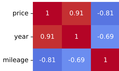
Spearman Correlation - Model: kuga | Fuel: 1
