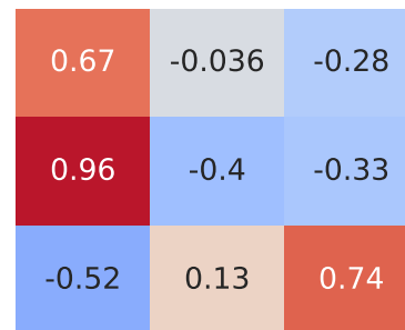
Pearson Correlation - Model: ka | Fuel: 4
