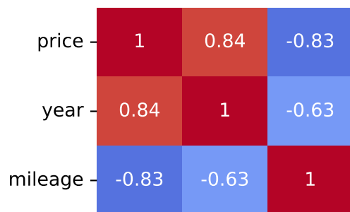
Pearson Correlation - Model: xc60 | Fuel: 1
