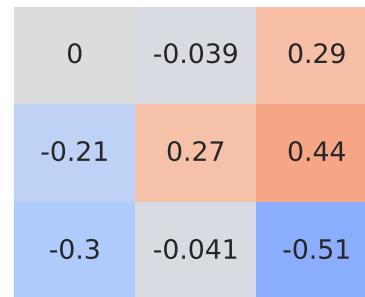
Spearman Correlation - Model: stonic | Fuel: 1
