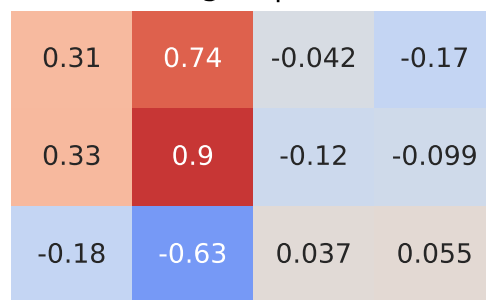
Spearman Correlation - Model: wrangler | Fuel: 1
