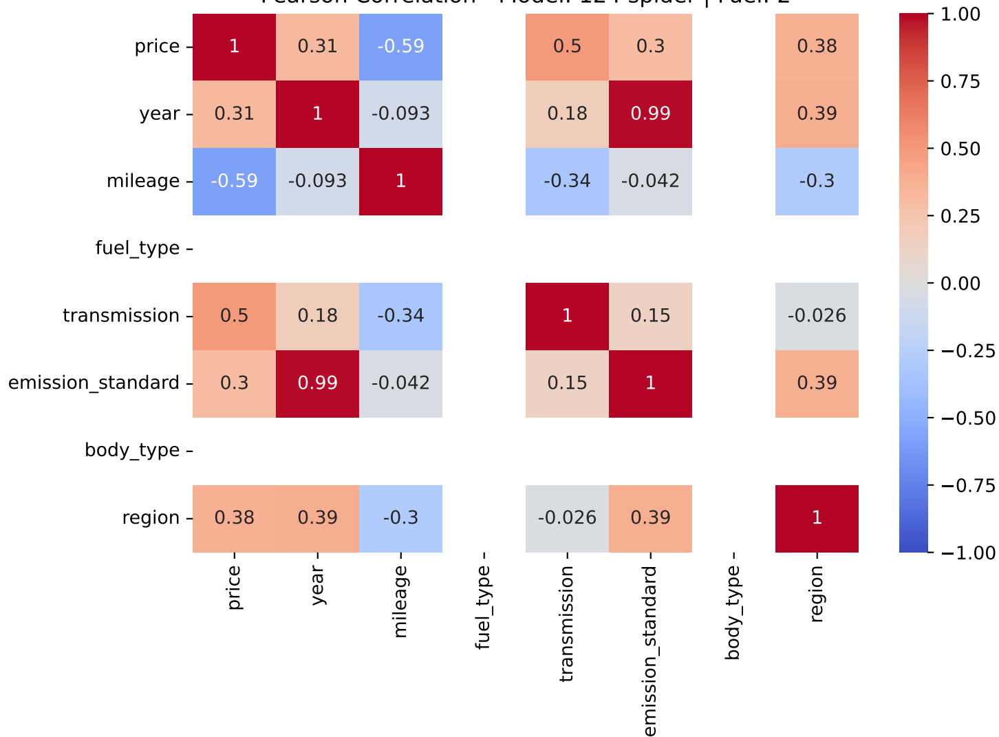
Pearson Correlation - Model: 124 spider | Fuel: 2
