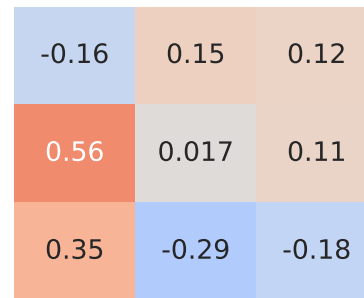
Spearman Correlation - Model: zafira tourer | Fuel: 5
