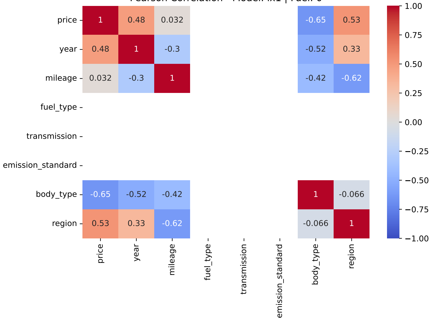
Pearson Correlation - Model: ix1 | Fuel: 0
