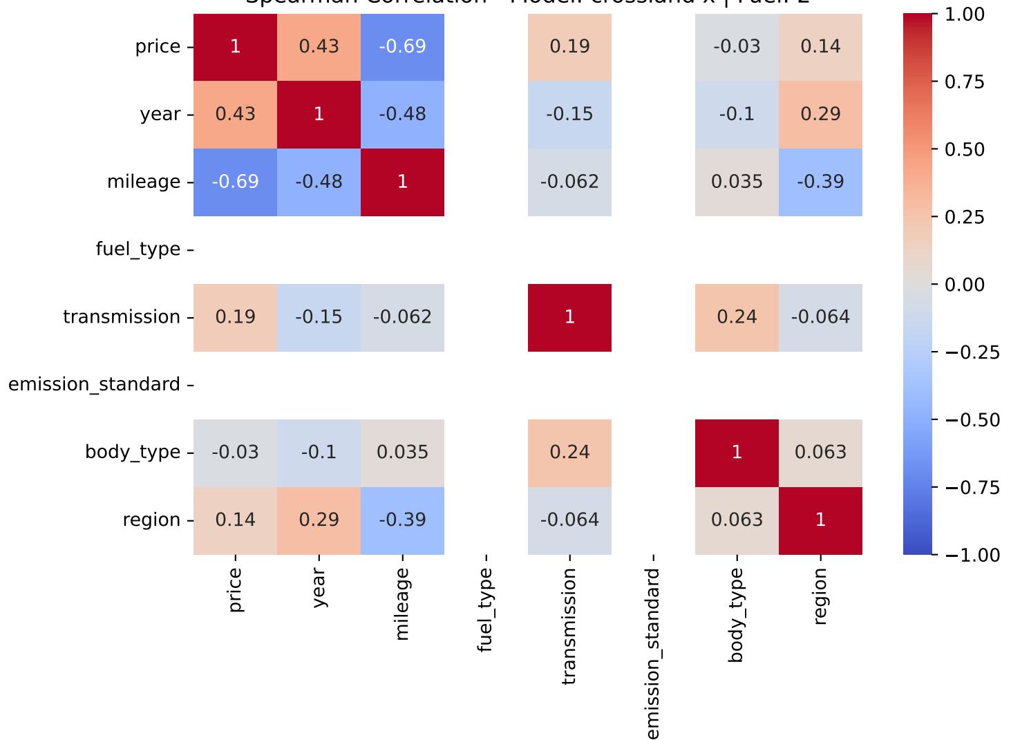
Spearman Correlation - Model: crossland x | Fuel: 2
