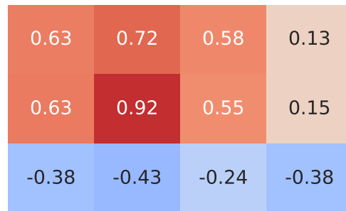
Pearson Correlation - Model: a4 | Fuel: 2
