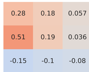
Pearson Correlation - Model: ypsilon | Fuel: 5
