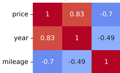
Spearman Correlation - Model: meriva | Fuel: 2
