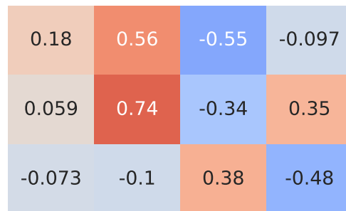
Spearman Correlation - Model: 407 | Fuel: 1
