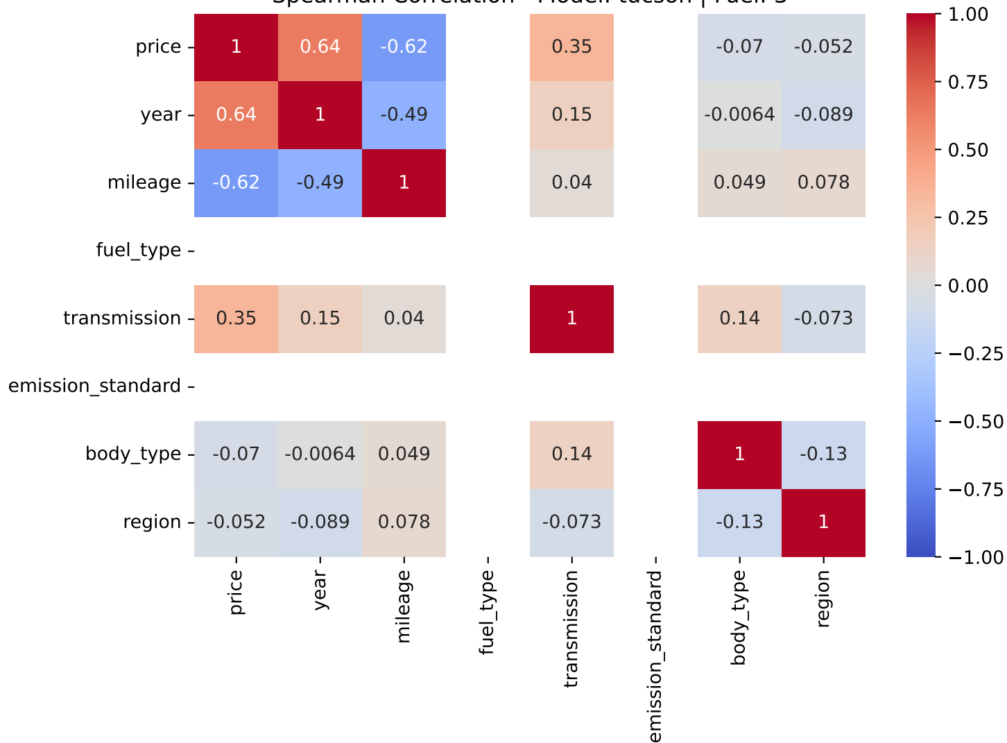
Spearman Correlation - Model: tucson | Fuel: 3
