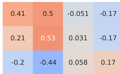
Spearman Correlation - Model: mokka | Fuel: 2
