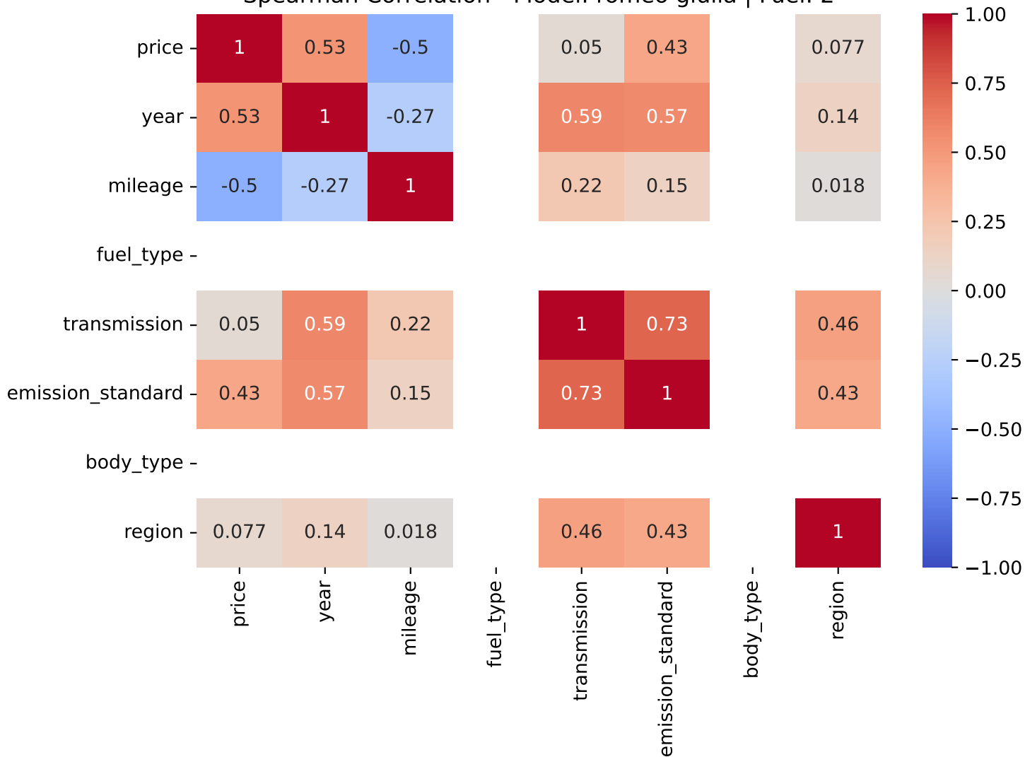
Spearman Correlation - Model: romeo giulia | Fuel: 2
