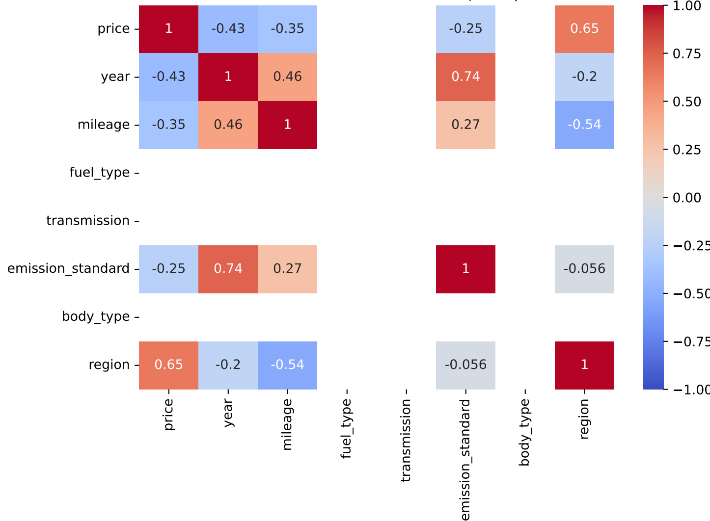
Pearson Correlation - Model: romeo spider | Fuel: 2
