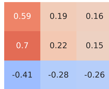
Spearman Correlation - Model: up | Fuel: 5
