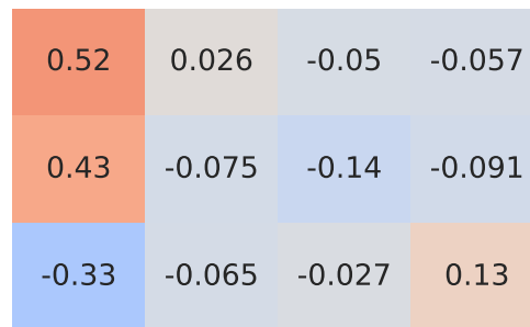
Pearson Correlation - Model: compass | Fuel: 2
