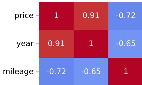
Pearson Correlation - Model: c1 | Fuel: 2
