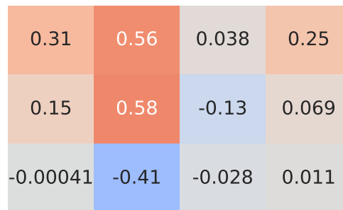
Spearman Correlation - Model: vitara | Fuel: 1
