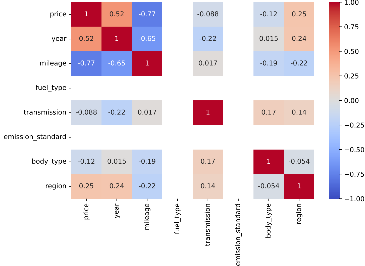
Spearman Correlation - Model: q5 sportback | Fuel: 3
