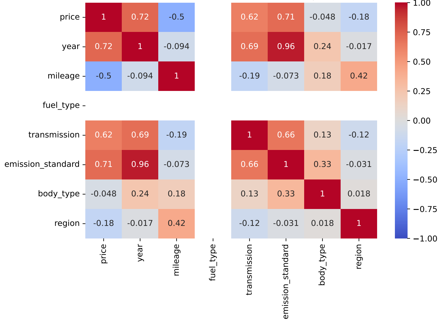
Pearson Correlation - Model: land cruiser | Fuel: 1
