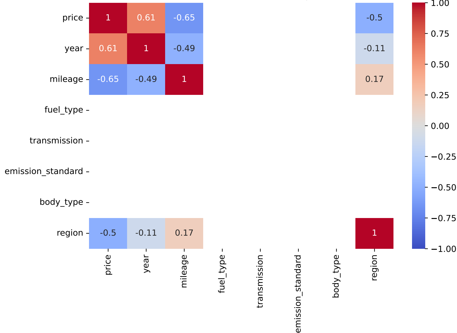
Pearson Correlation - Model: id.4 | Fuel: 0
