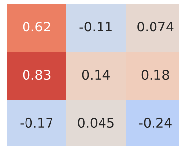
Pearson Correlation - Model: panda cross | Fuel: 1
