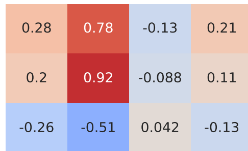
Pearson Correlation - Model: astra | Fuel: 2
