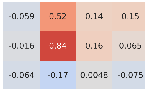
Pearson Correlation - Model: c3 picasso | Fuel: 1
