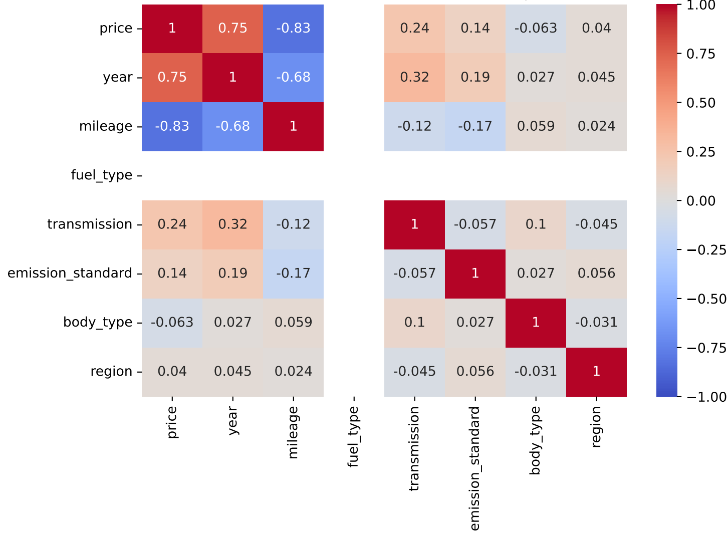
Spearman Correlation - Model: c5 aircross | Fuel: 1
