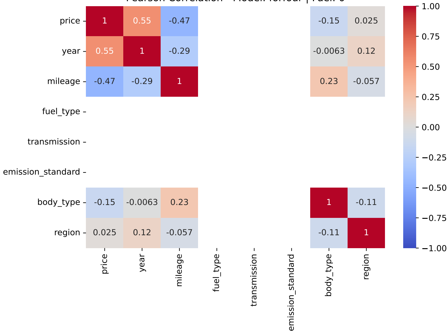
Pearson Correlation - Model: forfour | Fuel: 0
