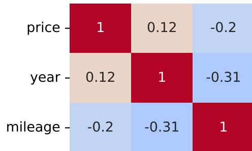
Pearson Correlation - Model: romeo 156 | Fuel: 2
