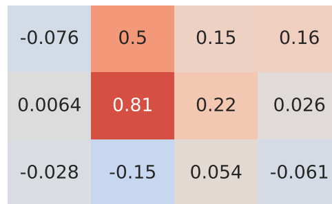
Spearman Correlation - Model: c3 picasso | Fuel: 1
