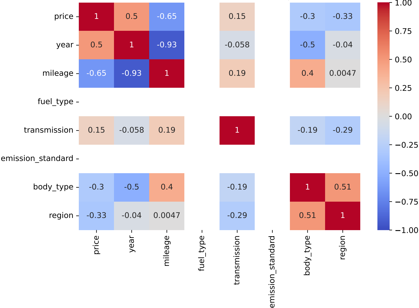
Spearman Correlation - Model: scala | Fuel: 2
