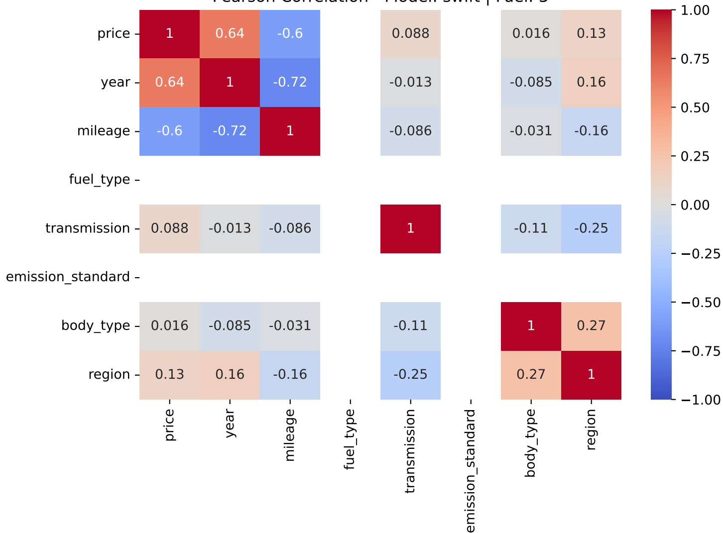
Pearson Correlation - Model: swift | Fuel: 3
