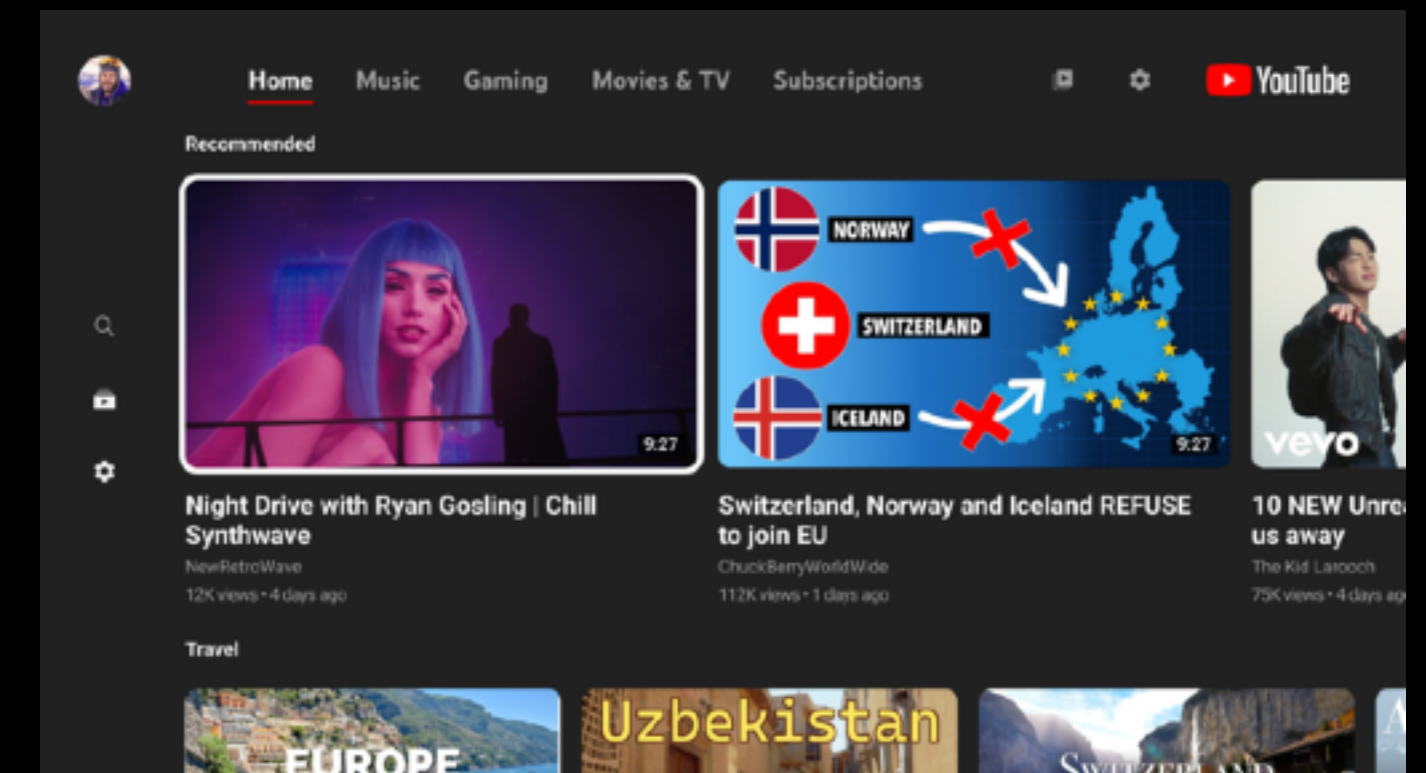
Hybrid
