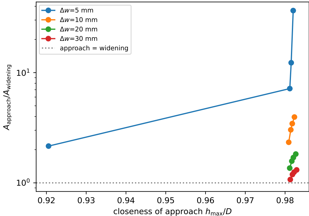
(b) Attractor controls the secondary peak
