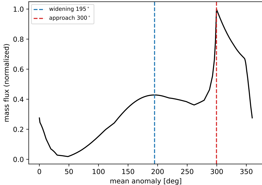
(a) Two gas-flux peaks ( \Delta w=10 , w_{\text{eff}}=7 mm)
