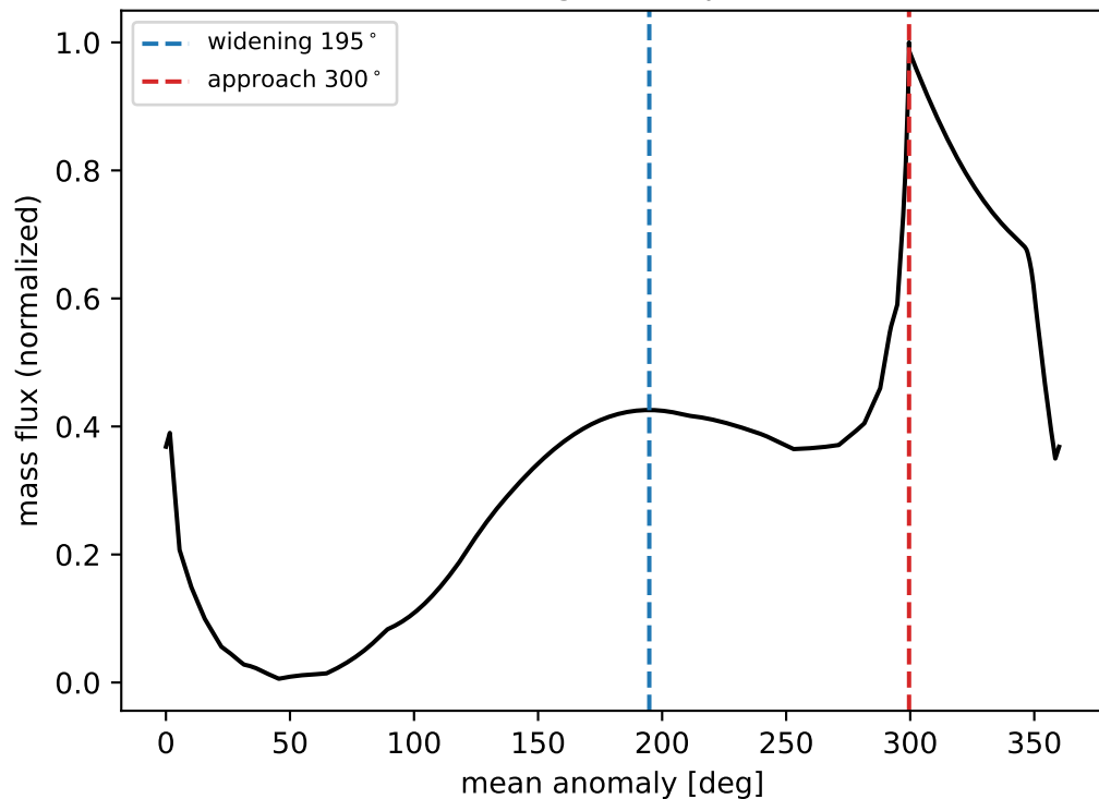
(a) Two gas-flux peaks
