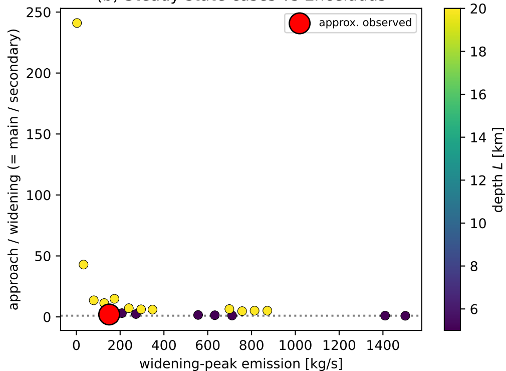
(b) Steady-state cases vs Enceladus
