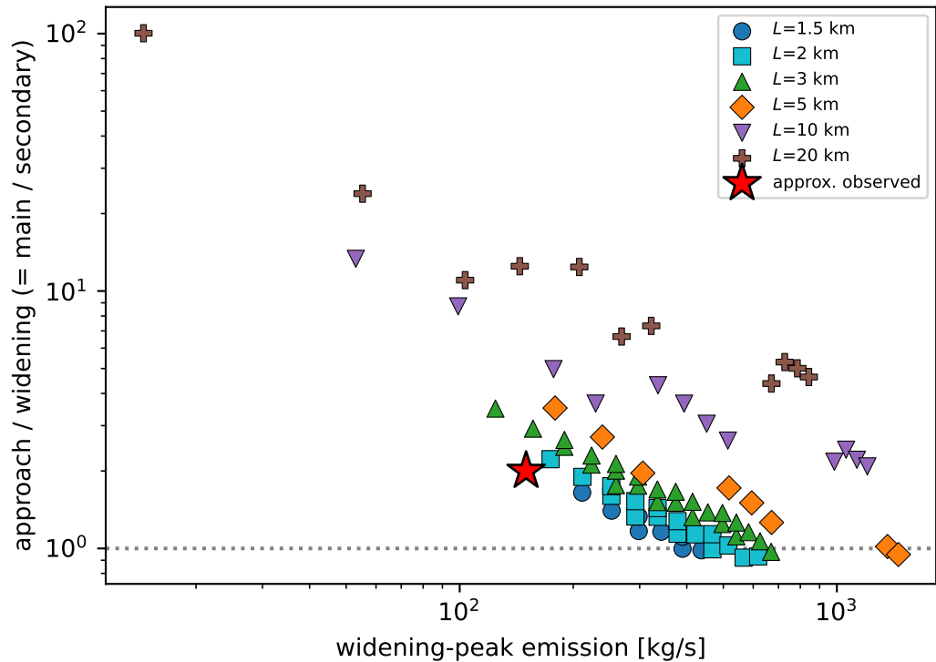
(b) Steady-state cases vs Enceladus
