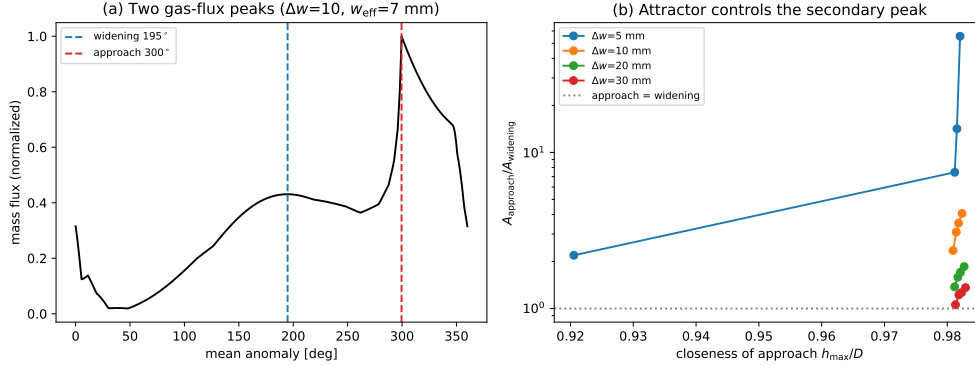
Figure 4. Predictor for the two diurnal mass-flux peaks (equilibrium depth 5 km). (a) The gas-flux curve for a sealed crack ( \Delta w = 10 mm, w_{\text{eff}} = 7 mm) showing the widening peak near the max-width phase and the approach peak near the max-water-level phase. (b) The approach-to-widening strength ratio rises steeply with the closeness of approach h_{\max}/D and crosses unity (approach becomes the main peak) as the sealing drives the water to the surface; curves are different absolute tidal swings \Delta w .
