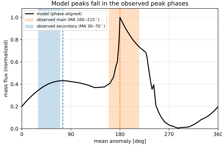
Figure 8. Model diurnal mass flux (normalized; the attractor case of Figure 7a) after applying the single permitted global phase offset that aligns the approach peak with the observed main peak. Shaded bands mark the observed main and secondary peak phases from the Cassini slab-density profile (Ingersoll, Ewald, et al. (2020); Figure 1); no observed flux curve is plotted, only the peak phases. The model’s second (widening) peak falls near the observed secondary band without further tuning, and the two model peaks reproduce the observed \sim 130^\circ separation.
