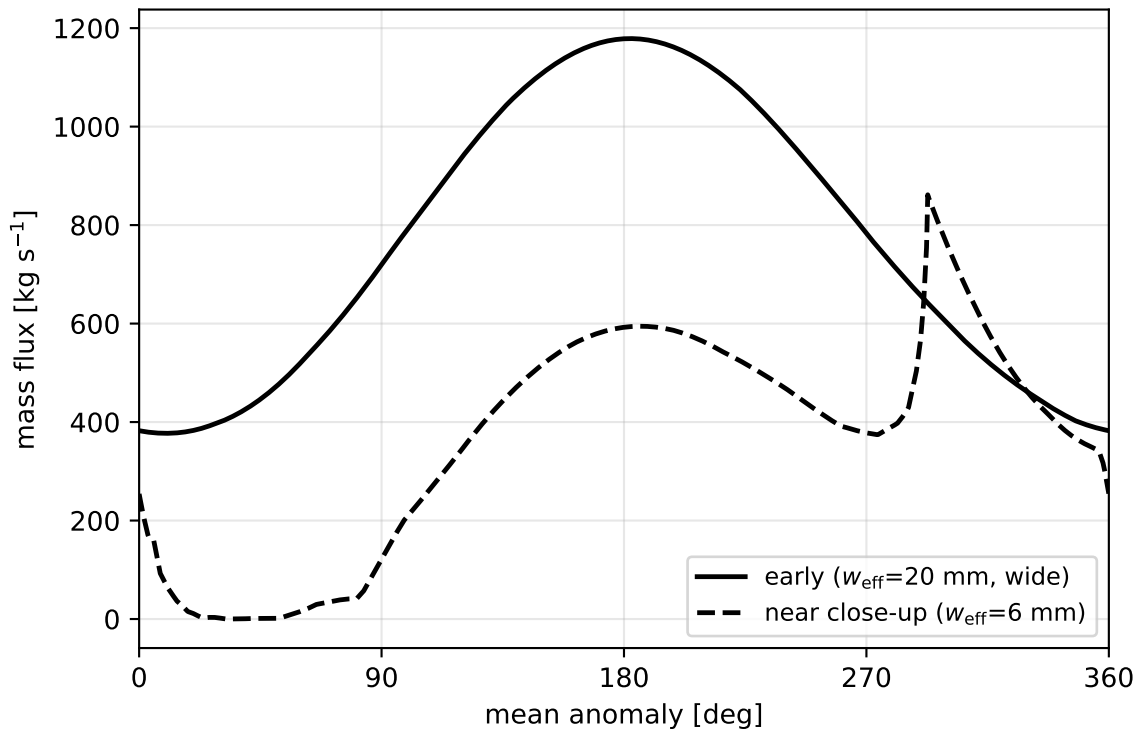
Mass flux as a crack seals ( L=5 km, \Delta w=20 mm)
