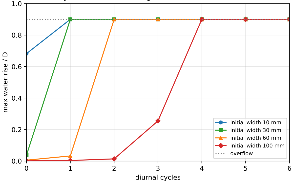
Any initial width converges to overflow ( \Delta w=12 mm)
