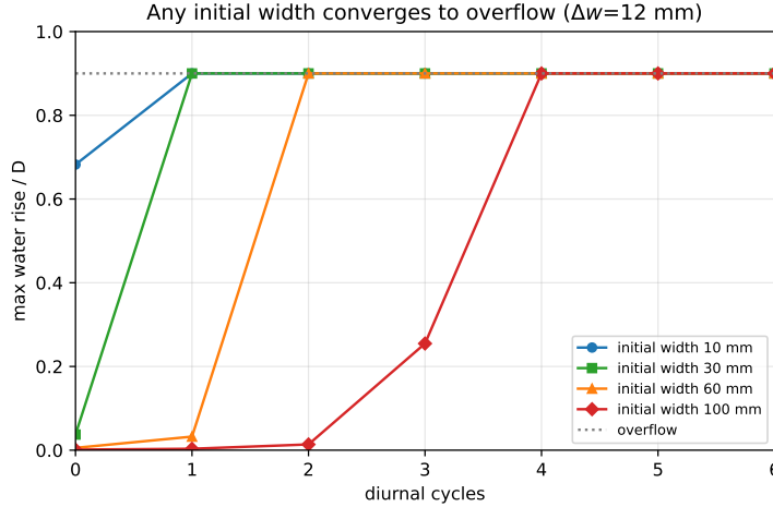
Figure 4. Convergence to the overflow attractor (equilibrium depth 5 km, \Delta w = 12 mm). Each curve follows the maximum water rise h_{\max}/D as wall condensation narrows the effective width, cycle by cycle, from a different initial width (1–10 cm). Regardless of the starting width, the water climbs to overflow within a few diurnal cycles; a wider initial gap only delays the approach. The common approach curve reflects that the water level is set by the current effective width alone, not by the crack’s original size.
