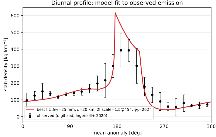
Figure 9. Best-fit model diurnal mass-flux profile (red) against the digitized observed slab-density profile (black points; error bars are the per-bin scatter spread, not measurement error; Ingersoll, Ewald, et al. (2020), Fig. 1). The crack is on the self-sealing attractor; free parameters are the tidal swing \Delta w , effective source depth L , the second-harmonic (double-cosine) amplitude and phase, a single global phase offset, and an overall amplitude. The double-cosine forcing improves the fit at every depth over a pure single cosine. The sharp main peak is the single-crack rapid-surge onset — the water reaching the surface at speed — which is smoothed once many crack segments are averaged (Figure 10).
