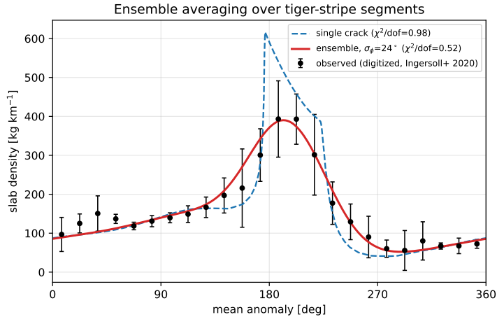
Figure 10. Single-crack versus ensemble-averaged diurnal profile against the observed data. The single crack (blue dashed) surges sharply and overshoots the peak; averaging over the along-strike spread of tiger-stripe segments (a Gaussian phase spread \sigma_\phi \approx 24^\circ ; red) rounds the peak to match the observations, improving the reduced \chi^2 from 0.98 to 0.52. Crack parameters are held at the single-crack best fit of Figure 9; only the ensemble spread, phase offset, and amplitude are adjusted.
