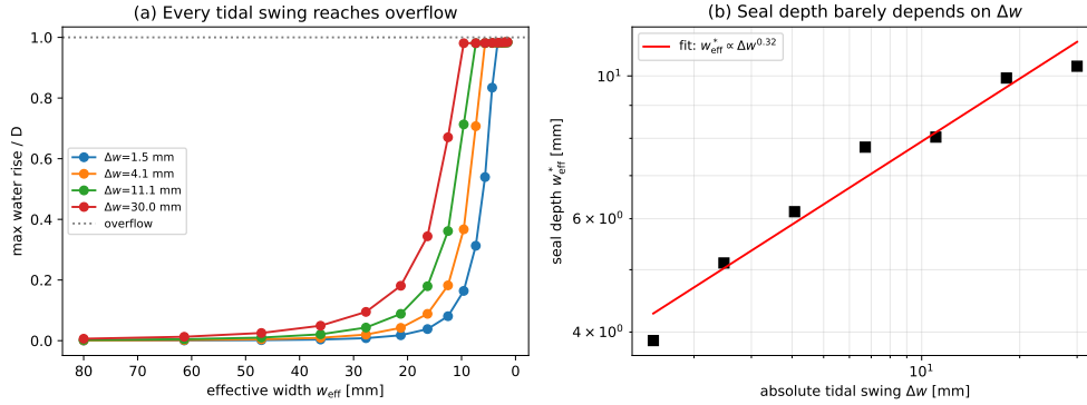
Figure 3. Self-sealing of the crack by wall condensation (effective-width model, equilibrium depth 5 km, surface D = 500\text{ m} above the equilibrium water level). For a fixed absolute tidal swing \Delta w = w_{\text{max}} - w_{\text{min}} of the walls, the ice lining lowers the mean width, i.e. the effective width w_{\text{eff}} . (a) The maximum water rise (as a fraction of D ) reaches overflow for every swing \Delta w once the crack has sealed far enough — there is no forcing threshold. (b) The swing sets only the seal depth w_{\text{eff}}^* at which overflow first occurs; it is of order millimetres and increases only weakly with the swing ( w_{\text{eff}}^* \propto \Delta w^{0.3} ).
