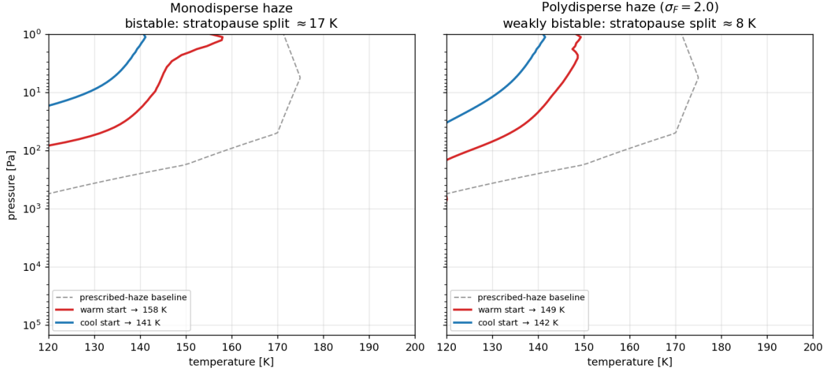
Figure 6: The stable states of the coupled haze feedback, found by relaxing the radiative–convective equilibrium from a warm (red) and a cool (blue) initial profile at the same fixed (transition-state) haze (dashed: the prescribed-haze baseline). Left : the monodisperse haze settles to two well-separated branches—a warm (158 K) and a cool (141 K) stratopause, \Delta T \approx 17 K (up to 31 K through the profile)—so the system is bistable. Right : the polydisperse (bimodal, \sigma_F = 2.0 ) haze settles to two branches only \sim 8 K apart, the warm branch having cooled from 158 to 149 K: the bistability is strongly suppressed but a weak residual multiplicity survives. Both splits are fully converged (stable as the heating residual falls below 0.3 \text{ K day}^{-1} ).
