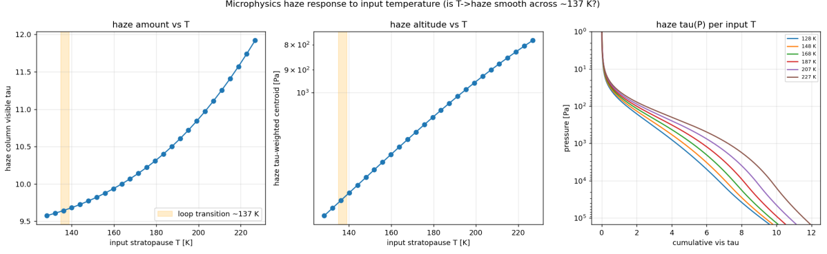
Figure 7: Microphysics haze response to the input temperature. Haze column optical depth (left), \tau -weighted centroid pressure (centre), and cumulative \tau(p) (right) all vary smoothly across the coupled transition (shaded, \sim 137 K): the T \rightarrow haze map has no cliff, so the bistability is radiative, not microphysical.
