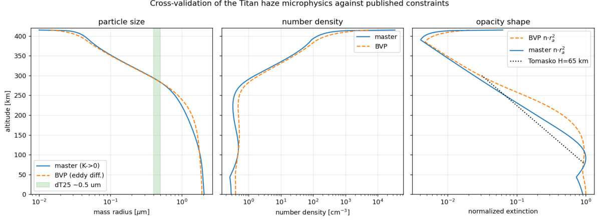
Figure 2: Cross-validation of the microphysics against published Titan constraints. Left: mass radius from the K \rightarrow 0 master ODE and the eddy-diffusion BVP, with the de Trenquell on et al. (2025) main-haze size ( \sim 0.5 \mu\text{m} ) shaded. Centre: number density. Right: normalized extinction n r_a^2 , with the Tomasko et al. (2008) H = 65 \text{ km} reference slope (dotted) anchored at 80 km.
