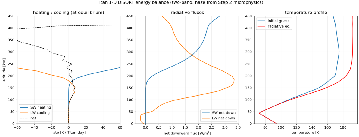
Figure 1: Two-band DISORT energy balance on the Titan column with the Step 2 haze. Left: shortwave heating, longwave cooling, and net rate at the relaxed state. Centre: net downward shortwave and longwave fluxes. Right: initial-guess vs. radiative-equilibrium temperature (surface fixed).
