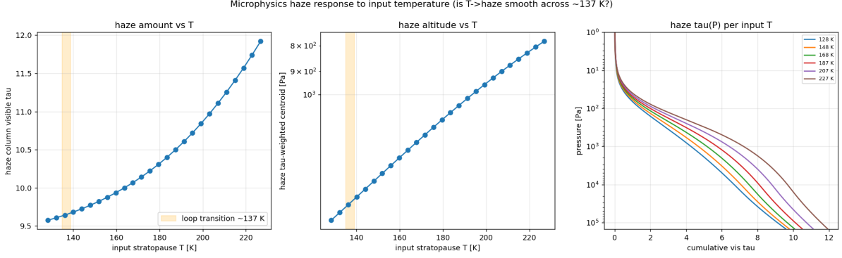
Figure 6: Microphysics haze response to the input temperature. Haze column optical depth (left), \tau -weighted centroid pressure (centre), and cumulative \tau(p) (right) all vary smoothly across the coupled transition (shaded, \sim 137 K): the T \rightarrow haze map has no cliff, so the bistability is radiative, not microphysical.
