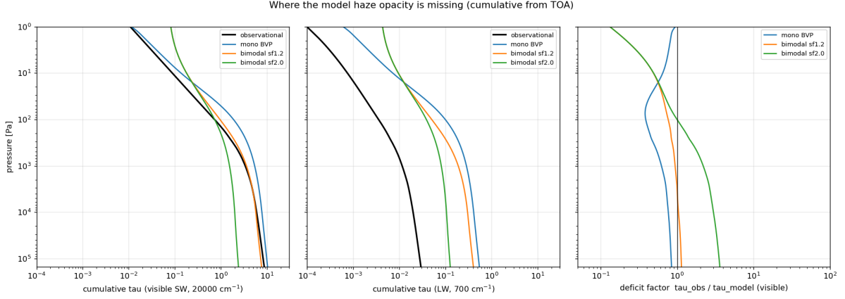
Figure 8: Why the lab-tholin coupled state is 40 K cold: cumulative haze optical depth from the top of atmosphere, observational (black) versus model hazes. Left: in the visible the model haze matches or exceeds the observational opacity at every level. Centre: in the thermal IR ( 700\text{ cm}^{-1} shown) the RDG/lab-tholin LW opacity exceeds the observational haze by 20–90 \times —the stratosphere cools an order of magnitude too efficiently per unit shortwave heating. Right: the visible deficit factor \tau_{\text{obs}}/\tau_{\text{model}} ; the residual 2.6\times model excess aloft explains the +11 K overshoot of the calibrated coupled fixed point.
