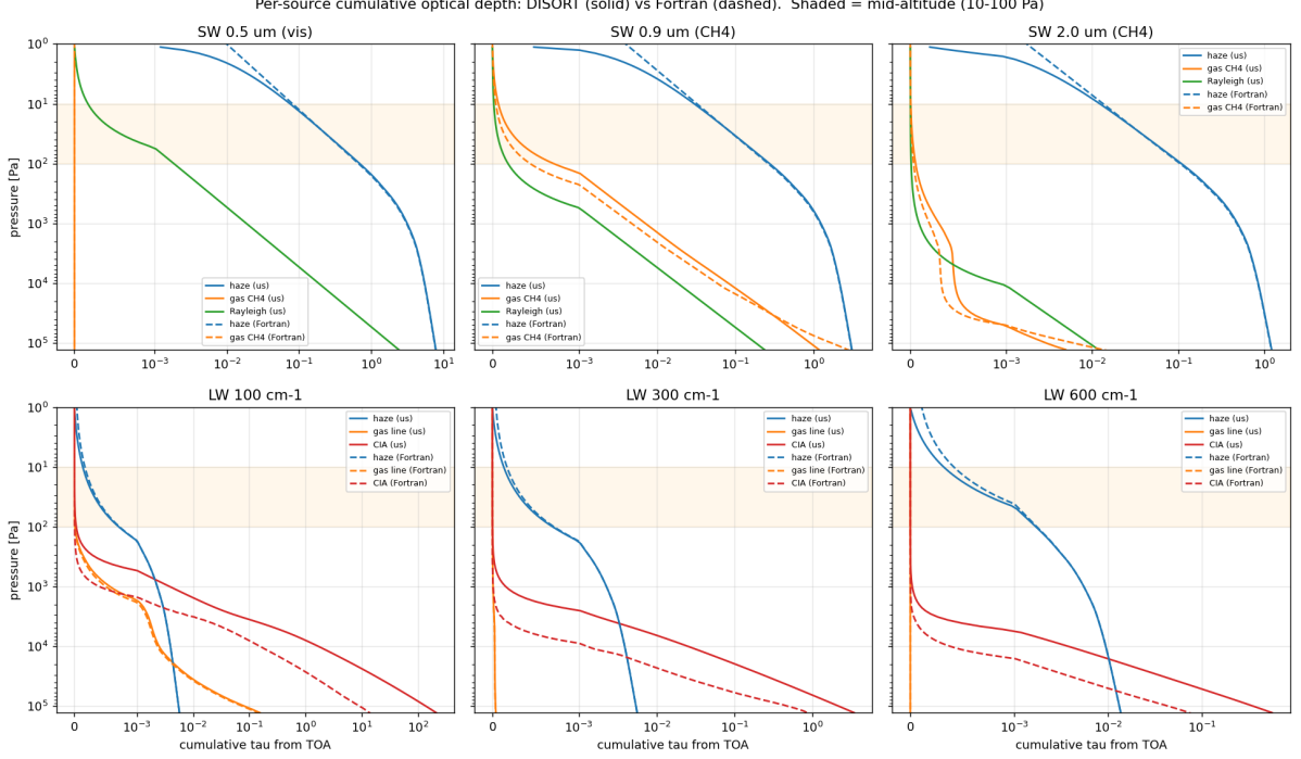
Figure 4: Cumulative optical depth from the top of atmosphere, by source, for our DISORT optics (solid) and the reference Fortran model (dashed), at the same state. Top row: shortwave (haze, CH 4 gas, Rayleigh) in three representative bands; bottom row: longwave (haze, gas lines, CIA). The shaded band marks the mid-altitude 10–100 Pa region. The haze dominates and matches closely; all sources agree to within a few percent through the mid-atmosphere, so the residual heating-rate difference there is the radiative-transfer solver, not the opacity.
