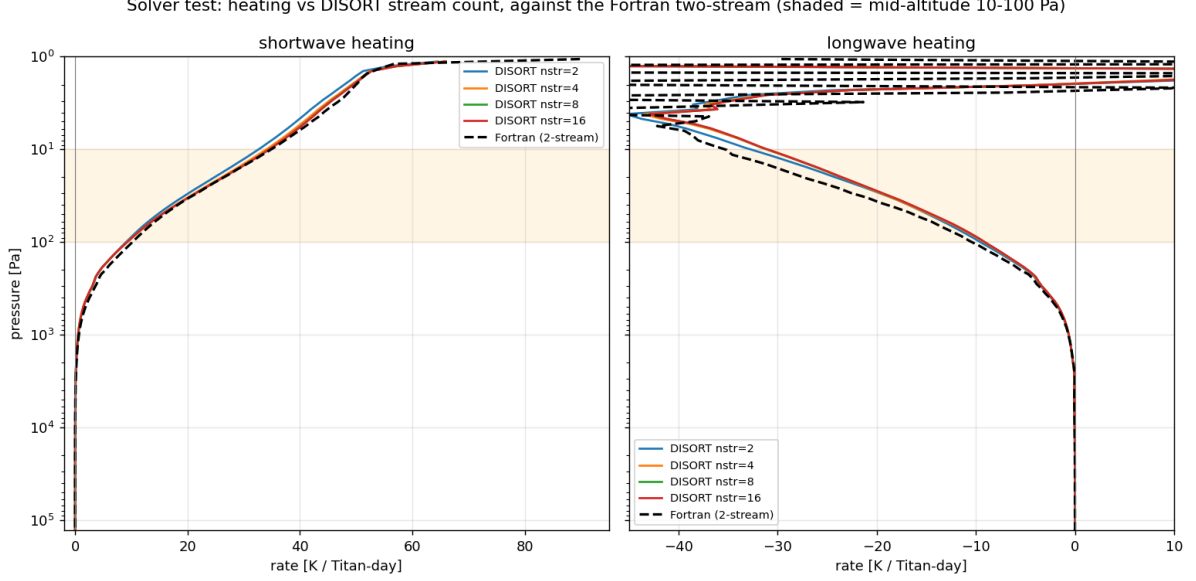
Figure 3: Solver test: heating rates from our DISORT optics at N_{\text{str}} = 2, 4, 8, 16 (coloured) against the reference two-stream model (dashed), at the same state. Shaded: mid-altitude 10–100 Pa. Shortwave (left) is insensitive to the stream count—the curves collapse and the eight-stream solution best matches the reference—so the shortwave difference is not the angular quadrature. Longwave (right) moves toward the reference as the stream count drops to two, matching its hemispheric-mean treatment, but recovers only part of the gap. (The longwave top P \lesssim 2 Pa is the reference’s unconverged, oscillating region.)
