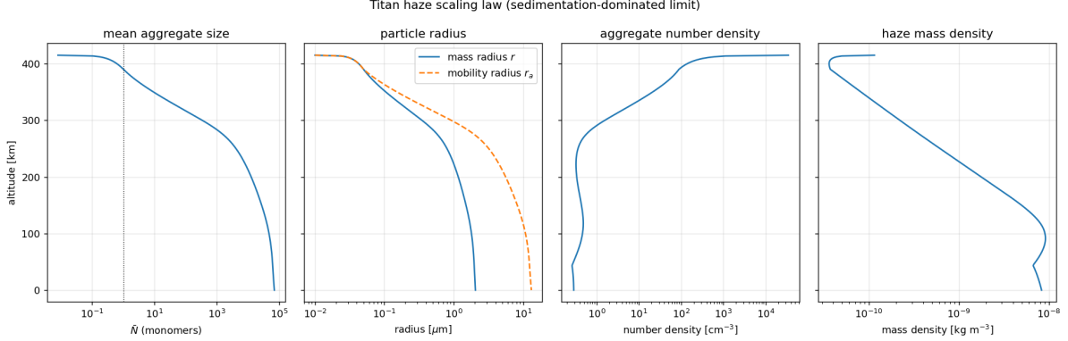
Figure 5: Steady haze profiles from the sedimentation-dominated scaling law (12) on the Titan reference column: mean aggregate size \bar{N} (dotted line marks the \bar{N} = 1 spherical/fractal switch), mass and mobility radii, aggregate number density, and haze mass density. Aggregates grow as they settle; r_a exceeds r in the fractal phase.
