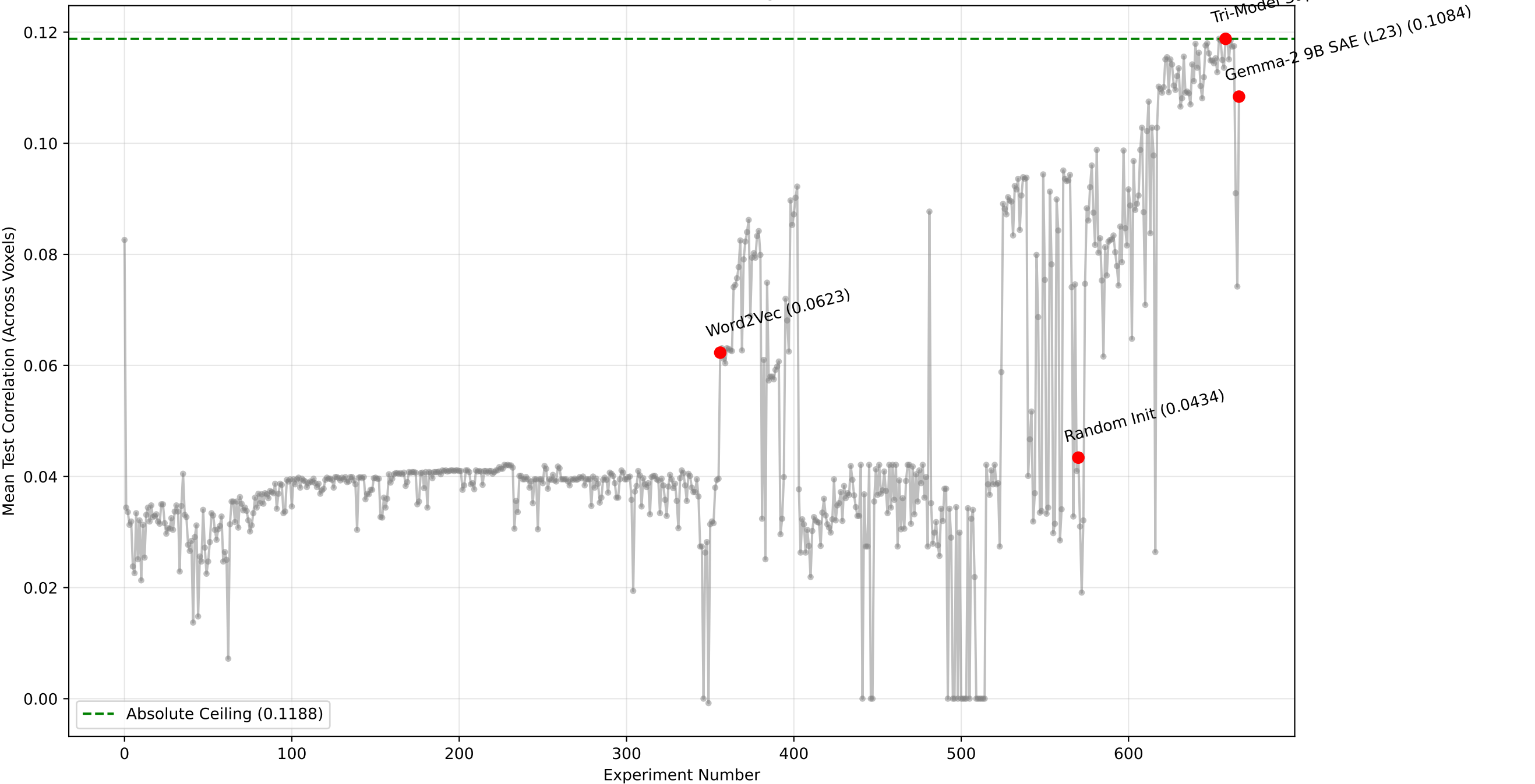
Evolution of fMRI Linear Encoding Performance
