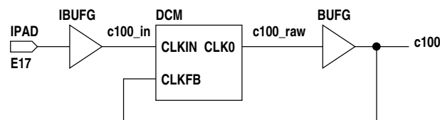
Figure 2: digital clock manager
