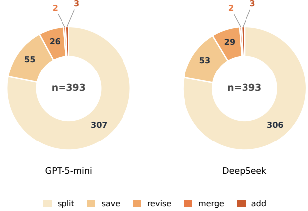
Fig. 1: Action distribution under a fixed GPT-5 mini first-round architecture. The figure compares subsequent structural evolution driven by GPT-5 mini and DeepSeek V3.2 on the same initial architecture.
