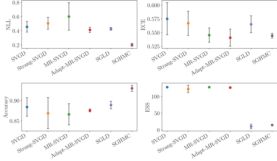
(c) spambase
