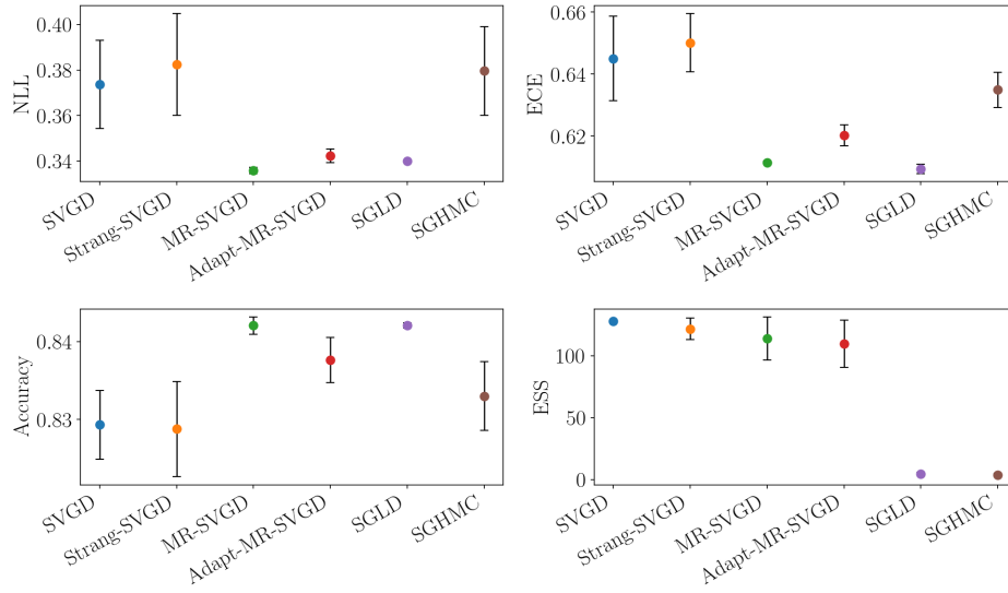
(c) a5a
