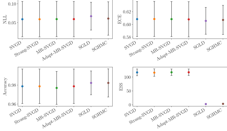
(a) breast_cancer
