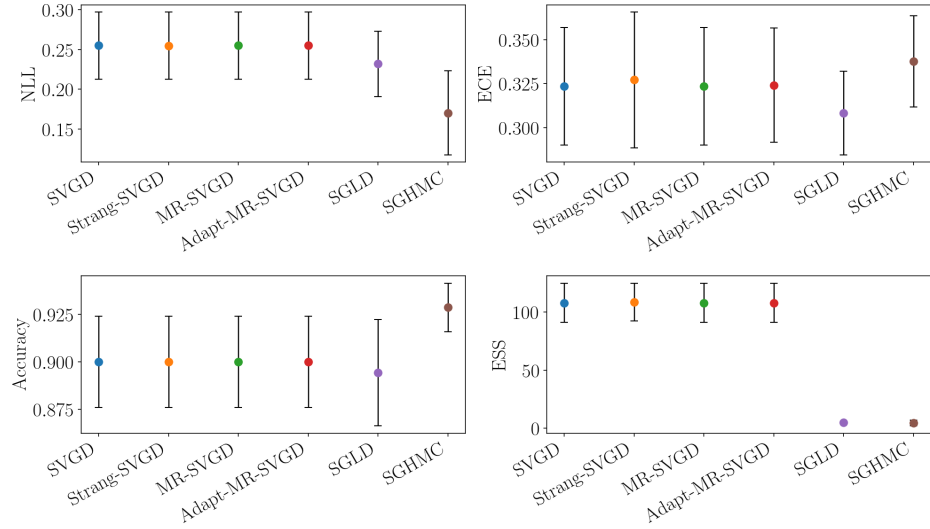
(b) ionosphere
