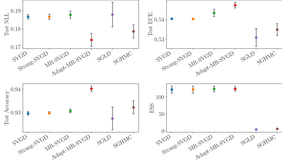
(a) Spambase
