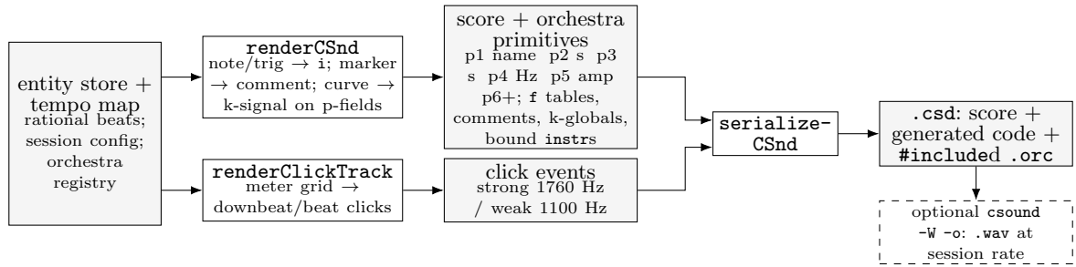
Fig. 2. Both Csound-family renderers share one serializer; source instruments stay in external .orc files, and curve bindings add generated copies without touching them.
