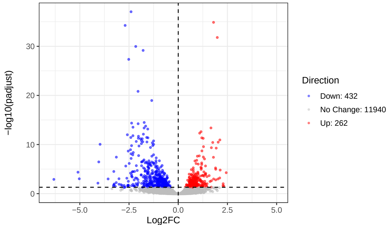
Volcano Plot – HGPS UMK57 vs DMSO
