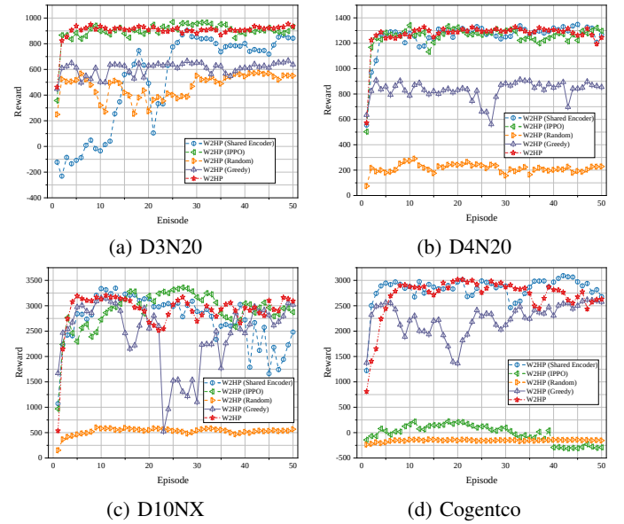
Fig. 4: Training rewards of W2HP and its variants under different network topologies.
